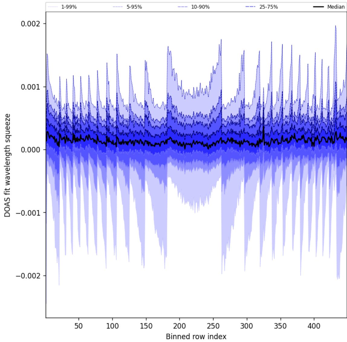
Figure 48: Along track statistics of “DOAS fit wavelength squeeze” for 2024-12-10 to 2024-12-11
