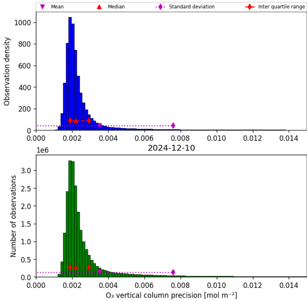
Figure 30: Histogram of “O 3 vertical column precision” for 2024-12-10 to 2024-12-11
