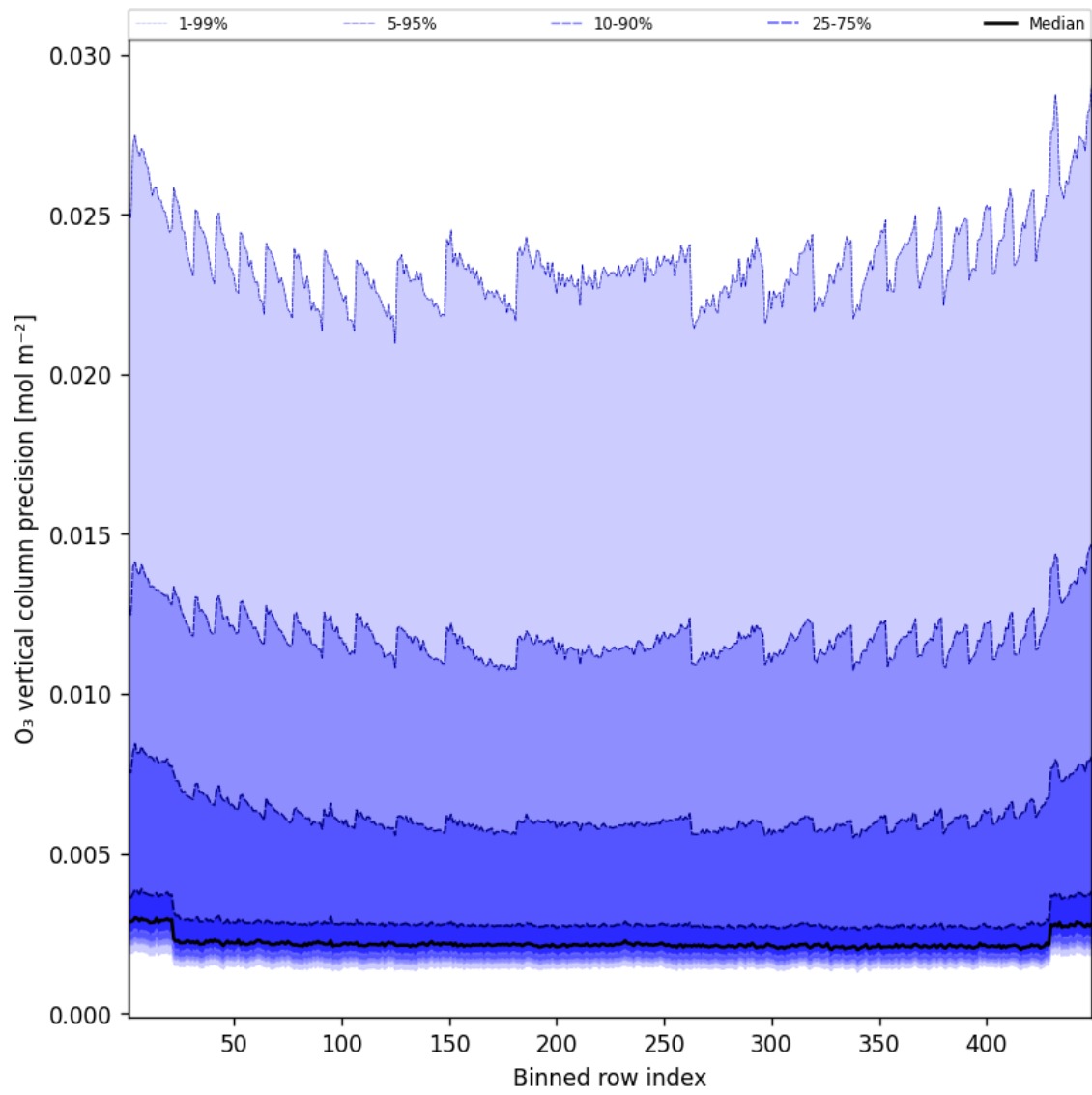
Figure 42: Along track statistics of “O 3 vertical column precision” for 2024-12-10 to 2024-12-11
