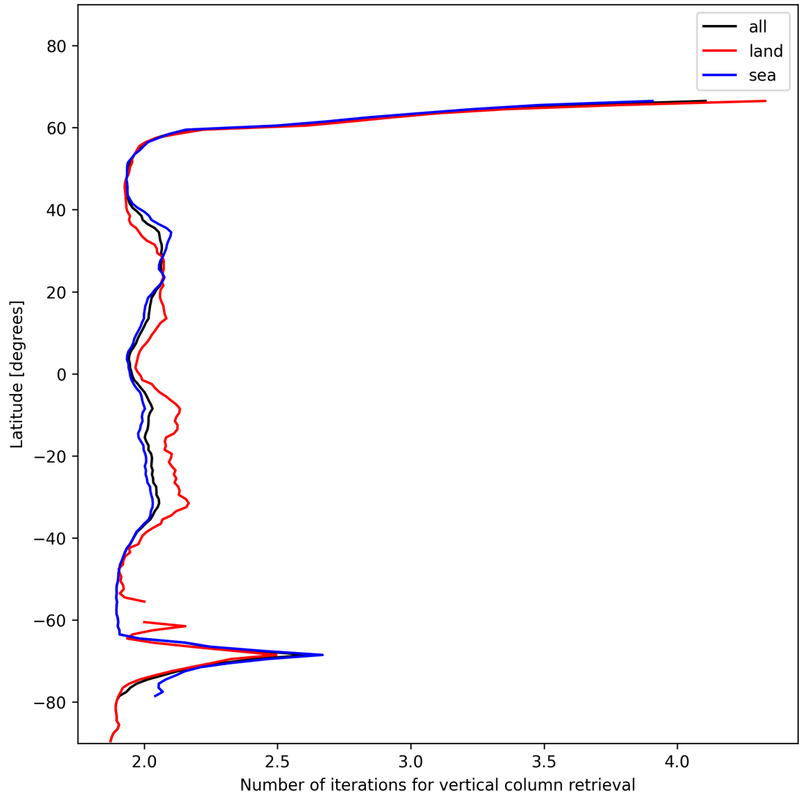
Figure 27: Zonal average of “Number of iterations for vertical column retrieval” for 2024-12-10 to 2024-12-11.
