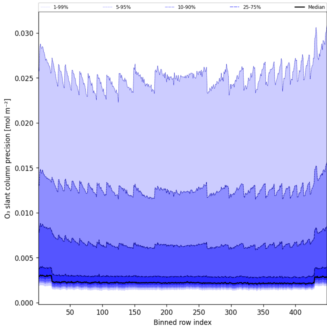
Figure 44: Along track statistics of “O 3 slant column precision” for 2024-12-10 to 2024-12-11
