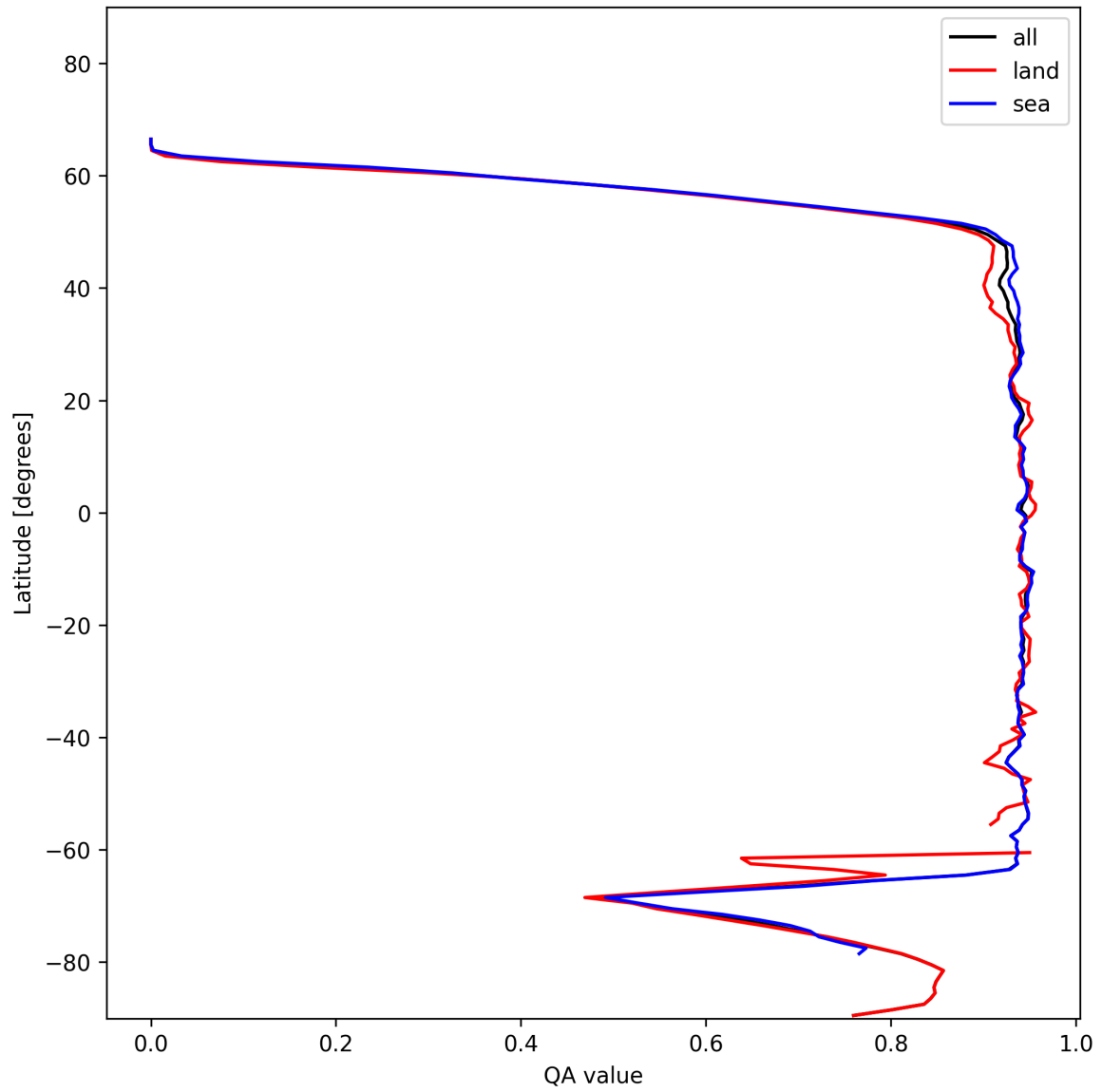
Figure 16: Zonal average of “QA value” for 2024-12-10 to 2024-12-11.
