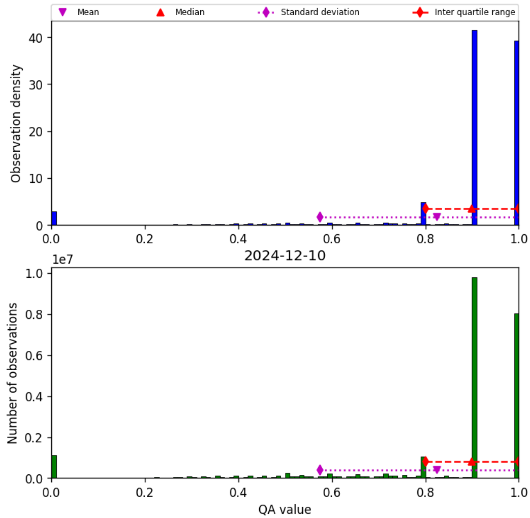
Figure 28: Histogram of “QA value” for 2024-12-10 to 2024-12-11
