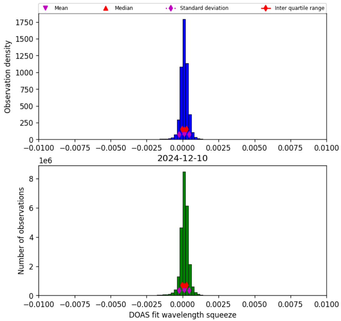
Figure 36: Histogram of “DOAS fit wavelength squeeze” for 2024-12-10 to 2024-12-11
