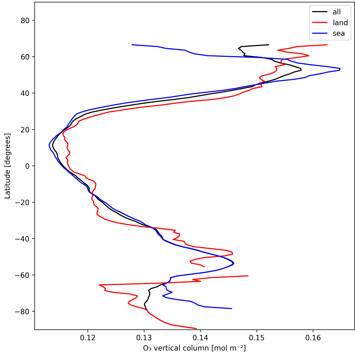
Figure 17: Zonal average of “O 3 vertical column” for 2024-12-10 to 2024-12-11.
