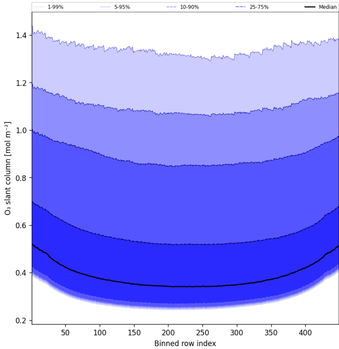
Figure 43: Along track statistics of “O 3 slant column” for 2024-12-10 to 2024-12-11
