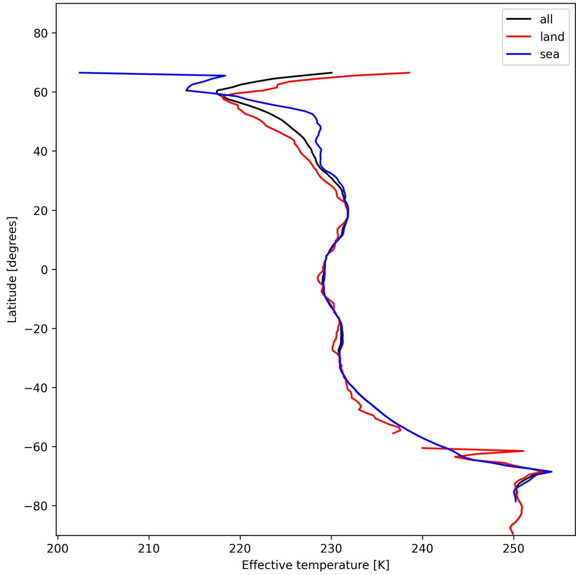
Figure 26: Zonal average of “Effective temperature” for 2024-12-10 to 2024-12-11.
