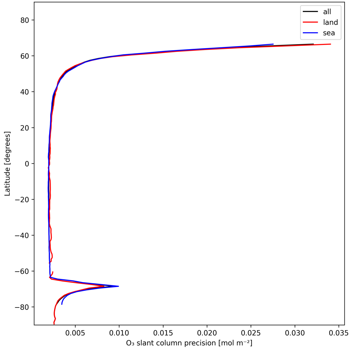
Figure 20: Zonal average of “O 3 slant column precision” for 2024-12-10 to 2024-12-11.
