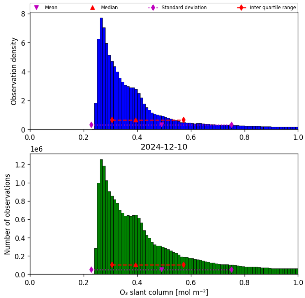
Figure 31: Histogram of “O 3 slant column” for 2024-12-10 to 2024-12-11
