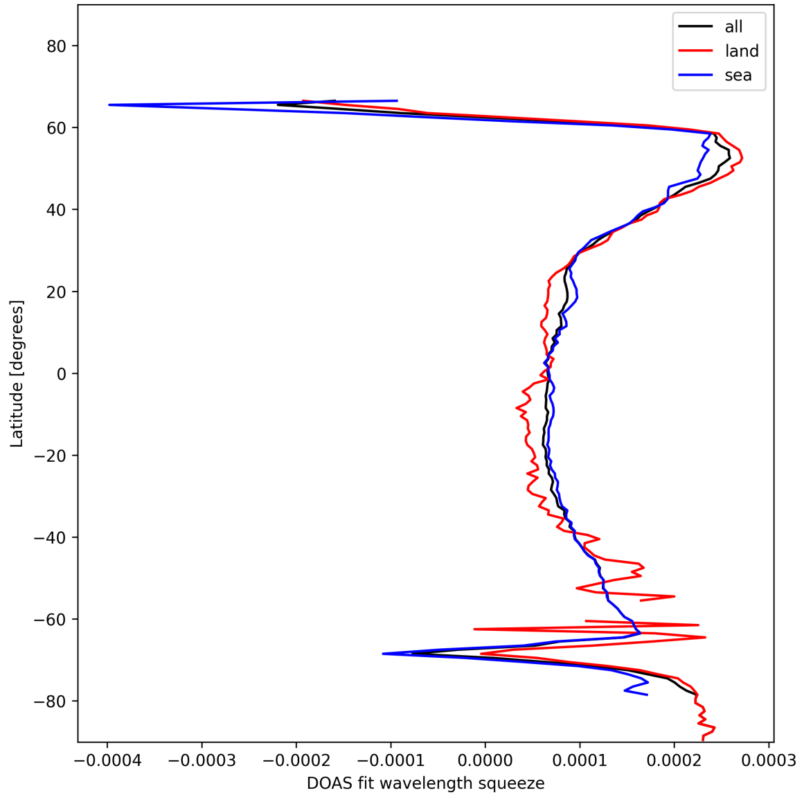
Figure 24: Zonal average of “DOAS fit wavelength squeeze” for 2024-12-10 to 2024-12-11.
