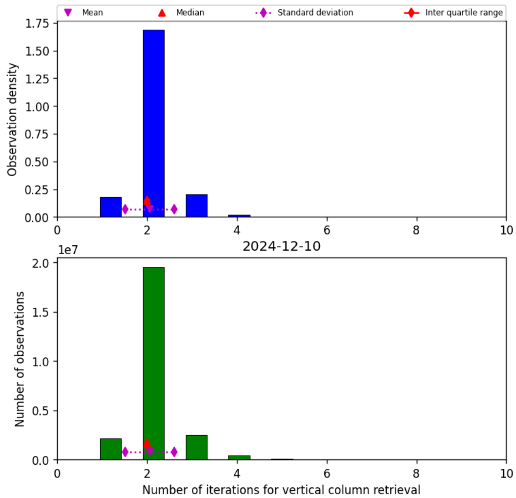
Figure 39: Histogram of “Number of iterations for vertical column retrieval” for 2024-12-10 to 2024-12-11
