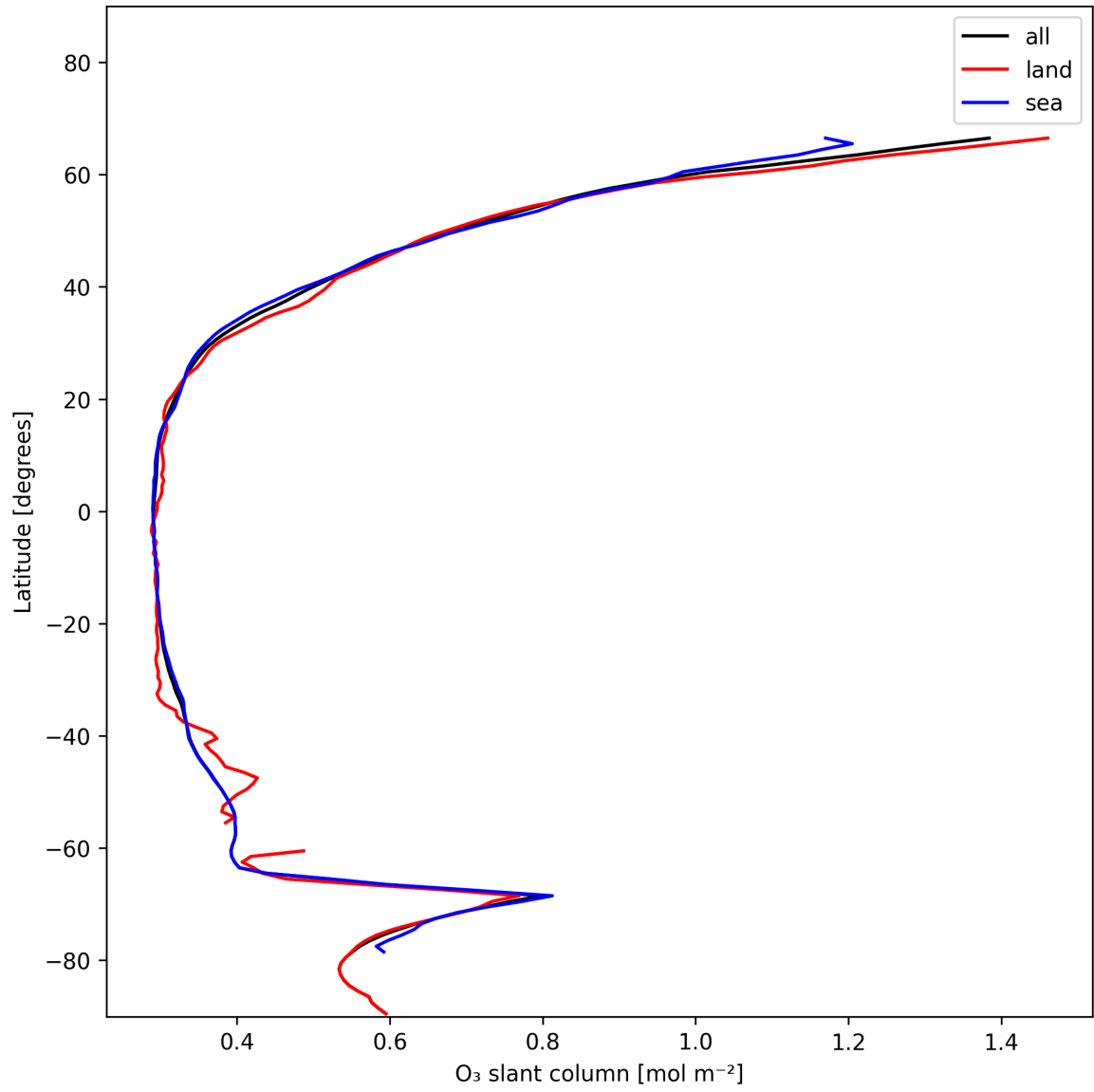
Figure 19: Zonal average of “O 3 slant column” for 2024-12-10 to 2024-12-11.
