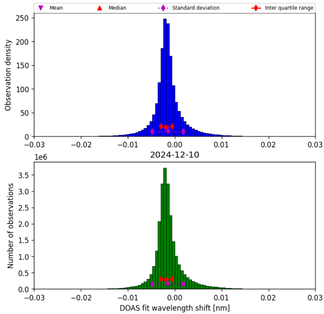
Figure 35: Histogram of “DOAS fit wavelength shift” for 2024-12-10 to 2024-12-11
