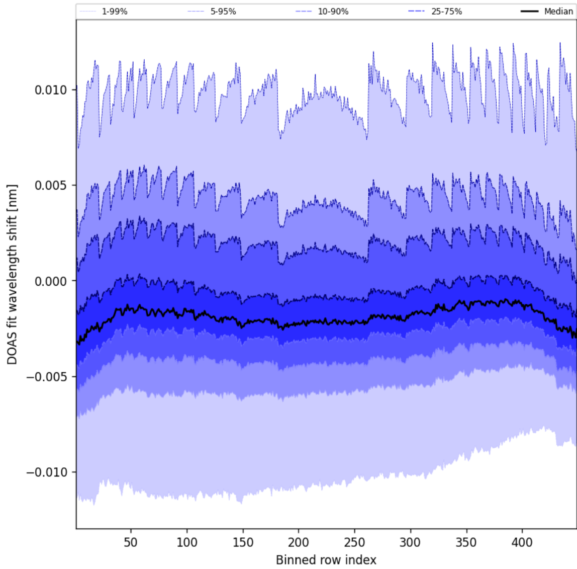
Figure 47: Along track statistics of “DOAS fit wavelength shift” for 2024-12-10 to 2024-12-11
