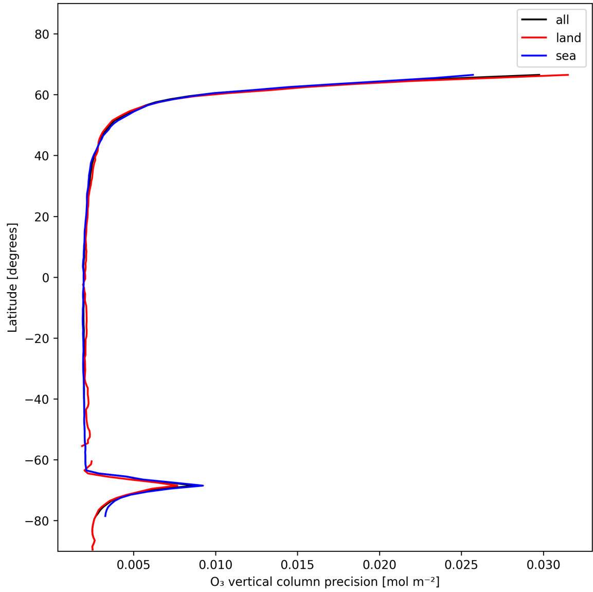
Figure 18: Zonal average of “O 3 vertical column precision” for 2024-12-10 to 2024-12-11.
