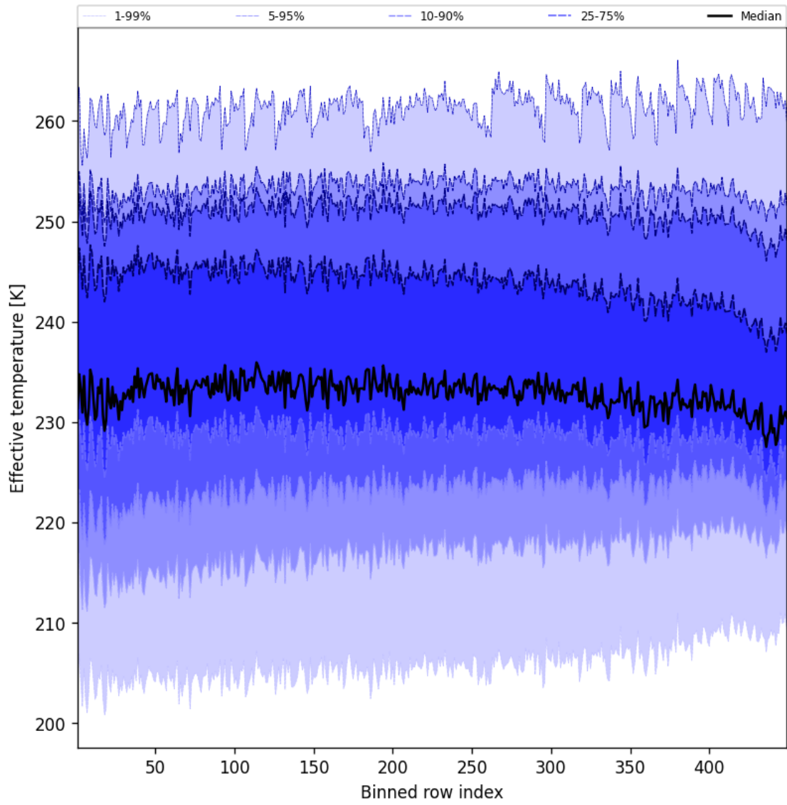
Figure 50: Along track statistics of “Effective temperature” for 2024-12-10 to 2024-12-11
