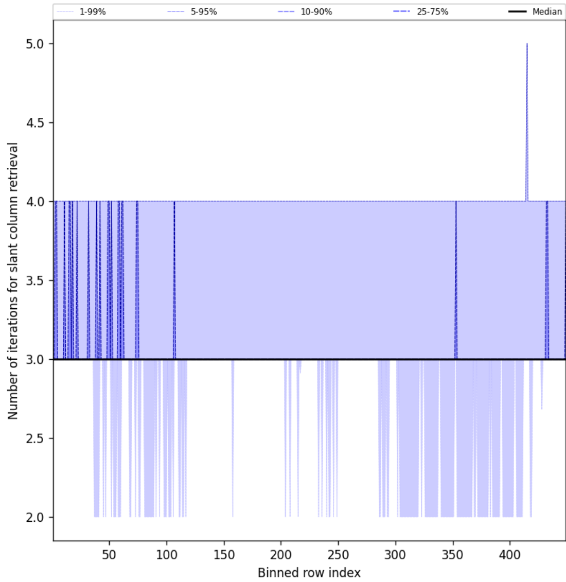
Figure 45: Along track statistics of “Number of iterations for slant column retrieval” for 2024-12-10 to 2024-12-11
