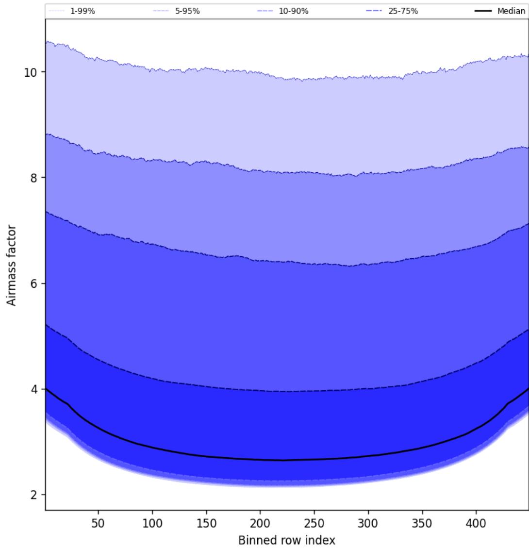
Figure 49: Along track statistics of “Airmass factor” for 2024-12-10 to 2024-12-11
