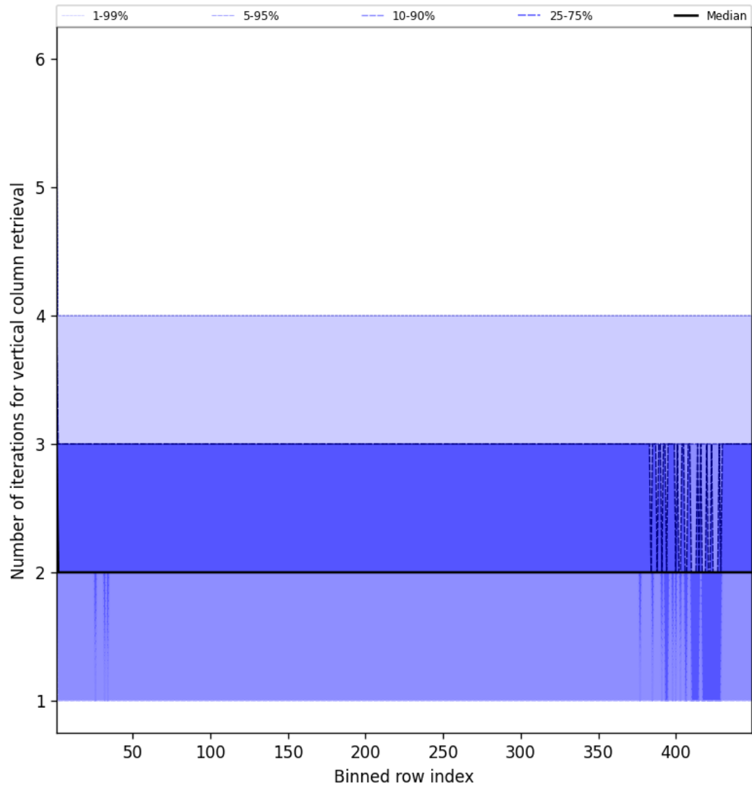
Figure 51: Along track statistics of “Number of iterations for vertical column retrieval” for 2024-12-10 to 2024-12-11
