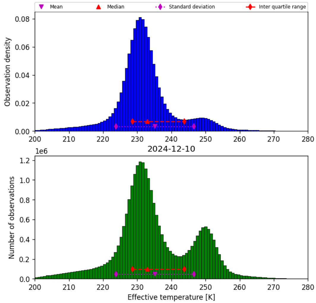
Figure 38: Histogram of “Effective temperature” for 2024-12-10 to 2024-12-11
