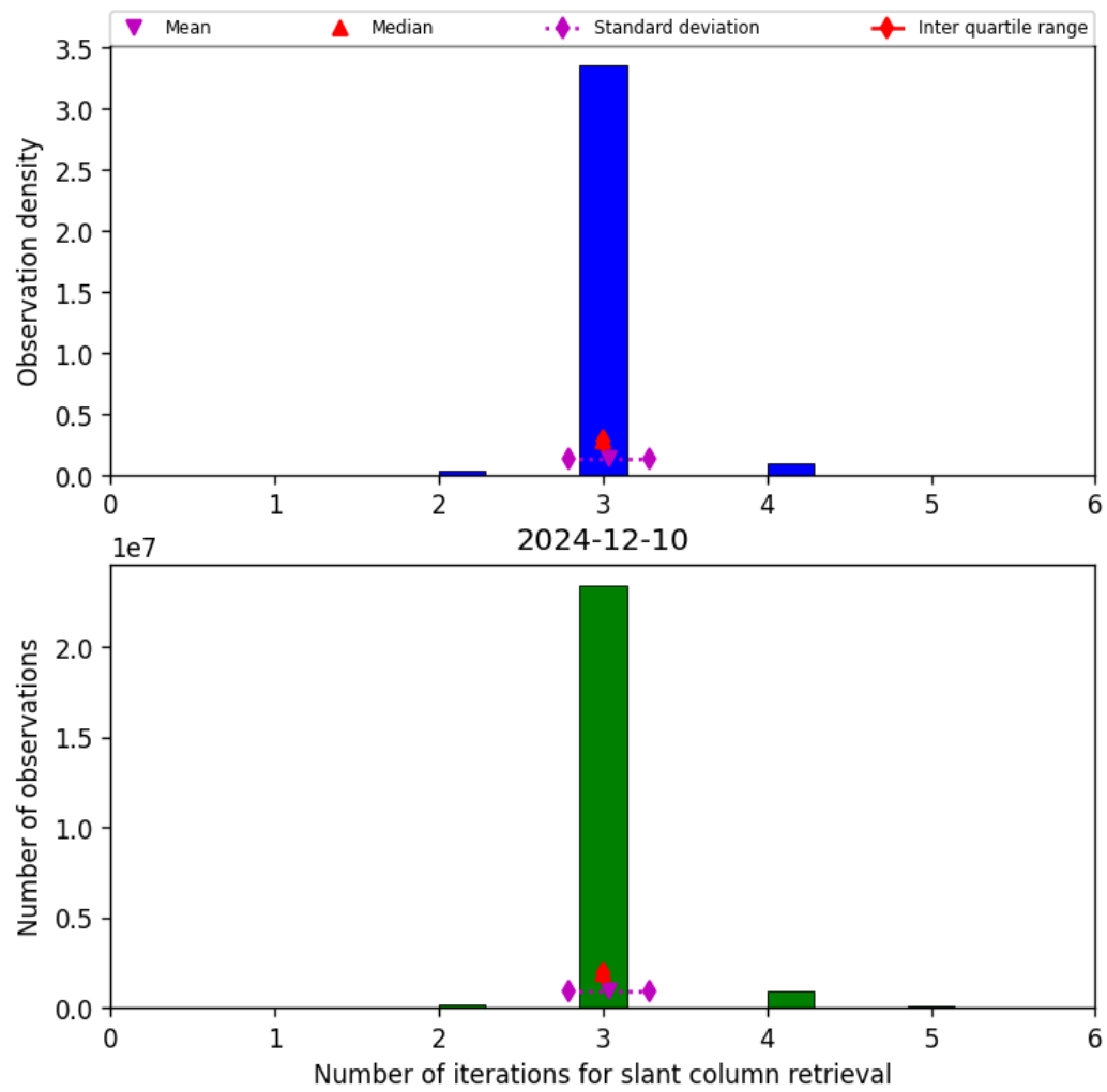
Figure 33: Histogram of “Number of iterations for slant column retrieval” for 2024-12-10 to 2024-12-11
