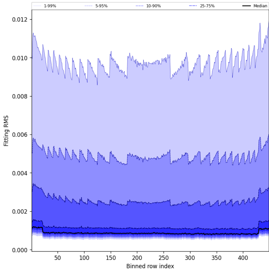
Figure 46: Along track statistics of “Fitting RMS” for 2024-12-10 to 2024-12-11
