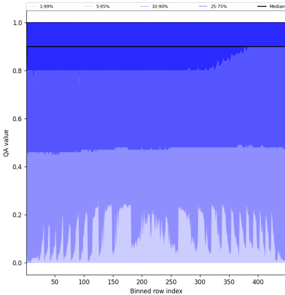
Figure 40: Along track statistics of “QA value” for 2024-12-10 to 2024-12-11
