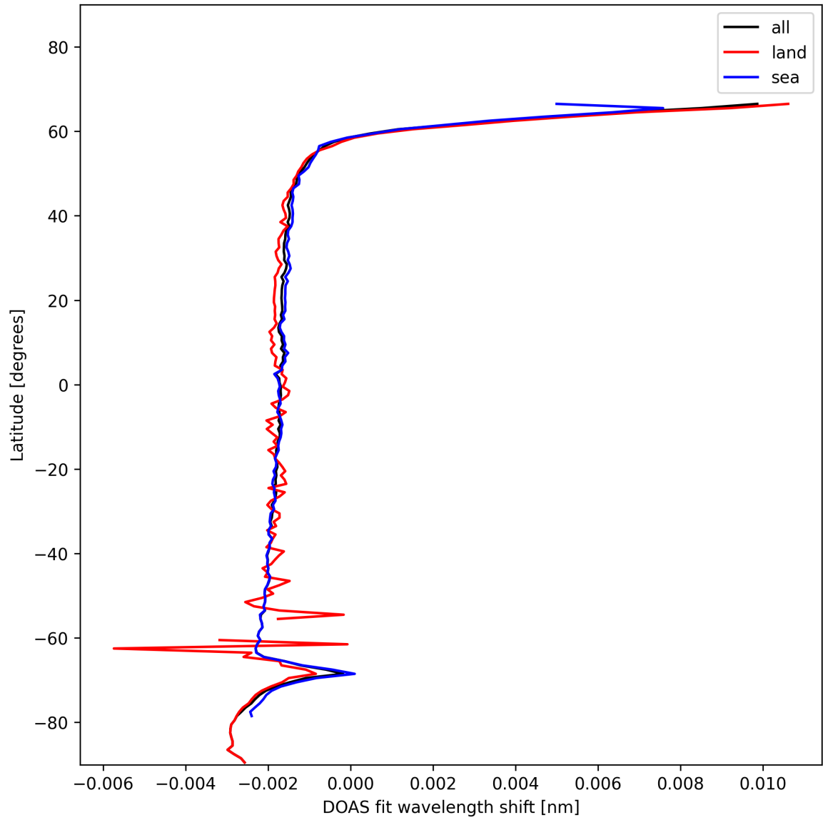
Figure 23: Zonal average of “DOAS fit wavelength shift” for 2024-12-10 to 2024-12-11.
