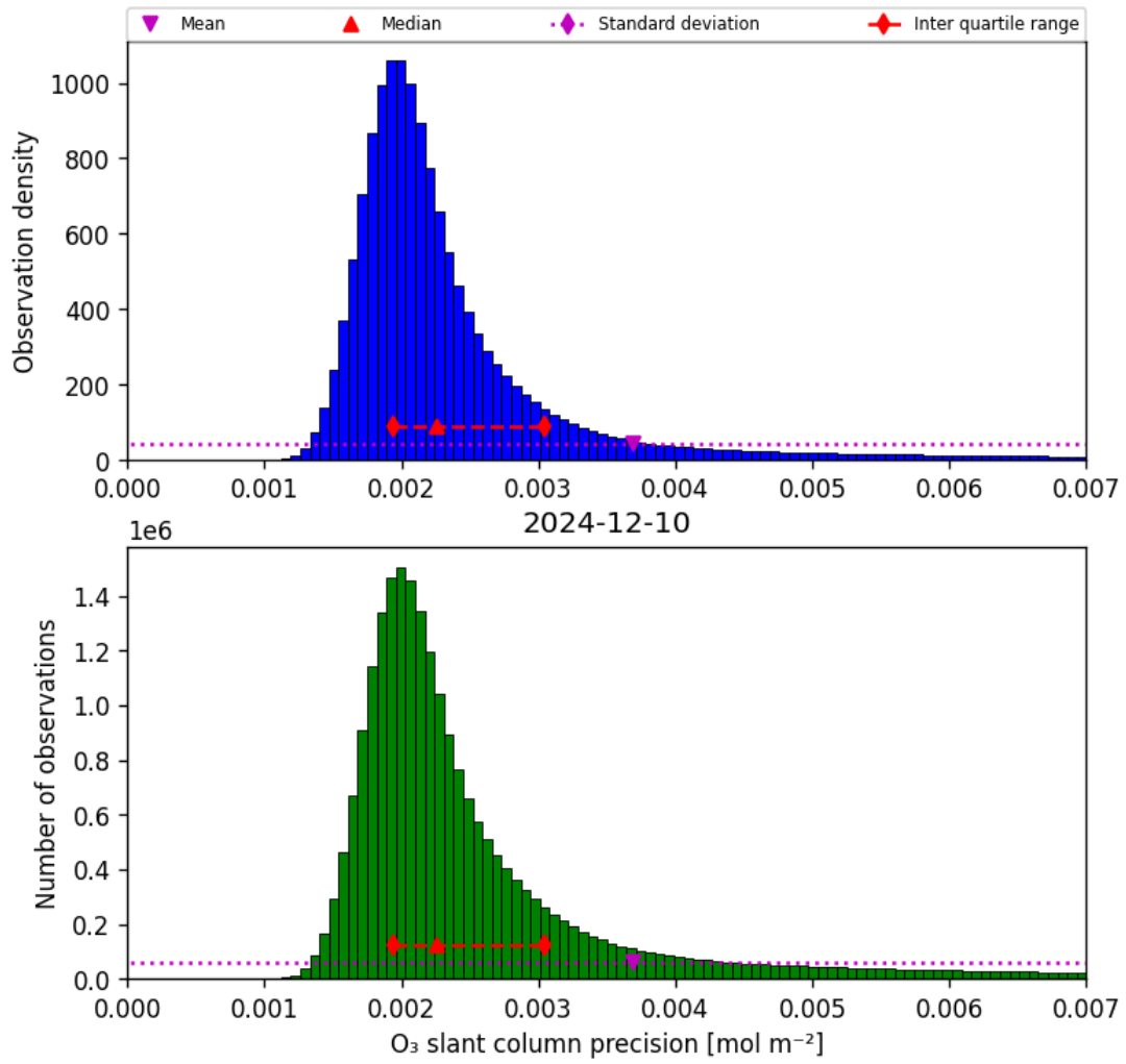
Figure 32: Histogram of “O 3 slant column precision” for 2024-12-10 to 2024-12-11
