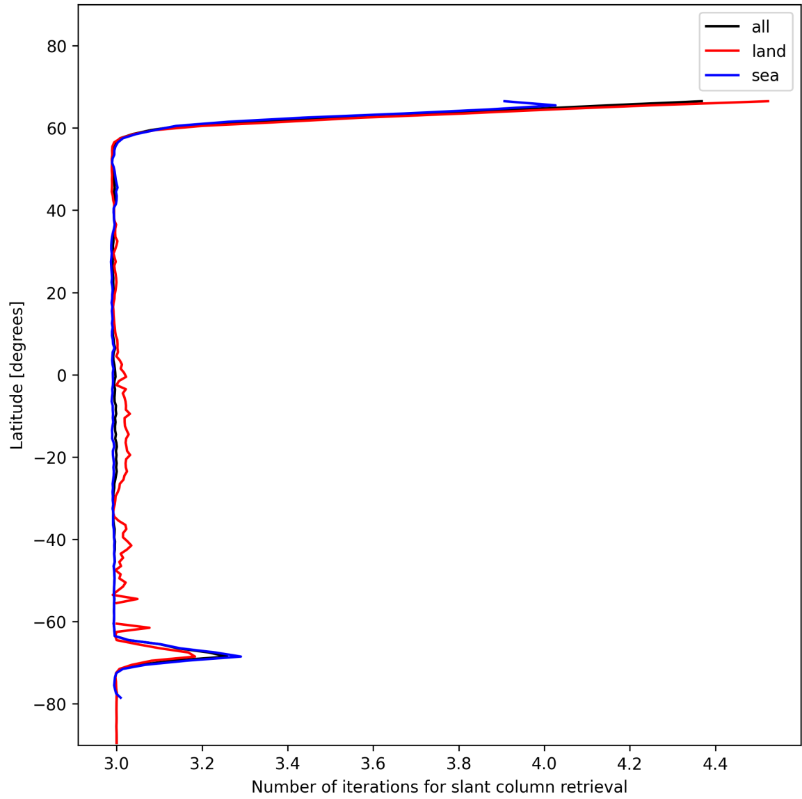
Figure 21: Zonal average of “Number of iterations for slant column retrieval” for 2024-12-10 to 2024-12-11.
