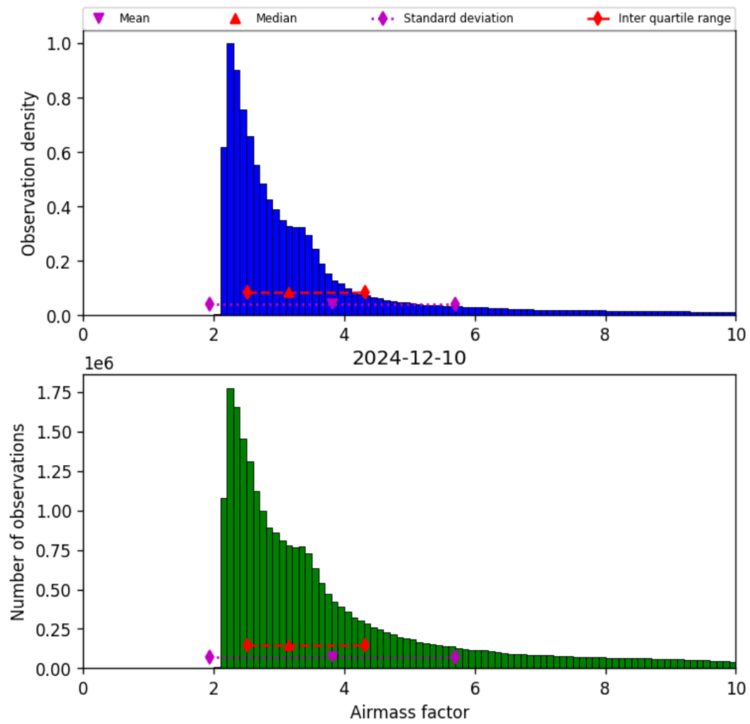
Figure 37: Histogram of “Airmass factor” for 2024-12-10 to 2024-12-11
