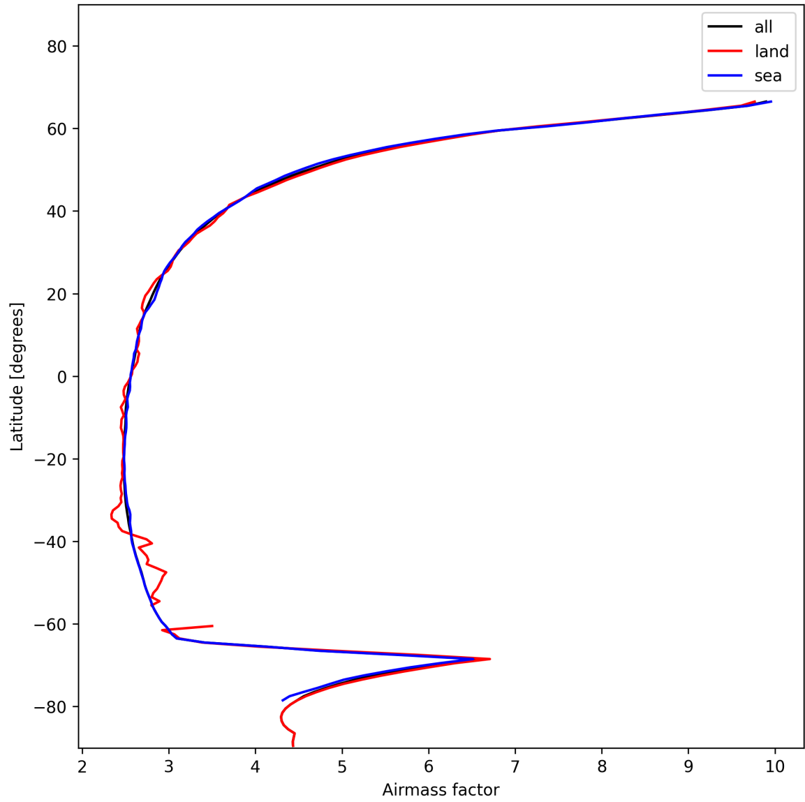
Figure 25: Zonal average of “Airmass factor” for 2024-12-10 to 2024-12-11.
