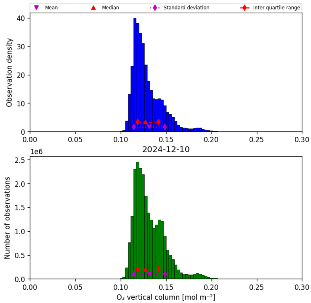
Figure 29: Histogram of “O 3 vertical column” for 2024-12-10 to 2024-12-11
