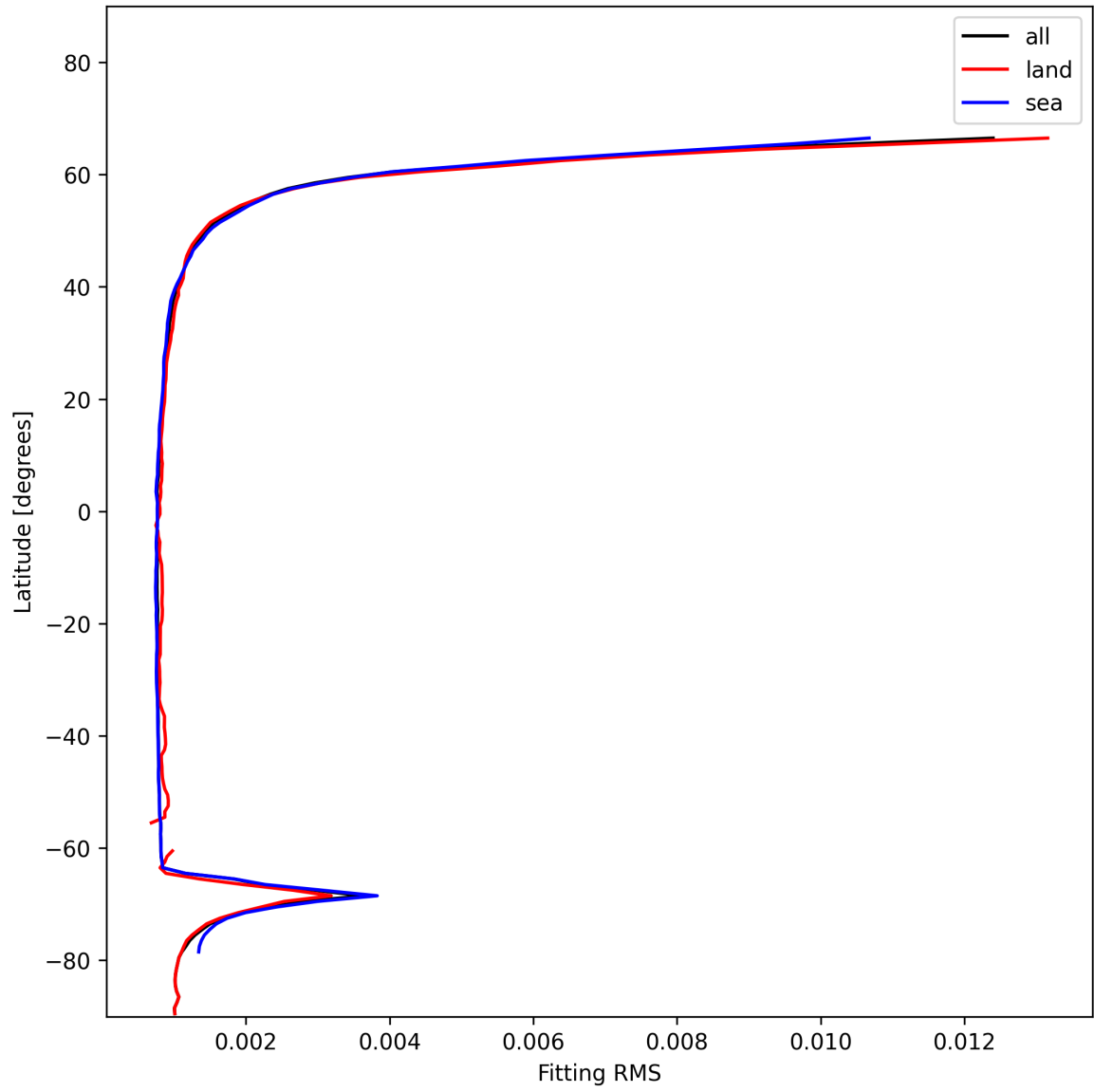
Figure 22: Zonal average of “Fitting RMS” for 2024-12-10 to 2024-12-11.
