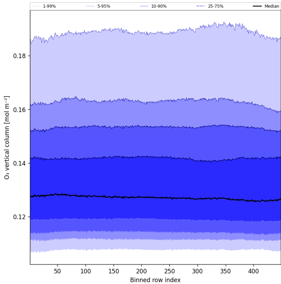
Figure 41: Along track statistics of “O 3 vertical column” for 2024-12-10 to 2024-12-11
