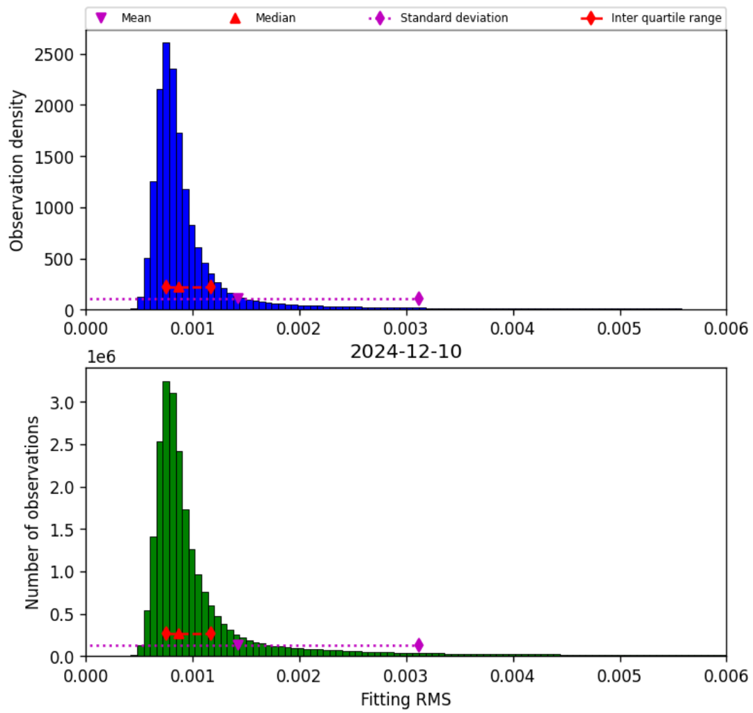
Figure 34: Histogram of “Fitting RMS” for 2024-12-10 to 2024-12-11
