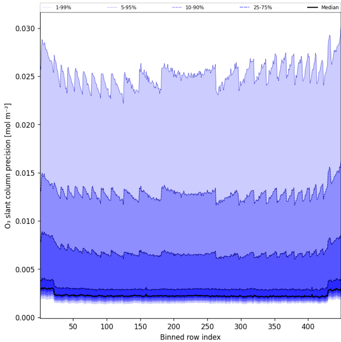
Figure 44: Along track statistics of “O 3 slant column precision” for 2024-12-11 to 2024-12-12
