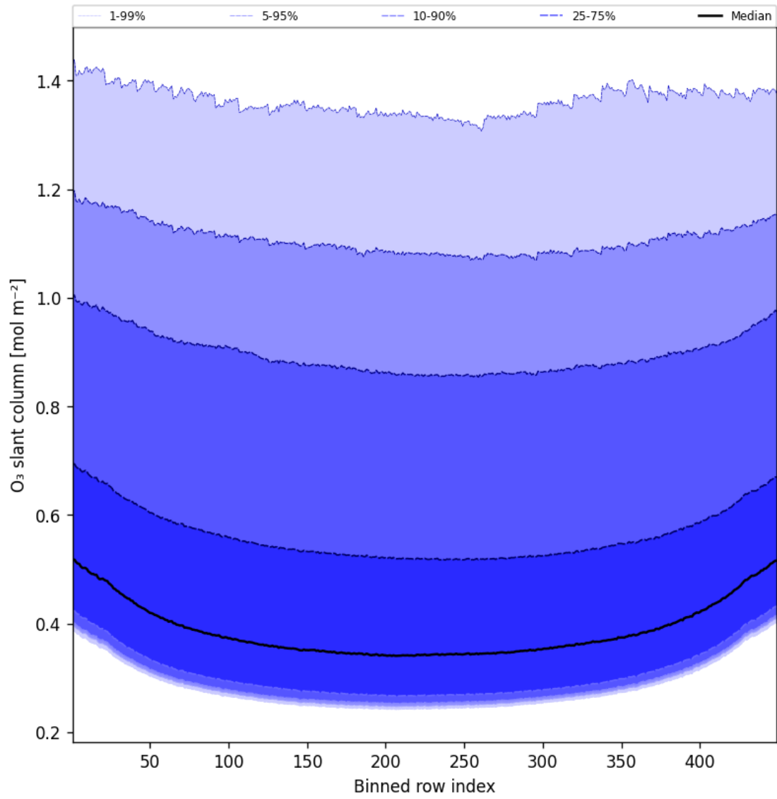
Figure 43: Along track statistics of “O 3 slant column” for 2024-12-11 to 2024-12-12
