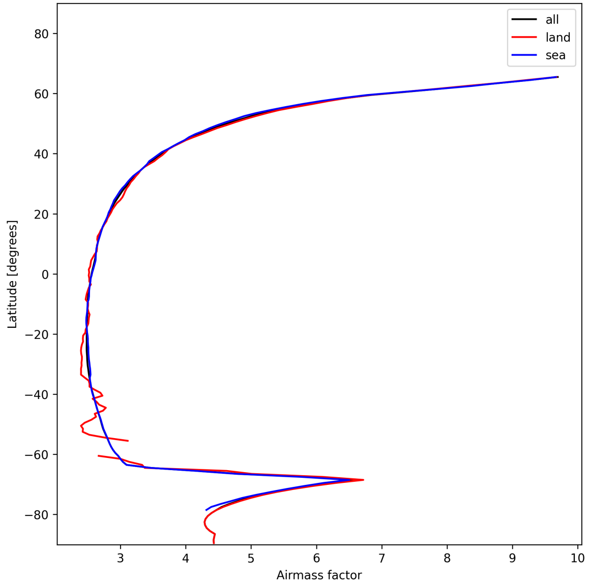
Figure 25: Zonal average of “Airmass factor” for 2024-12-11 to 2024-12-12.
