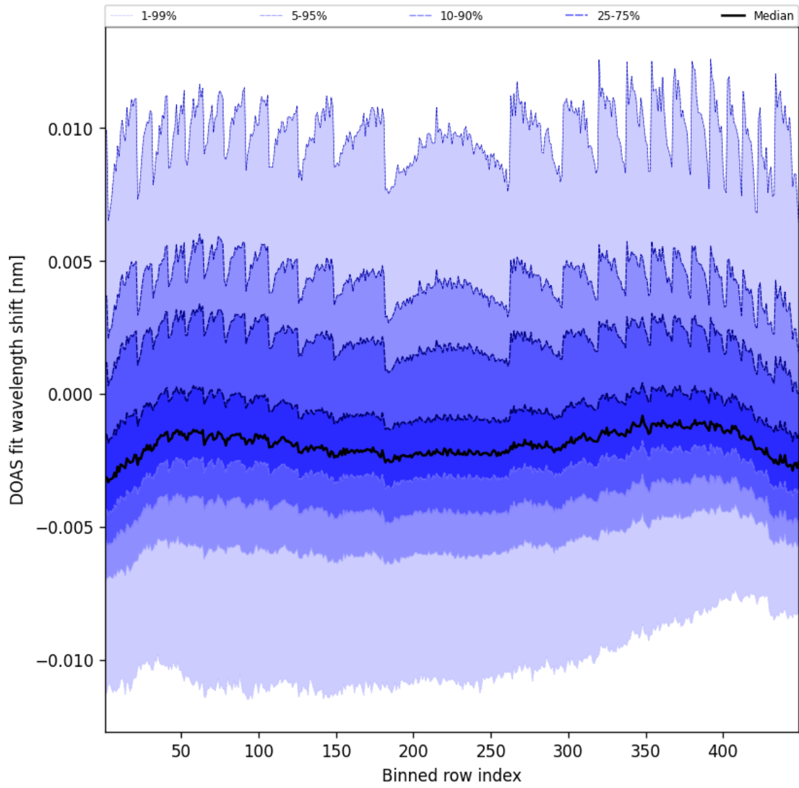
Figure 47: Along track statistics of “DOAS fit wavelength shift” for 2024-12-11 to 2024-12-12
