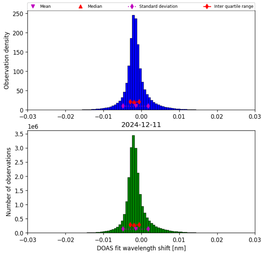
Figure 35: Histogram of “DOAS fit wavelength shift” for 2024-12-11 to 2024-12-12
