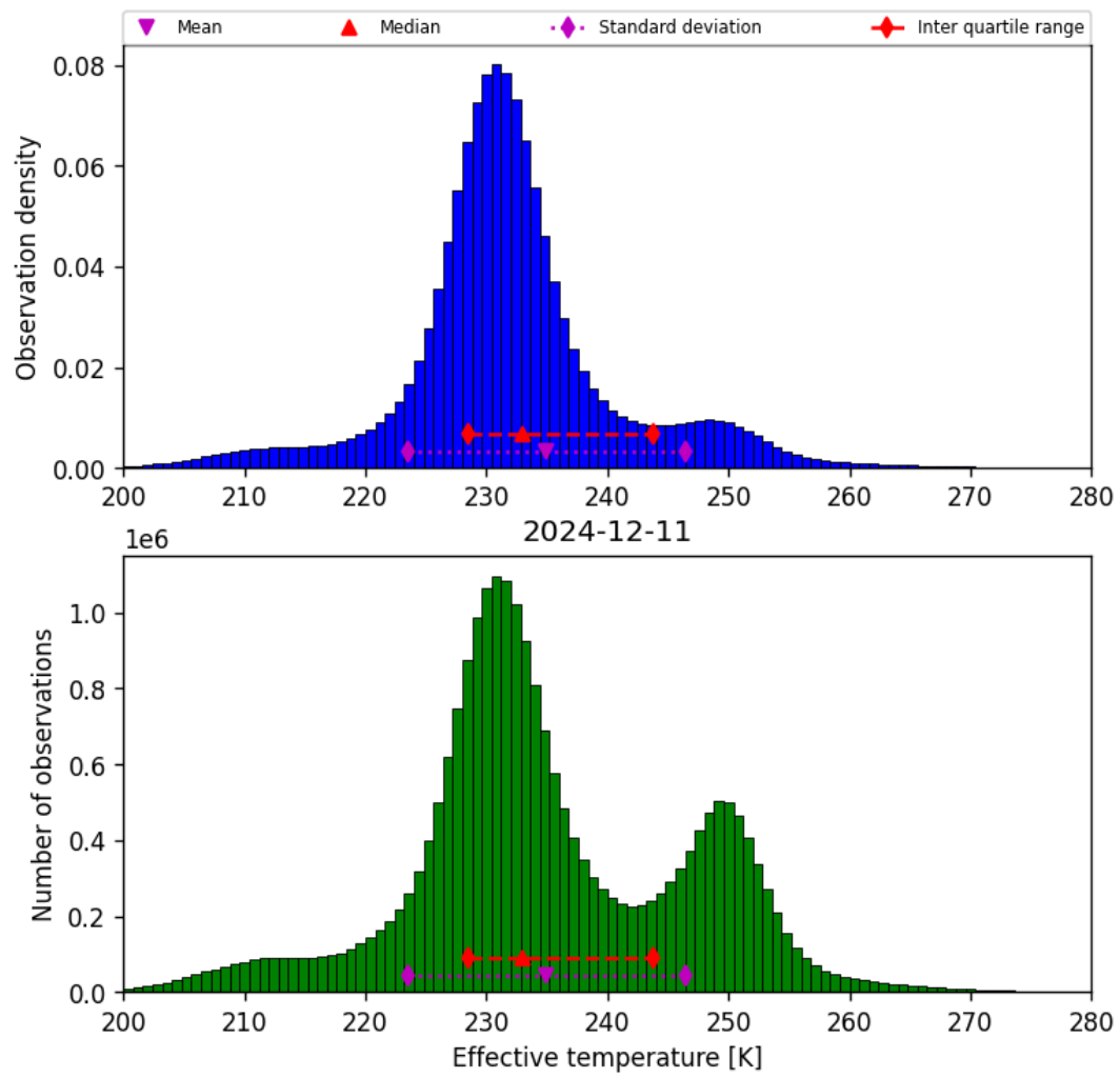
Figure 38: Histogram of “Effective temperature” for 2024-12-11 to 2024-12-12
