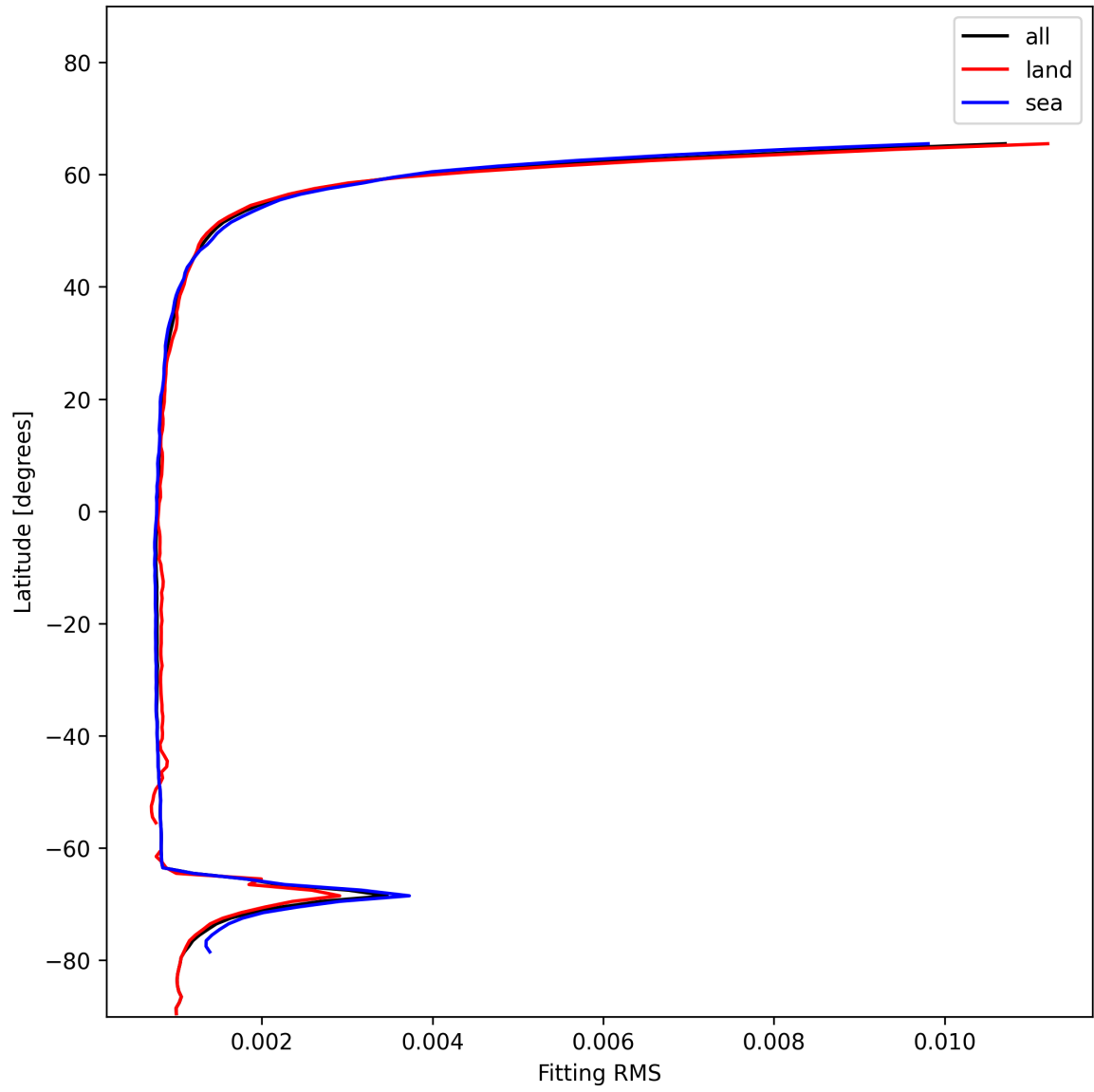
Figure 22: Zonal average of “Fitting RMS” for 2024-12-11 to 2024-12-12.
