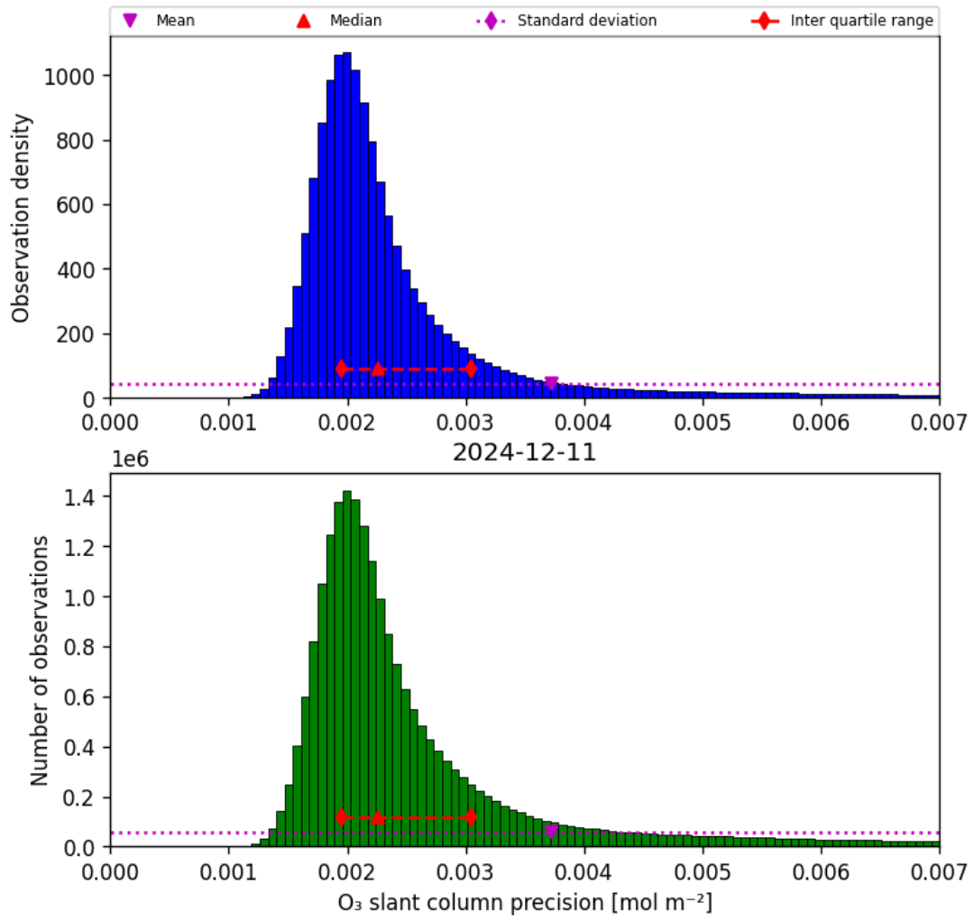
Figure 32: Histogram of “O 3 slant column precision” for 2024-12-11 to 2024-12-12
