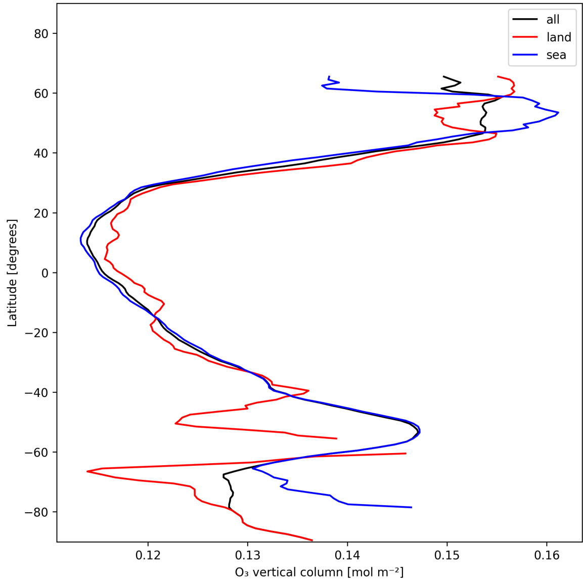
Figure 17: Zonal average of “O 3 vertical column” for 2024-12-11 to 2024-12-12.
