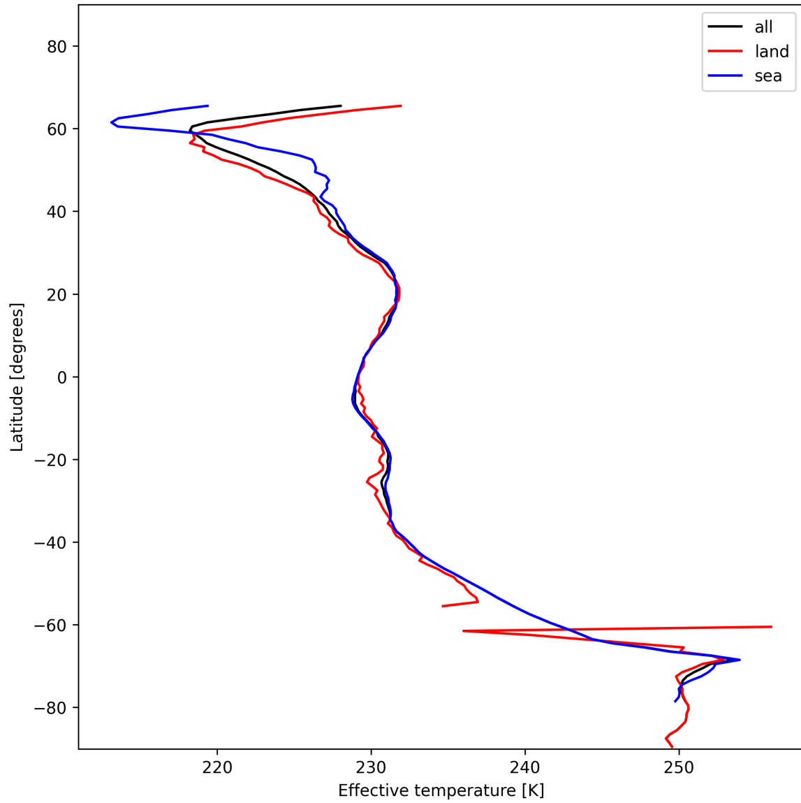
Figure 26: Zonal average of “Effective temperature” for 2024-12-11 to 2024-12-12.
