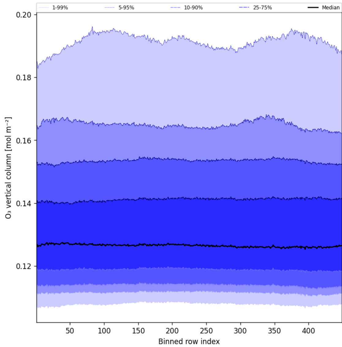
Figure 41: Along track statistics of “O 3 vertical column” for 2024-12-11 to 2024-12-12
