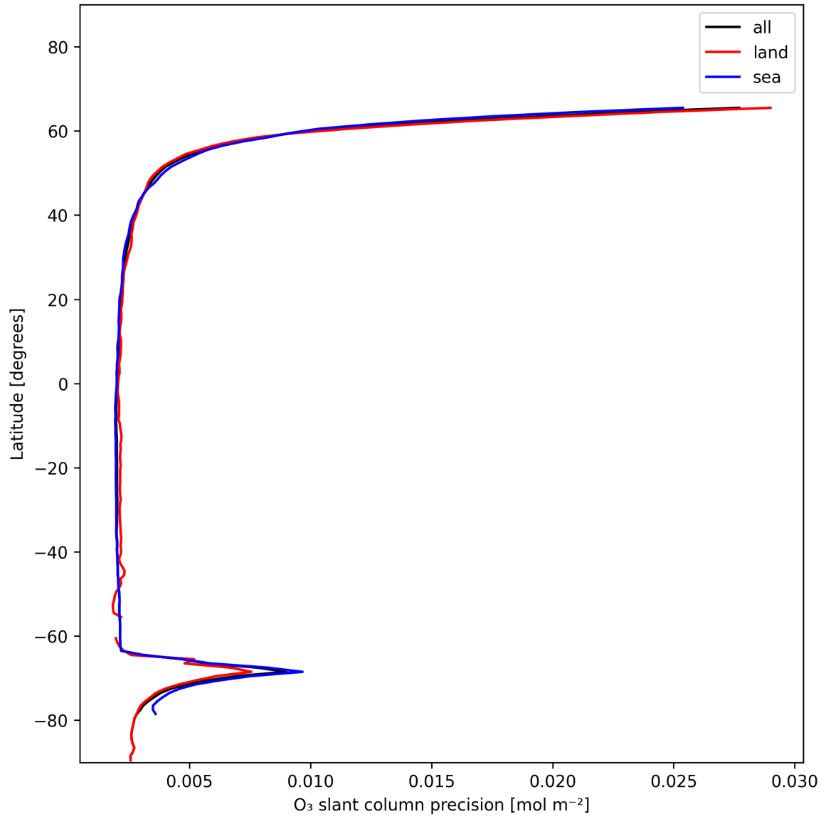
Figure 20: Zonal average of “O 3 slant column precision” for 2024-12-11 to 2024-12-12.
