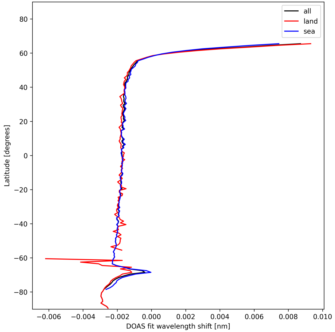
Figure 23: Zonal average of “DOAS fit wavelength shift” for 2024-12-11 to 2024-12-12.
