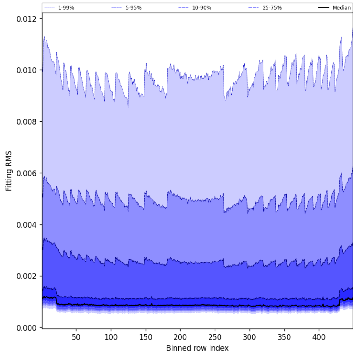
Figure 46: Along track statistics of “Fitting RMS” for 2024-12-11 to 2024-12-12
