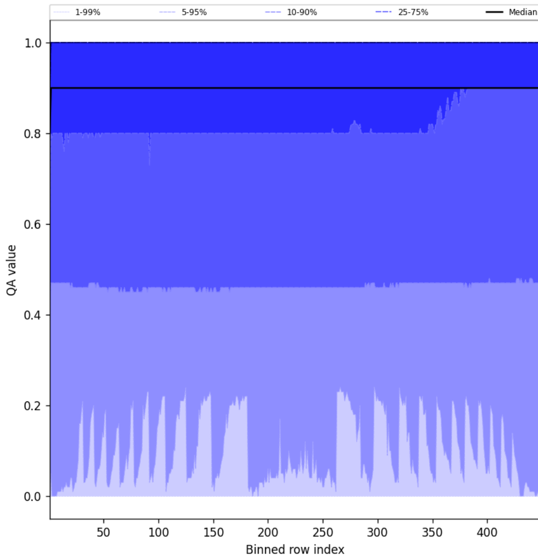
Figure 40: Along track statistics of “QA value” for 2024-12-11 to 2024-12-12
