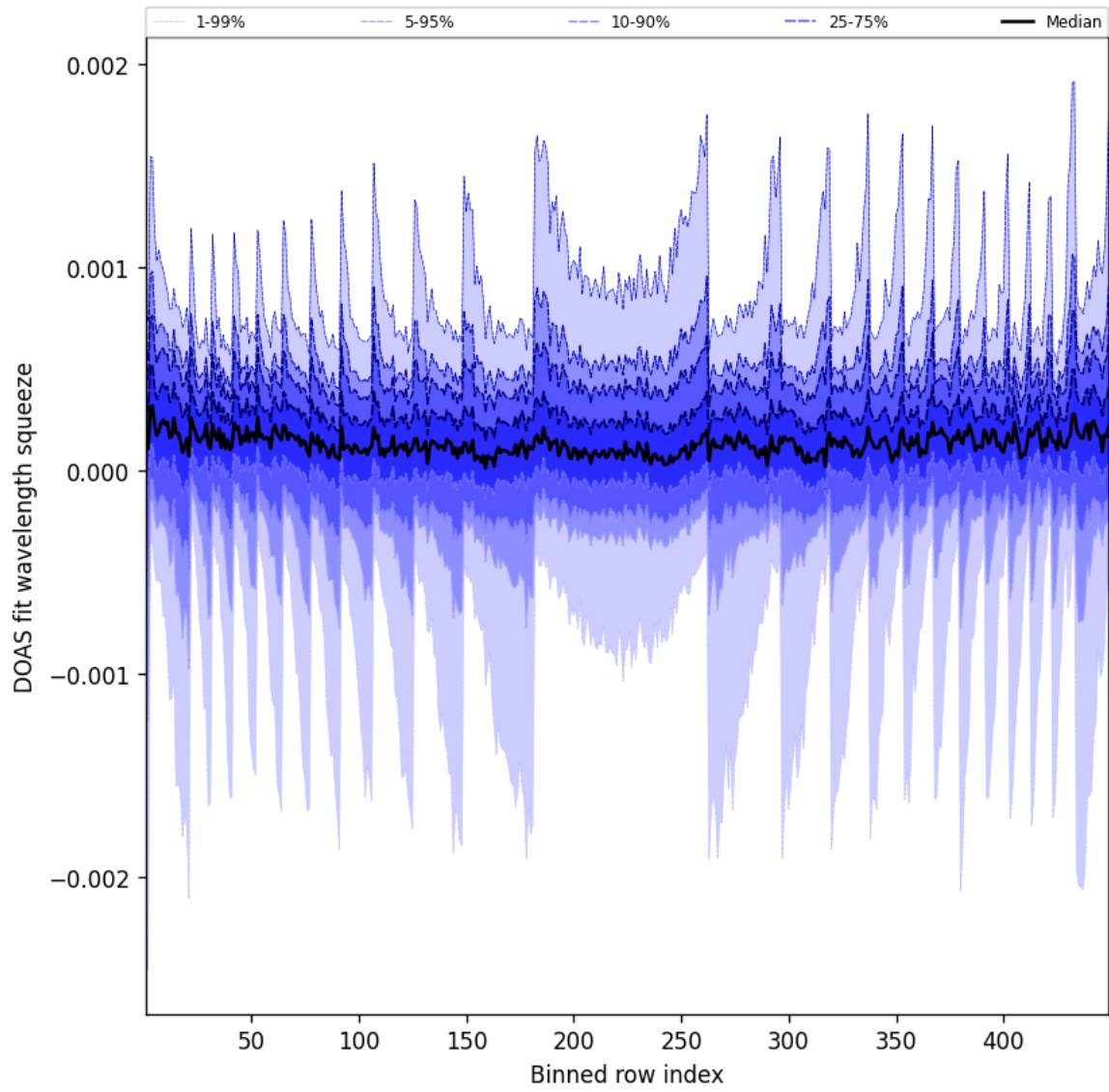
Figure 48: Along track statistics of “DOAS fit wavelength squeeze” for 2024-12-11 to 2024-12-12
