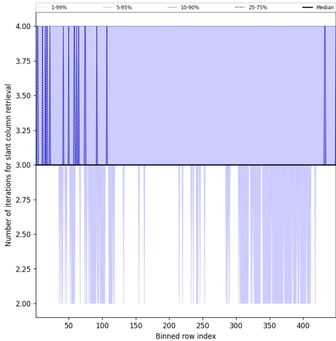
Figure 45: Along track statistics of “Number of iterations for slant column retrieval” for 2024-12-11 to 2024-12-12
