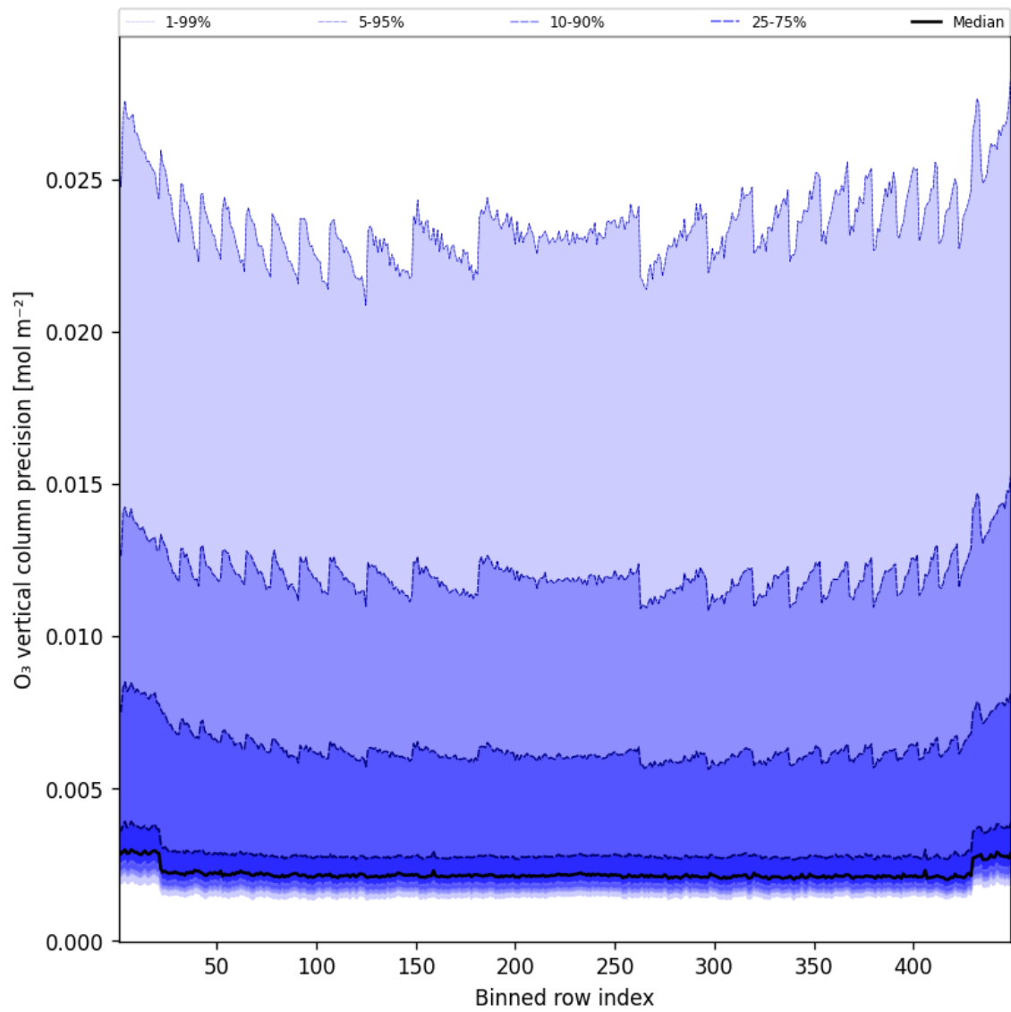
Figure 42: Along track statistics of “O 3 vertical column precision” for 2024-12-11 to 2024-12-12
