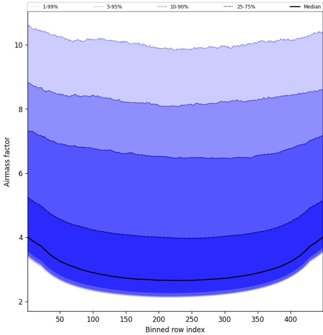
Figure 49: Along track statistics of “Airmass factor” for 2024-12-11 to 2024-12-12
