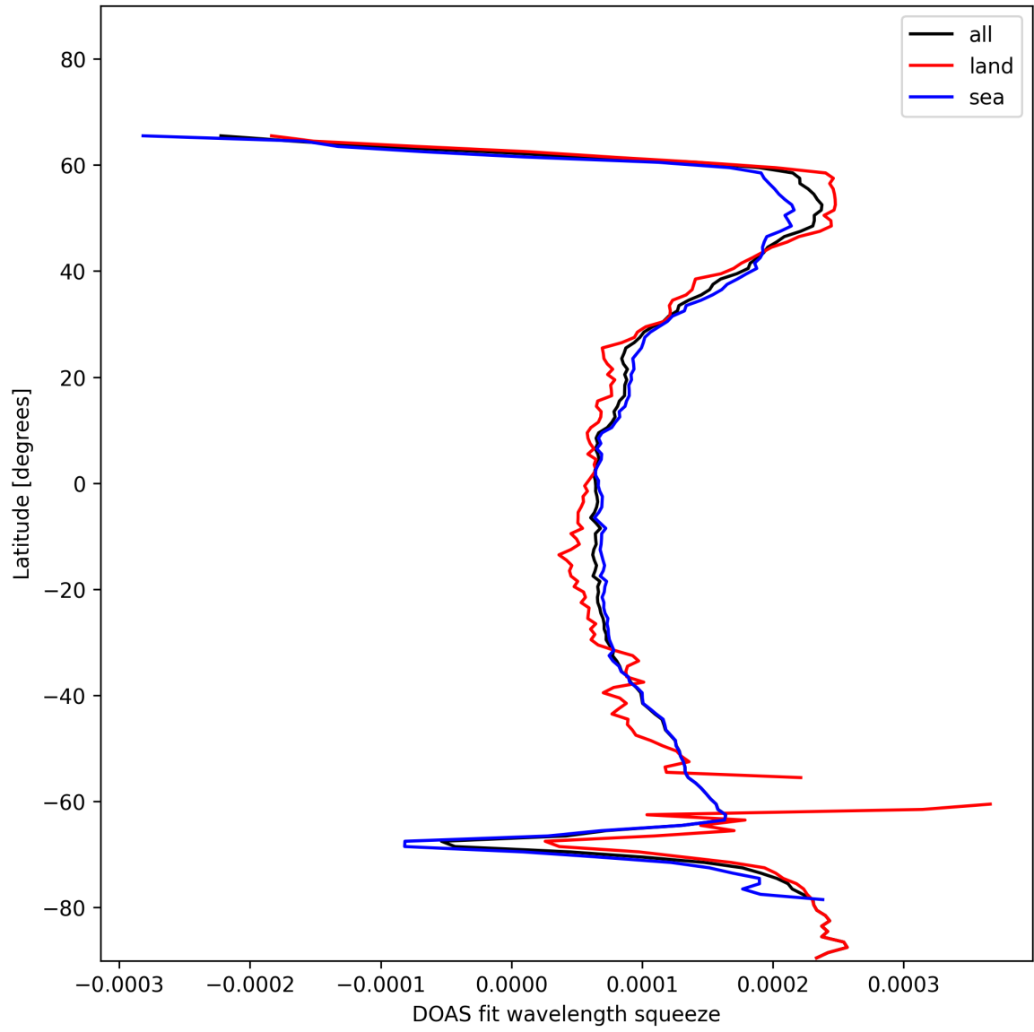
Figure 24: Zonal average of “DOAS fit wavelength squeeze” for 2024-12-13 to 2024-12-14.
