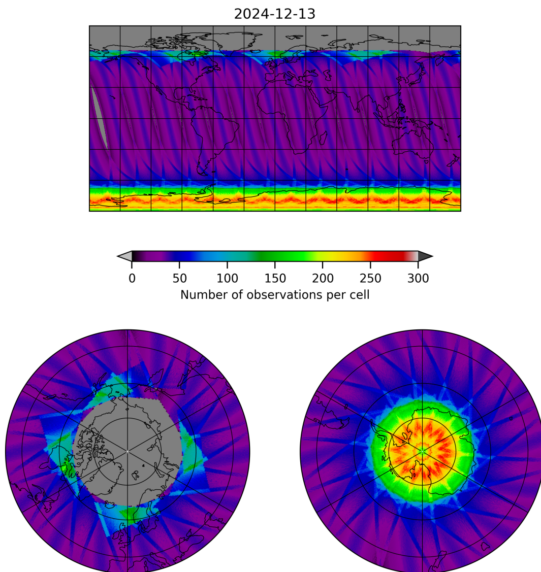
Figure 15: Map of the number of observations for 2024-12-13 to 2024-12-14
