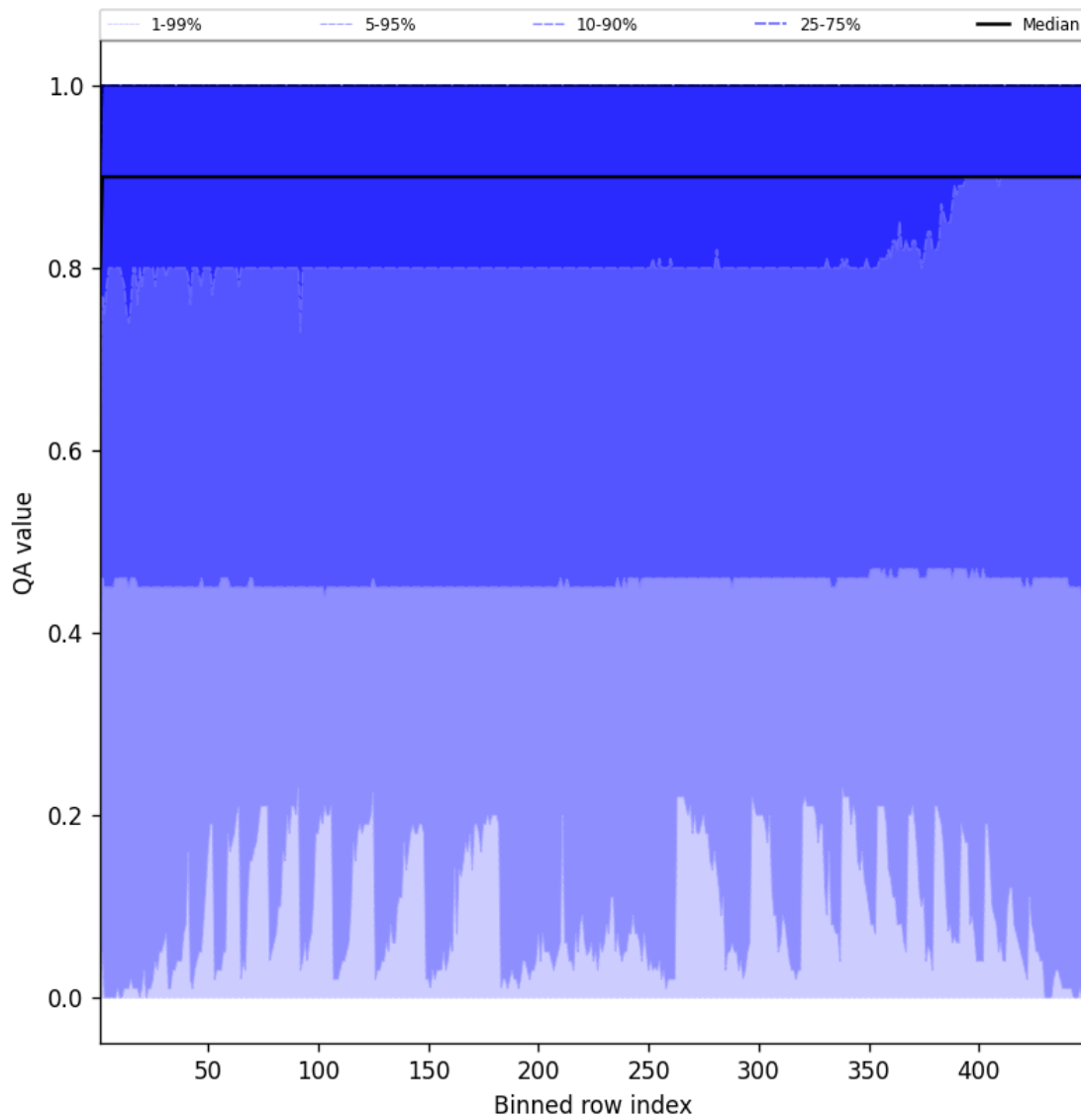
Figure 40: Along track statistics of “QA value” for 2024-12-13 to 2024-12-14
