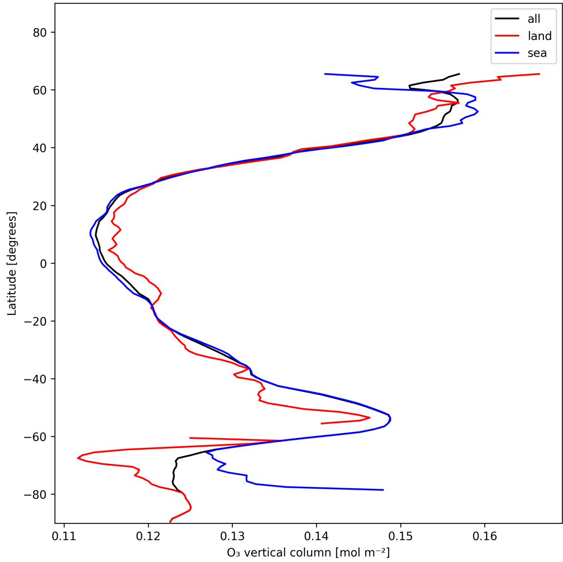
Figure 17: Zonal average of “O 3 vertical column” for 2024-12-13 to 2024-12-14.
