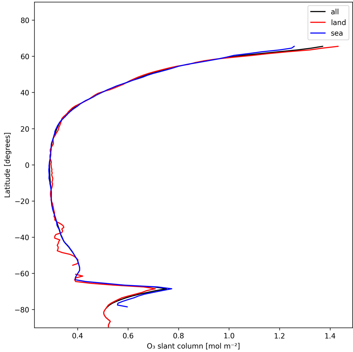
Figure 19: Zonal average of “O 3 slant column” for 2024-12-13 to 2024-12-14.
