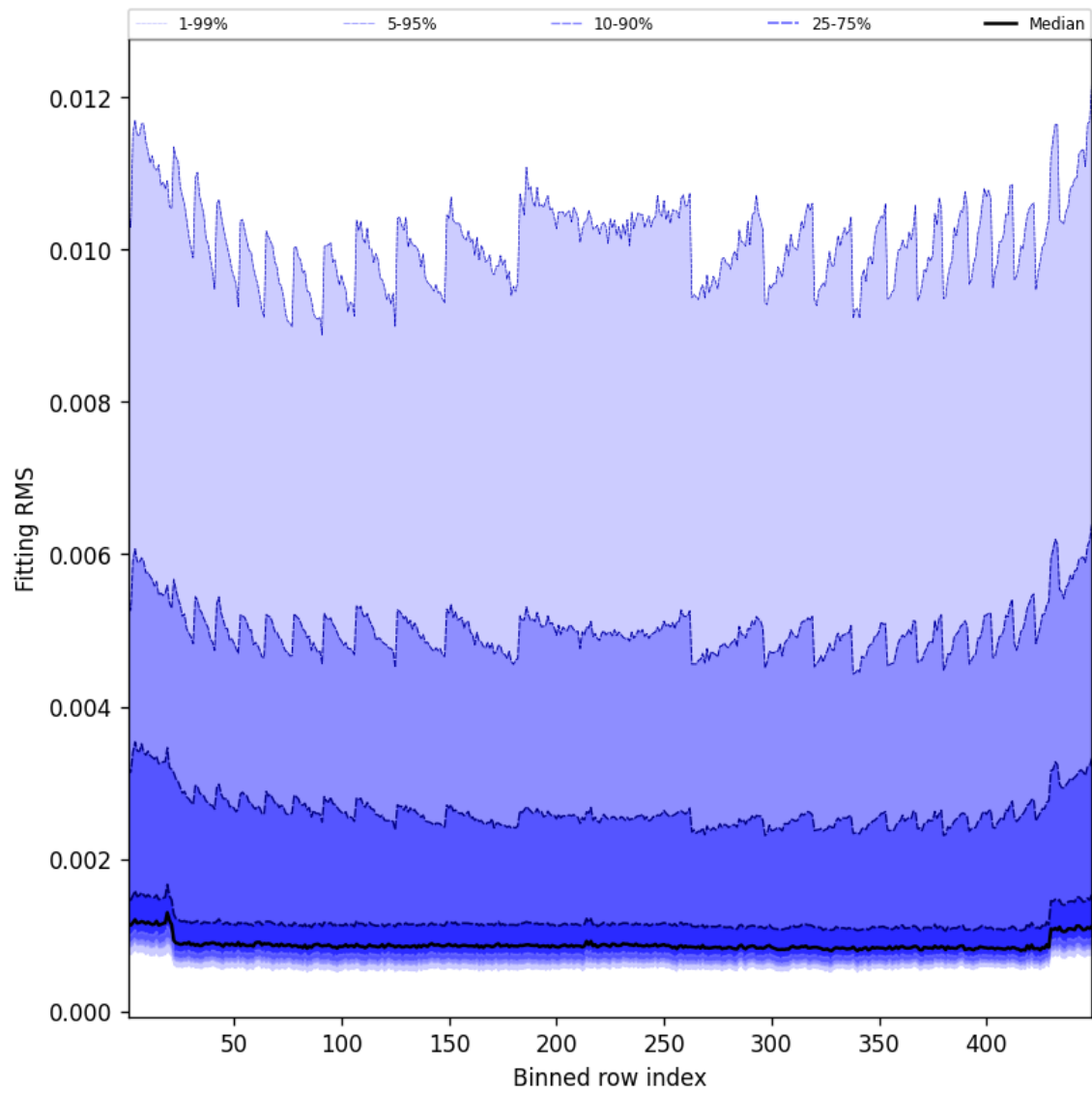
Figure 46: Along track statistics of “Fitting RMS” for 2024-12-13 to 2024-12-14
