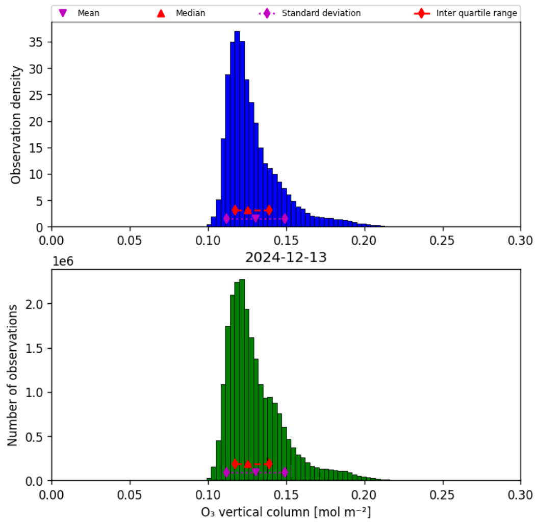
Figure 29: Histogram of “O 3 vertical column” for 2024-12-13 to 2024-12-14
