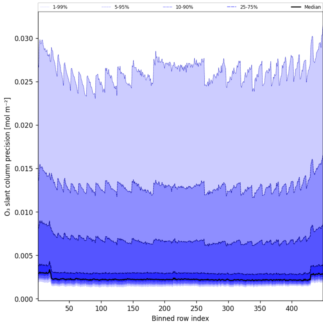
Figure 44: Along track statistics of “O 3 slant column precision” for 2024-12-13 to 2024-12-14
