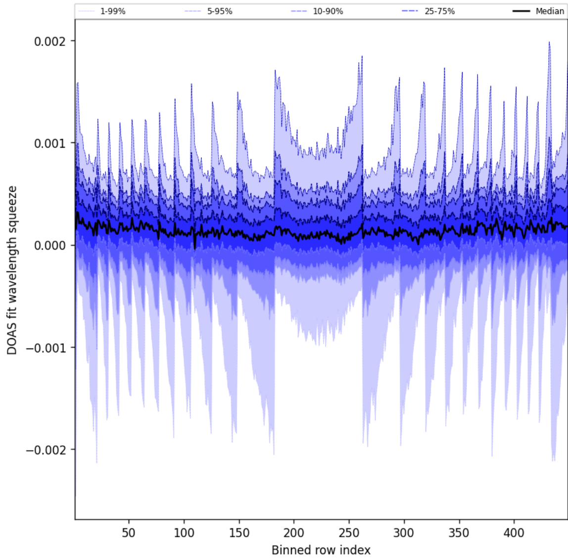
Figure 48: Along track statistics of “DOAS fit wavelength squeeze” for 2024-12-13 to 2024-12-14
