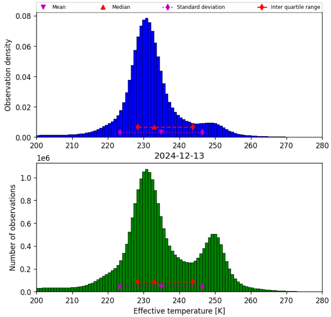
Figure 38: Histogram of “Effective temperature” for 2024-12-13 to 2024-12-14
