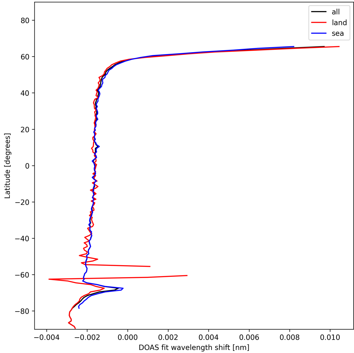
Figure 23: Zonal average of “DOAS fit wavelength shift” for 2024-12-13 to 2024-12-14.
