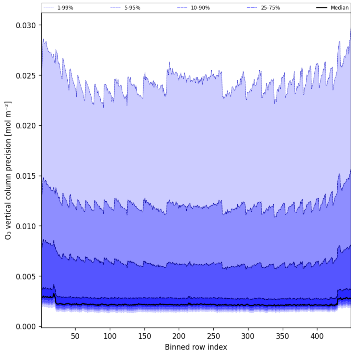
Figure 42: Along track statistics of “O 3 vertical column precision” for 2024-12-13 to 2024-12-14
