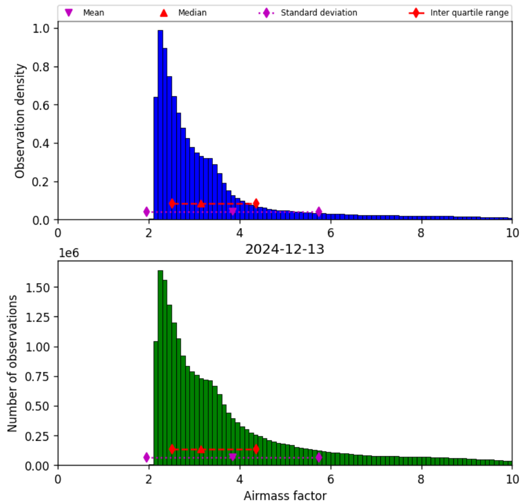
Figure 37: Histogram of “Airmass factor” for 2024-12-13 to 2024-12-14
