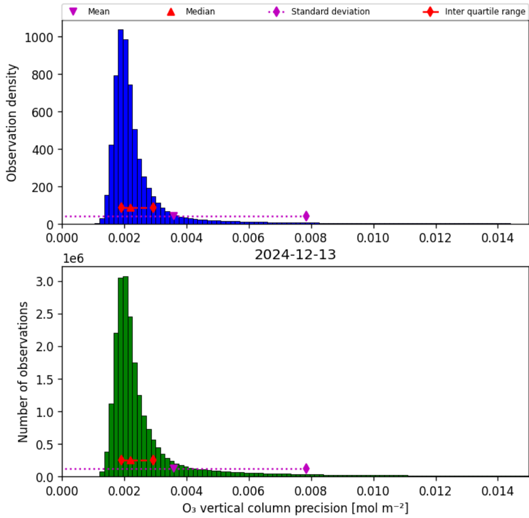
Figure 30: Histogram of “O 3 vertical column precision” for 2024-12-13 to 2024-12-14
