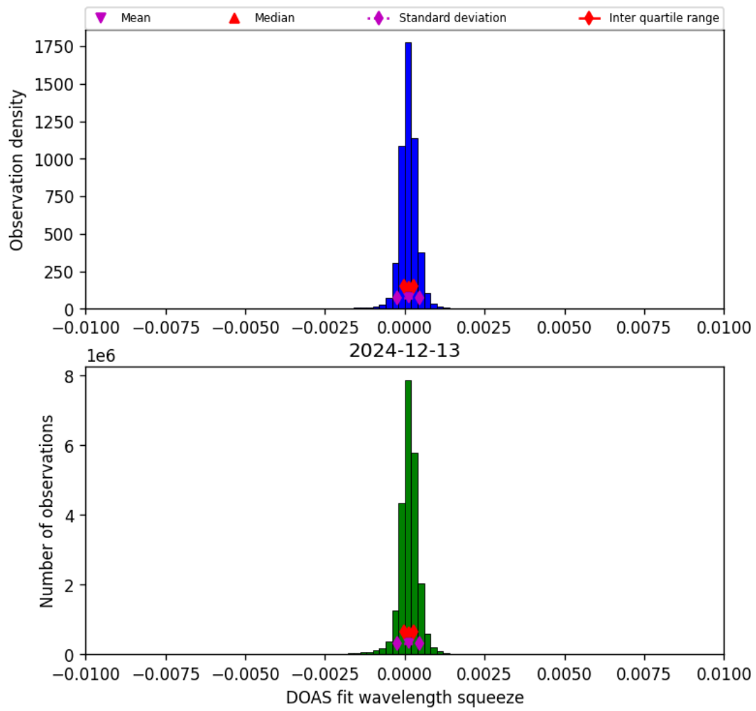
Figure 36: Histogram of “DOAS fit wavelength squeeze” for 2024-12-13 to 2024-12-14
