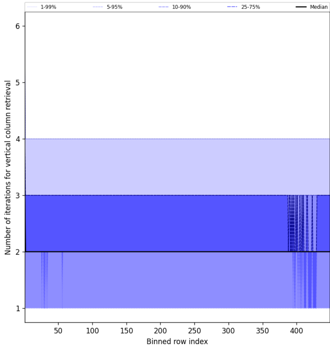
Figure 51: Along track statistics of “Number of iterations for vertical column retrieval” for 2024-12-13 to 2024-12-14
