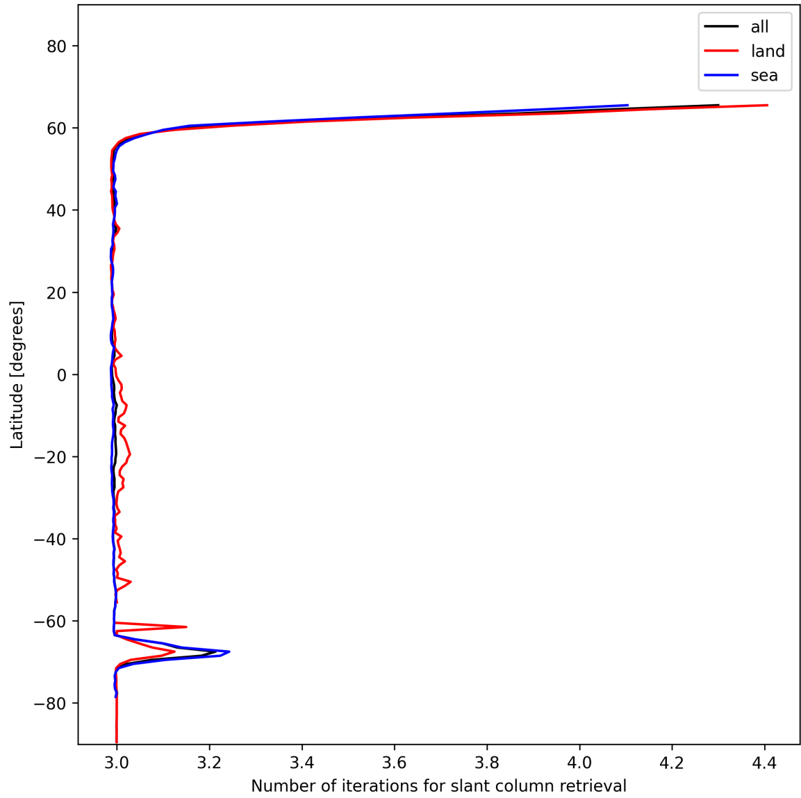
Figure 21: Zonal average of “Number of iterations for slant column retrieval” for 2024-12-13 to 2024-12-14.
