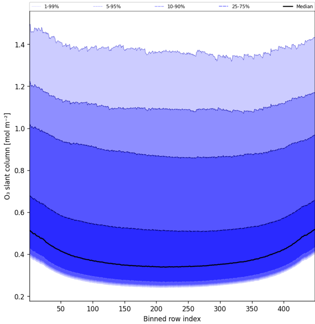
Figure 43: Along track statistics of “O 3 slant column” for 2024-12-13 to 2024-12-14
