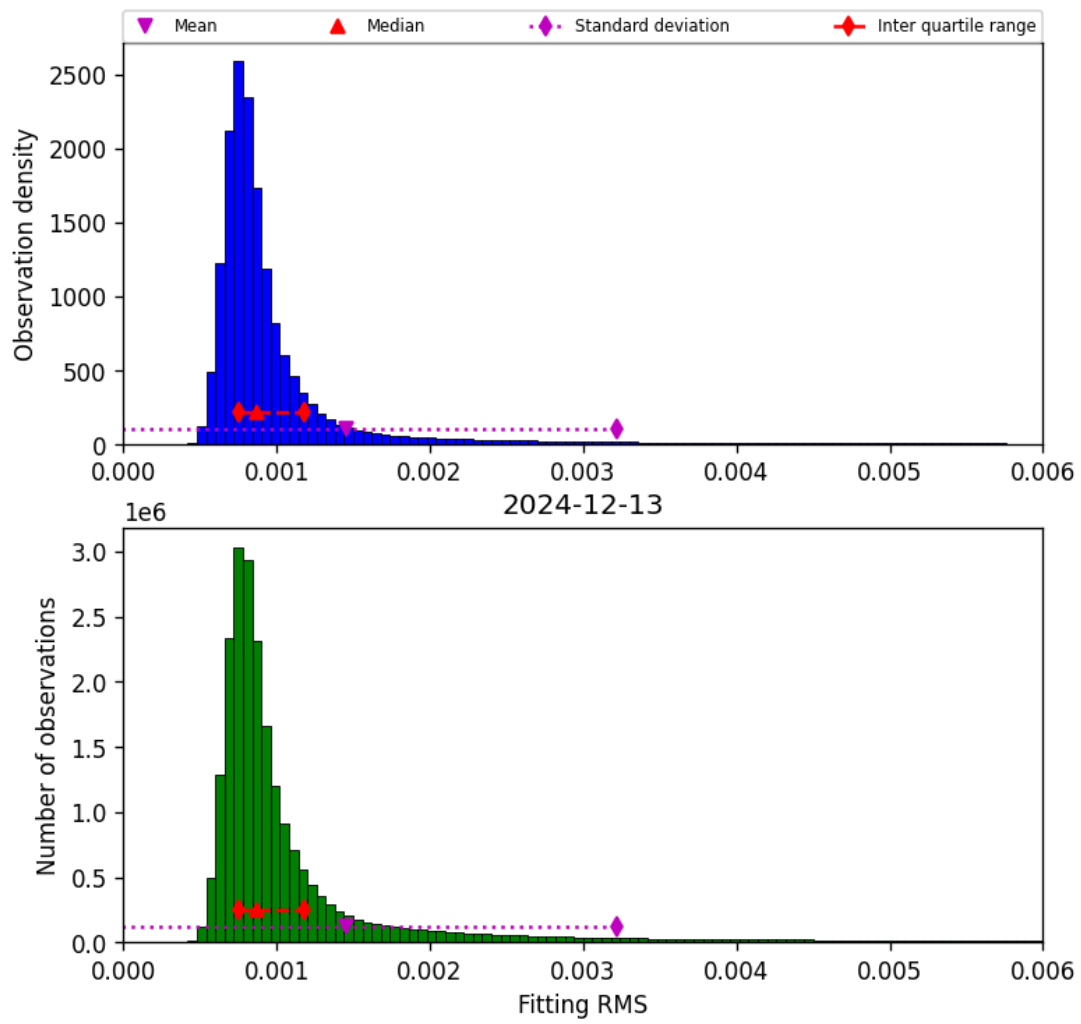
Figure 34: Histogram of “Fitting RMS” for 2024-12-13 to 2024-12-14
