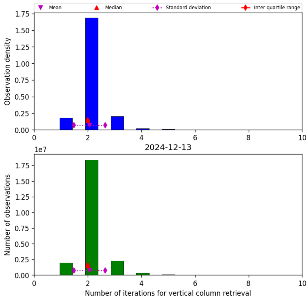
Figure 39: Histogram of “Number of iterations for vertical column retrieval” for 2024-12-13 to 2024-12-14
