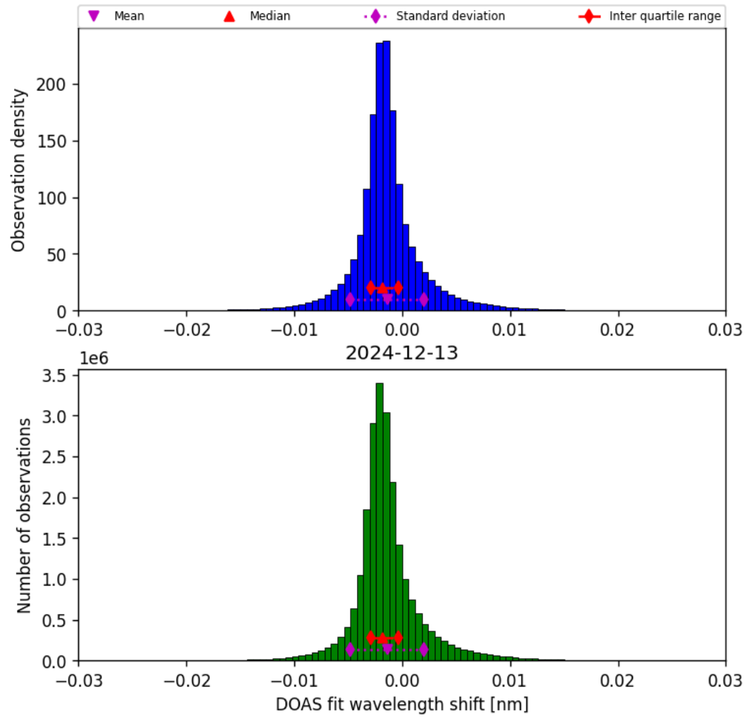
Figure 35: Histogram of “DOAS fit wavelength shift” for 2024-12-13 to 2024-12-14
