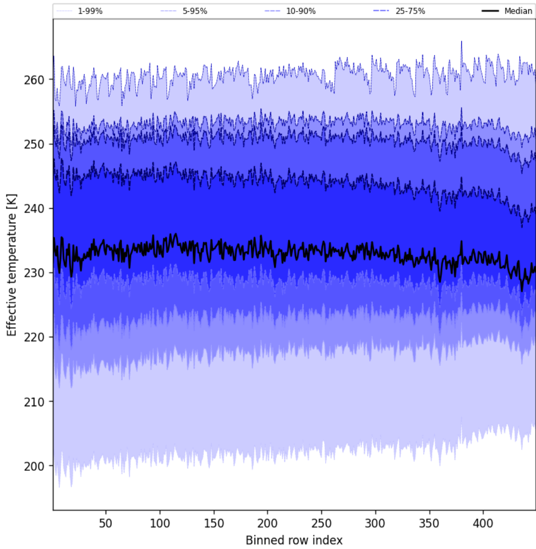
Figure 50: Along track statistics of “Effective temperature” for 2024-12-13 to 2024-12-14
