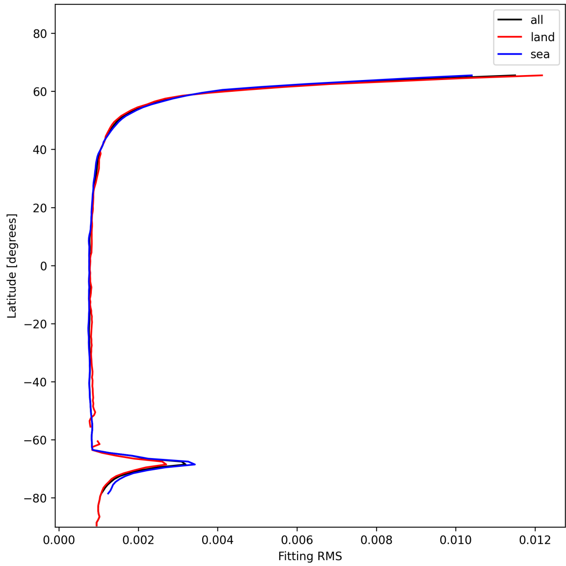
Figure 22: Zonal average of “Fitting RMS” for 2024-12-13 to 2024-12-14.
