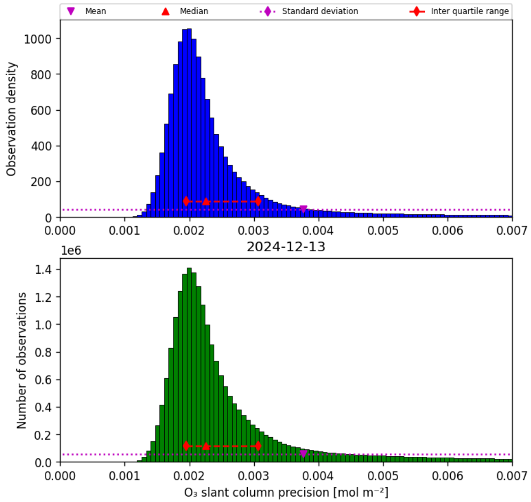
Figure 32: Histogram of “O 3 slant column precision” for 2024-12-13 to 2024-12-14
