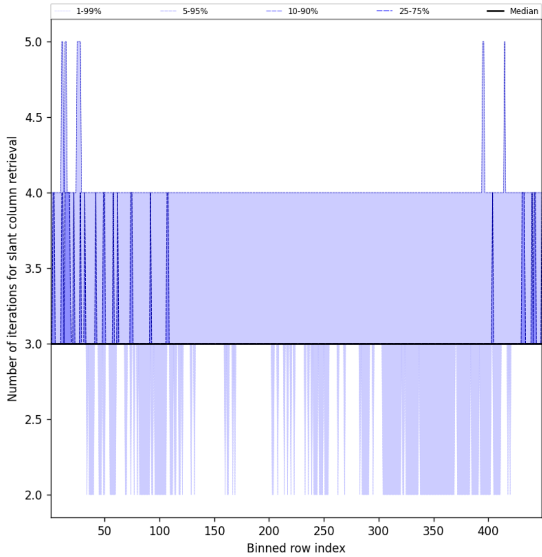
Figure 45: Along track statistics of “Number of iterations for slant column retrieval” for 2024-12-13 to 2024-12-14
