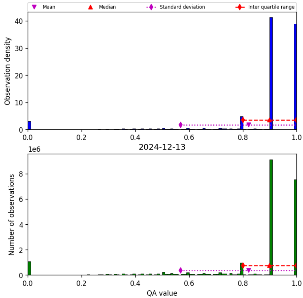
Figure 28: Histogram of “QA value” for 2024-12-13 to 2024-12-14
