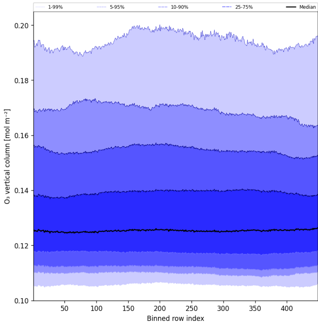
Figure 41: Along track statistics of “O 3 vertical column” for 2024-12-13 to 2024-12-14
