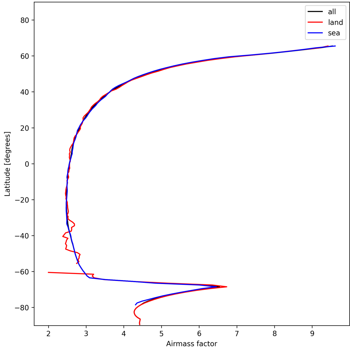
Figure 25: Zonal average of “Airmass factor” for 2024-12-13 to 2024-12-14.
