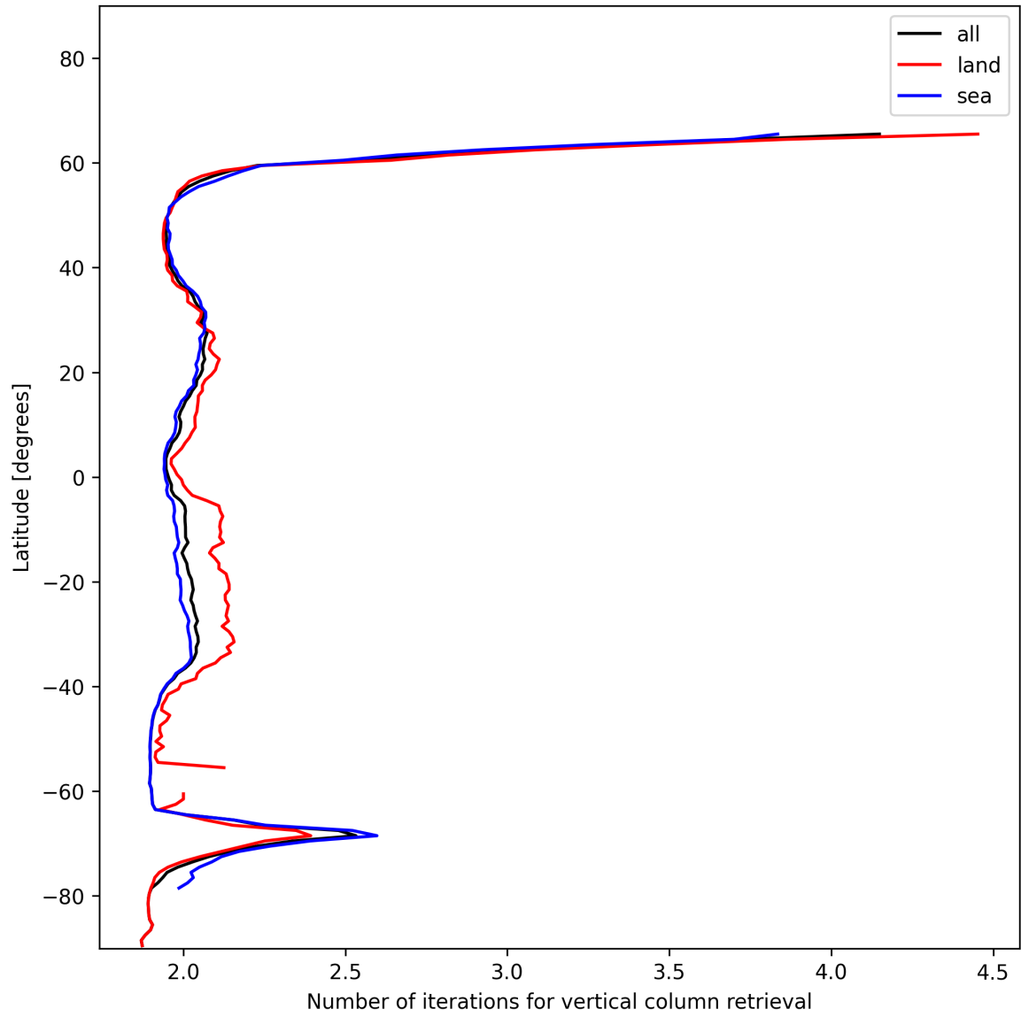
Figure 27: Zonal average of “Number of iterations for vertical column retrieval” for 2024-12-13 to 2024-12-14.
