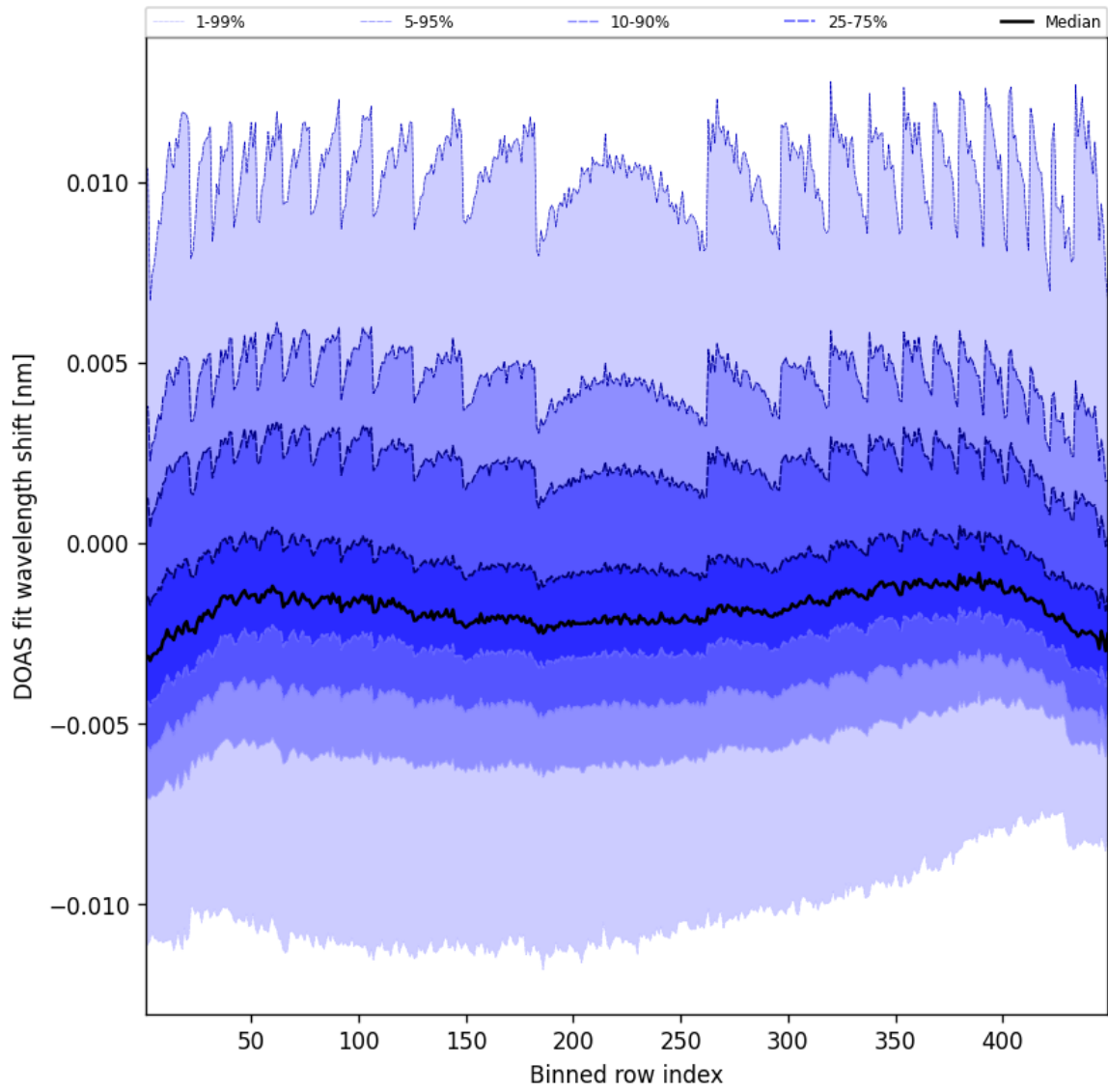
Figure 47: Along track statistics of "DOAS fit wavelength shift" for 2024-12-13 to 2024-12-14
