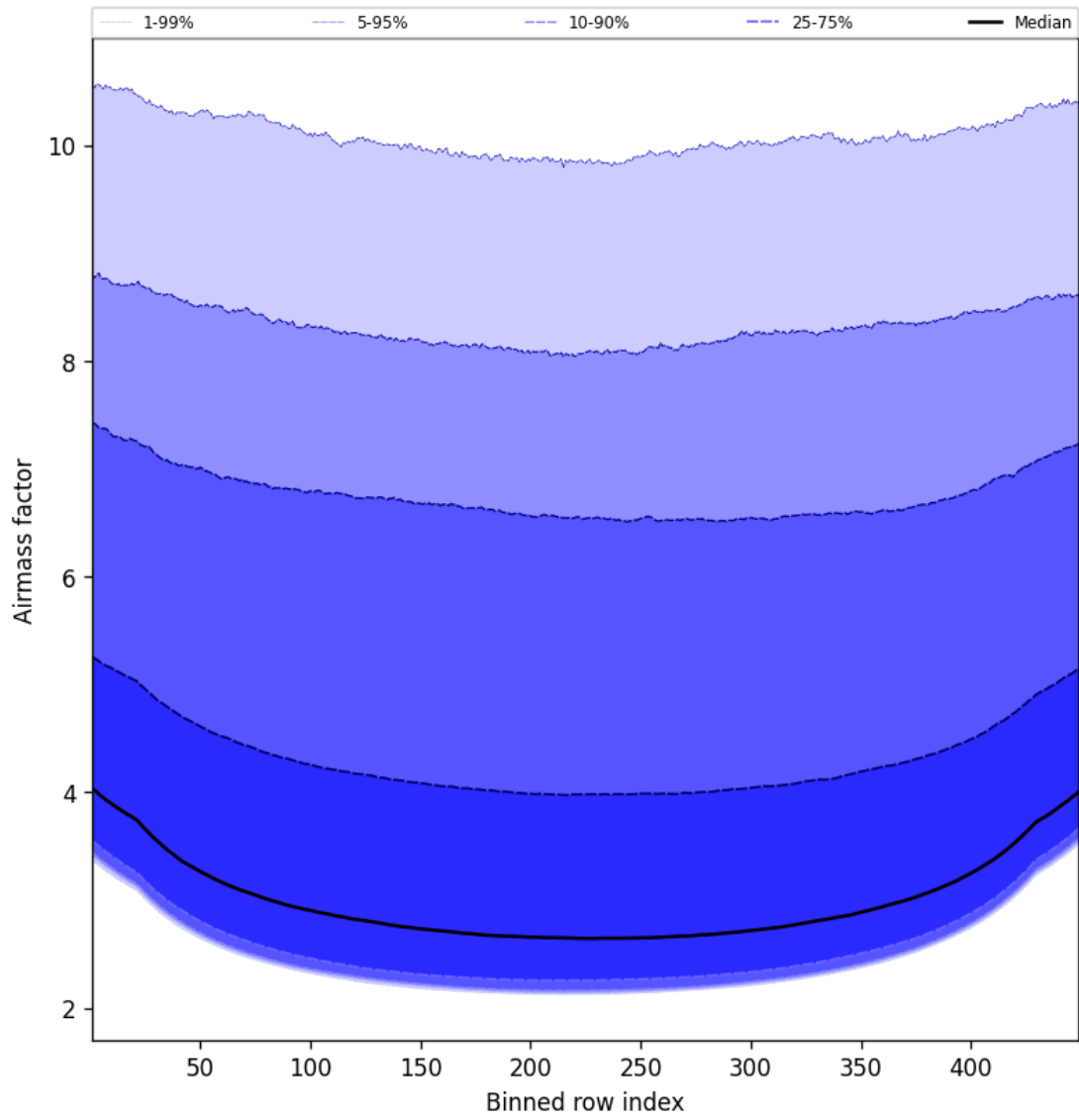
Figure 49: Along track statistics of “Airmass factor” for 2024-12-13 to 2024-12-14
