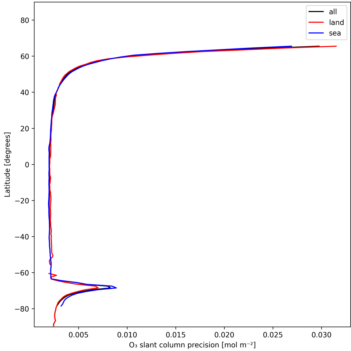
Figure 20: Zonal average of “O 3 slant column precision” for 2024-12-13 to 2024-12-14.
