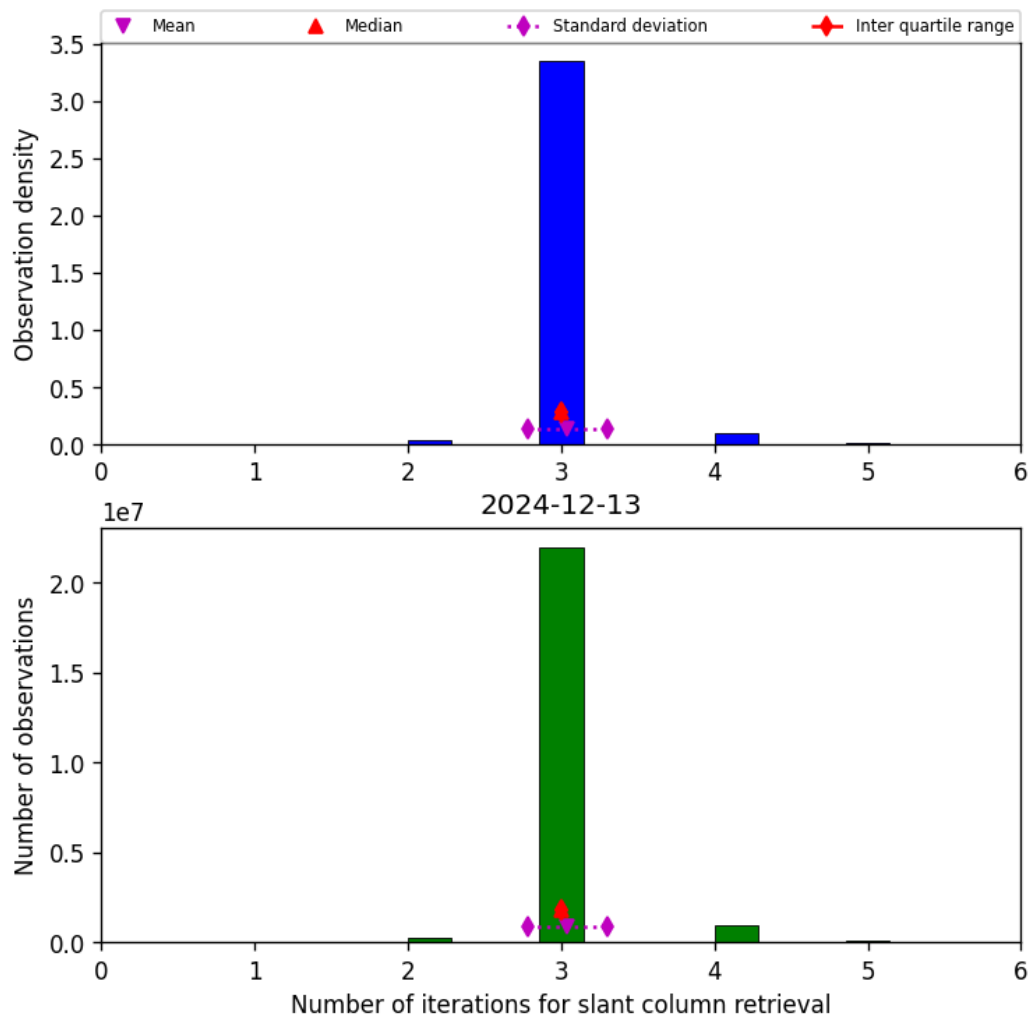
Figure 33: Histogram of “Number of iterations for slant column retrieval” for 2024-12-13 to 2024-12-14
