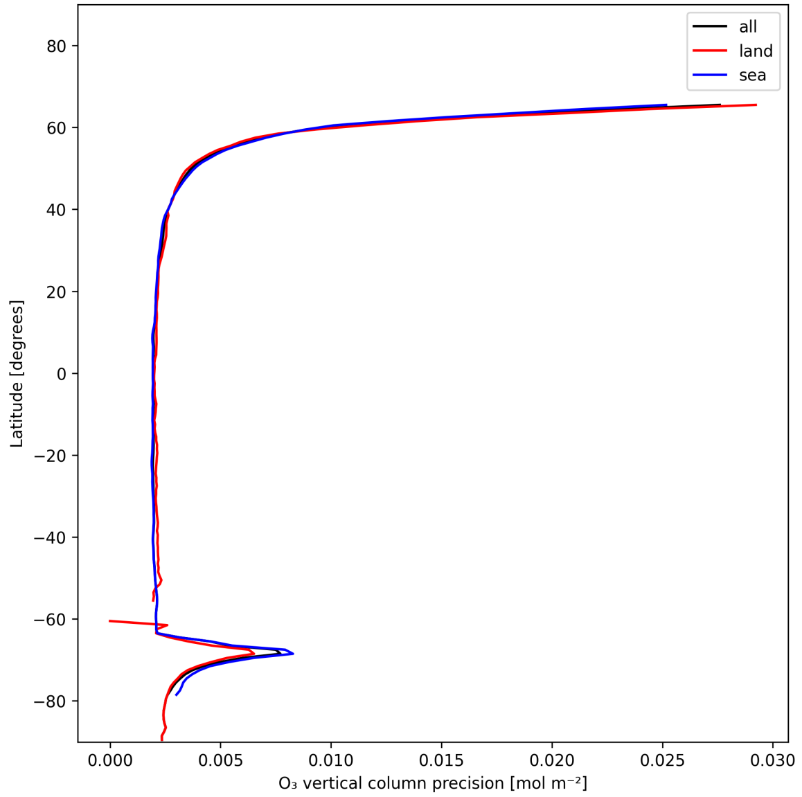
Figure 18: Zonal average of “O 3 vertical column precision” for 2024-12-13 to 2024-12-14.
