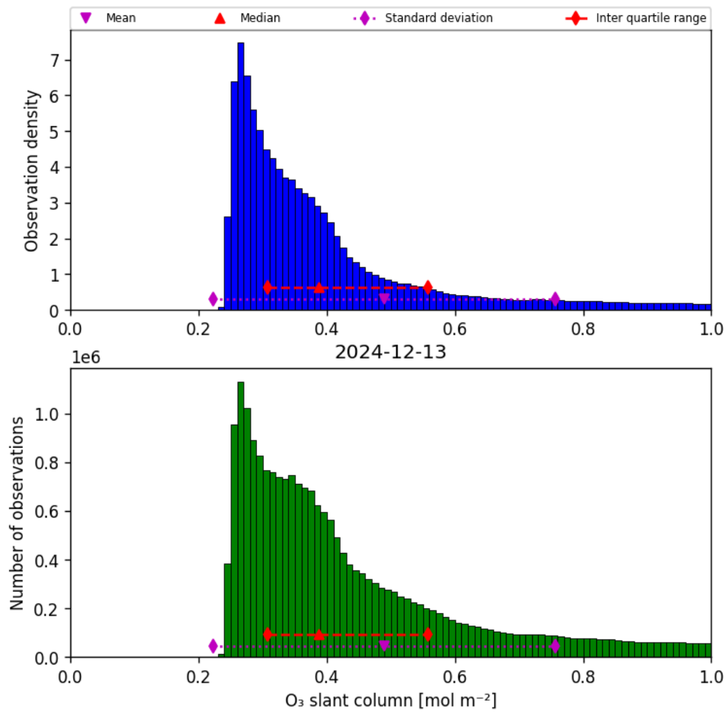
Figure 31: Histogram of “O 3 slant column” for 2024-12-13 to 2024-12-14
