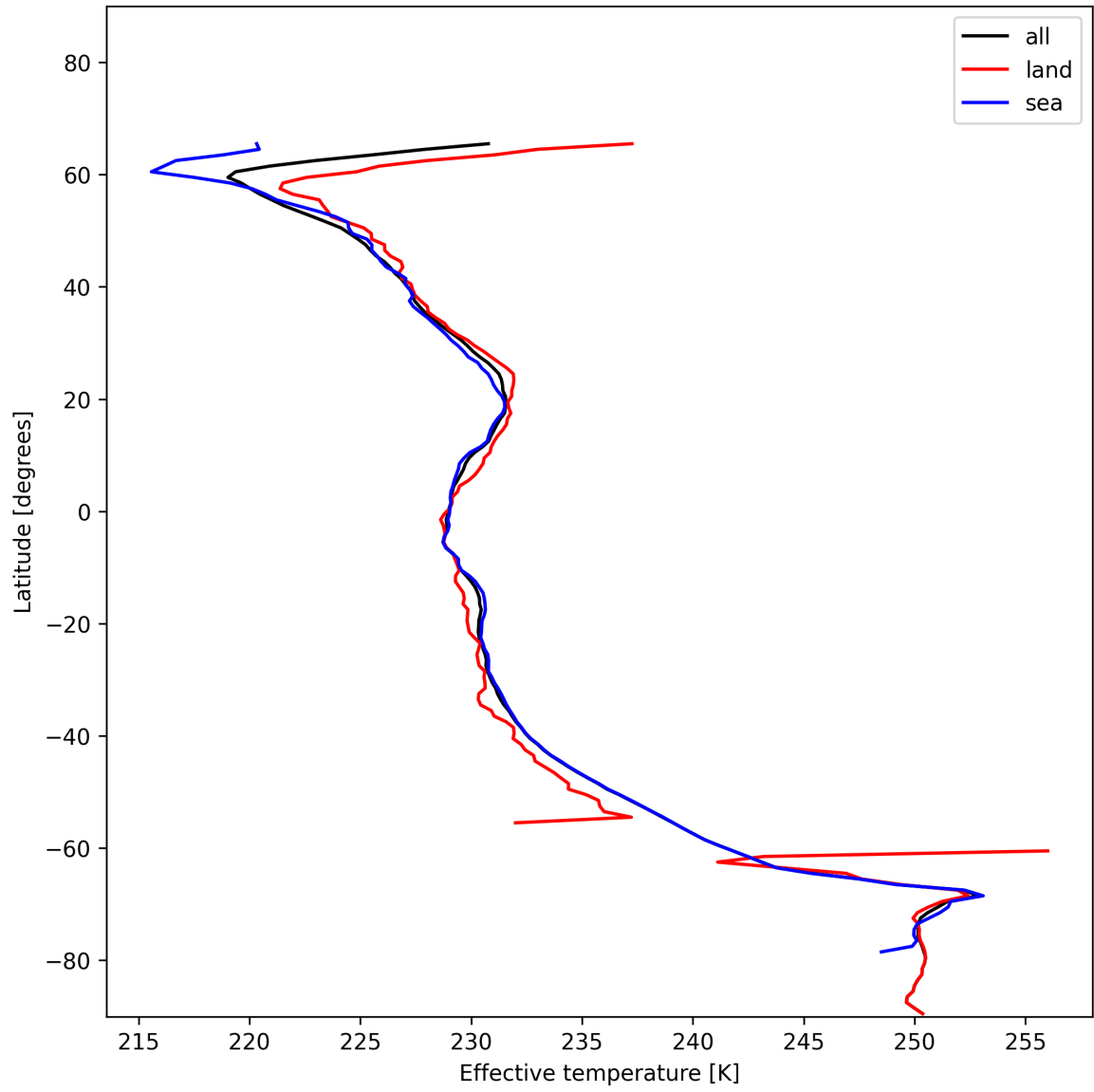
Figure 26: Zonal average of “Effective temperature” for 2024-12-13 to 2024-12-14.
