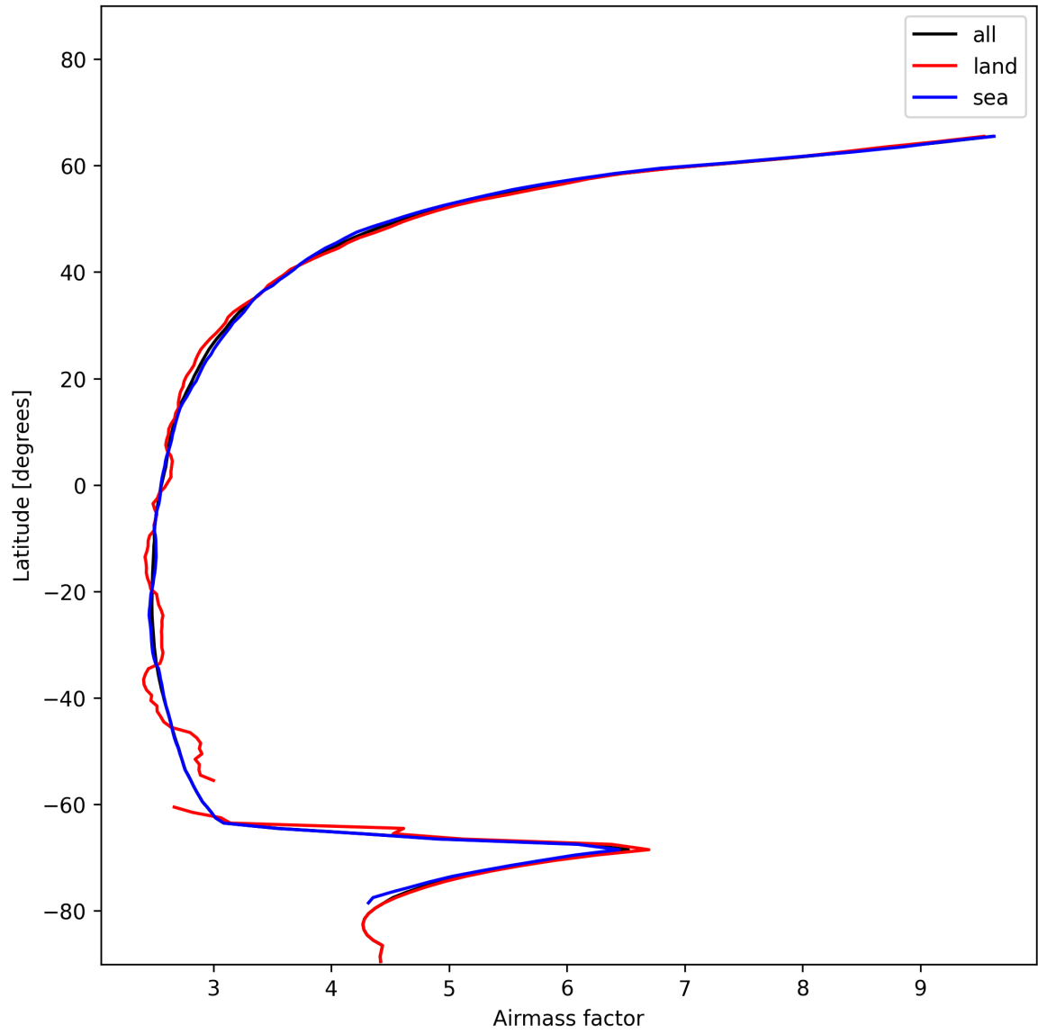
Figure 25: Zonal average of “Airmass factor” for 2024-12-14 to 2024-12-14.
