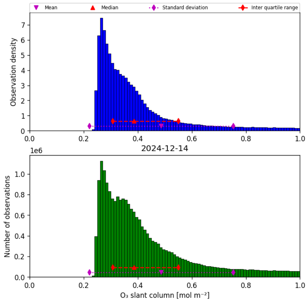
Figure 31: Histogram of “O 3 slant column” for 2024-12-14 to 2024-12-14
