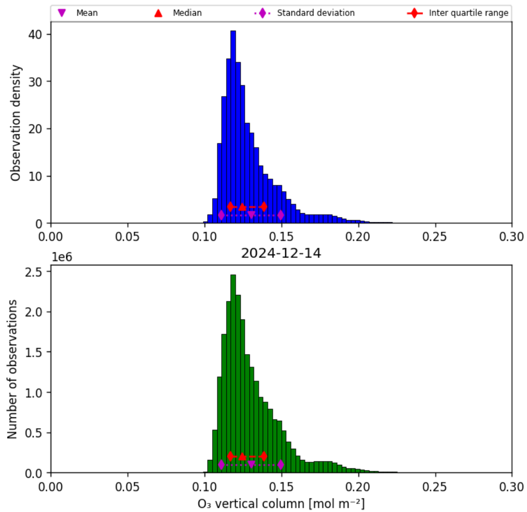
Figure 29: Histogram of “O 3 vertical column” for 2024-12-14 to 2024-12-14
