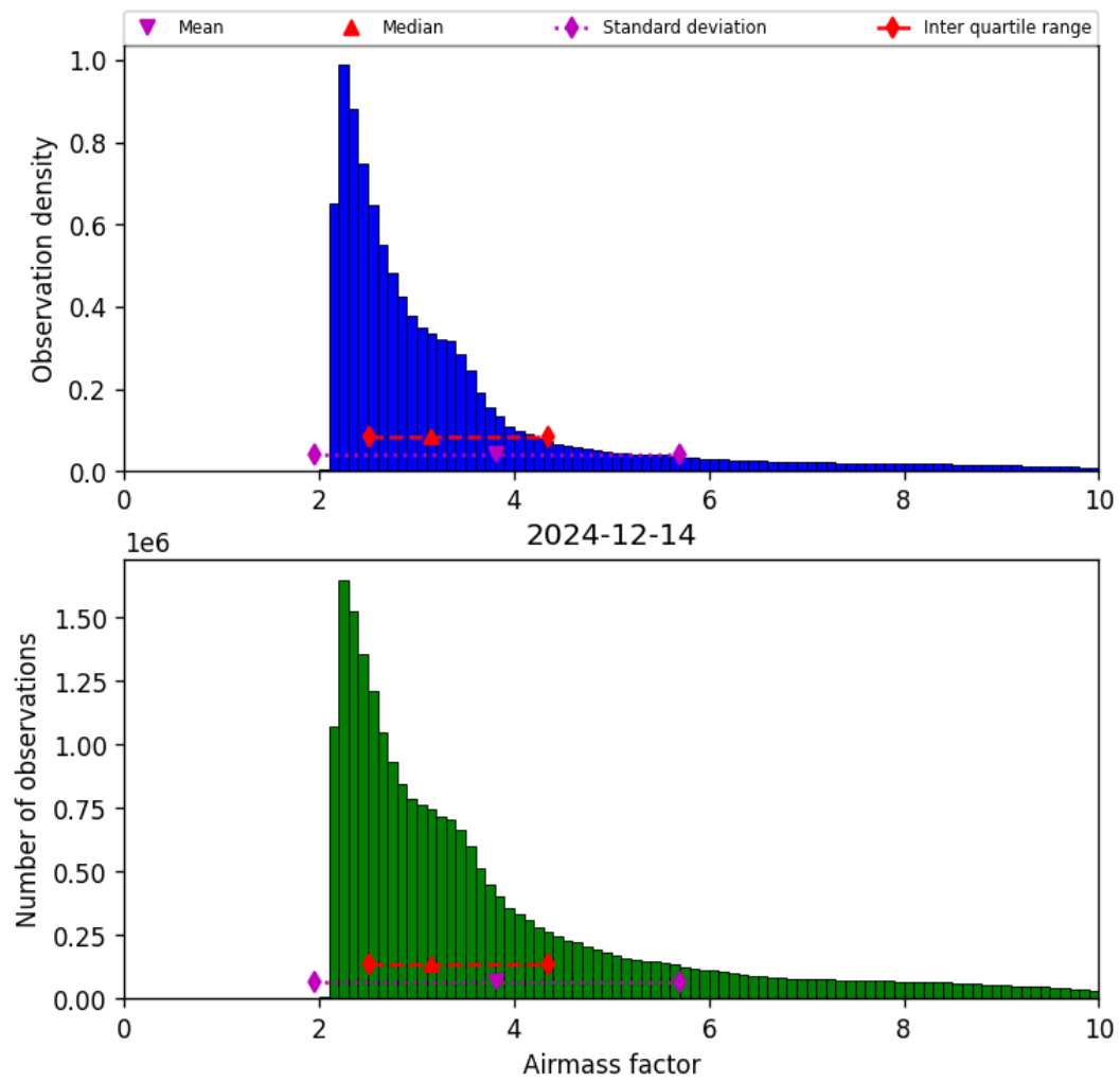
Figure 37: Histogram of "Airmass factor" for 2024-12-14 to 2024-12-14
