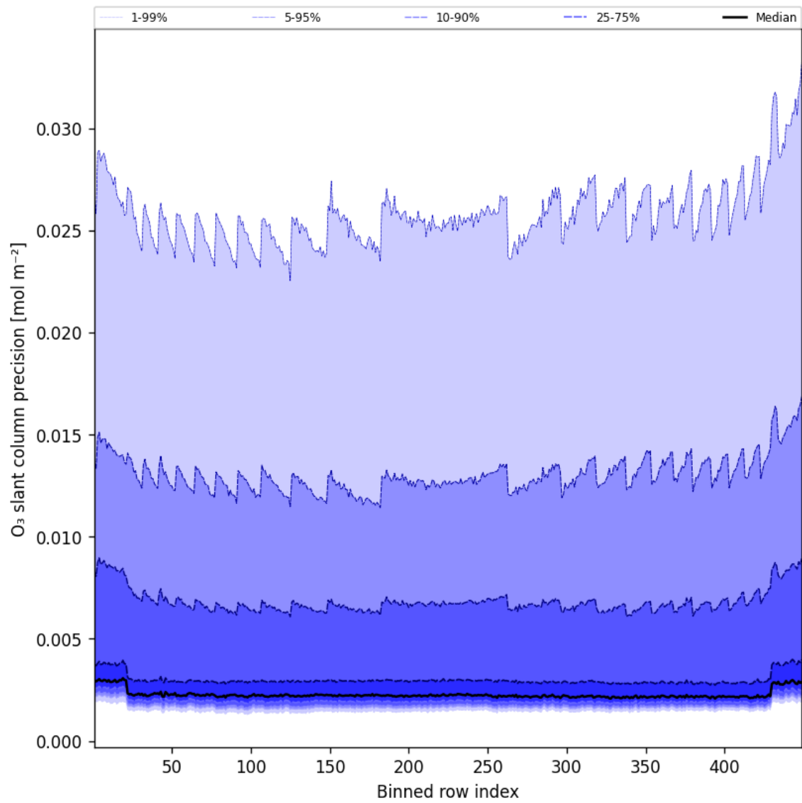
Figure 44: Along track statistics of “O 3 slant column precision” for 2024-12-14 to 2024-12-14
