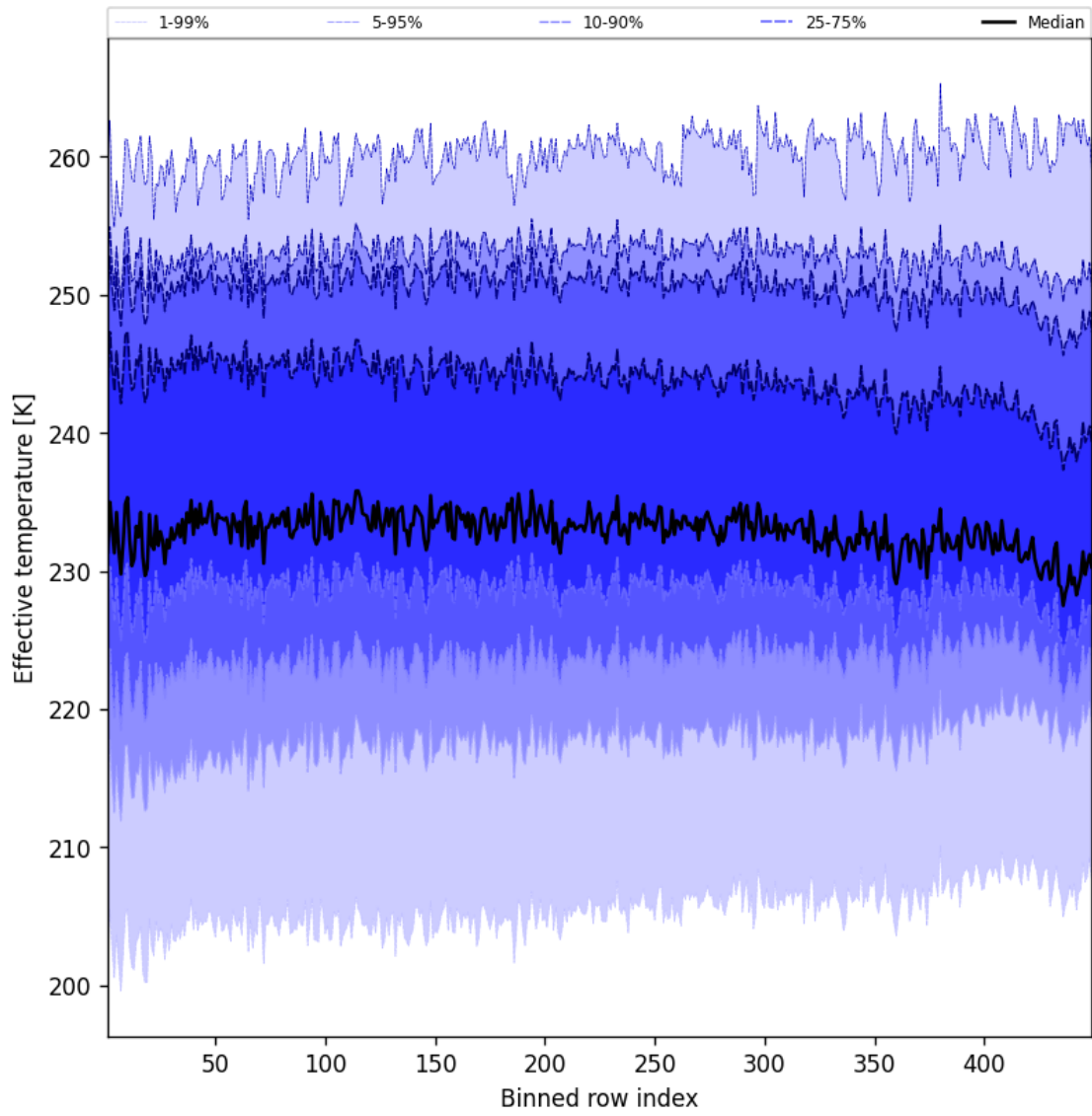
Figure 50: Along track statistics of “Effective temperature” for 2024-12-14 to 2024-12-14
