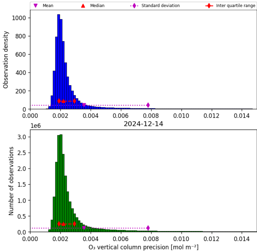
Figure 30: Histogram of “O 3 vertical column precision” for 2024-12-14 to 2024-12-14
