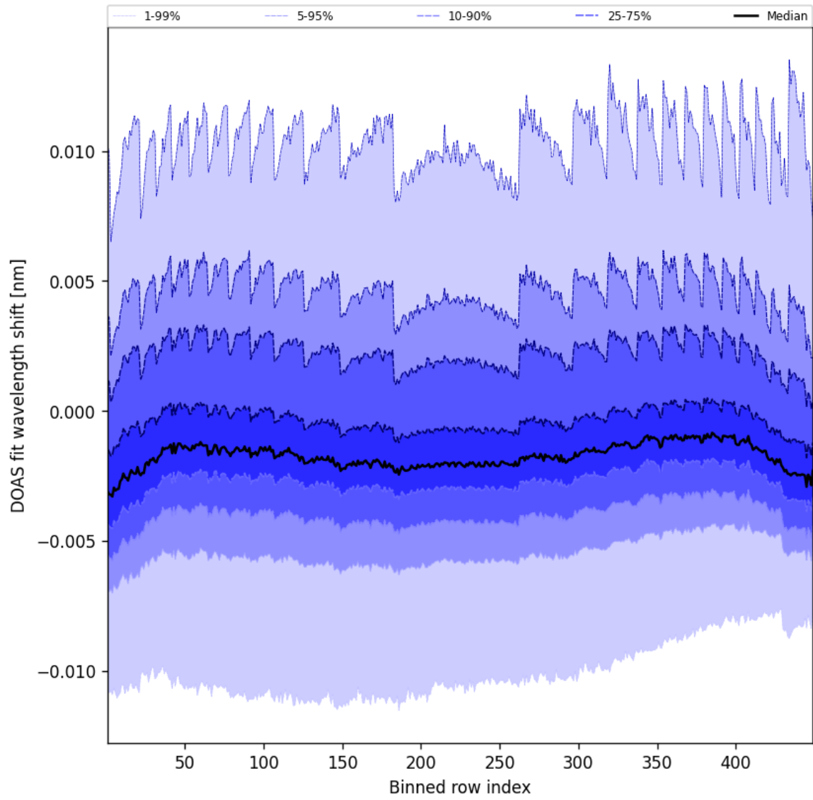
Figure 47: Along track statistics of "DOAS fit wavelength shift" for 2024-12-14 to 2024-12-14
