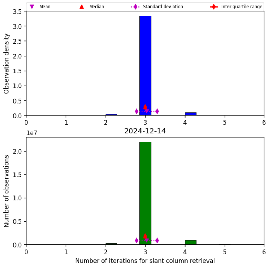
Figure 33: Histogram of "Number of iterations for slant column retrieval" for 2024-12-14 to 2024-12-14
