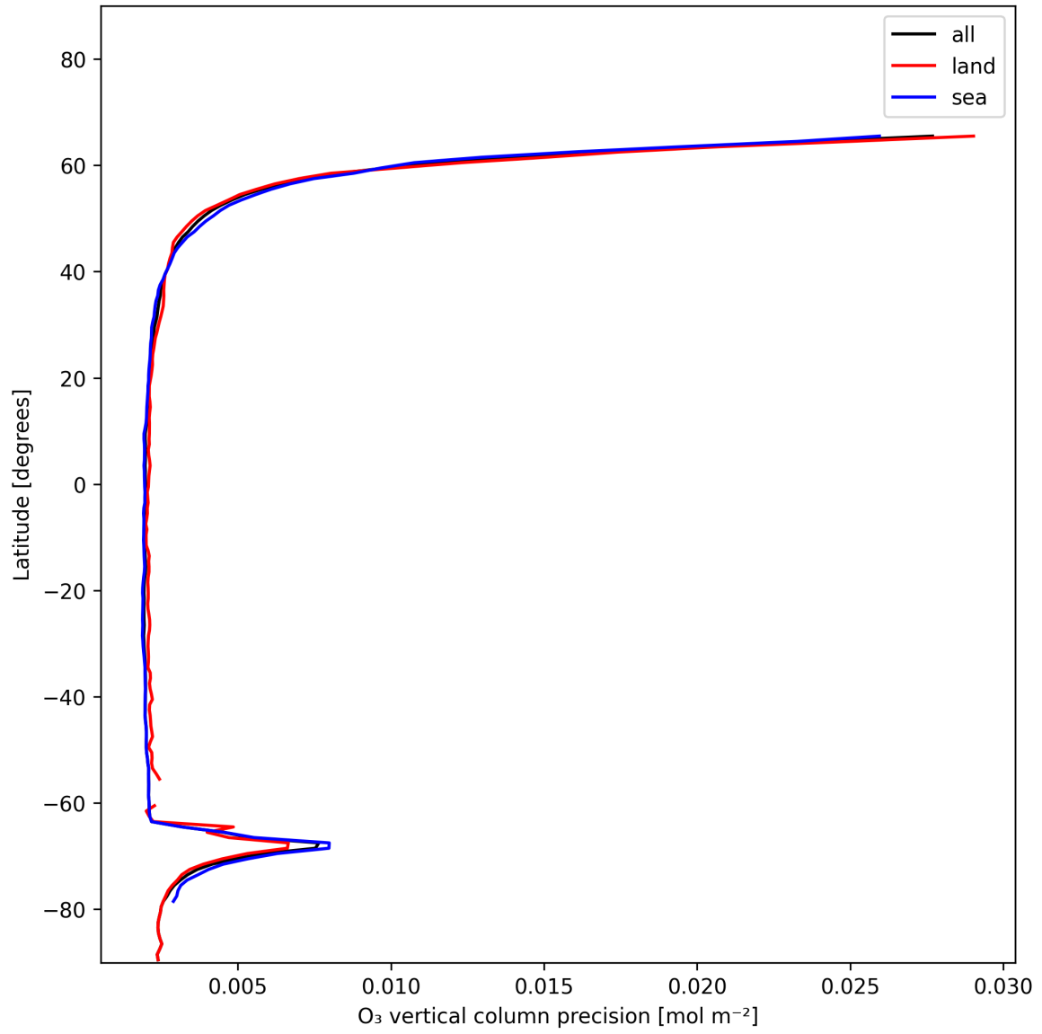
Figure 18: Zonal average of “O 3 vertical column precision” for 2024-12-14 to 2024-12-14.
