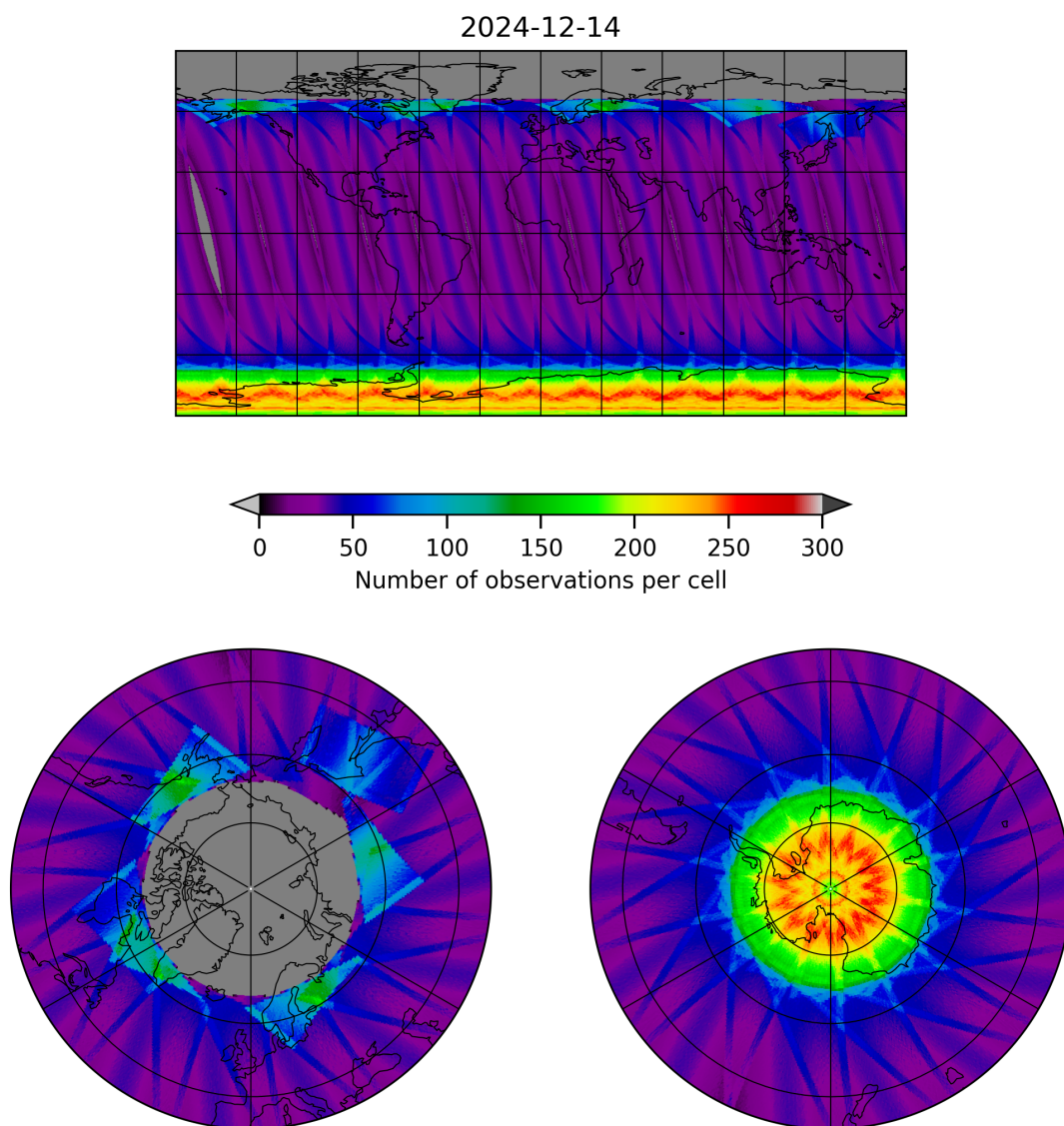
Figure 15: Map of the number of observations for 2024-12-14 to 2024-12-14
