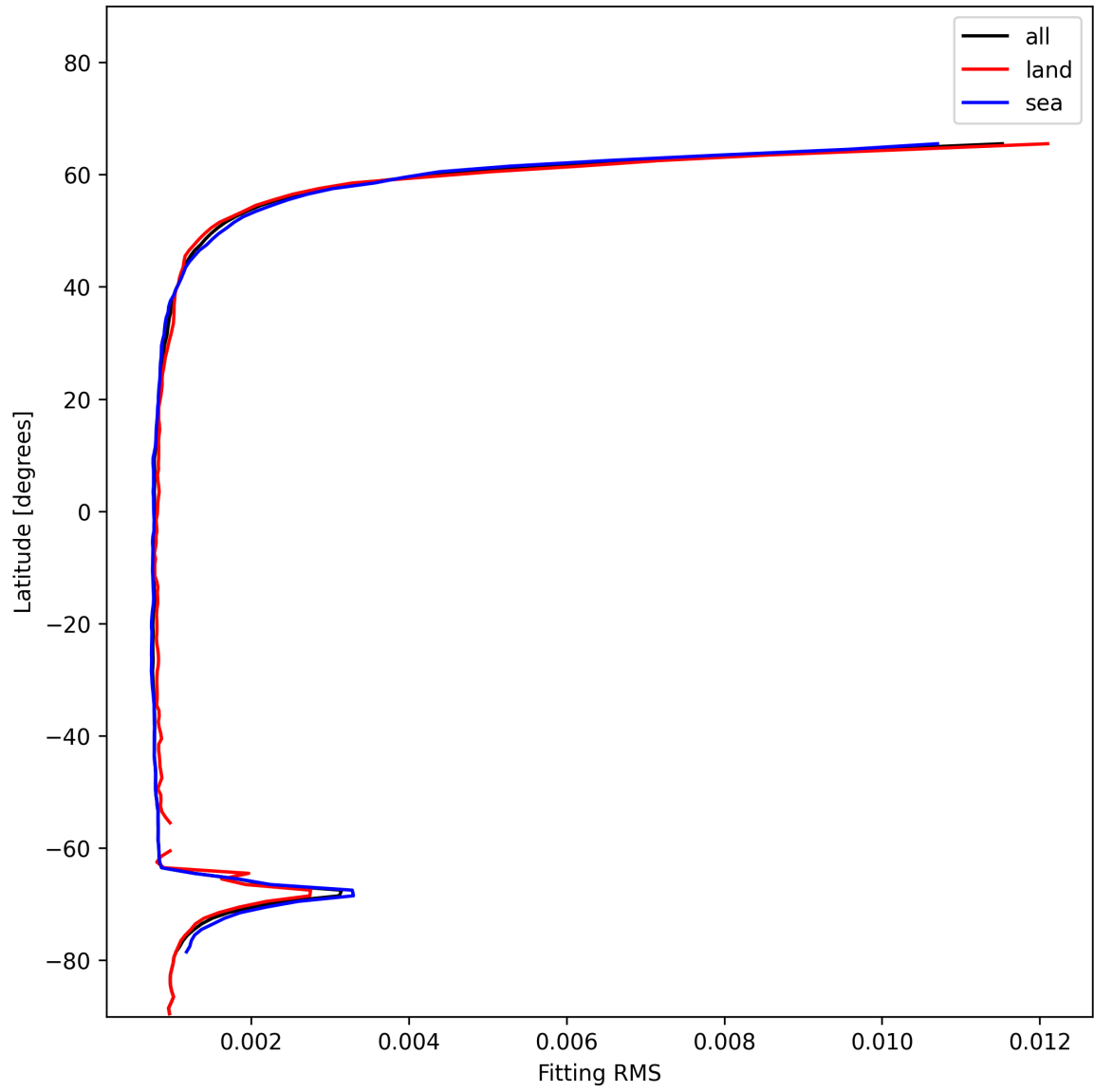
Figure 22: Zonal average of “Fitting RMS” for 2024-12-14 to 2024-12-14.
