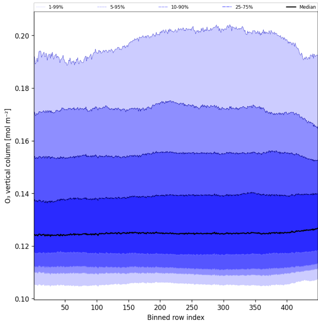
Figure 41: Along track statistics of “O 3 vertical column” for 2024-12-14 to 2024-12-14
