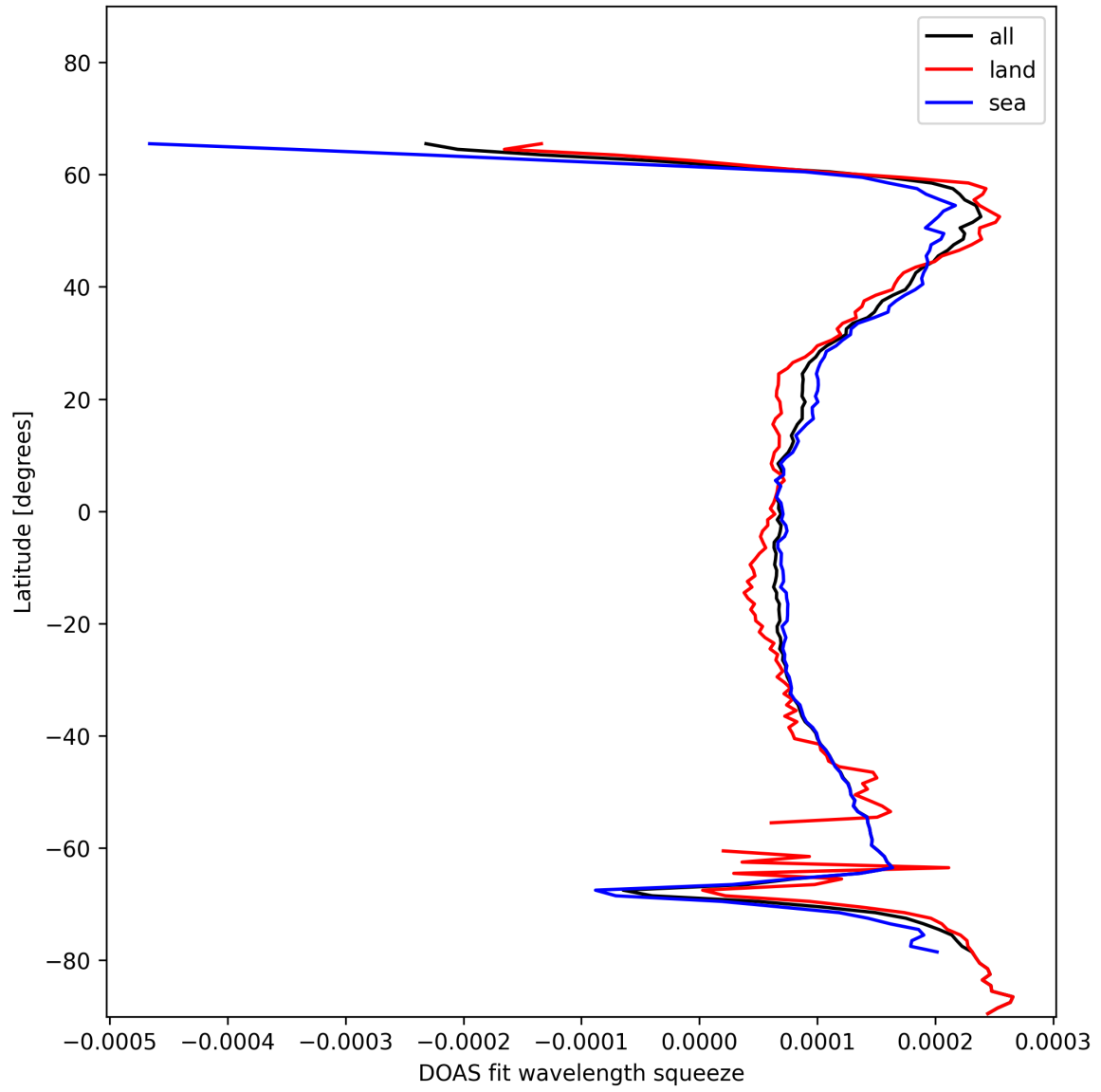
Figure 24: Zonal average of “DOAS fit wavelength squeeze” for 2024-12-14 to 2024-12-14.
