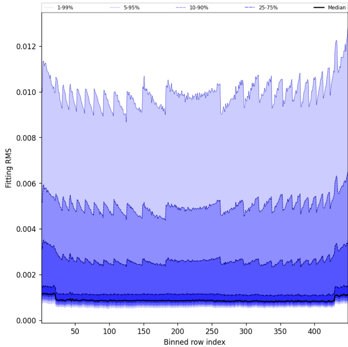
Figure 46: Along track statistics of “Fitting RMS” for 2024-12-14 to 2024-12-14
