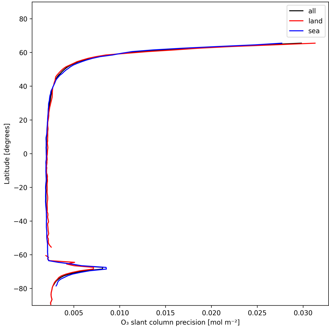
Figure 20: Zonal average of “O 3 slant column precision” for 2024-12-14 to 2024-12-14.
