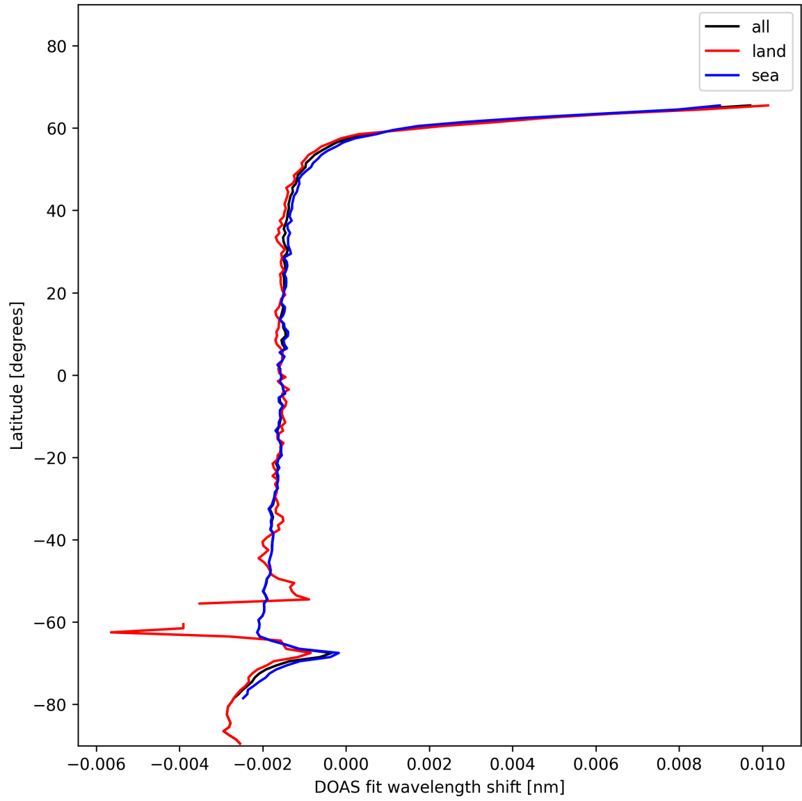
Figure 23: Zonal average of “DOAS fit wavelength shift” for 2024-12-14 to 2024-12-14.
