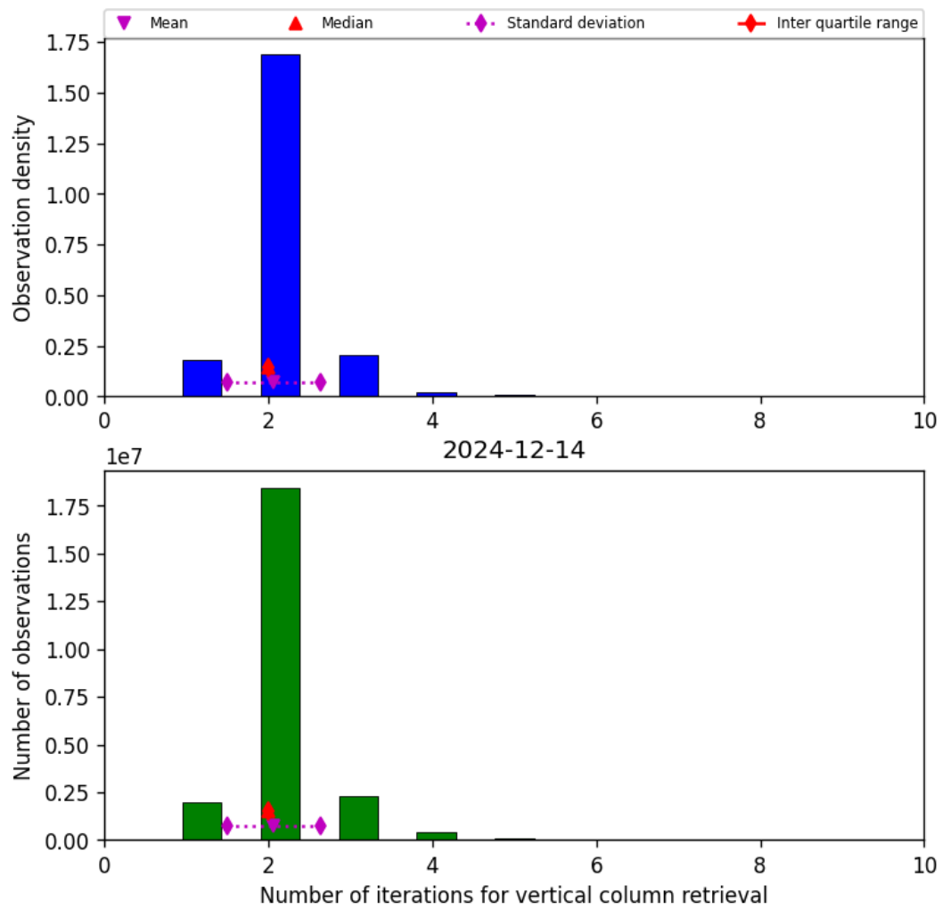
Figure 39: Histogram of “Number of iterations for vertical column retrieval” for 2024-12-14 to 2024-12-14
