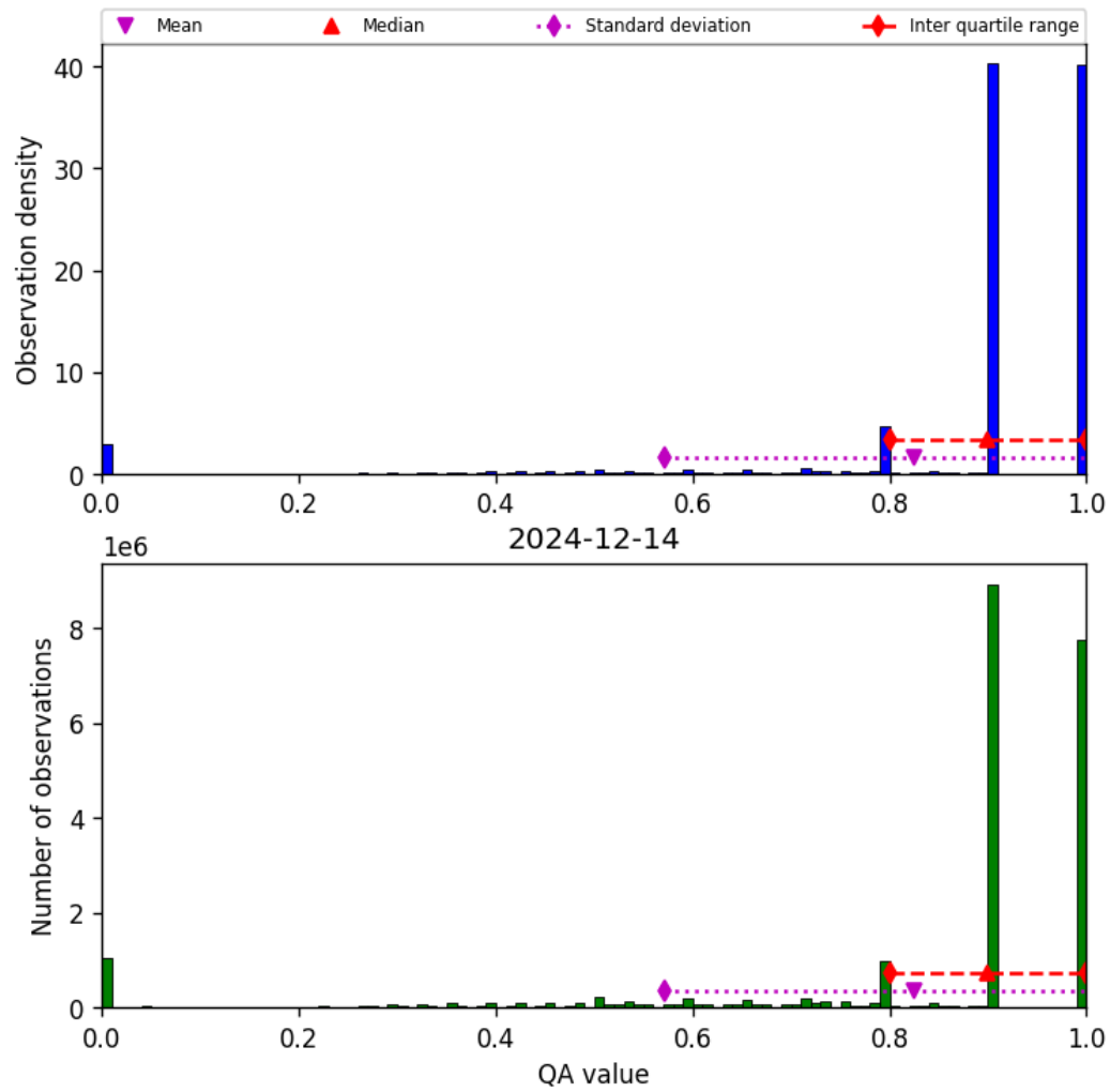
Figure 28: Histogram of “QA value” for 2024-12-14 to 2024-12-14
