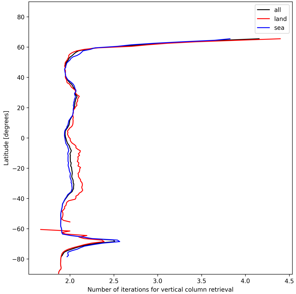
Figure 27: Zonal average of “Number of iterations for vertical column retrieval” for 2024-12-14 to 2024-12-14.
