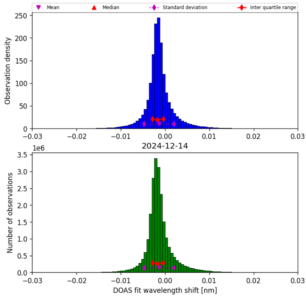
Figure 35: Histogram of “DOAS fit wavelength shift” for 2024-12-14 to 2024-12-14
