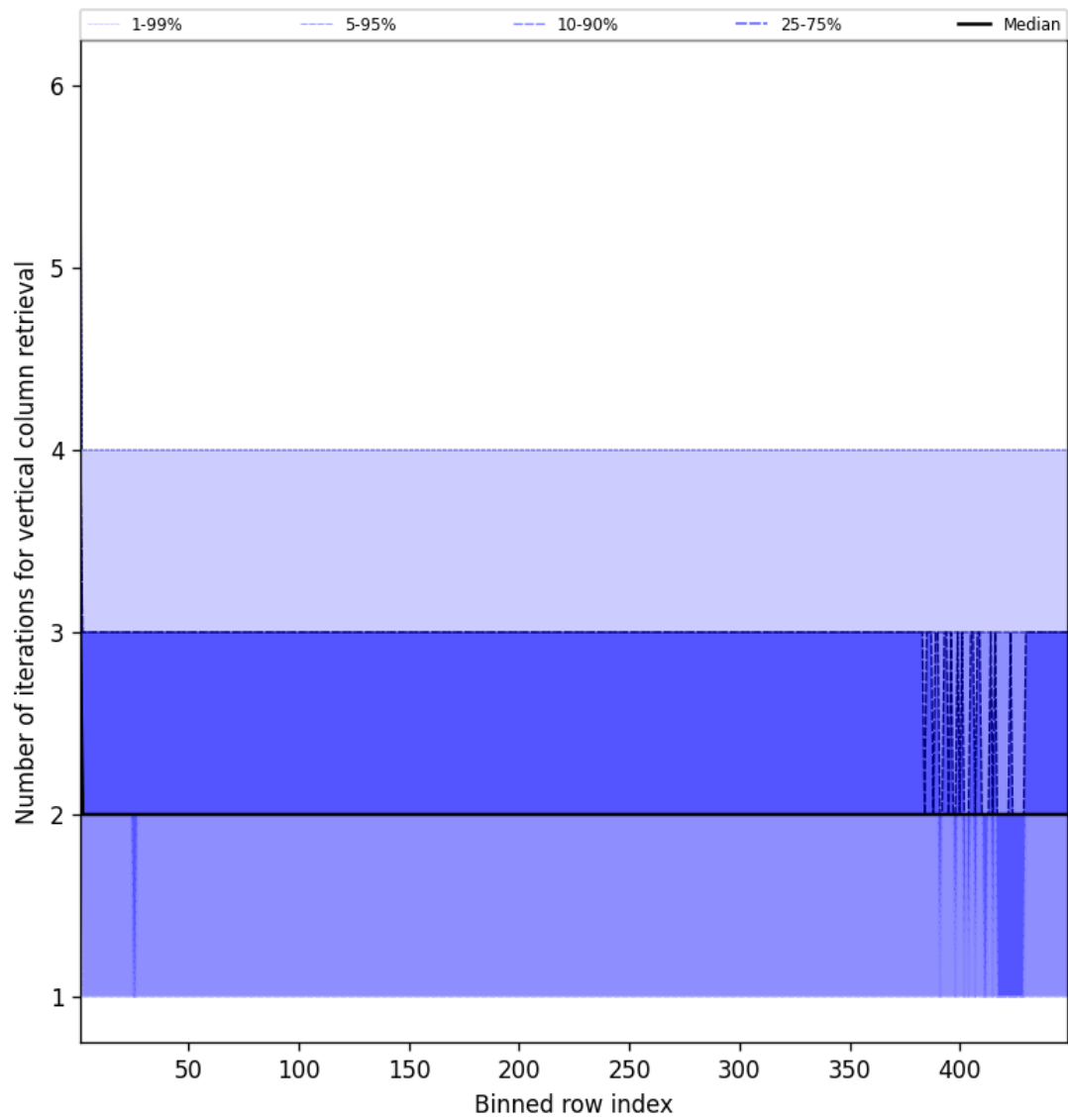
Figure 51: Along track statistics of “Number of iterations for vertical column retrieval” for 2024-12-14 to 2024-12-14
