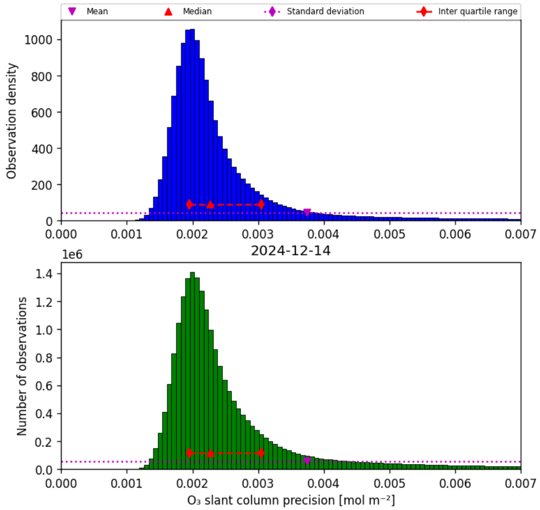
Figure 32: Histogram of “O 3 slant column precision” for 2024-12-14 to 2024-12-14
