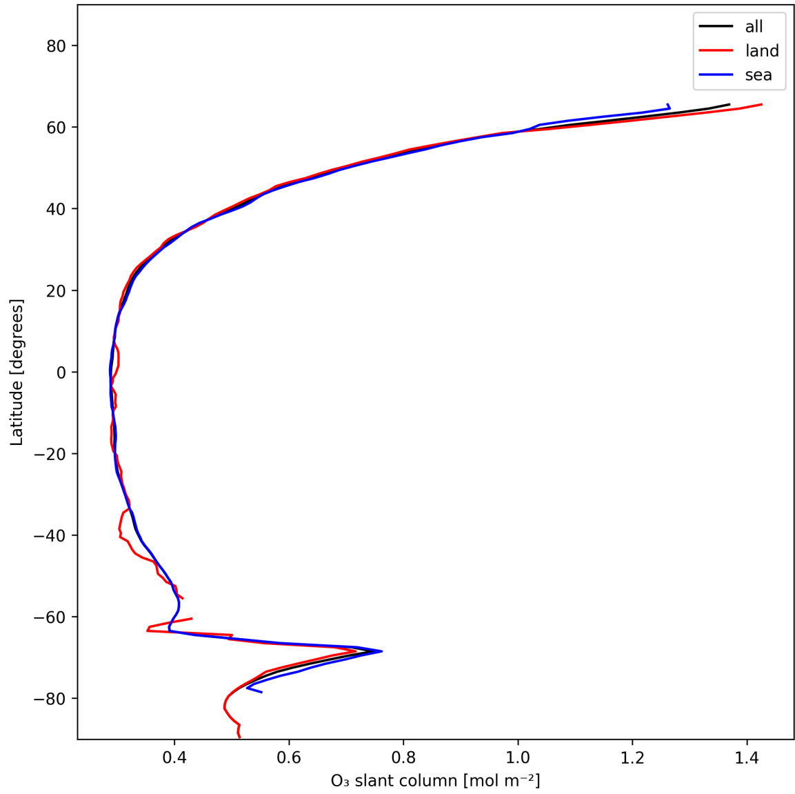
Figure 19: Zonal average of “O 3 slant column” for 2024-12-14 to 2024-12-14.
