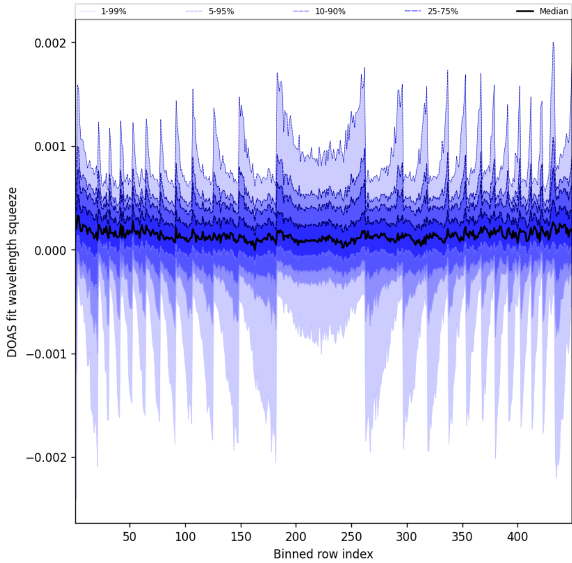
Figure 48: Along track statistics of “DOAS fit wavelength squeeze” for 2024-12-14 to 2024-12-14
