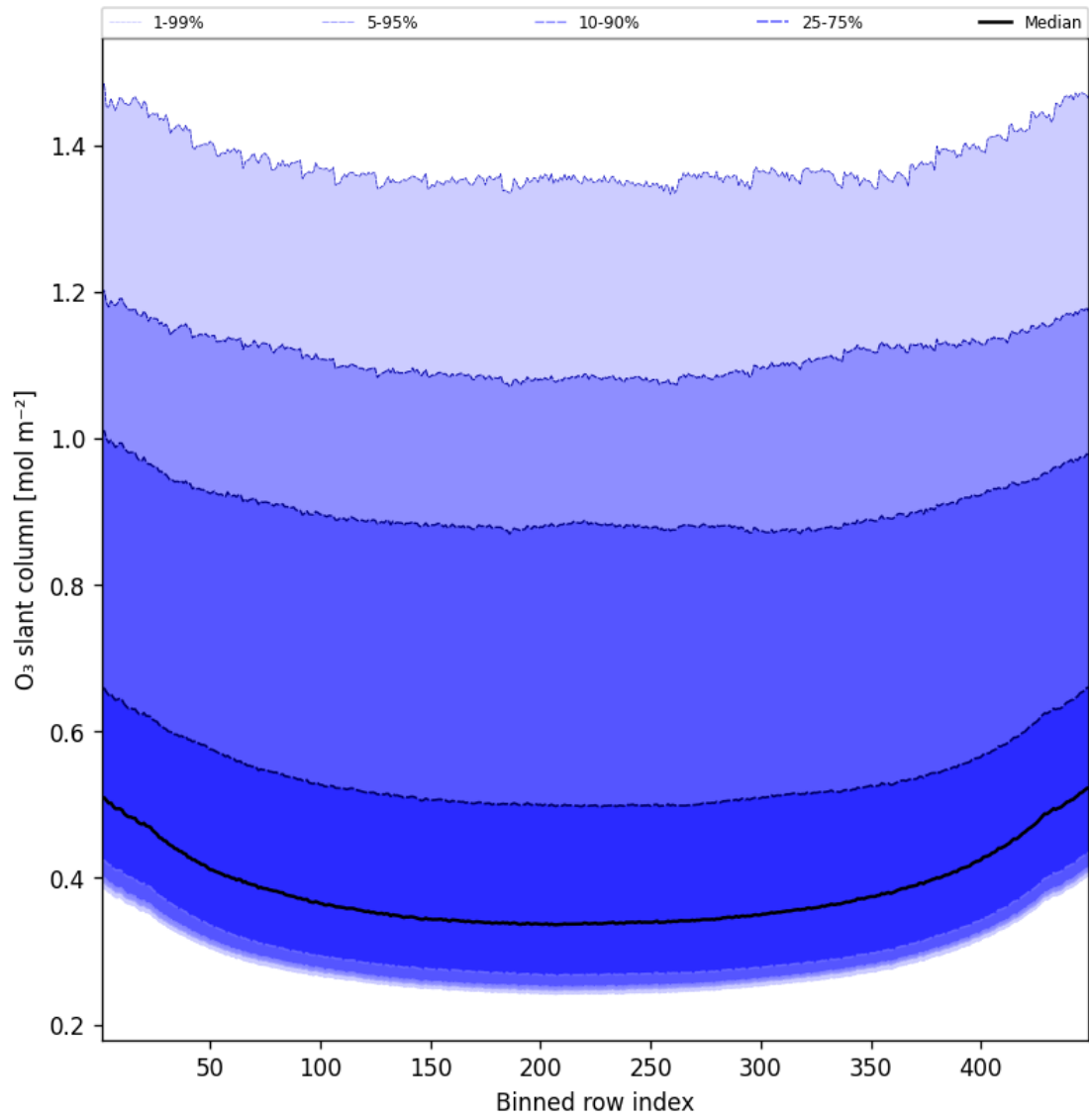
Figure 43: Along track statistics of “O 3 slant column” for 2024-12-14 to 2024-12-14
