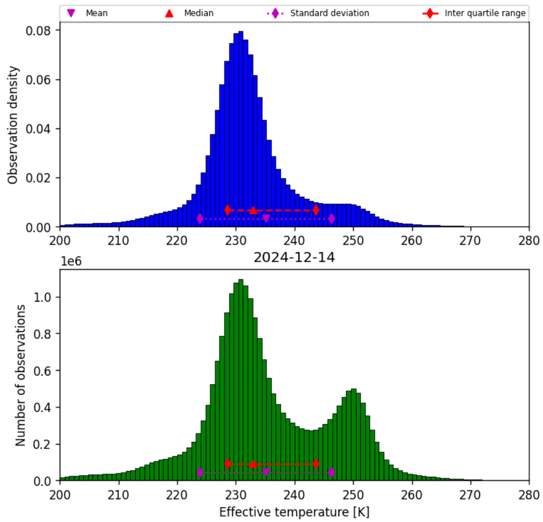
Figure 38: Histogram of “Effective temperature” for 2024-12-14 to 2024-12-14
