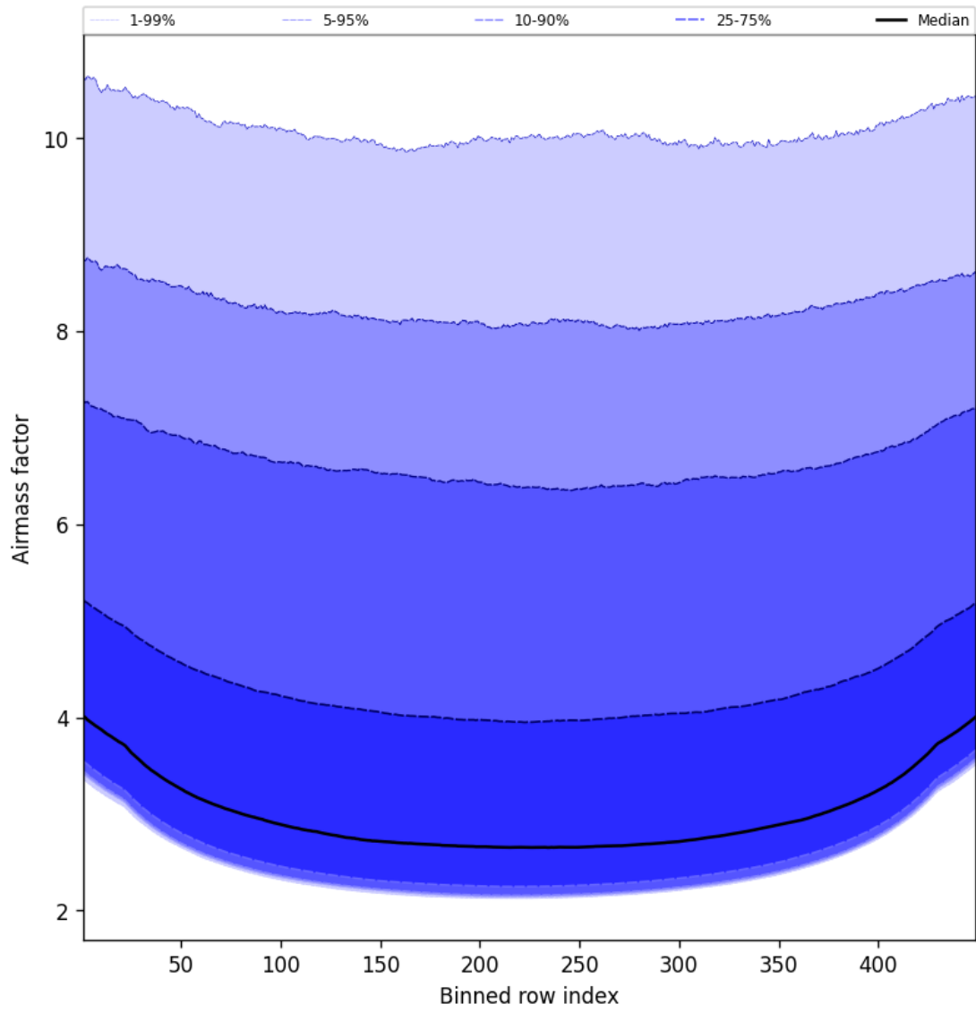
Figure 49: Along track statistics of “Airmass factor” for 2024-12-14 to 2024-12-14
