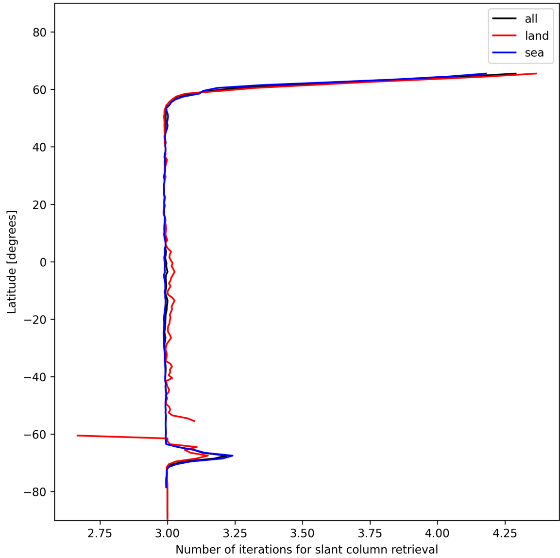
Figure 21: Zonal average of “Number of iterations for slant column retrieval” for 2024-12-14 to 2024-12-14.
