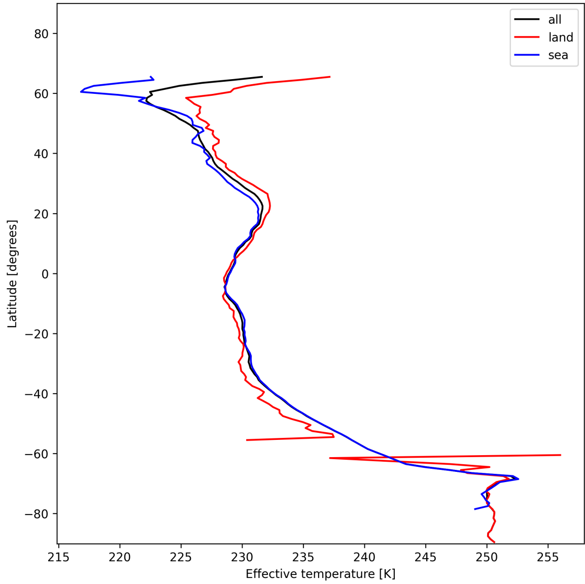
Figure 26: Zonal average of “Effective temperature” for 2024-12-14 to 2024-12-14.
