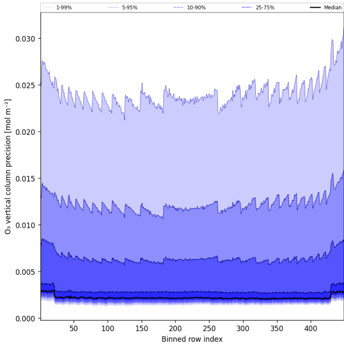
Figure 42: Along track statistics of “O 3 vertical column precision” for 2024-12-14 to 2024-12-14
