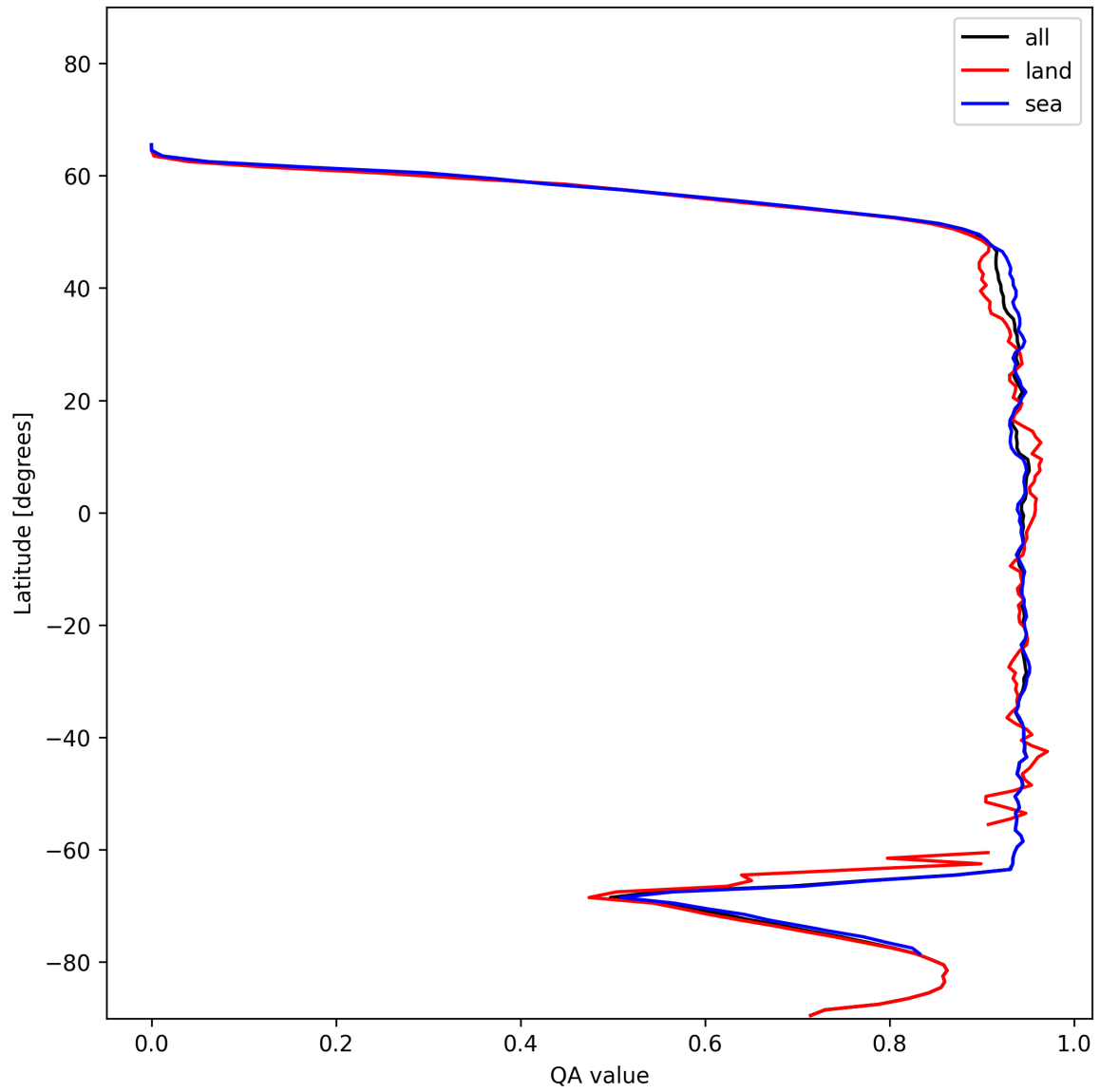
Figure 16: Zonal average of “QA value” for 2024-12-14 to 2024-12-14.
