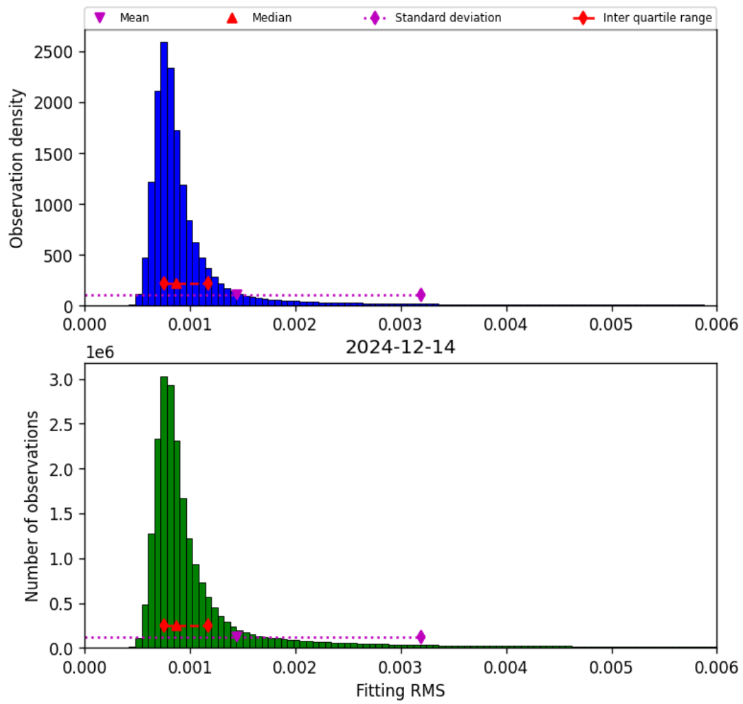
Figure 34: Histogram of “Fitting RMS” for 2024-12-14 to 2024-12-14
