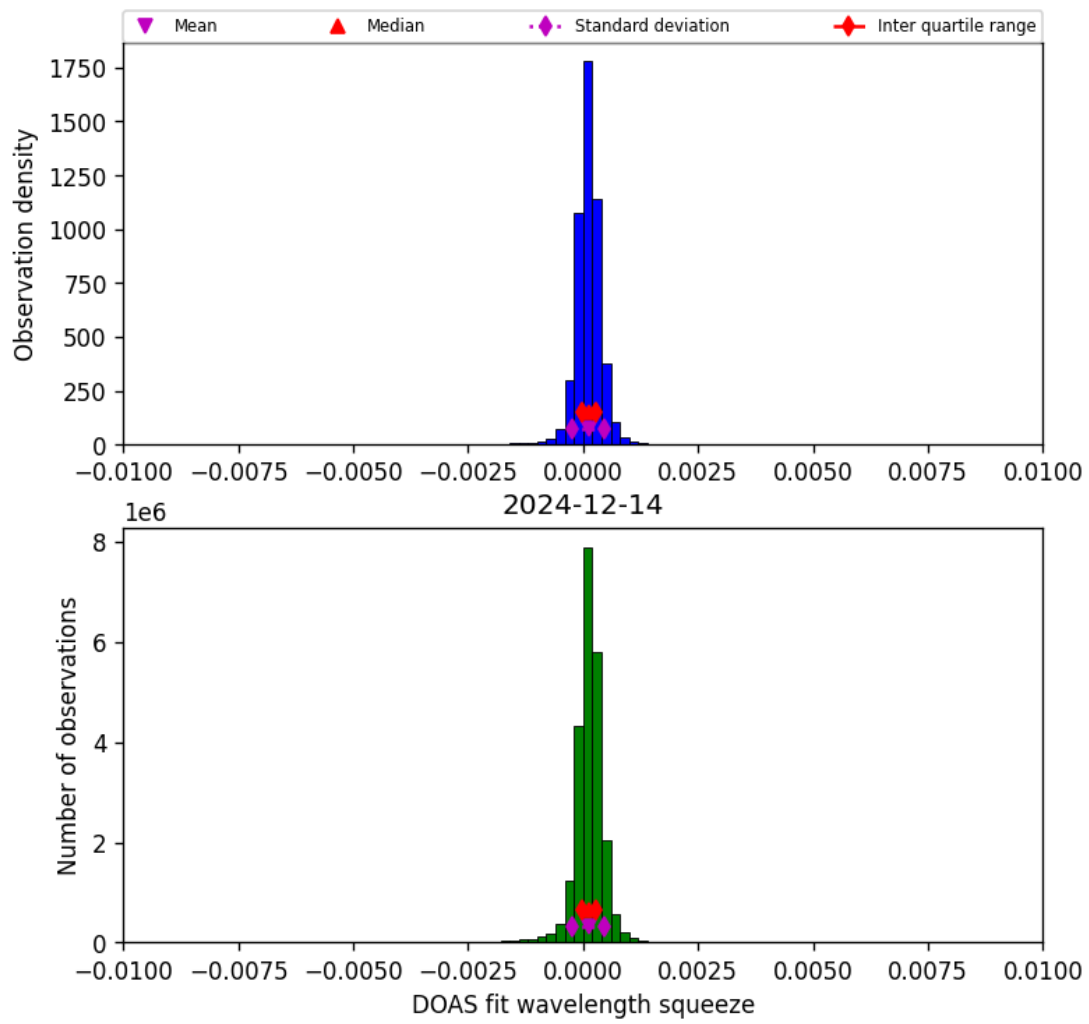
Figure 36: Histogram of “DOAS fit wavelength squeeze” for 2024-12-14 to 2024-12-14
