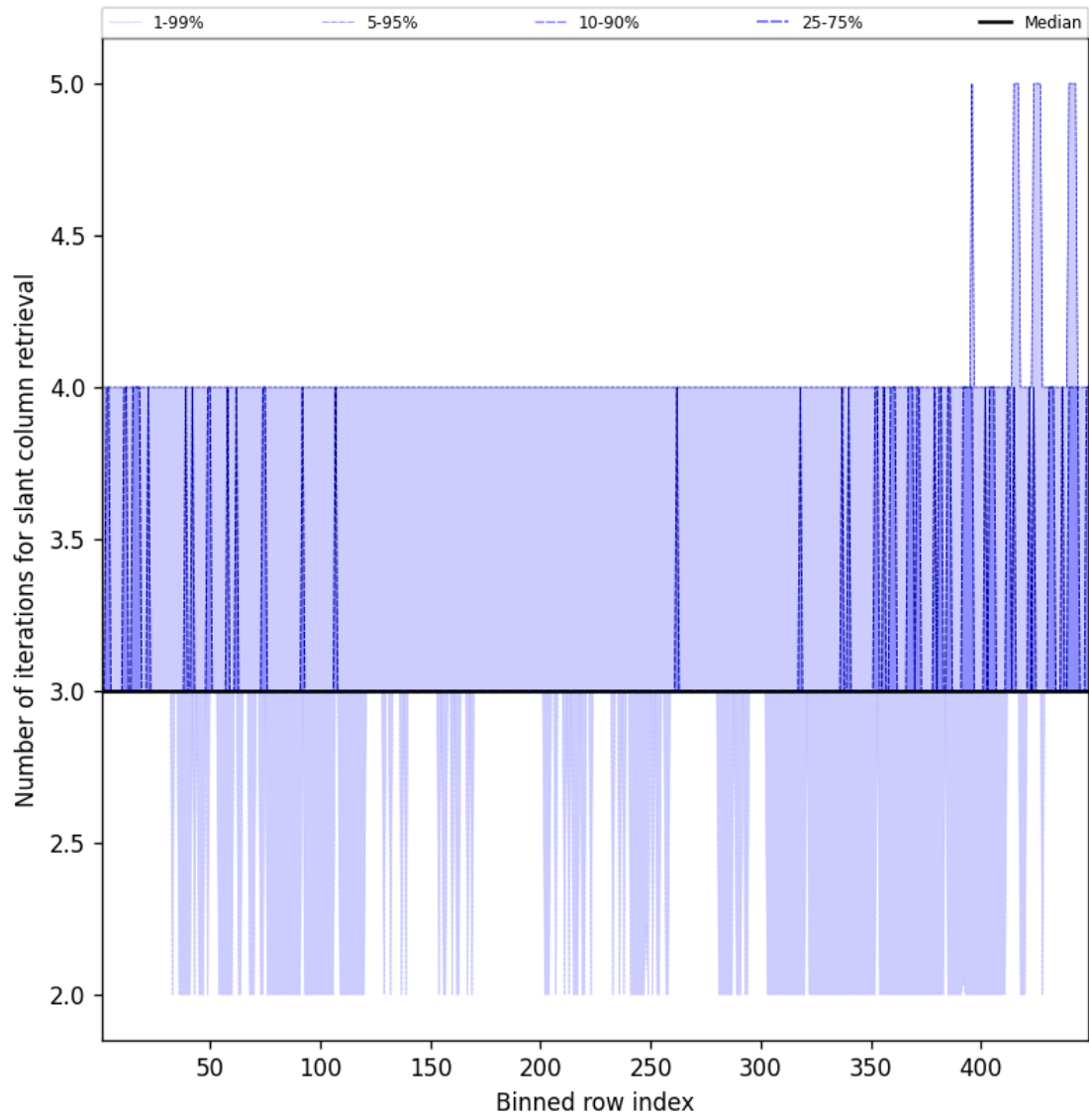
Figure 45: Along track statistics of “Number of iterations for slant column retrieval” for 2024-12-14 to 2024-12-14
