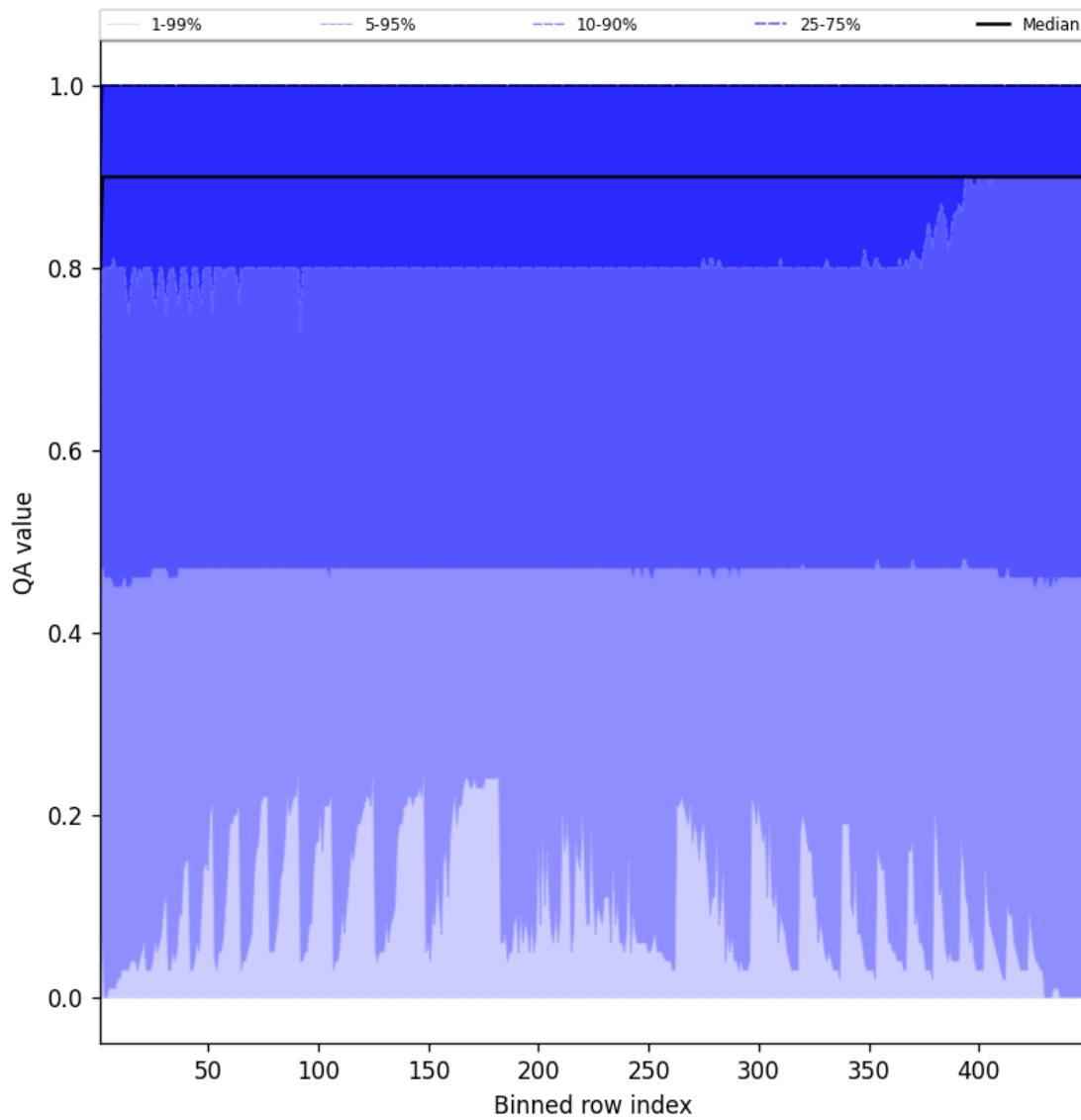
Figure 40: Along track statistics of “QA value” for 2024-12-14 to 2024-12-14
