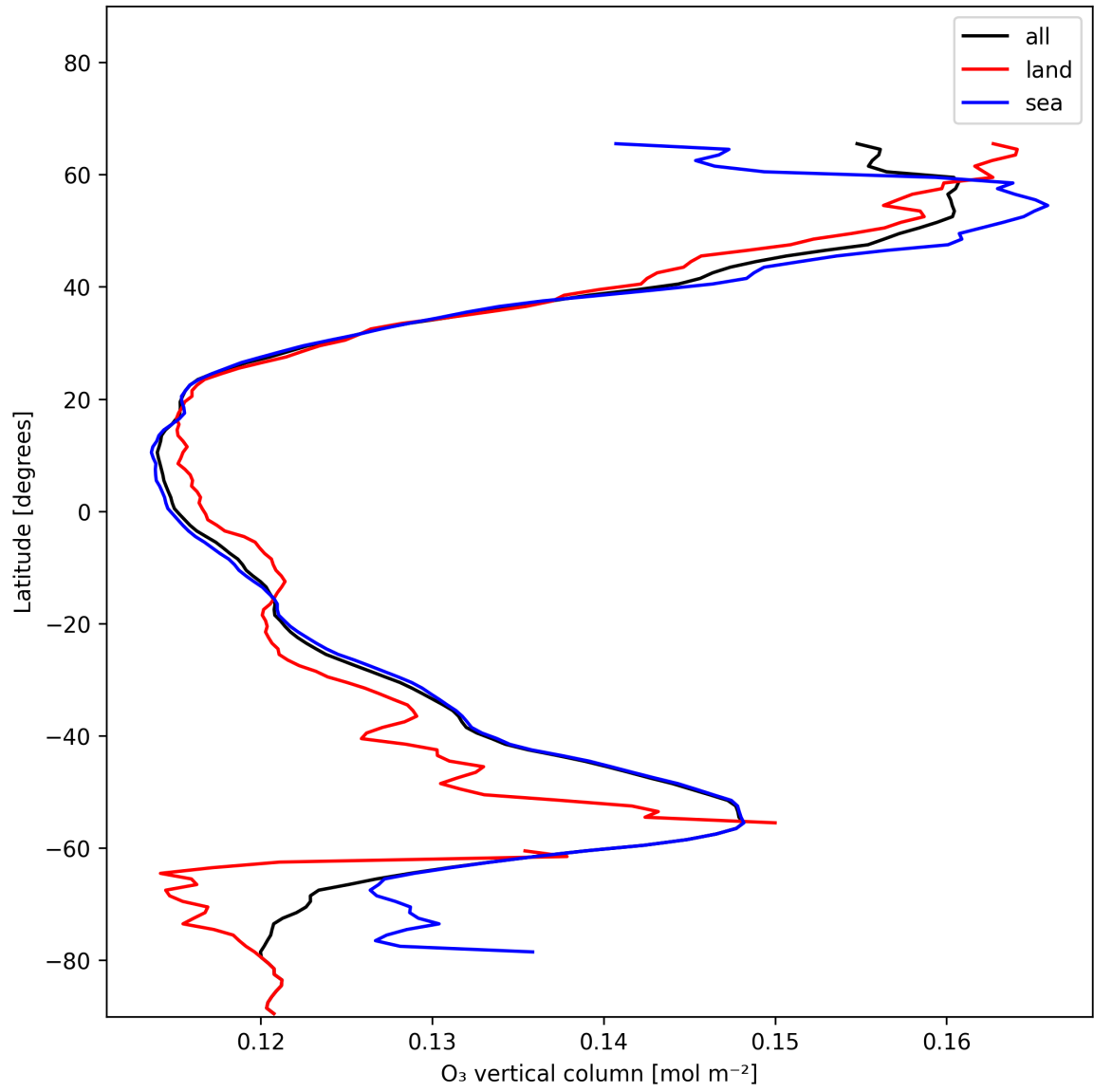
Figure 17: Zonal average of “O 3 vertical column” for 2024-12-14 to 2024-12-14.
