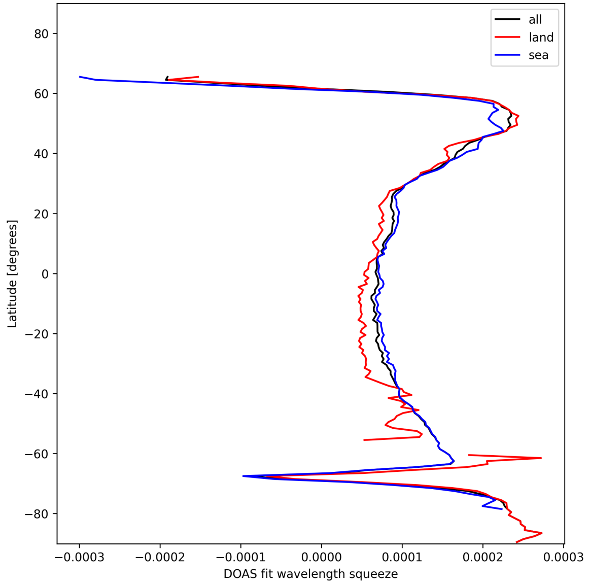
Figure 24: Zonal average of “DOAS fit wavelength squeeze” for 2024-12-16 to 2024-12-17.
