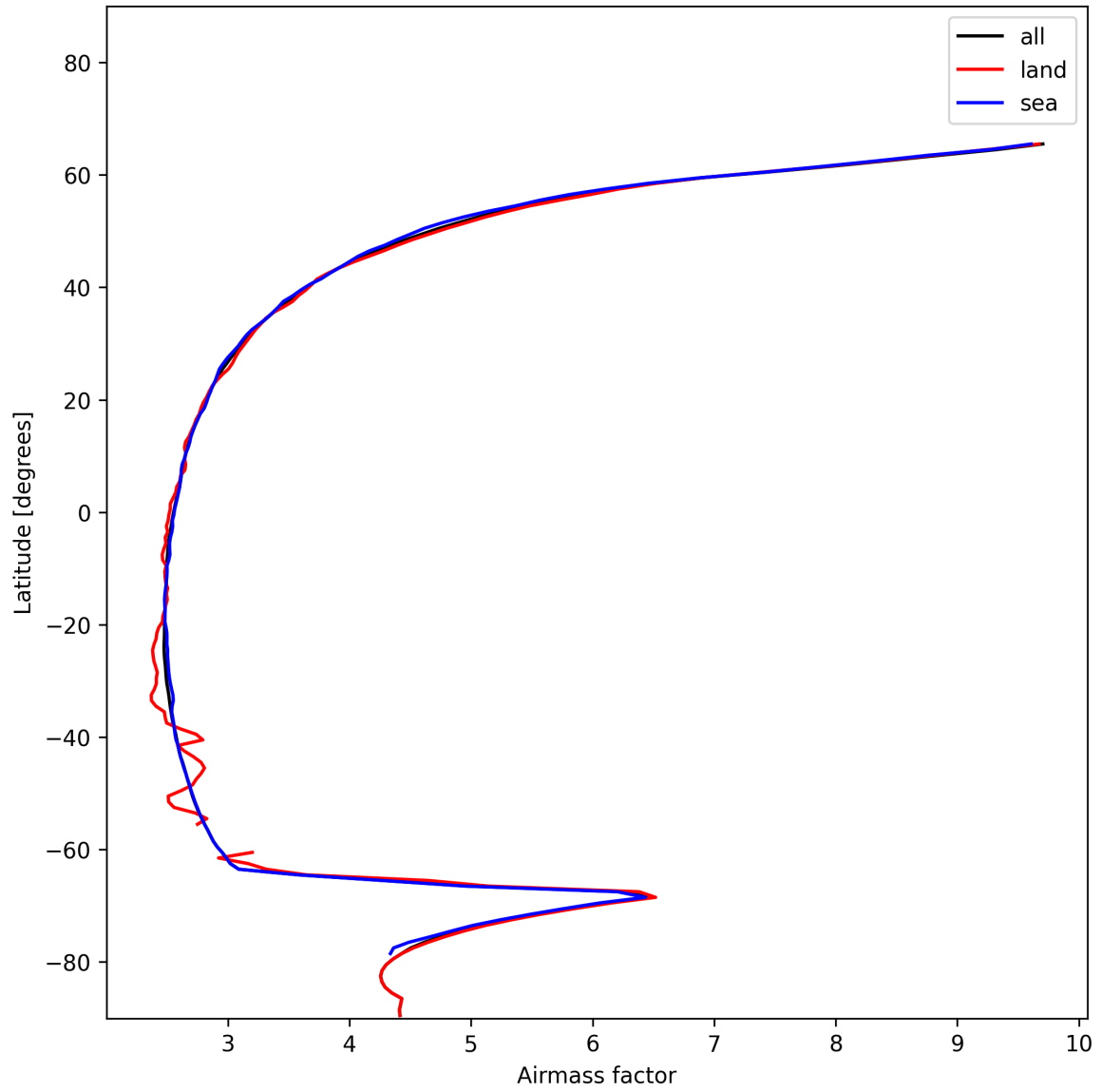
Figure 25: Zonal average of “Airmass factor” for 2024-12-16 to 2024-12-17.
