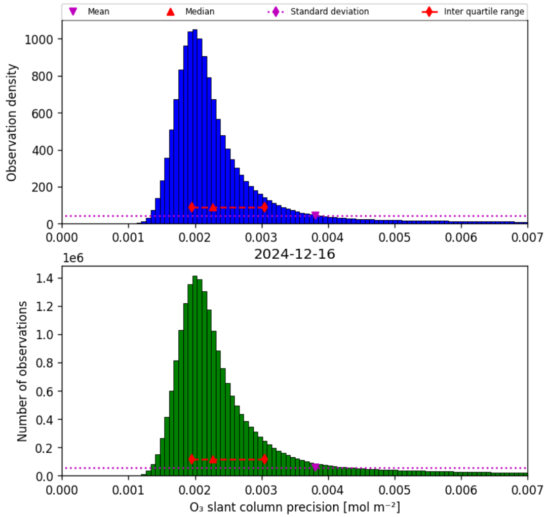
Figure 32: Histogram of “O 3 slant column precision” for 2024-12-16 to 2024-12-17
