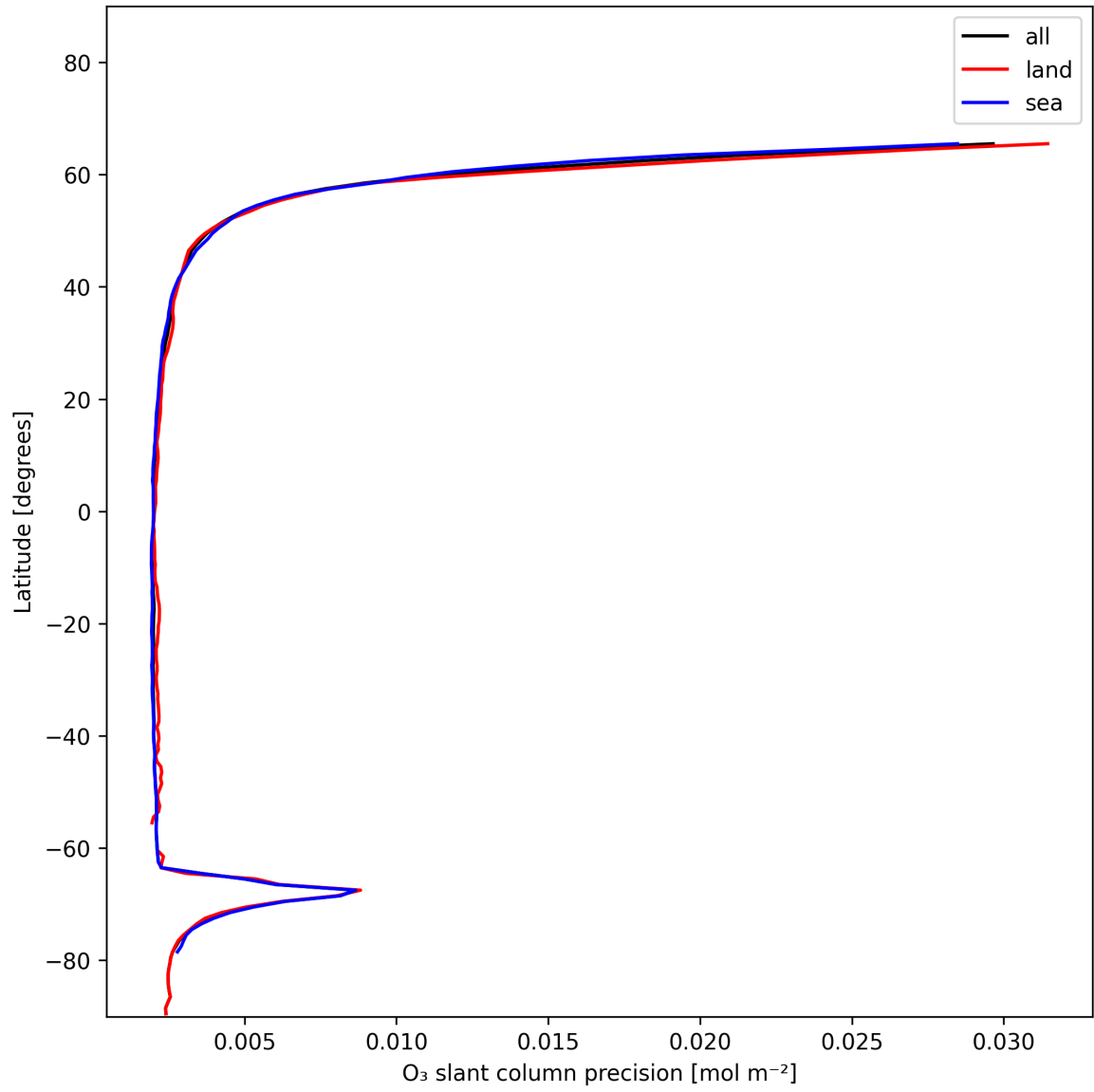
Figure 20: Zonal average of “O 3 slant column precision” for 2024-12-16 to 2024-12-17.
