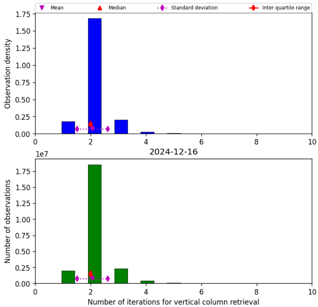
Figure 39: Histogram of “Number of iterations for vertical column retrieval” for 2024-12-16 to 2024-12-17
