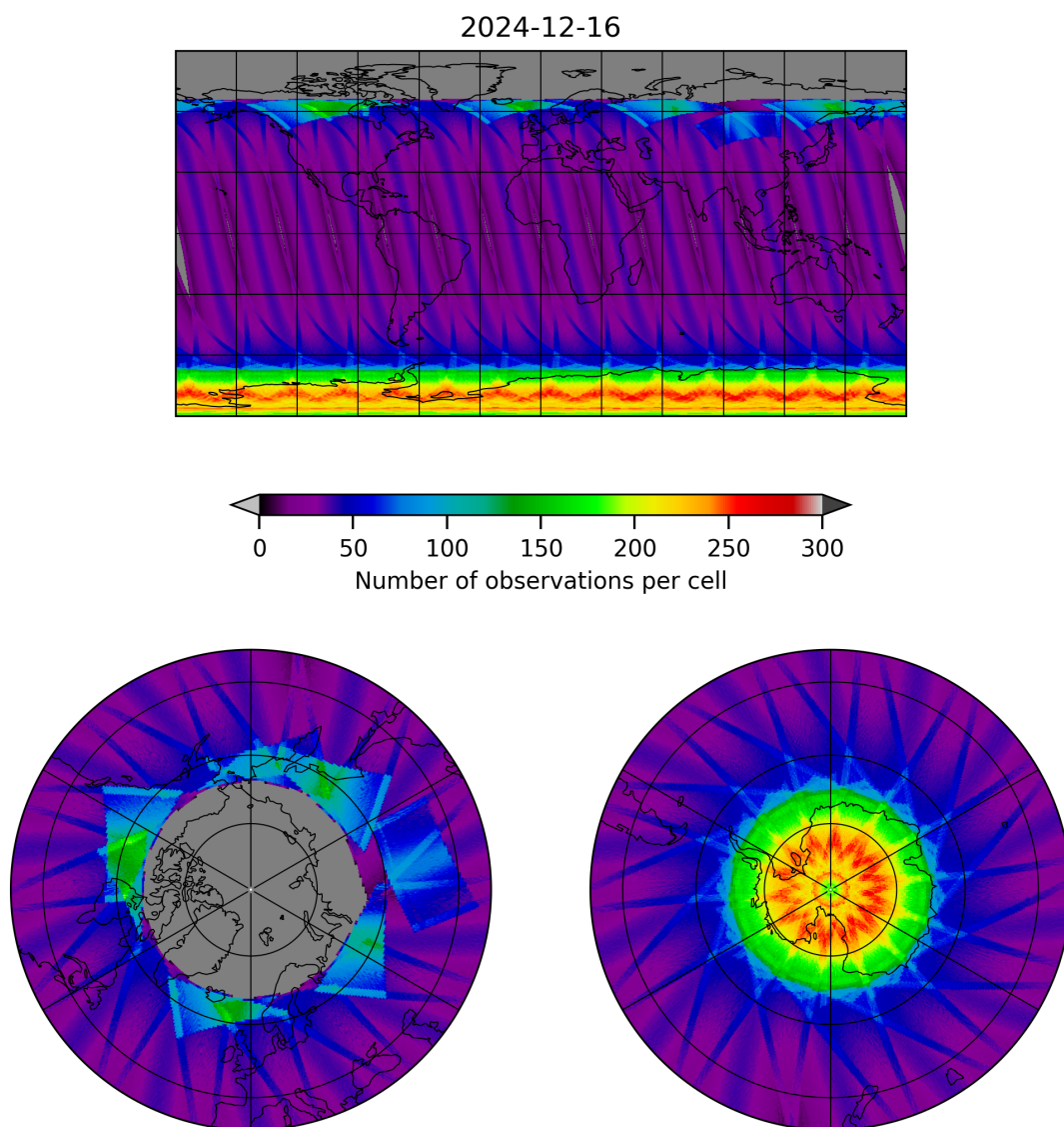
Figure 15: Map of the number of observations for 2024-12-16 to 2024-12-17
