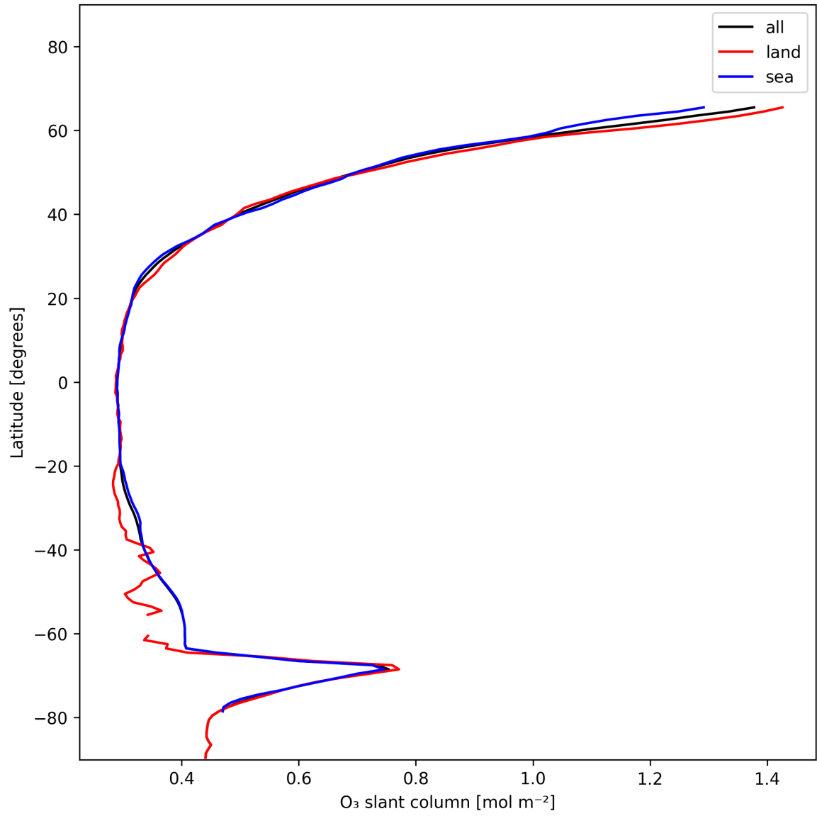
Figure 19: Zonal average of “O 3 slant column” for 2024-12-16 to 2024-12-17.
