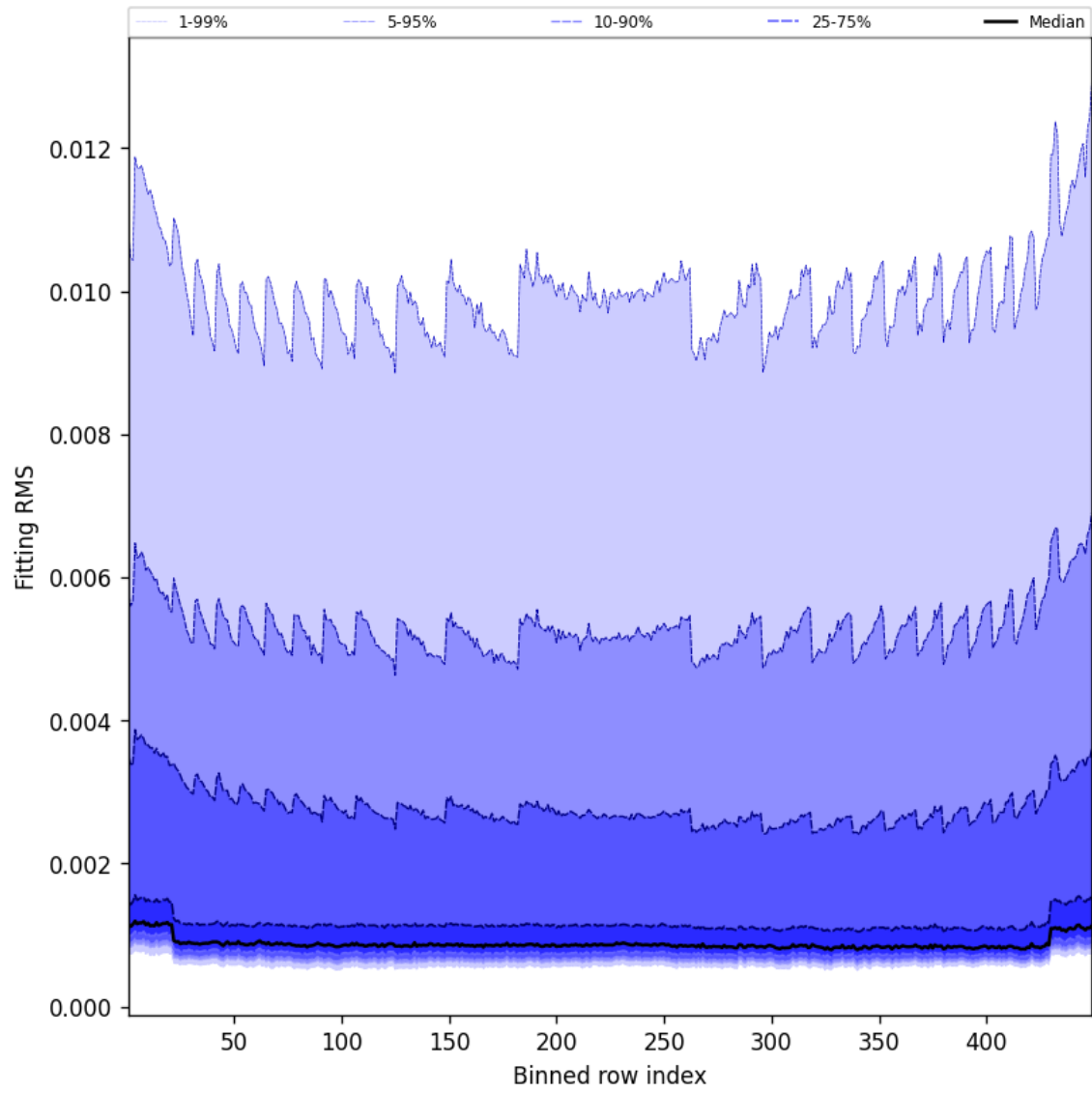
Figure 46: Along track statistics of “Fitting RMS” for 2024-12-16 to 2024-12-17
