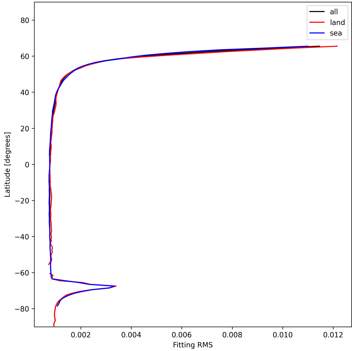
Figure 22: Zonal average of “Fitting RMS” for 2024-12-16 to 2024-12-17.
