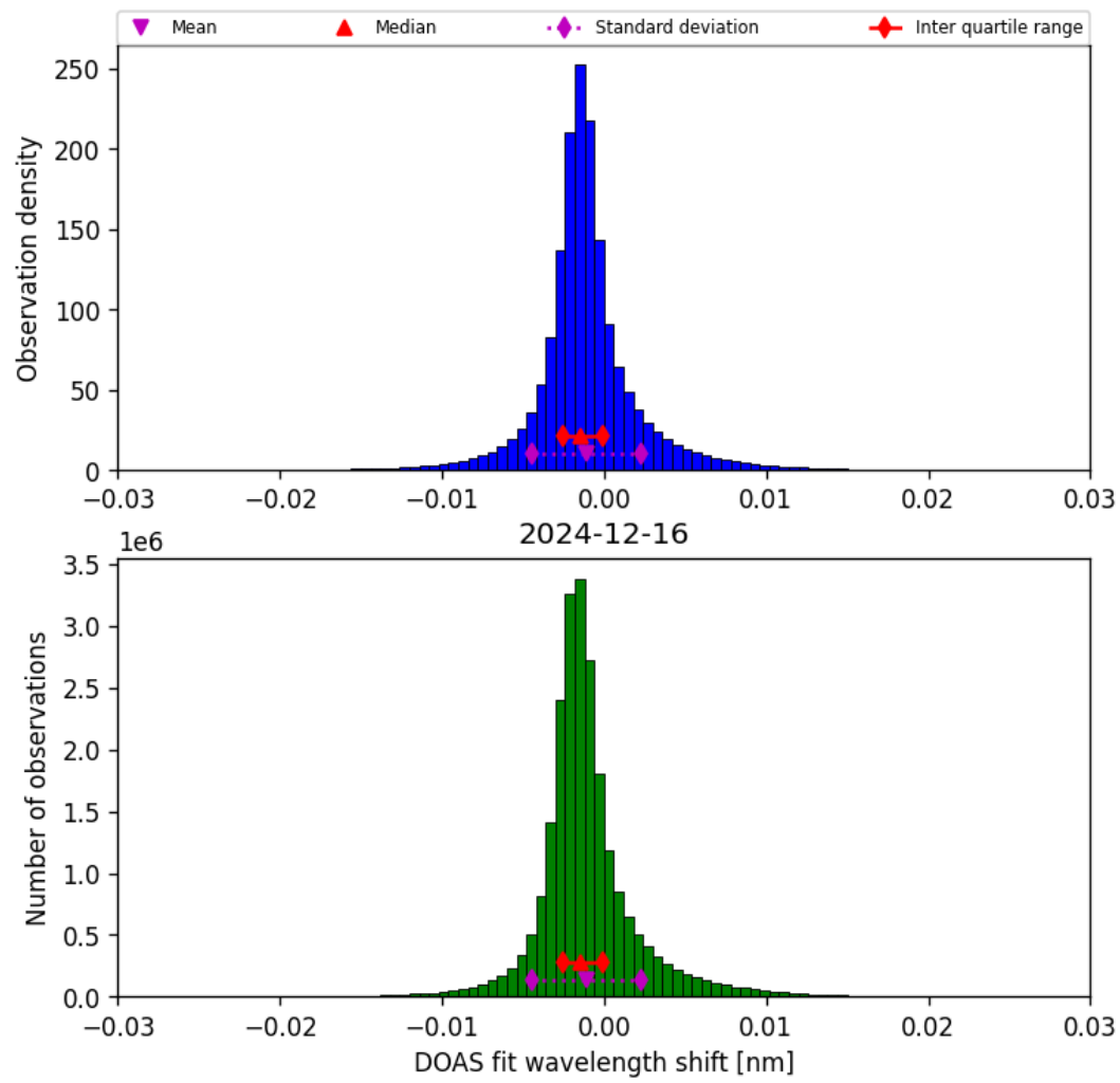
Figure 35: Histogram of “DOAS fit wavelength shift” for 2024-12-16 to 2024-12-17
