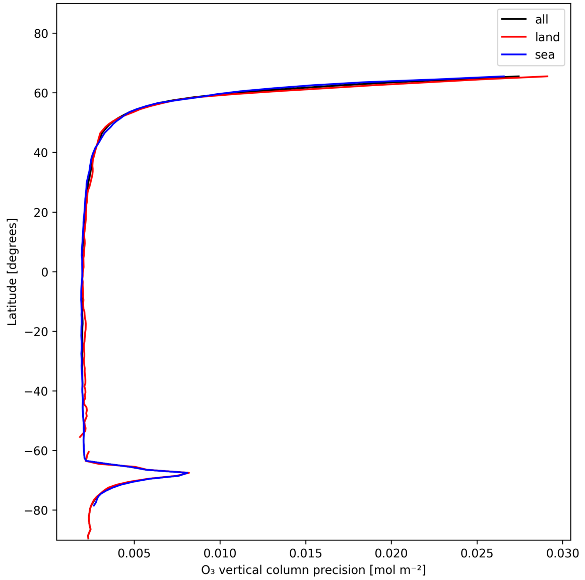
Figure 18: Zonal average of “O 3 vertical column precision” for 2024-12-16 to 2024-12-17.
