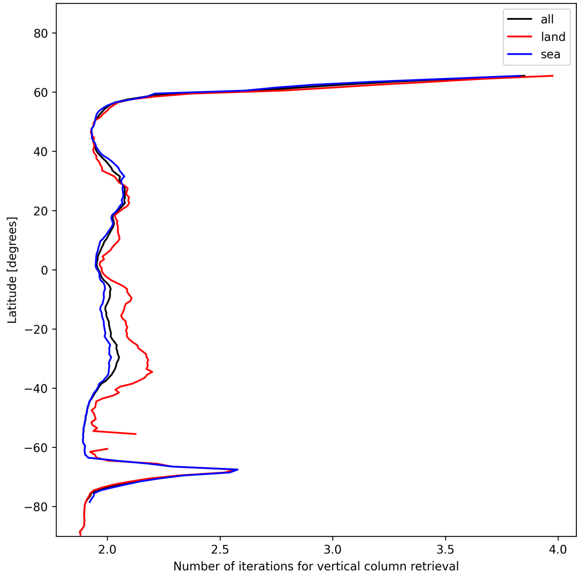
Figure 27: Zonal average of “Number of iterations for vertical column retrieval” for 2024-12-16 to 2024-12-17.
