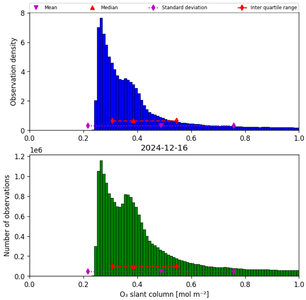
Figure 31: Histogram of “O 3 slant column” for 2024-12-16 to 2024-12-17
