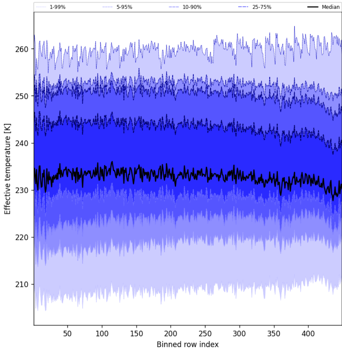
Figure 50: Along track statistics of “Effective temperature” for 2024-12-16 to 2024-12-17
