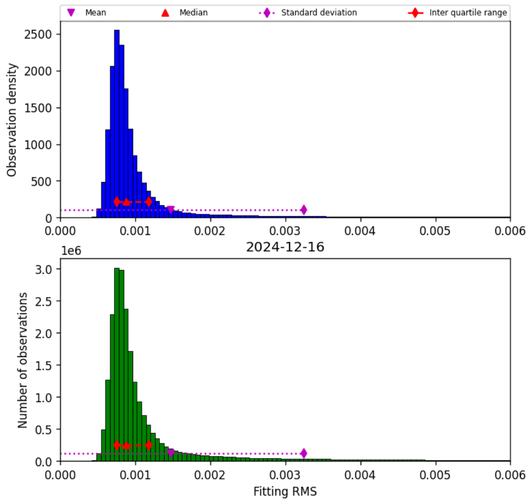
Figure 34: Histogram of “Fitting RMS” for 2024-12-16 to 2024-12-17
