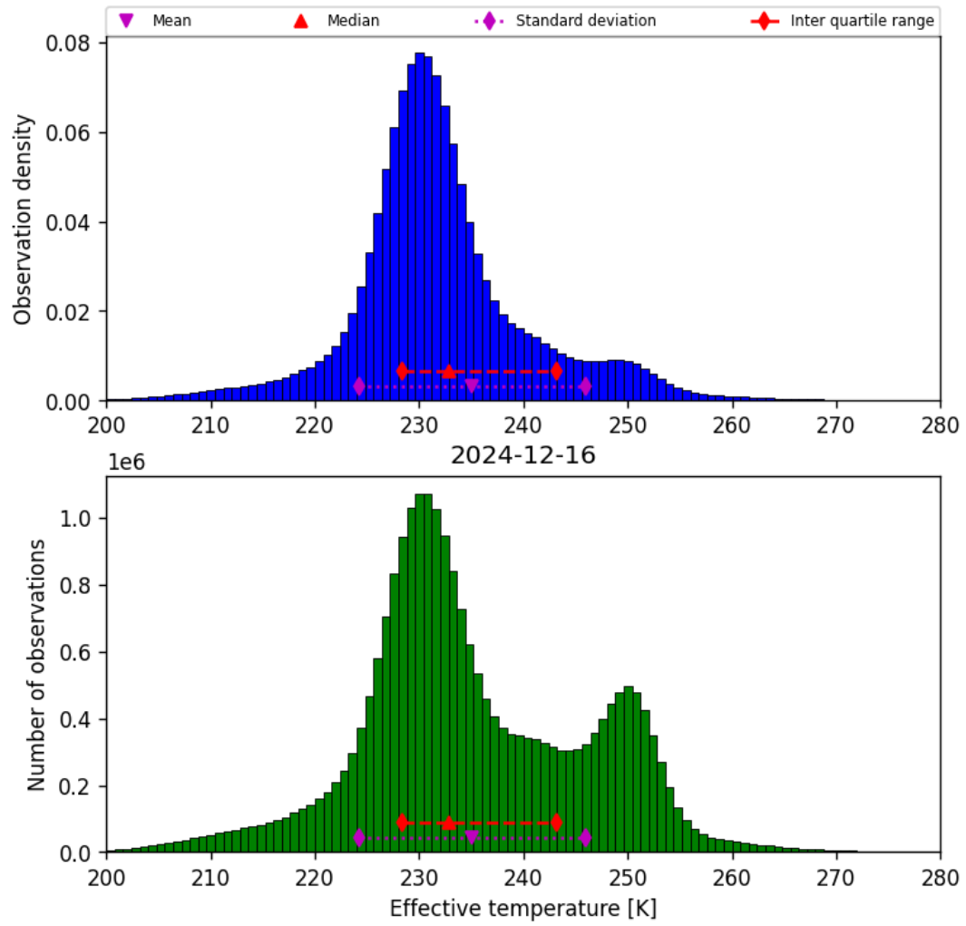
Figure 38: Histogram of “Effective temperature” for 2024-12-16 to 2024-12-17
