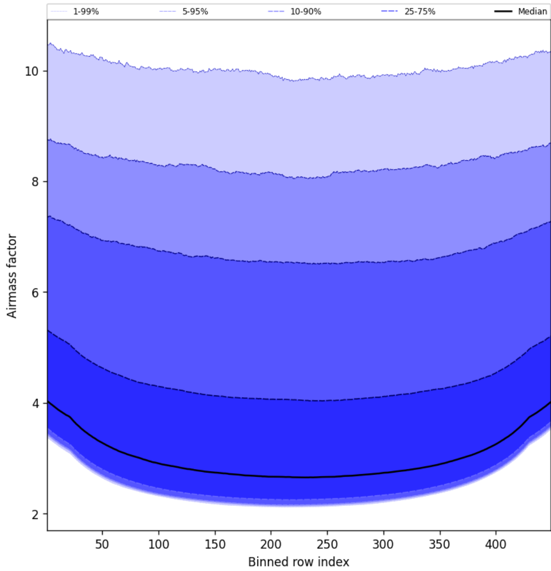
Figure 49: Along track statistics of “Airmass factor” for 2024-12-16 to 2024-12-17
