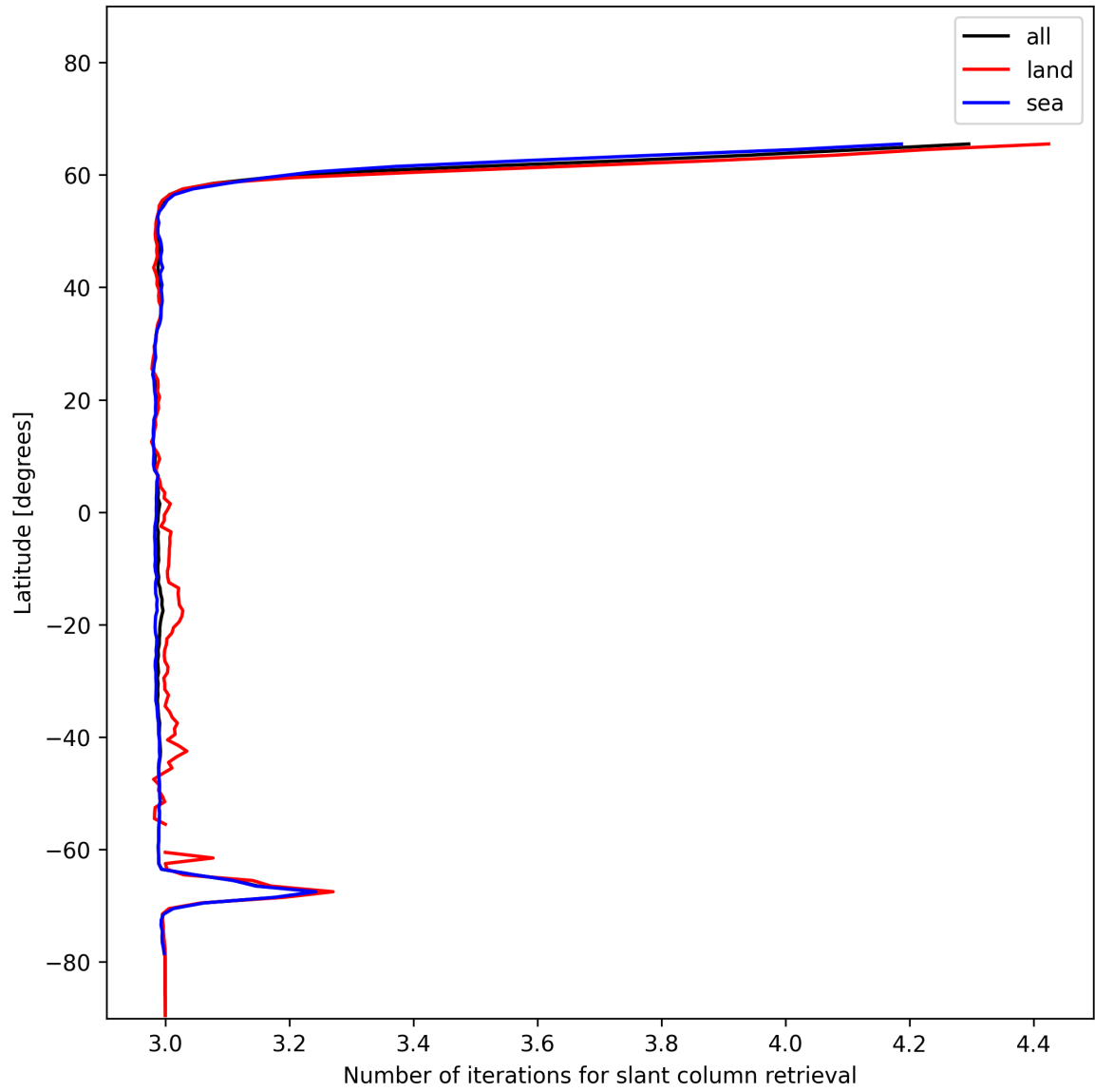
Figure 21: Zonal average of “Number of iterations for slant column retrieval” for 2024-12-16 to 2024-12-17.
