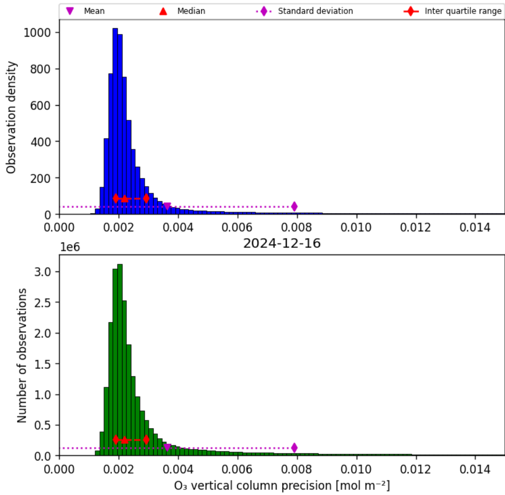
Figure 30: Histogram of “O 3 vertical column precision” for 2024-12-16 to 2024-12-17
