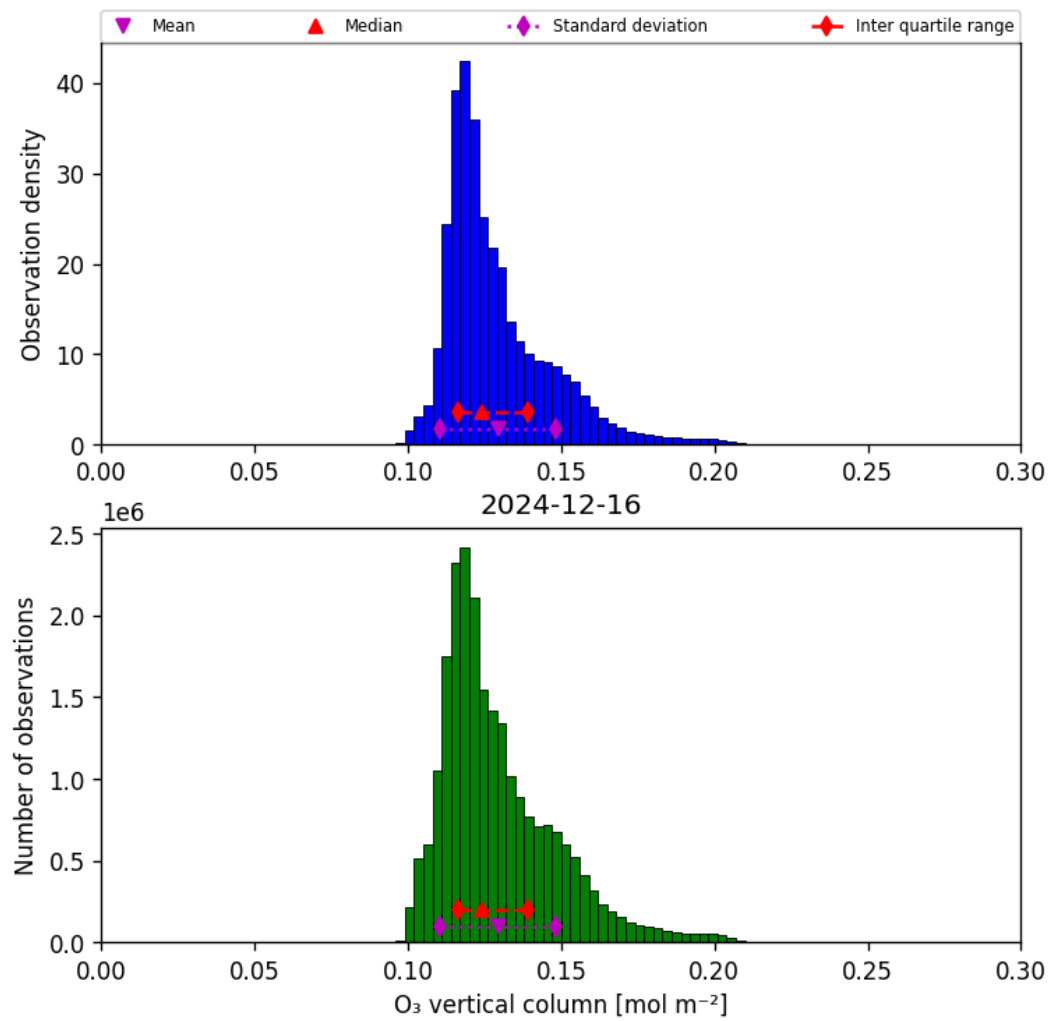
Figure 29: Histogram of “O 3 vertical column” for 2024-12-16 to 2024-12-17
