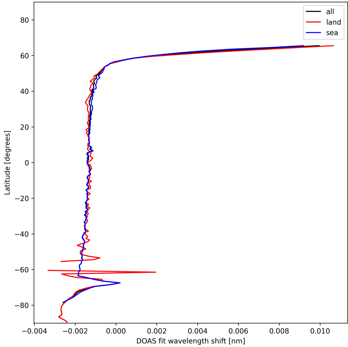
Figure 23: Zonal average of "DOAS fit wavelength shift" for 2024-12-16 to 2024-12-17.
