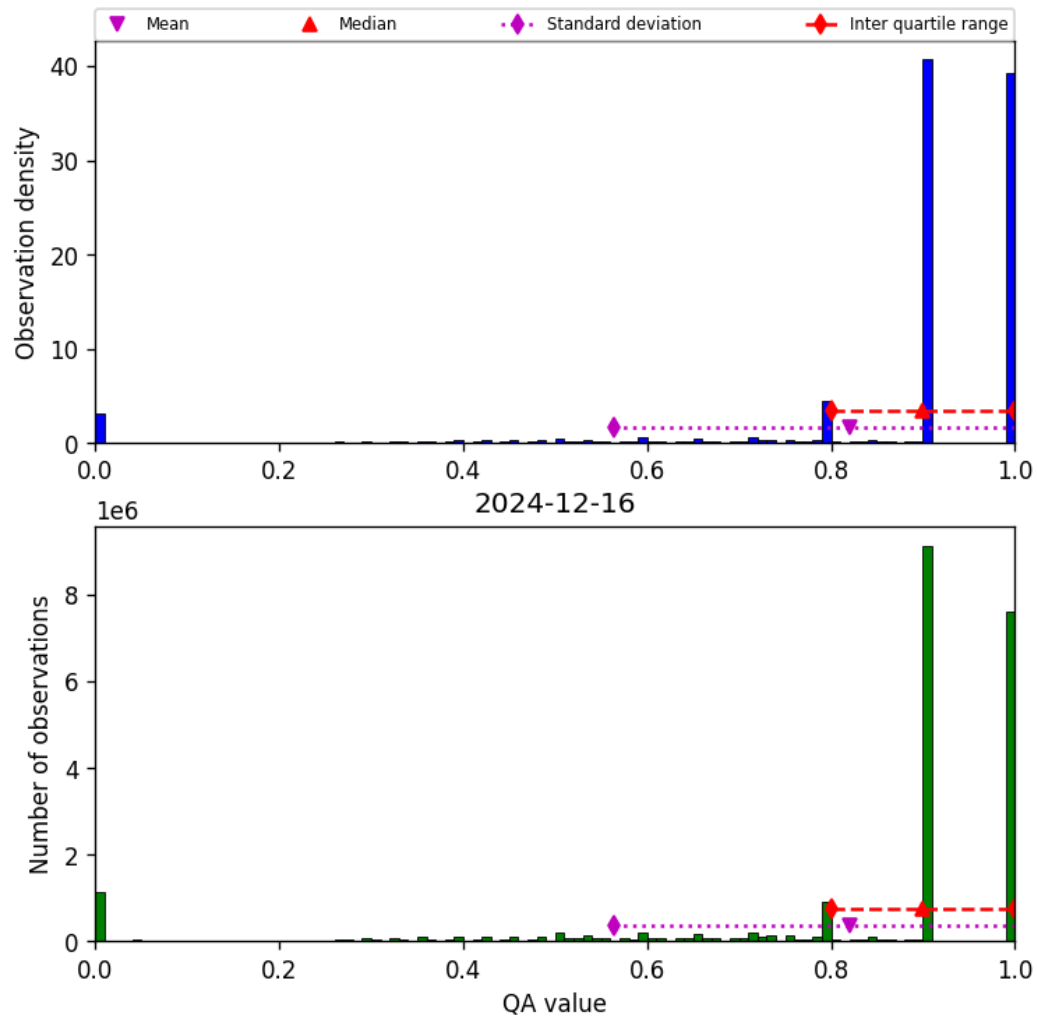
Figure 28: Histogram of “QA value” for 2024-12-16 to 2024-12-17
