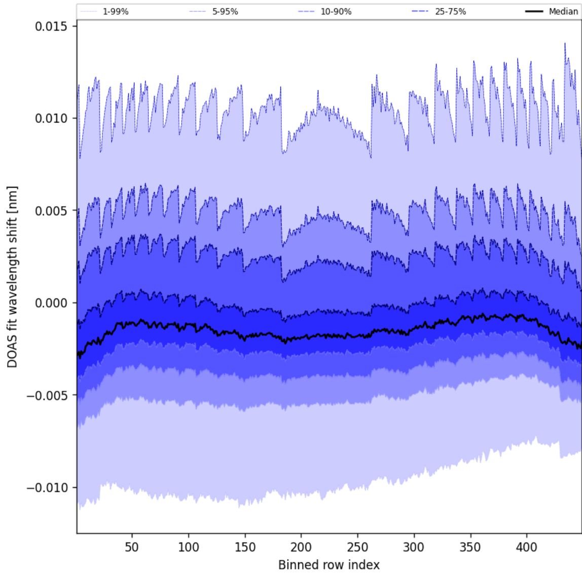
Figure 47: Along track statistics of “DOAS fit wavelength shift” for 2024-12-16 to 2024-12-17
