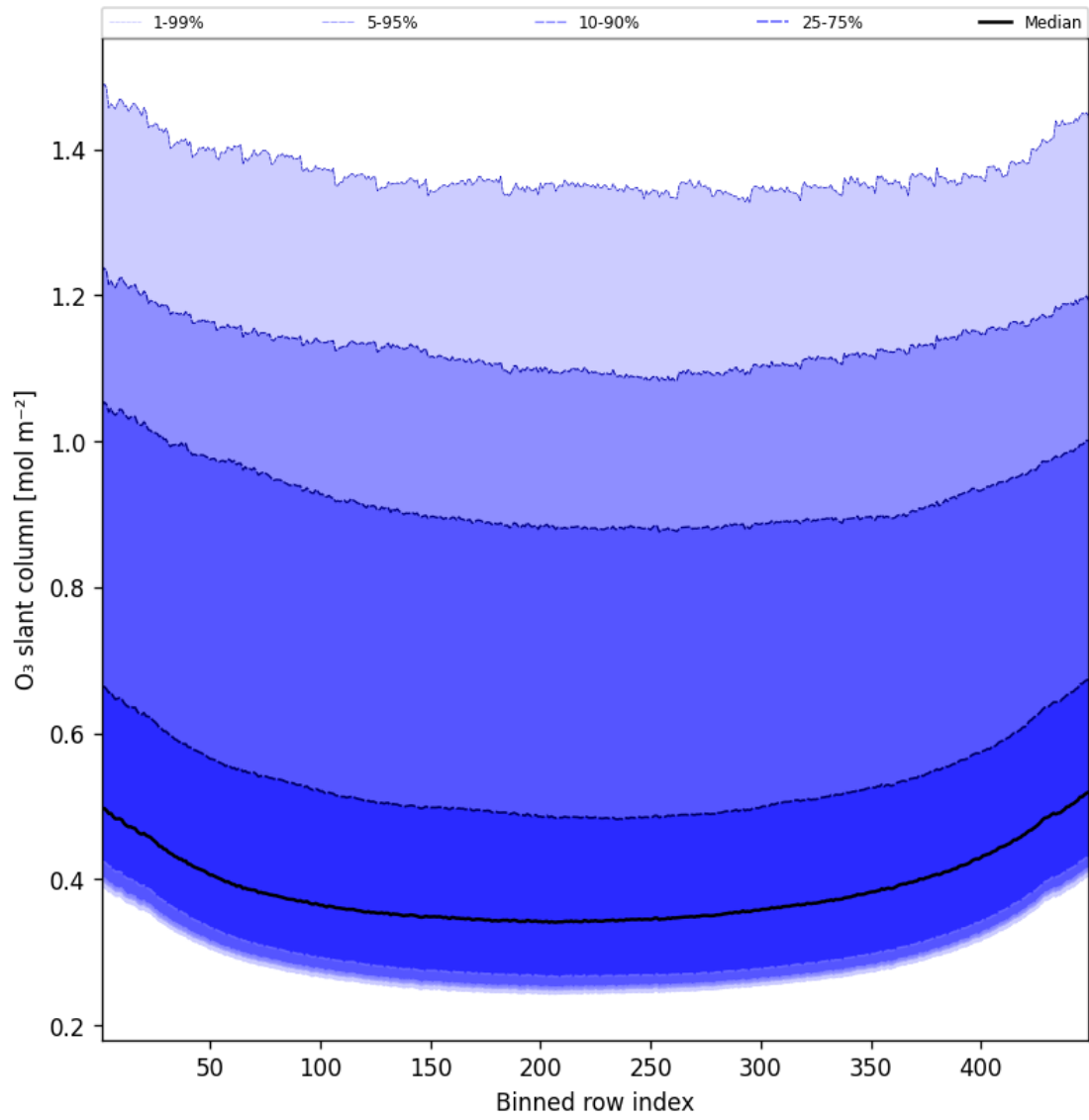
Figure 43: Along track statistics of “O 3 slant column” for 2024-12-16 to 2024-12-17
