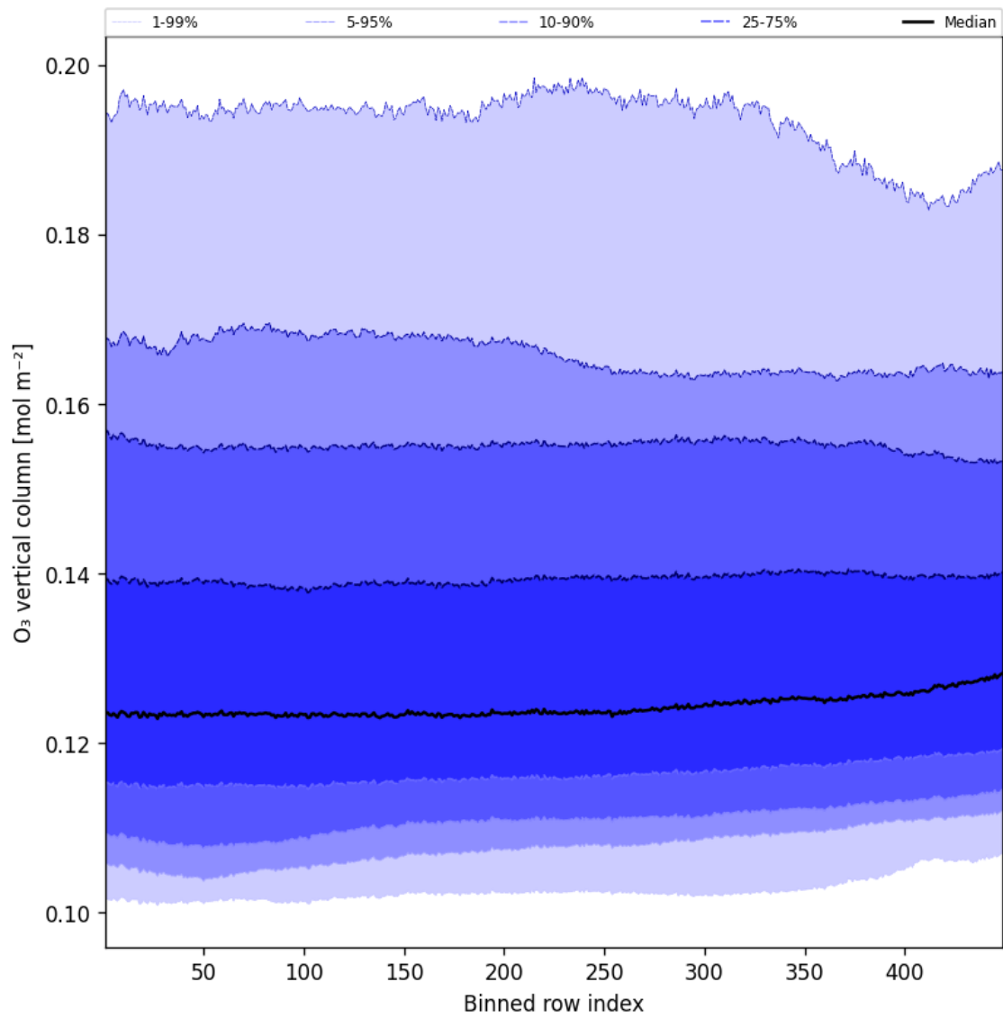
Figure 41: Along track statistics of “O 3 vertical column” for 2024-12-16 to 2024-12-17
