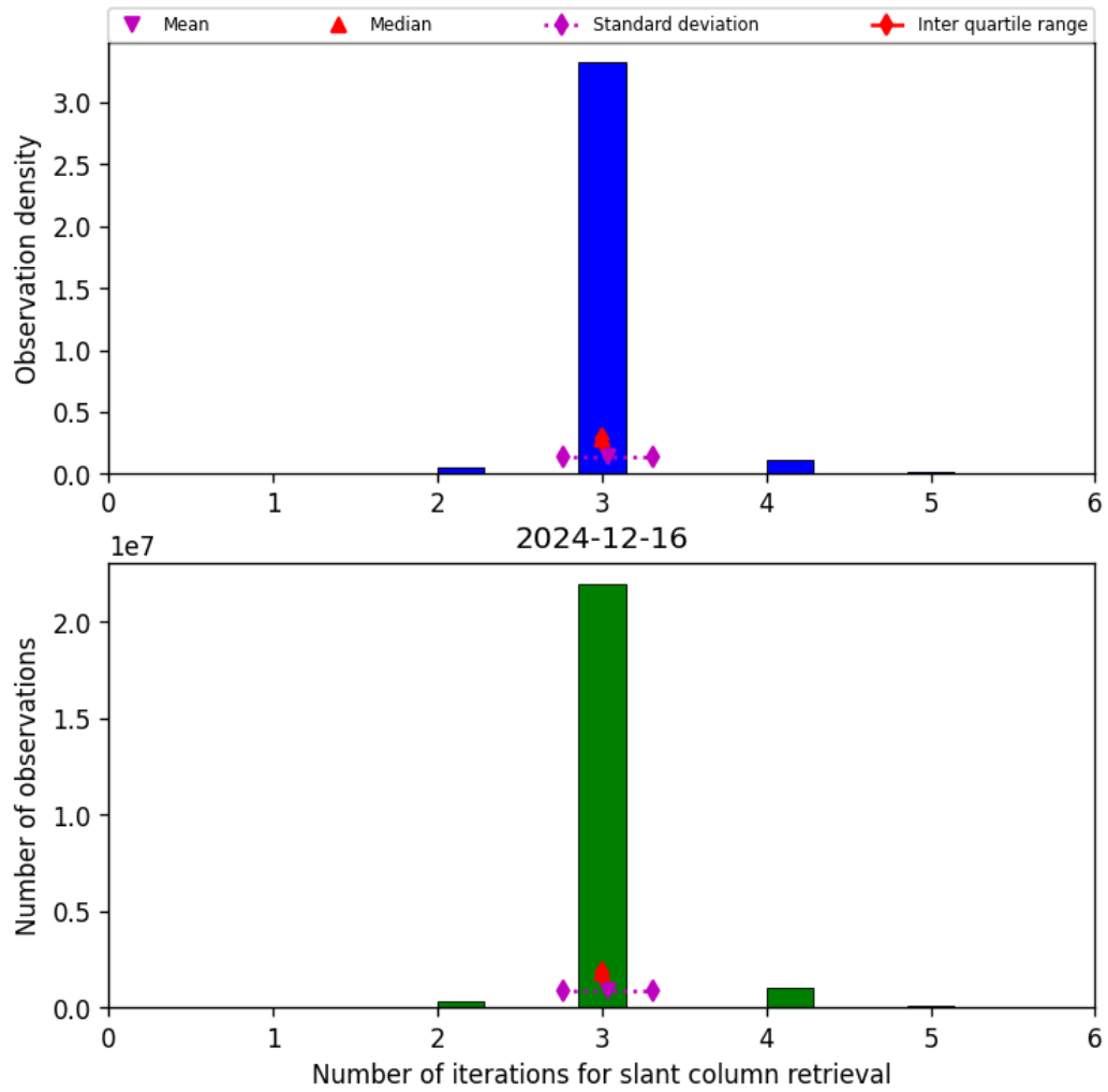
Figure 33: Histogram of “Number of iterations for slant column retrieval” for 2024-12-16 to 2024-12-17
