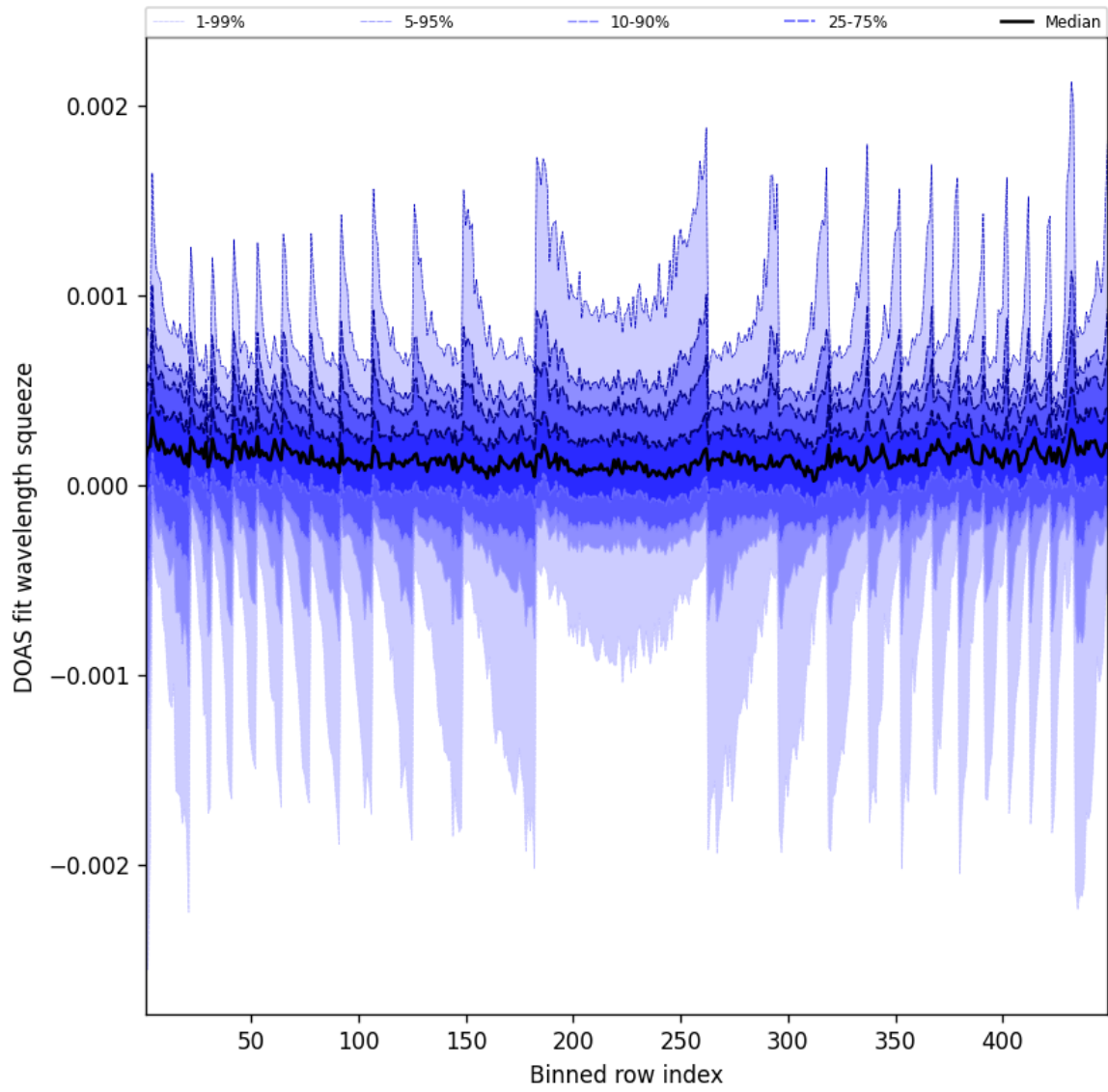
Figure 48: Along track statistics of “DOAS fit wavelength squeeze” for 2024-12-16 to 2024-12-17
