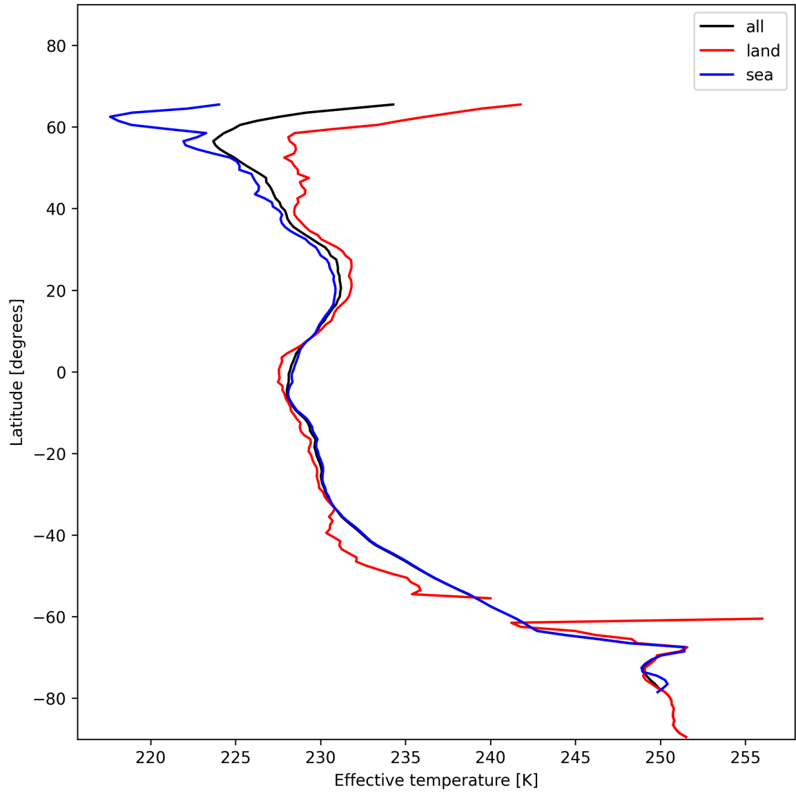
Figure 26: Zonal average of “Effective temperature” for 2024-12-16 to 2024-12-17.
