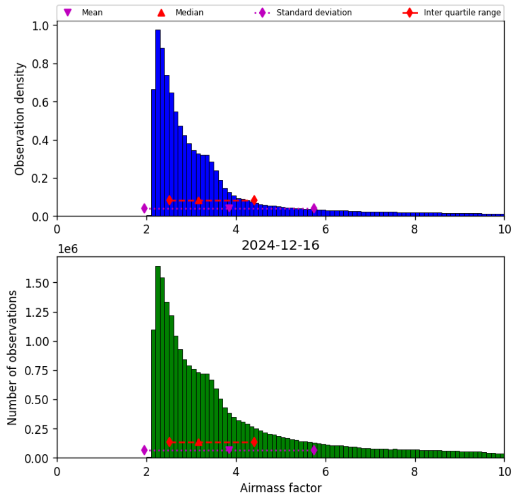
Figure 37: Histogram of “Airmass factor” for 2024-12-16 to 2024-12-17
