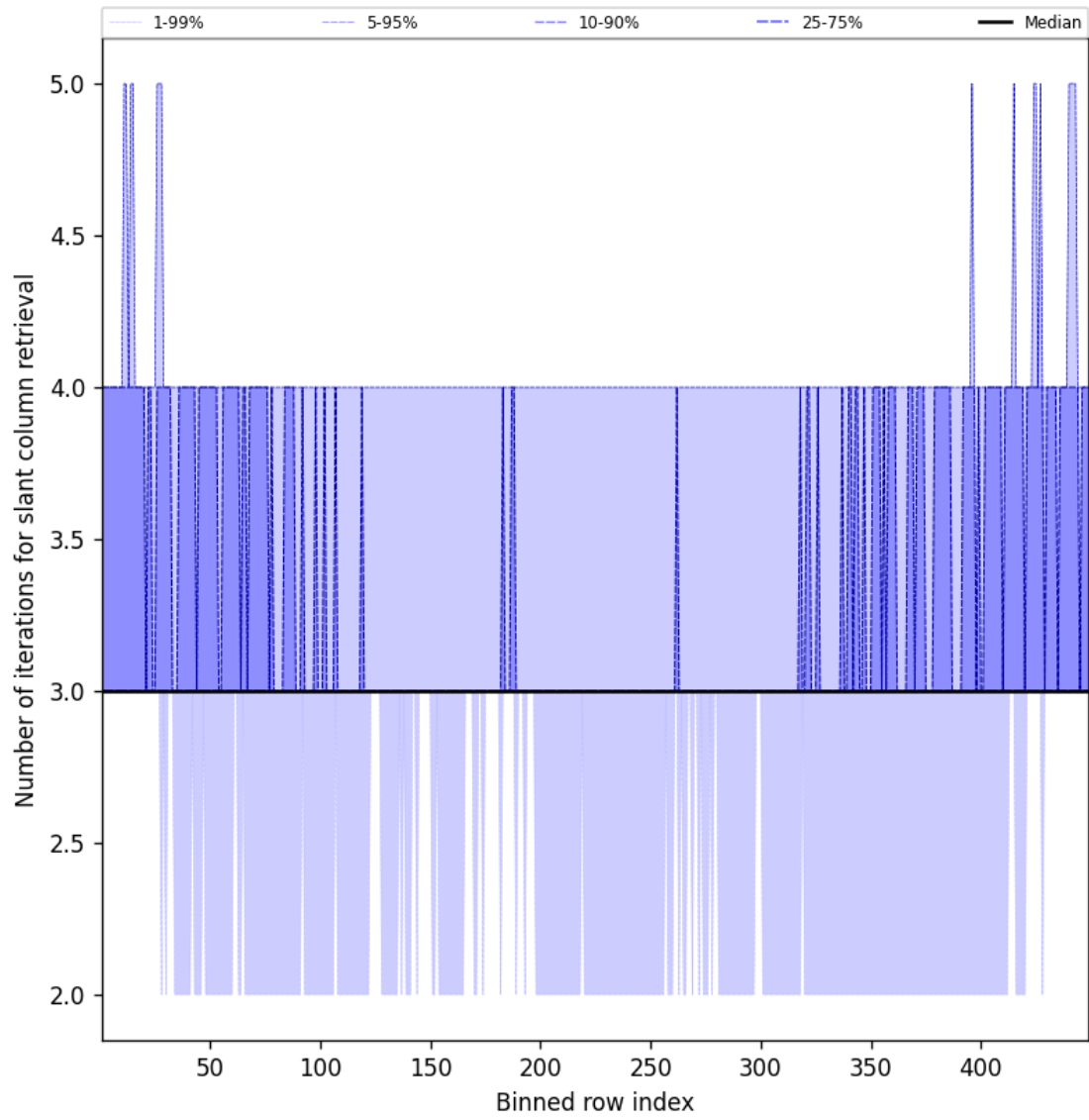
Figure 45: Along track statistics of “Number of iterations for slant column retrieval” for 2024-12-16 to 2024-12-17
