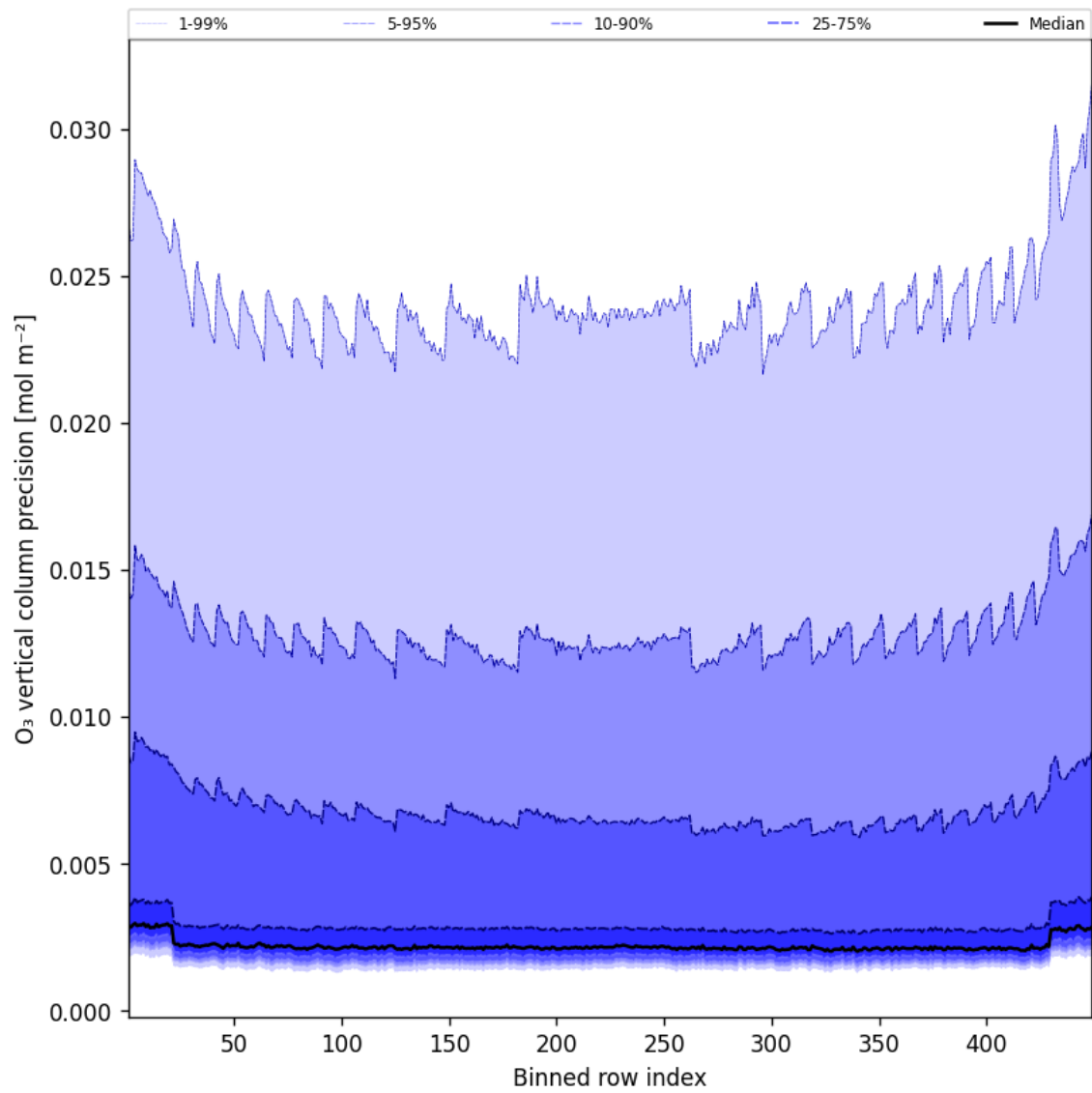
Figure 42: Along track statistics of “O 3 vertical column precision” for 2024-12-16 to 2024-12-17
