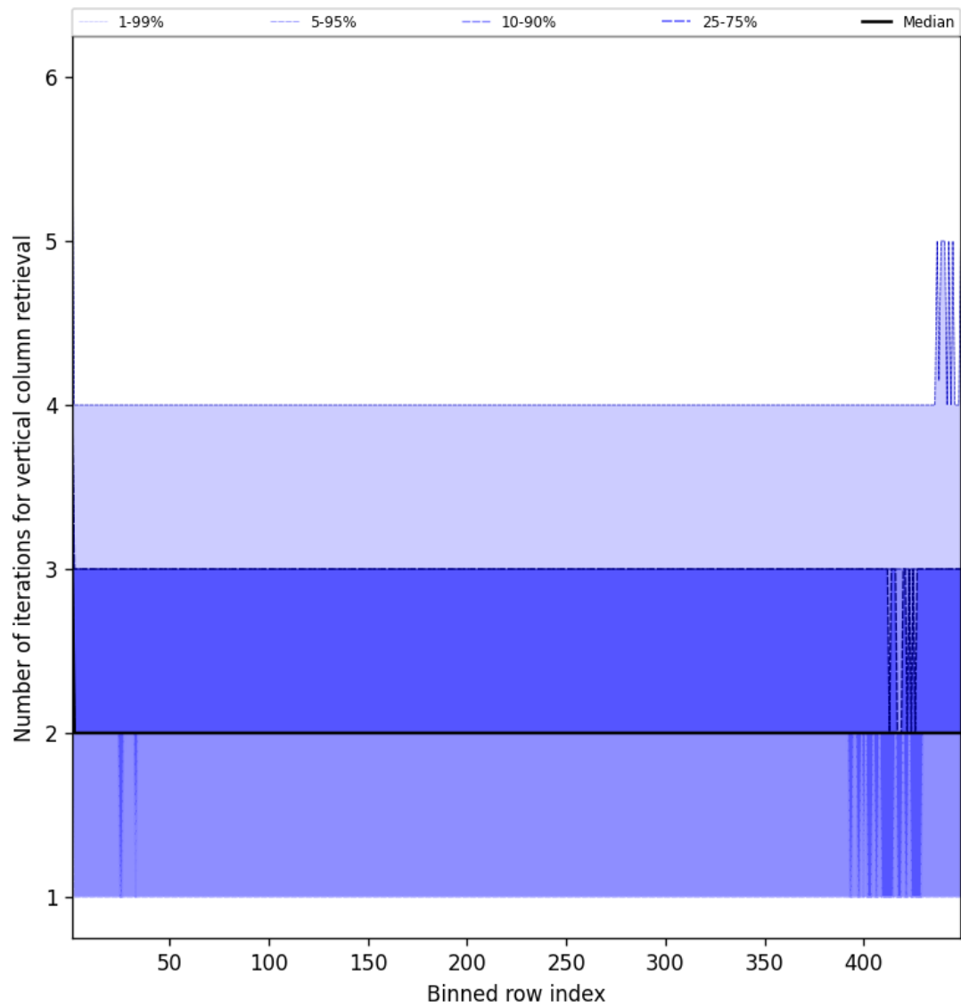
Figure 51: Along track statistics of “Number of iterations for vertical column retrieval” for 2024-12-16 to 2024-12-17
