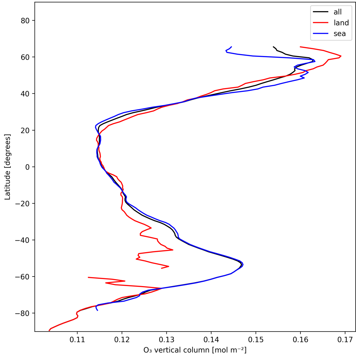
Figure 17: Zonal average of “O 3 vertical column” for 2024-12-16 to 2024-12-17.
