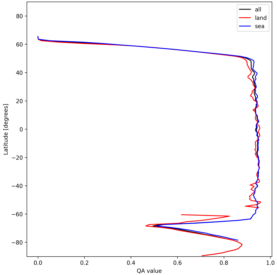
Figure 16: Zonal average of “QA value” for 2024-12-16 to 2024-12-17.
