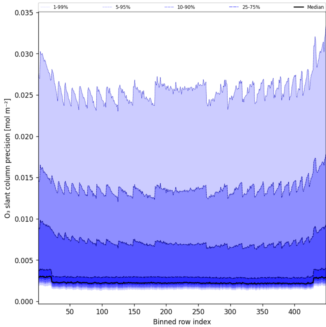
Figure 44: Along track statistics of “O 3 slant column precision” for 2024-12-16 to 2024-12-17
