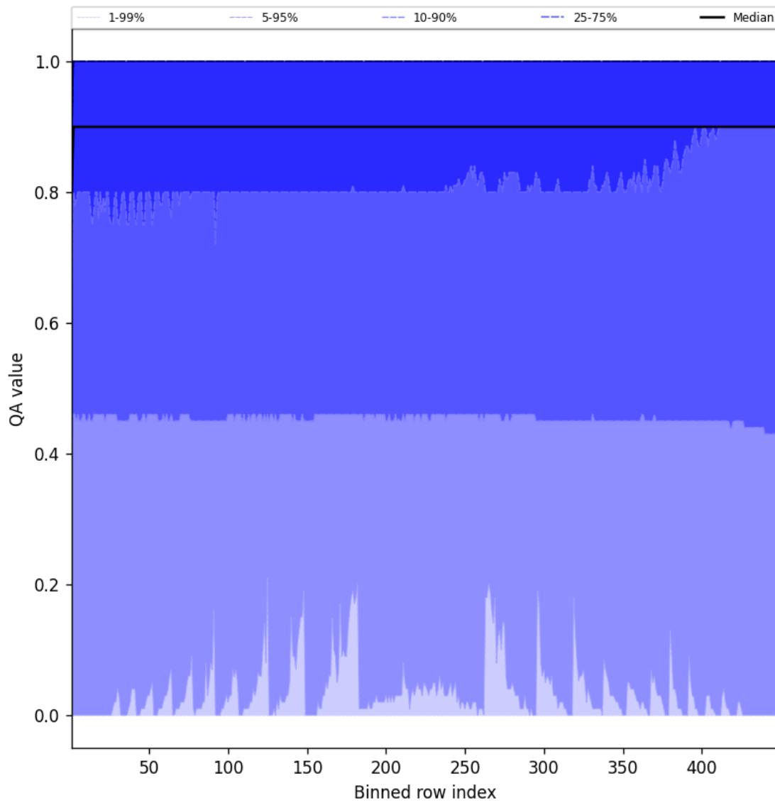
Figure 40: Along track statistics of “QA value” for 2024-12-16 to 2024-12-17
