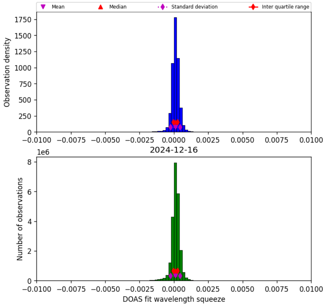
Figure 36: Histogram of “DOAS fit wavelength squeeze” for 2024-12-16 to 2024-12-17
