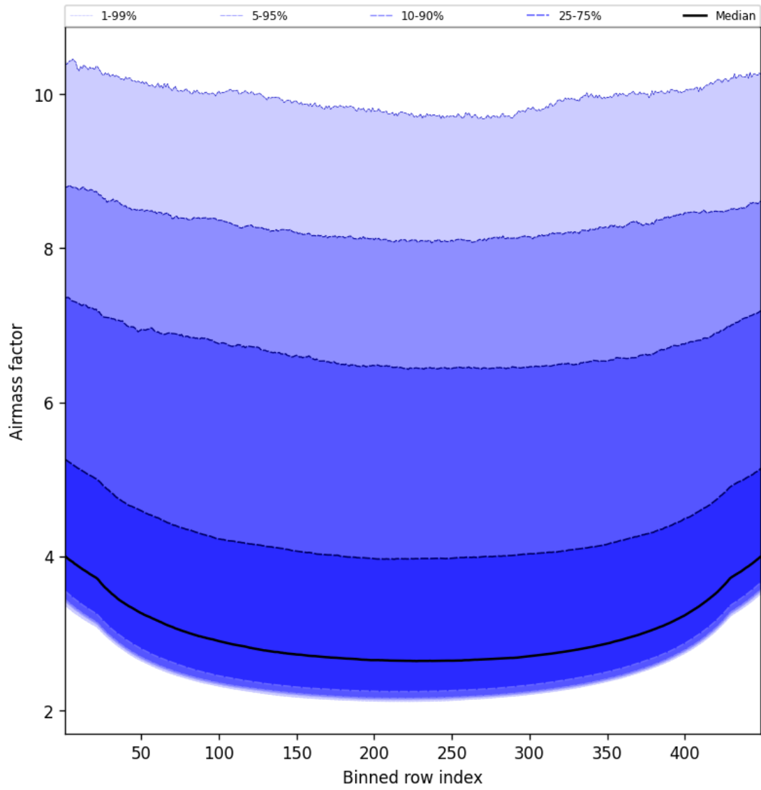
Figure 49: Along track statistics of “Airmass factor” for 2024-12-17 to 2024-12-18
