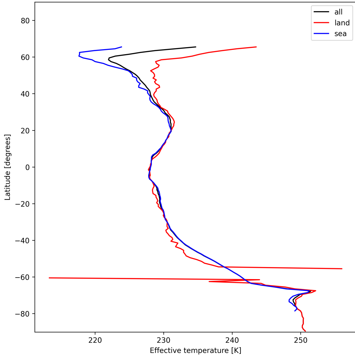
Figure 26: Zonal average of “Effective temperature” for 2024-12-17 to 2024-12-18.
