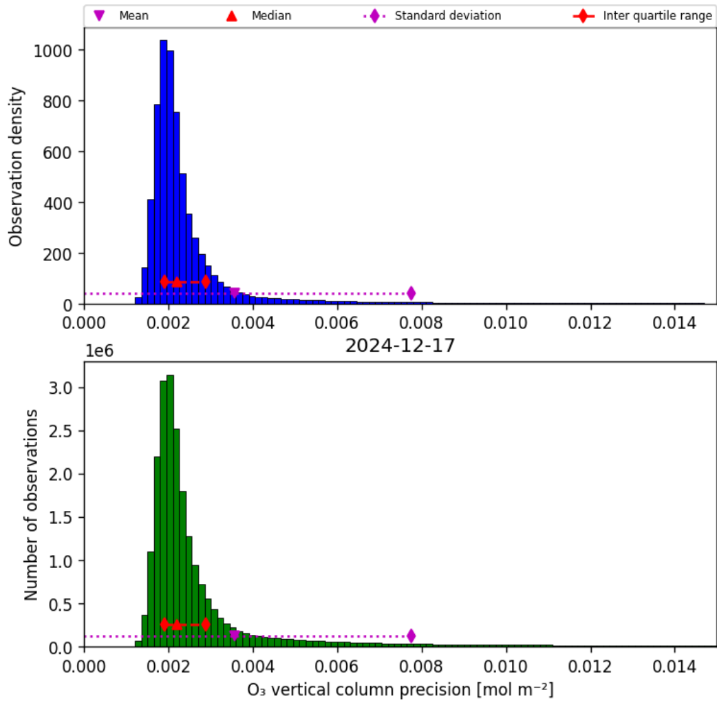
Figure 30: Histogram of “O 3 vertical column precision” for 2024-12-17 to 2024-12-18
