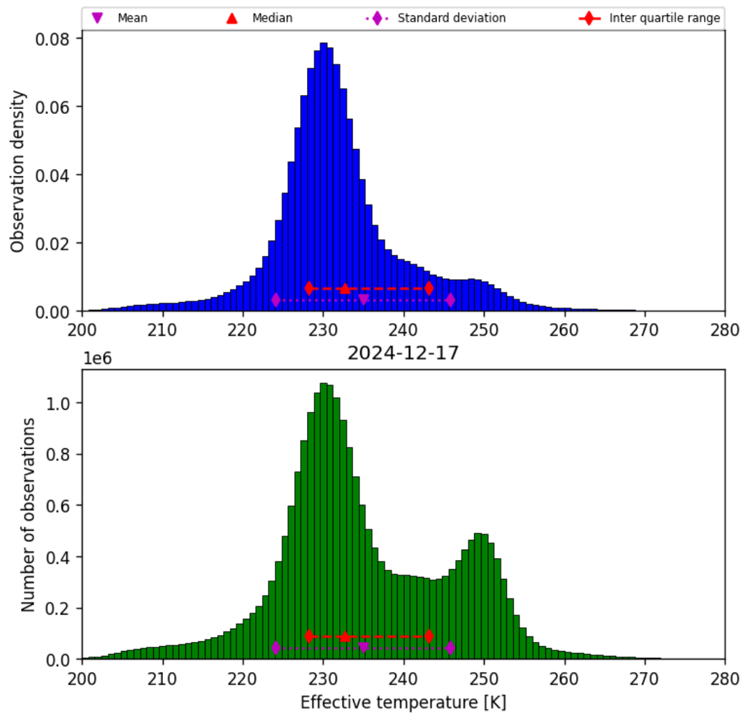
Figure 38: Histogram of “Effective temperature” for 2024-12-17 to 2024-12-18
