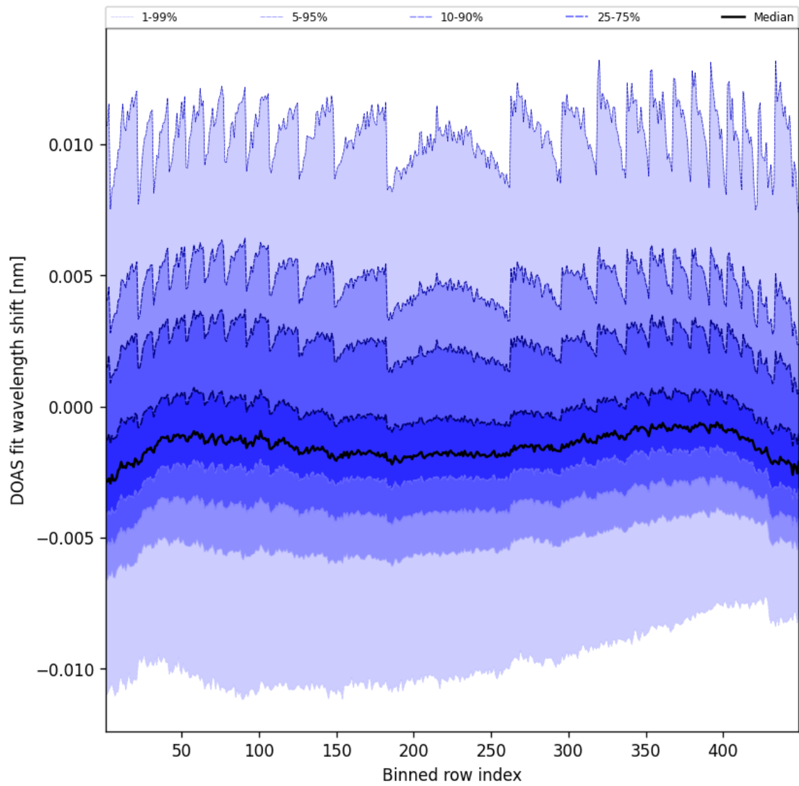
Figure 47: Along track statistics of “DOAS fit wavelength shift” for 2024-12-17 to 2024-12-18
