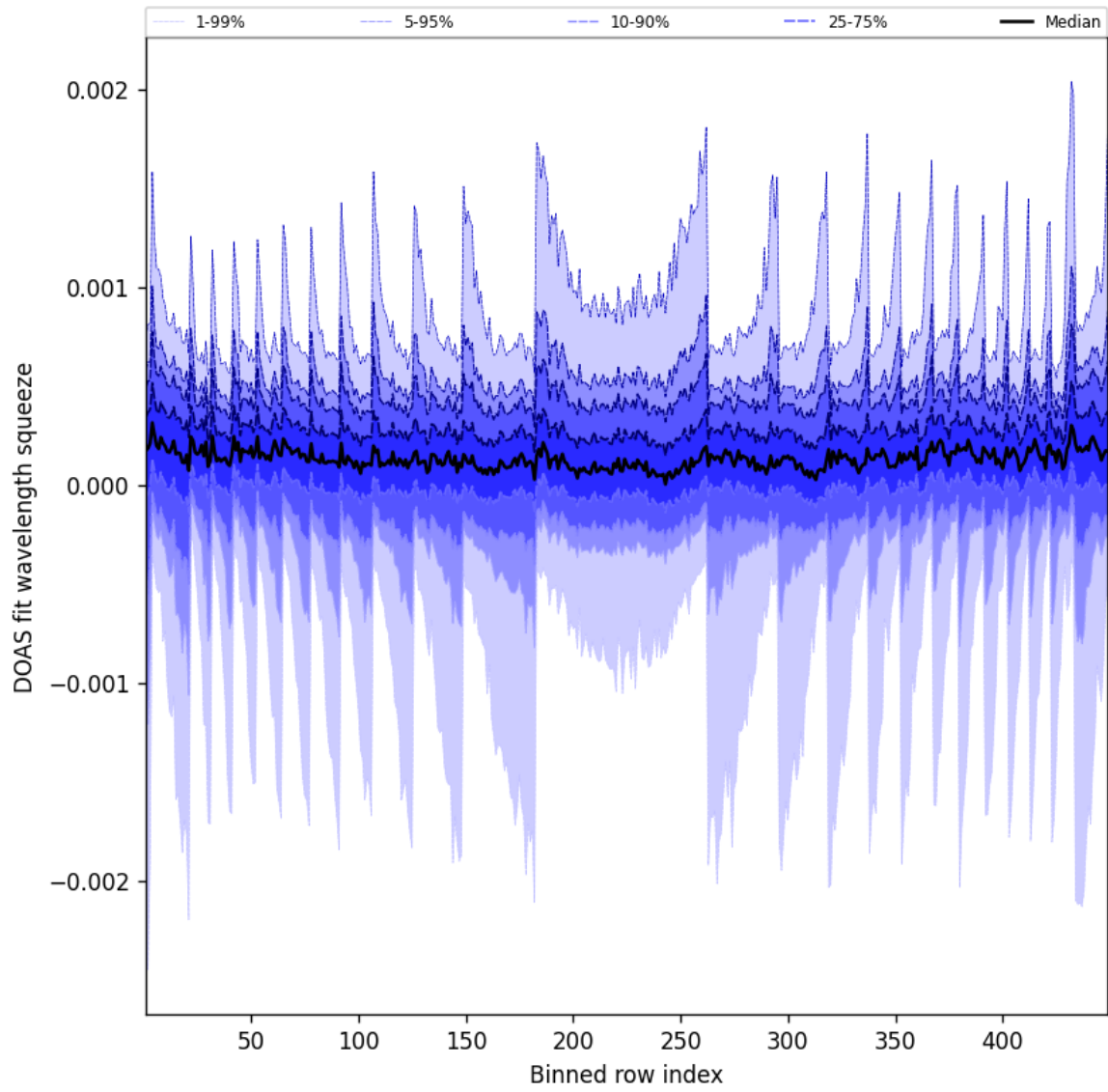
Figure 48: Along track statistics of “DOAS fit wavelength squeeze” for 2024-12-17 to 2024-12-18
