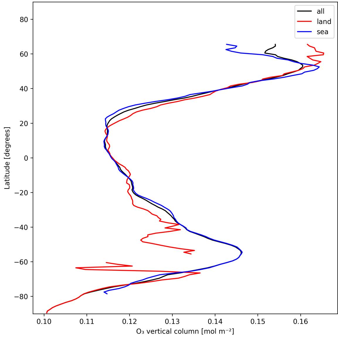
Figure 17: Zonal average of “O 3 vertical column” for 2024-12-17 to 2024-12-18.
