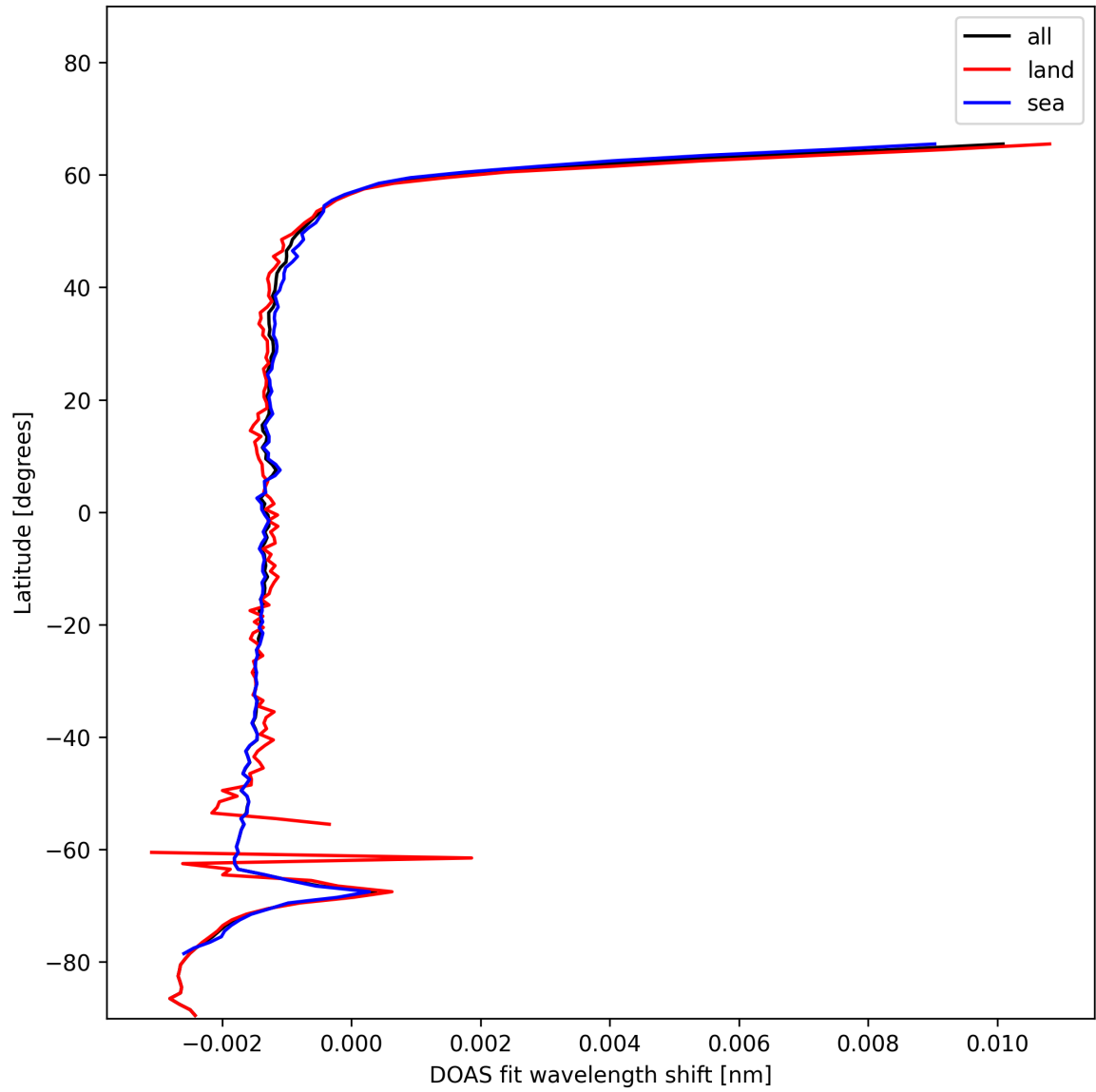
Figure 23: Zonal average of “DOAS fit wavelength shift” for 2024-12-17 to 2024-12-18.
