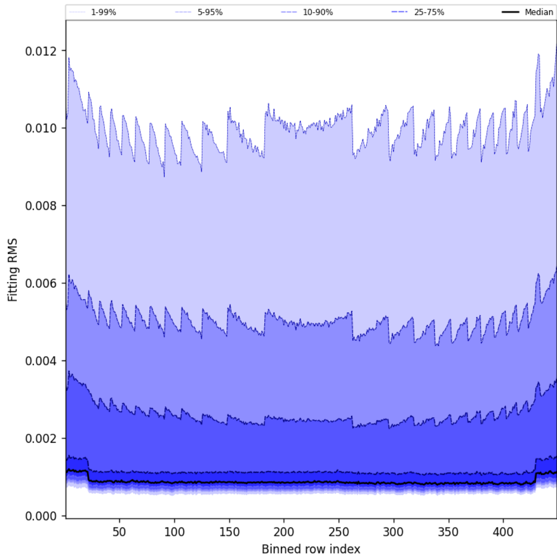
Figure 46: Along track statistics of “Fitting RMS” for 2024-12-17 to 2024-12-18
