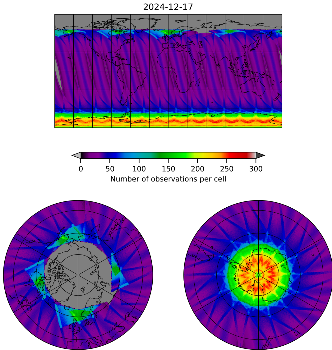
Figure 15: Map of the number of observations for 2024-12-17 to 2024-12-18
