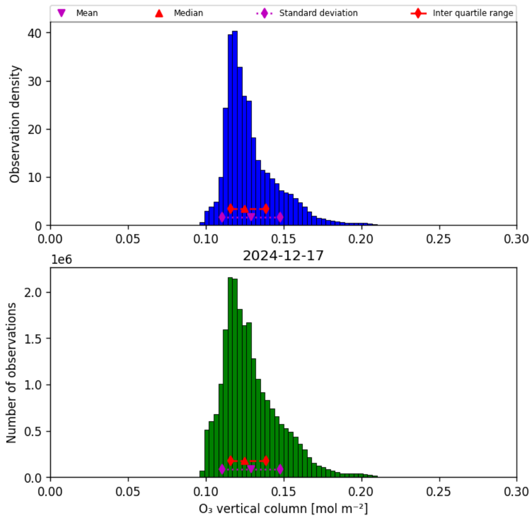
Figure 29: Histogram of “O 3 vertical column” for 2024-12-17 to 2024-12-18
