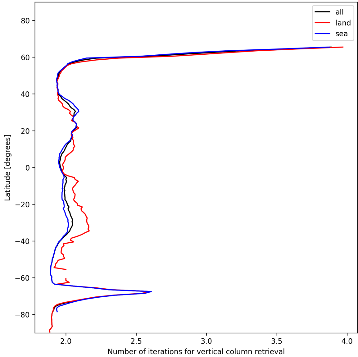
Figure 27: Zonal average of “Number of iterations for vertical column retrieval” for 2024-12-17 to 2024-12-18.
