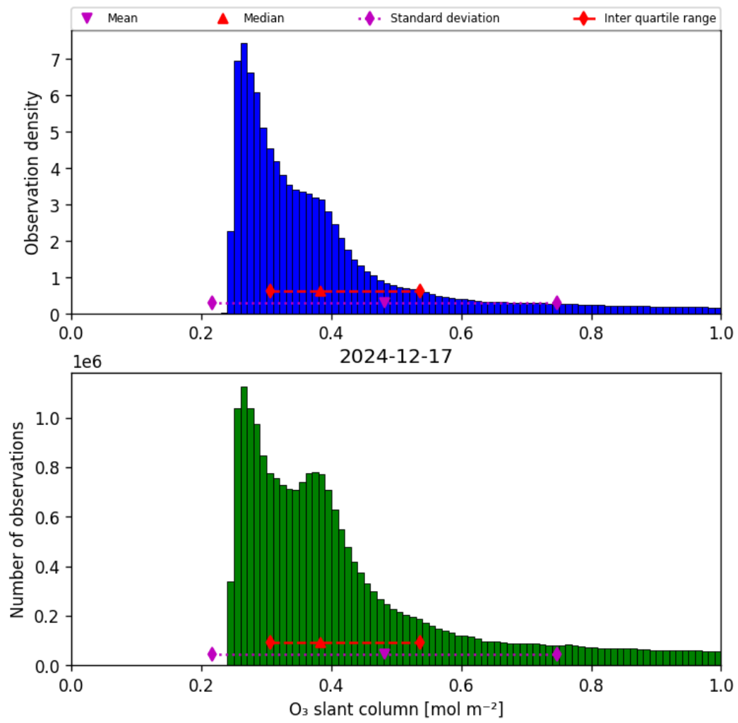
Figure 31: Histogram of “O 3 slant column” for 2024-12-17 to 2024-12-18
