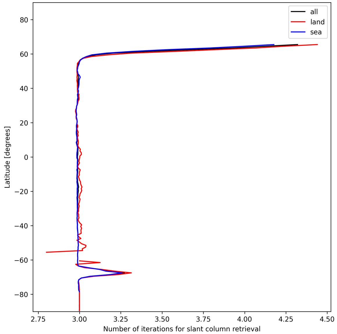
Figure 21: Zonal average of “Number of iterations for slant column retrieval” for 2024-12-17 to 2024-12-18.
