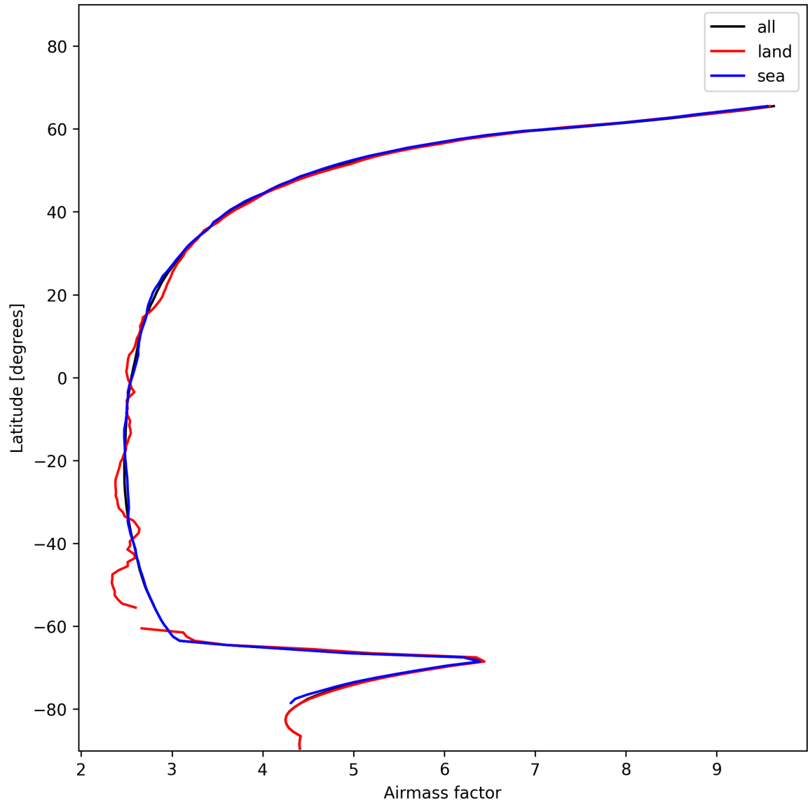
Figure 25: Zonal average of “Airmass factor” for 2024-12-17 to 2024-12-18.
