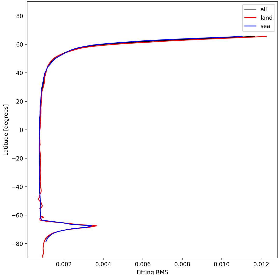
Figure 22: Zonal average of “Fitting RMS” for 2024-12-17 to 2024-12-18.
