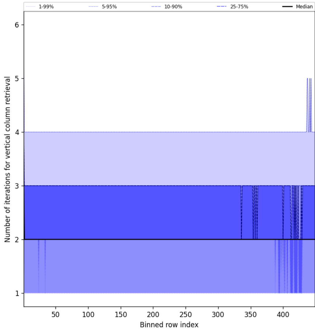
Figure 51: Along track statistics of “Number of iterations for vertical column retrieval” for 2024-12-17 to 2024-12-18
