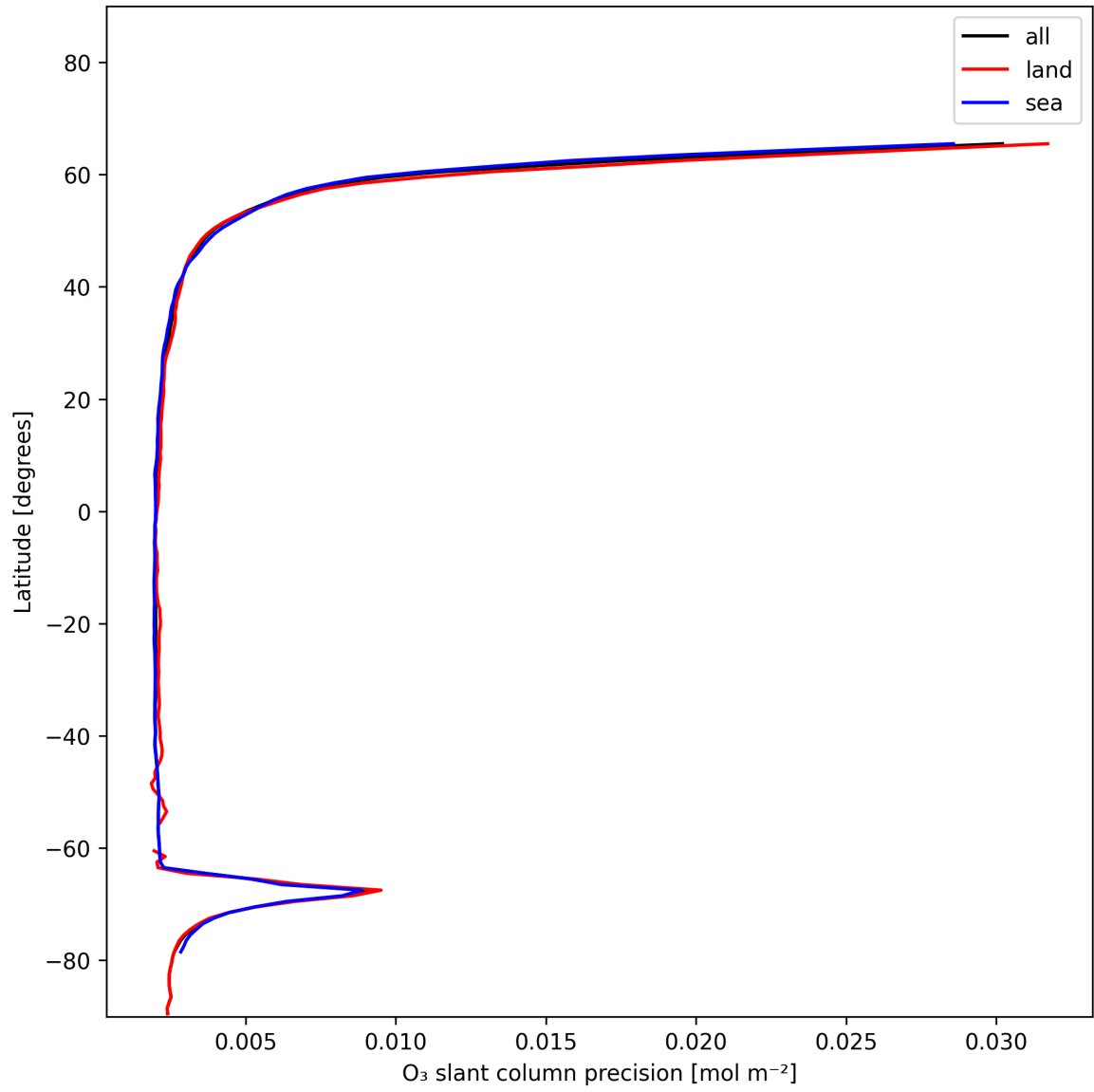
Figure 20: Zonal average of “O 3 slant column precision” for 2024-12-17 to 2024-12-18.
