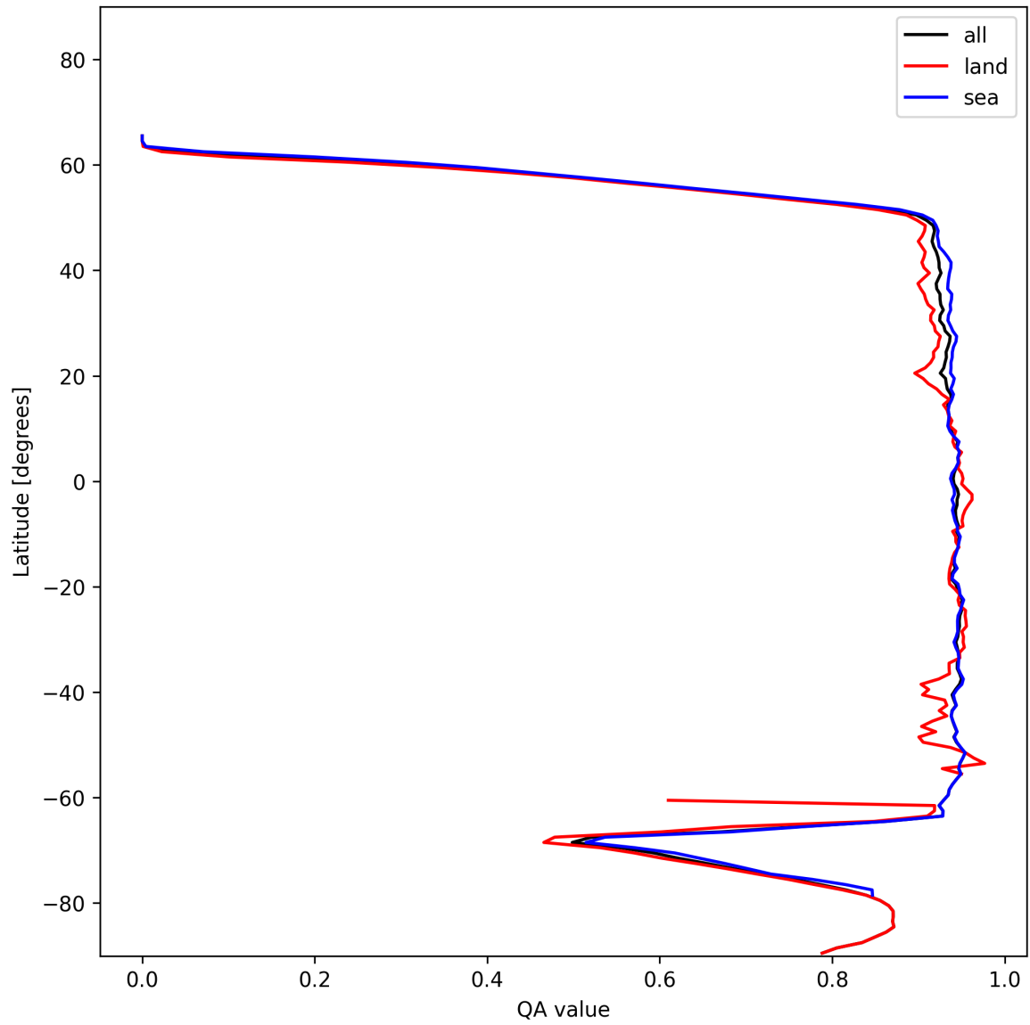
Figure 16: Zonal average of “QA value” for 2024-12-17 to 2024-12-18.
