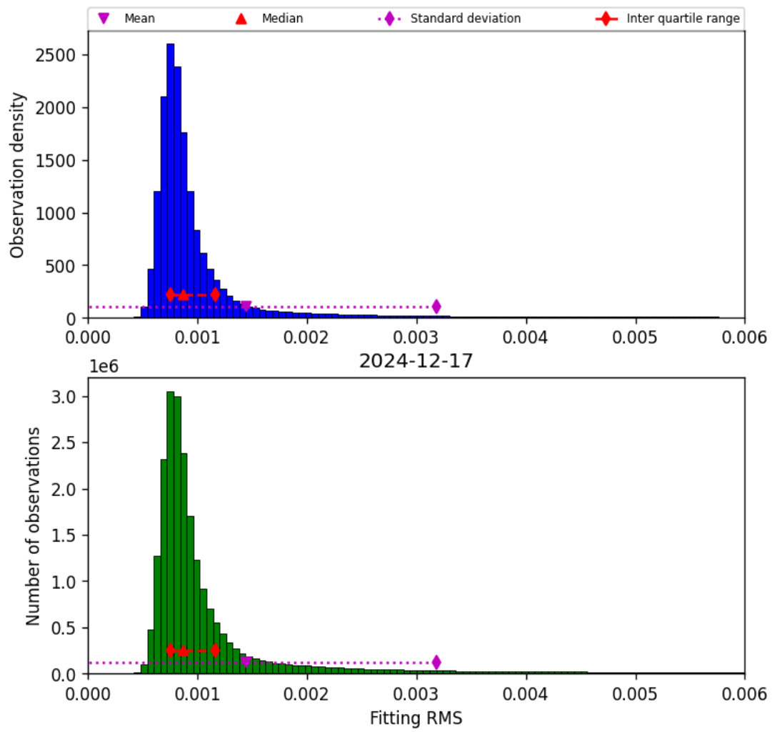
Figure 34: Histogram of "Fitting RMS" for 2024-12-17 to 2024-12-18
