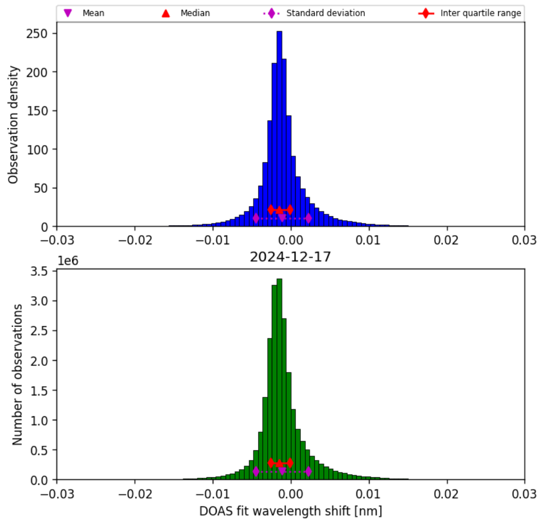
Figure 35: Histogram of “DOAS fit wavelength shift” for 2024-12-17 to 2024-12-18
