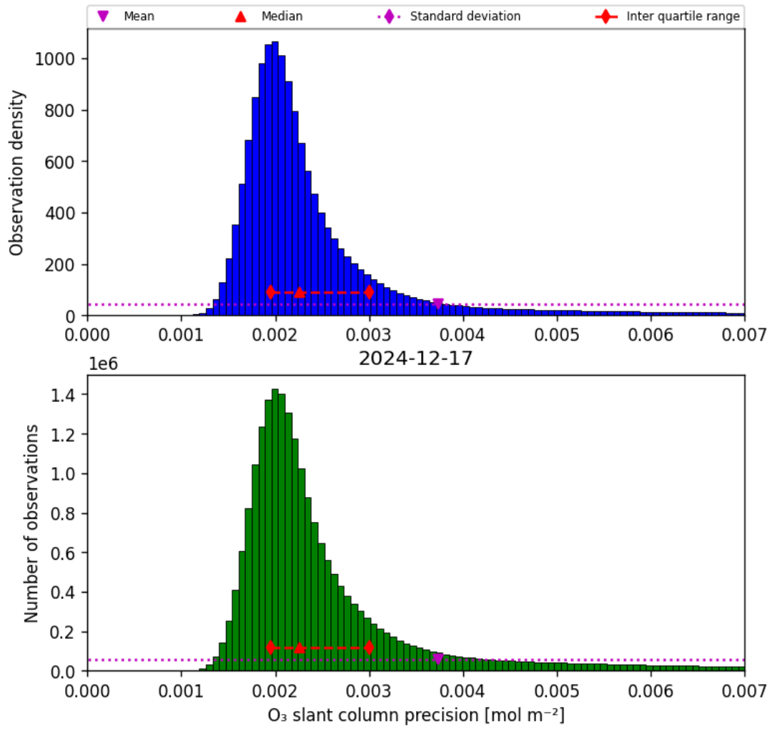
Figure 32: Histogram of “O 3 slant column precision” for 2024-12-17 to 2024-12-18
