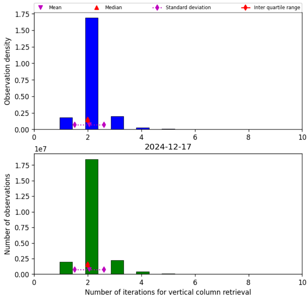
Figure 39: Histogram of “Number of iterations for vertical column retrieval” for 2024-12-17 to 2024-12-18
