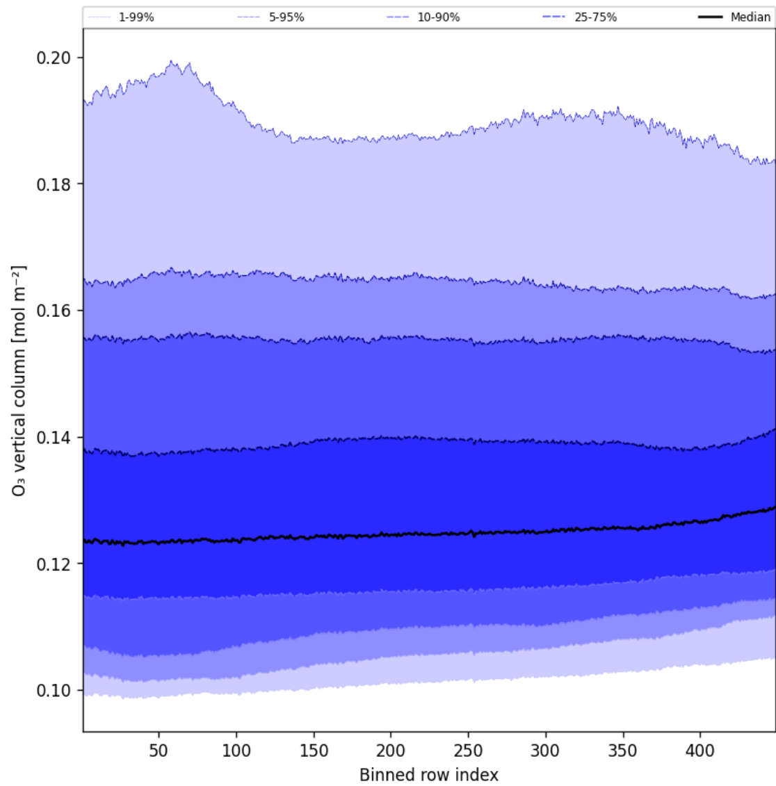
Figure 41: Along track statistics of “O 3 vertical column” for 2024-12-17 to 2024-12-18
