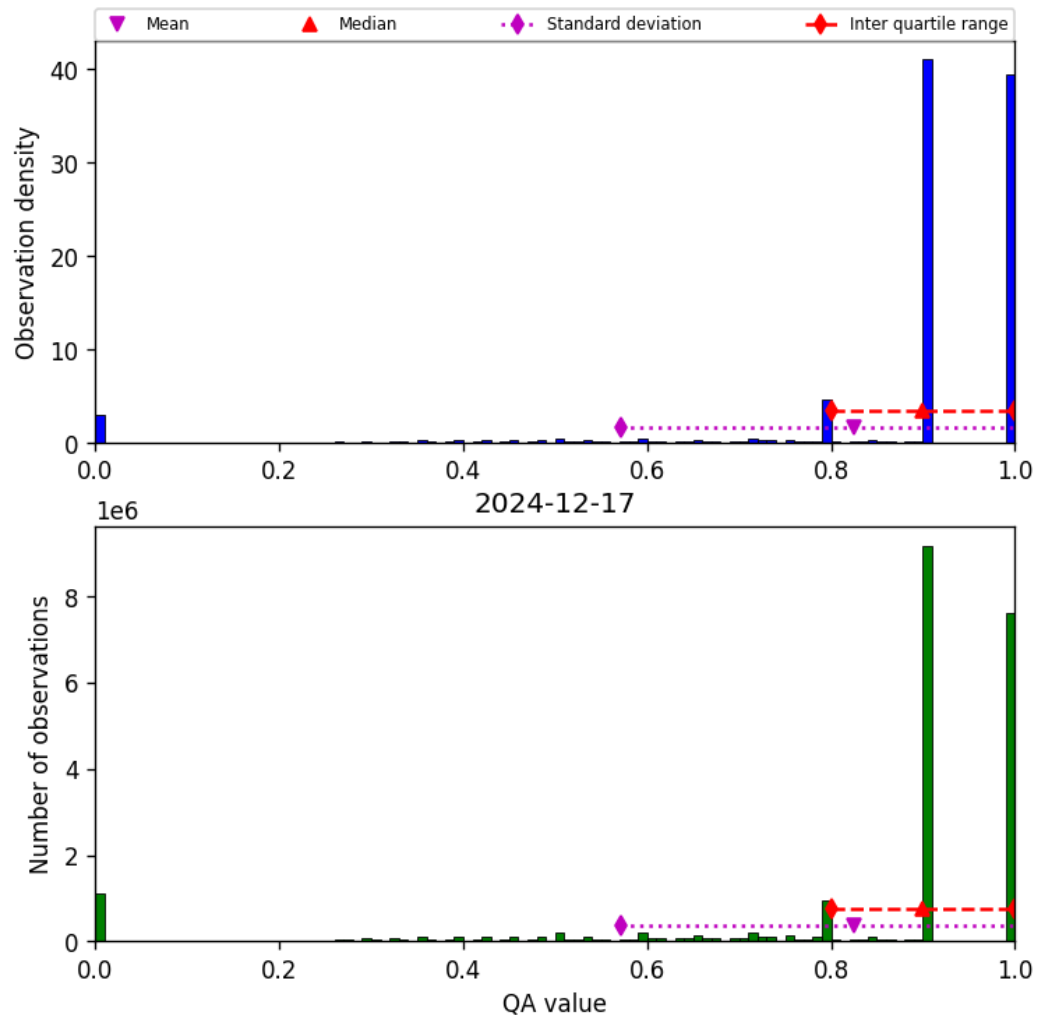
Figure 28: Histogram of “QA value” for 2024-12-17 to 2024-12-18
