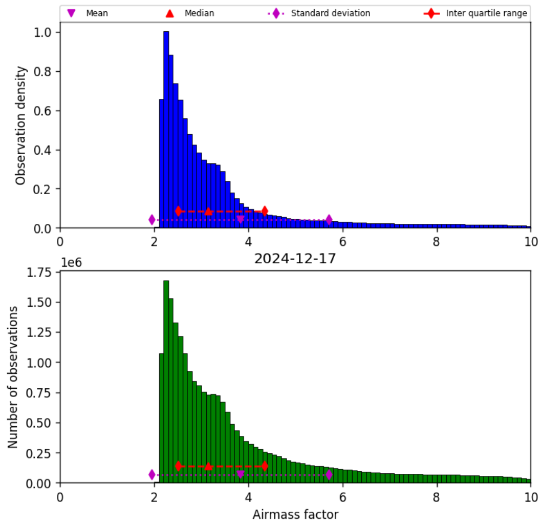
Figure 37: Histogram of “Airmass factor” for 2024-12-17 to 2024-12-18
