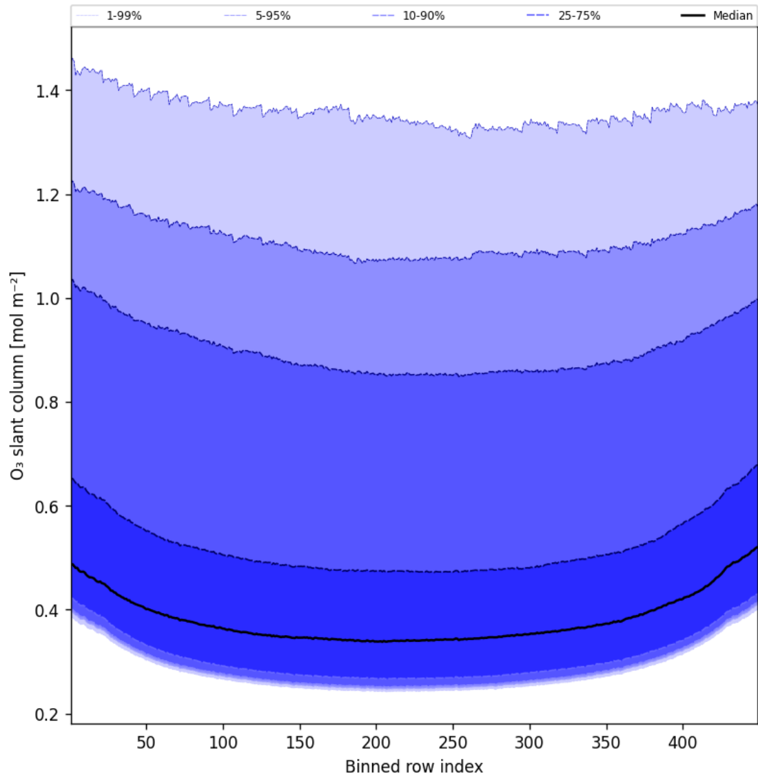
Figure 43: Along track statistics of “O 3 slant column” for 2024-12-17 to 2024-12-18
