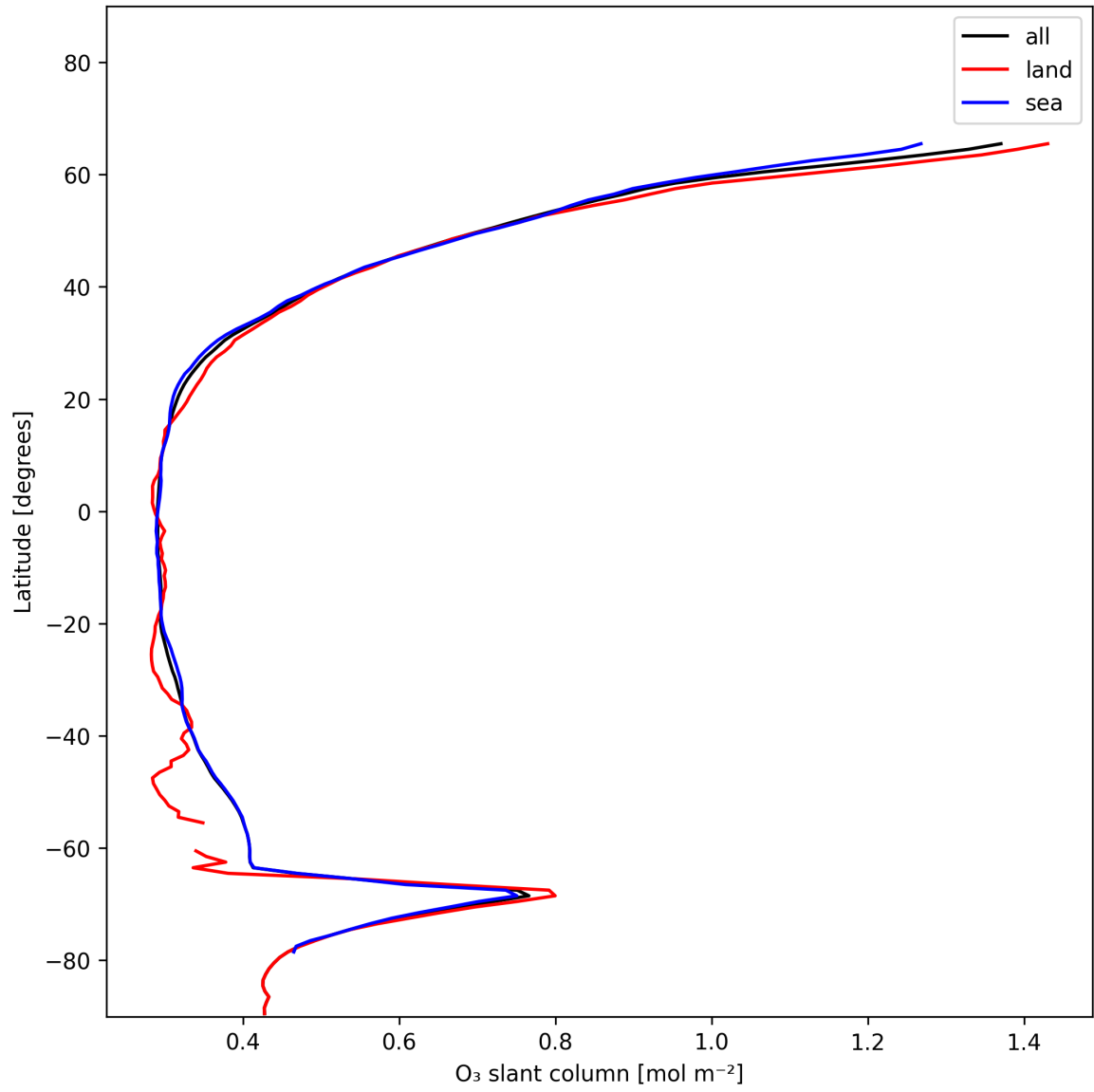
Figure 19: Zonal average of “O 3 slant column” for 2024-12-17 to 2024-12-18.
