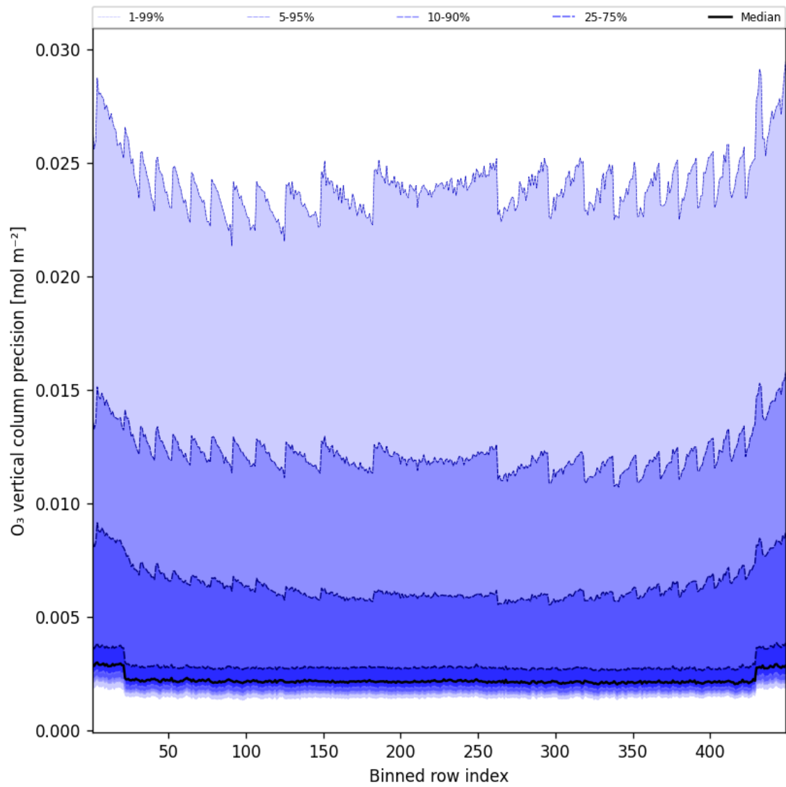
Figure 42: Along track statistics of “O 3 vertical column precision” for 2024-12-17 to 2024-12-18
