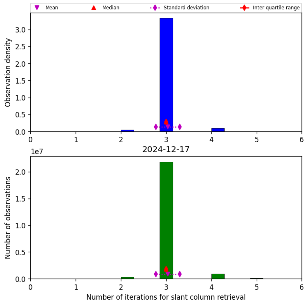
Figure 33: Histogram of “Number of iterations for slant column retrieval” for 2024-12-17 to 2024-12-18
