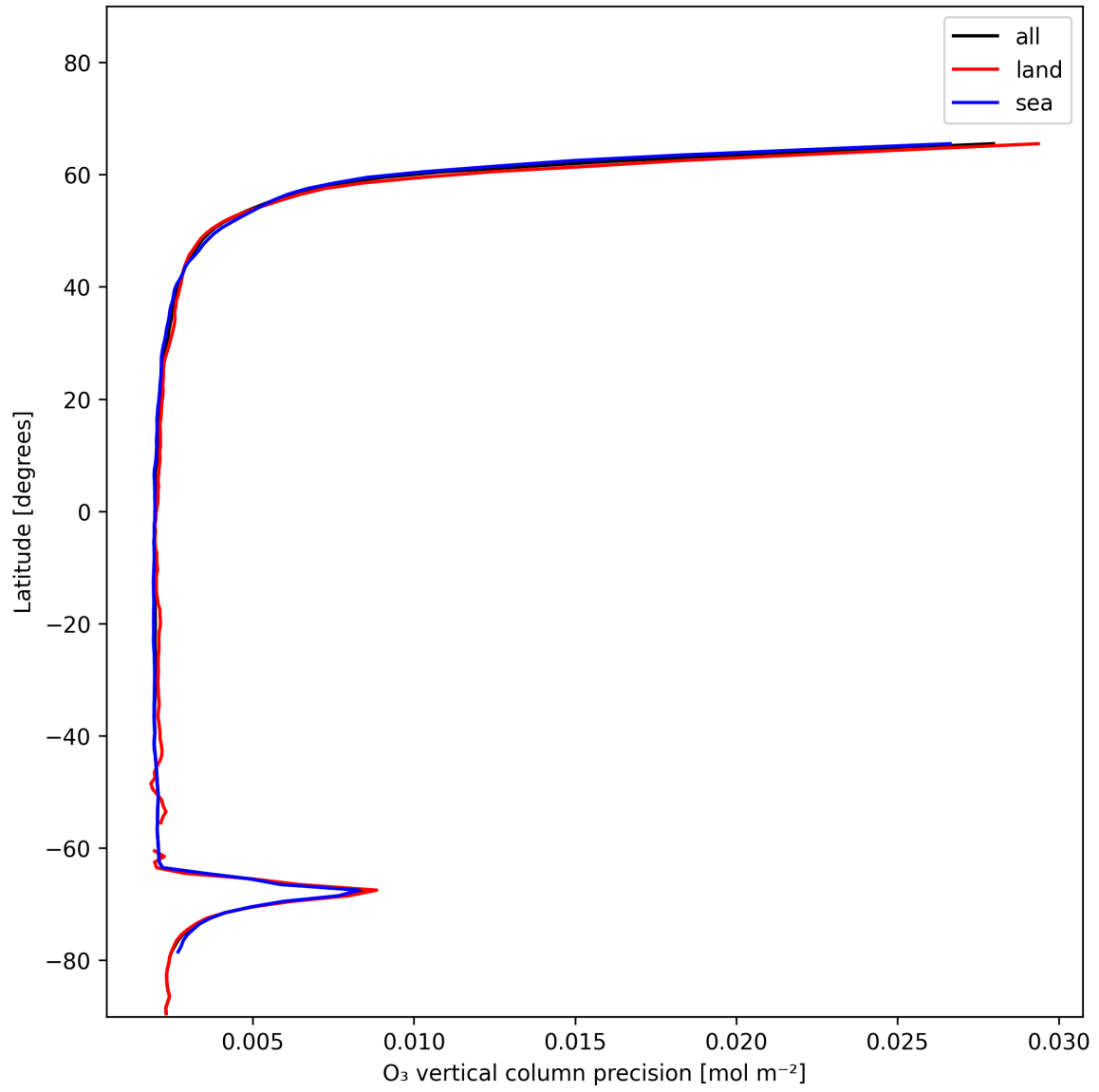
Figure 18: Zonal average of “O 3 vertical column precision” for 2024-12-17 to 2024-12-18.
