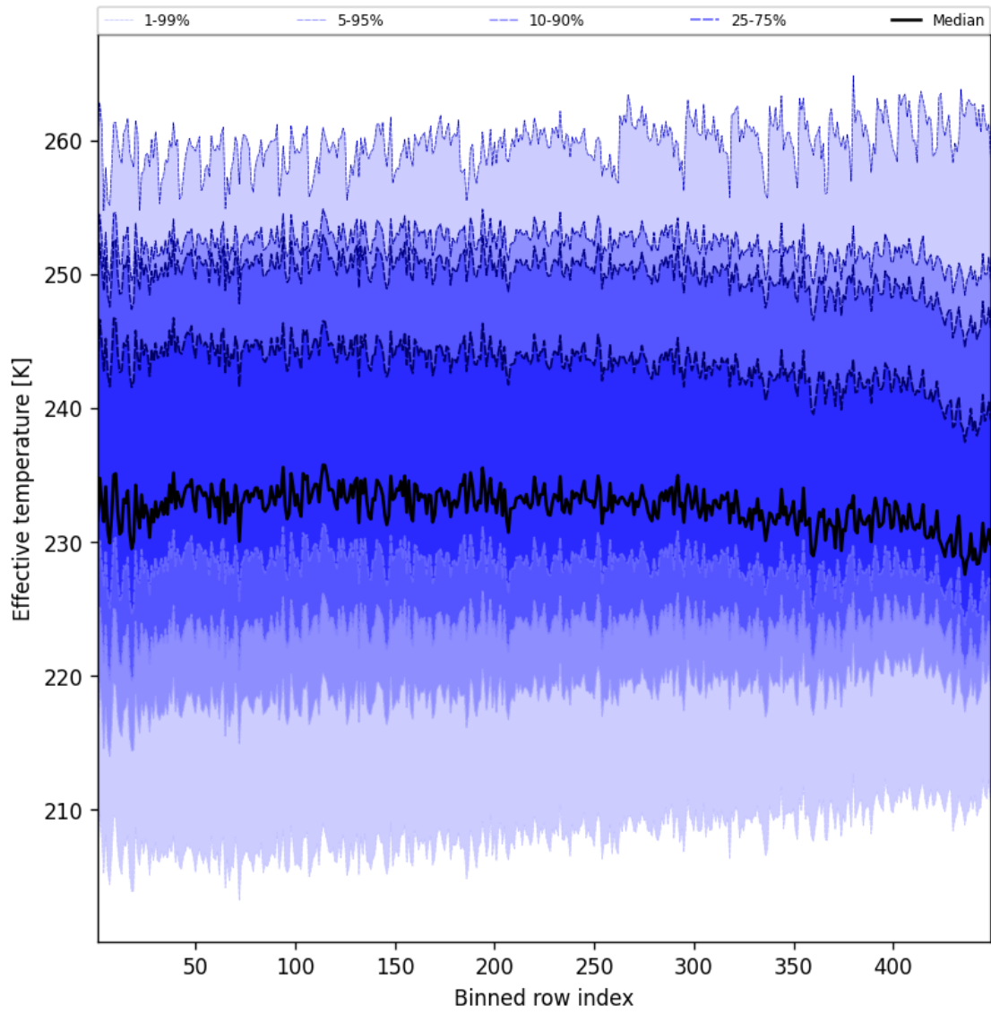
Figure 50: Along track statistics of “Effective temperature” for 2024-12-17 to 2024-12-18
