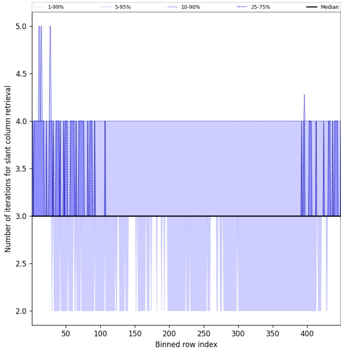
Figure 45: Along track statistics of “Number of iterations for slant column retrieval” for 2024-12-17 to 2024-12-18
