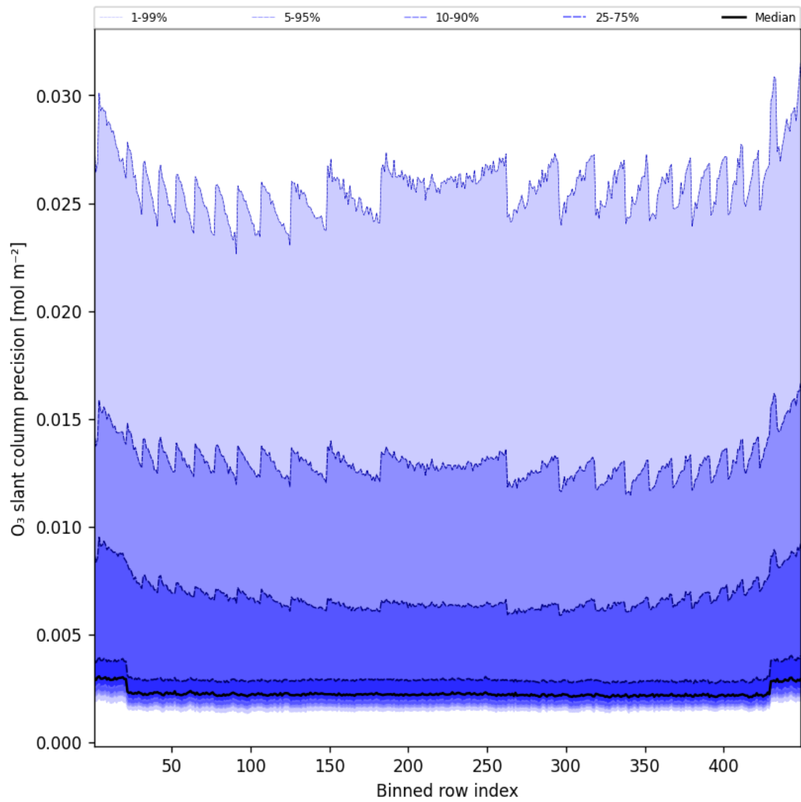
Figure 44: Along track statistics of “O 3 slant column precision” for 2024-12-17 to 2024-12-18
