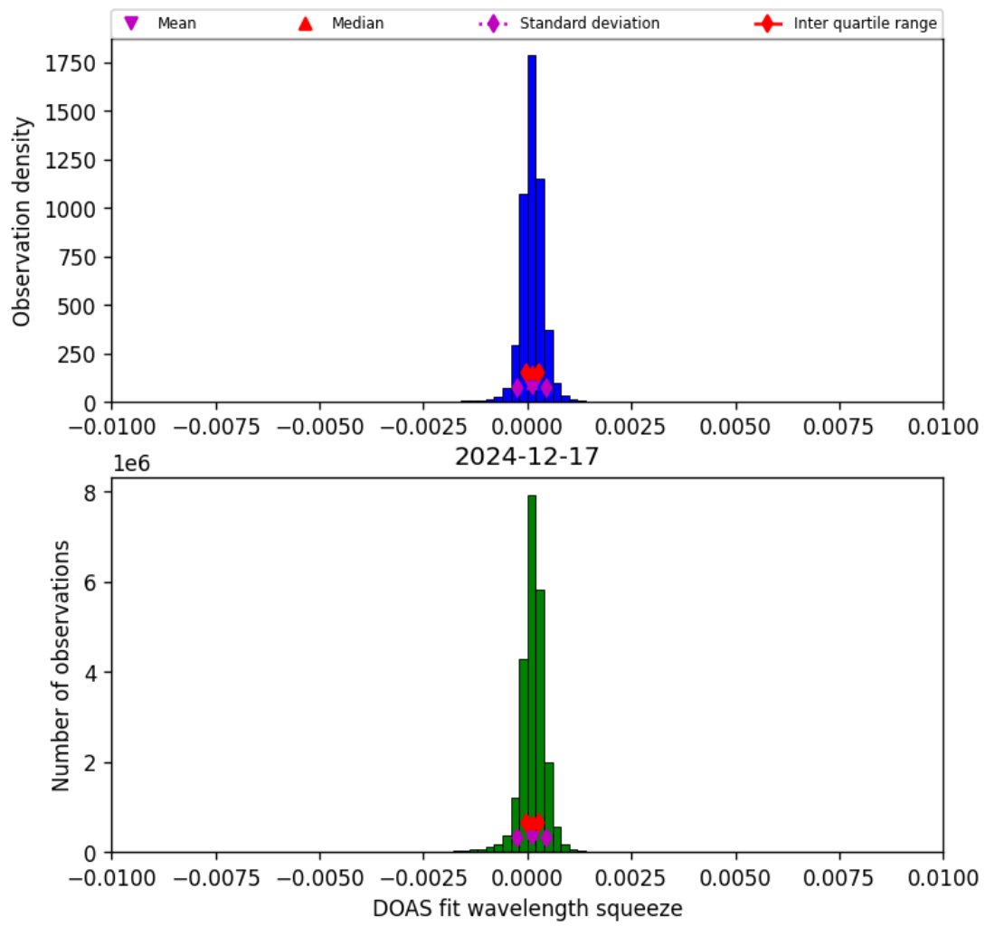
Figure 36: Histogram of “DOAS fit wavelength squeeze” for 2024-12-17 to 2024-12-18
