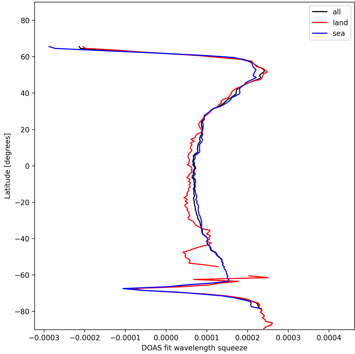
Figure 24: Zonal average of “DOAS fit wavelength squeeze” for 2024-12-17 to 2024-12-18.
