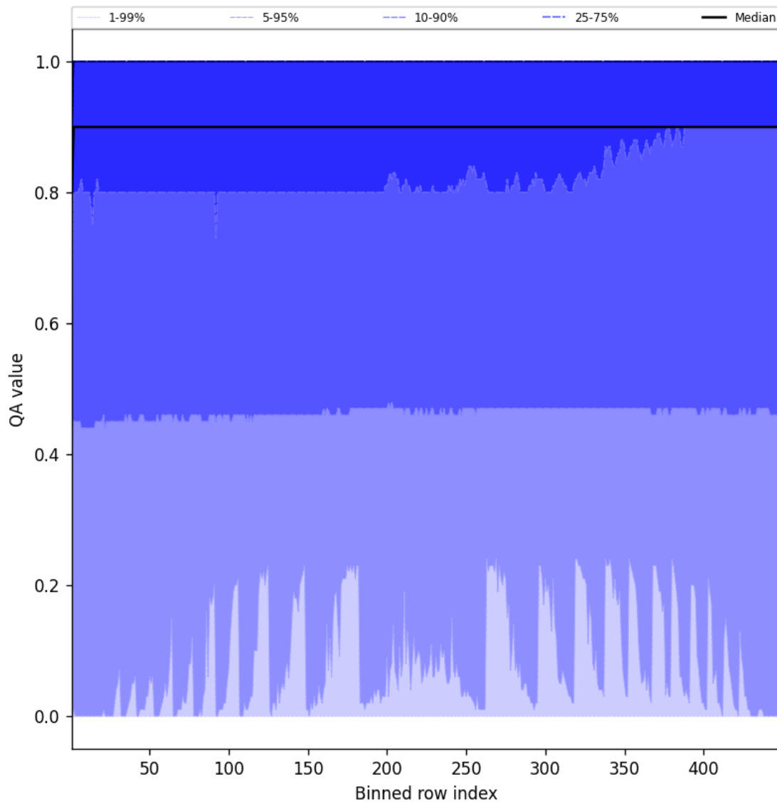
Figure 40: Along track statistics of “QA value” for 2024-12-17 to 2024-12-18
