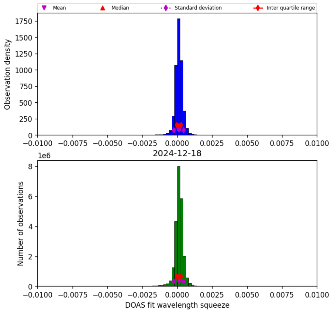
Figure 36: Histogram of “DOAS fit wavelength squeeze” for 2024-12-18 to 2024-12-19
