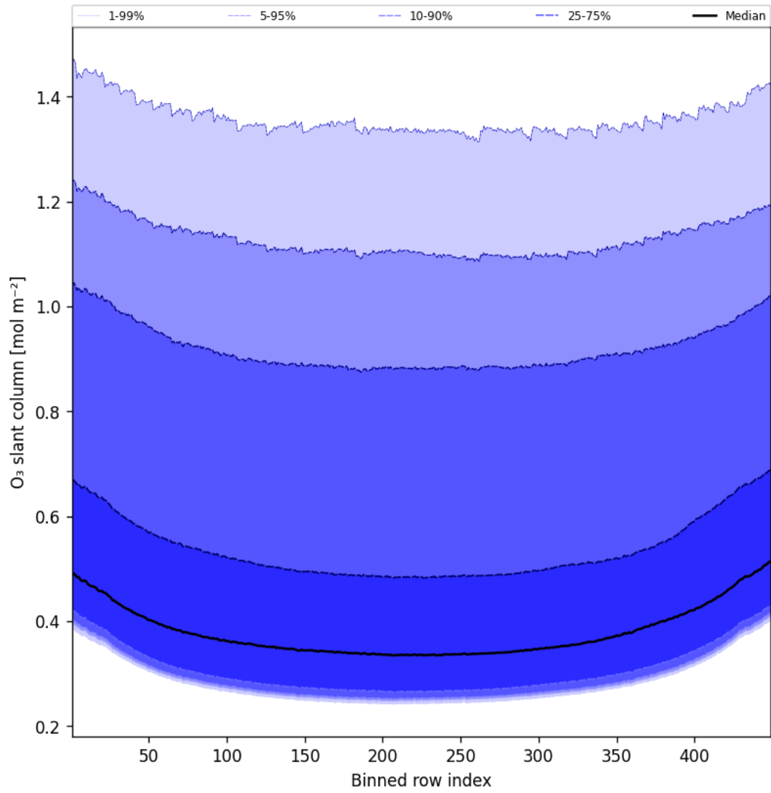
Figure 43: Along track statistics of “O 3 slant column” for 2024-12-18 to 2024-12-19
