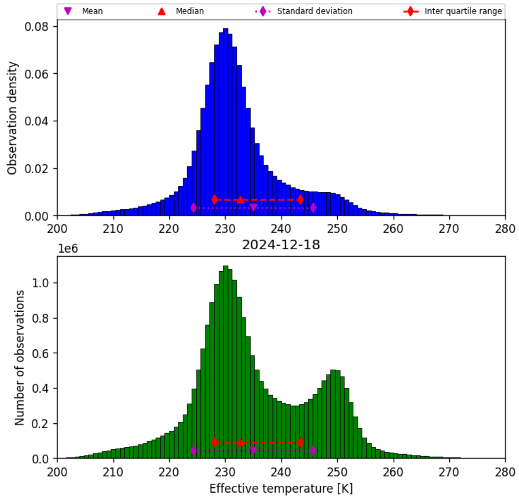
Figure 38: Histogram of “Effective temperature” for 2024-12-18 to 2024-12-19
