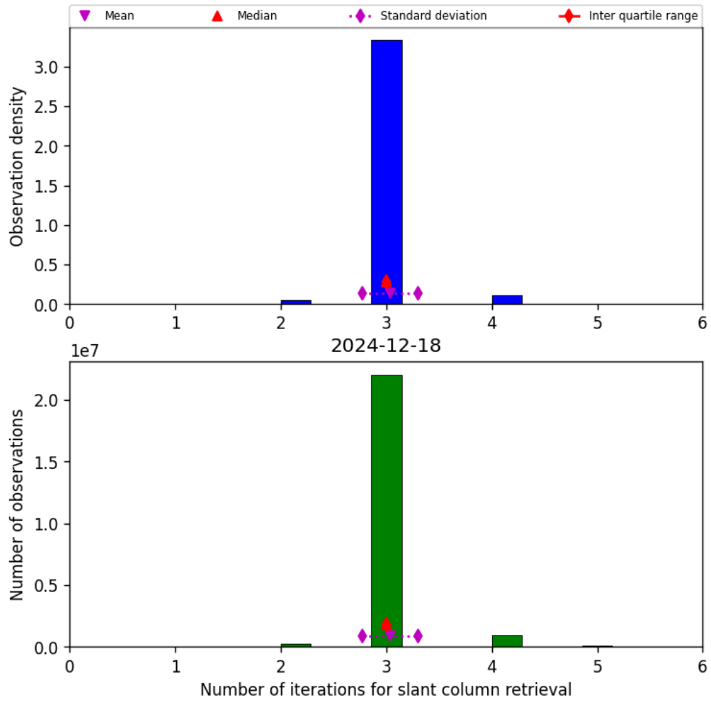
Figure 33: Histogram of “Number of iterations for slant column retrieval” for 2024-12-18 to 2024-12-19
