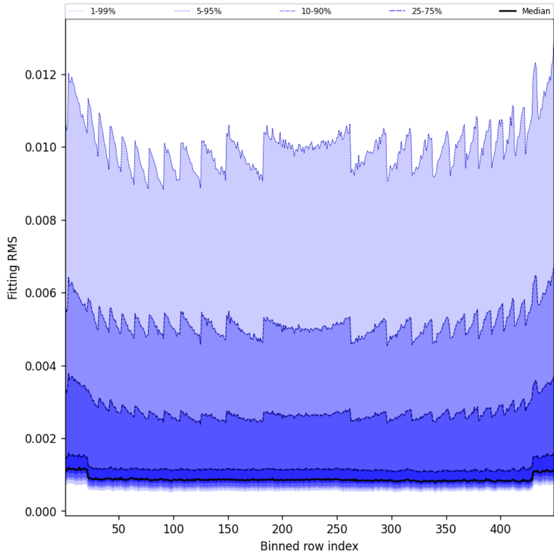
Figure 46: Along track statistics of “Fitting RMS” for 2024-12-18 to 2024-12-19
