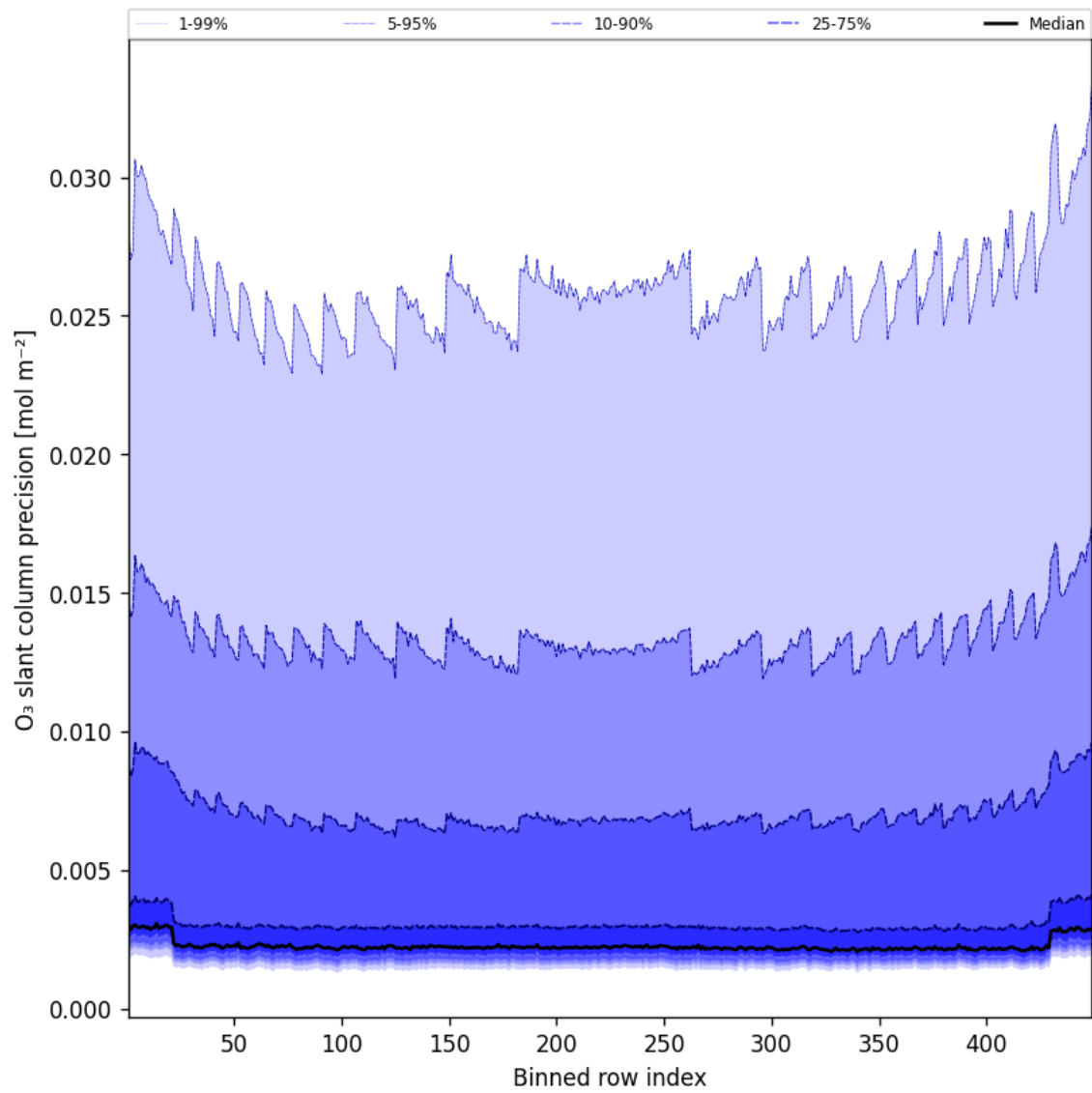
Figure 44: Along track statistics of “O 3 slant column precision” for 2024-12-18 to 2024-12-19
