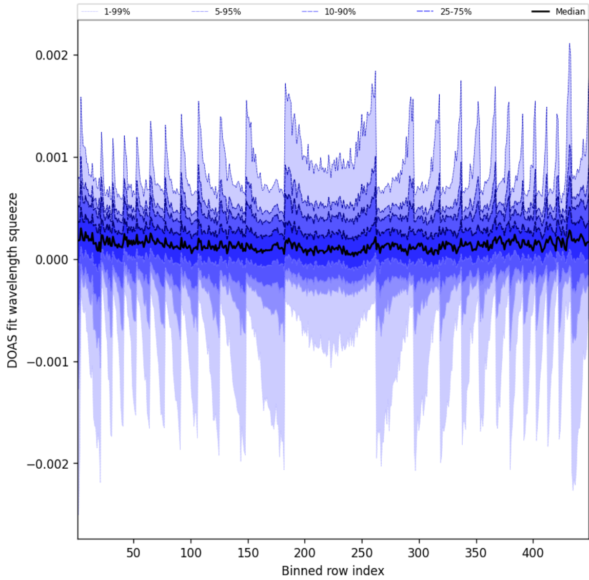
Figure 48: Along track statistics of “DOAS fit wavelength squeeze” for 2024-12-18 to 2024-12-19
