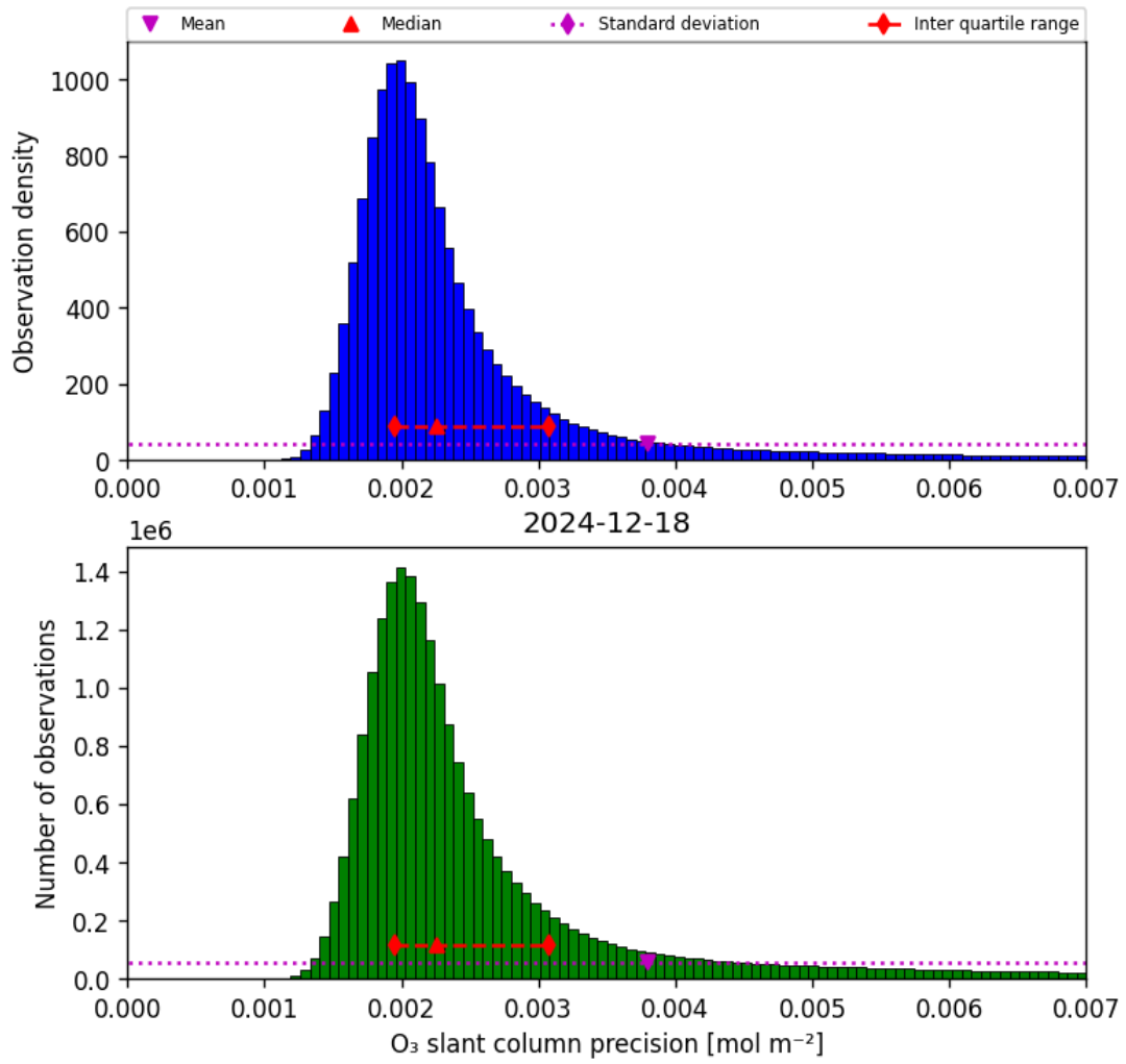
Figure 32: Histogram of “O 3 slant column precision” for 2024-12-18 to 2024-12-19
