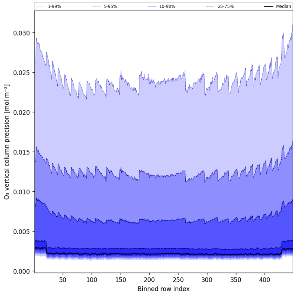
Figure 42: Along track statistics of “O 3 vertical column precision” for 2024-12-18 to 2024-12-19
