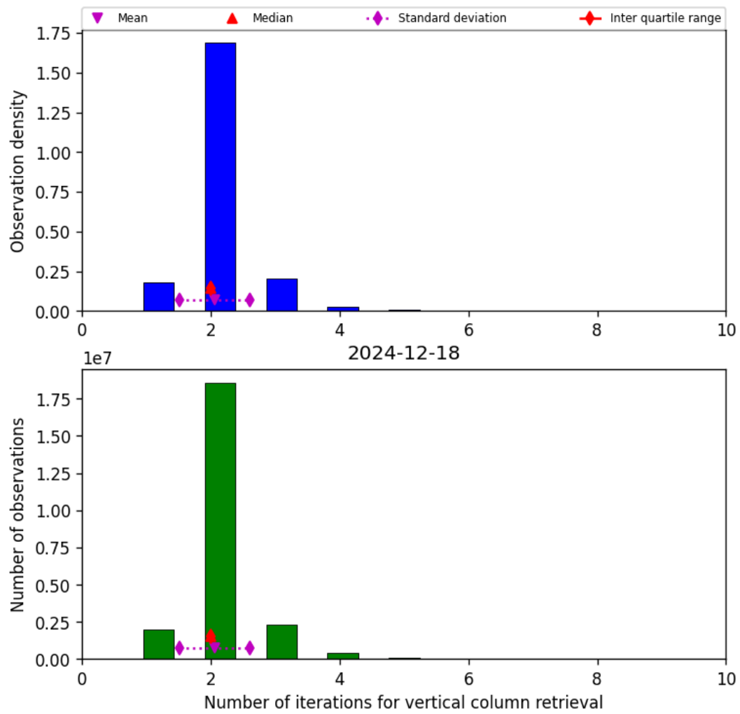
Figure 39: Histogram of “Number of iterations for vertical column retrieval” for 2024-12-18 to 2024-12-19
