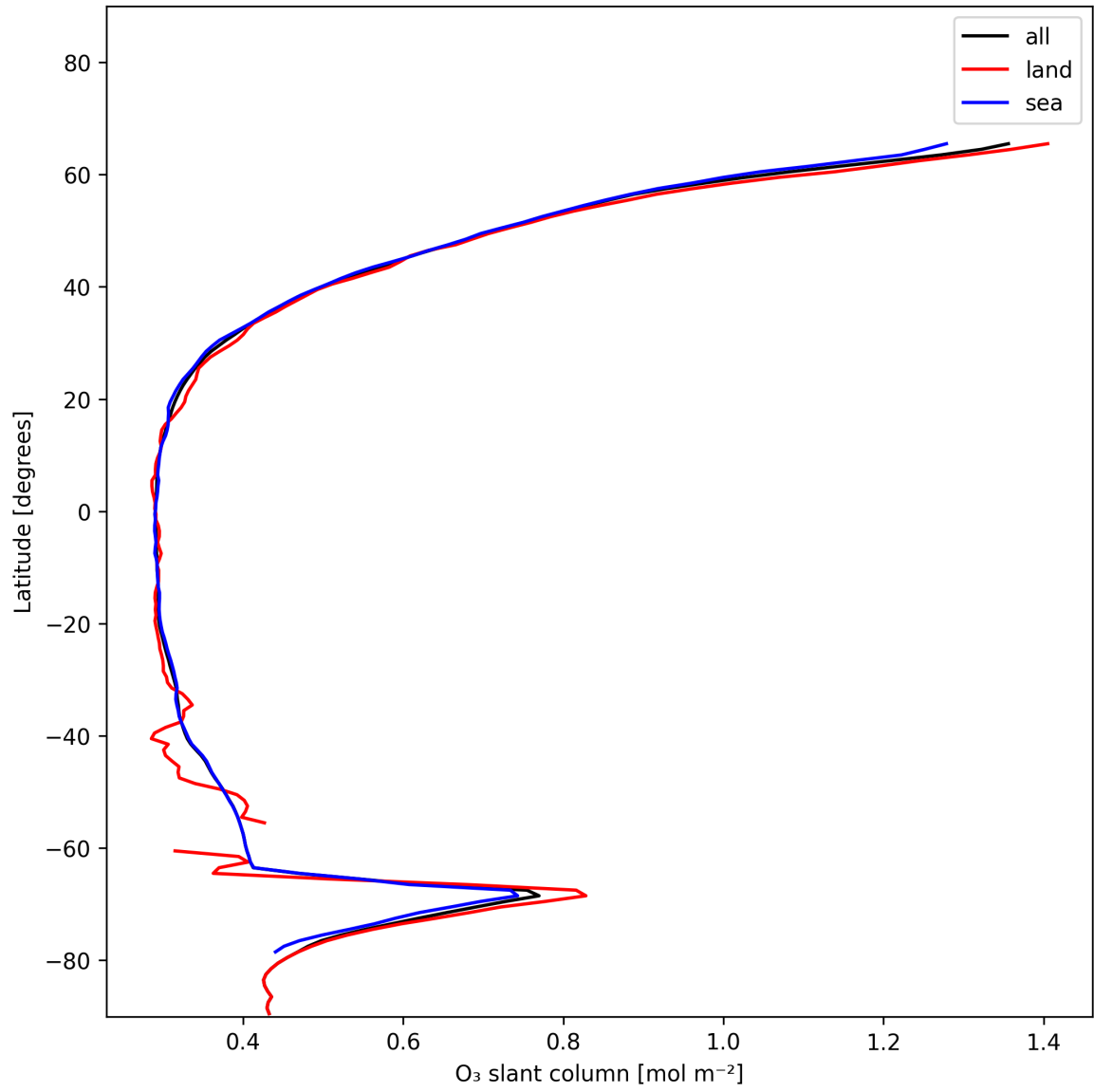
Figure 19: Zonal average of “O 3 slant column” for 2024-12-18 to 2024-12-19.
