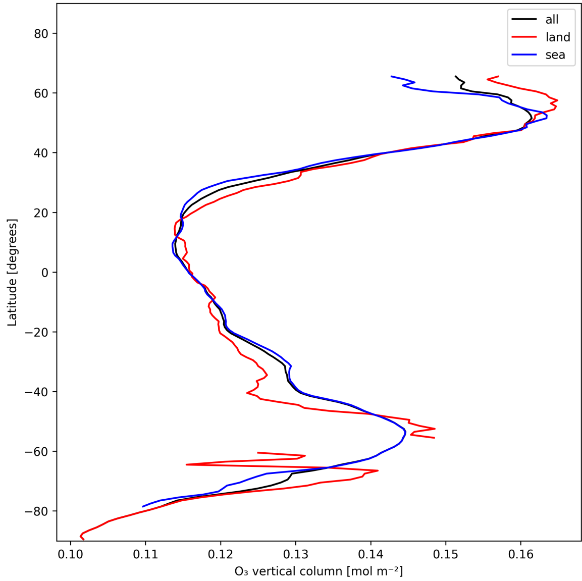
Figure 17: Zonal average of “O 3 vertical column” for 2024-12-18 to 2024-12-19.
