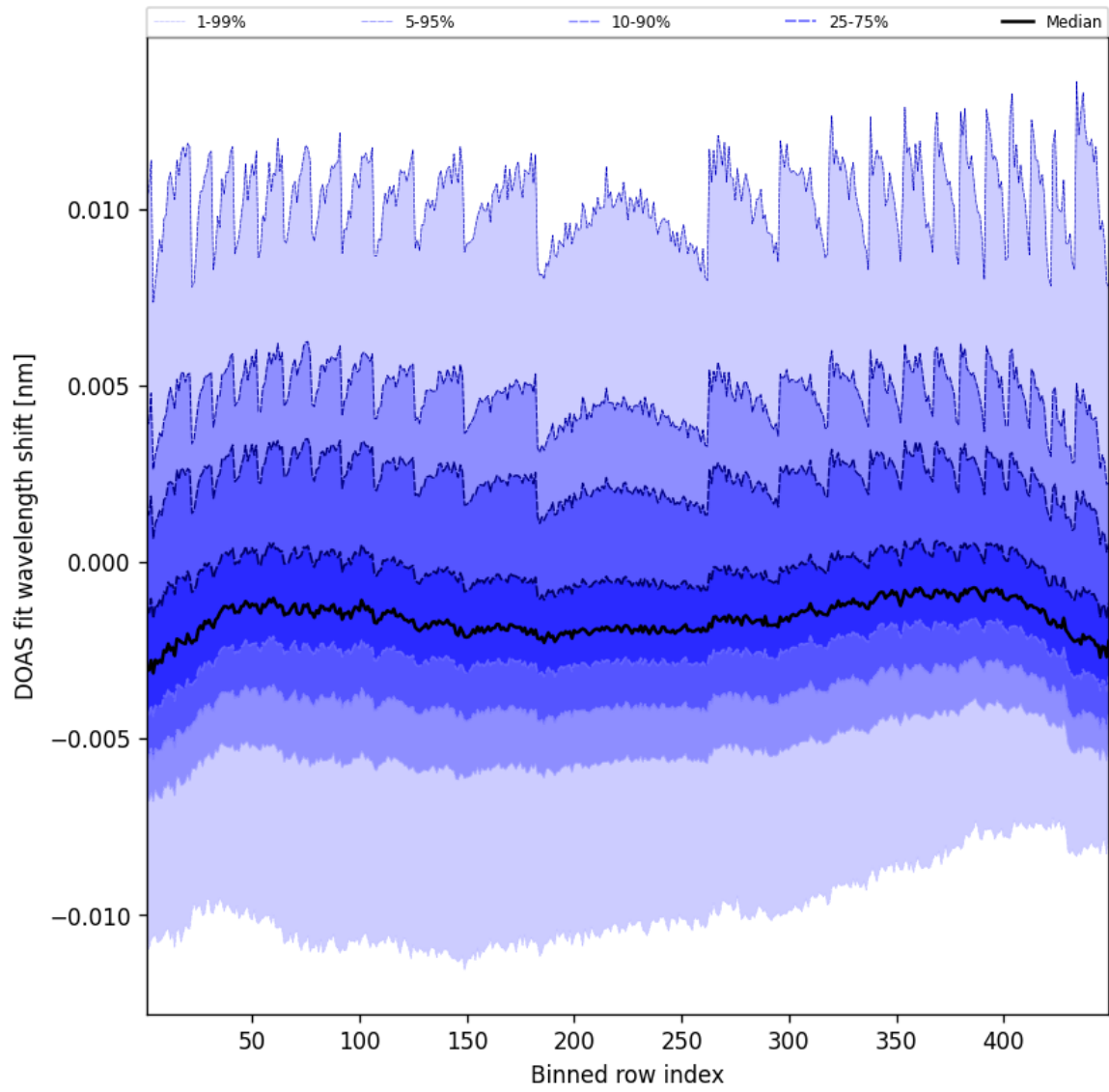
Figure 47: Along track statistics of “DOAS fit wavelength shift” for 2024-12-18 to 2024-12-19
