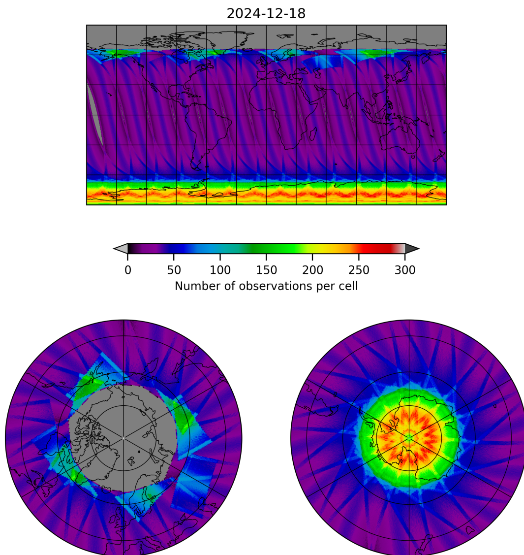
Figure 15: Map of the number of observations for 2024-12-18 to 2024-12-19
