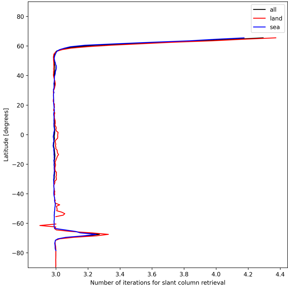
Figure 21: Zonal average of “Number of iterations for slant column retrieval” for 2024-12-18 to 2024-12-19.
