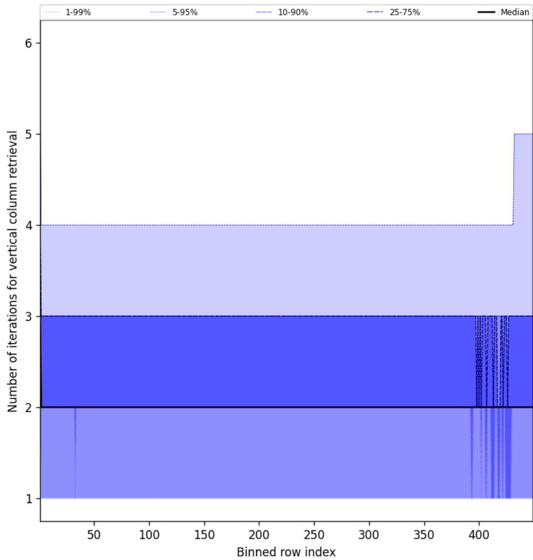
Figure 51: Along track statistics of “Number of iterations for vertical column retrieval” for 2024-12-18 to 2024-12-19
