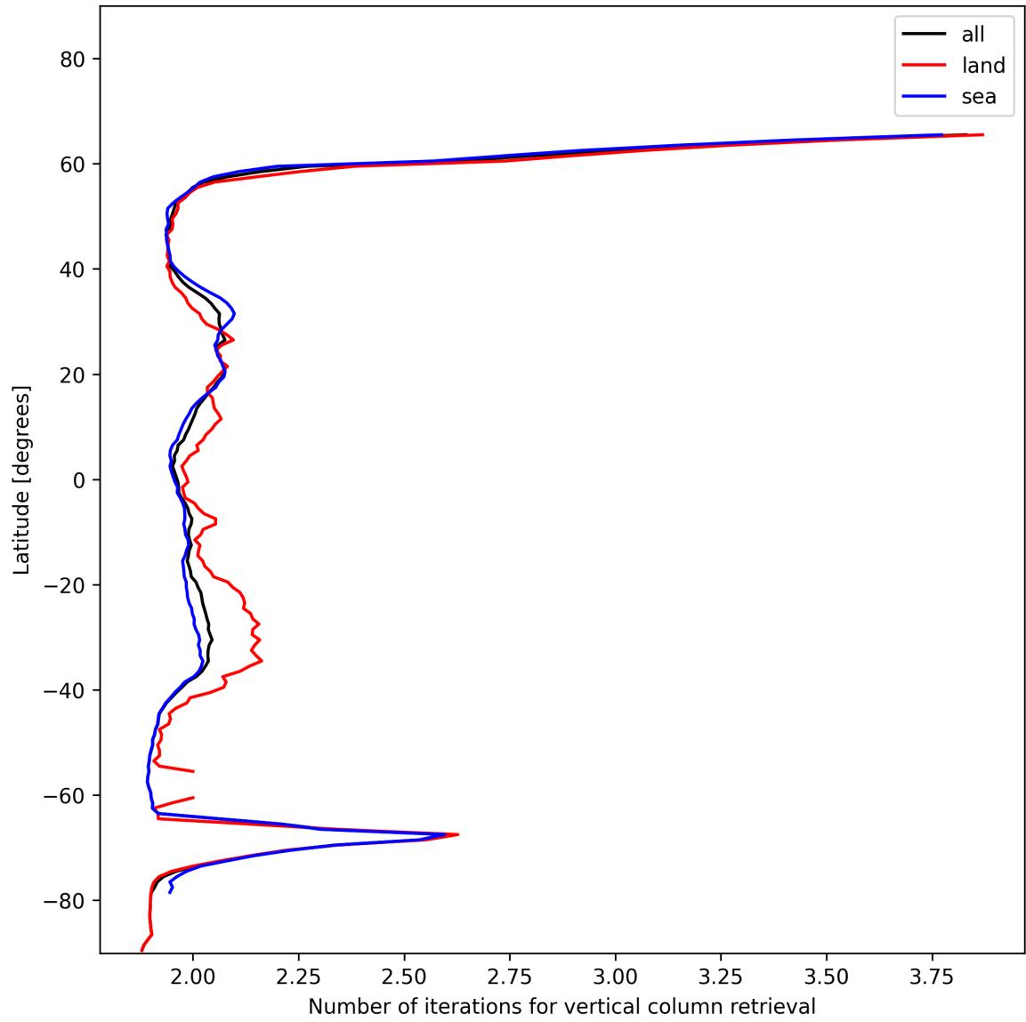
Figure 27: Zonal average of “Number of iterations for vertical column retrieval” for 2024-12-18 to 2024-12-19.
