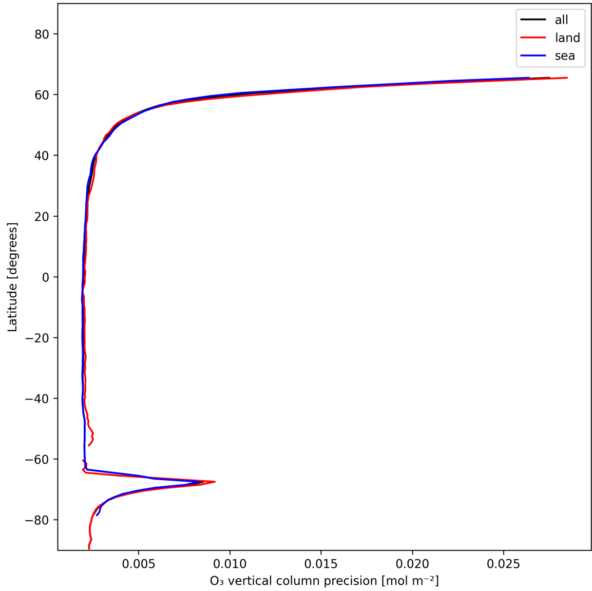
Figure 18: Zonal average of “O 3 vertical column precision” for 2024-12-18 to 2024-12-19.
