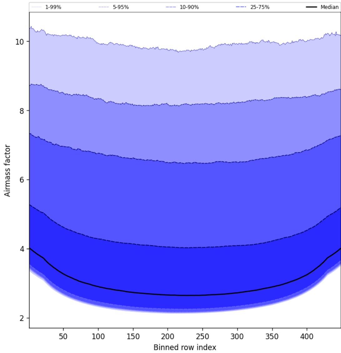
Figure 49: Along track statistics of “Airmass factor” for 2024-12-18 to 2024-12-19
