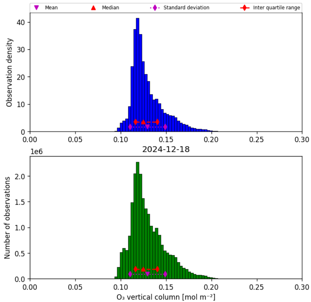
Figure 29: Histogram of “O 3 vertical column” for 2024-12-18 to 2024-12-19
