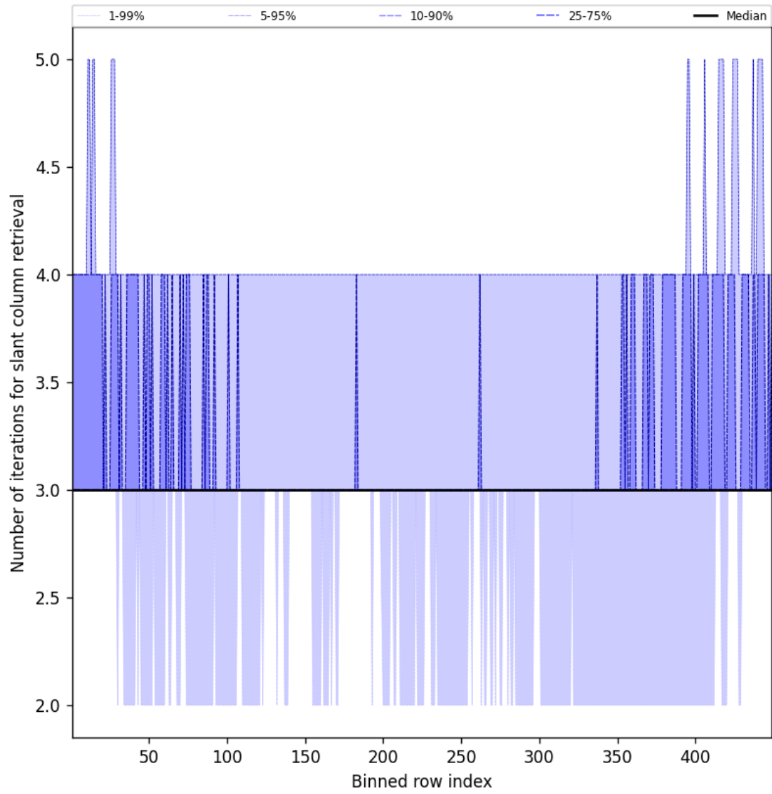
Figure 45: Along track statistics of “Number of iterations for slant column retrieval” for 2024-12-18 to 2024-12-19
