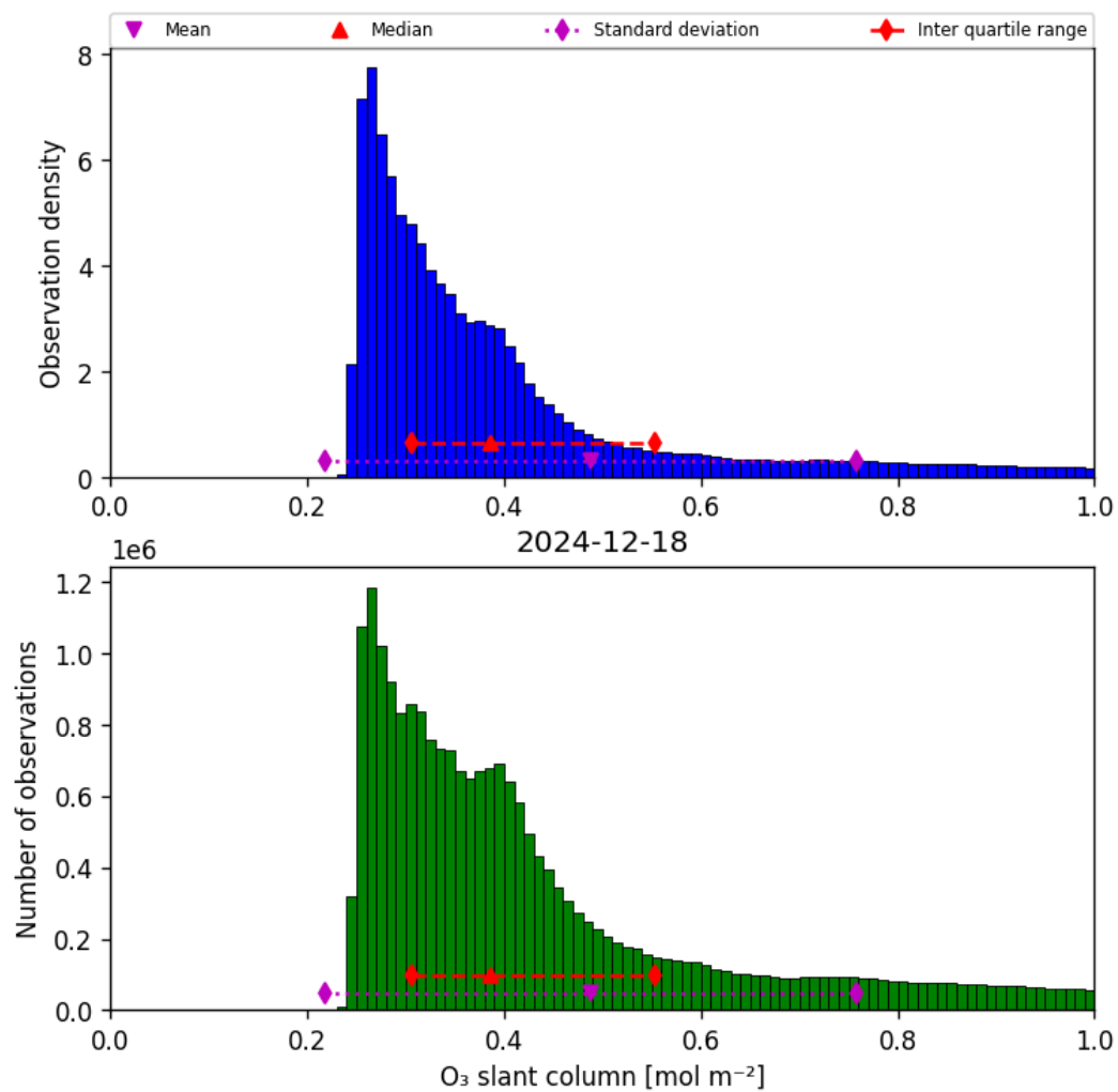
Figure 31: Histogram of “O 3 slant column” for 2024-12-18 to 2024-12-19
