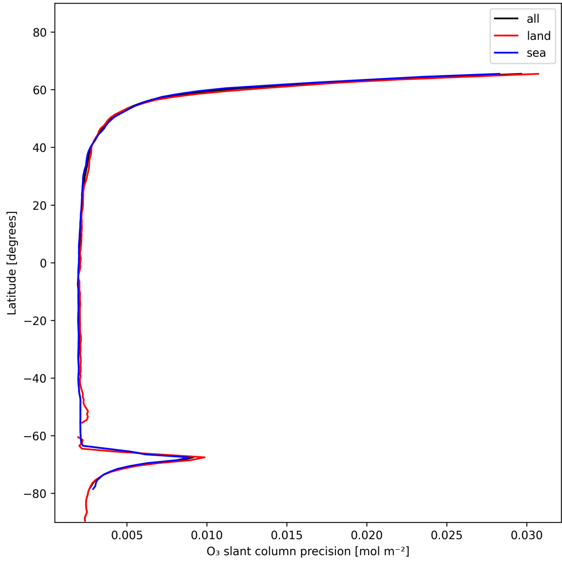
Figure 20: Zonal average of “O 3 slant column precision” for 2024-12-18 to 2024-12-19.
