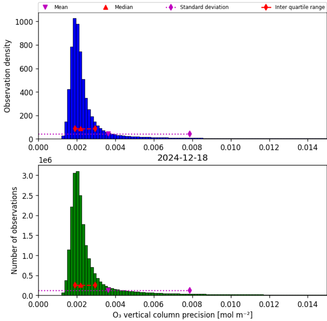
Figure 30: Histogram of “O 3 vertical column precision” for 2024-12-18 to 2024-12-19
