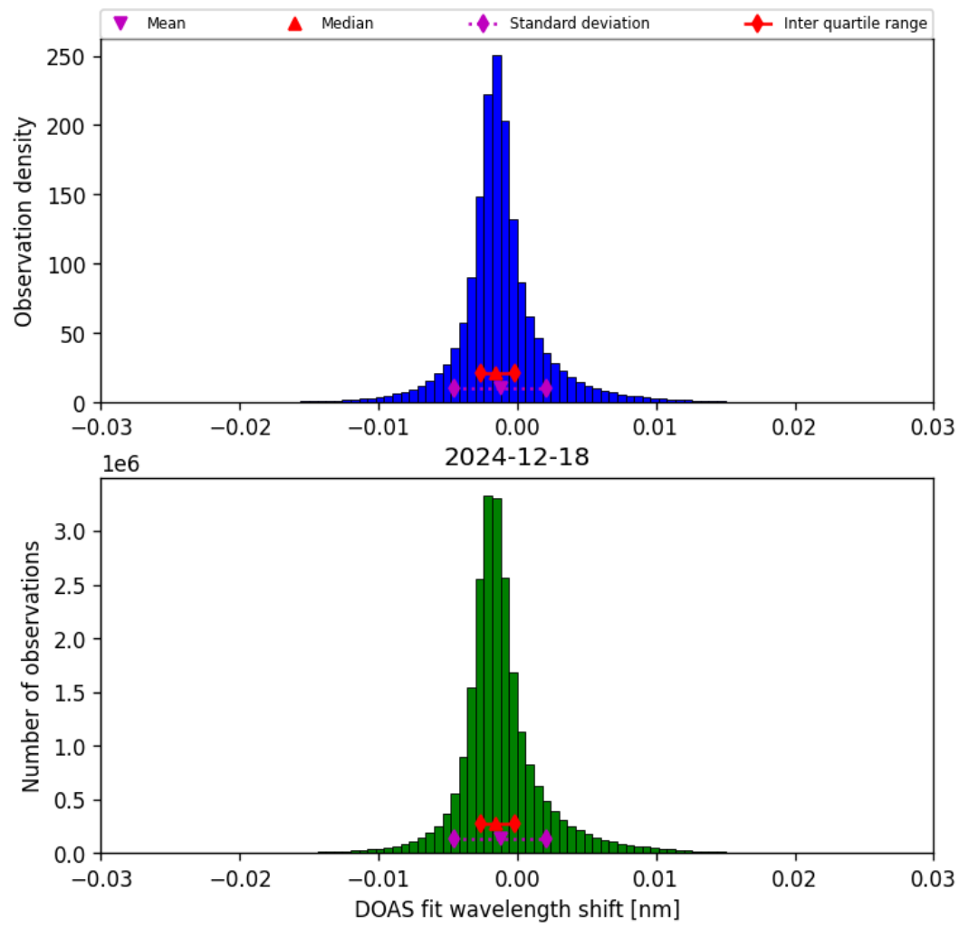
Figure 35: Histogram of “DOAS fit wavelength shift” for 2024-12-18 to 2024-12-19
