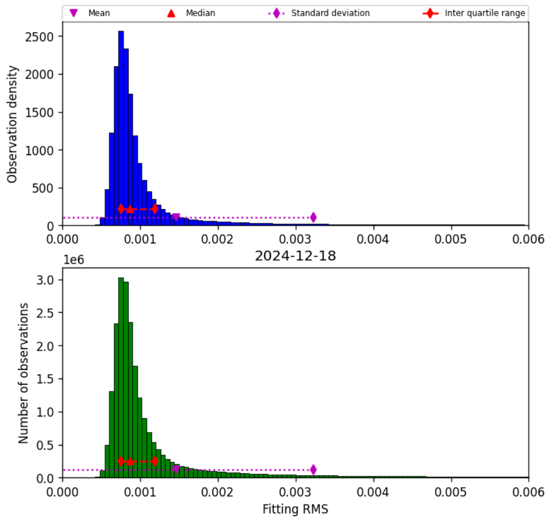
Figure 34: Histogram of “Fitting RMS” for 2024-12-18 to 2024-12-19
