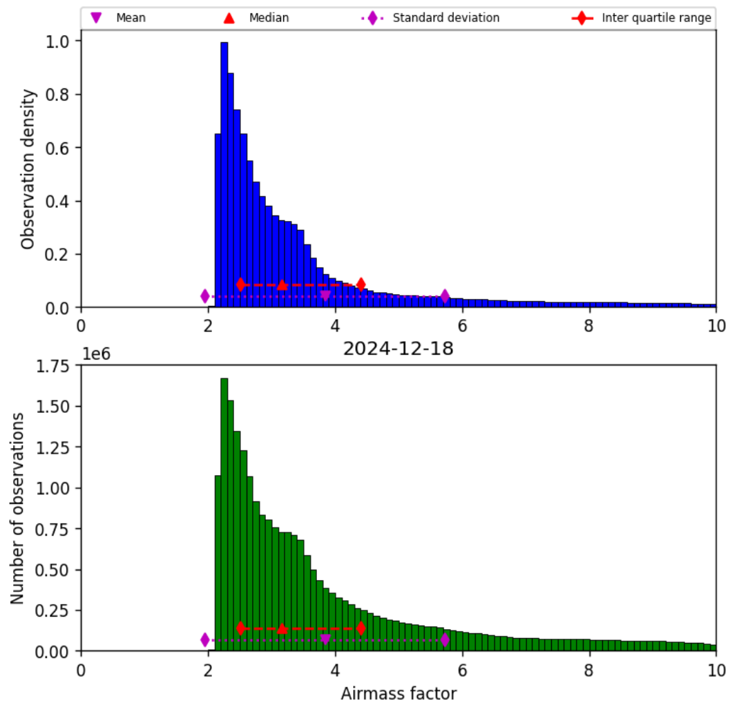
Figure 37: Histogram of “Airmass factor” for 2024-12-18 to 2024-12-19
