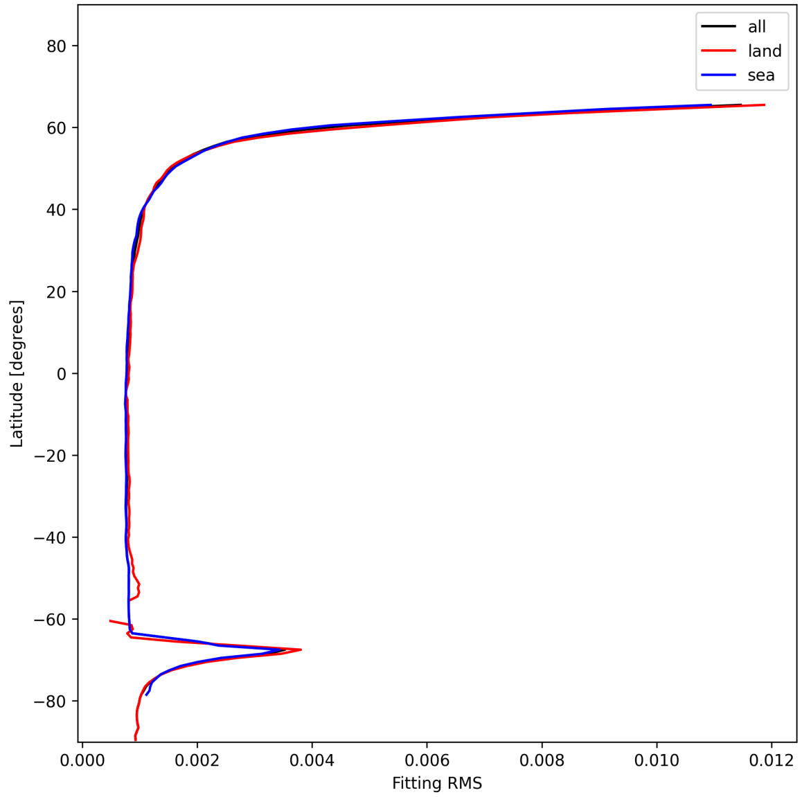
Figure 22: Zonal average of “Fitting RMS” for 2024-12-18 to 2024-12-19.
