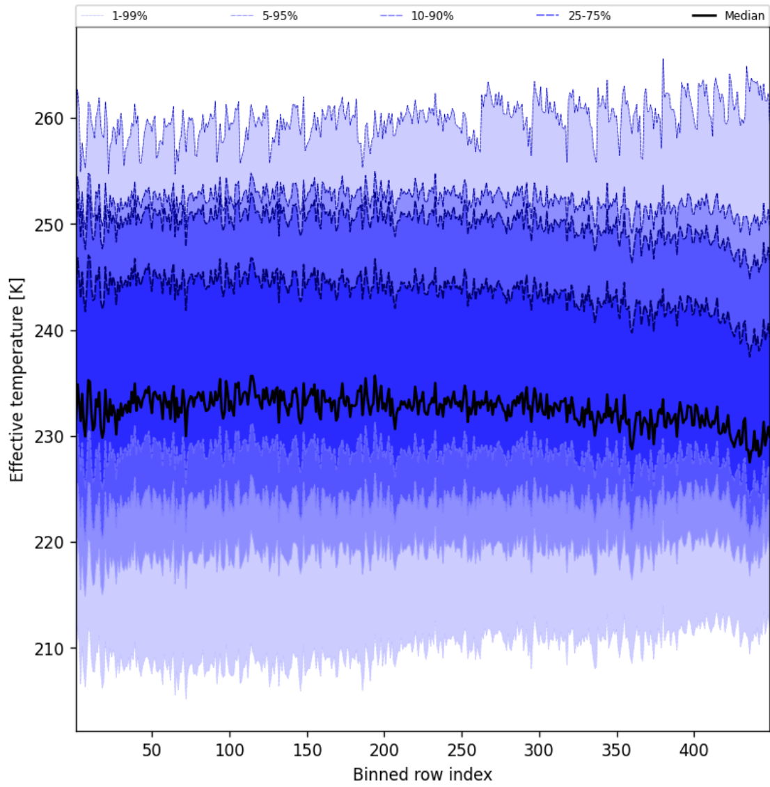
Figure 50: Along track statistics of “Effective temperature” for 2024-12-18 to 2024-12-19
