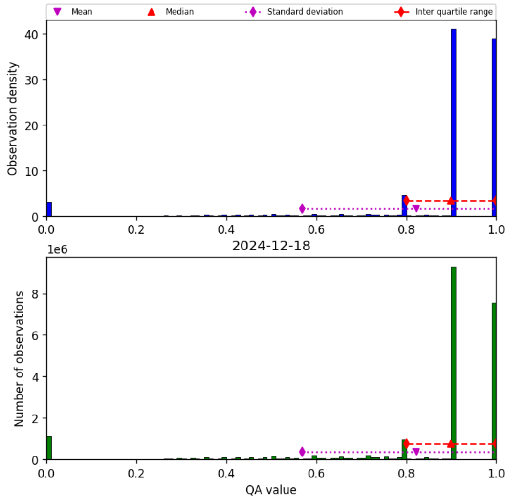
Figure 28: Histogram of “QA value” for 2024-12-18 to 2024-12-19
