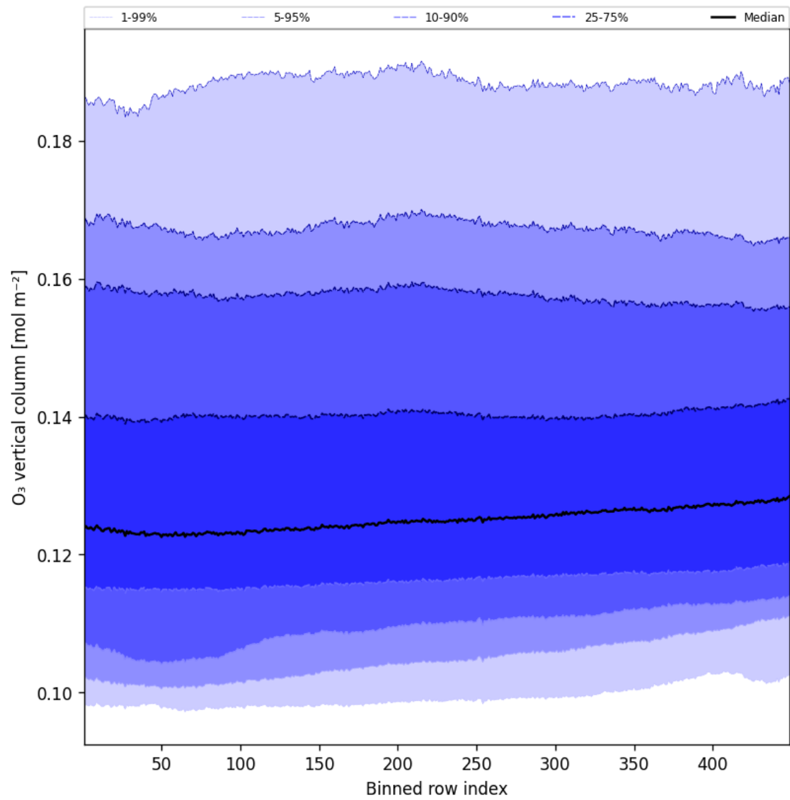
Figure 41: Along track statistics of “O 3 vertical column” for 2024-12-18 to 2024-12-19
