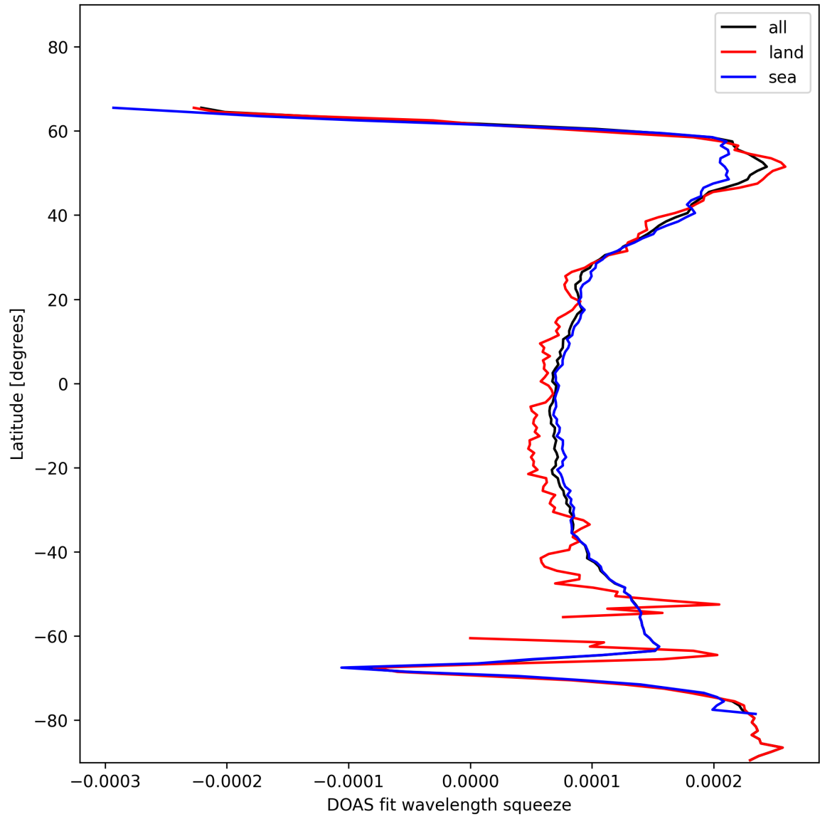
Figure 24: Zonal average of “DOAS fit wavelength squeeze” for 2024-12-18 to 2024-12-19.
