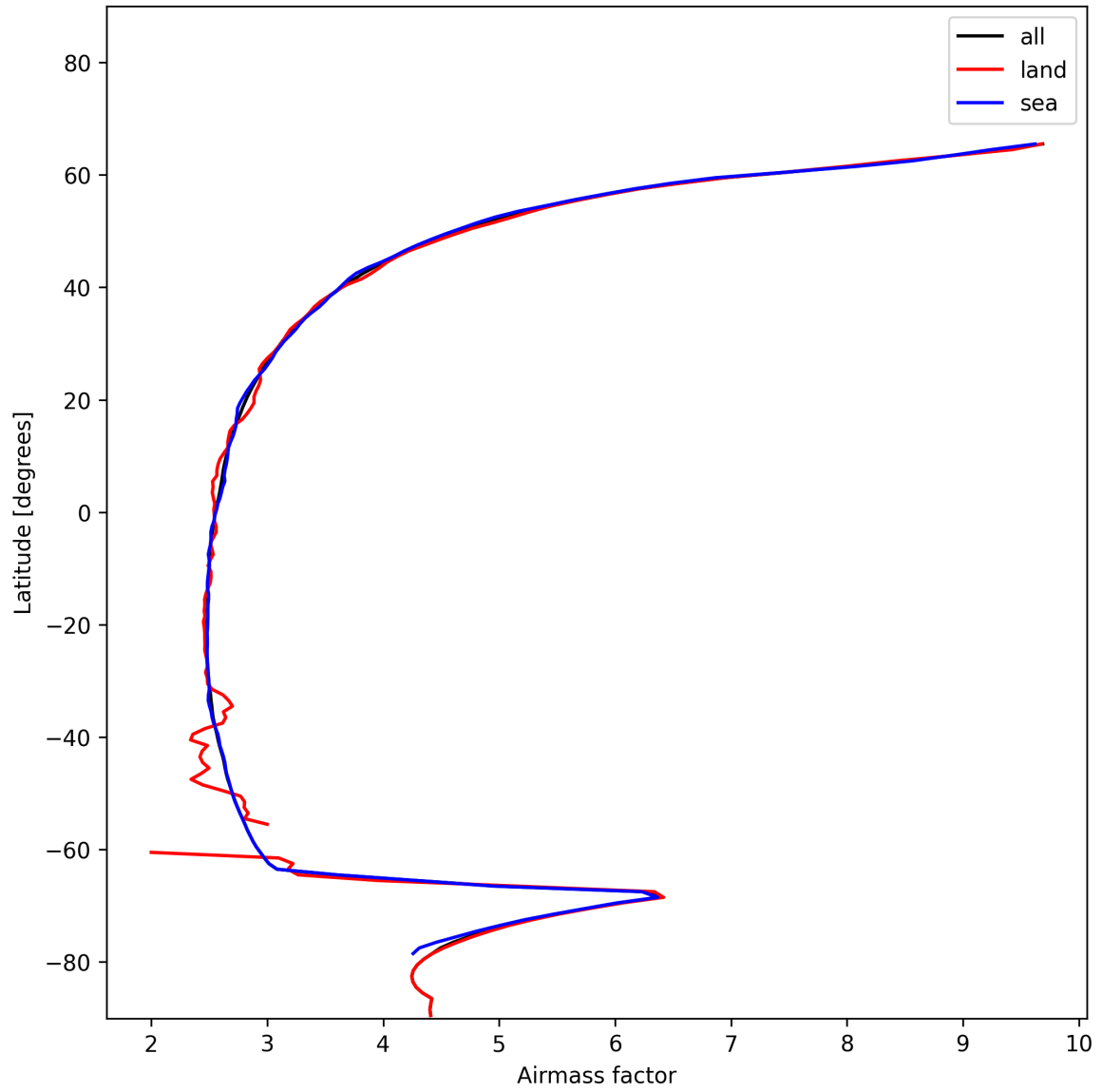
Figure 25: Zonal average of “Airmass factor” for 2024-12-18 to 2024-12-19.
