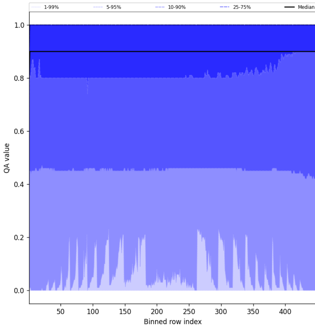
Figure 40: Along track statistics of “QA value” for 2024-12-18 to 2024-12-19
