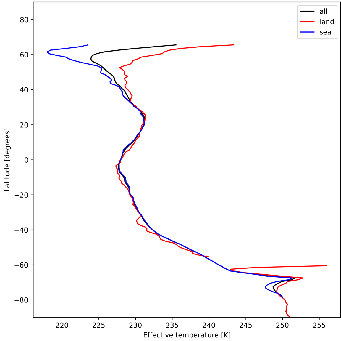
Figure 26: Zonal average of “Effective temperature” for 2024-12-18 to 2024-12-19.
