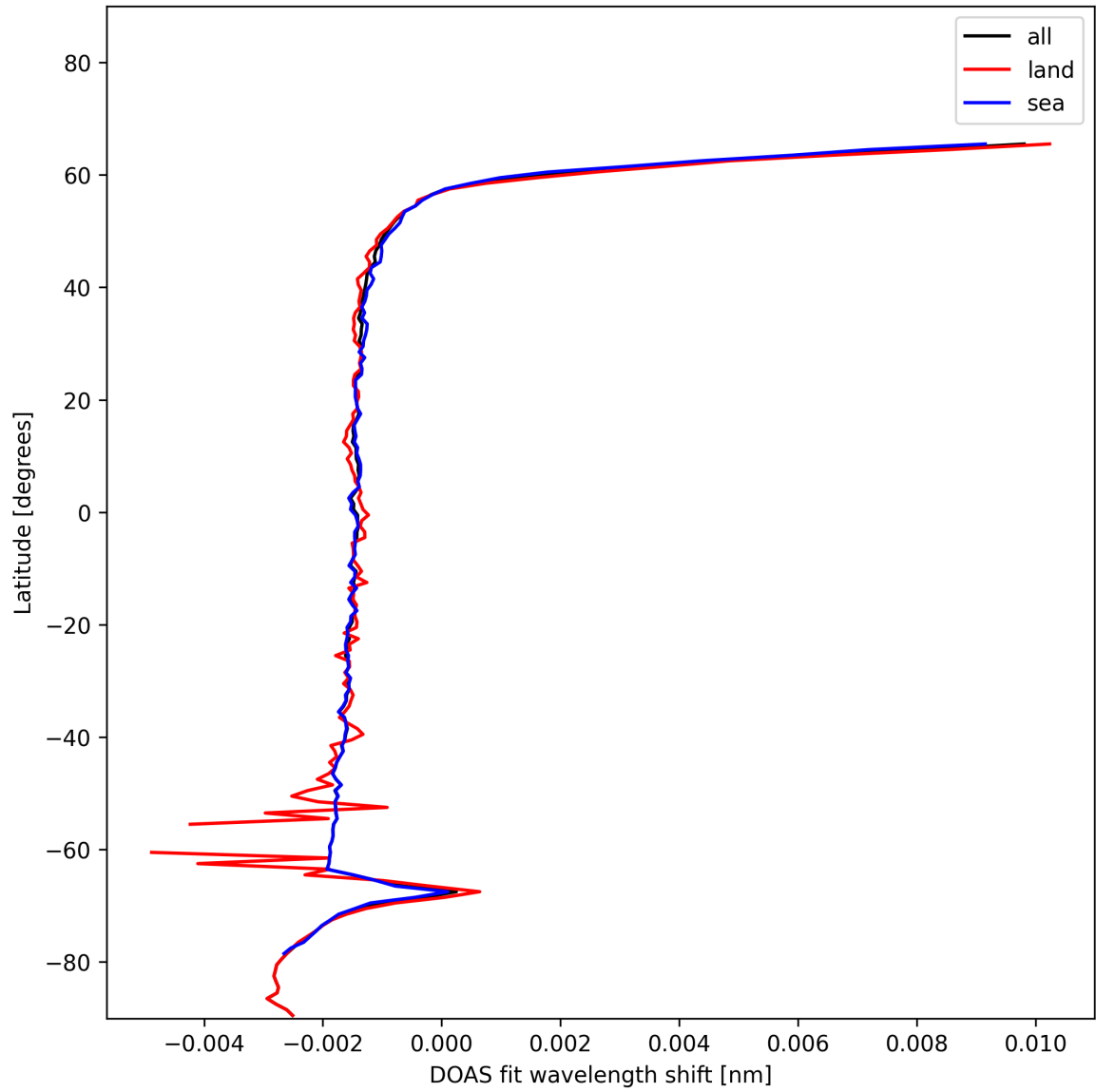
Figure 23: Zonal average of “DOAS fit wavelength shift” for 2024-12-18 to 2024-12-19.
