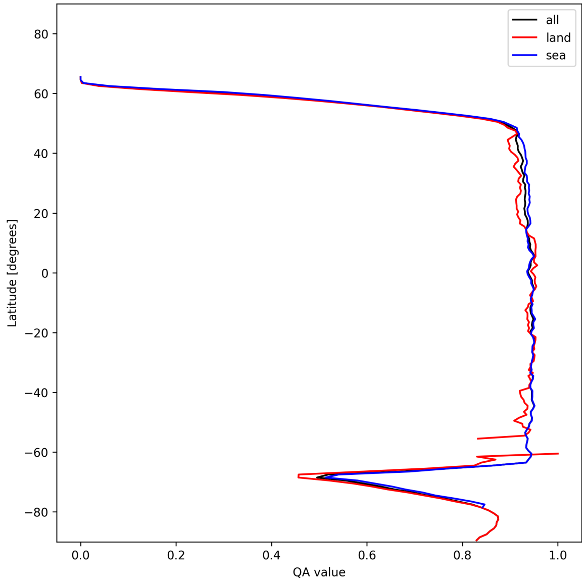
Figure 16: Zonal average of “QA value” for 2024-12-18 to 2024-12-19.
