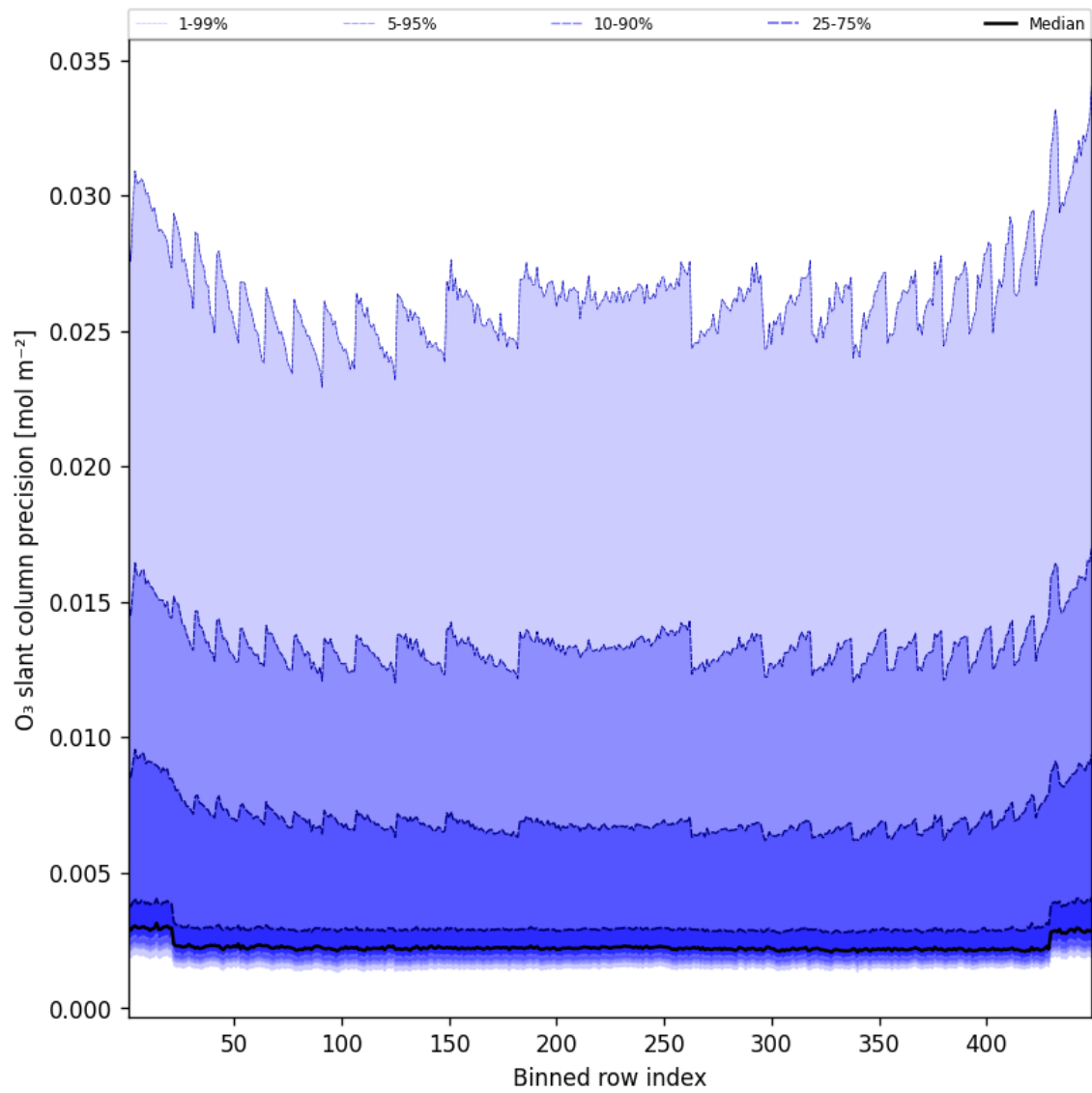
Figure 44: Along track statistics of “O 3 slant column precision” for 2024-12-19 to 2024-12-19
