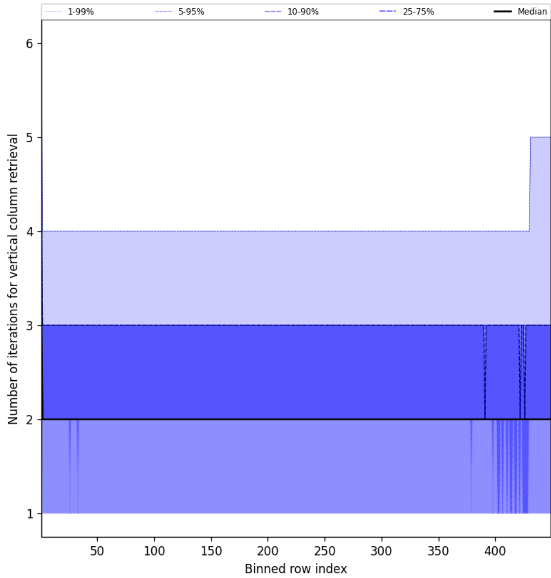
Figure 51: Along track statistics of “Number of iterations for vertical column retrieval” for 2024-12-19 to 2024-12-19
