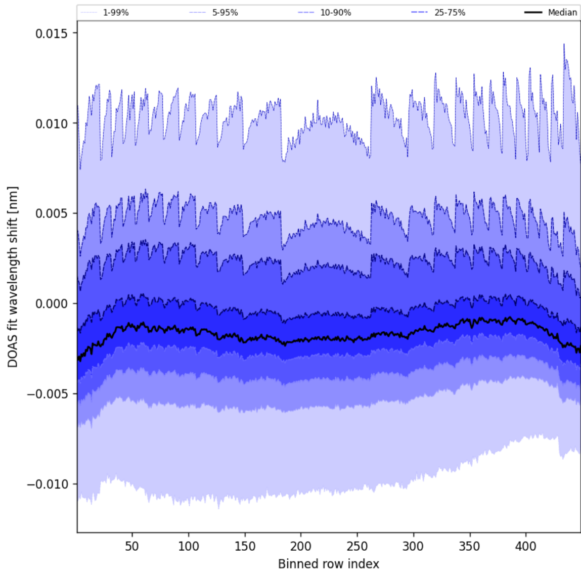
Figure 47: Along track statistics of “DOAS fit wavelength shift” for 2024-12-19 to 2024-12-19
