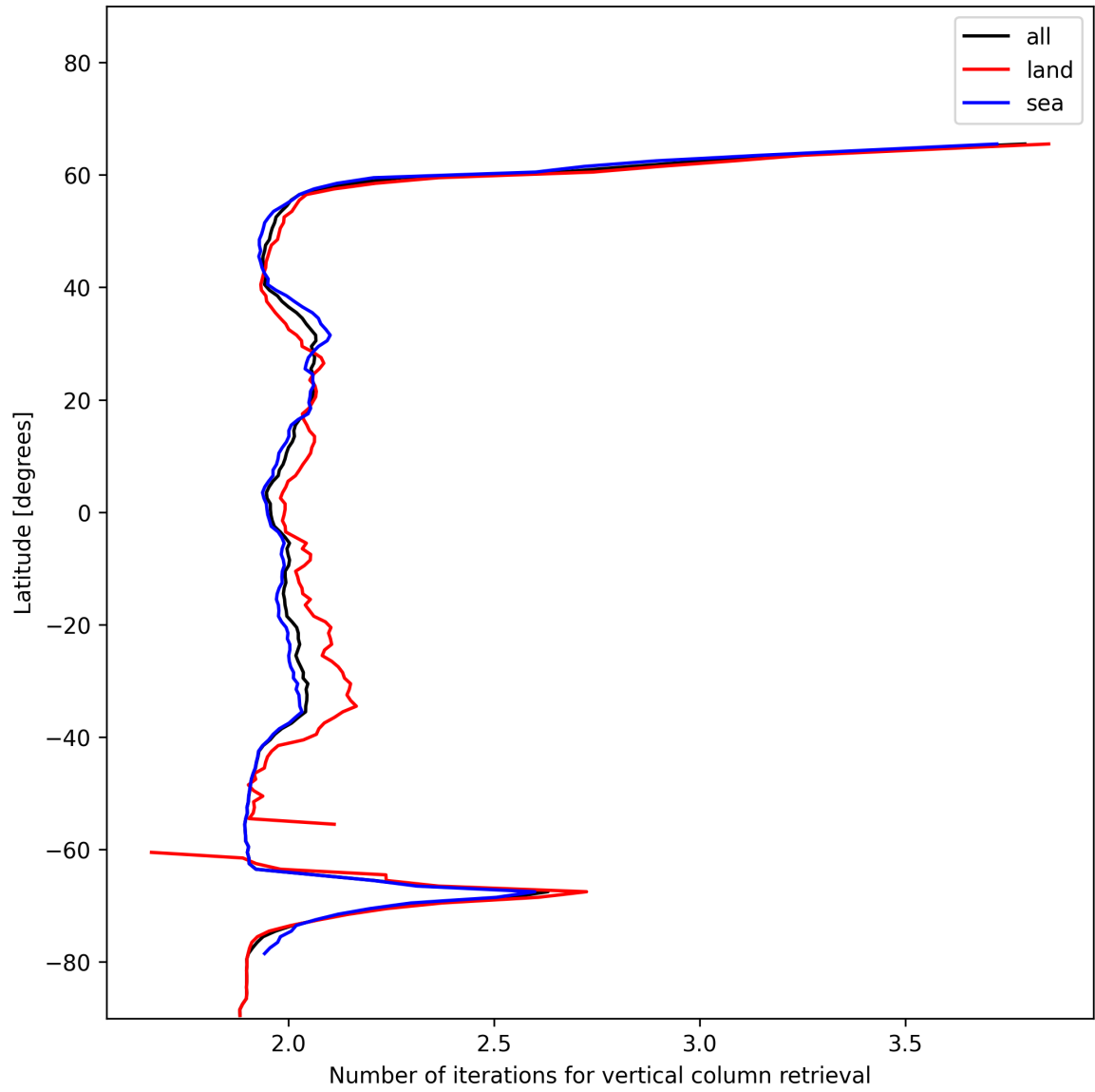
Figure 27: Zonal average of “Number of iterations for vertical column retrieval” for 2024-12-19 to 2024-12-19.
