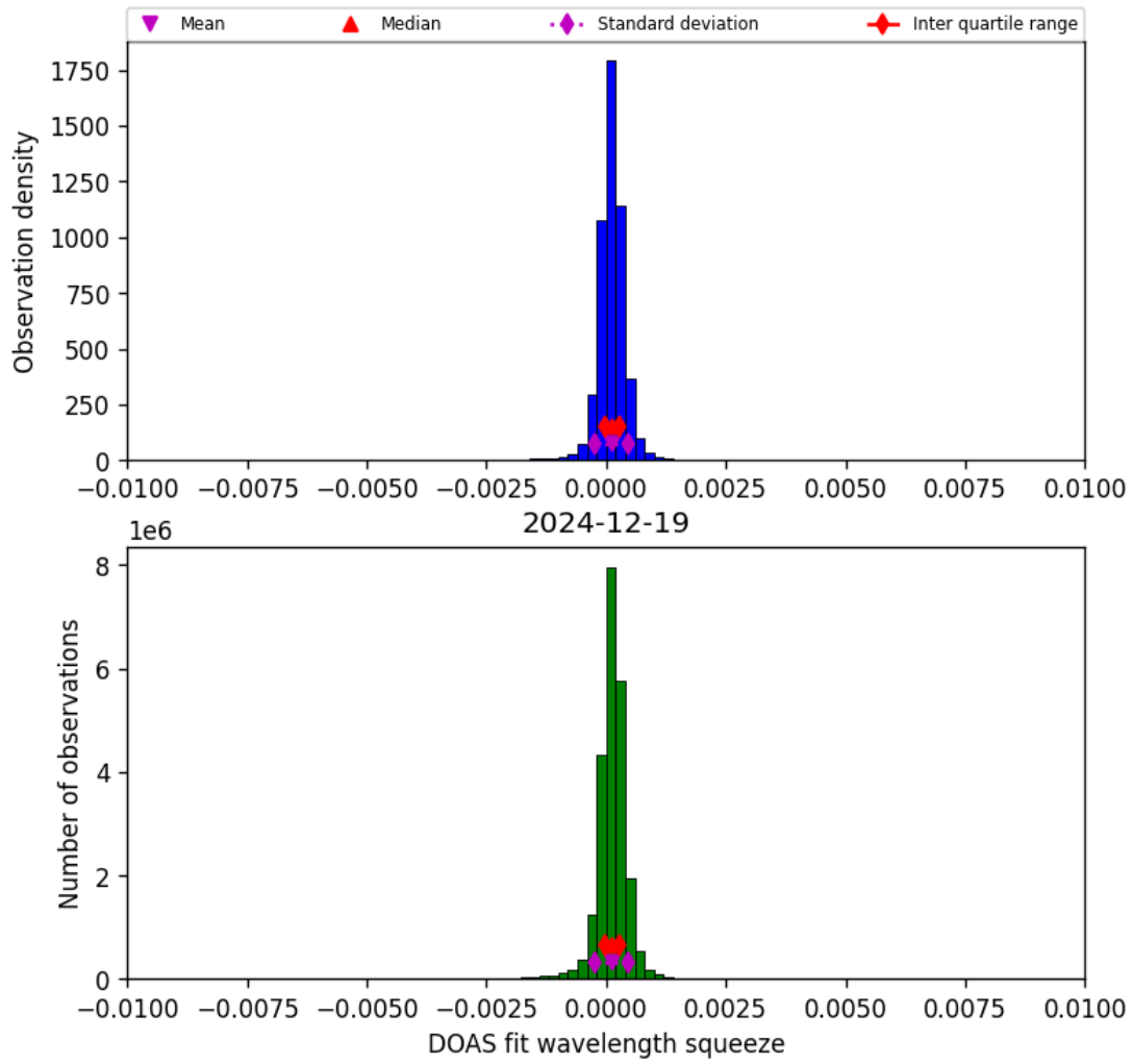
Figure 36: Histogram of “DOAS fit wavelength squeeze” for 2024-12-19 to 2024-12-19
