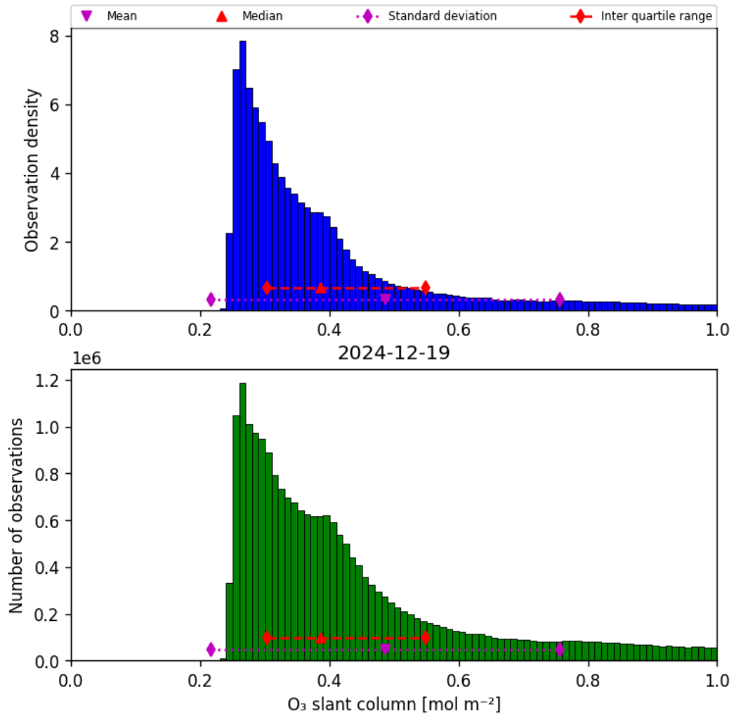
Figure 31: Histogram of “O 3 slant column” for 2024-12-19 to 2024-12-19
