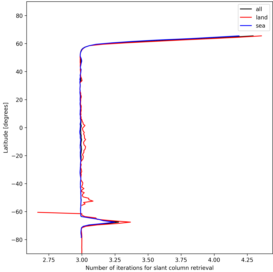
Figure 21: Zonal average of “Number of iterations for slant column retrieval” for 2024-12-19 to 2024-12-19.
