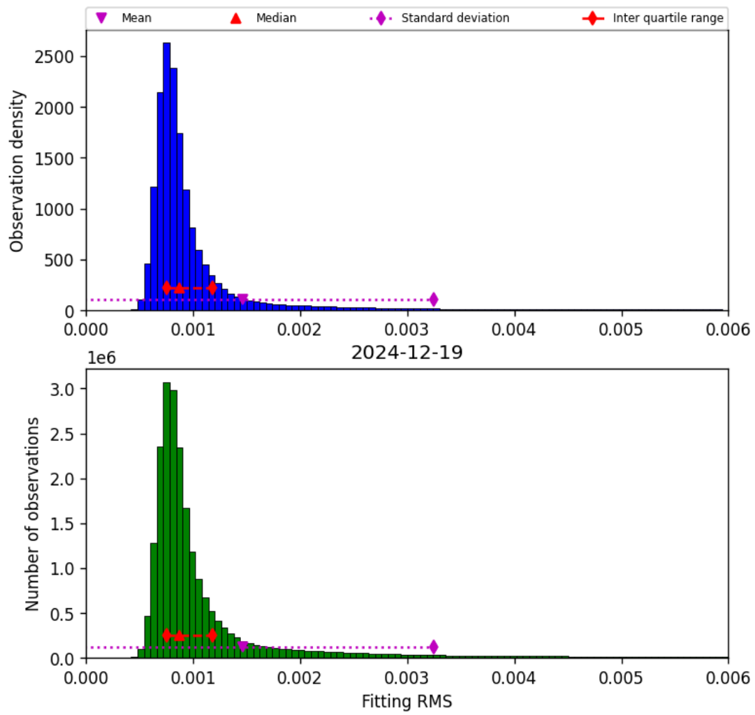
Figure 34: Histogram of “Fitting RMS” for 2024-12-19 to 2024-12-19
