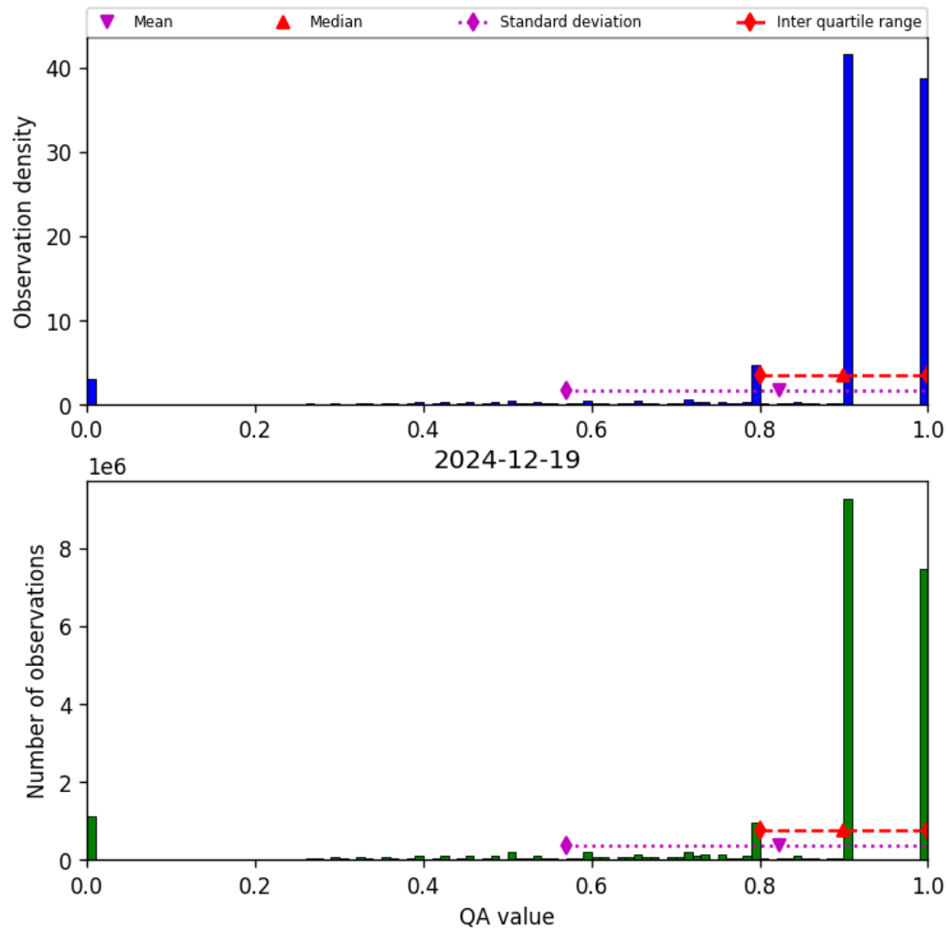
Figure 28: Histogram of “QA value” for 2024-12-19 to 2024-12-19
