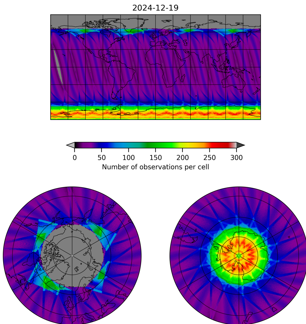
Figure 15: Map of the number of observations for 2024-12-19 to 2024-12-19
