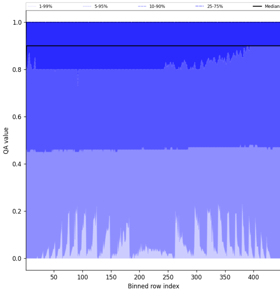
Figure 40: Along track statistics of “QA value” for 2024-12-19 to 2024-12-19
