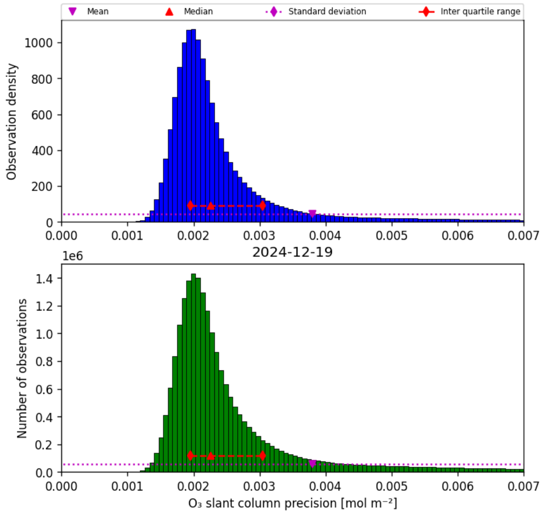
Figure 32: Histogram of “O 3 slant column precision” for 2024-12-19 to 2024-12-19
