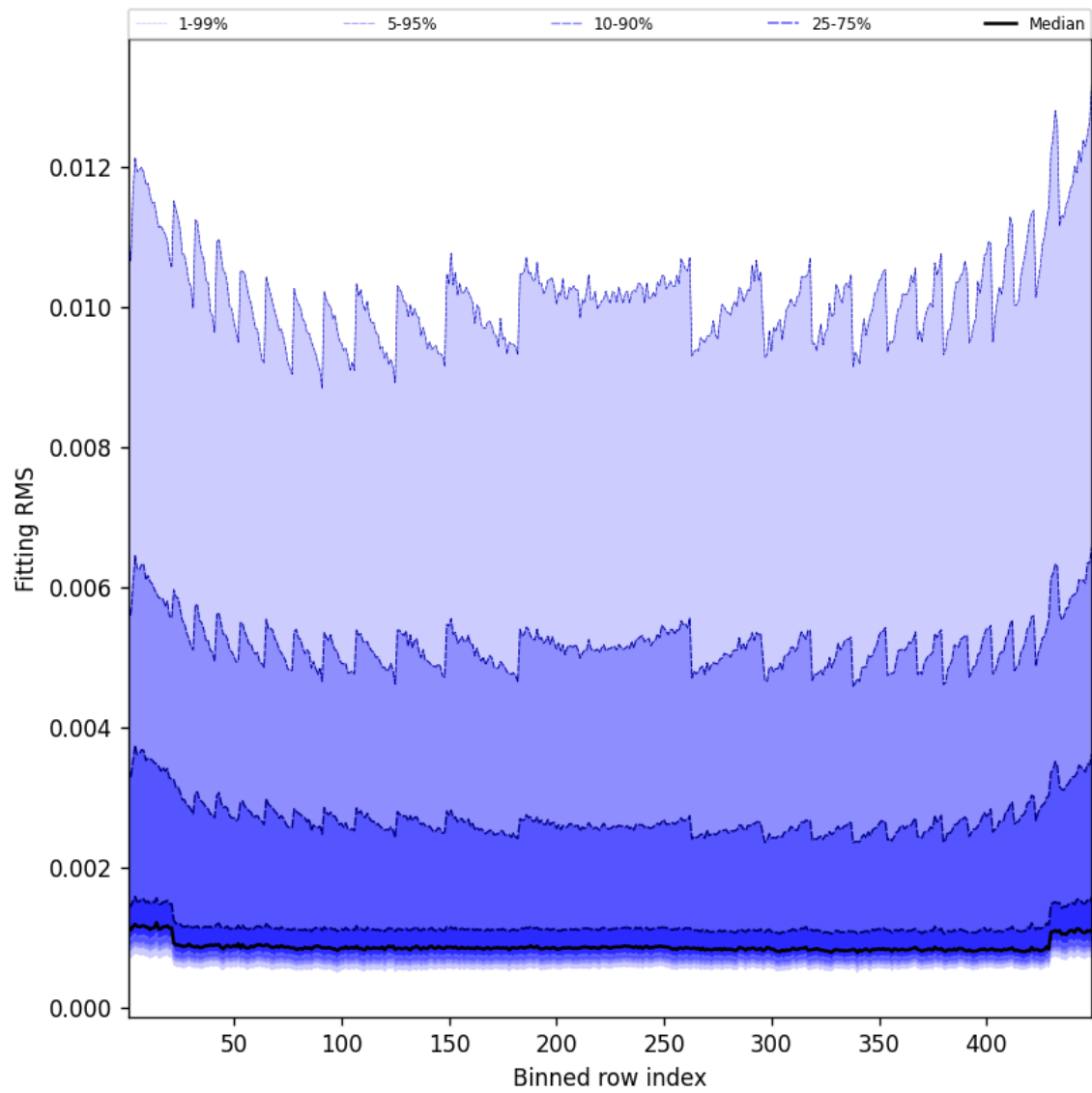
Figure 46: Along track statistics of “Fitting RMS” for 2024-12-19 to 2024-12-19
