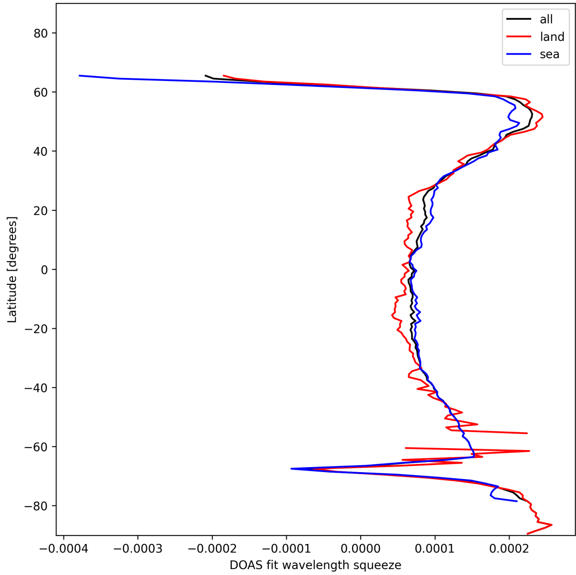
Figure 24: Zonal average of “DOAS fit wavelength squeeze” for 2024-12-19 to 2024-12-19.
