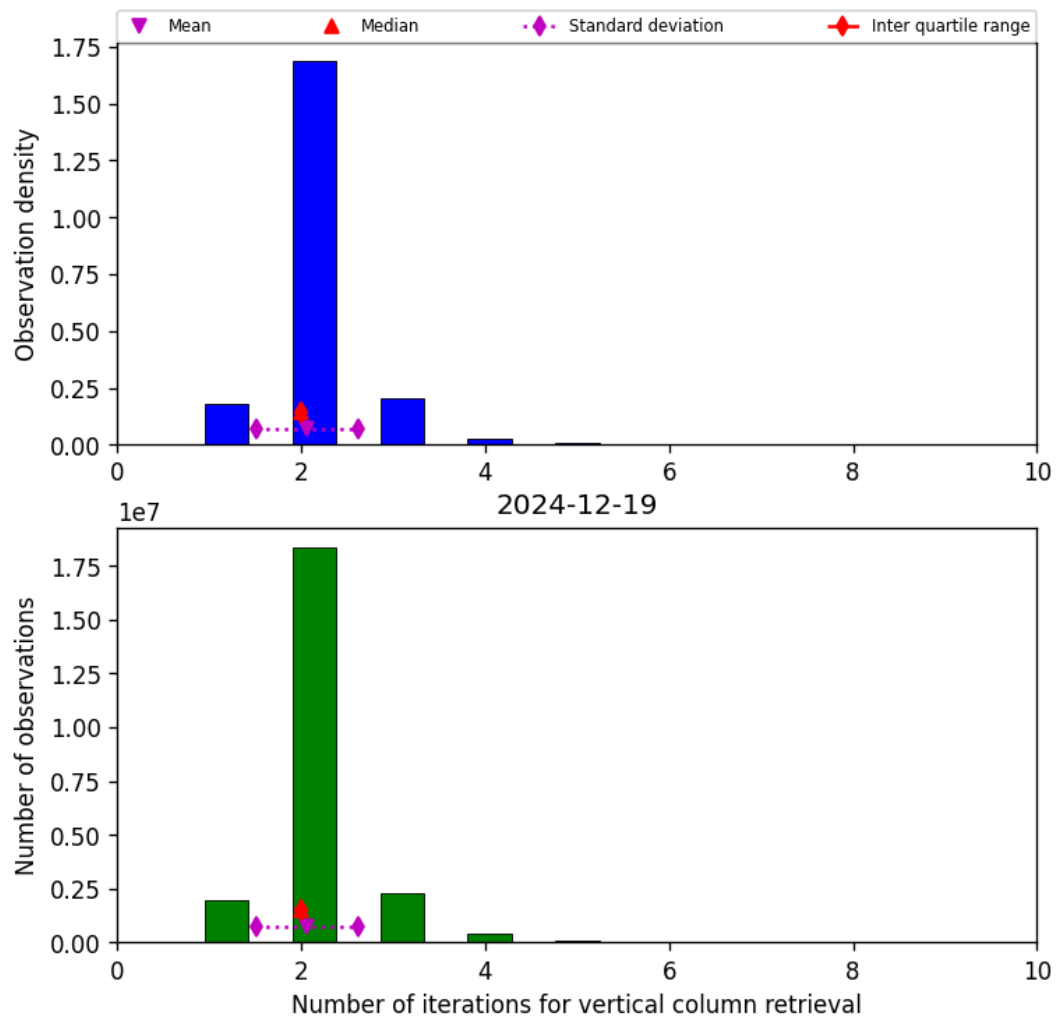
Figure 39: Histogram of “Number of iterations for vertical column retrieval” for 2024-12-19 to 2024-12-19
