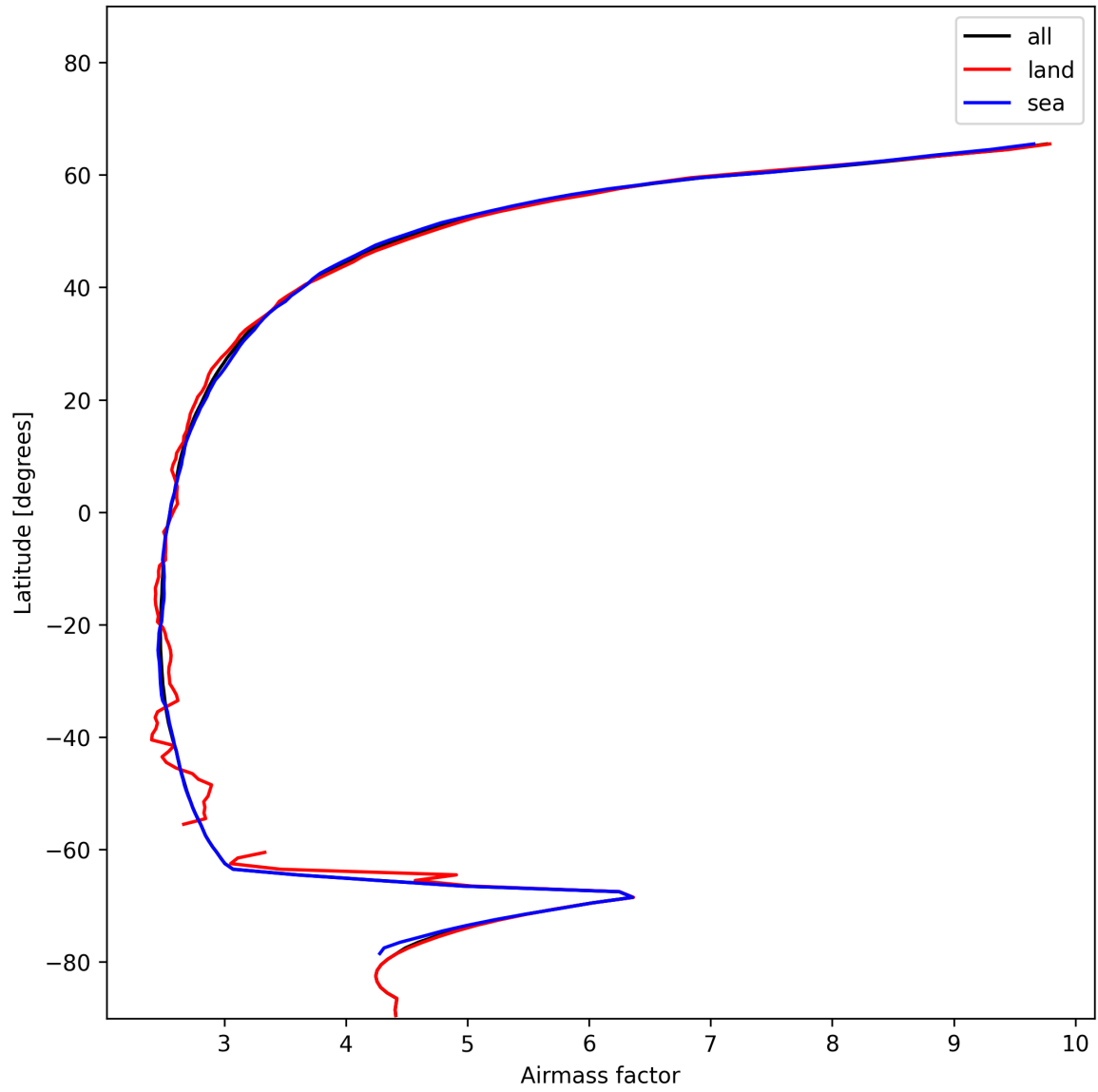
Figure 25: Zonal average of “Airmass factor” for 2024-12-19 to 2024-12-19.
