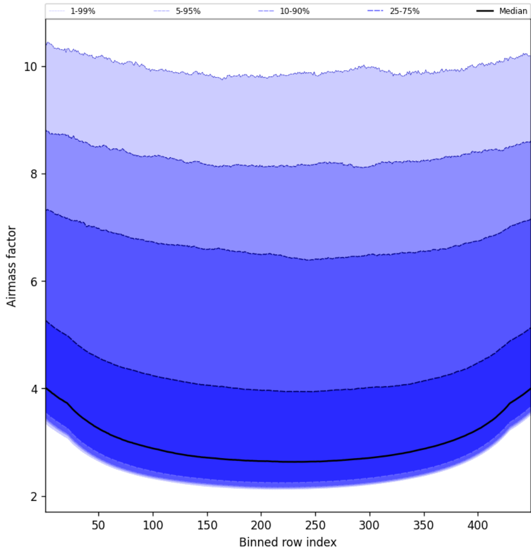
Figure 49: Along track statistics of “Airmass factor” for 2024-12-19 to 2024-12-19
