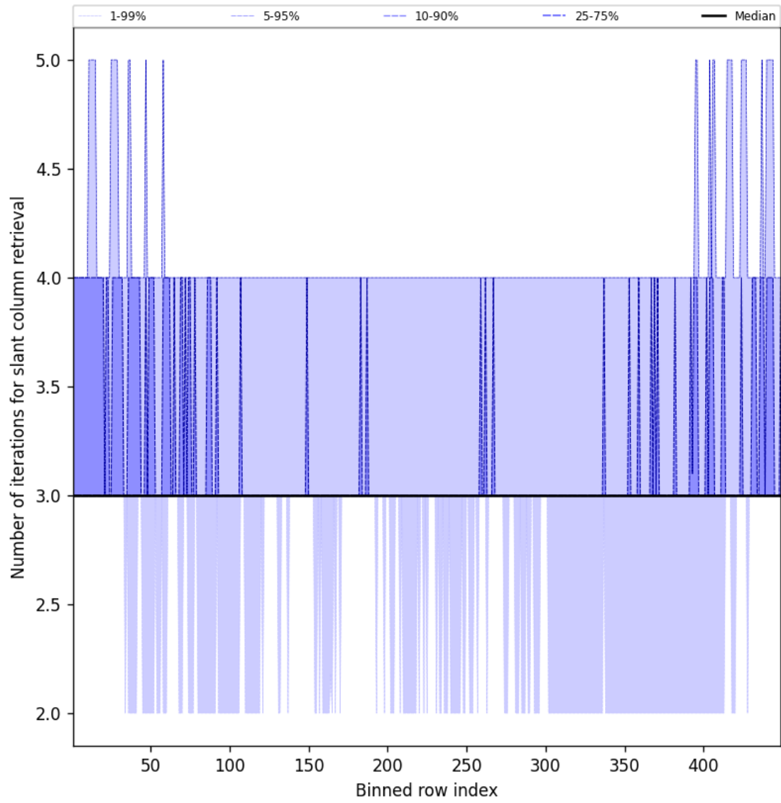
Figure 45: Along track statistics of “Number of iterations for slant column retrieval” for 2024-12-19 to 2024-12-19
