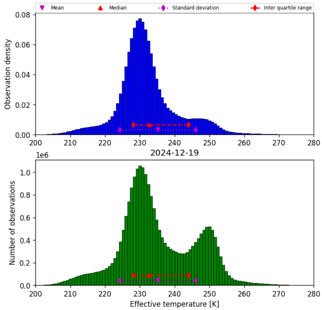
Figure 38: Histogram of “Effective temperature” for 2024-12-19 to 2024-12-19
