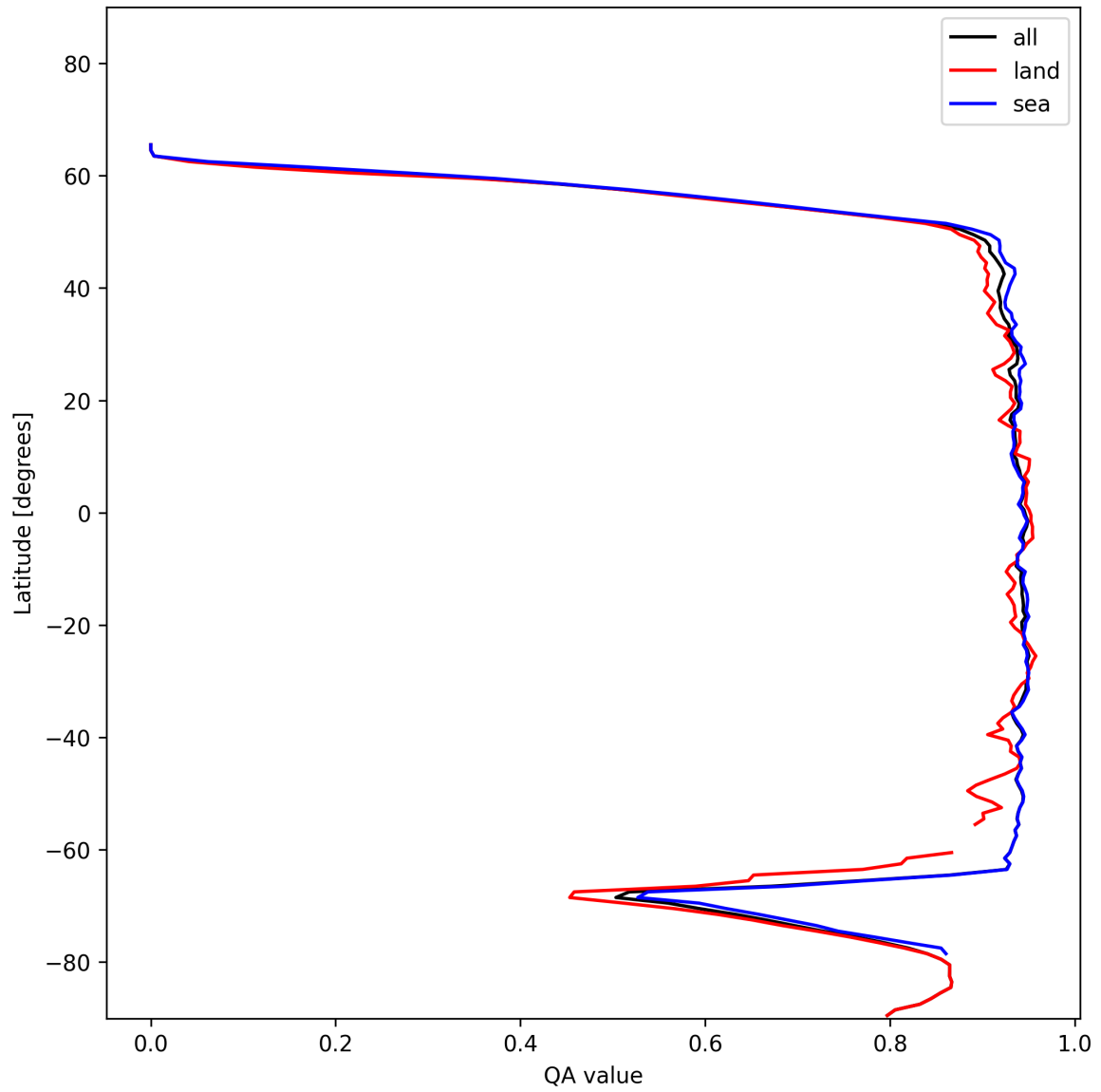
Figure 16: Zonal average of “QA value” for 2024-12-19 to 2024-12-19.
