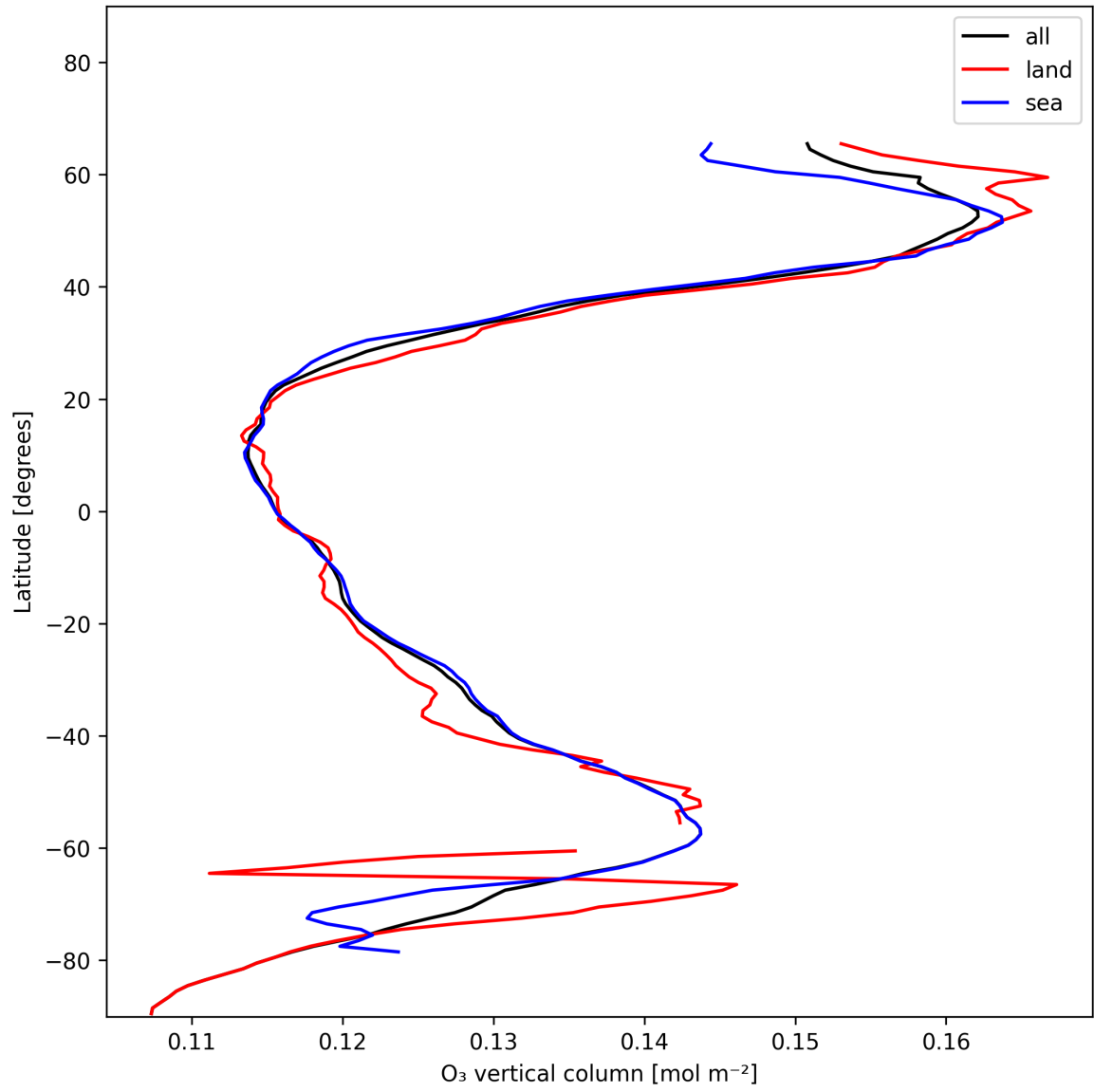
Figure 17: Zonal average of “O 3 vertical column” for 2024-12-19 to 2024-12-19.
