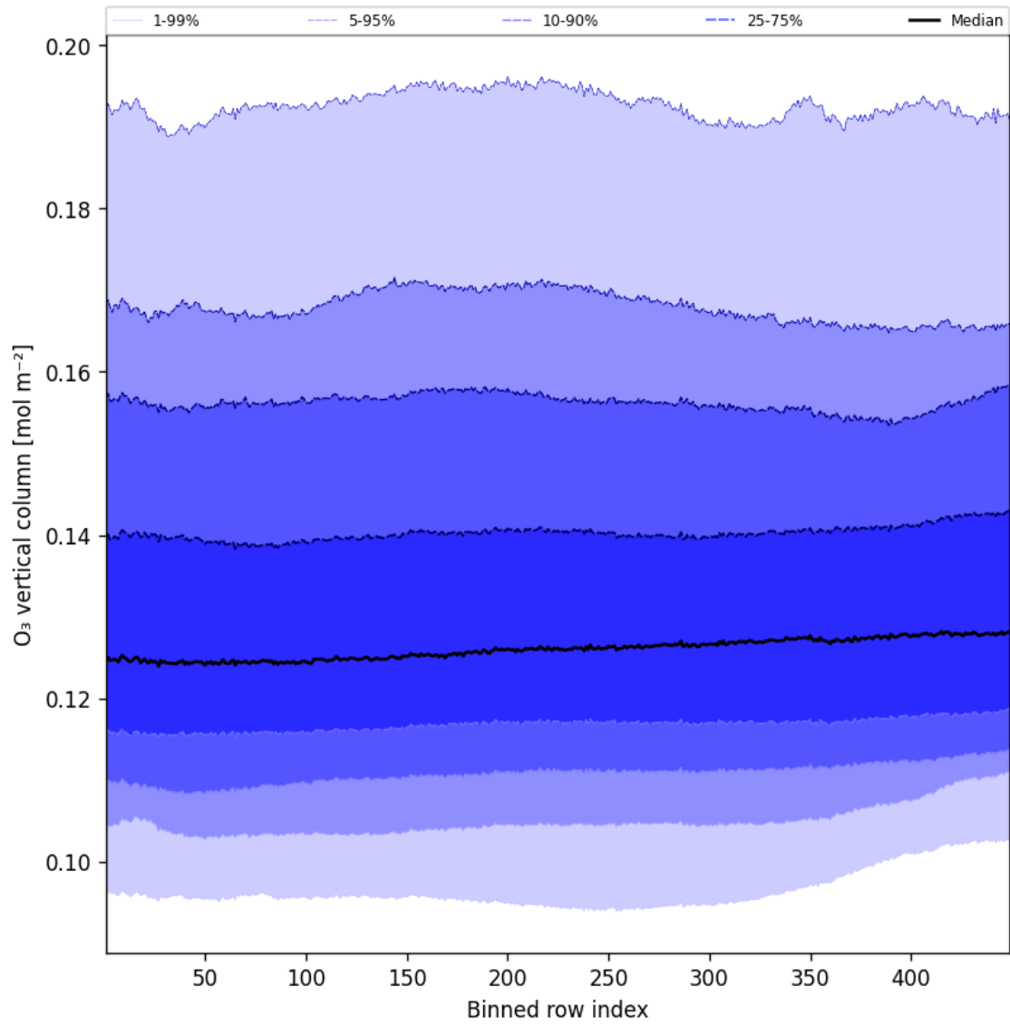
Figure 41: Along track statistics of “O 3 vertical column” for 2024-12-19 to 2024-12-19
