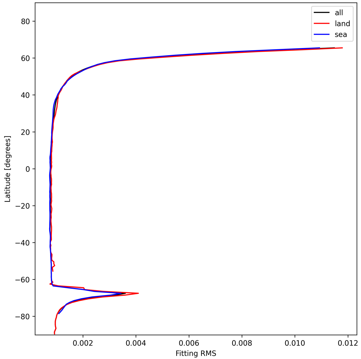
Figure 22: Zonal average of “Fitting RMS” for 2024-12-19 to 2024-12-19.
