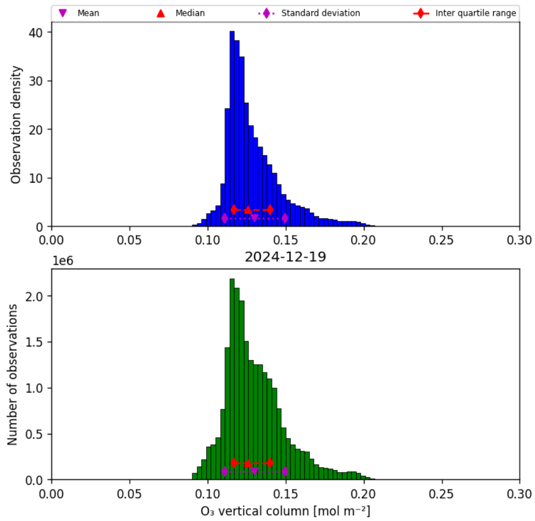
Figure 29: Histogram of “O 3 vertical column” for 2024-12-19 to 2024-12-19
