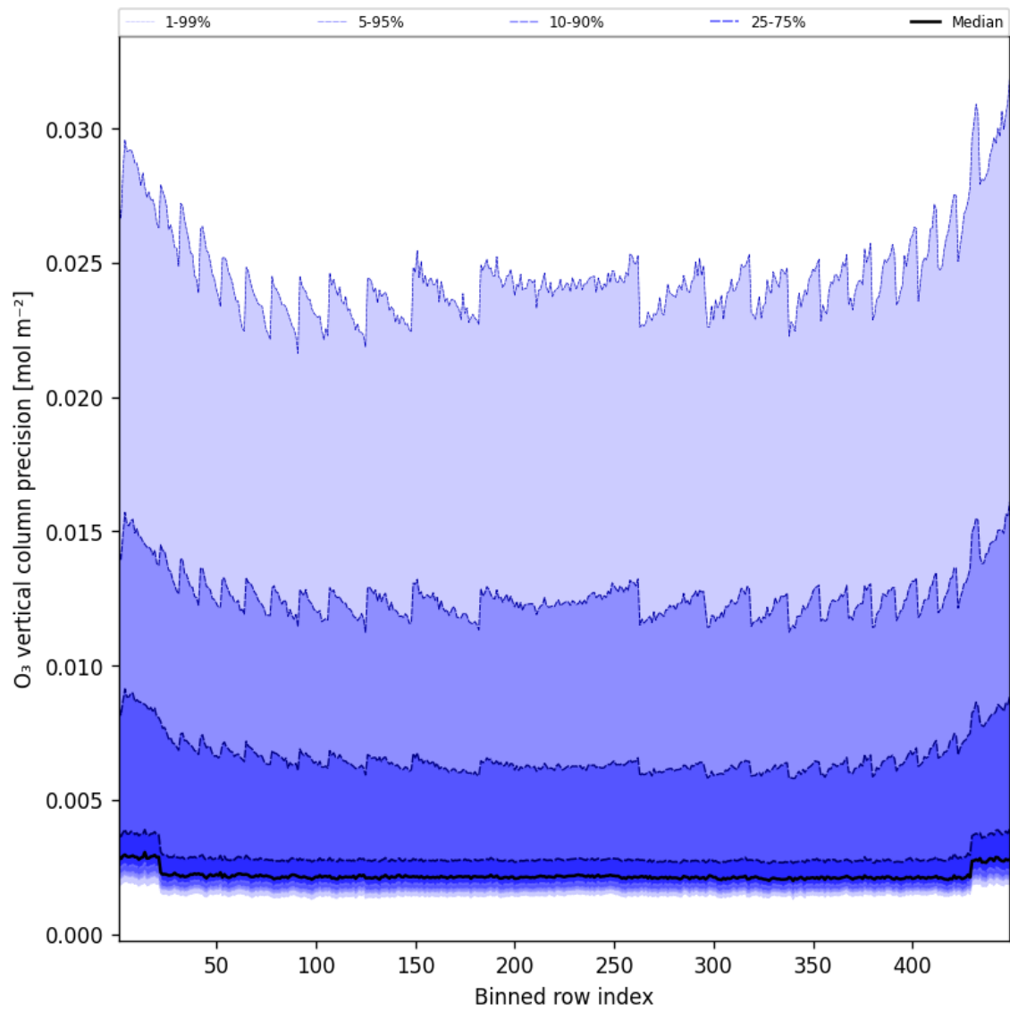
Figure 42: Along track statistics of “O 3 vertical column precision” for 2024-12-19 to 2024-12-19
