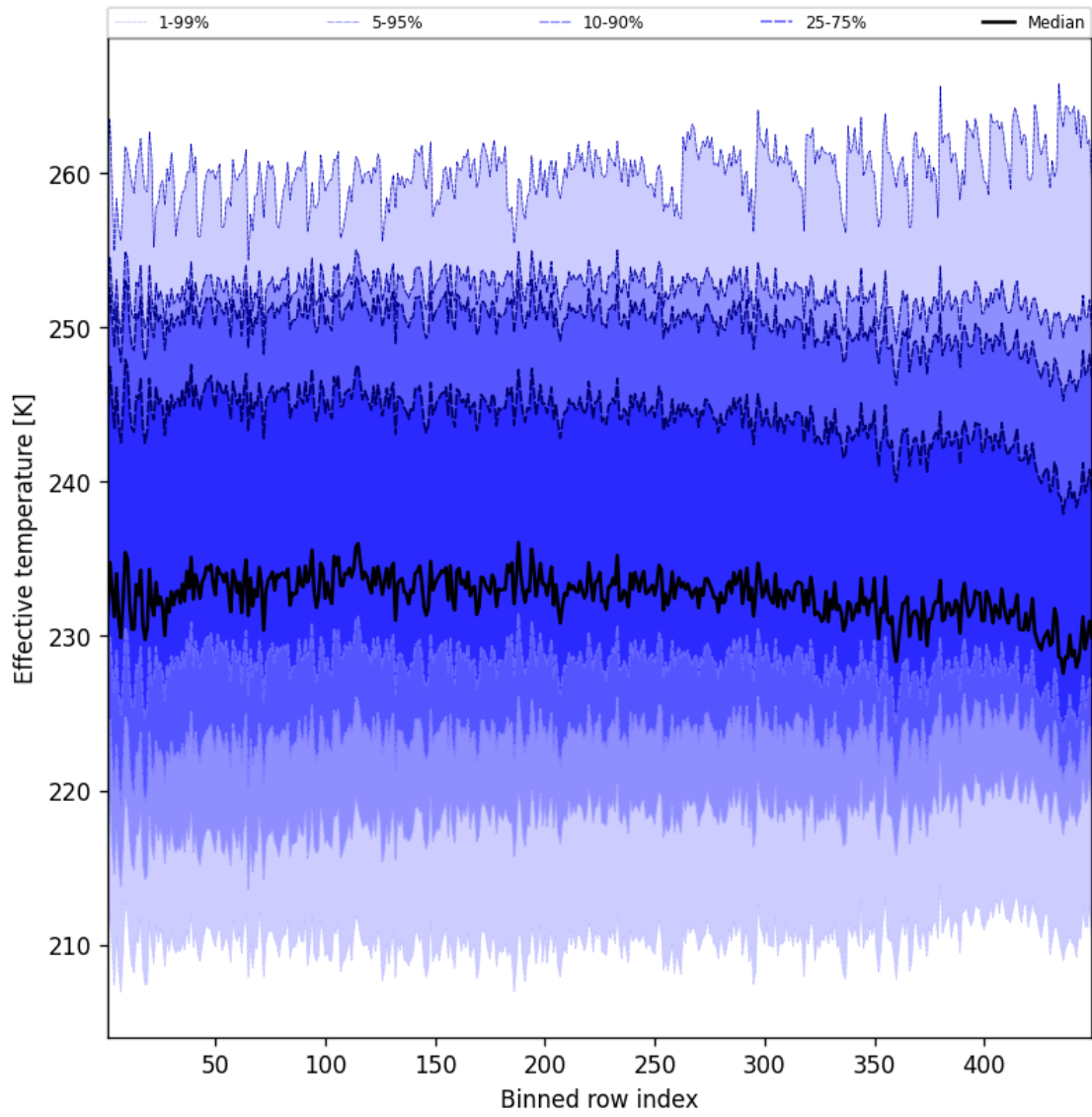
Figure 50: Along track statistics of “Effective temperature” for 2024-12-19 to 2024-12-19
