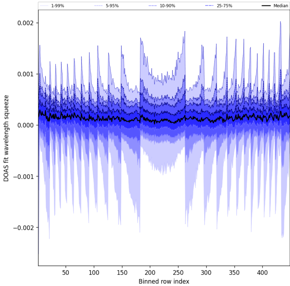
Figure 48: Along track statistics of “DOAS fit wavelength squeeze” for 2024-12-19 to 2024-12-19
