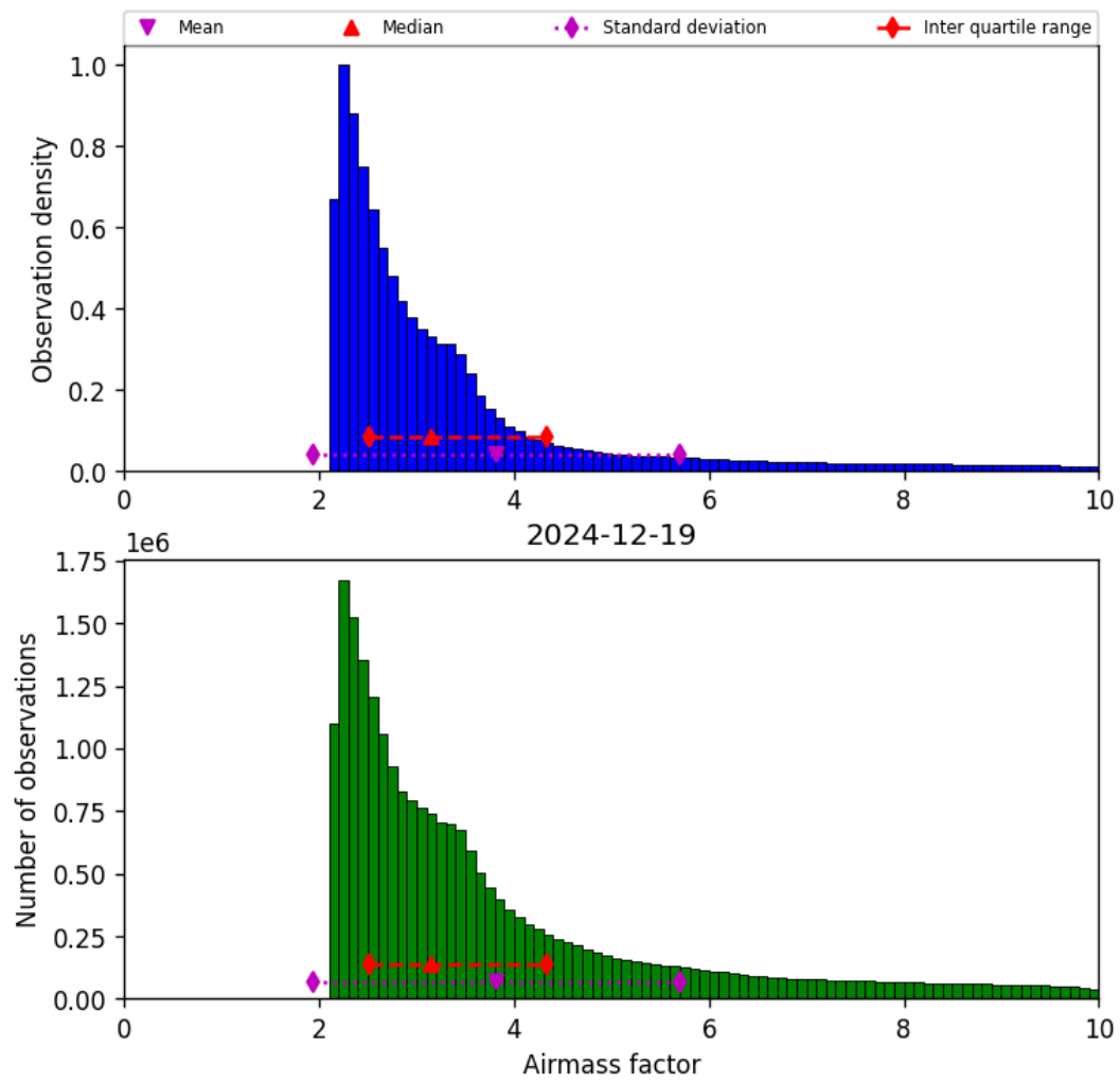
Figure 37: Histogram of “Airmass factor” for 2024-12-19 to 2024-12-19
