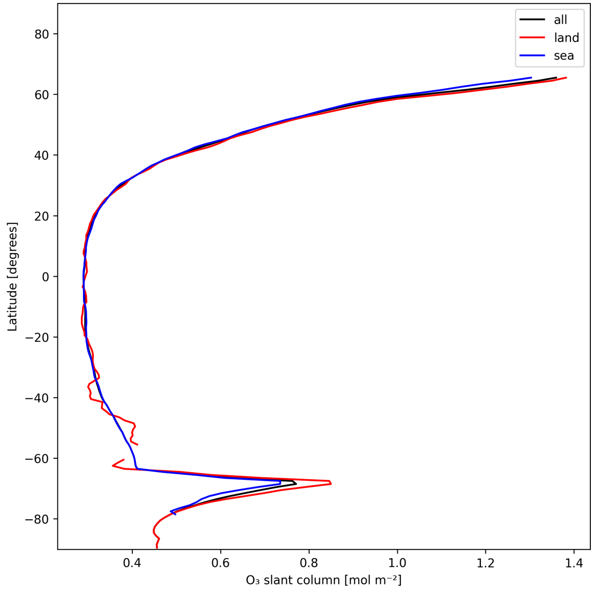
Figure 19: Zonal average of “O 3 slant column” for 2024-12-19 to 2024-12-19.
