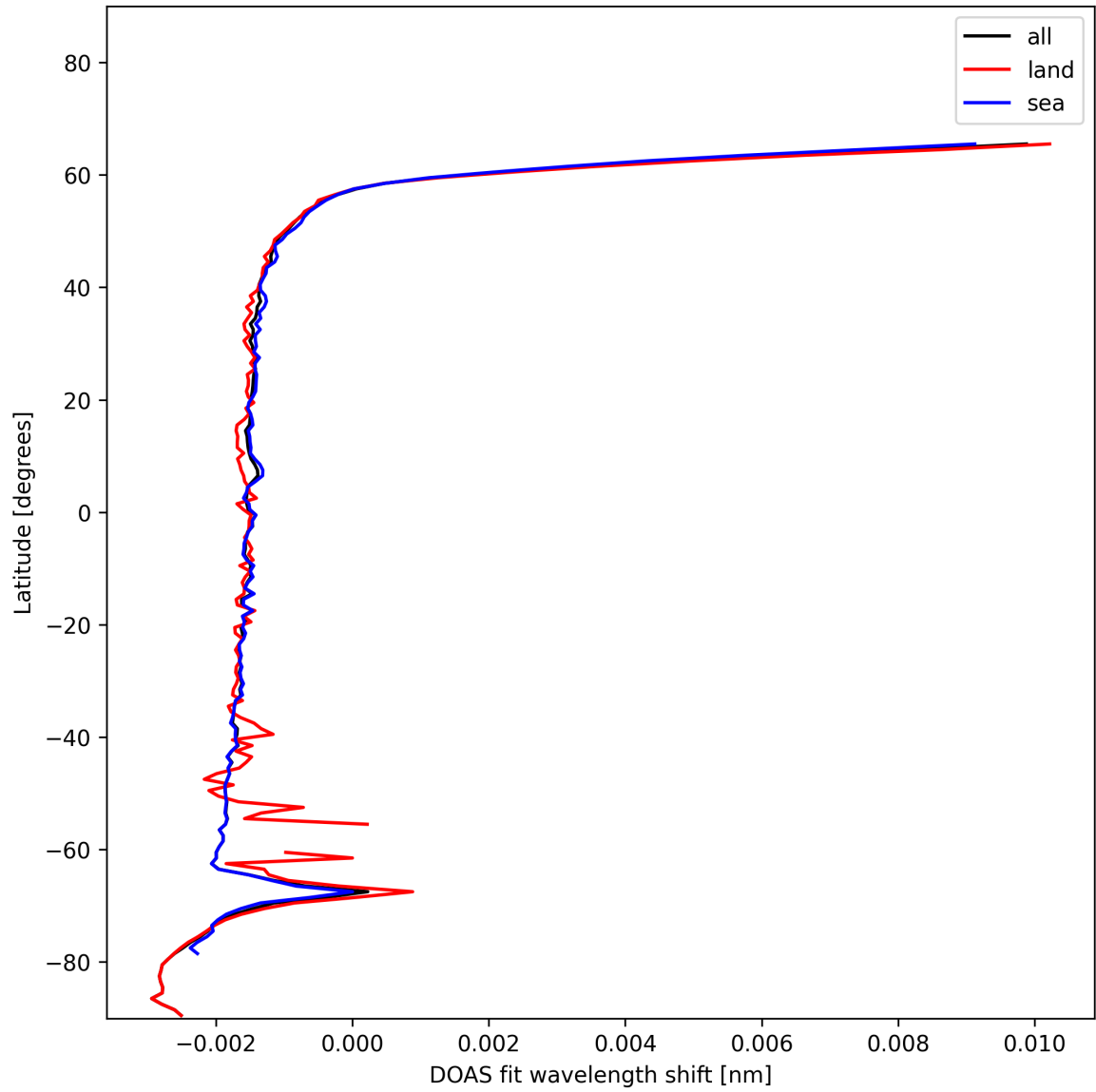
Figure 23: Zonal average of “DOAS fit wavelength shift” for 2024-12-19 to 2024-12-19.
