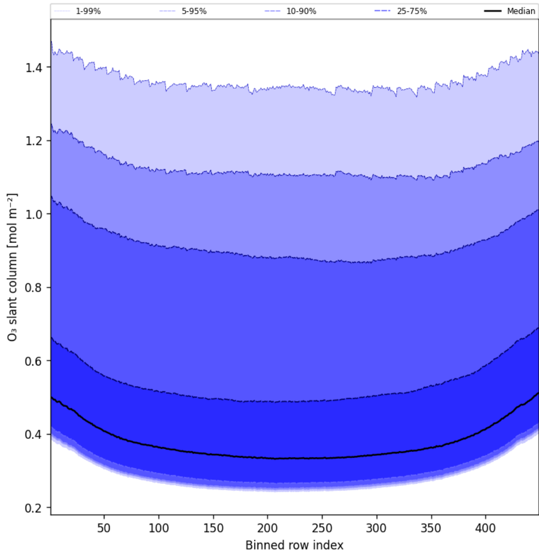
Figure 43: Along track statistics of “O 3 slant column” for 2024-12-19 to 2024-12-19
