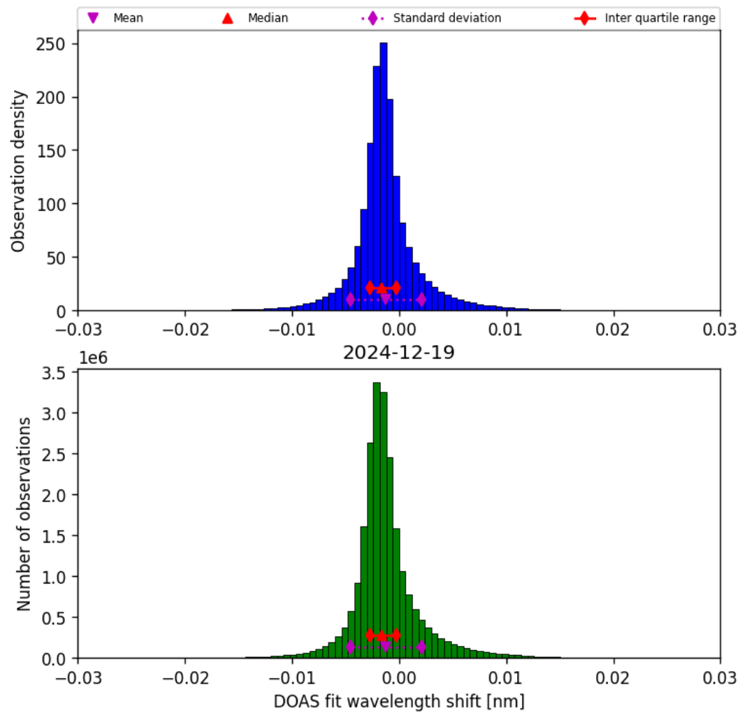
Figure 35: Histogram of “DOAS fit wavelength shift” for 2024-12-19 to 2024-12-19
