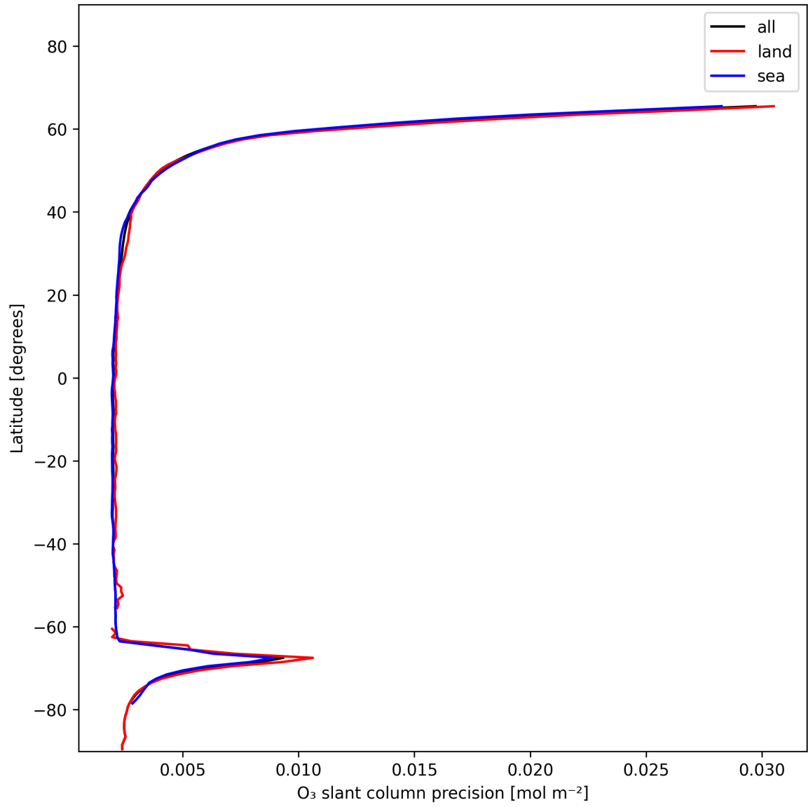
Figure 20: Zonal average of “O 3 slant column precision” for 2024-12-19 to 2024-12-19.
