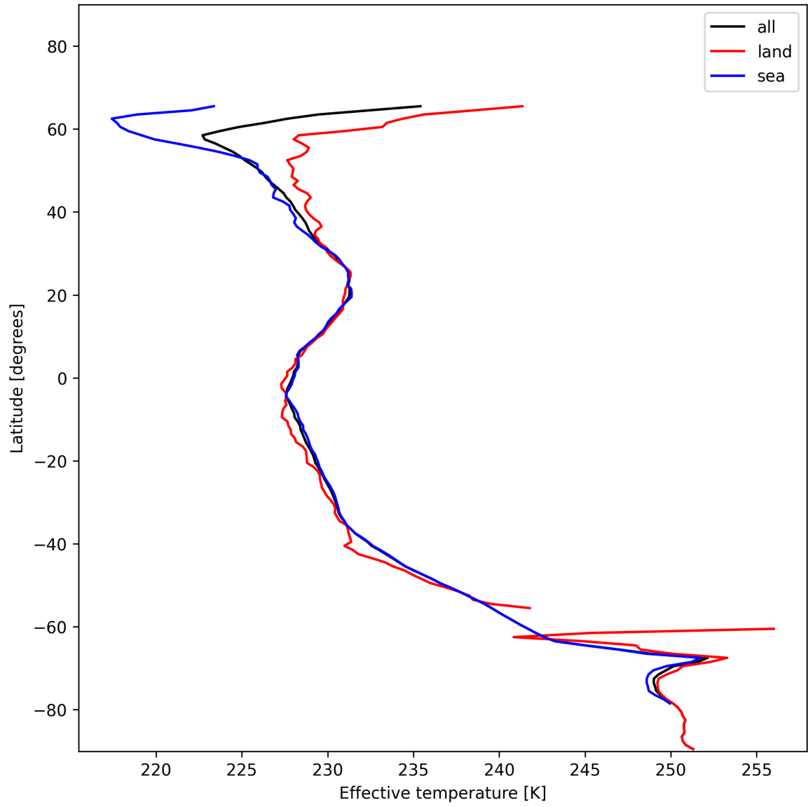
Figure 26: Zonal average of “Effective temperature” for 2024-12-19 to 2024-12-19.
