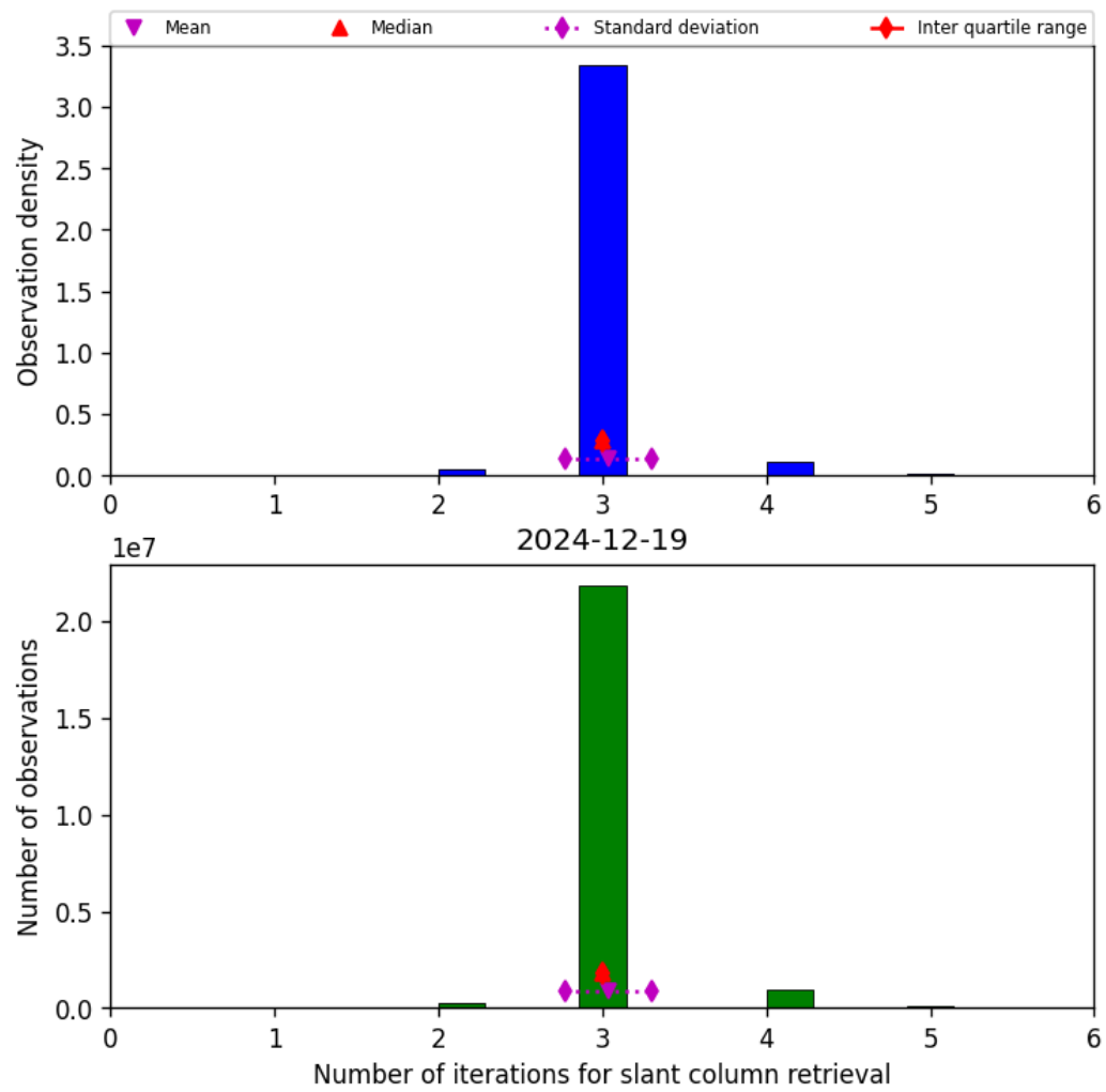
Figure 33: Histogram of "Number of iterations for slant column retrieval" for 2024-12-19 to 2024-12-19
