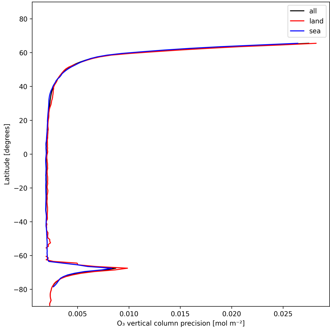
Figure 18: Zonal average of “O 3 vertical column precision” for 2024-12-19 to 2024-12-19.
