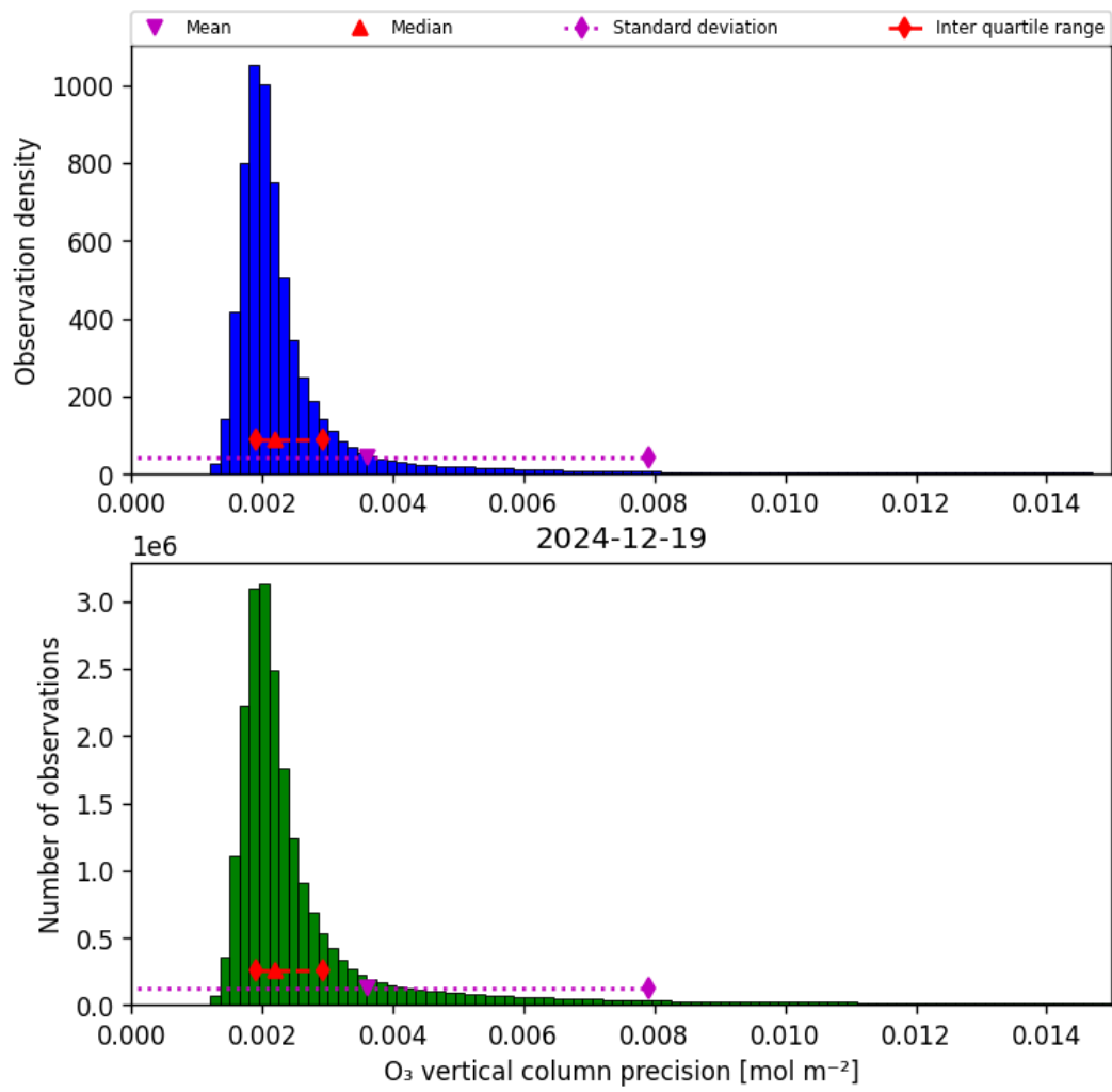
Figure 30: Histogram of “O 3 vertical column precision” for 2024-12-19 to 2024-12-19
