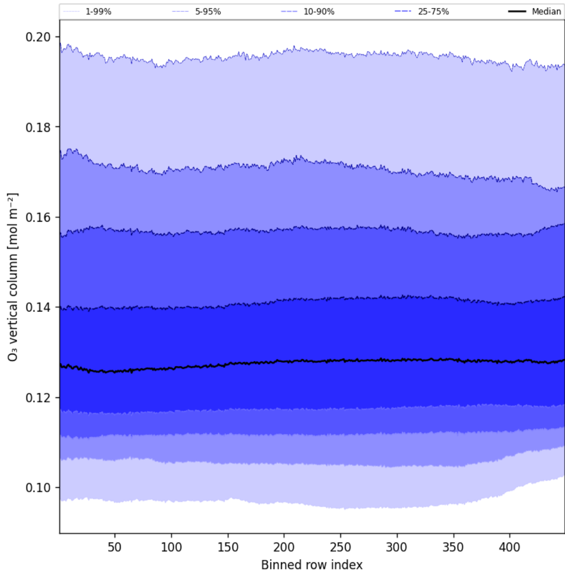
Figure 41: Along track statistics of “O 3 vertical column” for 2024-12-20 to 2024-12-20
