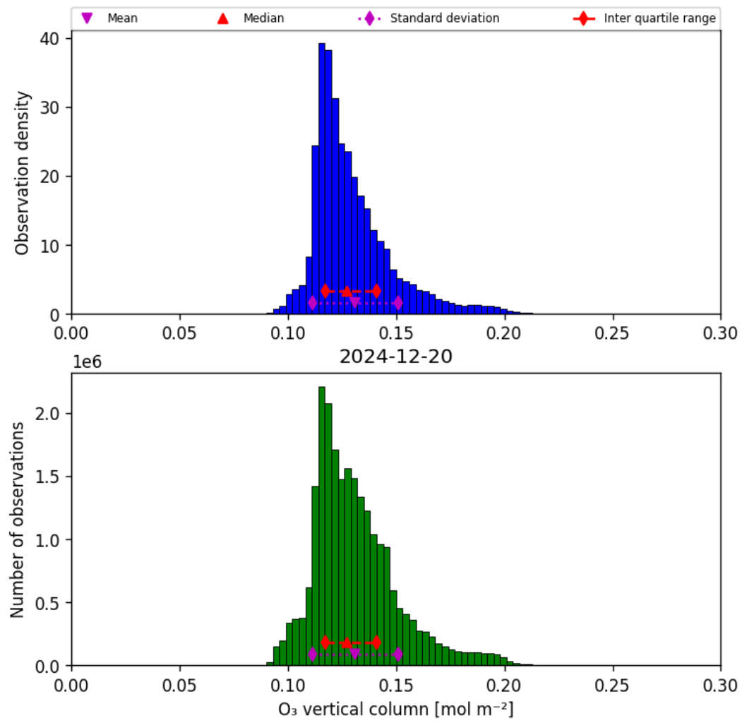
Figure 29: Histogram of “O 3 vertical column” for 2024-12-20 to 2024-12-20
