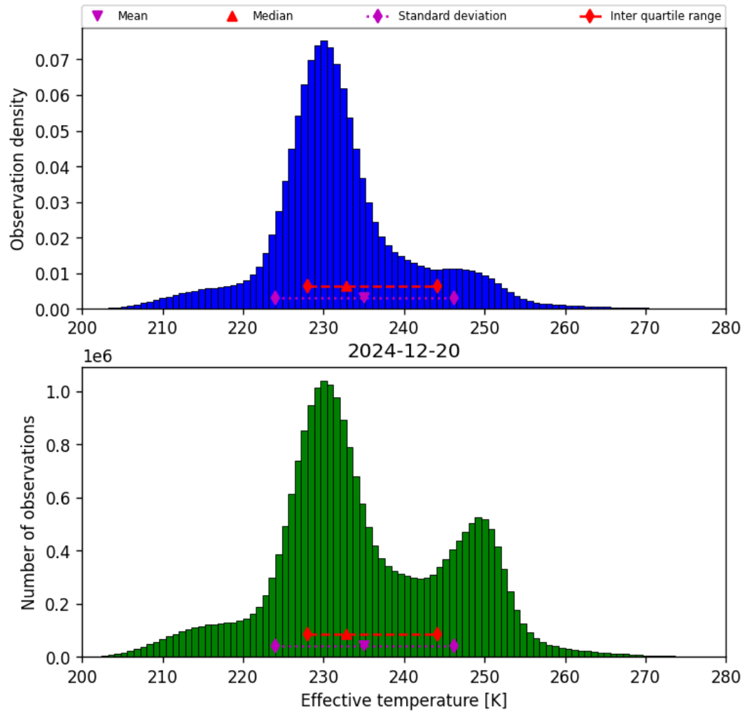
Figure 38: Histogram of “Effective temperature” for 2024-12-20 to 2024-12-20
