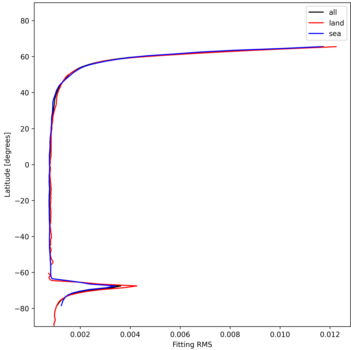
Figure 22: Zonal average of “Fitting RMS” for 2024-12-20 to 2024-12-20.
