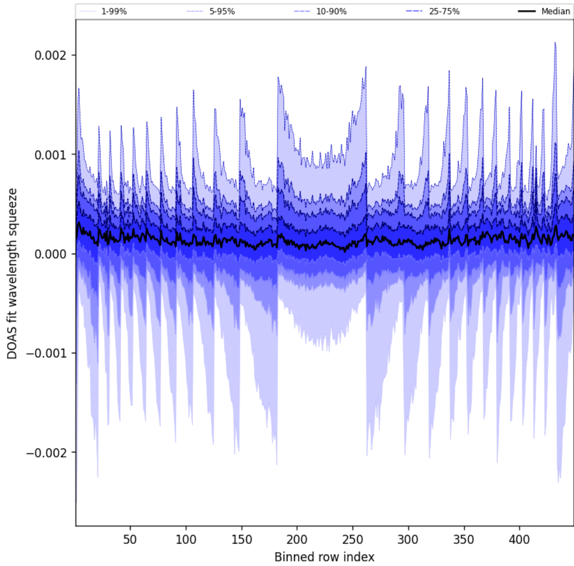
Figure 48: Along track statistics of “DOAS fit wavelength squeeze” for 2024-12-20 to 2024-12-20
