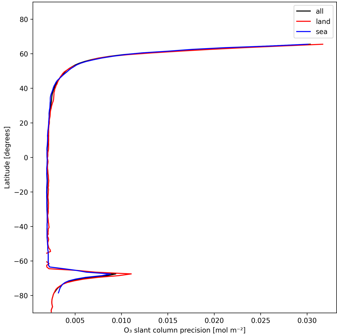
Figure 20: Zonal average of “O 3 slant column precision” for 2024-12-20 to 2024-12-20.
