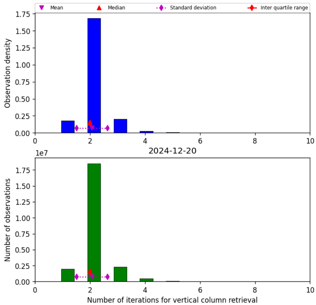
Figure 39: Histogram of “Number of iterations for vertical column retrieval” for 2024-12-20 to 2024-12-20
