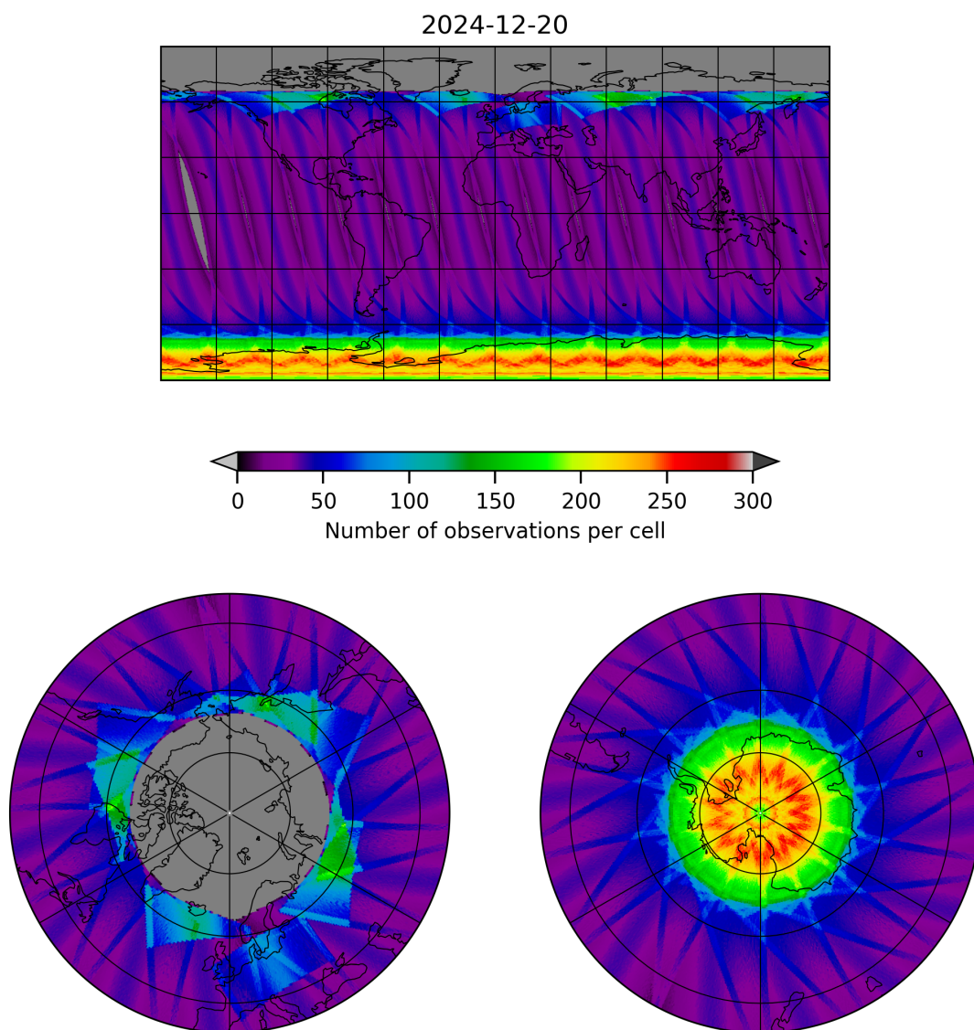
Figure 15: Map of the number of observations for 2024-12-20 to 2024-12-20
