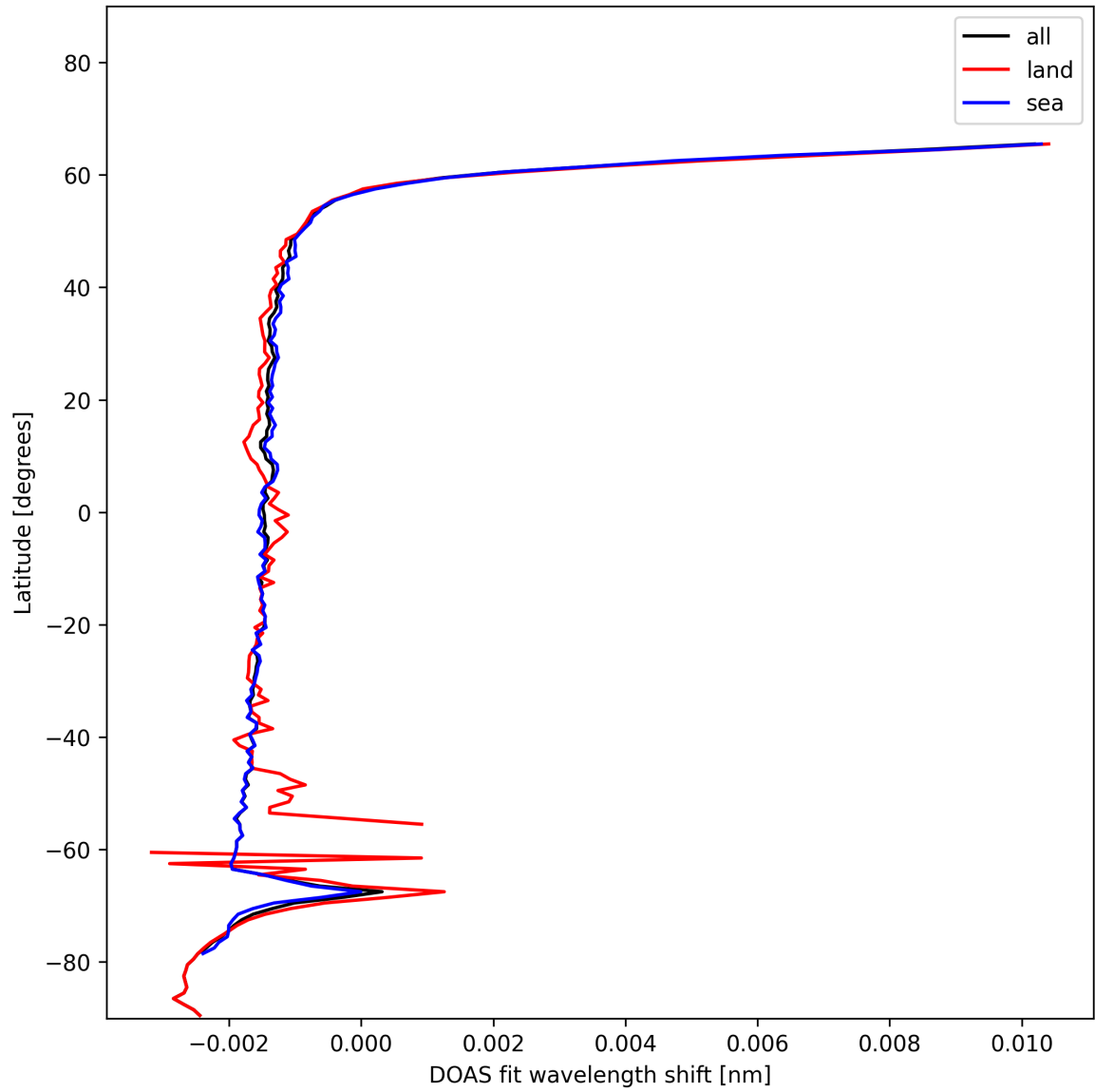
Figure 23: Zonal average of “DOAS fit wavelength shift” for 2024-12-20 to 2024-12-20.
