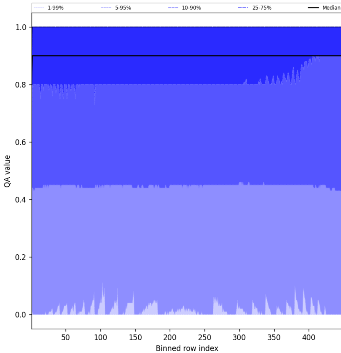
Figure 40: Along track statistics of “QA value” for 2024-12-20 to 2024-12-20
