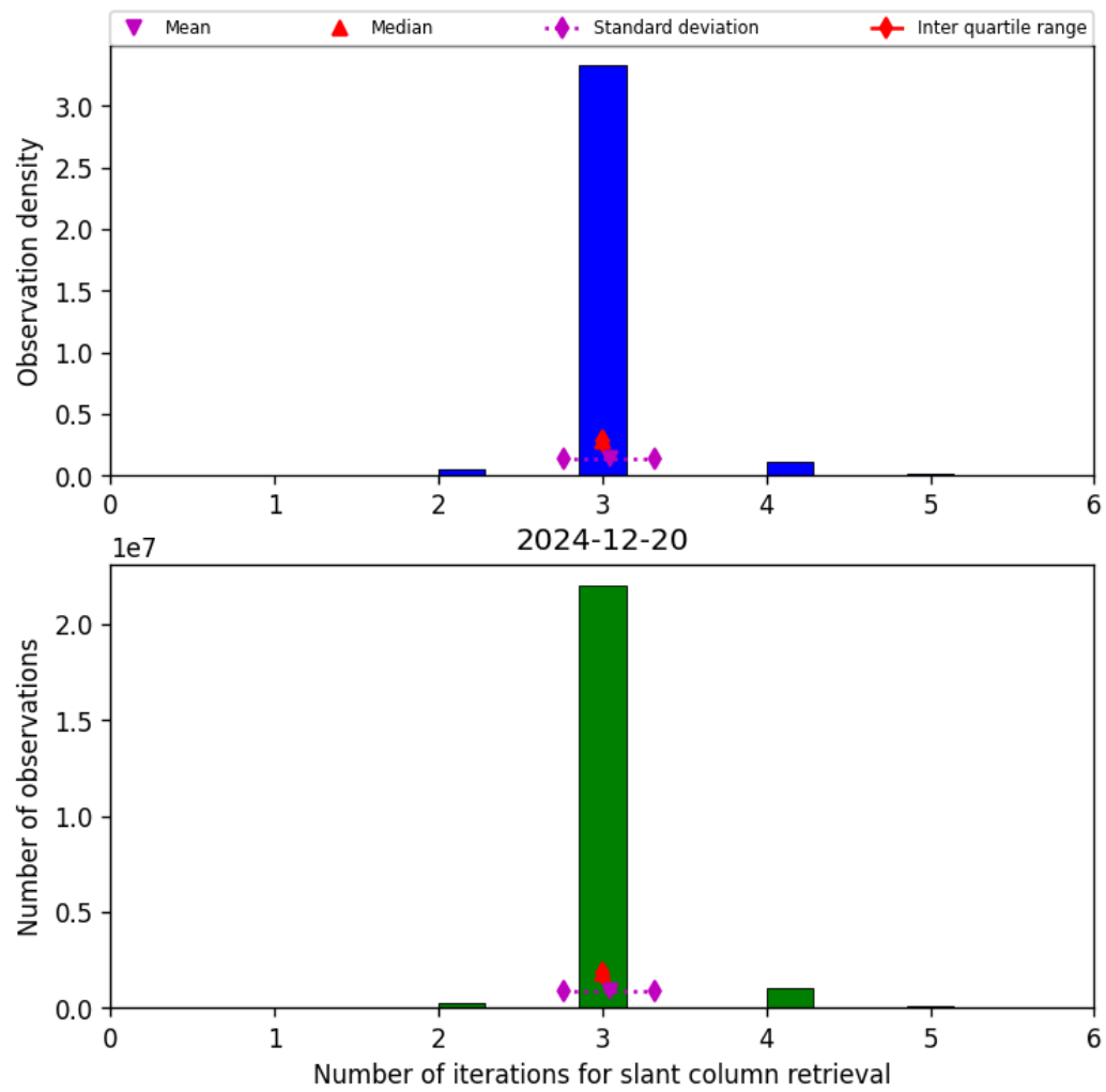
Figure 33: Histogram of “Number of iterations for slant column retrieval” for 2024-12-20 to 2024-12-20
