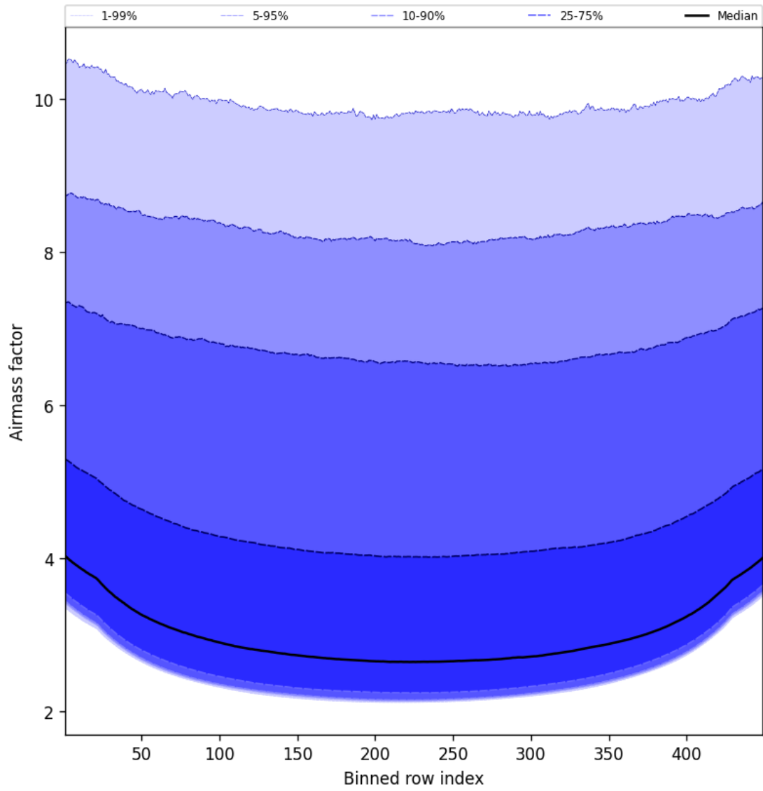
Figure 49: Along track statistics of “Airmass factor” for 2024-12-20 to 2024-12-20
