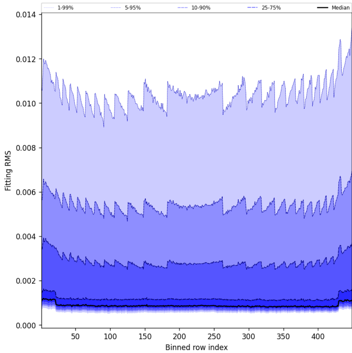
Figure 46: Along track statistics of “Fitting RMS” for 2024-12-20 to 2024-12-20
