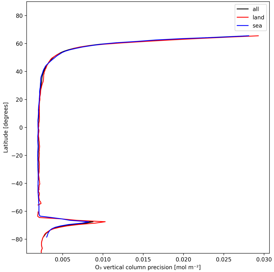
Figure 18: Zonal average of “O 3 vertical column precision” for 2024-12-20 to 2024-12-20.
