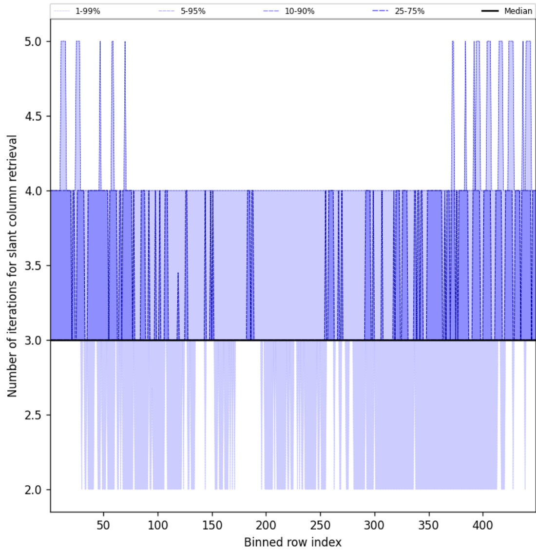
Figure 45: Along track statistics of “Number of iterations for slant column retrieval” for 2024-12-20 to 2024-12-20
