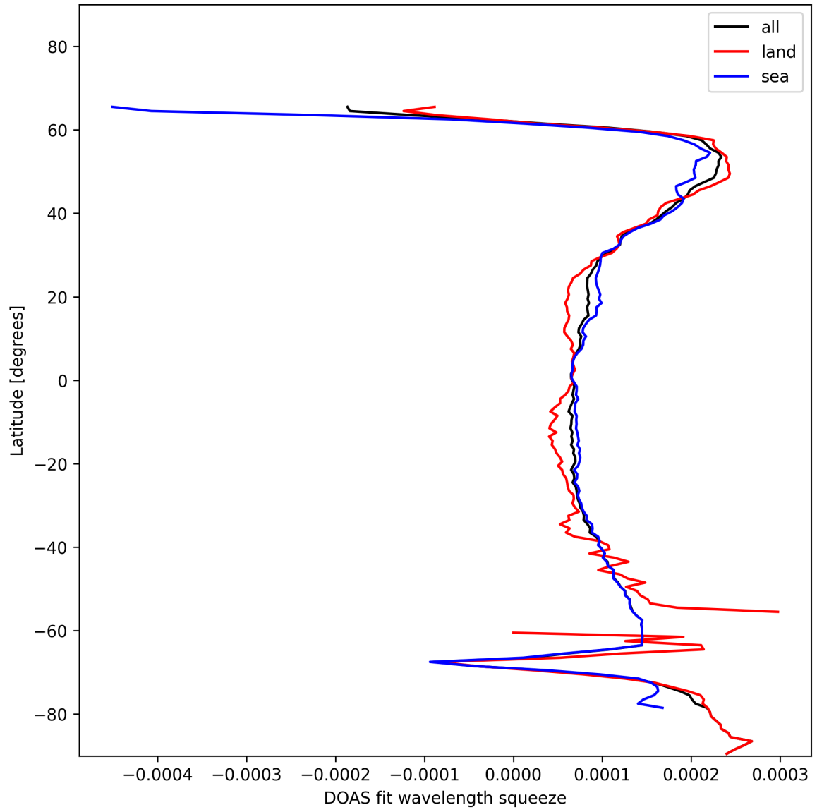
Figure 24: Zonal average of “DOAS fit wavelength squeeze” for 2024-12-20 to 2024-12-20.
