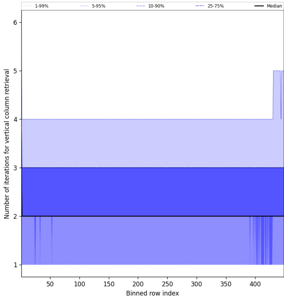
Figure 51: Along track statistics of “Number of iterations for vertical column retrieval” for 2024-12-20 to 2024-12-20
