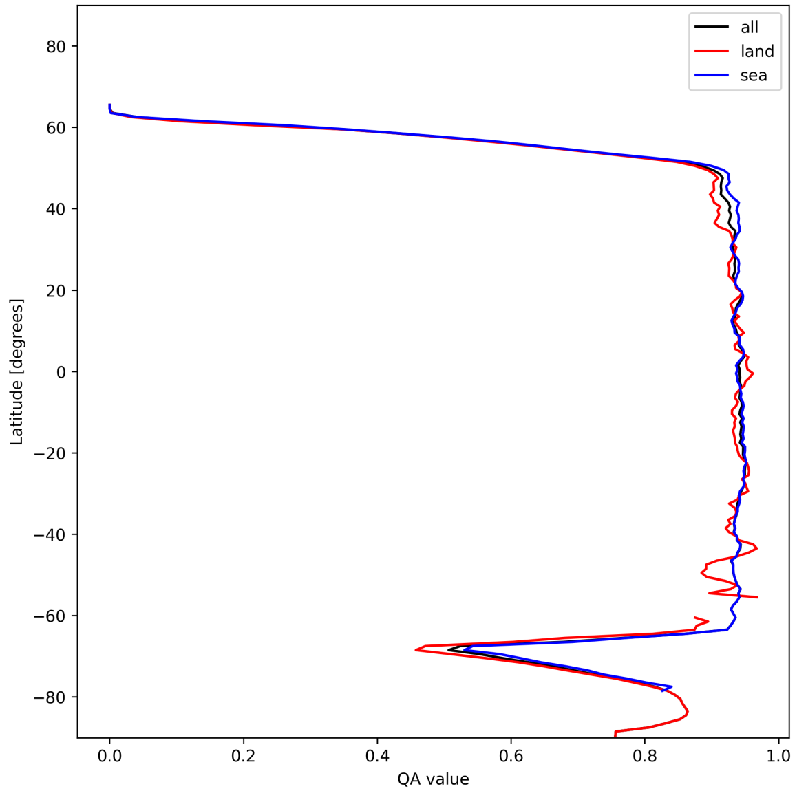
Figure 16: Zonal average of “QA value” for 2024-12-20 to 2024-12-20.
