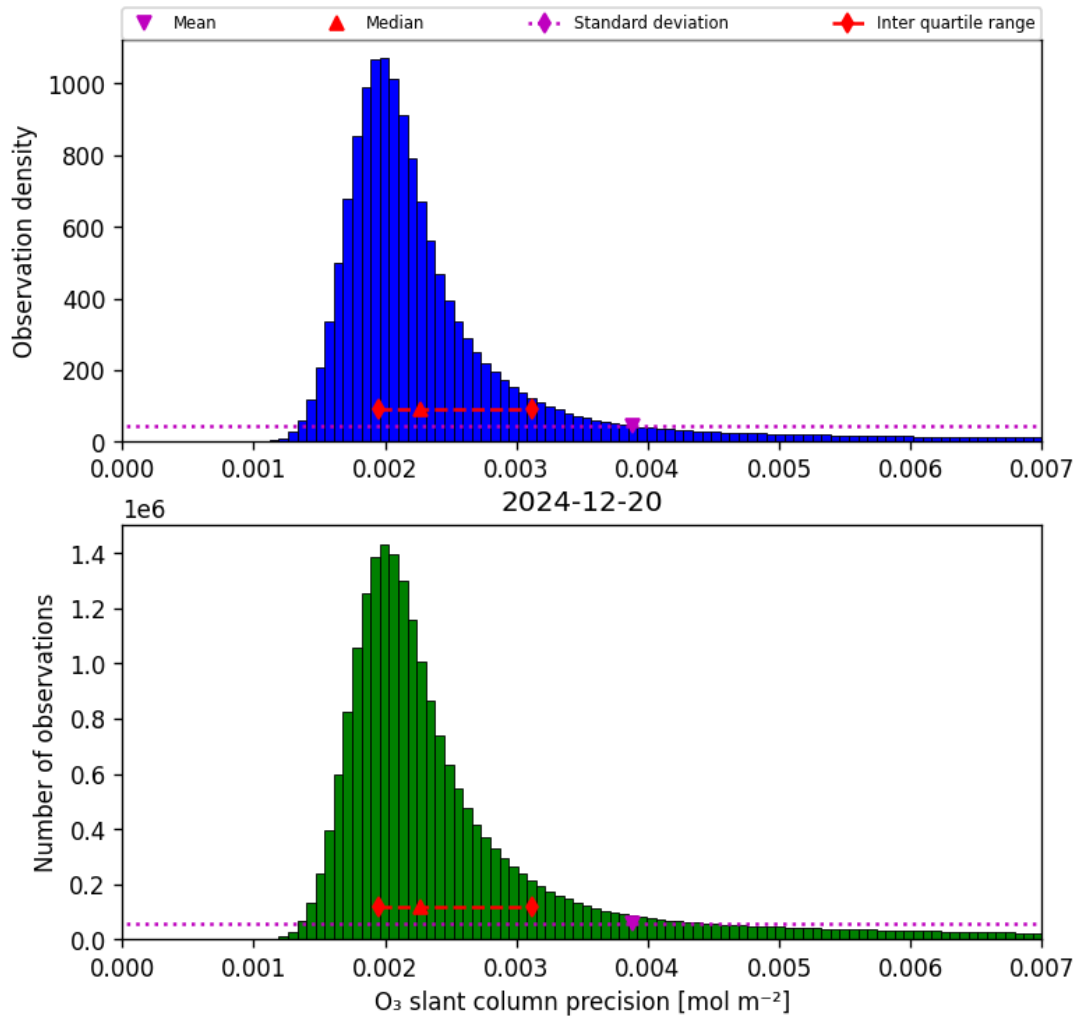
Figure 32: Histogram of “O 3 slant column precision” for 2024-12-20 to 2024-12-20
