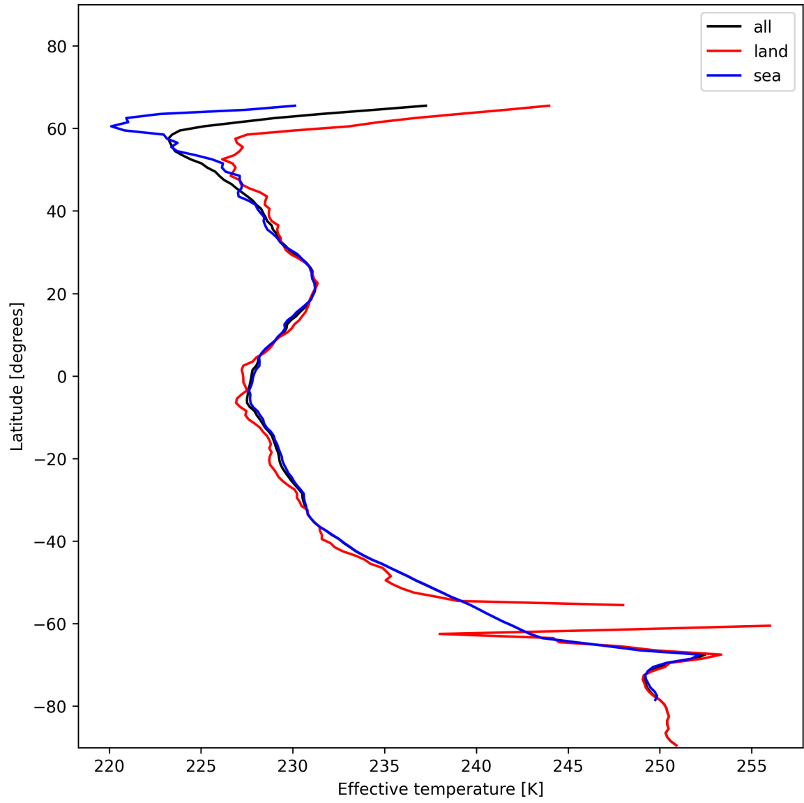
Figure 26: Zonal average of “Effective temperature” for 2024-12-20 to 2024-12-20.
