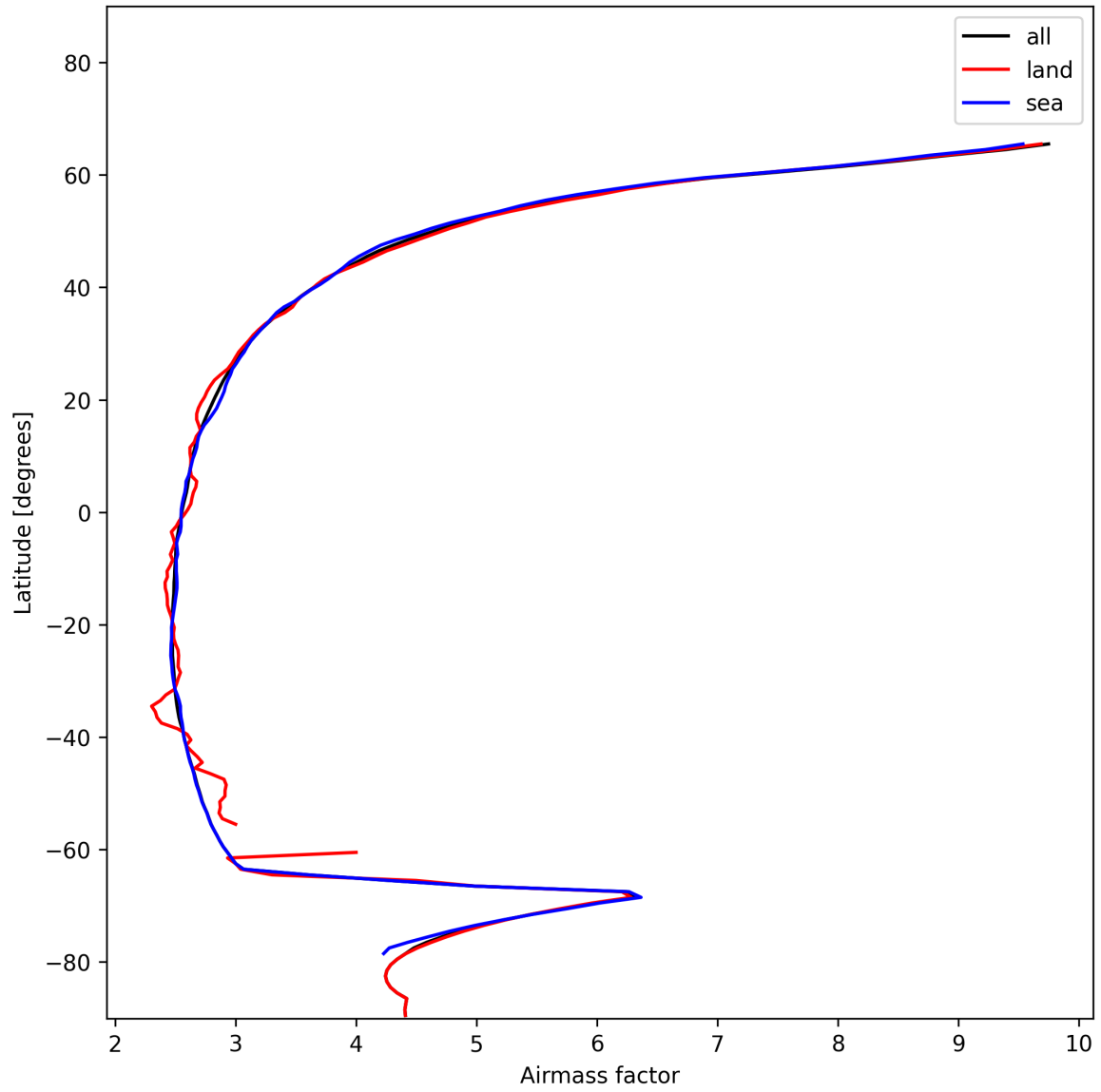
Figure 25: Zonal average of “Airmass factor” for 2024-12-20 to 2024-12-20.
