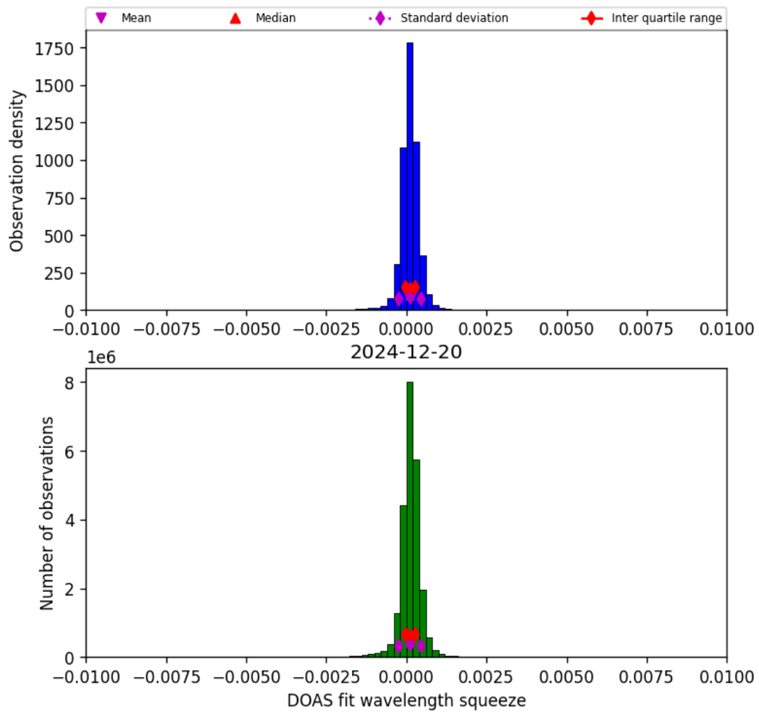
Figure 36: Histogram of “DOAS fit wavelength squeeze” for 2024-12-20 to 2024-12-20
