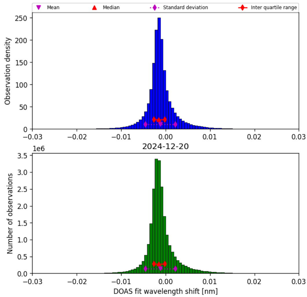
Figure 35: Histogram of “DOAS fit wavelength shift” for 2024-12-20 to 2024-12-20
