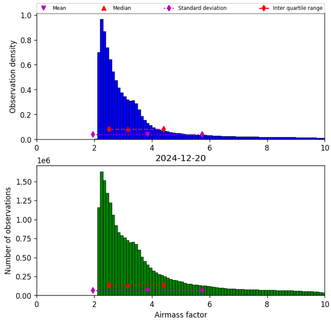
Figure 37: Histogram of “Airmass factor” for 2024-12-20 to 2024-12-20
