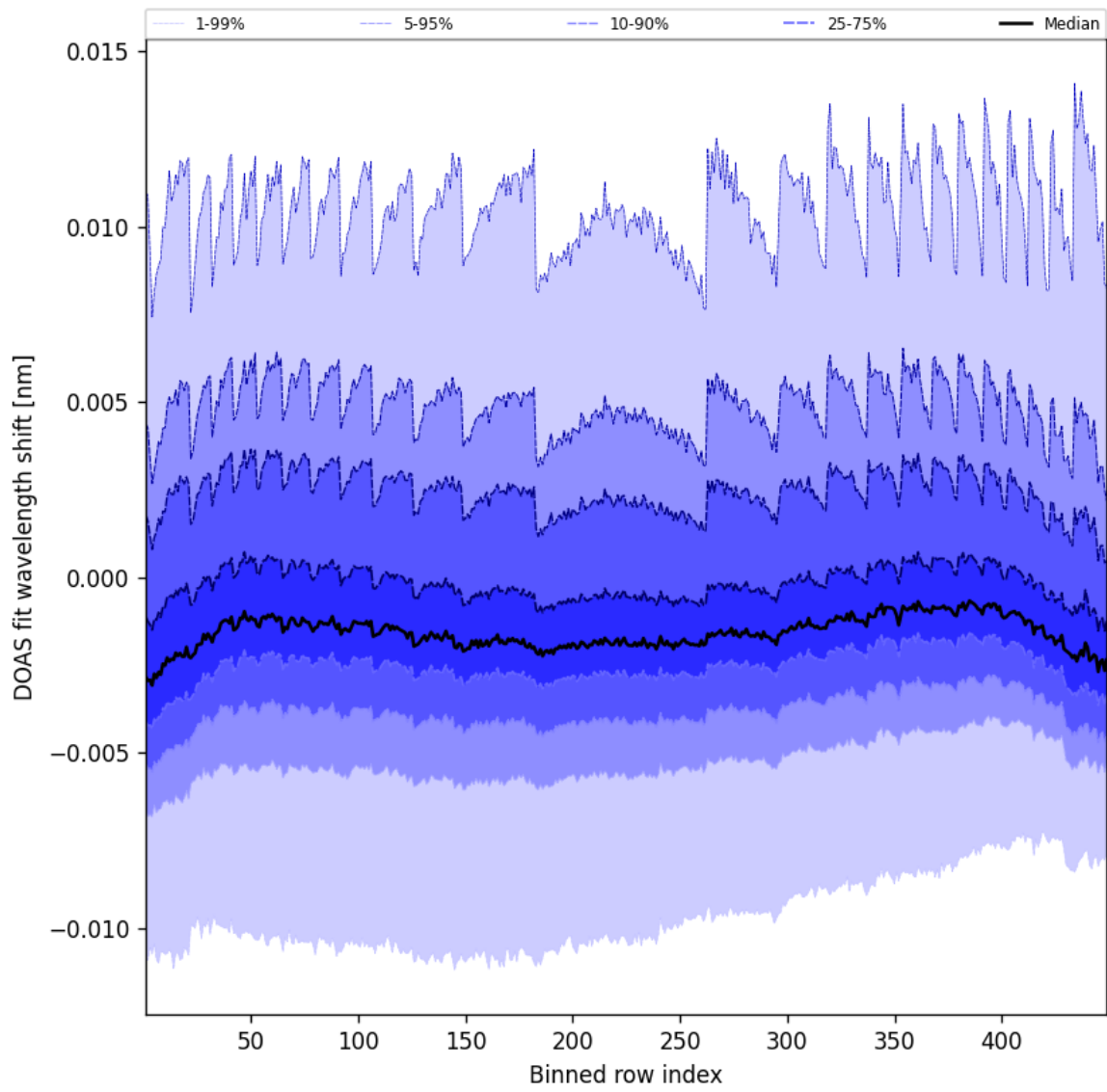
Figure 47: Along track statistics of "DOAS fit wavelength shift" for 2024-12-20 to 2024-12-20
