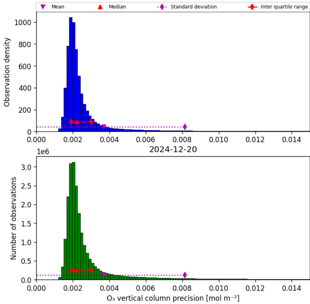
Figure 30: Histogram of “O 3 vertical column precision” for 2024-12-20 to 2024-12-20
