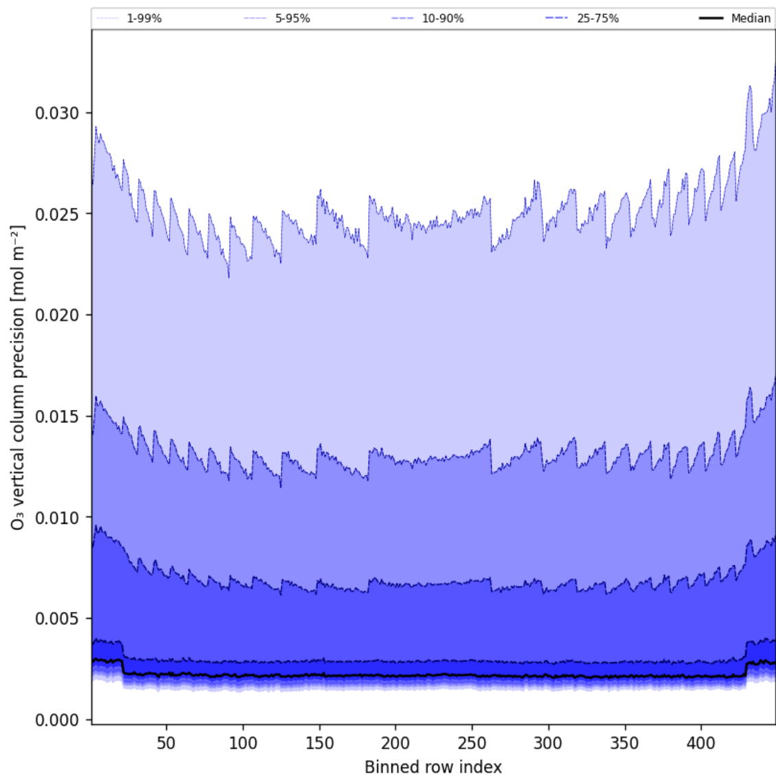
Figure 42: Along track statistics of “O 3 vertical column precision” for 2024-12-20 to 2024-12-20
