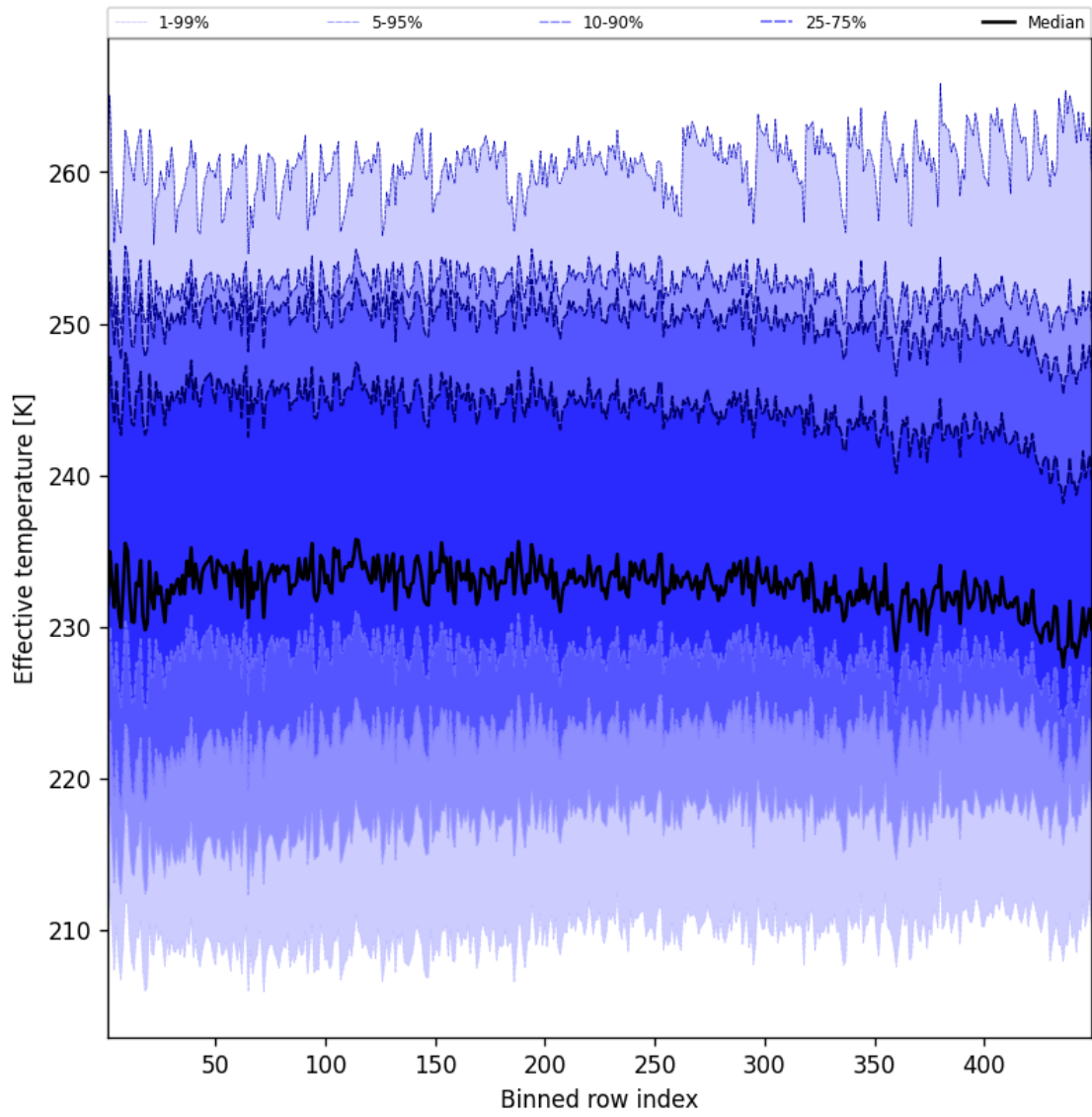
Figure 50: Along track statistics of “Effective temperature” for 2024-12-20 to 2024-12-20
