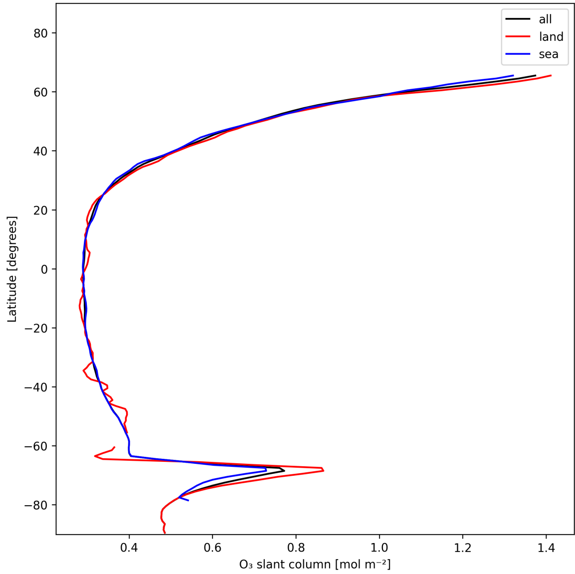
Figure 19: Zonal average of “O 3 slant column” for 2024-12-20 to 2024-12-20.
