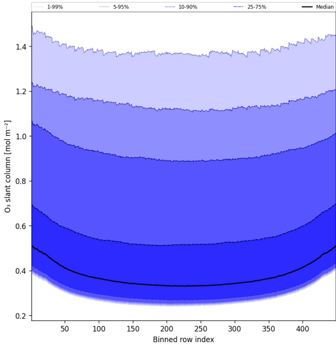
Figure 43: Along track statistics of “O 3 slant column” for 2024-12-20 to 2024-12-20
