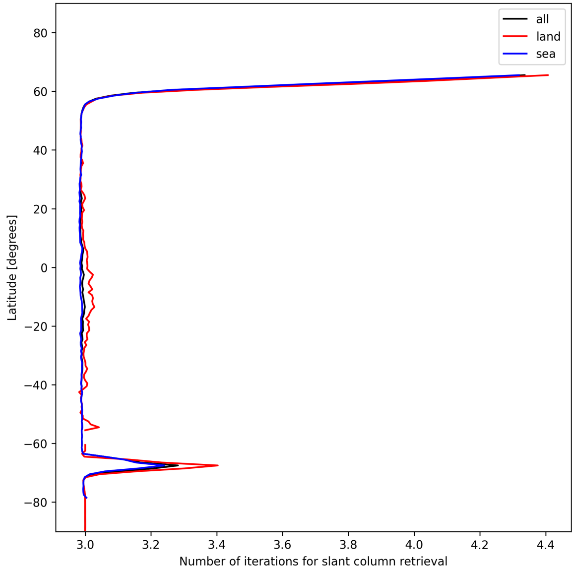
Figure 21: Zonal average of “Number of iterations for slant column retrieval” for 2024-12-20 to 2024-12-20.
