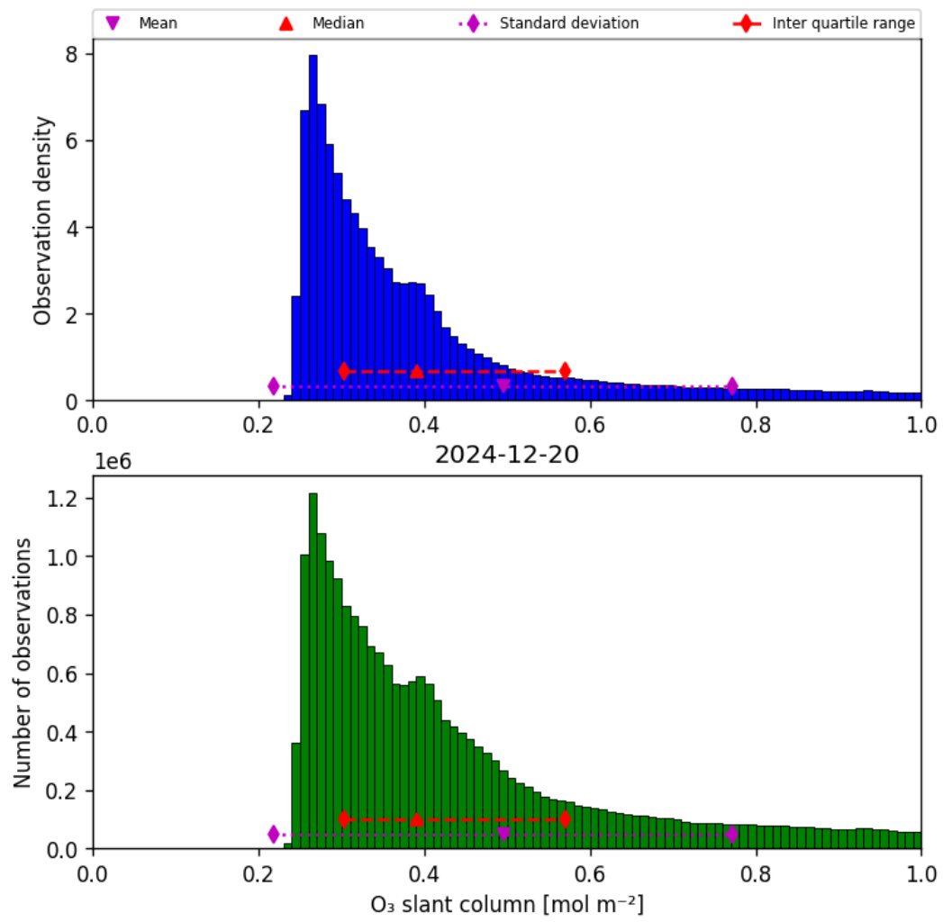
Figure 31: Histogram of “O 3 slant column” for 2024-12-20 to 2024-12-20
