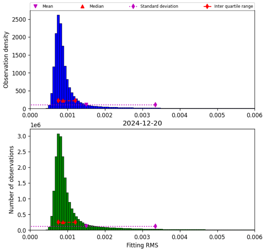
Figure 34: Histogram of “Fitting RMS” for 2024-12-20 to 2024-12-20
