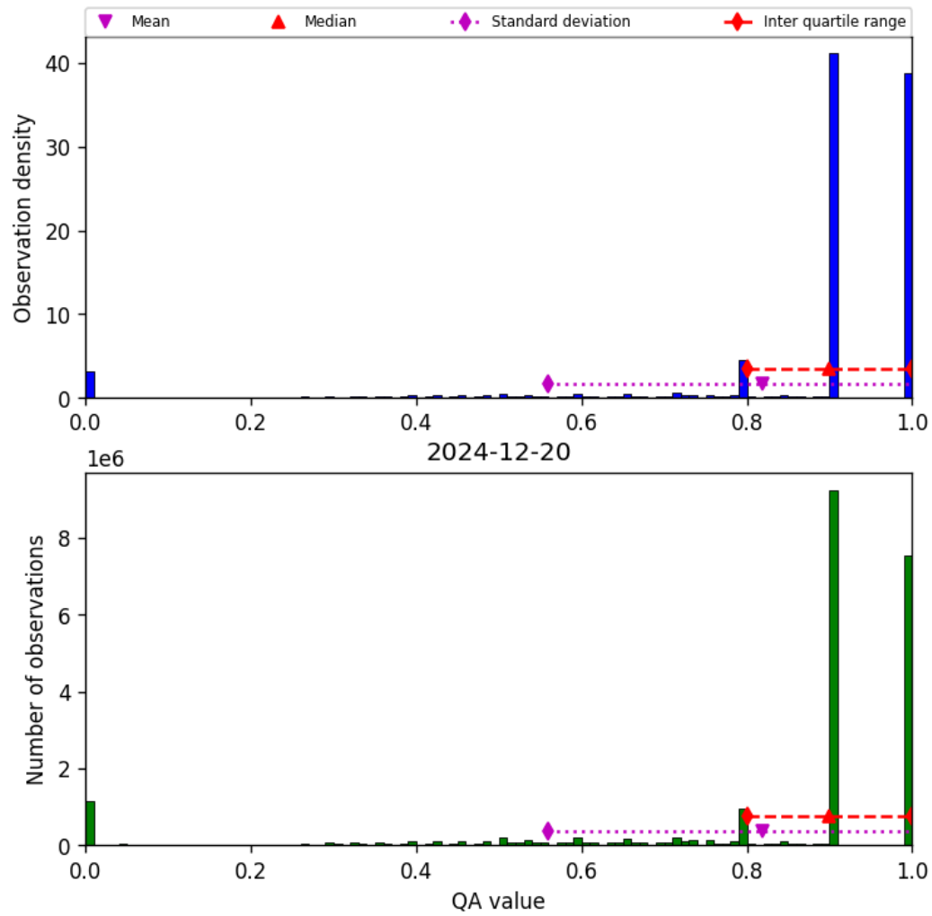
Figure 28: Histogram of “QA value” for 2024-12-20 to 2024-12-20
