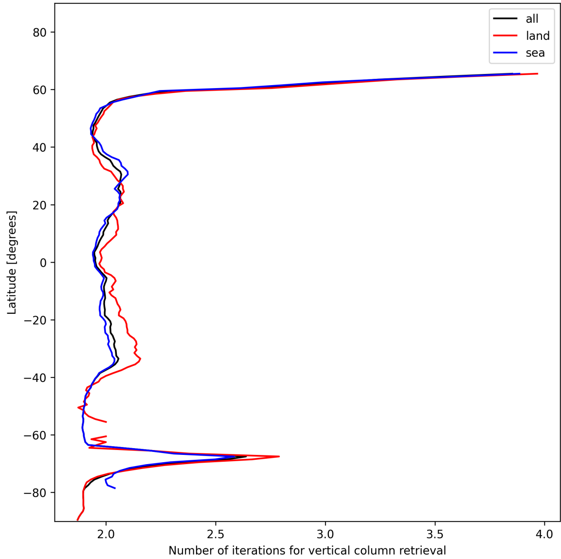
Figure 27: Zonal average of “Number of iterations for vertical column retrieval” for 2024-12-20 to 2024-12-20.
