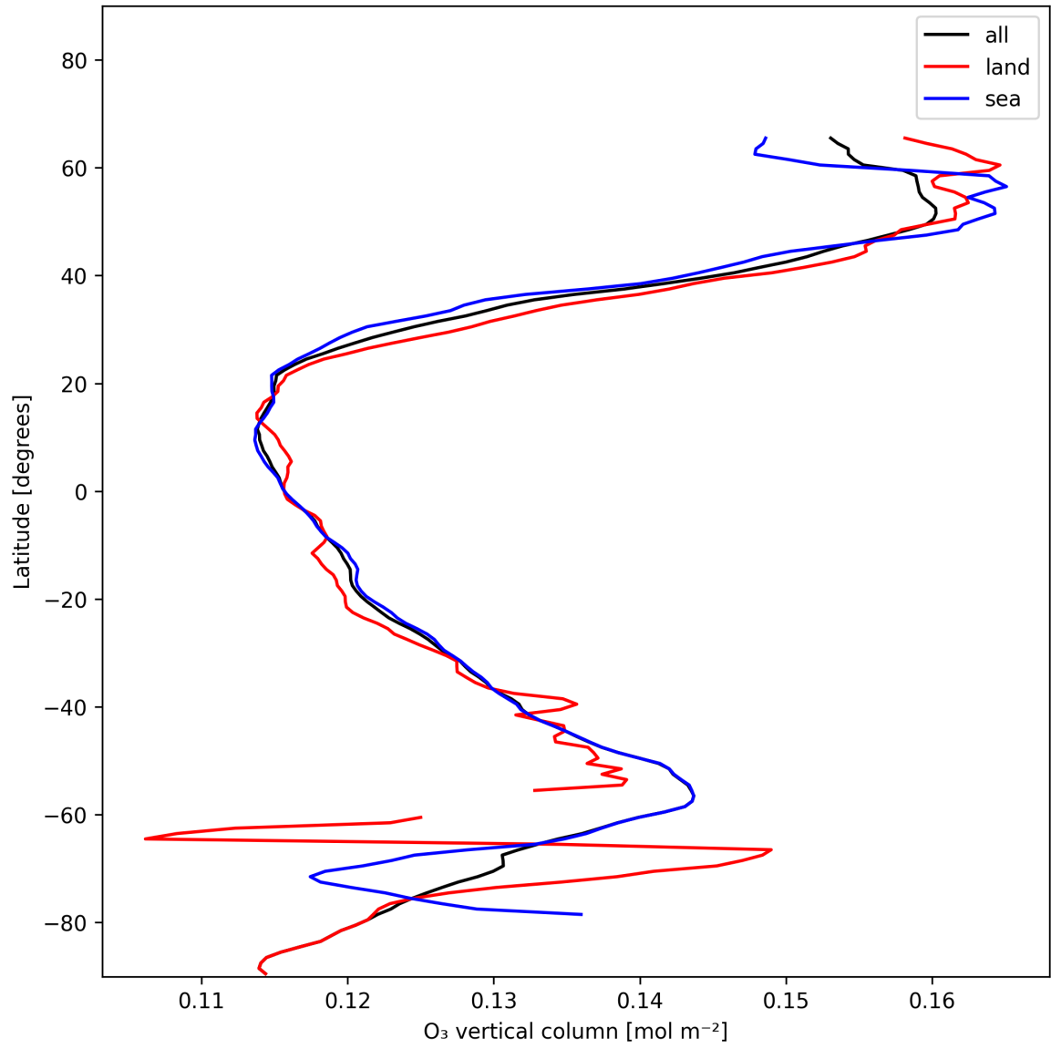
Figure 17: Zonal average of “O 3 vertical column” for 2024-12-20 to 2024-12-20.
