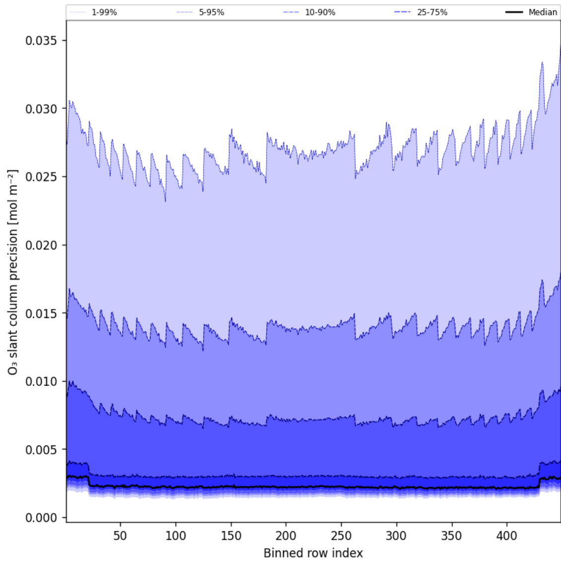
Figure 44: Along track statistics of "O 3 slant column precision" for 2024-12-20 to 2024-12-20
