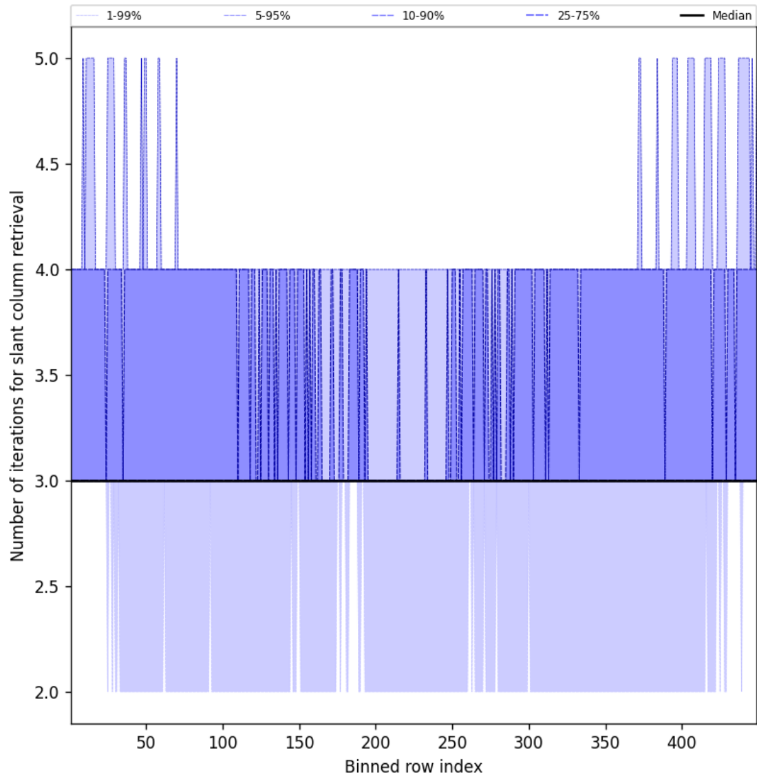
Figure 45: Along track statistics of “Number of iterations for slant column retrieval” for 2024-12-21 to 2024-12-22
