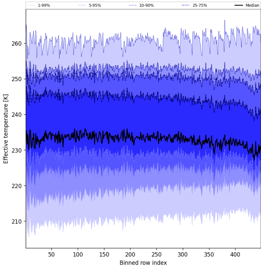
Figure 50: Along track statistics of “Effective temperature” for 2024-12-21 to 2024-12-22
