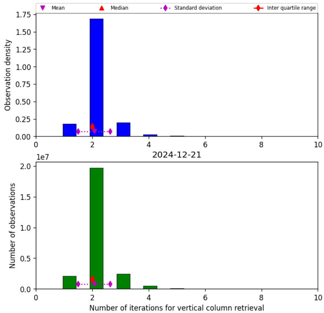
Figure 39: Histogram of “Number of iterations for vertical column retrieval” for 2024-12-21 to 2024-12-22
