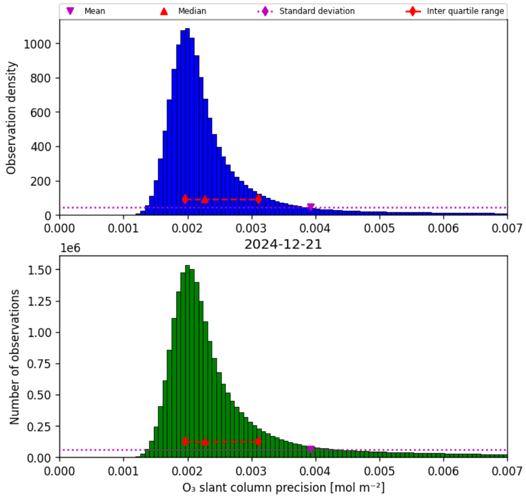
Figure 32: Histogram of “O 3 slant column precision” for 2024-12-21 to 2024-12-22
