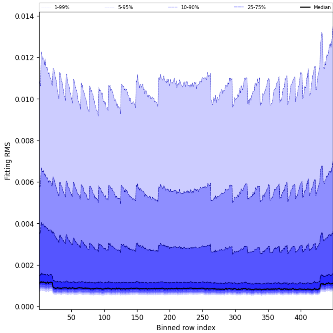
Figure 46: Along track statistics of “Fitting RMS” for 2024-12-21 to 2024-12-22
