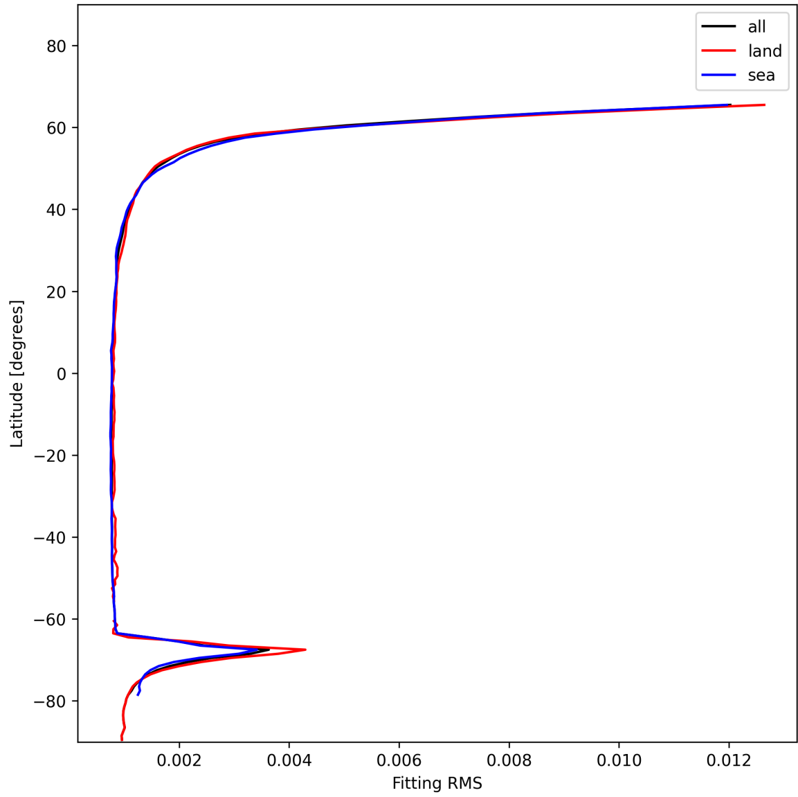
Figure 22: Zonal average of “Fitting RMS” for 2024-12-21 to 2024-12-22.
