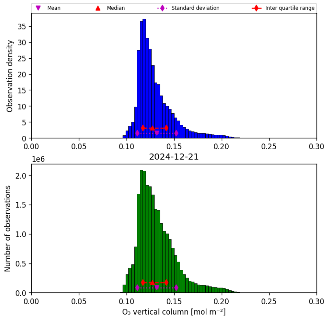
Figure 29: Histogram of “O 3 vertical column” for 2024-12-21 to 2024-12-22
