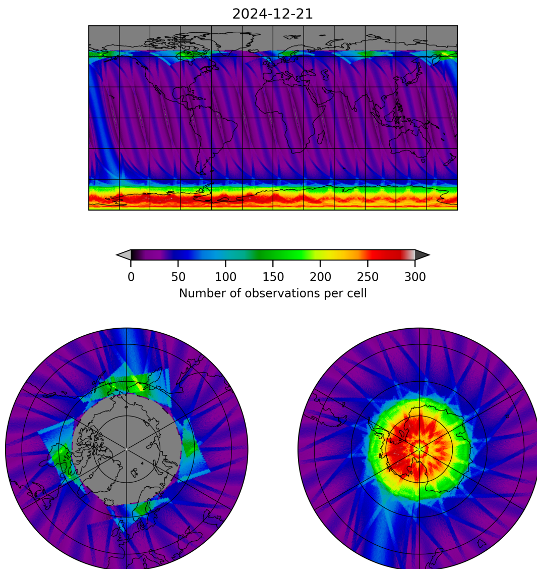
Figure 15: Map of the number of observations for 2024-12-21 to 2024-12-22
