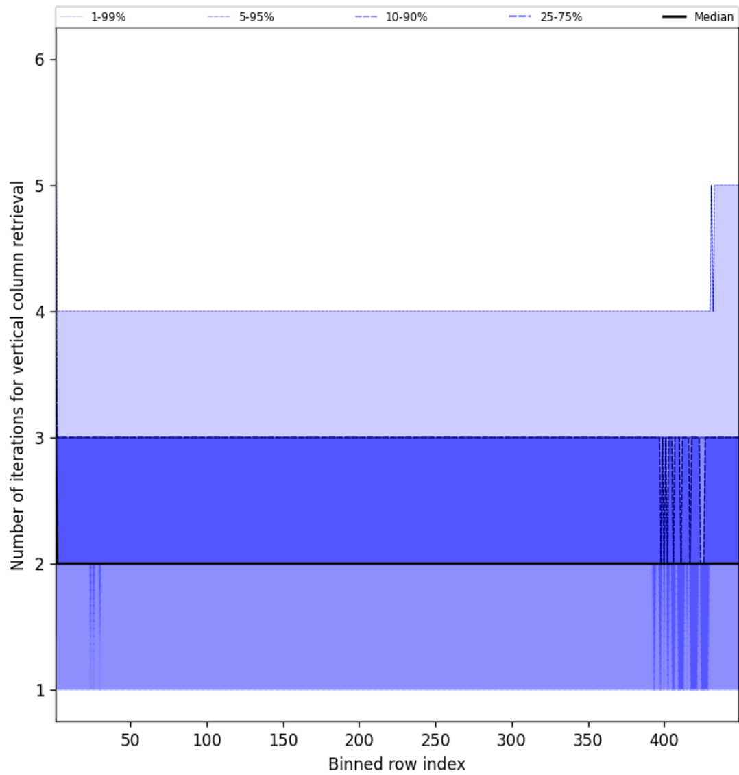
Figure 51: Along track statistics of “Number of iterations for vertical column retrieval” for 2024-12-21 to 2024-12-22
