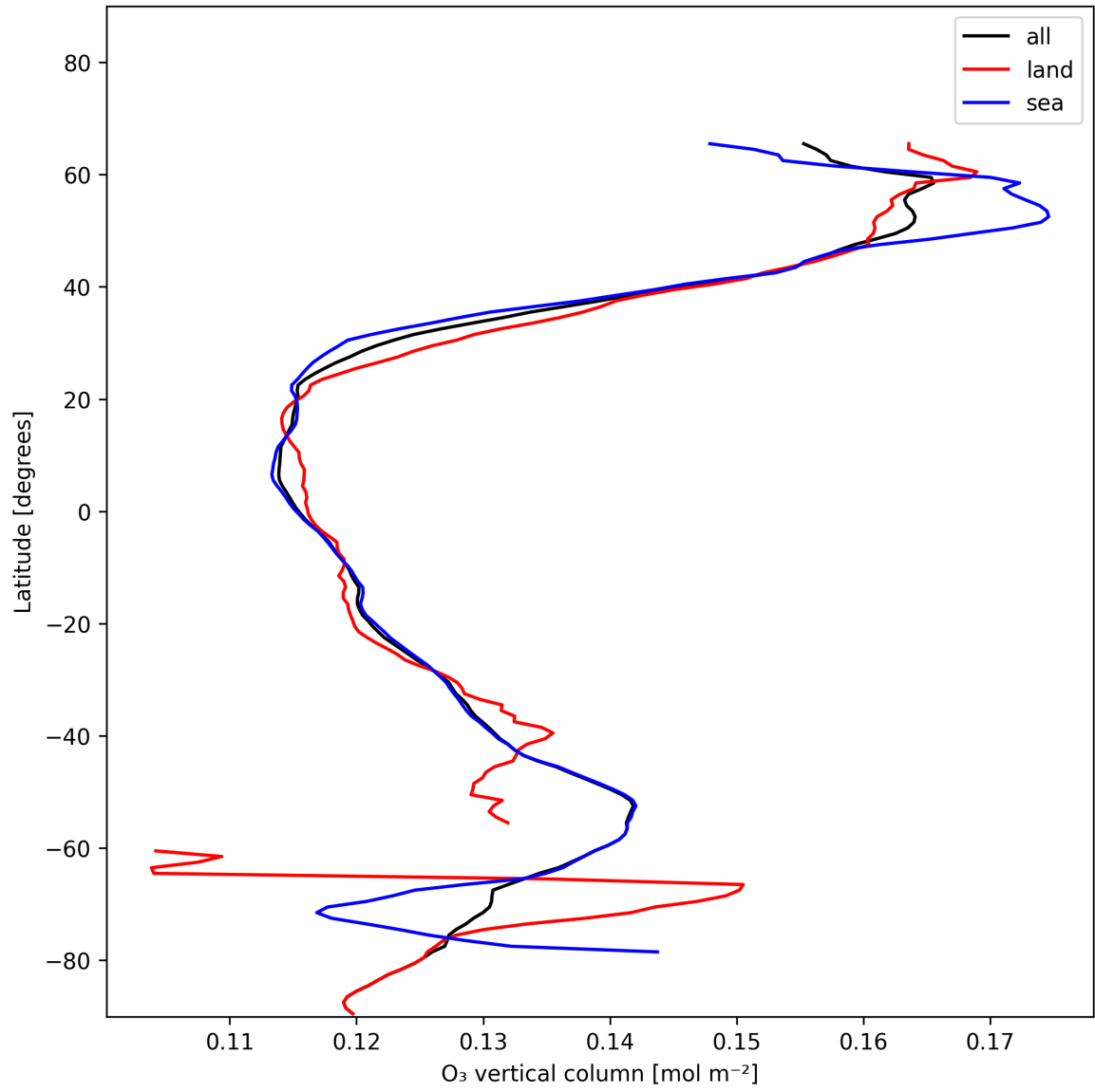
Figure 17: Zonal average of “O 3 vertical column” for 2024-12-21 to 2024-12-22.
