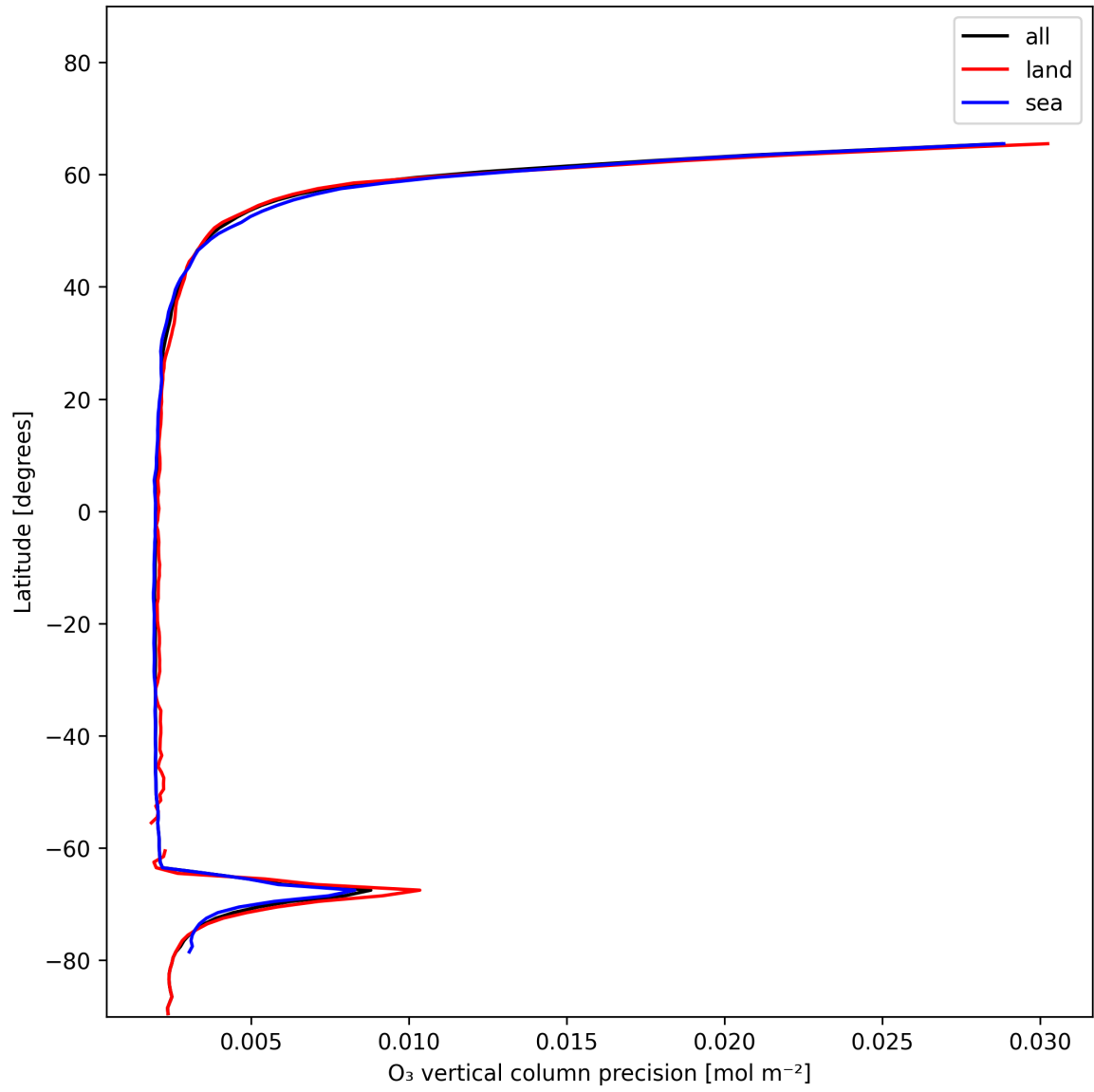
Figure 18: Zonal average of “O 3 vertical column precision” for 2024-12-21 to 2024-12-22.
