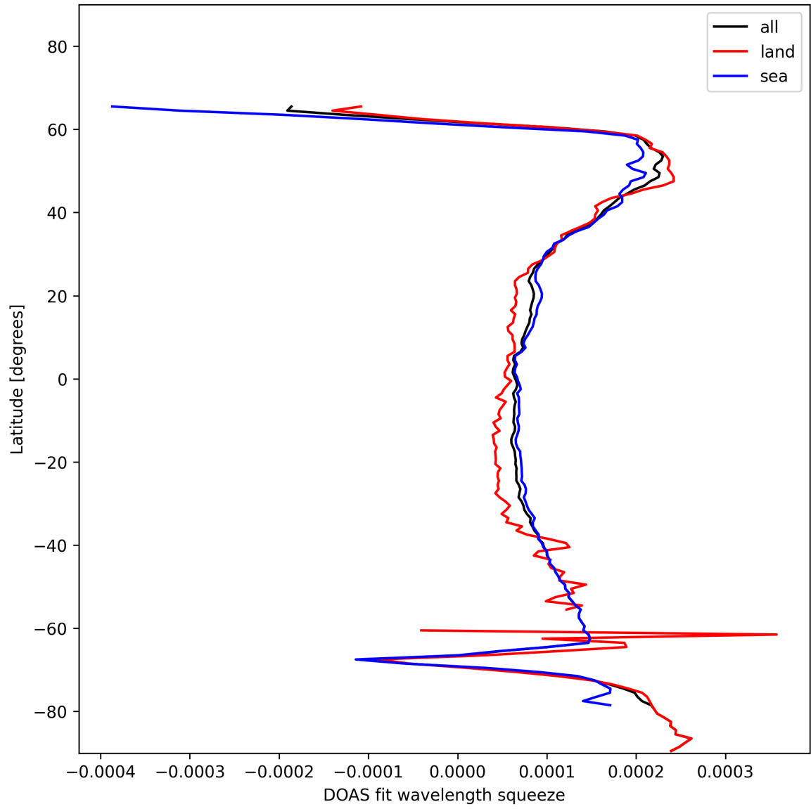
Figure 24: Zonal average of “DOAS fit wavelength squeeze” for 2024-12-21 to 2024-12-22.
