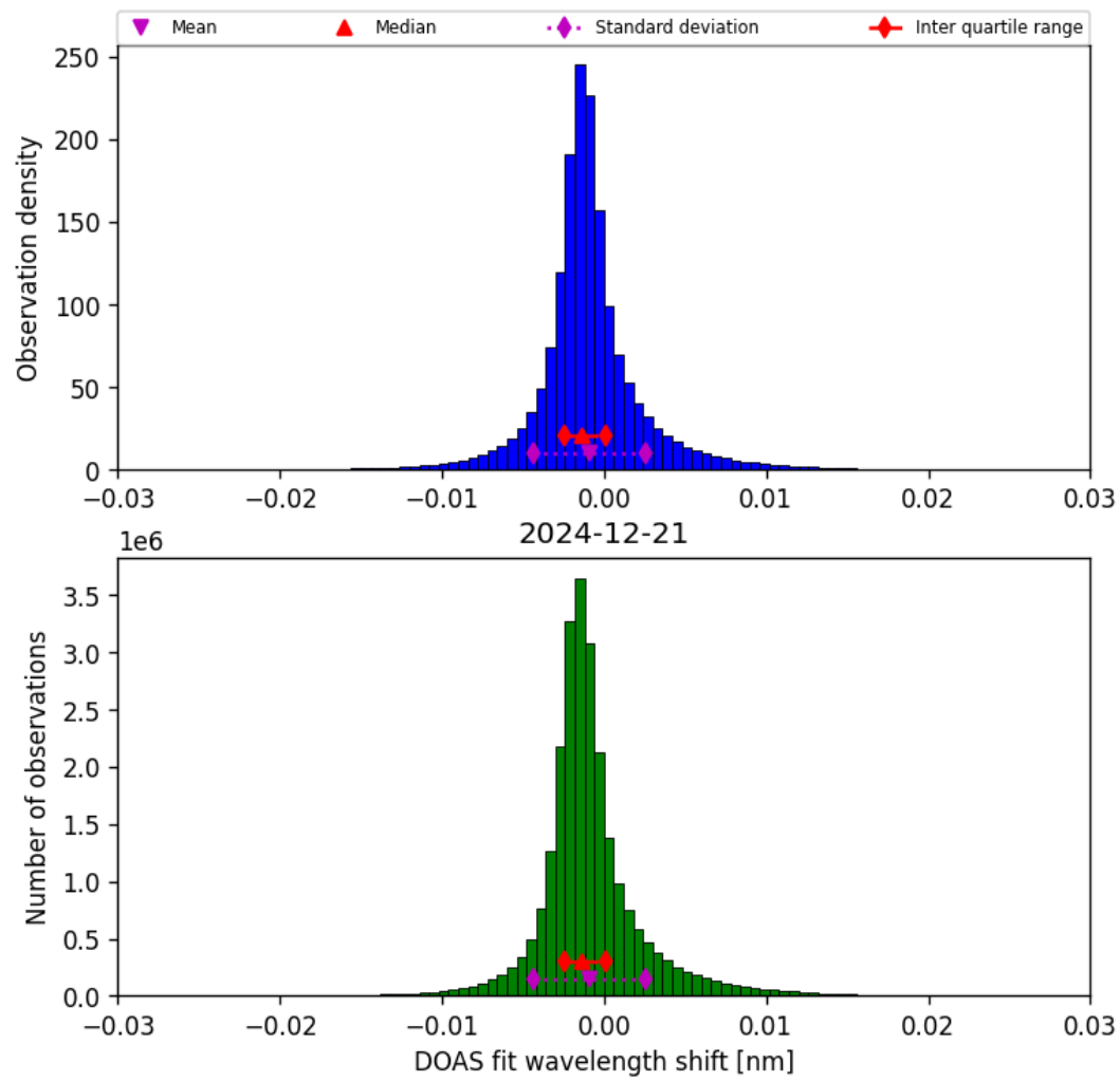
Figure 35: Histogram of “DOAS fit wavelength shift” for 2024-12-21 to 2024-12-22
