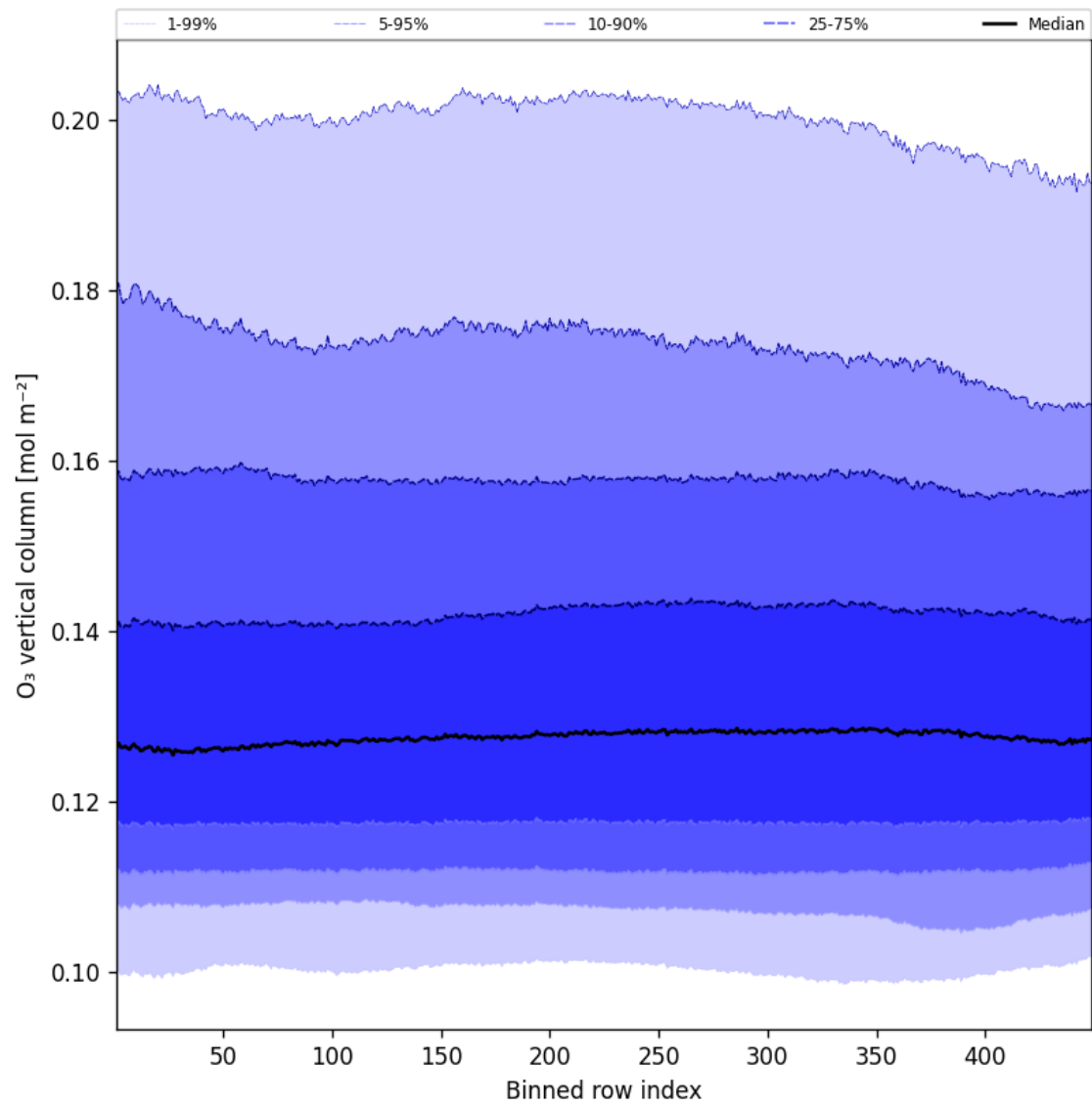
Figure 41: Along track statistics of “O 3 vertical column” for 2024-12-21 to 2024-12-22
