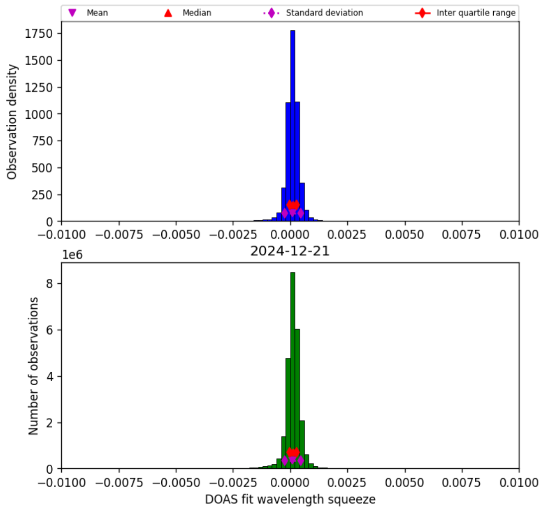
Figure 36: Histogram of “DOAS fit wavelength squeeze” for 2024-12-21 to 2024-12-22
