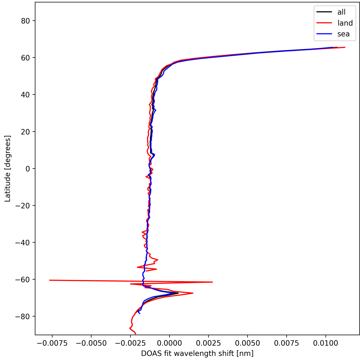
Figure 23: Zonal average of "DOAS fit wavelength shift" for 2024-12-21 to 2024-12-22.
