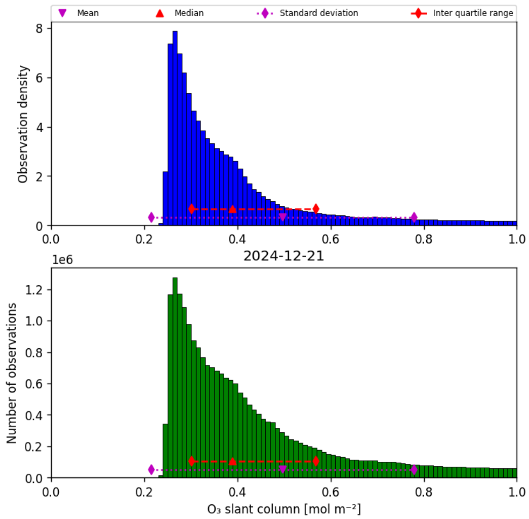
Figure 31: Histogram of “O 3 slant column” for 2024-12-21 to 2024-12-22
