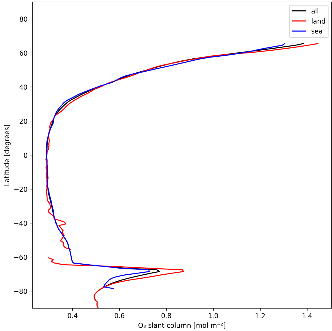
Figure 19: Zonal average of “O 3 slant column” for 2024-12-21 to 2024-12-22.
