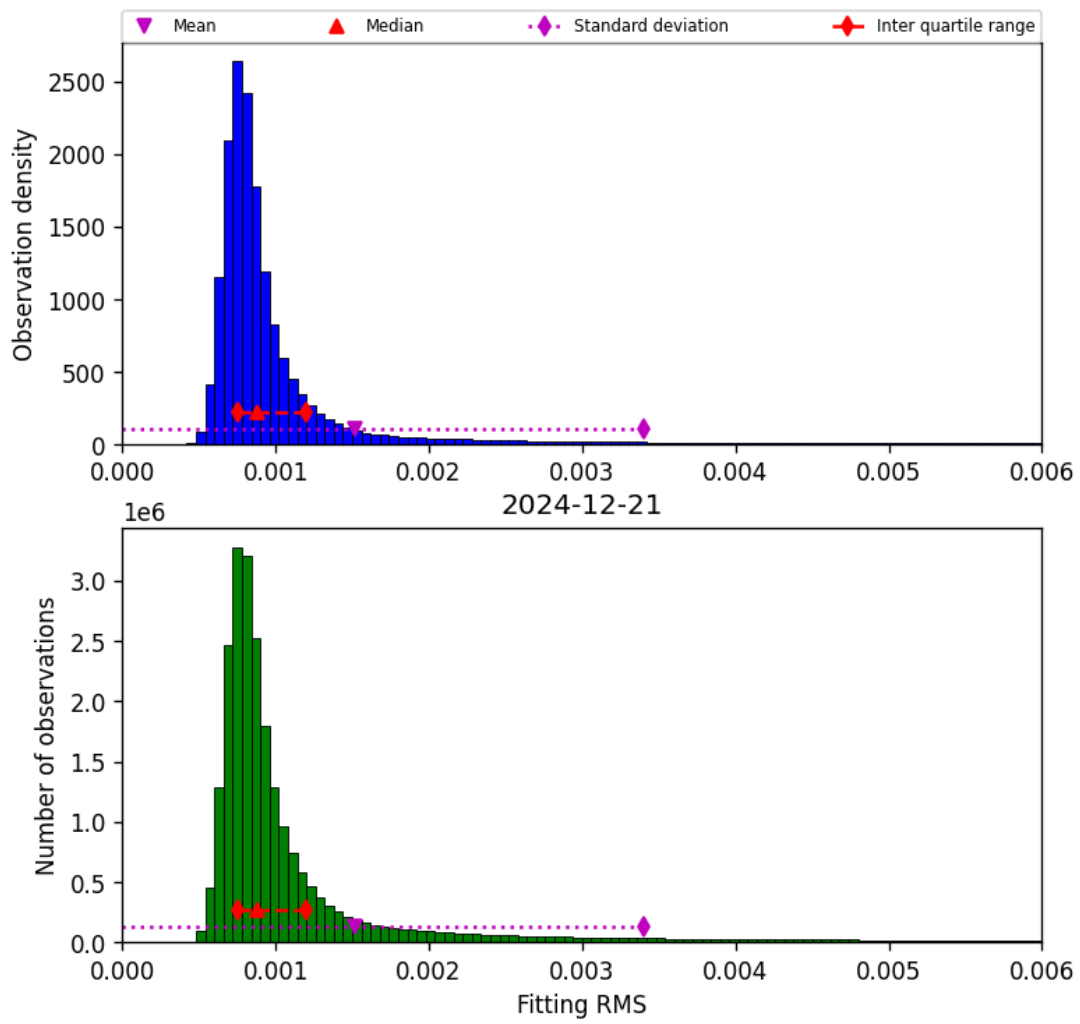
Figure 34: Histogram of “Fitting RMS” for 2024-12-21 to 2024-12-22
