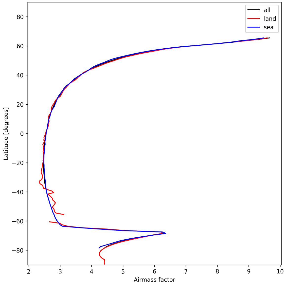
Figure 25: Zonal average of “Airmass factor” for 2024-12-21 to 2024-12-22.
