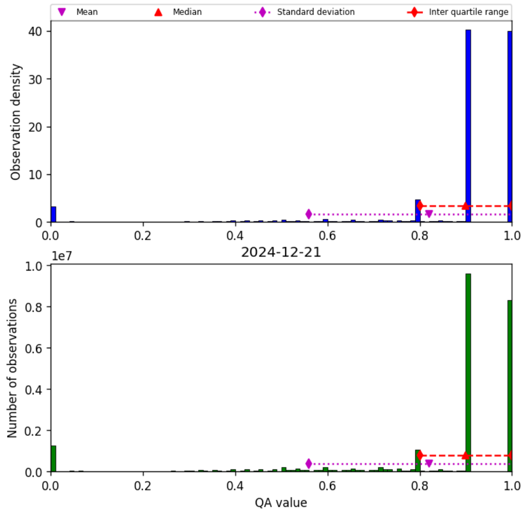
Figure 28: Histogram of “QA value” for 2024-12-21 to 2024-12-22
