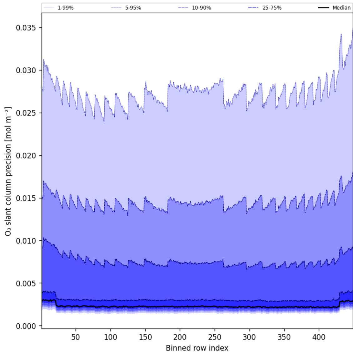
Figure 44: Along track statistics of “O 3 slant column precision” for 2024-12-21 to 2024-12-22
