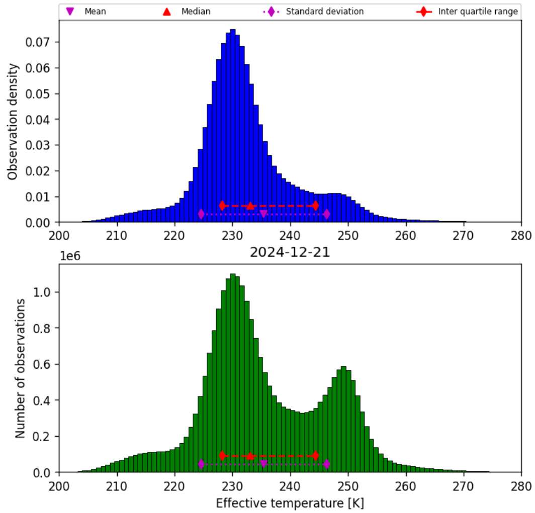
Figure 38: Histogram of “Effective temperature” for 2024-12-21 to 2024-12-22
