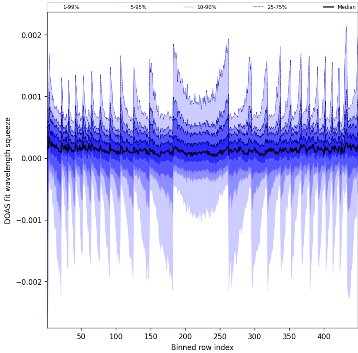
Figure 48: Along track statistics of “DOAS fit wavelength squeeze” for 2024-12-21 to 2024-12-22
