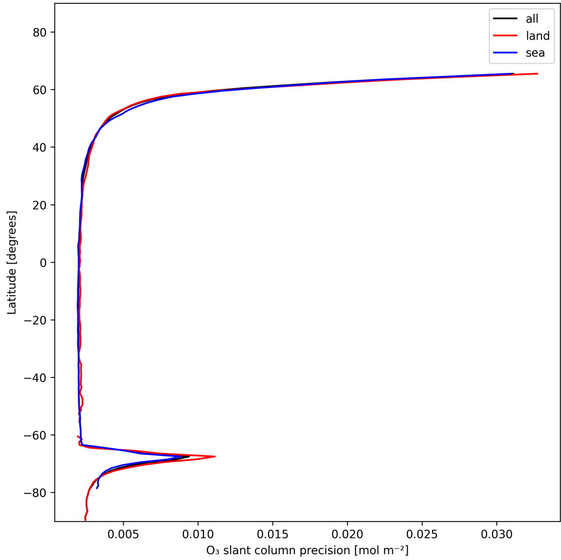
Figure 20: Zonal average of “O 3 slant column precision” for 2024-12-21 to 2024-12-22.
