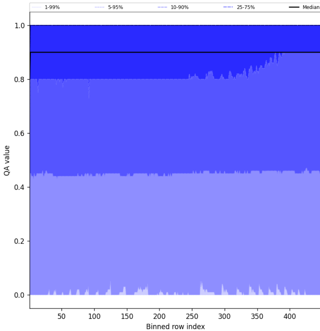
Figure 40: Along track statistics of “QA value” for 2024-12-21 to 2024-12-22
