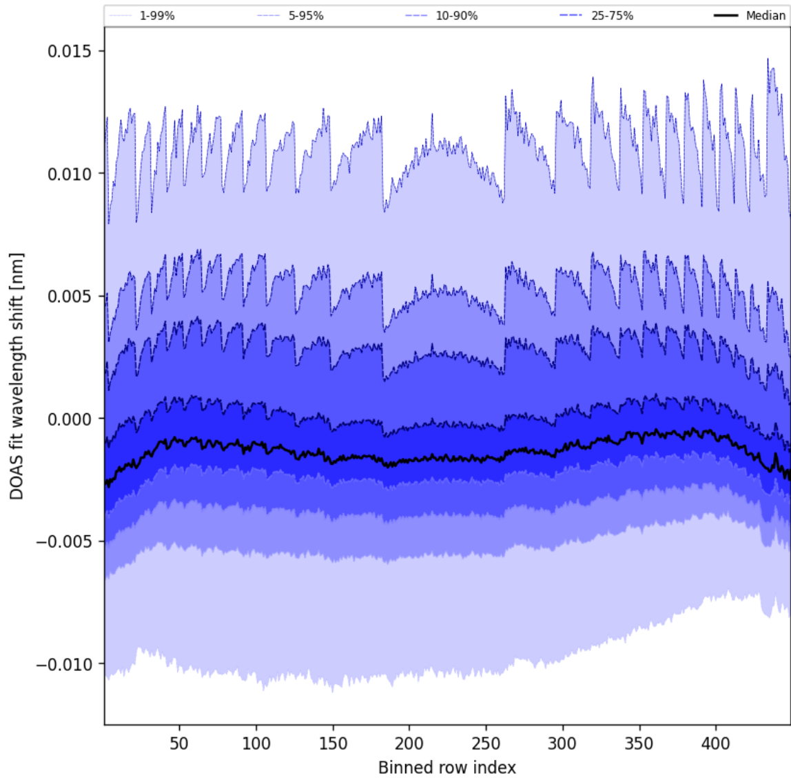
Figure 47: Along track statistics of “DOAS fit wavelength shift” for 2024-12-21 to 2024-12-22
