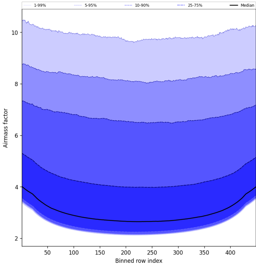
Figure 49: Along track statistics of “Airmass factor” for 2024-12-21 to 2024-12-22
