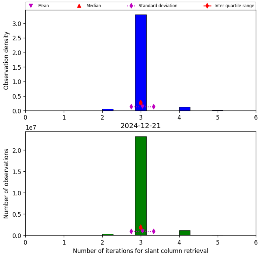
Figure 33: Histogram of “Number of iterations for slant column retrieval” for 2024-12-21 to 2024-12-22
