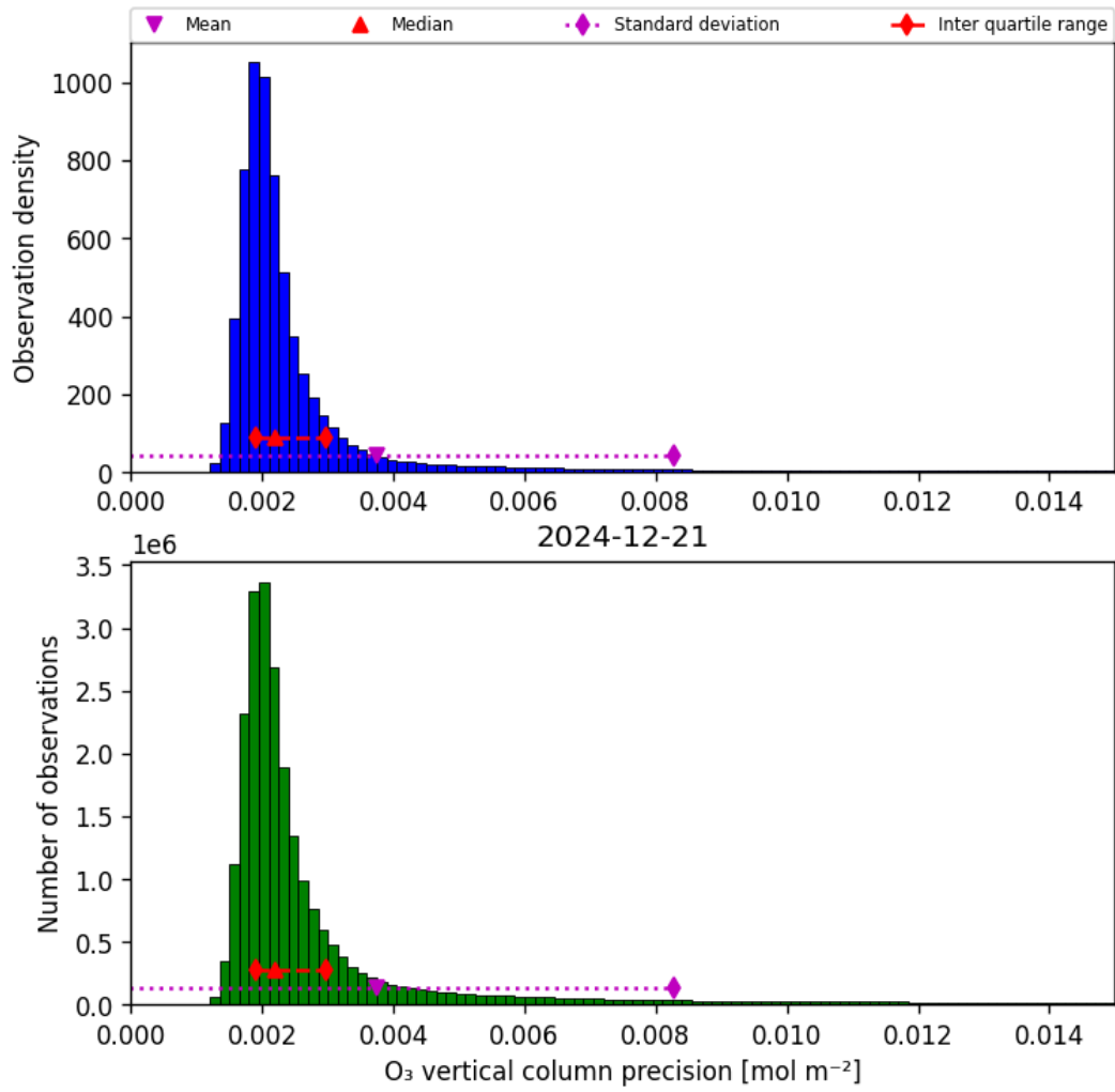
Figure 30: Histogram of “O 3 vertical column precision” for 2024-12-21 to 2024-12-22
