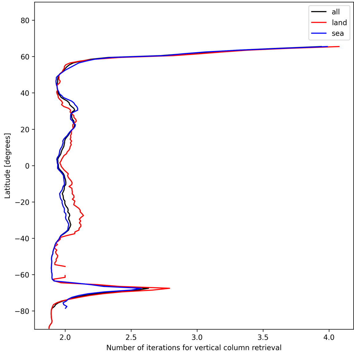
Figure 27: Zonal average of “Number of iterations for vertical column retrieval” for 2024-12-21 to 2024-12-22.
