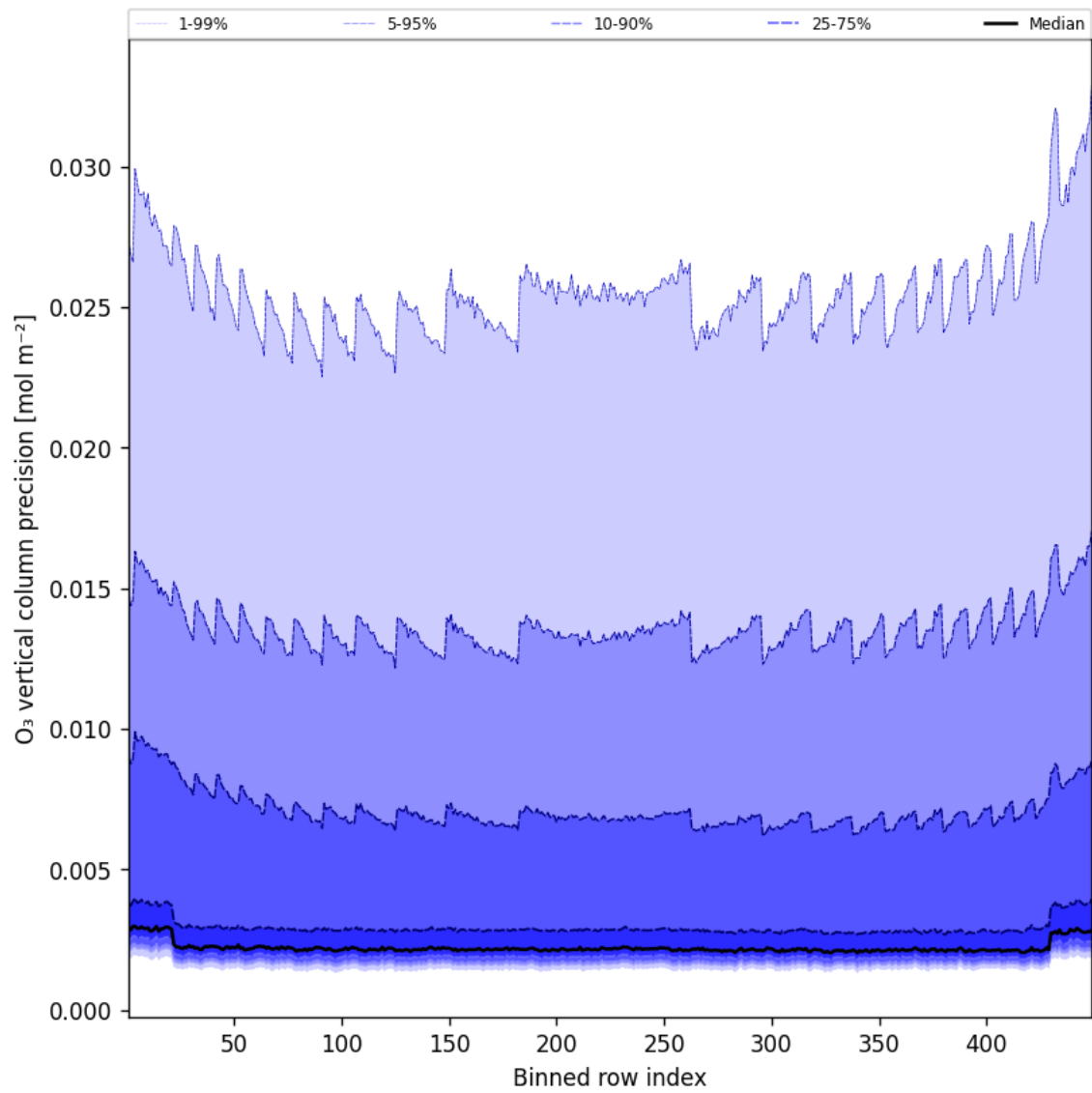
Figure 42: Along track statistics of “O 3 vertical column precision” for 2024-12-21 to 2024-12-22
