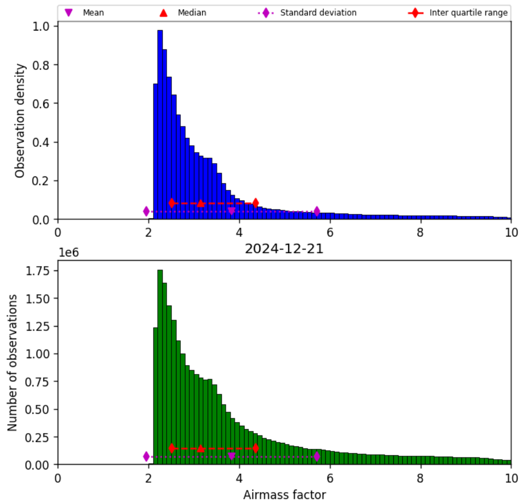
Figure 37: Histogram of “Airmass factor” for 2024-12-21 to 2024-12-22
