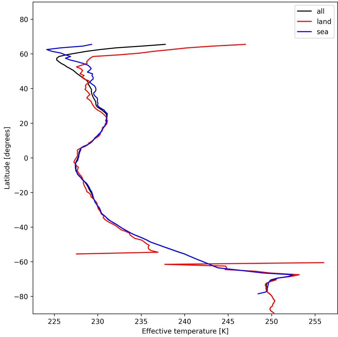
Figure 26: Zonal average of “Effective temperature” for 2024-12-21 to 2024-12-22.
