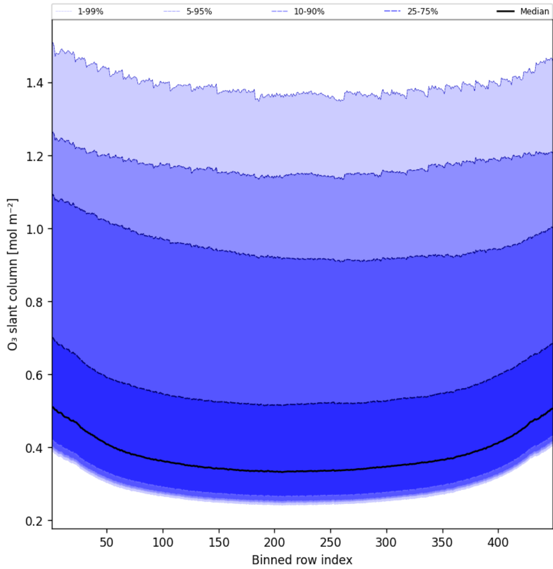
Figure 43: Along track statistics of “O 3 slant column” for 2024-12-21 to 2024-12-22
