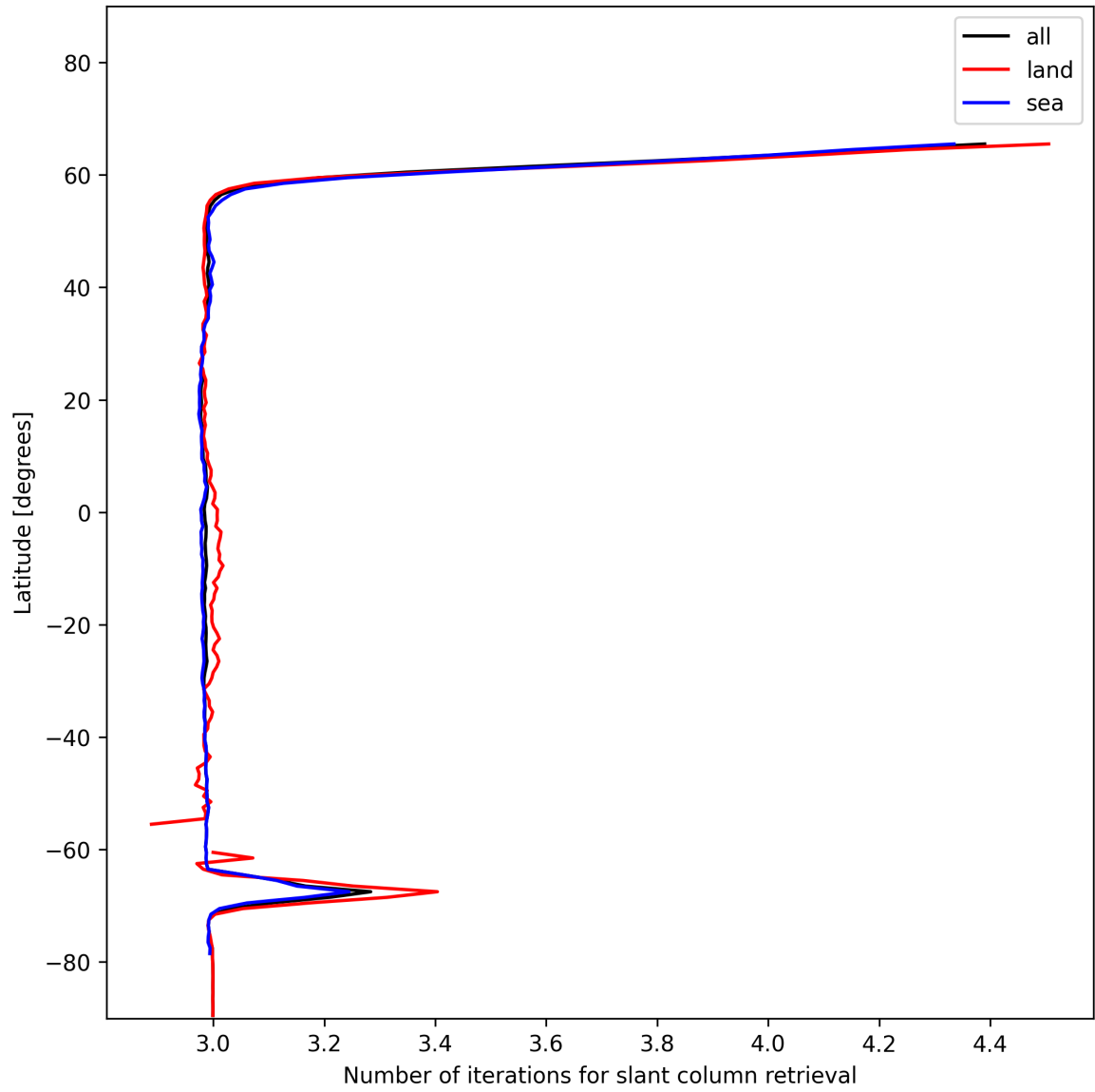
Figure 21: Zonal average of “Number of iterations for slant column retrieval” for 2024-12-21 to 2024-12-22.
