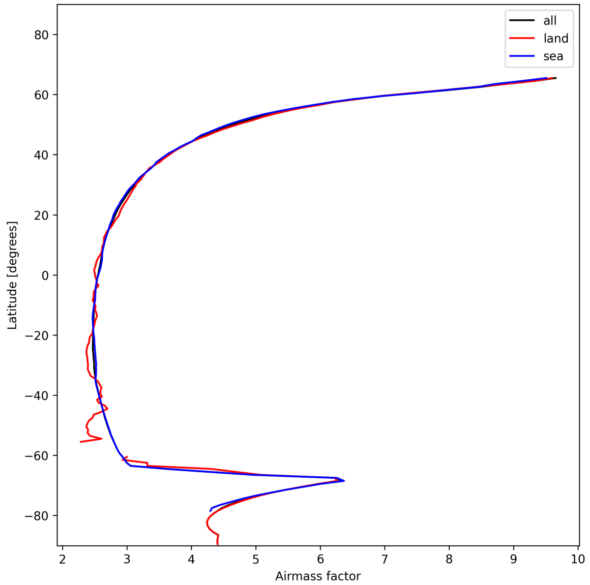
Figure 25: Zonal average of “Airmass factor” for 2024-12-22 to 2024-12-23.
