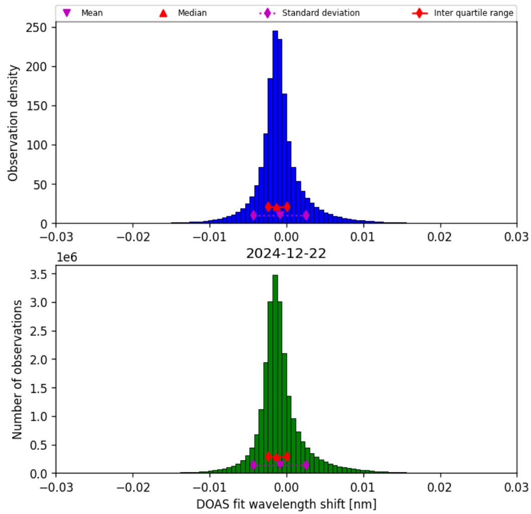
Figure 35: Histogram of “DOAS fit wavelength shift” for 2024-12-22 to 2024-12-23
