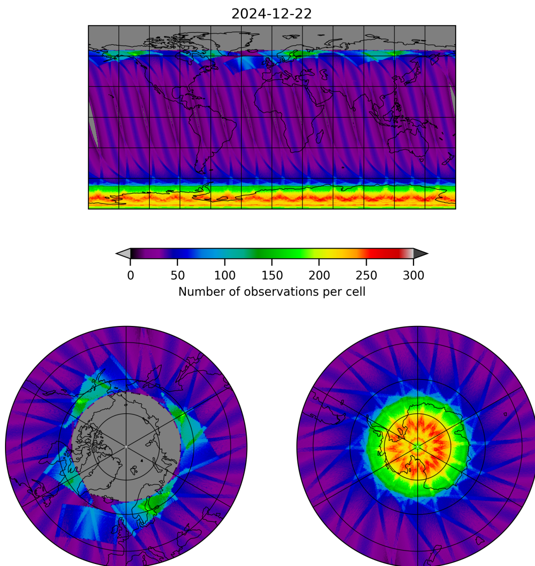
Figure 15: Map of the number of observations for 2024-12-22 to 2024-12-23
