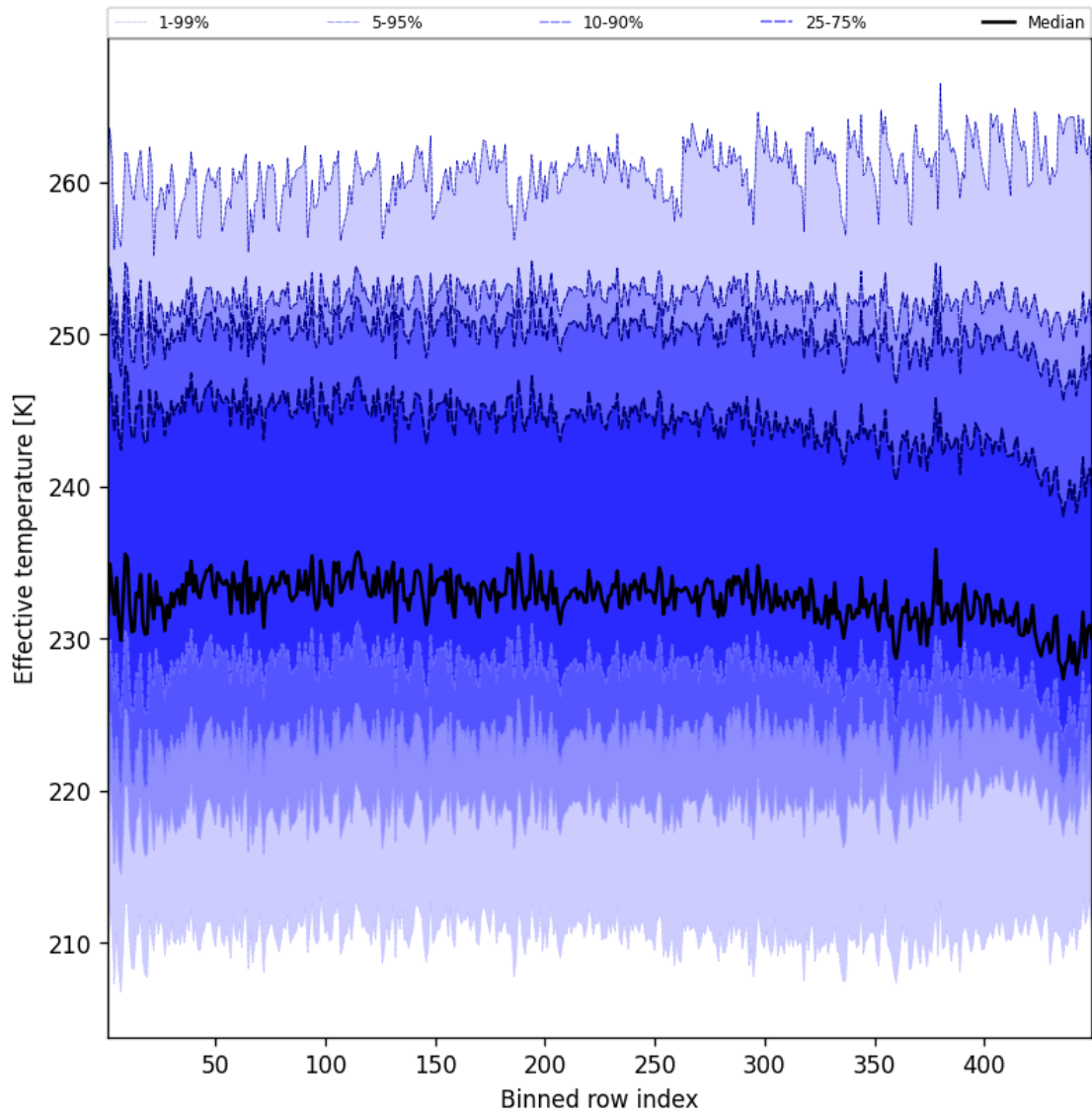
Figure 50: Along track statistics of “Effective temperature” for 2024-12-22 to 2024-12-23
