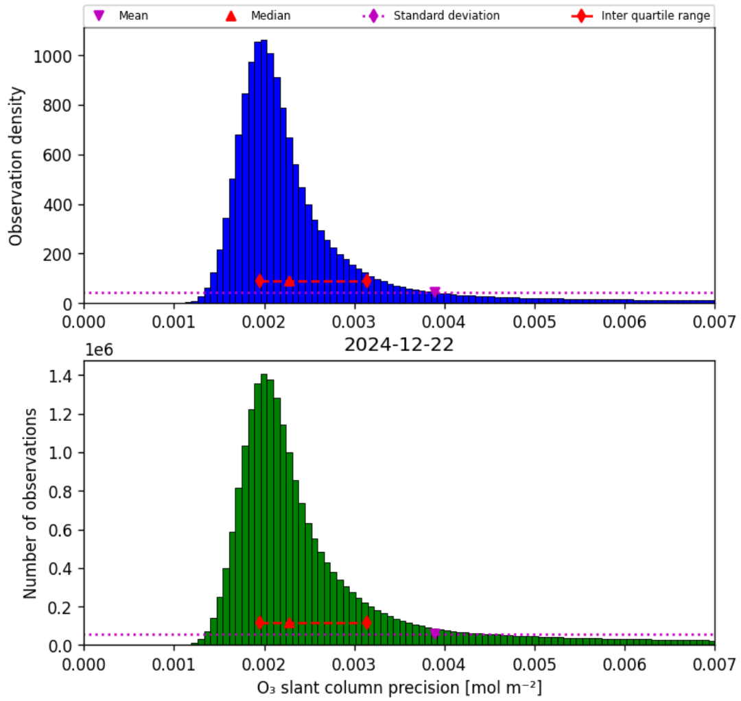
Figure 32: Histogram of “O 3 slant column precision” for 2024-12-22 to 2024-12-23
