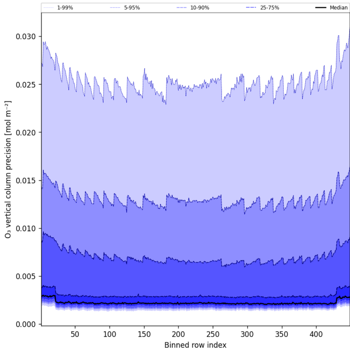
Figure 42: Along track statistics of “O 3 vertical column precision” for 2024-12-22 to 2024-12-23
