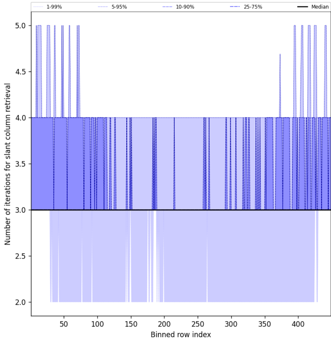
Figure 45: Along track statistics of “Number of iterations for slant column retrieval” for 2024-12-22 to 2024-12-23
