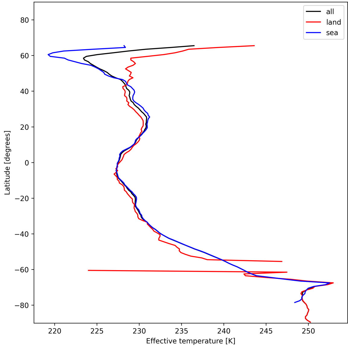
Figure 26: Zonal average of “Effective temperature” for 2024-12-22 to 2024-12-23.
