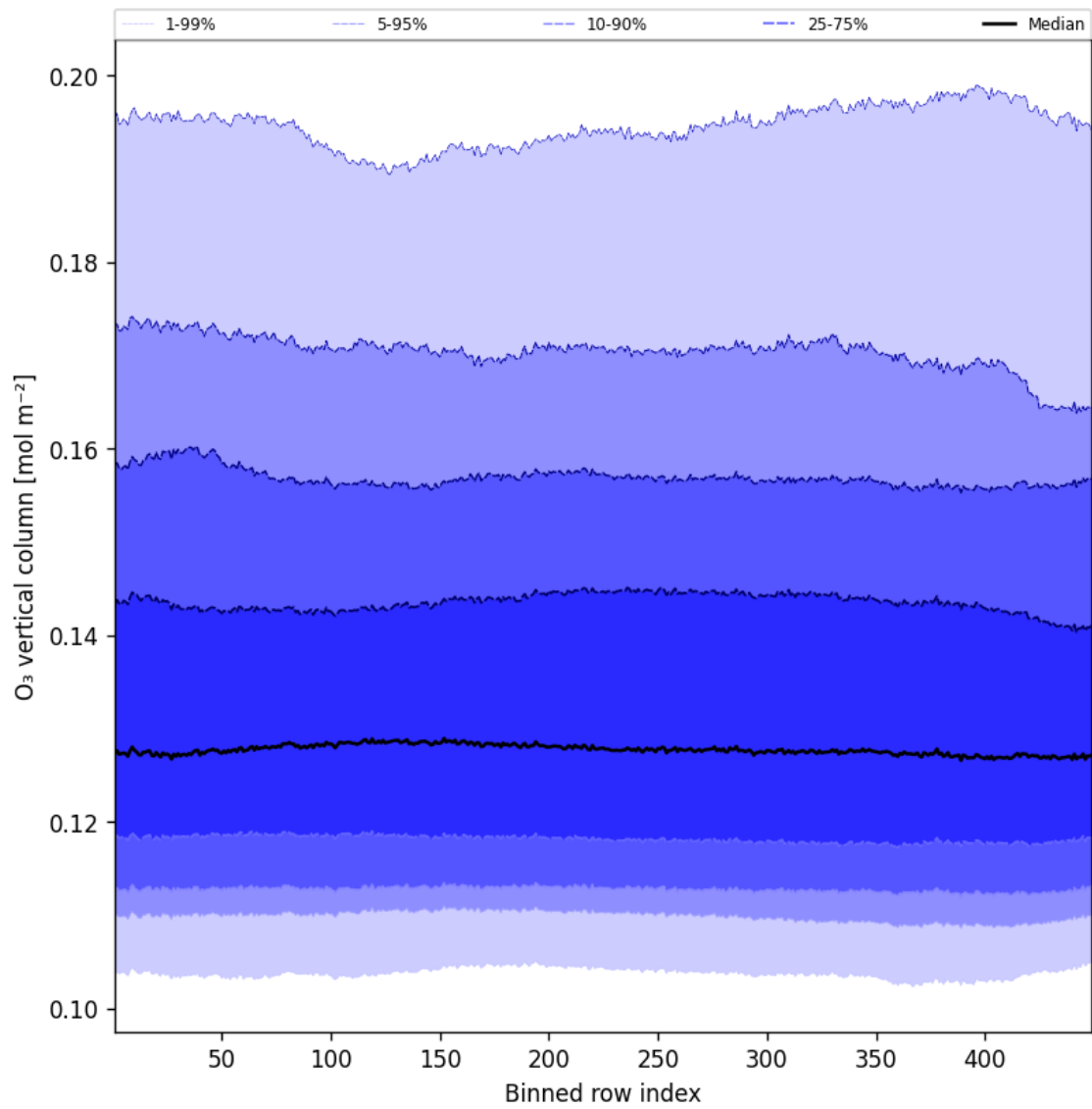
Figure 41: Along track statistics of “O 3 vertical column” for 2024-12-22 to 2024-12-23
