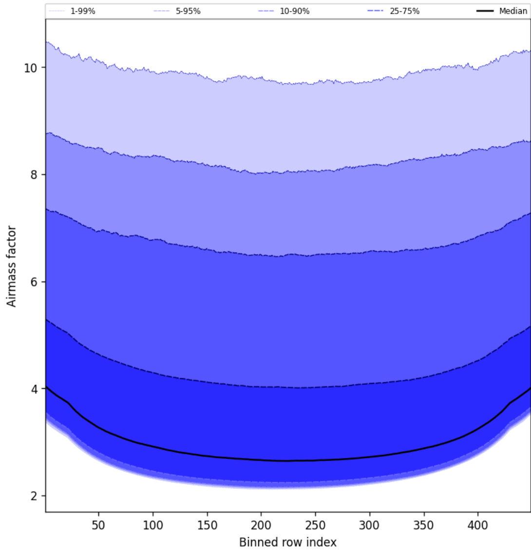
Figure 49: Along track statistics of “Airmass factor” for 2024-12-22 to 2024-12-23
