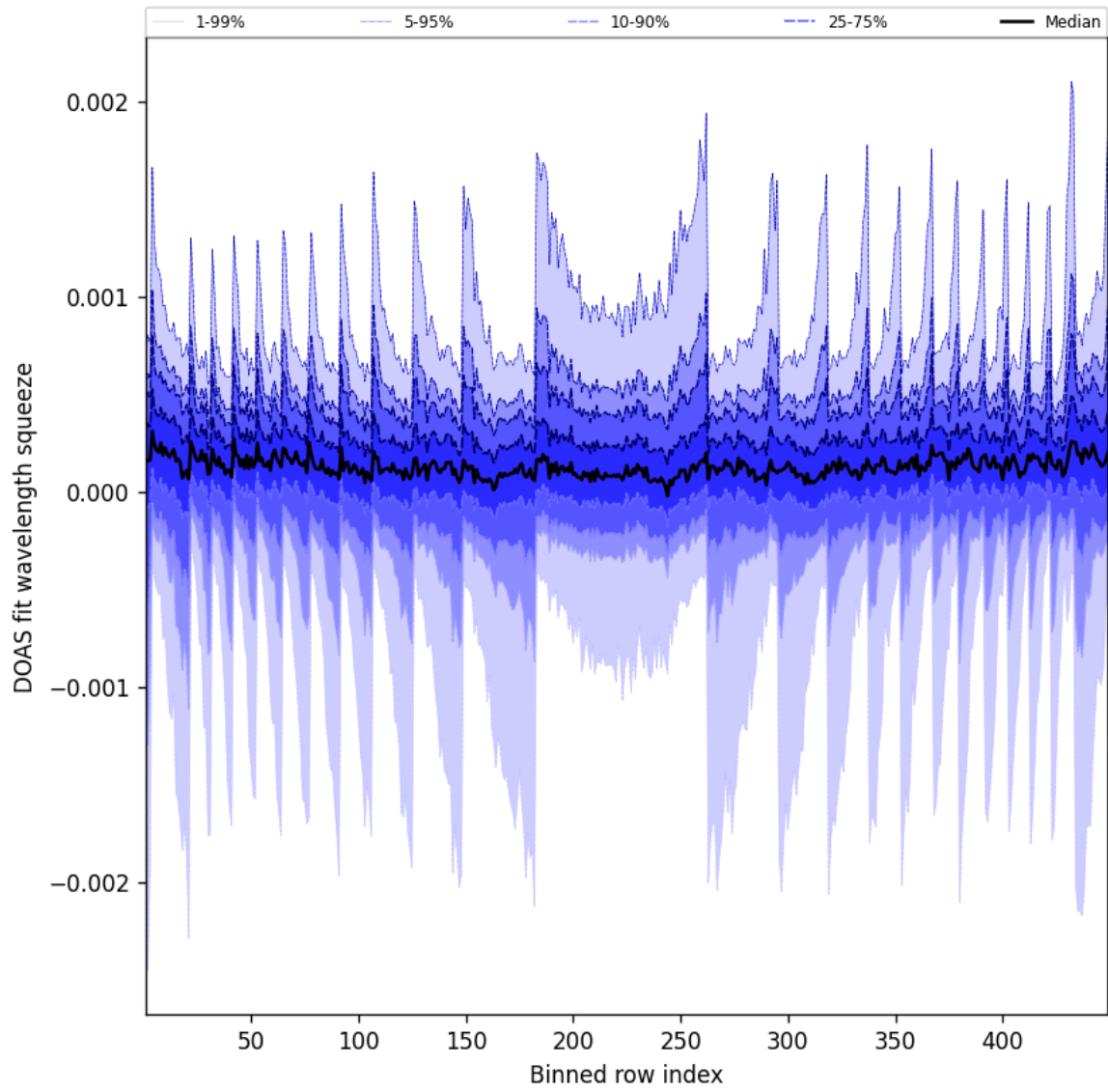
Figure 48: Along track statistics of “DOAS fit wavelength squeeze” for 2024-12-22 to 2024-12-23
