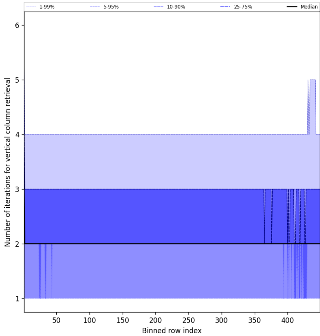
Figure 51: Along track statistics of “Number of iterations for vertical column retrieval” for 2024-12-22 to 2024-12-23
