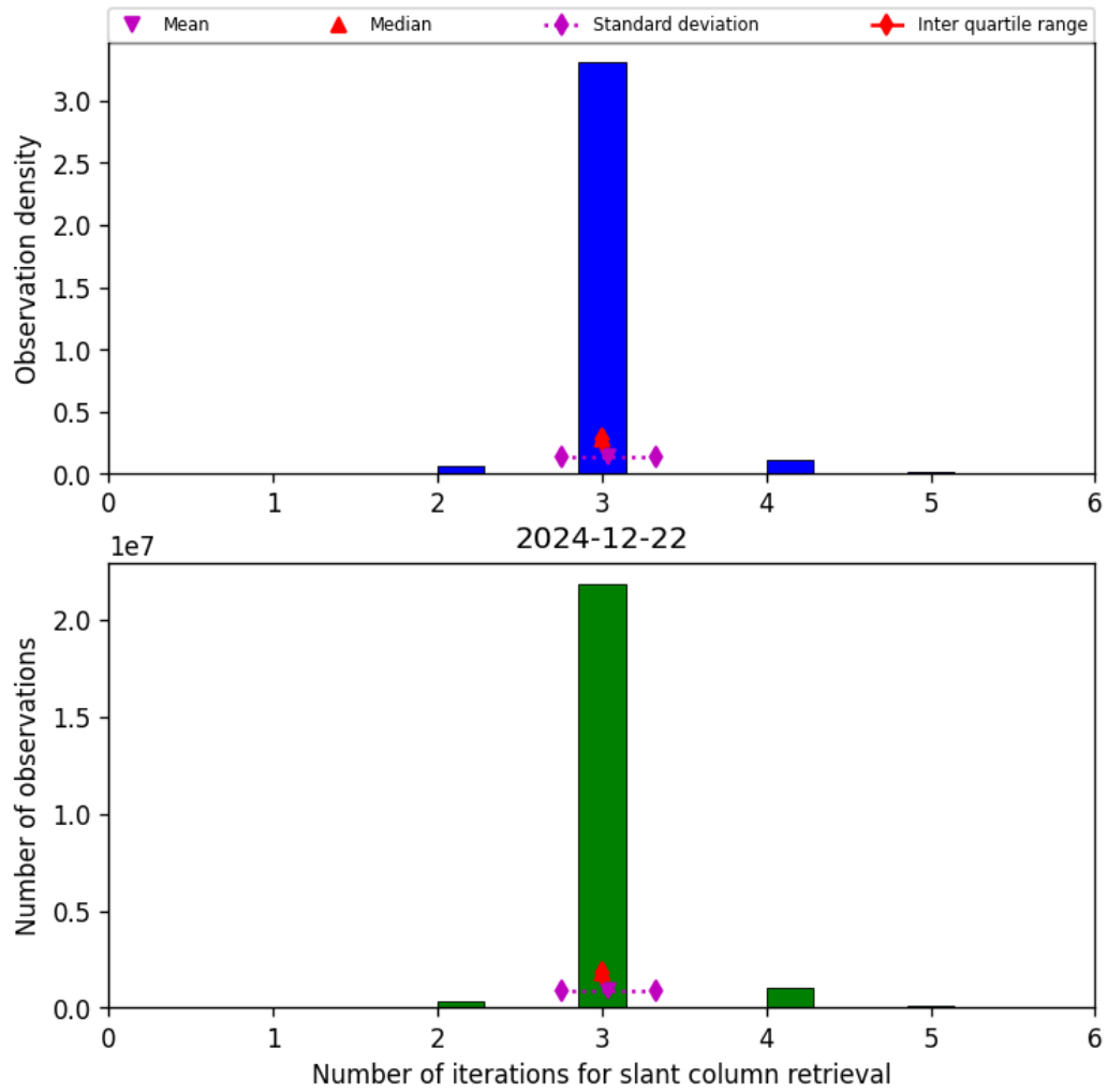
Figure 33: Histogram of “Number of iterations for slant column retrieval” for 2024-12-22 to 2024-12-23
