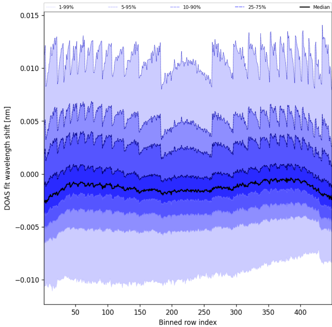
Figure 47: Along track statistics of “DOAS fit wavelength shift” for 2024-12-22 to 2024-12-23
