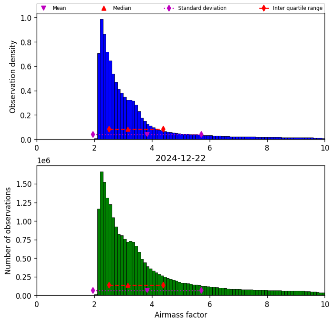
Figure 37: Histogram of “Airmass factor” for 2024-12-22 to 2024-12-23
