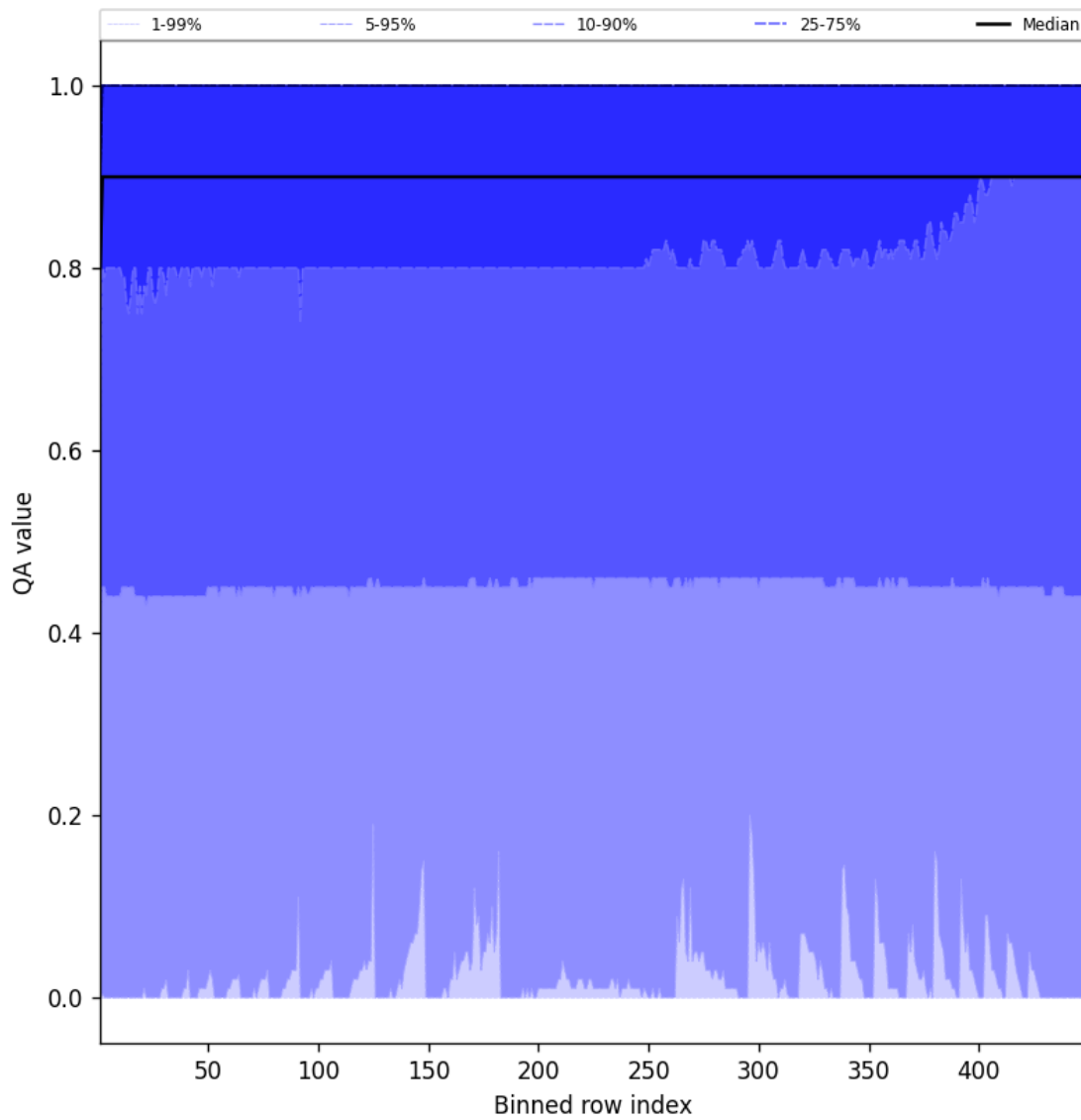
Figure 40: Along track statistics of “QA value” for 2024-12-22 to 2024-12-23
