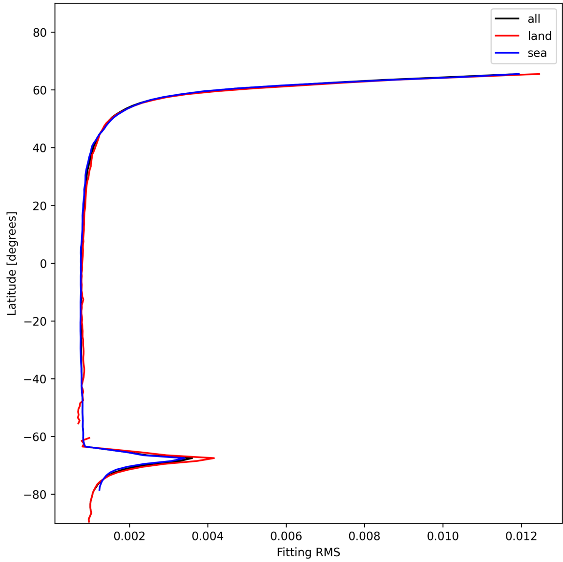
Figure 22: Zonal average of “Fitting RMS” for 2024-12-22 to 2024-12-23.
