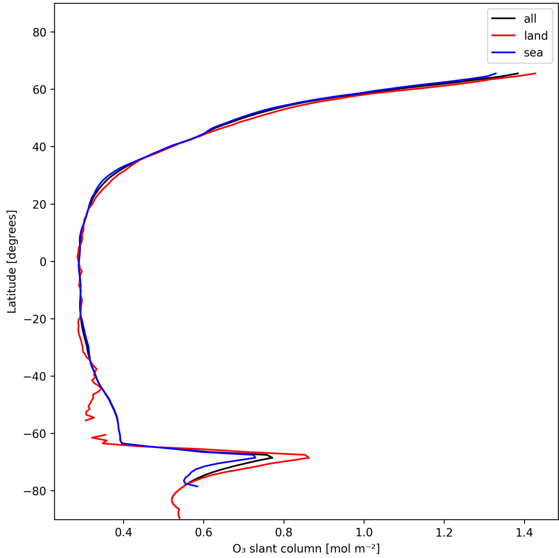
Figure 19: Zonal average of “O 3 slant column” for 2024-12-22 to 2024-12-23.
