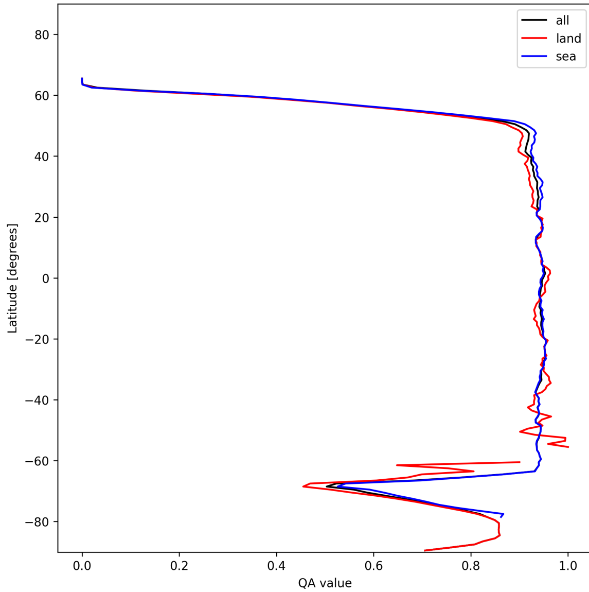
Figure 16: Zonal average of “QA value” for 2024-12-22 to 2024-12-23.
