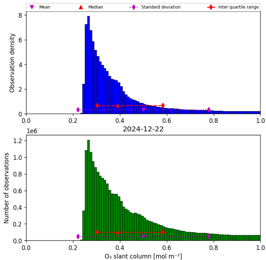
Figure 31: Histogram of “O 3 slant column” for 2024-12-22 to 2024-12-23
