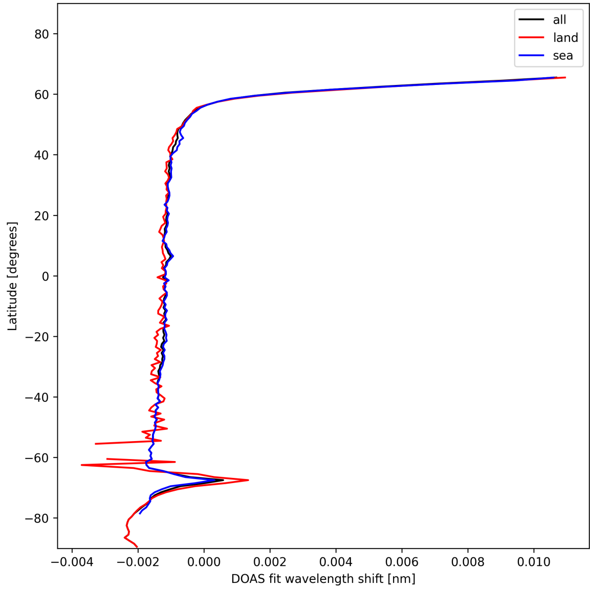
Figure 23: Zonal average of “DOAS fit wavelength shift” for 2024-12-22 to 2024-12-23.
