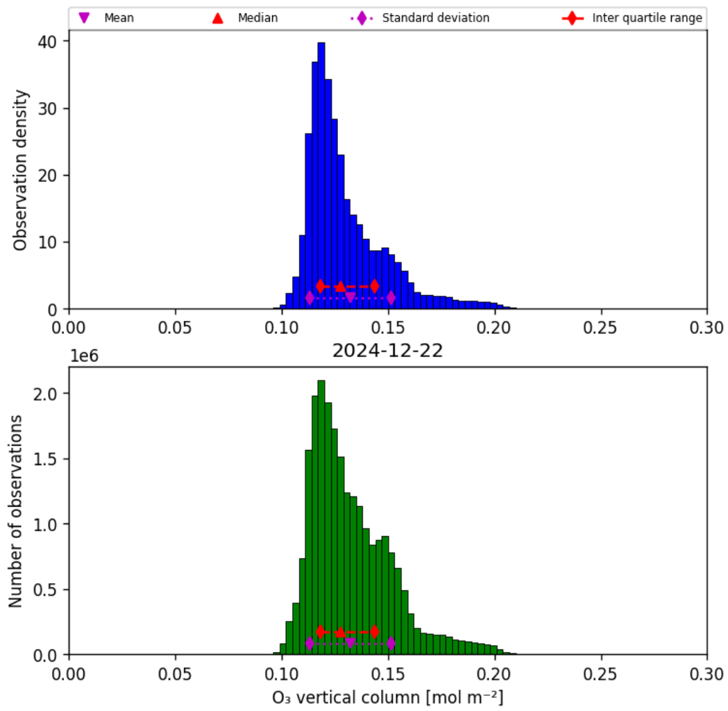
Figure 29: Histogram of “O 3 vertical column” for 2024-12-22 to 2024-12-23
