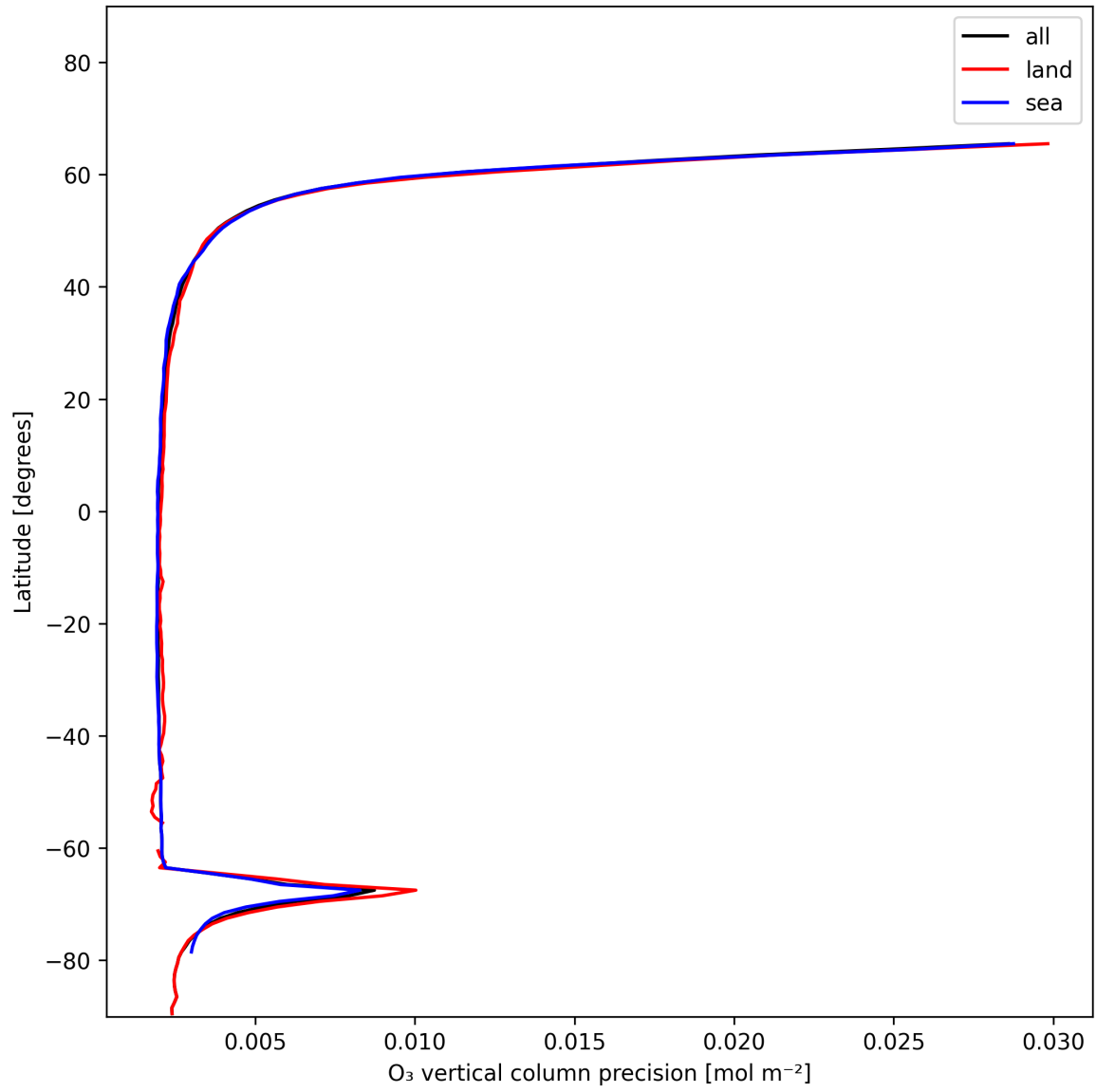
Figure 18: Zonal average of “O 3 vertical column precision” for 2024-12-22 to 2024-12-23.
