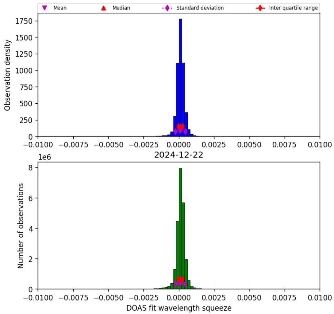
Figure 36: Histogram of “DOAS fit wavelength squeeze” for 2024-12-22 to 2024-12-23
