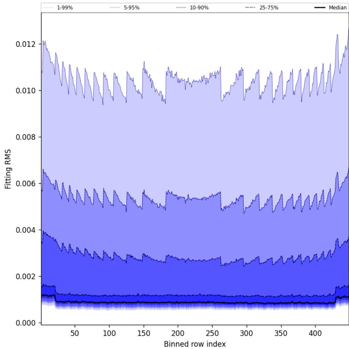
Figure 46: Along track statistics of “Fitting RMS” for 2024-12-22 to 2024-12-23
