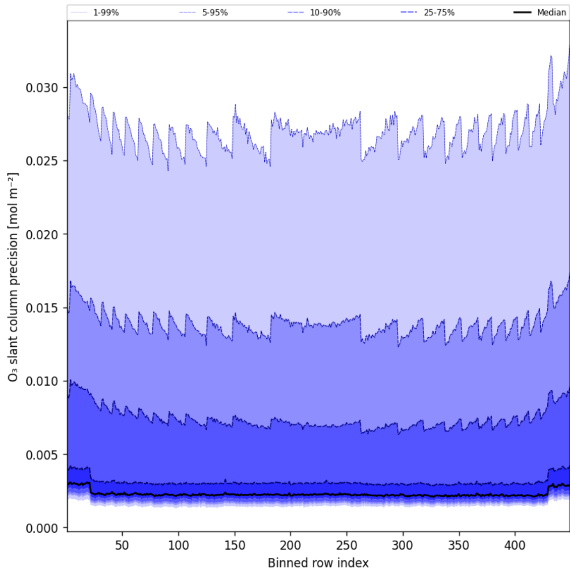
Figure 44: Along track statistics of “O 3 slant column precision” for 2024-12-22 to 2024-12-23
