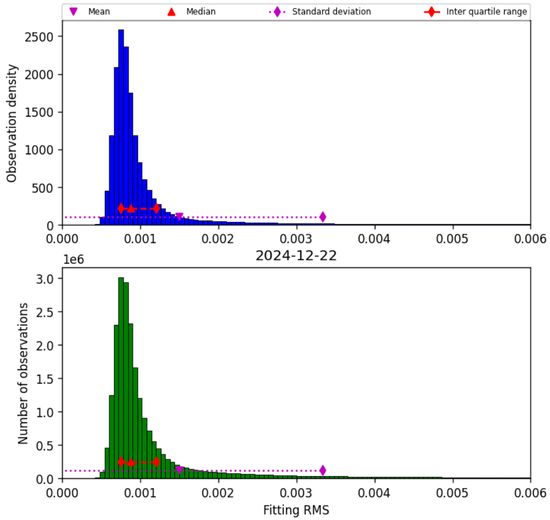
Figure 34: Histogram of “Fitting RMS” for 2024-12-22 to 2024-12-23
