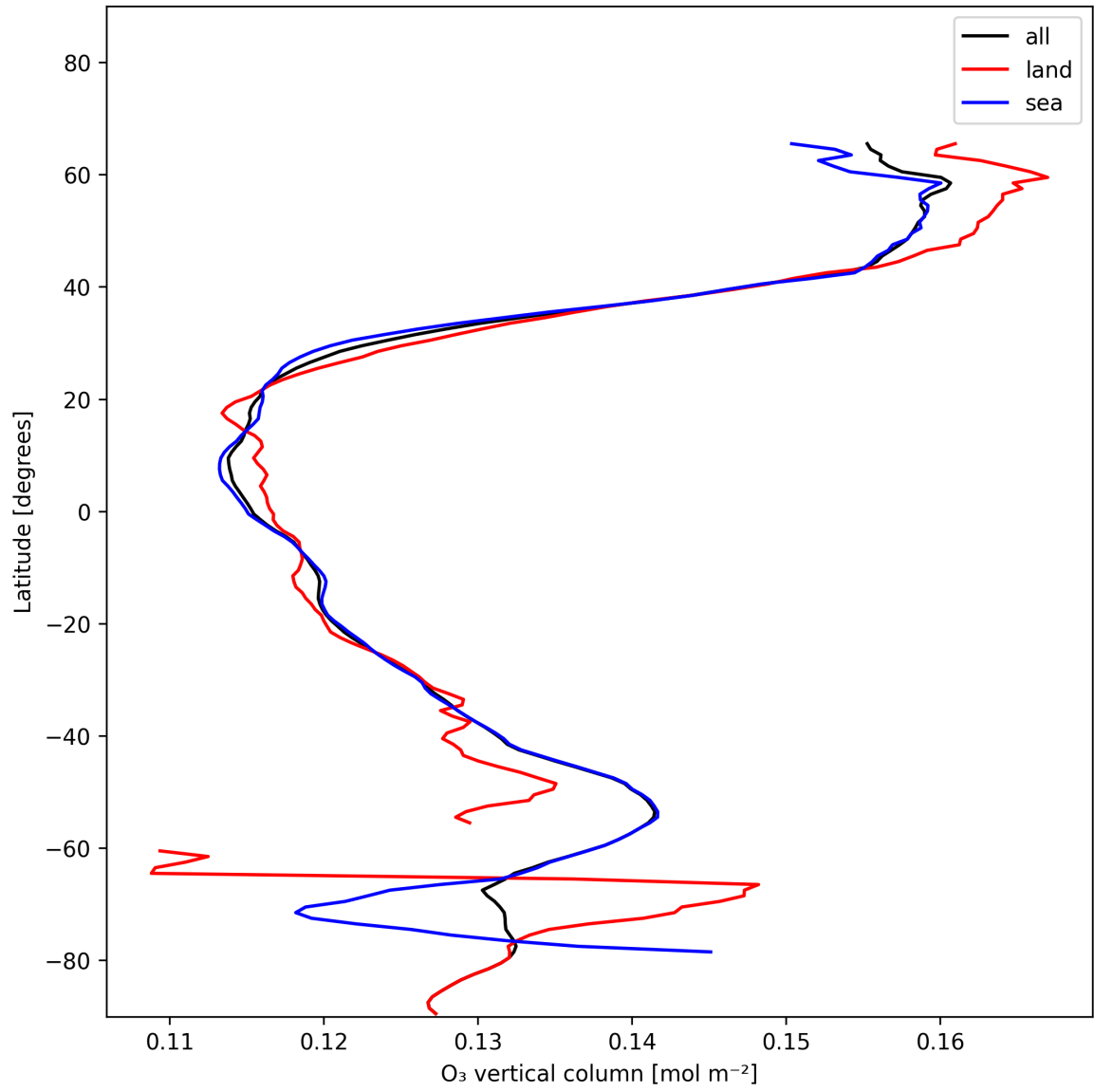
Figure 17: Zonal average of “O 3 vertical column” for 2024-12-22 to 2024-12-23.
