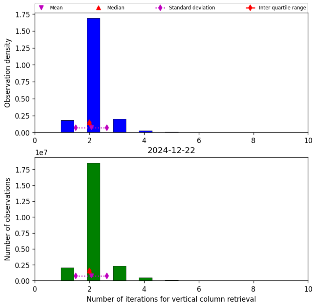
Figure 39: Histogram of “Number of iterations for vertical column retrieval” for 2024-12-22 to 2024-12-23
