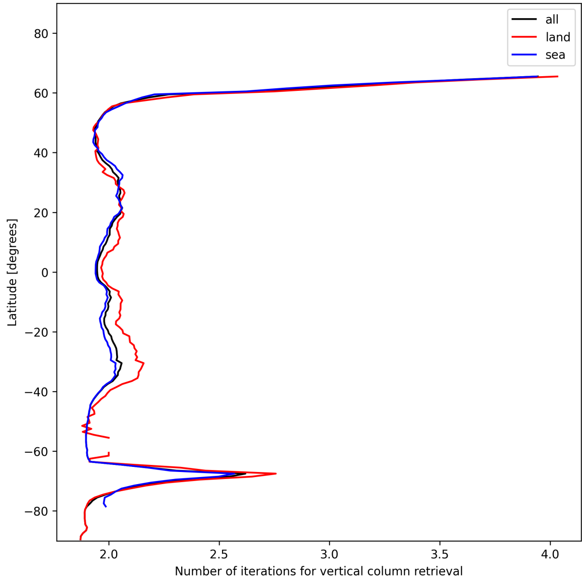
Figure 27: Zonal average of “Number of iterations for vertical column retrieval” for 2024-12-22 to 2024-12-23.
