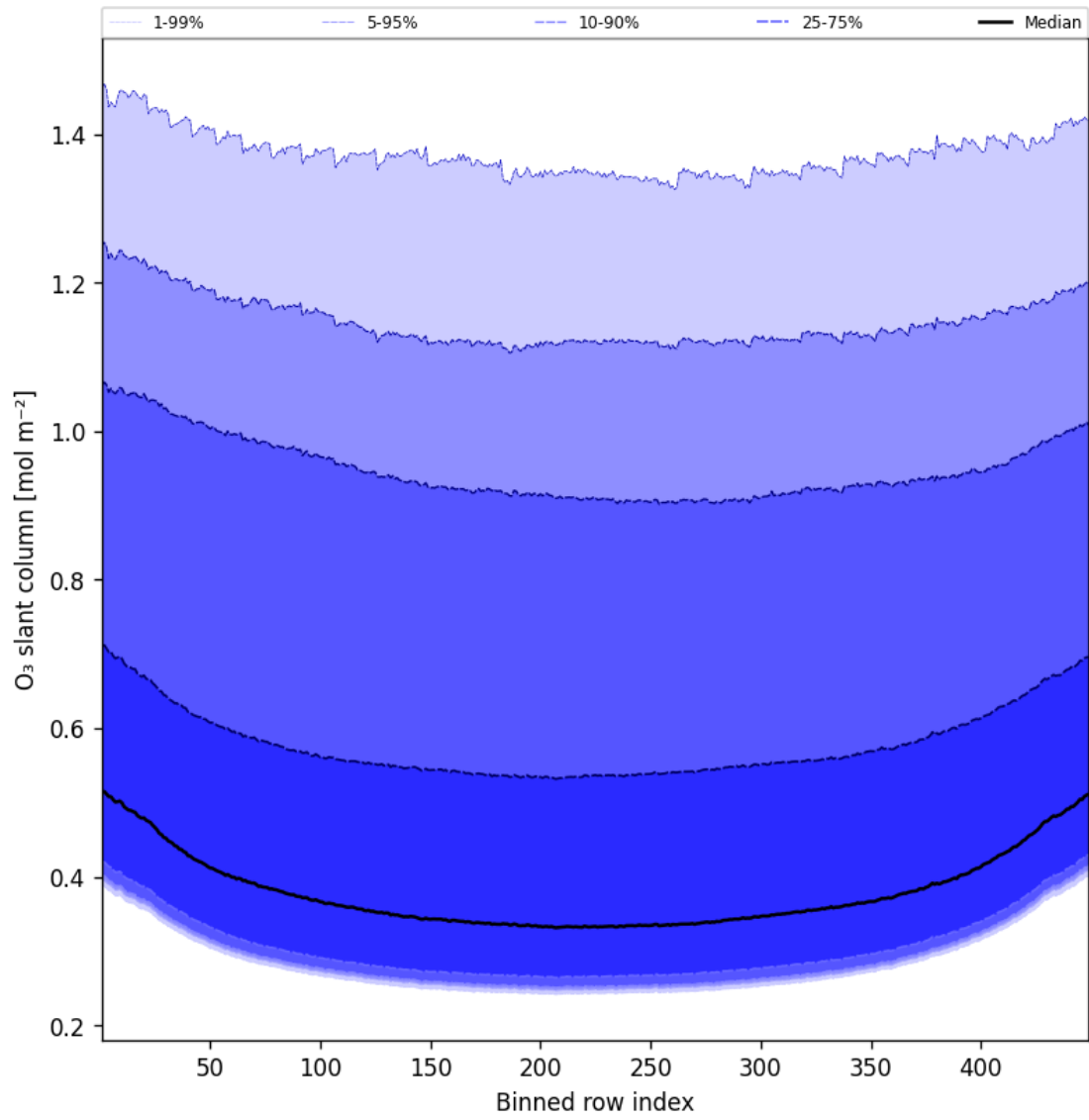
Figure 43: Along track statistics of “O 3 slant column” for 2024-12-22 to 2024-12-23
