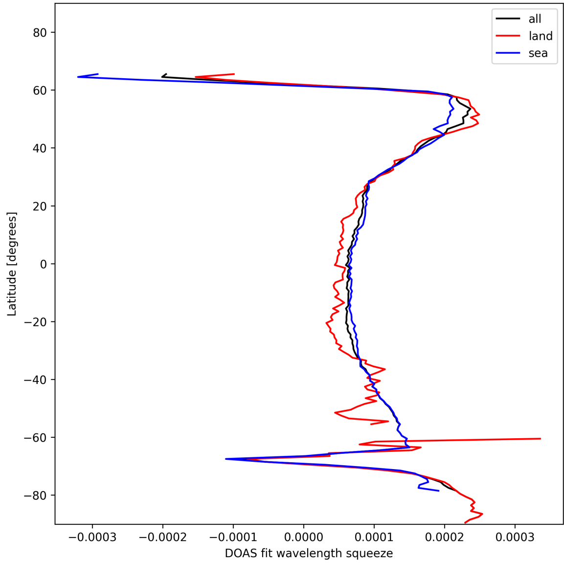
Figure 24: Zonal average of “DOAS fit wavelength squeeze” for 2024-12-22 to 2024-12-23.
