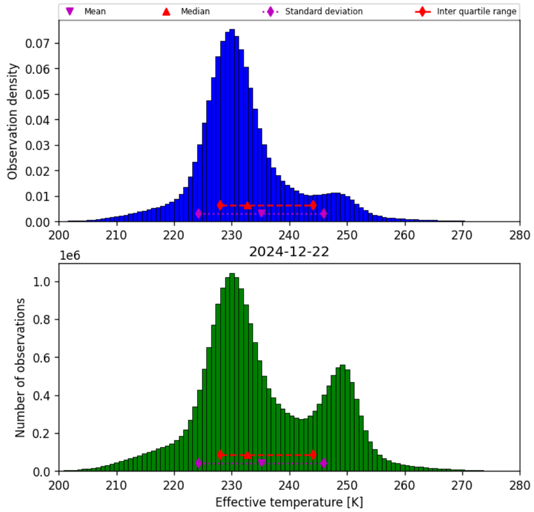
Figure 38: Histogram of “Effective temperature” for 2024-12-22 to 2024-12-23
