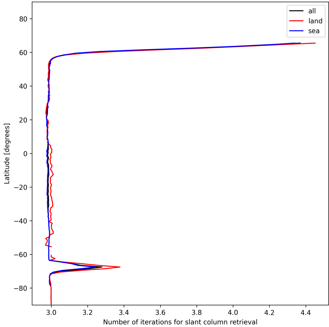
Figure 21: Zonal average of “Number of iterations for slant column retrieval” for 2024-12-22 to 2024-12-23.
