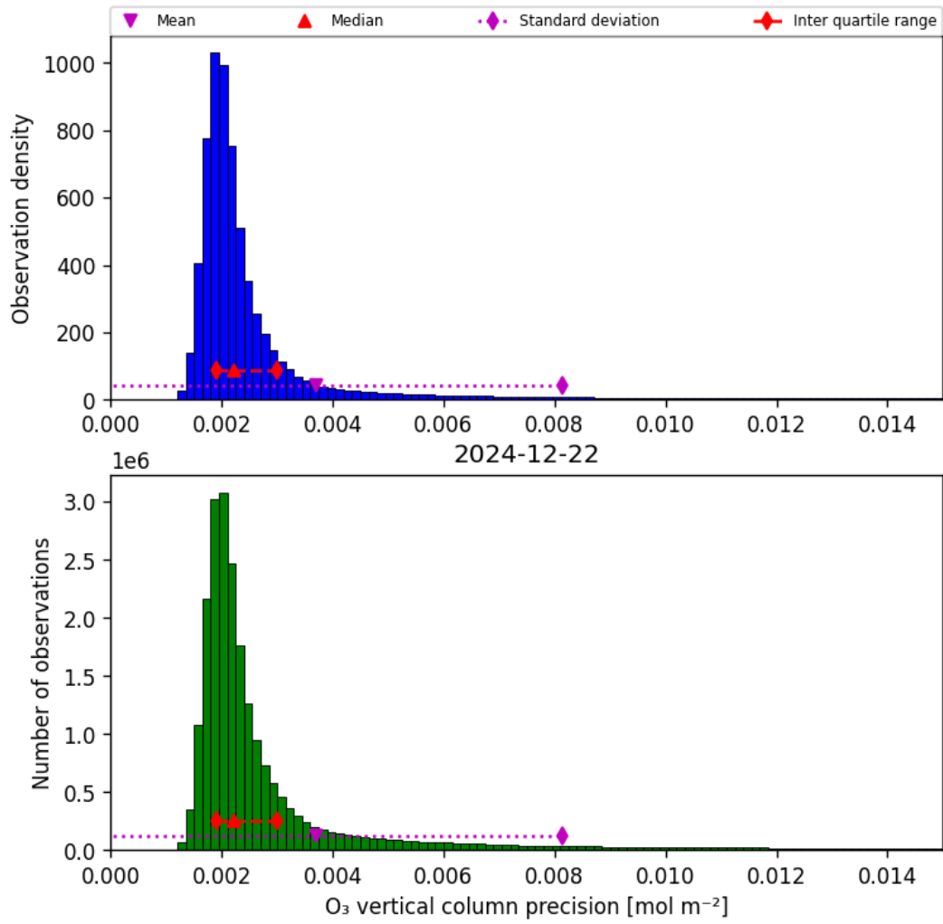
Figure 30: Histogram of “O 3 vertical column precision” for 2024-12-22 to 2024-12-23
