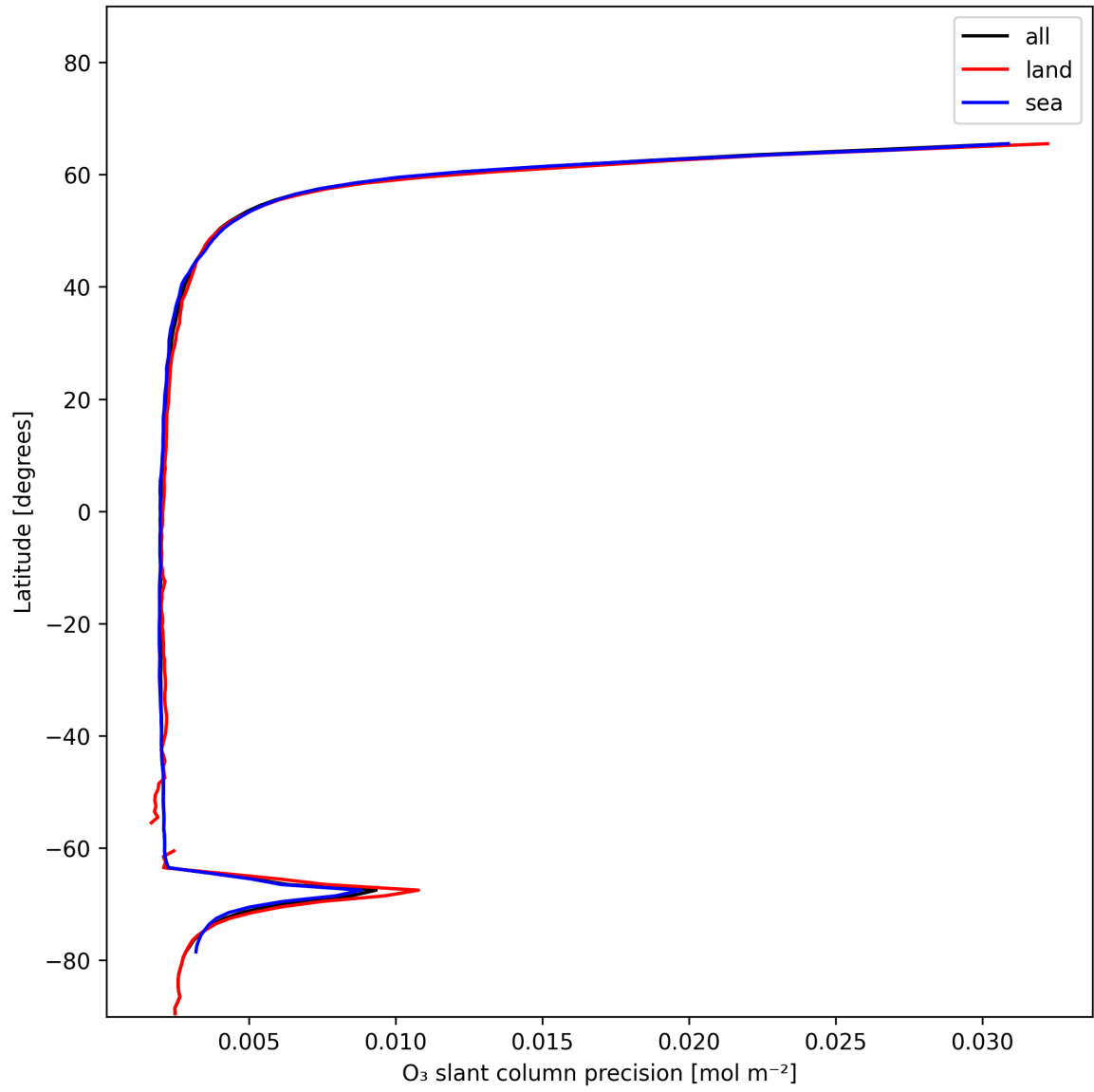
Figure 20: Zonal average of “O 3 slant column precision” for 2024-12-22 to 2024-12-23.
