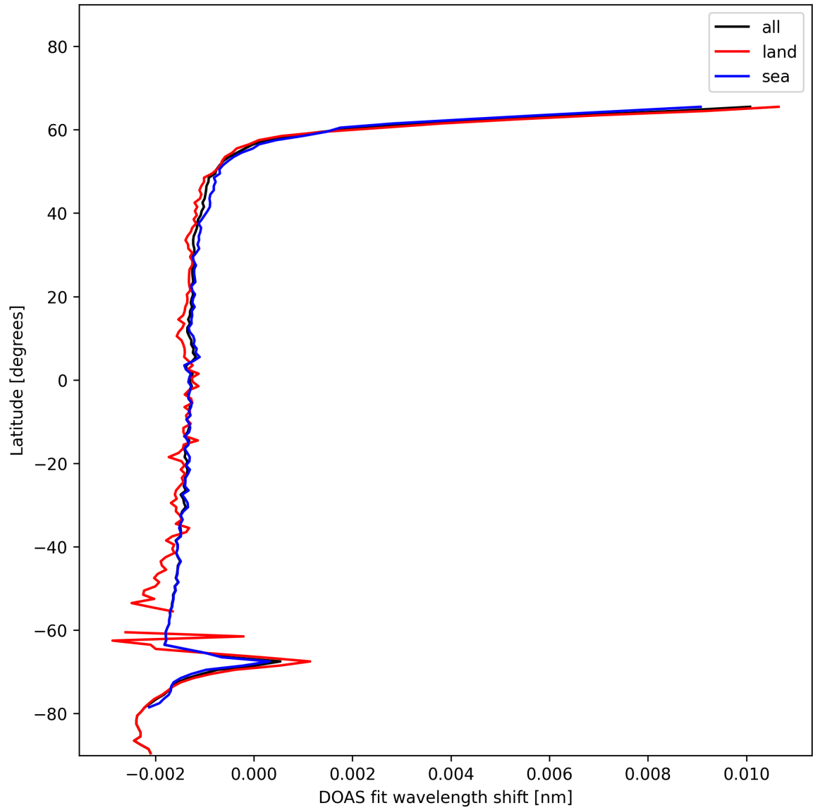
Figure 23: Zonal average of “DOAS fit wavelength shift” for 2024-12-23 to 2024-12-24.
