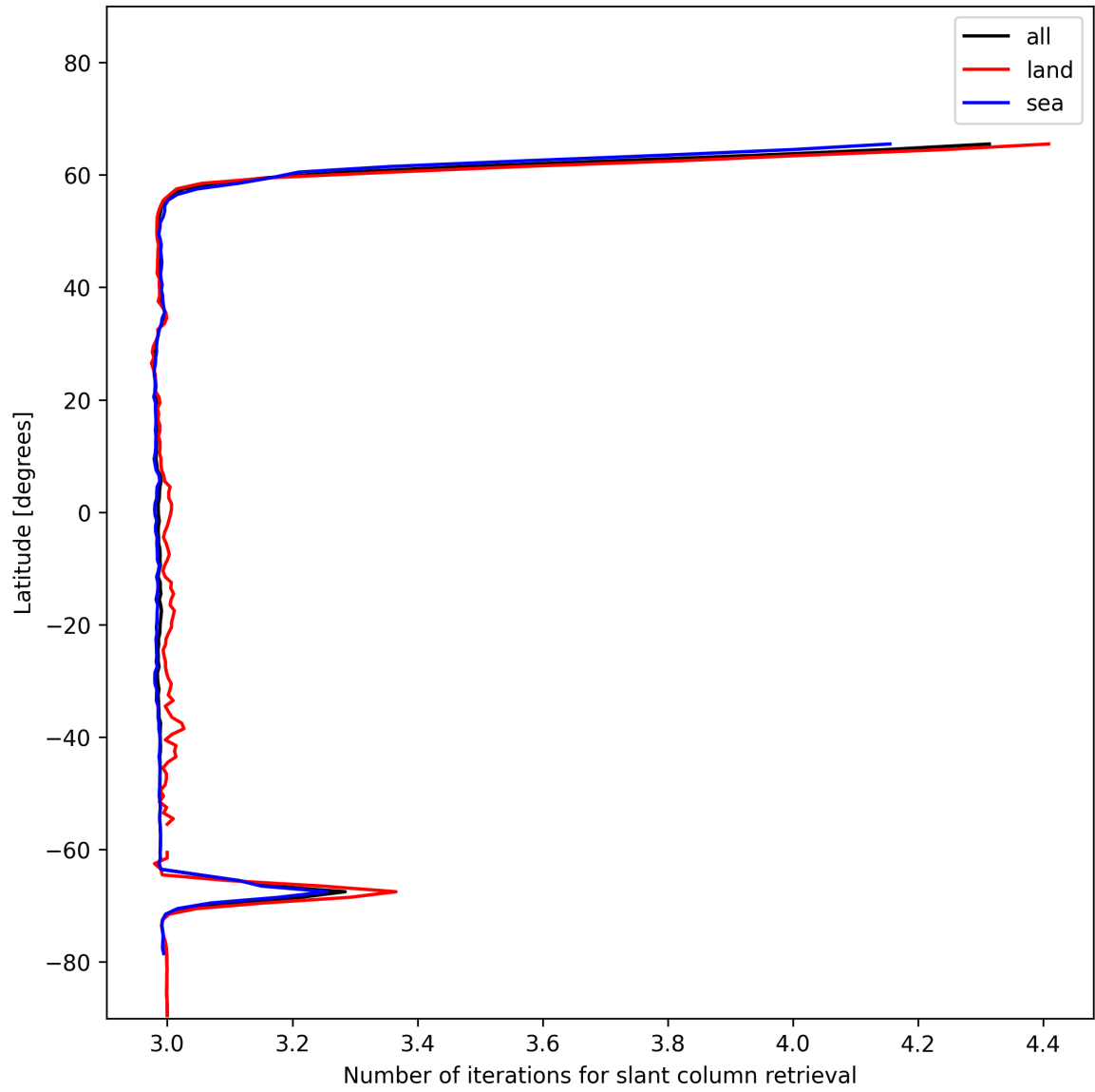
Figure 21: Zonal average of “Number of iterations for slant column retrieval” for 2024-12-23 to 2024-12-24.
