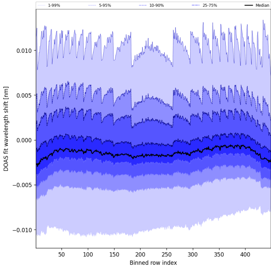
Figure 47: Along track statistics of “DOAS fit wavelength shift” for 2024-12-23 to 2024-12-24
