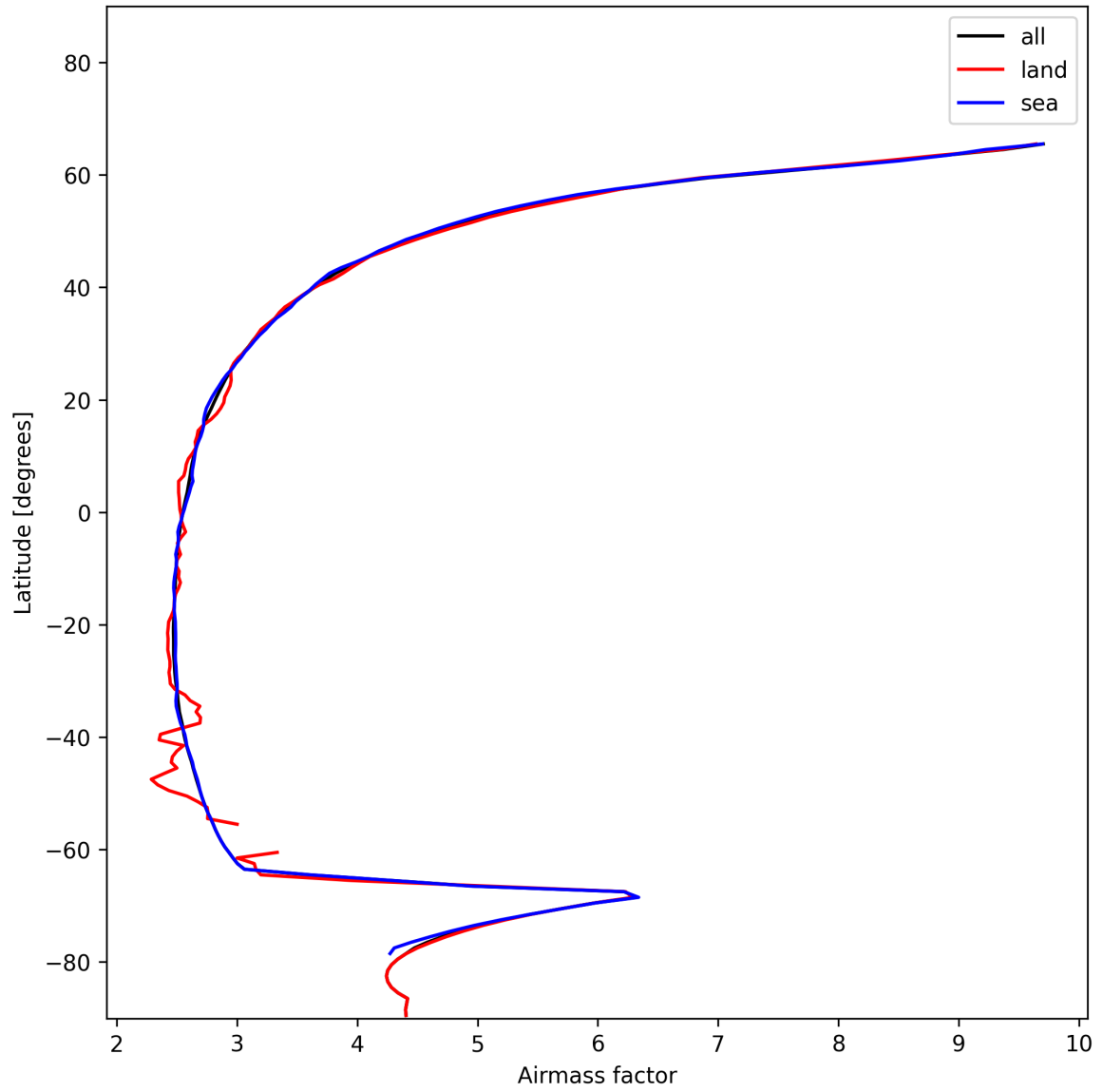
Figure 25: Zonal average of “Airmass factor” for 2024-12-23 to 2024-12-24.
