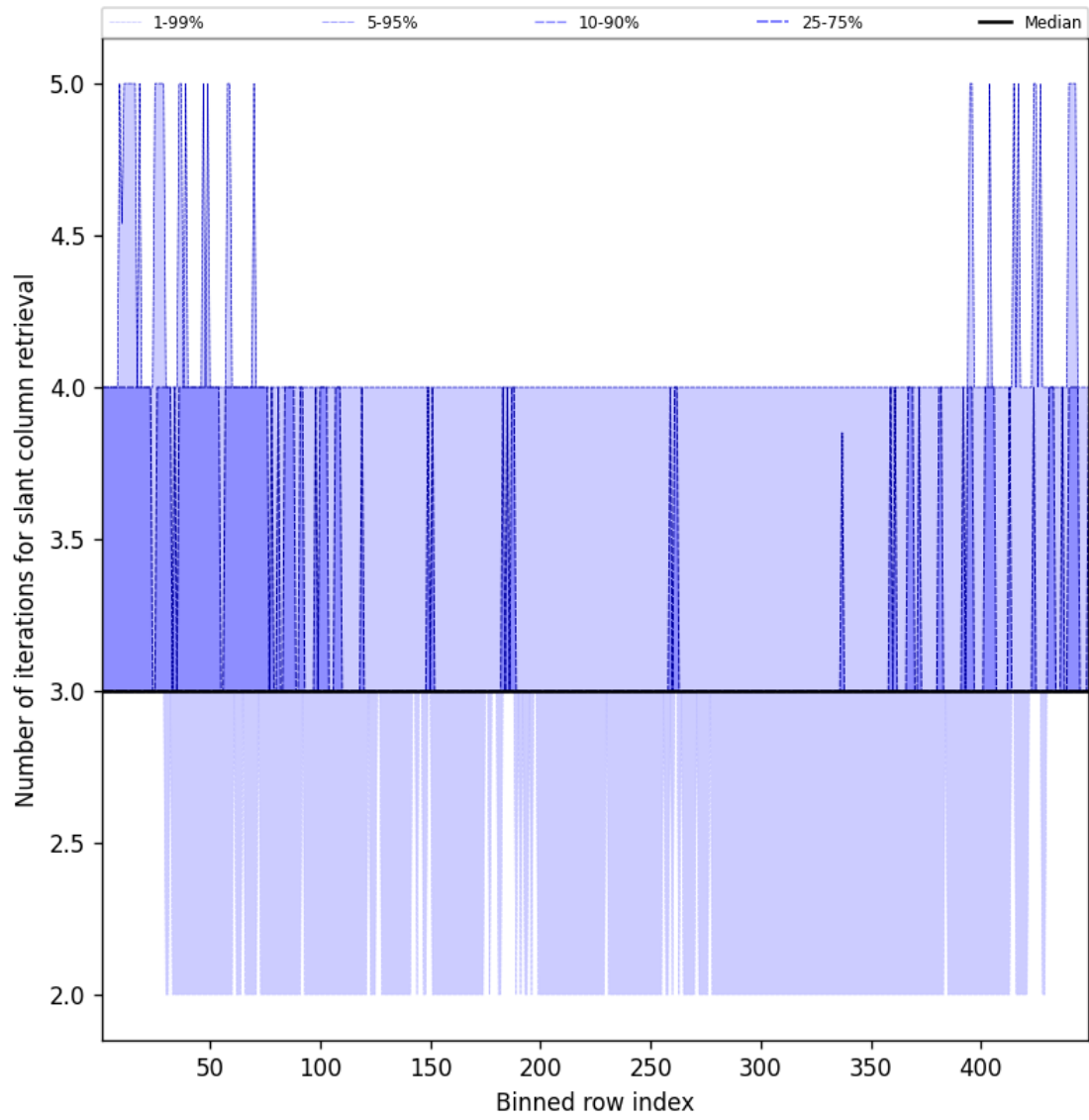
Figure 45: Along track statistics of “Number of iterations for slant column retrieval” for 2024-12-23 to 2024-12-24
