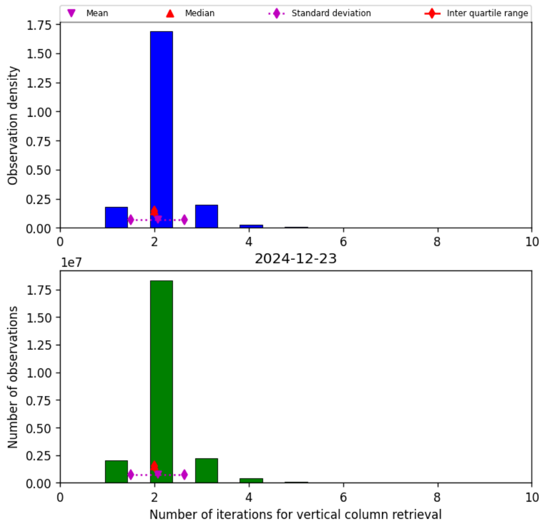
Figure 39: Histogram of “Number of iterations for vertical column retrieval” for 2024-12-23 to 2024-12-24
