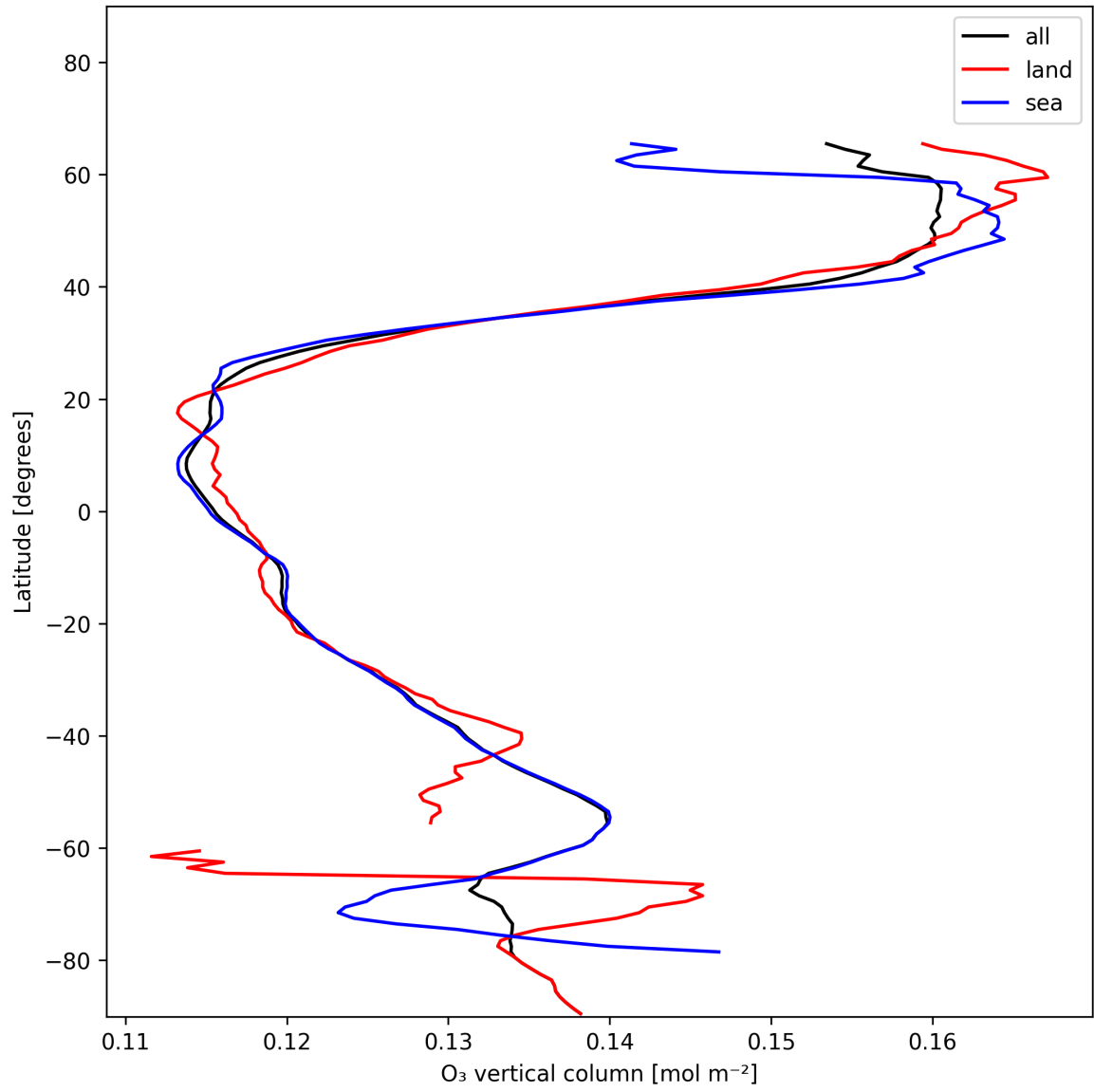
Figure 17: Zonal average of “O 3 vertical column” for 2024-12-23 to 2024-12-24.
