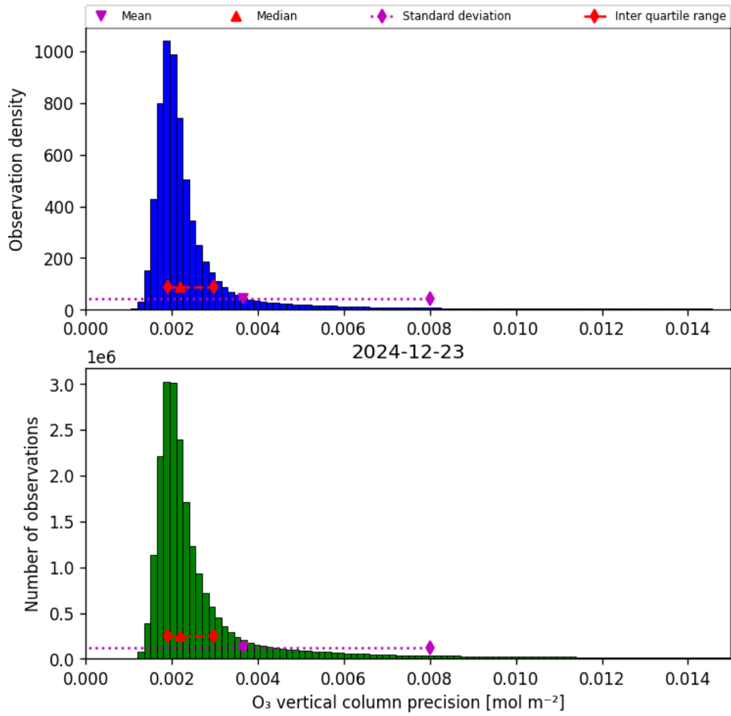
Figure 30: Histogram of “O 3 vertical column precision” for 2024-12-23 to 2024-12-24
