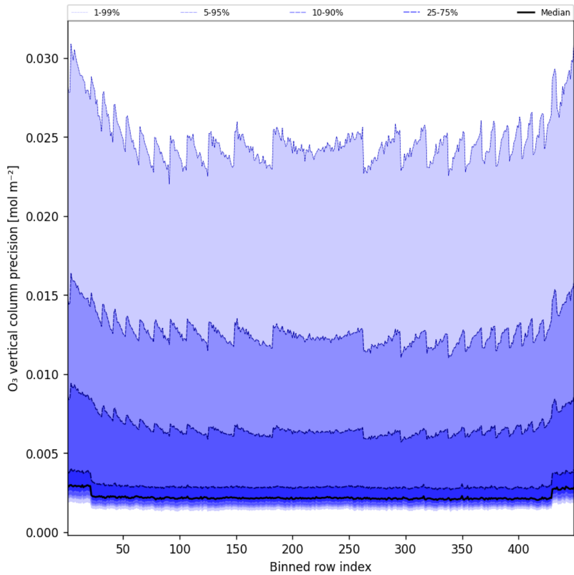
Figure 42: Along track statistics of “O 3 vertical column precision” for 2024-12-23 to 2024-12-24
