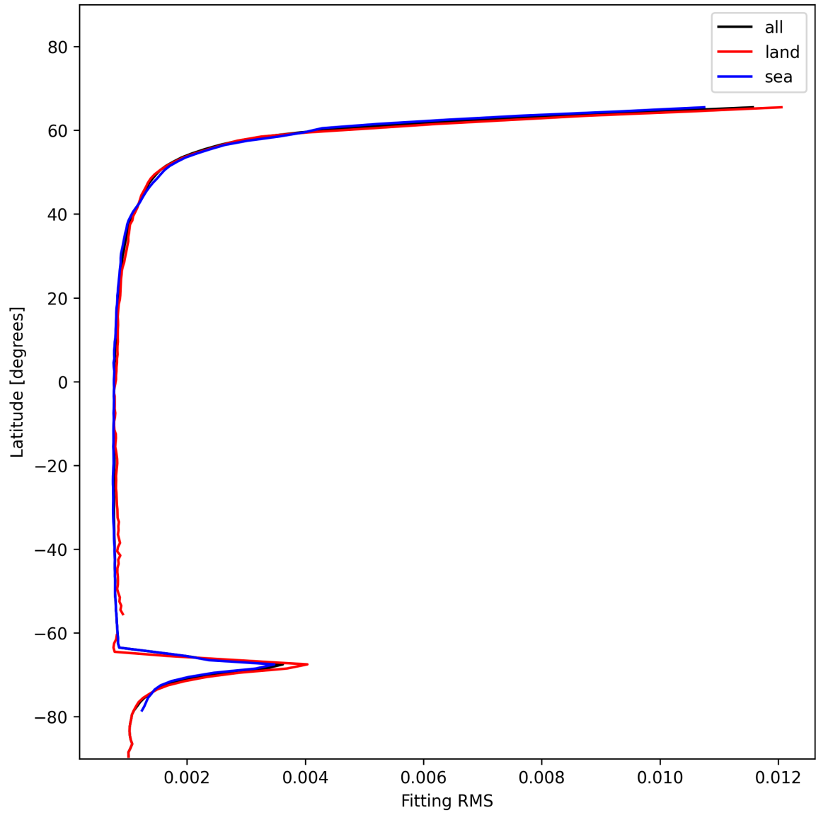
Figure 22: Zonal average of “Fitting RMS” for 2024-12-23 to 2024-12-24.
