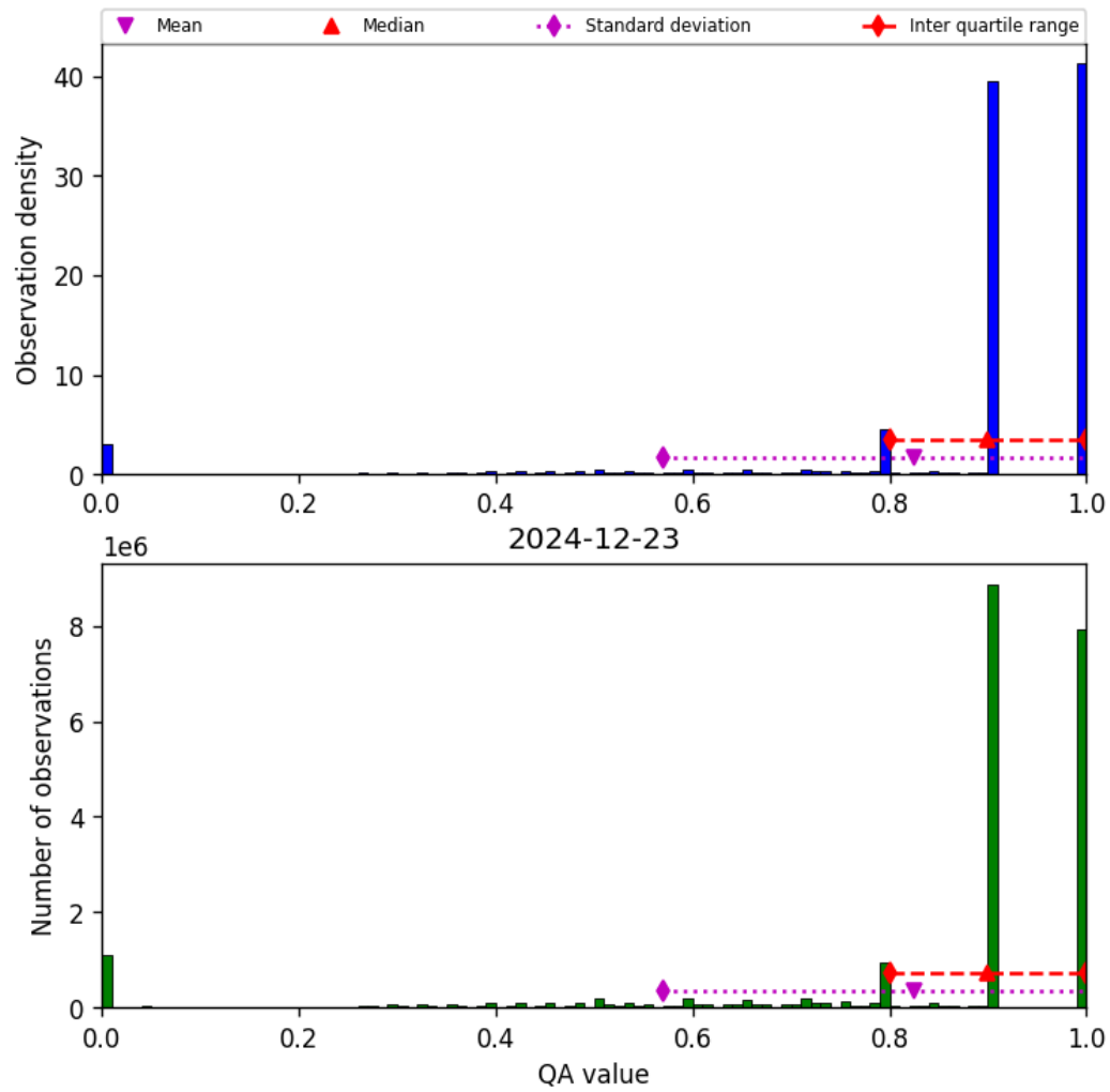
Figure 28: Histogram of “QA value” for 2024-12-23 to 2024-12-24
