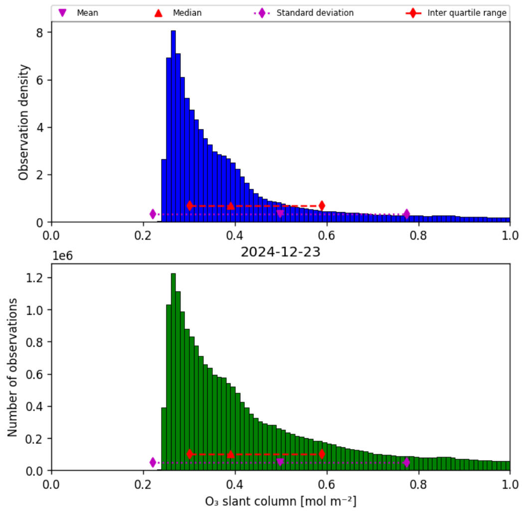
Figure 31: Histogram of “O 3 slant column” for 2024-12-23 to 2024-12-24
