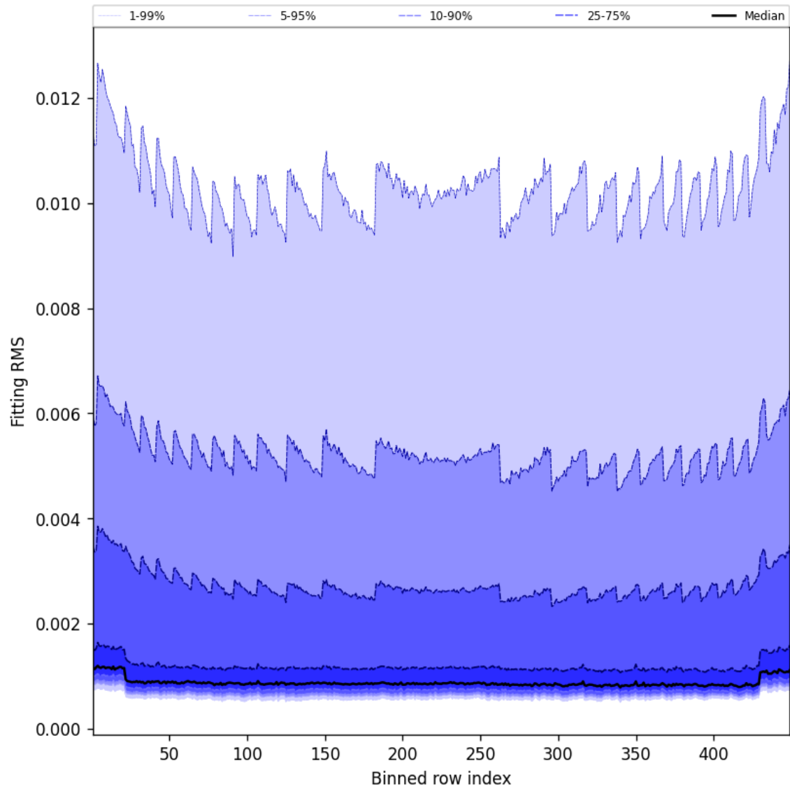
Figure 46: Along track statistics of “Fitting RMS” for 2024-12-23 to 2024-12-24
