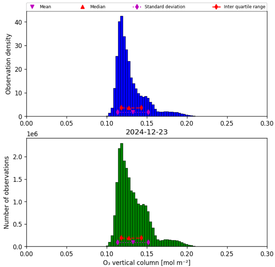
Figure 29: Histogram of “O 3 vertical column” for 2024-12-23 to 2024-12-24
