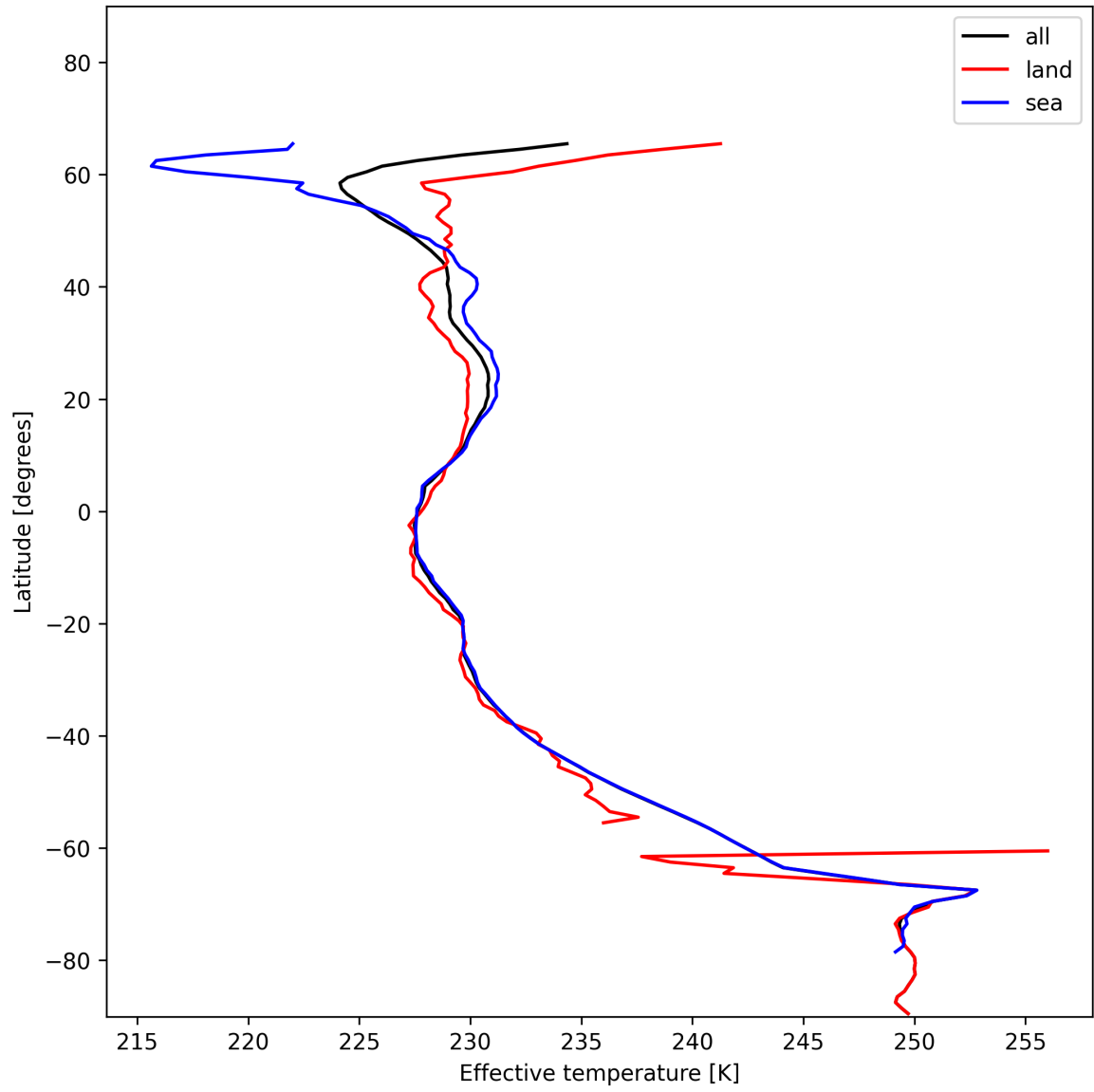
Figure 26: Zonal average of “Effective temperature” for 2024-12-23 to 2024-12-24.
