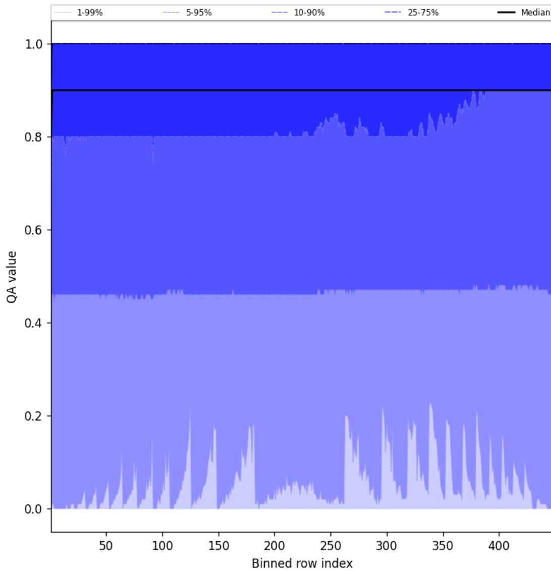
Figure 40: Along track statistics of “QA value” for 2024-12-23 to 2024-12-24
