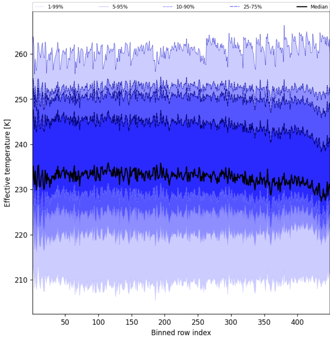
Figure 50: Along track statistics of “Effective temperature” for 2024-12-23 to 2024-12-24
