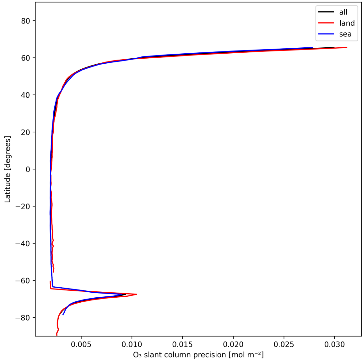
Figure 20: Zonal average of “O 3 slant column precision” for 2024-12-23 to 2024-12-24.
