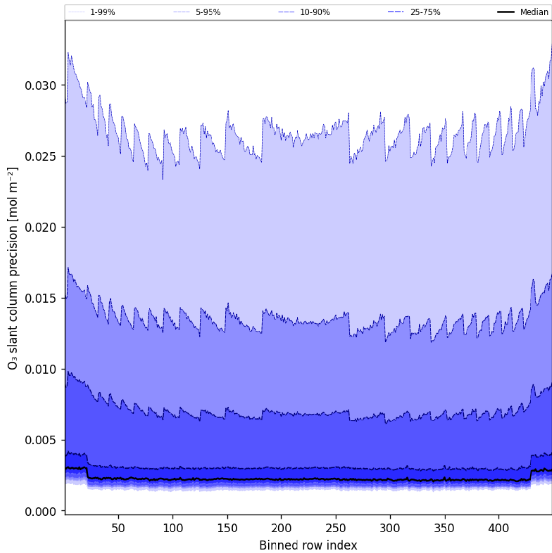
Figure 44: Along track statistics of “O 3 slant column precision” for 2024-12-23 to 2024-12-24
