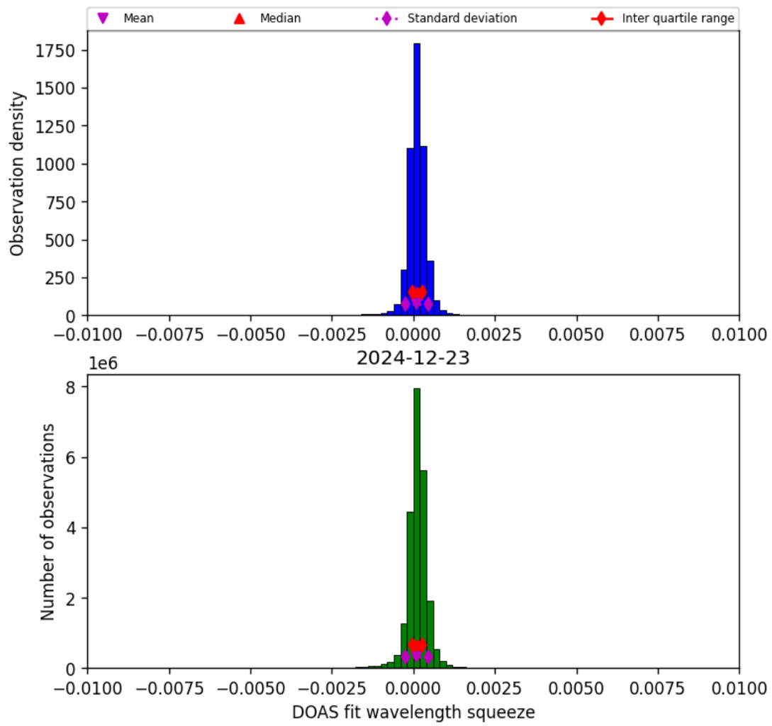
Figure 36: Histogram of “DOAS fit wavelength squeeze” for 2024-12-23 to 2024-12-24
