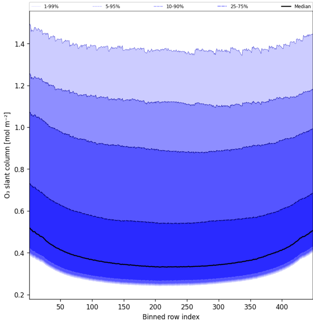
Figure 43: Along track statistics of “O 3 slant column” for 2024-12-23 to 2024-12-24
