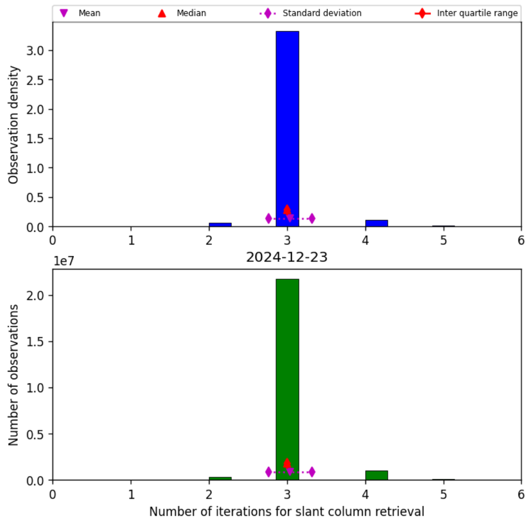
Figure 33: Histogram of “Number of iterations for slant column retrieval” for 2024-12-23 to 2024-12-24
