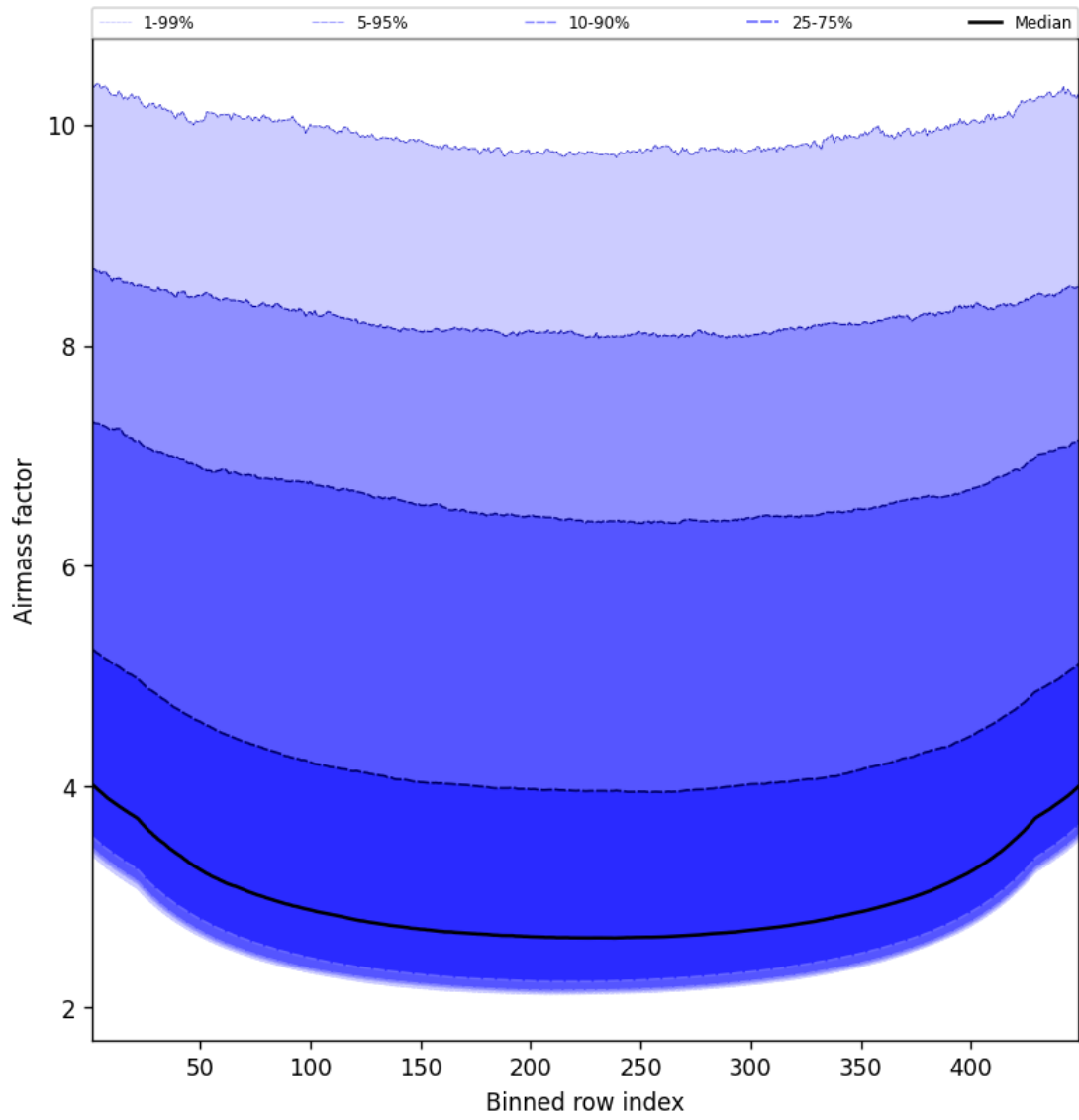
Figure 49: Along track statistics of “Airmass factor” for 2024-12-23 to 2024-12-24
