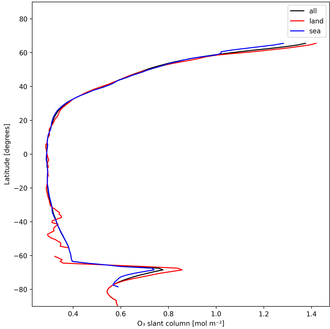
Figure 19: Zonal average of “O 3 slant column” for 2024-12-23 to 2024-12-24.
