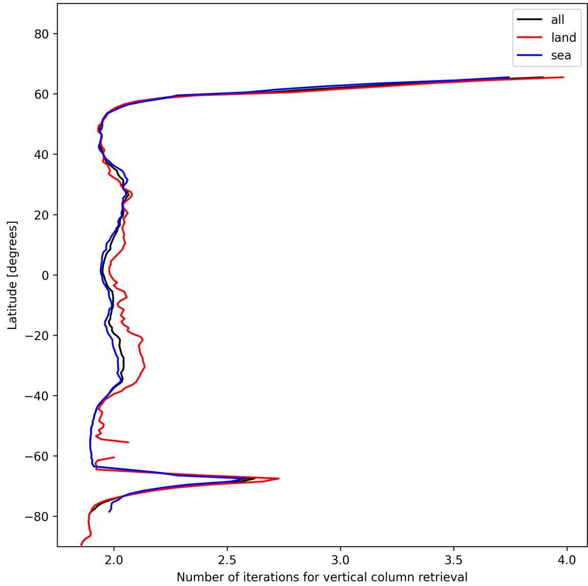
Figure 27: Zonal average of “Number of iterations for vertical column retrieval” for 2024-12-23 to 2024-12-24.
