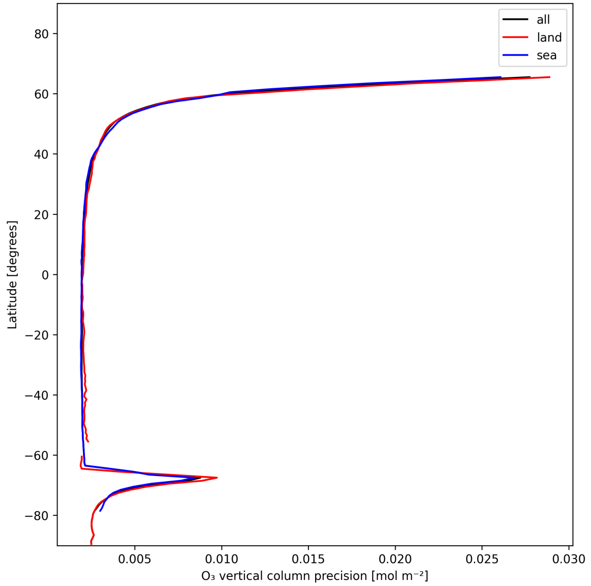
Figure 18: Zonal average of “O 3 vertical column precision” for 2024-12-23 to 2024-12-24.
