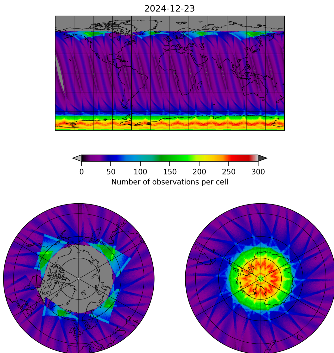
Figure 15: Map of the number of observations for 2024-12-23 to 2024-12-24
