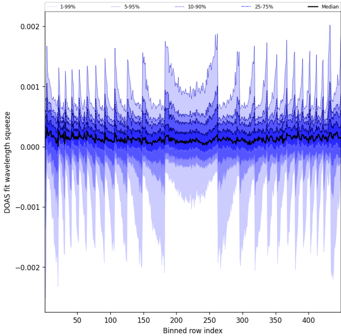
Figure 48: Along track statistics of “DOAS fit wavelength squeeze” for 2024-12-23 to 2024-12-24
