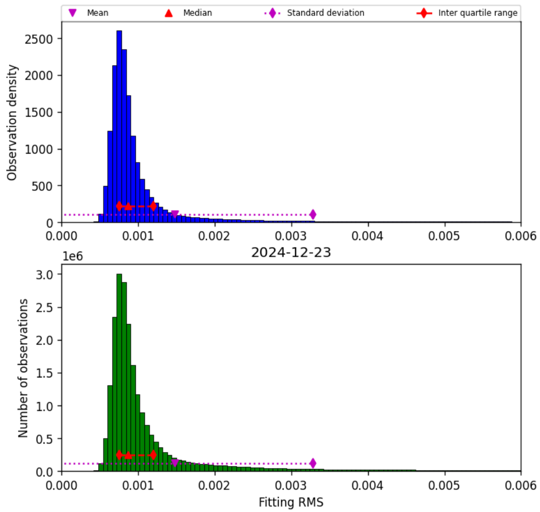
Figure 34: Histogram of “Fitting RMS” for 2024-12-23 to 2024-12-24
