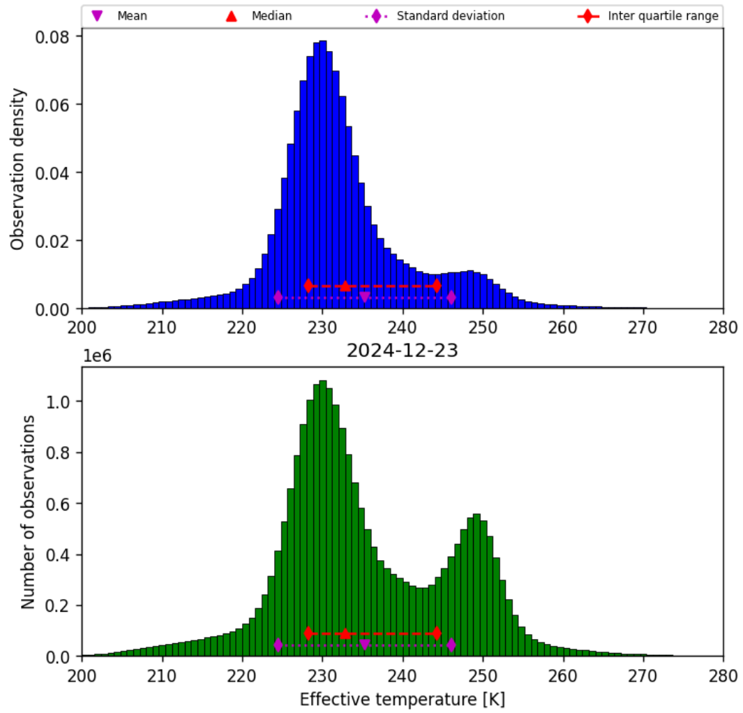
Figure 38: Histogram of “Effective temperature” for 2024-12-23 to 2024-12-24
