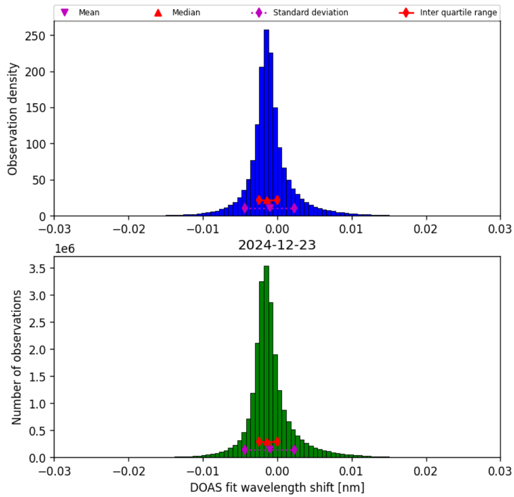
Figure 35: Histogram of “DOAS fit wavelength shift” for 2024-12-23 to 2024-12-24
