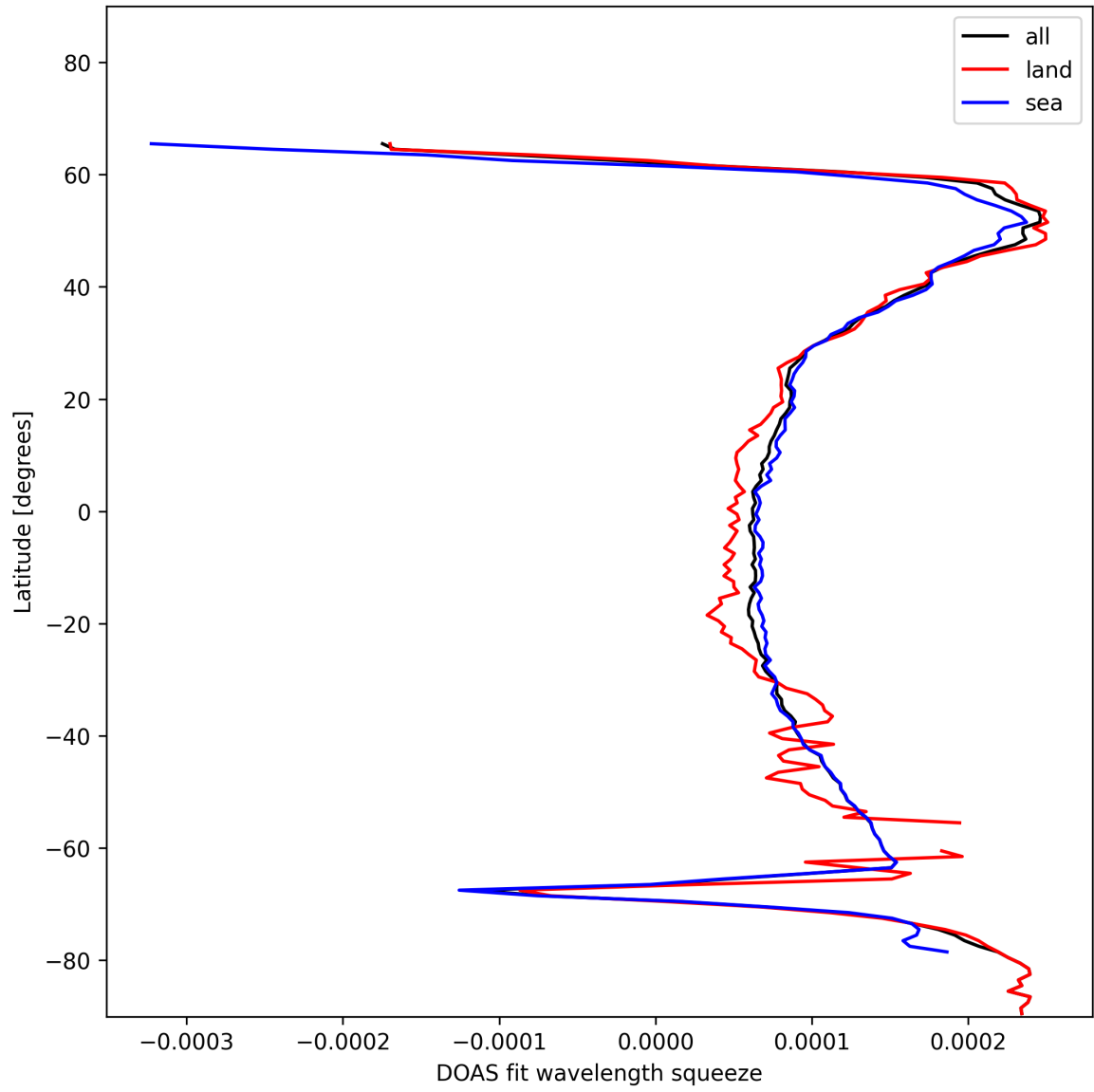
Figure 24: Zonal average of “DOAS fit wavelength squeeze” for 2024-12-23 to 2024-12-24.
