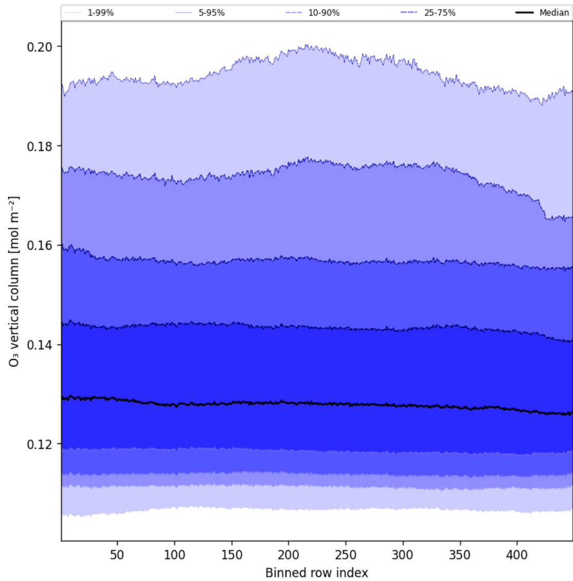
Figure 41: Along track statistics of “O 3 vertical column” for 2024-12-23 to 2024-12-24
