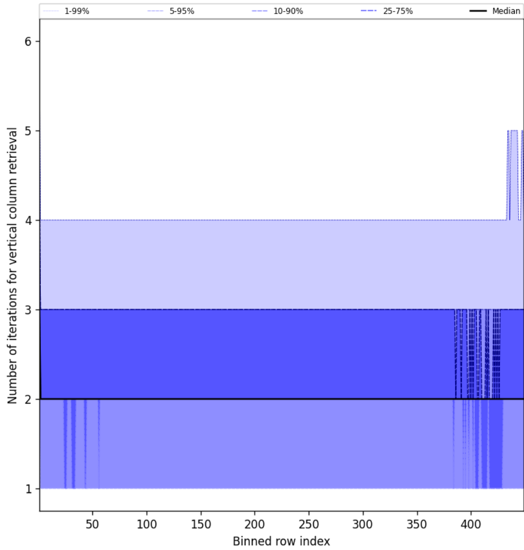
Figure 51: Along track statistics of “Number of iterations for vertical column retrieval” for 2024-12-23 to 2024-12-24
