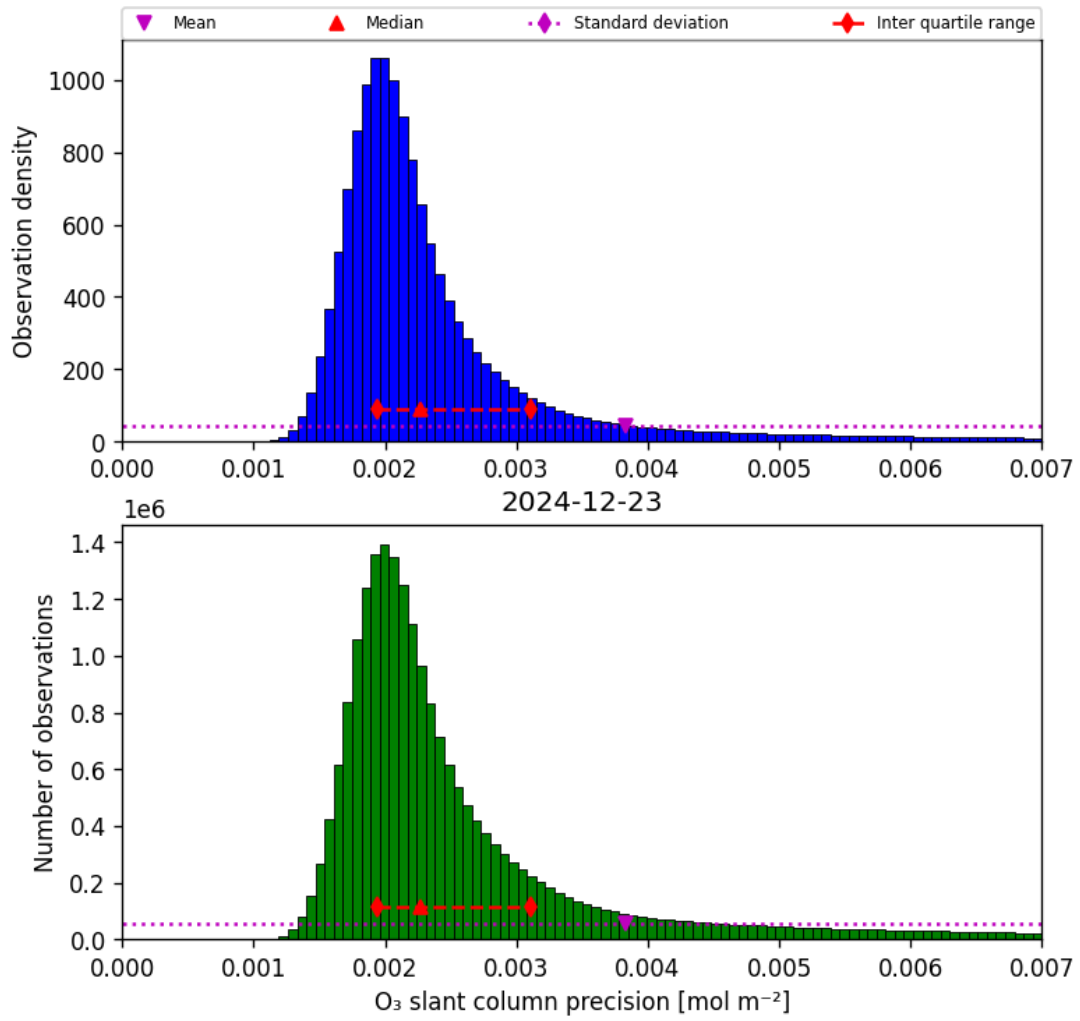
Figure 32: Histogram of “O 3 slant column precision” for 2024-12-23 to 2024-12-24
