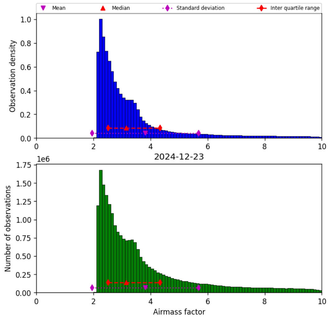
Figure 37: Histogram of “Airmass factor” for 2024-12-23 to 2024-12-24
