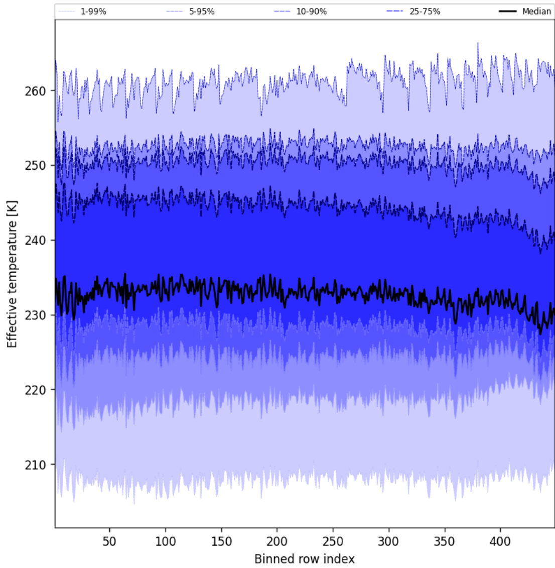
Figure 50: Along track statistics of “Effective temperature” for 2024-12-24 to 2024-12-25
