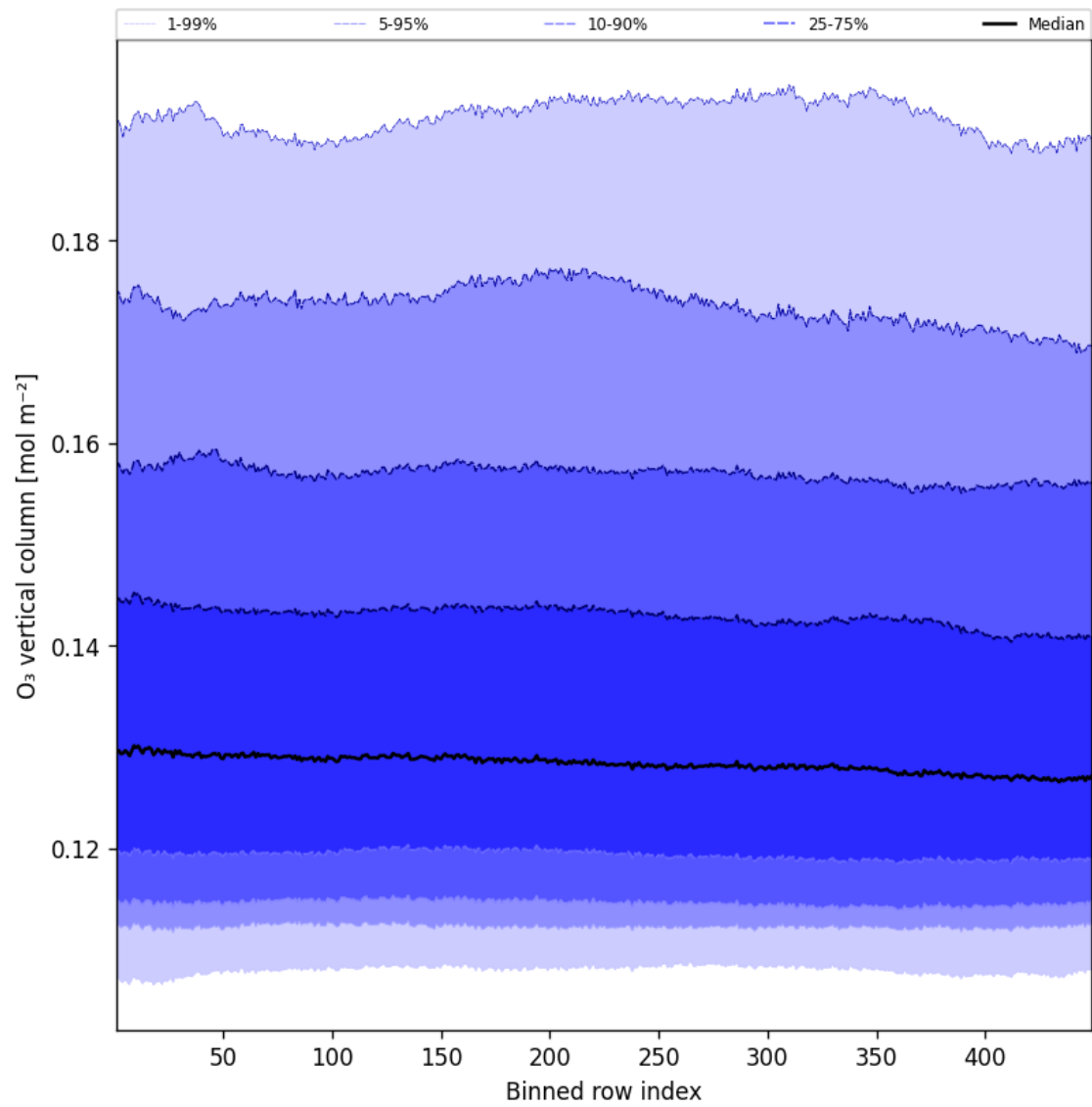
Figure 41: Along track statistics of “O 3 vertical column” for 2024-12-24 to 2024-12-25
