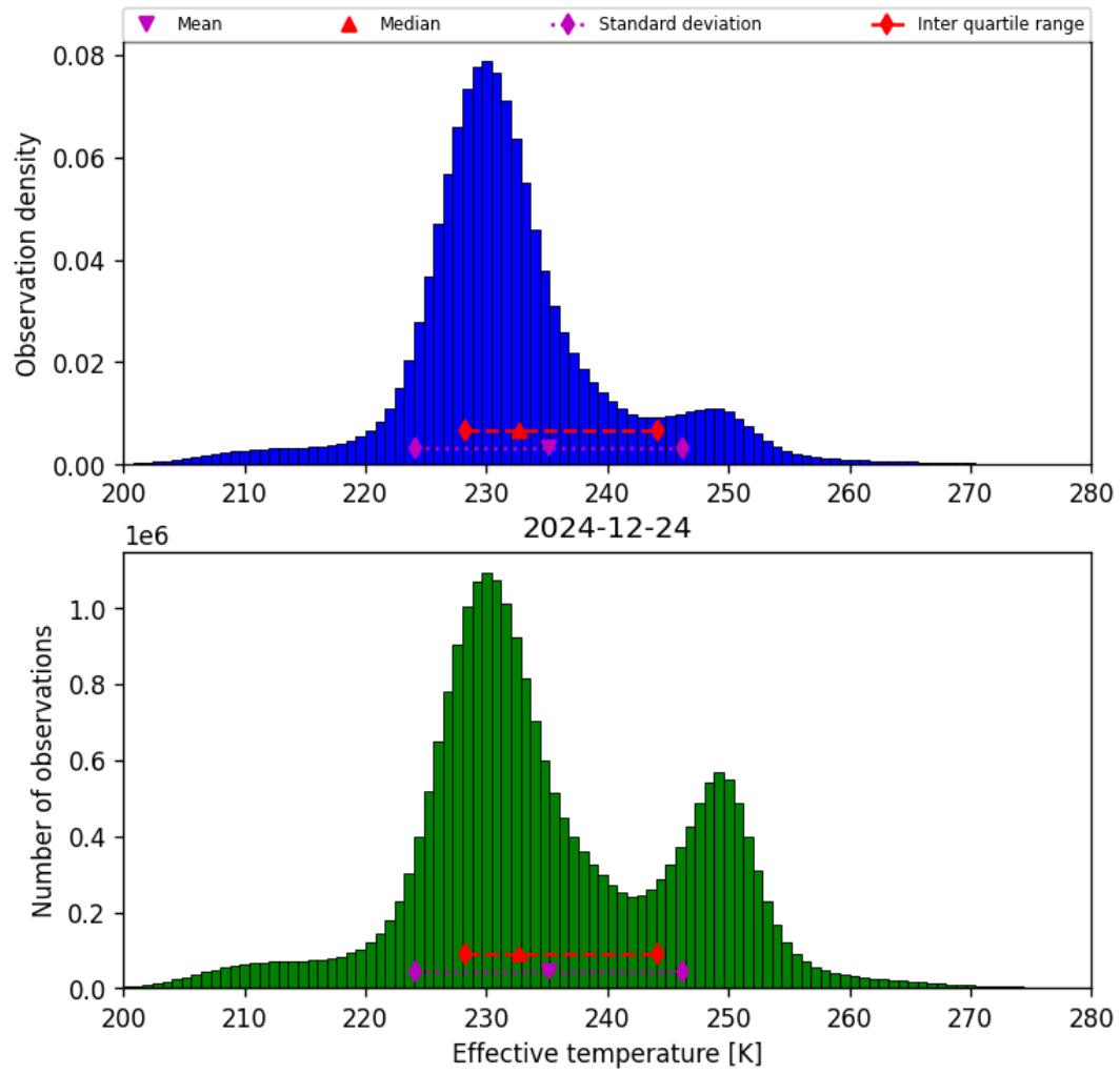
Figure 38: Histogram of “Effective temperature” for 2024-12-24 to 2024-12-25
