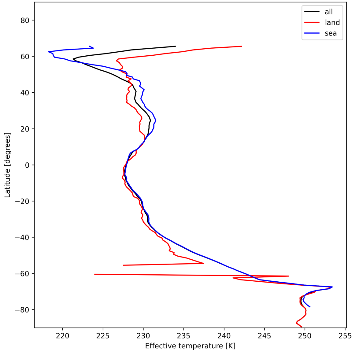
Figure 26: Zonal average of “Effective temperature” for 2024-12-24 to 2024-12-25.
