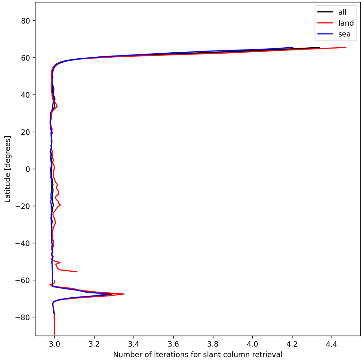
Figure 21: Zonal average of “Number of iterations for slant column retrieval” for 2024-12-24 to 2024-12-25.
