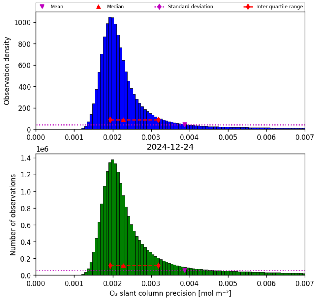
Figure 32: Histogram of “O 3 slant column precision” for 2024-12-24 to 2024-12-25
