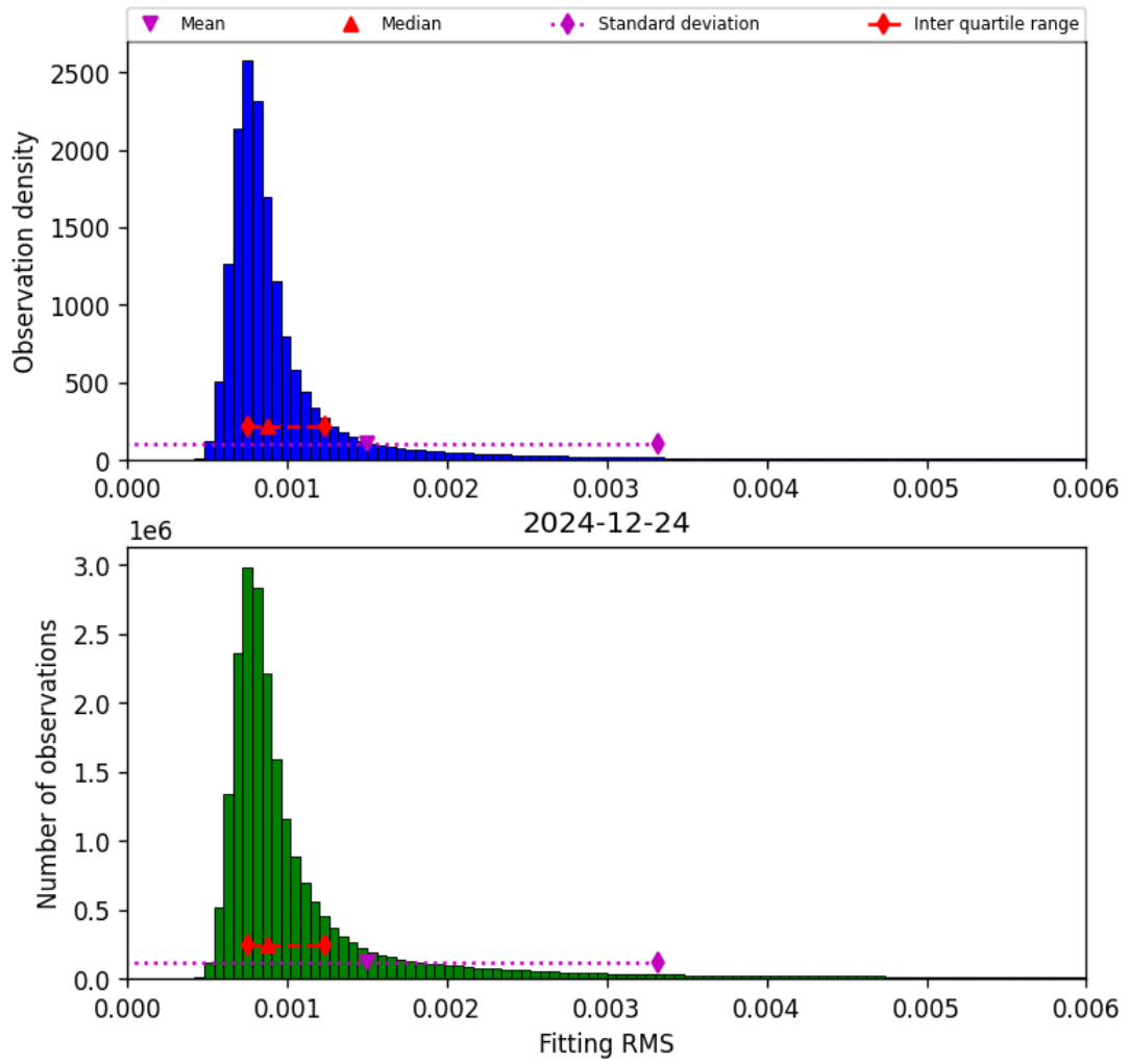
Figure 34: Histogram of “Fitting RMS” for 2024-12-24 to 2024-12-25
