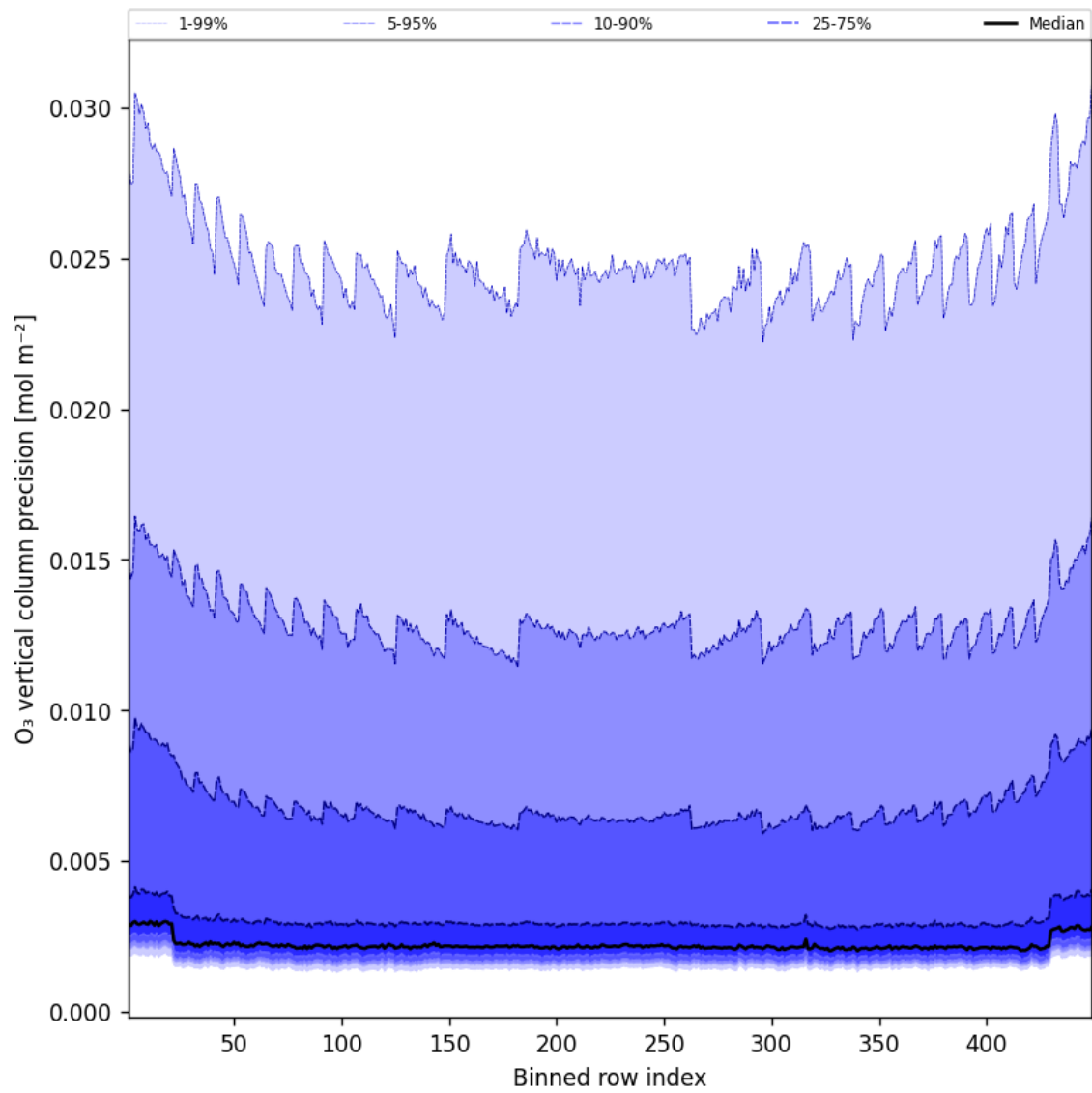
Figure 42: Along track statistics of “O 3 vertical column precision” for 2024-12-24 to 2024-12-25
