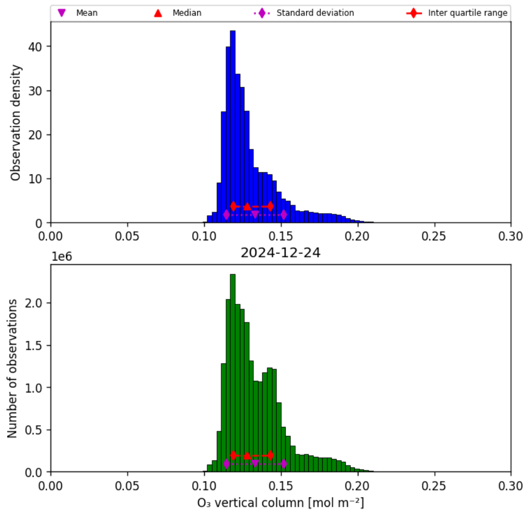
Figure 29: Histogram of “O 3 vertical column” for 2024-12-24 to 2024-12-25
