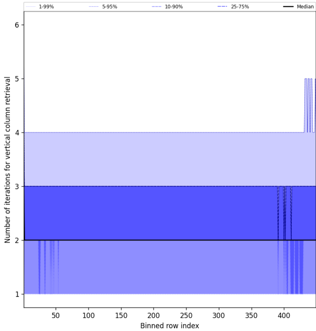
Figure 51: Along track statistics of “Number of iterations for vertical column retrieval” for 2024-12-24 to 2024-12-25
