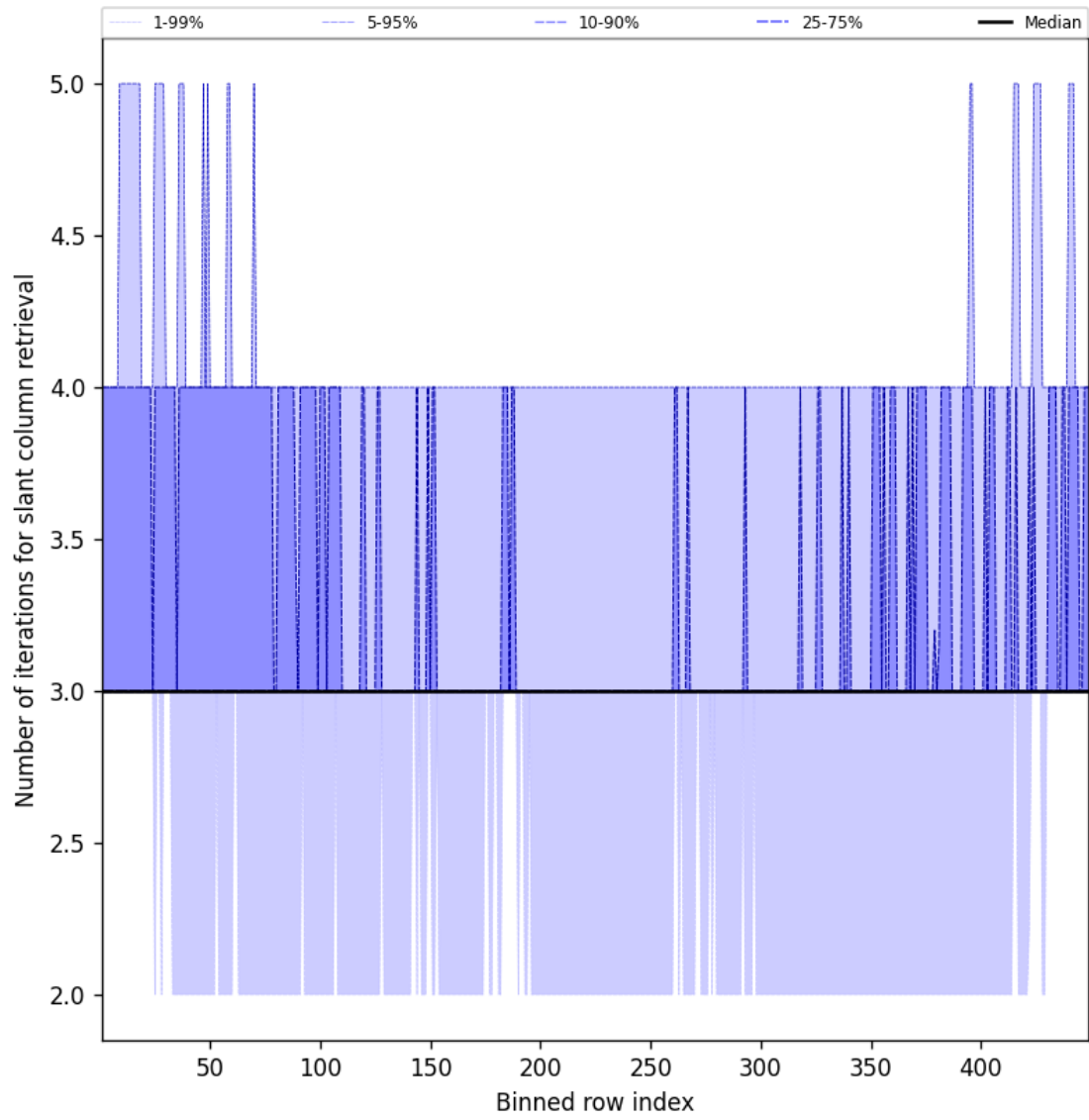
Figure 45: Along track statistics of “Number of iterations for slant column retrieval” for 2024-12-24 to 2024-12-25
