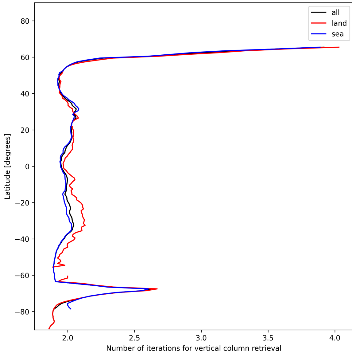
Figure 27: Zonal average of “Number of iterations for vertical column retrieval” for 2024-12-24 to 2024-12-25.
