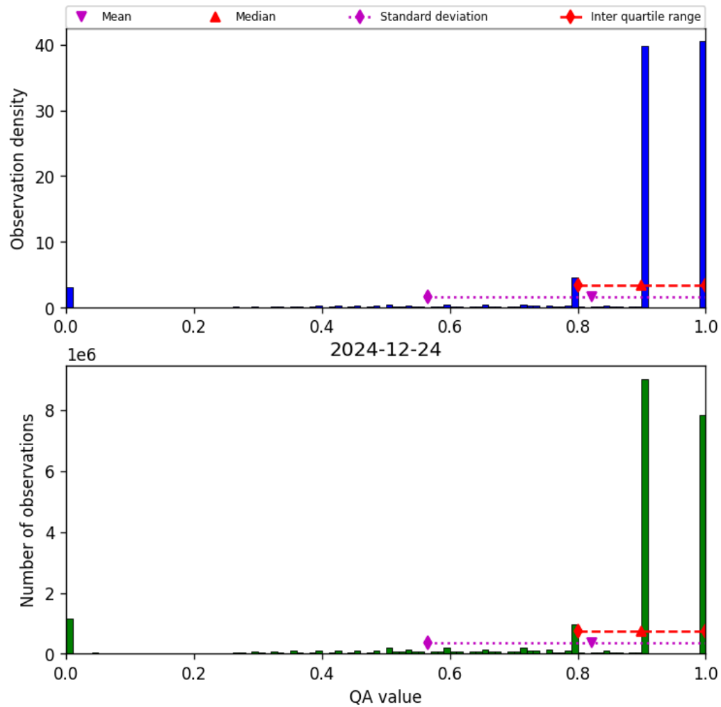
Figure 28: Histogram of “QA value” for 2024-12-24 to 2024-12-25
