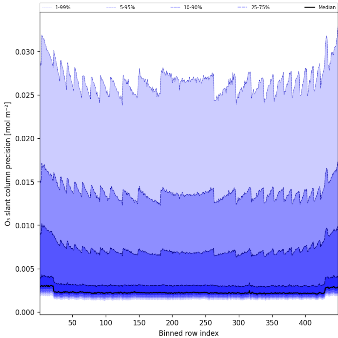
Figure 44: Along track statistics of “O 3 slant column precision” for 2024-12-24 to 2024-12-25
