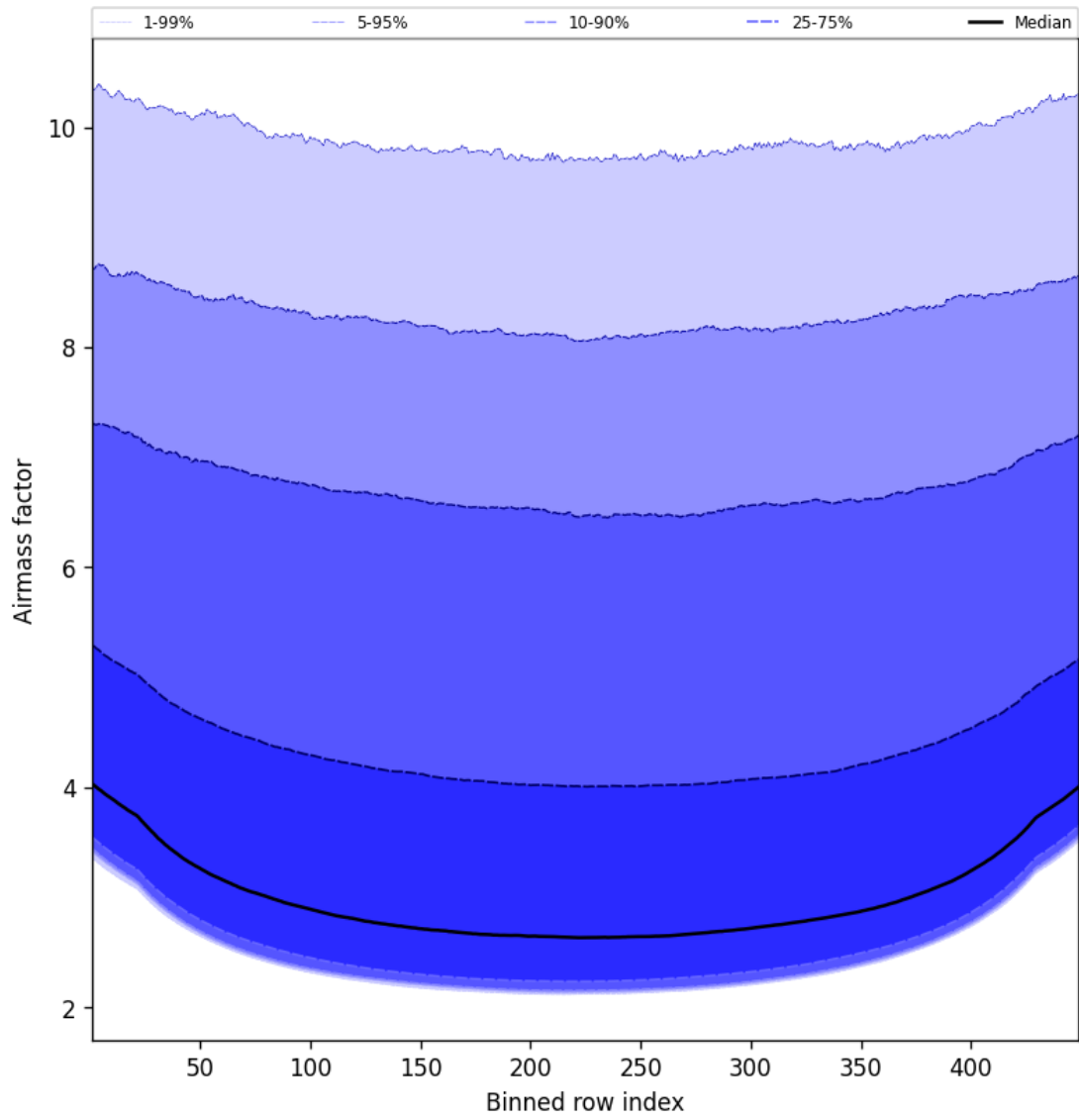
Figure 49: Along track statistics of “Airmass factor” for 2024-12-24 to 2024-12-25
