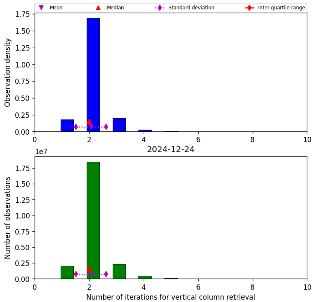
Figure 39: Histogram of “Number of iterations for vertical column retrieval” for 2024-12-24 to 2024-12-25
