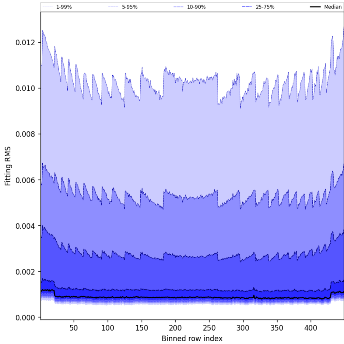
Figure 46: Along track statistics of “Fitting RMS” for 2024-12-24 to 2024-12-25
