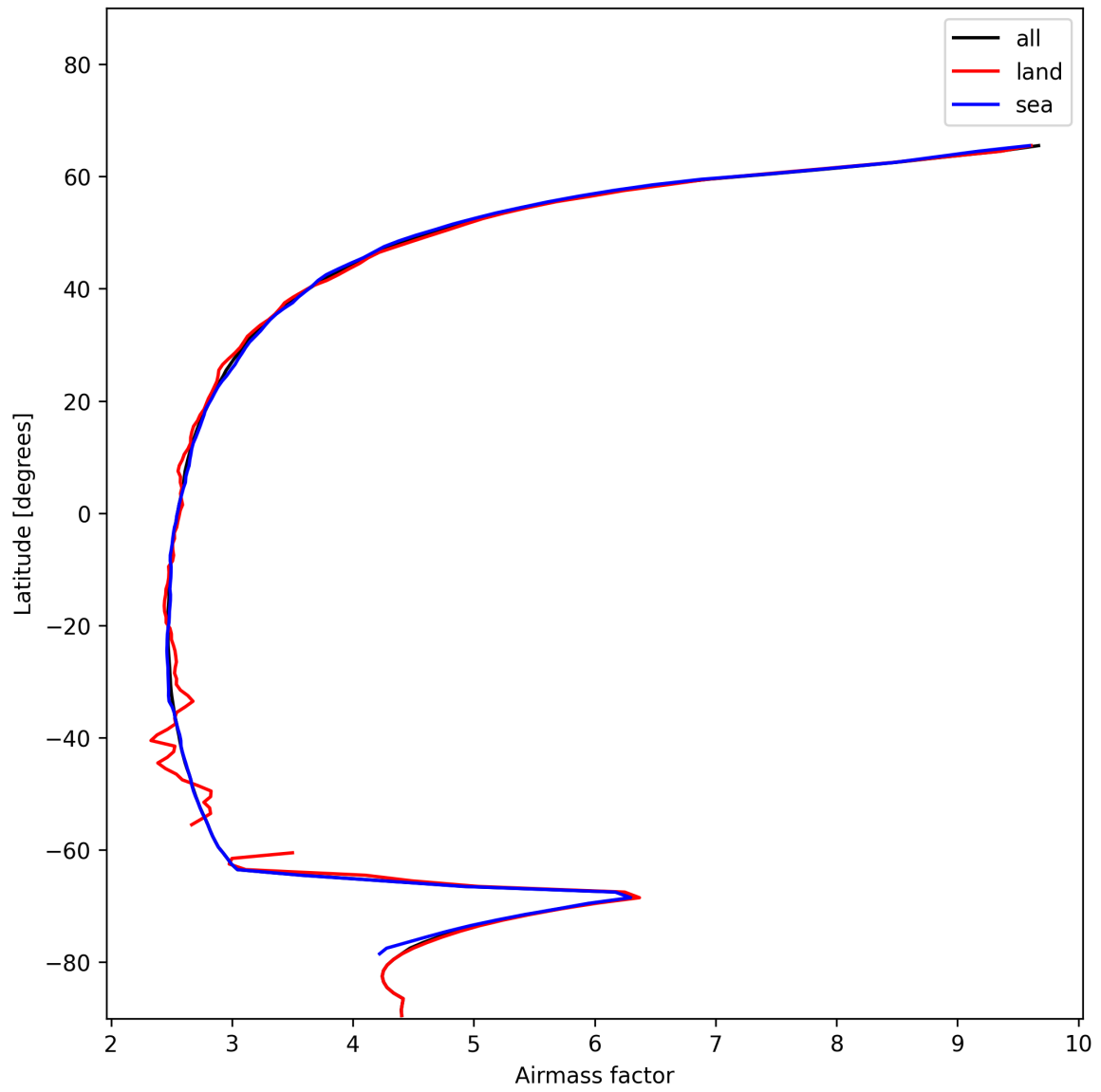
Figure 25: Zonal average of “Airmass factor” for 2024-12-24 to 2024-12-25.
