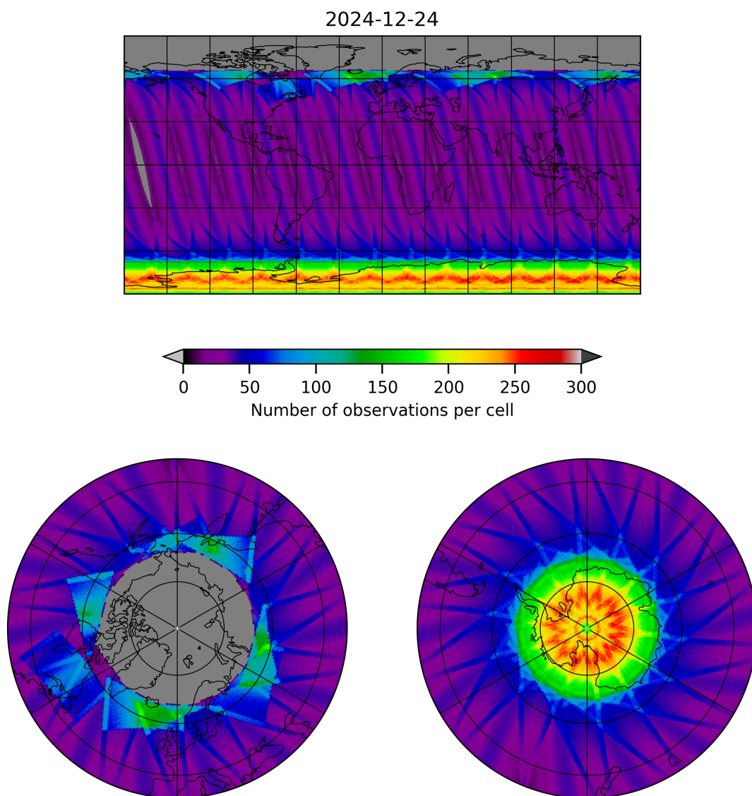
Figure 15: Map of the number of observations for 2024-12-24 to 2024-12-25
