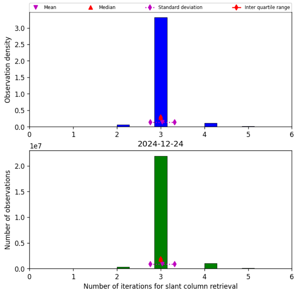
Figure 33: Histogram of “Number of iterations for slant column retrieval” for 2024-12-24 to 2024-12-25
