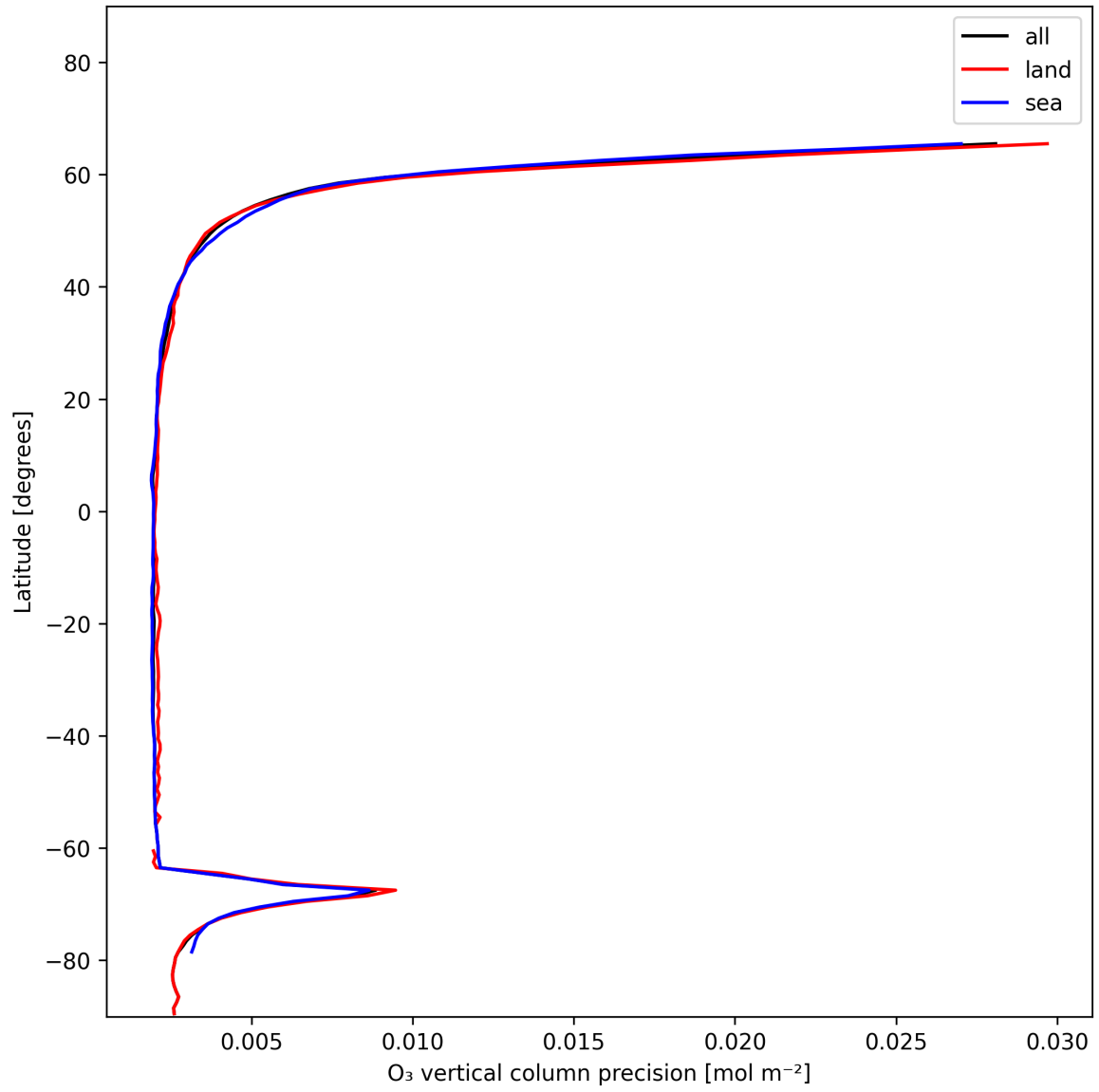
Figure 18: Zonal average of “O 3 vertical column precision” for 2024-12-24 to 2024-12-25.
