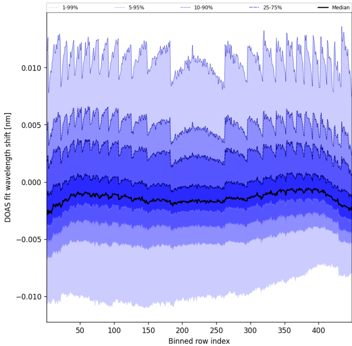
Figure 47: Along track statistics of “DOAS fit wavelength shift” for 2024-12-24 to 2024-12-25
