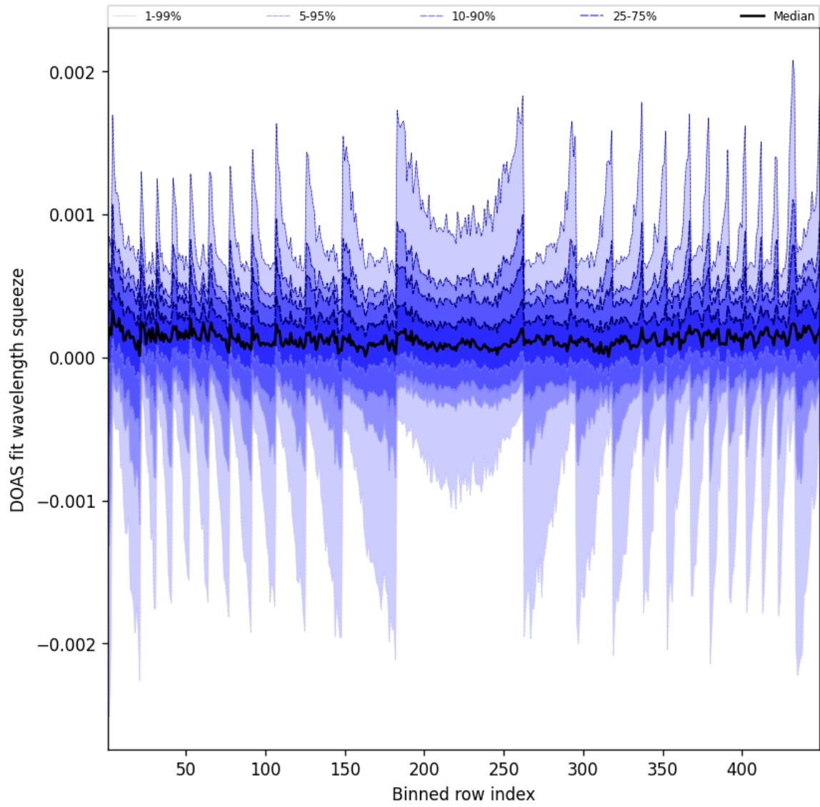
Figure 48: Along track statistics of “DOAS fit wavelength squeeze” for 2024-12-24 to 2024-12-25
