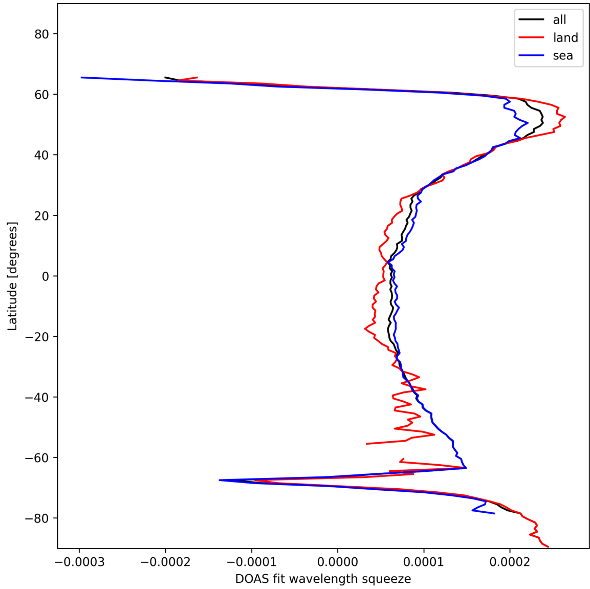
Figure 24: Zonal average of "DOAS fit wavelength squeeze" for 2024-12-24 to 2024-12-25.
