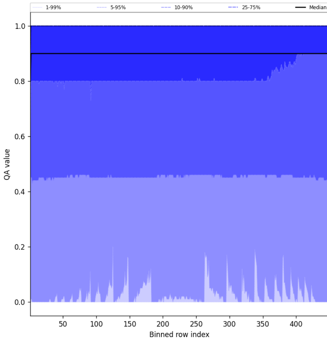
Figure 40: Along track statistics of “QA value” for 2024-12-24 to 2024-12-25
