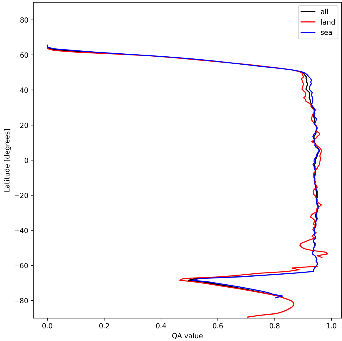
Figure 16: Zonal average of “QA value” for 2024-12-24 to 2024-12-25.
