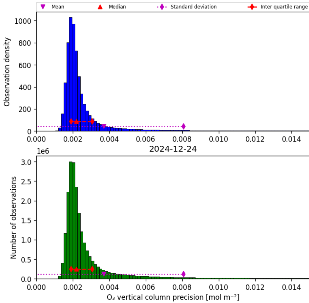
Figure 30: Histogram of “O 3 vertical column precision” for 2024-12-24 to 2024-12-25
