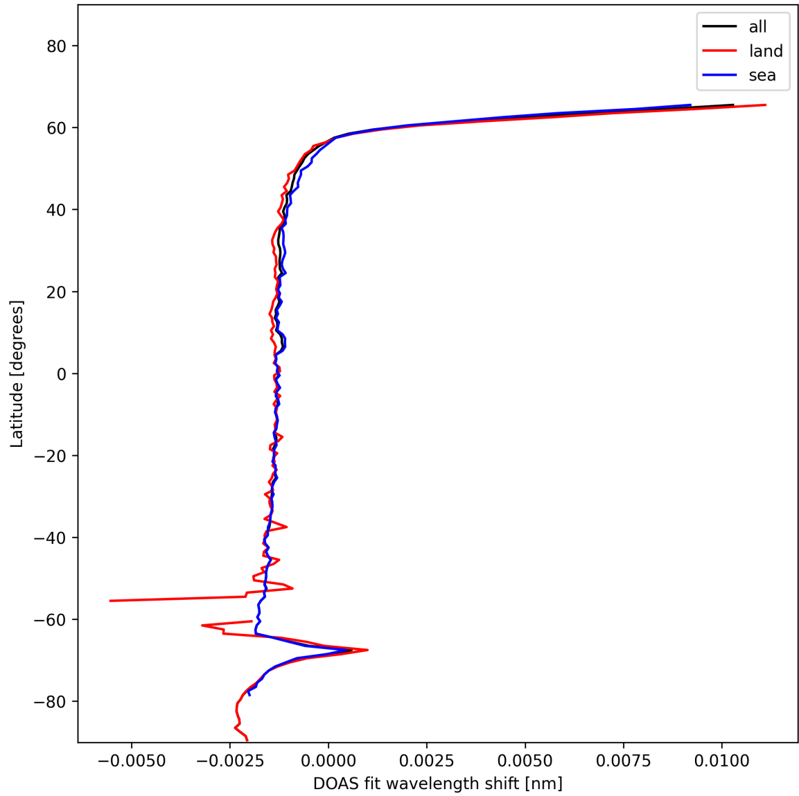
Figure 23: Zonal average of “DOAS fit wavelength shift” for 2024-12-24 to 2024-12-25.
