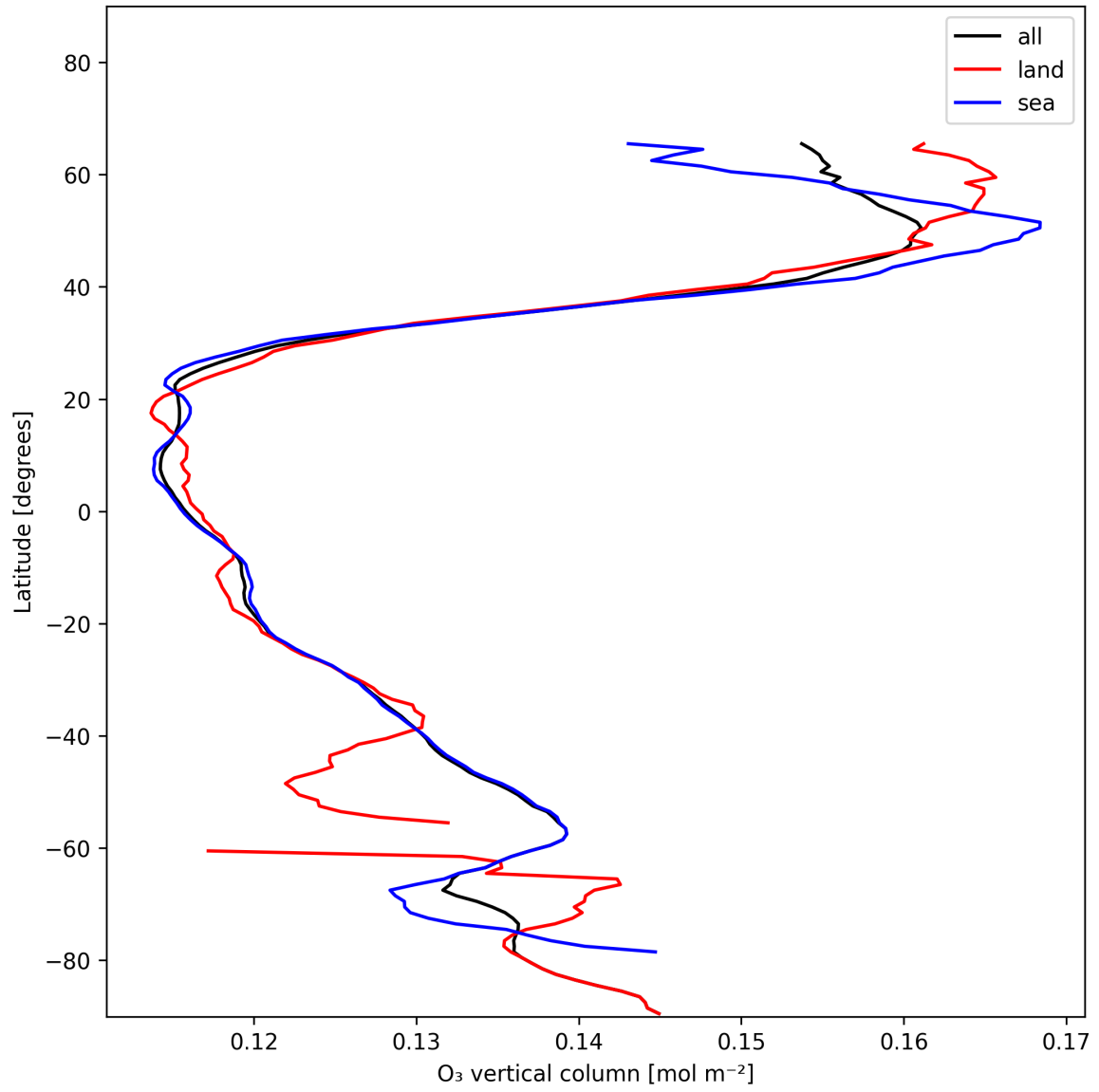
Figure 17: Zonal average of “O 3 vertical column” for 2024-12-24 to 2024-12-25.
