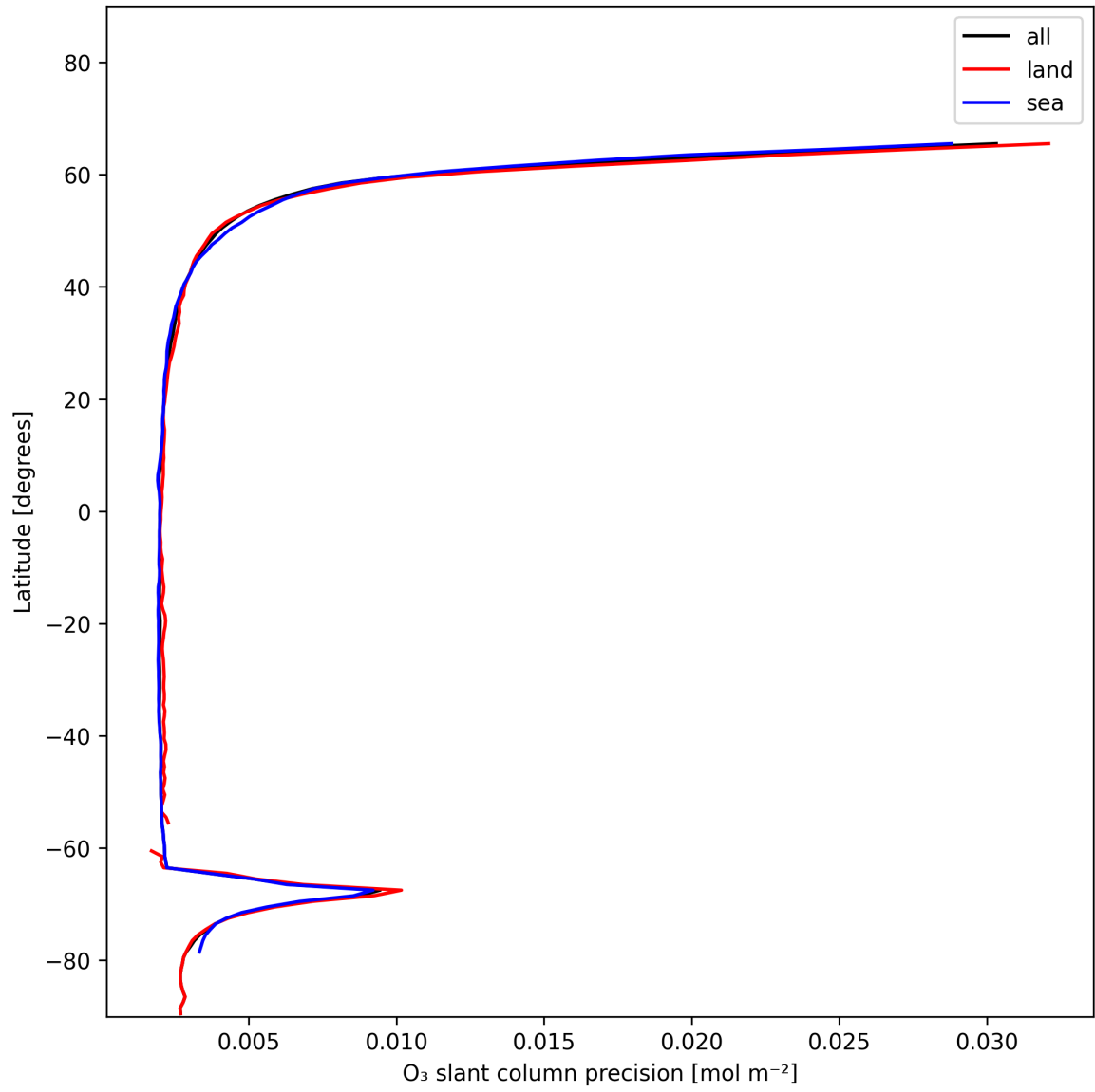
Figure 20: Zonal average of “O 3 slant column precision” for 2024-12-24 to 2024-12-25.
