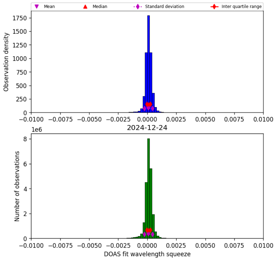
Figure 36: Histogram of “DOAS fit wavelength squeeze” for 2024-12-24 to 2024-12-25
