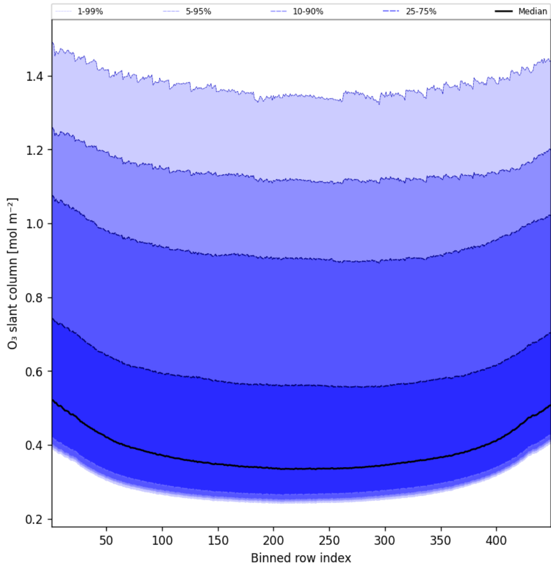
Figure 43: Along track statistics of “O 3 slant column” for 2024-12-24 to 2024-12-25
