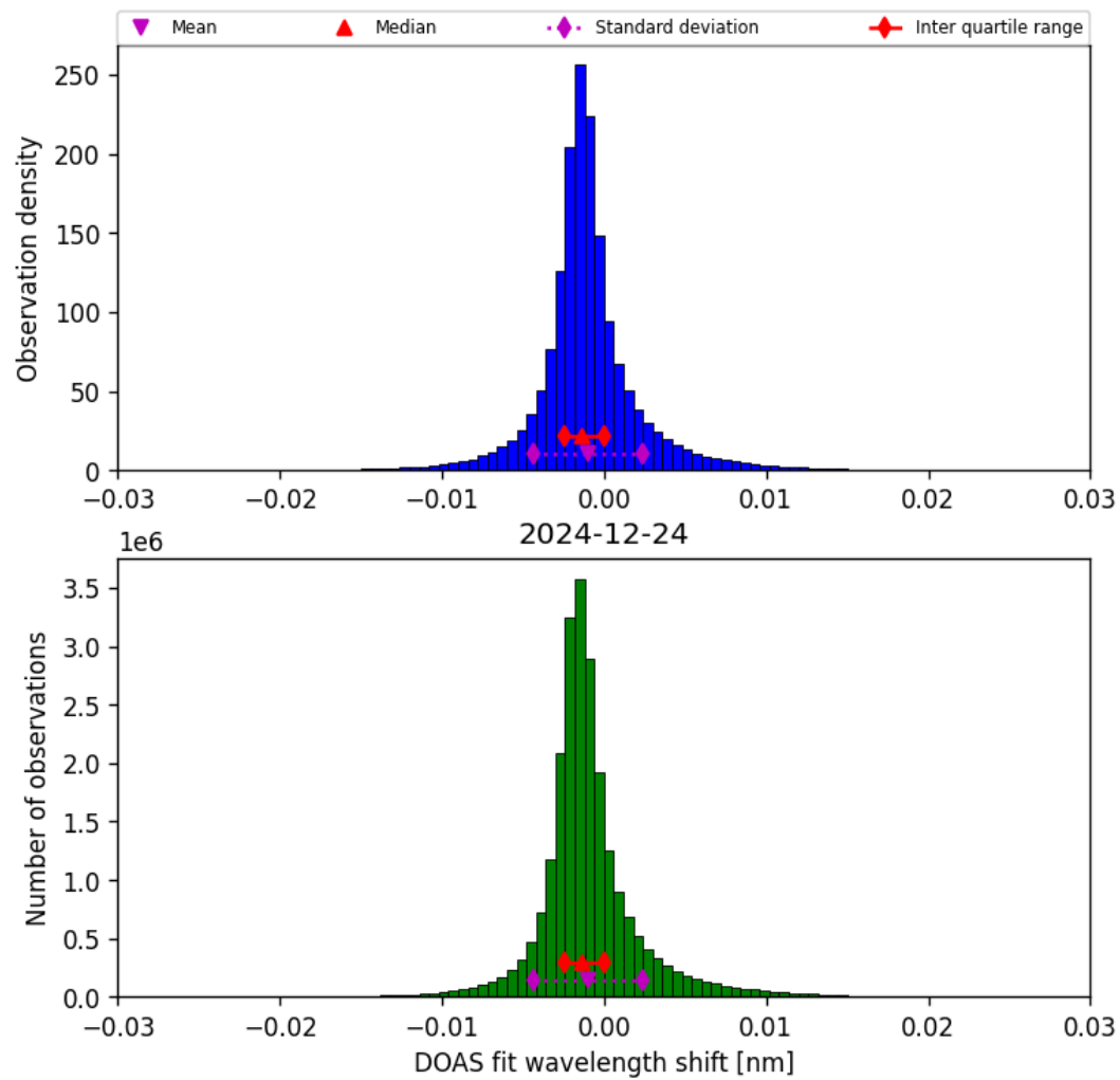
Figure 35: Histogram of “DOAS fit wavelength shift” for 2024-12-24 to 2024-12-25
