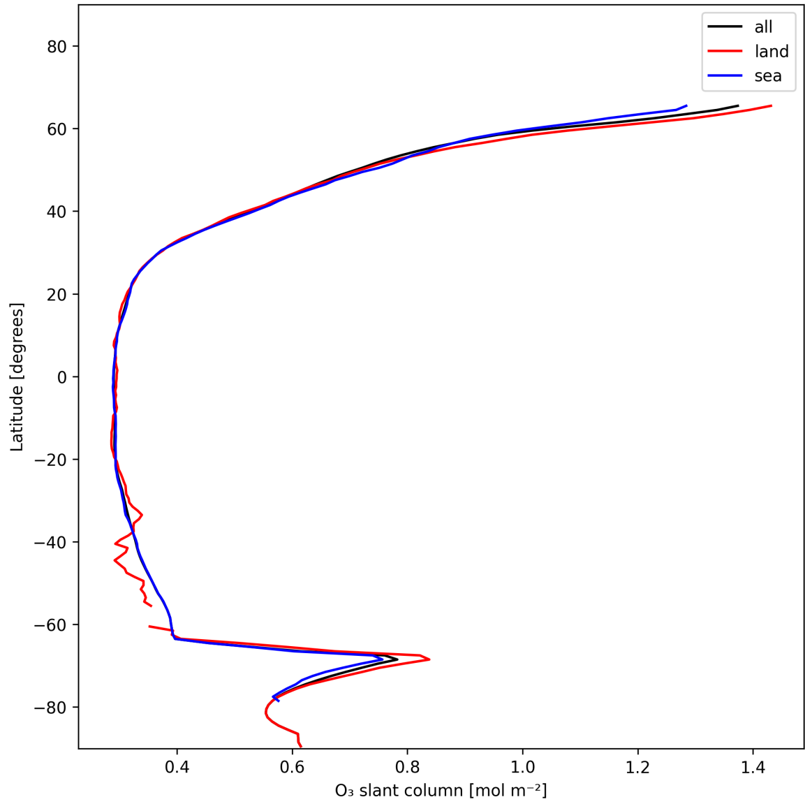
Figure 19: Zonal average of “O 3 slant column” for 2024-12-24 to 2024-12-25.
