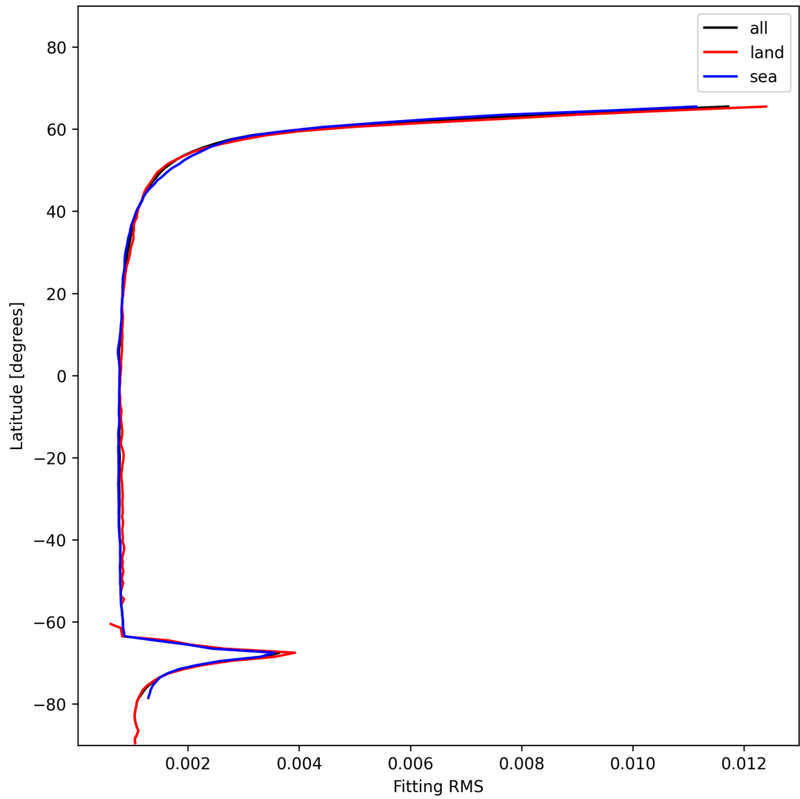
Figure 22: Zonal average of “Fitting RMS” for 2024-12-24 to 2024-12-25.
