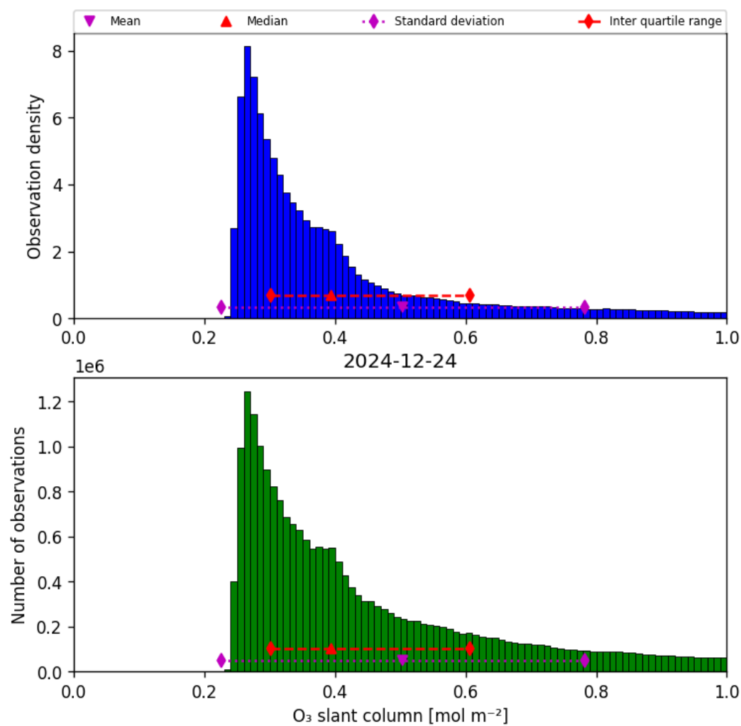
Figure 31: Histogram of “O 3 slant column” for 2024-12-24 to 2024-12-25
