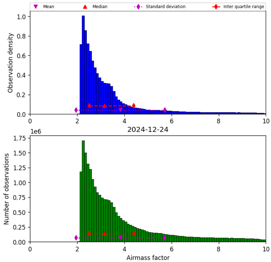
Figure 37: Histogram of “Airmass factor” for 2024-12-24 to 2024-12-25
