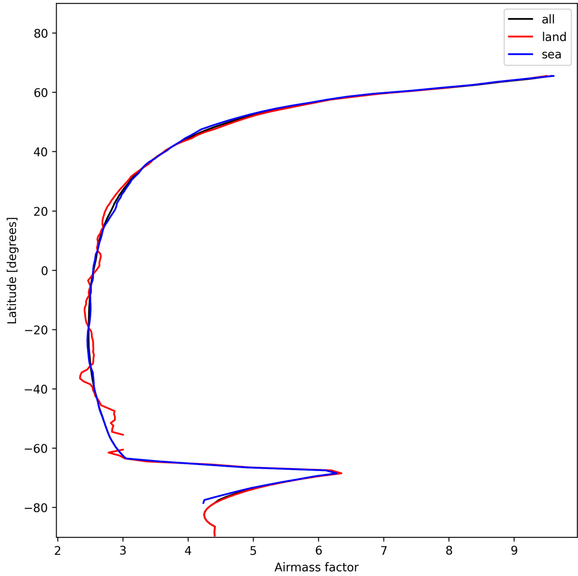
Figure 25: Zonal average of “Airmass factor” for 2024-12-25 to 2024-12-25.
