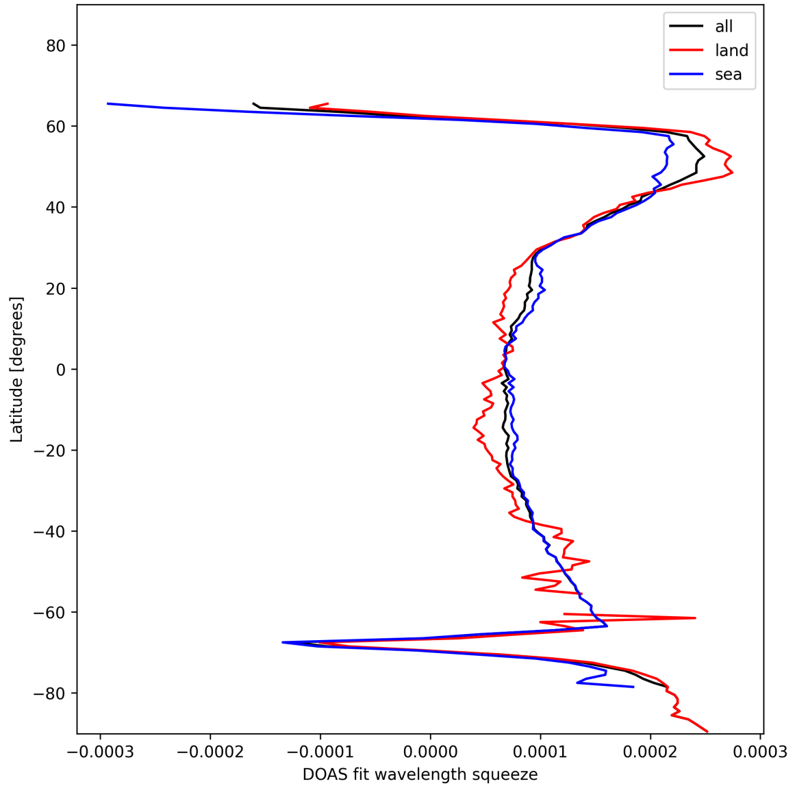
Figure 24: Zonal average of “DOAS fit wavelength squeeze” for 2024-12-25 to 2024-12-25.
