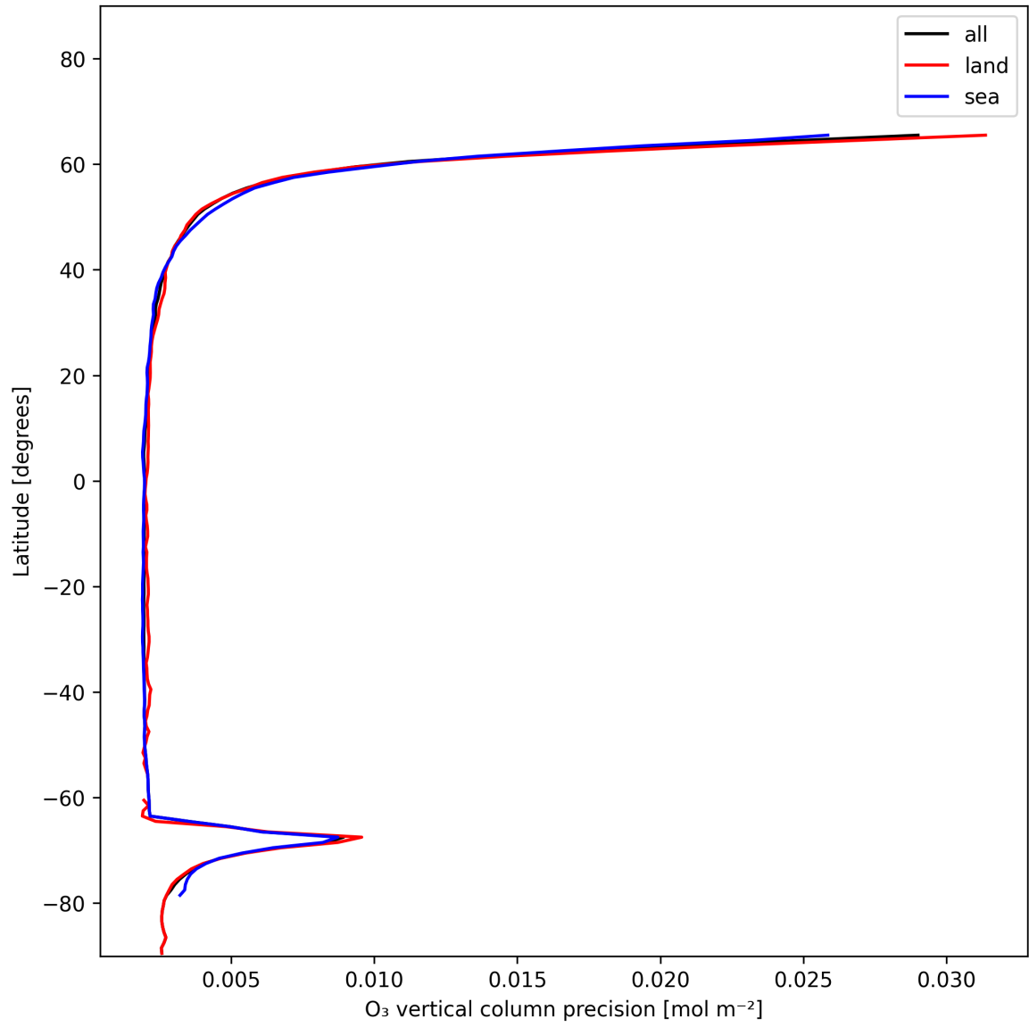
Figure 18: Zonal average of “O 3 vertical column precision” for 2024-12-25 to 2024-12-25.
