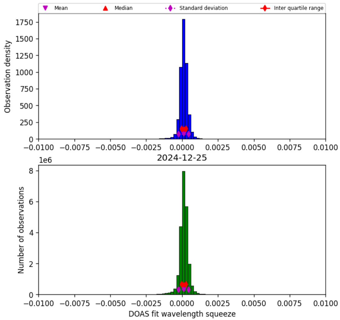
Figure 36: Histogram of “DOAS fit wavelength squeeze” for 2024-12-25 to 2024-12-25
