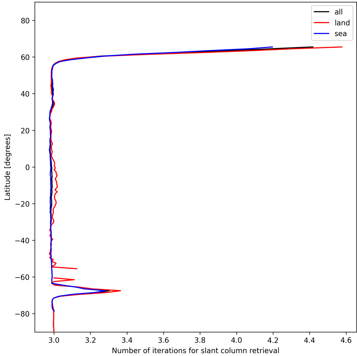
Figure 21: Zonal average of “Number of iterations for slant column retrieval” for 2024-12-25 to 2024-12-25.
