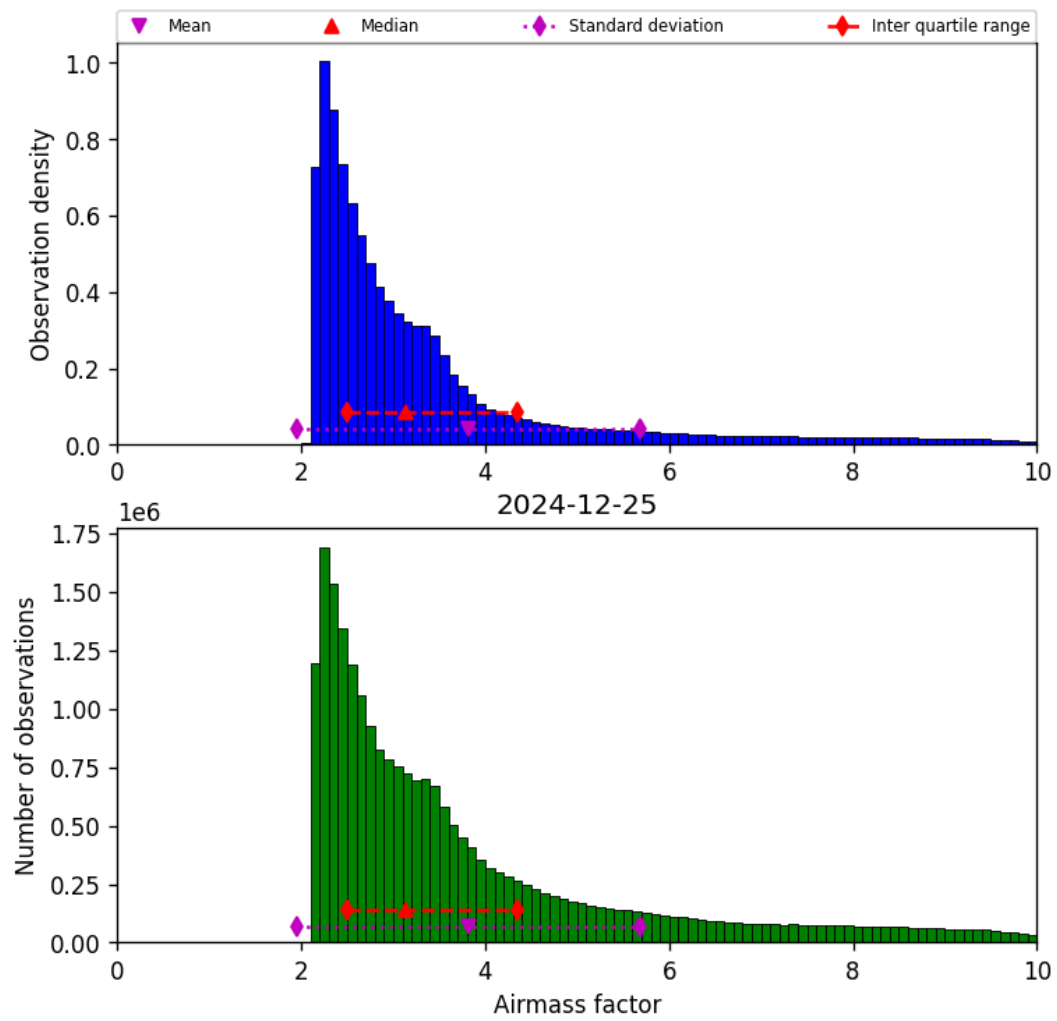
Figure 37: Histogram of “Airmass factor” for 2024-12-25 to 2024-12-25
