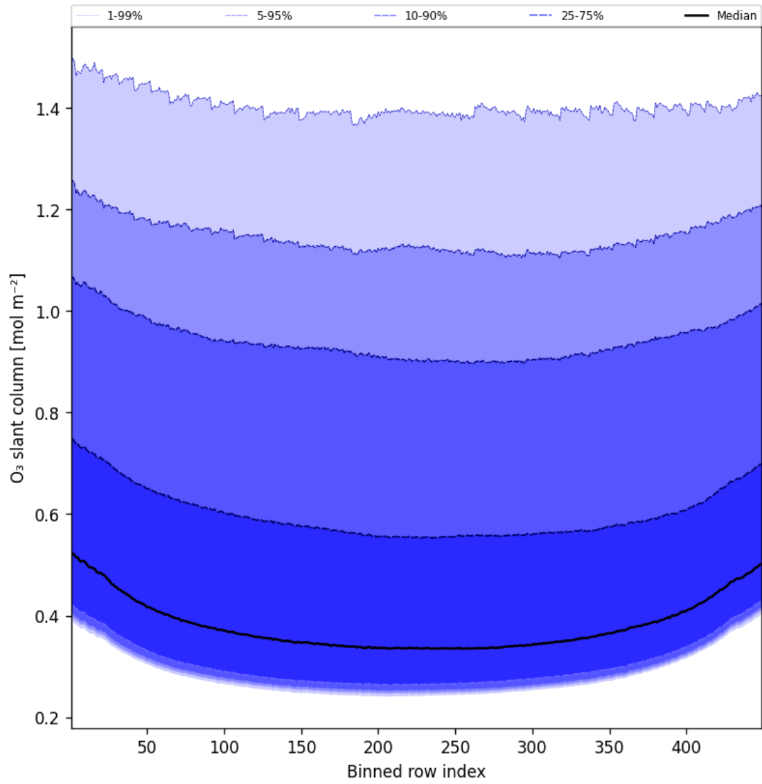
Figure 43: Along track statistics of “O 3 slant column” for 2024-12-25 to 2024-12-25
