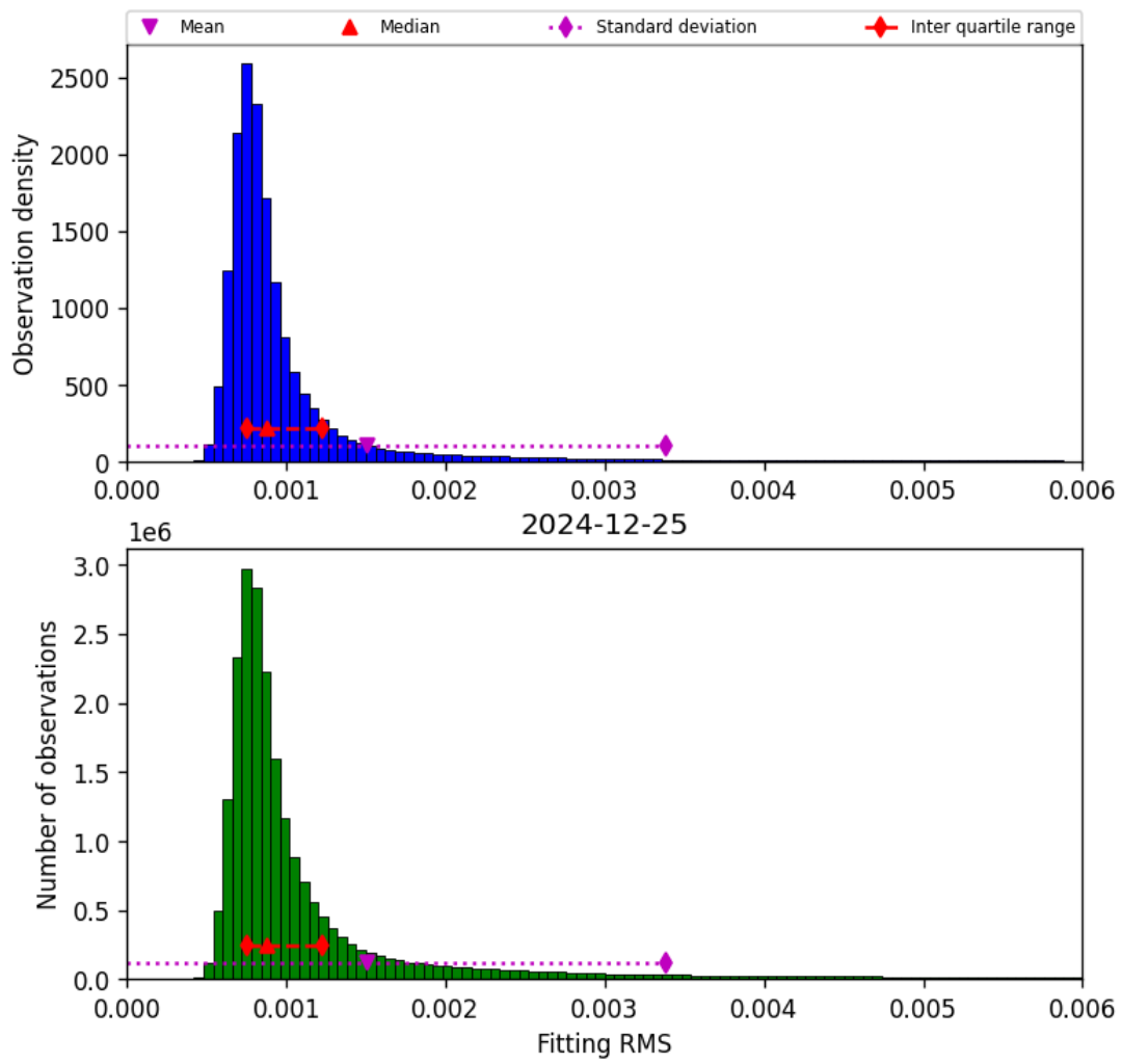
Figure 34: Histogram of “Fitting RMS” for 2024-12-25 to 2024-12-25
