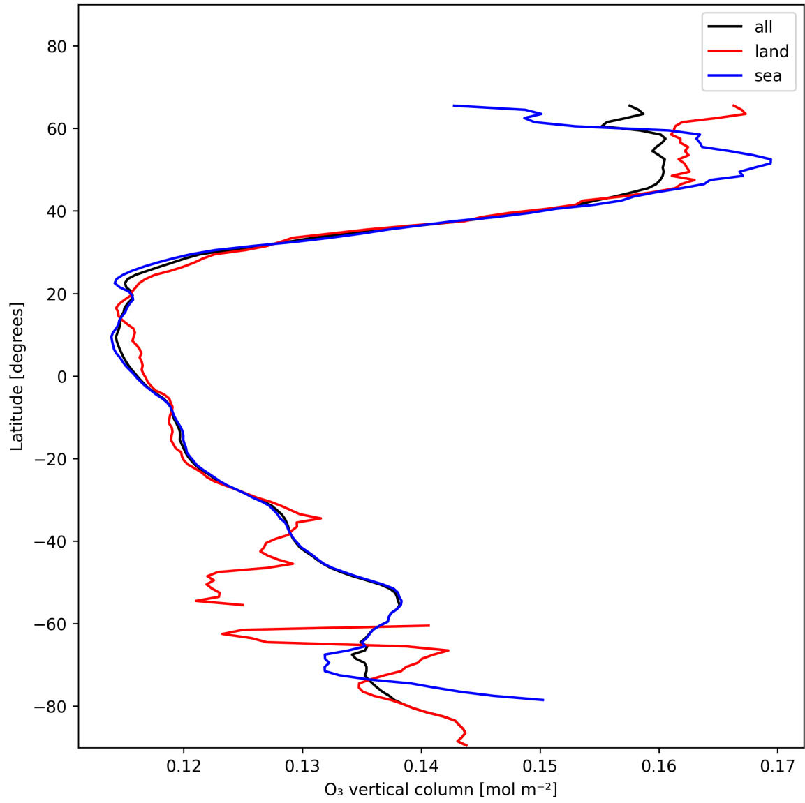
Figure 17: Zonal average of “O 3 vertical column” for 2024-12-25 to 2024-12-25.
