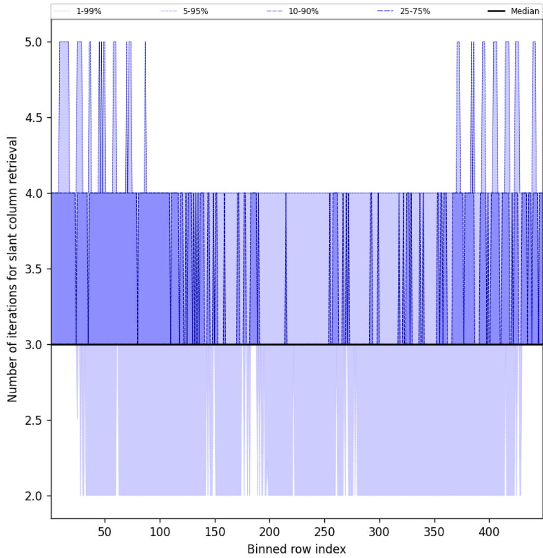
Figure 45: Along track statistics of “Number of iterations for slant column retrieval” for 2024-12-25 to 2024-12-25
