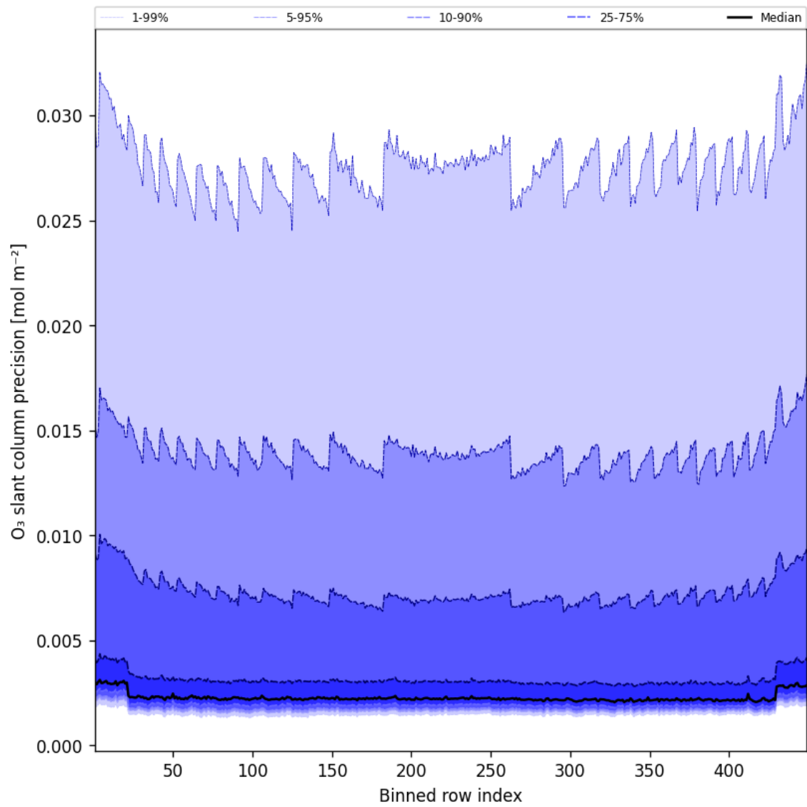
Figure 44: Along track statistics of “O 3 slant column precision” for 2024-12-25 to 2024-12-25
