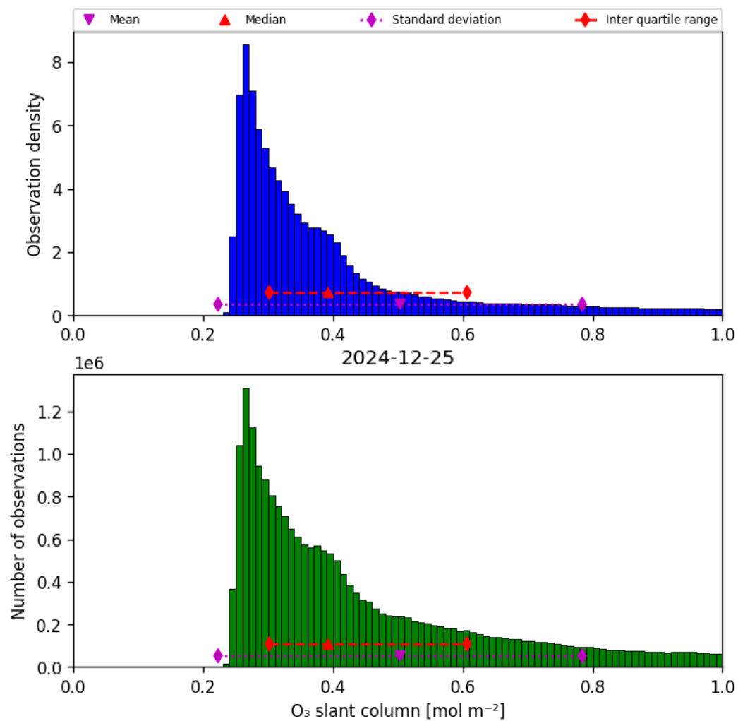
Figure 31: Histogram of “O 3 slant column” for 2024-12-25 to 2024-12-25
