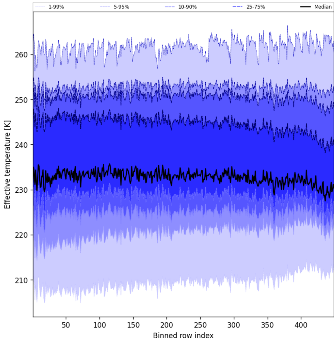
Figure 50: Along track statistics of “Effective temperature” for 2024-12-25 to 2024-12-25
