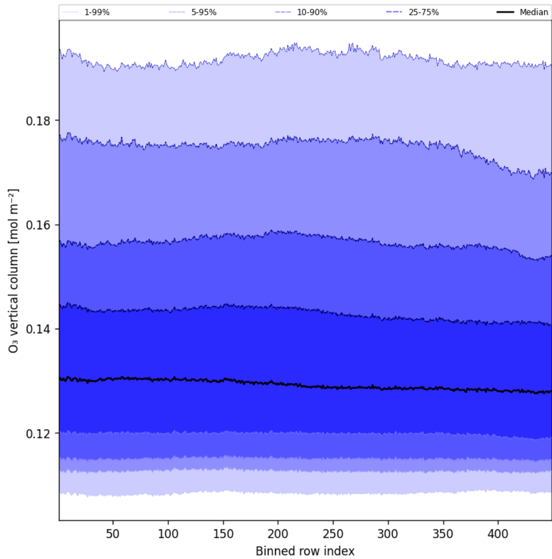
Figure 41: Along track statistics of “O 3 vertical column” for 2024-12-25 to 2024-12-25
