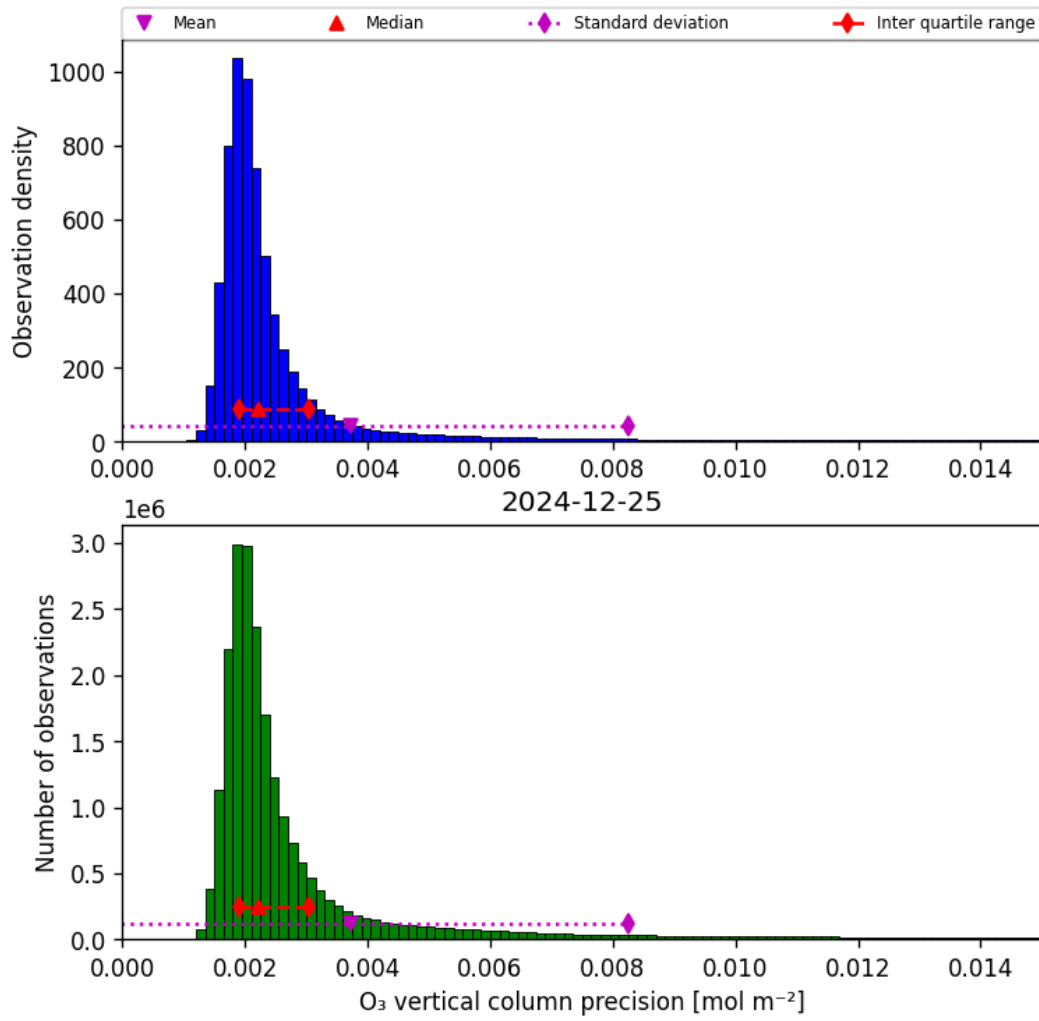
Figure 30: Histogram of “O 3 vertical column precision” for 2024-12-25 to 2024-12-25
