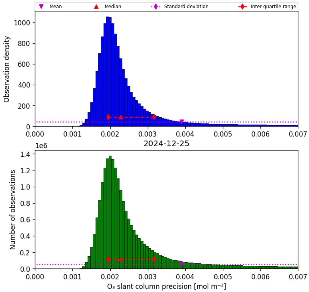
Figure 32: Histogram of “O 3 slant column precision” for 2024-12-25 to 2024-12-25
