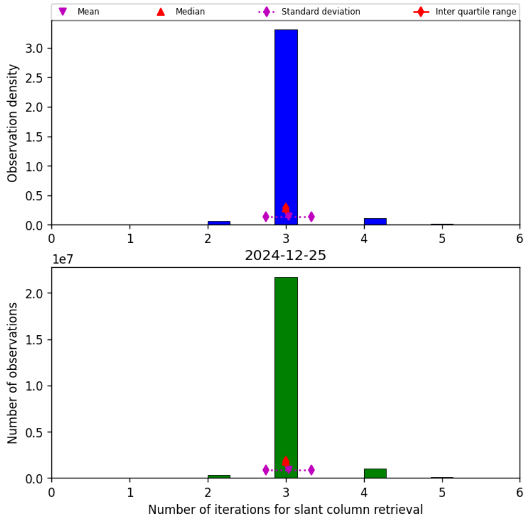
Figure 33: Histogram of "Number of iterations for slant column retrieval" for 2024-12-25 to 2024-12-25
