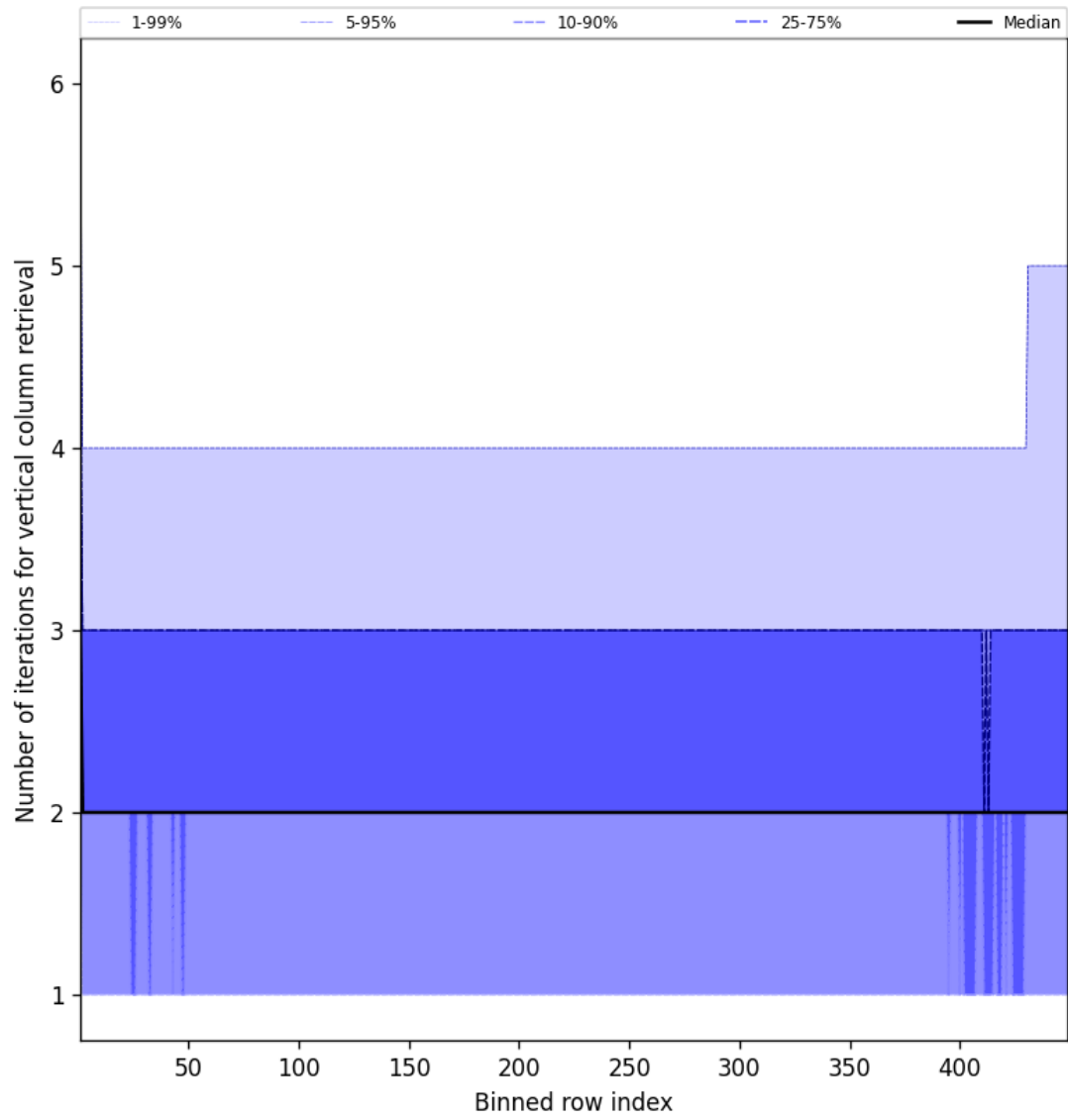
Figure 51: Along track statistics of “Number of iterations for vertical column retrieval” for 2024-12-25 to 2024-12-25
