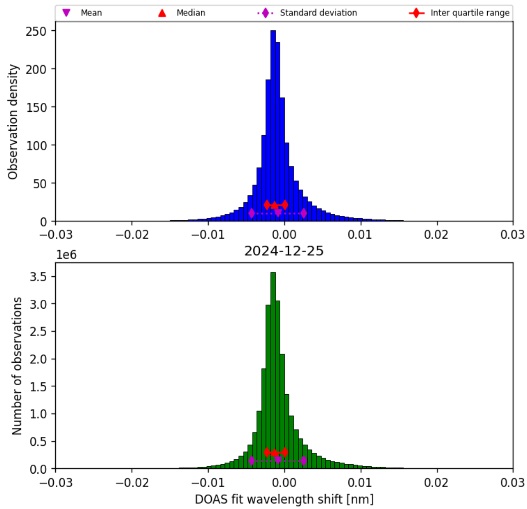
Figure 35: Histogram of “DOAS fit wavelength shift” for 2024-12-25 to 2024-12-25
