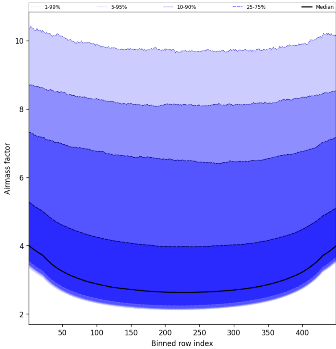
Figure 49: Along track statistics of “Airmass factor” for 2024-12-25 to 2024-12-25
