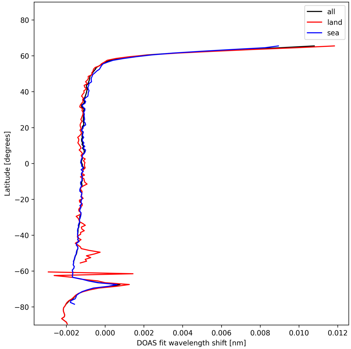
Figure 23: Zonal average of “DOAS fit wavelength shift” for 2024-12-25 to 2024-12-25.
