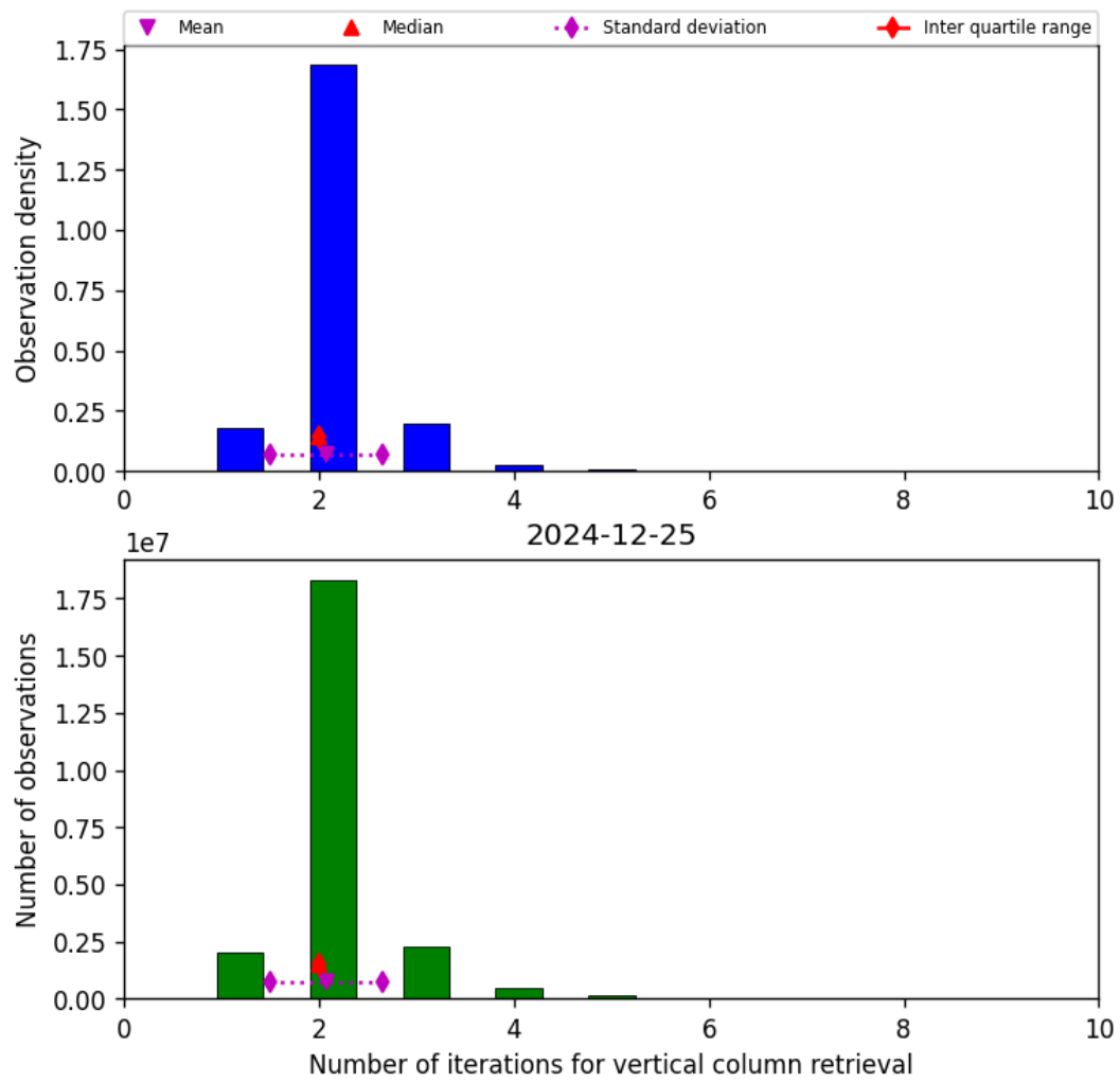
Figure 39: Histogram of “Number of iterations for vertical column retrieval” for 2024-12-25 to 2024-12-25
