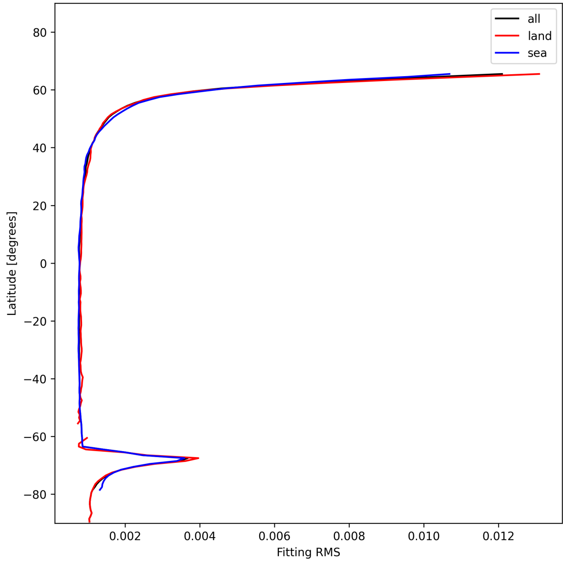
Figure 22: Zonal average of “Fitting RMS” for 2024-12-25 to 2024-12-25.
