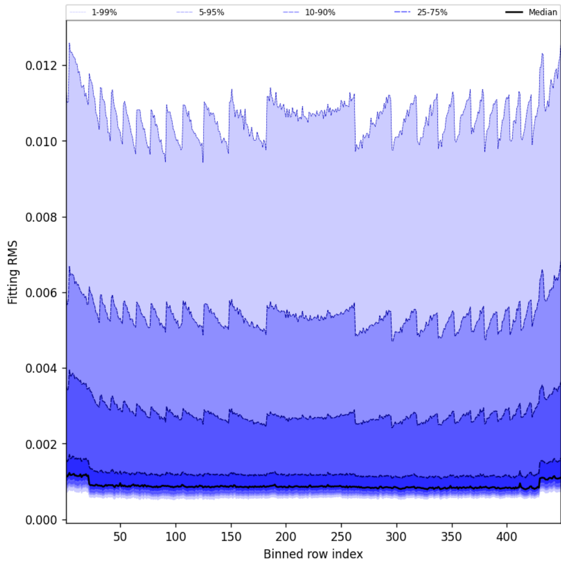
Figure 46: Along track statistics of “Fitting RMS” for 2024-12-25 to 2024-12-25
