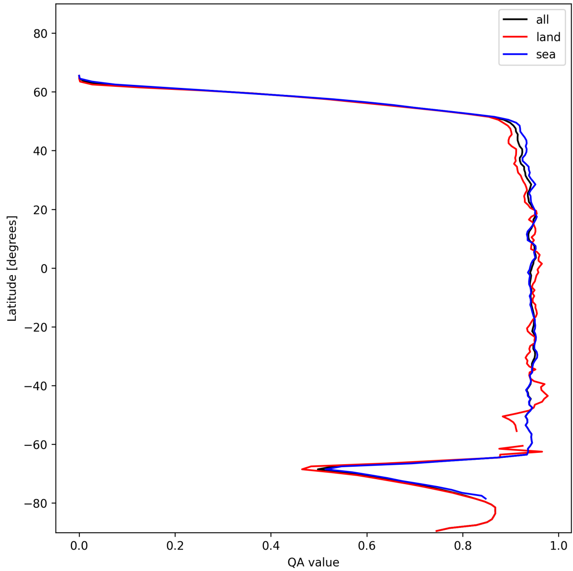
Figure 16: Zonal average of “QA value” for 2024-12-25 to 2024-12-25.
