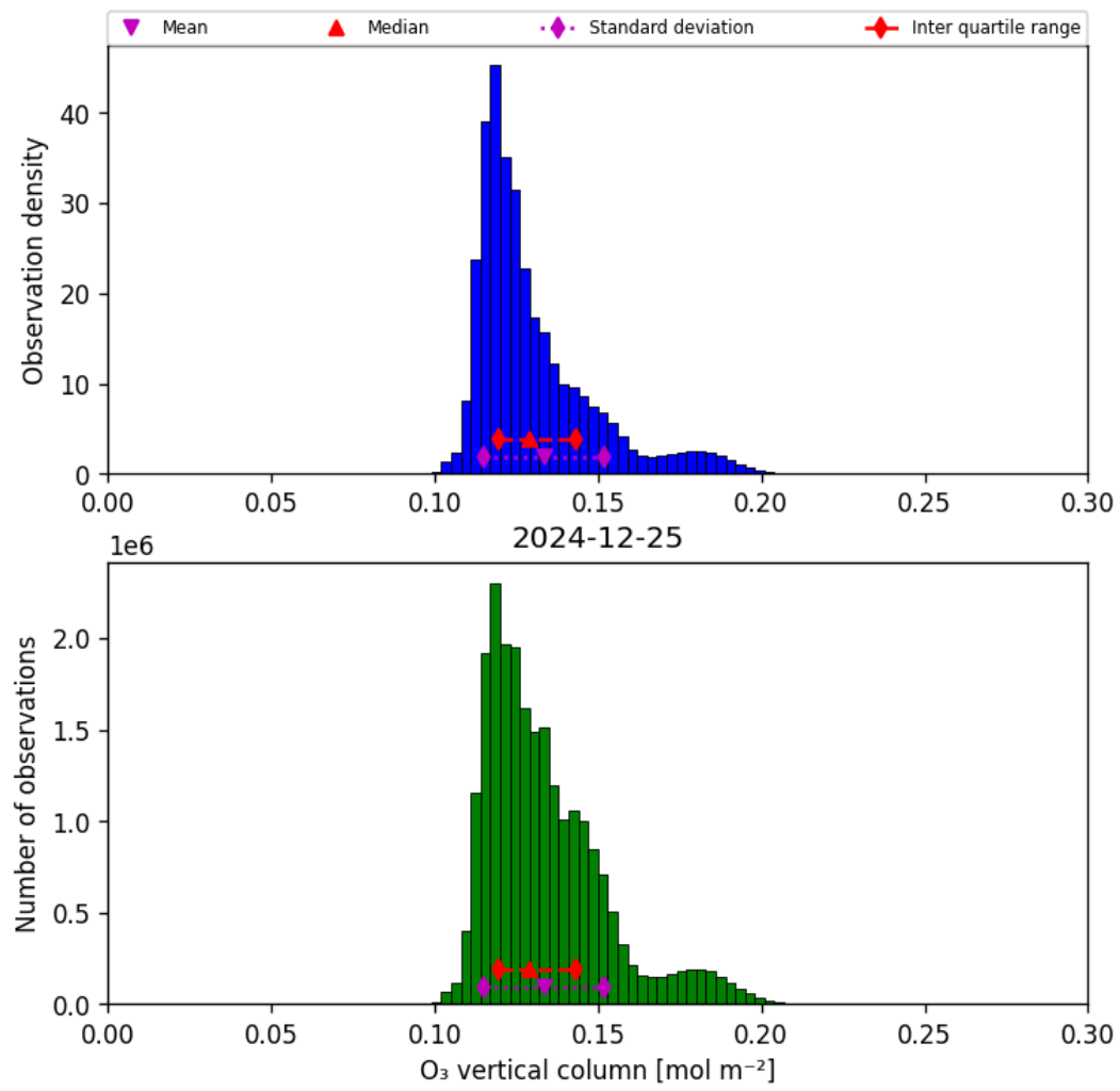
Figure 29: Histogram of “O 3 vertical column” for 2024-12-25 to 2024-12-25
