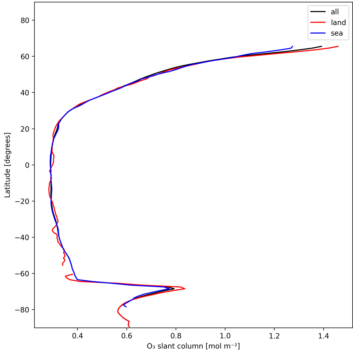
Figure 19: Zonal average of “O 3 slant column” for 2024-12-25 to 2024-12-25.
