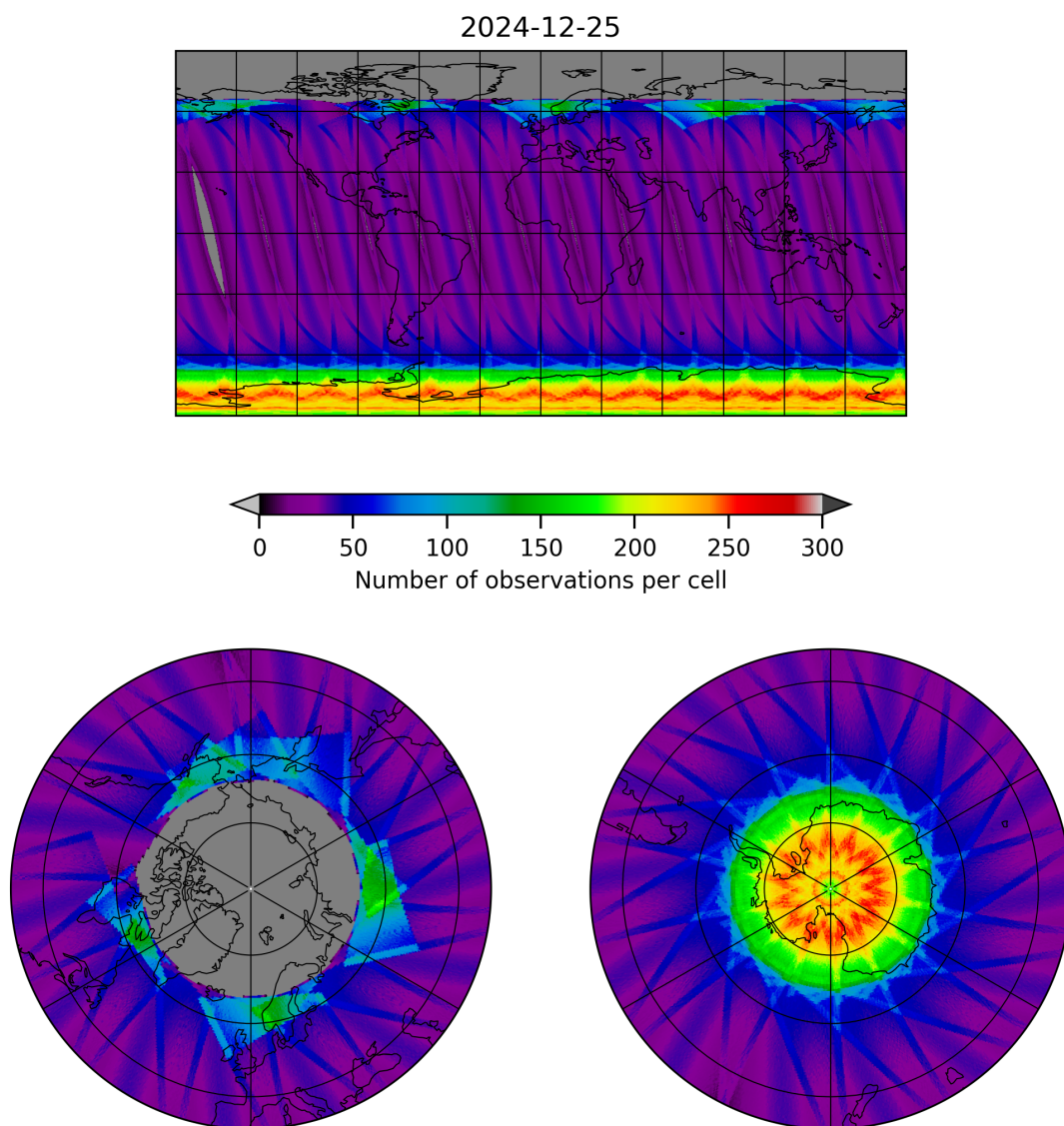
Figure 15: Map of the number of observations for 2024-12-25 to 2024-12-25
