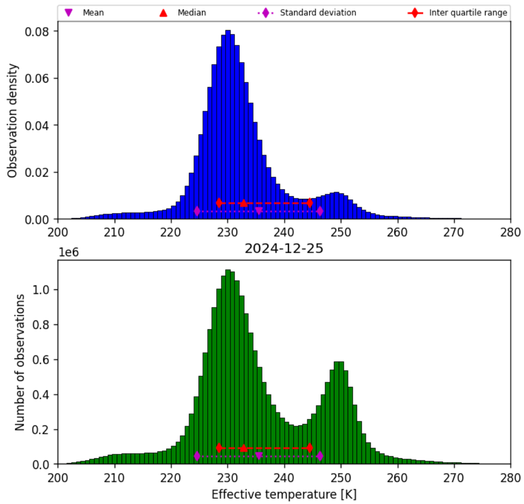
Figure 38: Histogram of “Effective temperature” for 2024-12-25 to 2024-12-25
