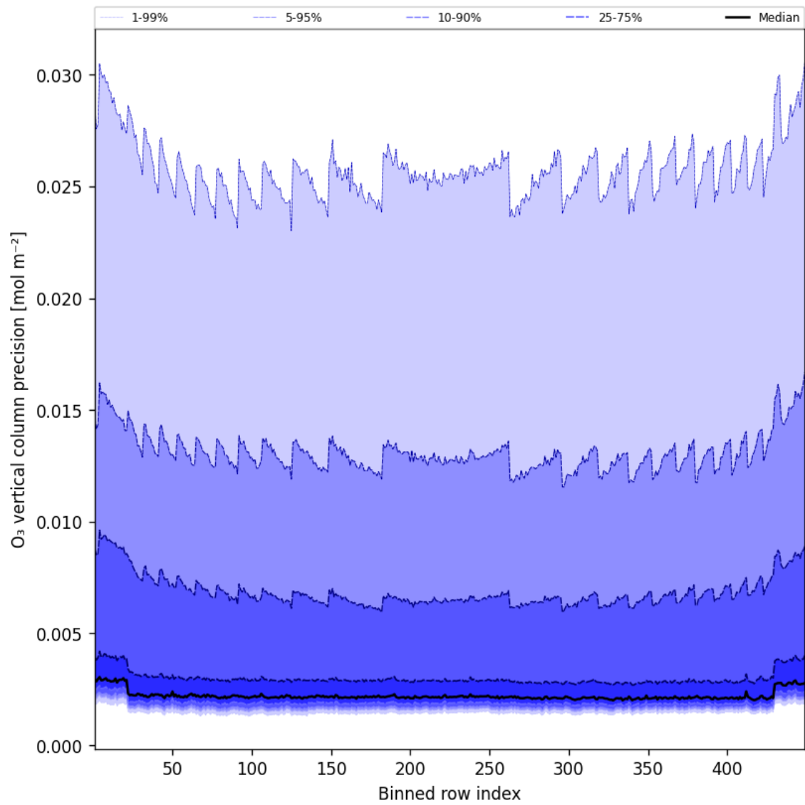
Figure 42: Along track statistics of “O 3 vertical column precision” for 2024-12-25 to 2024-12-25
