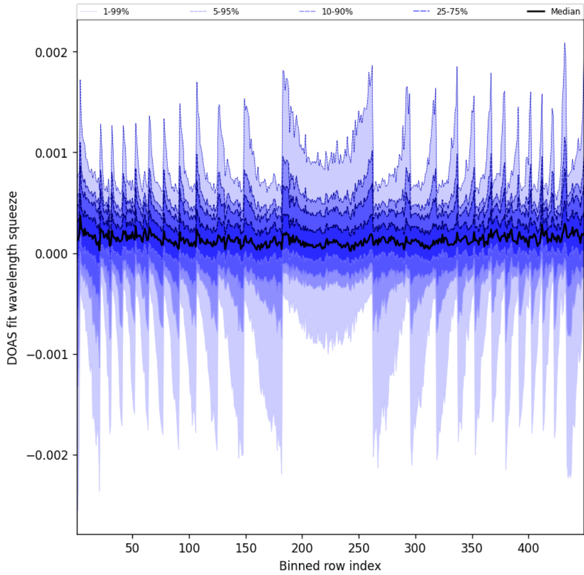
Figure 48: Along track statistics of “DOAS fit wavelength squeeze” for 2024-12-25 to 2024-12-25
