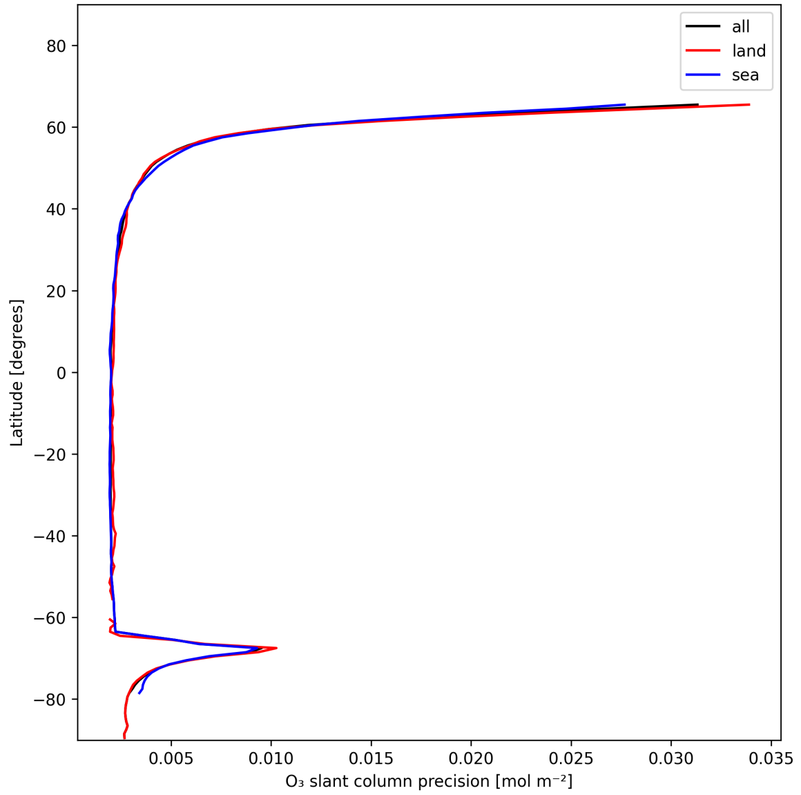
Figure 20: Zonal average of “O 3 slant column precision” for 2024-12-25 to 2024-12-25.
