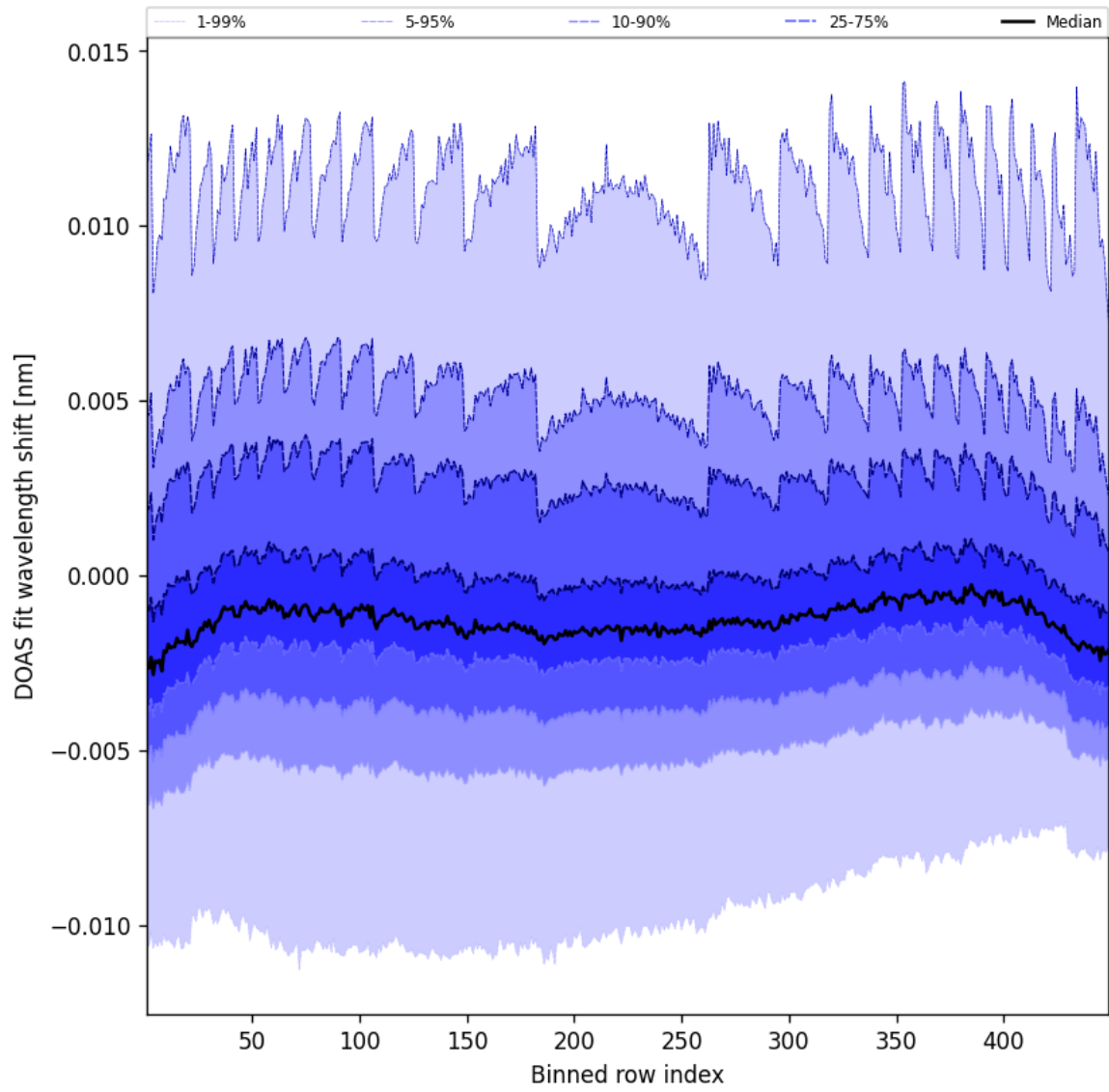
Figure 47: Along track statistics of “DOAS fit wavelength shift” for 2024-12-25 to 2024-12-25
