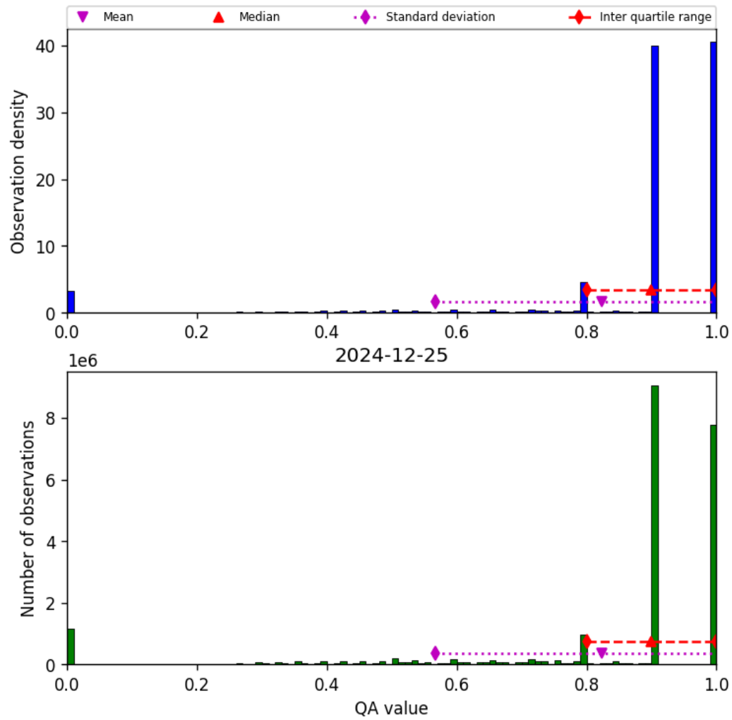
Figure 28: Histogram of “QA value” for 2024-12-25 to 2024-12-25
