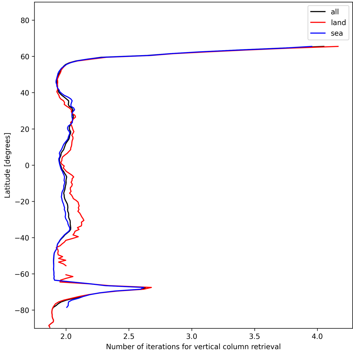
Figure 27: Zonal average of “Number of iterations for vertical column retrieval” for 2024-12-25 to 2024-12-25.
