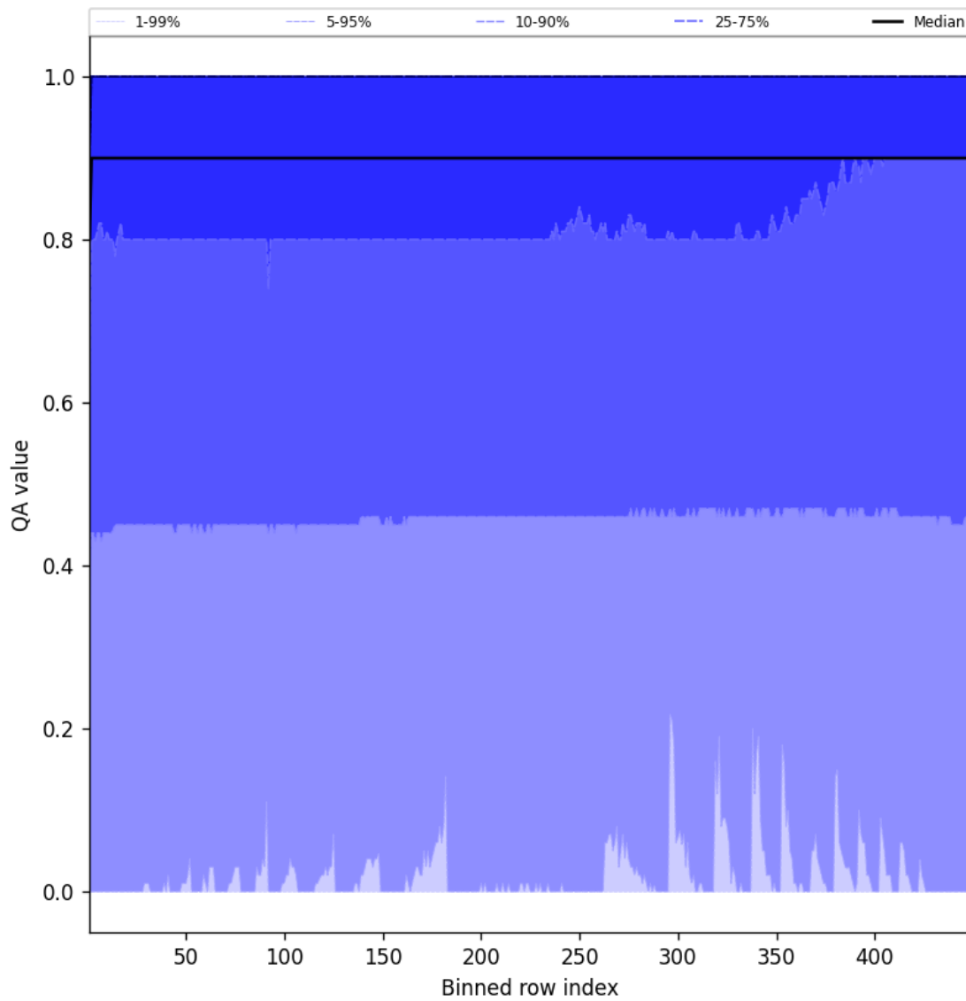
Figure 40: Along track statistics of “QA value” for 2024-12-25 to 2024-12-25
