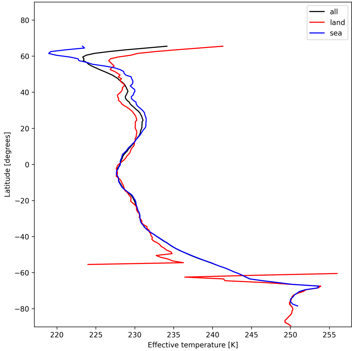
Figure 26: Zonal average of “Effective temperature” for 2024-12-25 to 2024-12-25.
