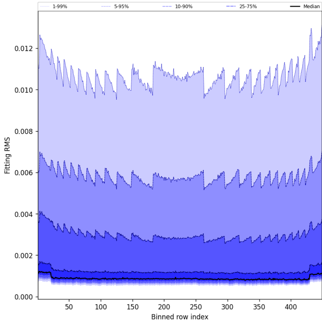
Figure 46: Along track statistics of “Fitting RMS” for 2024-12-29 to 2024-12-30
