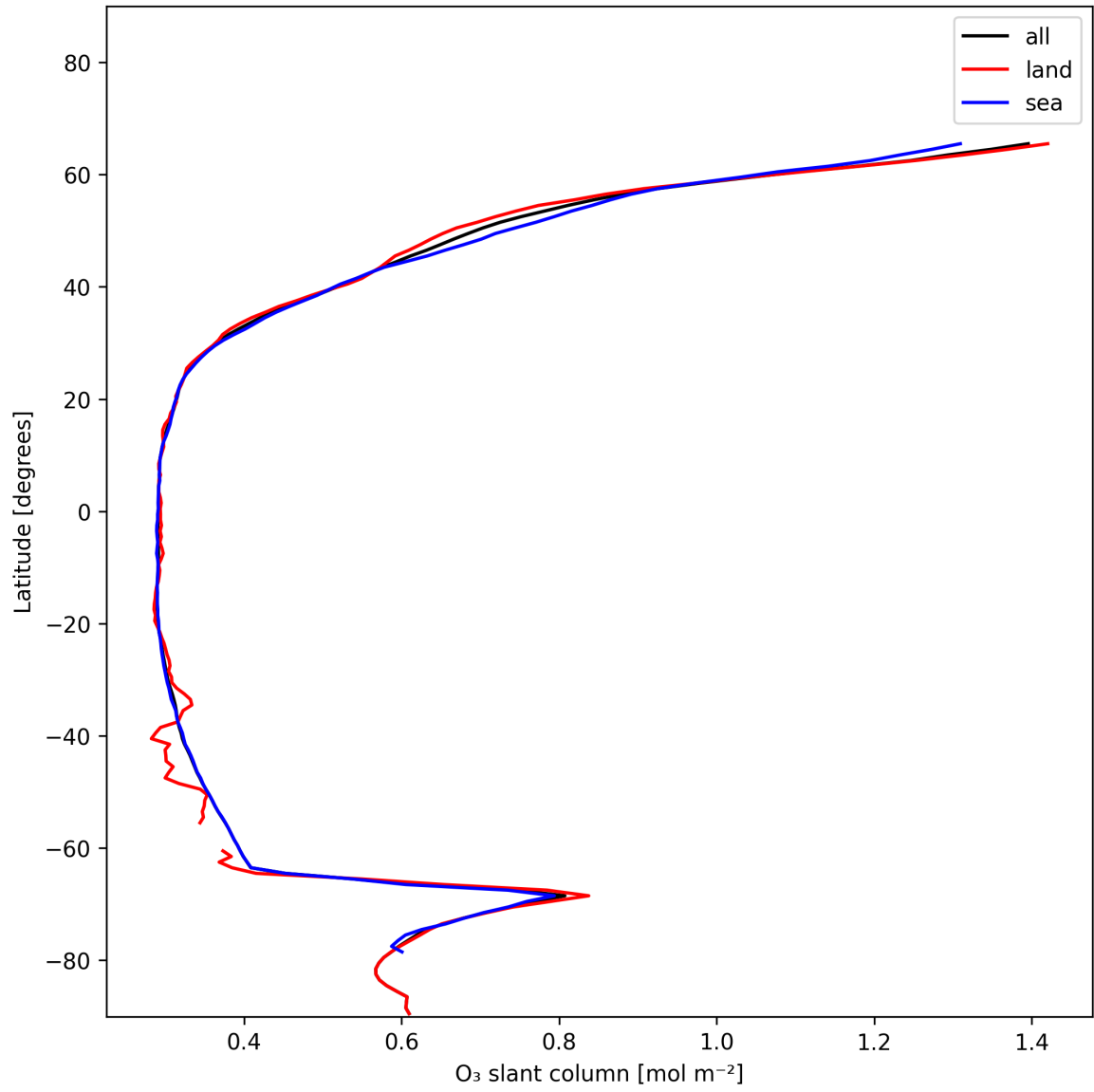
Figure 19: Zonal average of “O 3 slant column” for 2024-12-29 to 2024-12-30.
