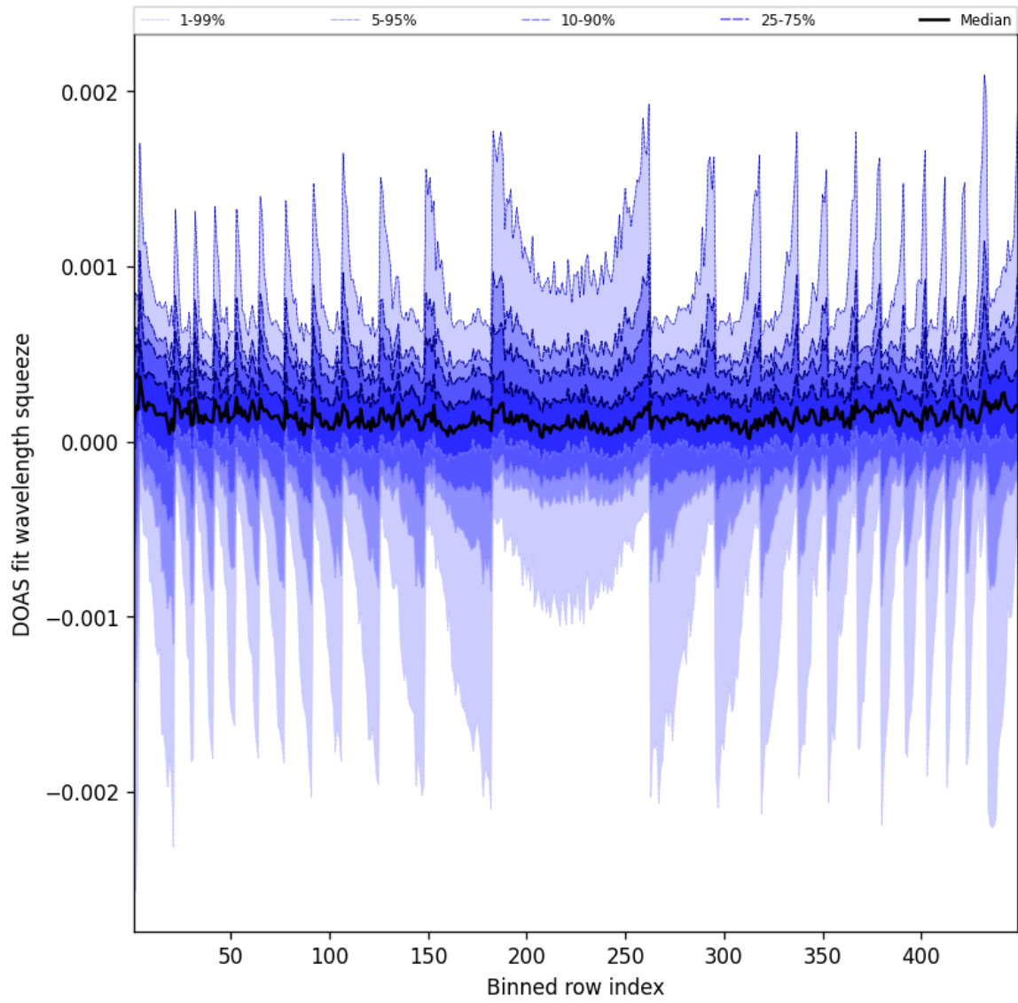
Figure 48: Along track statistics of “DOAS fit wavelength squeeze” for 2024-12-29 to 2024-12-30
