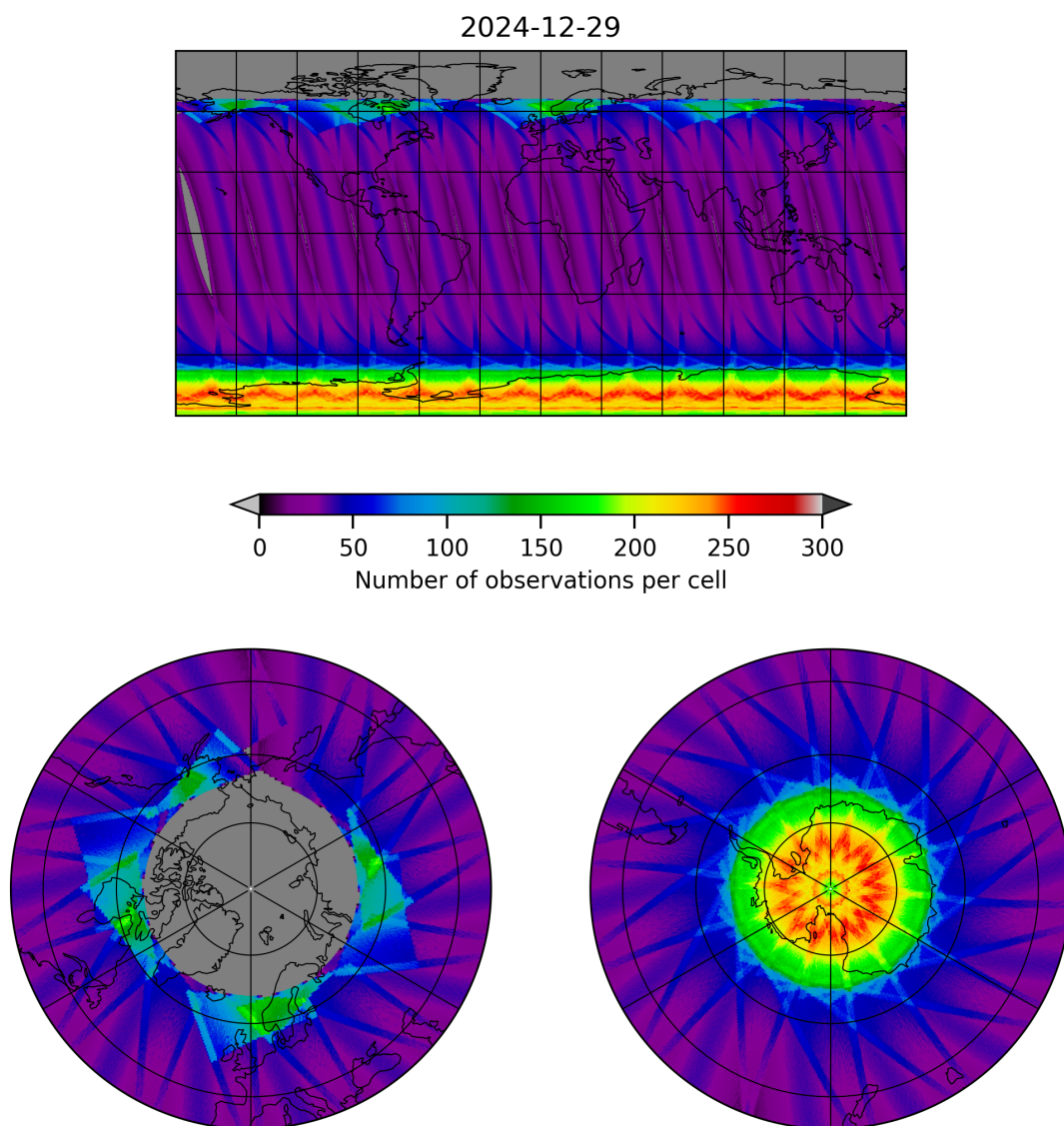
Figure 15: Map of the number of observations for 2024-12-29 to 2024-12-30
