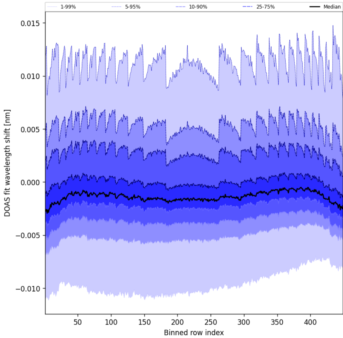
Figure 47: Along track statistics of “DOAS fit wavelength shift” for 2024-12-29 to 2024-12-30
