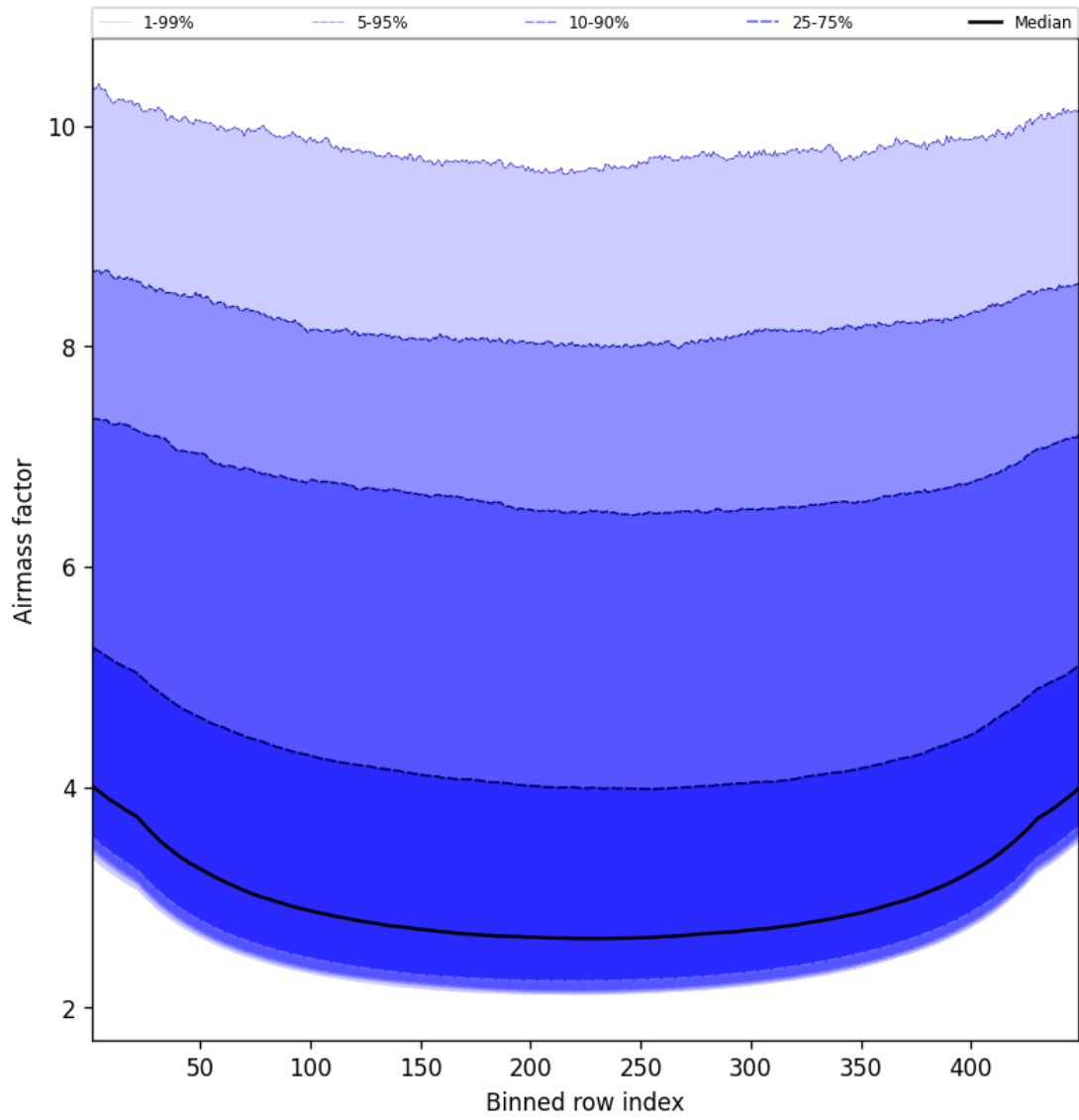
Figure 49: Along track statistics of “Airmass factor” for 2024-12-29 to 2024-12-30
