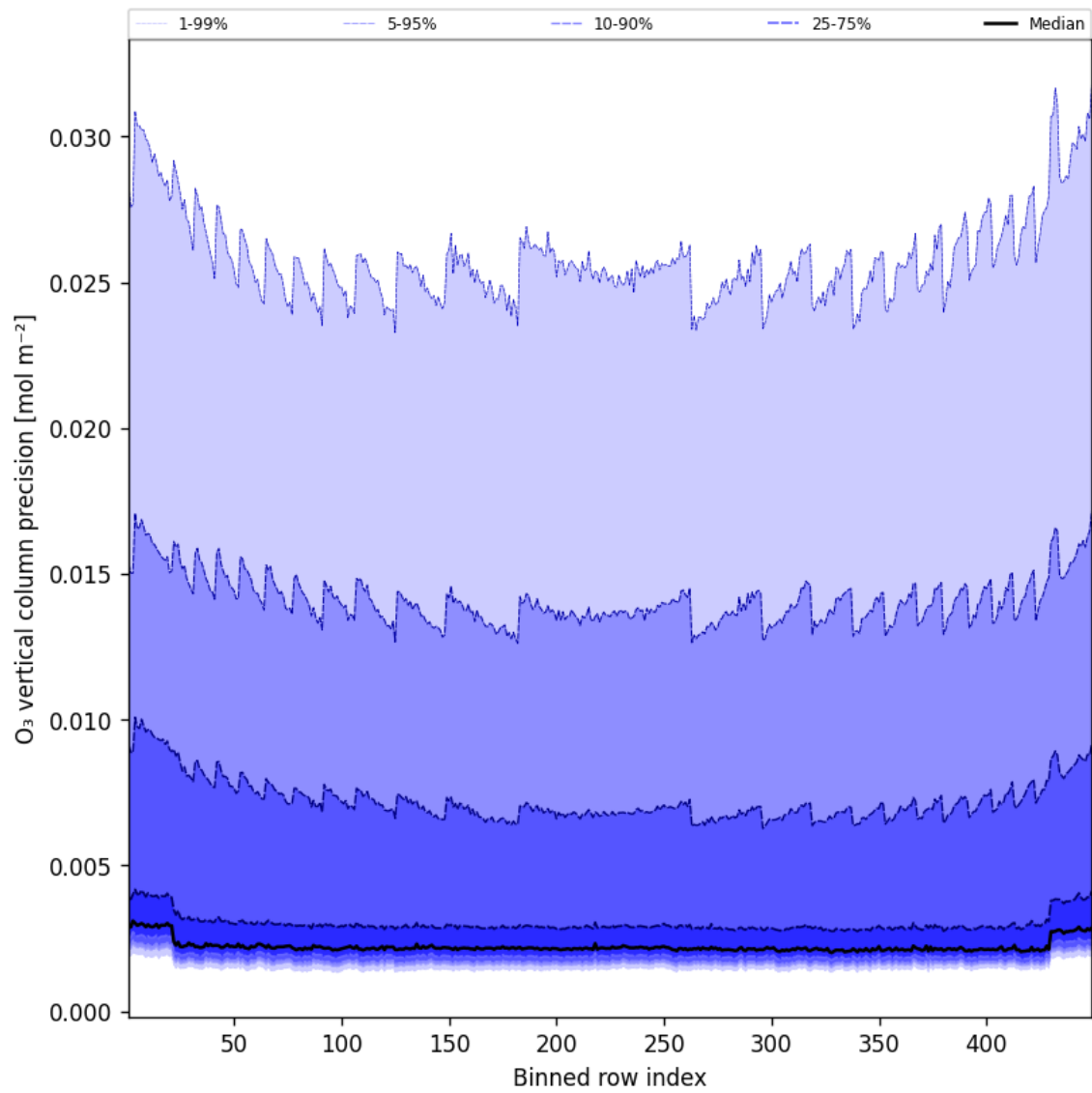
Figure 42: Along track statistics of “O 3 vertical column precision” for 2024-12-29 to 2024-12-30
