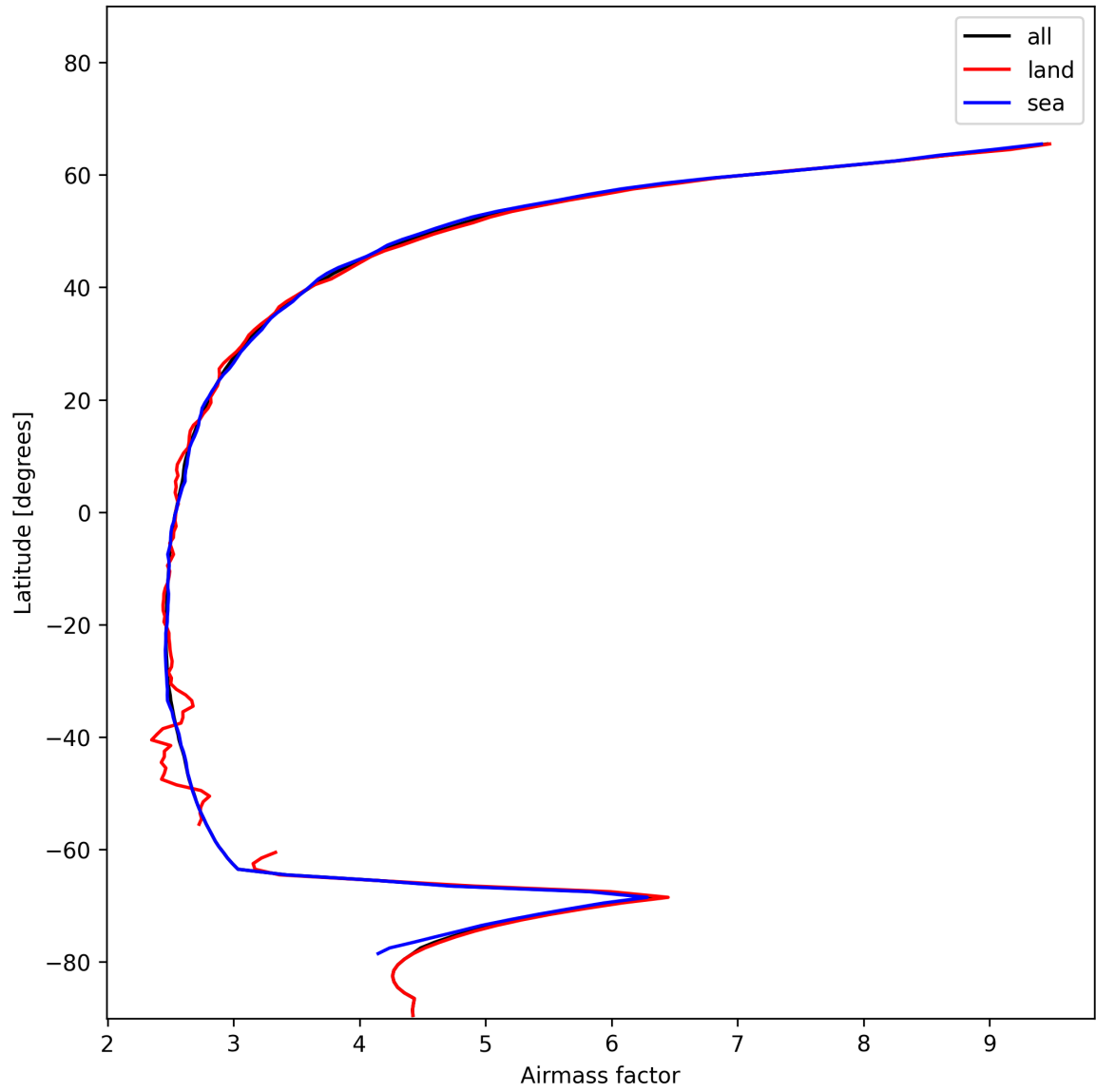
Figure 25: Zonal average of “Airmass factor” for 2024-12-29 to 2024-12-30.
