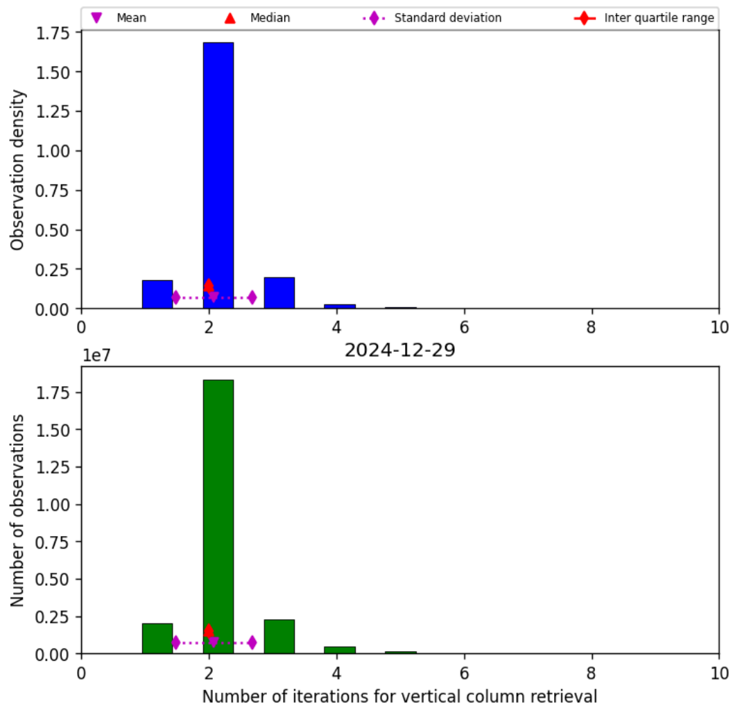
Figure 39: Histogram of “Number of iterations for vertical column retrieval” for 2024-12-29 to 2024-12-30
