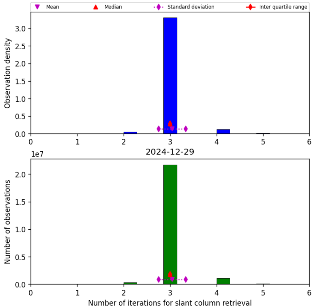
Figure 33: Histogram of “Number of iterations for slant column retrieval” for 2024-12-29 to 2024-12-30
