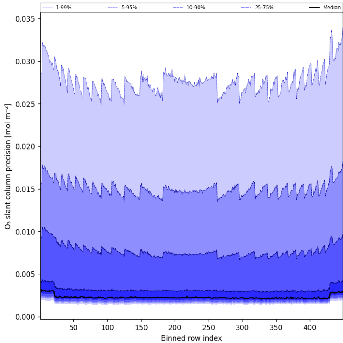
Figure 44: Along track statistics of “O 3 slant column precision” for 2024-12-29 to 2024-12-30
