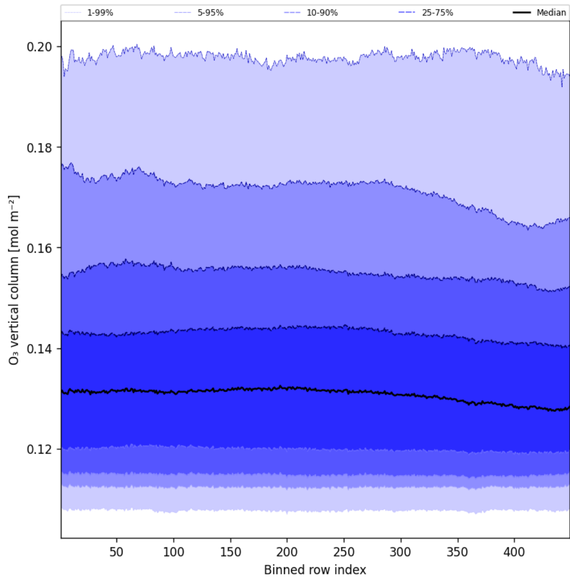
Figure 41: Along track statistics of “O 3 vertical column” for 2024-12-29 to 2024-12-30
