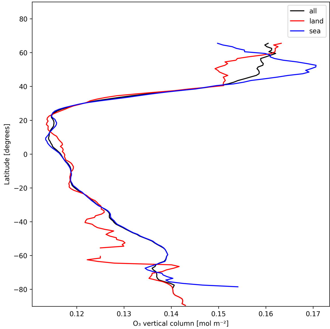
Figure 17: Zonal average of “O 3 vertical column” for 2024-12-29 to 2024-12-30.
