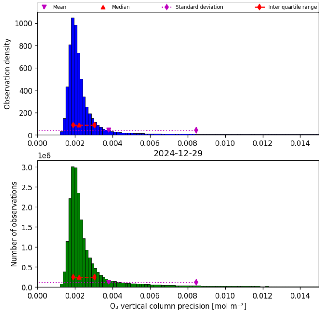
Figure 30: Histogram of “O 3 vertical column precision” for 2024-12-29 to 2024-12-30
