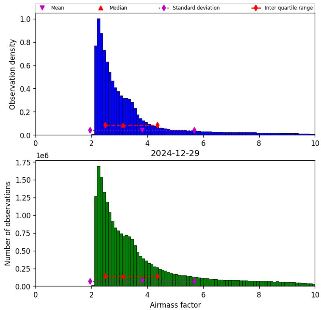
Figure 37: Histogram of “Airmass factor” for 2024-12-29 to 2024-12-30
