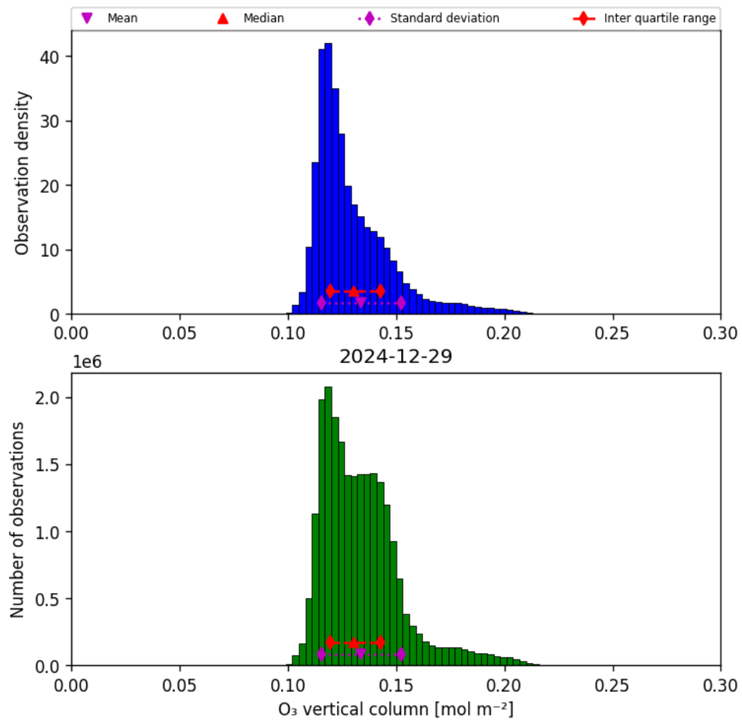
Figure 29: Histogram of “O 3 vertical column” for 2024-12-29 to 2024-12-30
