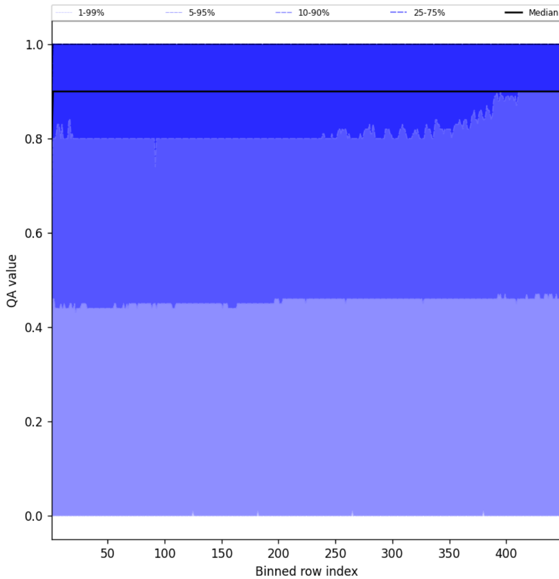
Figure 40: Along track statistics of “QA value” for 2024-12-29 to 2024-12-30
