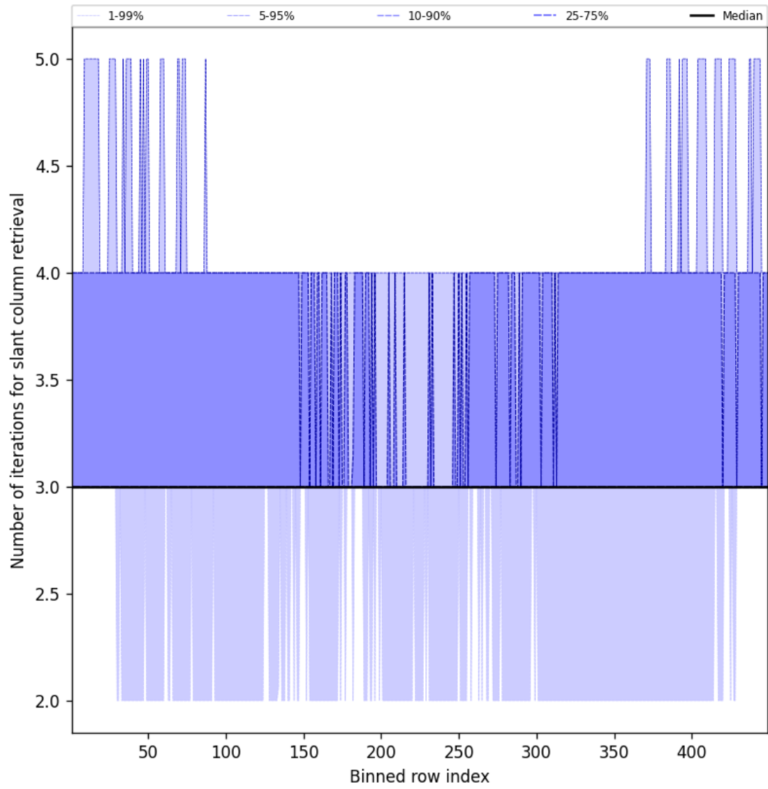
Figure 45: Along track statistics of “Number of iterations for slant column retrieval” for 2024-12-29 to 2024-12-30
