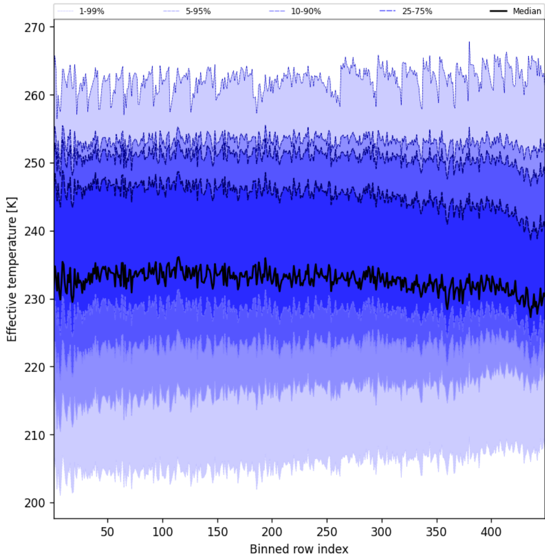
Figure 50: Along track statistics of “Effective temperature” for 2024-12-29 to 2024-12-30
