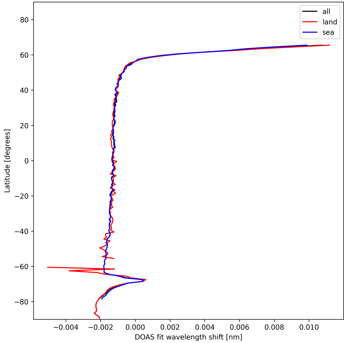
Figure 23: Zonal average of “DOAS fit wavelength shift” for 2024-12-29 to 2024-12-30.
