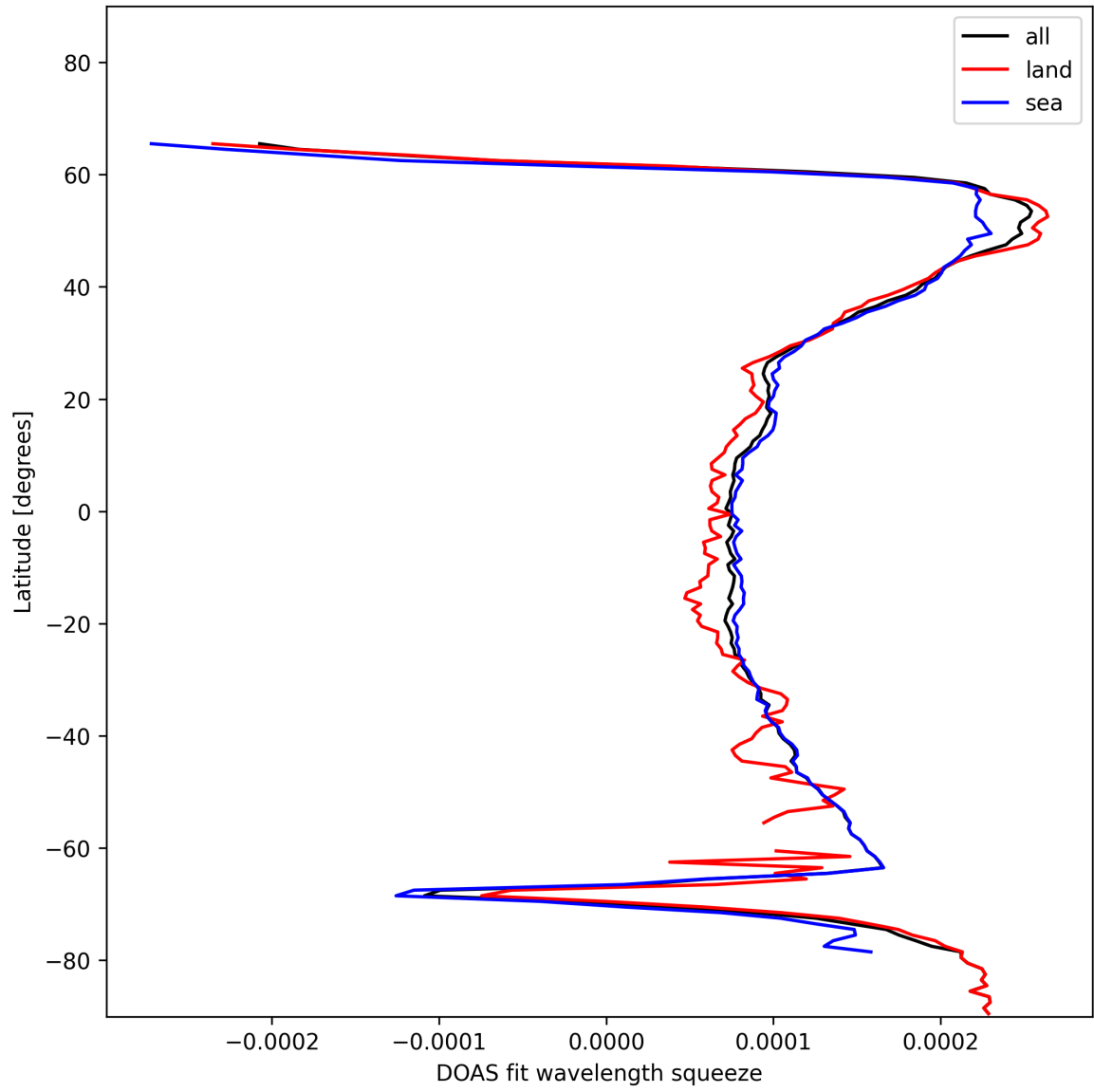
Figure 24: Zonal average of “DOAS fit wavelength squeeze” for 2024-12-29 to 2024-12-30.
