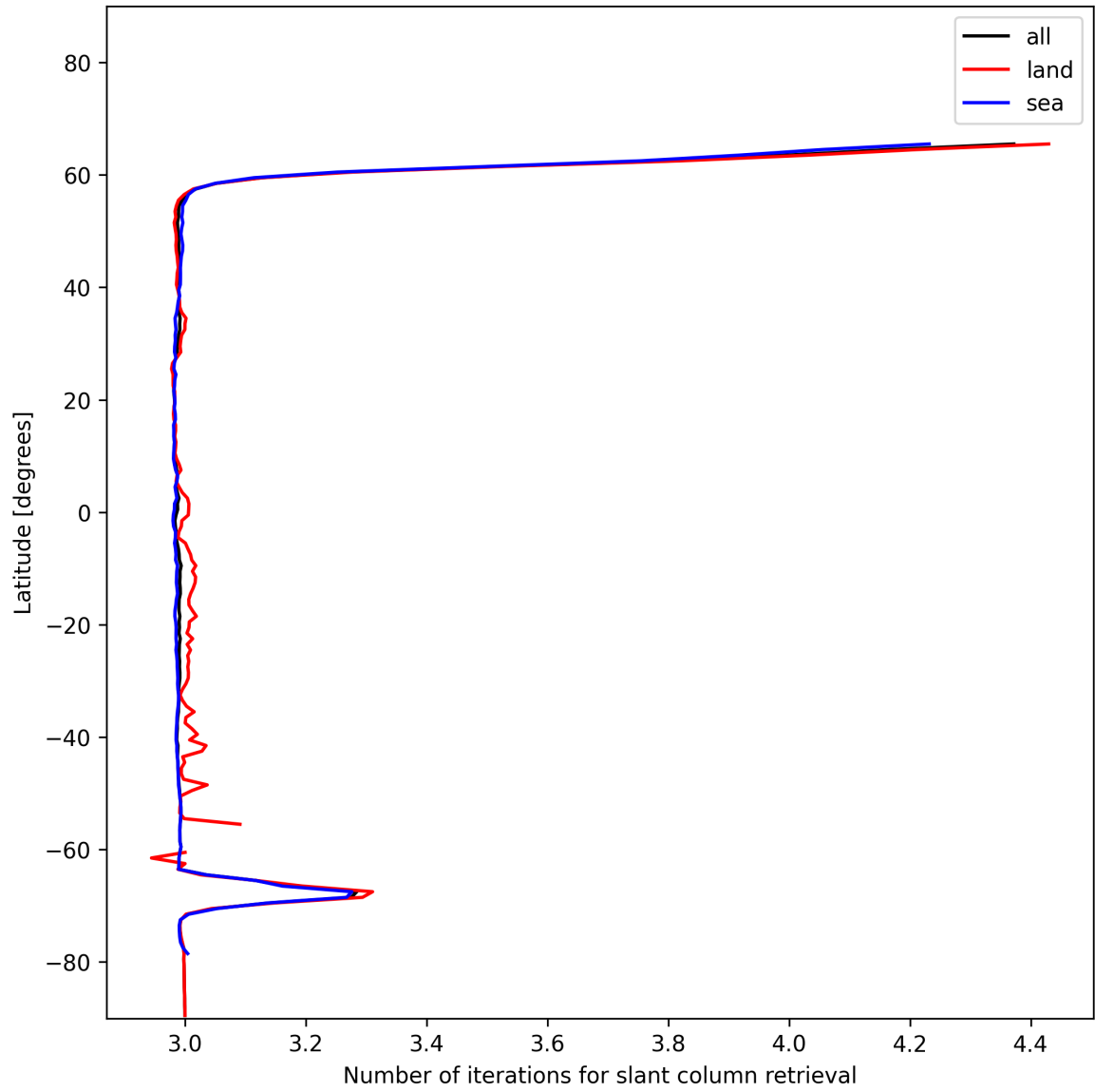
Figure 21: Zonal average of “Number of iterations for slant column retrieval” for 2024-12-29 to 2024-12-30.
