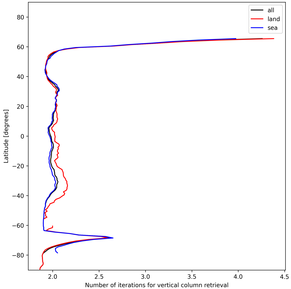
Figure 27: Zonal average of “Number of iterations for vertical column retrieval” for 2024-12-29 to 2024-12-30.
