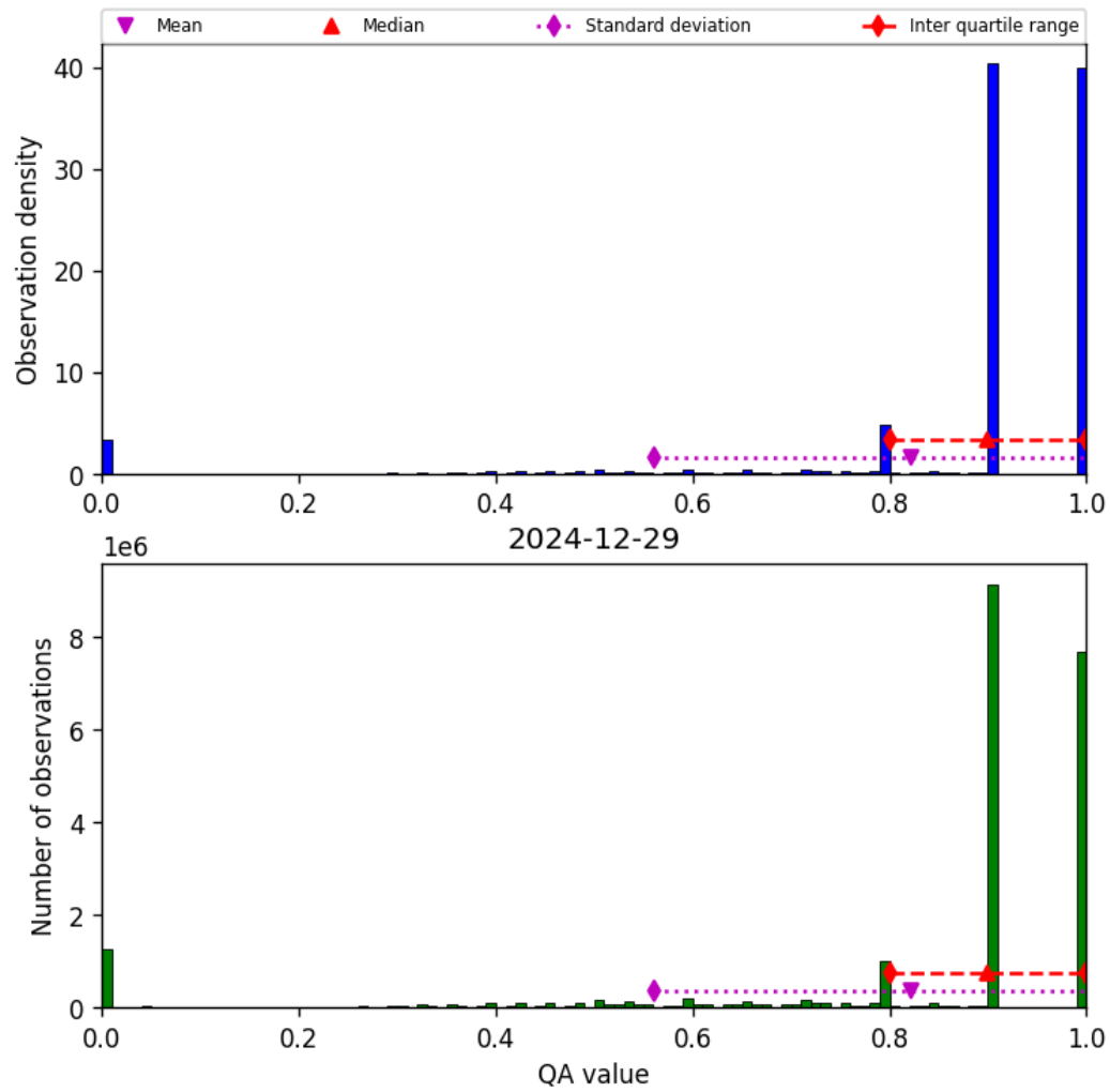
Figure 28: Histogram of “QA value” for 2024-12-29 to 2024-12-30
