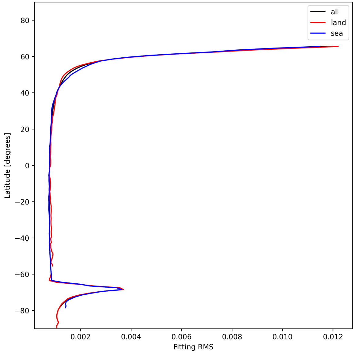
Figure 22: Zonal average of “Fitting RMS” for 2024-12-29 to 2024-12-30.
