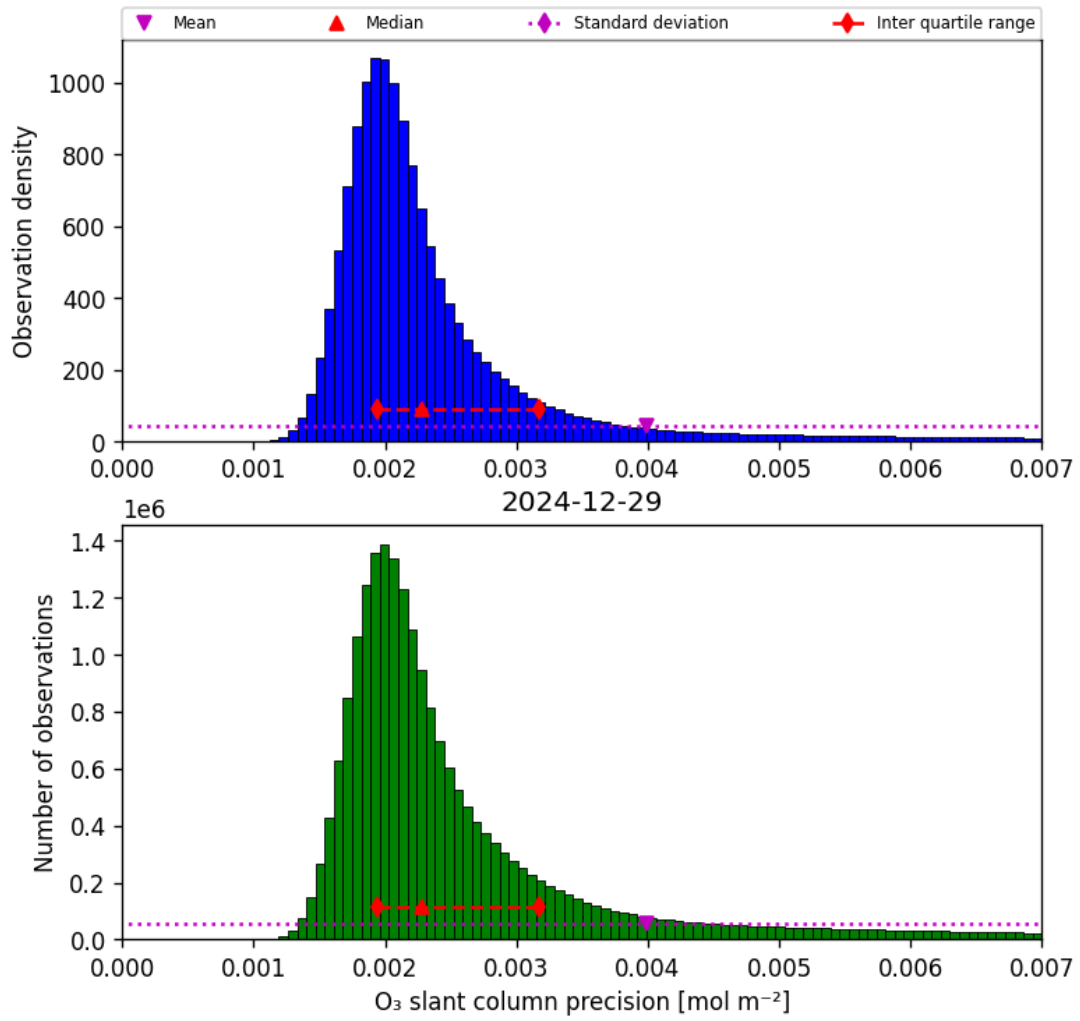
Figure 32: Histogram of “O 3 slant column precision” for 2024-12-29 to 2024-12-30
