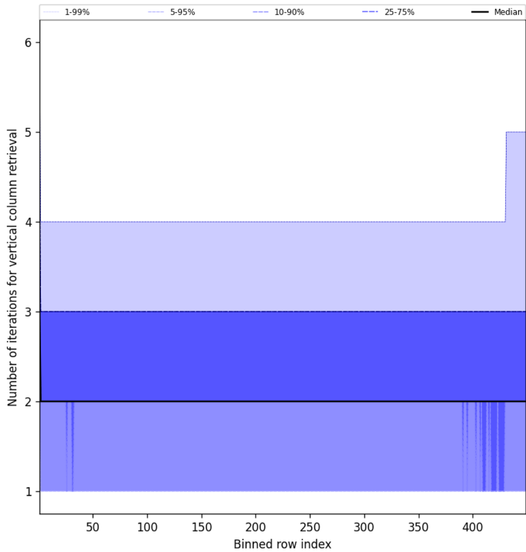
Figure 51: Along track statistics of “Number of iterations for vertical column retrieval” for 2024-12-29 to 2024-12-30
