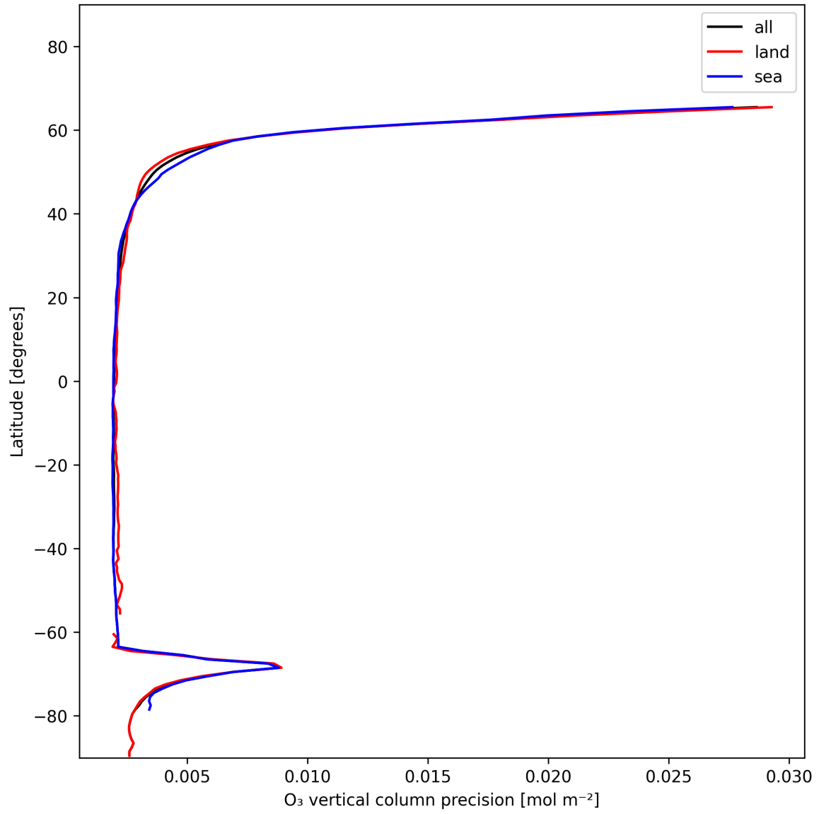
Figure 18: Zonal average of “O 3 vertical column precision” for 2024-12-29 to 2024-12-30.
