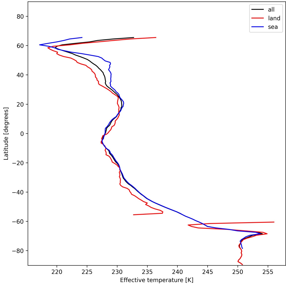
Figure 26: Zonal average of “Effective temperature” for 2024-12-29 to 2024-12-30.
