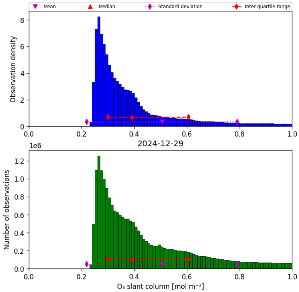
Figure 31: Histogram of “O 3 slant column” for 2024-12-29 to 2024-12-30
