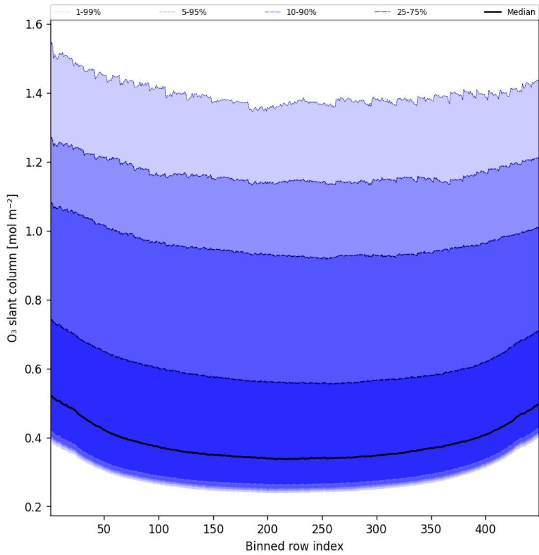
Figure 43: Along track statistics of “O 3 slant column” for 2024-12-29 to 2024-12-30
