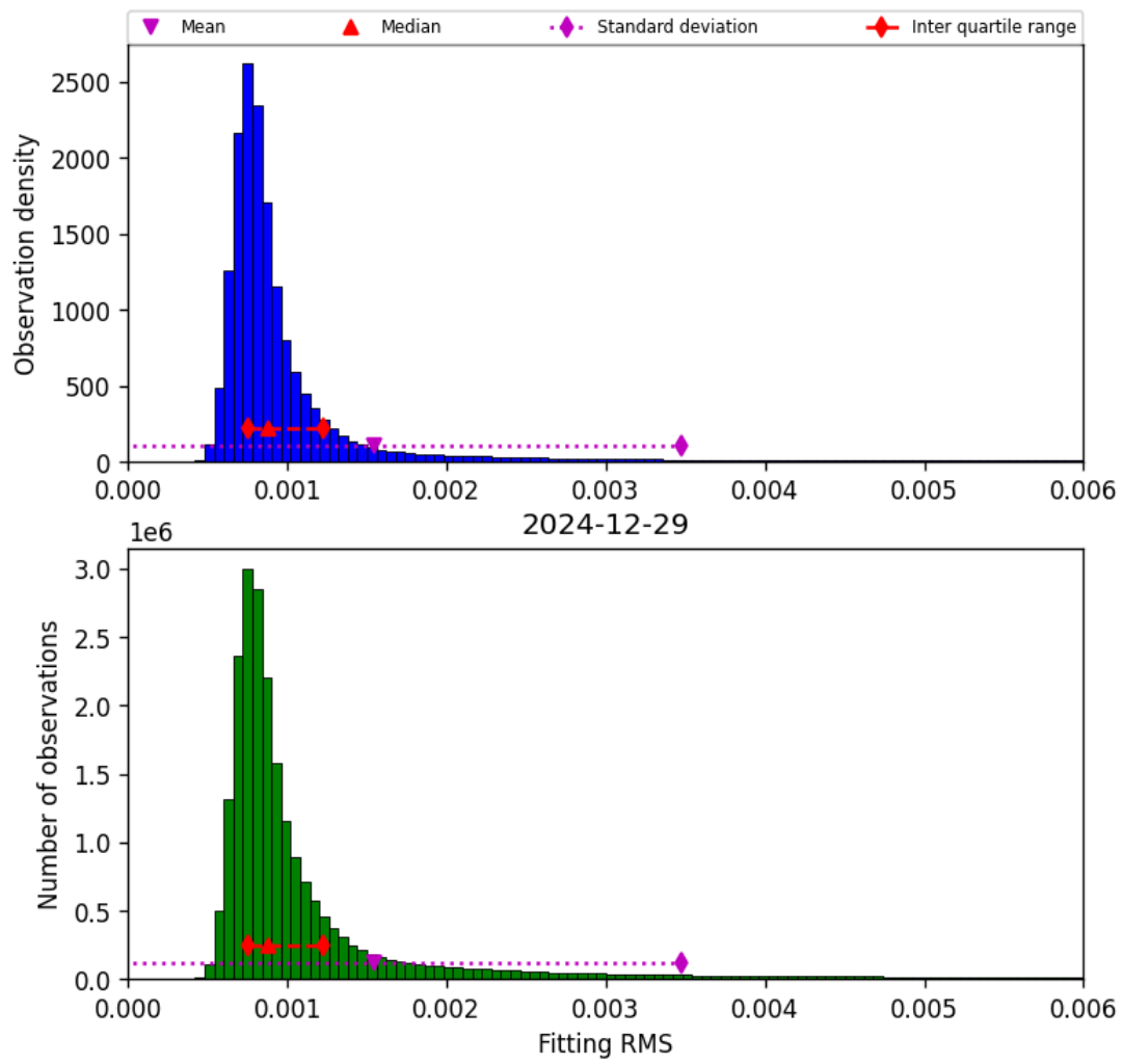
Figure 34: Histogram of “Fitting RMS” for 2024-12-29 to 2024-12-30
