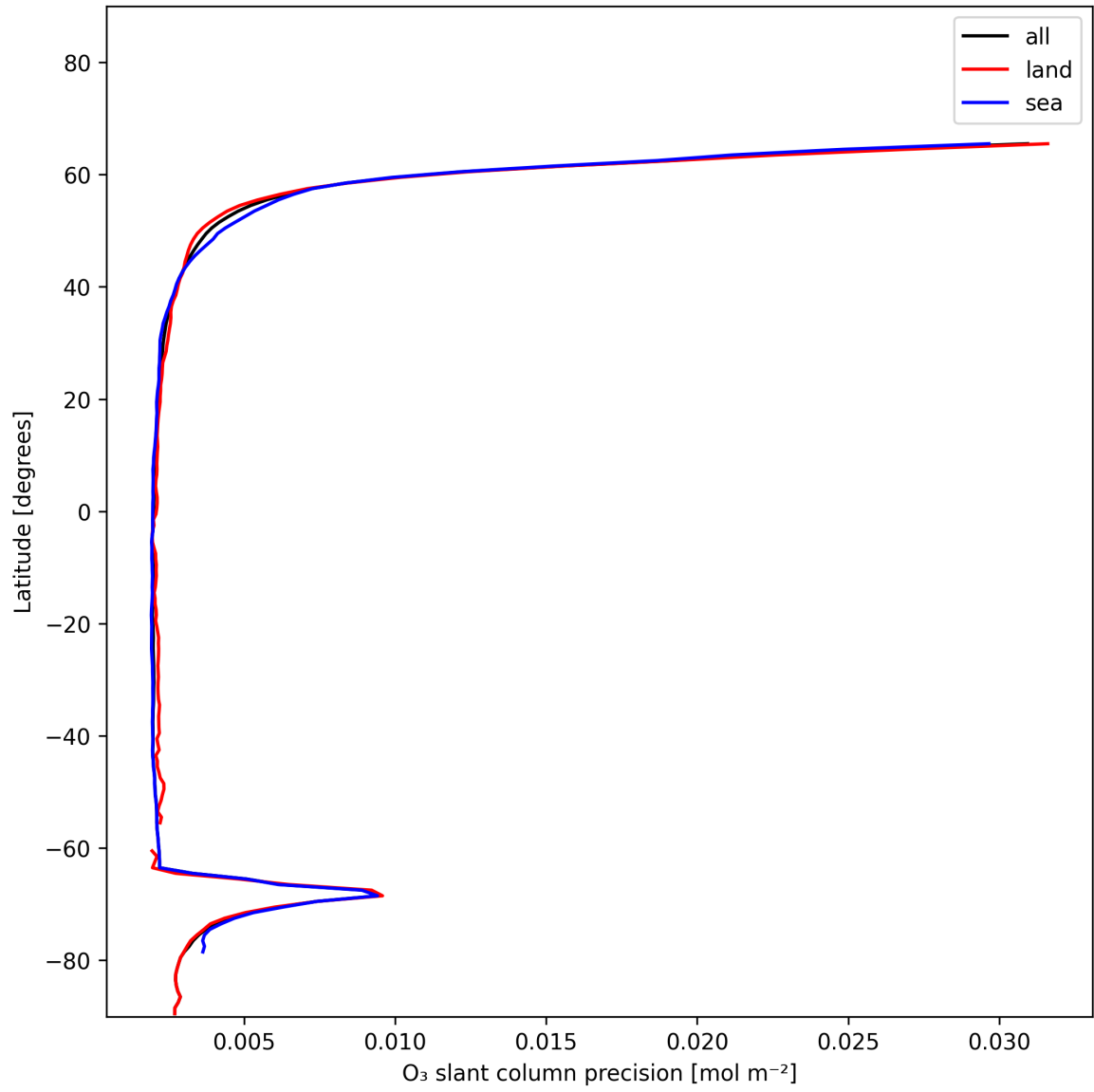
Figure 20: Zonal average of “O 3 slant column precision” for 2024-12-29 to 2024-12-30.
