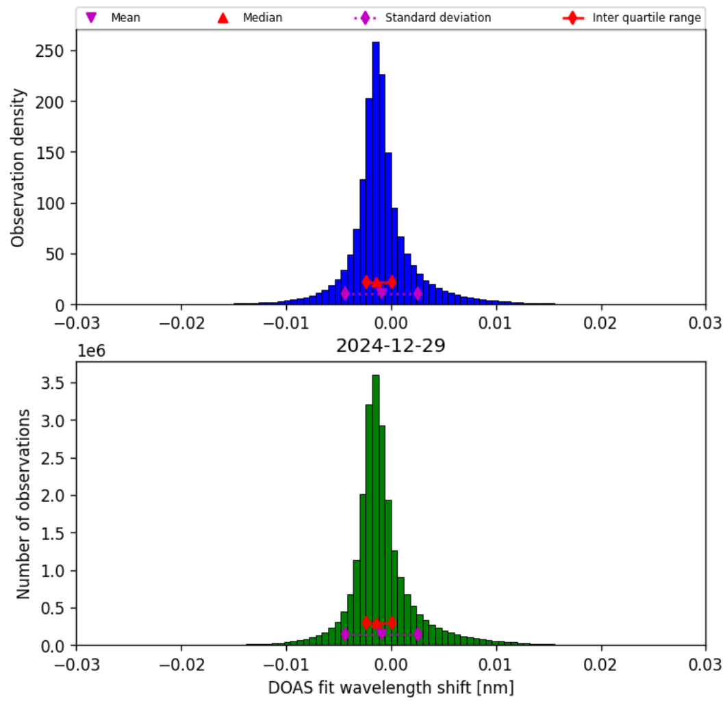
Figure 35: Histogram of “DOAS fit wavelength shift” for 2024-12-29 to 2024-12-30
