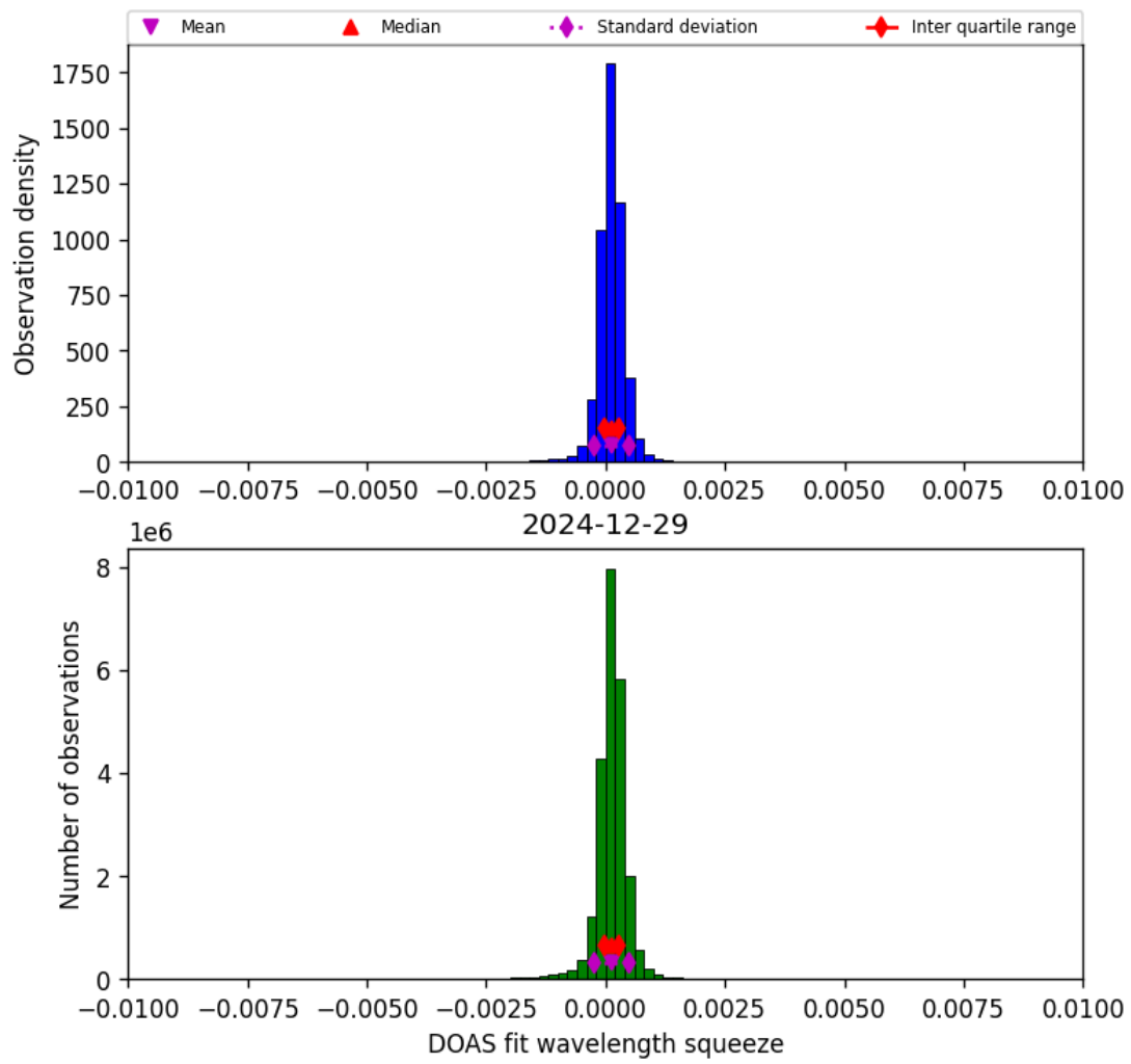
Figure 36: Histogram of “DOAS fit wavelength squeeze” for 2024-12-29 to 2024-12-30
