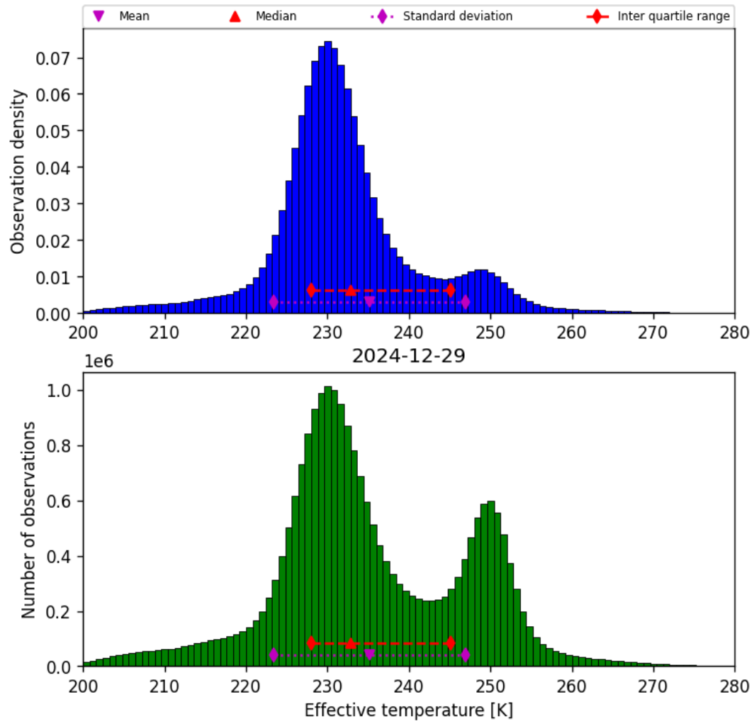
Figure 38: Histogram of “Effective temperature” for 2024-12-29 to 2024-12-30
