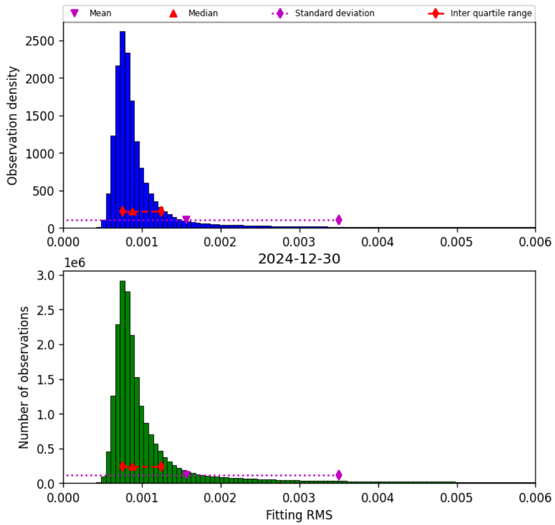
Figure 34: Histogram of “Fitting RMS” for 2024-12-30 to 2024-12-30
