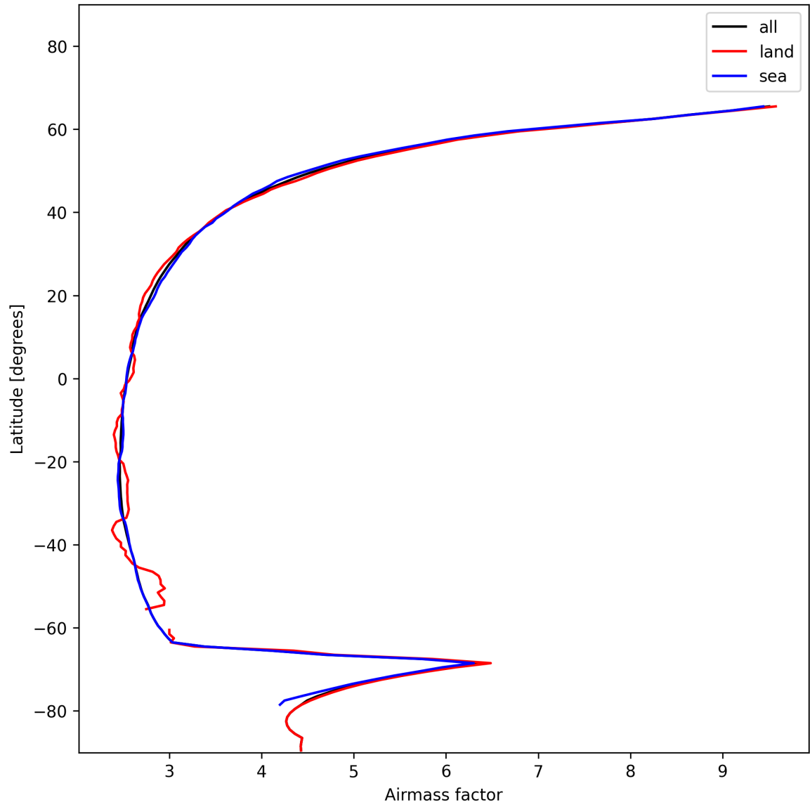
Figure 25: Zonal average of “Airmass factor” for 2024-12-30 to 2024-12-30.
