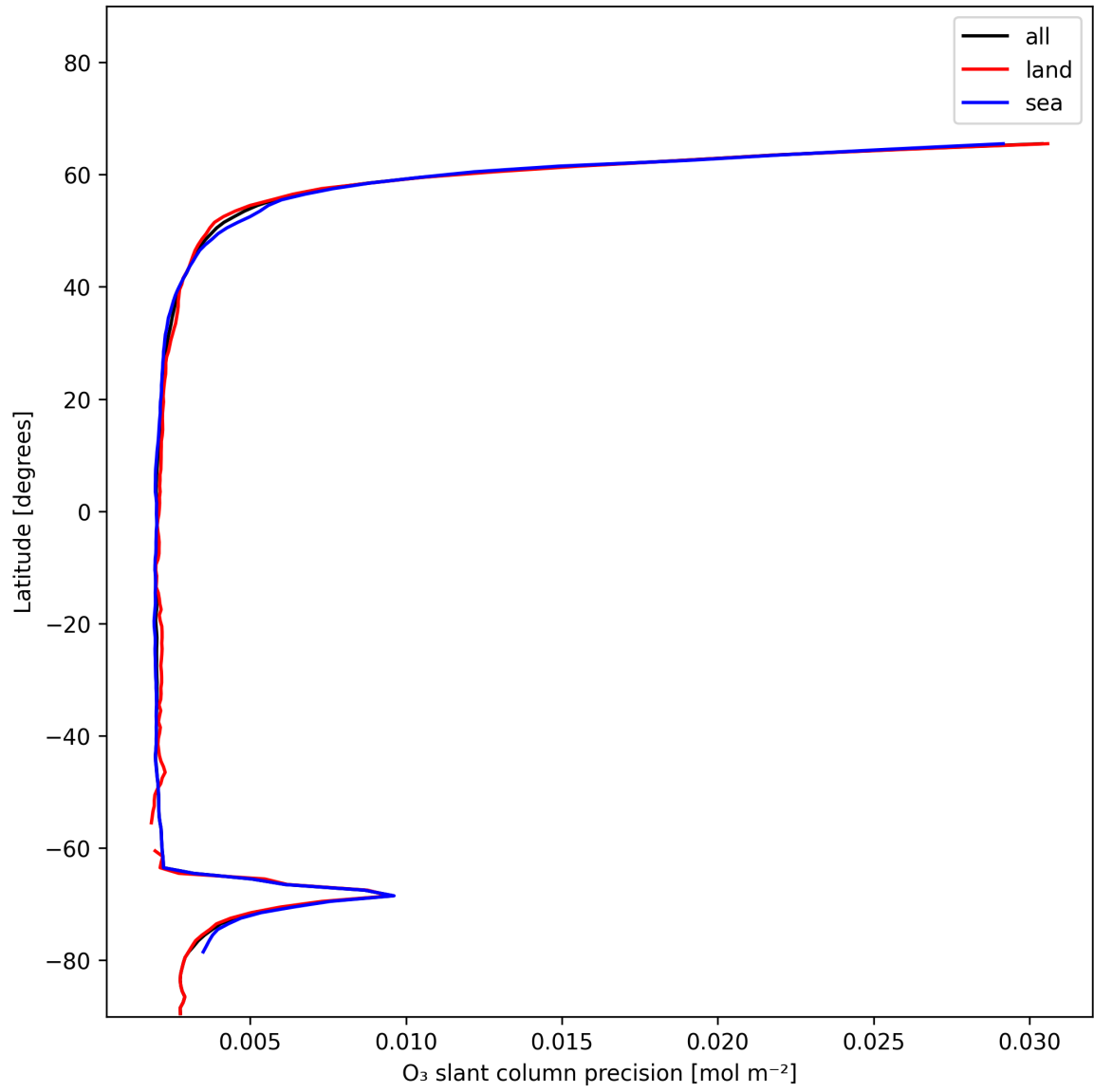
Figure 20: Zonal average of “O 3 slant column precision” for 2024-12-30 to 2024-12-30.
