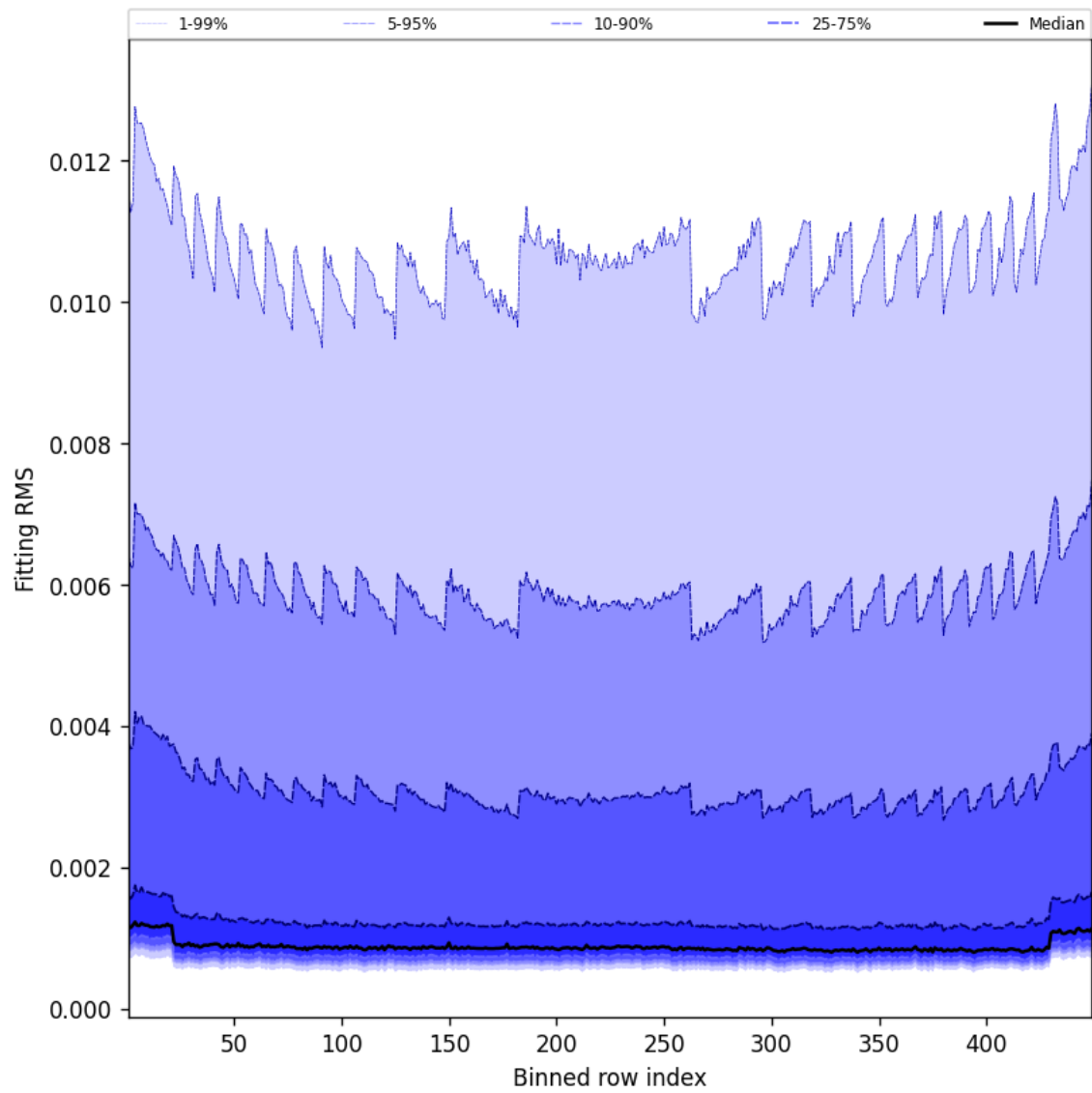
Figure 46: Along track statistics of “Fitting RMS” for 2024-12-30 to 2024-12-30
