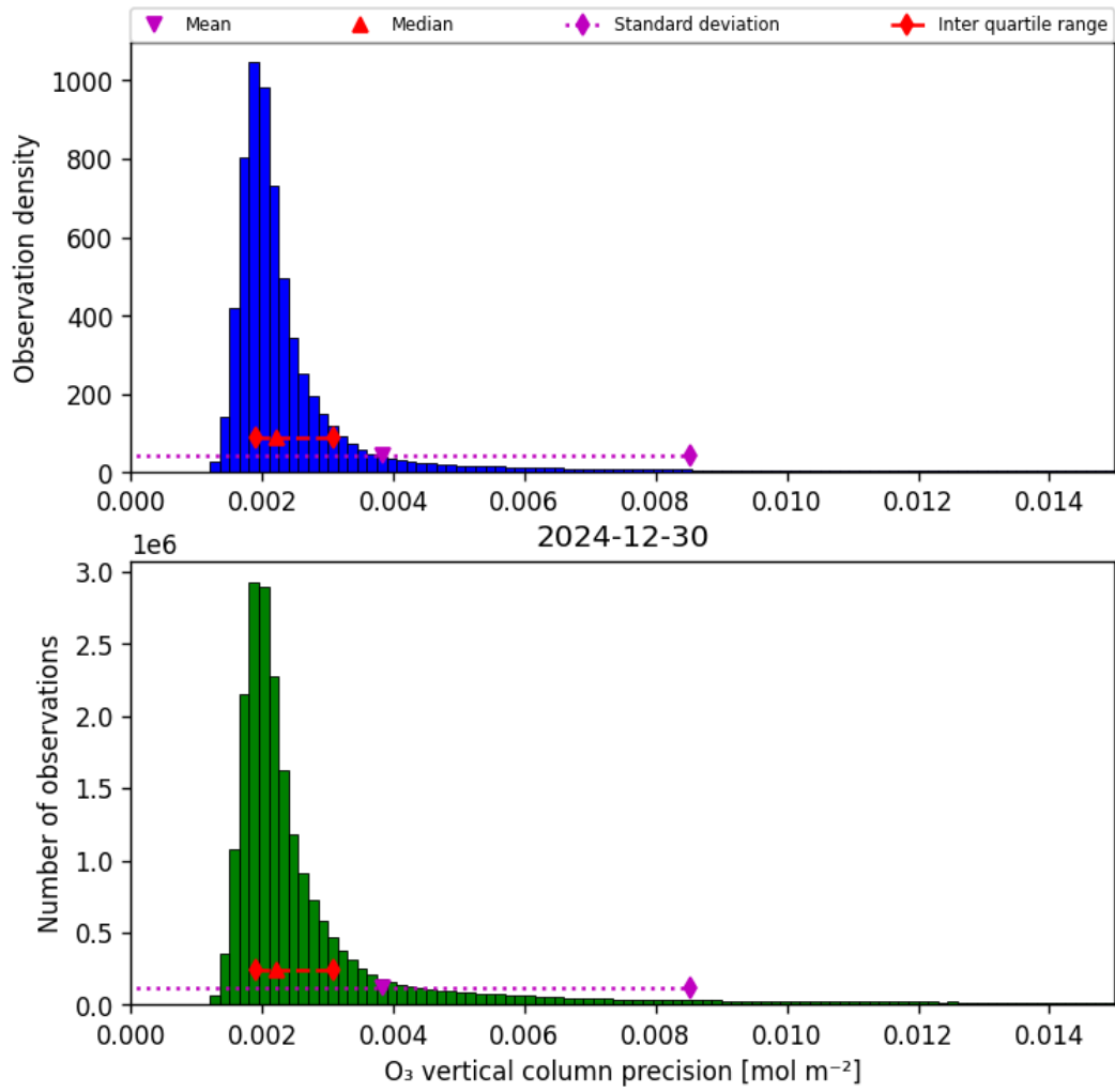
Figure 30: Histogram of “O 3 vertical column precision” for 2024-12-30 to 2024-12-30
