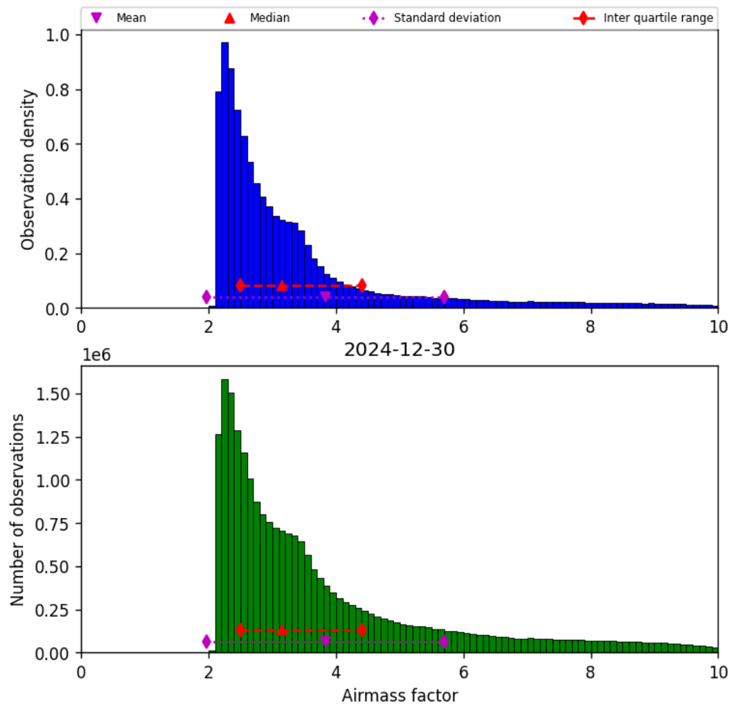
Figure 37: Histogram of “Airmass factor” for 2024-12-30 to 2024-12-30
