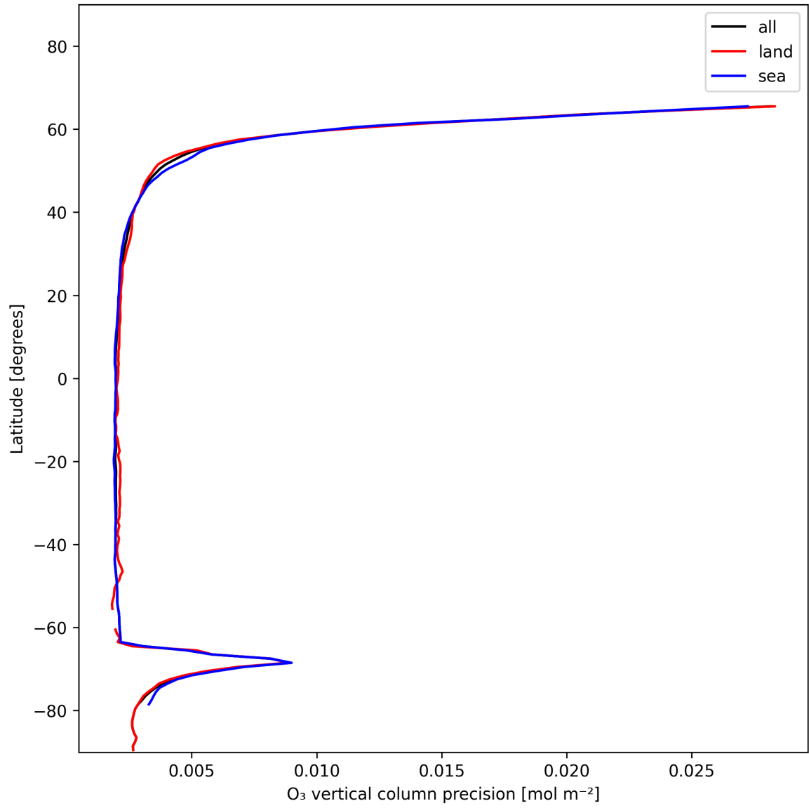
Figure 18: Zonal average of “O 3 vertical column precision” for 2024-12-30 to 2024-12-30.
