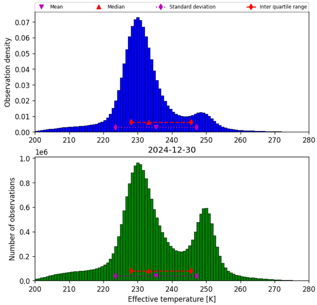
Figure 38: Histogram of “Effective temperature” for 2024-12-30 to 2024-12-30
