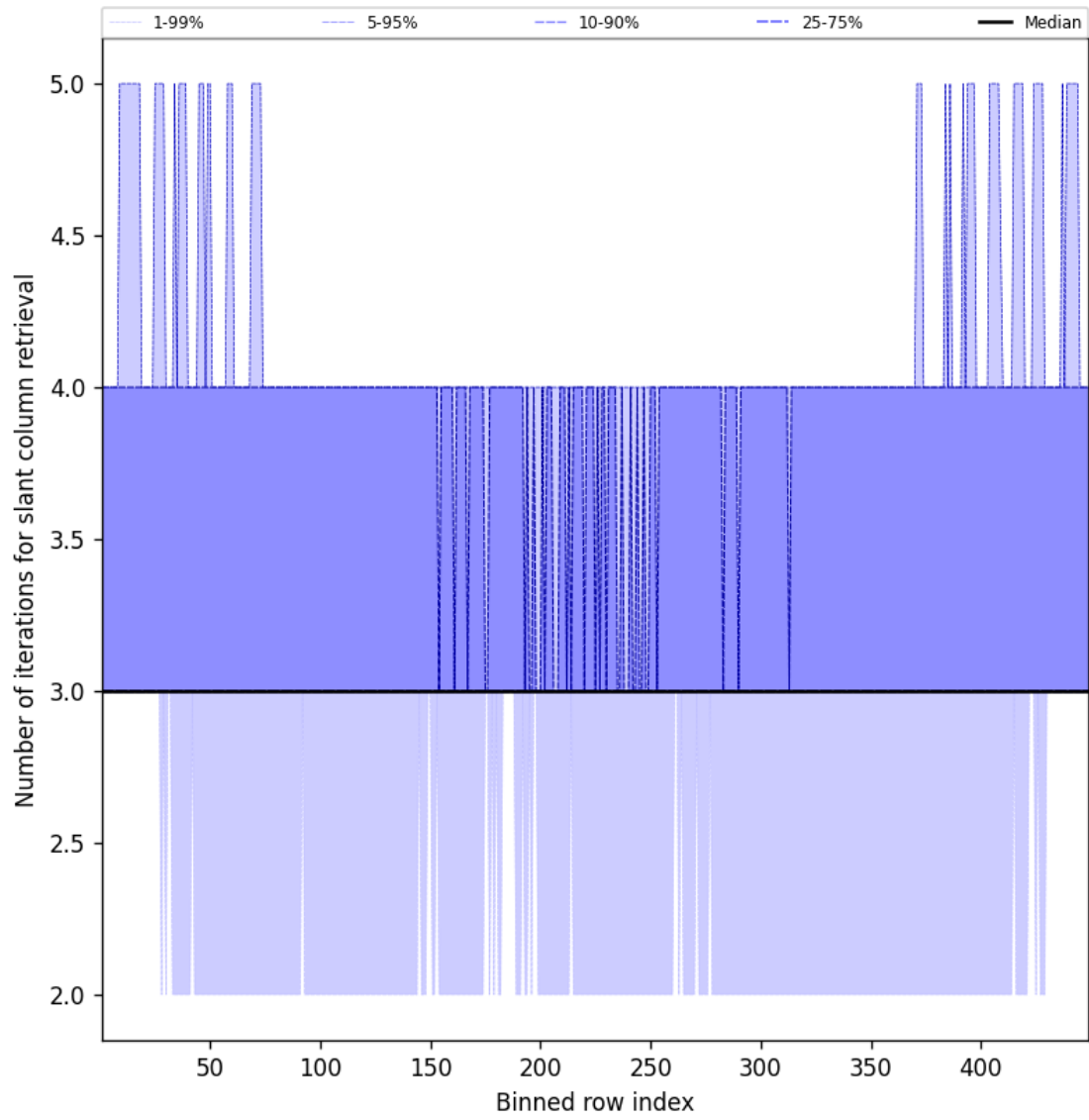
Figure 45: Along track statistics of “Number of iterations for slant column retrieval” for 2024-12-30 to 2024-12-30
