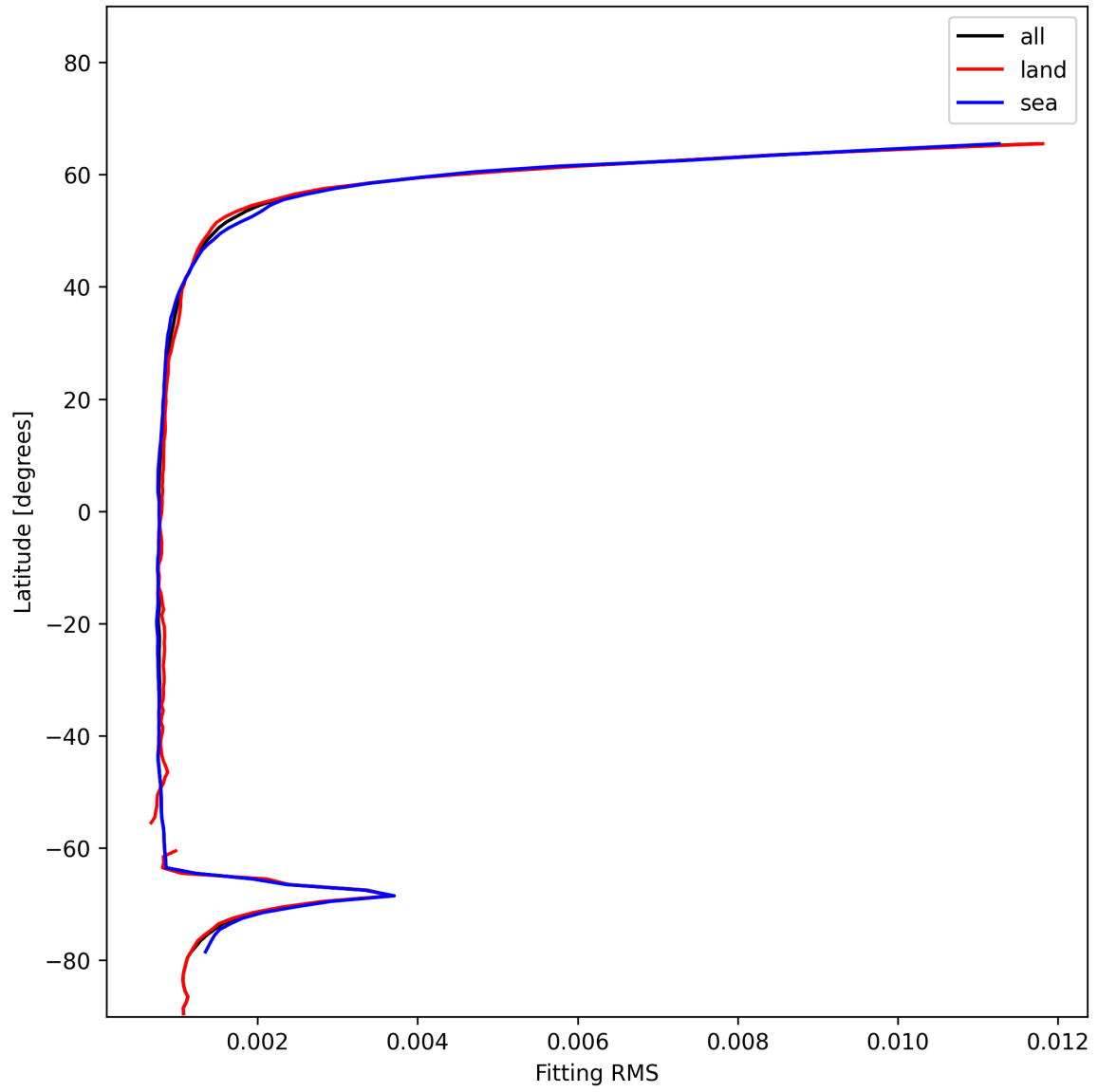
Figure 22: Zonal average of “Fitting RMS” for 2024-12-30 to 2024-12-30.
