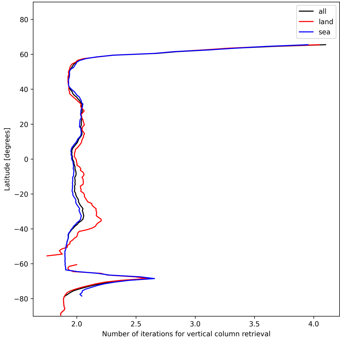
Figure 27: Zonal average of “Number of iterations for vertical column retrieval” for 2024-12-30 to 2024-12-30.
