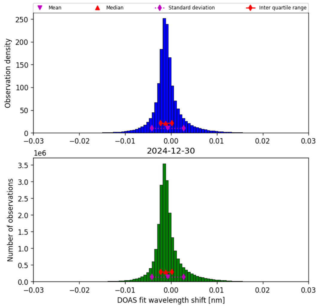
Figure 35: Histogram of “DOAS fit wavelength shift” for 2024-12-30 to 2024-12-30
