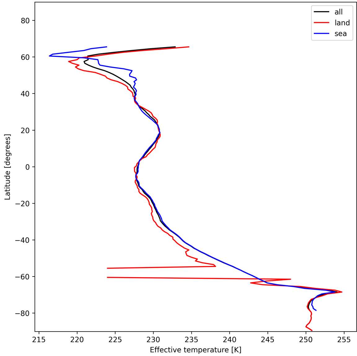
Figure 26: Zonal average of “Effective temperature” for 2024-12-30 to 2024-12-30.
