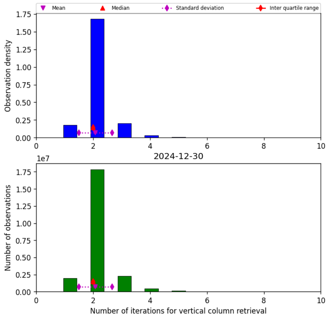
Figure 39: Histogram of “Number of iterations for vertical column retrieval” for 2024-12-30 to 2024-12-30
