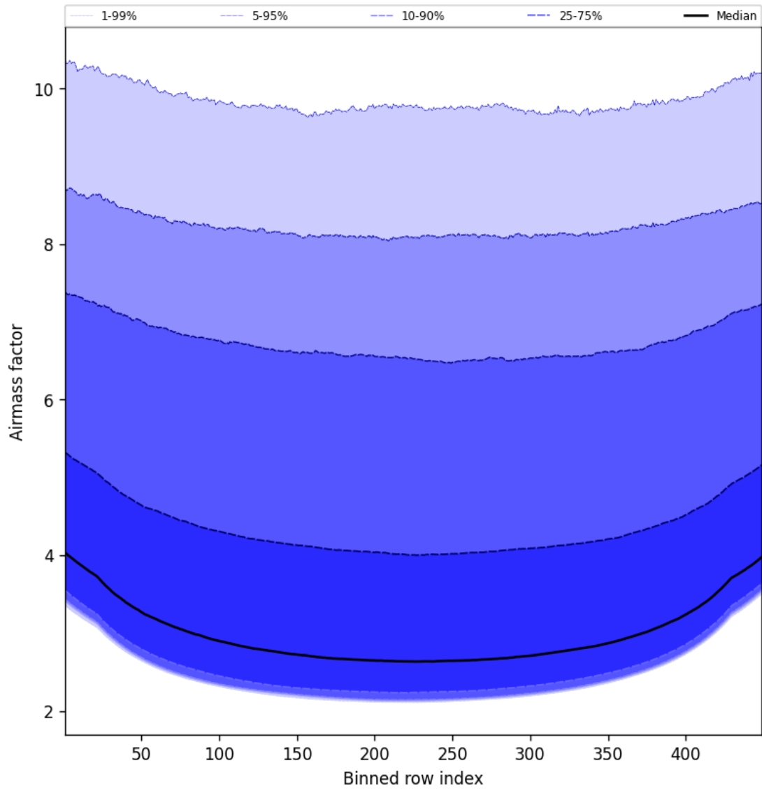
Figure 49: Along track statistics of “Airmass factor” for 2024-12-30 to 2024-12-30
