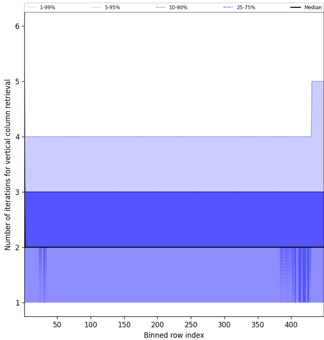
Figure 51: Along track statistics of “Number of iterations for vertical column retrieval” for 2024-12-30 to 2024-12-30
