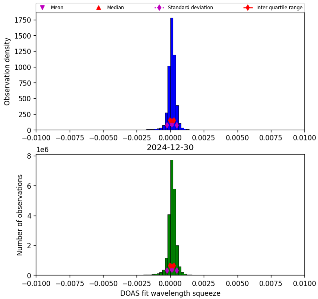
Figure 36: Histogram of “DOAS fit wavelength squeeze” for 2024-12-30 to 2024-12-30
