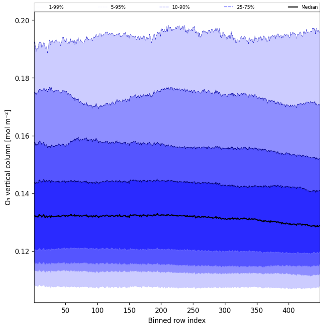
Figure 41: Along track statistics of “O 3 vertical column” for 2024-12-30 to 2024-12-30
