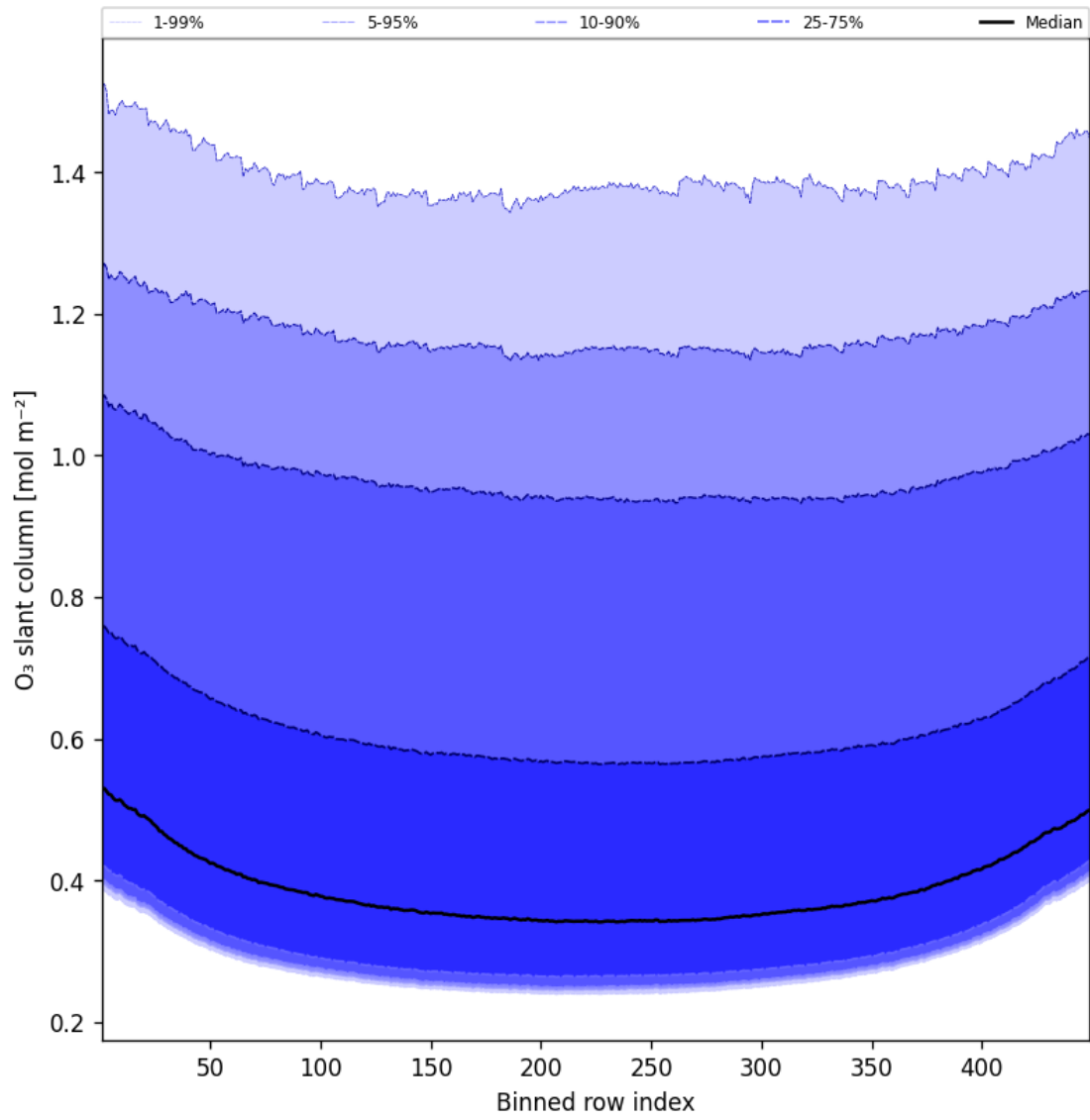
Figure 43: Along track statistics of “O 3 slant column” for 2024-12-30 to 2024-12-30
