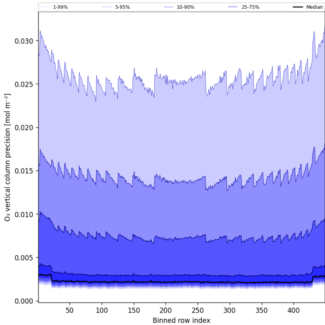
Figure 42: Along track statistics of “O 3 vertical column precision” for 2024-12-30 to 2024-12-30
