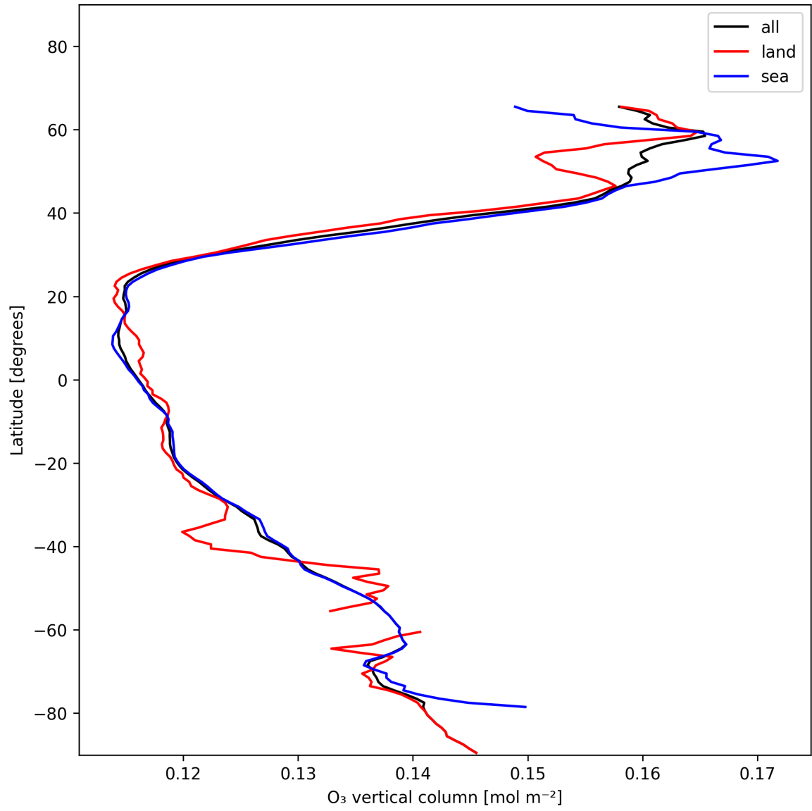
Figure 17: Zonal average of “O 3 vertical column” for 2024-12-30 to 2024-12-30.
