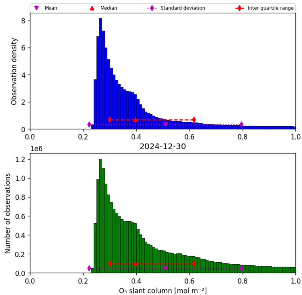
Figure 31: Histogram of "O 3 slant column" for 2024-12-30 to 2024-12-30
