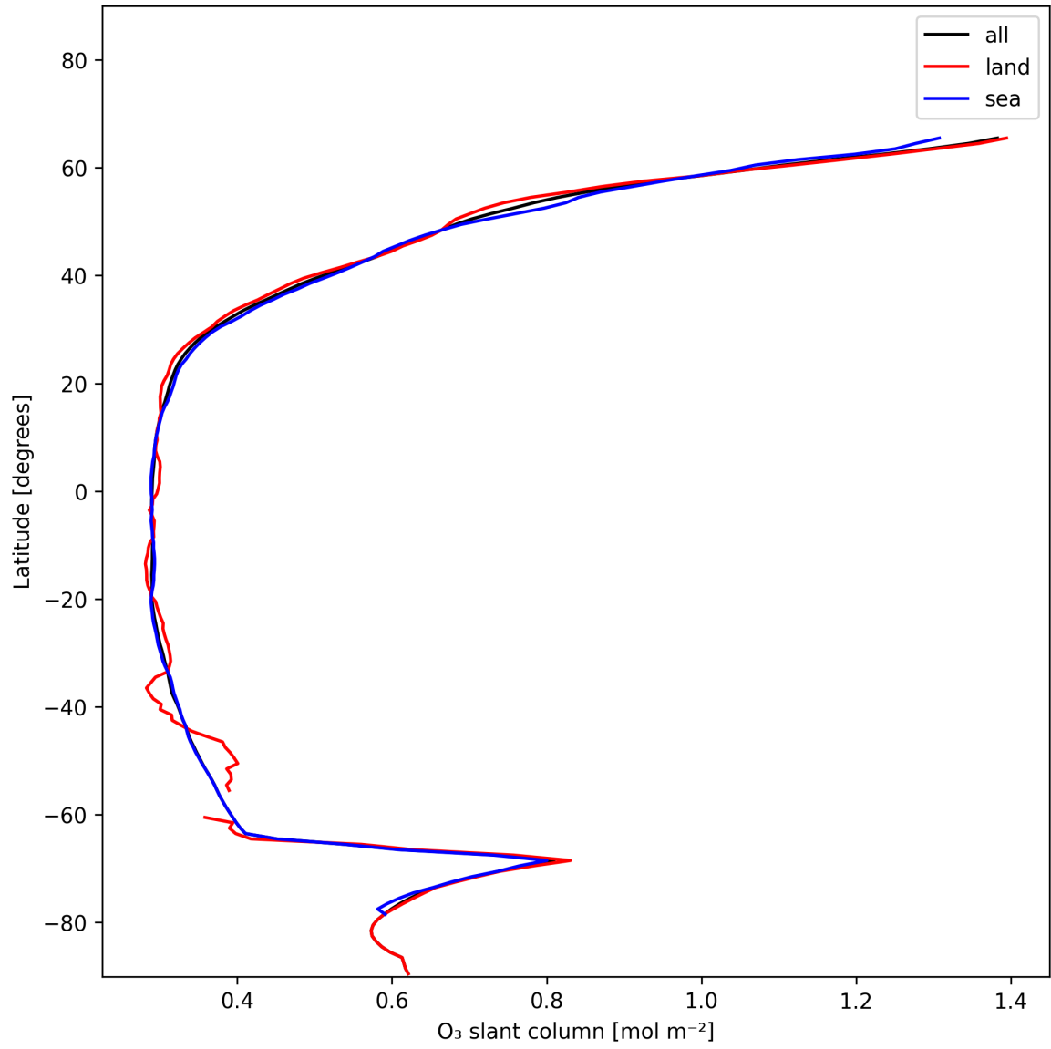
Figure 19: Zonal average of “O 3 slant column” for 2024-12-30 to 2024-12-30.
