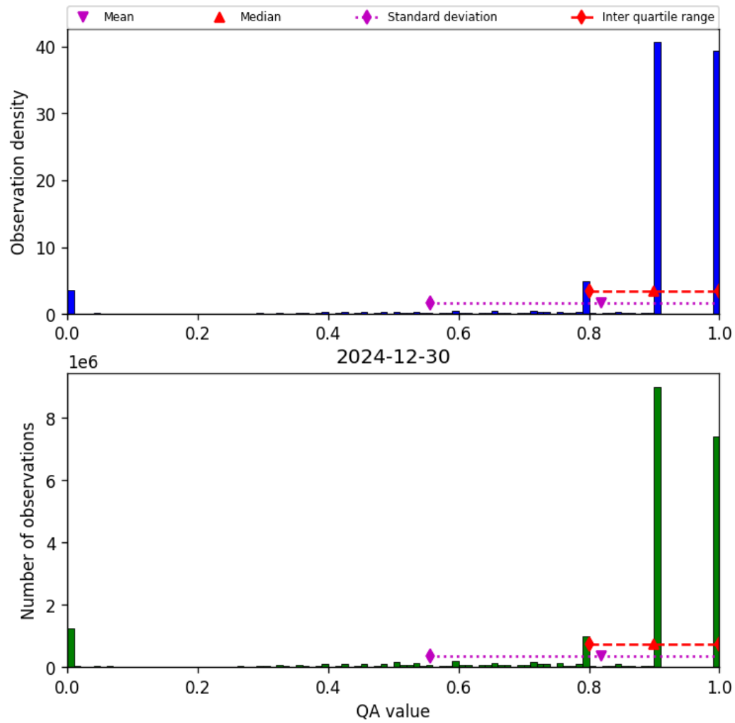
Figure 28: Histogram of “QA value” for 2024-12-30 to 2024-12-30
