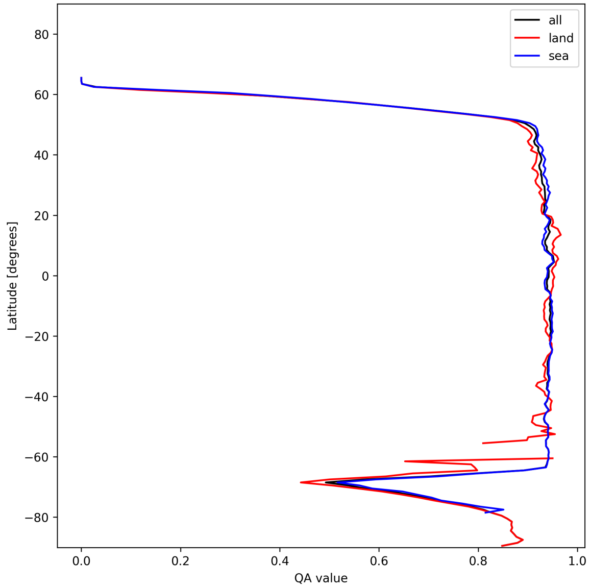
Figure 16: Zonal average of “QA value” for 2024-12-30 to 2024-12-30.
