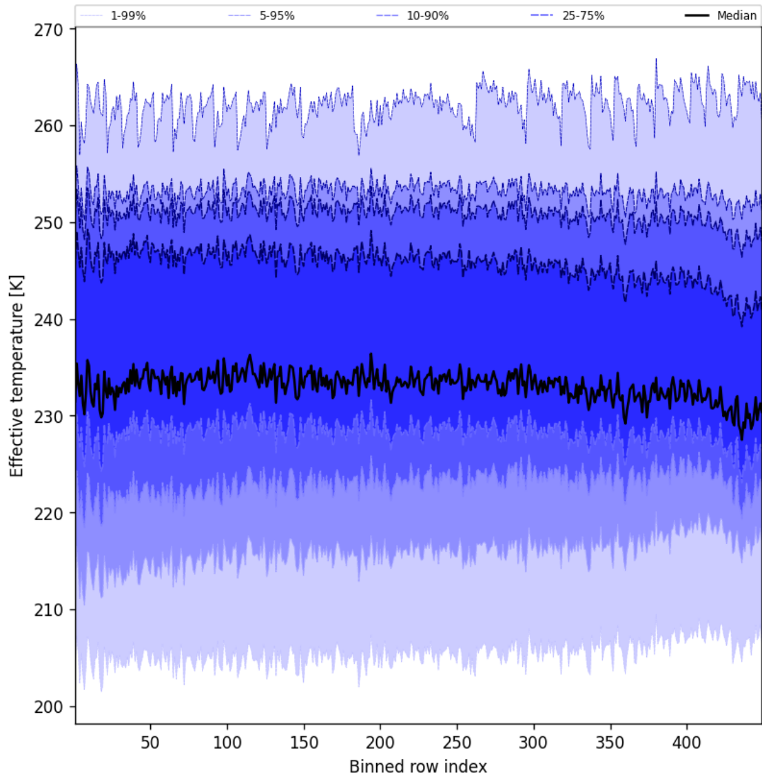
Figure 50: Along track statistics of “Effective temperature” for 2024-12-30 to 2024-12-30
