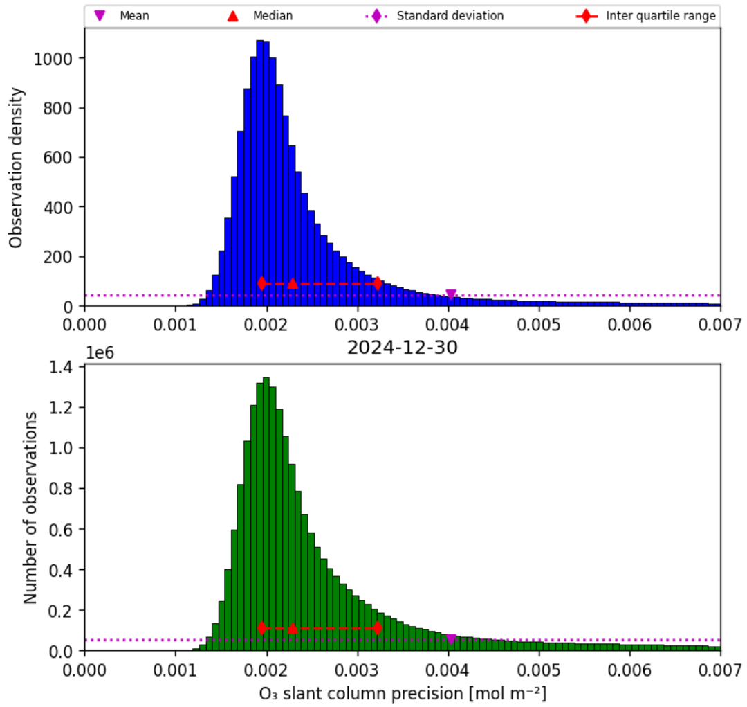
Figure 32: Histogram of “O 3 slant column precision” for 2024-12-30 to 2024-12-30
