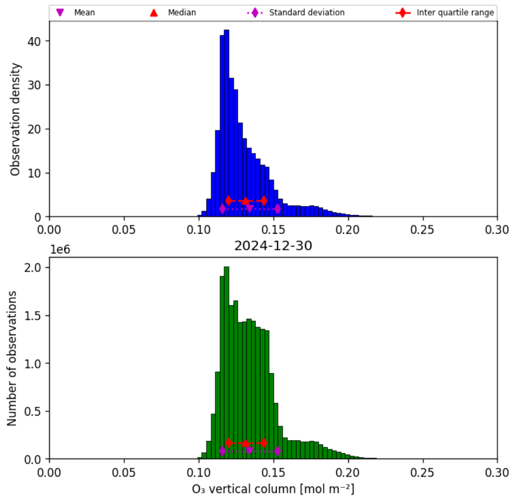
Figure 29: Histogram of “O 3 vertical column” for 2024-12-30 to 2024-12-30
