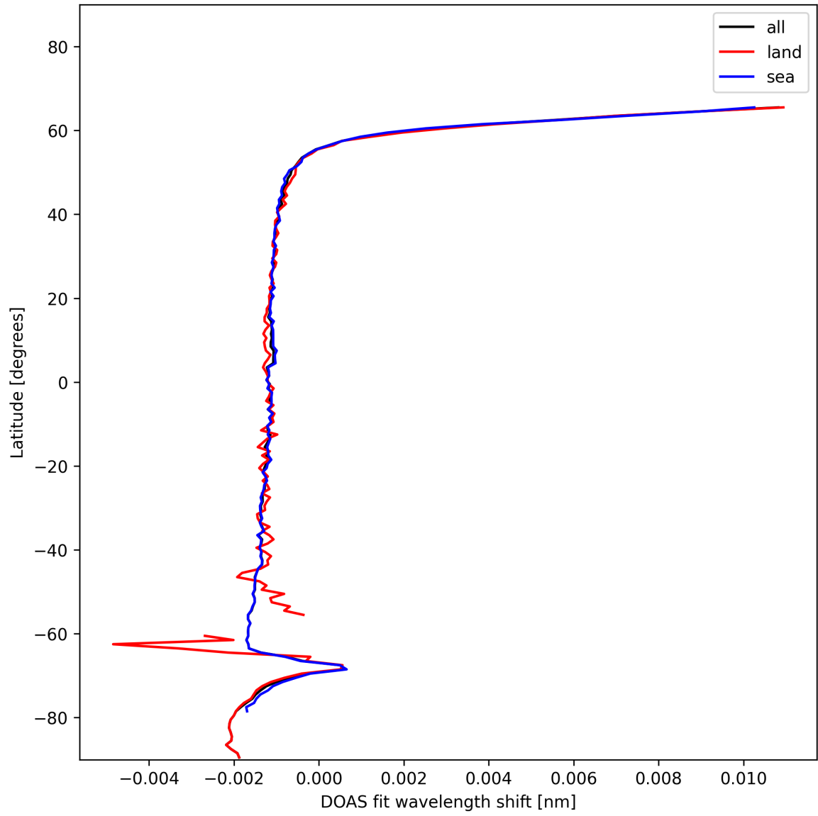
Figure 23: Zonal average of “DOAS fit wavelength shift” for 2024-12-30 to 2024-12-30.
