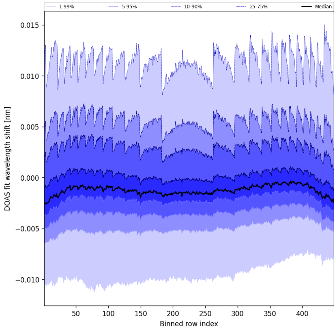
Figure 47: Along track statistics of “DOAS fit wavelength shift” for 2024-12-30 to 2024-12-30
