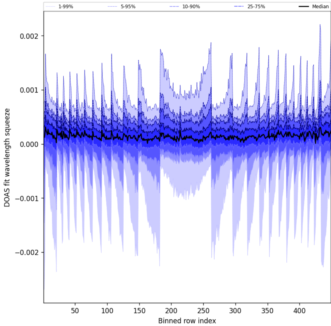
Figure 48: Along track statistics of “DOAS fit wavelength squeeze” for 2024-12-30 to 2024-12-30
