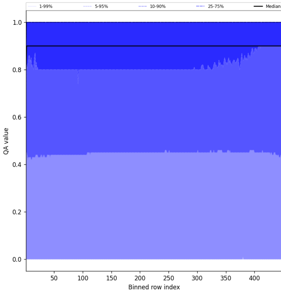
Figure 40: Along track statistics of “QA value” for 2024-12-30 to 2024-12-30
