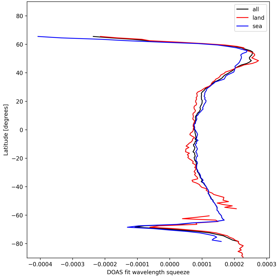
Figure 24: Zonal average of “DOAS fit wavelength squeeze” for 2024-12-30 to 2024-12-30.
