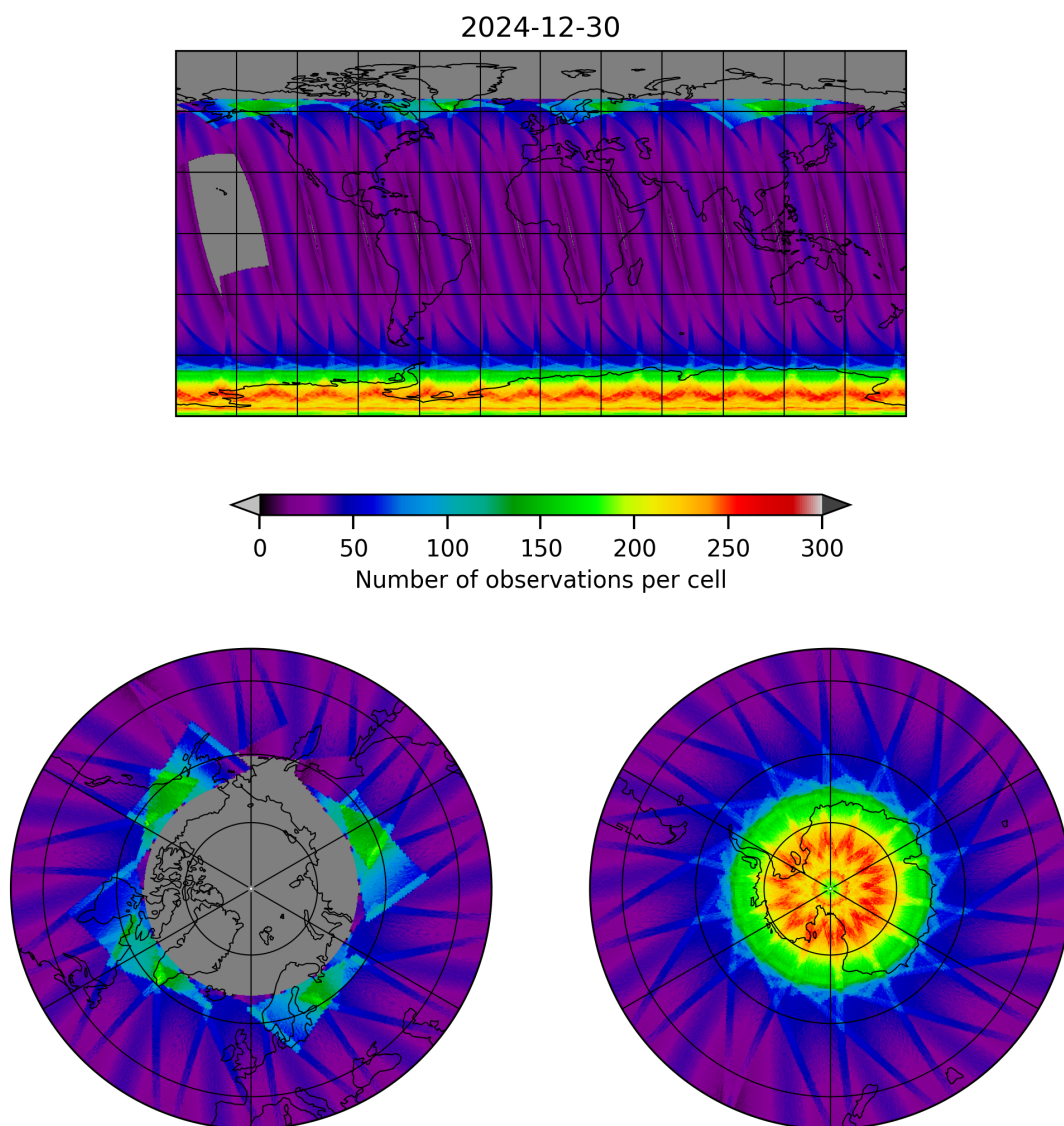
Figure 15: Map of the number of observations for 2024-12-30 to 2024-12-30
