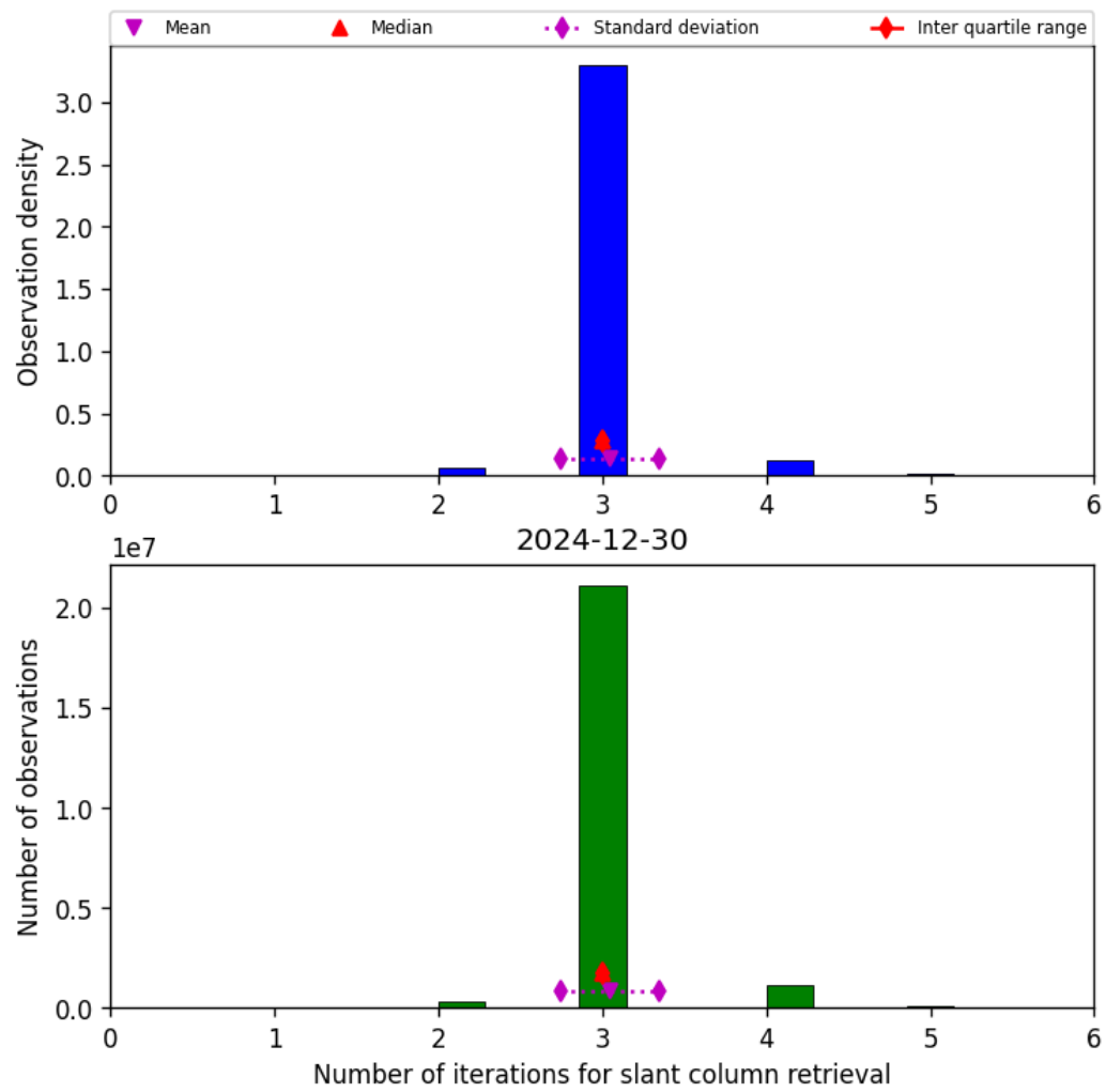
Figure 33: Histogram of “Number of iterations for slant column retrieval” for 2024-12-30 to 2024-12-30
