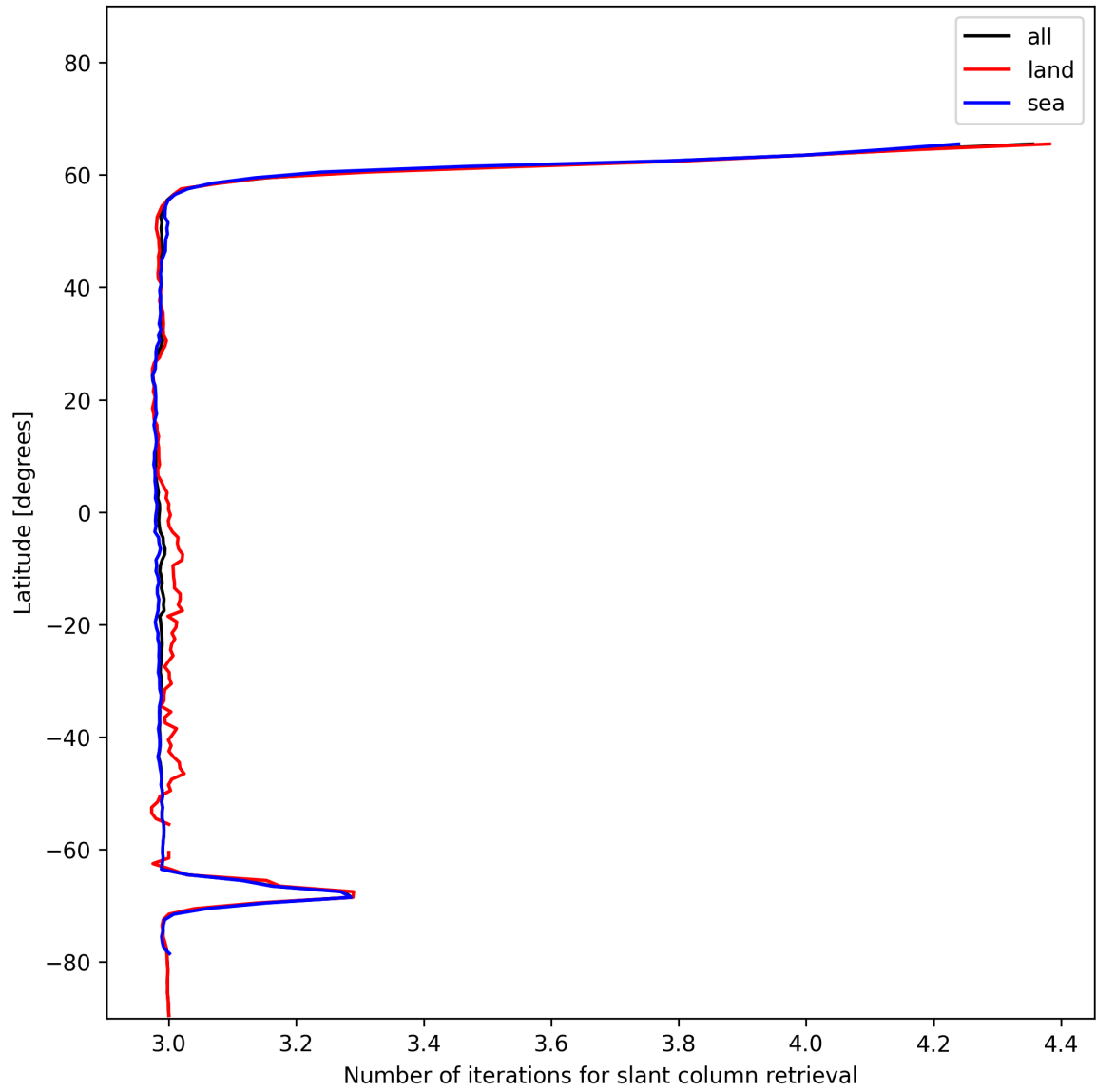
Figure 21: Zonal average of “Number of iterations for slant column retrieval” for 2024-12-30 to 2024-12-30.
