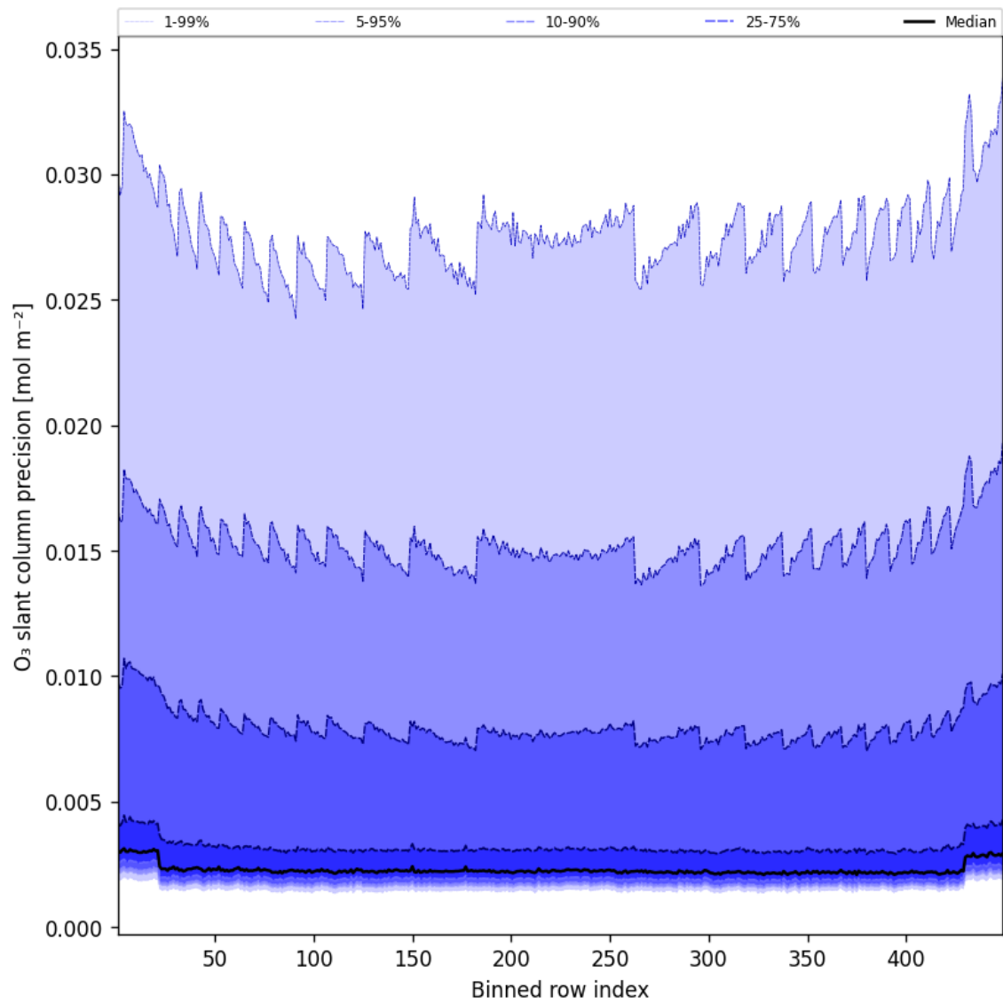
Figure 44: Along track statistics of “O 3 slant column precision” for 2024-12-30 to 2024-12-30
