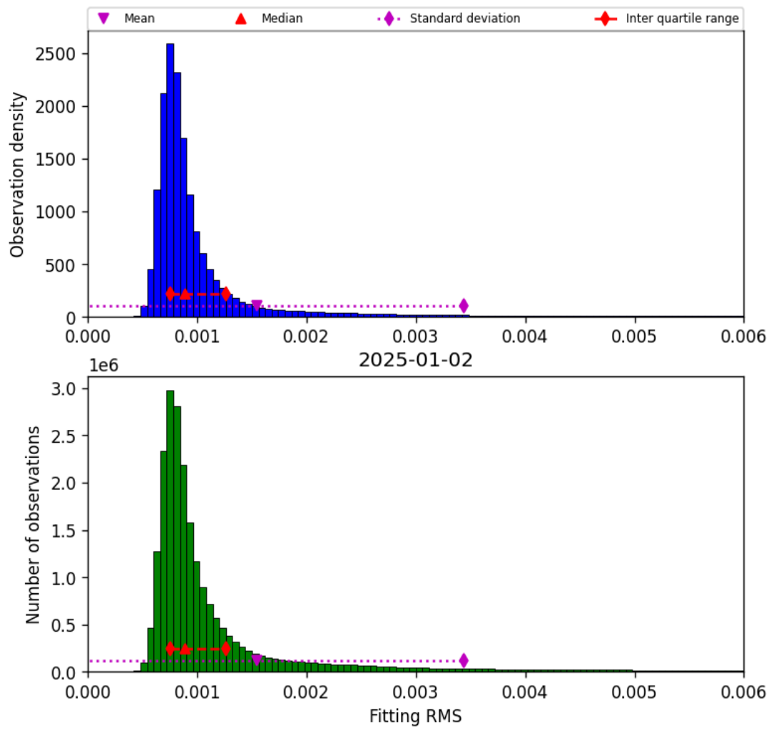
Figure 34: Histogram of “Fitting RMS” for 2025-01-02 to 2025-01-03
