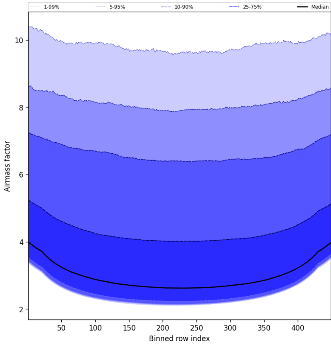
Figure 49: Along track statistics of “Airmass factor” for 2025-01-02 to 2025-01-03
