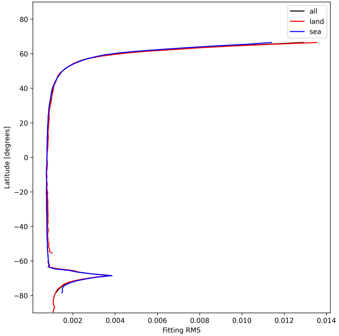
Figure 22: Zonal average of “Fitting RMS” for 2025-01-02 to 2025-01-03.
