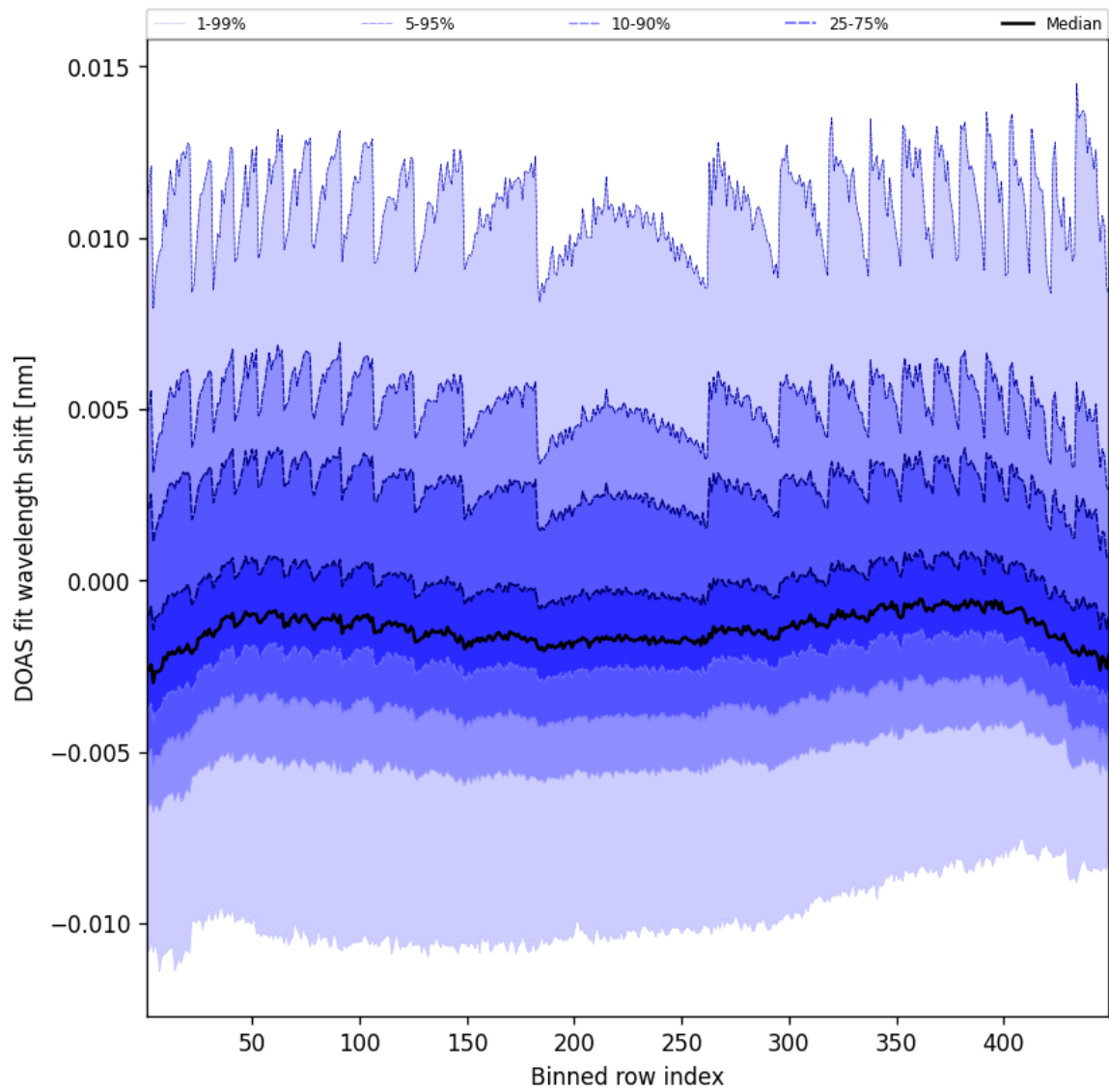
Figure 47: Along track statistics of “DOAS fit wavelength shift” for 2025-01-02 to 2025-01-03
