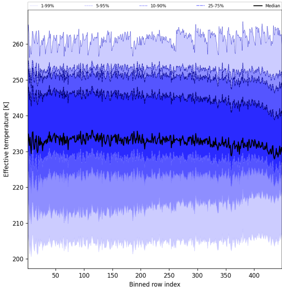
Figure 50: Along track statistics of “Effective temperature” for 2025-01-02 to 2025-01-03
