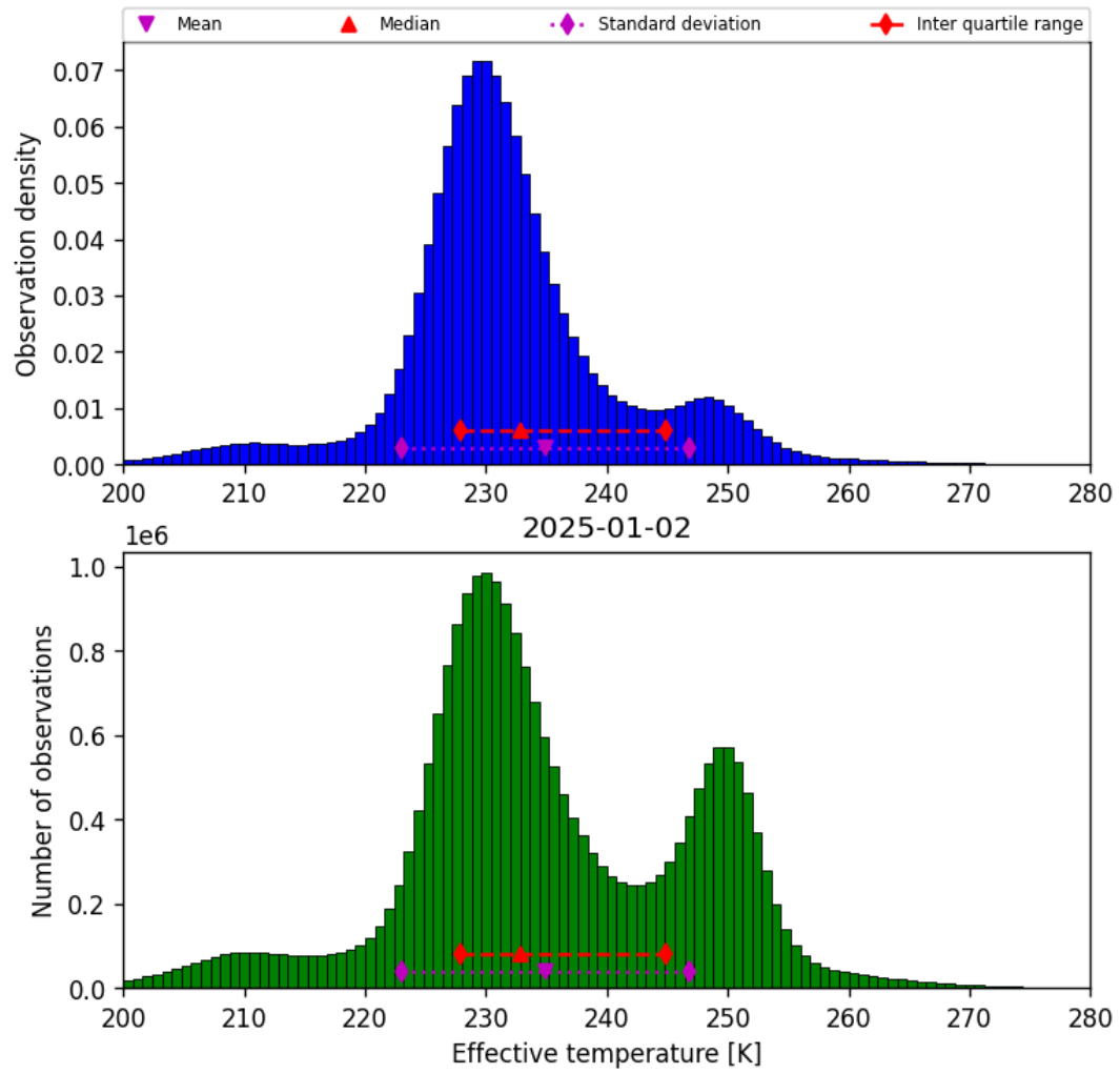
Figure 38: Histogram of “Effective temperature” for 2025-01-02 to 2025-01-03
