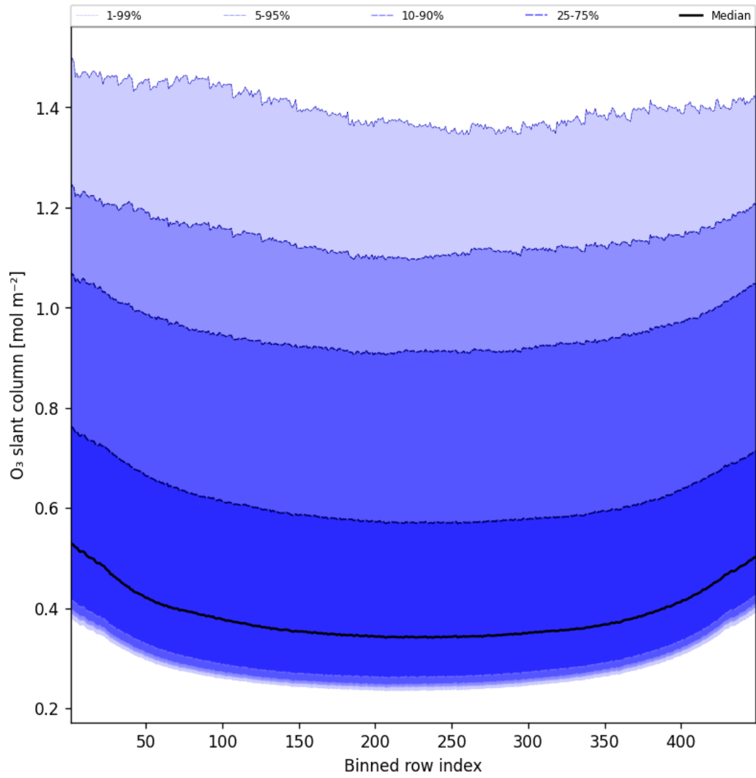
Figure 43: Along track statistics of “O 3 slant column” for 2025-01-02 to 2025-01-03
