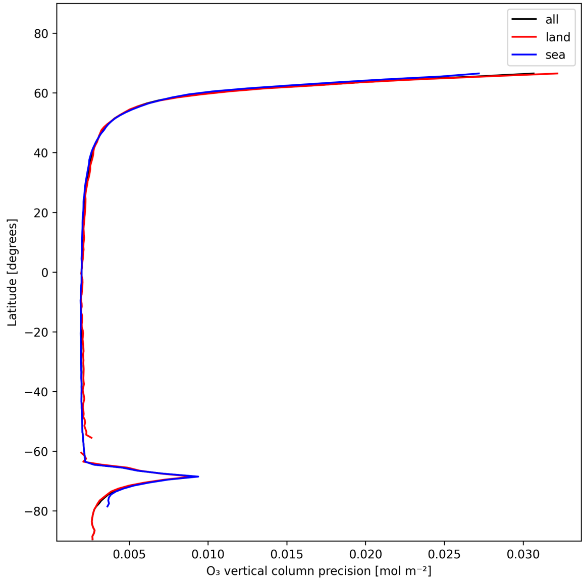
Figure 18: Zonal average of “O 3 vertical column precision” for 2025-01-02 to 2025-01-03.
