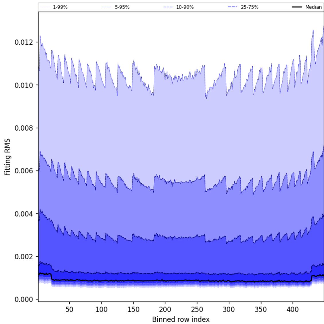
Figure 46: Along track statistics of “Fitting RMS” for 2025-01-02 to 2025-01-03
