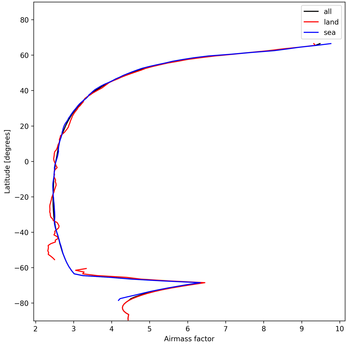
Figure 25: Zonal average of “Airmass factor” for 2025-01-02 to 2025-01-03.
