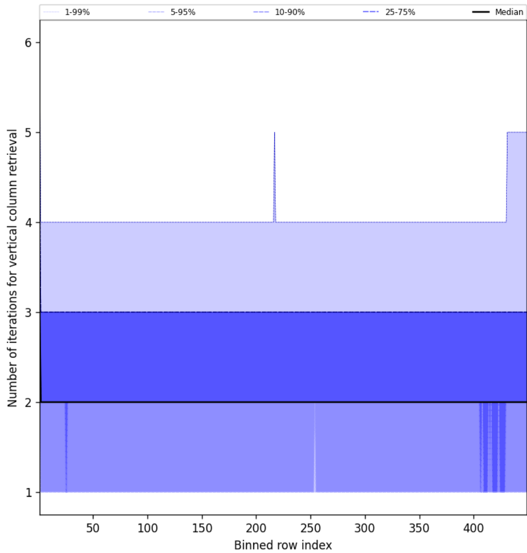
Figure 51: Along track statistics of “Number of iterations for vertical column retrieval” for 2025-01-02 to 2025-01-03
