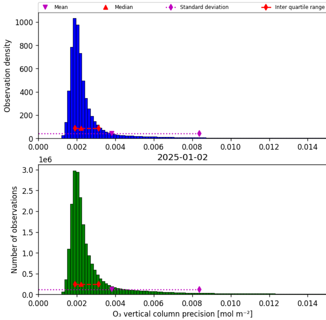
Figure 30: Histogram of “O 3 vertical column precision” for 2025-01-02 to 2025-01-03
