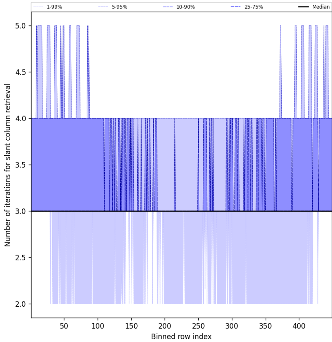
Figure 45: Along track statistics of “Number of iterations for slant column retrieval” for 2025-01-02 to 2025-01-03
