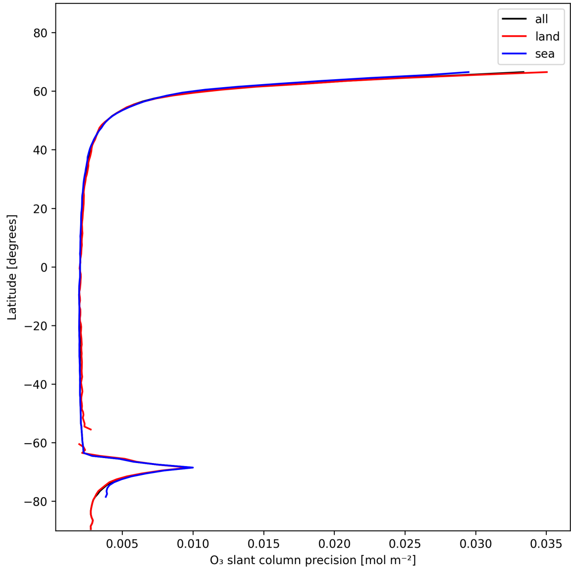
Figure 20: Zonal average of “O 3 slant column precision” for 2025-01-02 to 2025-01-03.
