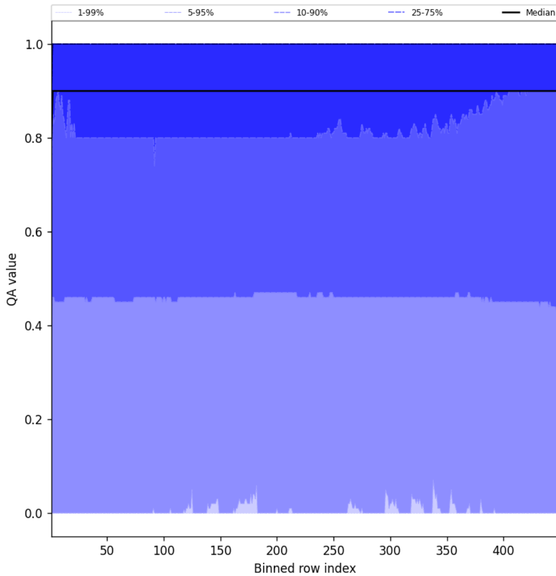
Figure 40: Along track statistics of “QA value” for 2025-01-02 to 2025-01-03
