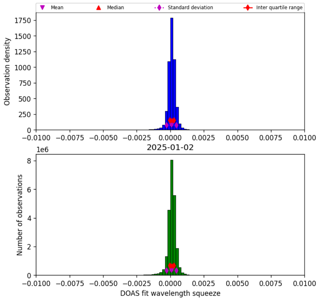
Figure 36: Histogram of “DOAS fit wavelength squeeze” for 2025-01-02 to 2025-01-03
