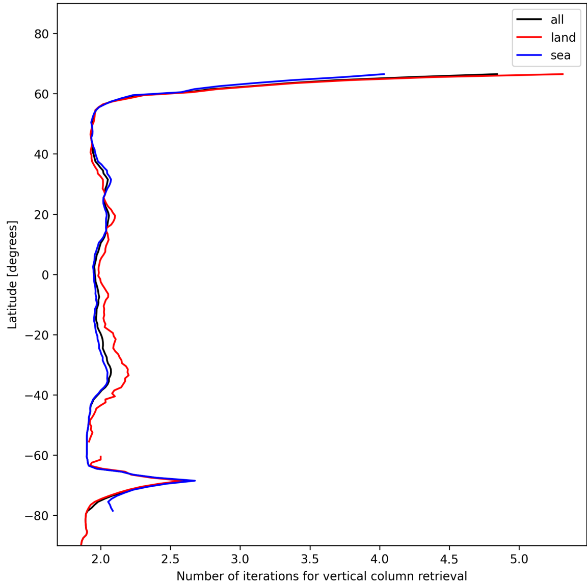
Figure 27: Zonal average of “Number of iterations for vertical column retrieval” for 2025-01-02 to 2025-01-03.
