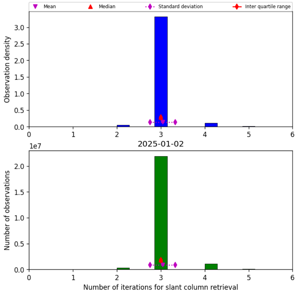
Figure 33: Histogram of “Number of iterations for slant column retrieval” for 2025-01-02 to 2025-01-03
