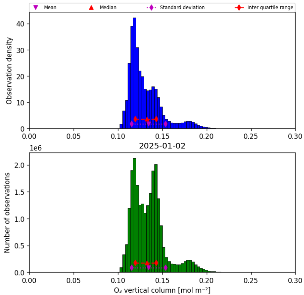
Figure 29: Histogram of “O 3 vertical column” for 2025-01-02 to 2025-01-03
