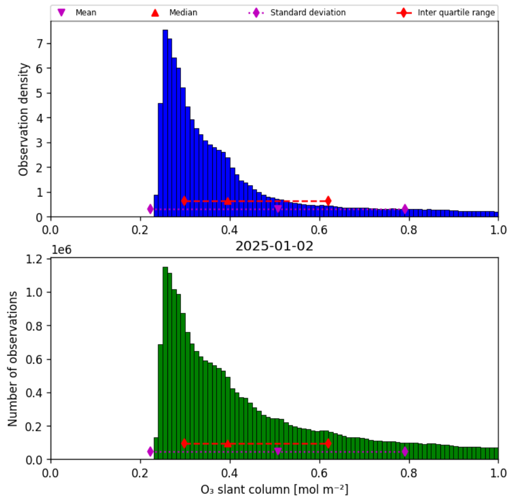
Figure 31: Histogram of “O 3 slant column” for 2025-01-02 to 2025-01-03
