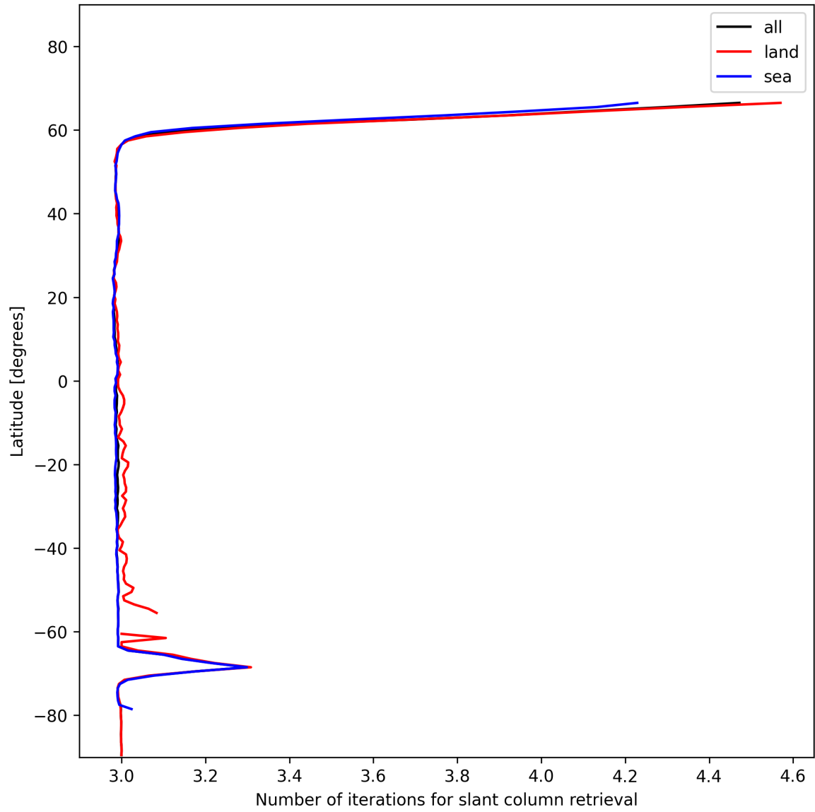
Figure 21: Zonal average of “Number of iterations for slant column retrieval” for 2025-01-02 to 2025-01-03.
