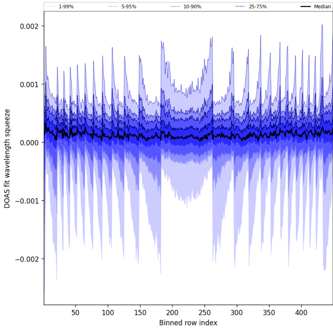
Figure 48: Along track statistics of “DOAS fit wavelength squeeze” for 2025-01-02 to 2025-01-03
