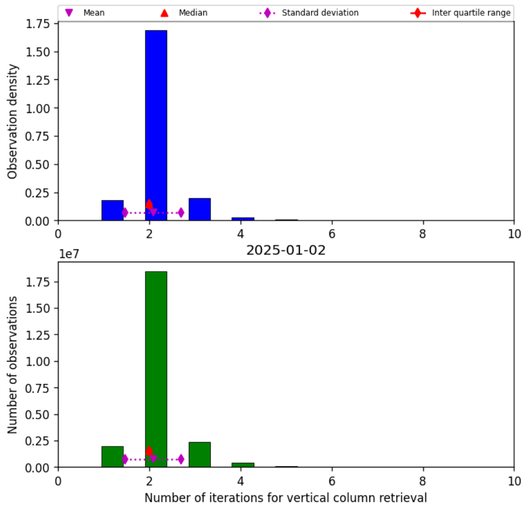
Figure 39: Histogram of “Number of iterations for vertical column retrieval” for 2025-01-02 to 2025-01-03
