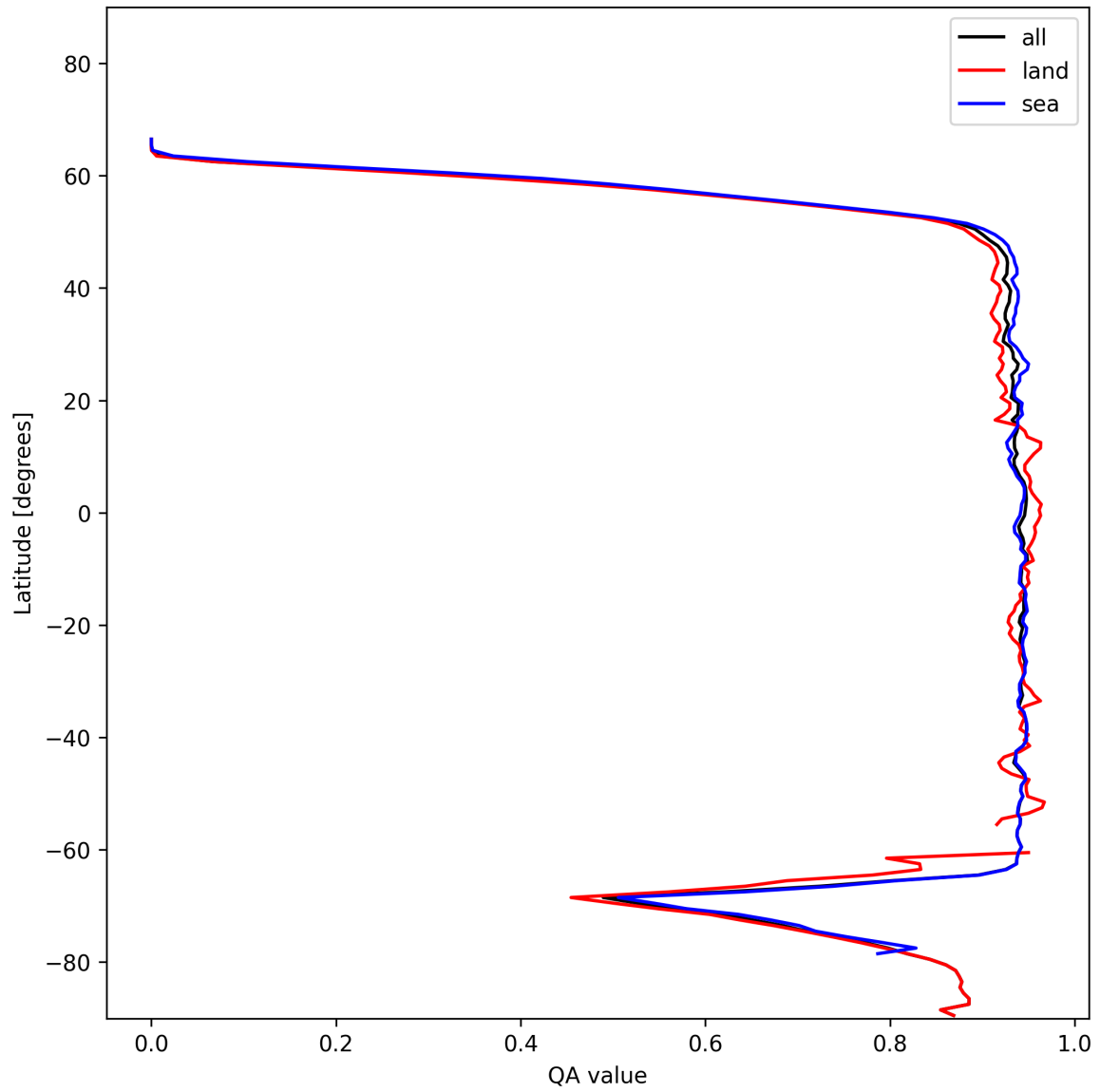
Figure 16: Zonal average of “QA value” for 2025-01-02 to 2025-01-03.
