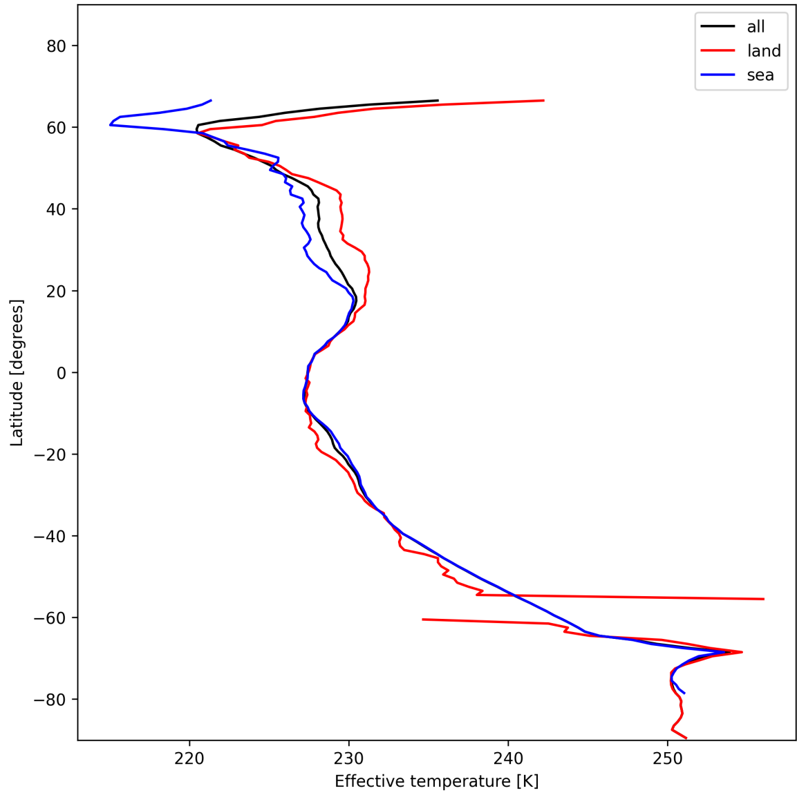
Figure 26: Zonal average of “Effective temperature” for 2025-01-02 to 2025-01-03.
