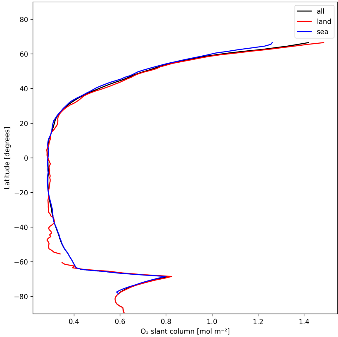
Figure 19: Zonal average of “O 3 slant column” for 2025-01-02 to 2025-01-03.
