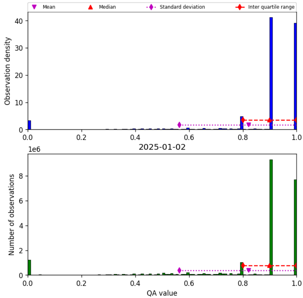
Figure 28: Histogram of “QA value” for 2025-01-02 to 2025-01-03
