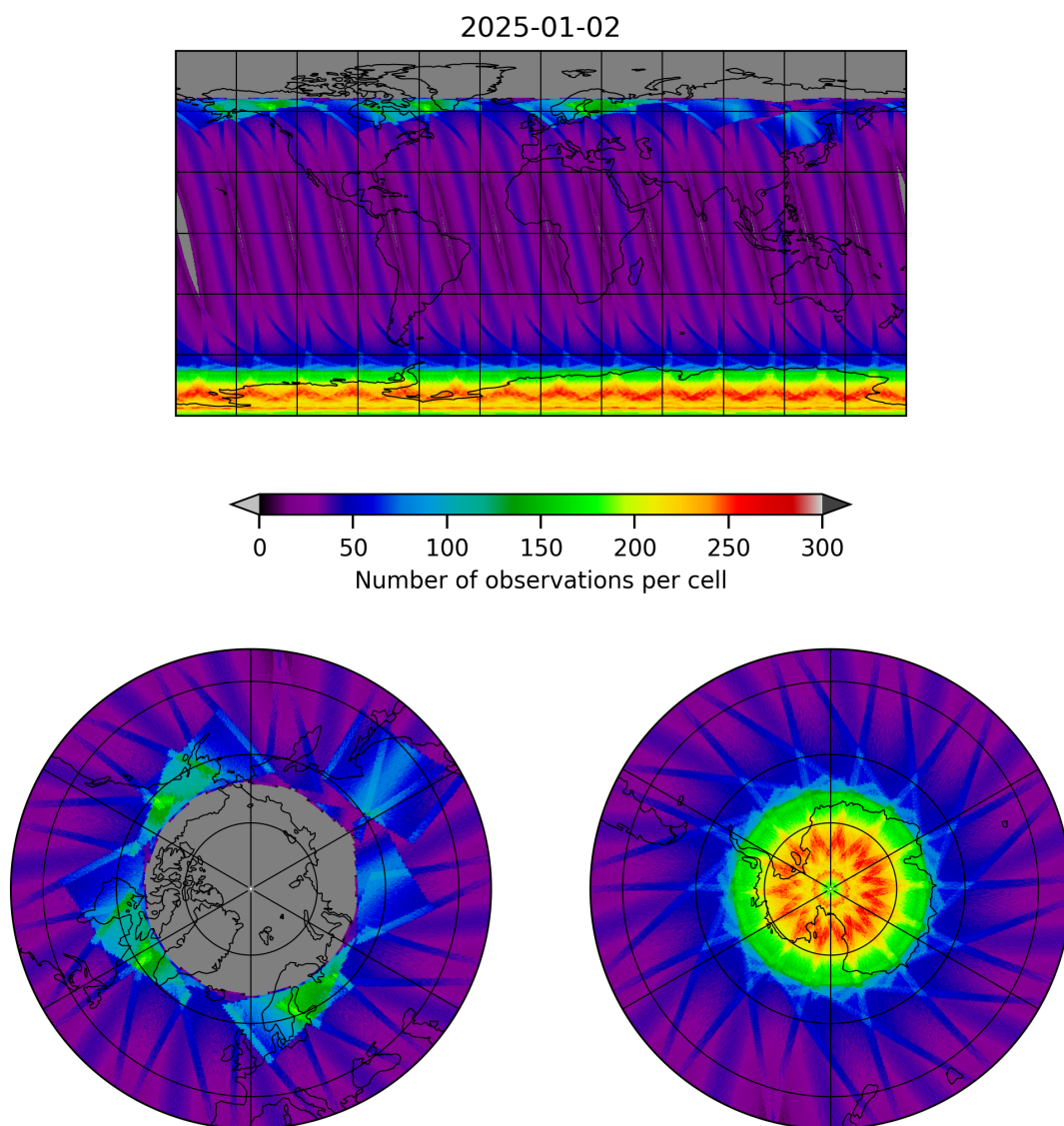
Figure 15: Map of the number of observations for 2025-01-02 to 2025-01-03
