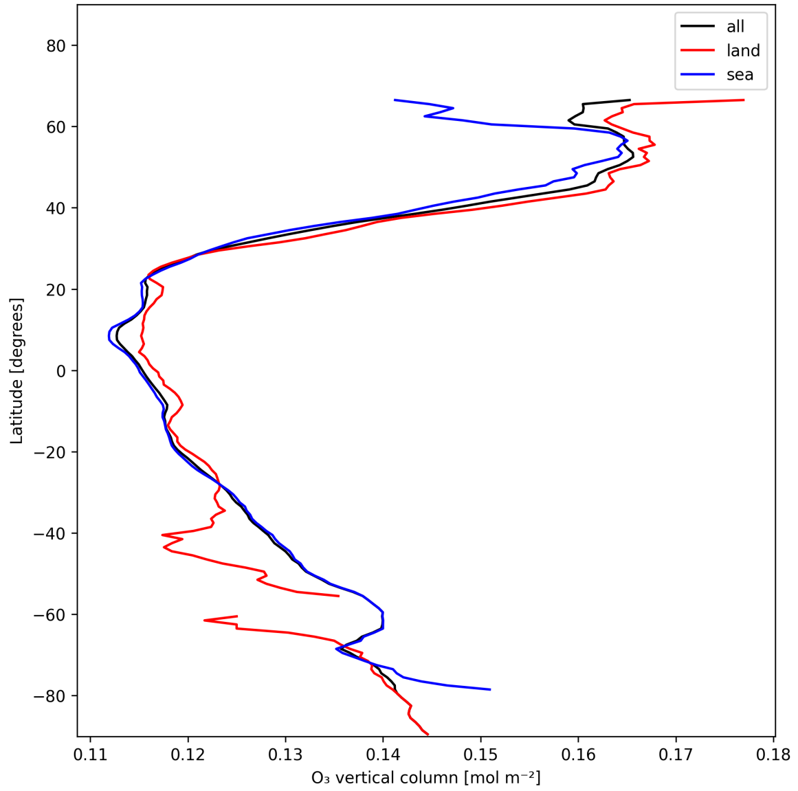
Figure 17: Zonal average of “O 3 vertical column” for 2025-01-02 to 2025-01-03.
