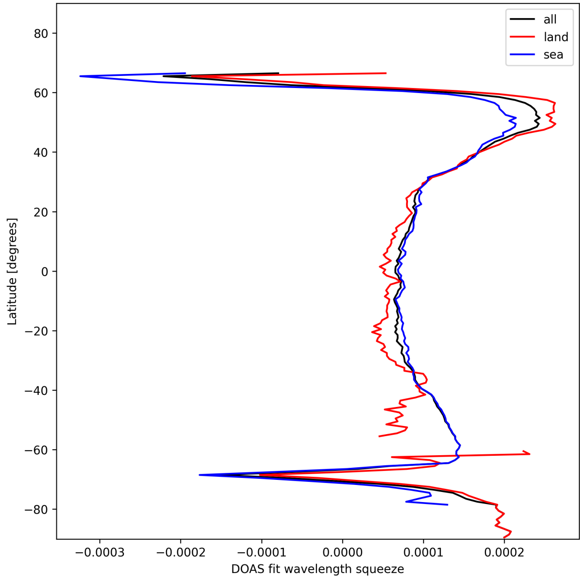
Figure 24: Zonal average of “DOAS fit wavelength squeeze” for 2025-01-02 to 2025-01-03.
