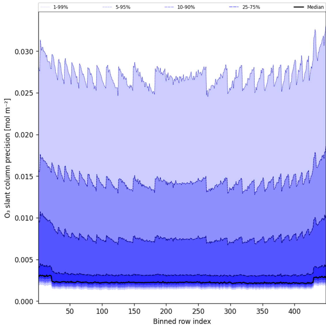
Figure 44: Along track statistics of “O 3 slant column precision” for 2025-01-02 to 2025-01-03
