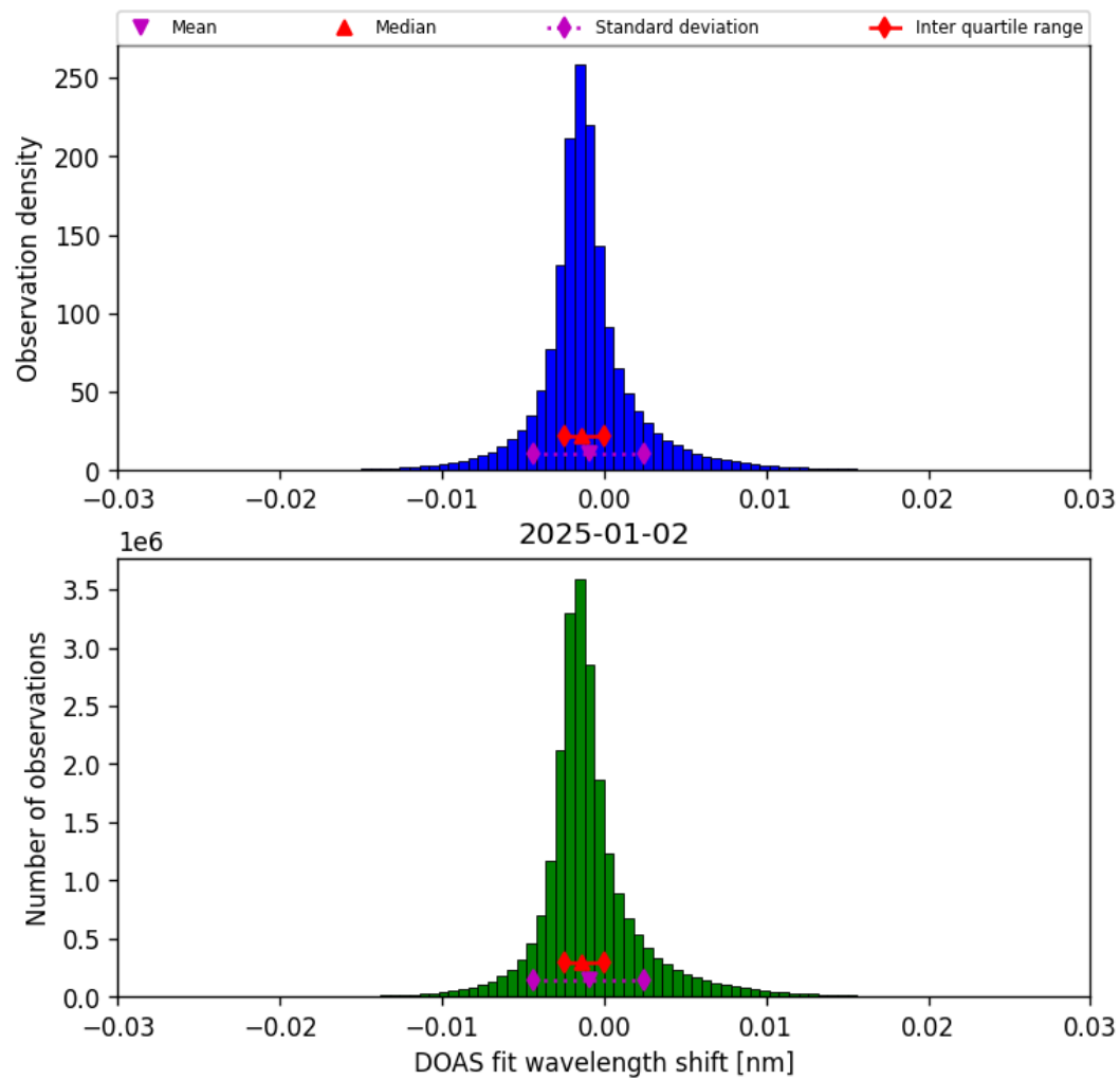
Figure 35: Histogram of “DOAS fit wavelength shift” for 2025-01-02 to 2025-01-03
