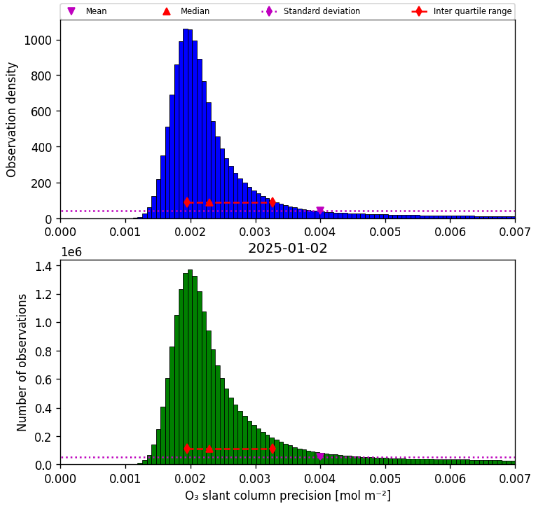
Figure 32: Histogram of "O 3 slant column precision" for 2025-01-02 to 2025-01-03
