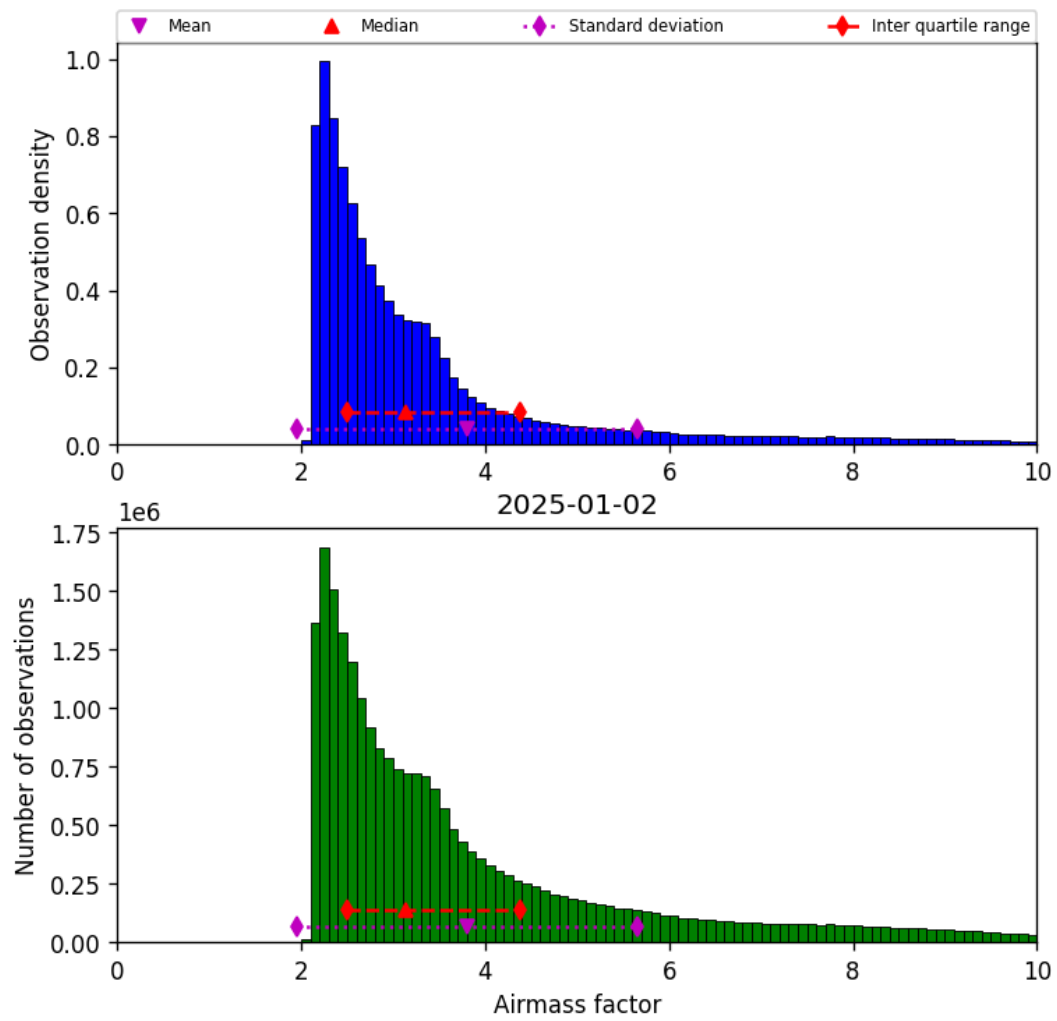
Figure 37: Histogram of “Airmass factor” for 2025-01-02 to 2025-01-03
