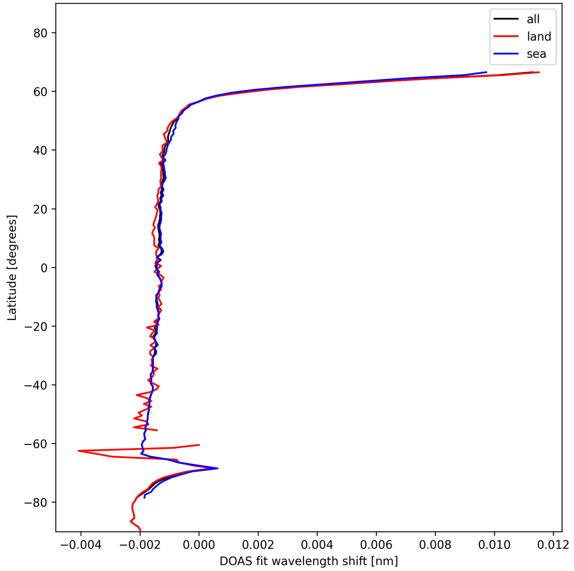
Figure 23: Zonal average of “DOAS fit wavelength shift” for 2025-01-02 to 2025-01-03.
