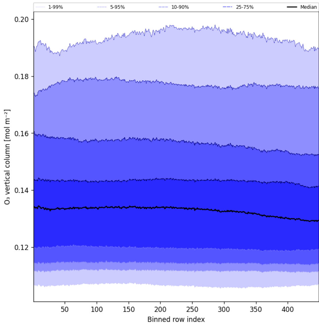
Figure 41: Along track statistics of “O 3 vertical column” for 2025-01-02 to 2025-01-03
