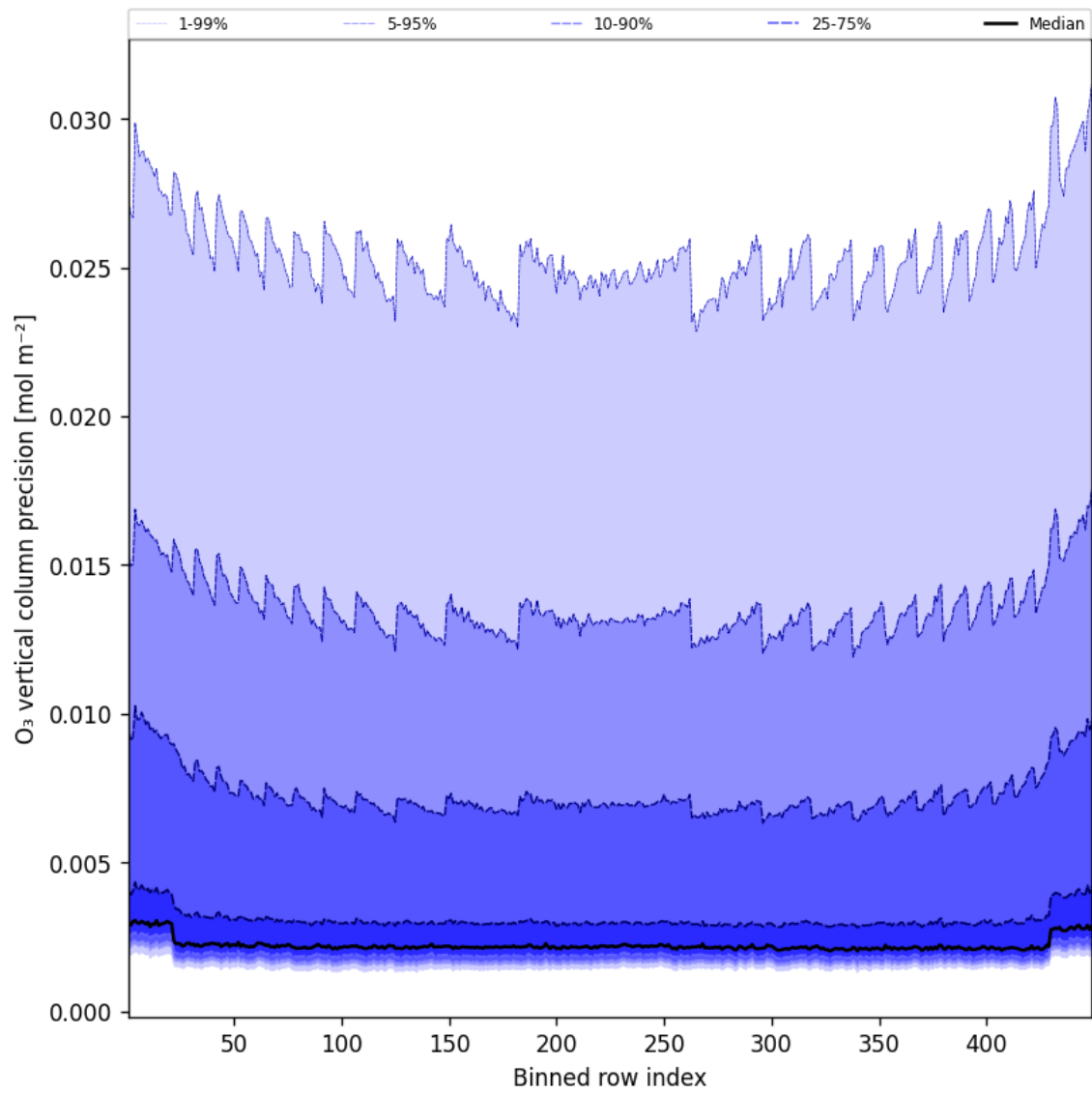
Figure 42: Along track statistics of “O 3 vertical column precision” for 2025-01-02 to 2025-01-03
