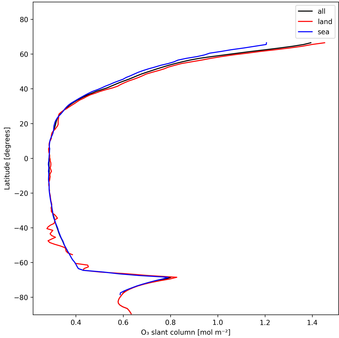
Figure 19: Zonal average of “O 3 slant column” for 2025-01-03 to 2025-01-04.
