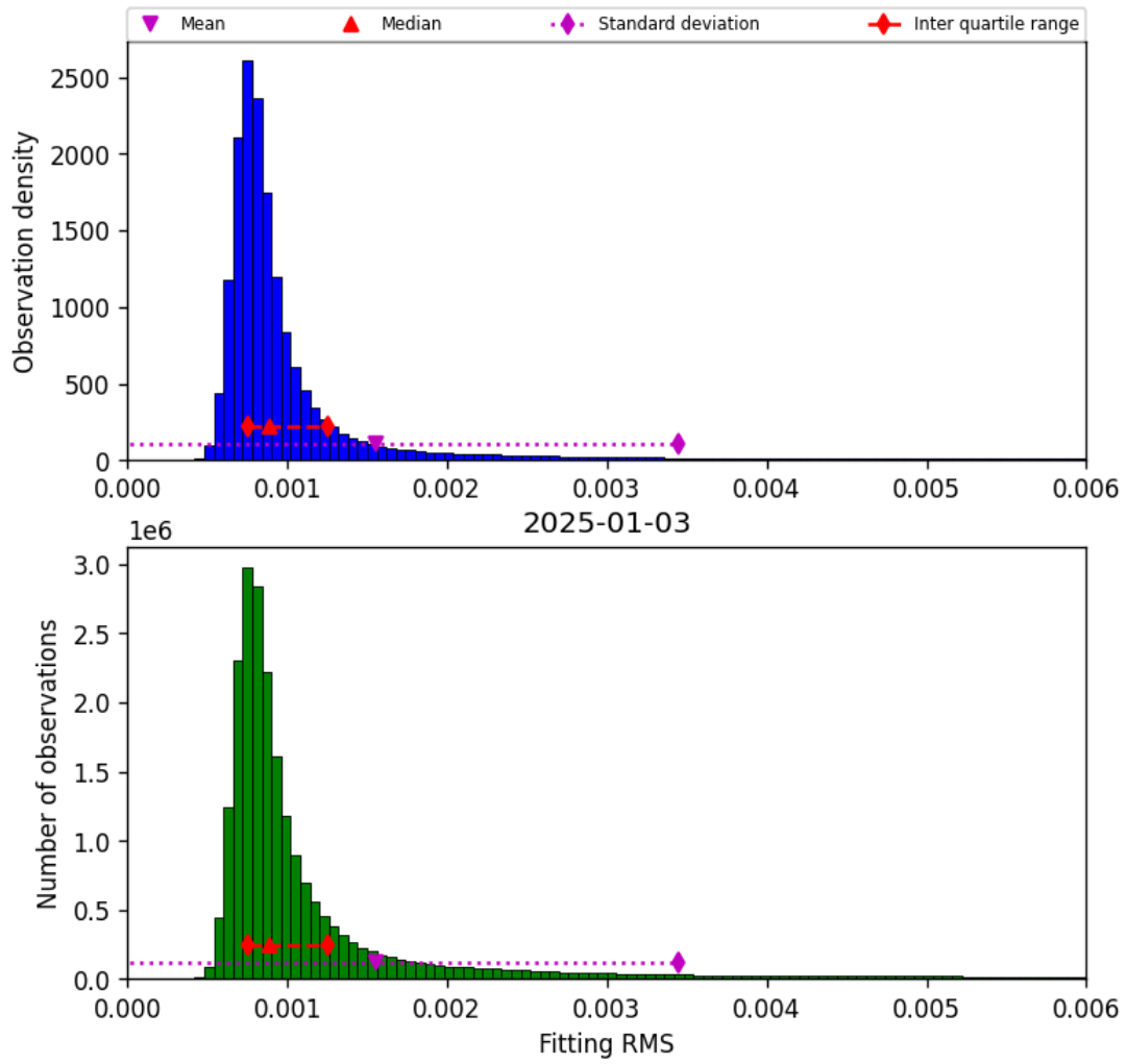
Figure 34: Histogram of “Fitting RMS” for 2025-01-03 to 2025-01-04
