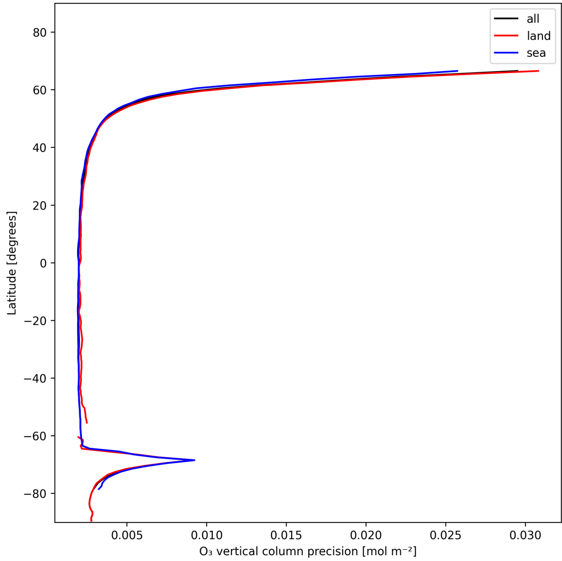
Figure 18: Zonal average of “O 3 vertical column precision” for 2025-01-03 to 2025-01-04.
