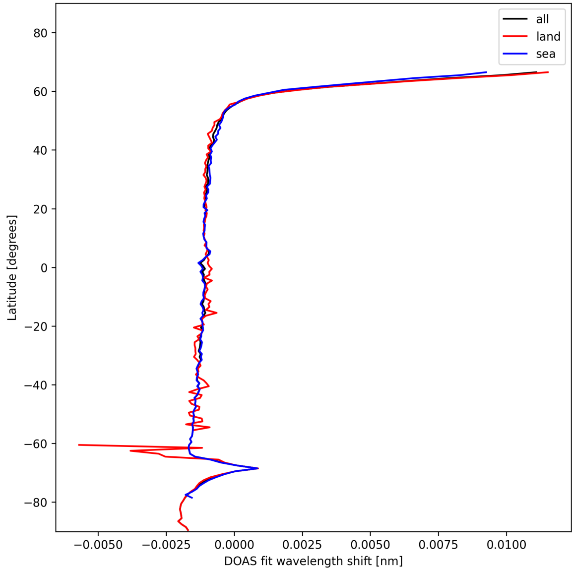
Figure 23: Zonal average of “DOAS fit wavelength shift” for 2025-01-03 to 2025-01-04.
