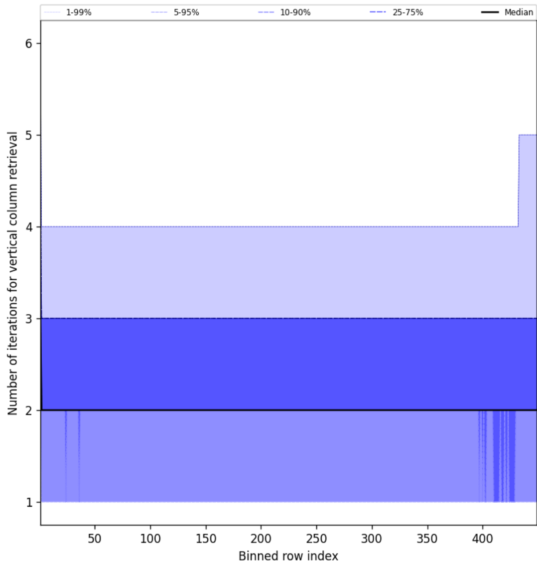
Figure 51: Along track statistics of “Number of iterations for vertical column retrieval” for 2025-01-03 to 2025-01-04
