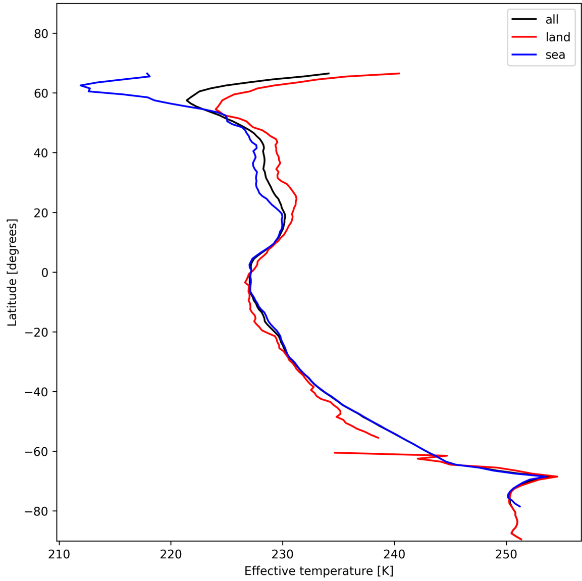
Figure 26: Zonal average of “Effective temperature” for 2025-01-03 to 2025-01-04.
