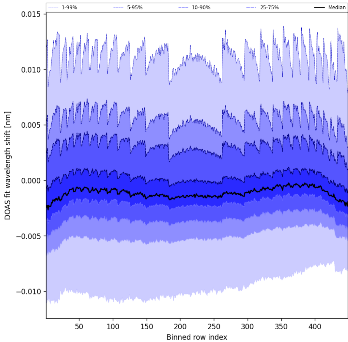
Figure 47: Along track statistics of “DOAS fit wavelength shift” for 2025-01-03 to 2025-01-04
