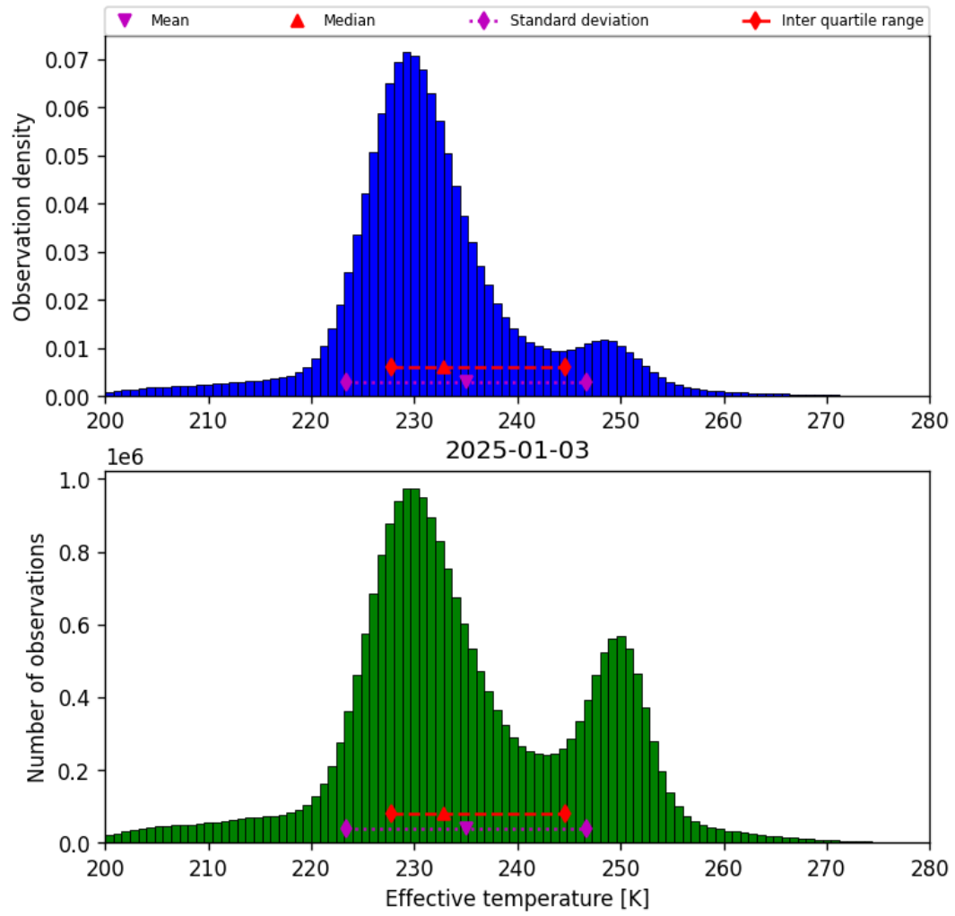
Figure 38: Histogram of “Effective temperature” for 2025-01-03 to 2025-01-04
