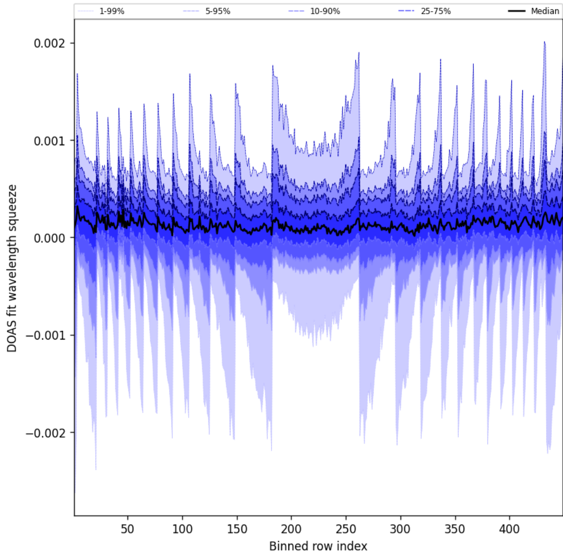
Figure 48: Along track statistics of “DOAS fit wavelength squeeze” for 2025-01-03 to 2025-01-04
