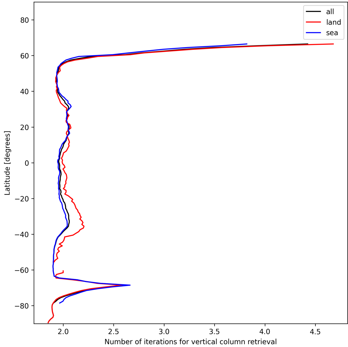
Figure 27: Zonal average of “Number of iterations for vertical column retrieval” for 2025-01-03 to 2025-01-04.
