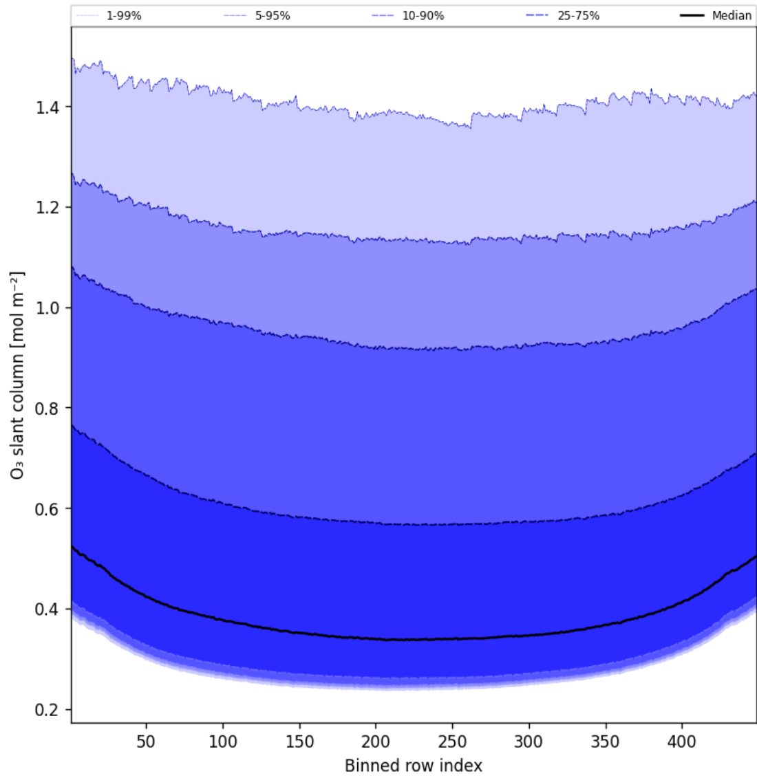
Figure 43: Along track statistics of “O 3 slant column” for 2025-01-03 to 2025-01-04
