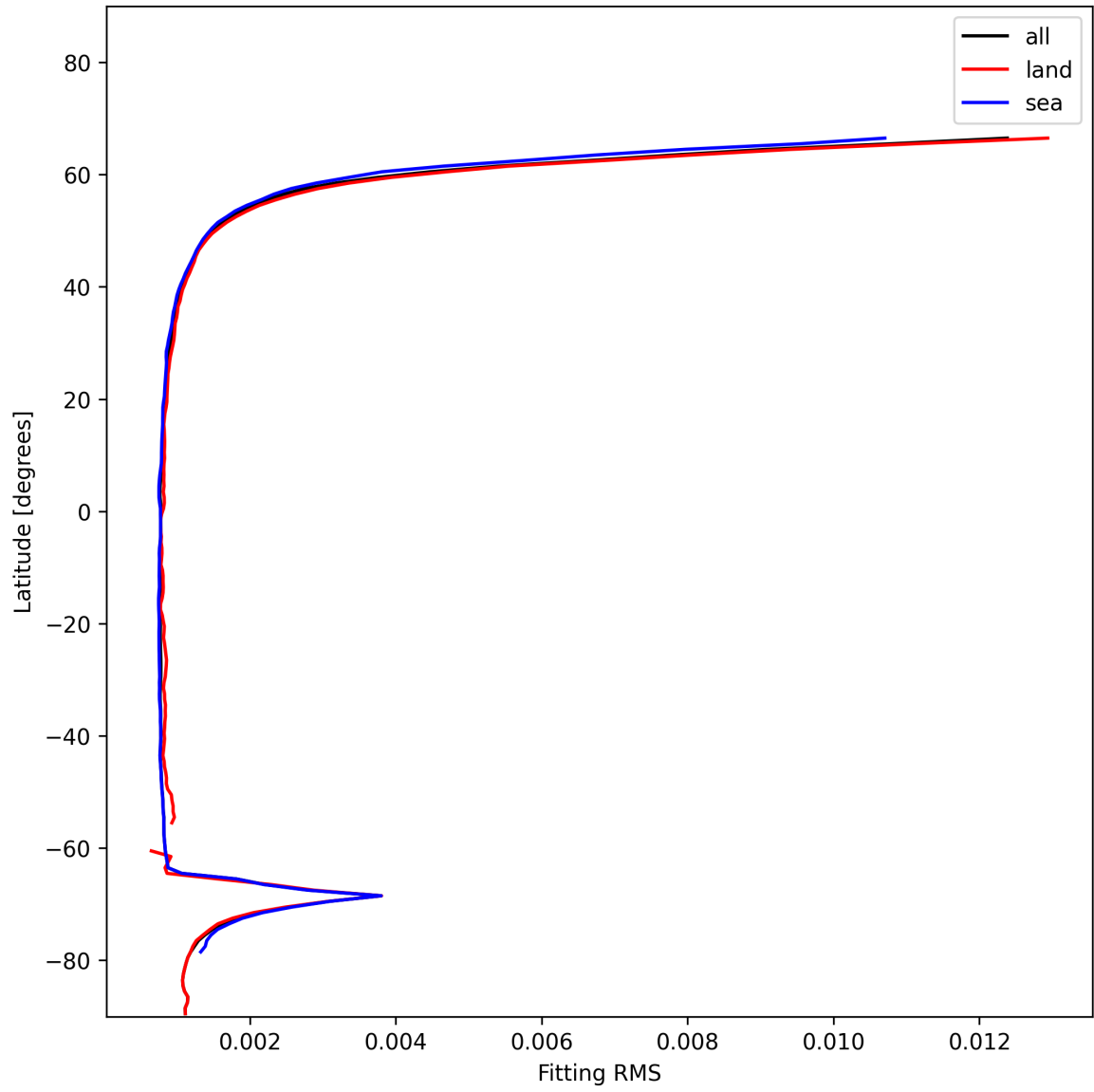
Figure 22: Zonal average of “Fitting RMS” for 2025-01-03 to 2025-01-04.
