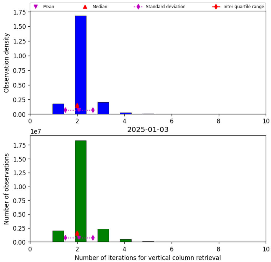
Figure 39: Histogram of “Number of iterations for vertical column retrieval” for 2025-01-03 to 2025-01-04
