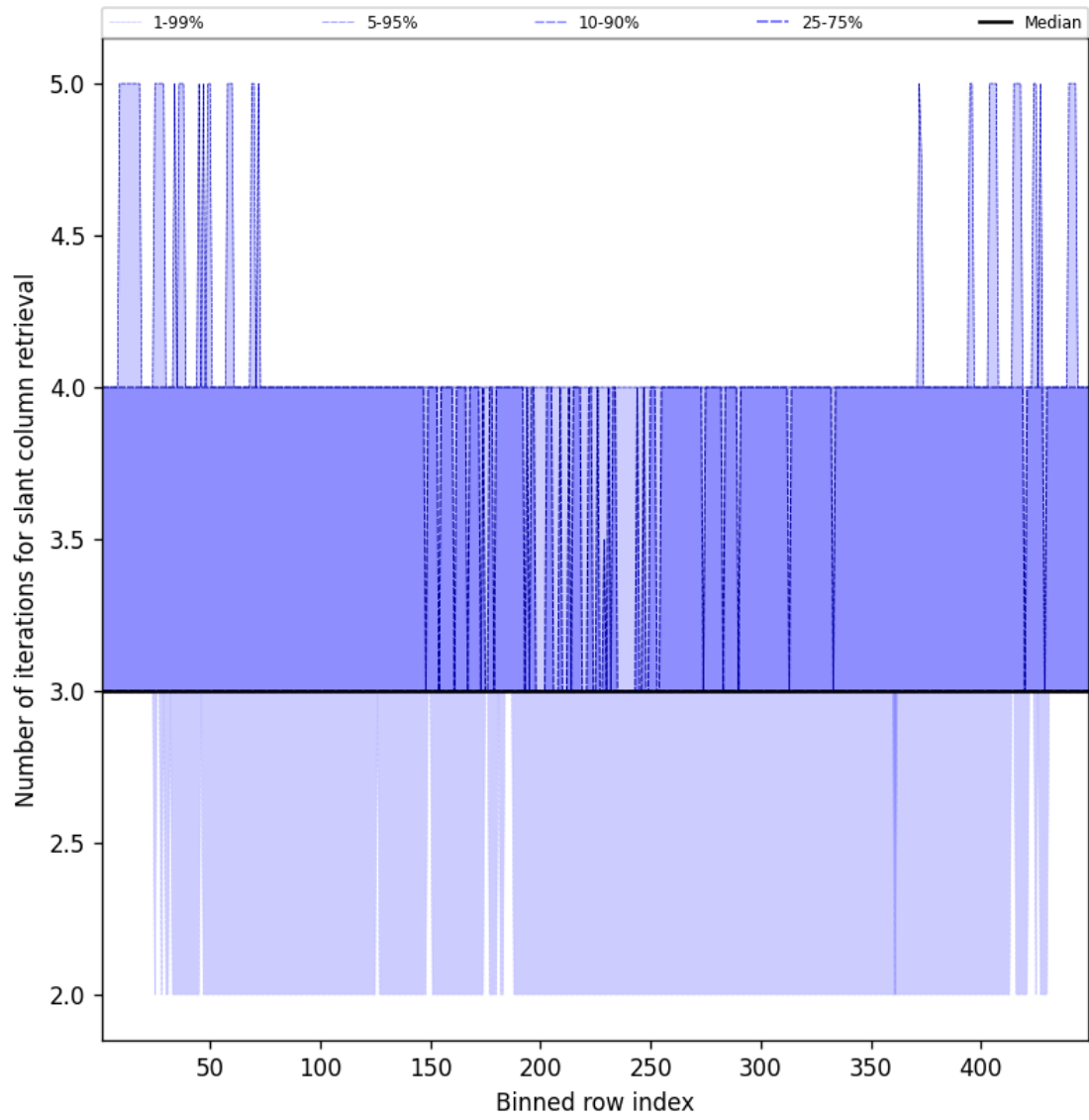
Figure 45: Along track statistics of “Number of iterations for slant column retrieval” for 2025-01-03 to 2025-01-04
