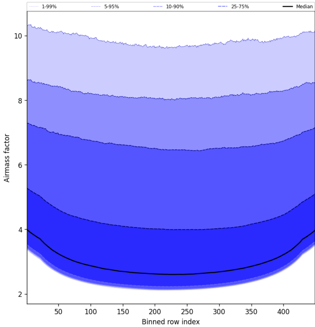
Figure 49: Along track statistics of “Airmass factor” for 2025-01-03 to 2025-01-04
