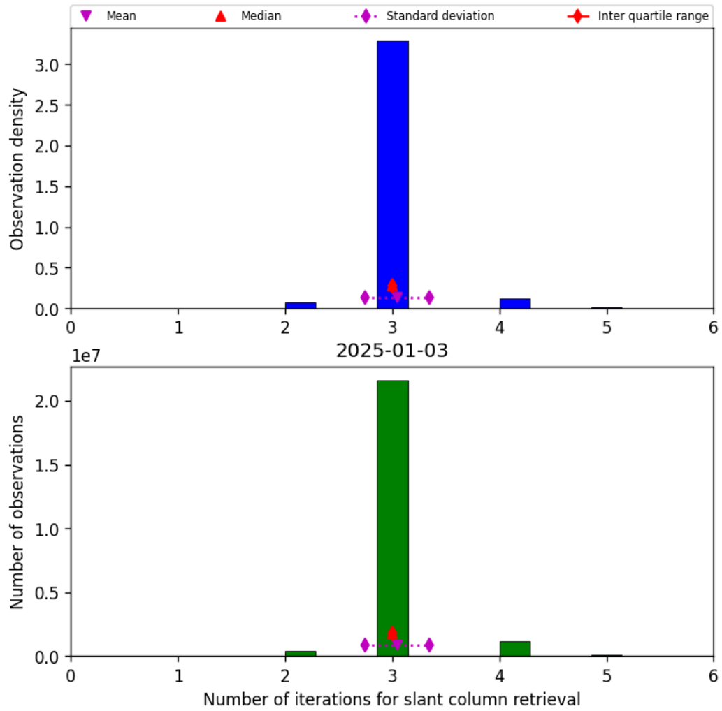
Figure 33: Histogram of “Number of iterations for slant column retrieval” for 2025-01-03 to 2025-01-04
