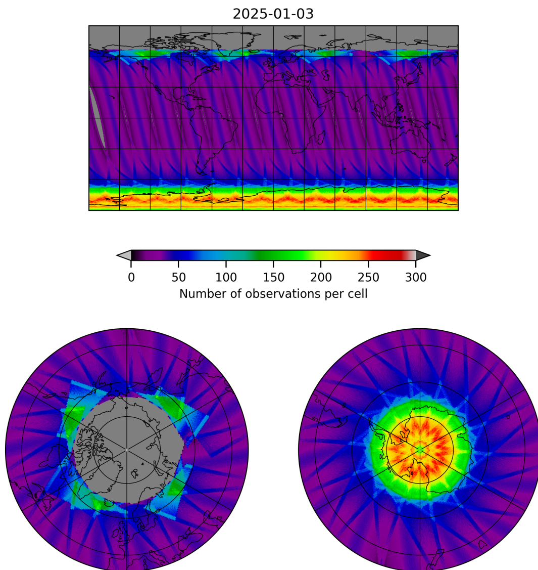
Figure 15: Map of the number of observations for 2025-01-03 to 2025-01-04
