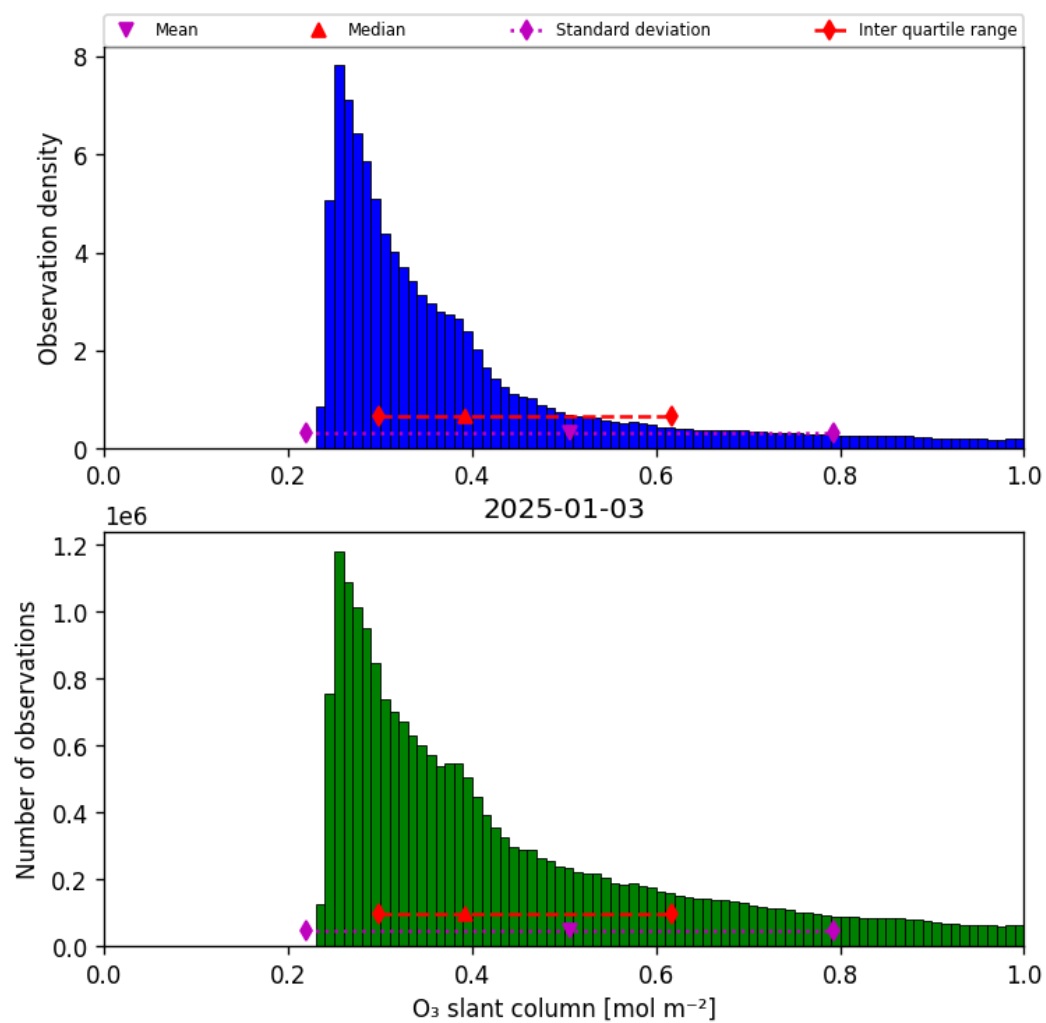
Figure 31: Histogram of “O 3 slant column” for 2025-01-03 to 2025-01-04
