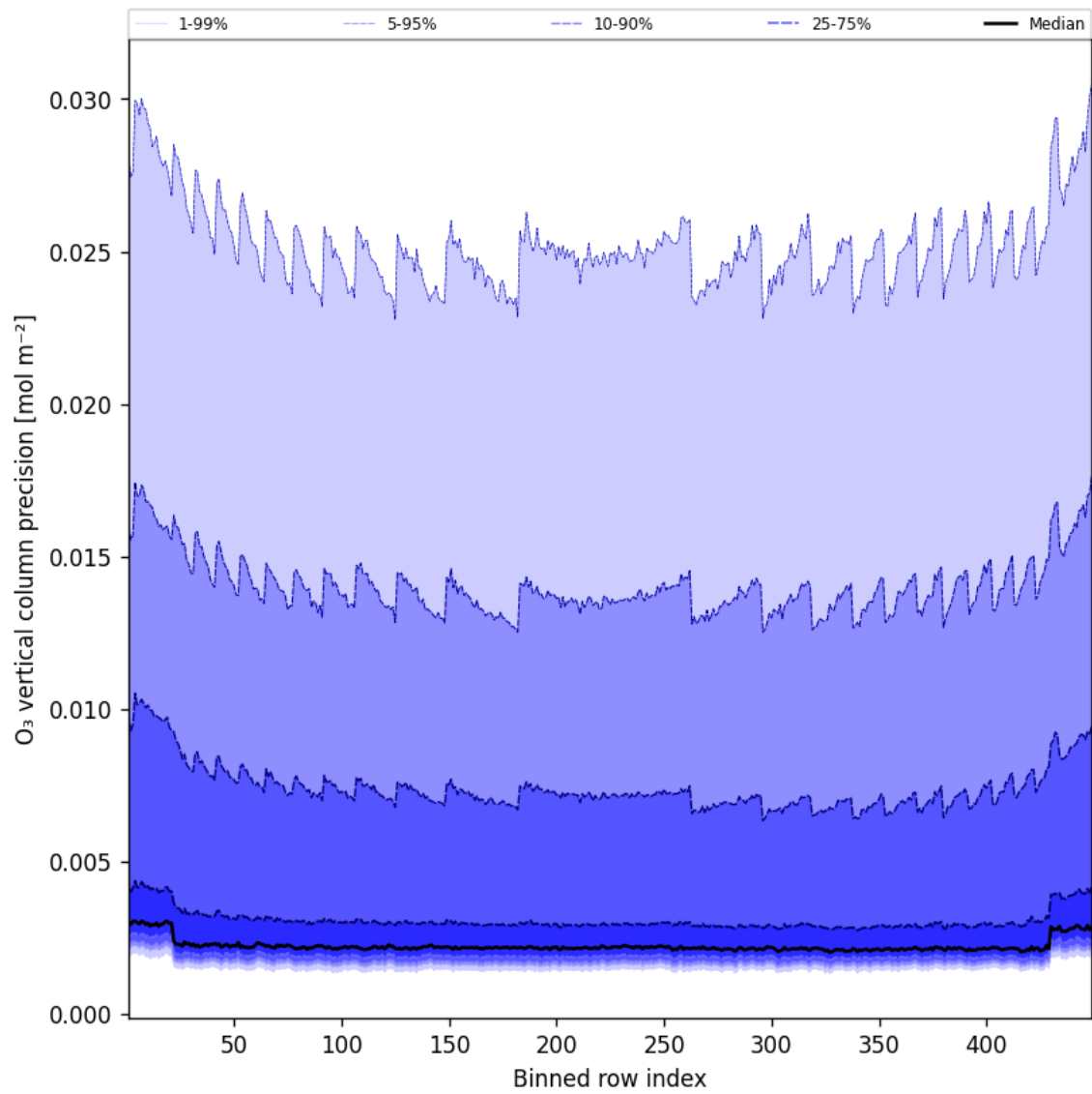
Figure 42: Along track statistics of “O 3 vertical column precision” for 2025-01-03 to 2025-01-04
