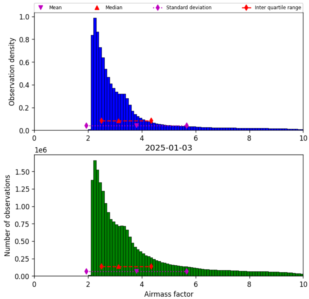
Figure 37: Histogram of “Airmass factor” for 2025-01-03 to 2025-01-04
