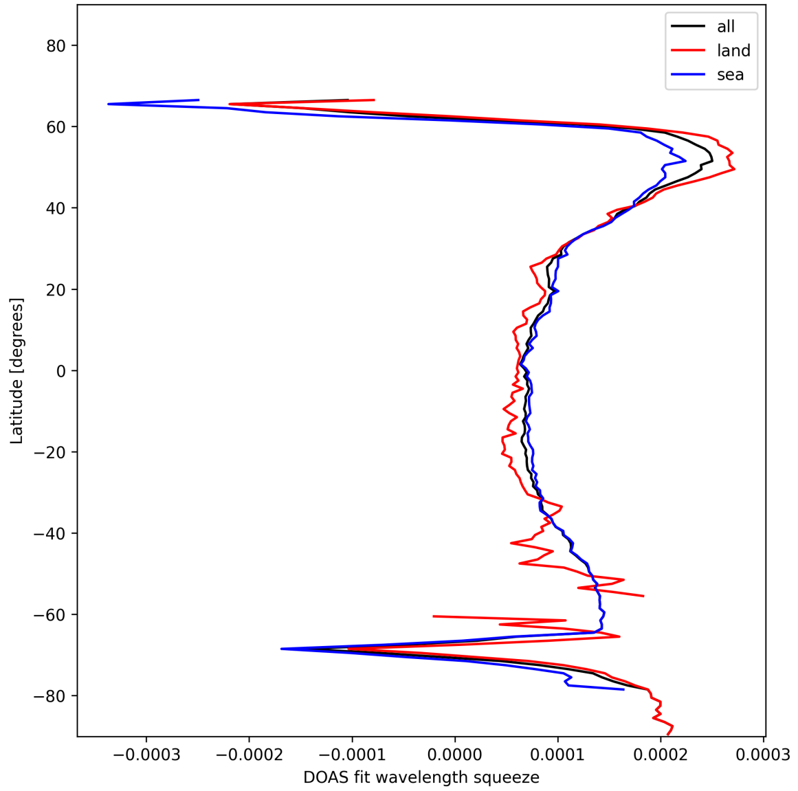
Figure 24: Zonal average of “DOAS fit wavelength squeeze” for 2025-01-03 to 2025-01-04.
