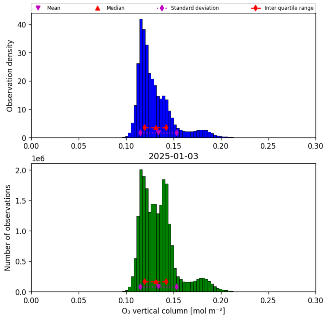
Figure 29: Histogram of “O 3 vertical column” for 2025-01-03 to 2025-01-04
