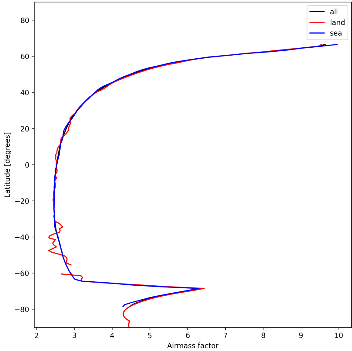
Figure 25: Zonal average of “Airmass factor” for 2025-01-03 to 2025-01-04.
