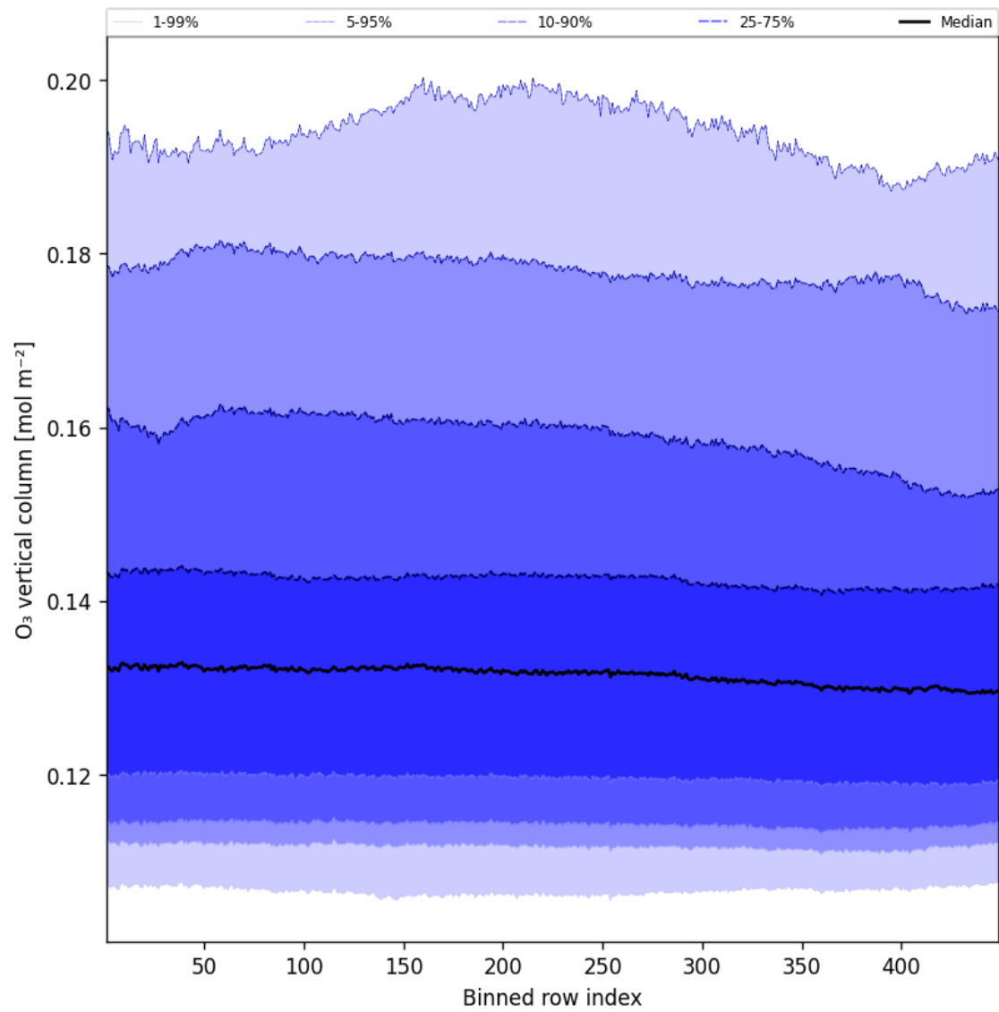
Figure 41: Along track statistics of “O 3 vertical column” for 2025-01-03 to 2025-01-04
