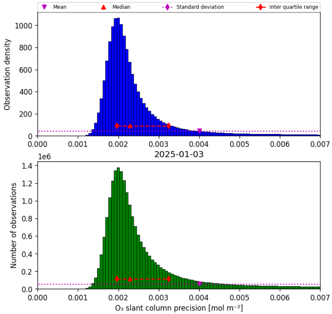
Figure 32: Histogram of “O 3 slant column precision” for 2025-01-03 to 2025-01-04
