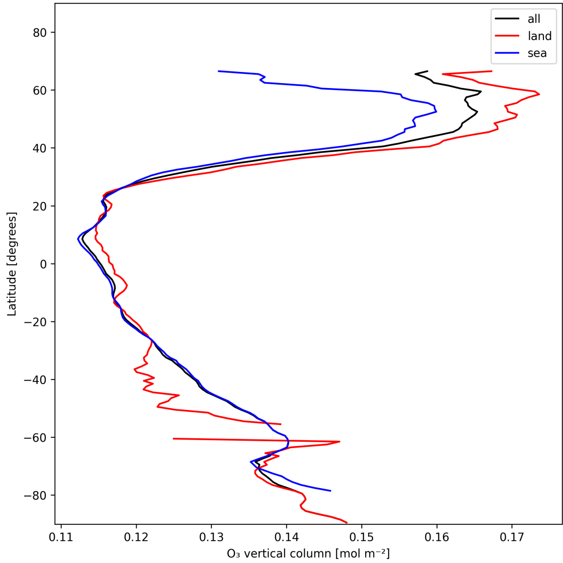
Figure 17: Zonal average of “O 3 vertical column” for 2025-01-03 to 2025-01-04.
