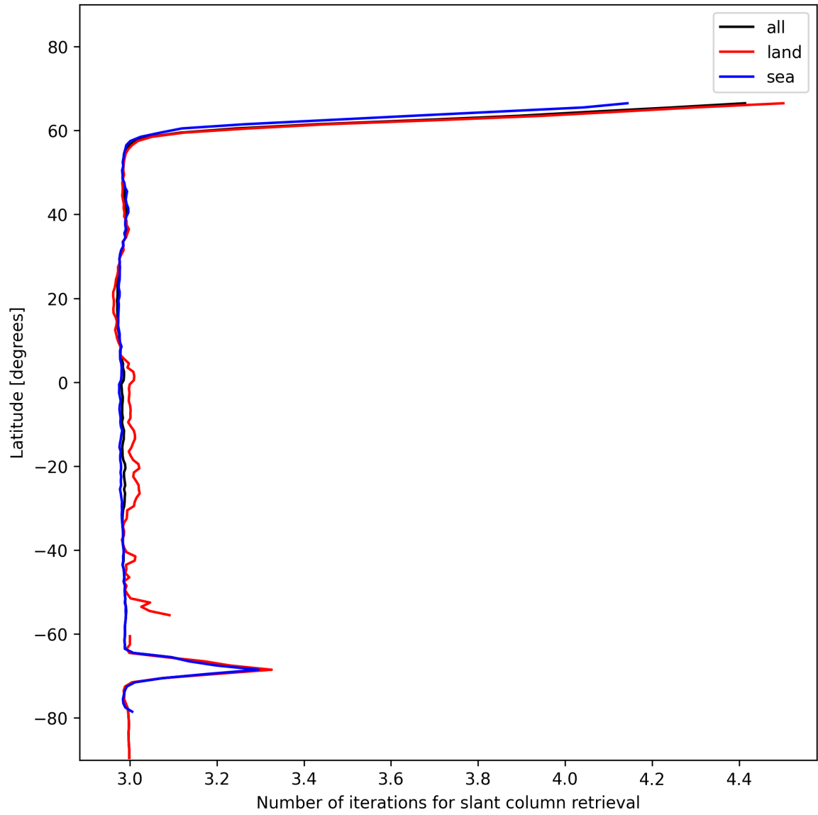
Figure 21: Zonal average of “Number of iterations for slant column retrieval” for 2025-01-03 to 2025-01-04.
