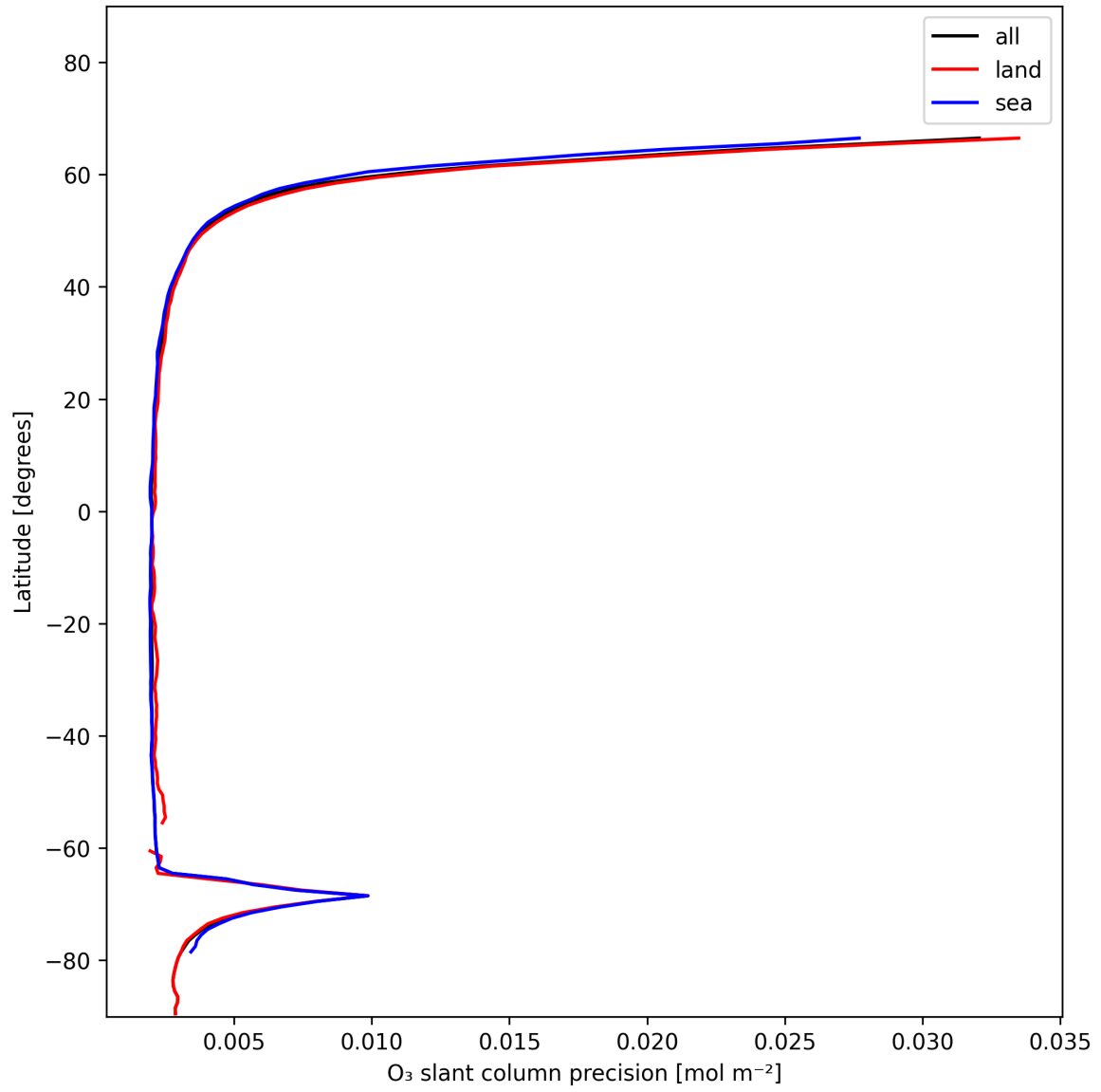
Figure 20: Zonal average of “O 3 slant column precision” for 2025-01-03 to 2025-01-04.
