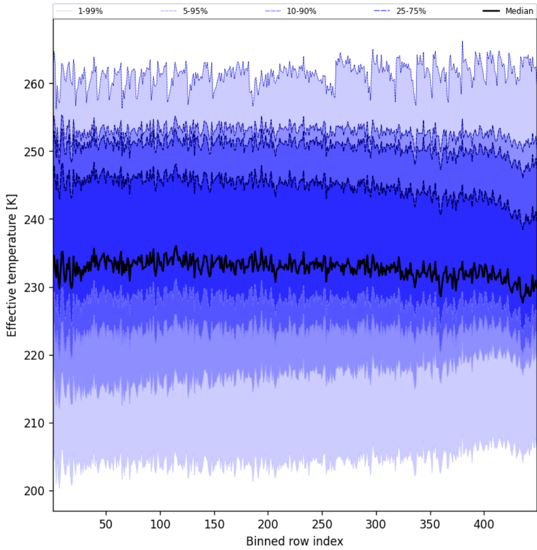
Figure 50: Along track statistics of “Effective temperature” for 2025-01-03 to 2025-01-04
