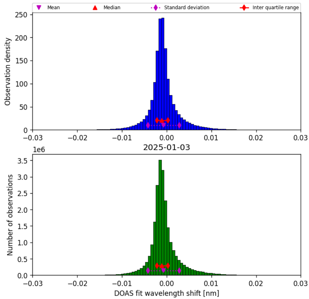
Figure 35: Histogram of “DOAS fit wavelength shift” for 2025-01-03 to 2025-01-04
