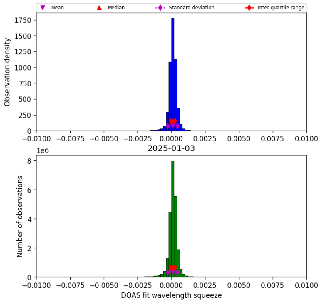
Figure 36: Histogram of “DOAS fit wavelength squeeze” for 2025-01-03 to 2025-01-04
