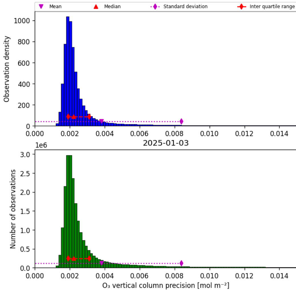
Figure 30: Histogram of “O 3 vertical column precision” for 2025-01-03 to 2025-01-04
