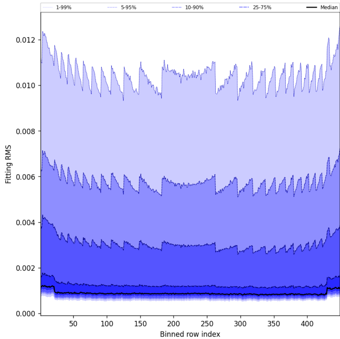
Figure 46: Along track statistics of “Fitting RMS” for 2025-01-03 to 2025-01-04
