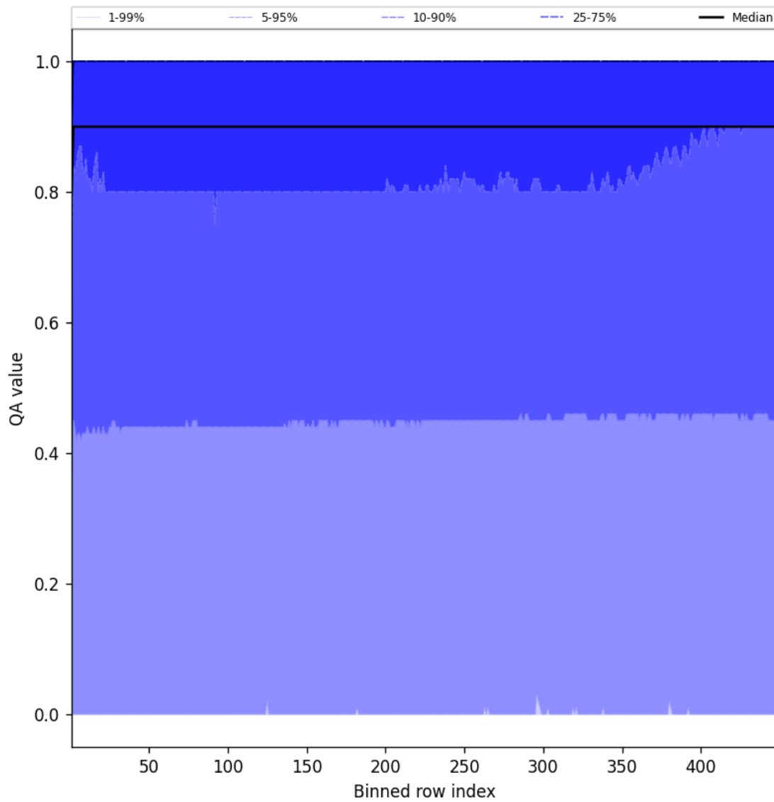
Figure 40: Along track statistics of “QA value” for 2025-01-03 to 2025-01-04
