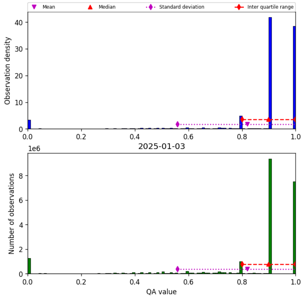
Figure 28: Histogram of “QA value” for 2025-01-03 to 2025-01-04
