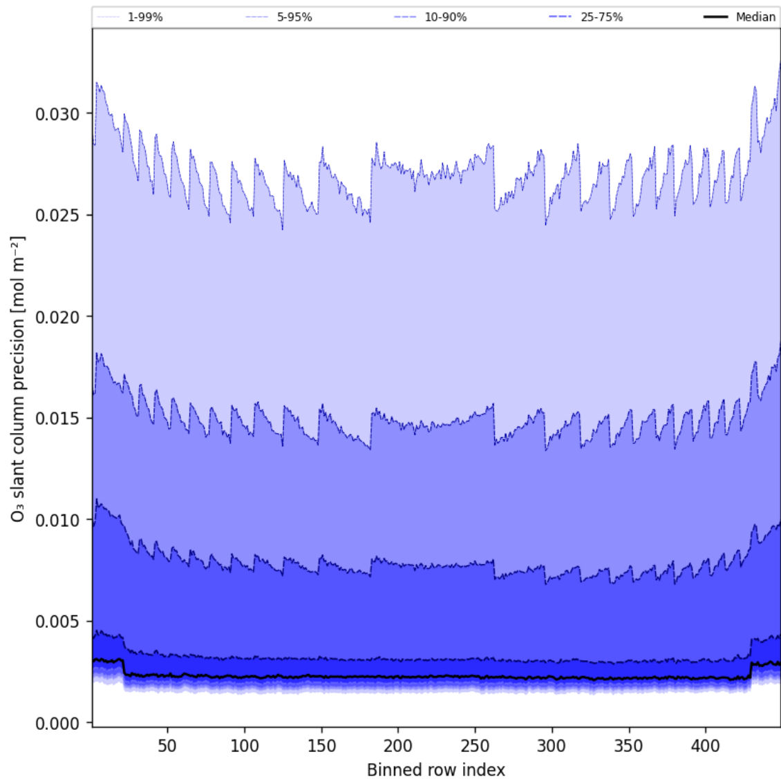
Figure 44: Along track statistics of “O 3 slant column precision” for 2025-01-03 to 2025-01-04
