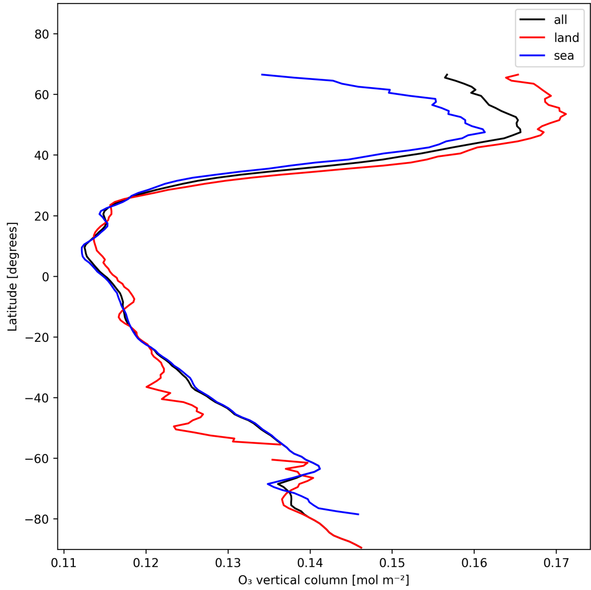
Figure 17: Zonal average of “O 3 vertical column” for 2025-01-04 to 2025-01-04.
