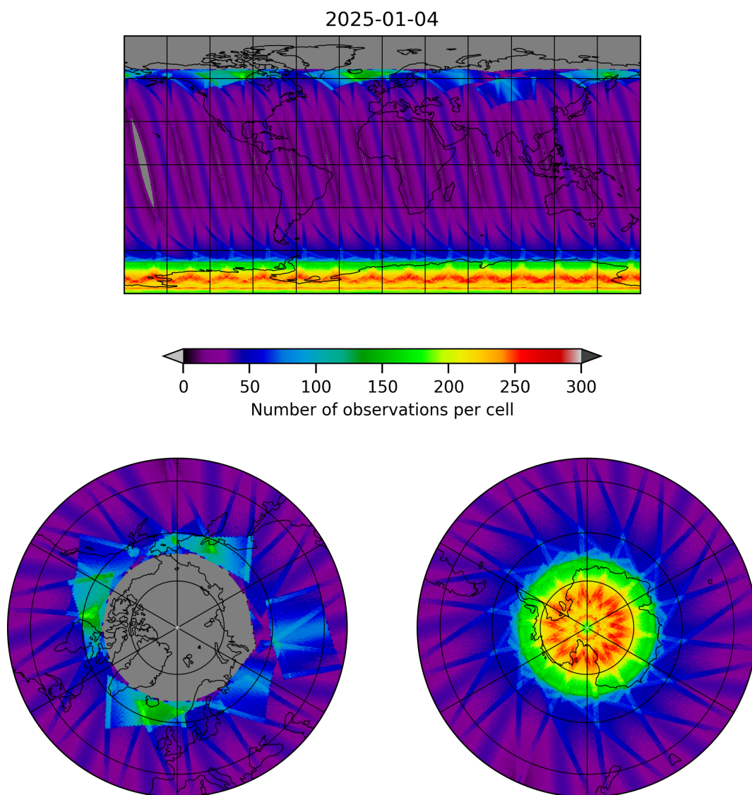
Figure 15: Map of the number of observations for 2025-01-04 to 2025-01-04
