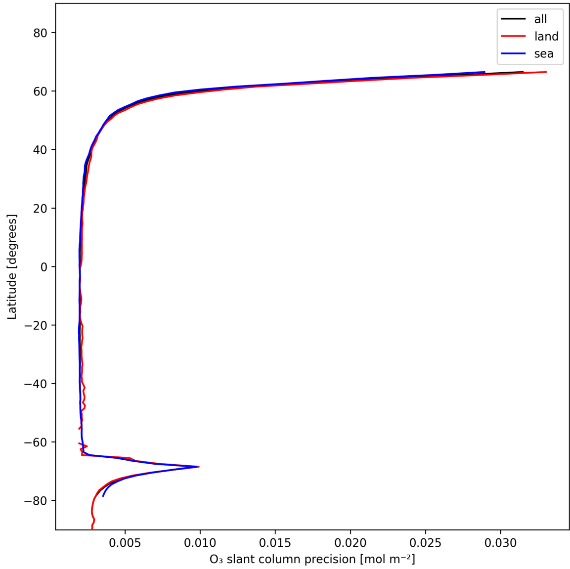
Figure 20: Zonal average of “O 3 slant column precision” for 2025-01-04 to 2025-01-04.
