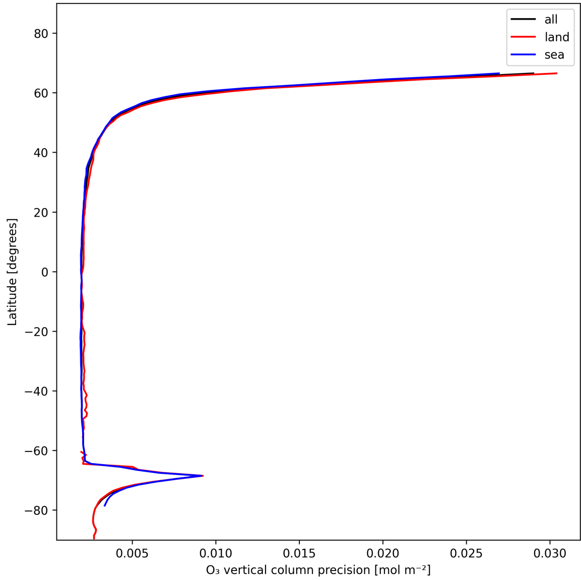
Figure 18: Zonal average of “O 3 vertical column precision” for 2025-01-04 to 2025-01-04.
