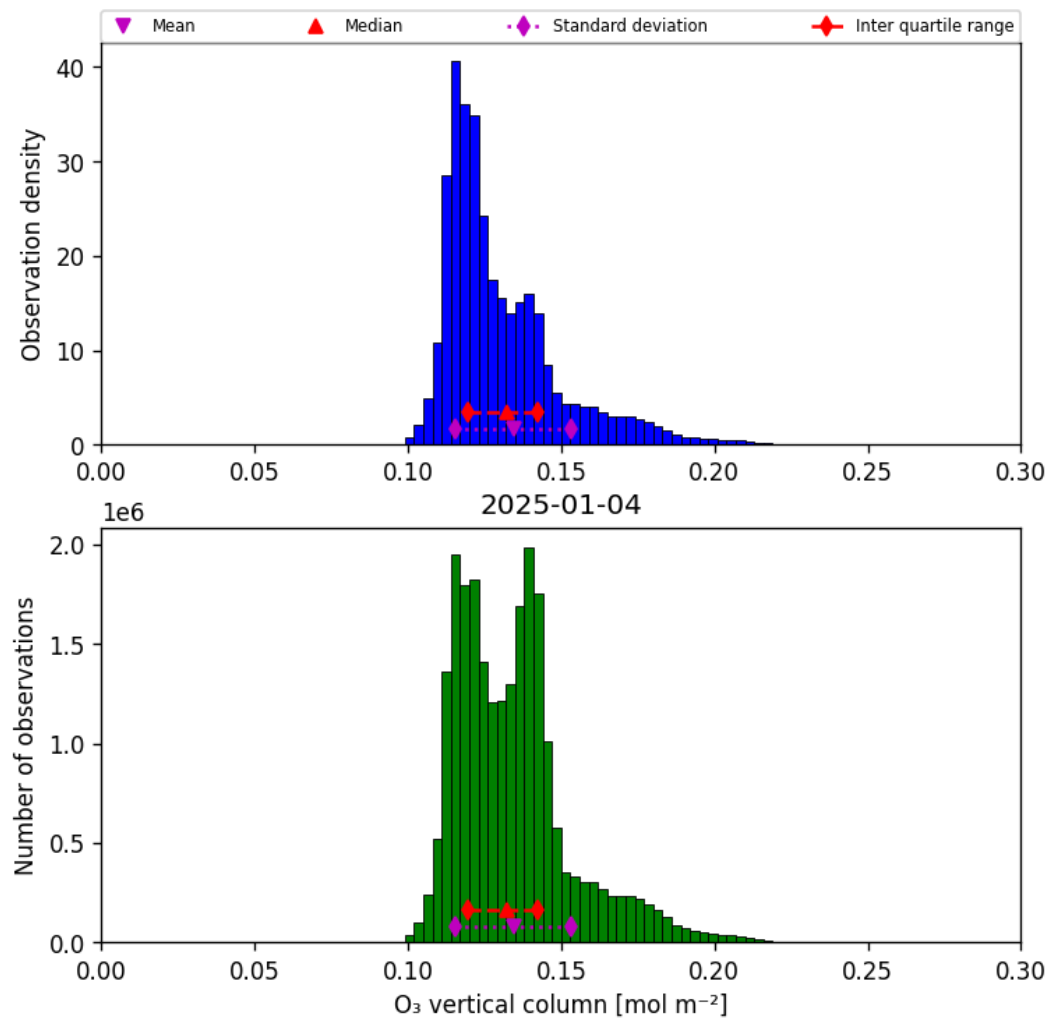
Figure 29: Histogram of “O 3 vertical column” for 2025-01-04 to 2025-01-04
