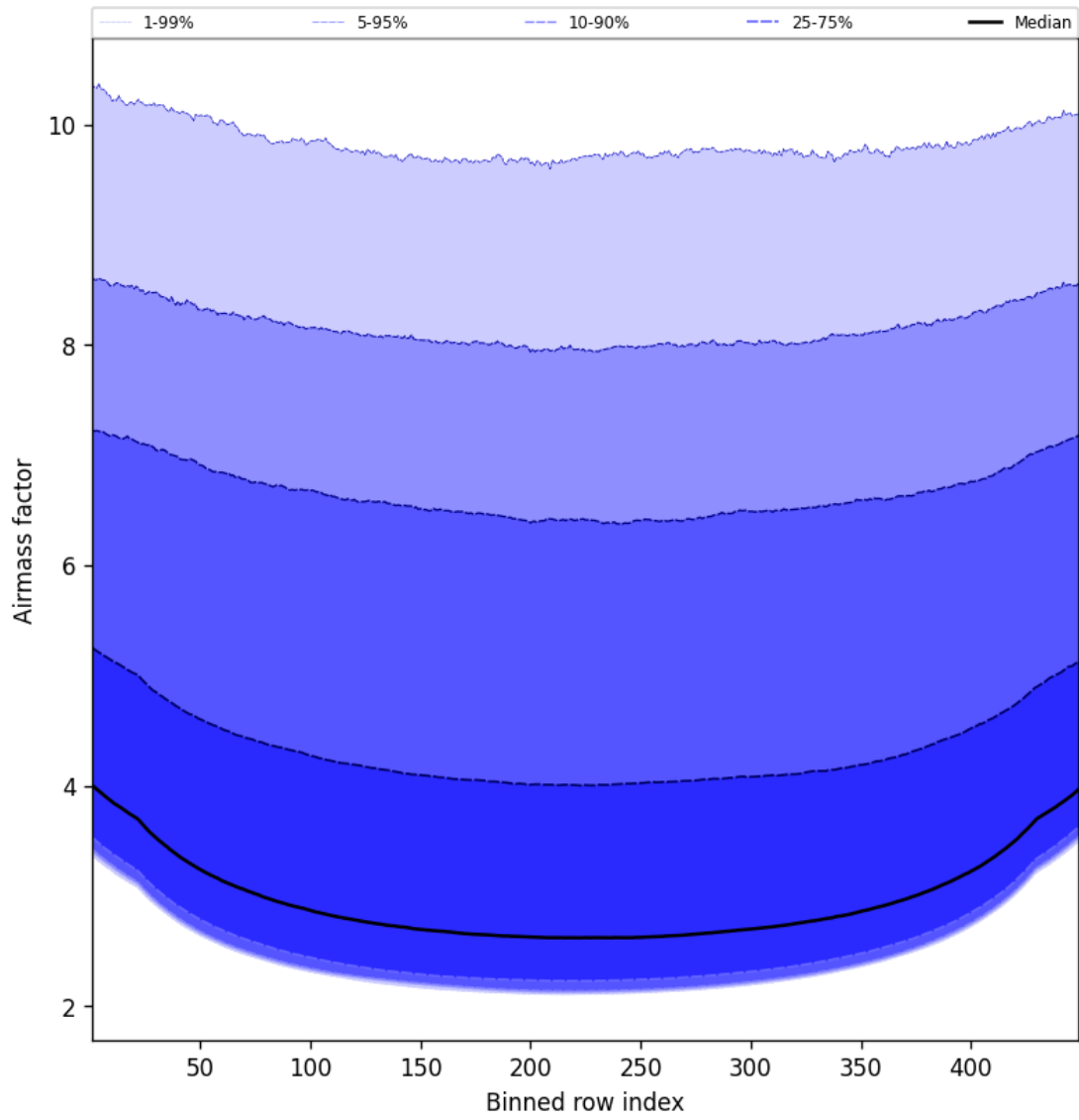
Figure 49: Along track statistics of “Airmass factor” for 2025-01-04 to 2025-01-04
