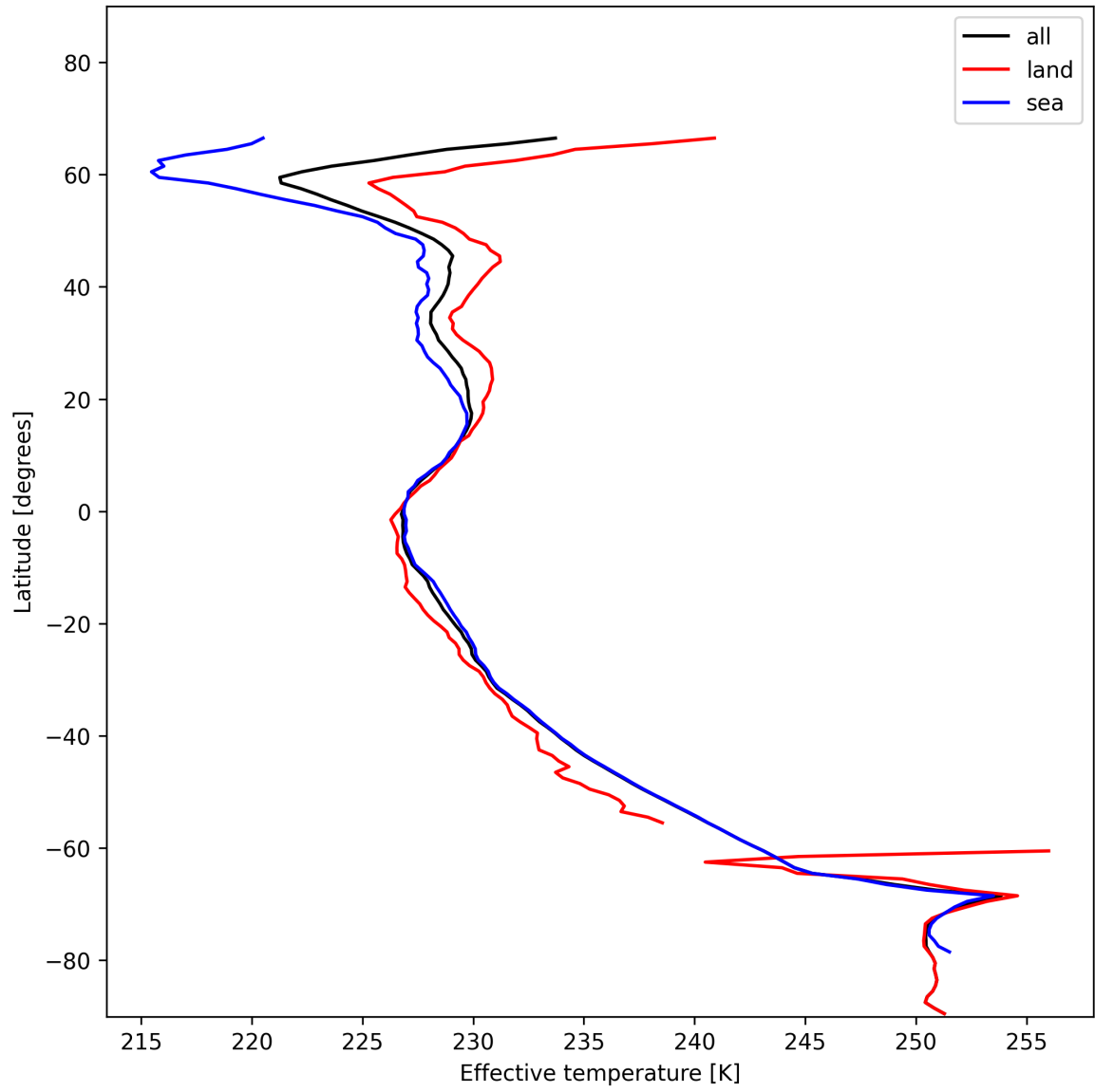
Figure 26: Zonal average of “Effective temperature” for 2025-01-04 to 2025-01-04.
