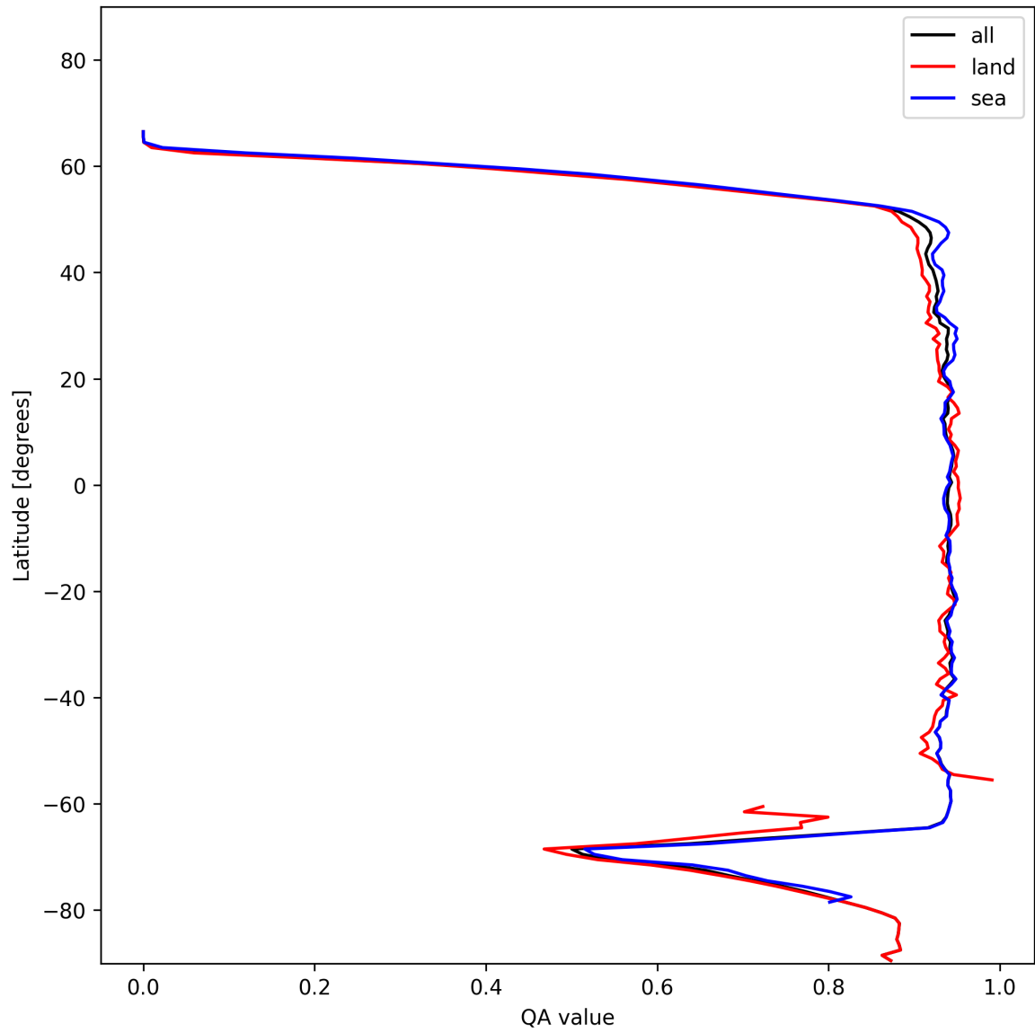
Figure 16: Zonal average of "QA value" for 2025-01-04 to 2025-01-04.
