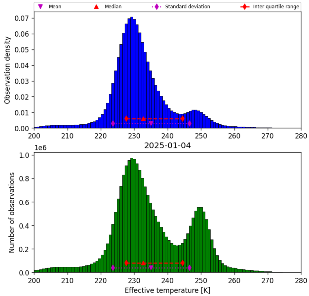
Figure 38: Histogram of “Effective temperature” for 2025-01-04 to 2025-01-04
