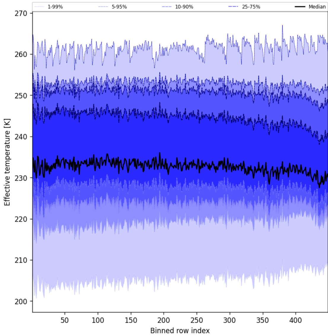
Figure 50: Along track statistics of “Effective temperature” for 2025-01-04 to 2025-01-04
