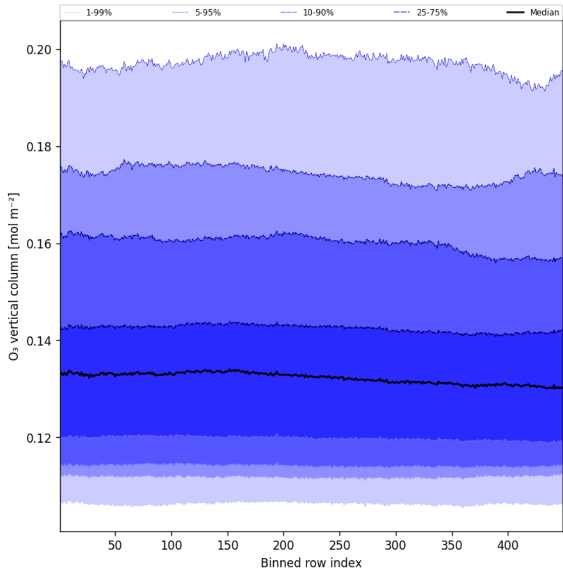
Figure 41: Along track statistics of “O 3 vertical column” for 2025-01-04 to 2025-01-04
