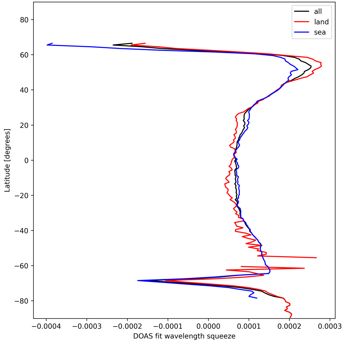
Figure 24: Zonal average of “DOAS fit wavelength squeeze” for 2025-01-04 to 2025-01-04.
