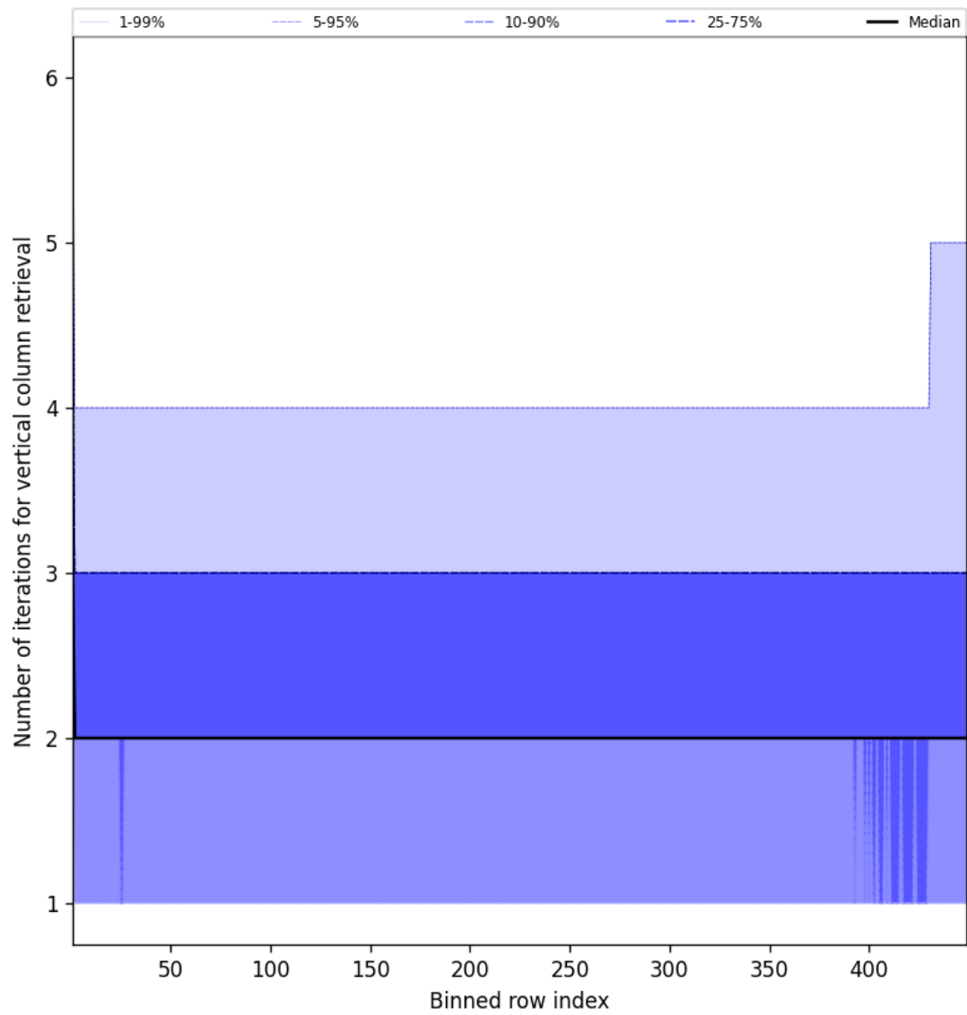
Figure 51: Along track statistics of “Number of iterations for vertical column retrieval” for 2025-01-04 to 2025-01-04
