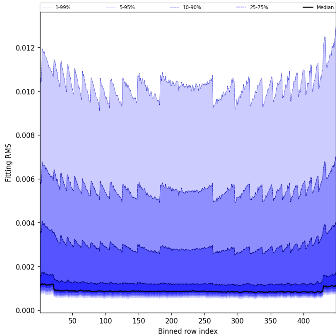
Figure 46: Along track statistics of “Fitting RMS” for 2025-01-04 to 2025-01-04
