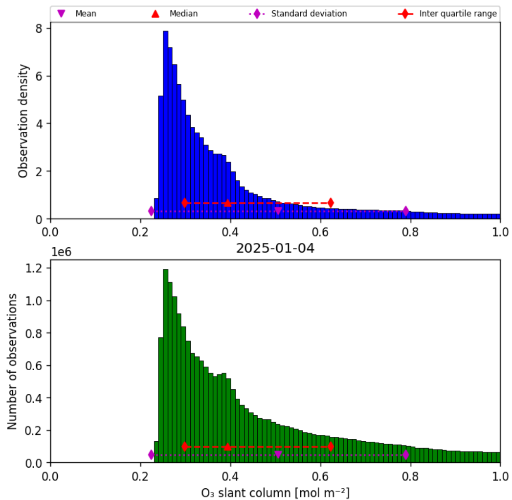
Figure 31: Histogram of “O 3 slant column” for 2025-01-04 to 2025-01-04
