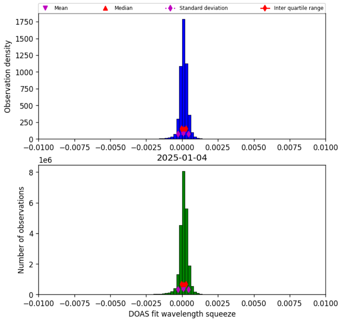
Figure 36: Histogram of “DOAS fit wavelength squeeze” for 2025-01-04 to 2025-01-04
