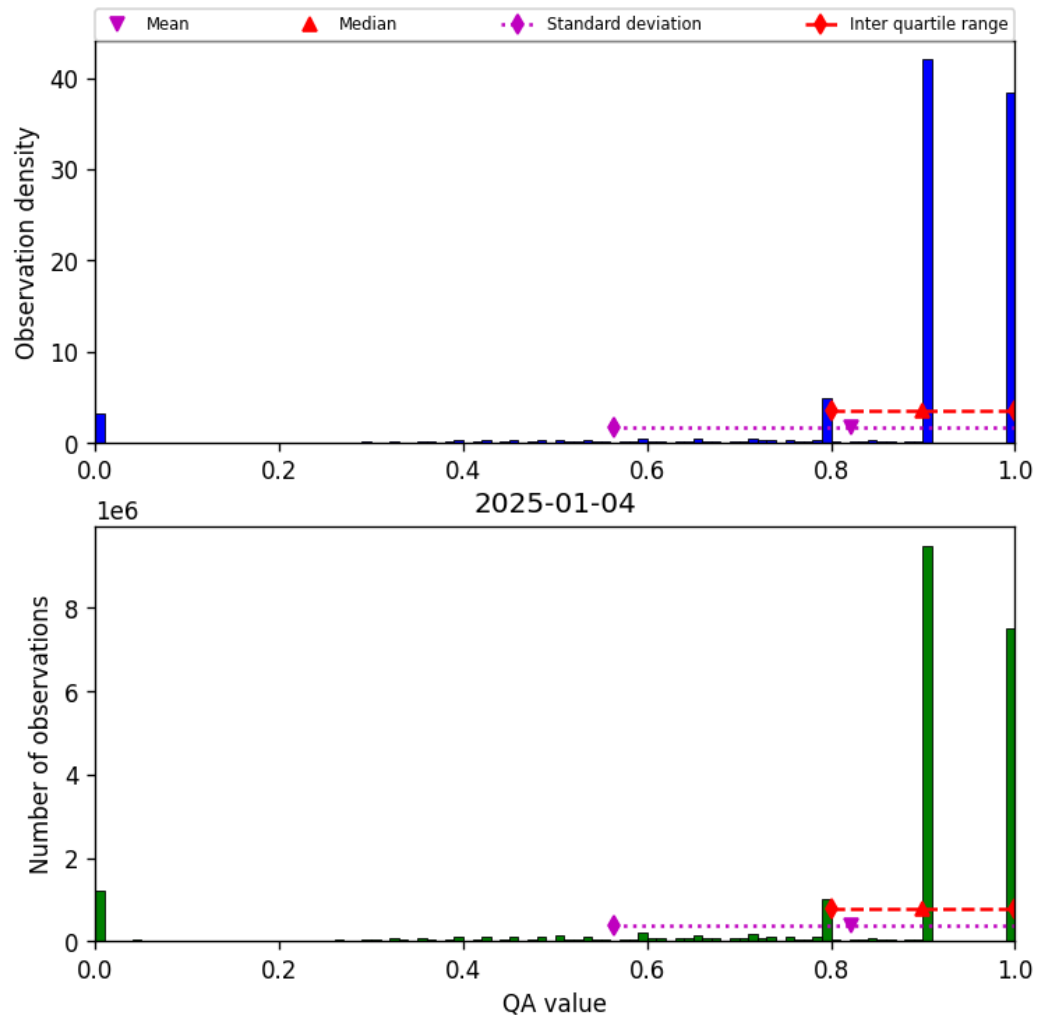
Figure 28: Histogram of “QA value” for 2025-01-04 to 2025-01-04
