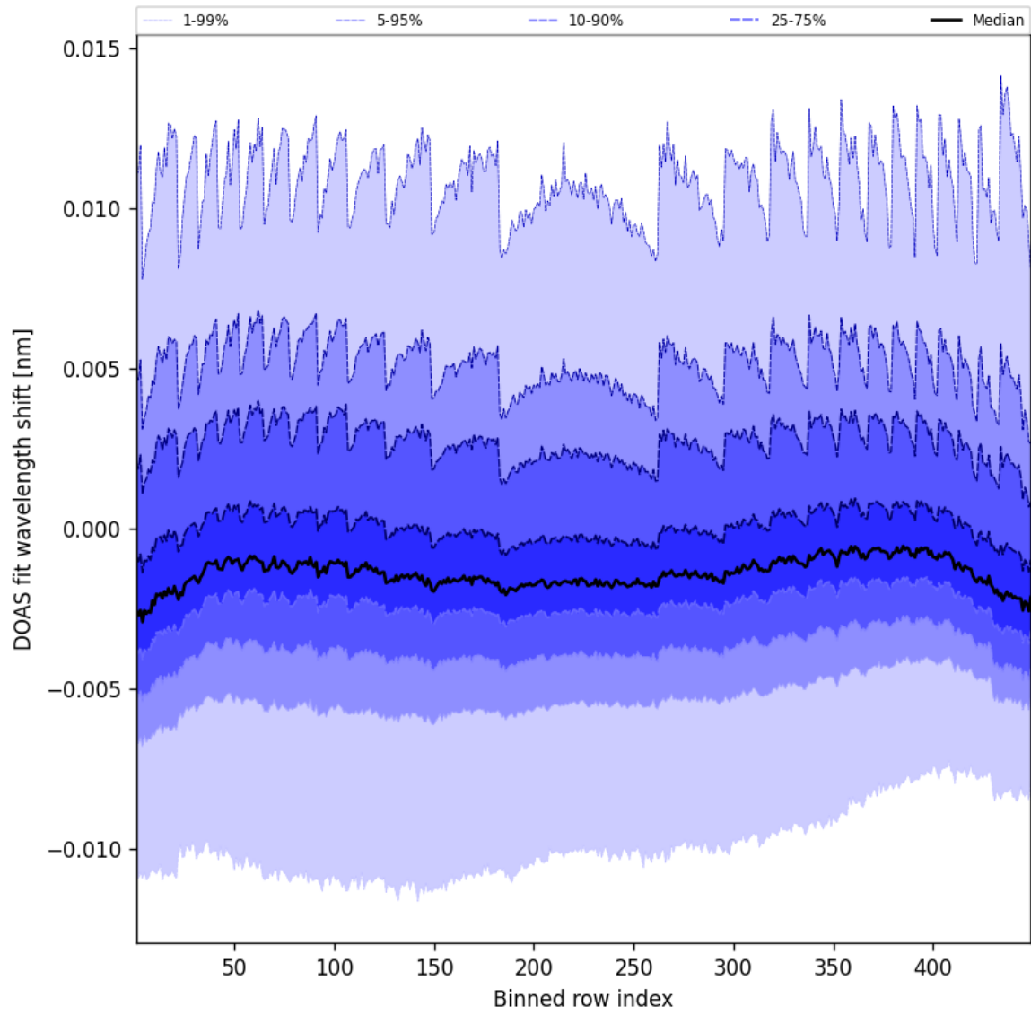
Figure 47: Along track statistics of “DOAS fit wavelength shift” for 2025-01-04 to 2025-01-04
