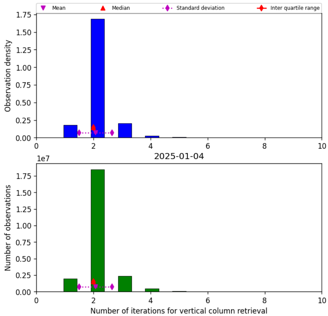
Figure 39: Histogram of “Number of iterations for vertical column retrieval” for 2025-01-04 to 2025-01-04
