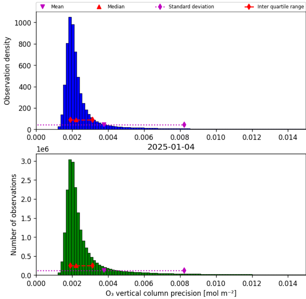
Figure 30: Histogram of “O 3 vertical column precision” for 2025-01-04 to 2025-01-04
