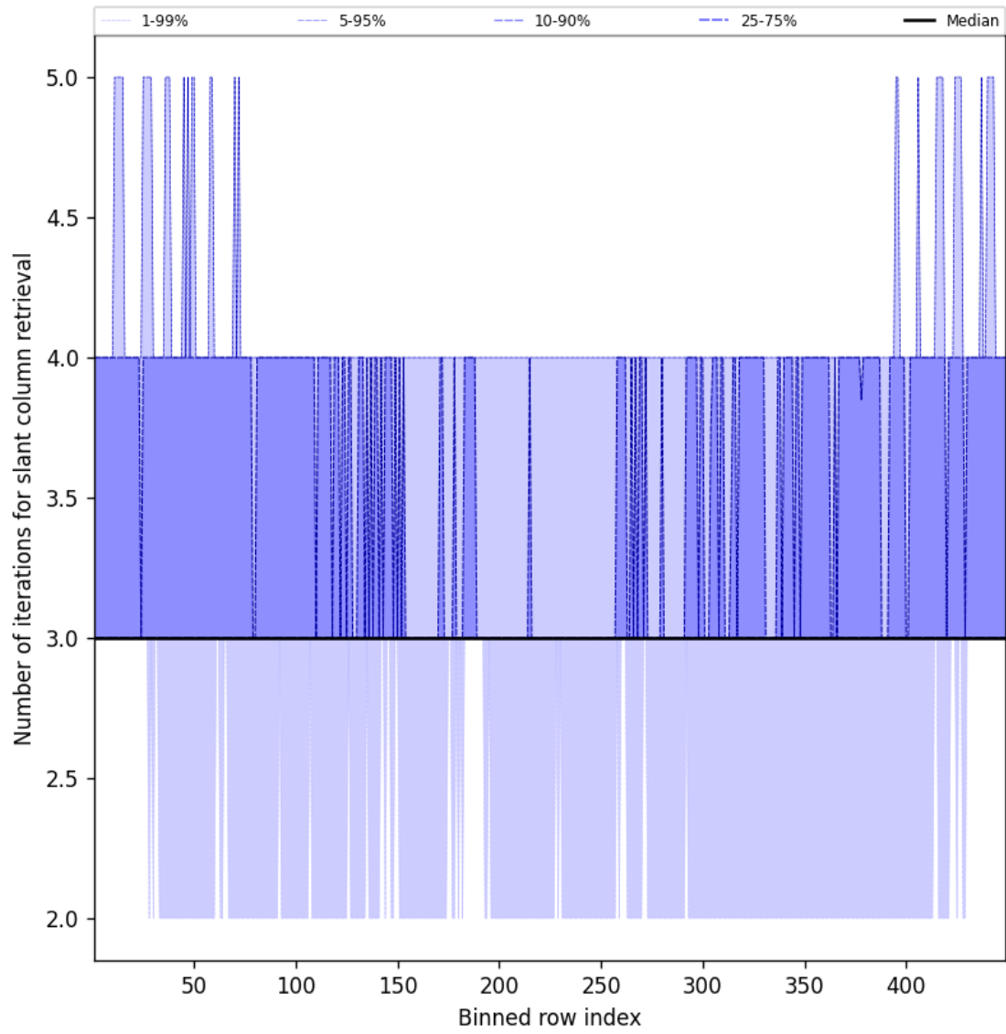
Figure 45: Along track statistics of “Number of iterations for slant column retrieval” for 2025-01-04 to 2025-01-04
