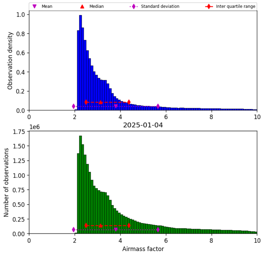
Figure 37: Histogram of “Airmass factor” for 2025-01-04 to 2025-01-04
