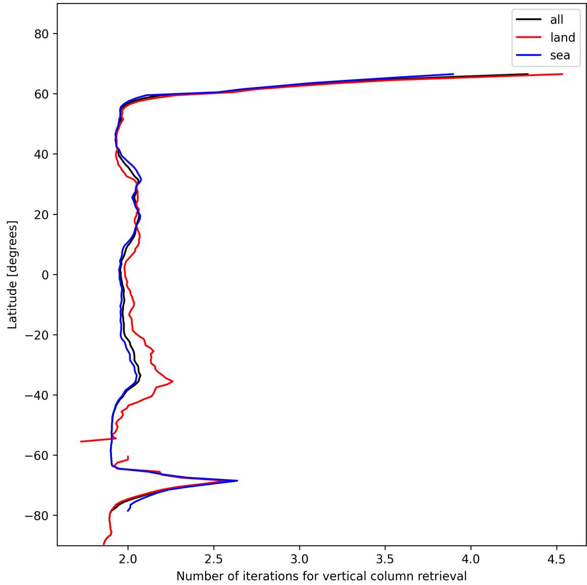
Figure 27: Zonal average of “Number of iterations for vertical column retrieval” for 2025-01-04 to 2025-01-04.
