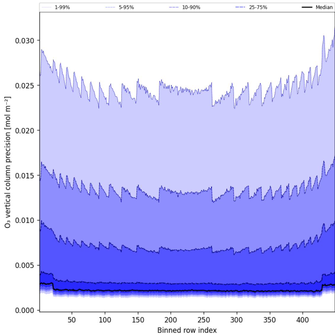
Figure 42: Along track statistics of “O 3 vertical column precision” for 2025-01-04 to 2025-01-04
