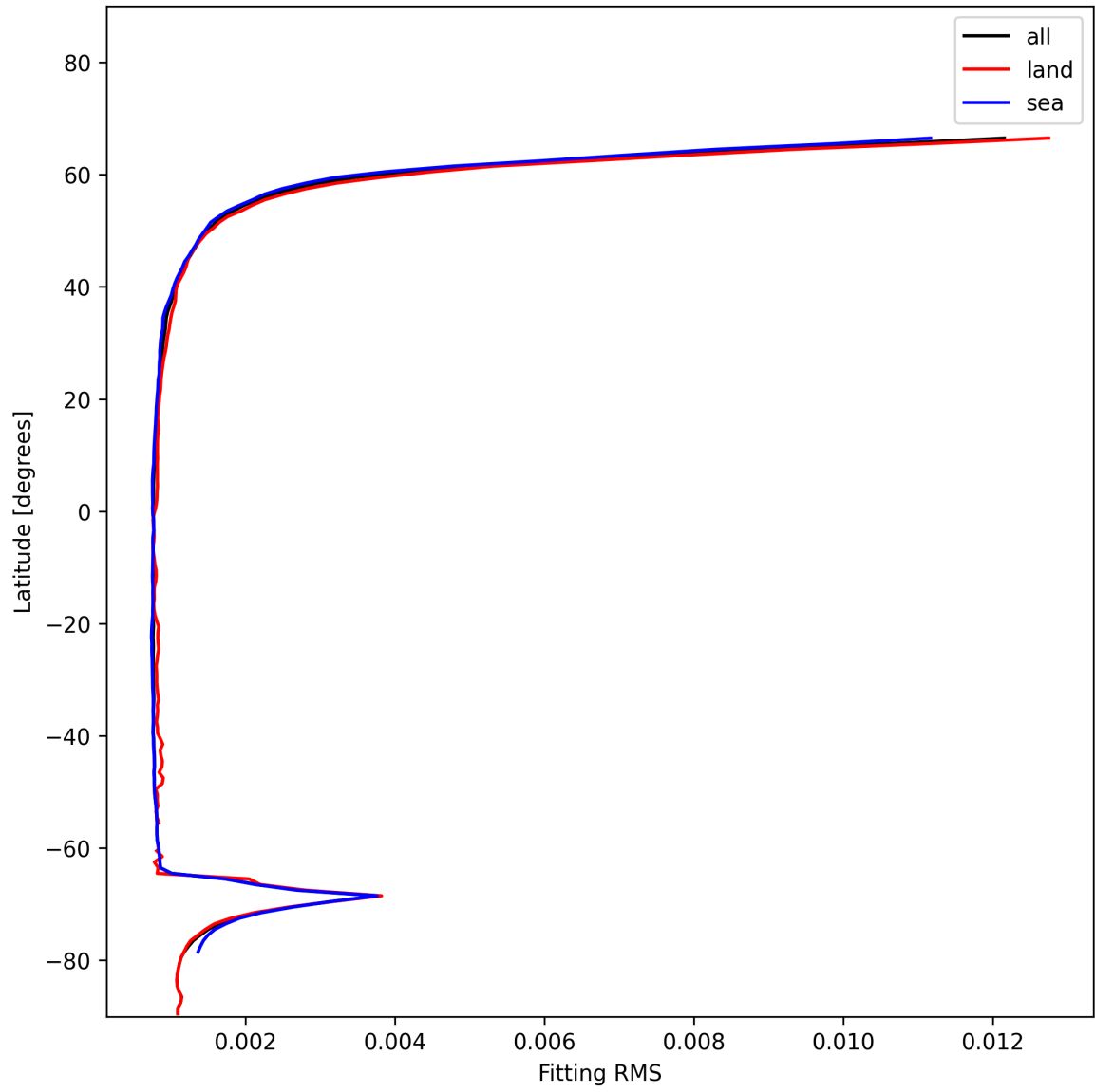
Figure 22: Zonal average of “Fitting RMS” for 2025-01-04 to 2025-01-04.
