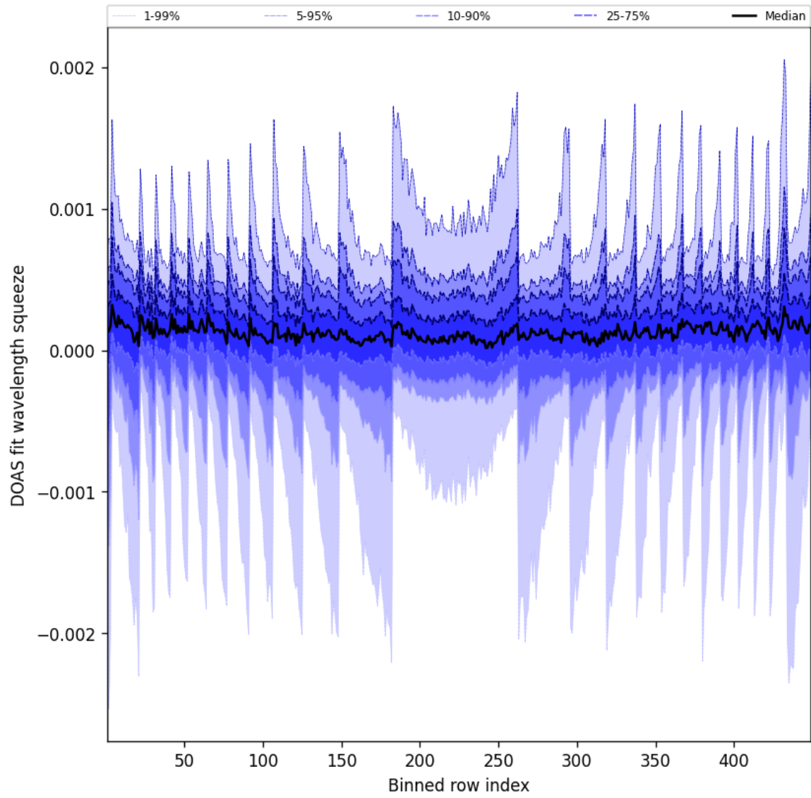
Figure 48: Along track statistics of “DOAS fit wavelength squeeze” for 2025-01-04 to 2025-01-04
