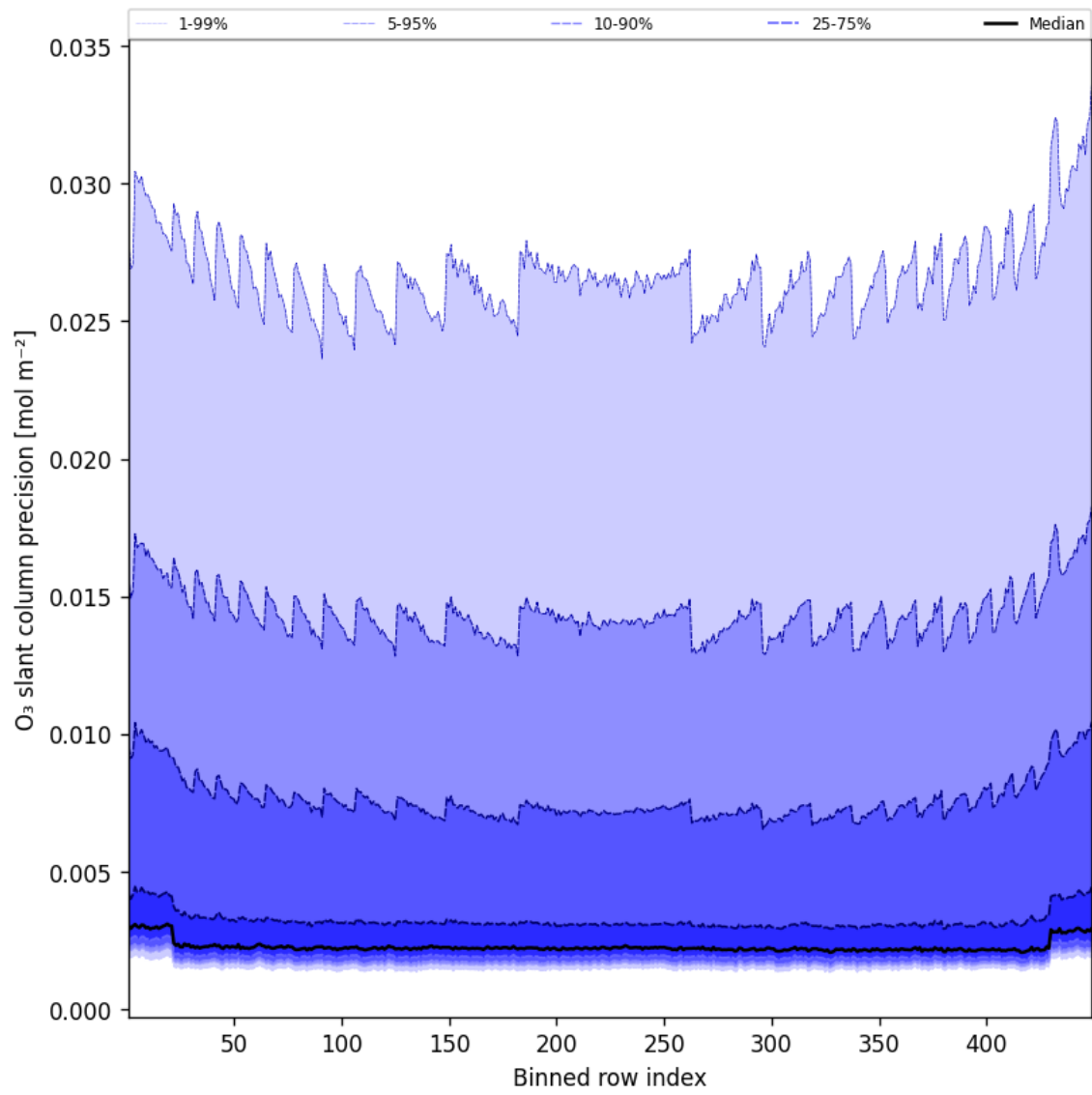
Figure 44: Along track statistics of “O 3 slant column precision” for 2025-01-04 to 2025-01-04
