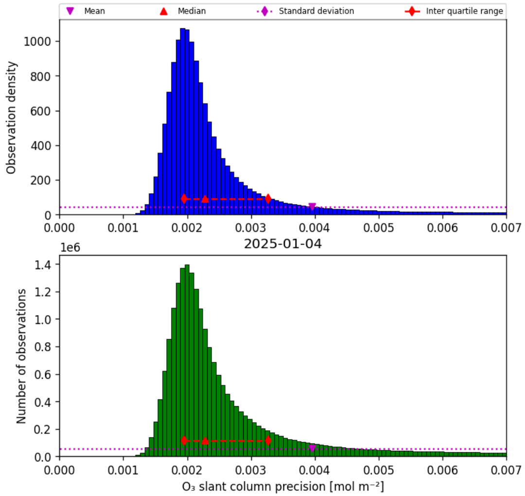
Figure 32: Histogram of “O 3 slant column precision” for 2025-01-04 to 2025-01-04
