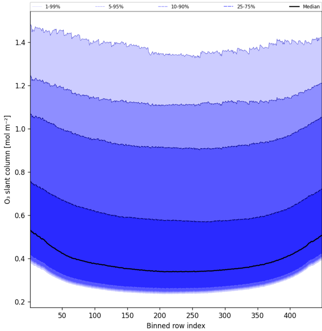
Figure 43: Along track statistics of “O 3 slant column” for 2025-01-04 to 2025-01-04
