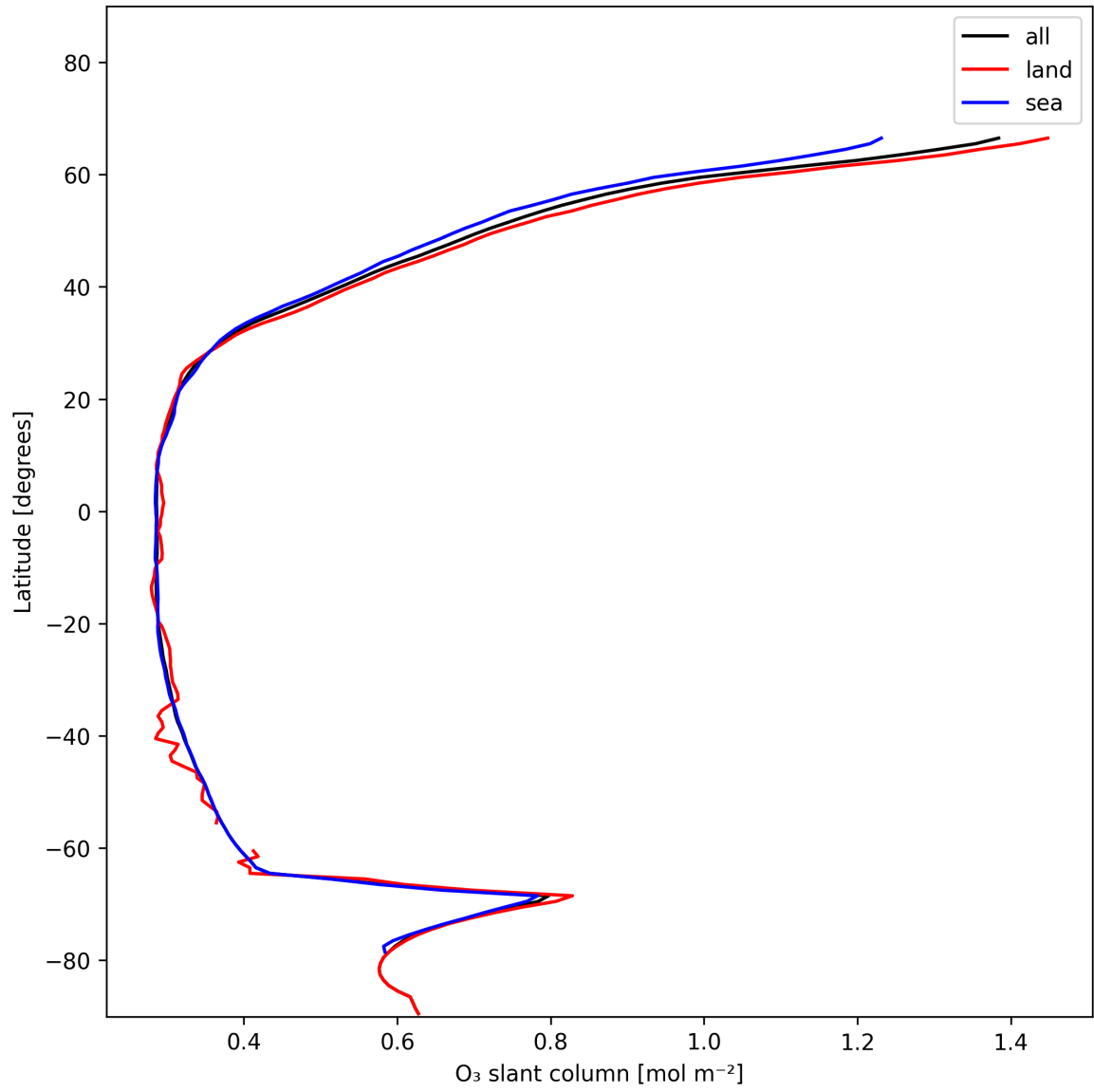
Figure 19: Zonal average of “O 3 slant column” for 2025-01-04 to 2025-01-04.
