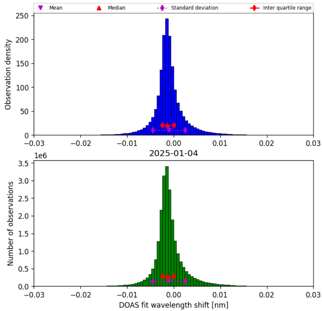
Figure 35: Histogram of “DOAS fit wavelength shift” for 2025-01-04 to 2025-01-04
