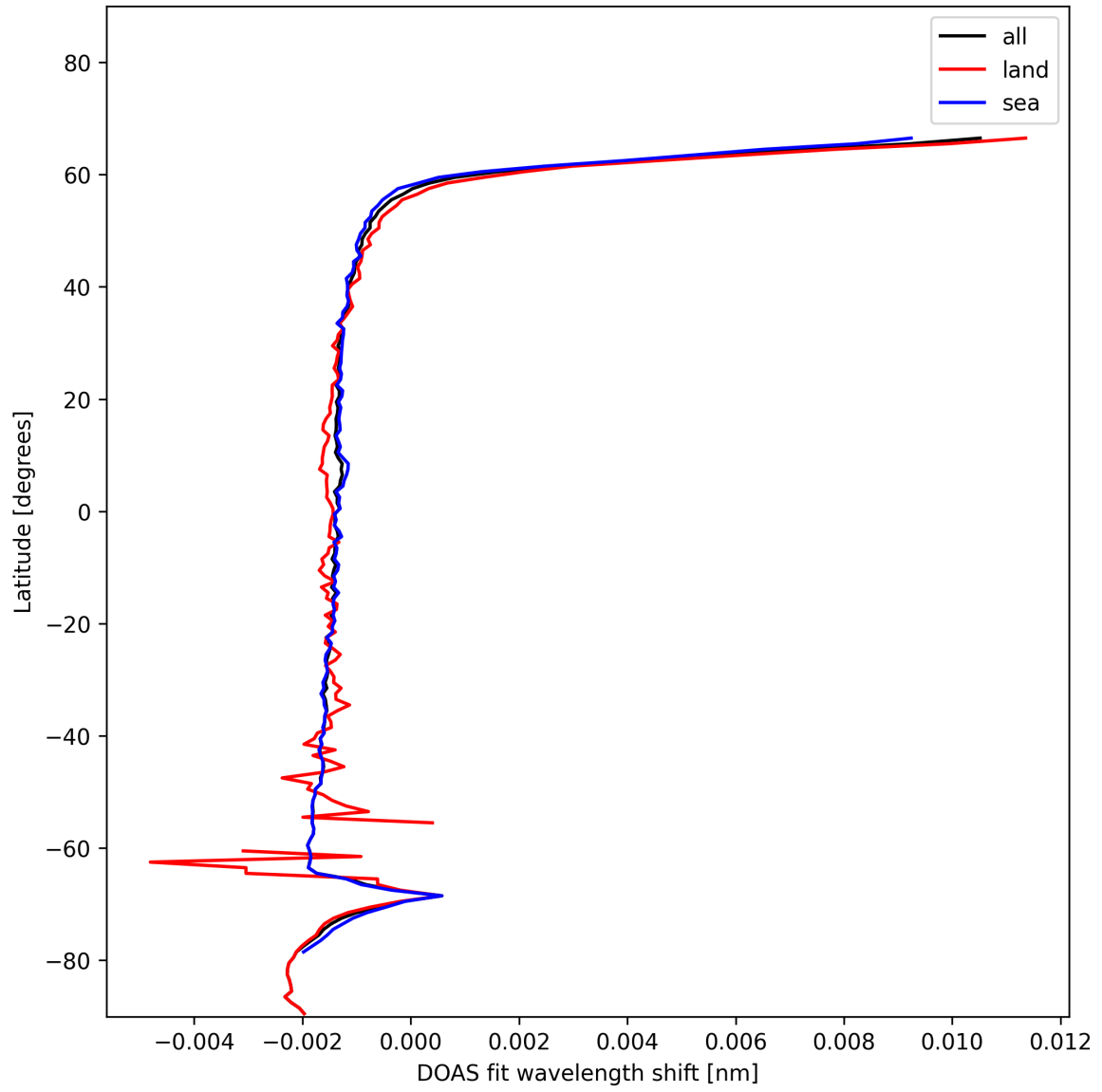
Figure 23: Zonal average of “DOAS fit wavelength shift” for 2025-01-04 to 2025-01-04.
