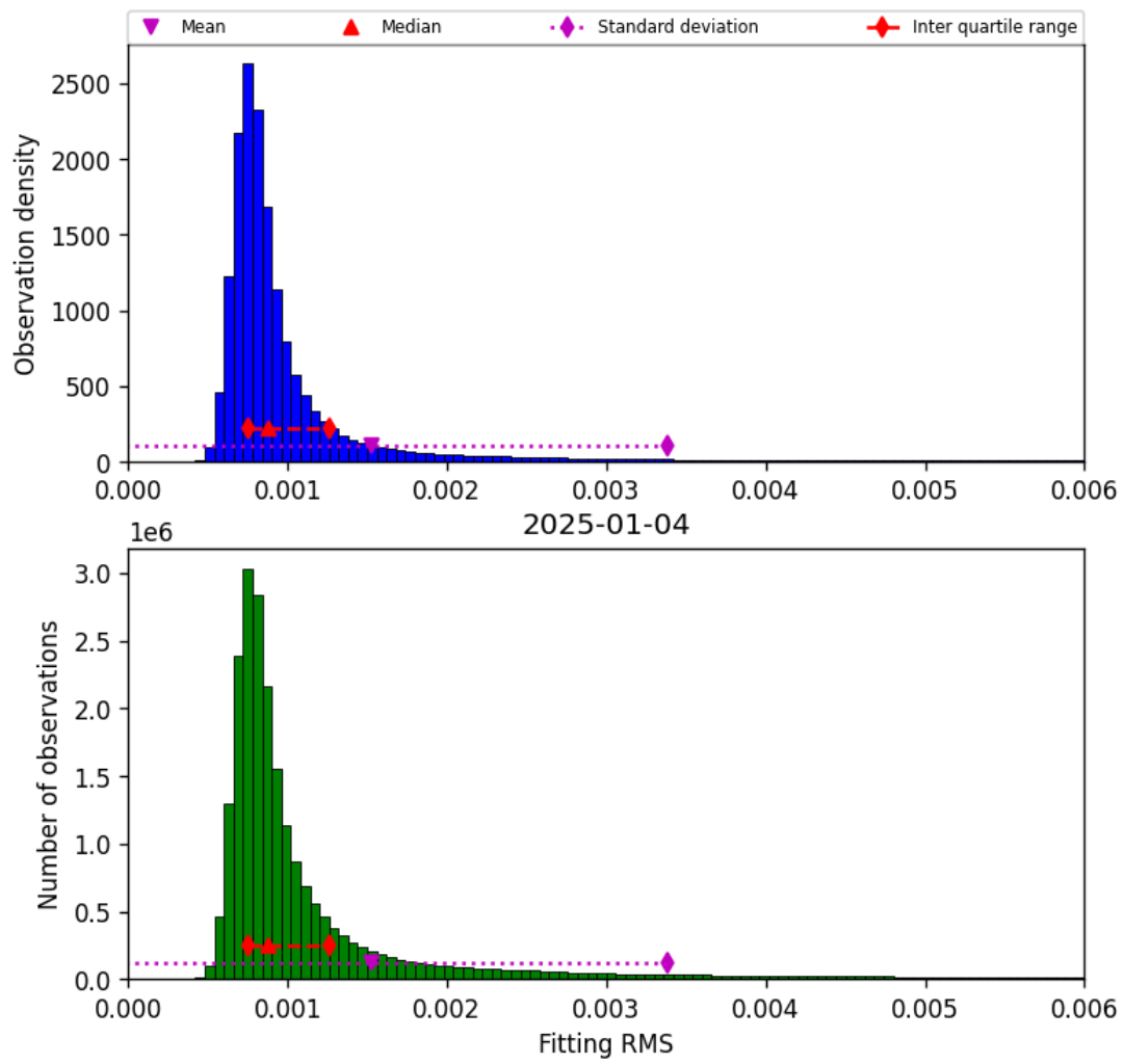
Figure 34: Histogram of “Fitting RMS” for 2025-01-04 to 2025-01-04
