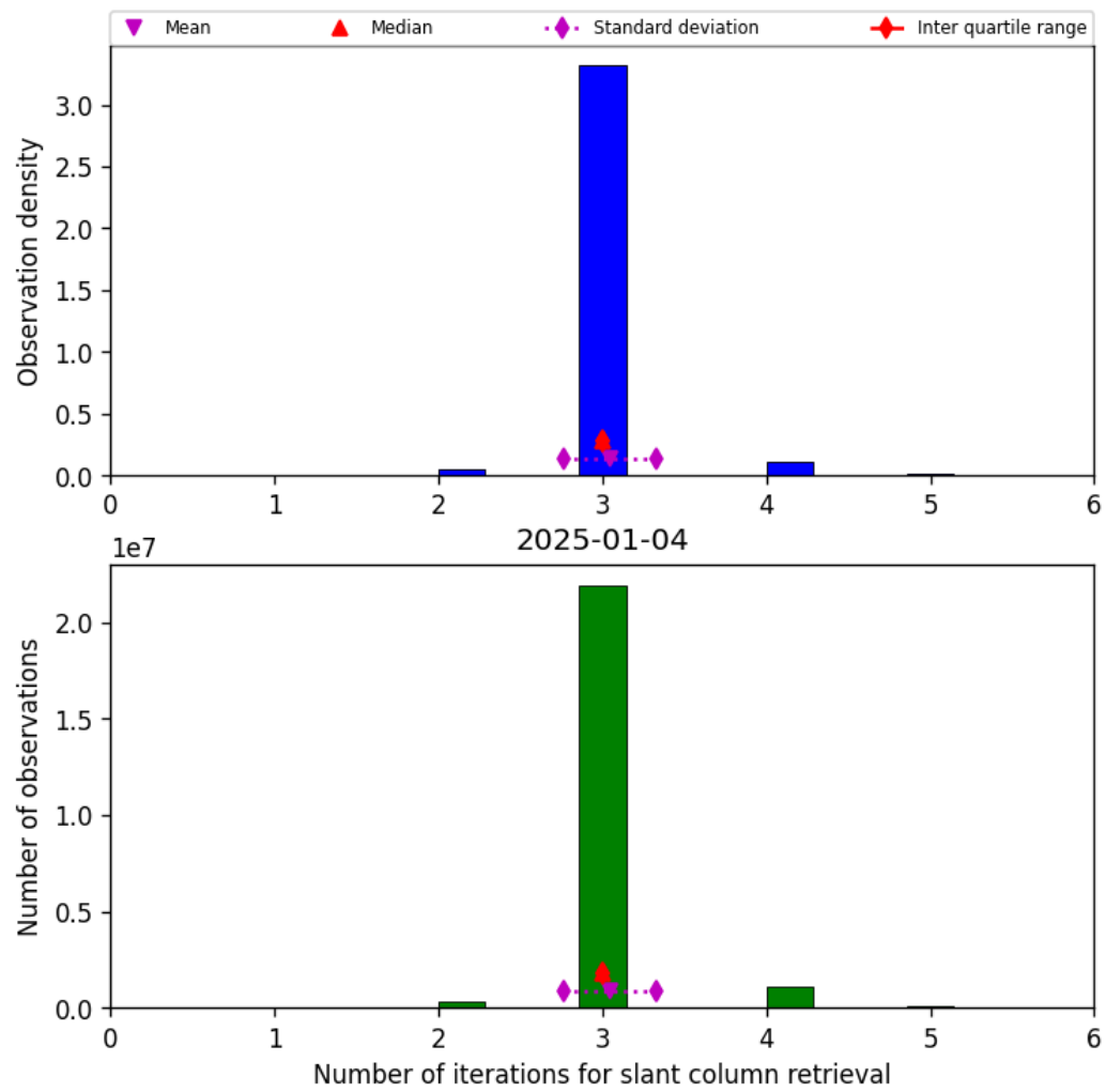
Figure 33: Histogram of “Number of iterations for slant column retrieval” for 2025-01-04 to 2025-01-04
