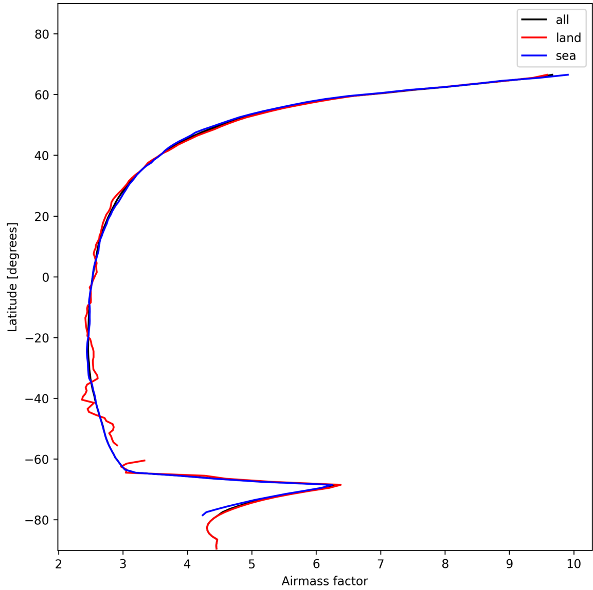
Figure 25: Zonal average of “Airmass factor” for 2025-01-04 to 2025-01-04.
