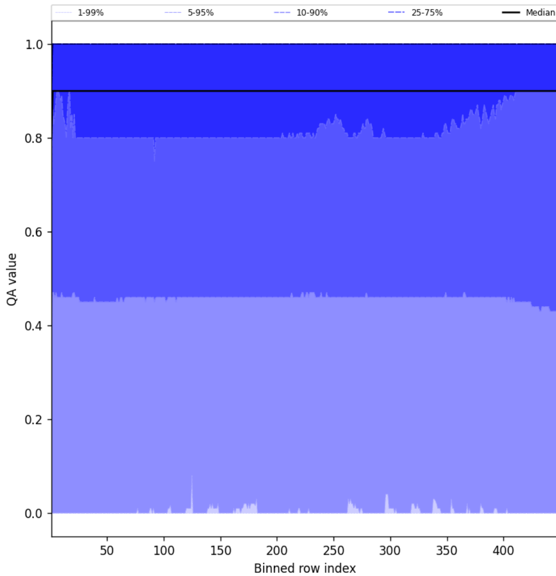
Figure 40: Along track statistics of “QA value” for 2025-01-04 to 2025-01-04
