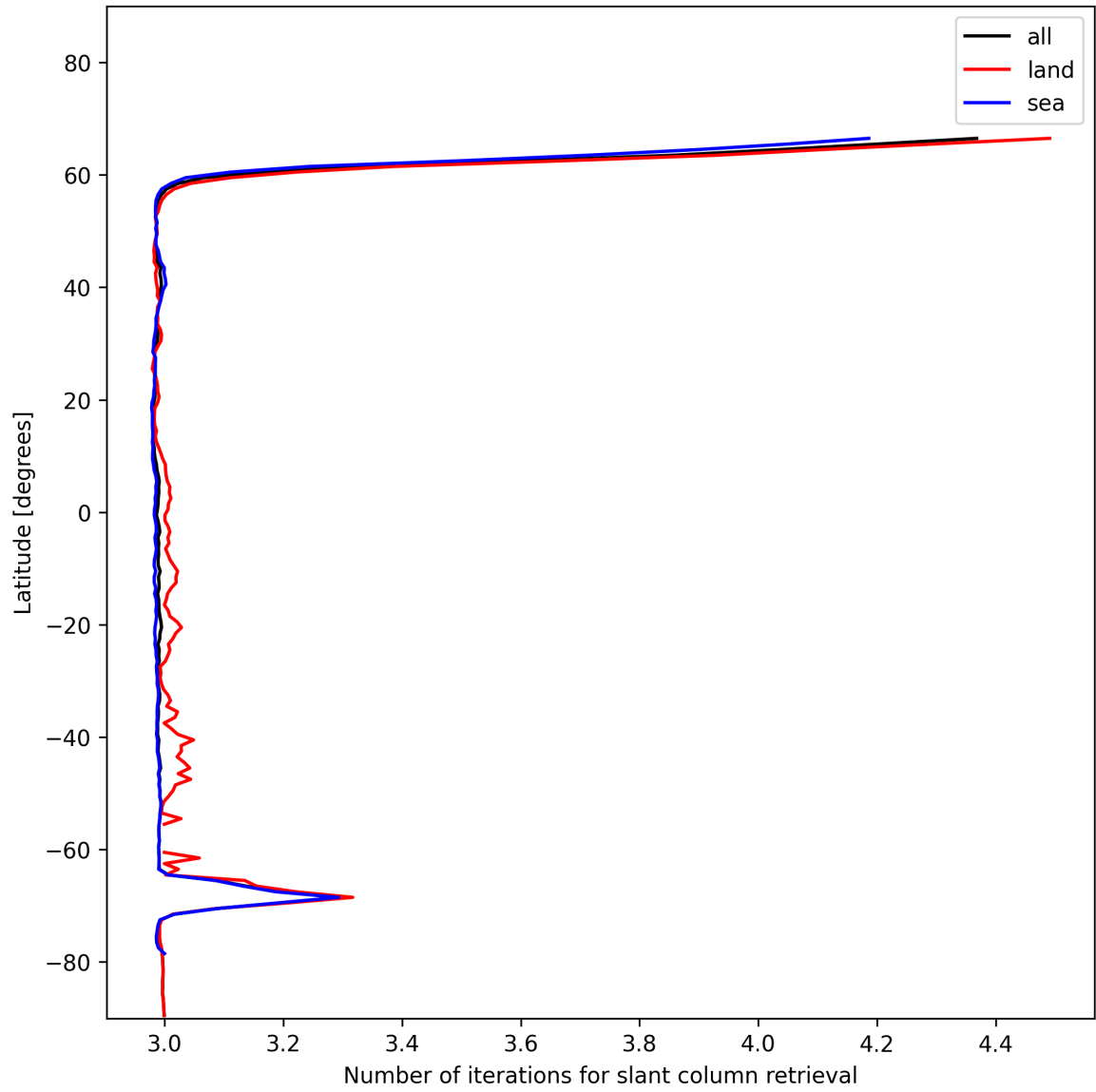
Figure 21: Zonal average of “Number of iterations for slant column retrieval” for 2025-01-04 to 2025-01-04.
