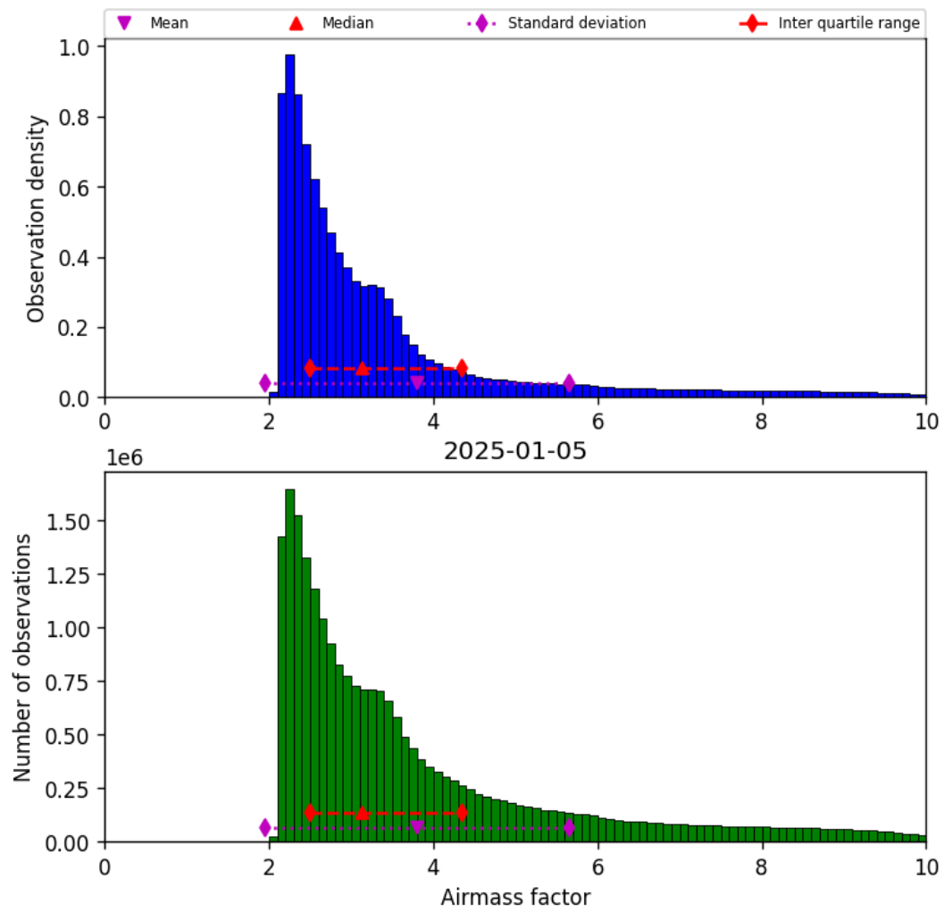
Figure 37: Histogram of “Airmass factor” for 2025-01-05 to 2025-01-05
