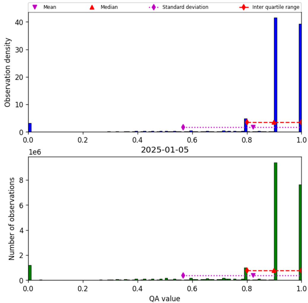
Figure 28: Histogram of “QA value” for 2025-01-05 to 2025-01-05
