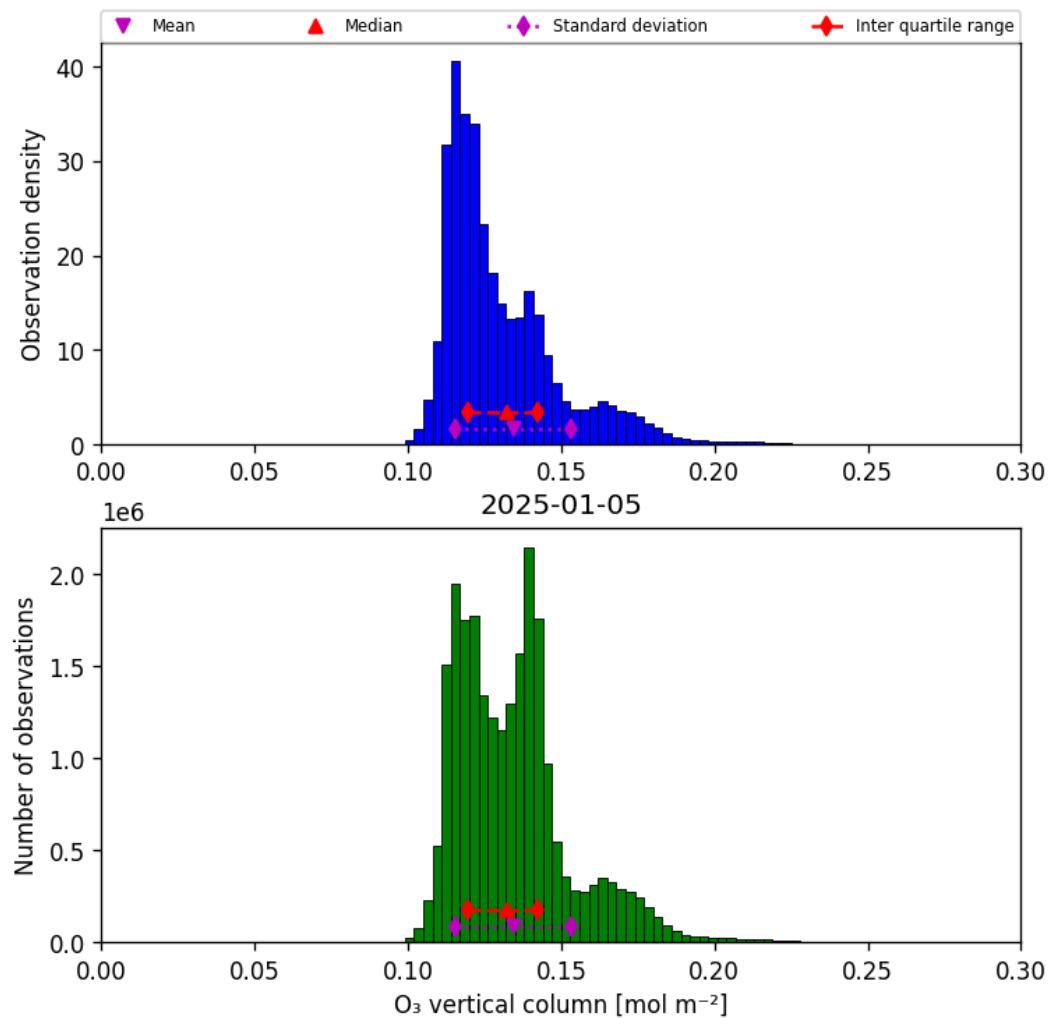
Figure 29: Histogram of “O 3 vertical column” for 2025-01-05 to 2025-01-05
