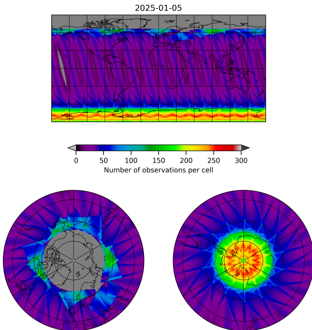
Figure 15: Map of the number of observations for 2025-01-05 to 2025-01-05
