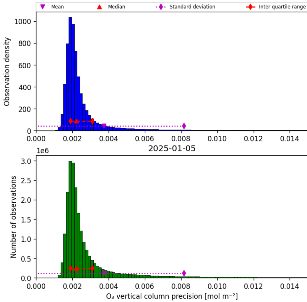
Figure 30: Histogram of “O 3 vertical column precision” for 2025-01-05 to 2025-01-05
