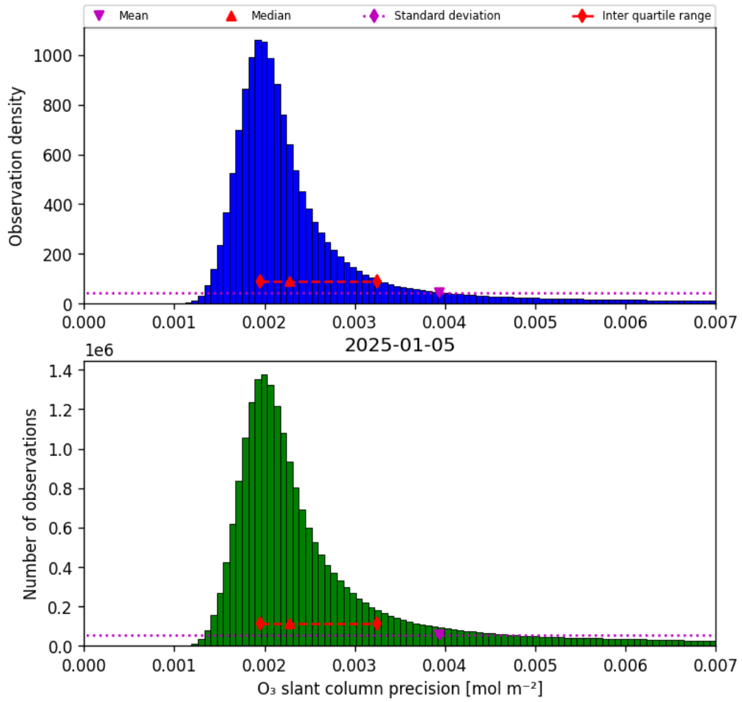
Figure 32: Histogram of “O 3 slant column precision” for 2025-01-05 to 2025-01-05
