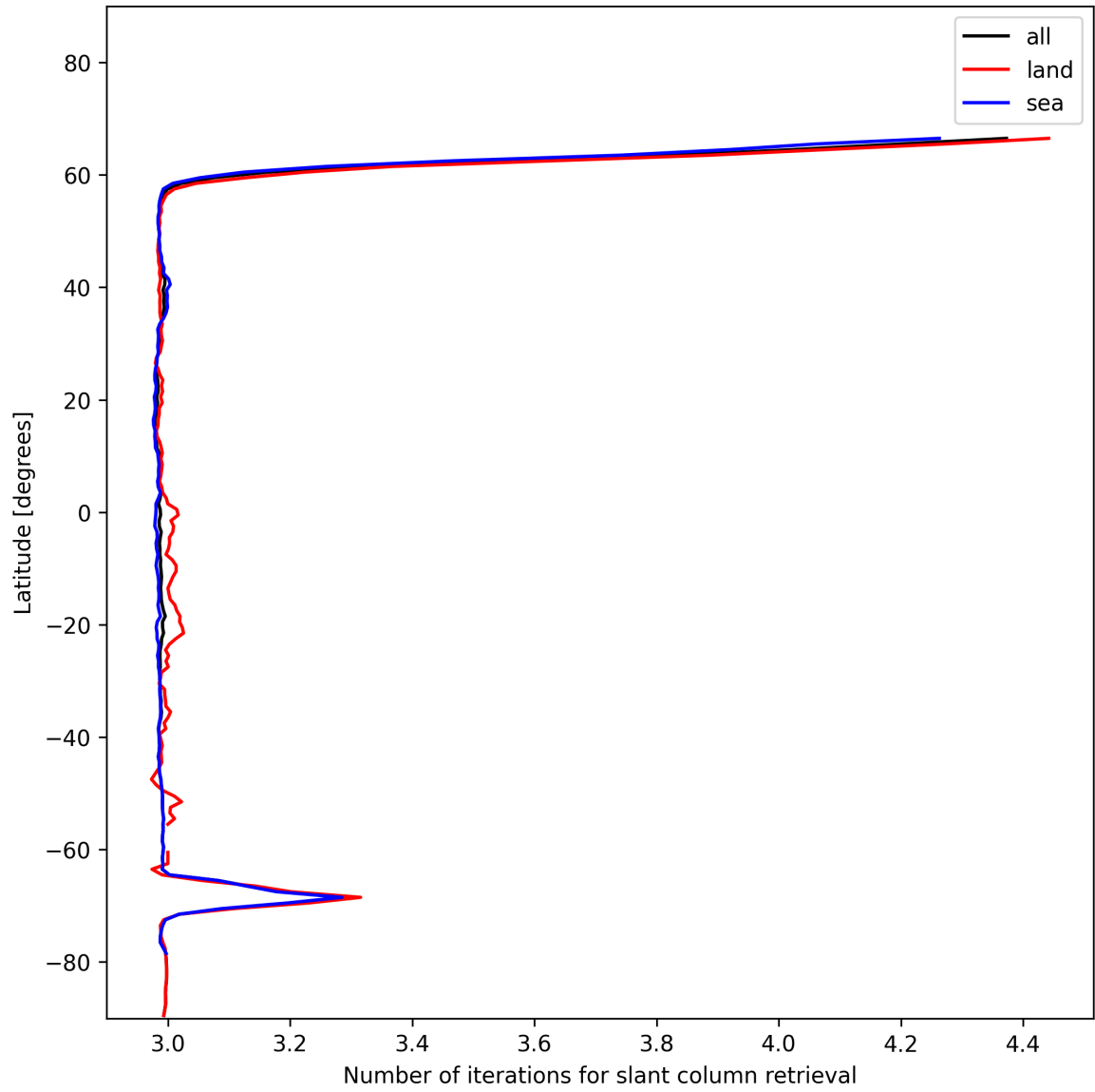
Figure 21: Zonal average of “Number of iterations for slant column retrieval” for 2025-01-05 to 2025-01-05.
