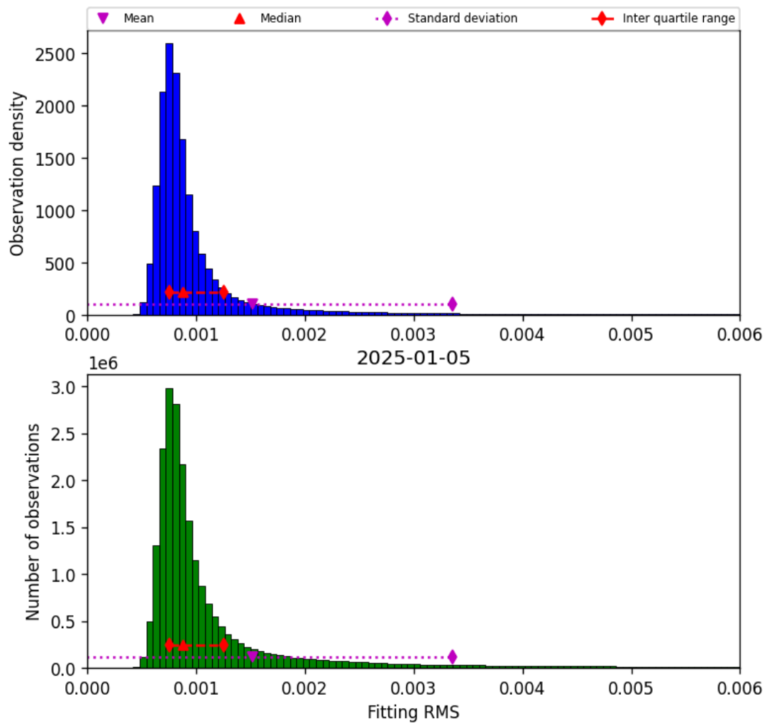
Figure 34: Histogram of “Fitting RMS” for 2025-01-05 to 2025-01-05
