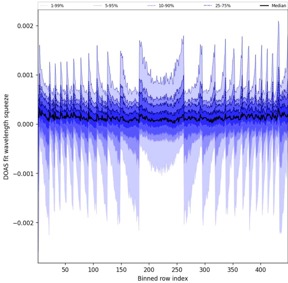
Figure 48: Along track statistics of “DOAS fit wavelength squeeze” for 2025-01-05 to 2025-01-05
