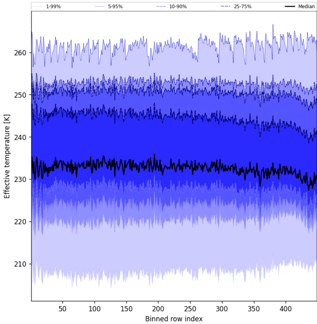
Figure 50: Along track statistics of “Effective temperature” for 2025-01-05 to 2025-01-05
