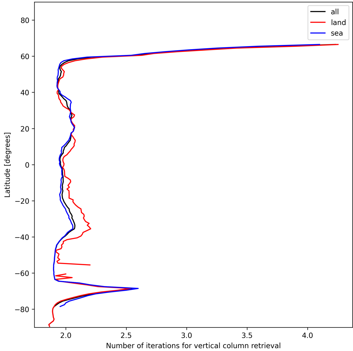
Figure 27: Zonal average of “Number of iterations for vertical column retrieval” for 2025-01-05 to 2025-01-05.
