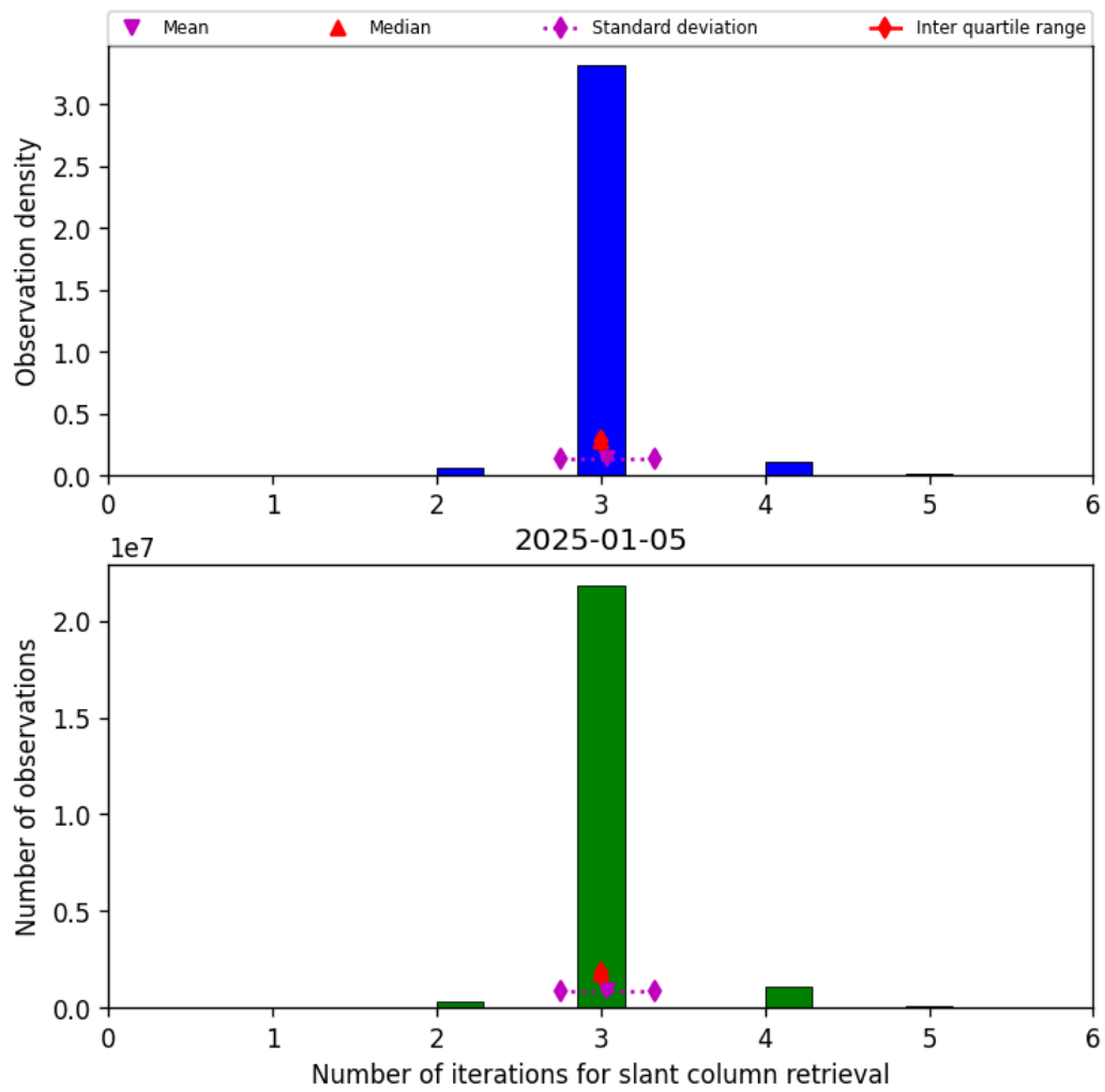
Figure 33: Histogram of "Number of iterations for slant column retrieval" for 2025-01-05 to 2025-01-05
