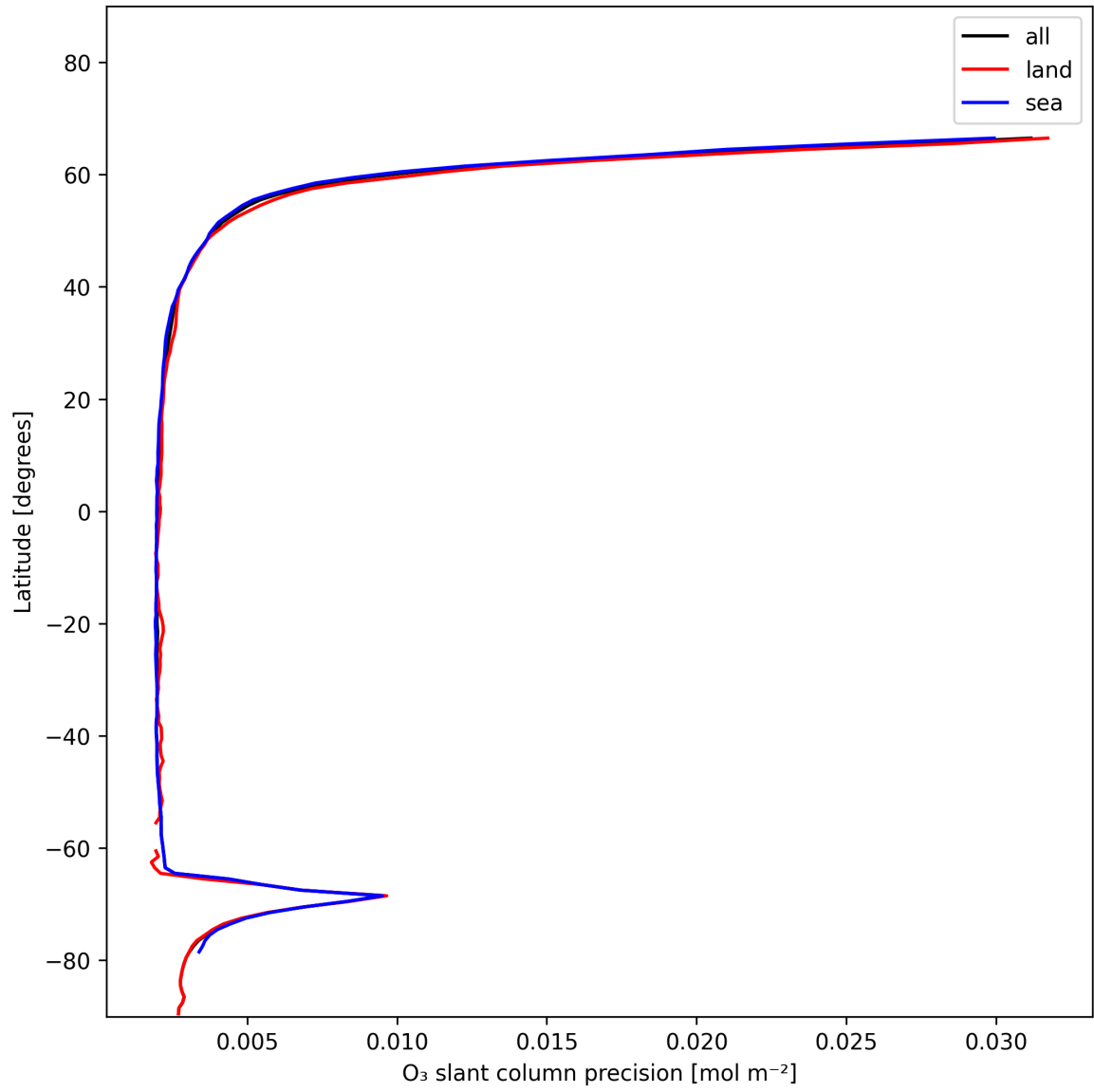
Figure 20: Zonal average of “O 3 slant column precision” for 2025-01-05 to 2025-01-05.
