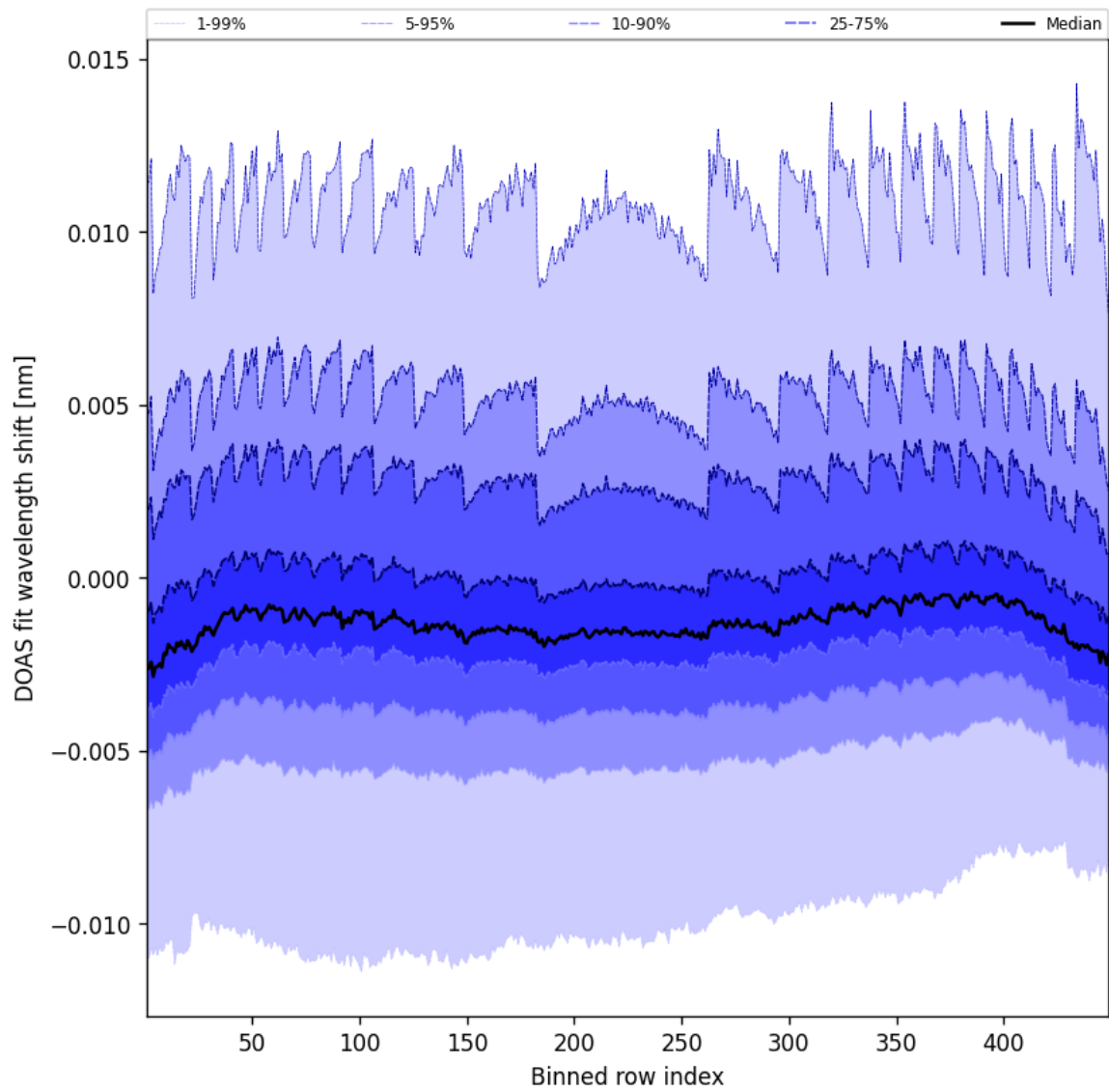
Figure 47: Along track statistics of "DOAS fit wavelength shift" for 2025-01-05 to 2025-01-05
