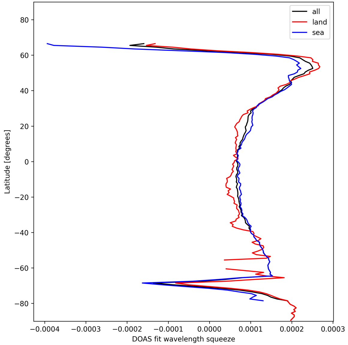
Figure 24: Zonal average of “DOAS fit wavelength squeeze” for 2025-01-05 to 2025-01-05.
