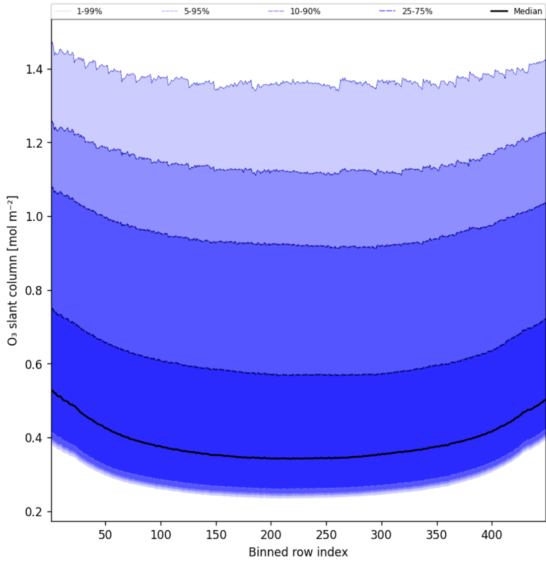
Figure 43: Along track statistics of “O 3 slant column” for 2025-01-05 to 2025-01-05
