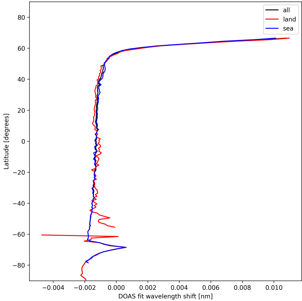
Figure 23: Zonal average of “DOAS fit wavelength shift” for 2025-01-05 to 2025-01-05.
