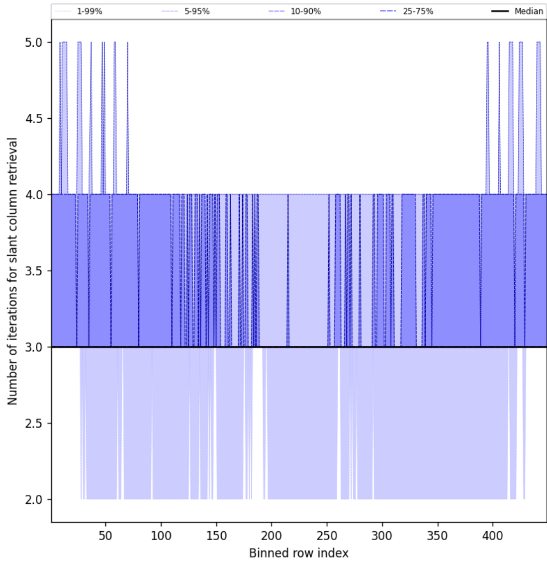
Figure 45: Along track statistics of “Number of iterations for slant column retrieval” for 2025-01-05 to 2025-01-05
