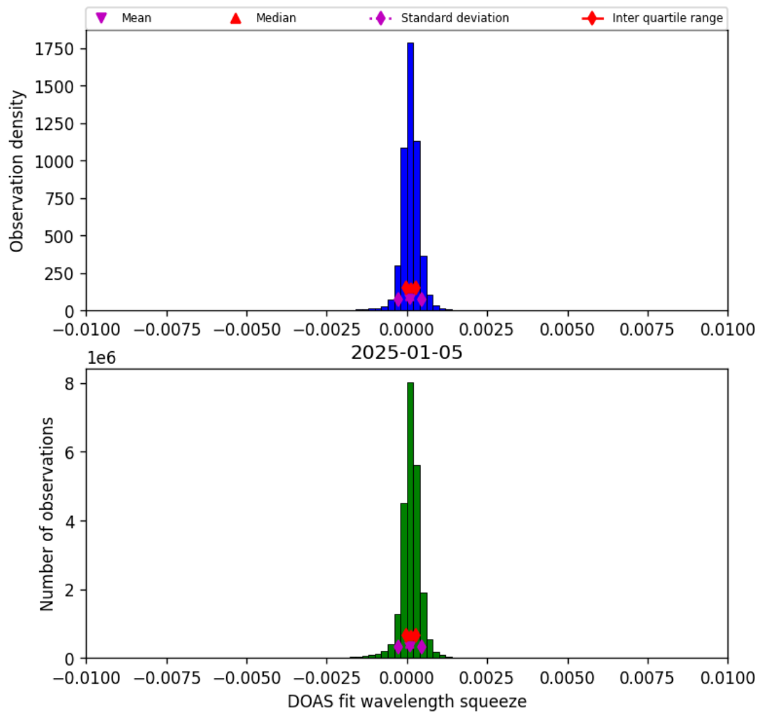
Figure 36: Histogram of “DOAS fit wavelength squeeze” for 2025-01-05 to 2025-01-05
