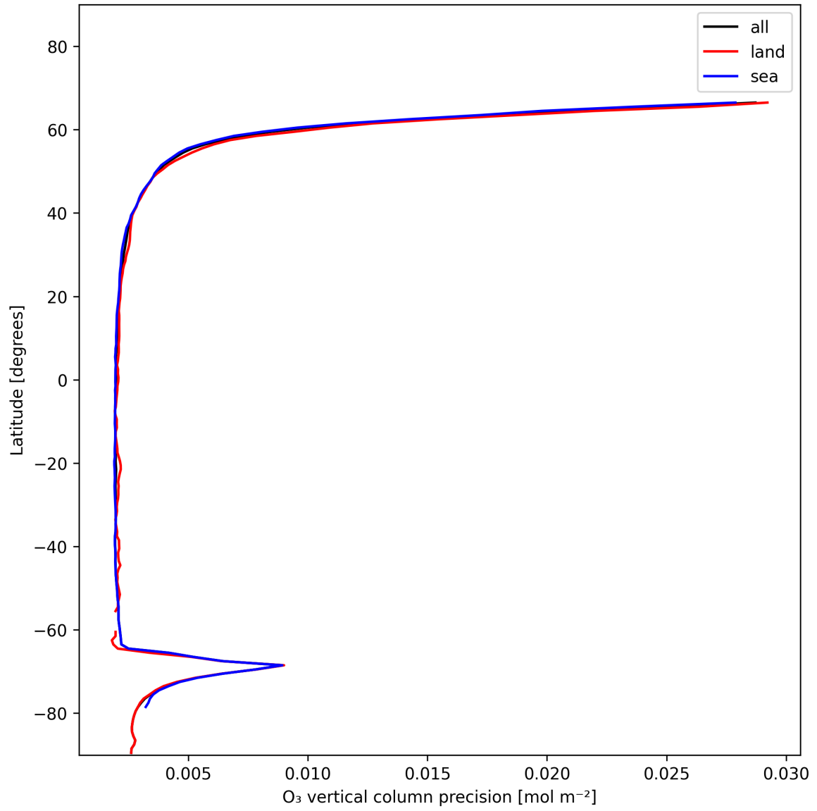
Figure 18: Zonal average of “O 3 vertical column precision” for 2025-01-05 to 2025-01-05.
