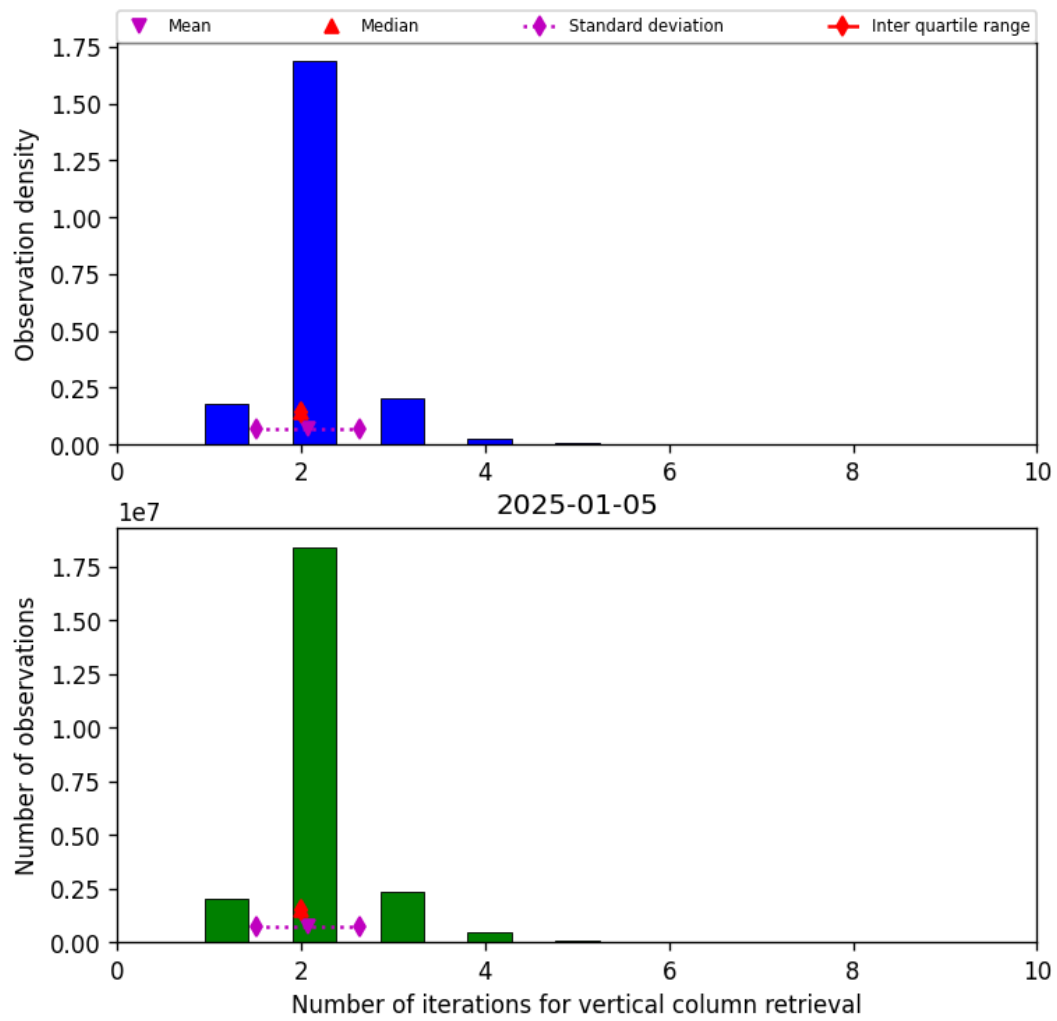
Figure 39: Histogram of “Number of iterations for vertical column retrieval” for 2025-01-05 to 2025-01-05
