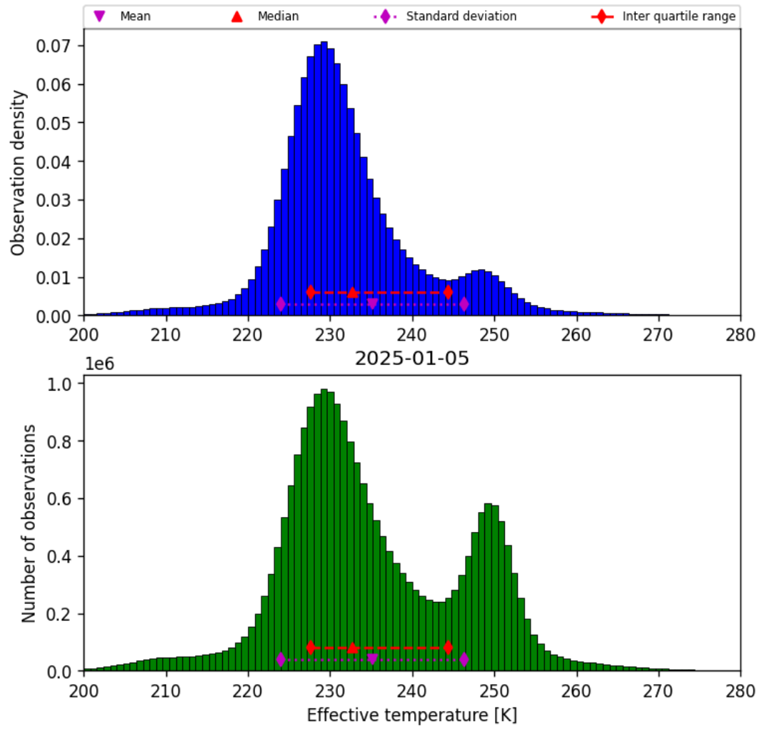
Figure 38: Histogram of “Effective temperature” for 2025-01-05 to 2025-01-05
