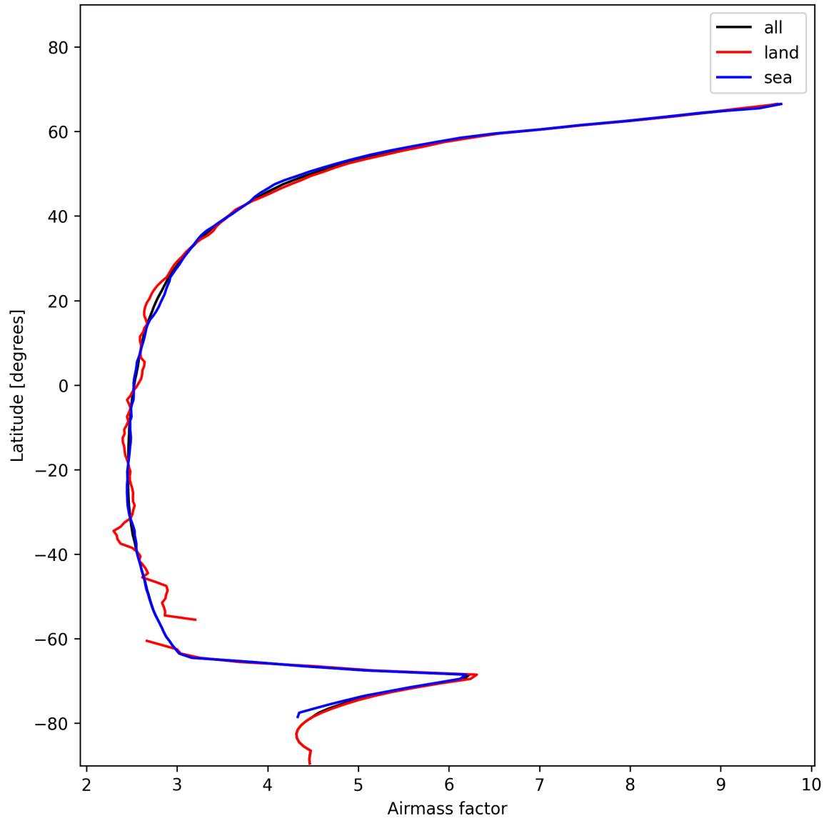
Figure 25: Zonal average of “Airmass factor” for 2025-01-05 to 2025-01-05.
