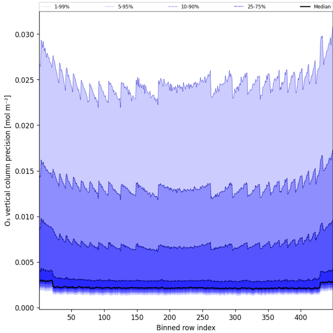
Figure 42: Along track statistics of “O 3 vertical column precision” for 2025-01-05 to 2025-01-05
