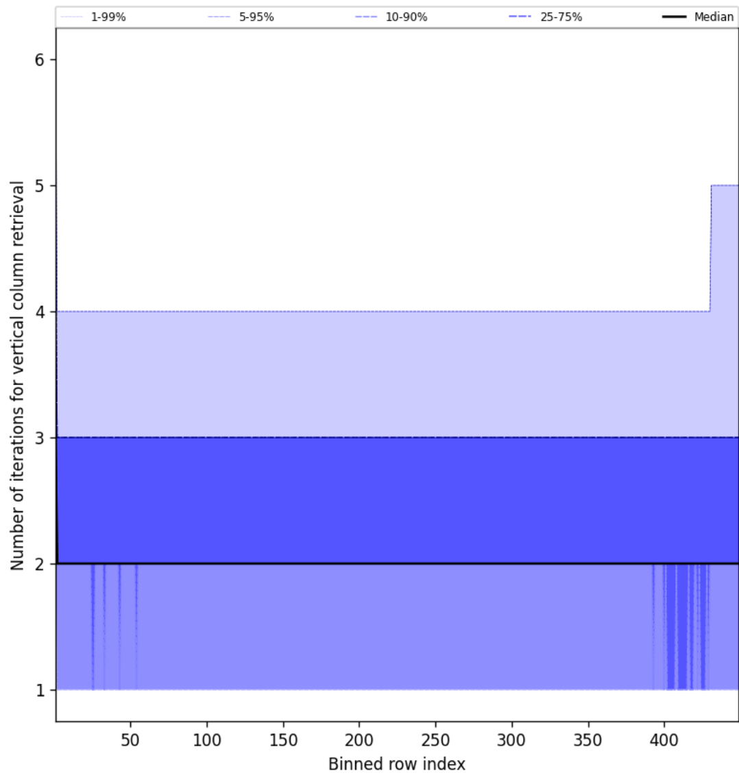
Figure 51: Along track statistics of “Number of iterations for vertical column retrieval” for 2025-01-05 to 2025-01-05
