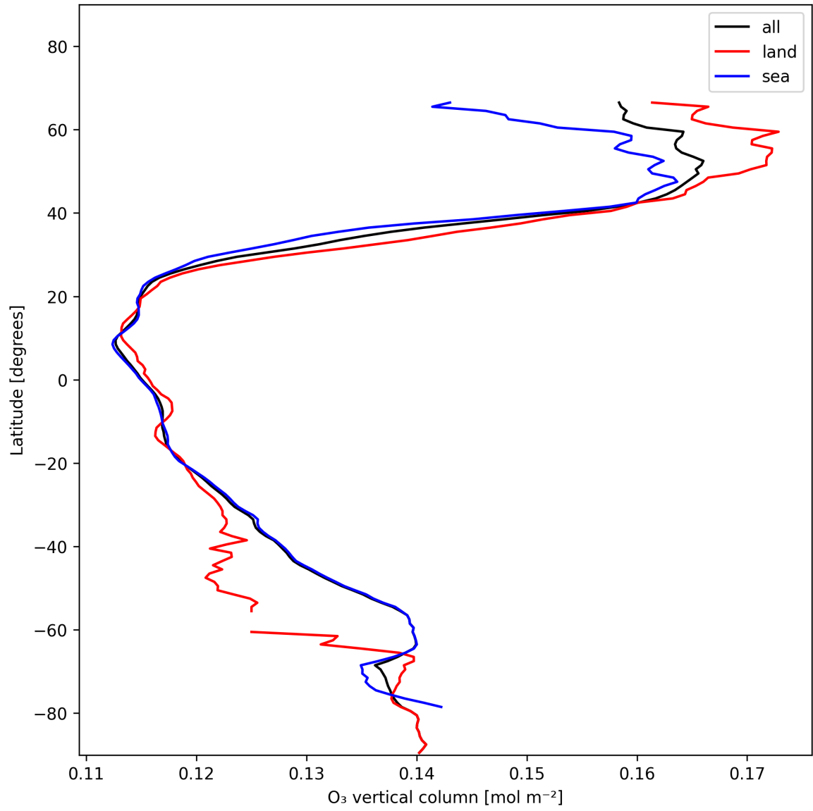
Figure 17: Zonal average of “O 3 vertical column” for 2025-01-05 to 2025-01-05.
