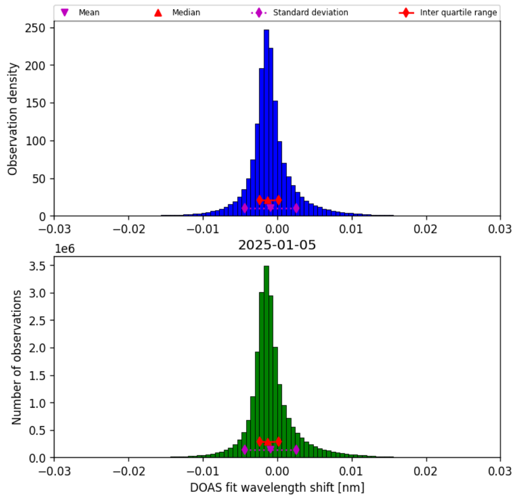
Figure 35: Histogram of “DOAS fit wavelength shift” for 2025-01-05 to 2025-01-05
