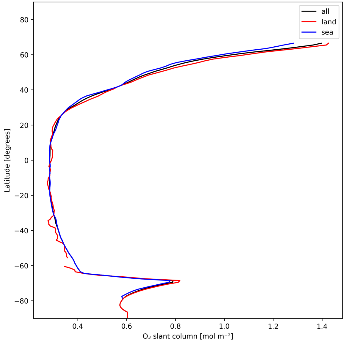
Figure 19: Zonal average of “O 3 slant column” for 2025-01-05 to 2025-01-05.
