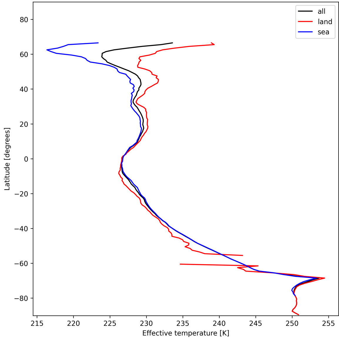
Figure 26: Zonal average of “Effective temperature” for 2025-01-05 to 2025-01-05.
