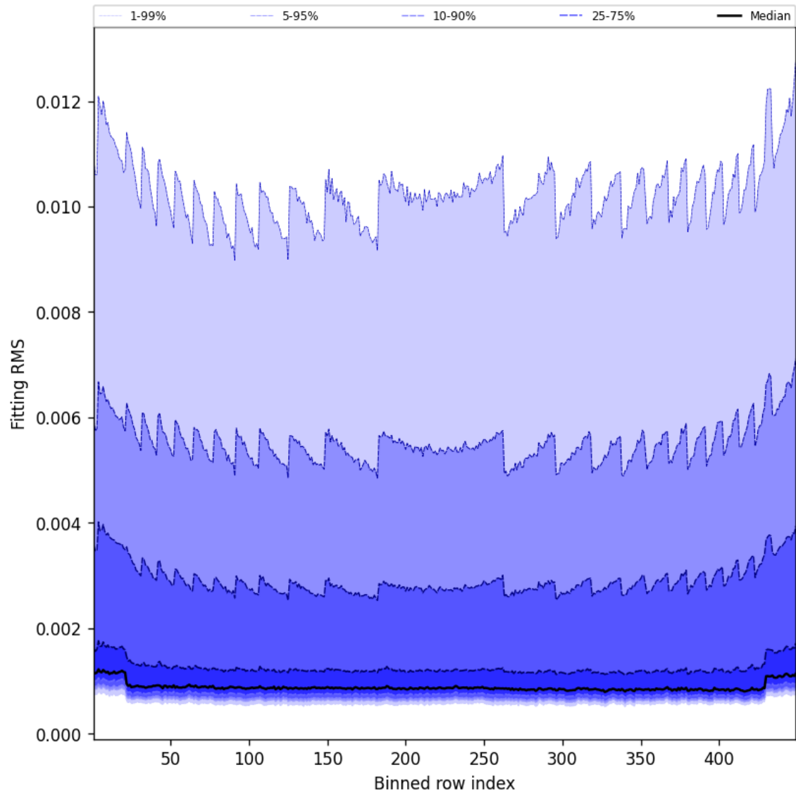
Figure 46: Along track statistics of “Fitting RMS” for 2025-01-05 to 2025-01-05
