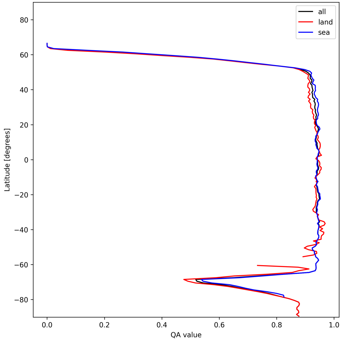
Figure 16: Zonal average of “QA value” for 2025-01-05 to 2025-01-05.
