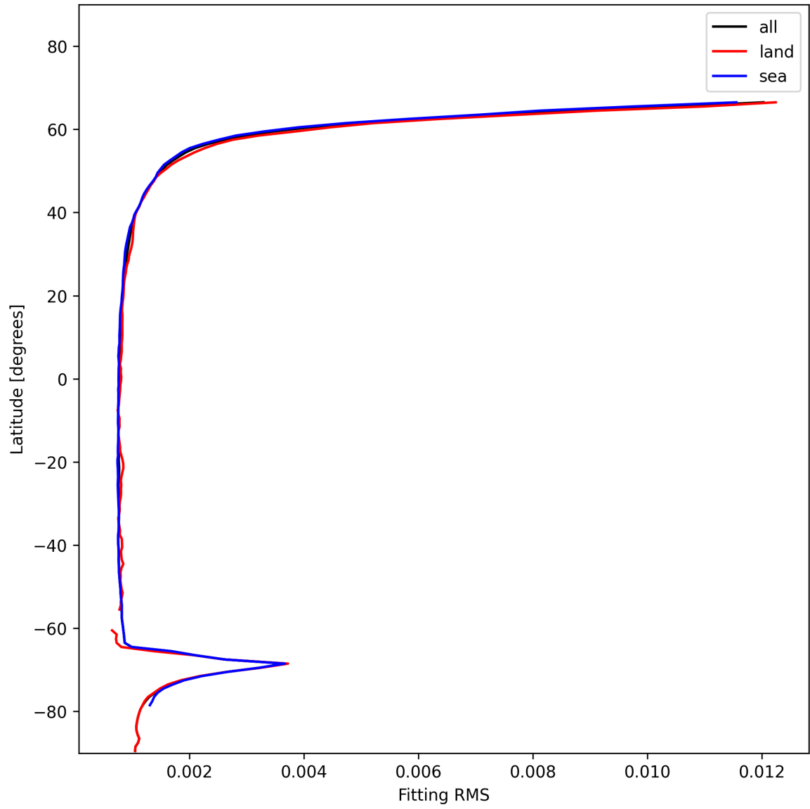
Figure 22: Zonal average of “Fitting RMS” for 2025-01-05 to 2025-01-05.
