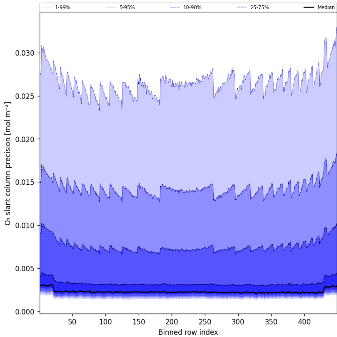
Figure 44: Along track statistics of “O 3 slant column precision” for 2025-01-05 to 2025-01-05
