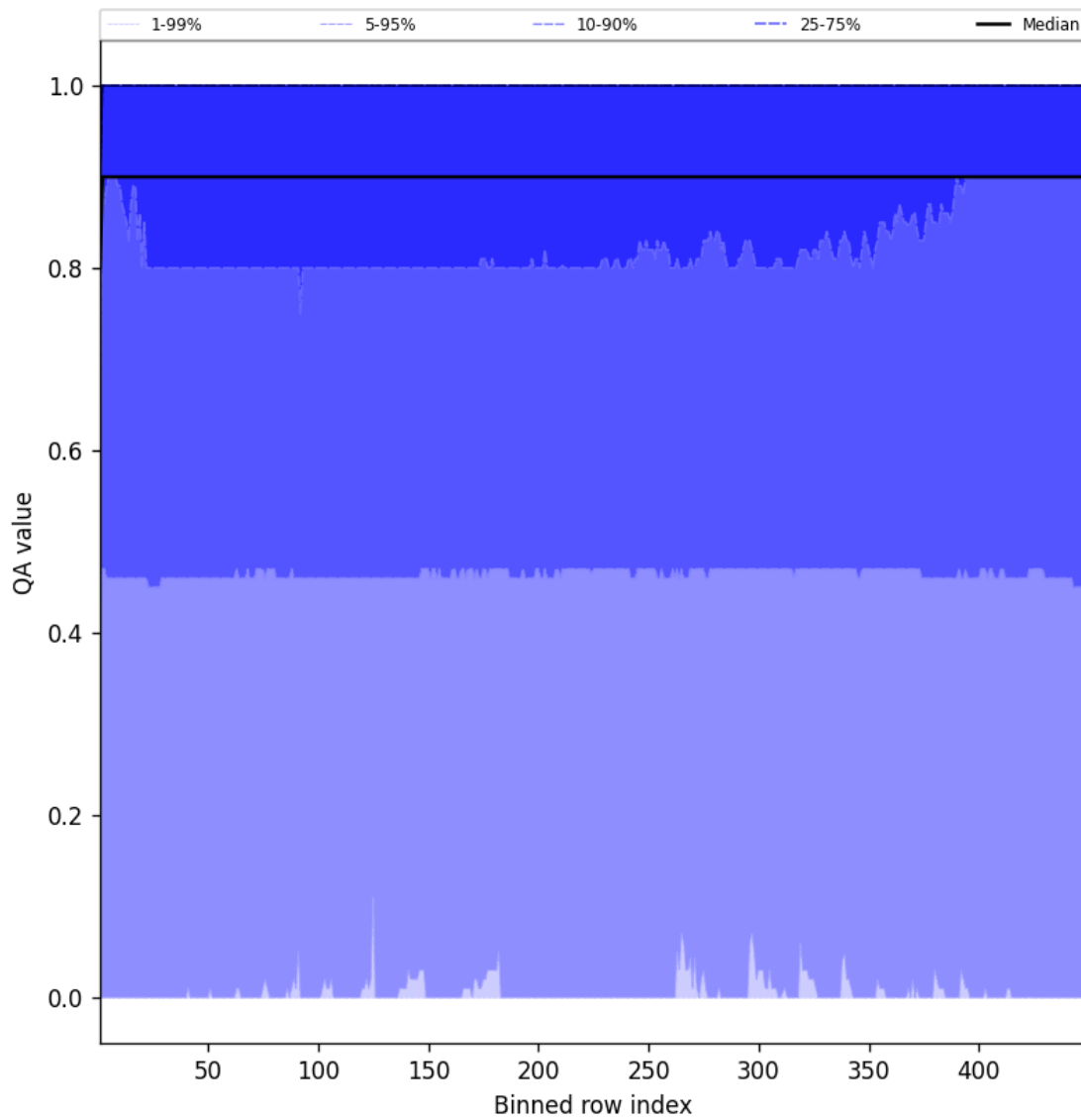
Figure 40: Along track statistics of “QA value” for 2025-01-05 to 2025-01-05
