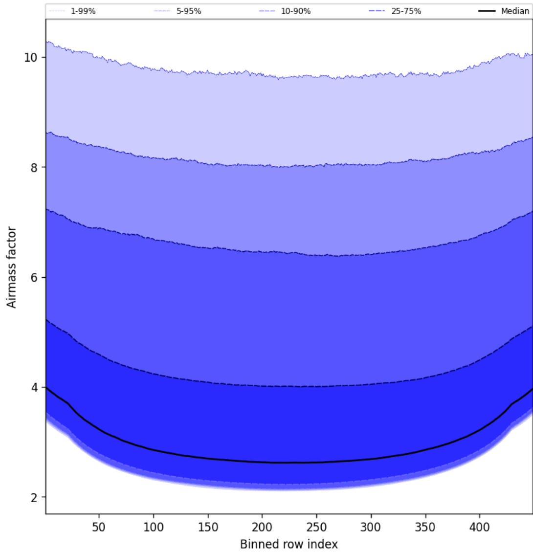
Figure 49: Along track statistics of “Airmass factor” for 2025-01-05 to 2025-01-05
