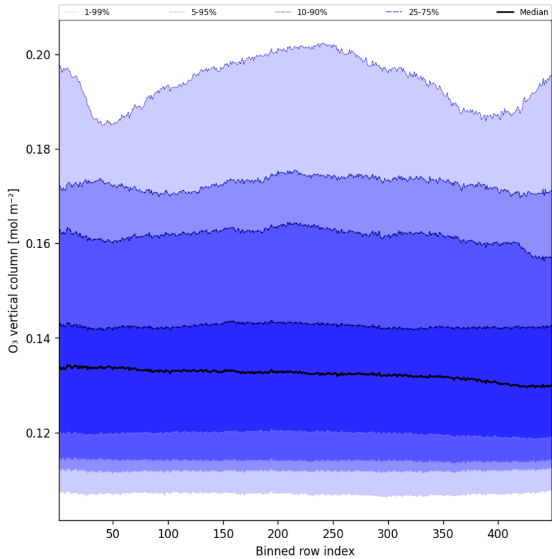
Figure 41: Along track statistics of “O 3 vertical column” for 2025-01-05 to 2025-01-05
