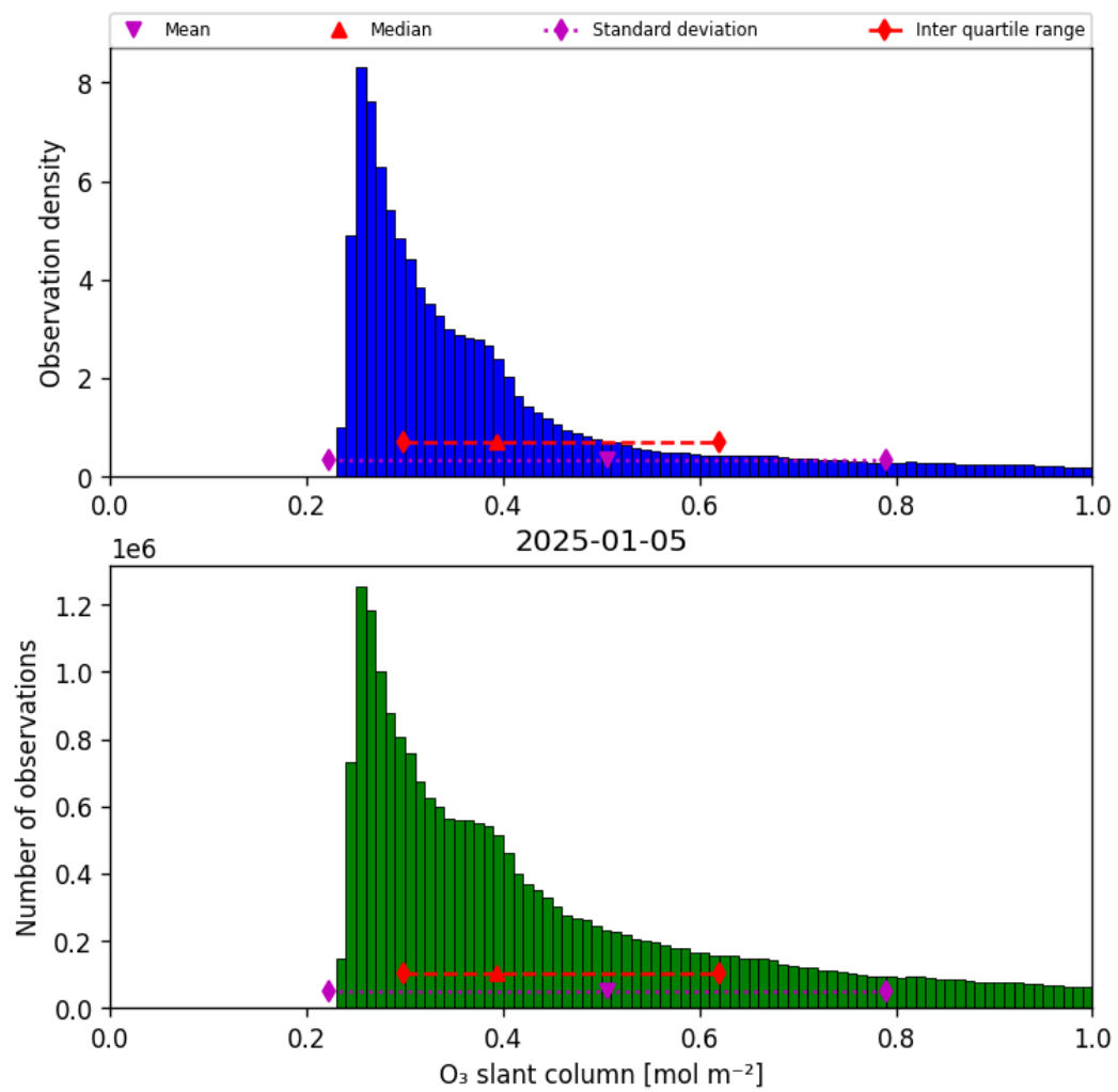
Figure 31: Histogram of “O 3 slant column” for 2025-01-05 to 2025-01-05
