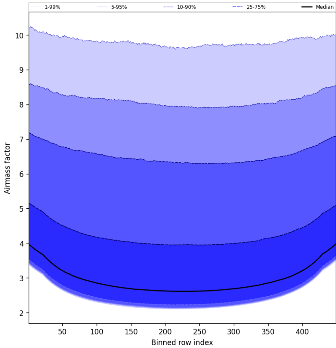
Figure 49: Along track statistics of “Airmass factor” for 2025-01-06 to 2025-01-07
