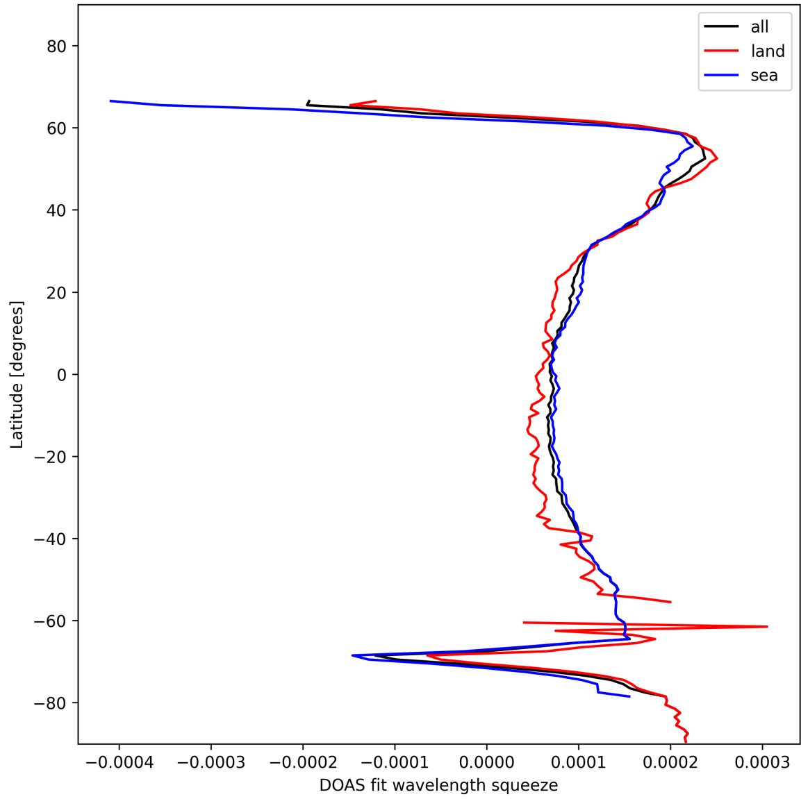
Figure 24: Zonal average of “DOAS fit wavelength squeeze” for 2025-01-06 to 2025-01-07.
