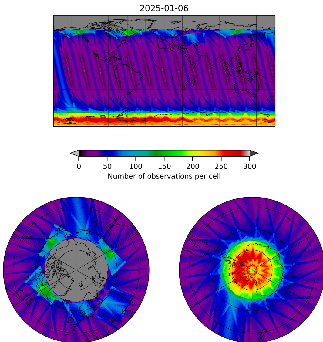
Figure 15: Map of the number of observations for 2025-01-06 to 2025-01-07
