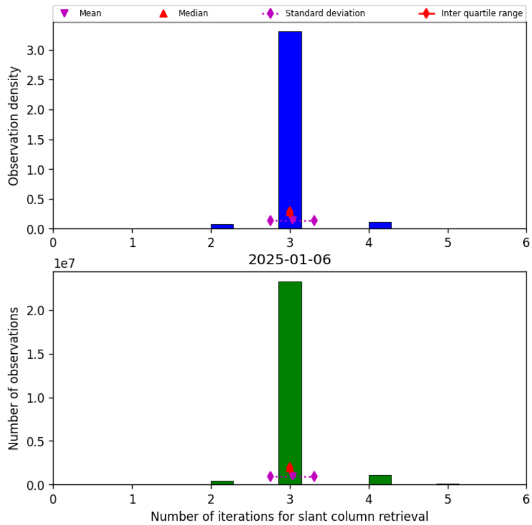
Figure 33: Histogram of “Number of iterations for slant column retrieval” for 2025-01-06 to 2025-01-07
