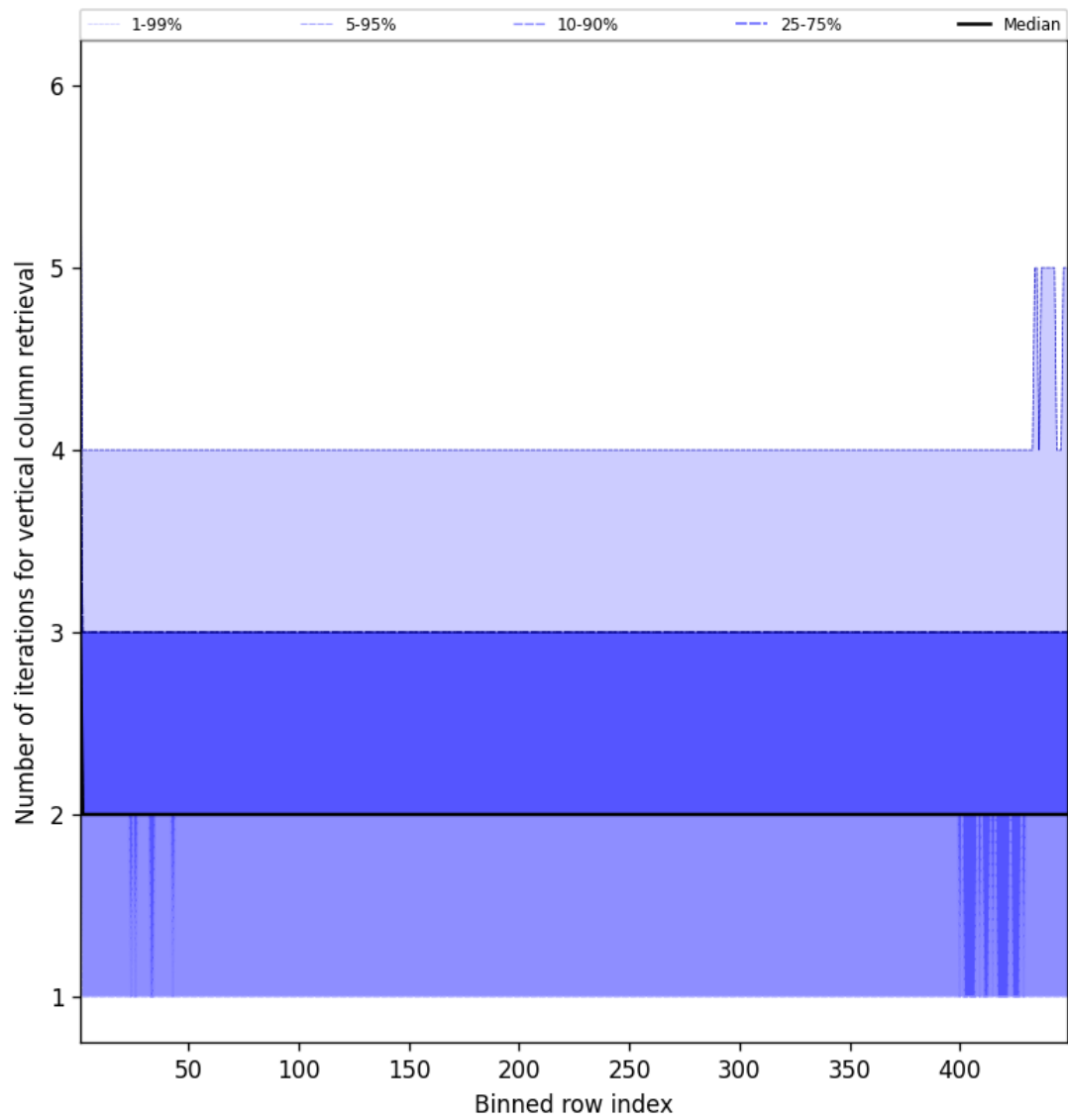
Figure 51: Along track statistics of “Number of iterations for vertical column retrieval” for 2025-01-06 to 2025-01-07
