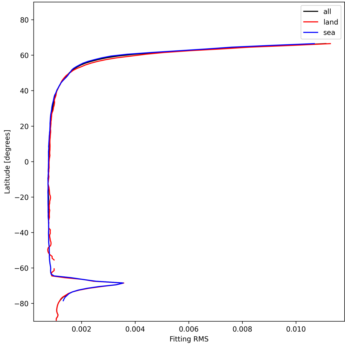
Figure 22: Zonal average of “Fitting RMS” for 2025-01-06 to 2025-01-07.
