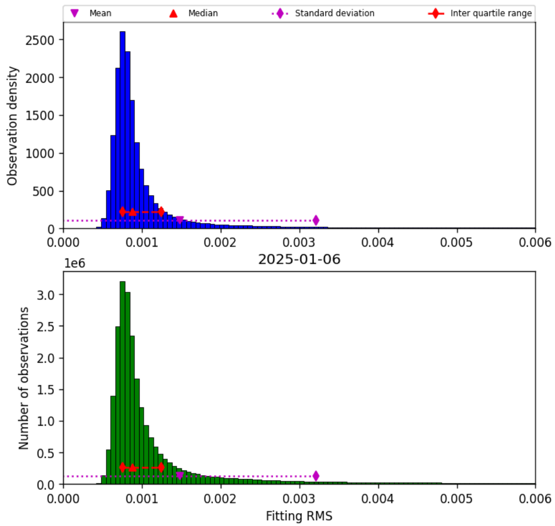
Figure 34: Histogram of “Fitting RMS” for 2025-01-06 to 2025-01-07
