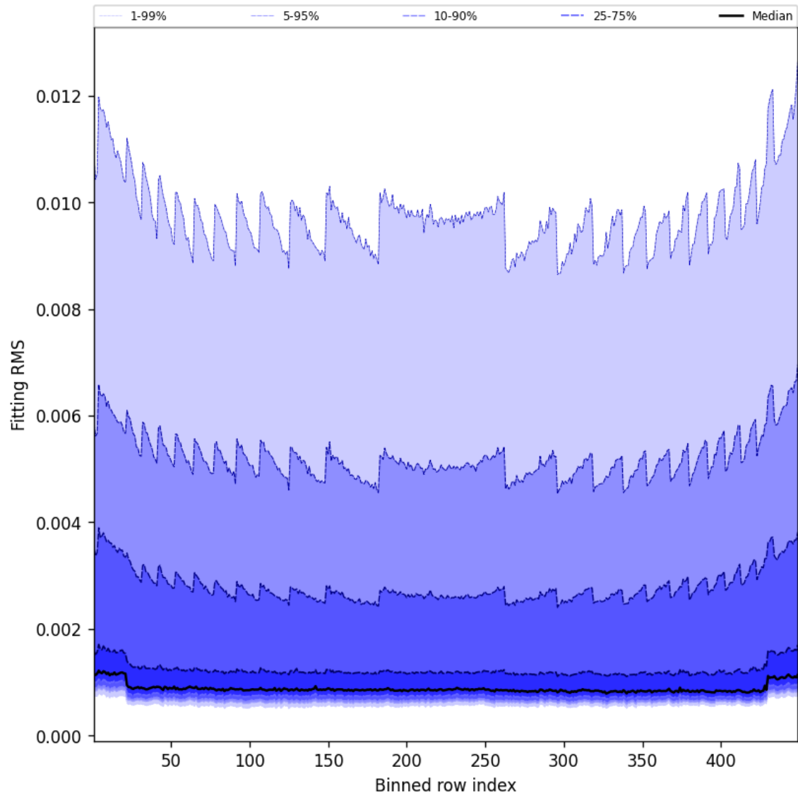
Figure 46: Along track statistics of “Fitting RMS” for 2025-01-06 to 2025-01-07
