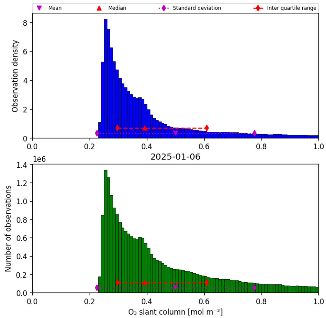
Figure 31: Histogram of “O 3 slant column” for 2025-01-06 to 2025-01-07
