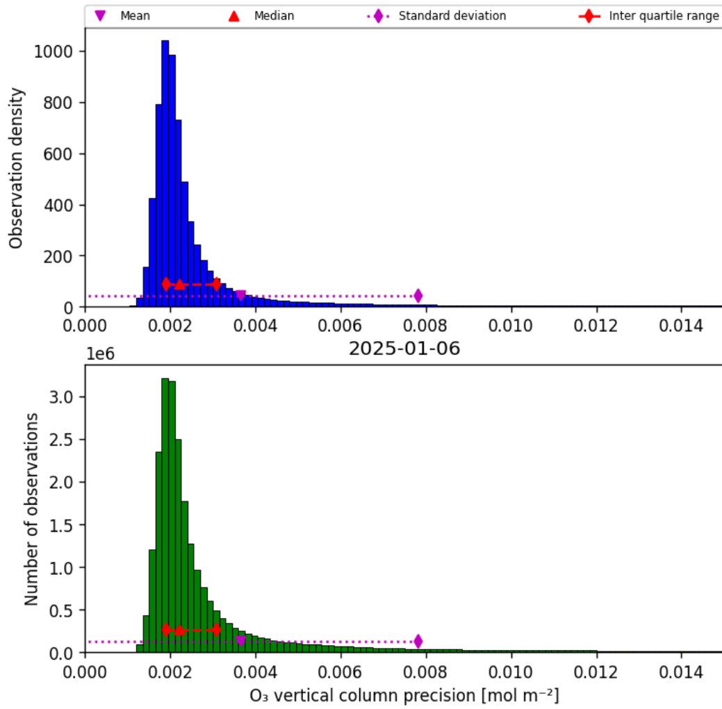
Figure 30: Histogram of “O 3 vertical column precision” for 2025-01-06 to 2025-01-07
