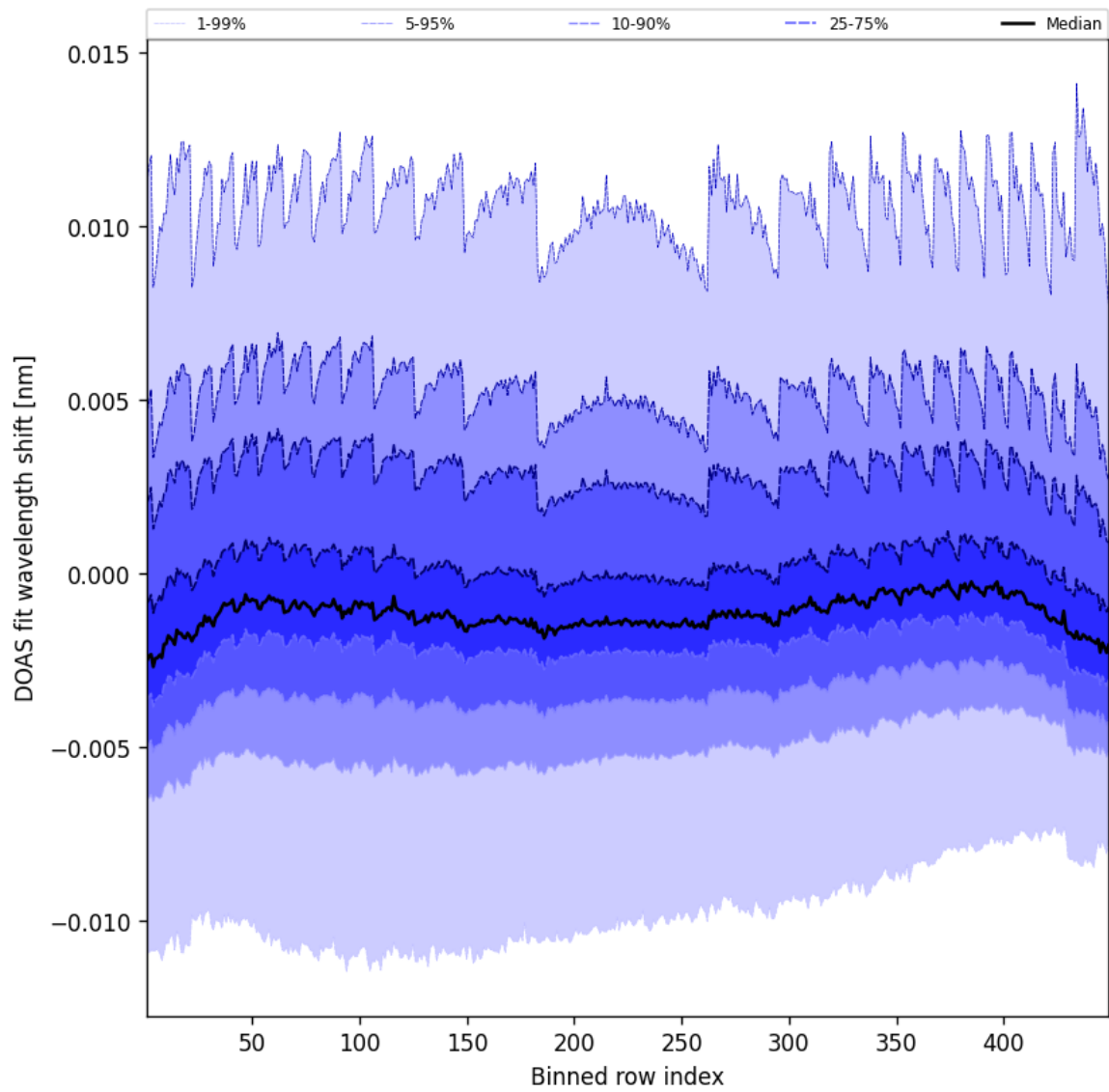
Figure 47: Along track statistics of “DOAS fit wavelength shift” for 2025-01-06 to 2025-01-07
