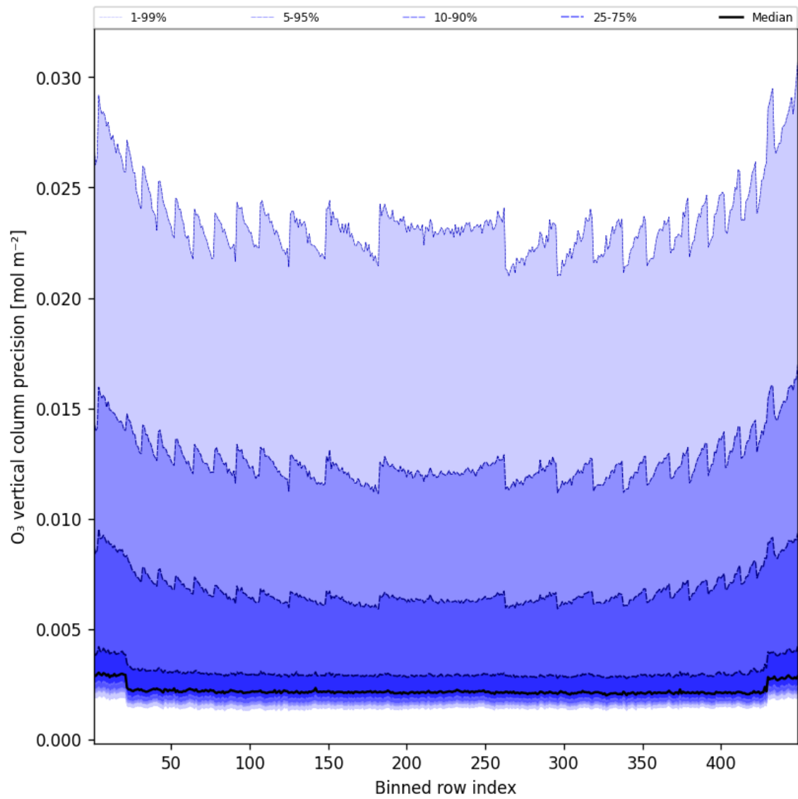
Figure 42: Along track statistics of “O 3 vertical column precision” for 2025-01-06 to 2025-01-07
