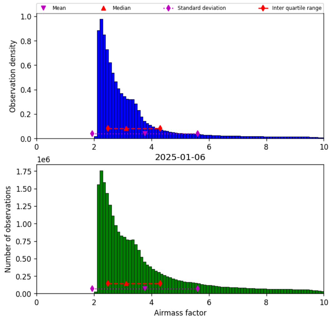
Figure 37: Histogram of “Airmass factor” for 2025-01-06 to 2025-01-07
