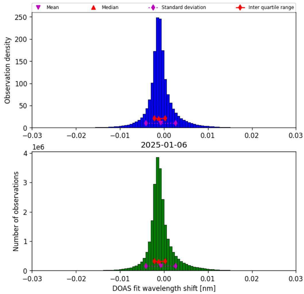
Figure 35: Histogram of “DOAS fit wavelength shift” for 2025-01-06 to 2025-01-07
