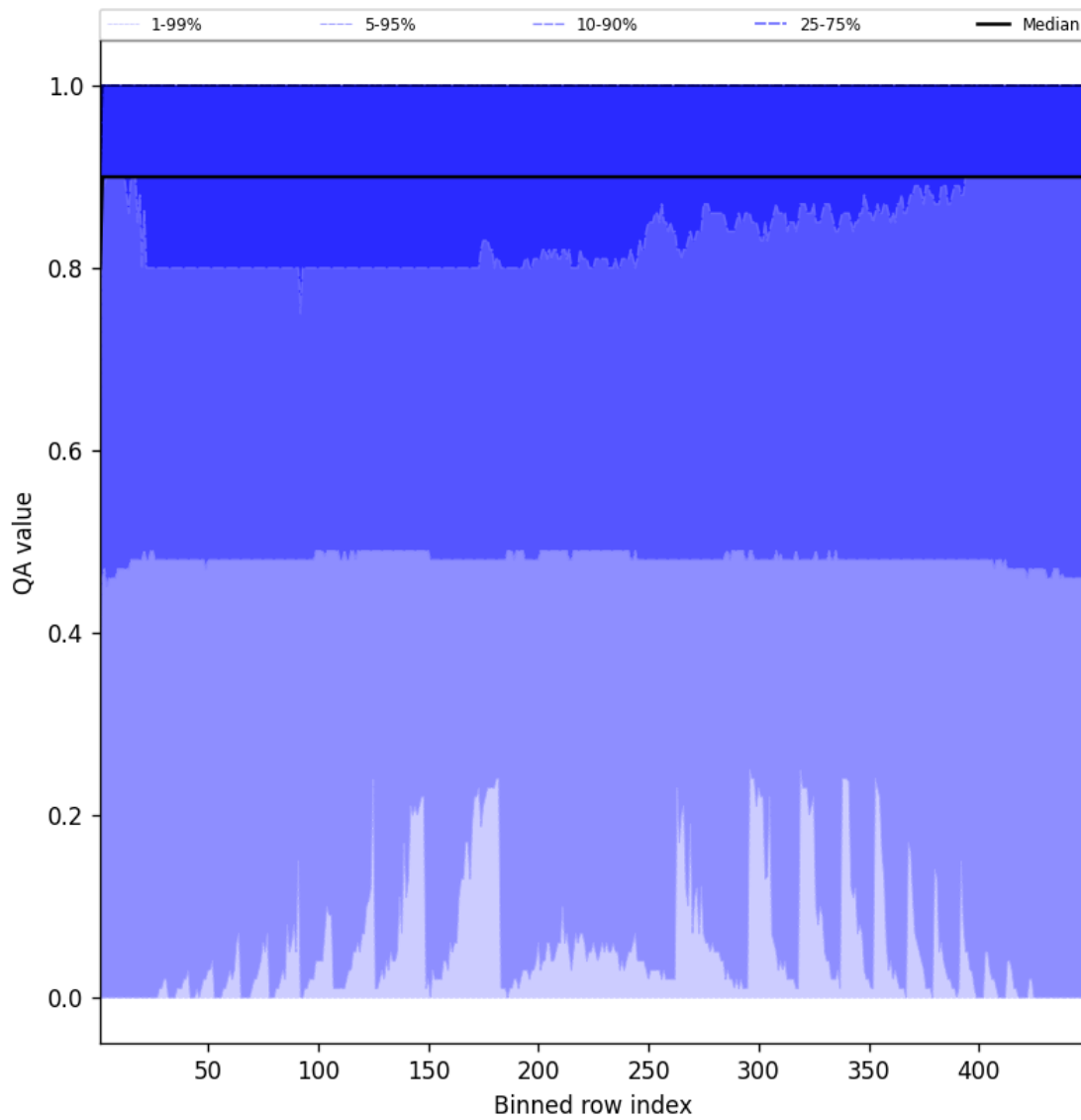
Figure 40: Along track statistics of “QA value” for 2025-01-06 to 2025-01-07
