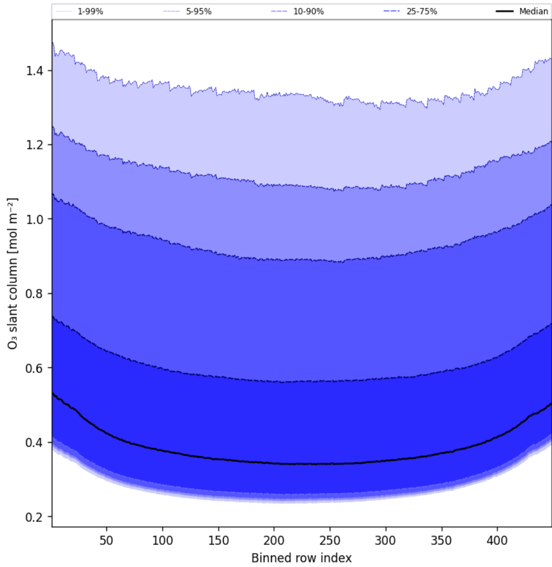
Figure 43: Along track statistics of “O 3 slant column” for 2025-01-06 to 2025-01-07
