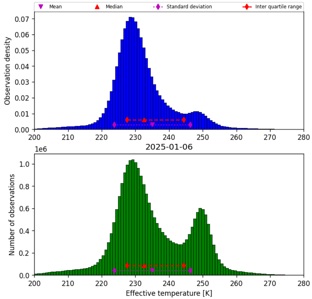
Figure 38: Histogram of “Effective temperature” for 2025-01-06 to 2025-01-07
