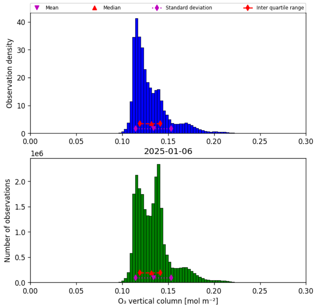
Figure 29: Histogram of “O 3 vertical column” for 2025-01-06 to 2025-01-07
