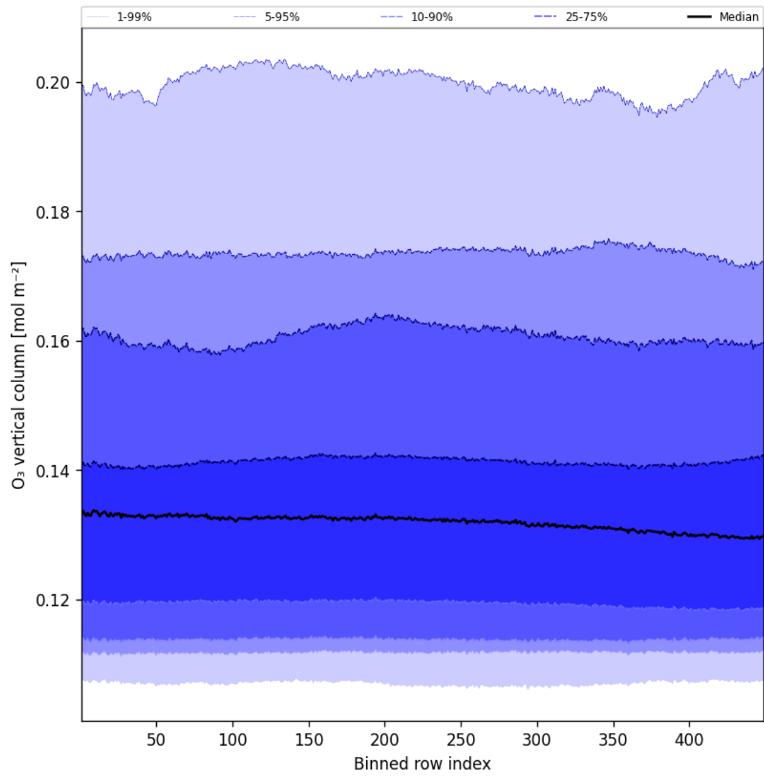
Figure 41: Along track statistics of “ \text{O}_3 vertical column” for 2025-01-06 to 2025-01-07
