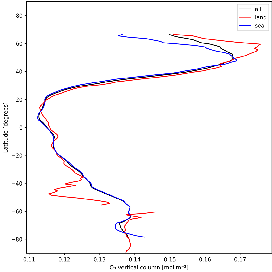
Figure 17: Zonal average of “O 3 vertical column” for 2025-01-06 to 2025-01-07.
