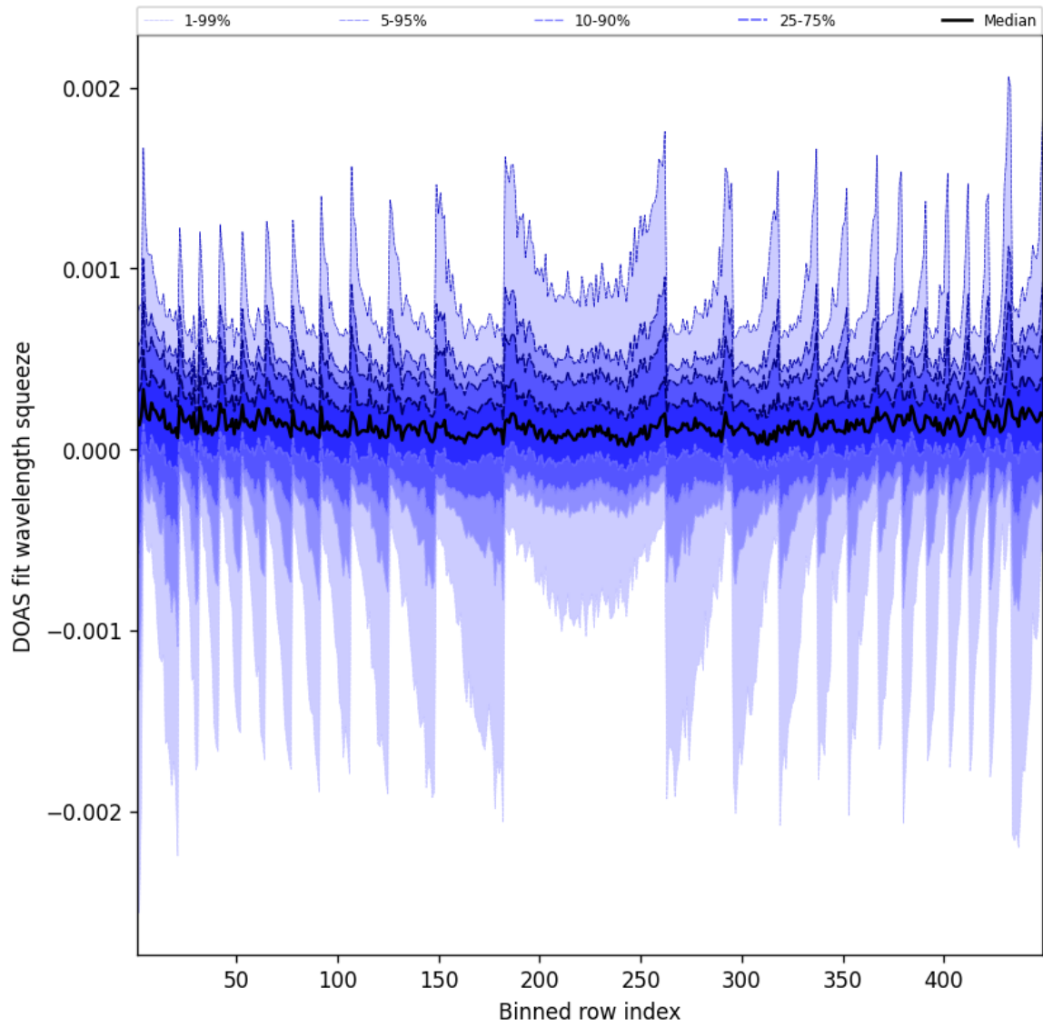
Figure 48: Along track statistics of “DOAS fit wavelength squeeze” for 2025-01-06 to 2025-01-07
