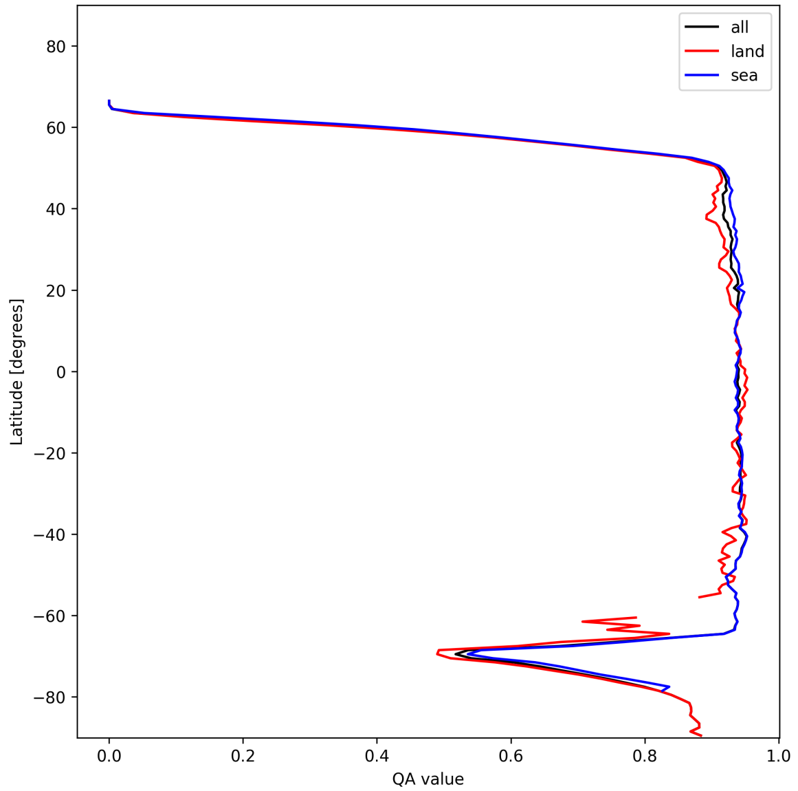
Figure 16: Zonal average of "QA value" for 2025-01-06 to 2025-01-07.
