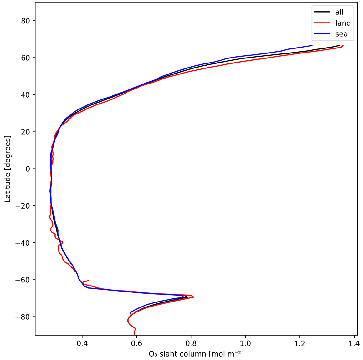
Figure 19: Zonal average of “O 3 slant column” for 2025-01-06 to 2025-01-07.
