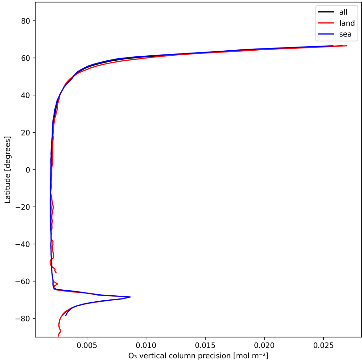
Figure 18: Zonal average of “O 3 vertical column precision” for 2025-01-06 to 2025-01-07.
