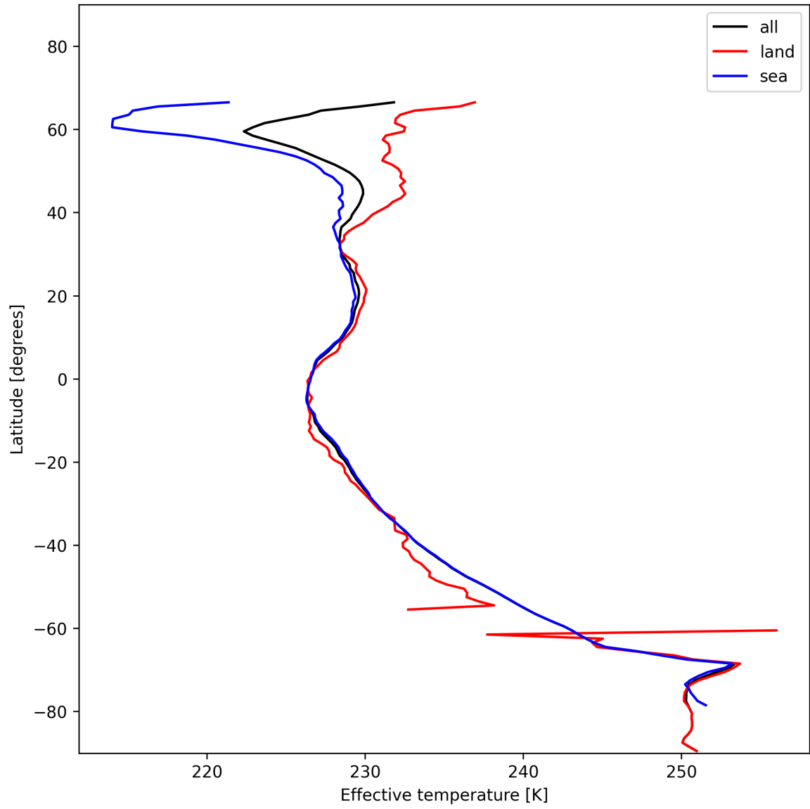
Figure 26: Zonal average of “Effective temperature” for 2025-01-06 to 2025-01-07.
