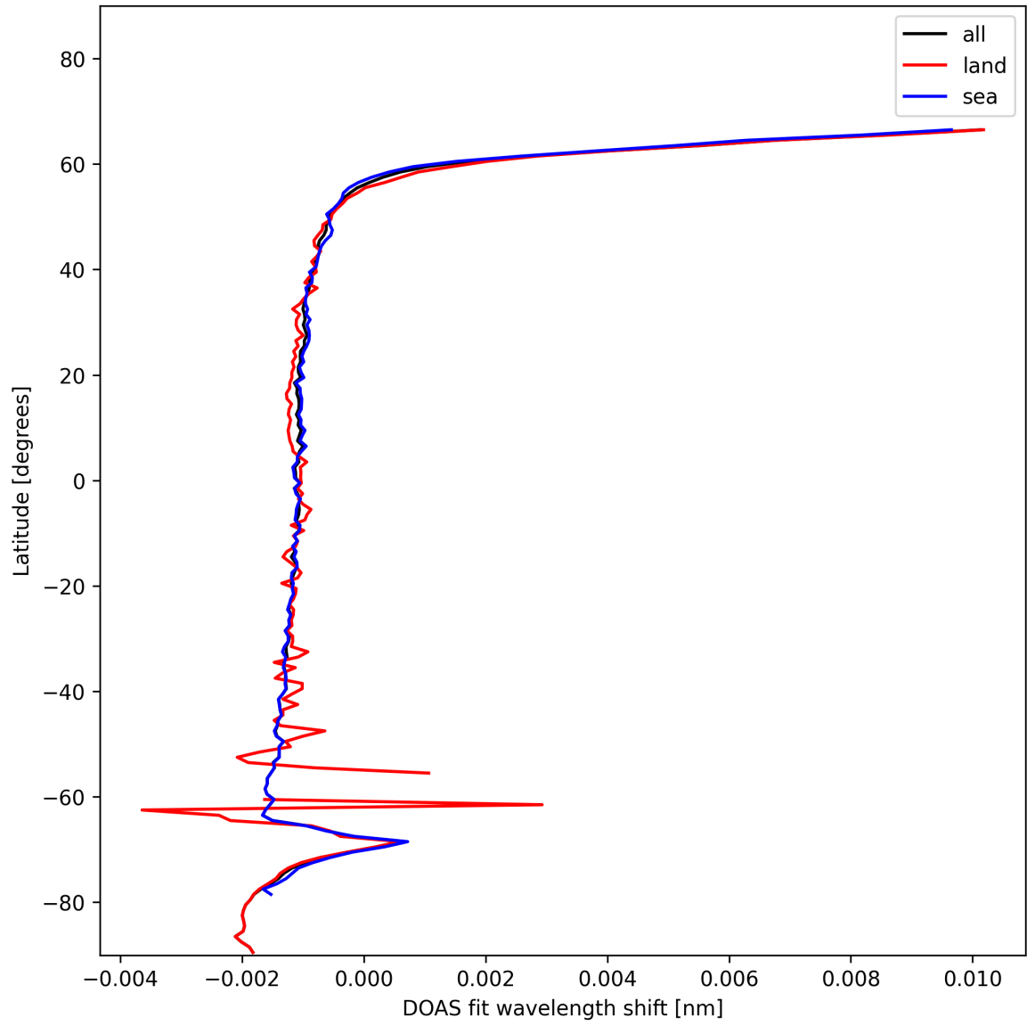
Figure 23: Zonal average of “DOAS fit wavelength shift” for 2025-01-06 to 2025-01-07.
