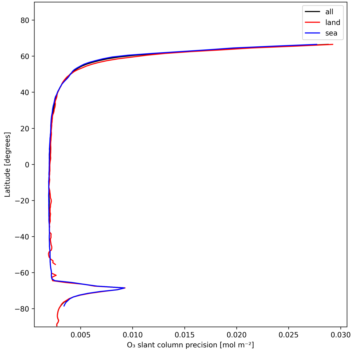
Figure 20: Zonal average of “O 3 slant column precision” for 2025-01-06 to 2025-01-07.
