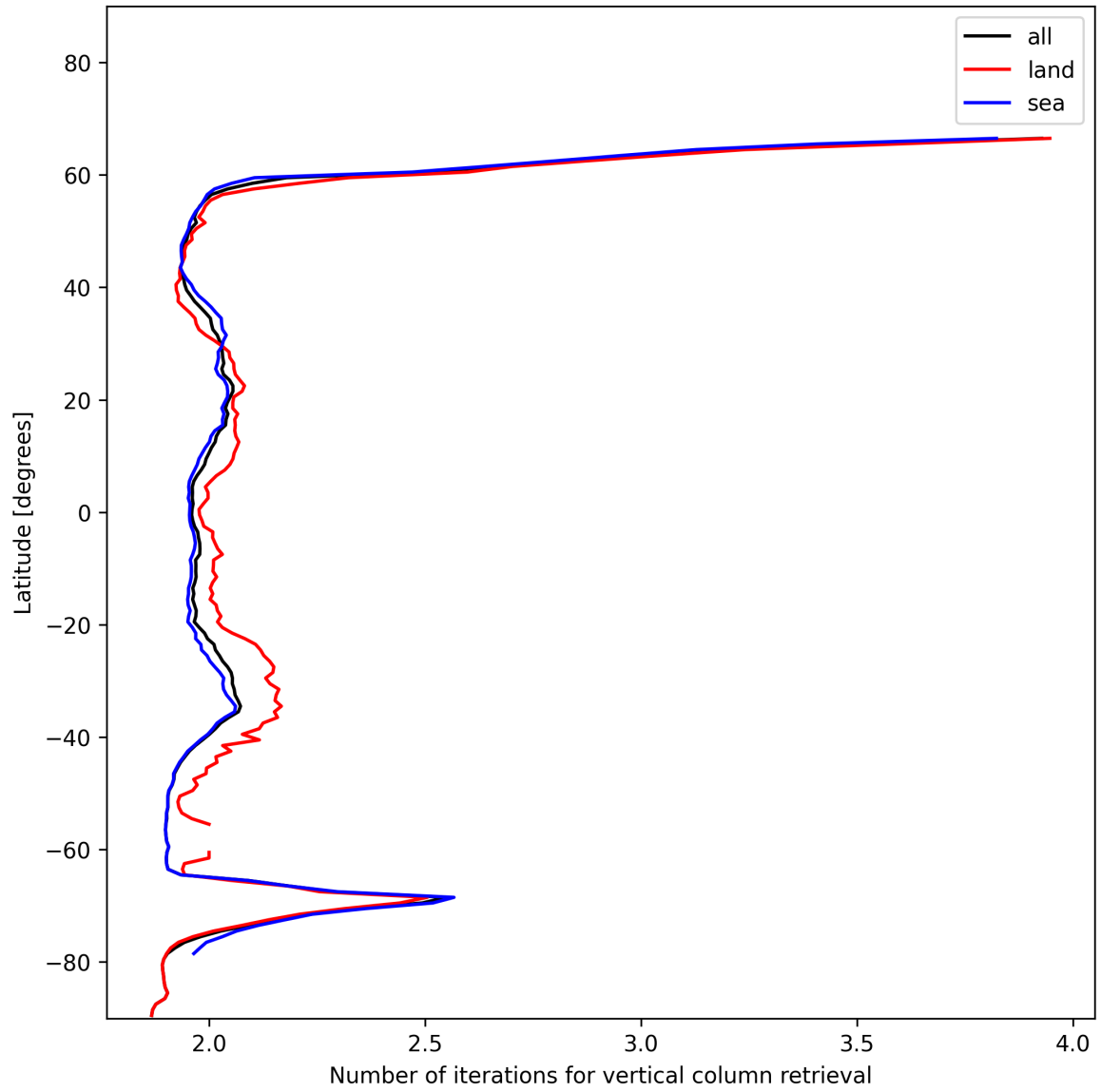
Figure 27: Zonal average of “Number of iterations for vertical column retrieval” for 2025-01-06 to 2025-01-07.
