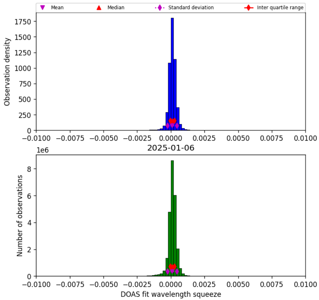
Figure 36: Histogram of “DOAS fit wavelength squeeze” for 2025-01-06 to 2025-01-07
