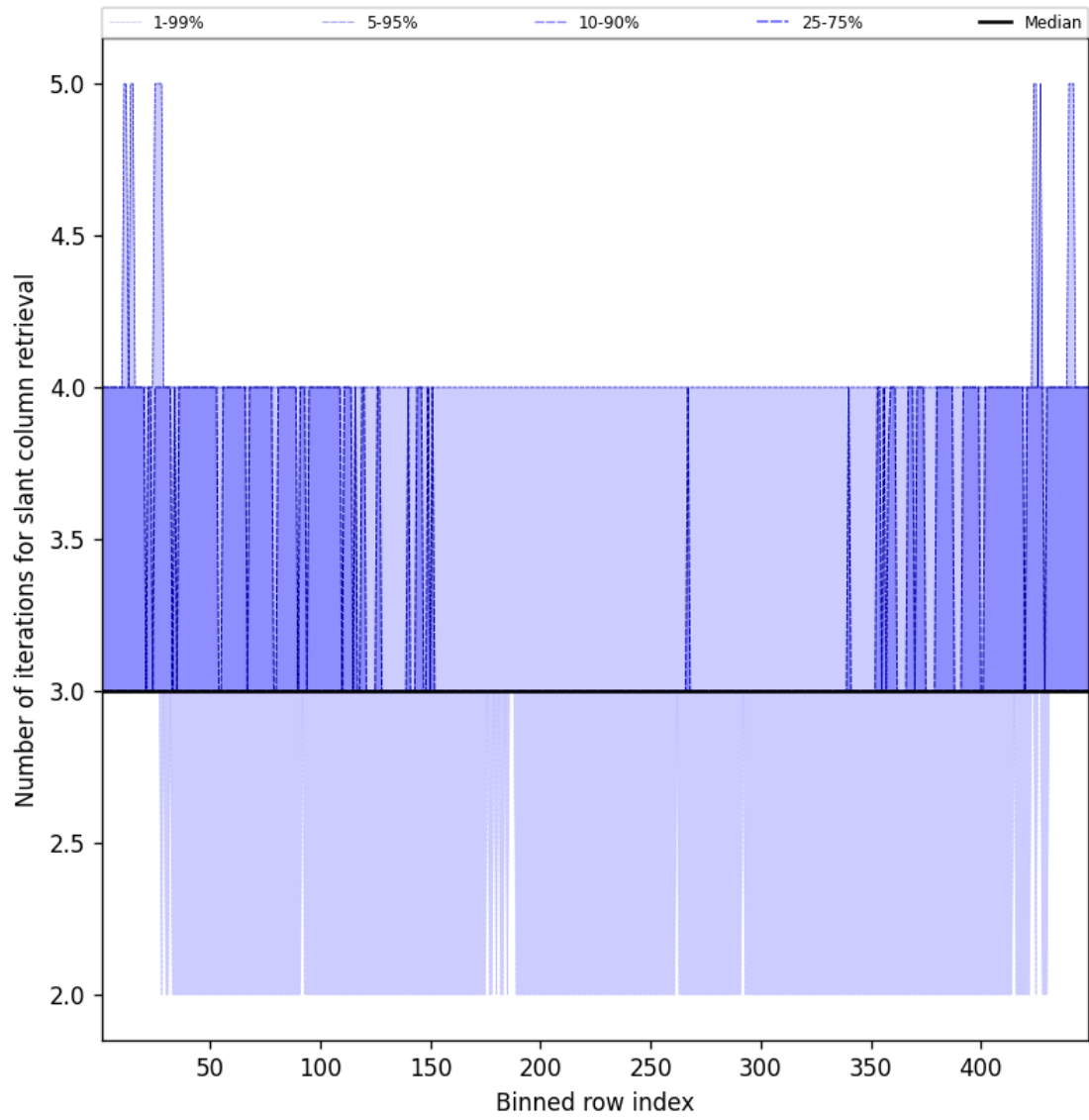
Figure 45: Along track statistics of “Number of iterations for slant column retrieval” for 2025-01-06 to 2025-01-07
