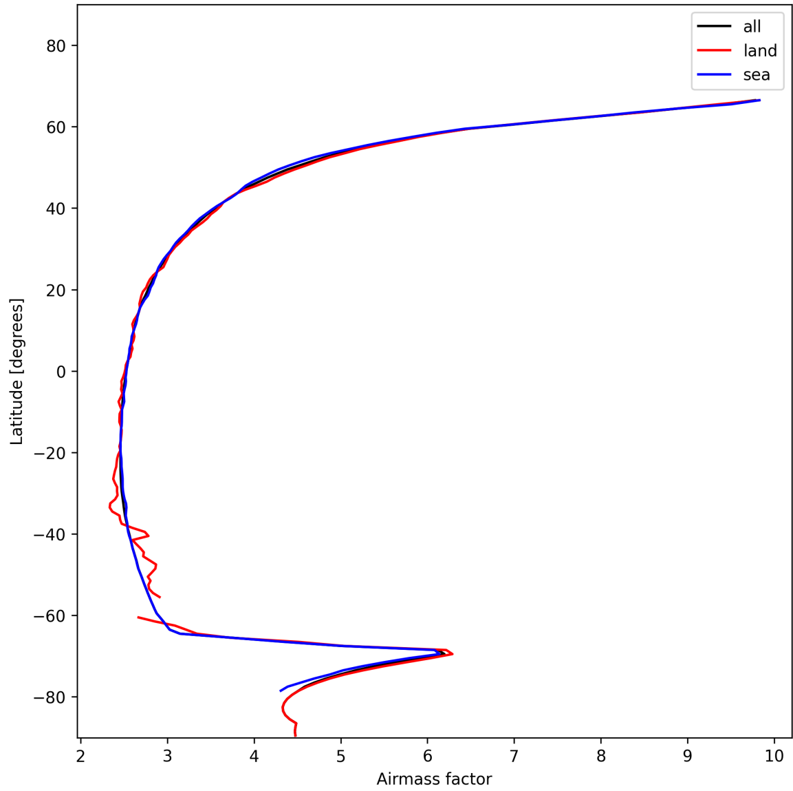
Figure 25: Zonal average of “Airmass factor” for 2025-01-06 to 2025-01-07.
