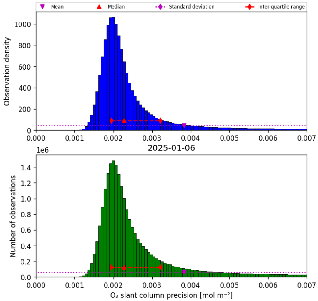
Figure 32: Histogram of “O 3 slant column precision” for 2025-01-06 to 2025-01-07
