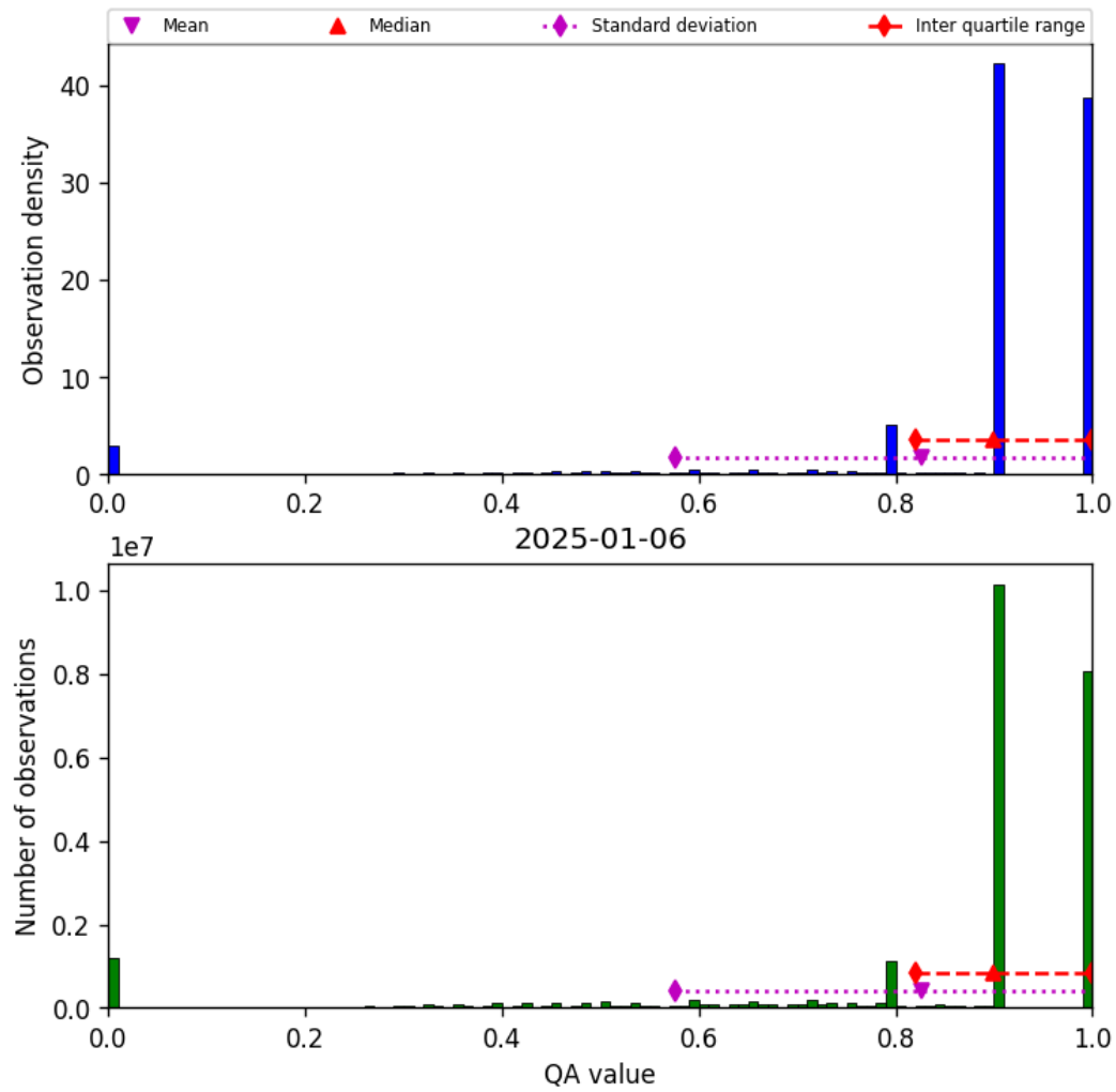
Figure 28: Histogram of “QA value” for 2025-01-06 to 2025-01-07
