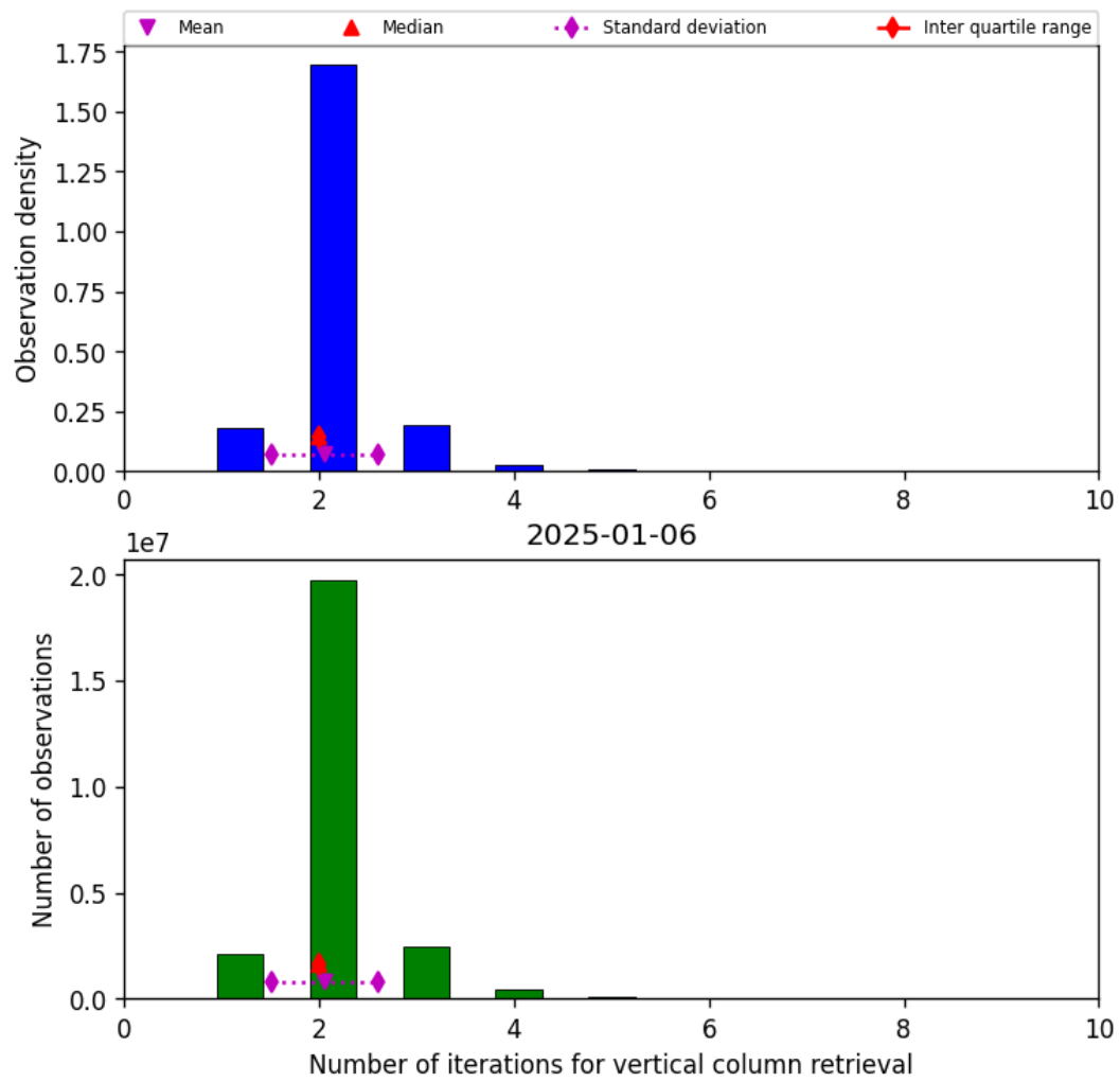
Figure 39: Histogram of “Number of iterations for vertical column retrieval” for 2025-01-06 to 2025-01-07
