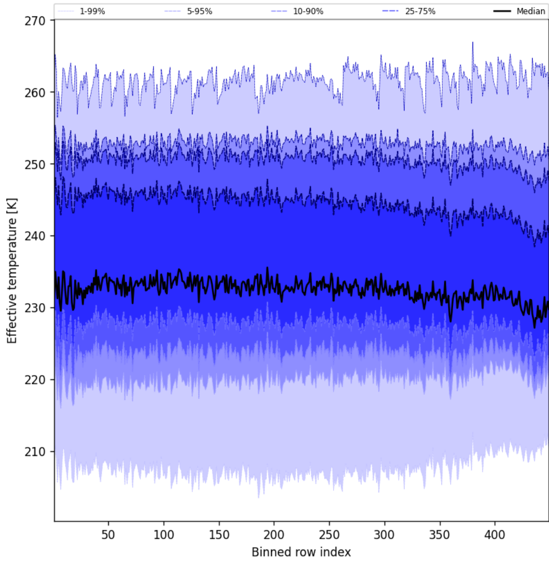
Figure 50: Along track statistics of “Effective temperature” for 2025-01-06 to 2025-01-07
