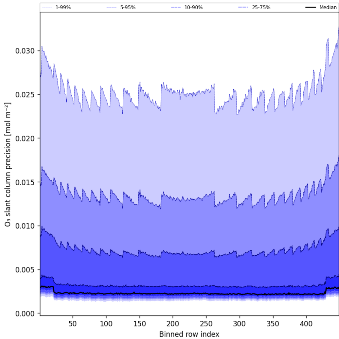
Figure 44: Along track statistics of “O 3 slant column precision” for 2025-01-06 to 2025-01-07
