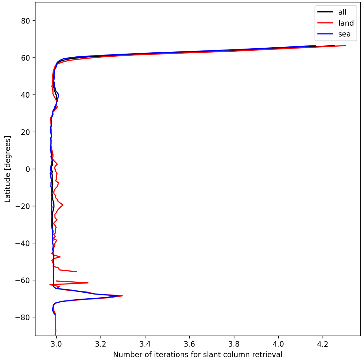
Figure 21: Zonal average of “Number of iterations for slant column retrieval” for 2025-01-06 to 2025-01-07.
