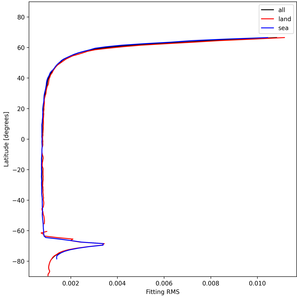
Figure 22: Zonal average of “Fitting RMS” for 2025-01-07 to 2025-01-08.
