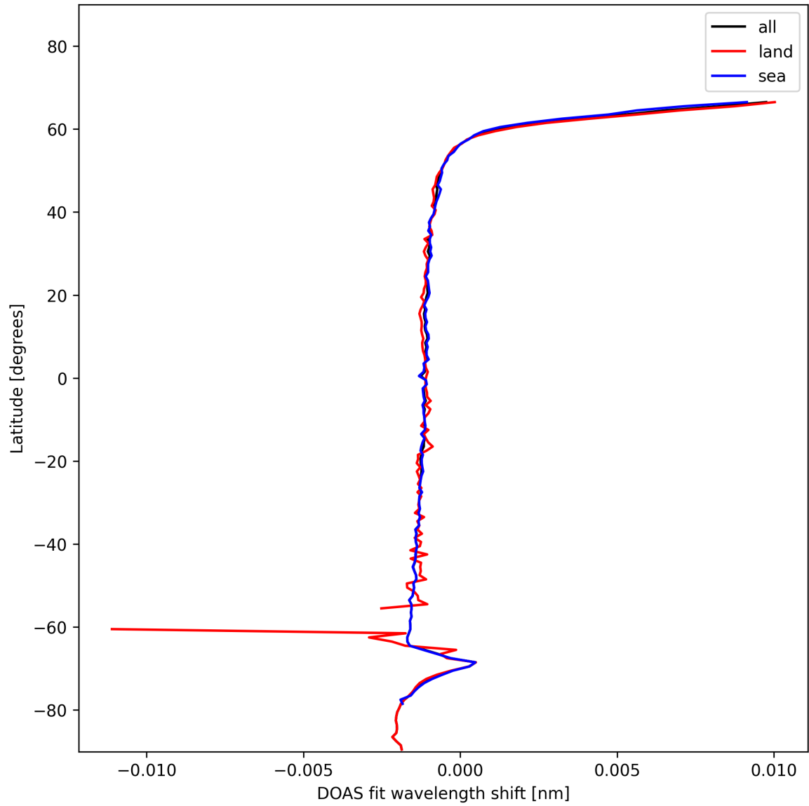
Figure 23: Zonal average of "DOAS fit wavelength shift" for 2025-01-07 to 2025-01-08.
