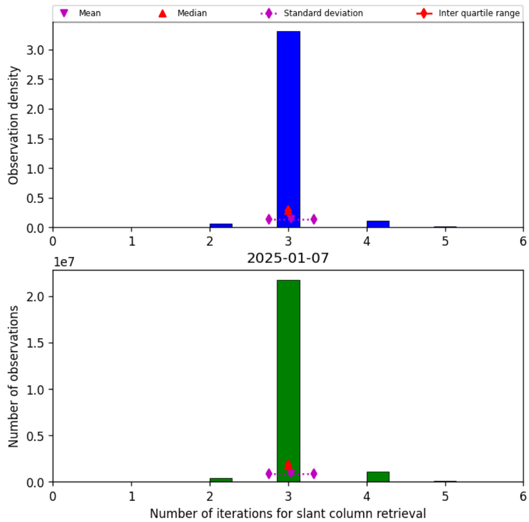
Figure 33: Histogram of “Number of iterations for slant column retrieval” for 2025-01-07 to 2025-01-08
