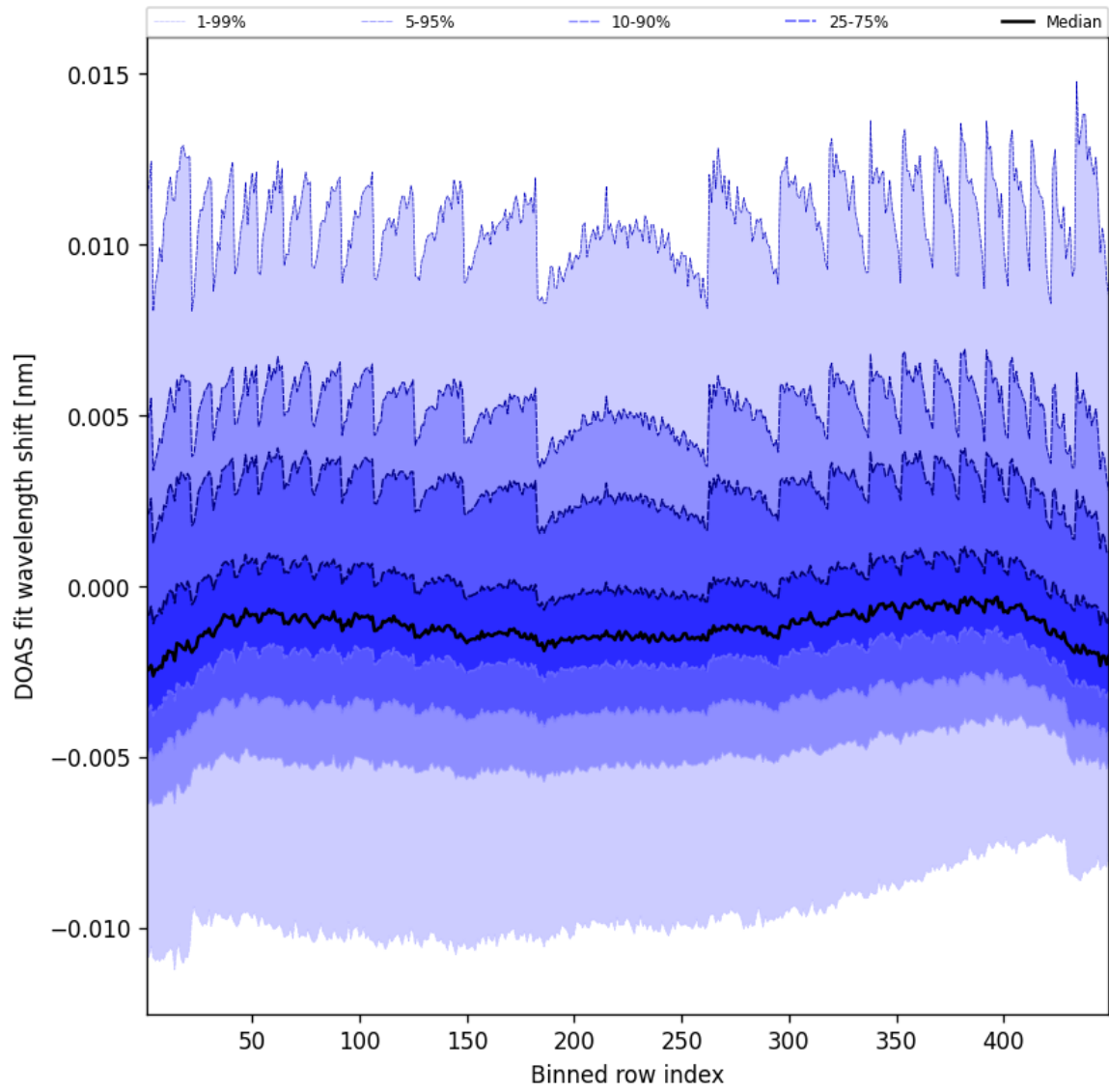
Figure 47: Along track statistics of “DOAS fit wavelength shift” for 2025-01-07 to 2025-01-08
