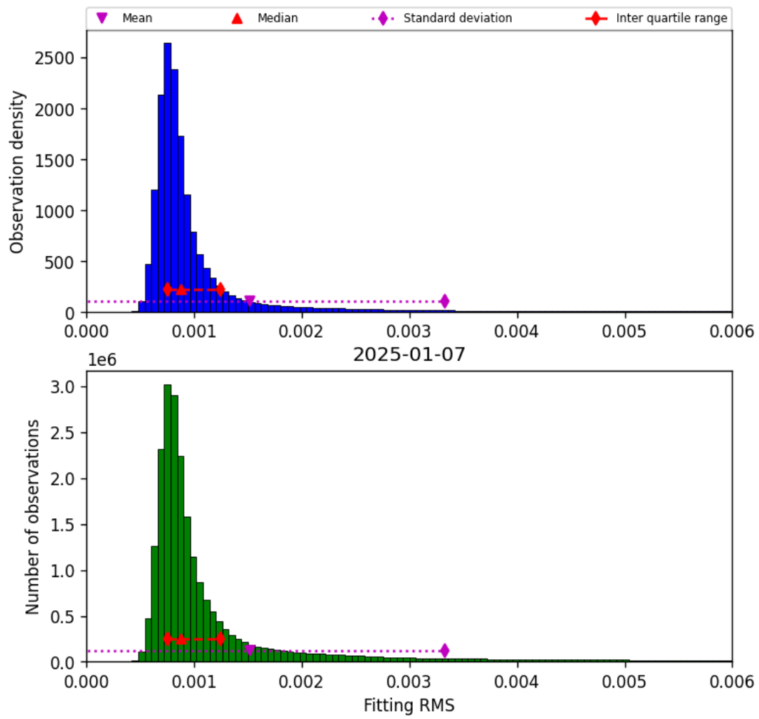
Figure 34: Histogram of “Fitting RMS” for 2025-01-07 to 2025-01-08
