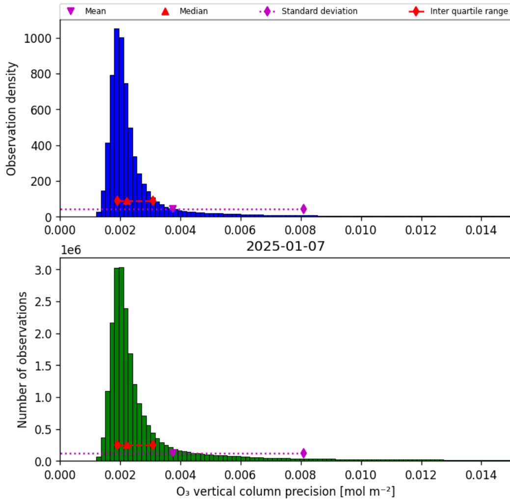
Figure 30: Histogram of “O 3 vertical column precision” for 2025-01-07 to 2025-01-08
