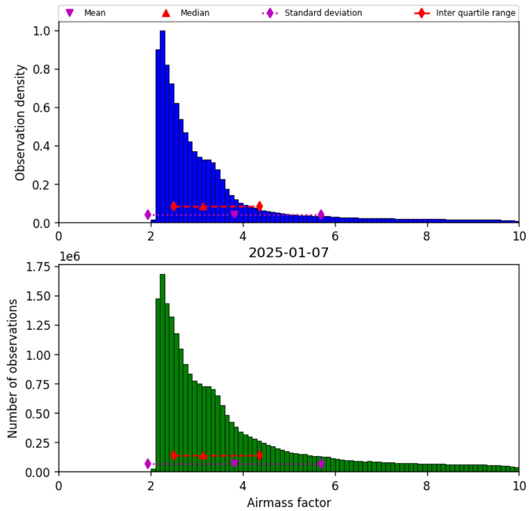
Figure 37: Histogram of “Airmass factor” for 2025-01-07 to 2025-01-08
