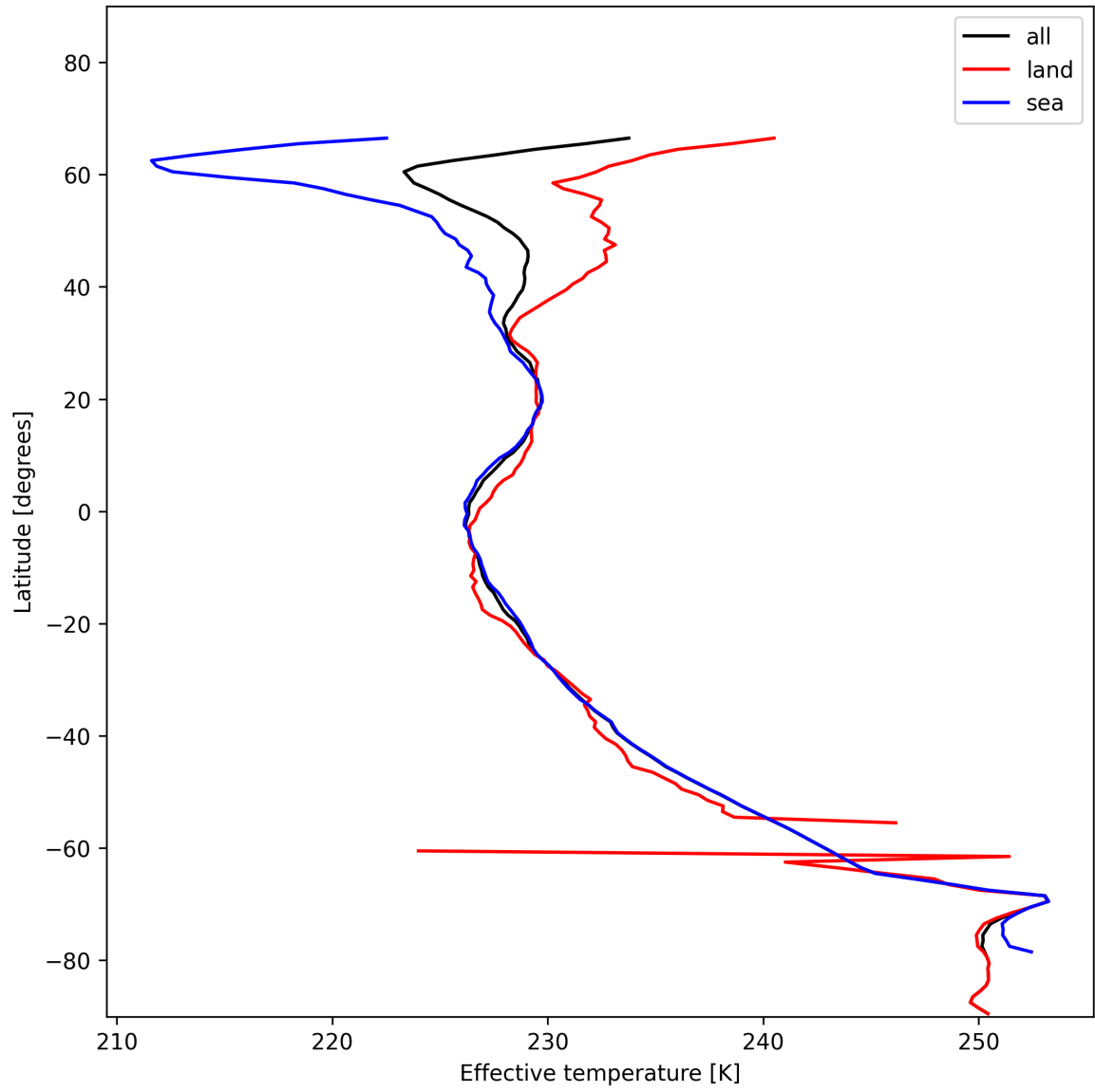
Figure 26: Zonal average of “Effective temperature” for 2025-01-07 to 2025-01-08.
