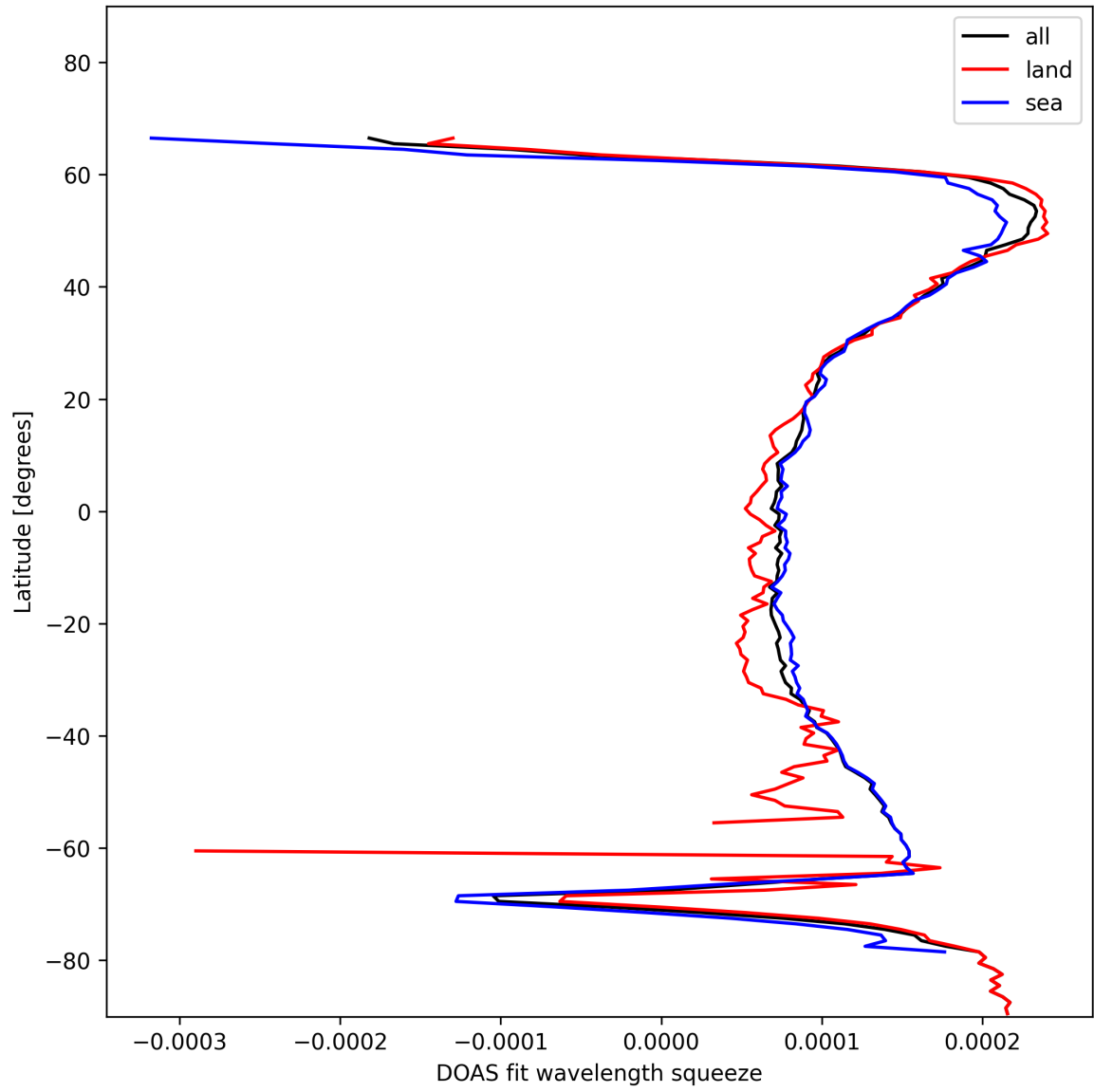
Figure 24: Zonal average of “DOAS fit wavelength squeeze” for 2025-01-07 to 2025-01-08.
