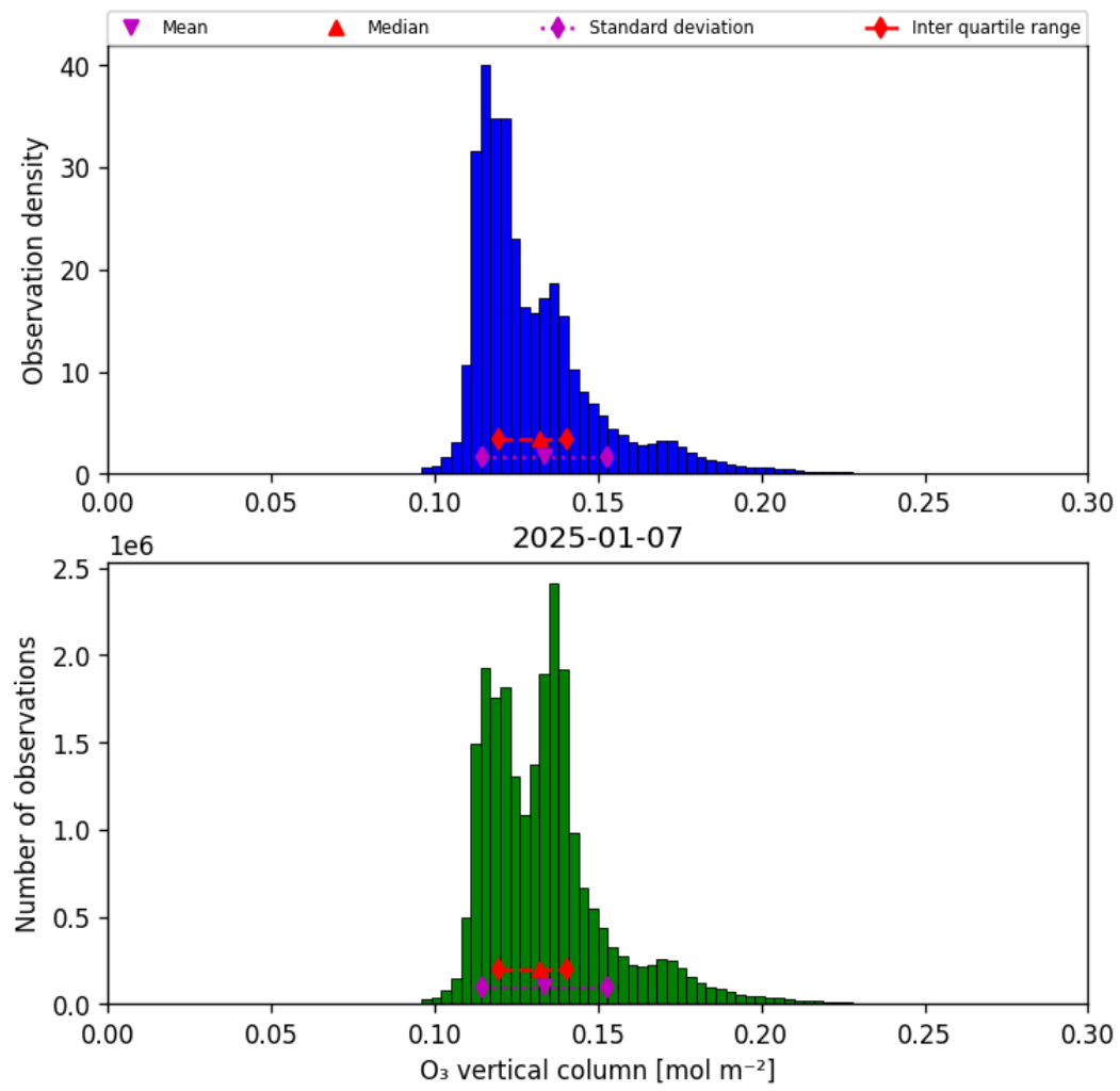
Figure 29: Histogram of “O 3 vertical column” for 2025-01-07 to 2025-01-08
