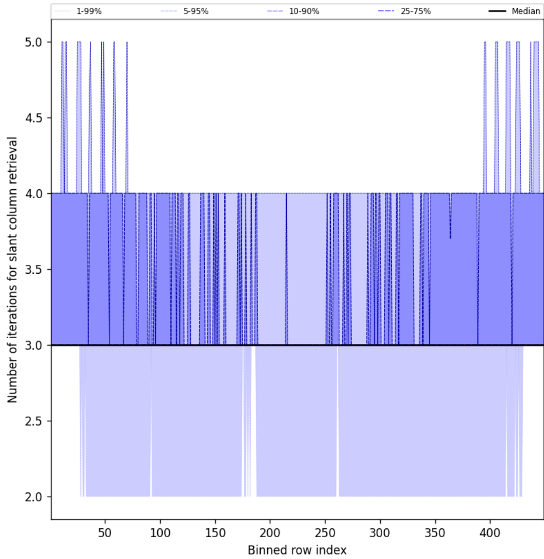
Figure 45: Along track statistics of “Number of iterations for slant column retrieval” for 2025-01-07 to 2025-01-08
