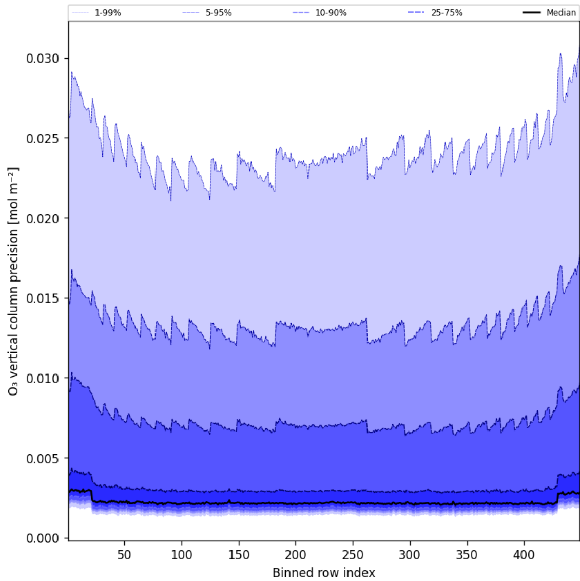
Figure 42: Along track statistics of “O 3 vertical column precision” for 2025-01-07 to 2025-01-08
