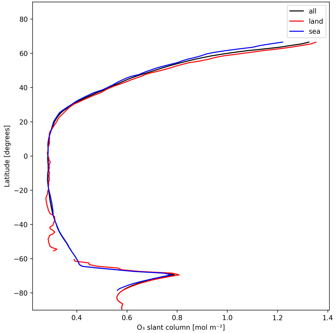
Figure 19: Zonal average of “O 3 slant column” for 2025-01-07 to 2025-01-08.
