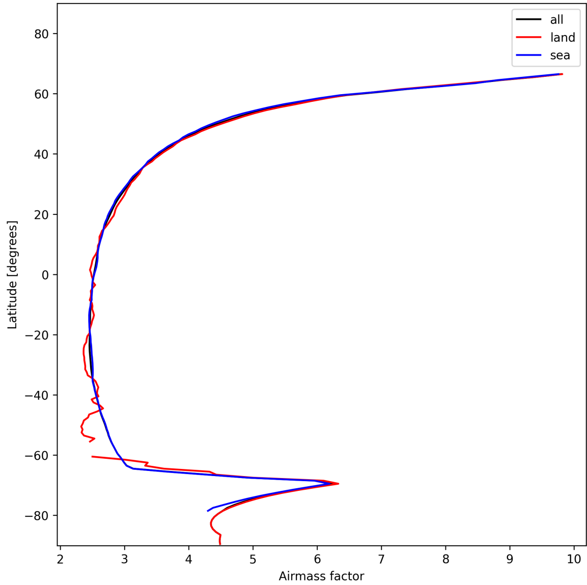
Figure 25: Zonal average of “Airmass factor” for 2025-01-07 to 2025-01-08.
