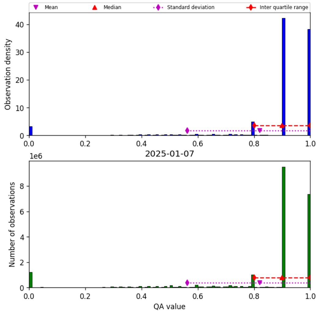
Figure 28: Histogram of “QA value” for 2025-01-07 to 2025-01-08
