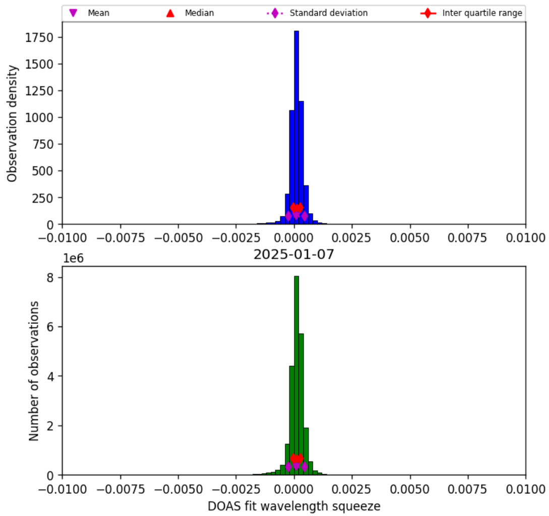
Figure 36: Histogram of “DOAS fit wavelength squeeze” for 2025-01-07 to 2025-01-08
