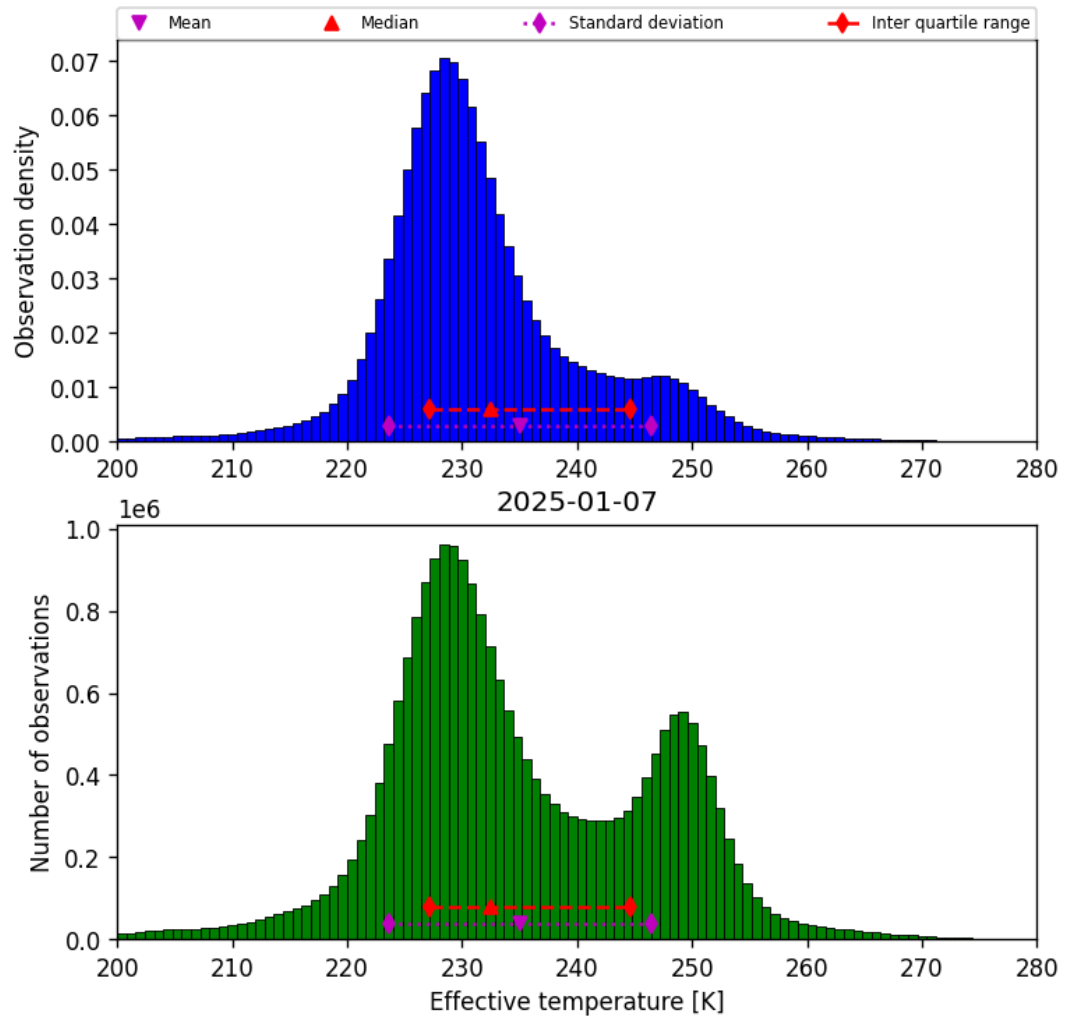
Figure 38: Histogram of “Effective temperature” for 2025-01-07 to 2025-01-08
