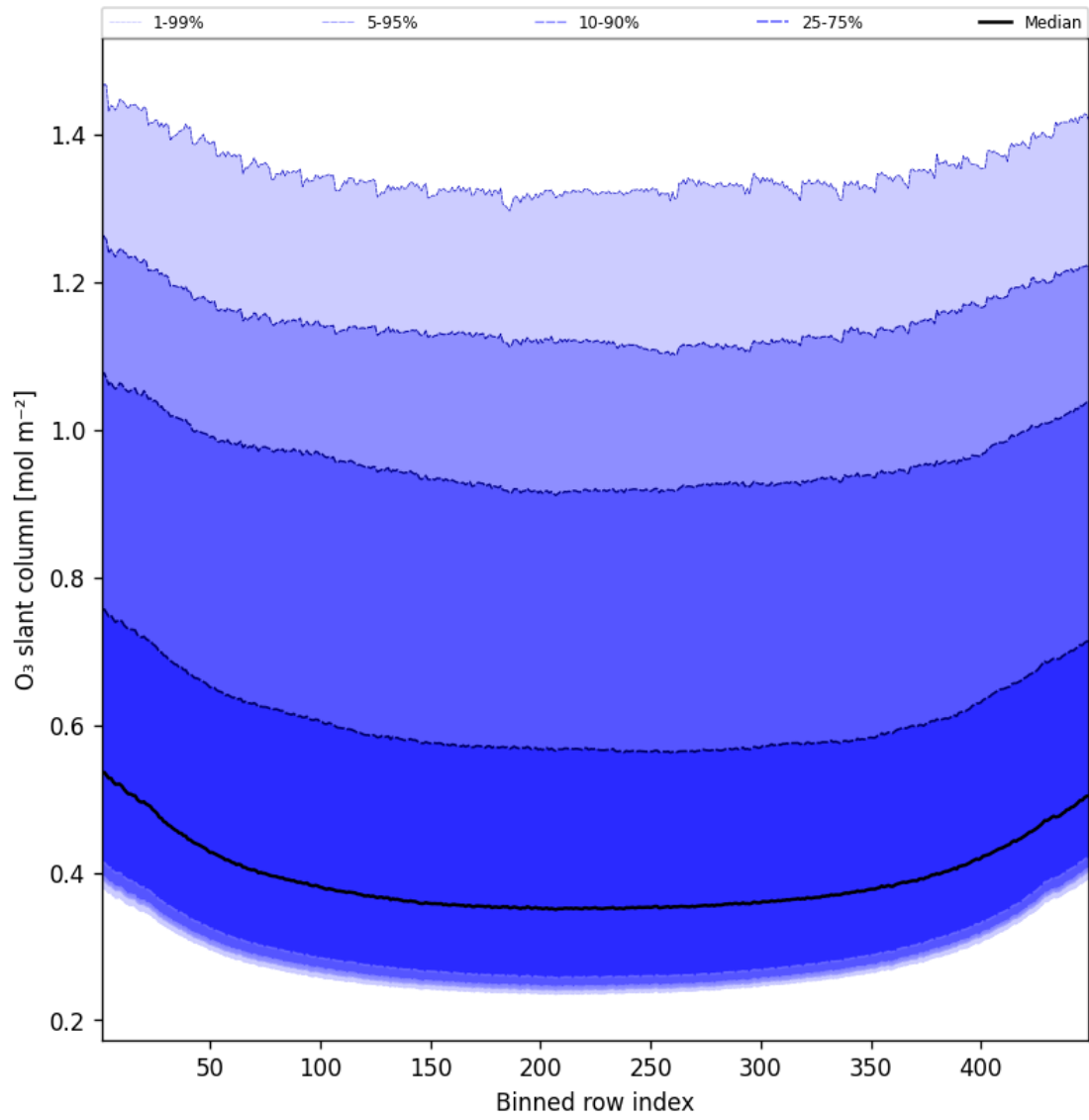
Figure 43: Along track statistics of “O 3 slant column” for 2025-01-07 to 2025-01-08
