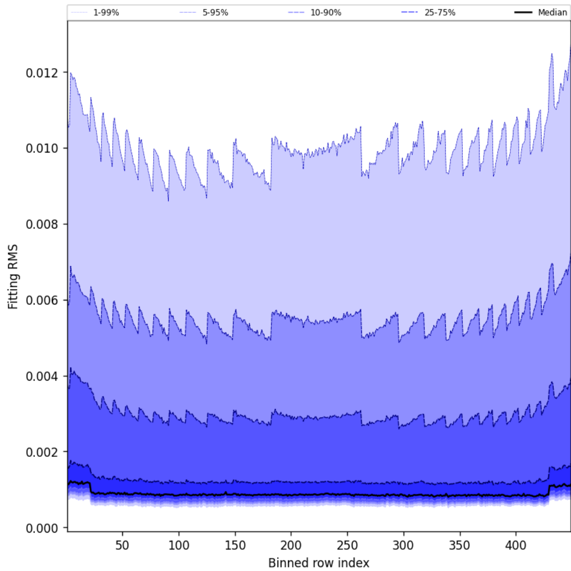
Figure 46: Along track statistics of “Fitting RMS” for 2025-01-07 to 2025-01-08
