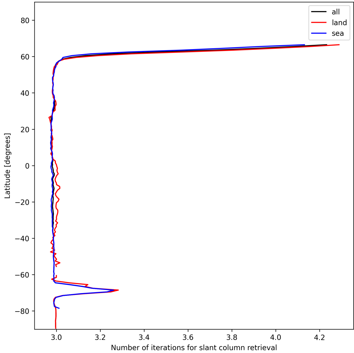
Figure 21: Zonal average of “Number of iterations for slant column retrieval” for 2025-01-07 to 2025-01-08.
