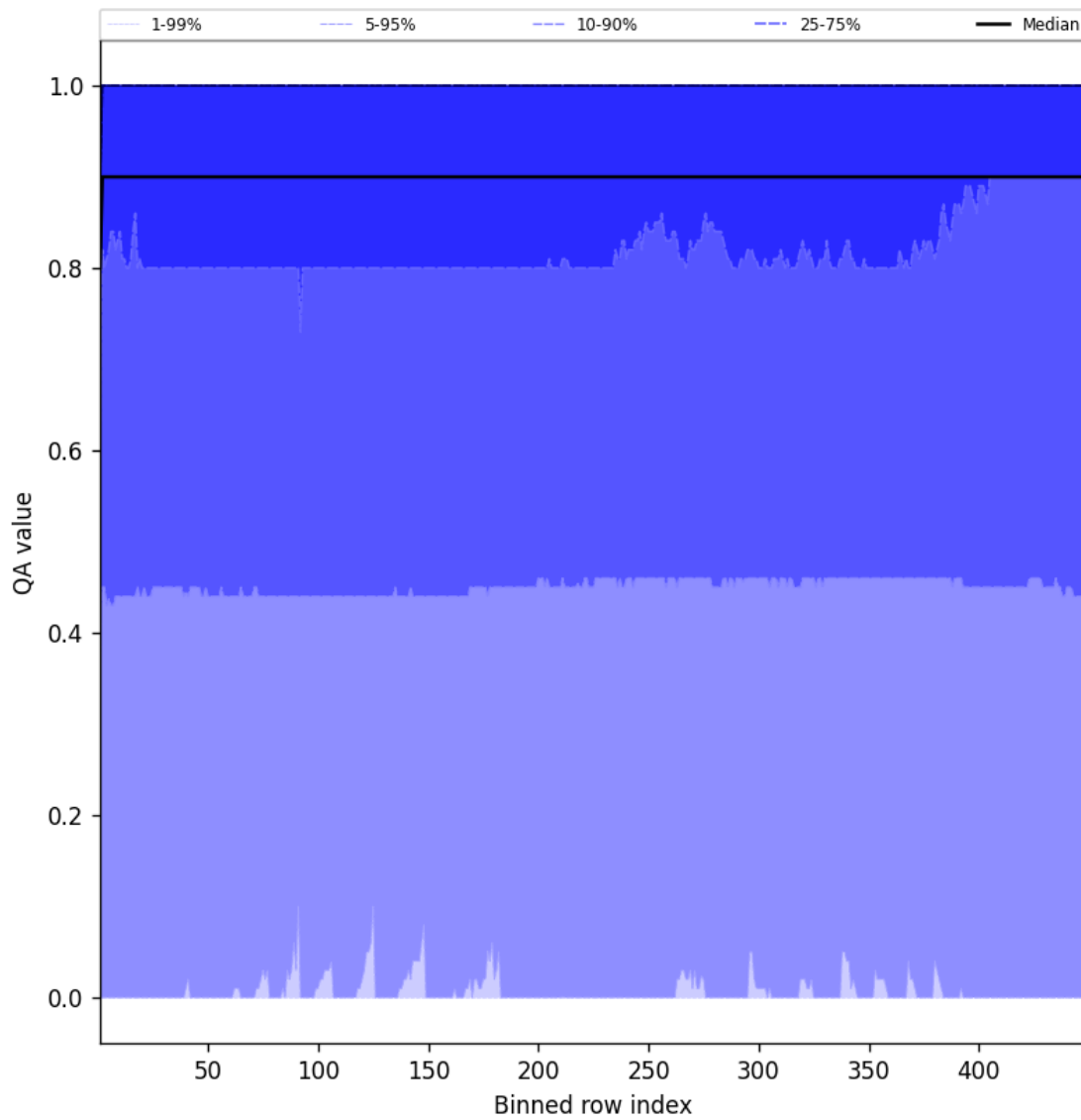
Figure 40: Along track statistics of “QA value” for 2025-01-07 to 2025-01-08
