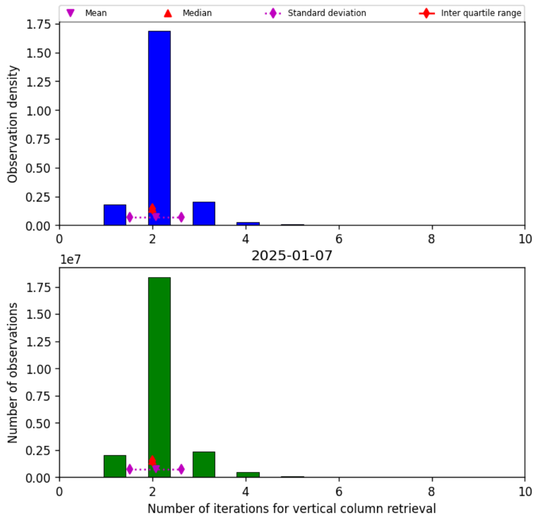
Figure 39: Histogram of “Number of iterations for vertical column retrieval” for 2025-01-07 to 2025-01-08
