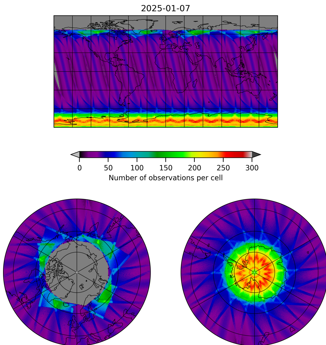
Figure 15: Map of the number of observations for 2025-01-07 to 2025-01-08
