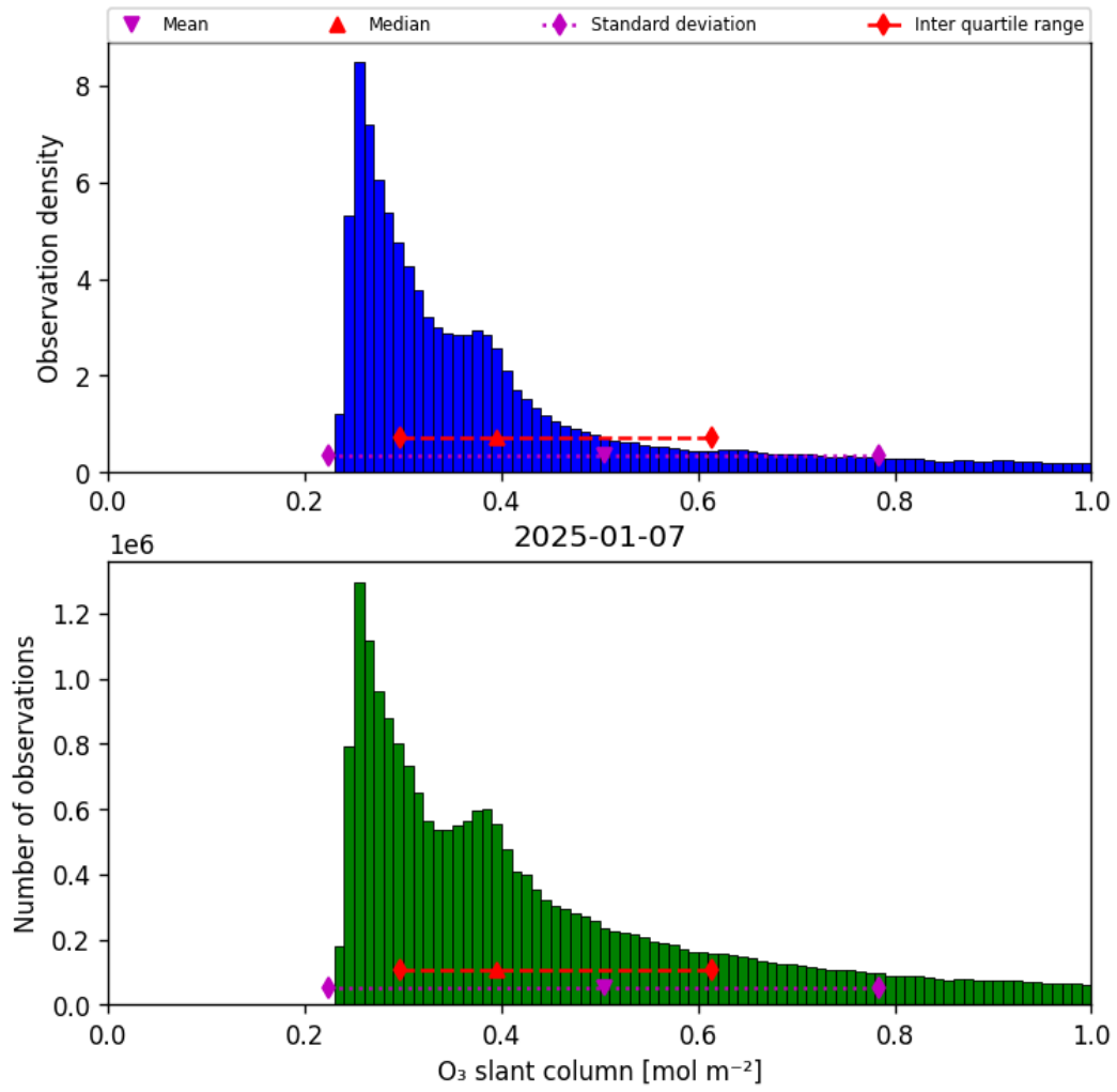
Figure 31: Histogram of “O 3 slant column” for 2025-01-07 to 2025-01-08
