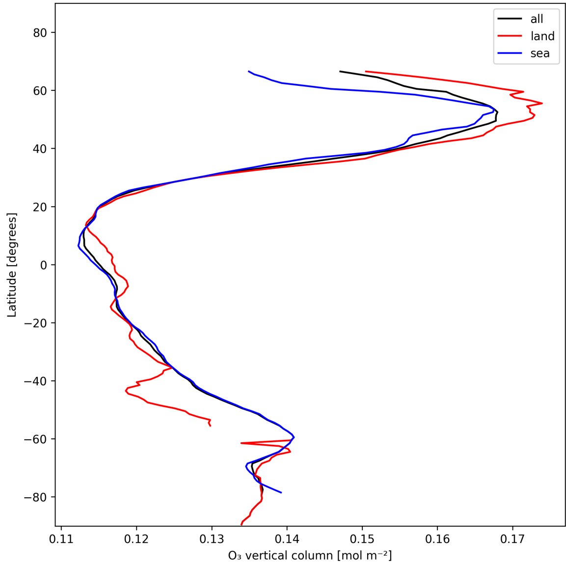
Figure 17: Zonal average of “O 3 vertical column” for 2025-01-07 to 2025-01-08.
