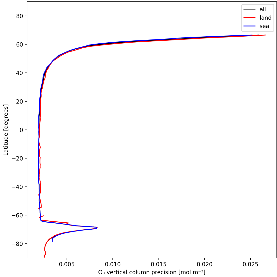
Figure 18: Zonal average of “O 3 vertical column precision” for 2025-01-07 to 2025-01-08.
