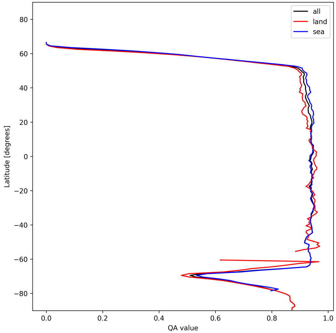
Figure 16: Zonal average of "QA value" for 2025-01-07 to 2025-01-08.
