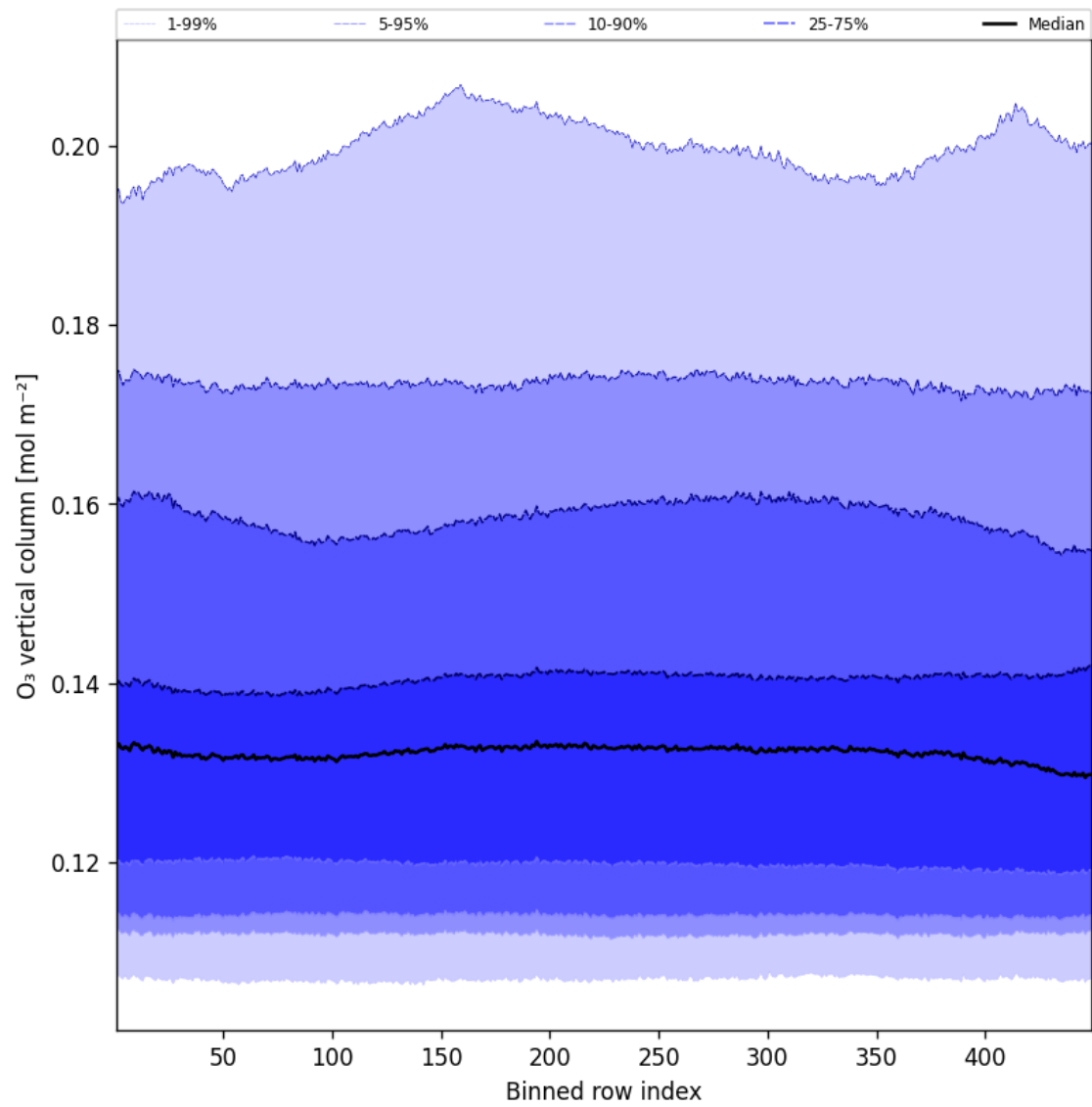
Figure 41: Along track statistics of “O 3 vertical column” for 2025-01-07 to 2025-01-08
