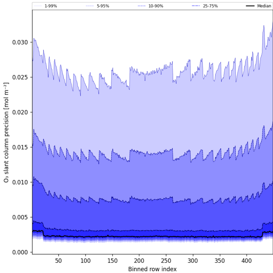
Figure 44: Along track statistics of “O 3 slant column precision” for 2025-01-07 to 2025-01-08
