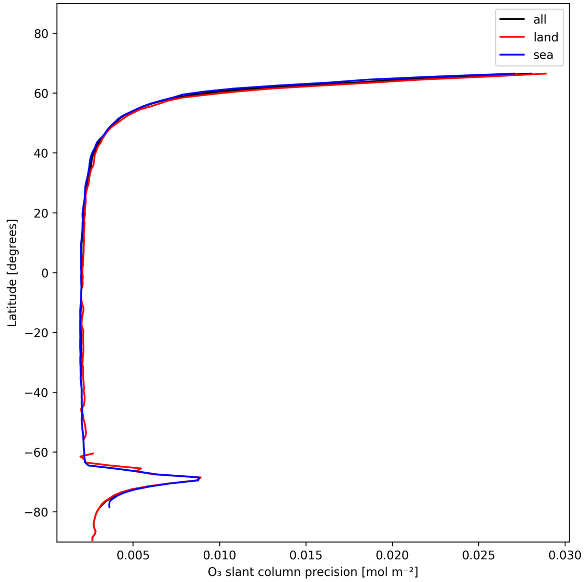
Figure 20: Zonal average of “O 3 slant column precision” for 2025-01-07 to 2025-01-08.
