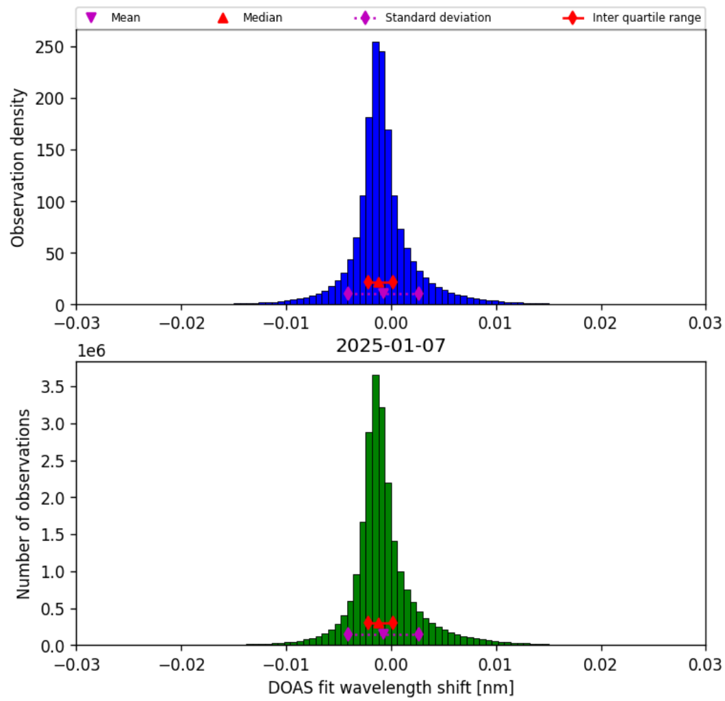
Figure 35: Histogram of “DOAS fit wavelength shift” for 2025-01-07 to 2025-01-08
