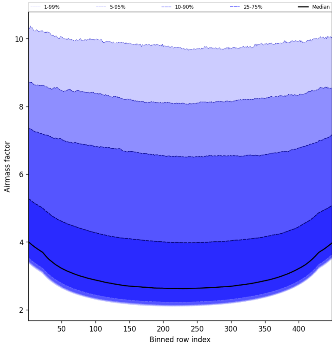
Figure 49: Along track statistics of “Airmass factor” for 2025-01-07 to 2025-01-08
