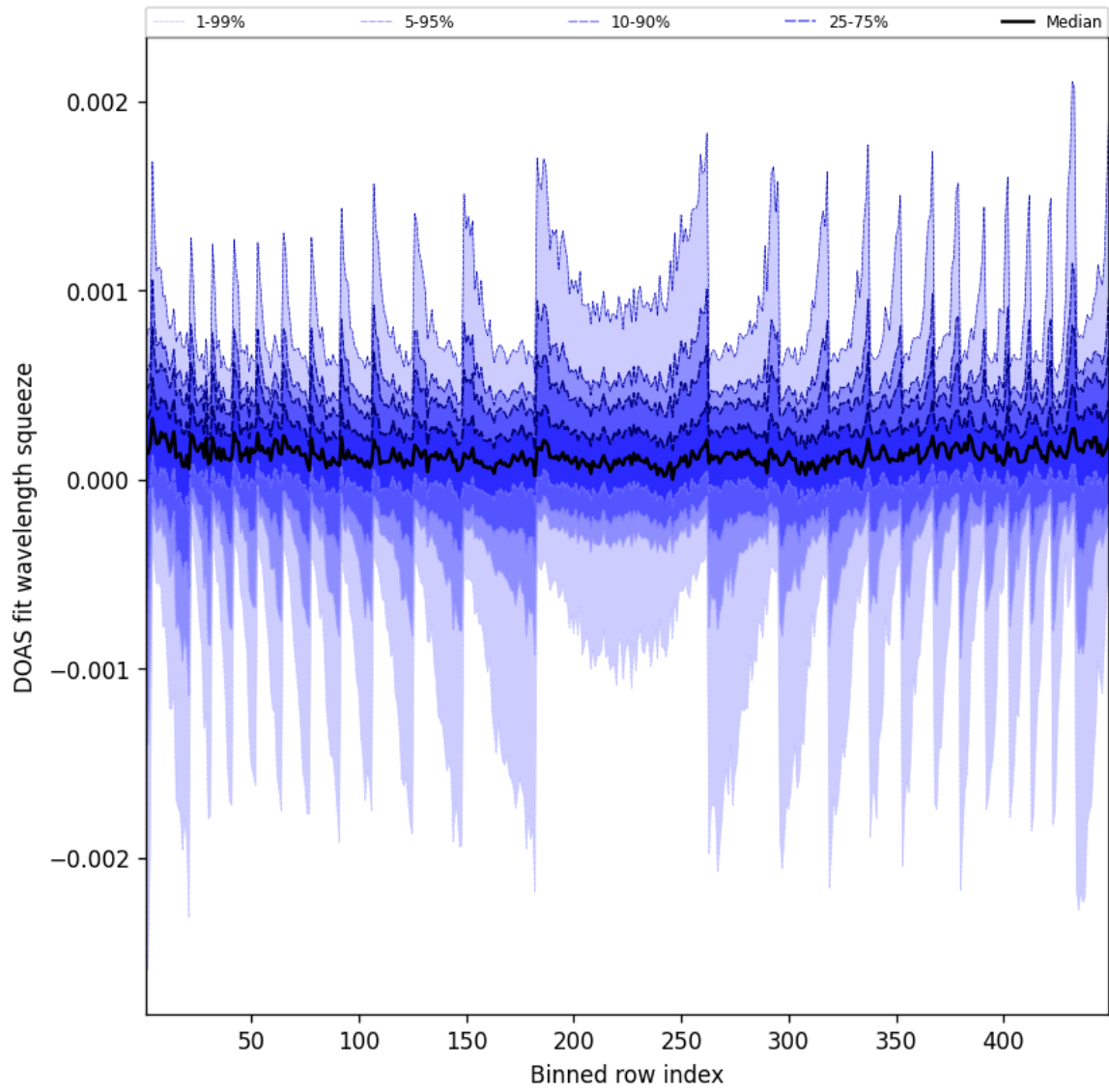
Figure 48: Along track statistics of “DOAS fit wavelength squeeze” for 2025-01-07 to 2025-01-08
