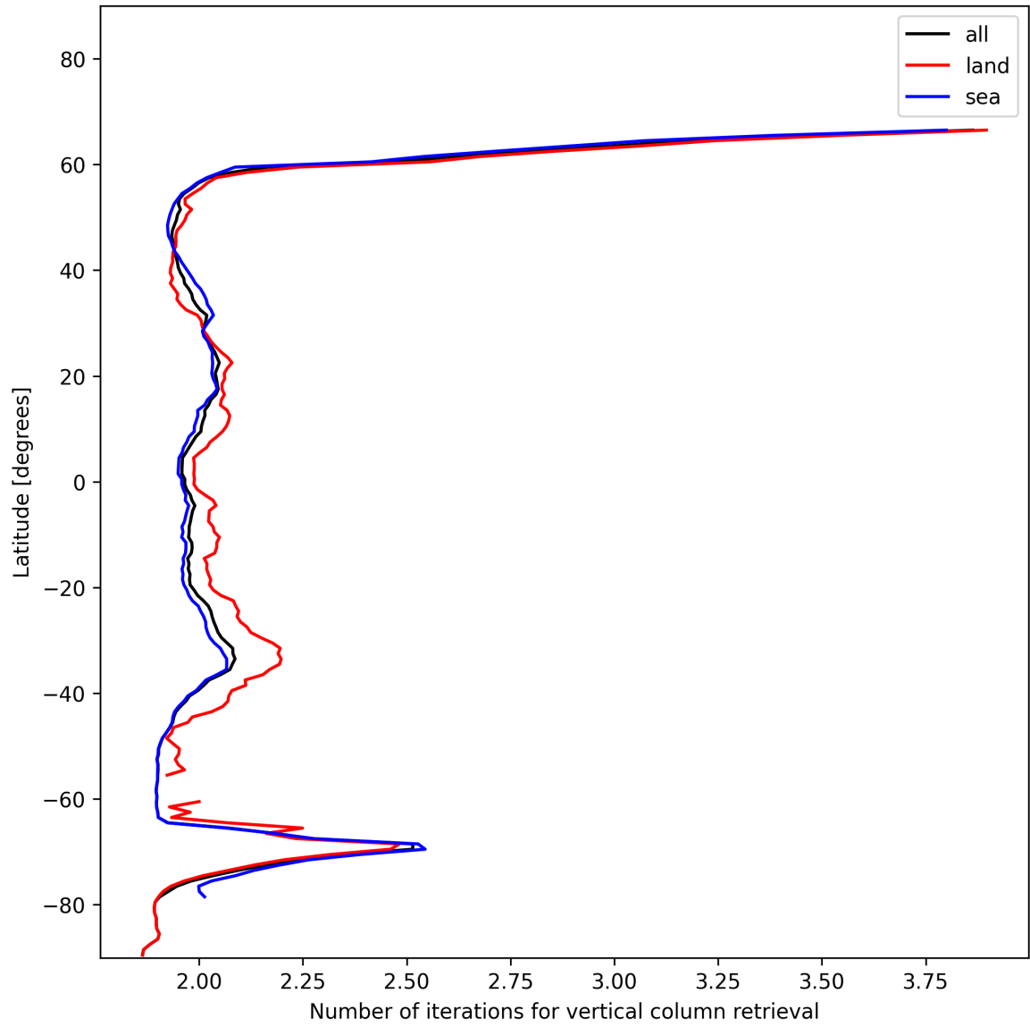
Figure 27: Zonal average of “Number of iterations for vertical column retrieval” for 2025-01-07 to 2025-01-08.
