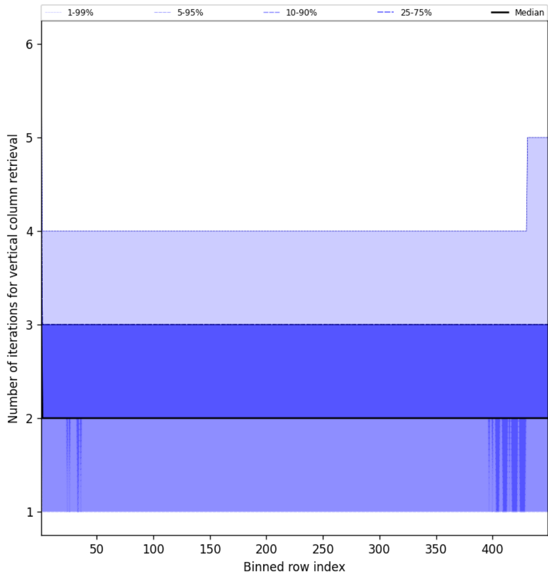
Figure 51: Along track statistics of “Number of iterations for vertical column retrieval” for 2025-01-07 to 2025-01-08
