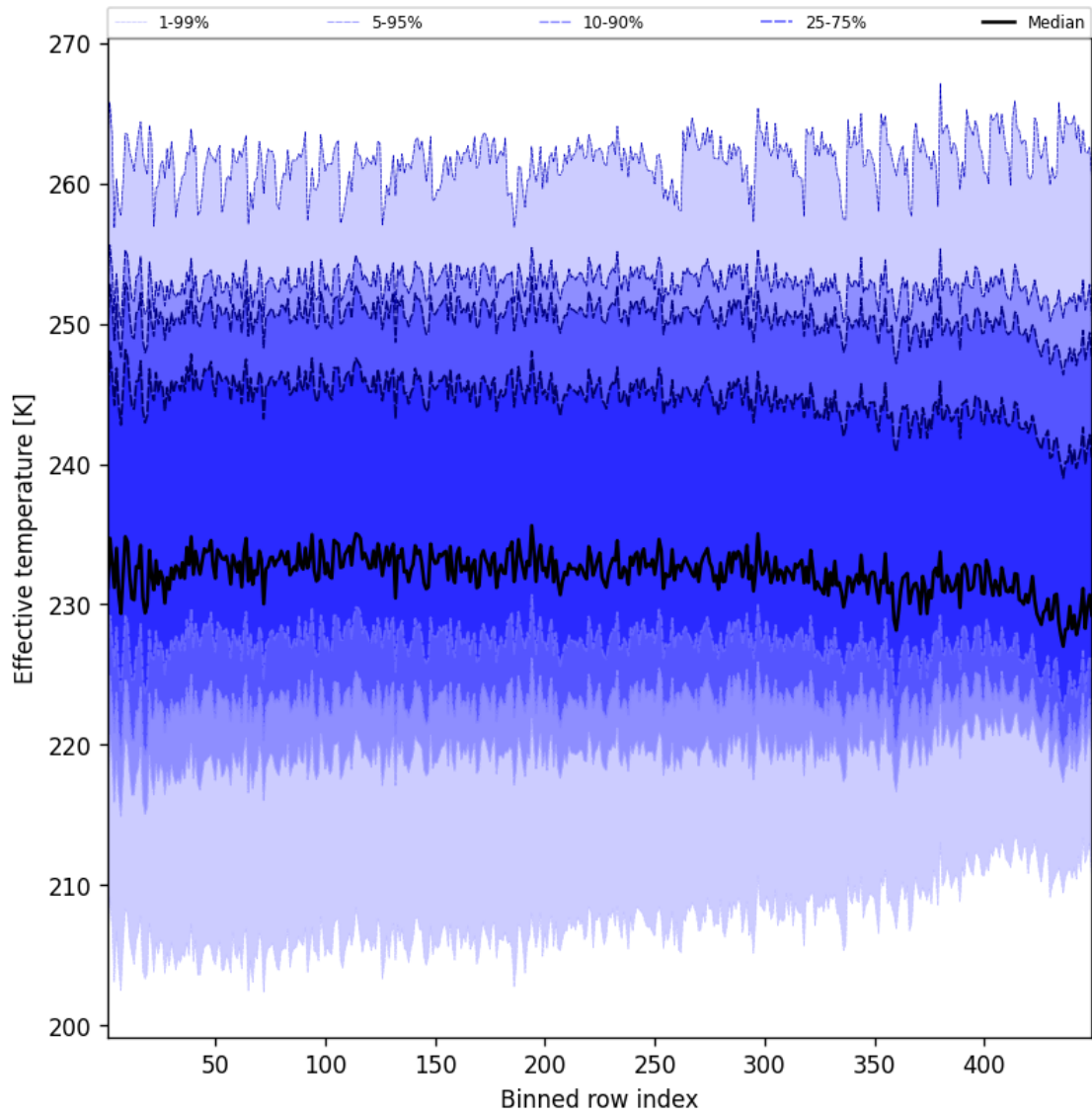
Figure 50: Along track statistics of “Effective temperature” for 2025-01-07 to 2025-01-08
