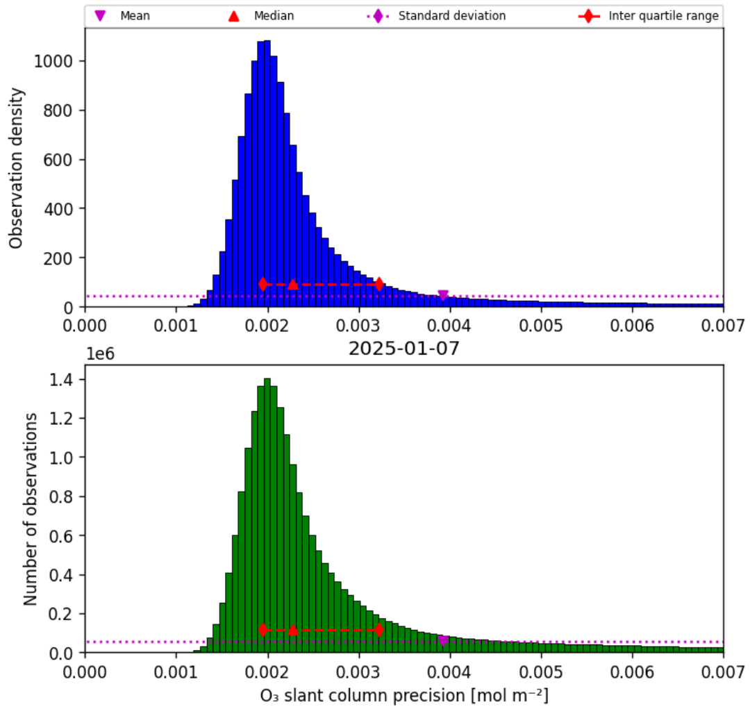
Figure 32: Histogram of “O 3 slant column precision” for 2025-01-07 to 2025-01-08
