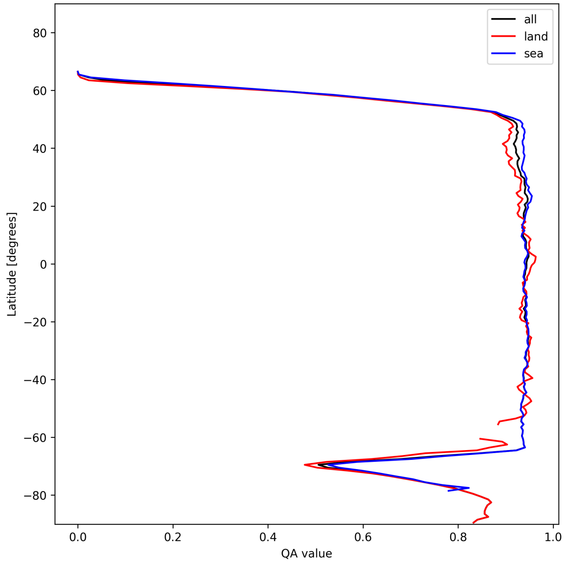
Figure 16: Zonal average of “QA value” for 2025-01-08 to 2025-01-09.
