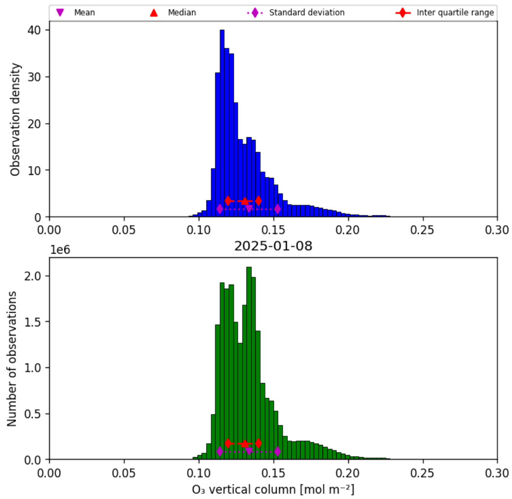
Figure 29: Histogram of “O 3 vertical column” for 2025-01-08 to 2025-01-09
