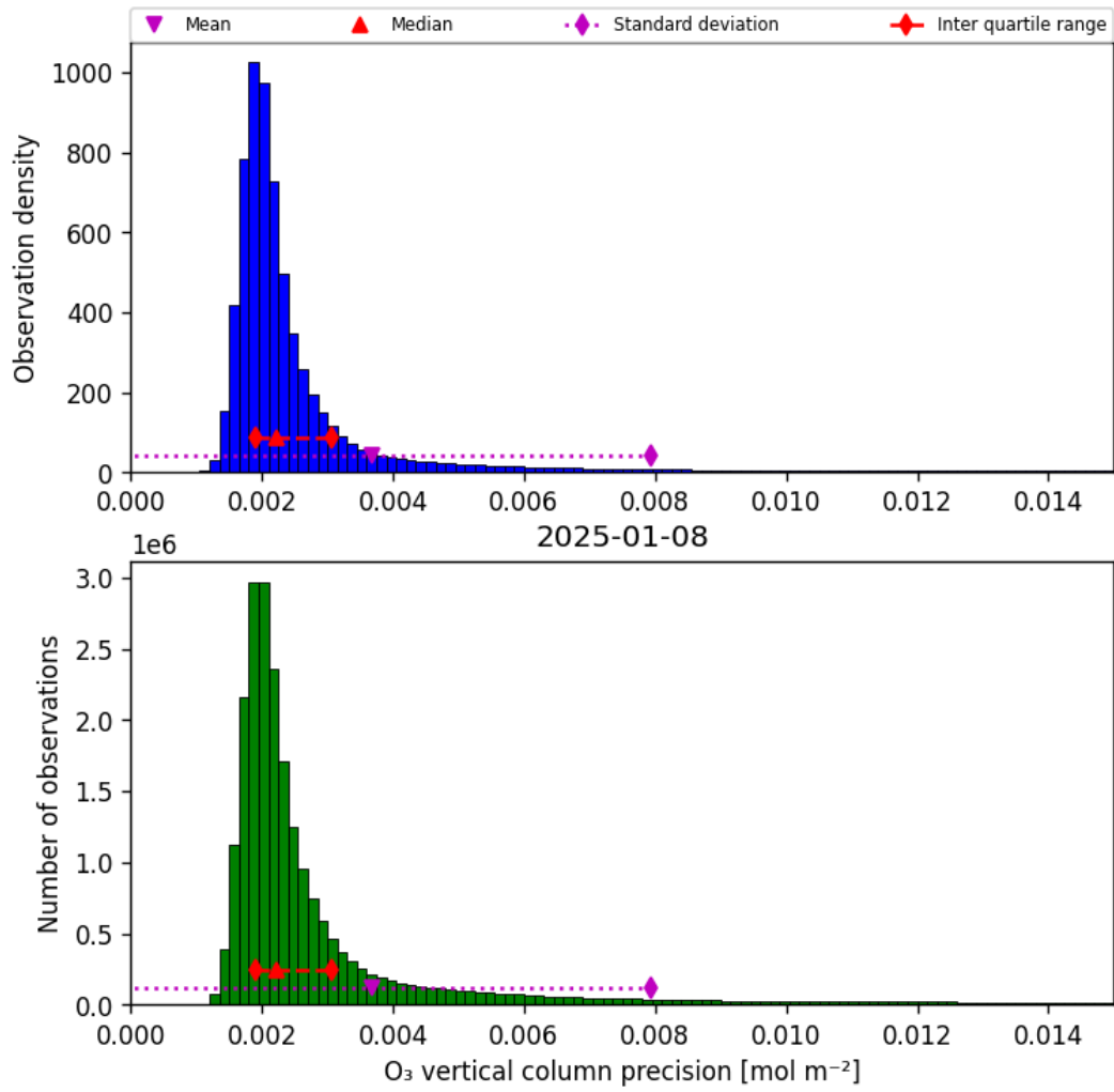
Figure 30: Histogram of “O 3 vertical column precision” for 2025-01-08 to 2025-01-09
