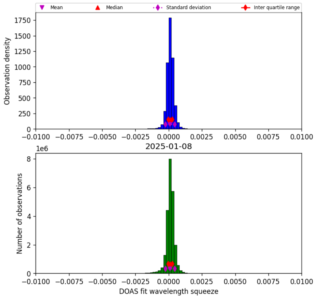
Figure 36: Histogram of “DOAS fit wavelength squeeze” for 2025-01-08 to 2025-01-09
