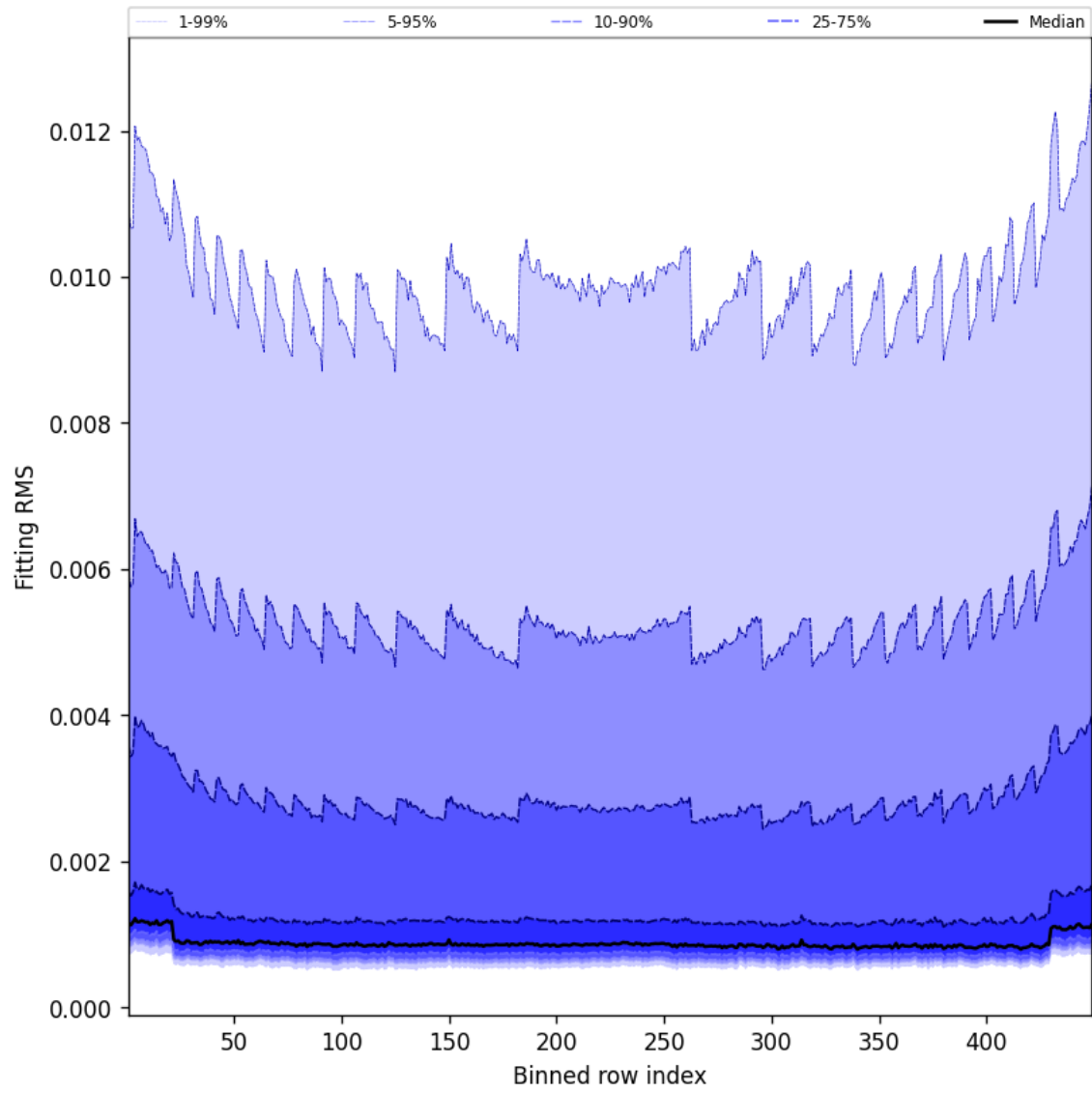
Figure 46: Along track statistics of “Fitting RMS” for 2025-01-08 to 2025-01-09
