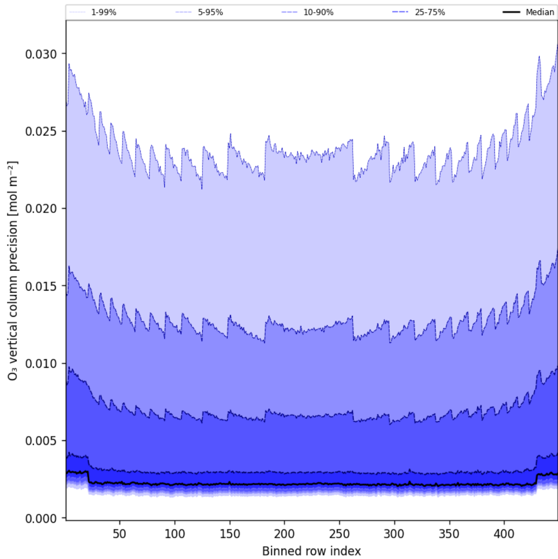
Figure 42: Along track statistics of “O 3 vertical column precision” for 2025-01-08 to 2025-01-09
