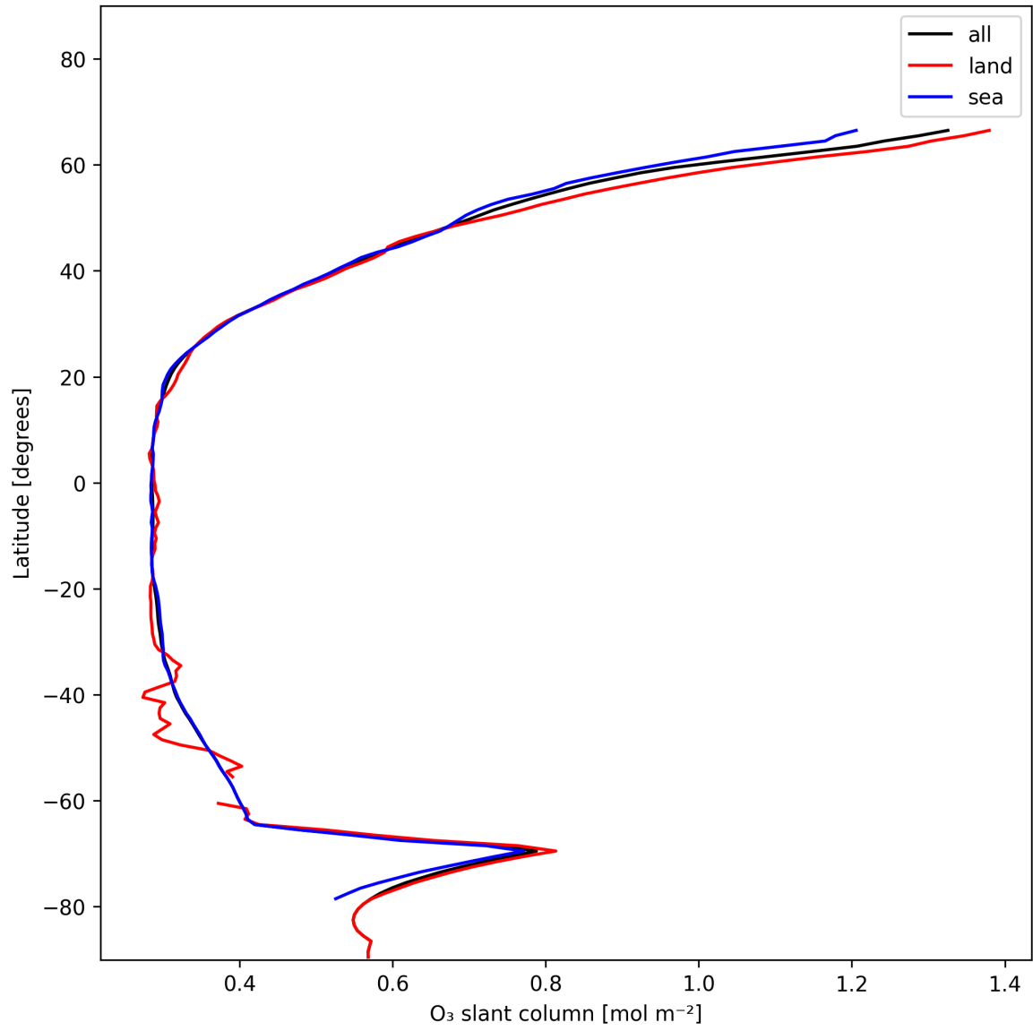
Figure 19: Zonal average of “O 3 slant column” for 2025-01-08 to 2025-01-09.
