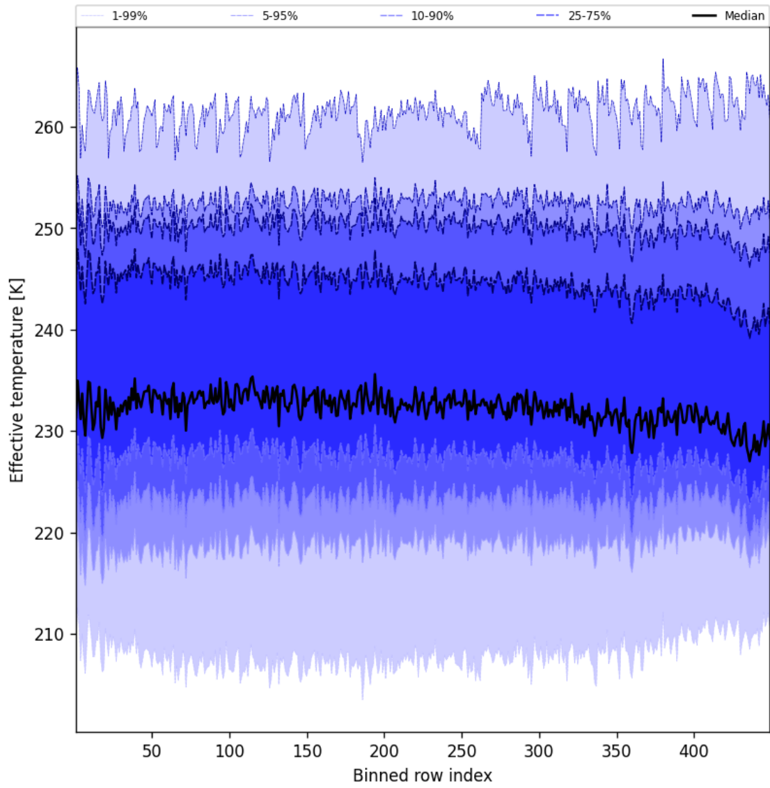
Figure 50: Along track statistics of “Effective temperature” for 2025-01-08 to 2025-01-09
