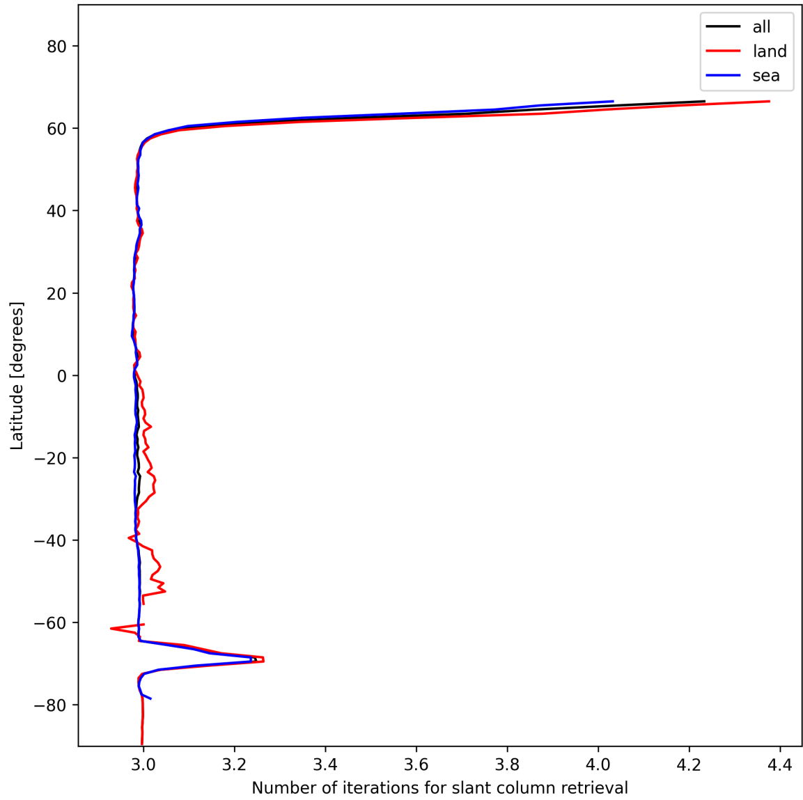
Figure 21: Zonal average of “Number of iterations for slant column retrieval” for 2025-01-08 to 2025-01-09.
