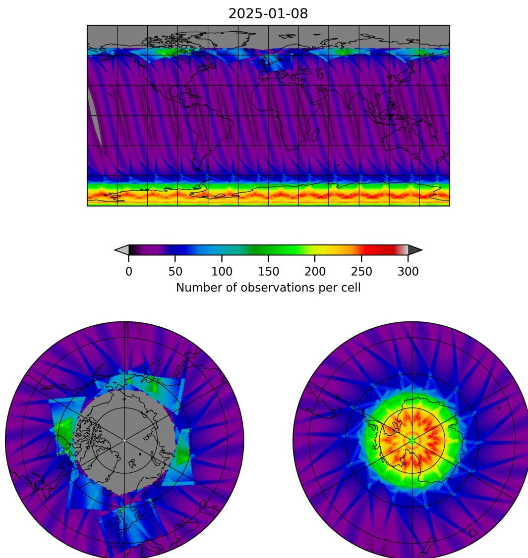
Figure 15: Map of the number of observations for 2025-01-08 to 2025-01-09
