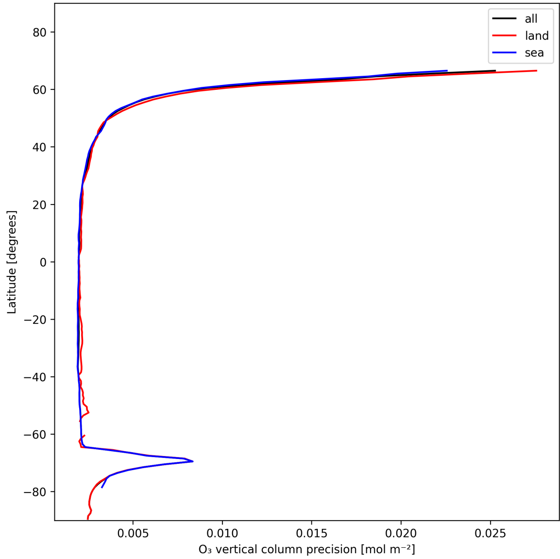
Figure 18: Zonal average of "O 3 vertical column precision" for 2025-01-08 to 2025-01-09.
