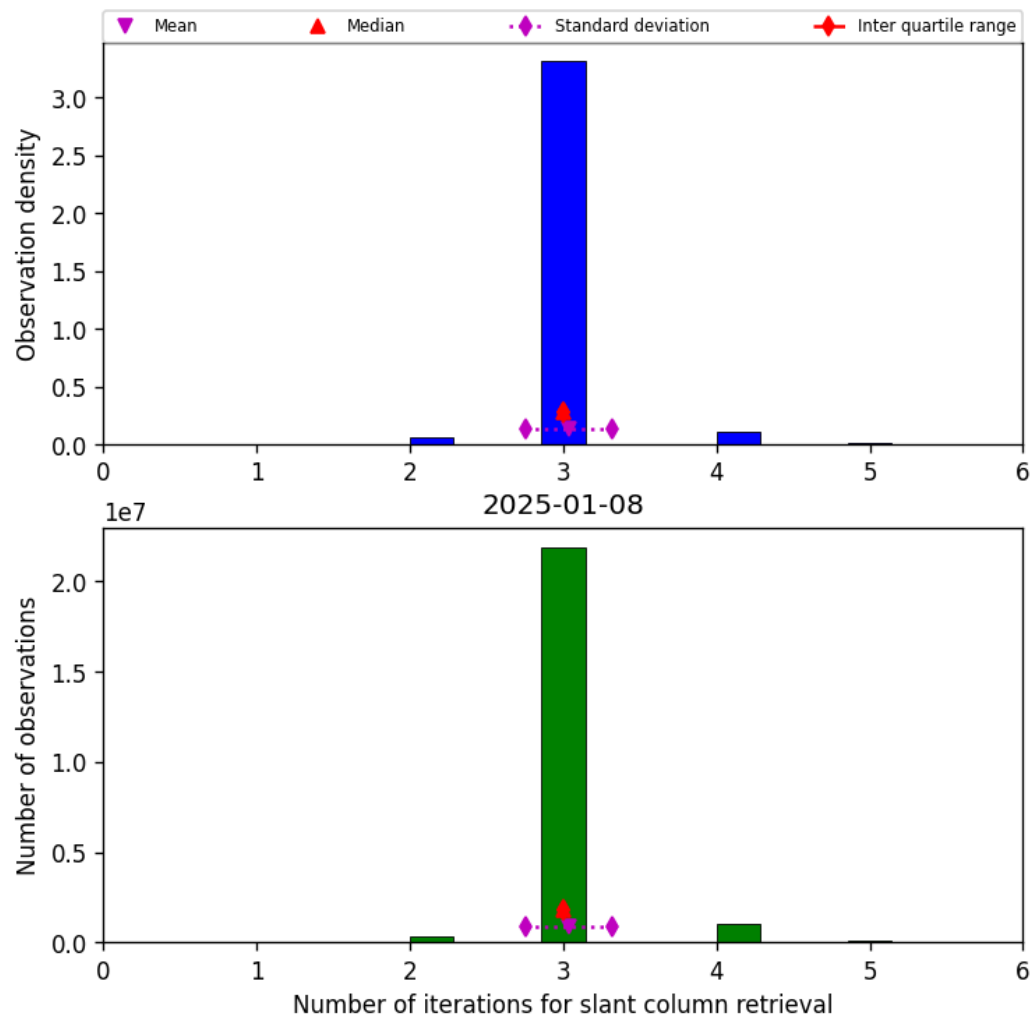
Figure 33: Histogram of “Number of iterations for slant column retrieval” for 2025-01-08 to 2025-01-09
