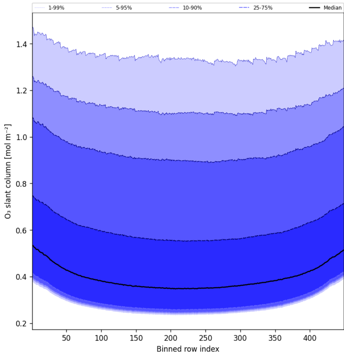
Figure 43: Along track statistics of “O 3 slant column” for 2025-01-08 to 2025-01-09
