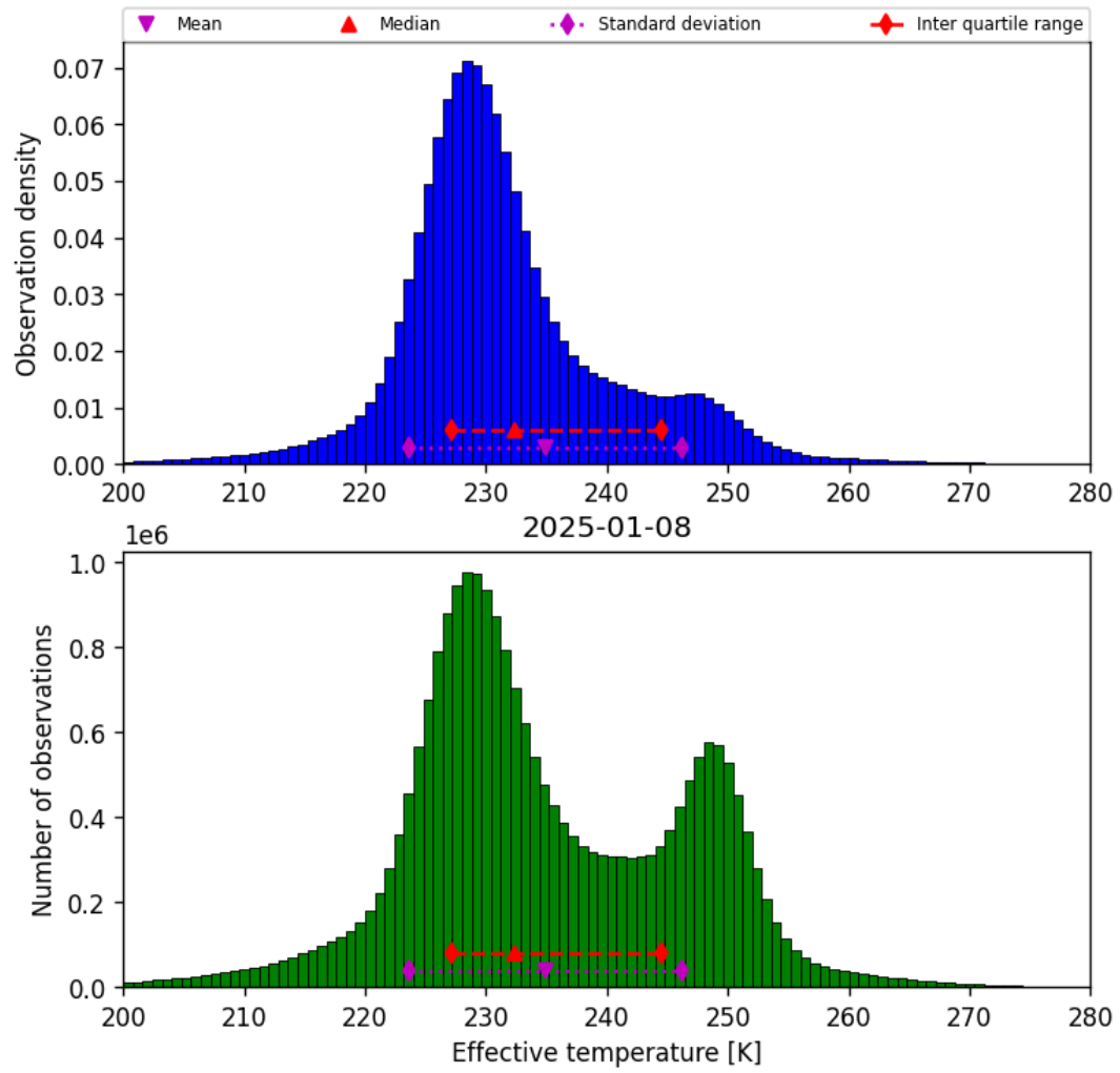
Figure 38: Histogram of “Effective temperature” for 2025-01-08 to 2025-01-09
