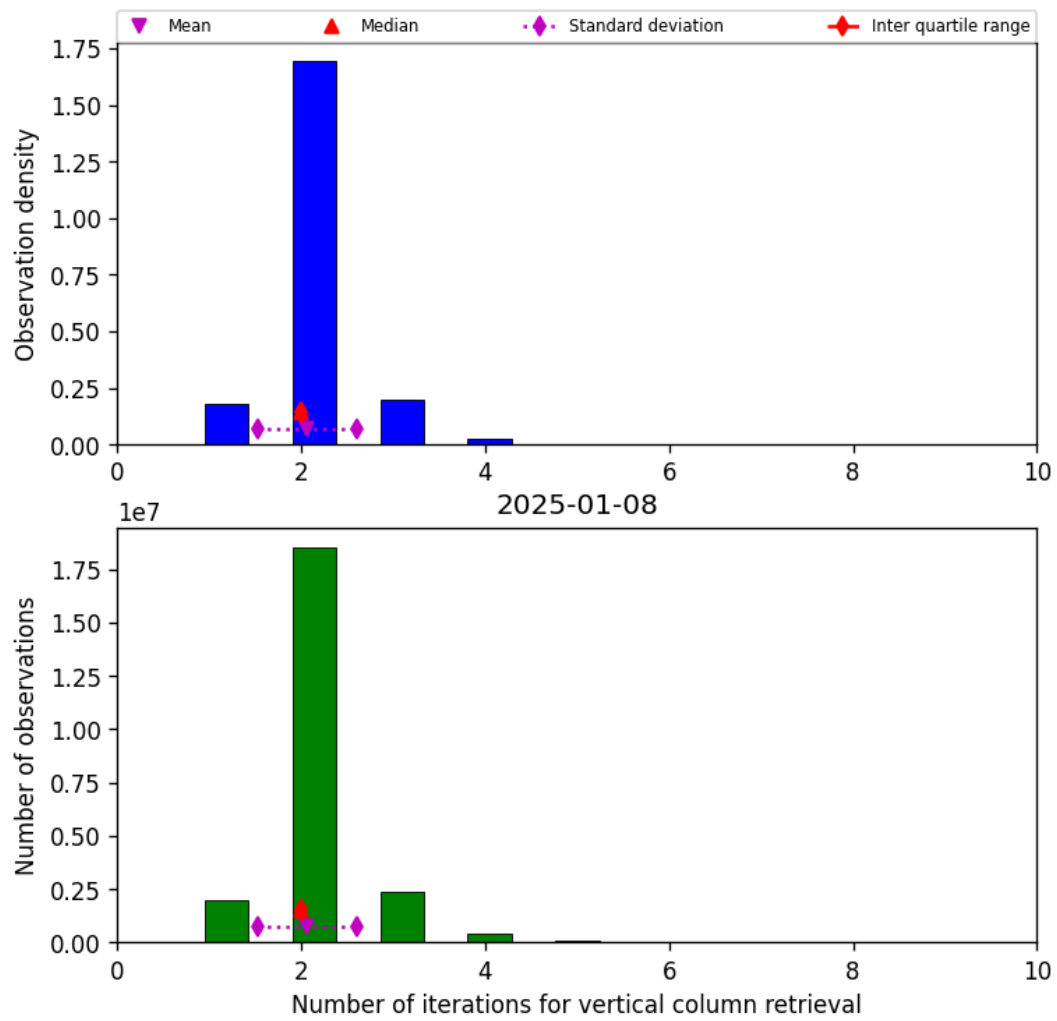
Figure 39: Histogram of “Number of iterations for vertical column retrieval” for 2025-01-08 to 2025-01-09
