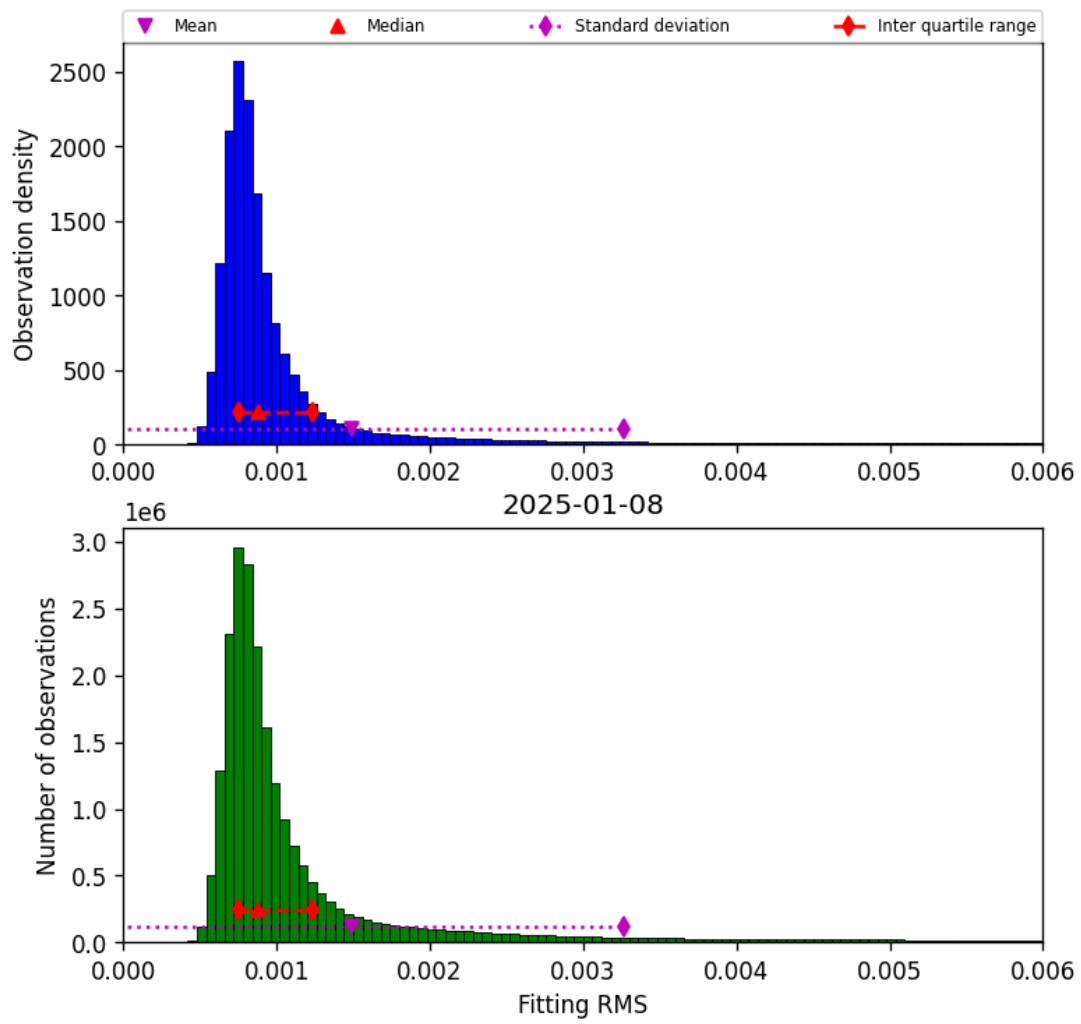
Figure 34: Histogram of "Fitting RMS" for 2025-01-08 to 2025-01-09
