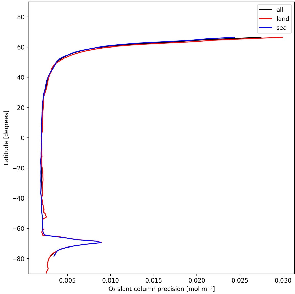
Figure 20: Zonal average of “O 3 slant column precision” for 2025-01-08 to 2025-01-09.
