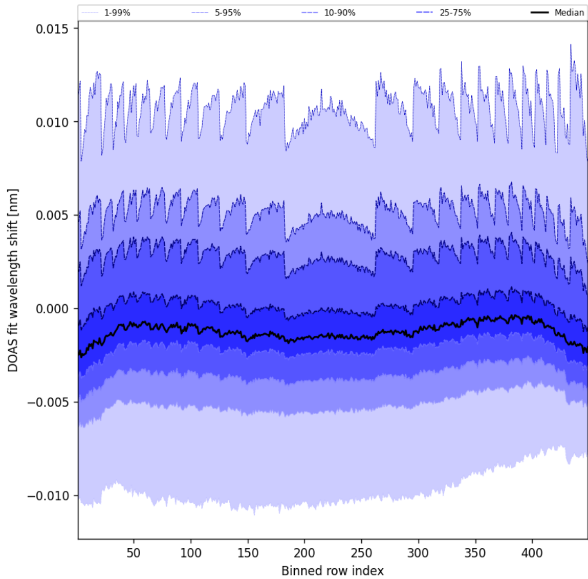
Figure 47: Along track statistics of “DOAS fit wavelength shift” for 2025-01-08 to 2025-01-09
