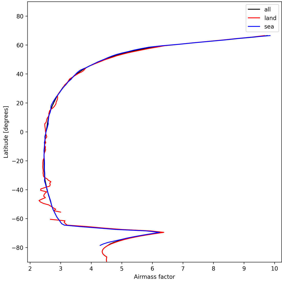
Figure 25: Zonal average of “Airmass factor” for 2025-01-08 to 2025-01-09.
