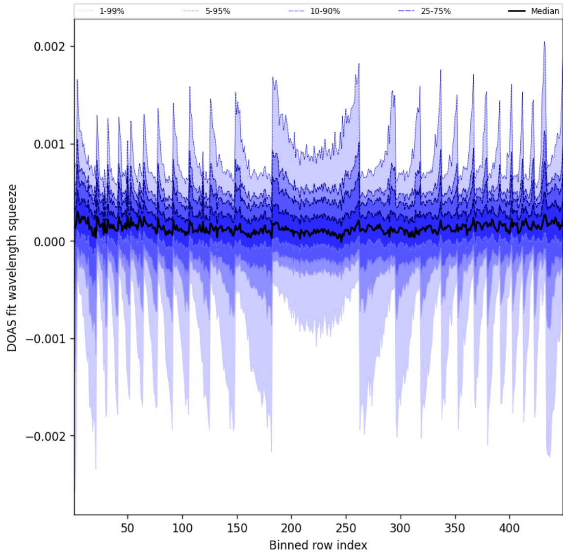
Figure 48: Along track statistics of “DOAS fit wavelength squeeze” for 2025-01-08 to 2025-01-09
