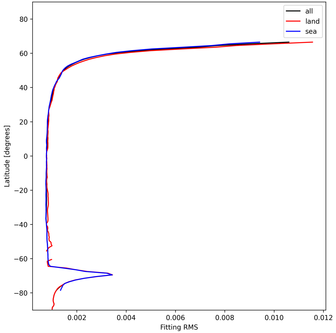
Figure 22: Zonal average of “Fitting RMS” for 2025-01-08 to 2025-01-09.
