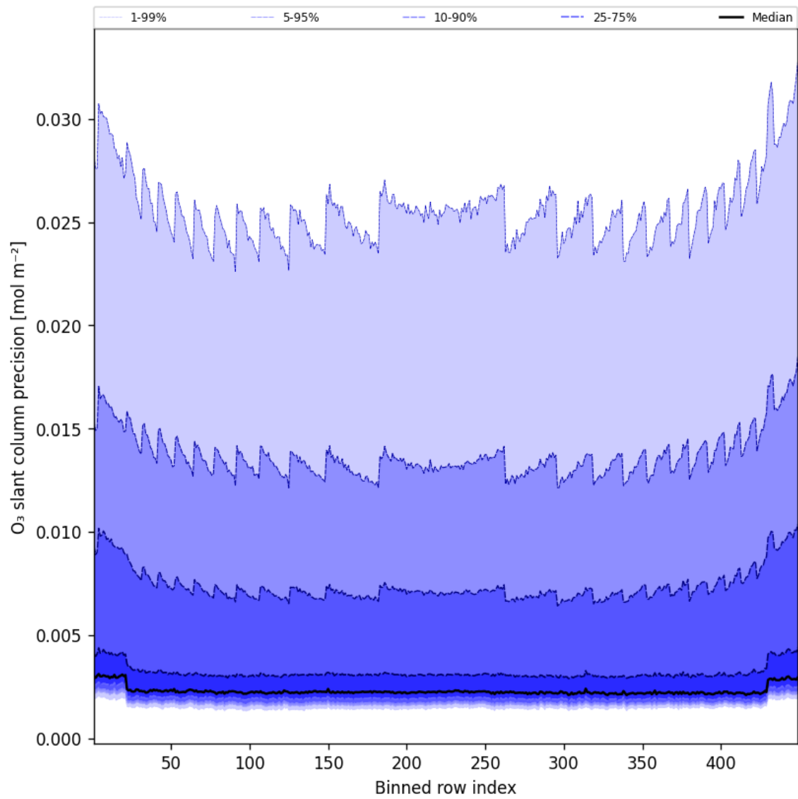
Figure 44: Along track statistics of “O 3 slant column precision” for 2025-01-08 to 2025-01-09
