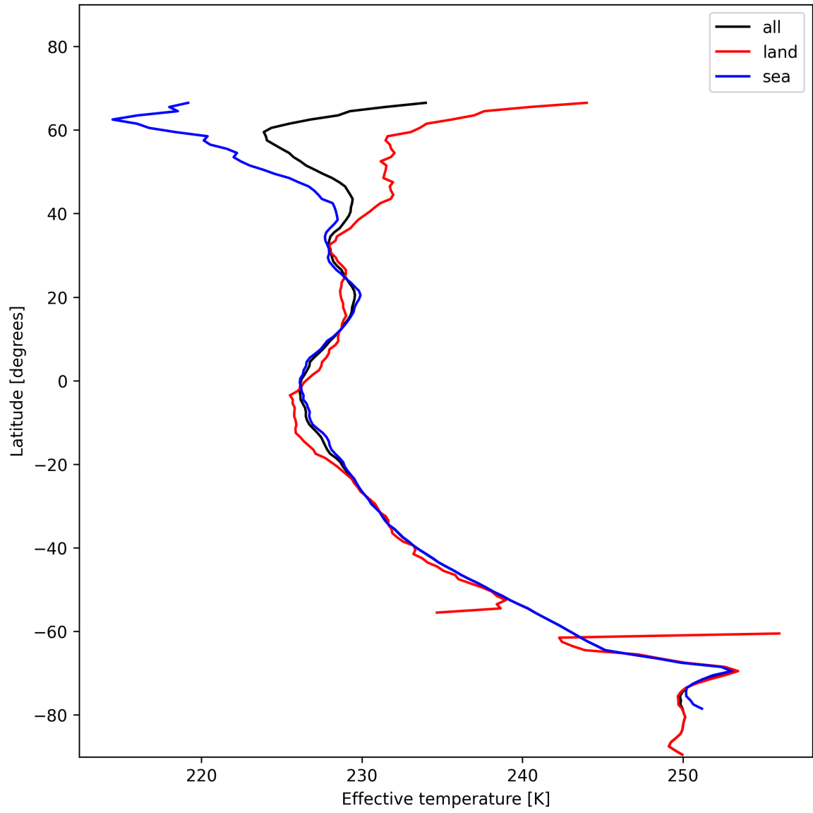
Figure 26: Zonal average of “Effective temperature” for 2025-01-08 to 2025-01-09.
