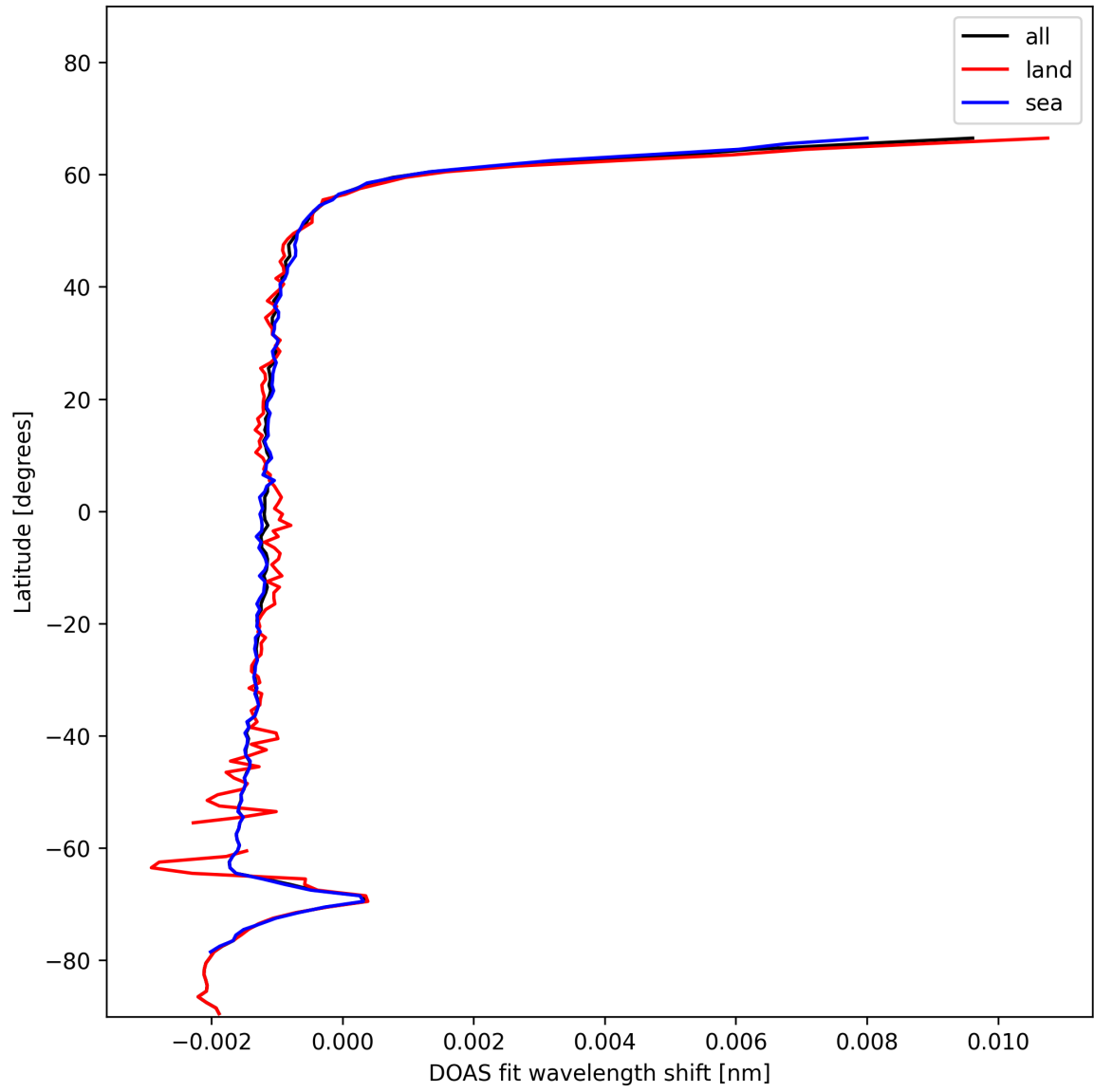
Figure 23: Zonal average of “DOAS fit wavelength shift” for 2025-01-08 to 2025-01-09.
