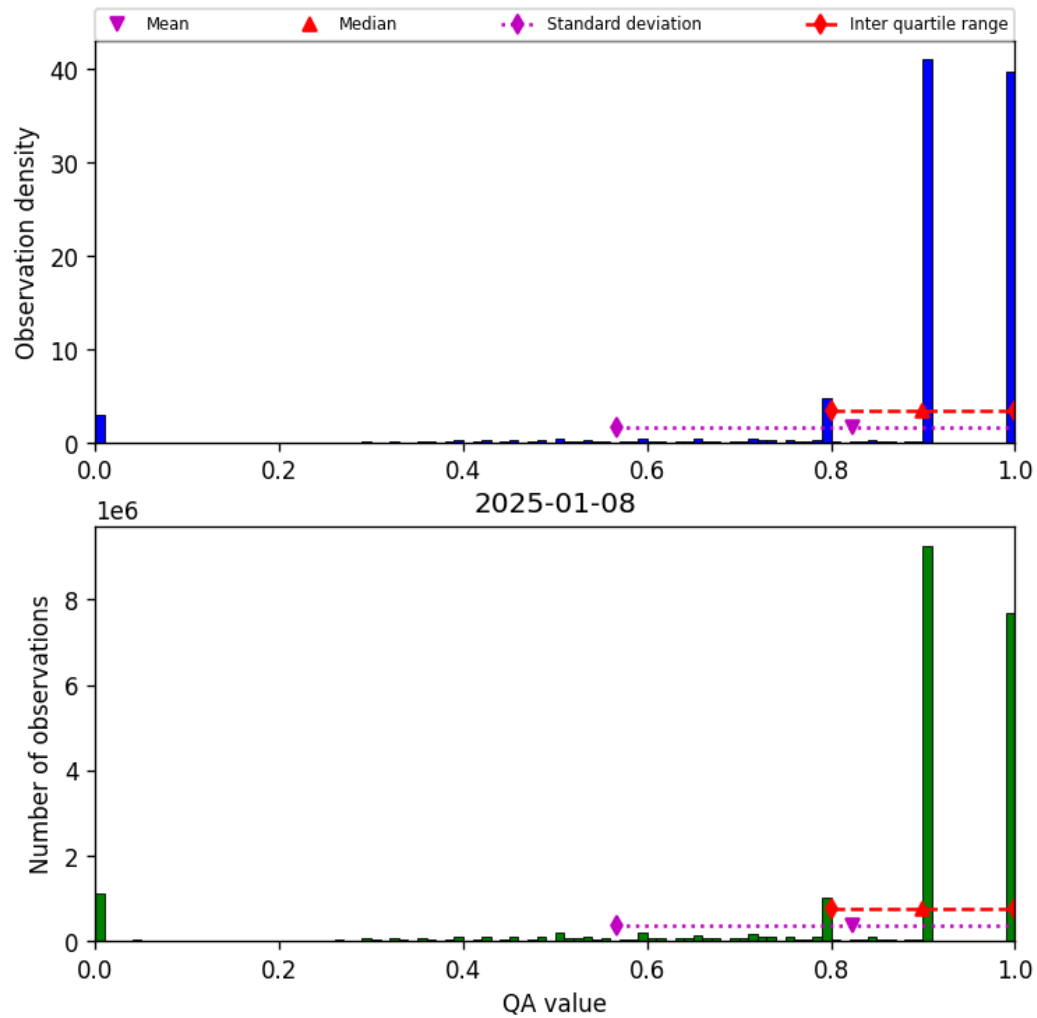
Figure 28: Histogram of “QA value” for 2025-01-08 to 2025-01-09
