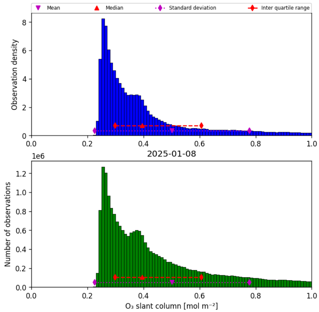
Figure 31: Histogram of “O 3 slant column” for 2025-01-08 to 2025-01-09
