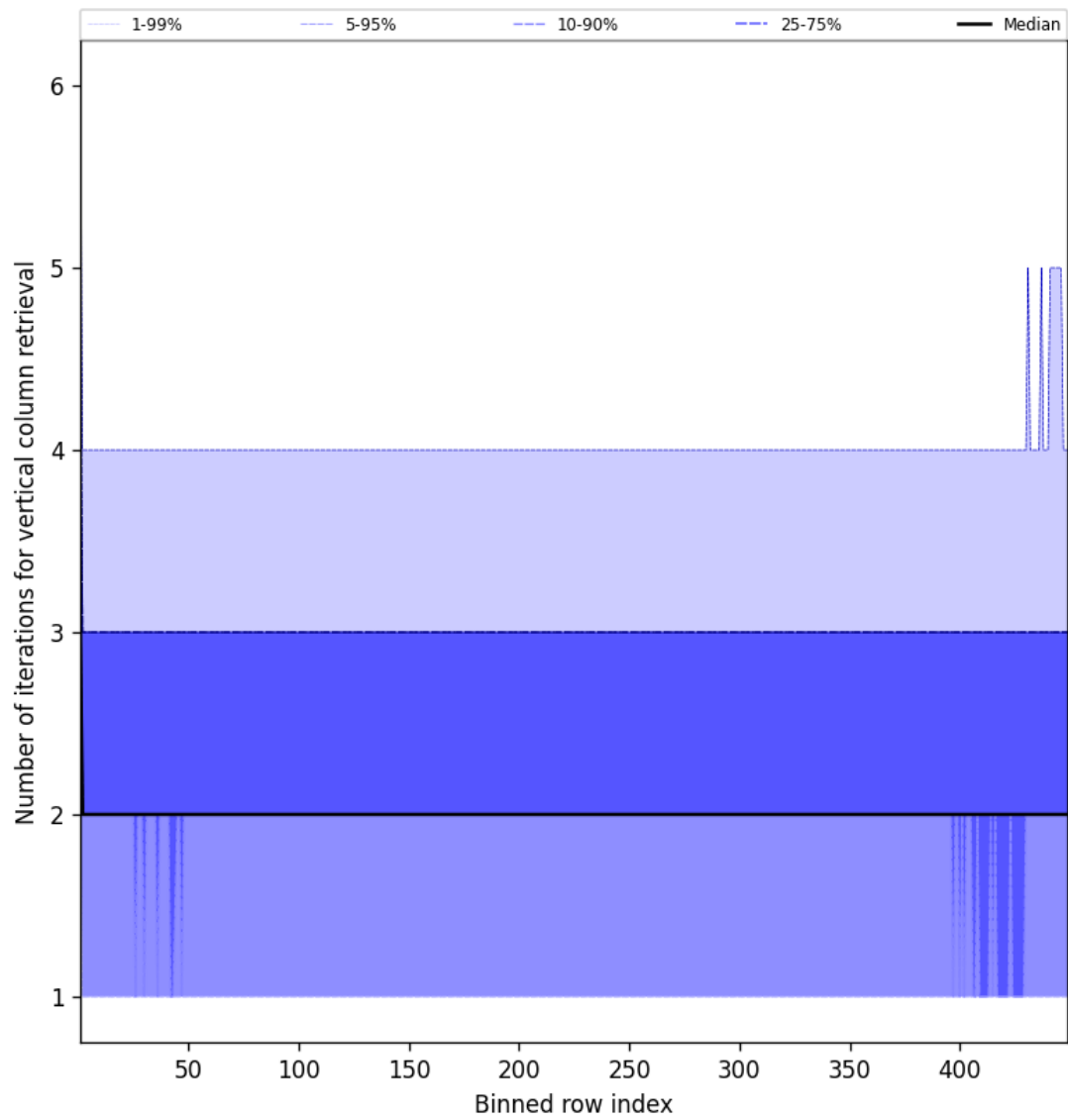
Figure 51: Along track statistics of “Number of iterations for vertical column retrieval” for 2025-01-08 to 2025-01-09
