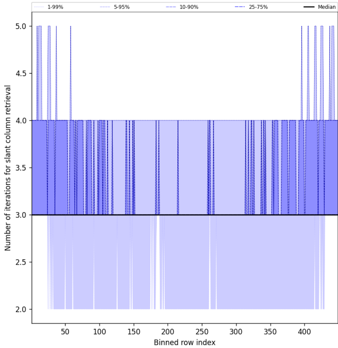
Figure 45: Along track statistics of “Number of iterations for slant column retrieval” for 2025-01-08 to 2025-01-09
