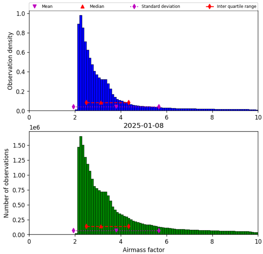
Figure 37: Histogram of “Airmass factor” for 2025-01-08 to 2025-01-09
