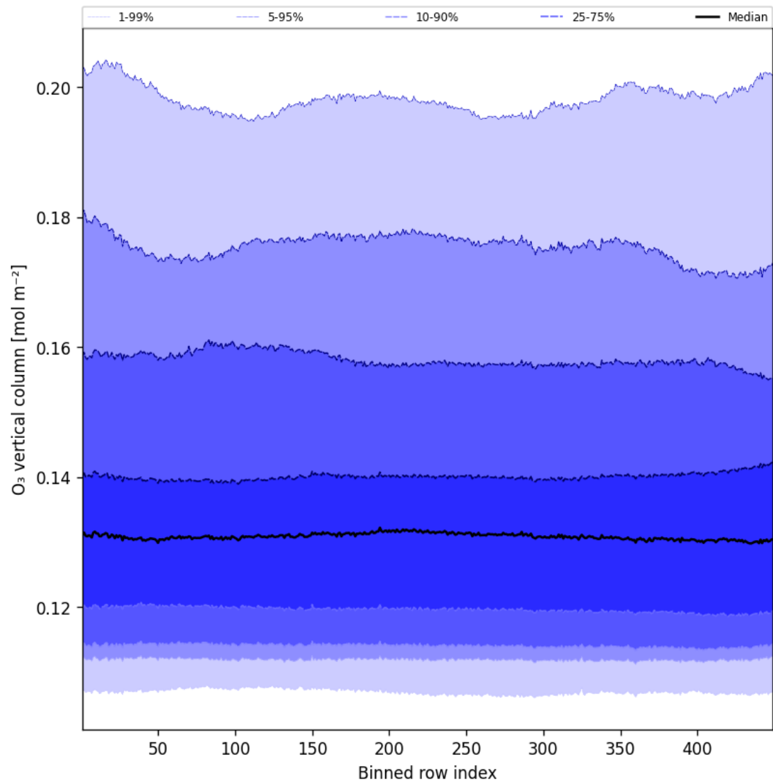
Figure 41: Along track statistics of “O 3 vertical column” for 2025-01-08 to 2025-01-09
