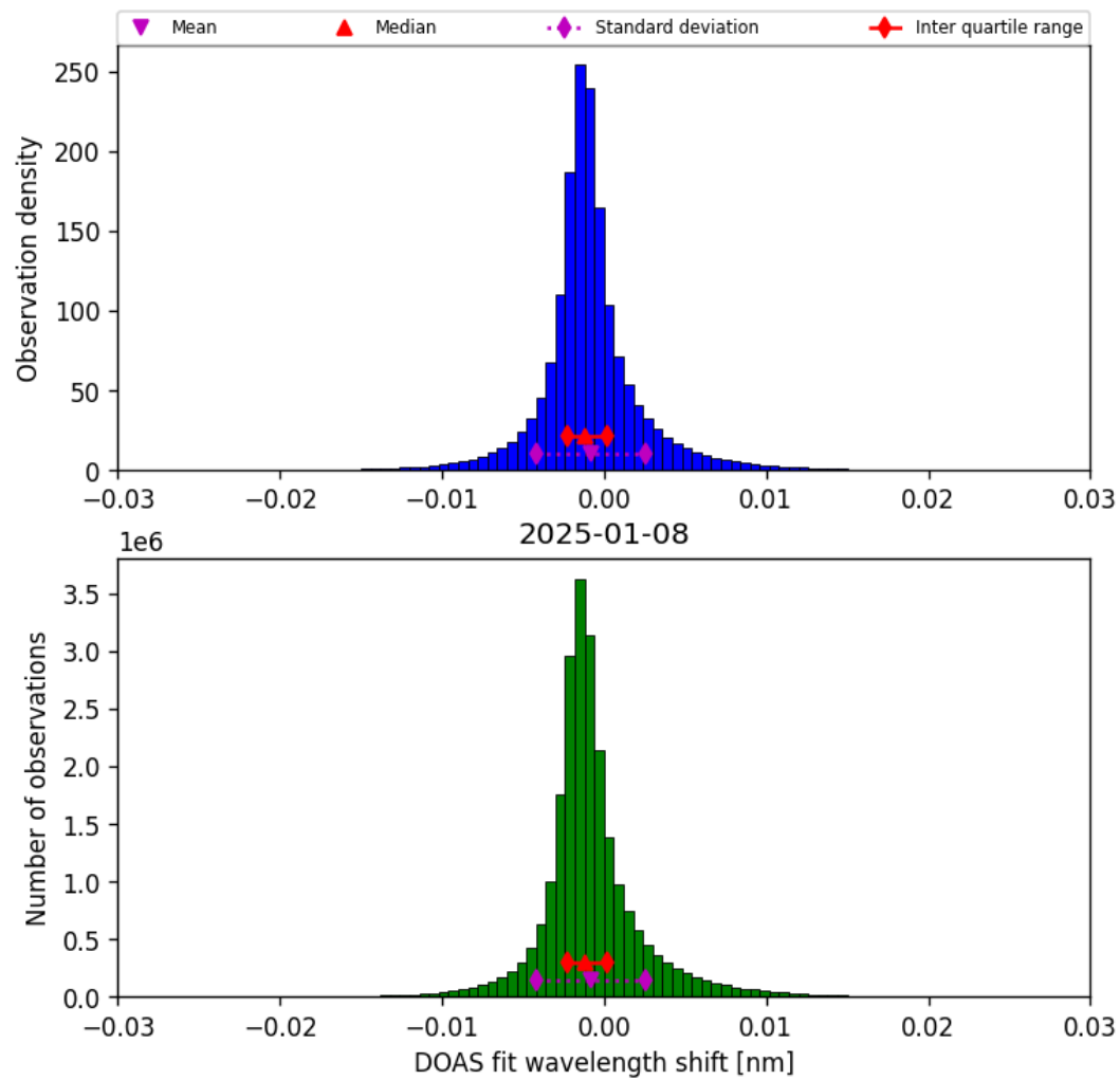
Figure 35: Histogram of “DOAS fit wavelength shift” for 2025-01-08 to 2025-01-09
