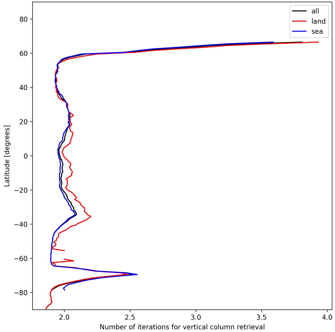
Figure 27: Zonal average of “Number of iterations for vertical column retrieval” for 2025-01-08 to 2025-01-09.
