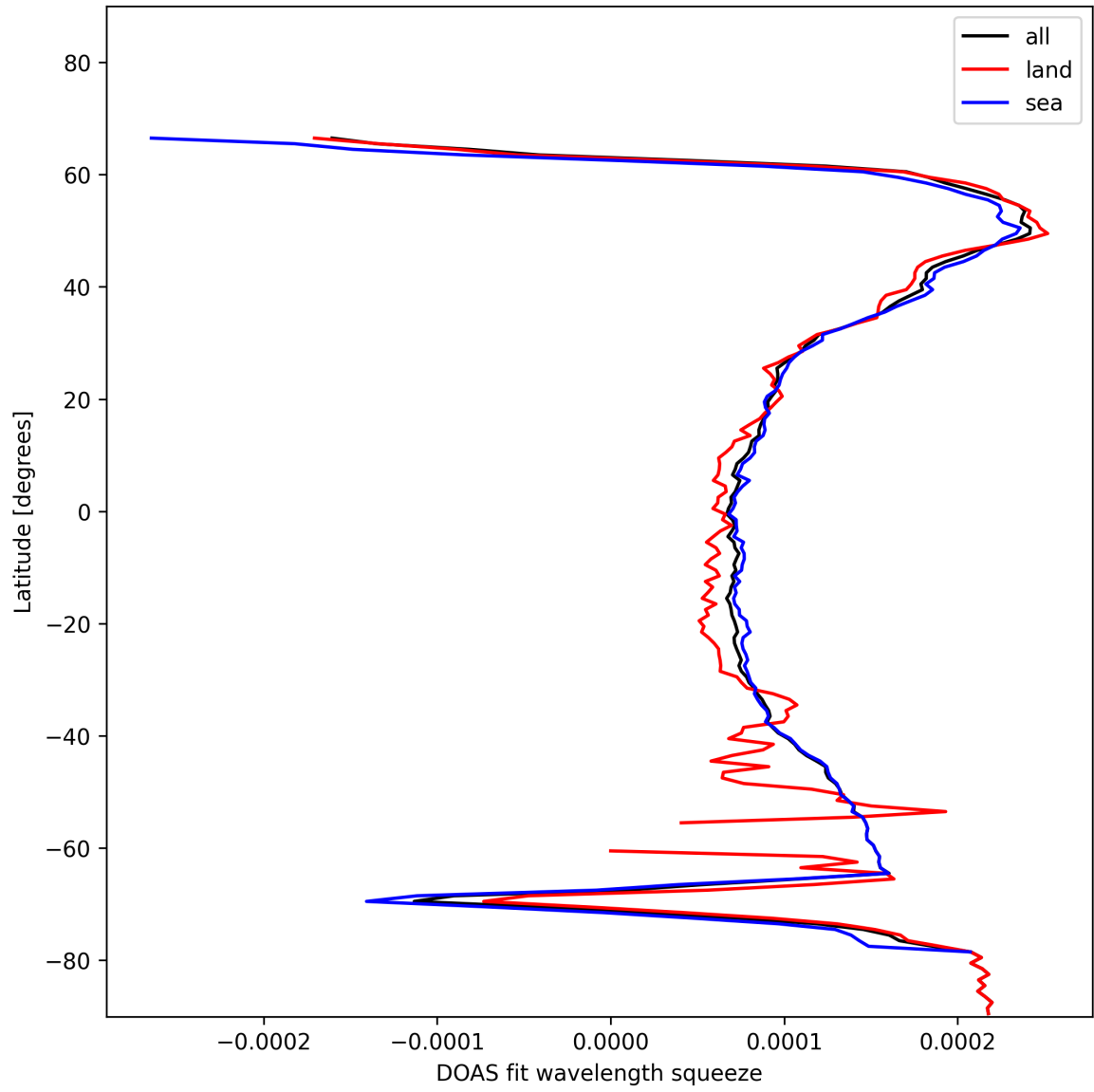
Figure 24: Zonal average of “DOAS fit wavelength squeeze” for 2025-01-08 to 2025-01-09.
