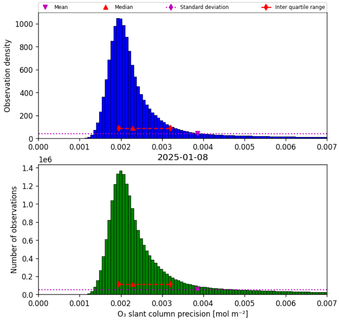
Figure 32: Histogram of “O 3 slant column precision” for 2025-01-08 to 2025-01-09
