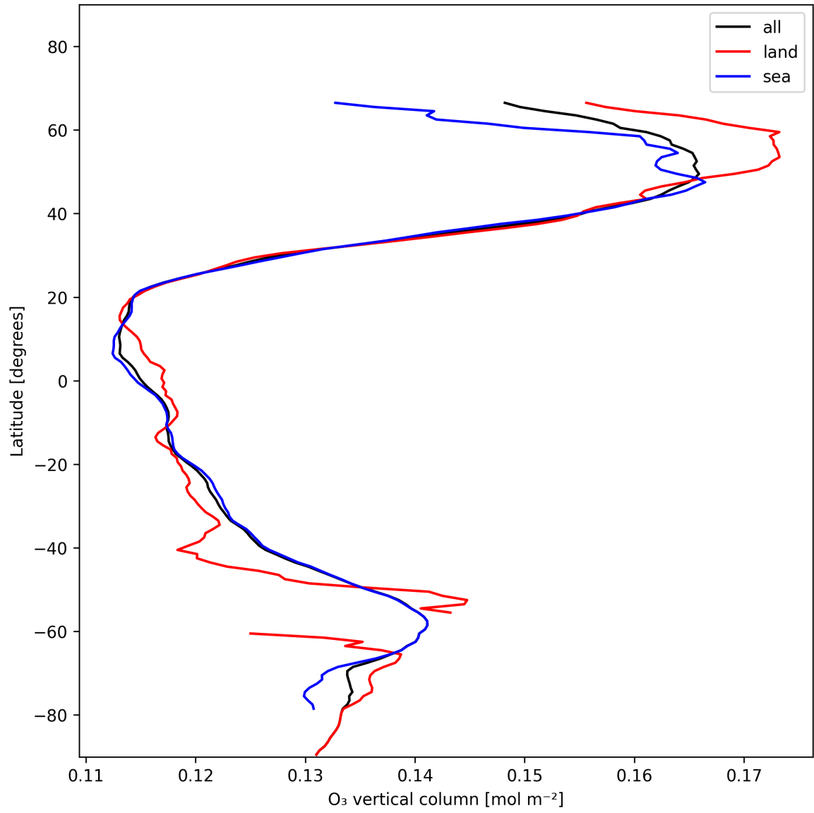
Figure 17: Zonal average of “O 3 vertical column” for 2025-01-08 to 2025-01-09.
