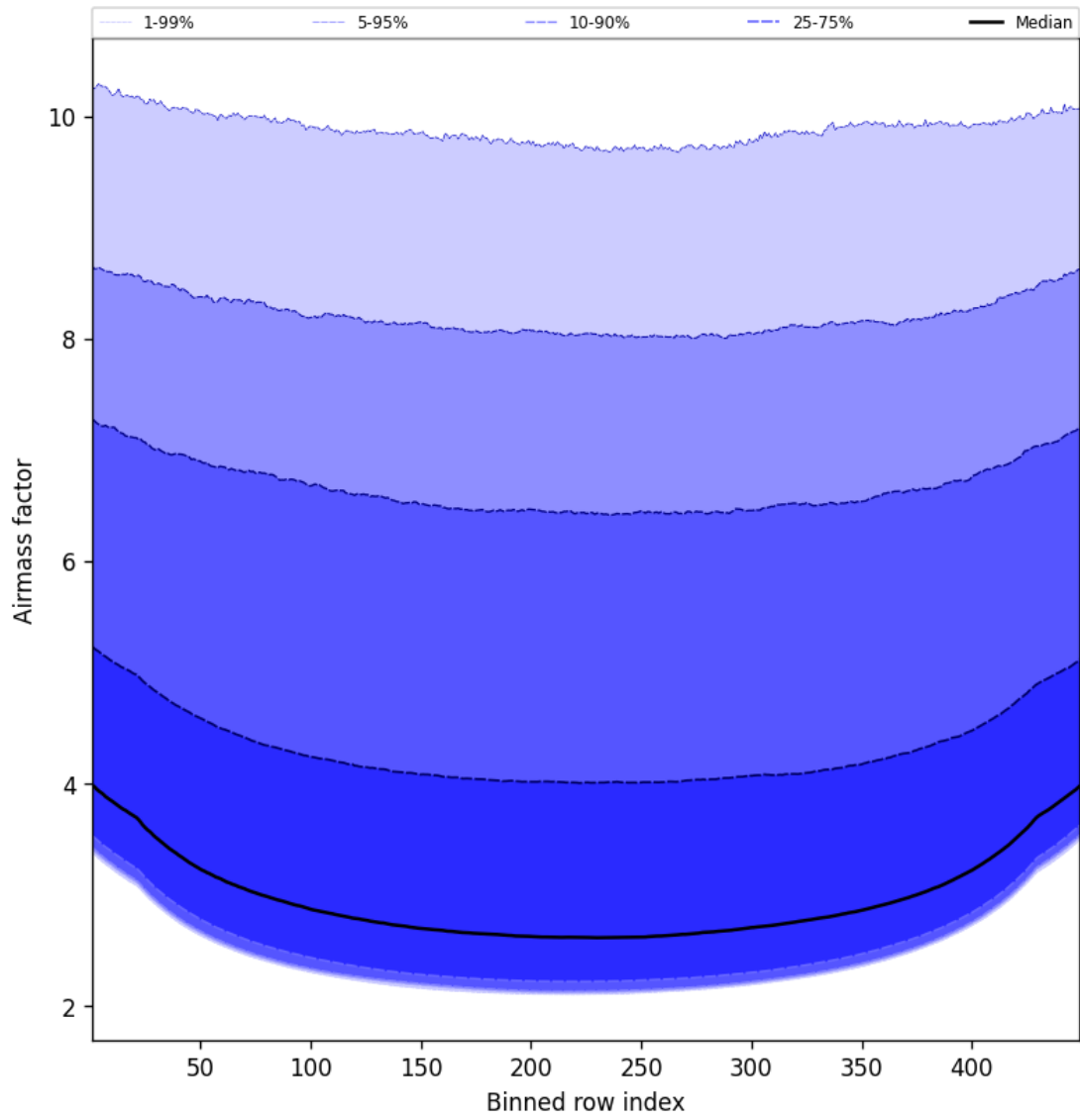
Figure 49: Along track statistics of “Airmass factor” for 2025-01-08 to 2025-01-09
