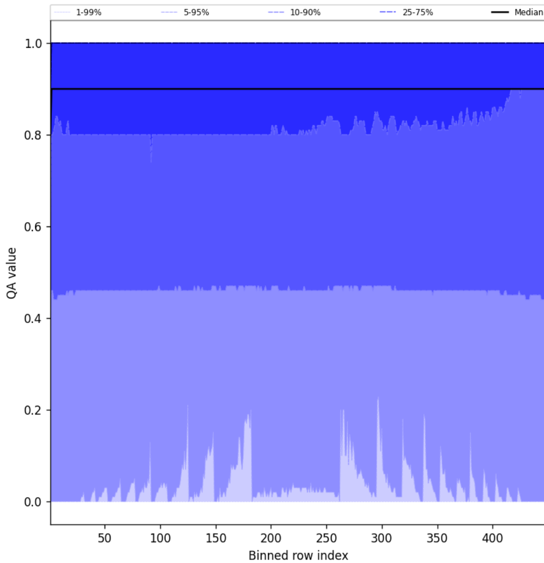
Figure 40: Along track statistics of “QA value” for 2025-01-08 to 2025-01-09
