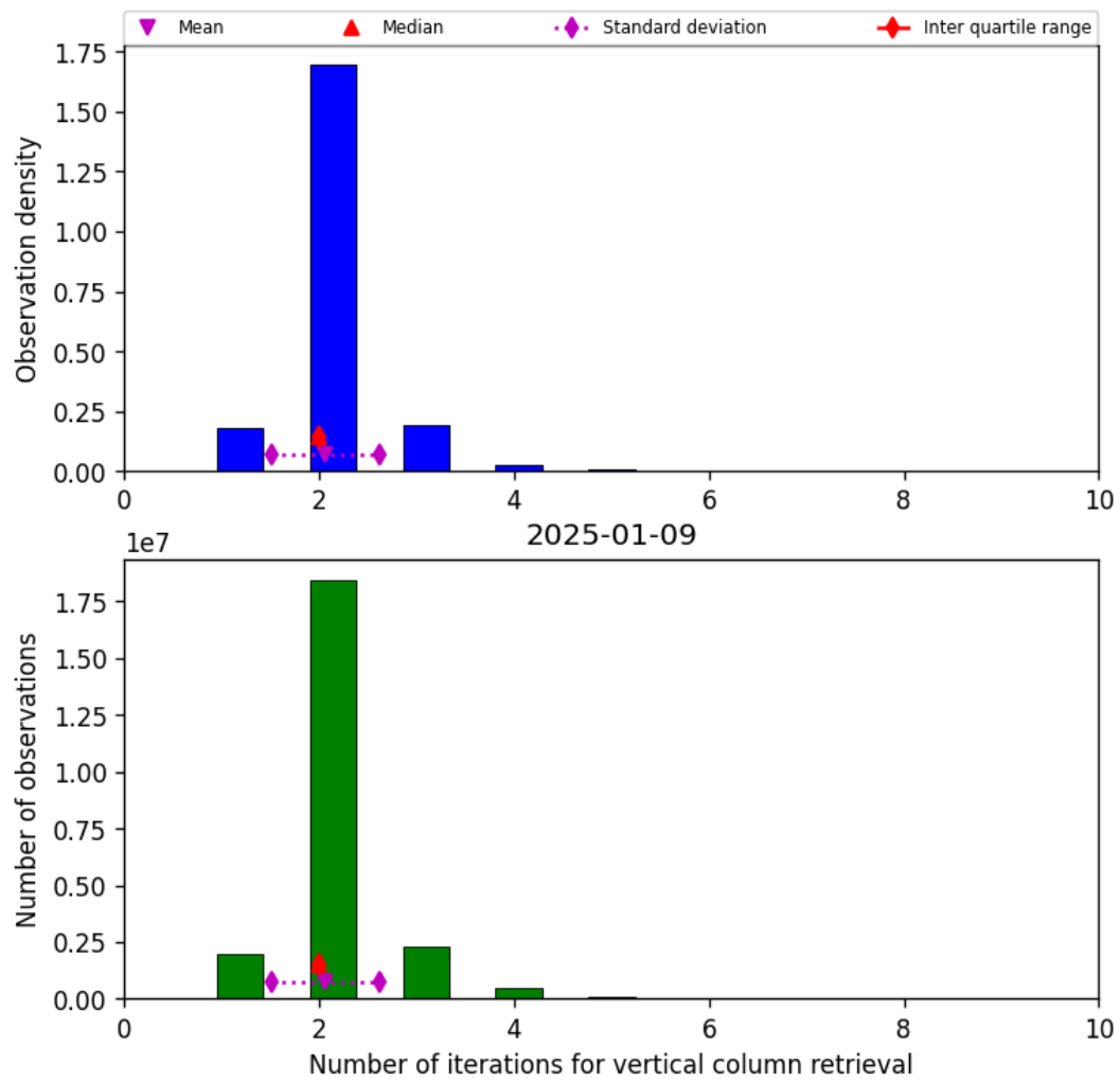
Figure 39: Histogram of “Number of iterations for vertical column retrieval” for 2025-01-09 to 2025-01-10
