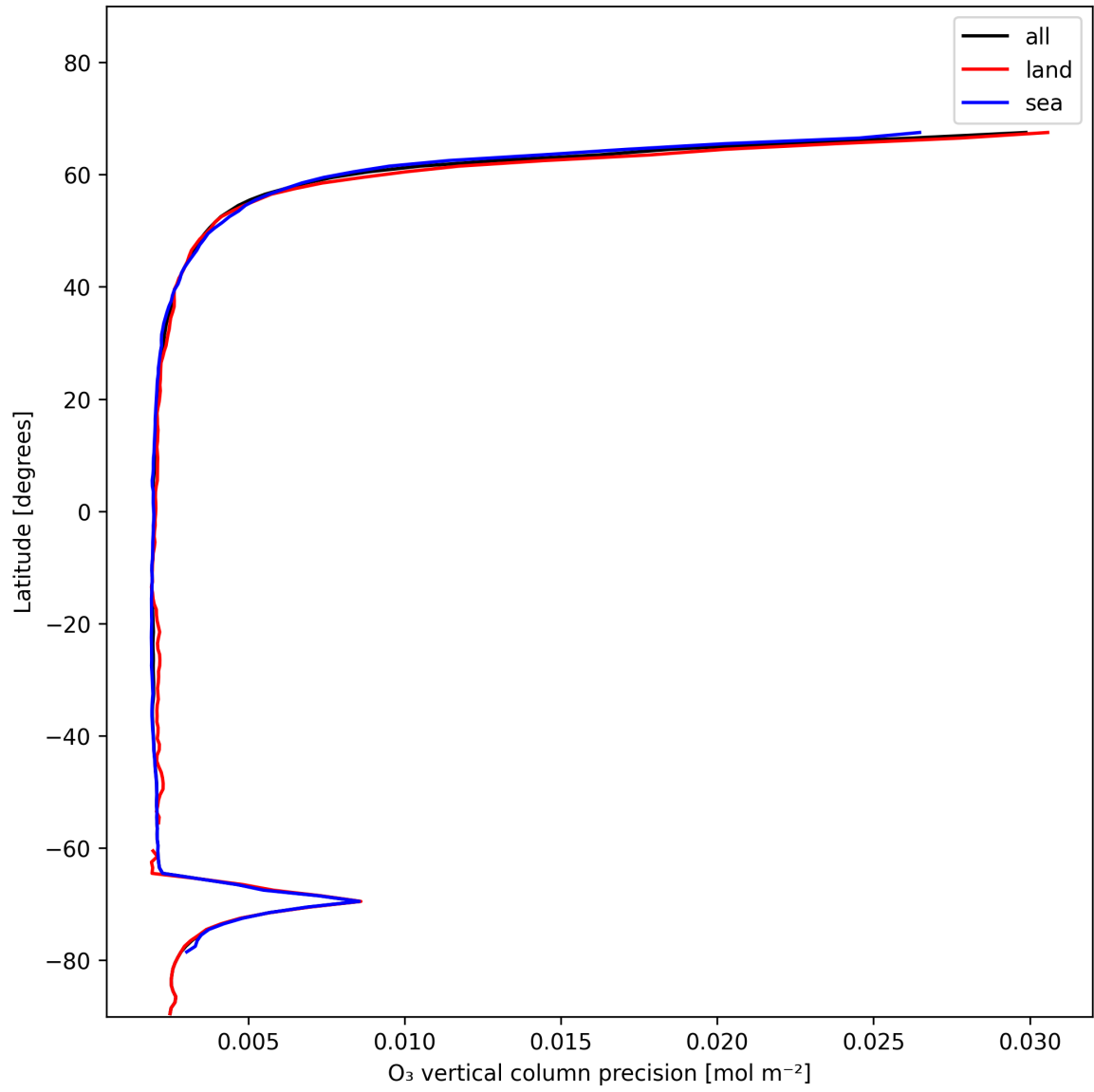
Figure 18: Zonal average of “O 3 vertical column precision” for 2025-01-09 to 2025-01-10.
