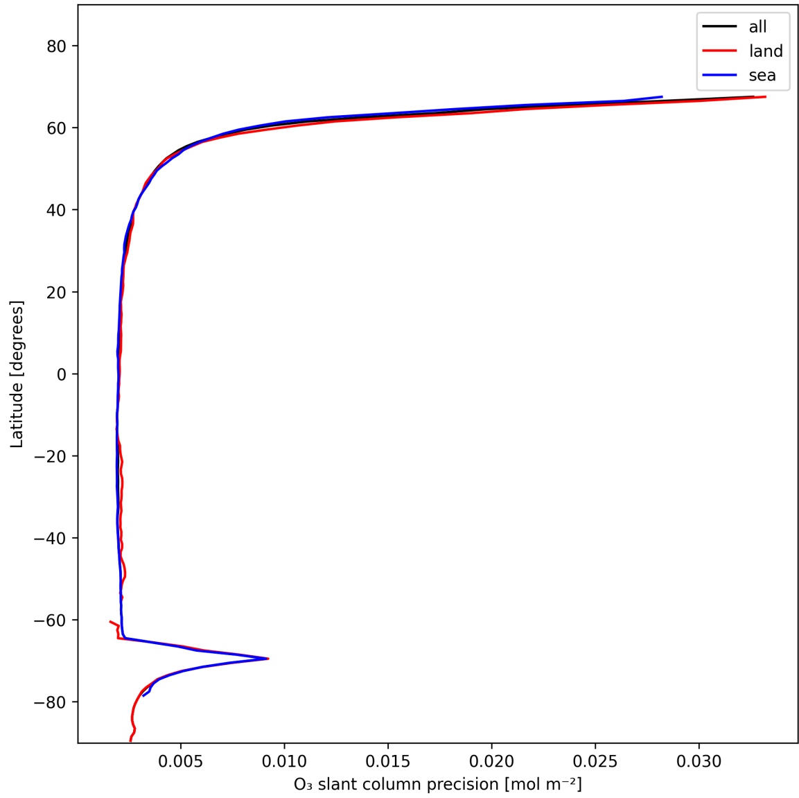
Figure 20: Zonal average of “O 3 slant column precision” for 2025-01-09 to 2025-01-10.
