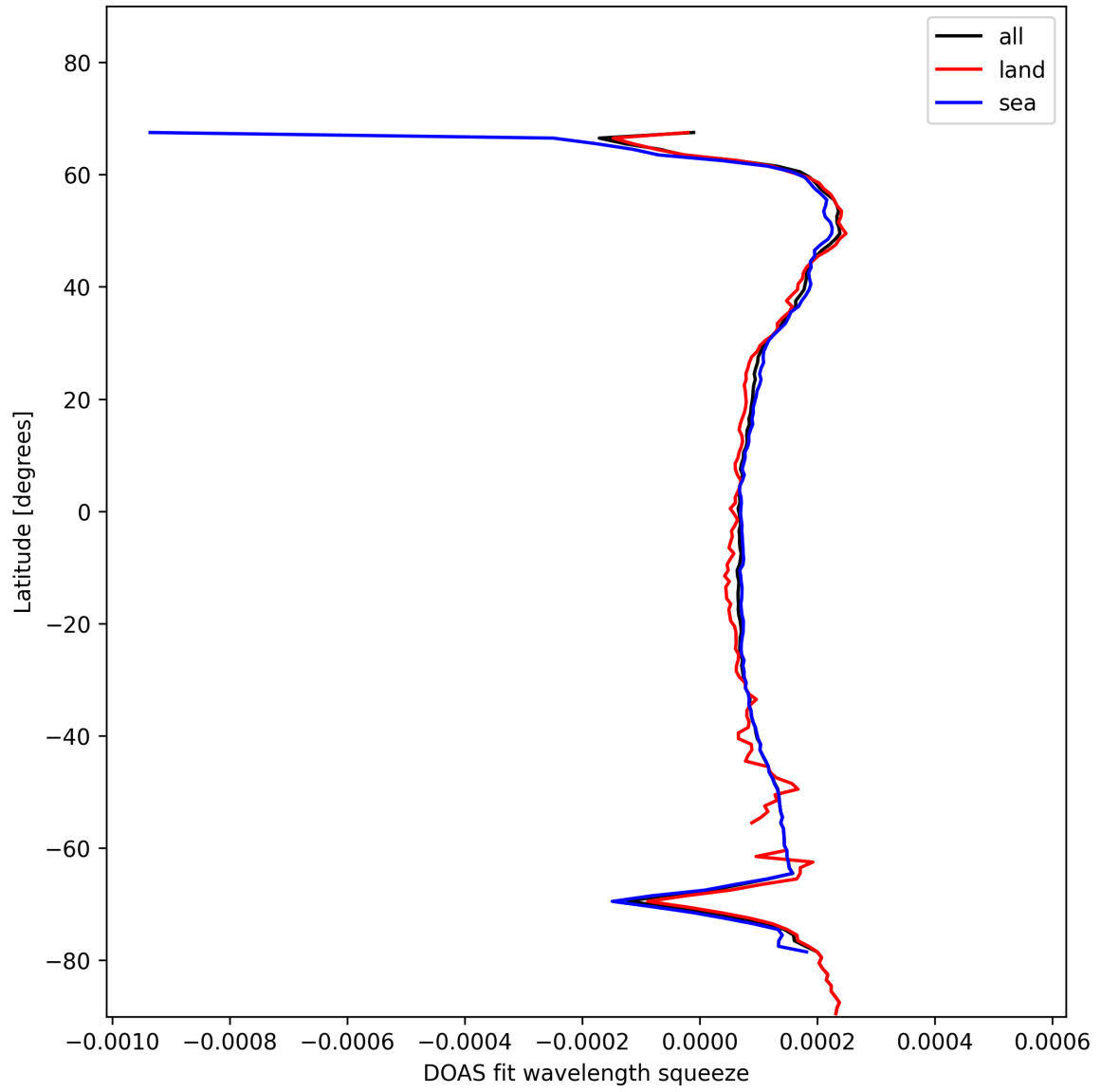
Figure 24: Zonal average of “DOAS fit wavelength squeeze” for 2025-01-09 to 2025-01-10.
