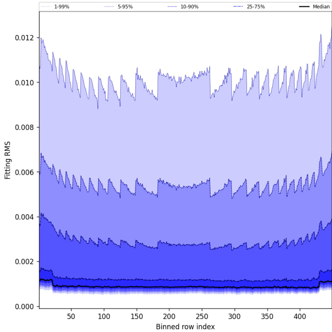
Figure 46: Along track statistics of “Fitting RMS” for 2025-01-09 to 2025-01-10
