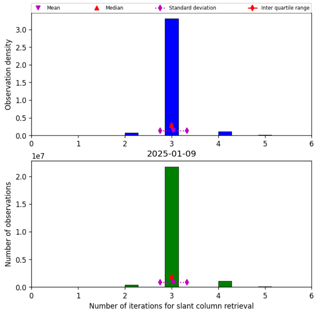
Figure 33: Histogram of "Number of iterations for slant column retrieval" for 2025-01-09 to 2025-01-10
