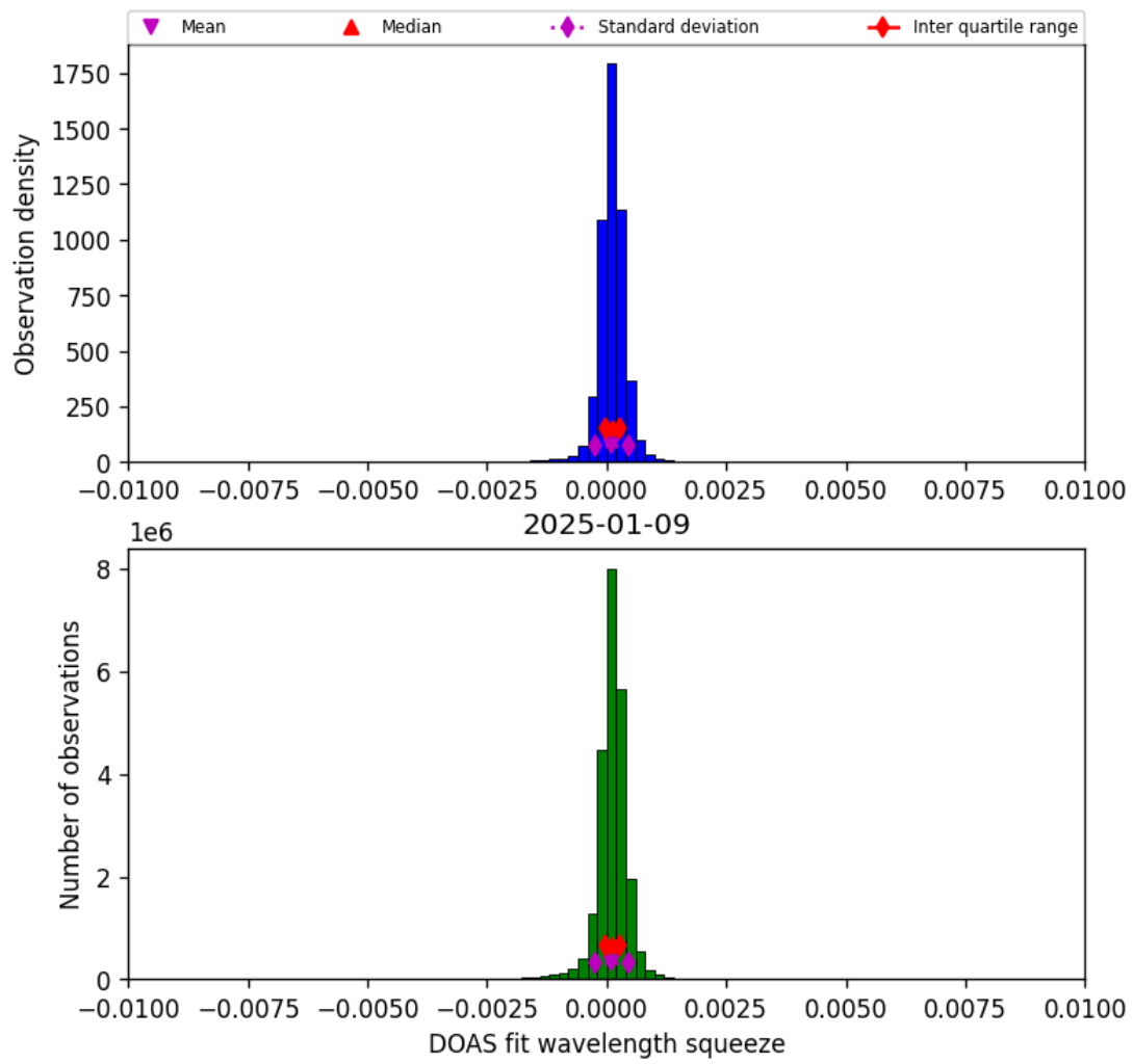
Figure 36: Histogram of “DOAS fit wavelength squeeze” for 2025-01-09 to 2025-01-10
