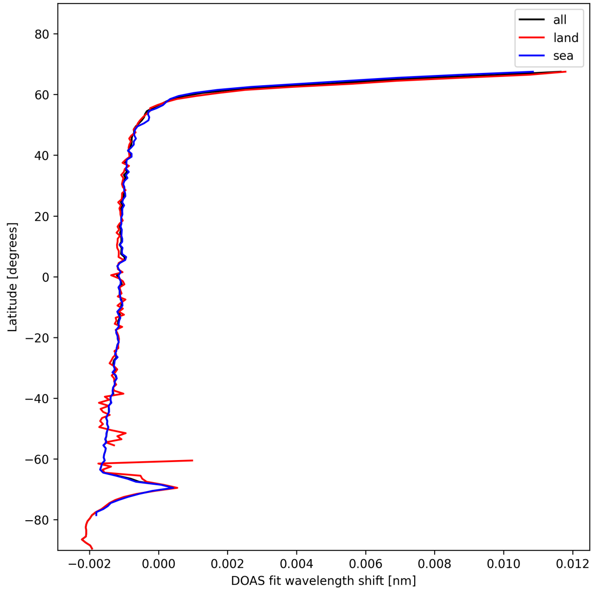
Figure 23: Zonal average of “DOAS fit wavelength shift” for 2025-01-09 to 2025-01-10.
