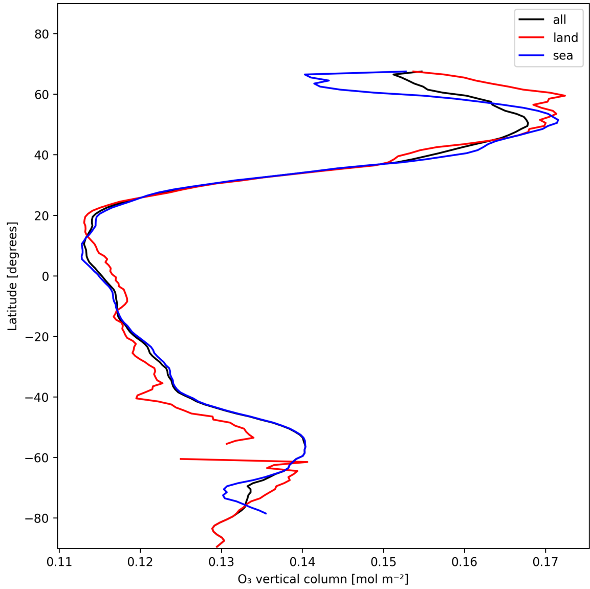
Figure 17: Zonal average of “O 3 vertical column” for 2025-01-09 to 2025-01-10.
