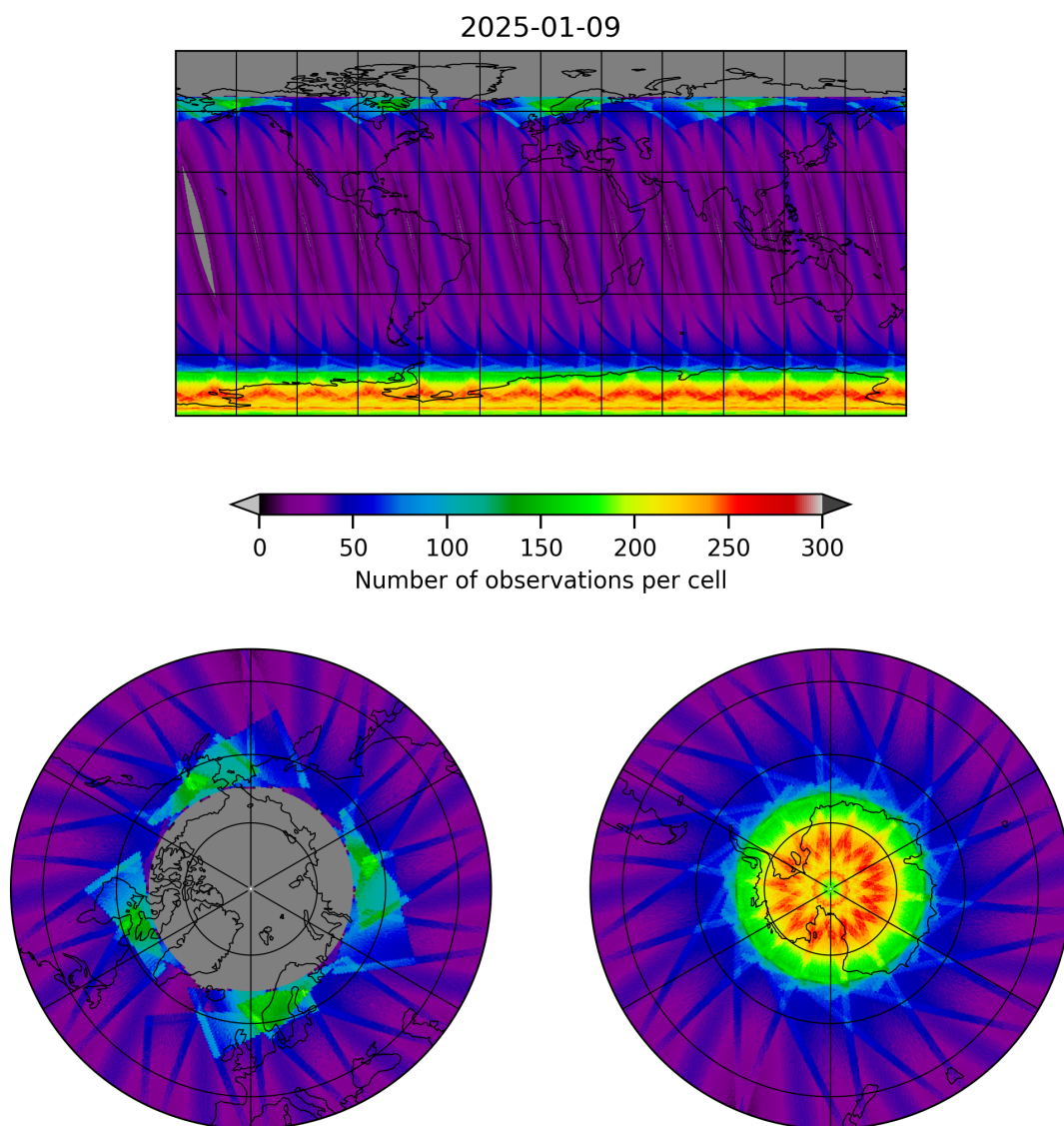
Figure 15: Map of the number of observations for 2025-01-09 to 2025-01-10
