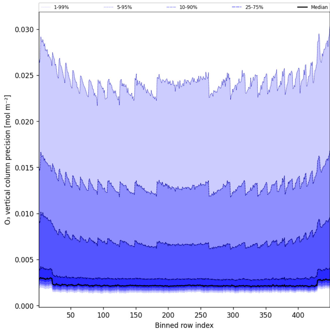
Figure 42: Along track statistics of “O 3 vertical column precision” for 2025-01-09 to 2025-01-10
