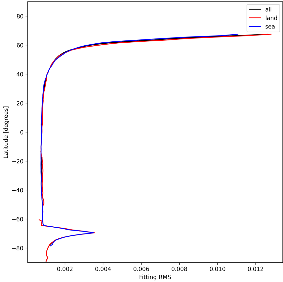
Figure 22: Zonal average of “Fitting RMS” for 2025-01-09 to 2025-01-10.
