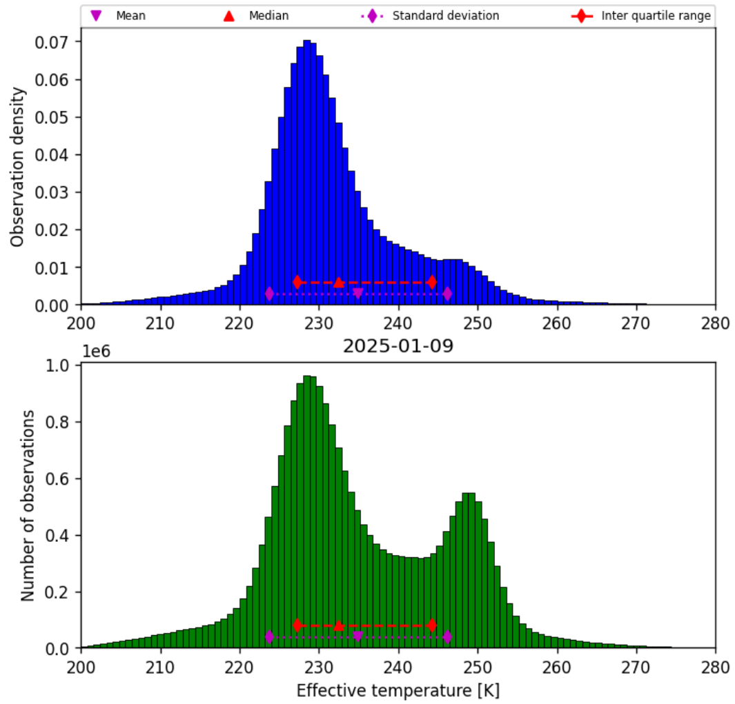
Figure 38: Histogram of “Effective temperature” for 2025-01-09 to 2025-01-10
