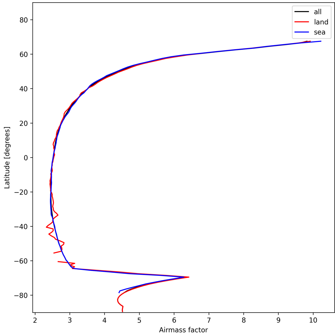
Figure 25: Zonal average of “Airmass factor” for 2025-01-09 to 2025-01-10.
