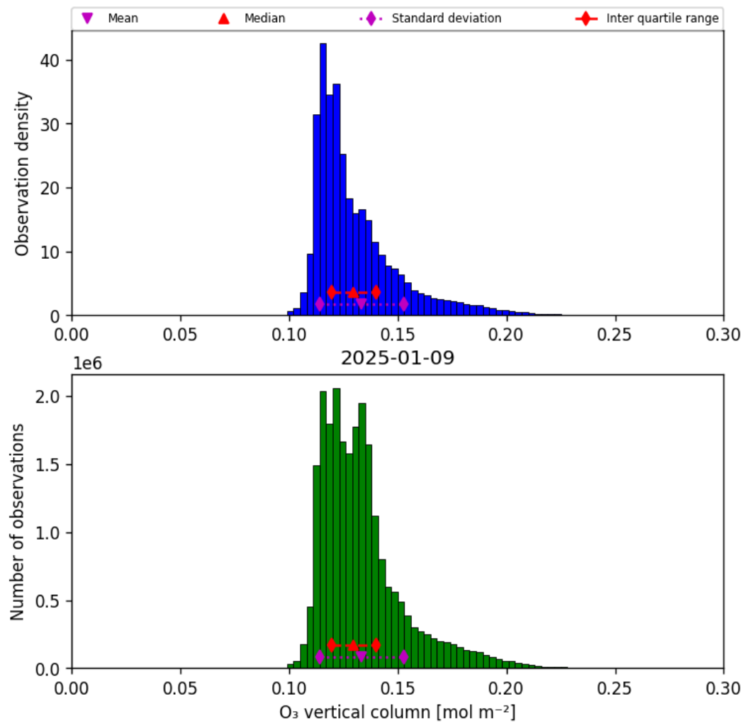
Figure 29: Histogram of “O 3 vertical column” for 2025-01-09 to 2025-01-10
