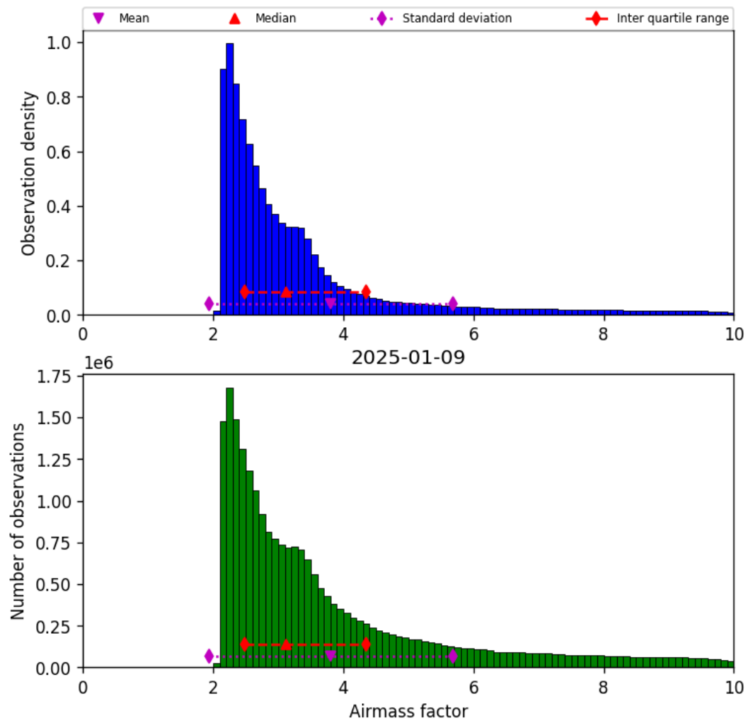
Figure 37: Histogram of “Airmass factor” for 2025-01-09 to 2025-01-10
