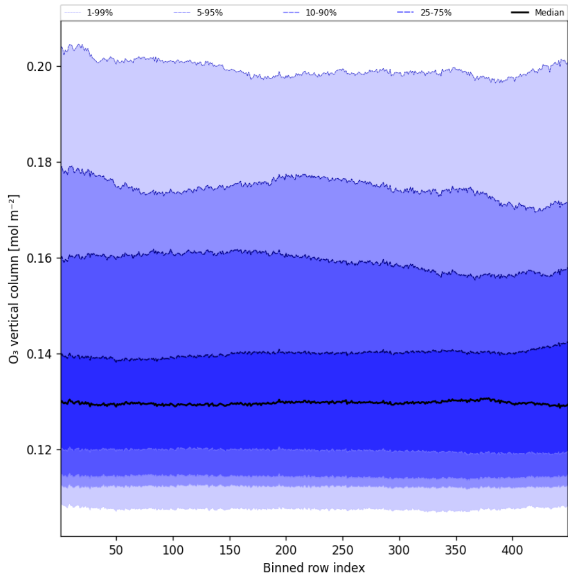
Figure 41: Along track statistics of “O 3 vertical column” for 2025-01-09 to 2025-01-10
