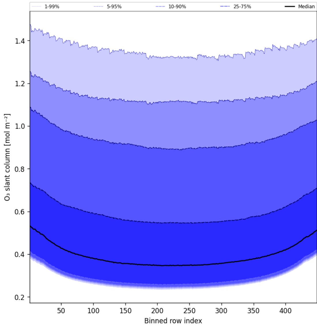
Figure 43: Along track statistics of “O 3 slant column” for 2025-01-09 to 2025-01-10
