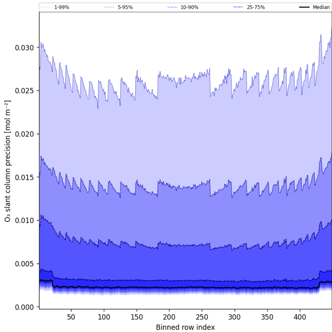
Figure 44: Along track statistics of “O 3 slant column precision” for 2025-01-09 to 2025-01-10
