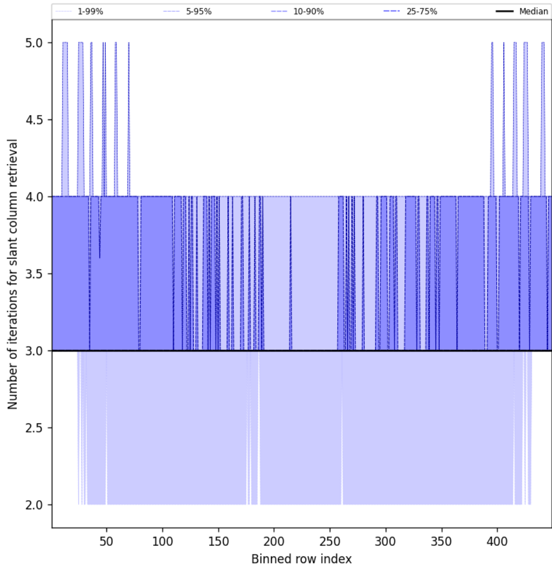
Figure 45: Along track statistics of “Number of iterations for slant column retrieval” for 2025-01-09 to 2025-01-10
