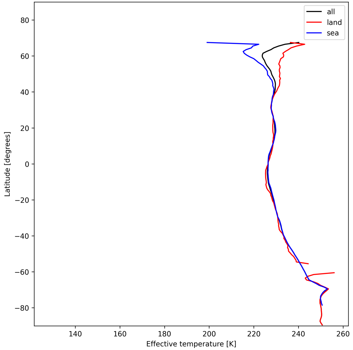
Figure 26: Zonal average of “Effective temperature” for 2025-01-09 to 2025-01-10.
