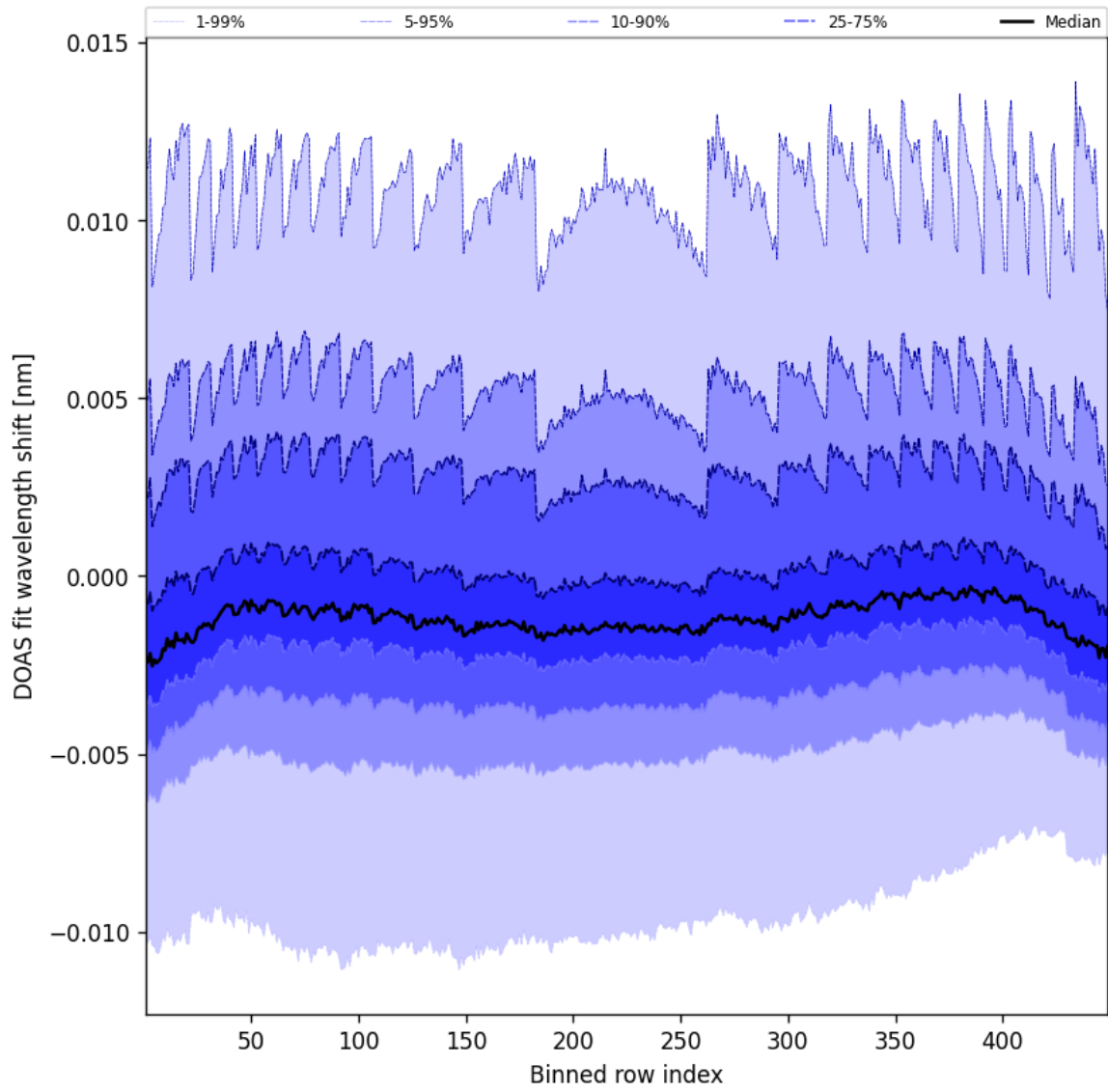
Figure 47: Along track statistics of “DOAS fit wavelength shift” for 2025-01-09 to 2025-01-10
