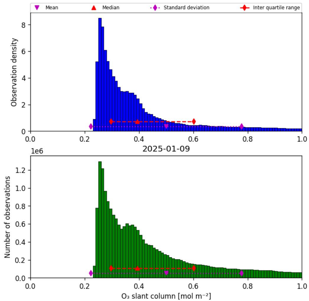
Figure 31: Histogram of “O 3 slant column” for 2025-01-09 to 2025-01-10
