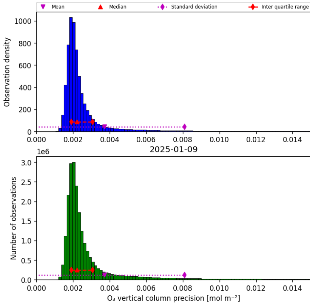
Figure 30: Histogram of “O 3 vertical column precision” for 2025-01-09 to 2025-01-10
