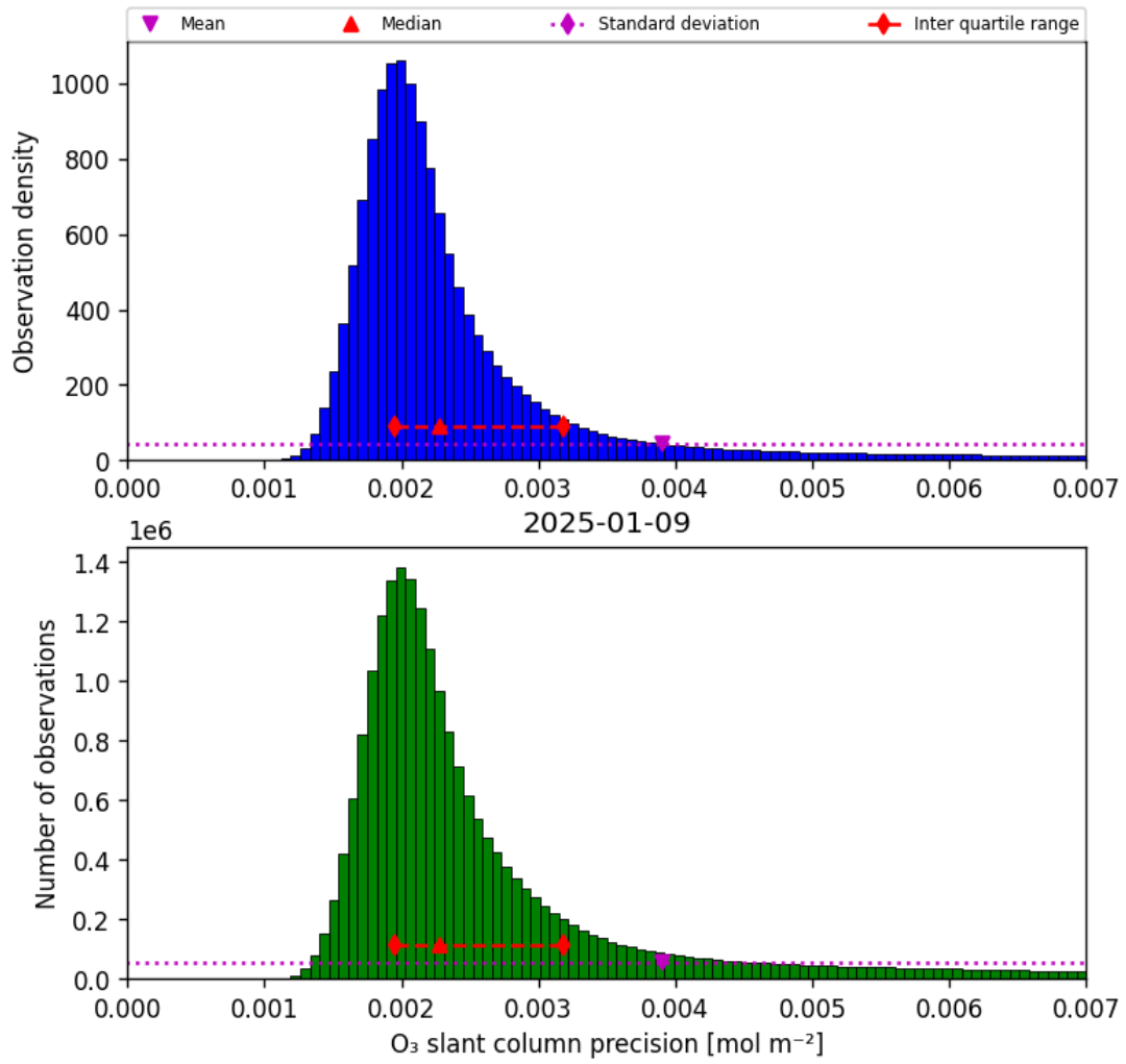
Figure 32: Histogram of "O 3 slant column precision" for 2025-01-09 to 2025-01-10
