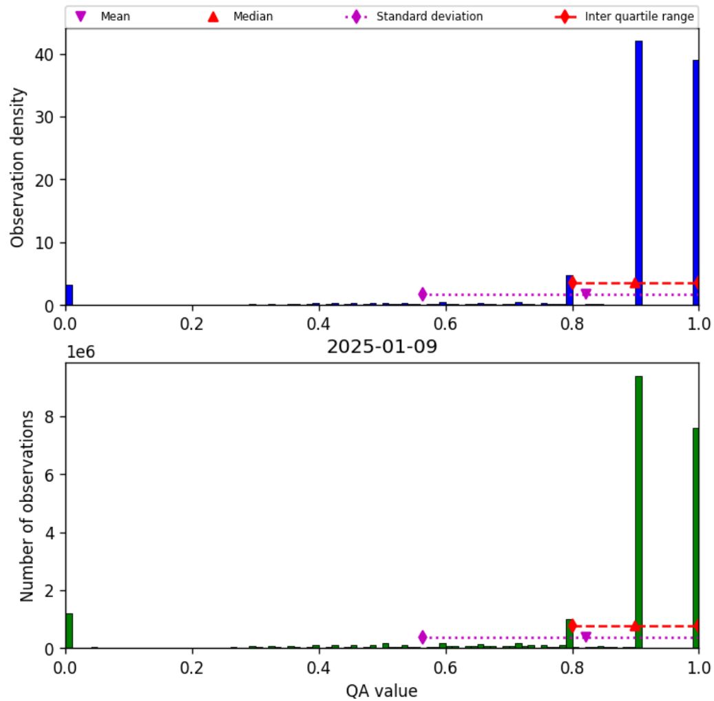
Figure 28: Histogram of “QA value” for 2025-01-09 to 2025-01-10
