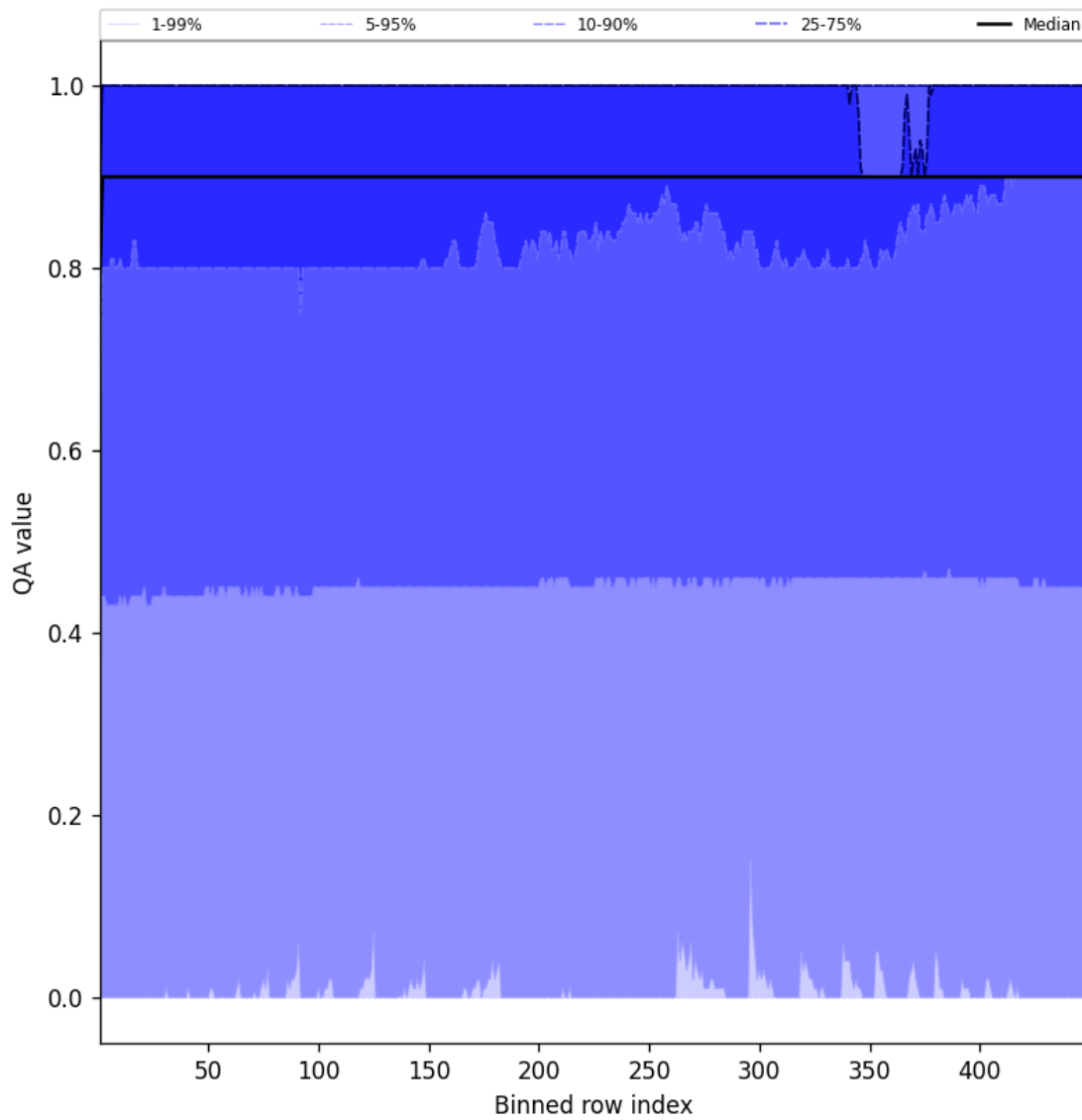
Figure 40: Along track statistics of “QA value” for 2025-01-09 to 2025-01-10
