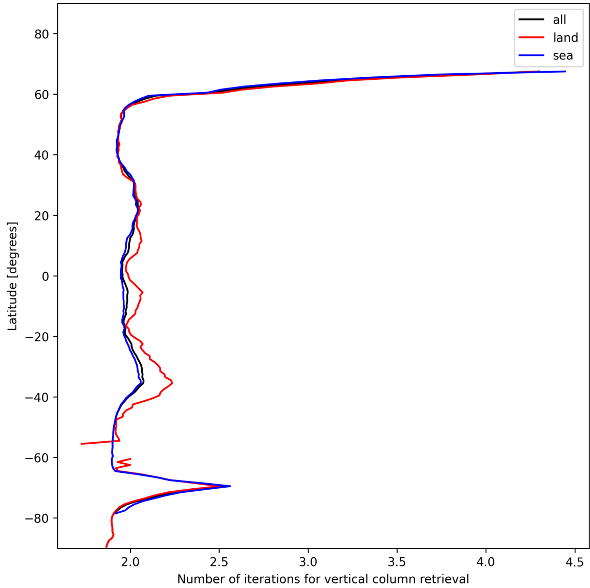
Figure 27: Zonal average of “Number of iterations for vertical column retrieval” for 2025-01-09 to 2025-01-10.
