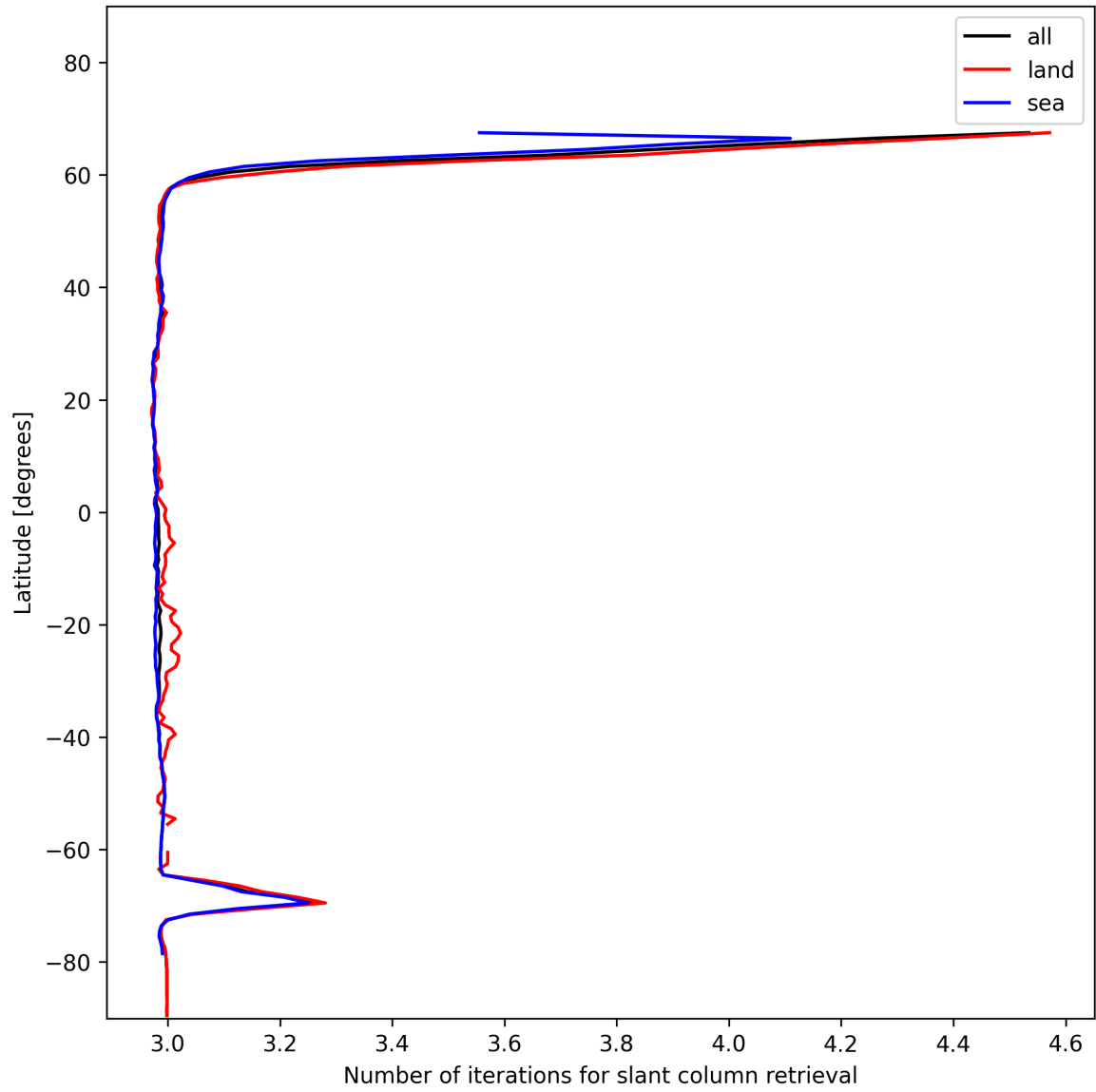
Figure 21: Zonal average of “Number of iterations for slant column retrieval” for 2025-01-09 to 2025-01-10.
