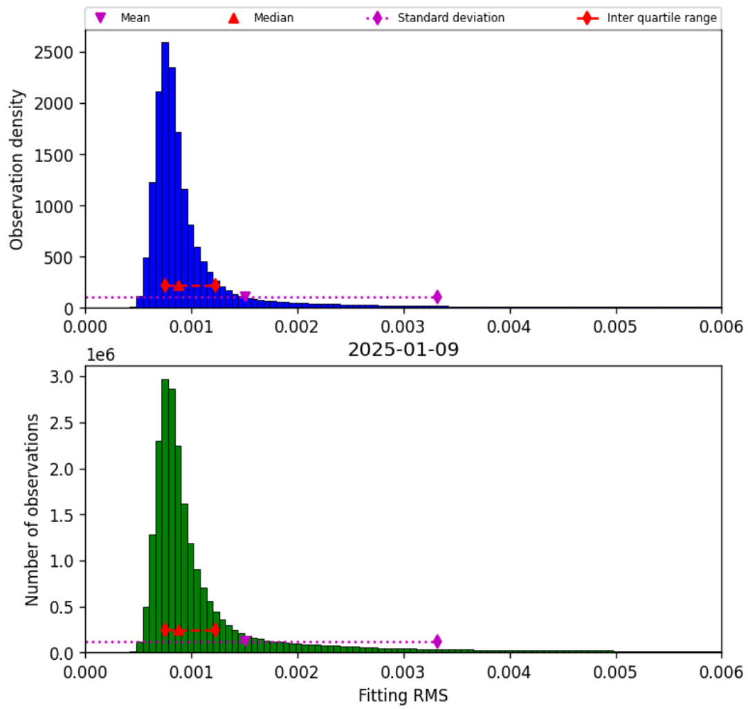
Figure 34: Histogram of “Fitting RMS” for 2025-01-09 to 2025-01-10
