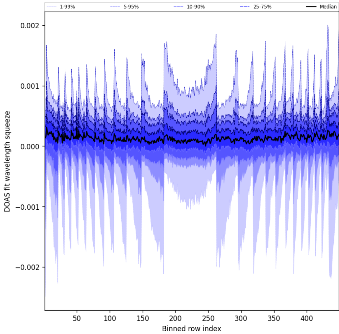
Figure 48: Along track statistics of “DOAS fit wavelength squeeze” for 2025-01-09 to 2025-01-10
