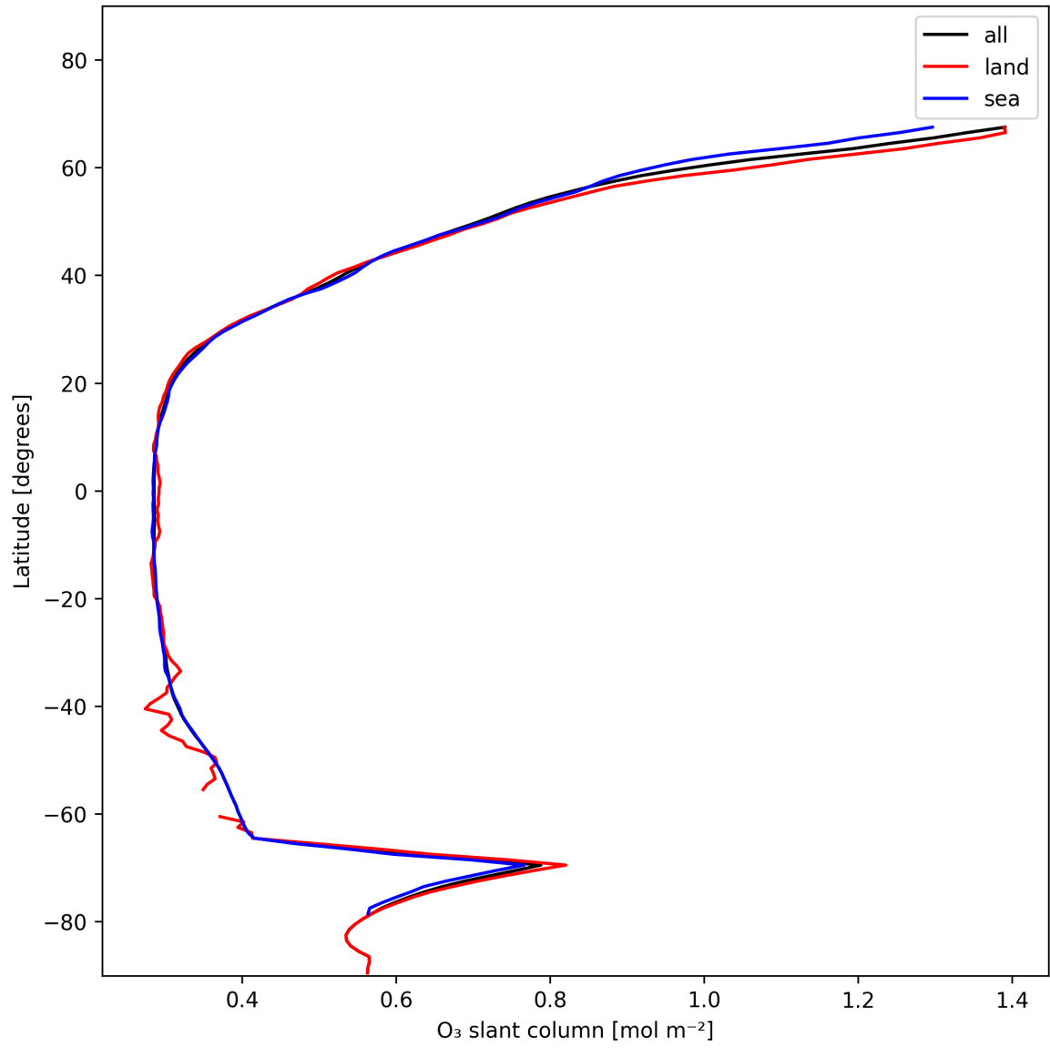
Figure 19: Zonal average of “O 3 slant column” for 2025-01-09 to 2025-01-10.
