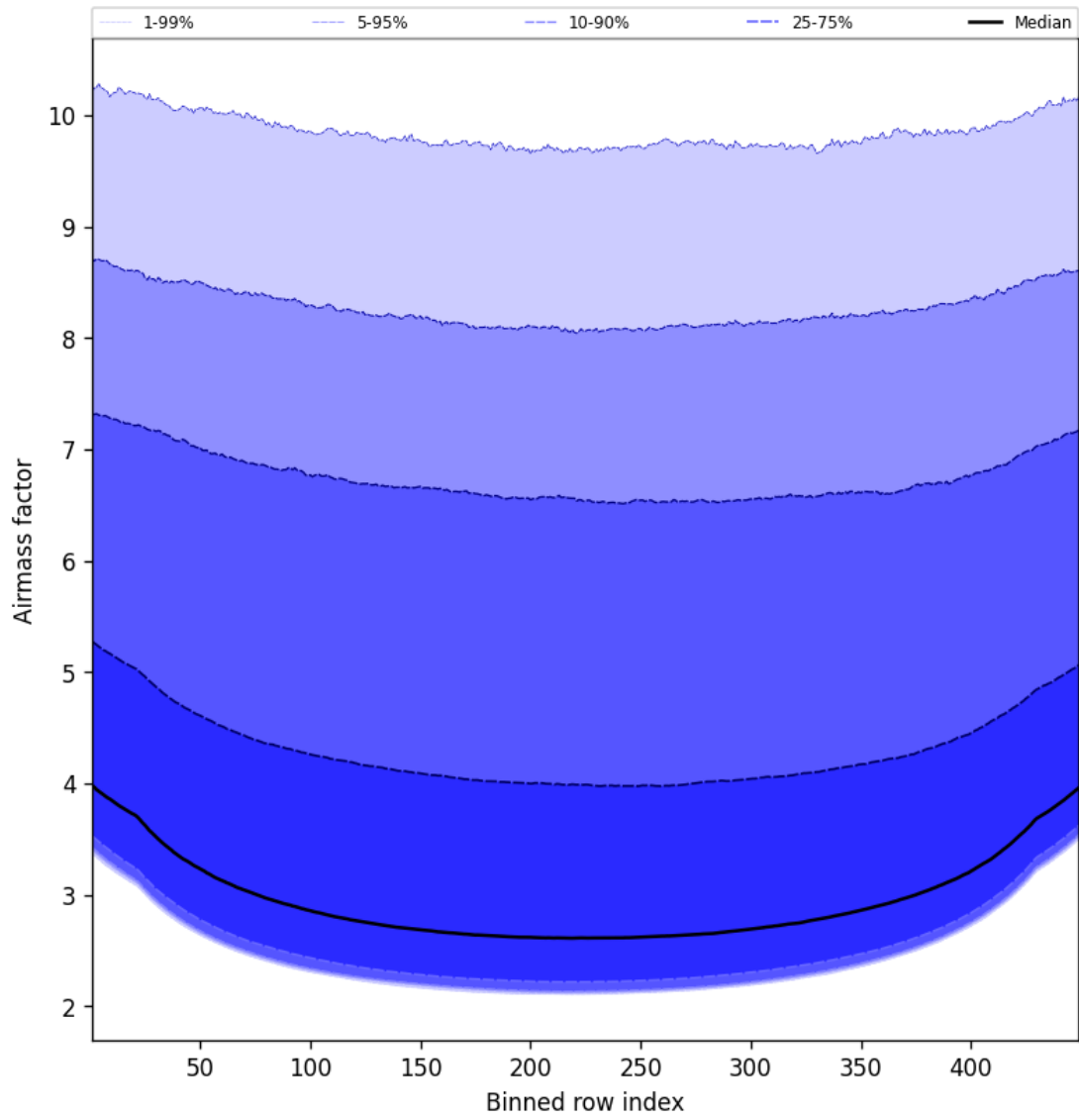
Figure 49: Along track statistics of “Airmass factor” for 2025-01-09 to 2025-01-10
