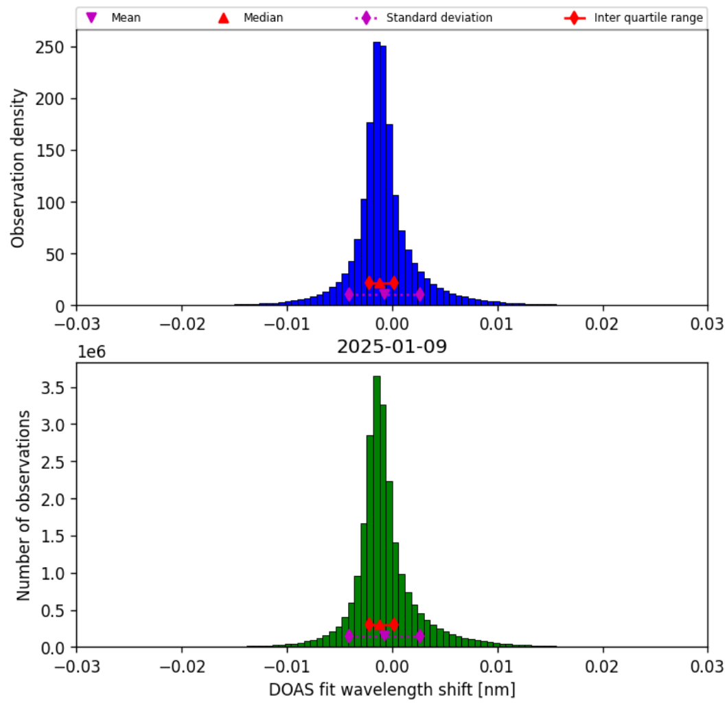
Figure 35: Histogram of “DOAS fit wavelength shift” for 2025-01-09 to 2025-01-10
