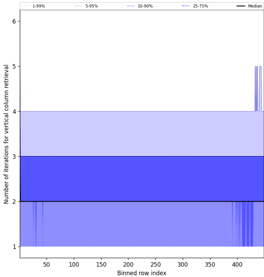
Figure 51: Along track statistics of “Number of iterations for vertical column retrieval” for 2025-01-09 to 2025-01-10
