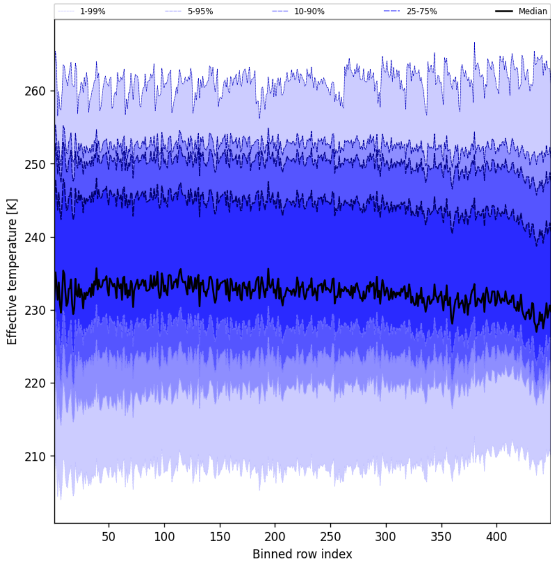
Figure 50: Along track statistics of “Effective temperature” for 2025-01-09 to 2025-01-10
