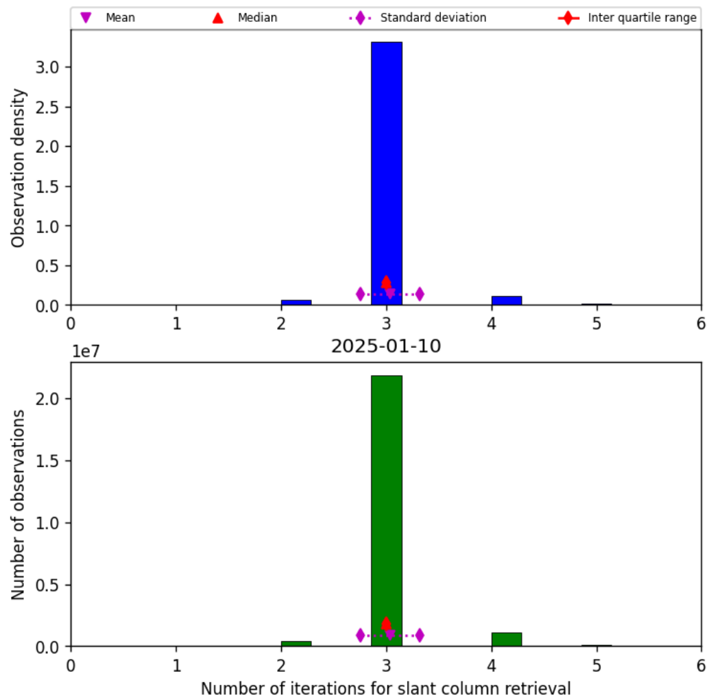
Figure 33: Histogram of “Number of iterations for slant column retrieval” for 2025-01-10 to 2025-01-10
