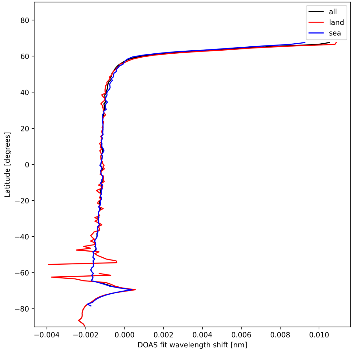
Figure 23: Zonal average of “DOAS fit wavelength shift” for 2025-01-10 to 2025-01-10.
