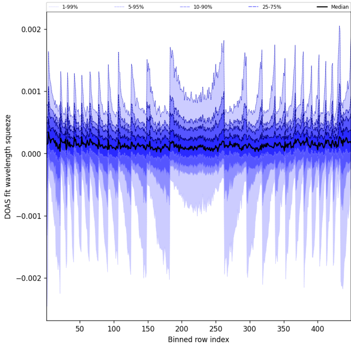
Figure 48: Along track statistics of “DOAS fit wavelength squeeze” for 2025-01-10 to 2025-01-10
