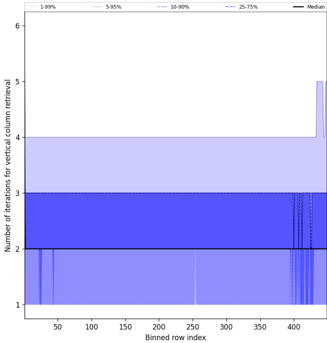
Figure 51: Along track statistics of “Number of iterations for vertical column retrieval” for 2025-01-10 to 2025-01-10
