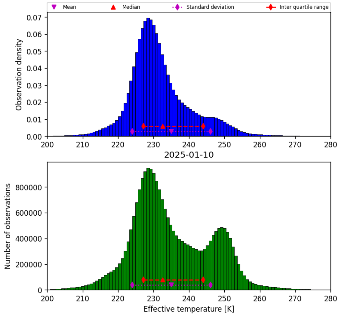
Figure 38: Histogram of “Effective temperature” for 2025-01-10 to 2025-01-10
