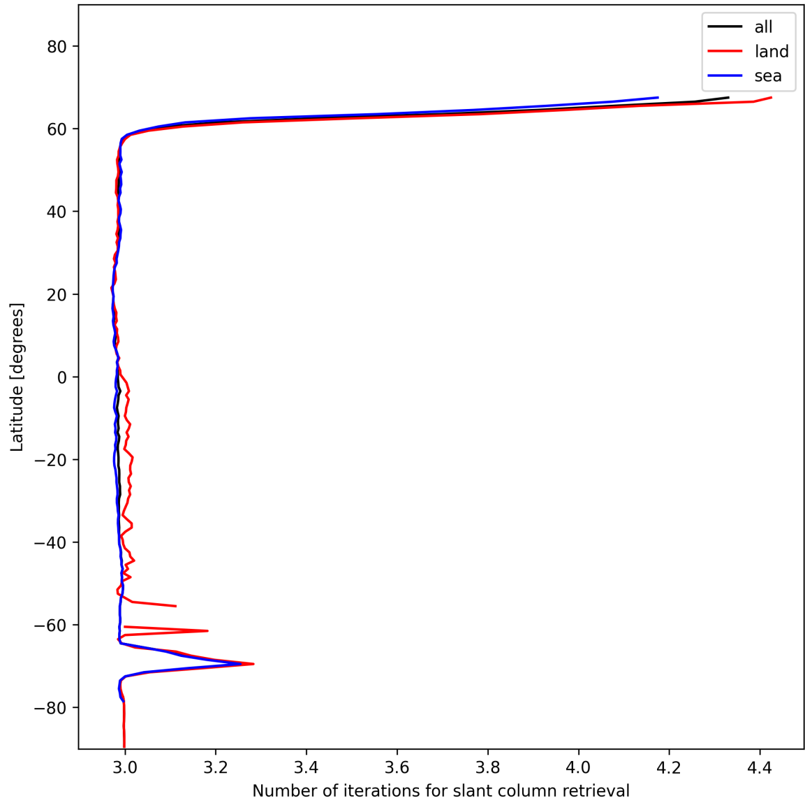
Figure 21: Zonal average of “Number of iterations for slant column retrieval” for 2025-01-10 to 2025-01-10.
