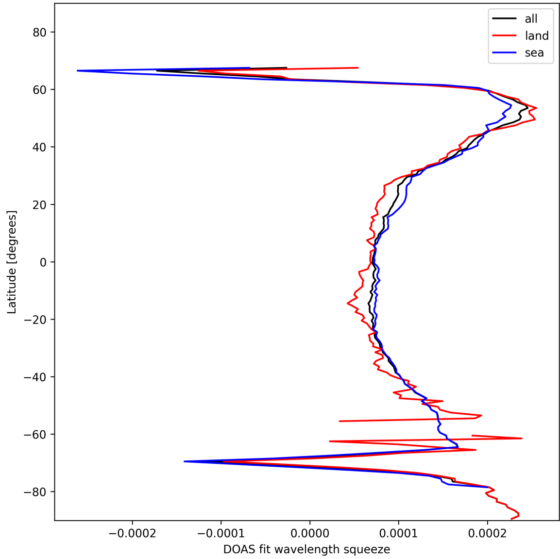
Figure 24: Zonal average of “DOAS fit wavelength squeeze” for 2025-01-10 to 2025-01-10.
