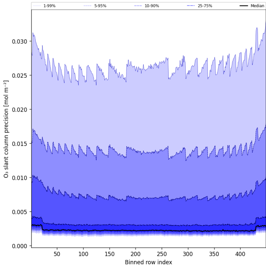
Figure 44: Along track statistics of “O 3 slant column precision” for 2025-01-10 to 2025-01-10
