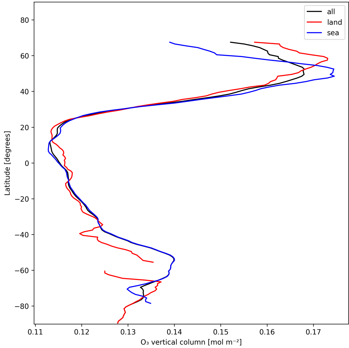
Figure 17: Zonal average of “O 3 vertical column” for 2025-01-10 to 2025-01-10.
