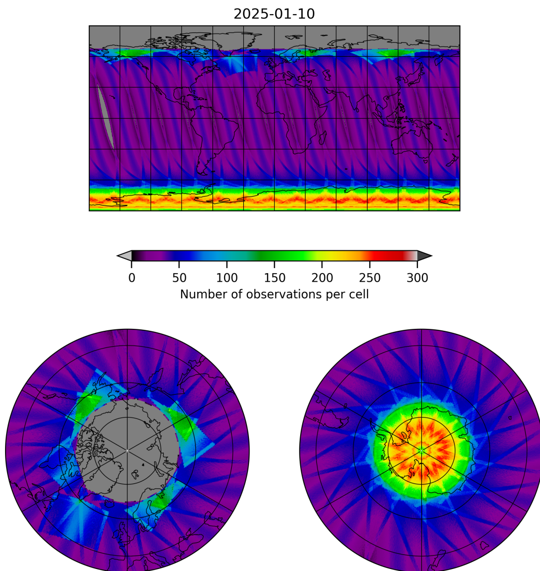
Figure 15: Map of the number of observations for 2025-01-10 to 2025-01-10
