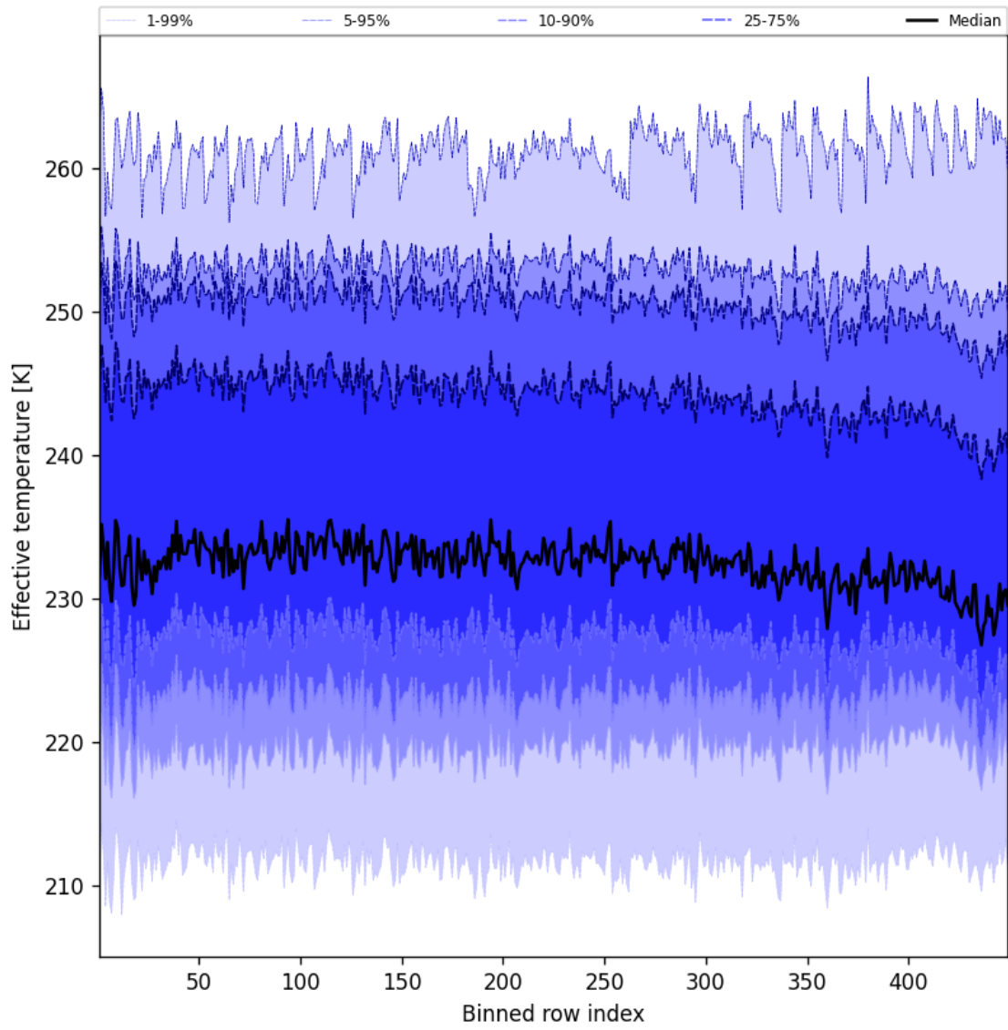
Figure 50: Along track statistics of “Effective temperature” for 2025-01-10 to 2025-01-10
