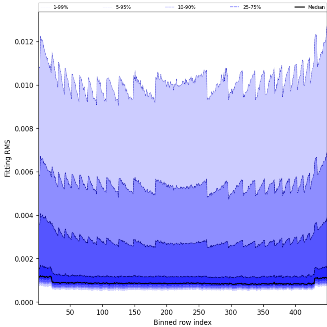
Figure 46: Along track statistics of “Fitting RMS” for 2025-01-10 to 2025-01-10
