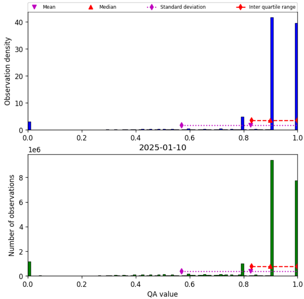
Figure 28: Histogram of “QA value” for 2025-01-10 to 2025-01-10
