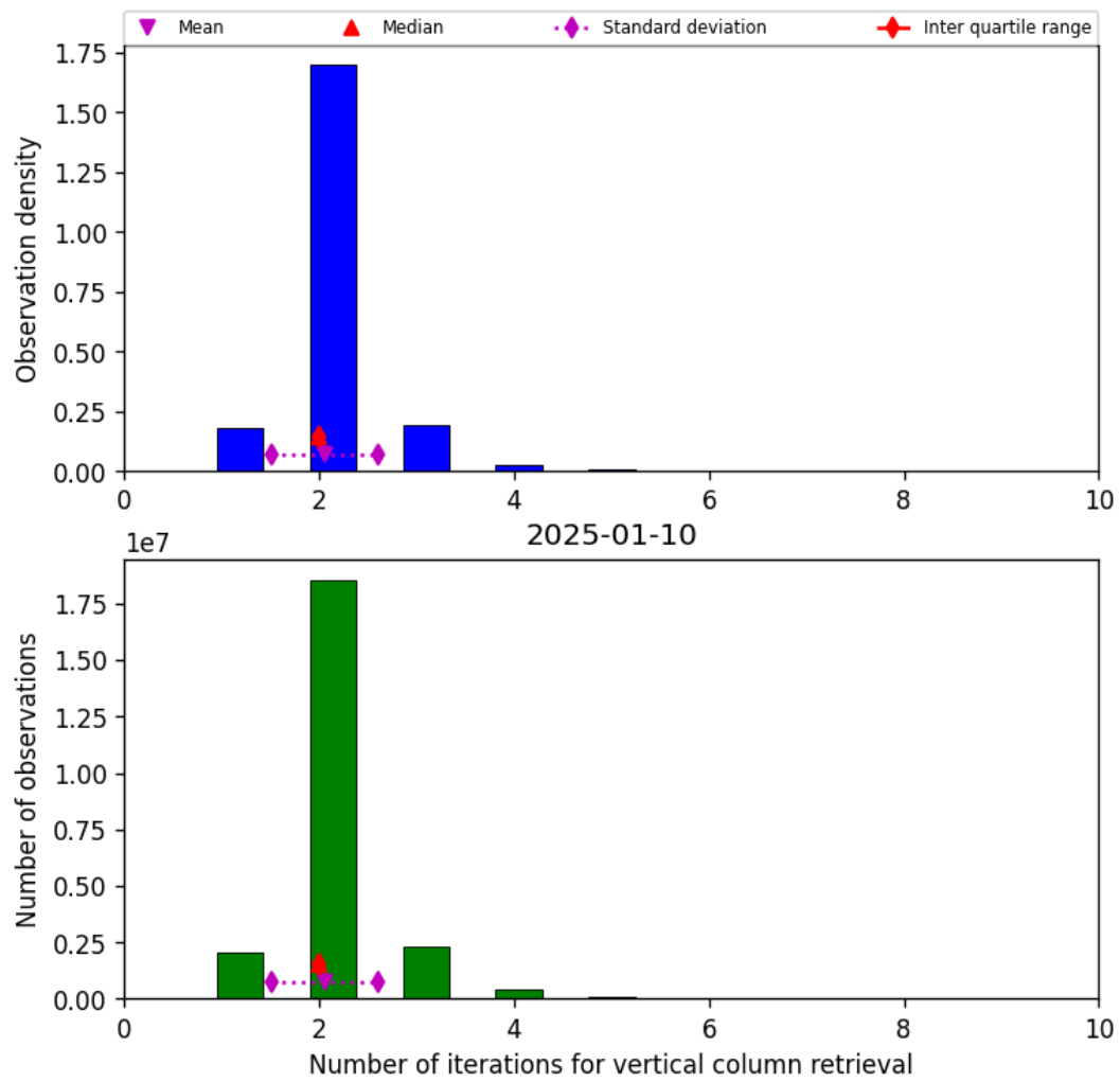
Figure 39: Histogram of “Number of iterations for vertical column retrieval” for 2025-01-10 to 2025-01-10
