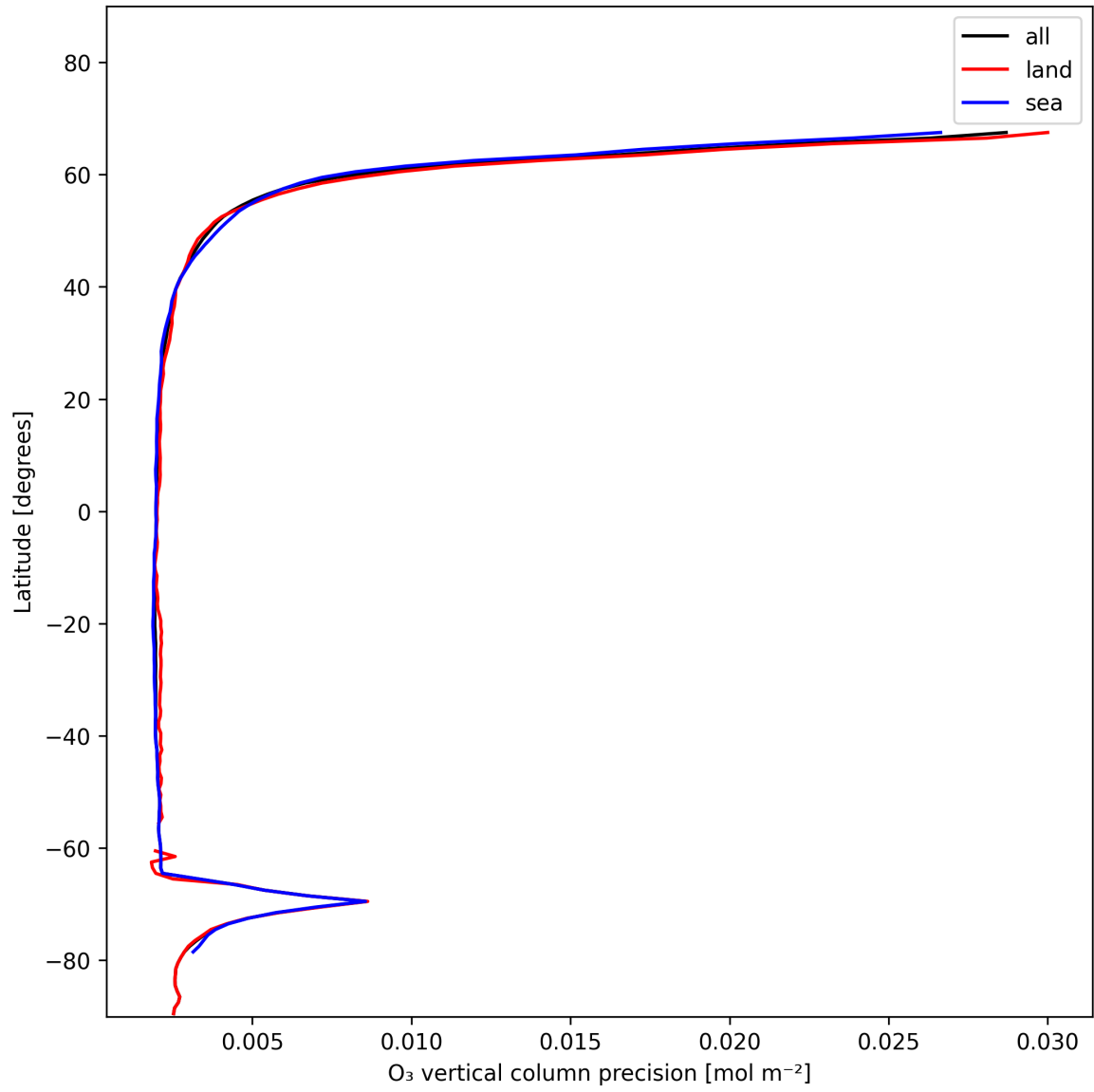
Figure 18: Zonal average of “O 3 vertical column precision” for 2025-01-10 to 2025-01-10.
