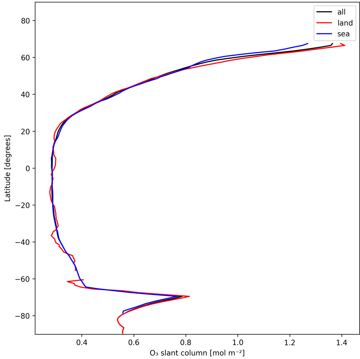
Figure 19: Zonal average of “O 3 slant column” for 2025-01-10 to 2025-01-10.
