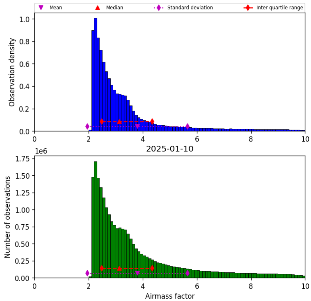
Figure 37: Histogram of “Airmass factor” for 2025-01-10 to 2025-01-10
