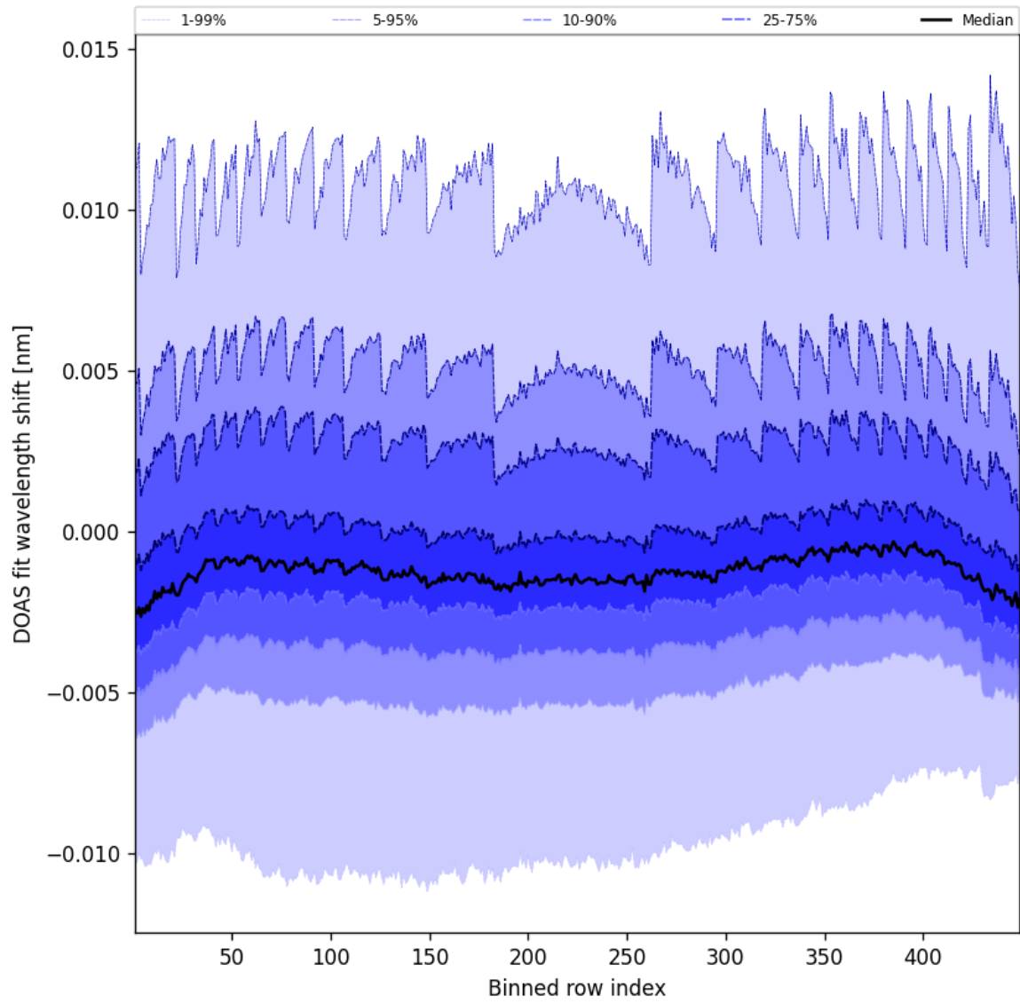
Figure 47: Along track statistics of “DOAS fit wavelength shift” for 2025-01-10 to 2025-01-10
