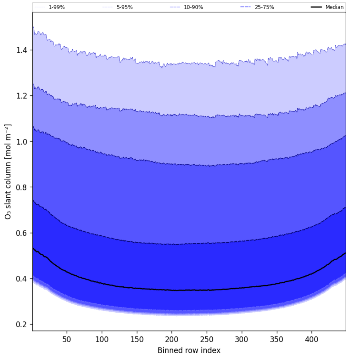
Figure 43: Along track statistics of “O 3 slant column” for 2025-01-10 to 2025-01-10
