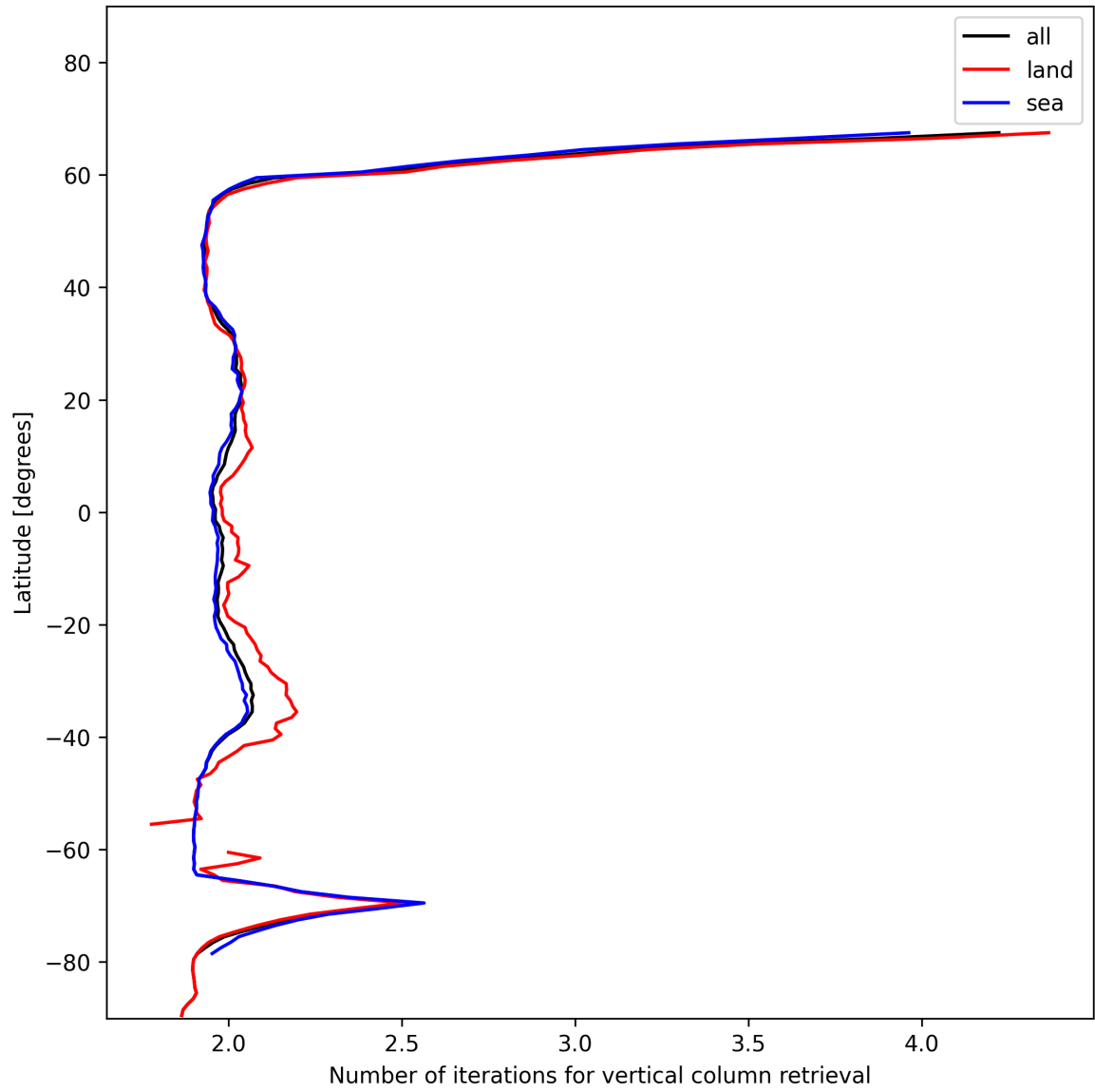
Figure 27: Zonal average of “Number of iterations for vertical column retrieval” for 2025-01-10 to 2025-01-10.
