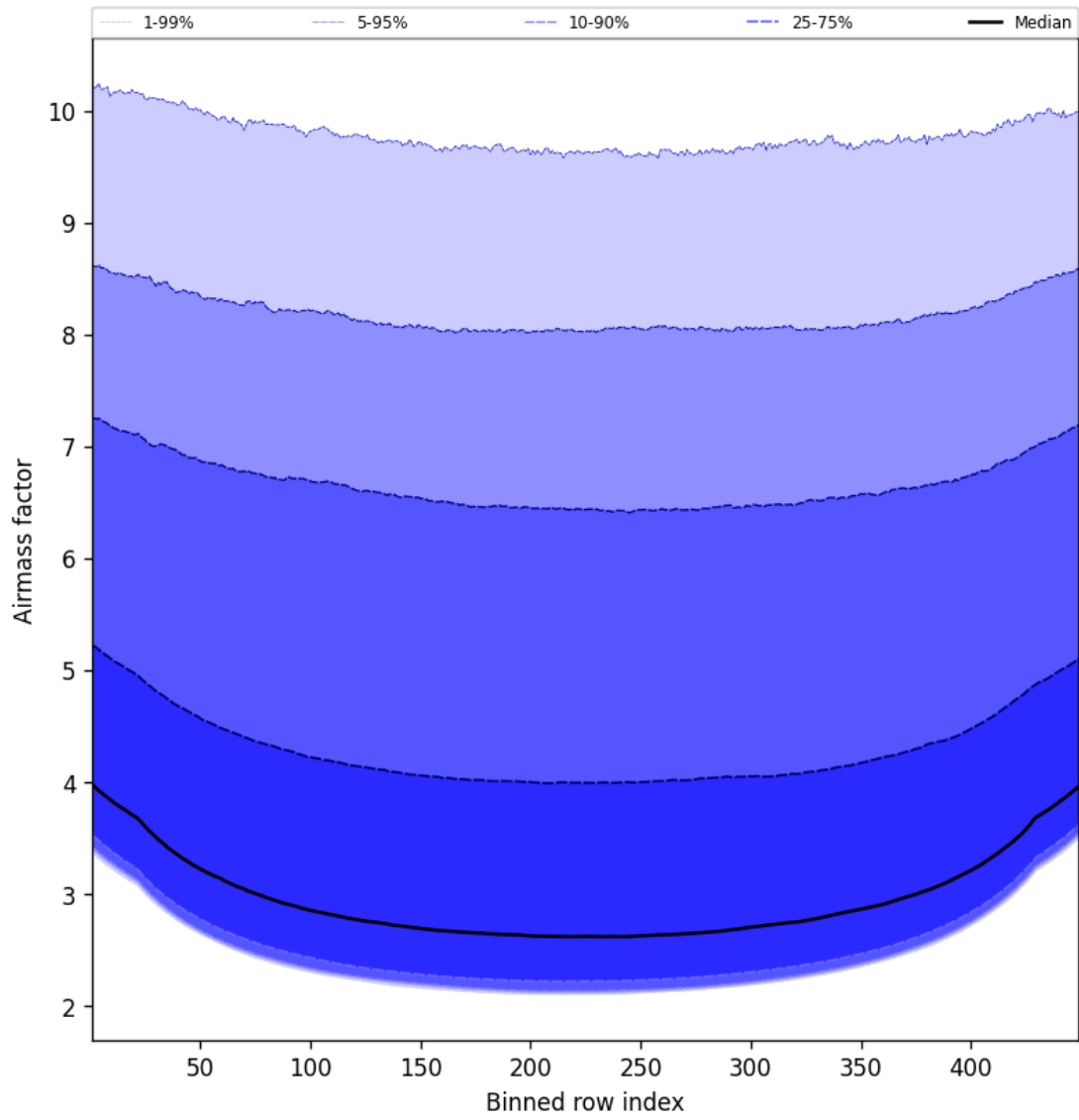
Figure 49: Along track statistics of “Airmass factor” for 2025-01-10 to 2025-01-10
