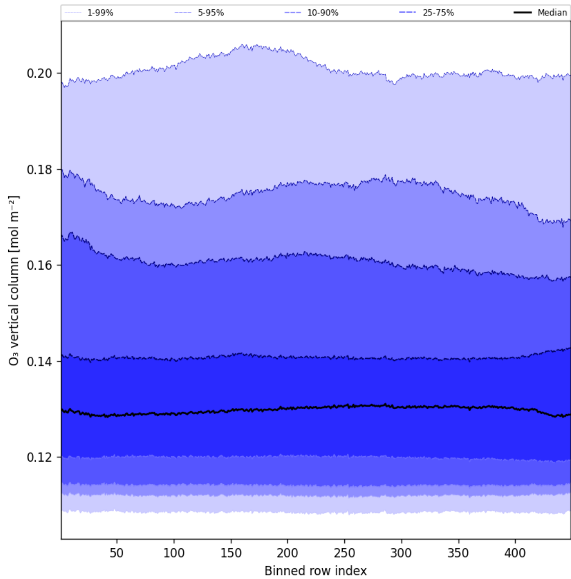
Figure 41: Along track statistics of “O 3 vertical column” for 2025-01-10 to 2025-01-10
