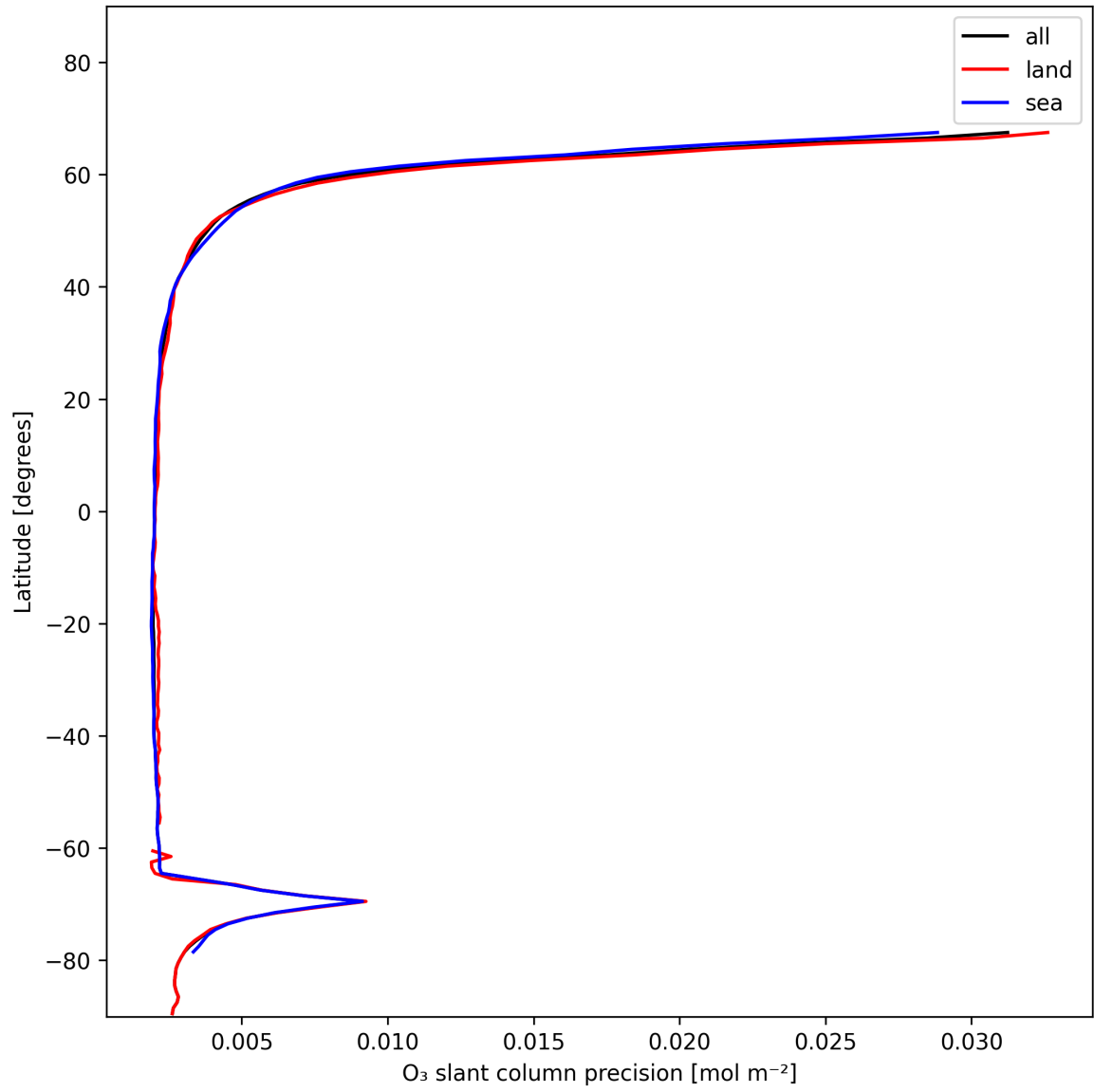
Figure 20: Zonal average of “O 3 slant column precision” for 2025-01-10 to 2025-01-10.
