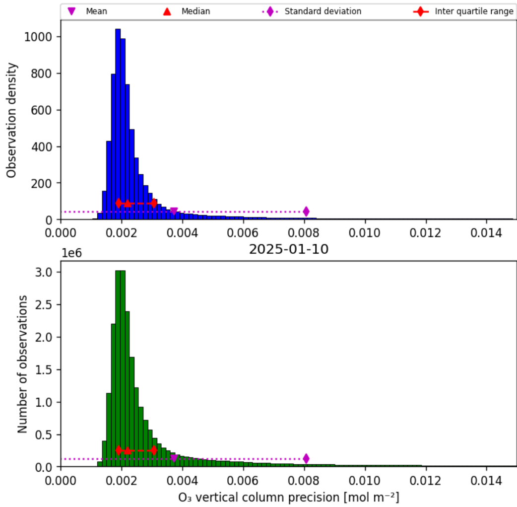
Figure 30: Histogram of “O 3 vertical column precision” for 2025-01-10 to 2025-01-10
