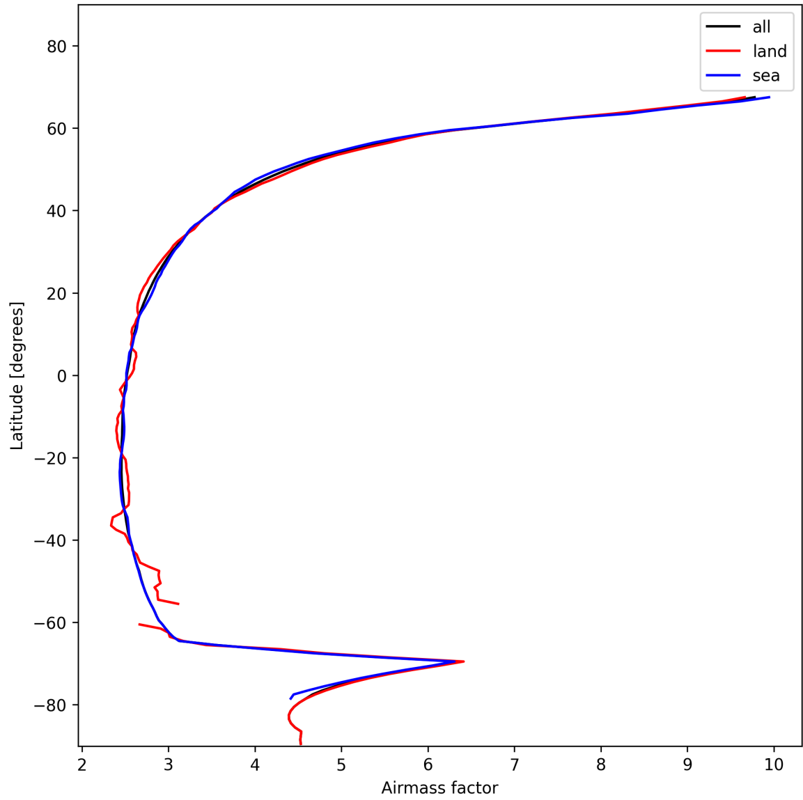
Figure 25: Zonal average of “Airmass factor” for 2025-01-10 to 2025-01-10.
