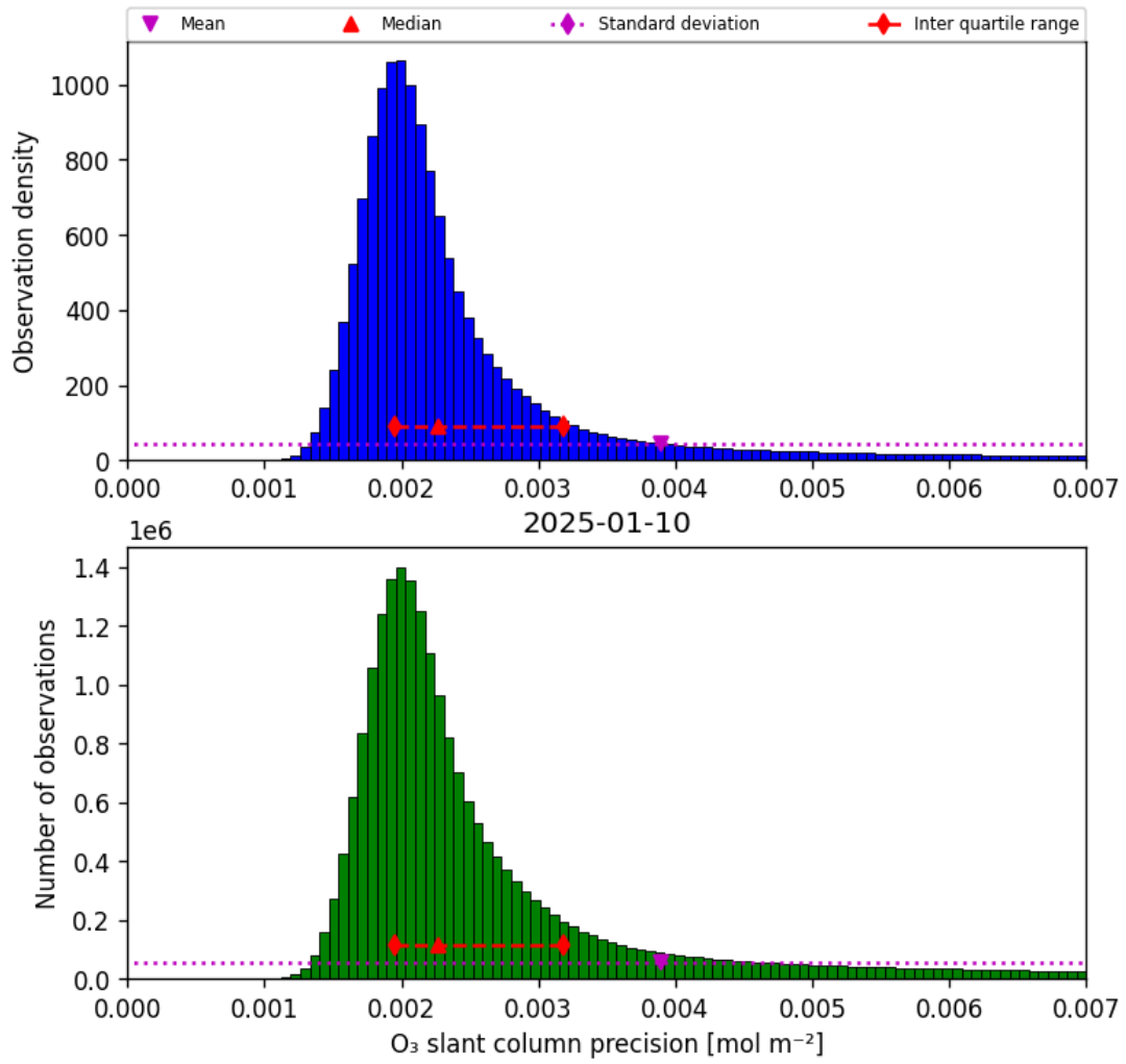
Figure 32: Histogram of “O 3 slant column precision” for 2025-01-10 to 2025-01-10
