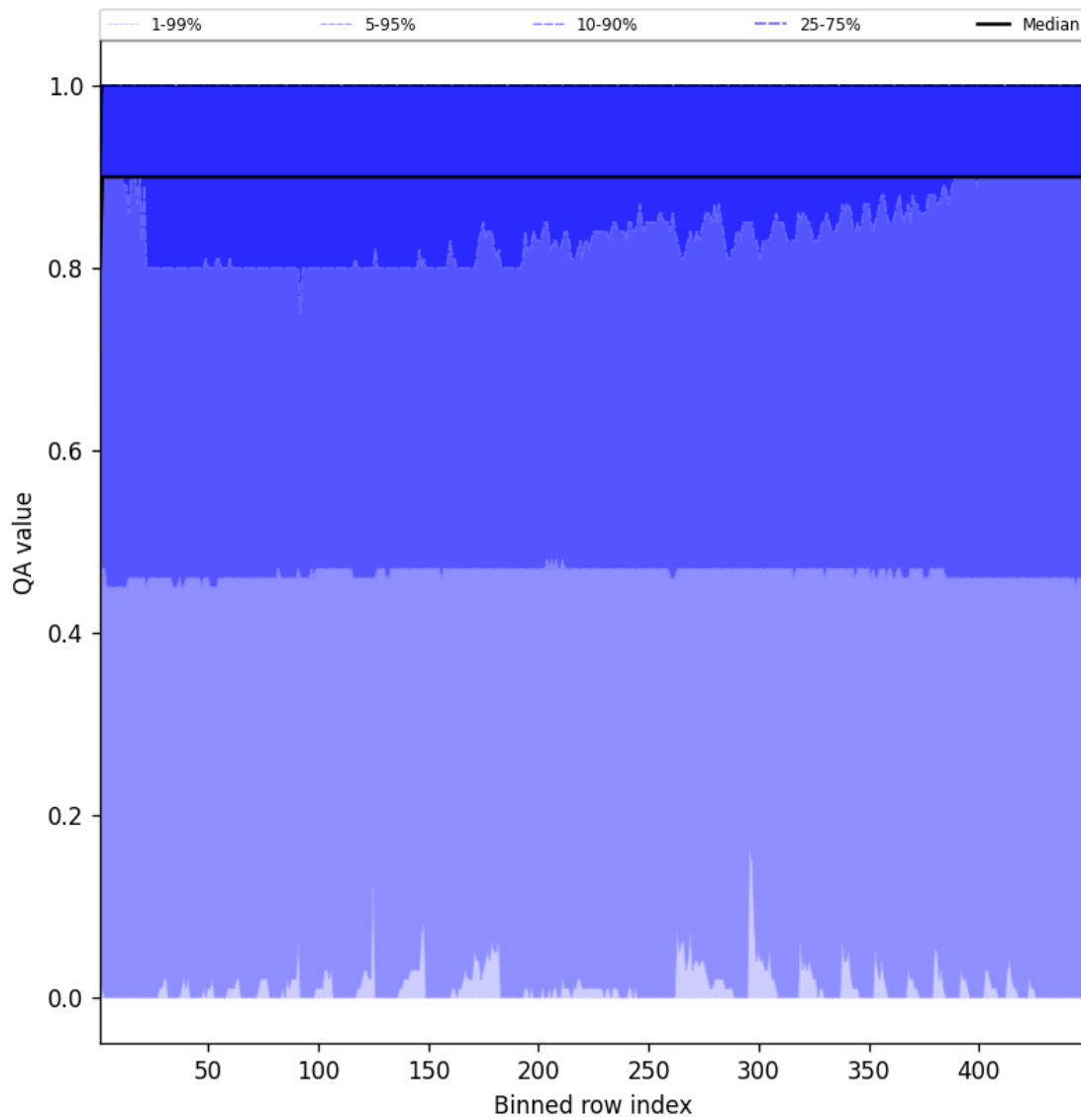
Figure 40: Along track statistics of “QA value” for 2025-01-10 to 2025-01-10
