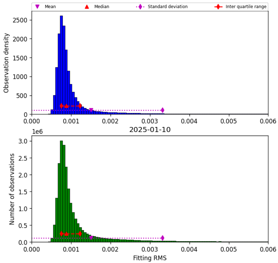
Figure 34: Histogram of “Fitting RMS” for 2025-01-10 to 2025-01-10
