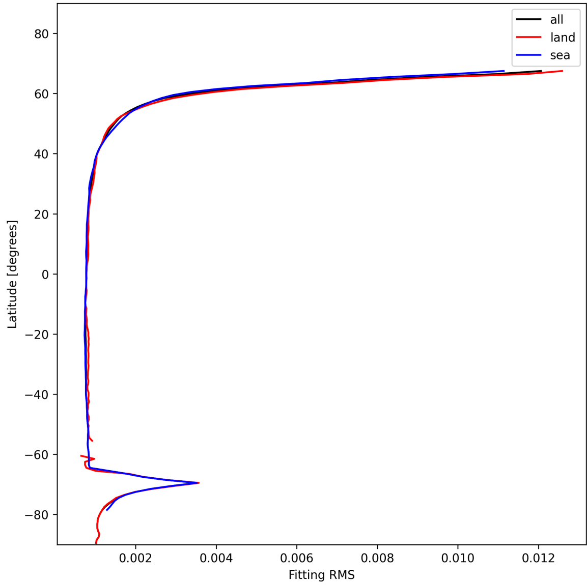
Figure 22: Zonal average of “Fitting RMS” for 2025-01-10 to 2025-01-10.
