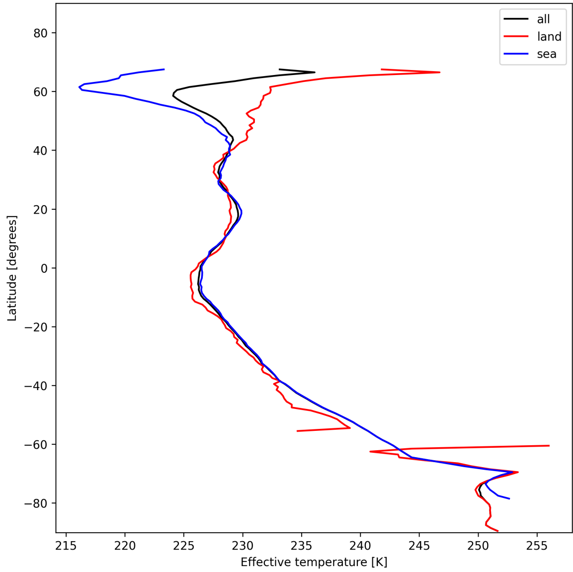
Figure 26: Zonal average of “Effective temperature” for 2025-01-10 to 2025-01-10.
