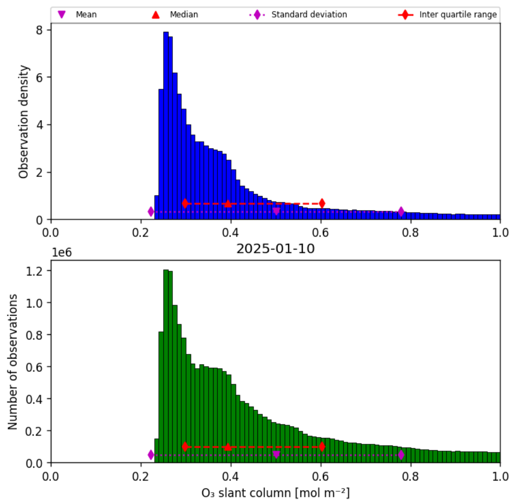
Figure 31: Histogram of “O 3 slant column” for 2025-01-10 to 2025-01-10
