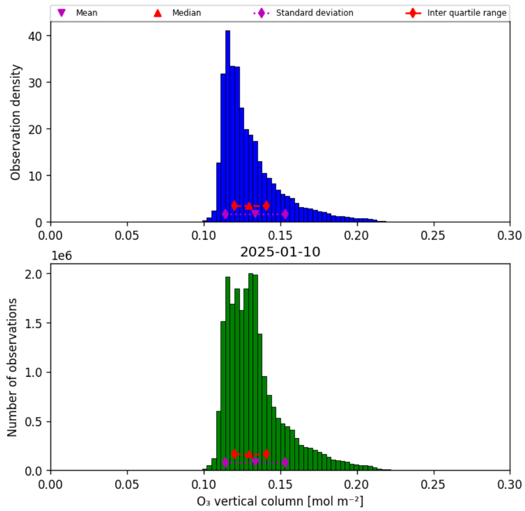
Figure 29: Histogram of “O 3 vertical column” for 2025-01-10 to 2025-01-10
