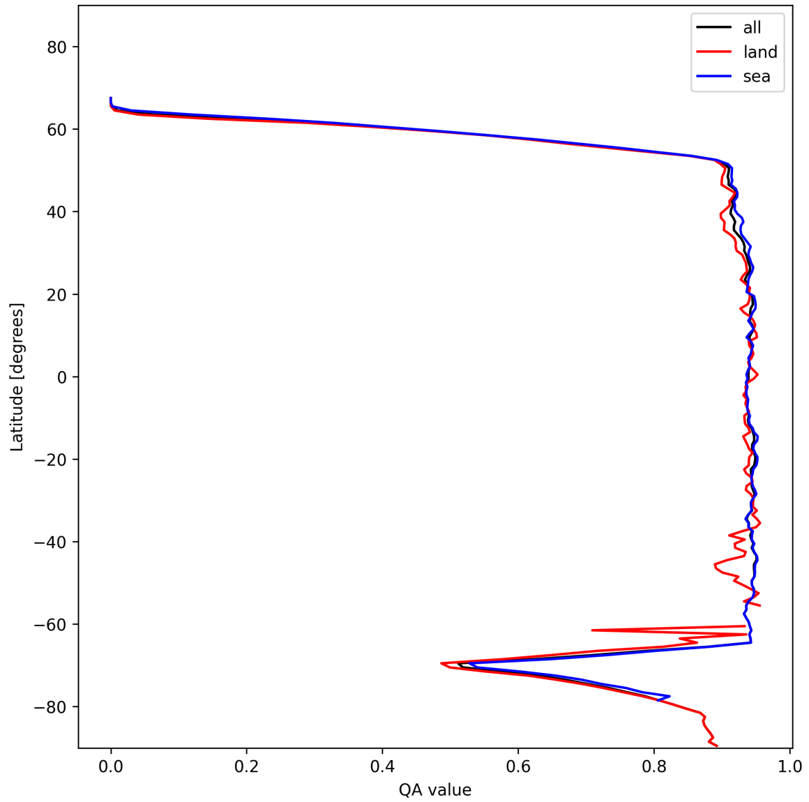
Figure 16: Zonal average of “QA value” for 2025-01-10 to 2025-01-10.
