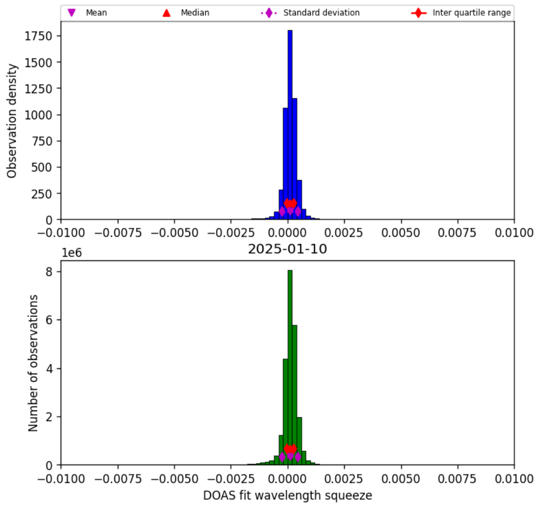
Figure 36: Histogram of “DOAS fit wavelength squeeze” for 2025-01-10 to 2025-01-10
