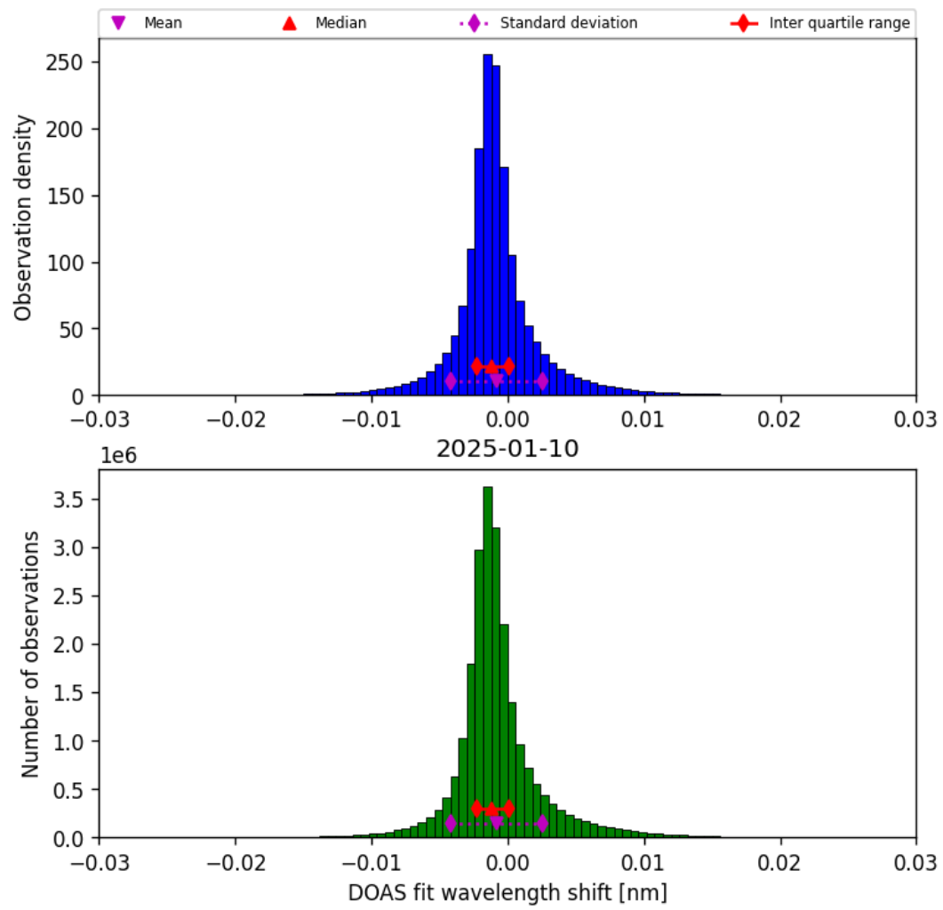
Figure 35: Histogram of “DOAS fit wavelength shift” for 2025-01-10 to 2025-01-10
