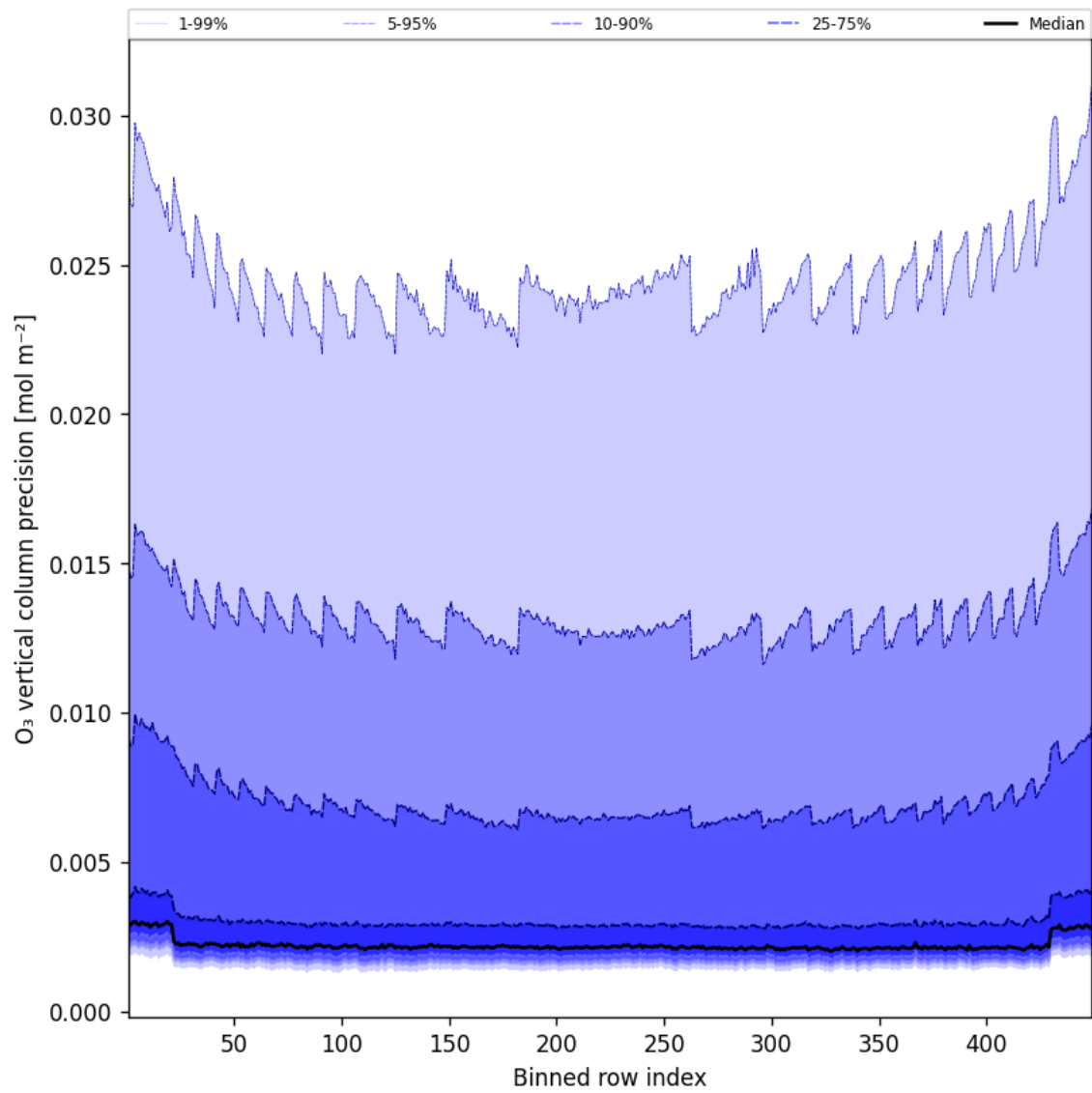
Figure 42: Along track statistics of “O 3 vertical column precision” for 2025-01-10 to 2025-01-10
