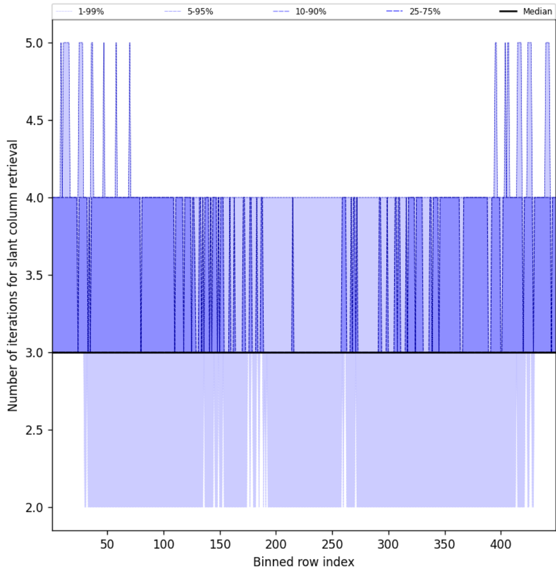
Figure 45: Along track statistics of “Number of iterations for slant column retrieval” for 2025-01-10 to 2025-01-10
