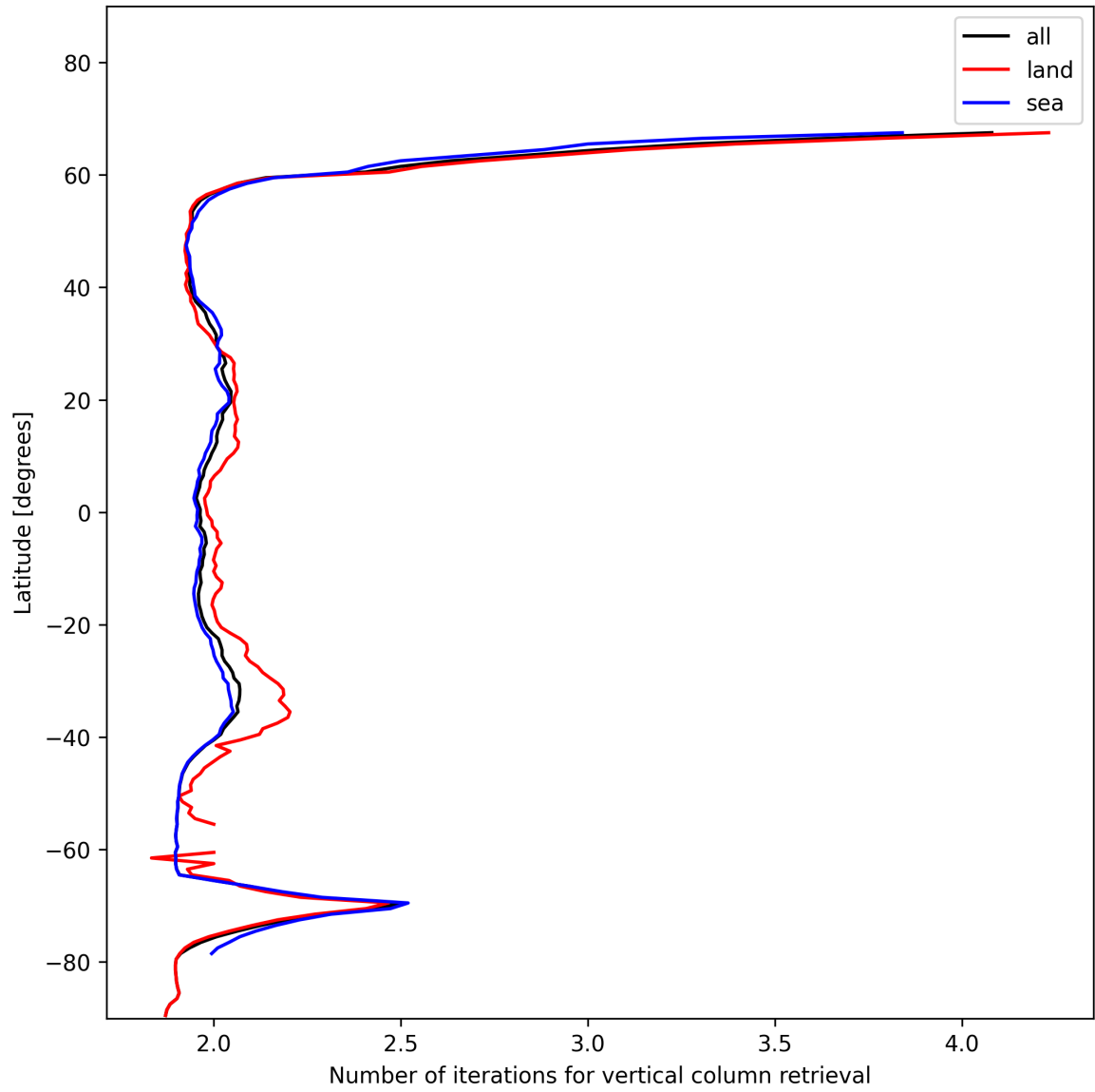
Figure 27: Zonal average of “Number of iterations for vertical column retrieval” for 2025-01-12 to 2025-01-13.
