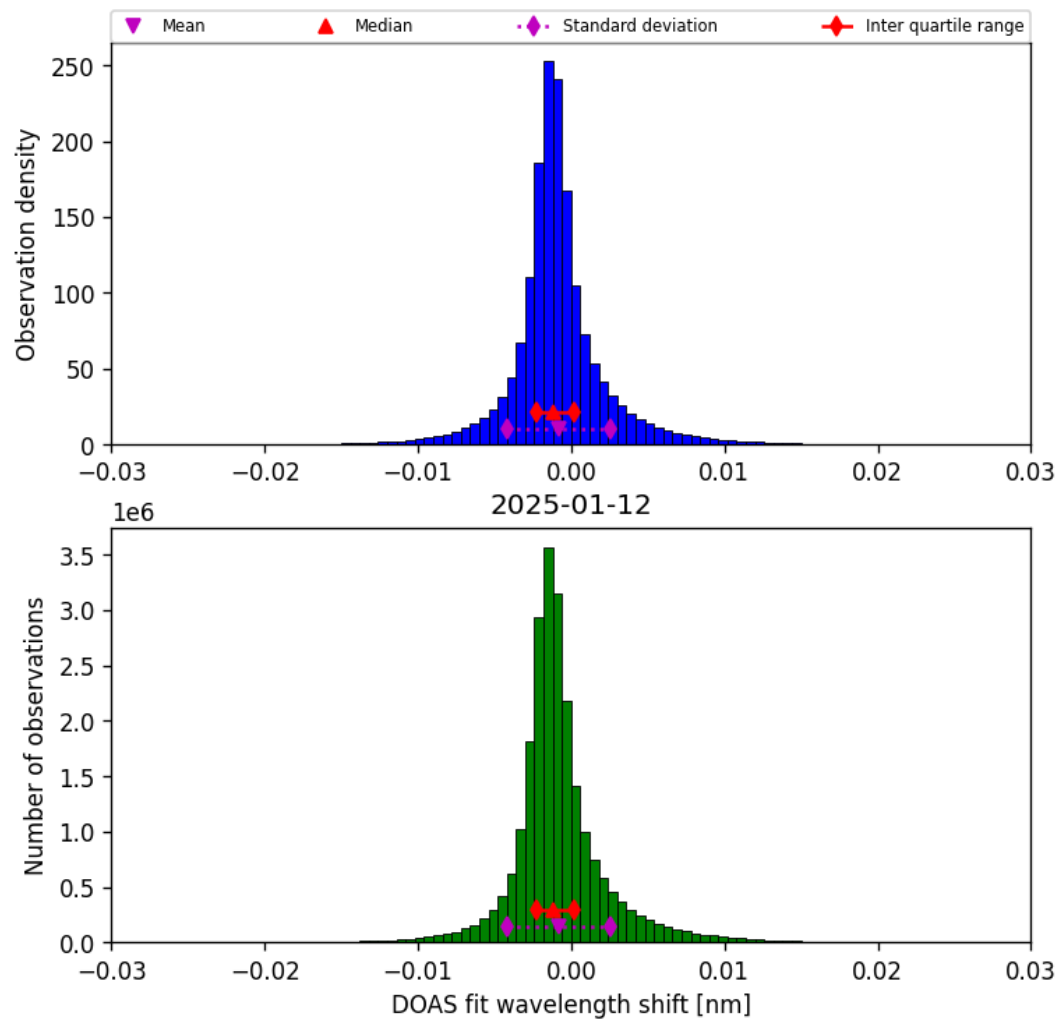
Figure 35: Histogram of “DOAS fit wavelength shift” for 2025-01-12 to 2025-01-13
