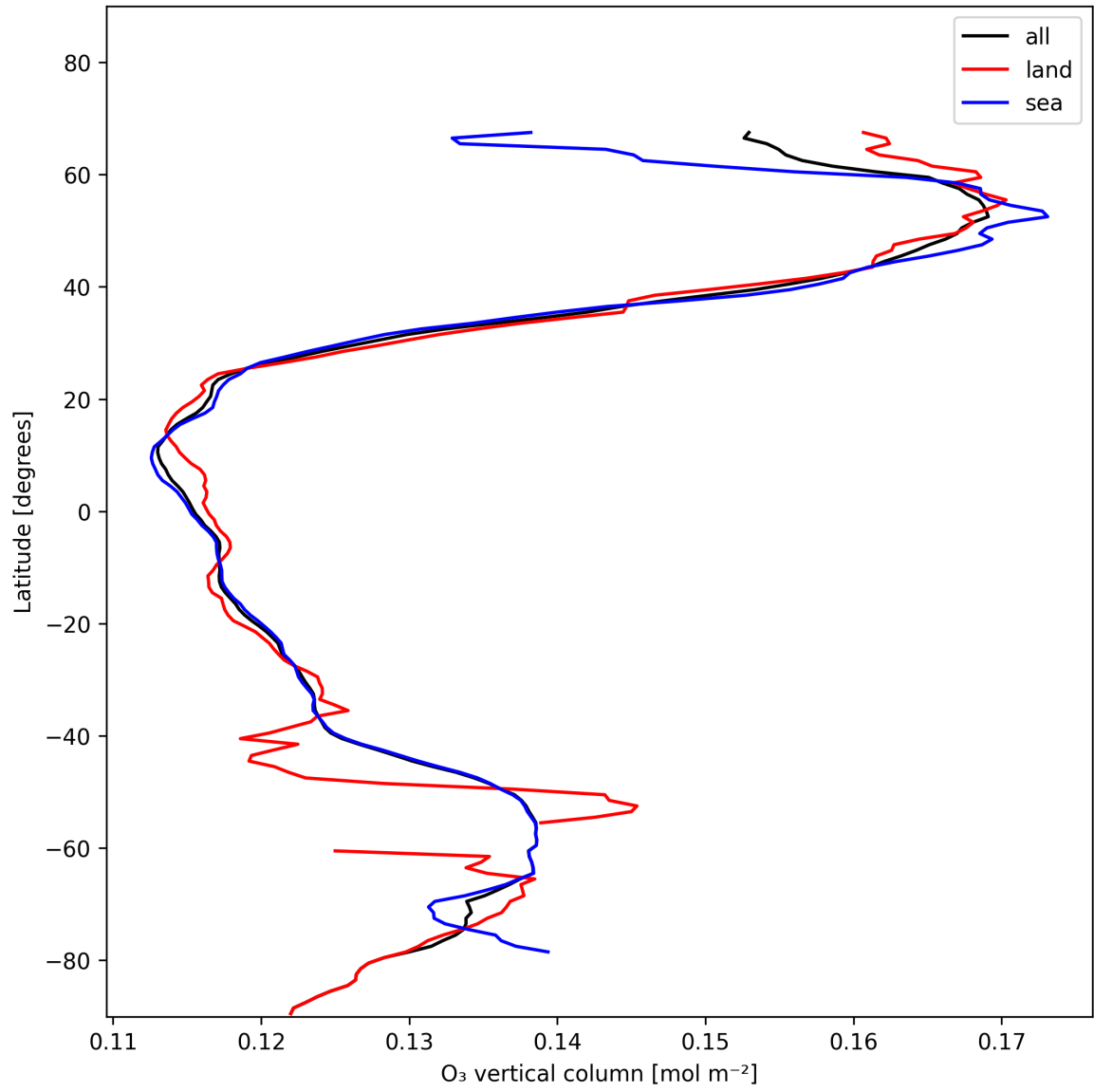
Figure 17: Zonal average of “O 3 vertical column” for 2025-01-12 to 2025-01-13.
