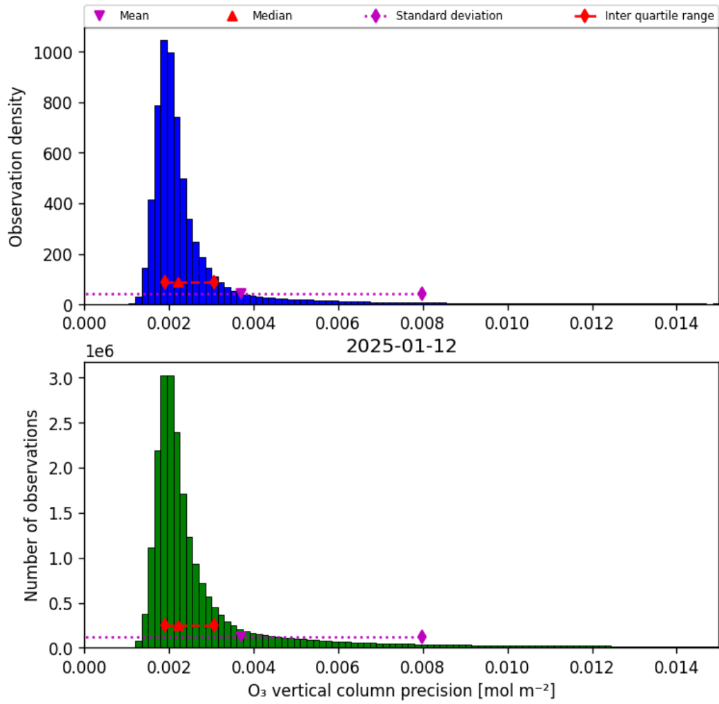
Figure 30: Histogram of “O 3 vertical column precision” for 2025-01-12 to 2025-01-13
