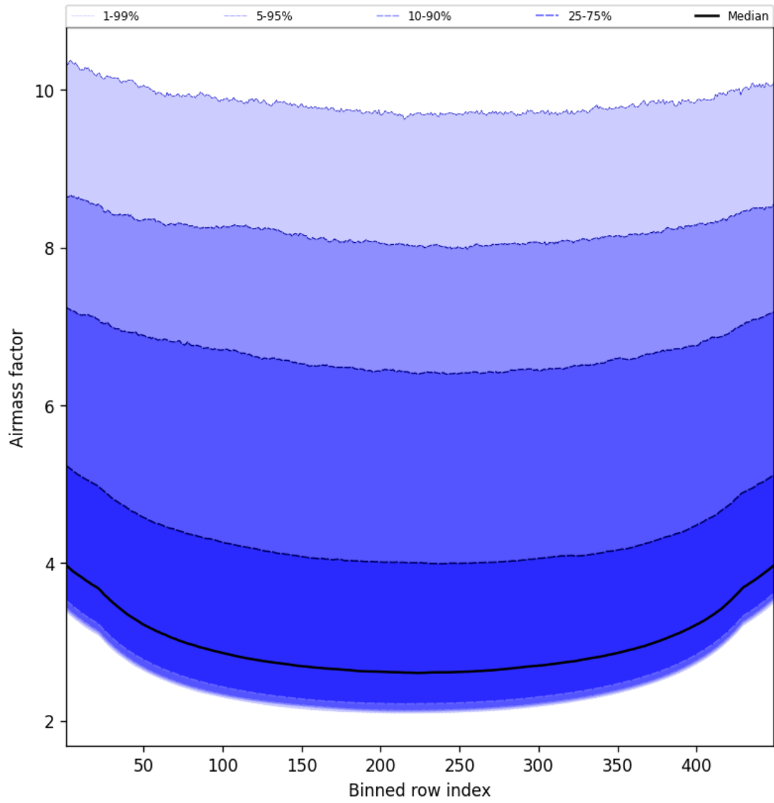
Figure 49: Along track statistics of “Airmass factor” for 2025-01-12 to 2025-01-13
