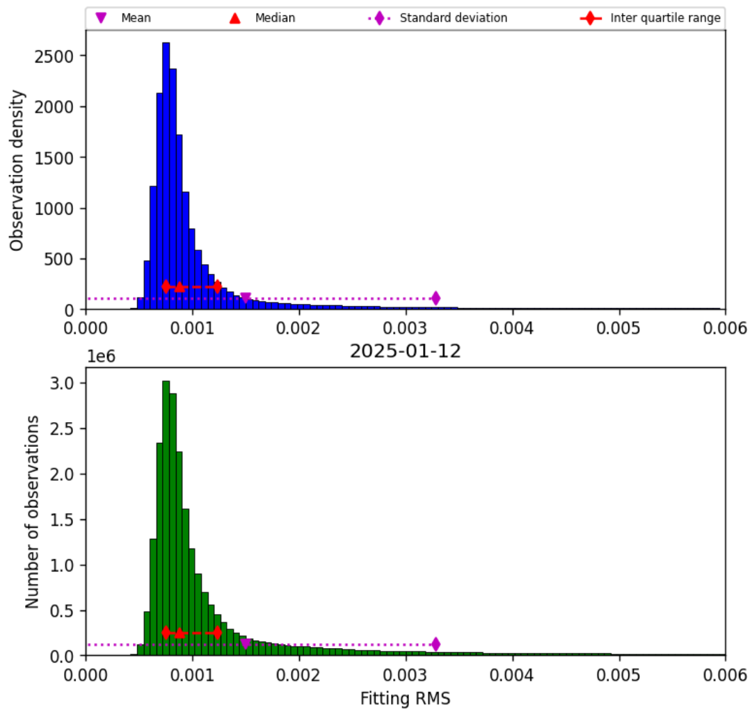
Figure 34: Histogram of “Fitting RMS” for 2025-01-12 to 2025-01-13
