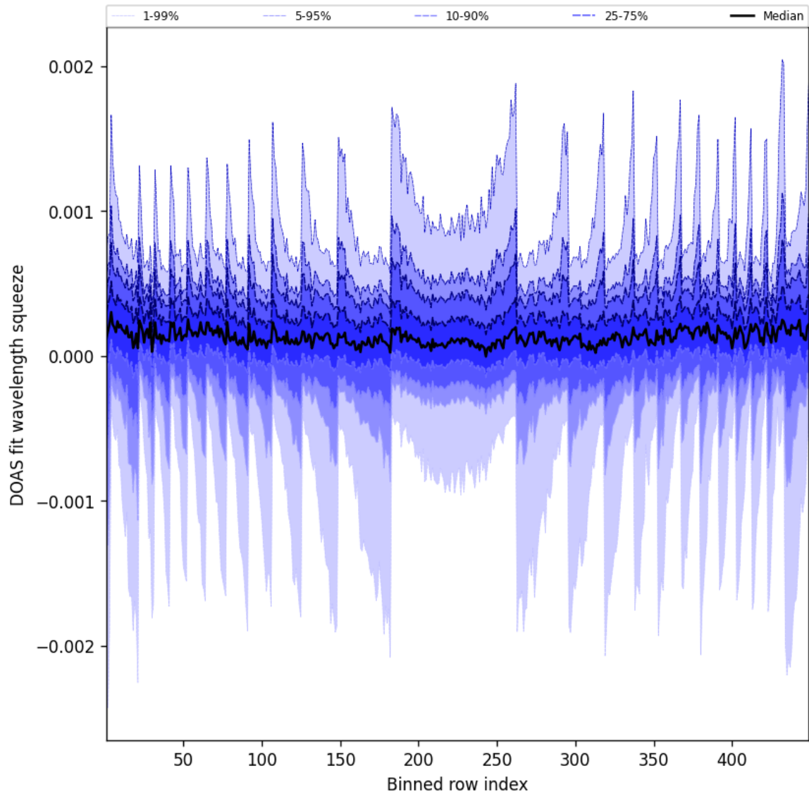
Figure 48: Along track statistics of “DOAS fit wavelength squeeze” for 2025-01-12 to 2025-01-13
