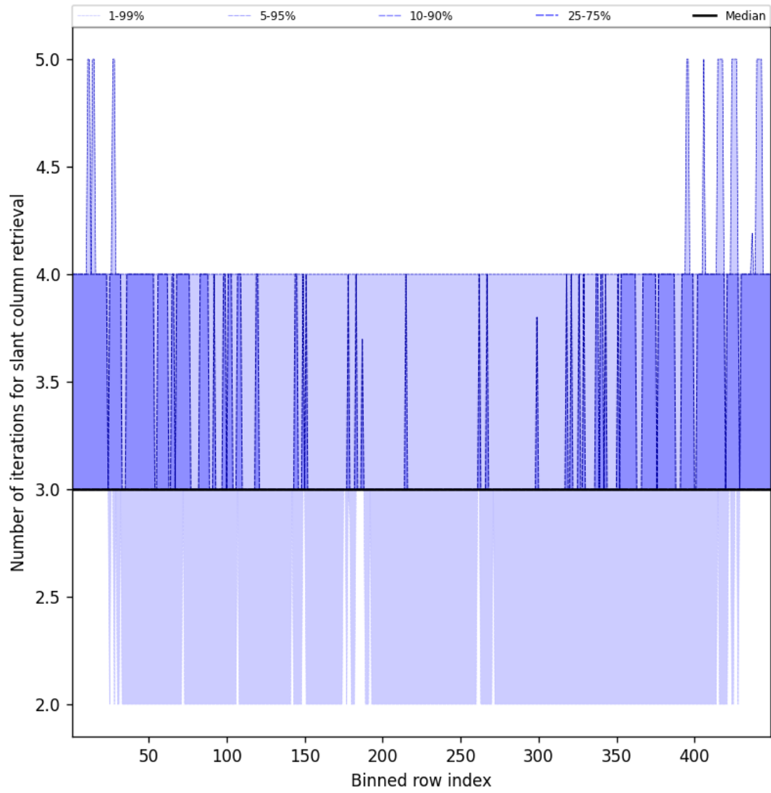
Figure 45: Along track statistics of “Number of iterations for slant column retrieval” for 2025-01-12 to 2025-01-13
