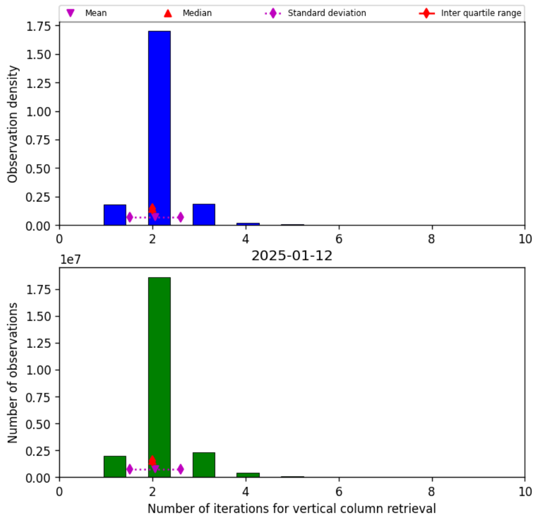
Figure 39: Histogram of “Number of iterations for vertical column retrieval” for 2025-01-12 to 2025-01-13
