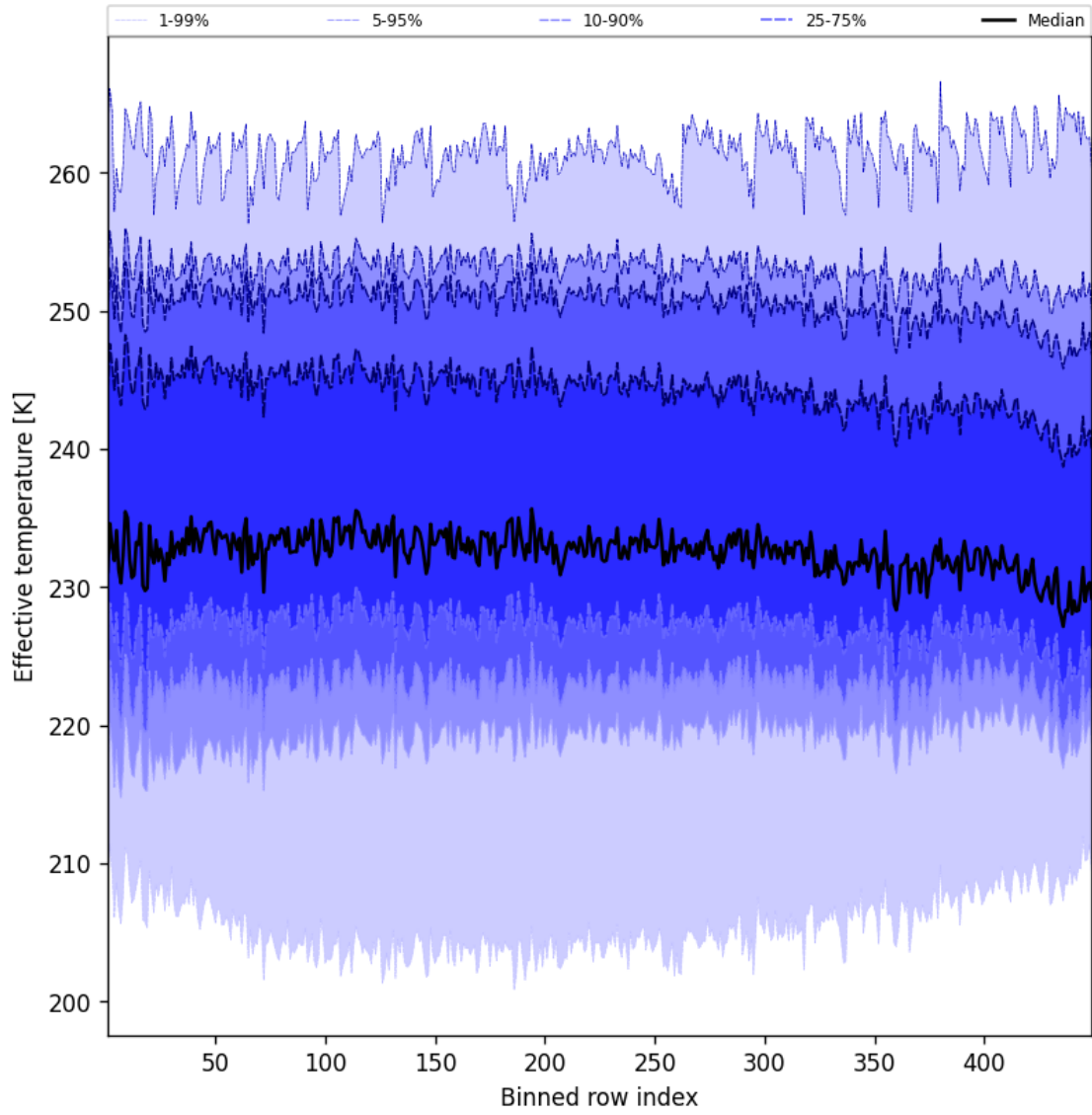
Figure 50: Along track statistics of “Effective temperature” for 2025-01-12 to 2025-01-13
