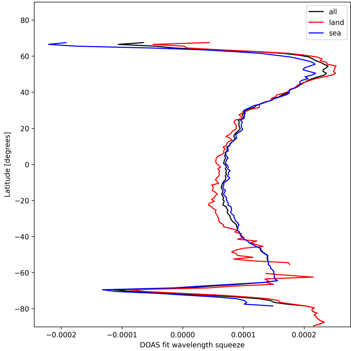
Figure 24: Zonal average of “DOAS fit wavelength squeeze” for 2025-01-12 to 2025-01-13.
