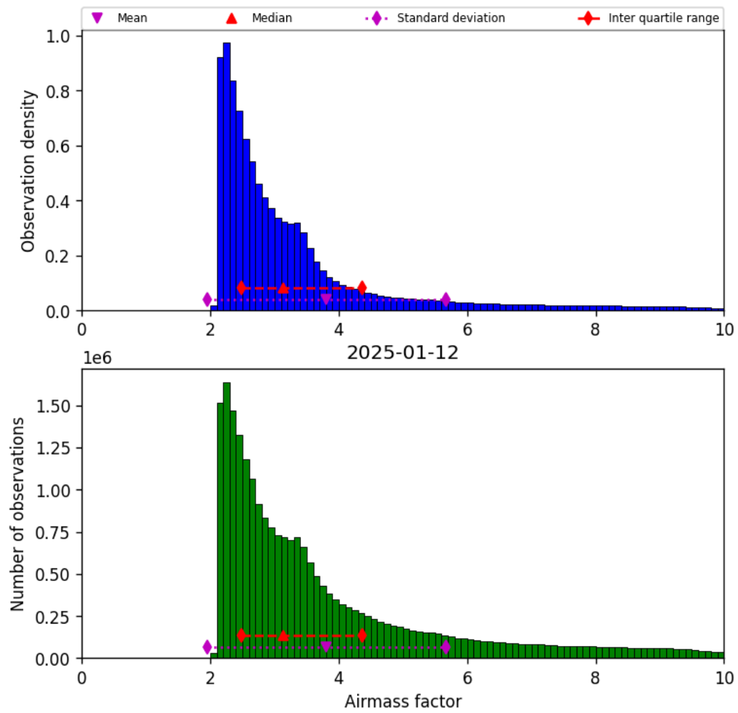
Figure 37: Histogram of “Airmass factor” for 2025-01-12 to 2025-01-13
