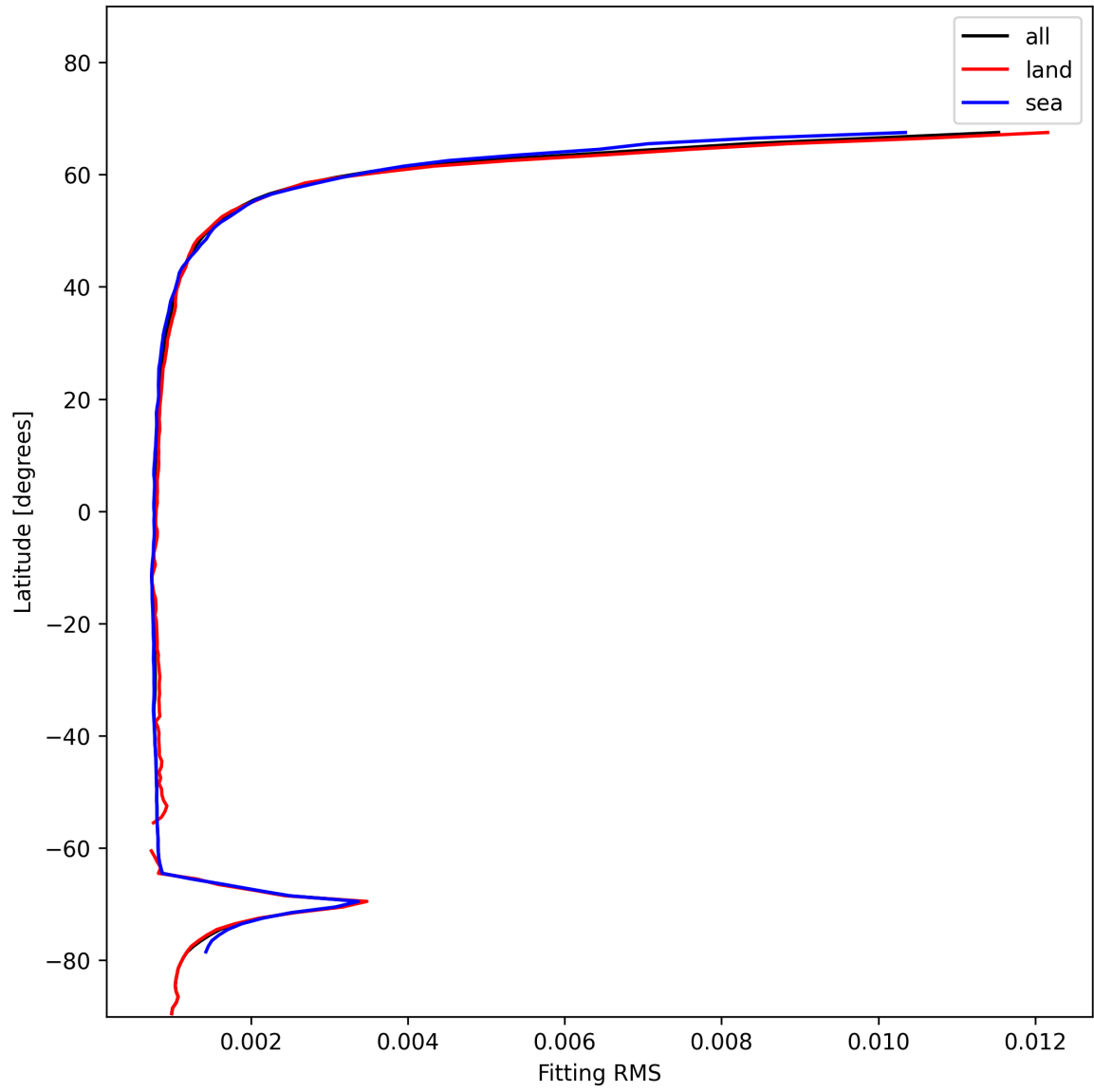
Figure 22: Zonal average of “Fitting RMS” for 2025-01-12 to 2025-01-13.
