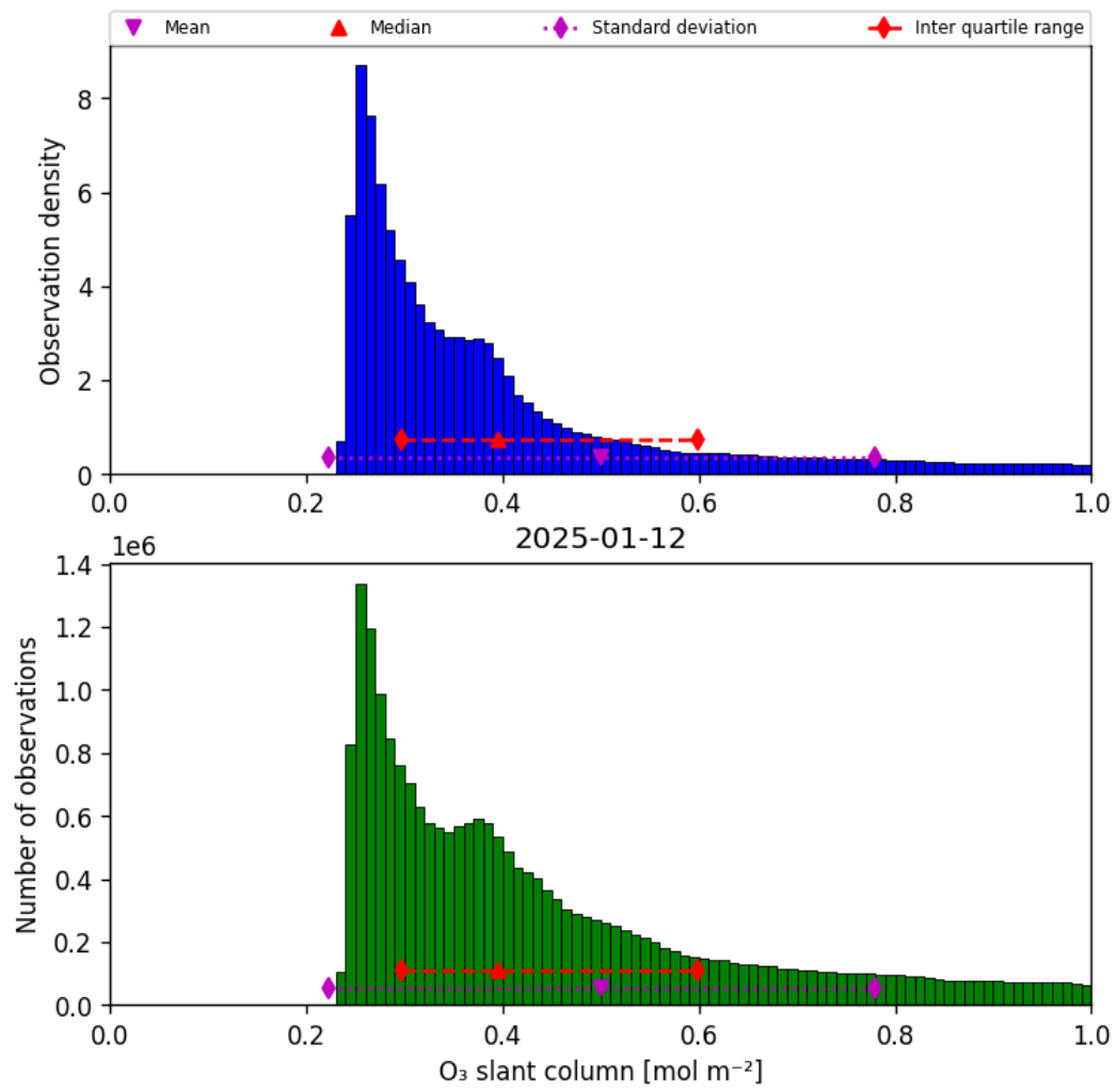
Figure 31: Histogram of “O 3 slant column” for 2025-01-12 to 2025-01-13
