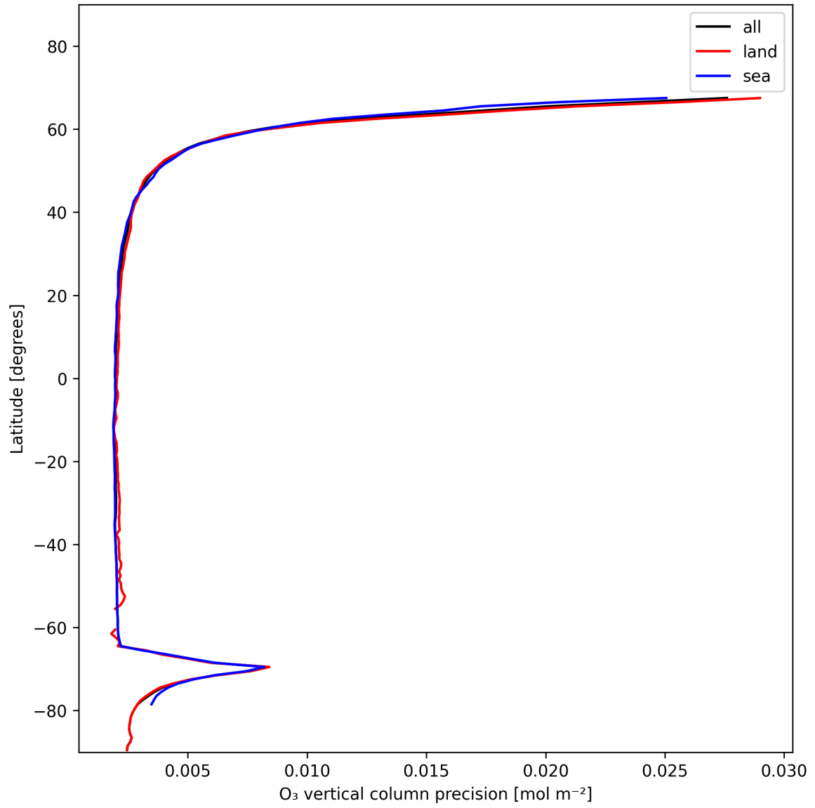
Figure 18: Zonal average of “O 3 vertical column precision” for 2025-01-12 to 2025-01-13.
