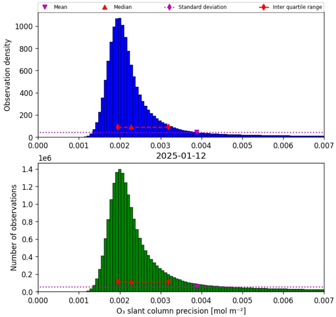
Figure 32: Histogram of “O 3 slant column precision” for 2025-01-12 to 2025-01-13
