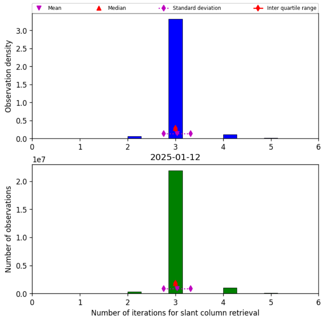
Figure 33: Histogram of “Number of iterations for slant column retrieval” for 2025-01-12 to 2025-01-13
