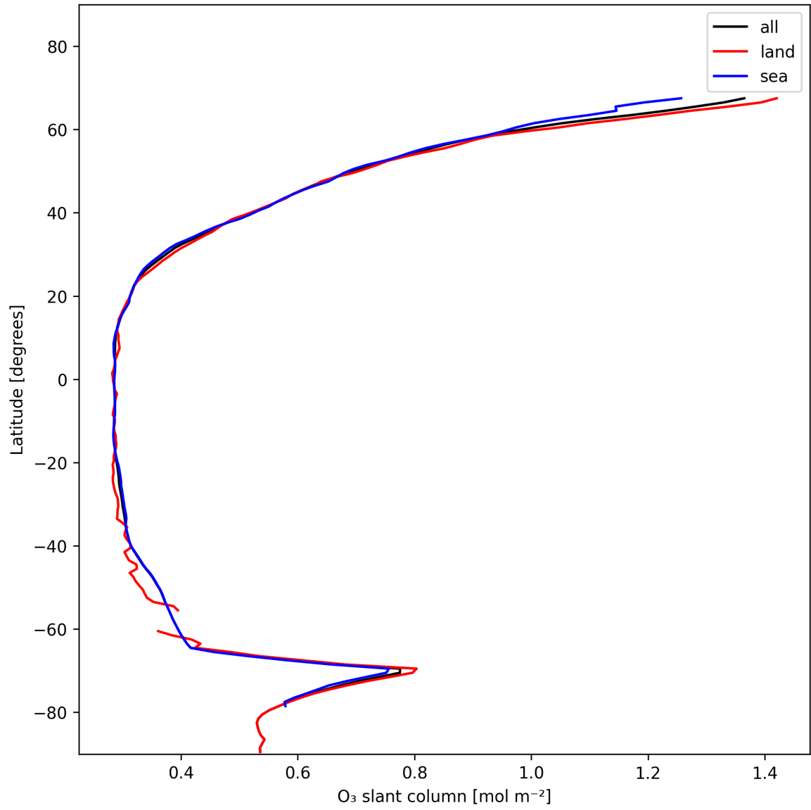
Figure 19: Zonal average of “O 3 slant column” for 2025-01-12 to 2025-01-13.
