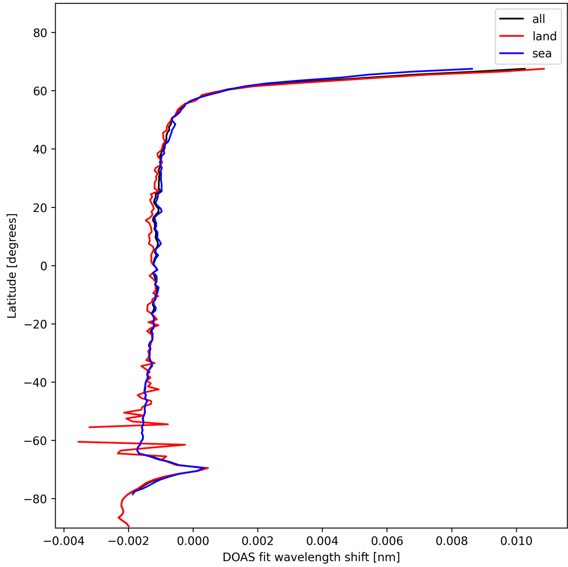
Figure 23: Zonal average of “DOAS fit wavelength shift” for 2025-01-12 to 2025-01-13.
