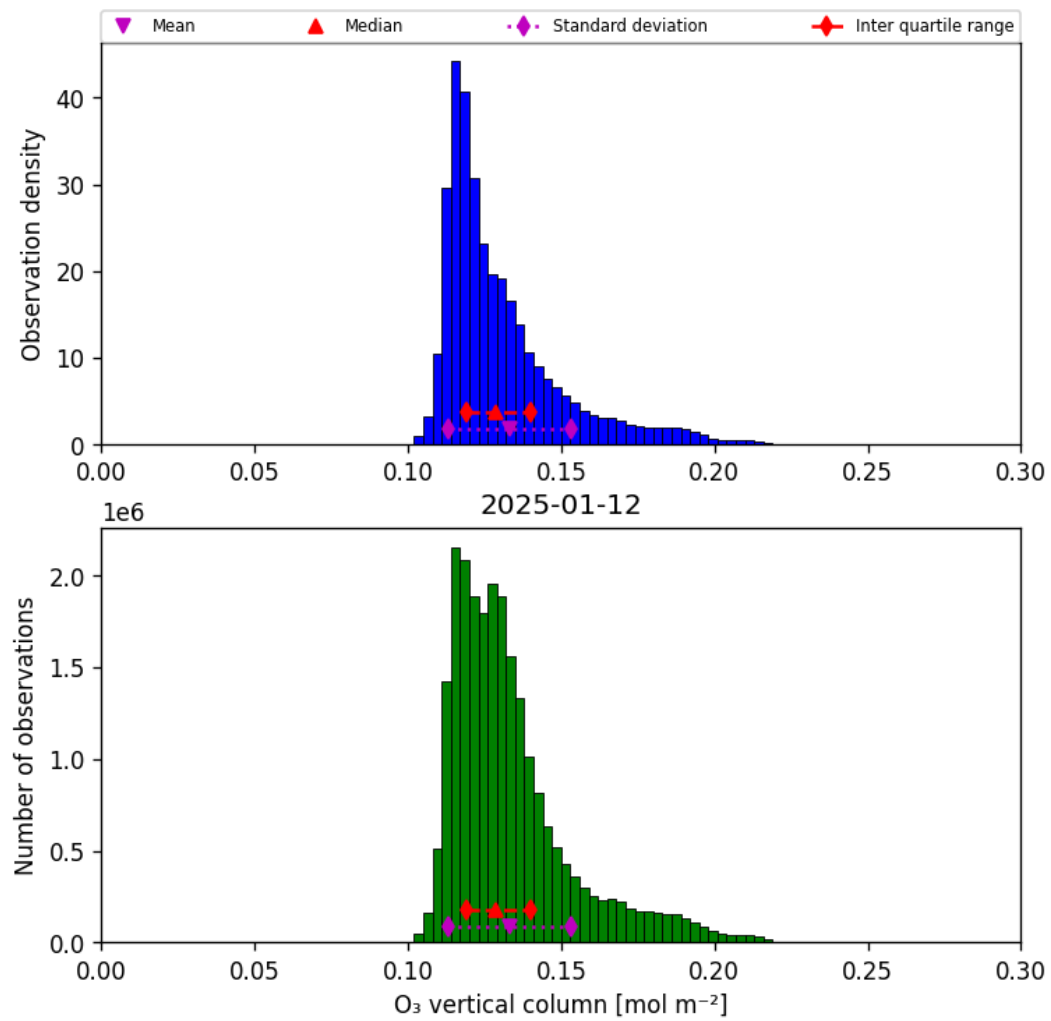
Figure 29: Histogram of “O 3 vertical column” for 2025-01-12 to 2025-01-13
