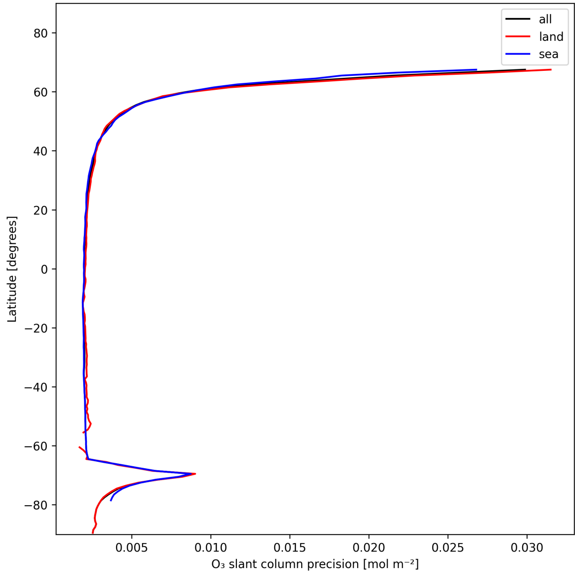
Figure 20: Zonal average of “O 3 slant column precision” for 2025-01-12 to 2025-01-13.
