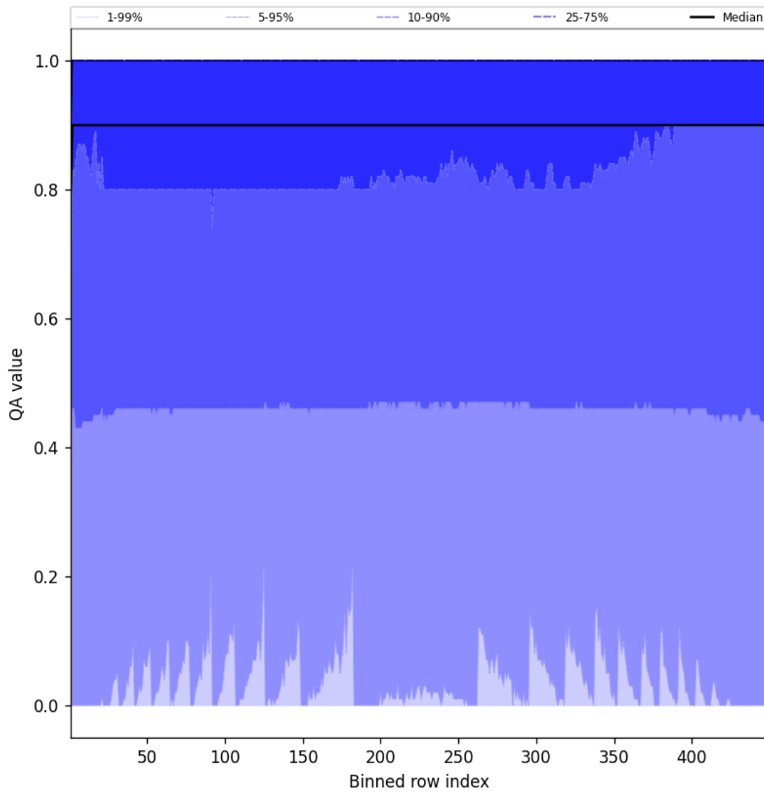
Figure 40: Along track statistics of “QA value” for 2025-01-12 to 2025-01-13
