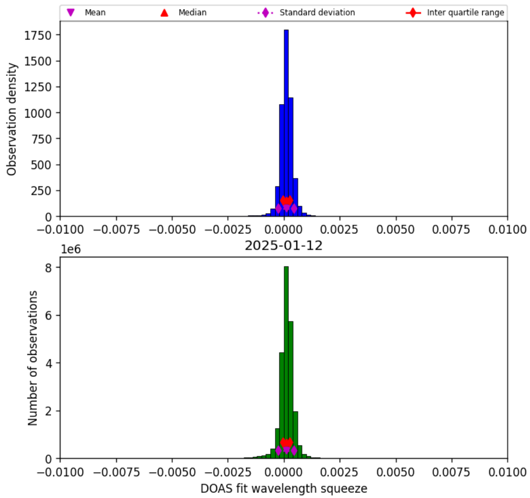
Figure 36: Histogram of “DOAS fit wavelength squeeze” for 2025-01-12 to 2025-01-13
