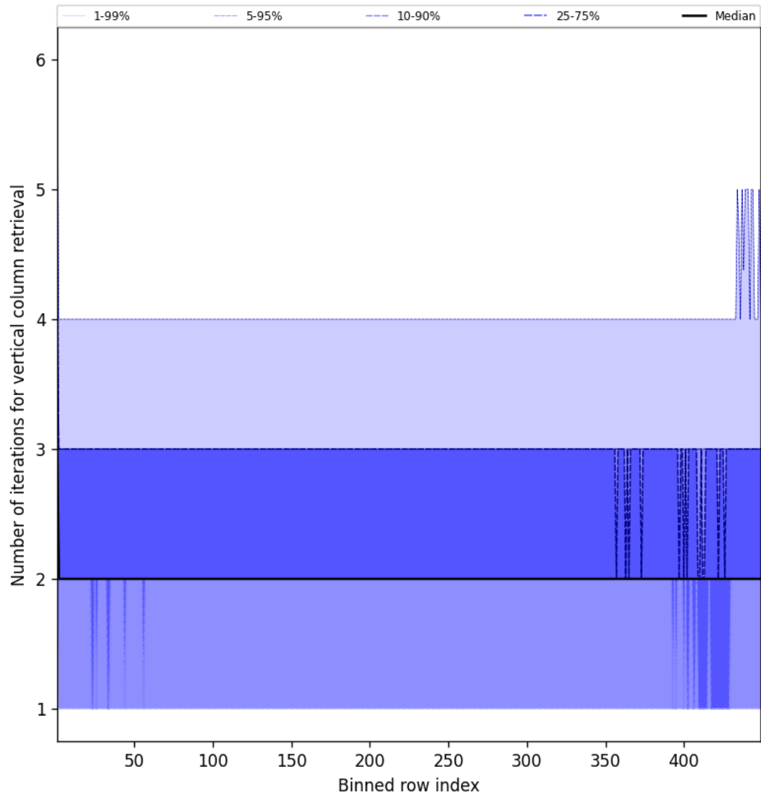
Figure 51: Along track statistics of “Number of iterations for vertical column retrieval” for 2025-01-12 to 2025-01-13
