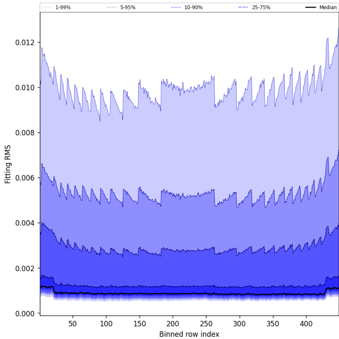
Figure 46: Along track statistics of “Fitting RMS” for 2025-01-12 to 2025-01-13
