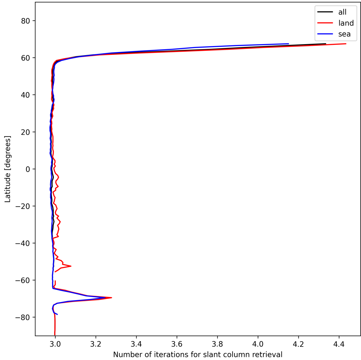
Figure 21: Zonal average of “Number of iterations for slant column retrieval” for 2025-01-12 to 2025-01-13.
