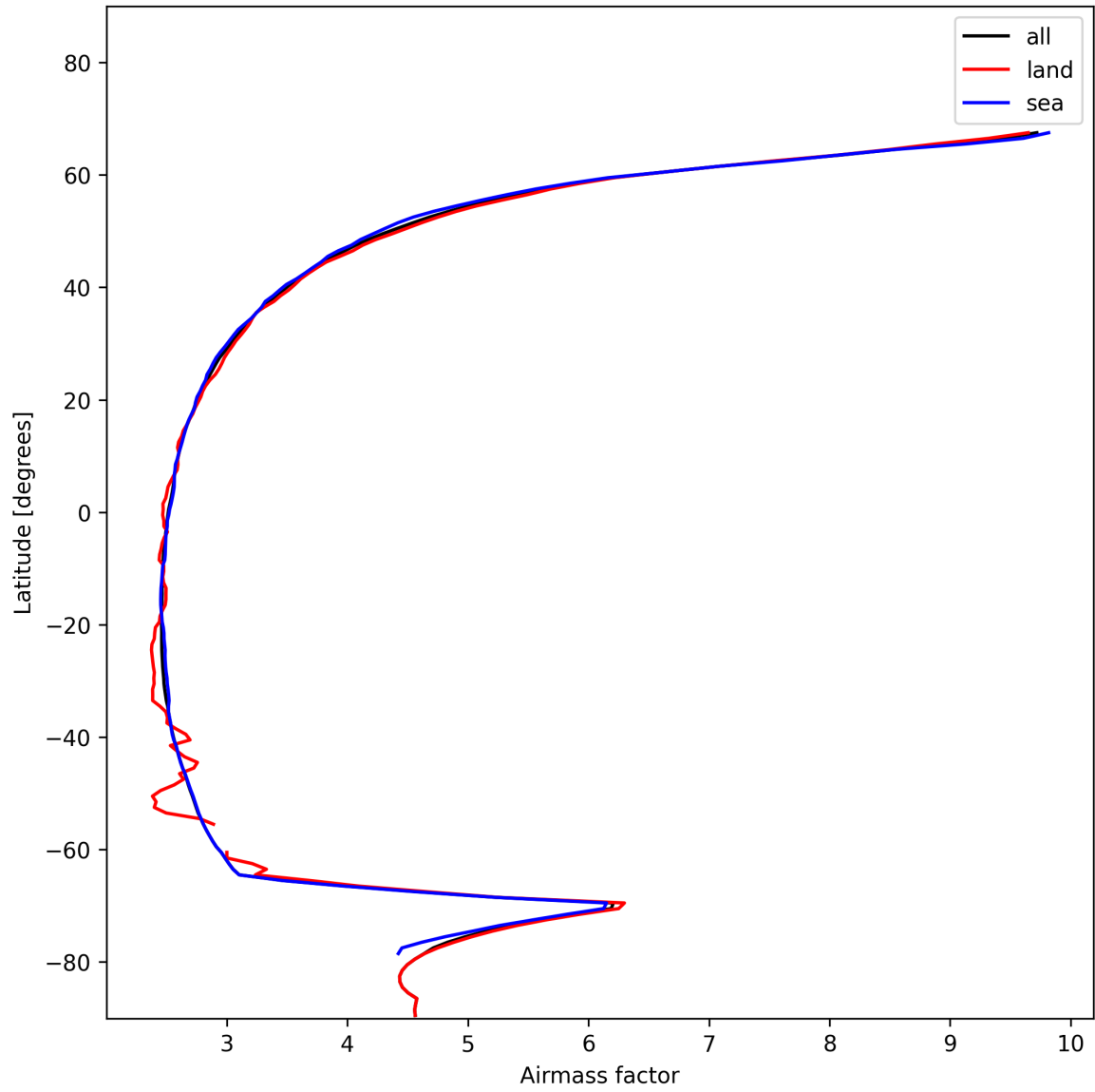
Figure 25: Zonal average of “Airmass factor” for 2025-01-12 to 2025-01-13.
