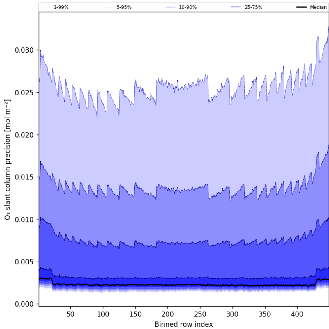
Figure 44: Along track statistics of “O 3 slant column precision” for 2025-01-12 to 2025-01-13
