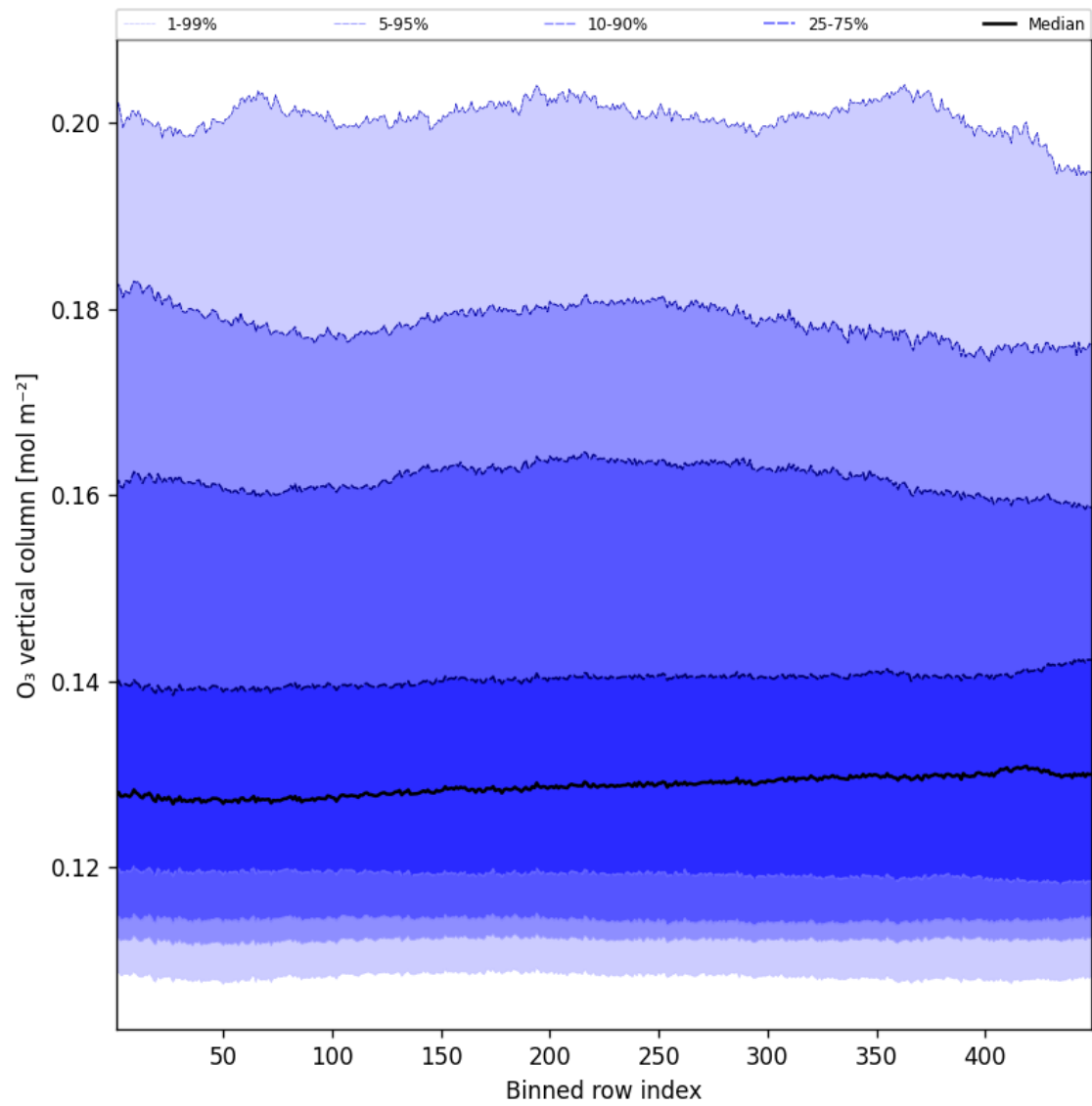
Figure 41: Along track statistics of “O 3 vertical column” for 2025-01-12 to 2025-01-13
