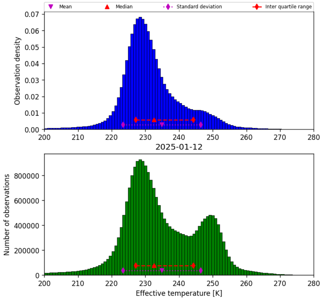
Figure 38: Histogram of “Effective temperature” for 2025-01-12 to 2025-01-13
