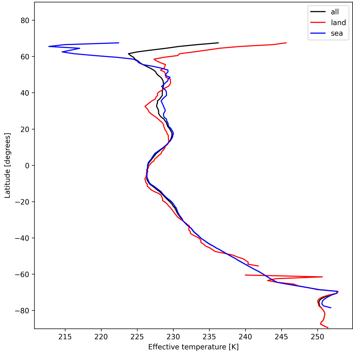
Figure 26: Zonal average of “Effective temperature” for 2025-01-12 to 2025-01-13.
