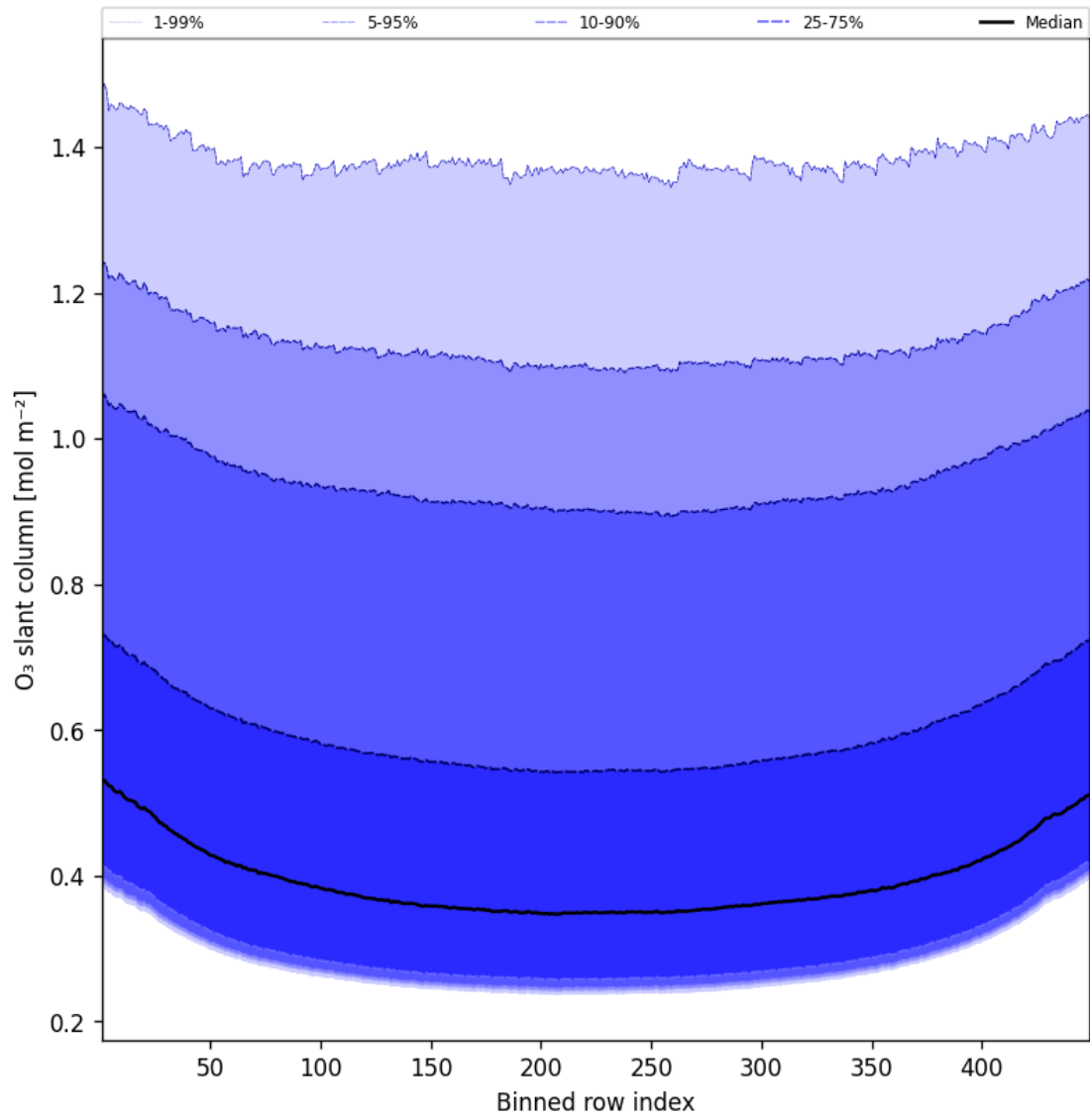
Figure 43: Along track statistics of “O 3 slant column” for 2025-01-12 to 2025-01-13
