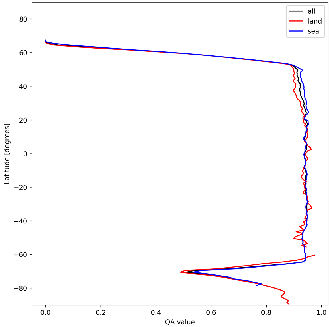
Figure 16: Zonal average of “QA value” for 2025-01-12 to 2025-01-13.
