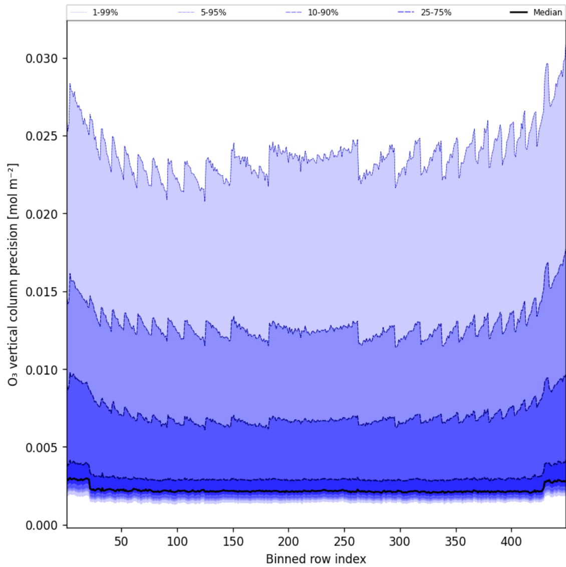
Figure 42: Along track statistics of “O 3 vertical column precision” for 2025-01-12 to 2025-01-13
