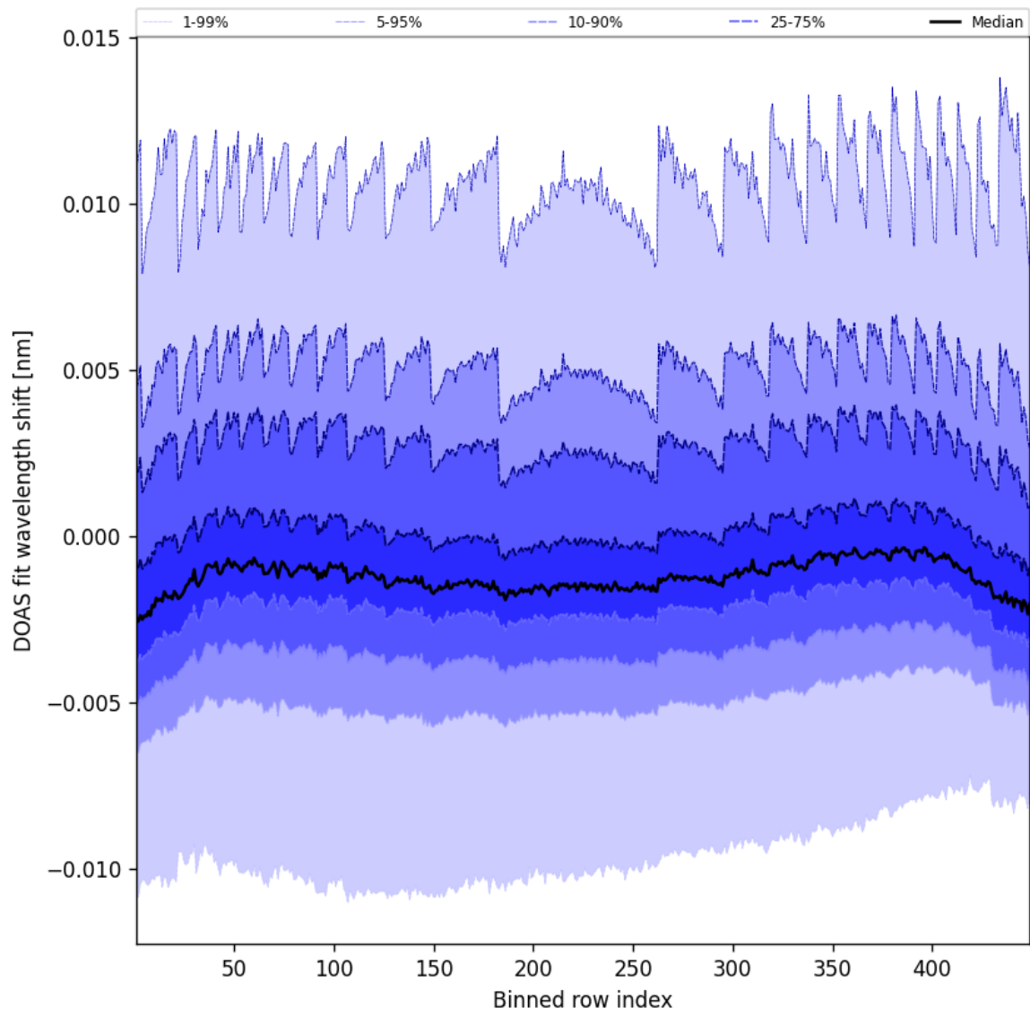
Figure 47: Along track statistics of “DOAS fit wavelength shift” for 2025-01-12 to 2025-01-13
