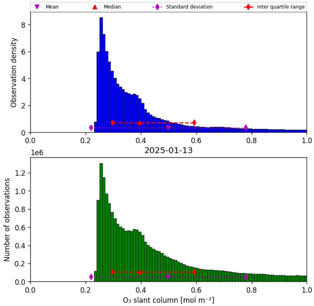
Figure 31: Histogram of “O 3 slant column” for 2025-01-13 to 2025-01-14
