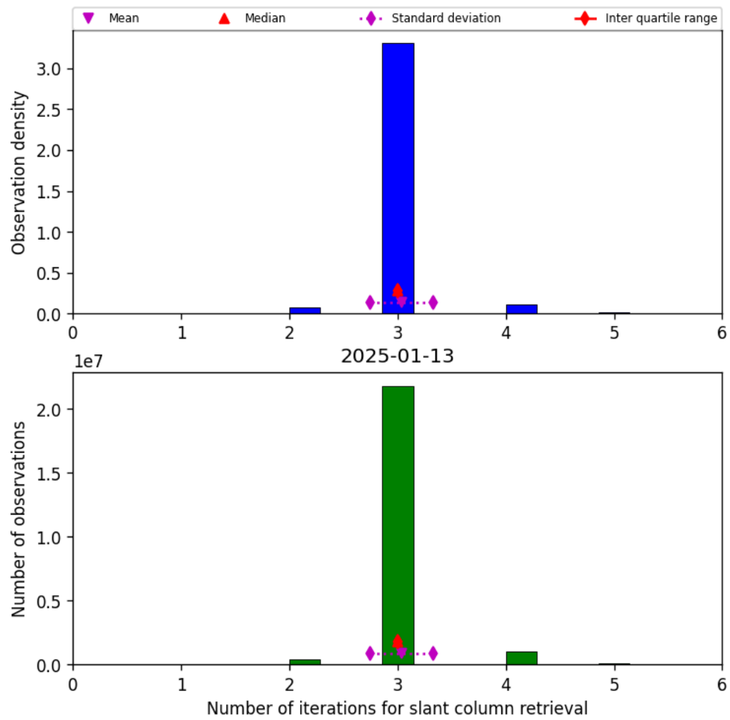
Figure 33: Histogram of “Number of iterations for slant column retrieval” for 2025-01-13 to 2025-01-14
