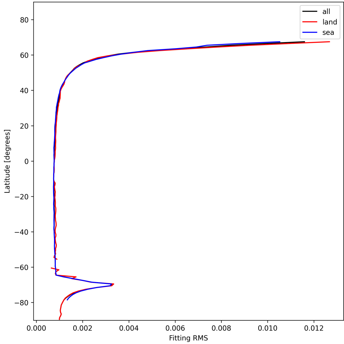
Figure 22: Zonal average of “Fitting RMS” for 2025-01-13 to 2025-01-14.
