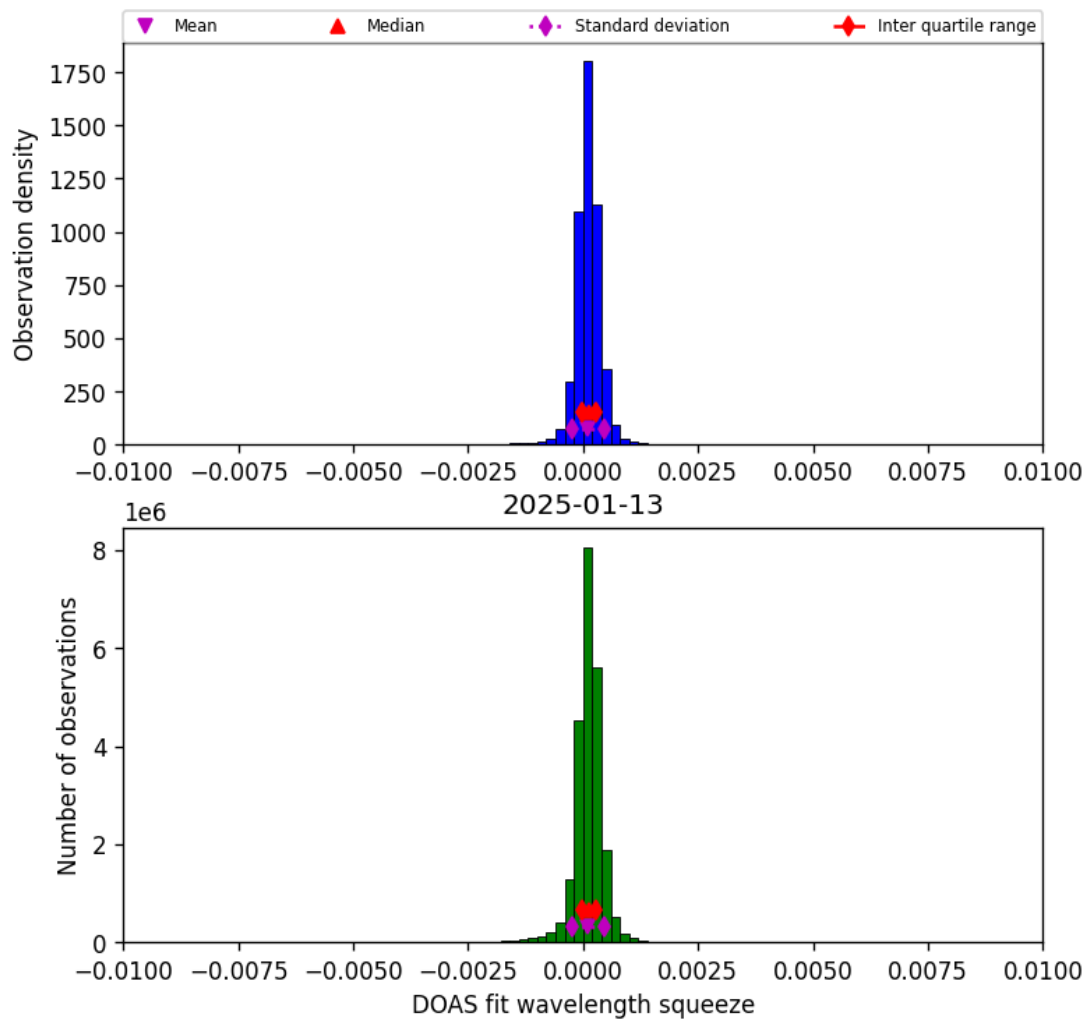
Figure 36: Histogram of “DOAS fit wavelength squeeze” for 2025-01-13 to 2025-01-14
