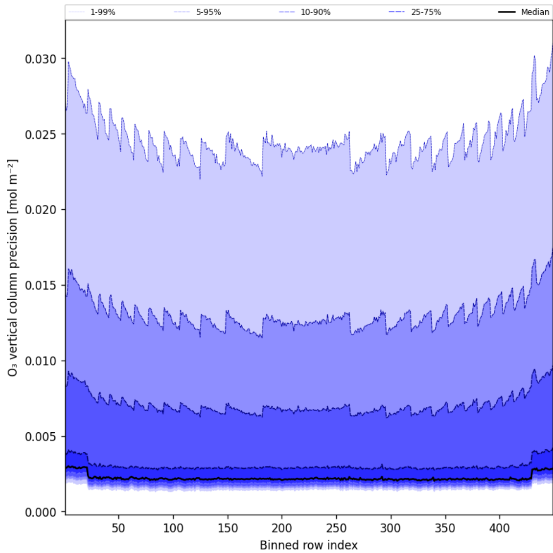
Figure 42: Along track statistics of “O 3 vertical column precision” for 2025-01-13 to 2025-01-14
