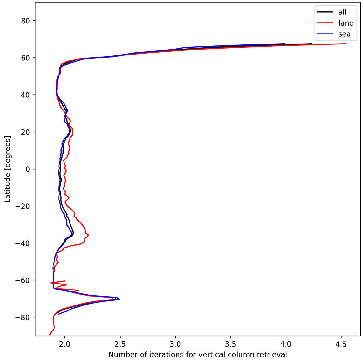
Figure 27: Zonal average of “Number of iterations for vertical column retrieval” for 2025-01-13 to 2025-01-14.
