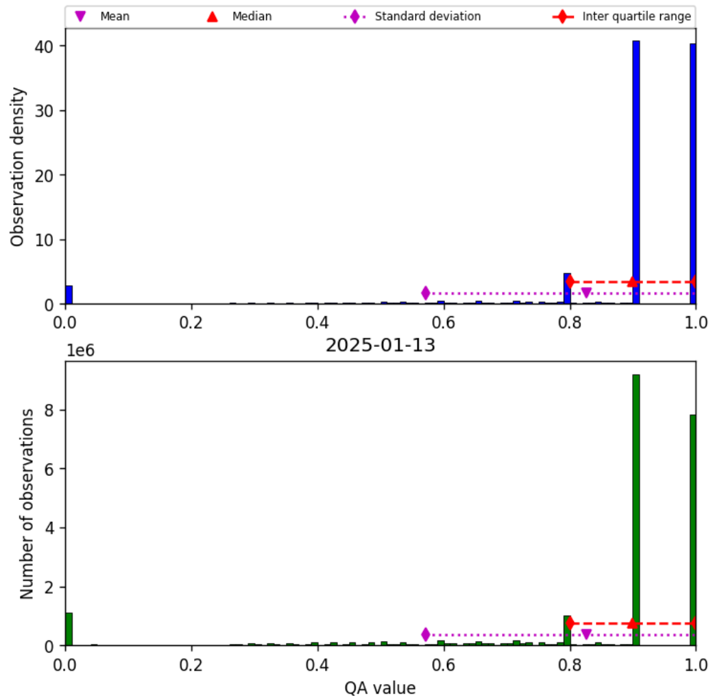
Figure 28: Histogram of “QA value” for 2025-01-13 to 2025-01-14
