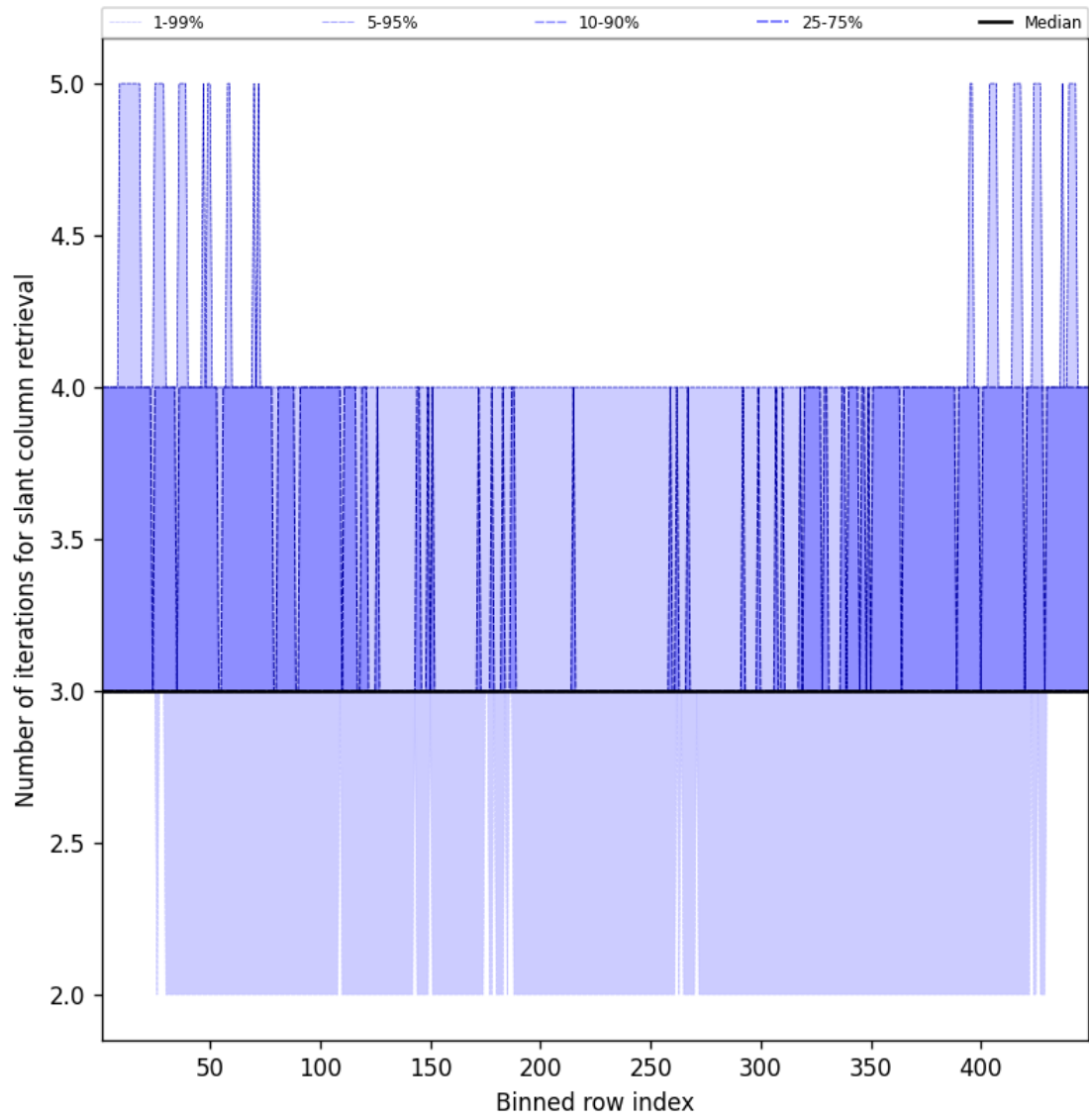
Figure 45: Along track statistics of “Number of iterations for slant column retrieval” for 2025-01-13 to 2025-01-14
