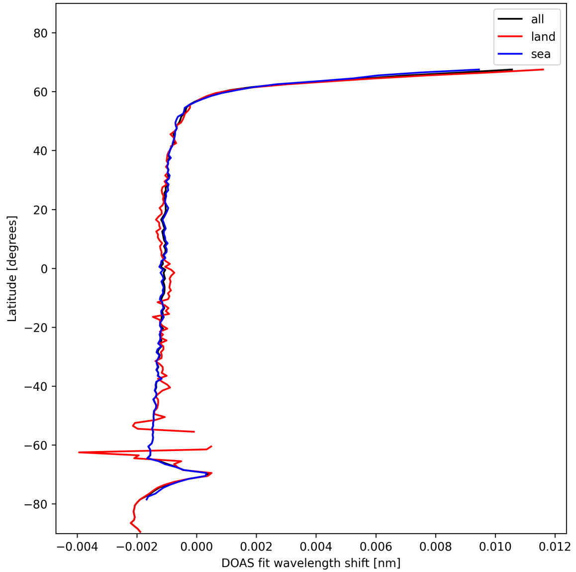
Figure 23: Zonal average of “DOAS fit wavelength shift” for 2025-01-13 to 2025-01-14.
