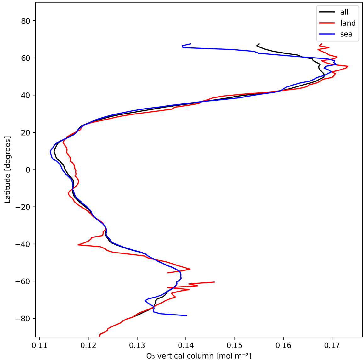
Figure 17: Zonal average of “O 3 vertical column” for 2025-01-13 to 2025-01-14.
