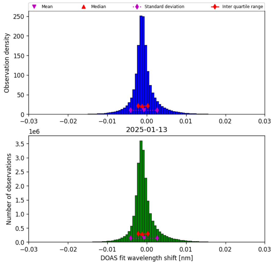
Figure 35: Histogram of “DOAS fit wavelength shift” for 2025-01-13 to 2025-01-14
