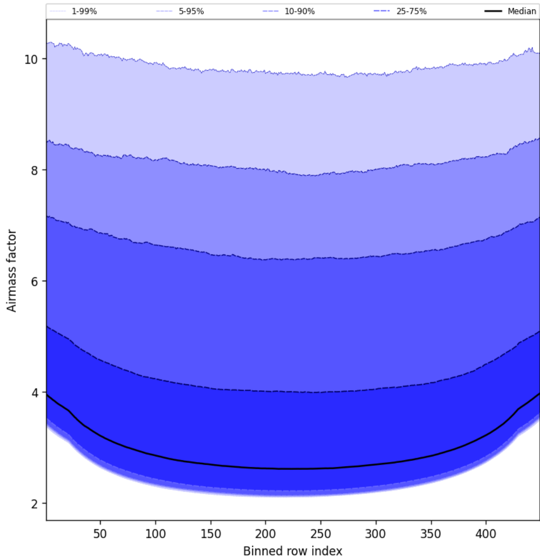
Figure 49: Along track statistics of “Airmass factor” for 2025-01-13 to 2025-01-14
