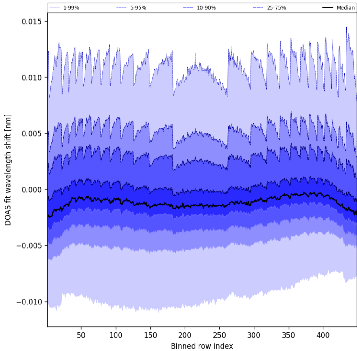
Figure 47: Along track statistics of “DOAS fit wavelength shift” for 2025-01-13 to 2025-01-14
