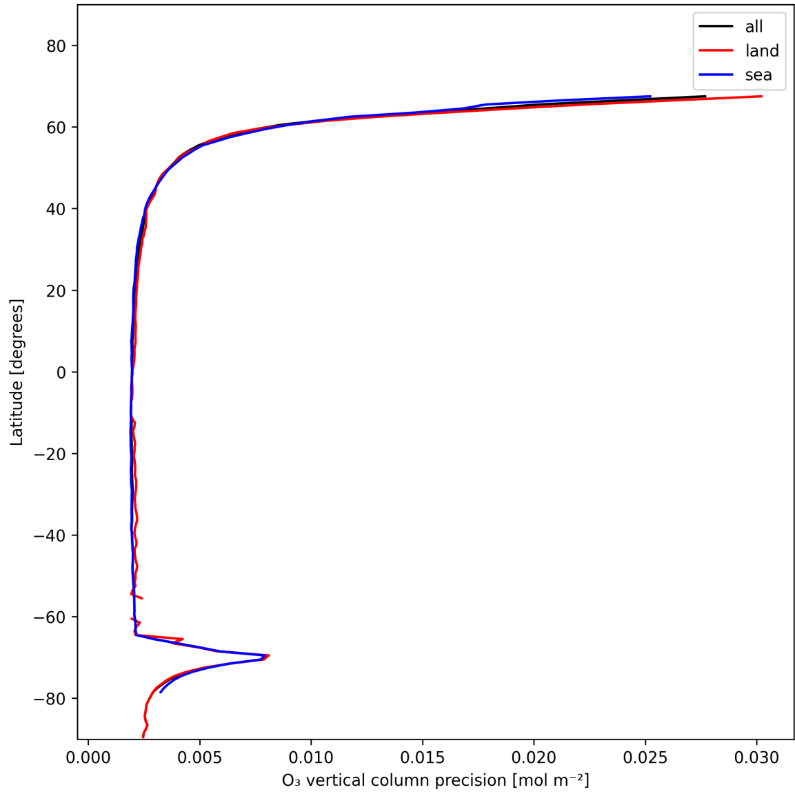
Figure 18: Zonal average of “O 3 vertical column precision” for 2025-01-13 to 2025-01-14.
