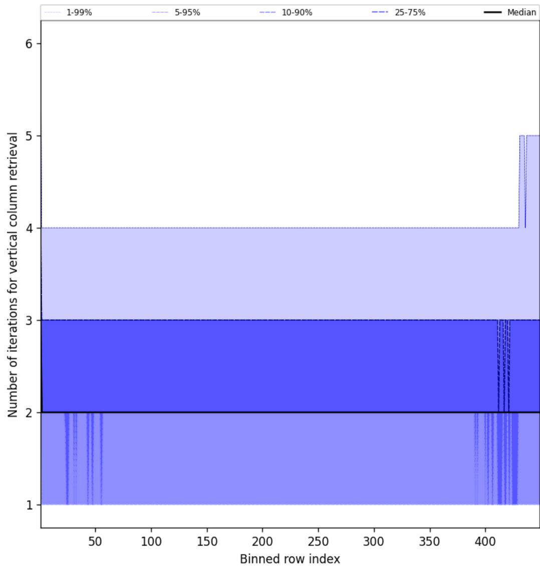
Figure 51: Along track statistics of “Number of iterations for vertical column retrieval” for 2025-01-13 to 2025-01-14
