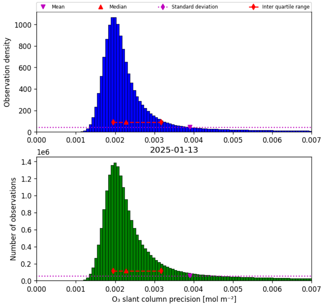
Figure 32: Histogram of “O 3 slant column precision” for 2025-01-13 to 2025-01-14
