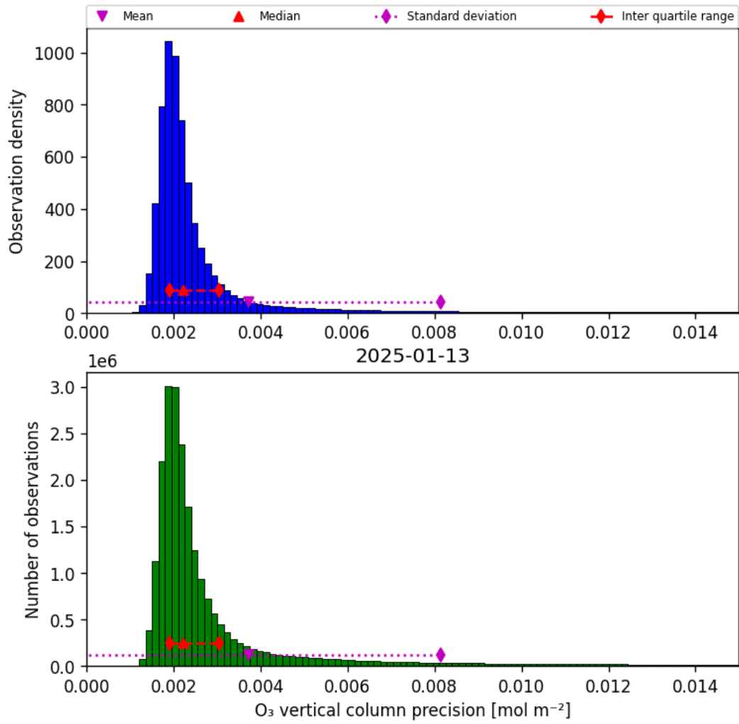
Figure 30: Histogram of “O 3 vertical column precision” for 2025-01-13 to 2025-01-14
