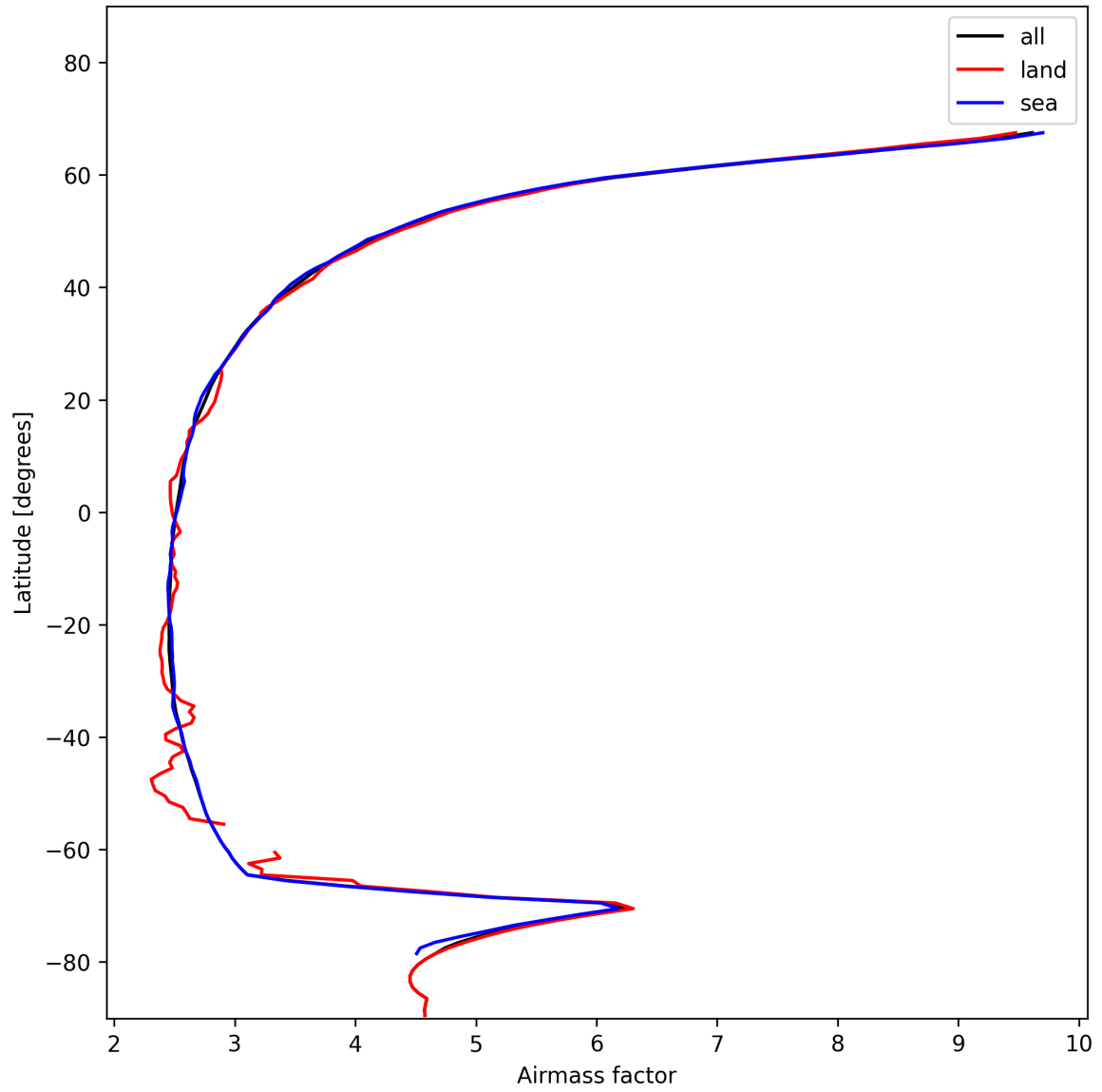
Figure 25: Zonal average of “Airmass factor” for 2025-01-13 to 2025-01-14.
