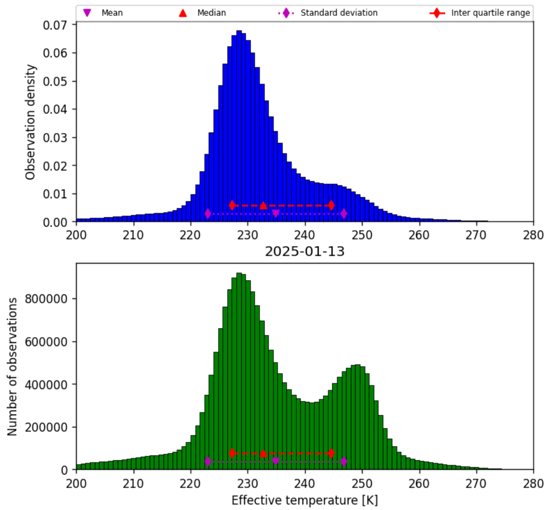
Figure 38: Histogram of “Effective temperature” for 2025-01-13 to 2025-01-14
