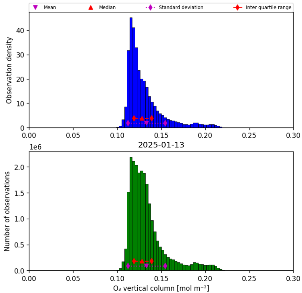
Figure 29: Histogram of “O 3 vertical column” for 2025-01-13 to 2025-01-14
