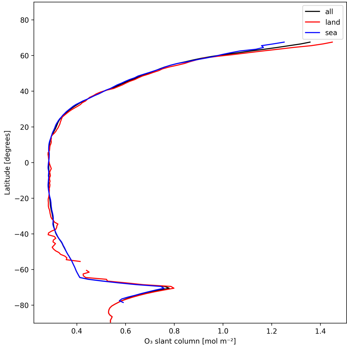
Figure 19: Zonal average of “O 3 slant column” for 2025-01-13 to 2025-01-14.
