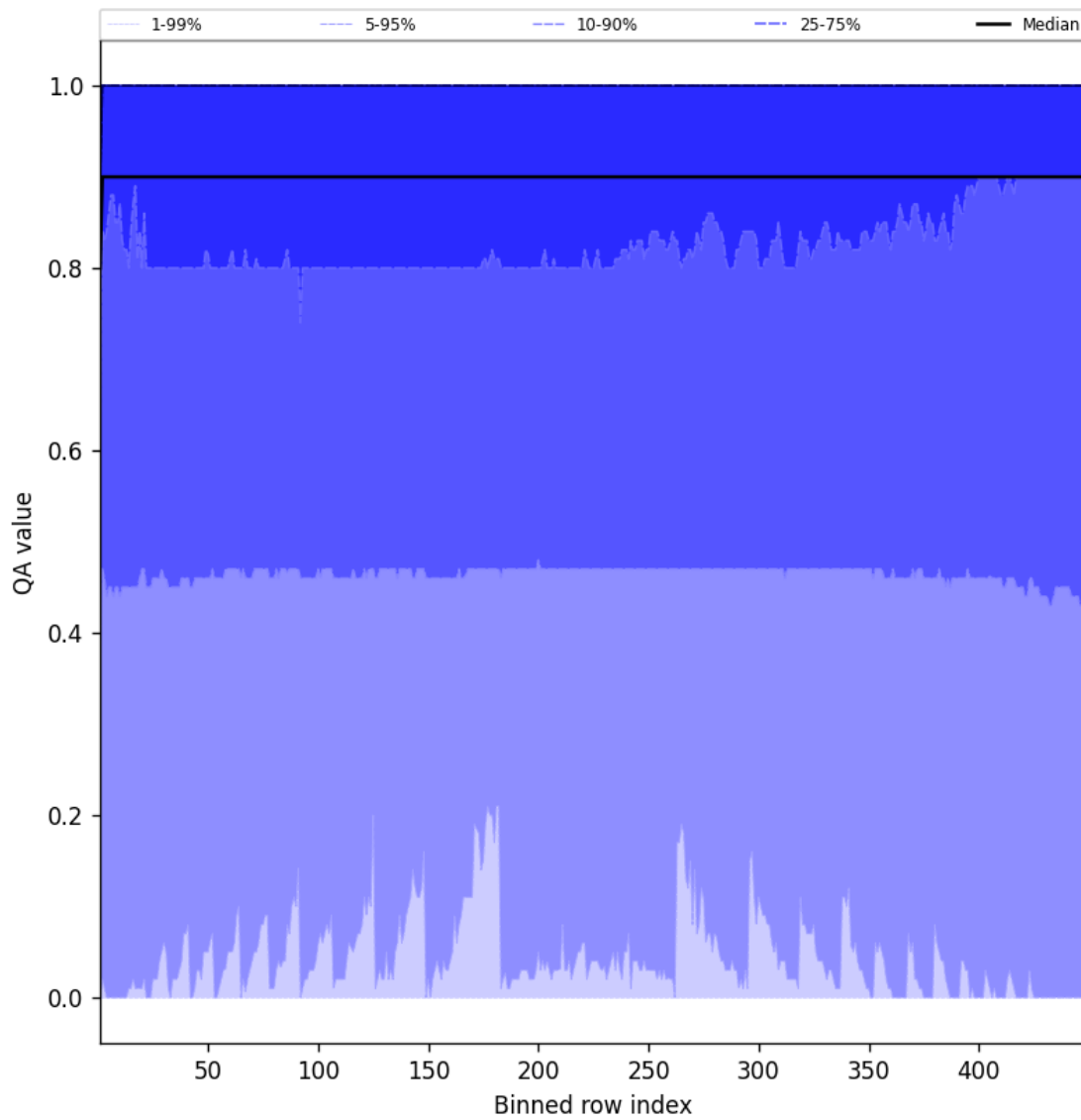
Figure 40: Along track statistics of “QA value” for 2025-01-13 to 2025-01-14
