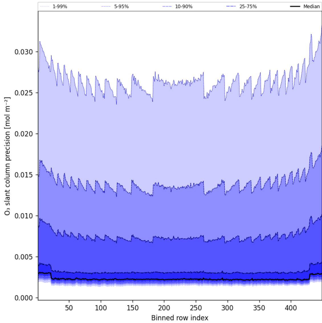
Figure 44: Along track statistics of “O 3 slant column precision” for 2025-01-13 to 2025-01-14
