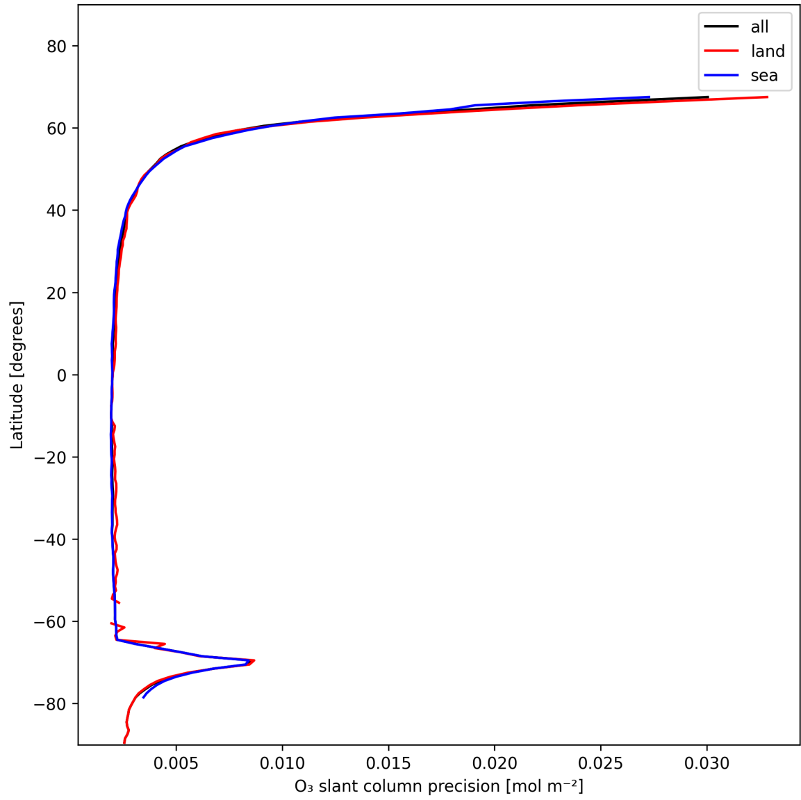
Figure 20: Zonal average of “O 3 slant column precision” for 2025-01-13 to 2025-01-14.
