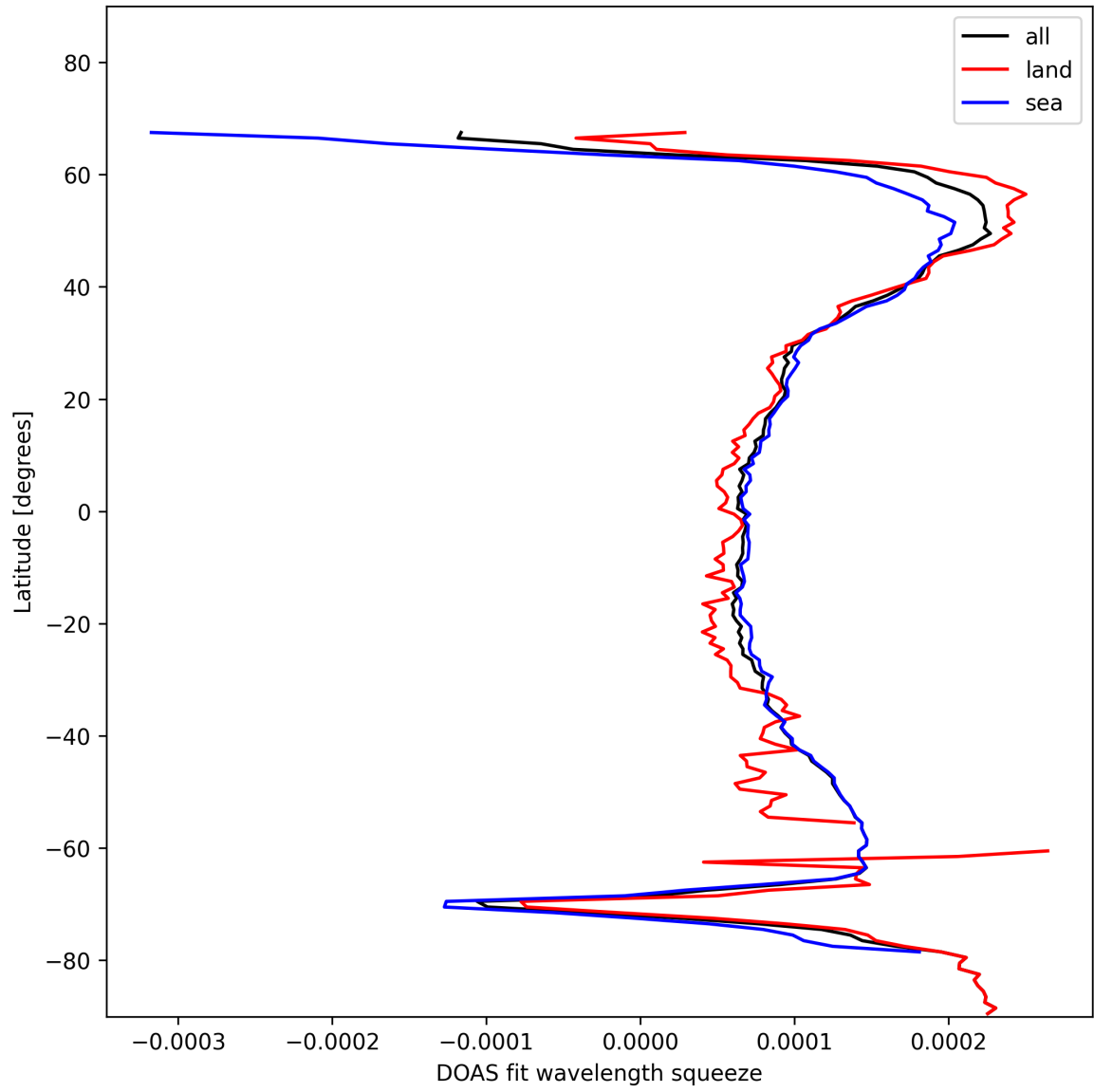
Figure 24: Zonal average of “DOAS fit wavelength squeeze” for 2025-01-13 to 2025-01-14.
