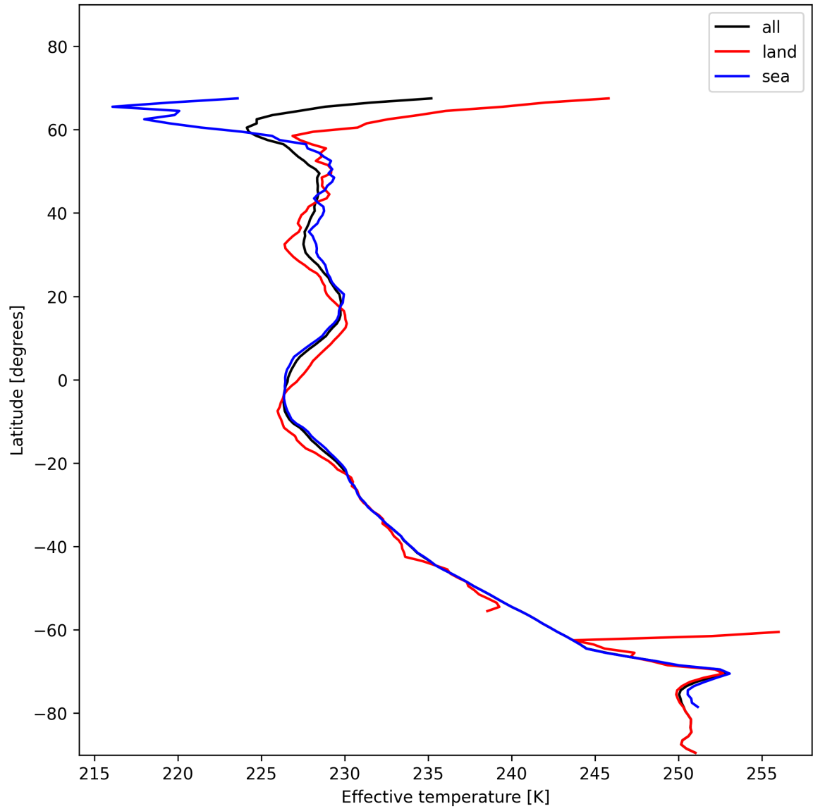
Figure 26: Zonal average of “Effective temperature” for 2025-01-13 to 2025-01-14.
