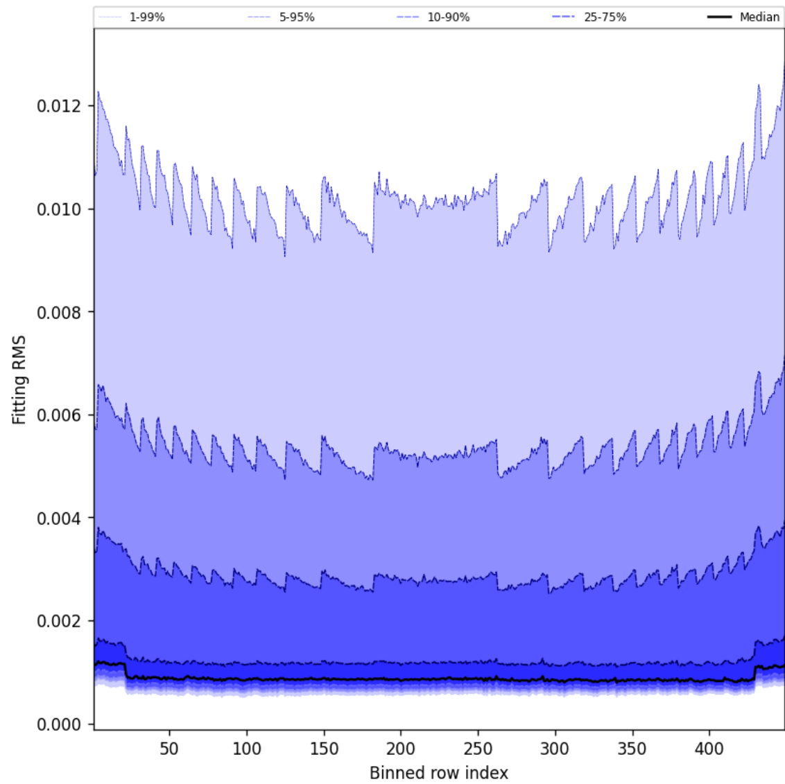
Figure 46: Along track statistics of “Fitting RMS” for 2025-01-13 to 2025-01-14
