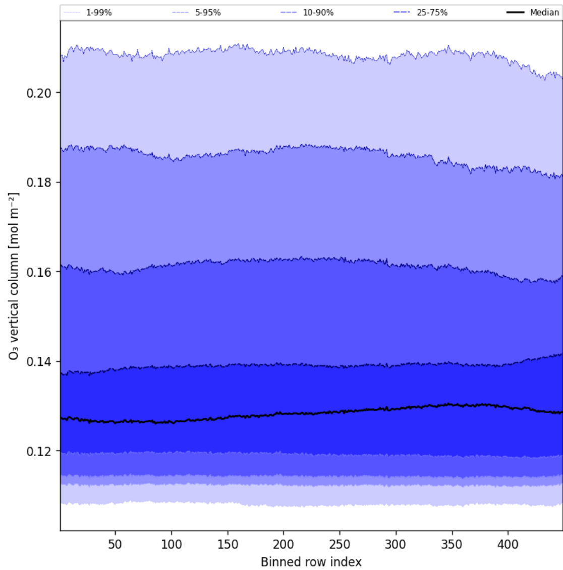
Figure 41: Along track statistics of “ O_3 vertical column” for 2025-01-13 to 2025-01-14
