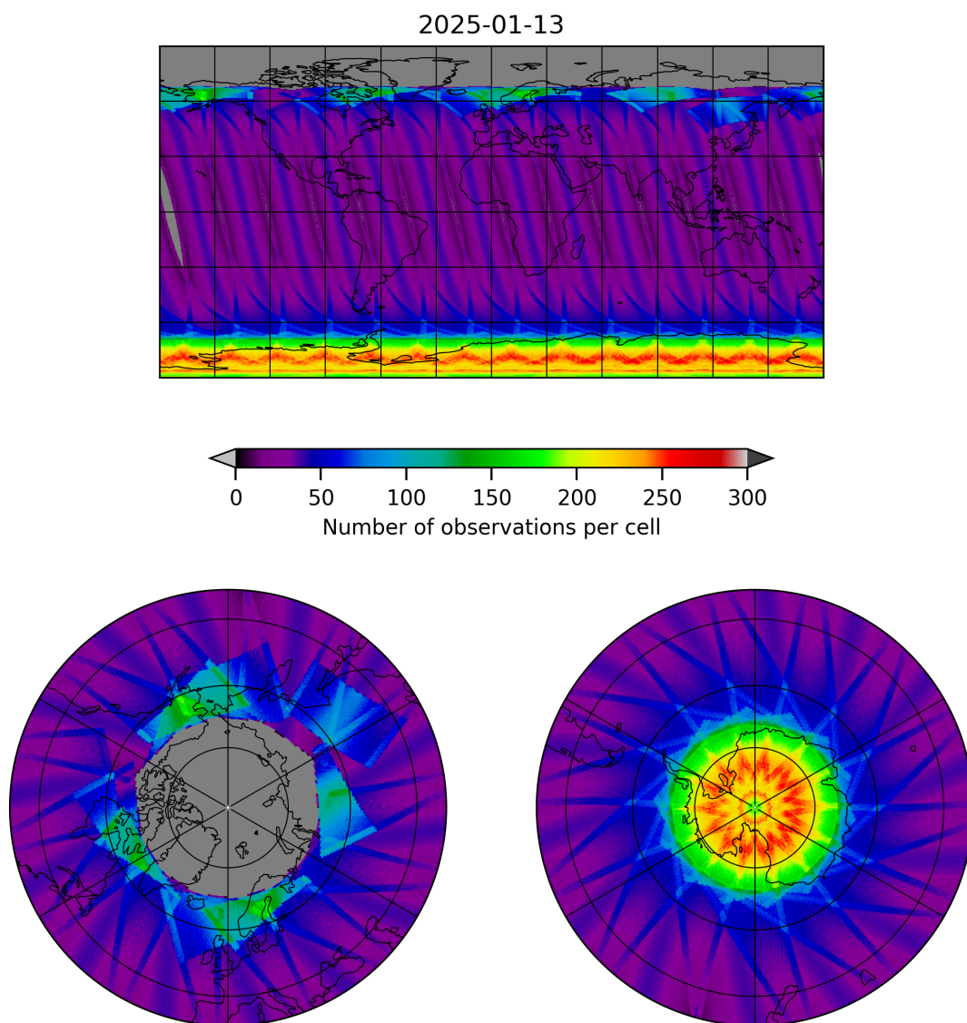
Figure 15: Map of the number of observations for 2025-01-13 to 2025-01-14
