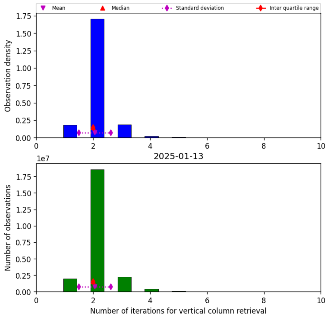
Figure 39: Histogram of “Number of iterations for vertical column retrieval” for 2025-01-13 to 2025-01-14
