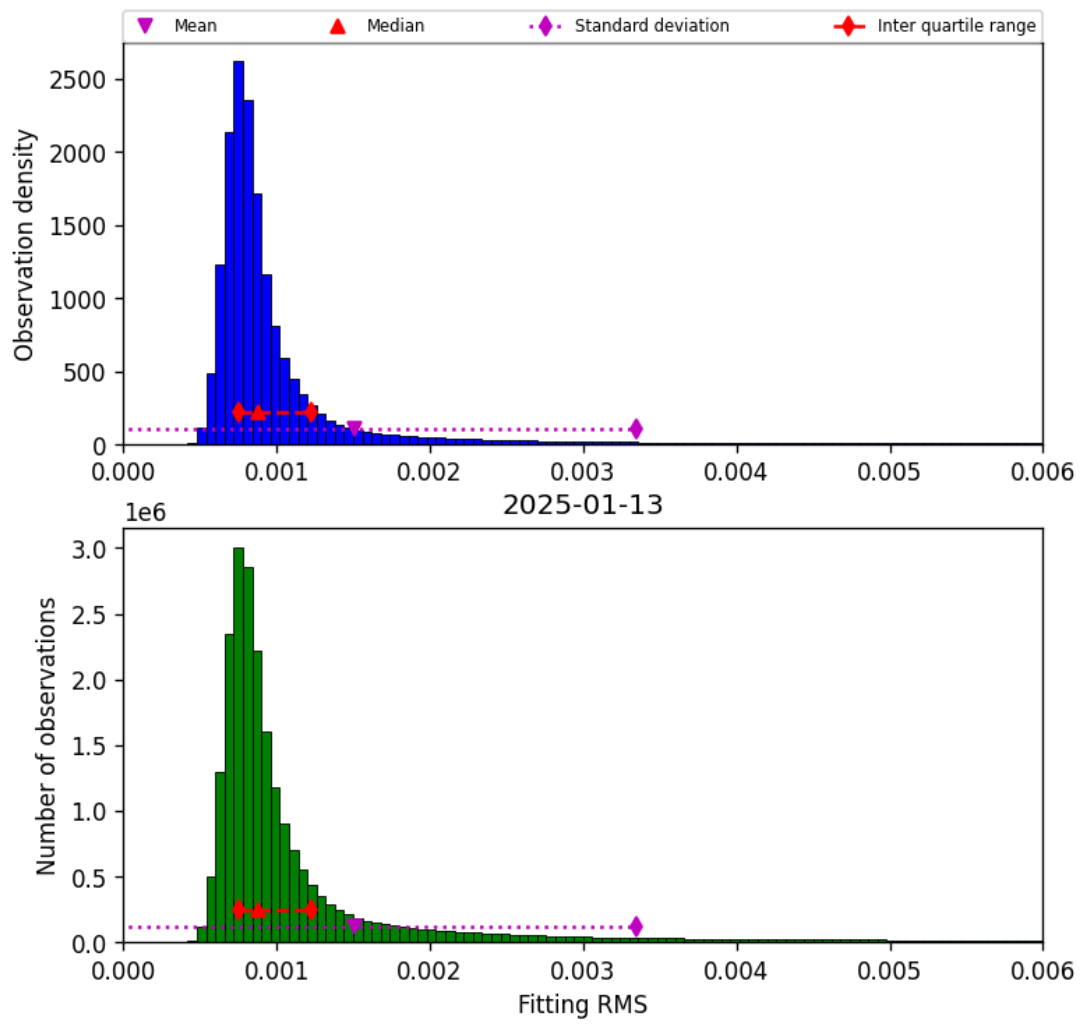
Figure 34: Histogram of “Fitting RMS” for 2025-01-13 to 2025-01-14
