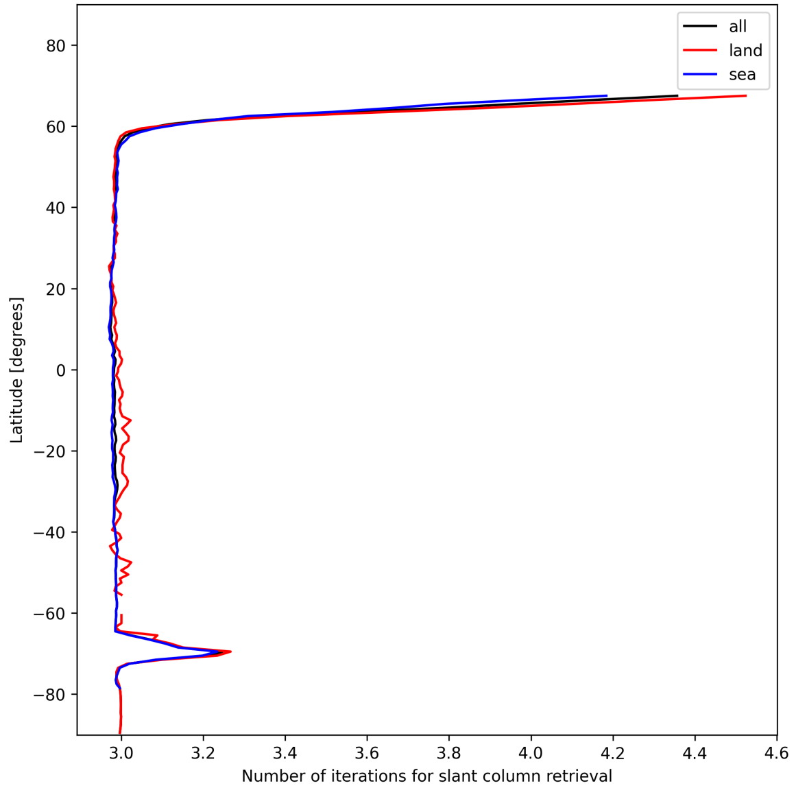
Figure 21: Zonal average of “Number of iterations for slant column retrieval” for 2025-01-13 to 2025-01-14.
