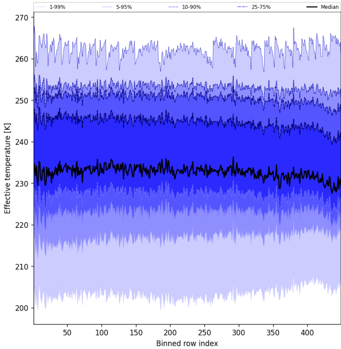
Figure 50: Along track statistics of “Effective temperature” for 2025-01-13 to 2025-01-14
