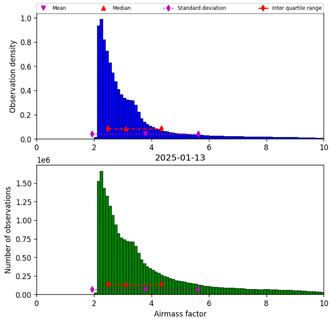
Figure 37: Histogram of “Airmass factor” for 2025-01-13 to 2025-01-14
