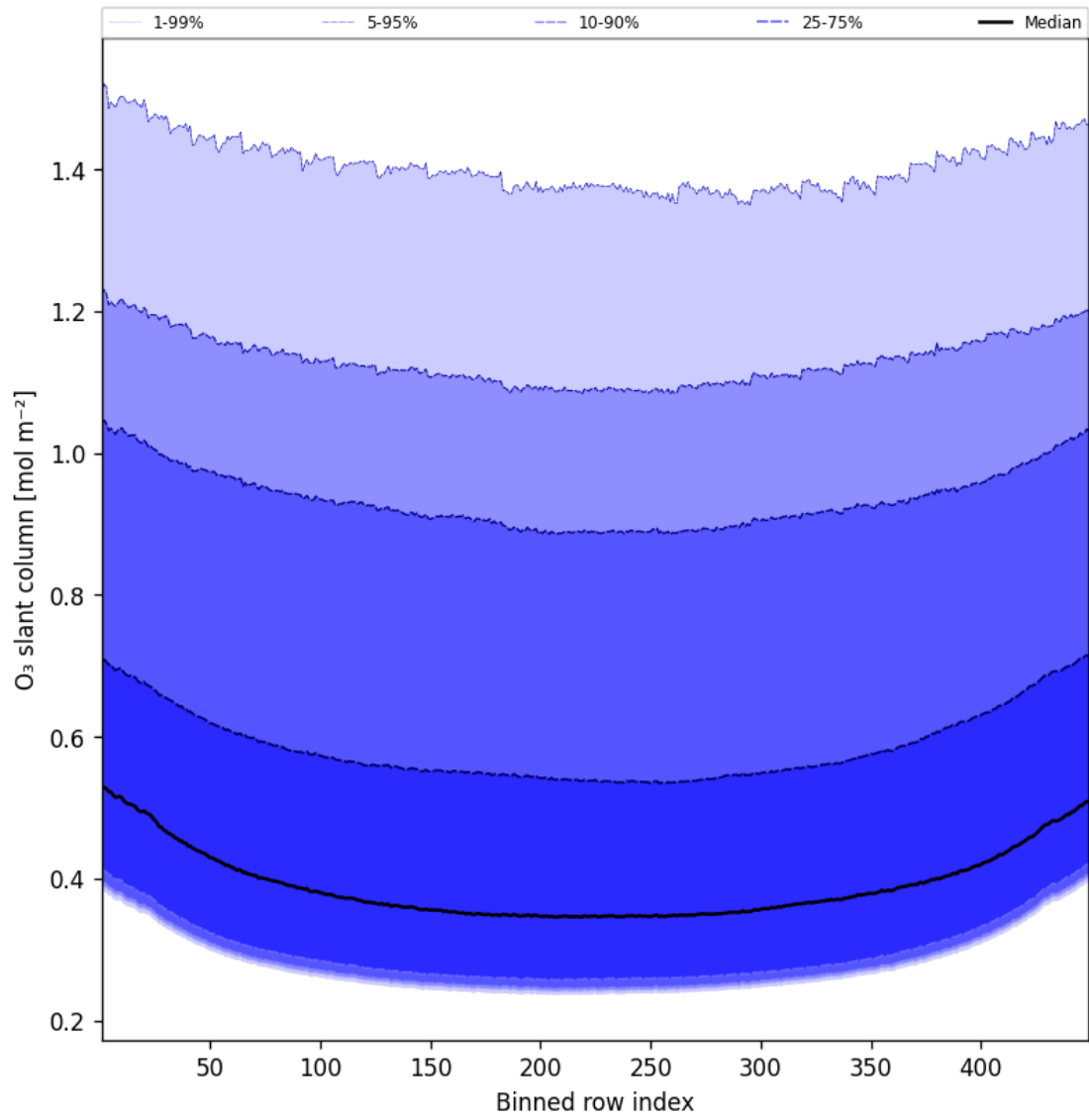
Figure 43: Along track statistics of “O 3 slant column” for 2025-01-13 to 2025-01-14
