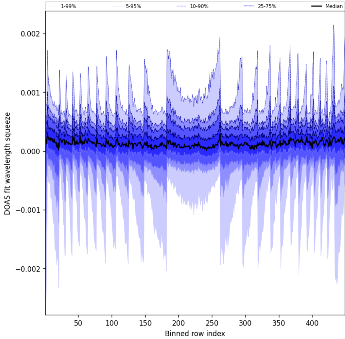
Figure 48: Along track statistics of “DOAS fit wavelength squeeze” for 2025-01-13 to 2025-01-14
