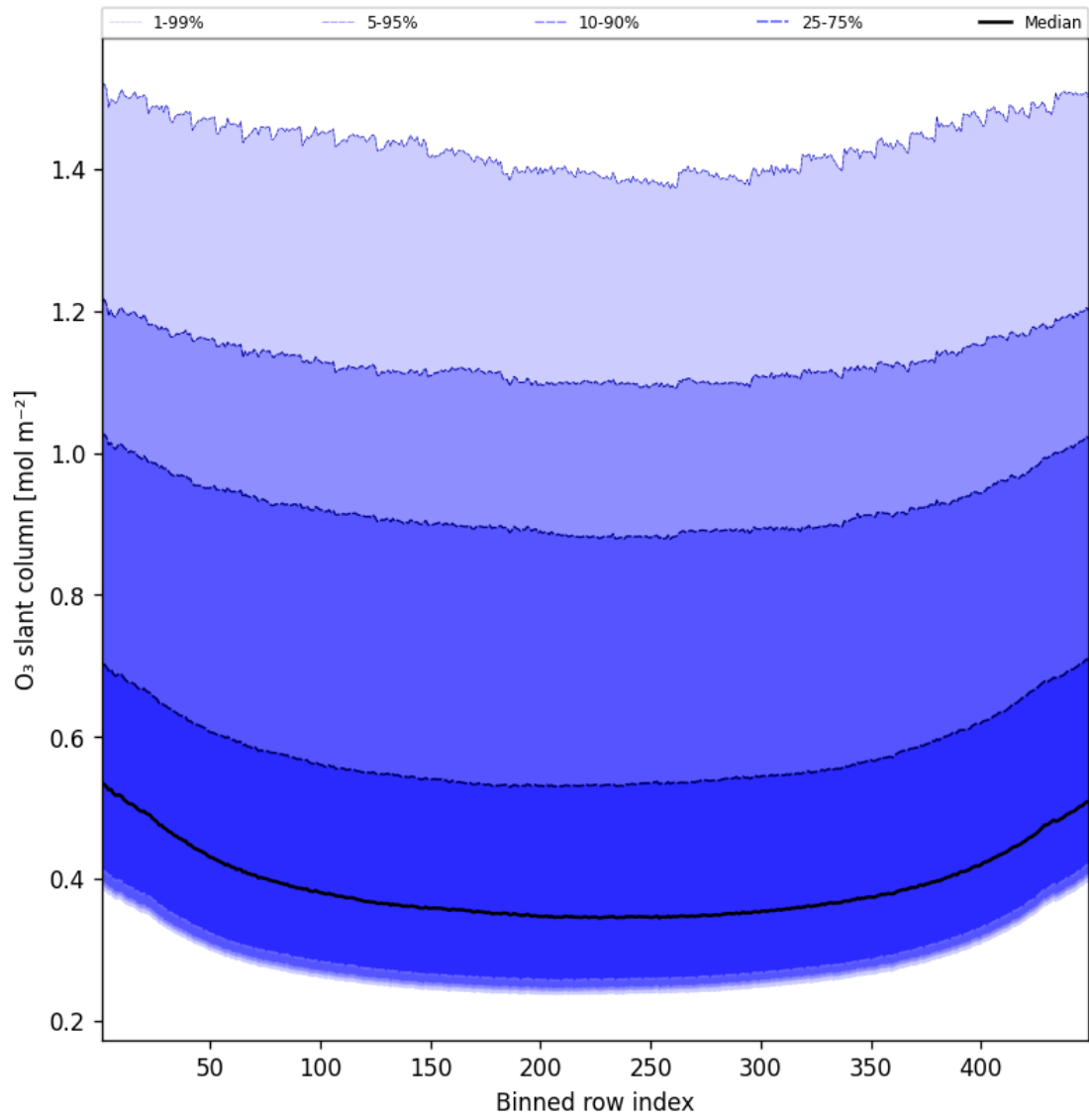
Figure 43: Along track statistics of “O 3 slant column” for 2025-01-14 to 2025-01-15
