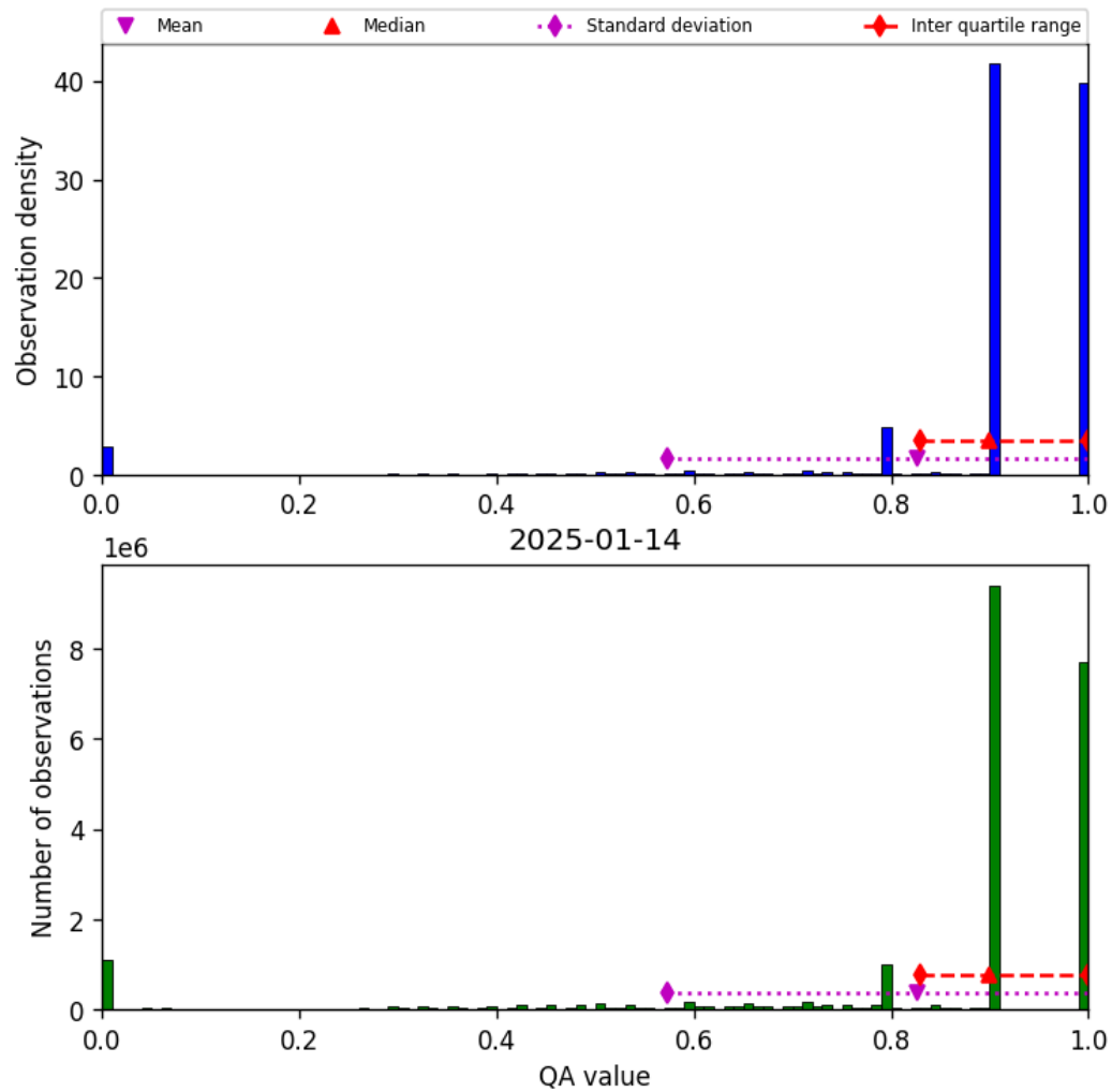
Figure 28: Histogram of “QA value” for 2025-01-14 to 2025-01-15
