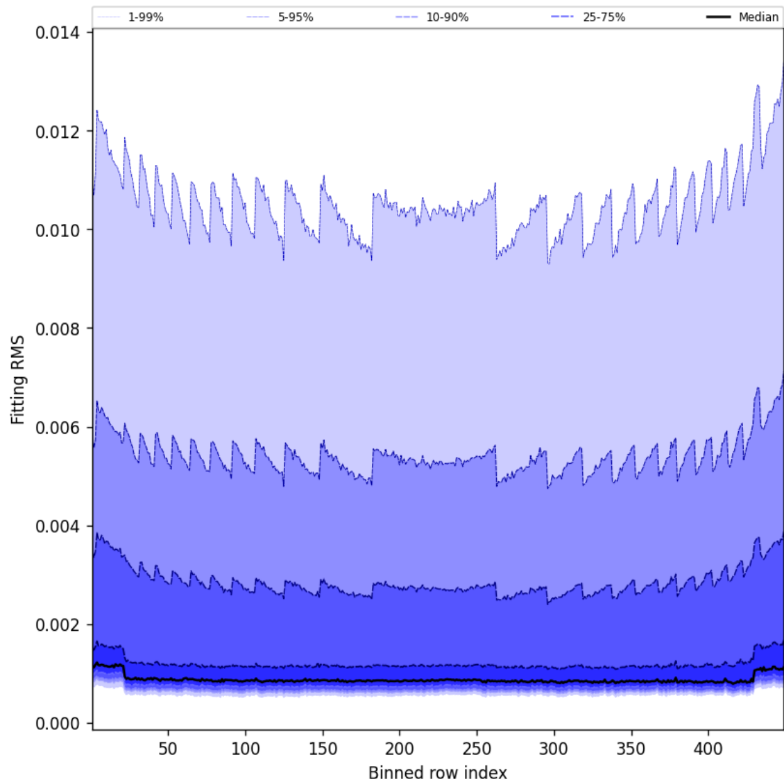
Figure 46: Along track statistics of “Fitting RMS” for 2025-01-14 to 2025-01-15
