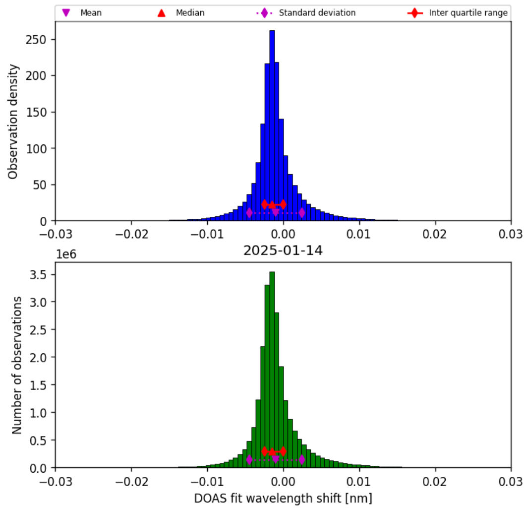
Figure 35: Histogram of “DOAS fit wavelength shift” for 2025-01-14 to 2025-01-15
