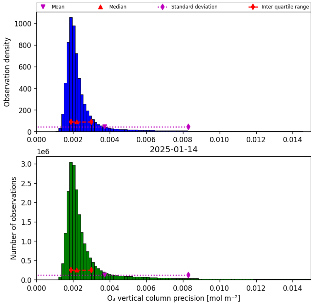
Figure 30: Histogram of “O 3 vertical column precision” for 2025-01-14 to 2025-01-15
