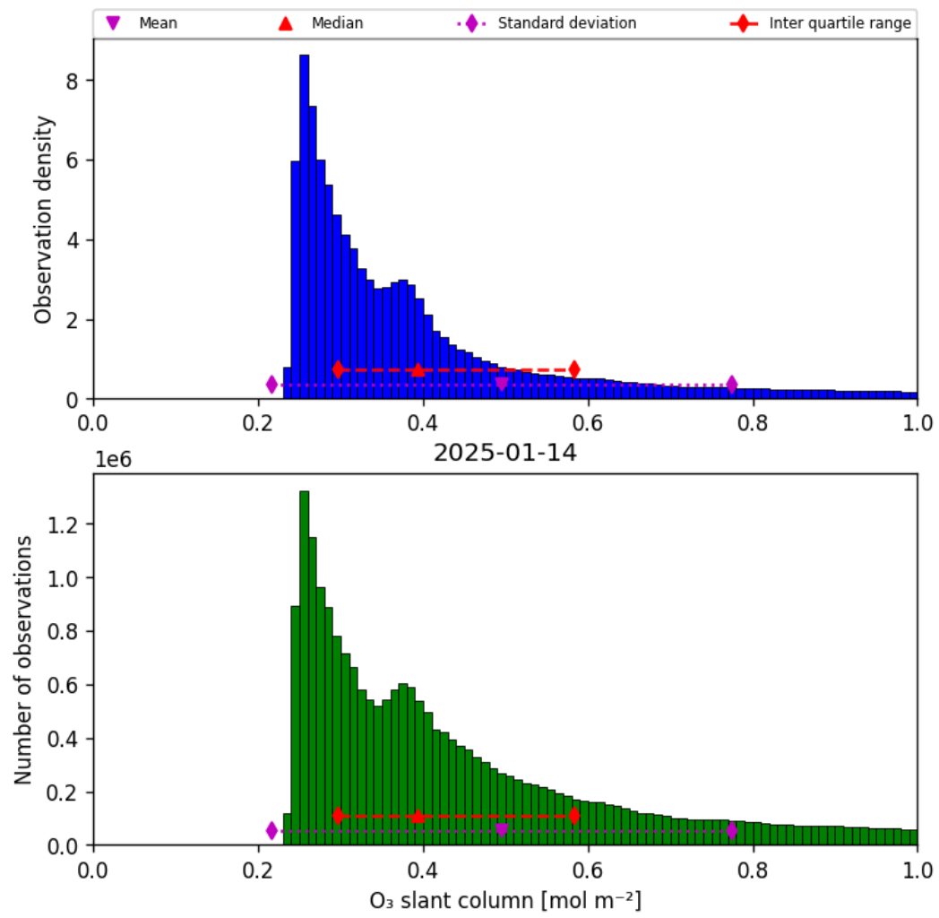
Figure 31: Histogram of “O 3 slant column” for 2025-01-14 to 2025-01-15
