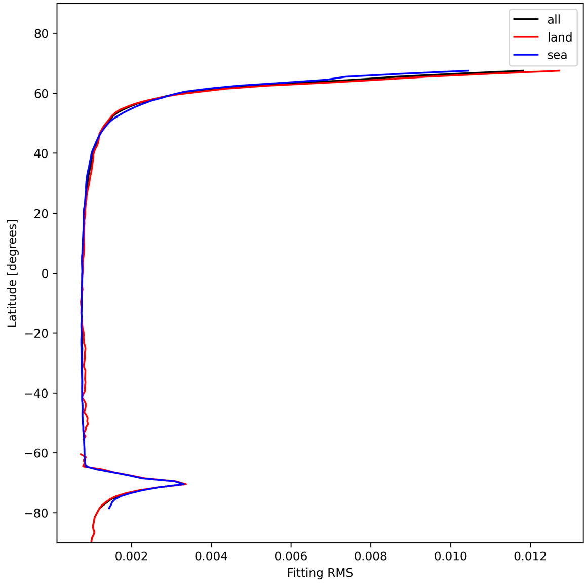
Figure 22: Zonal average of “Fitting RMS” for 2025-01-14 to 2025-01-15.
