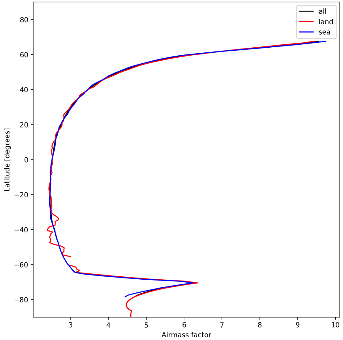
Figure 25: Zonal average of “Airmass factor” for 2025-01-14 to 2025-01-15.
