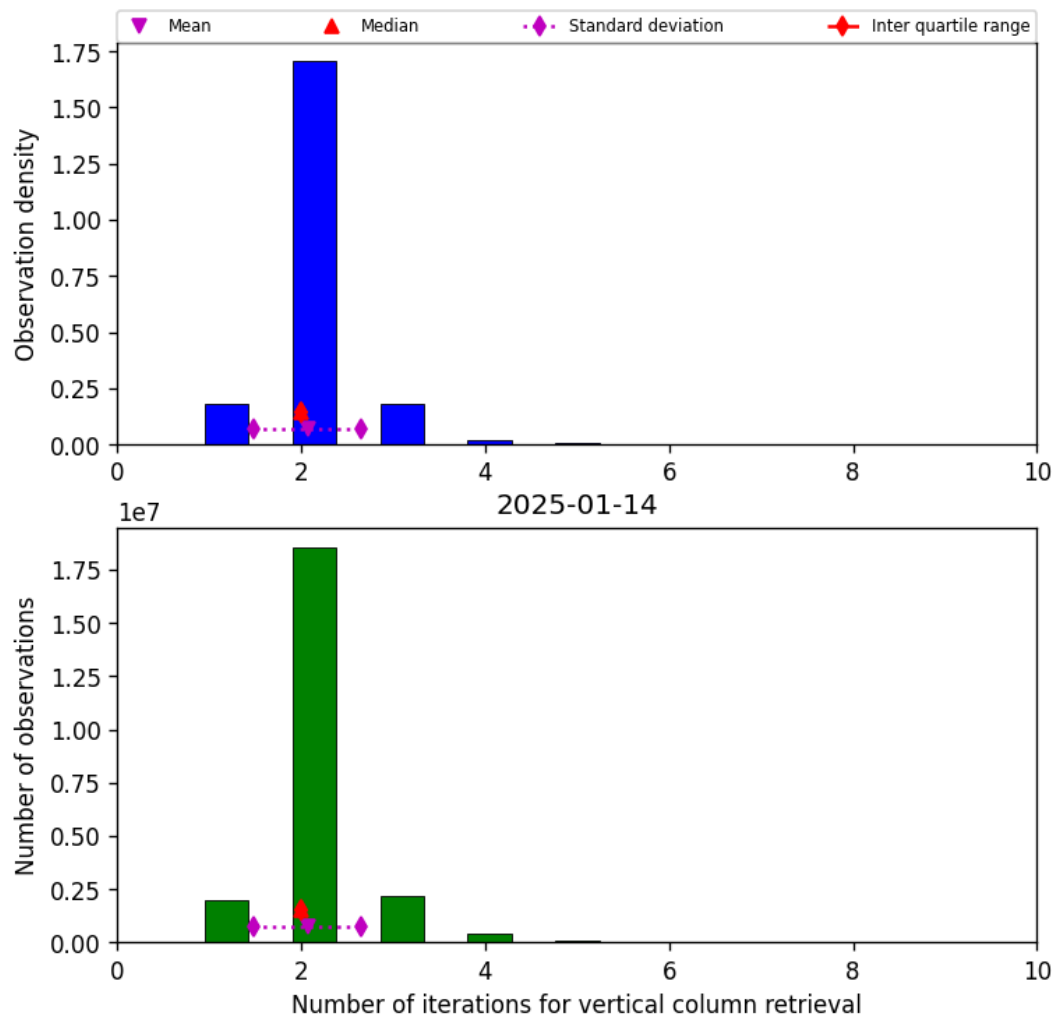
Figure 39: Histogram of “Number of iterations for vertical column retrieval” for 2025-01-14 to 2025-01-15
