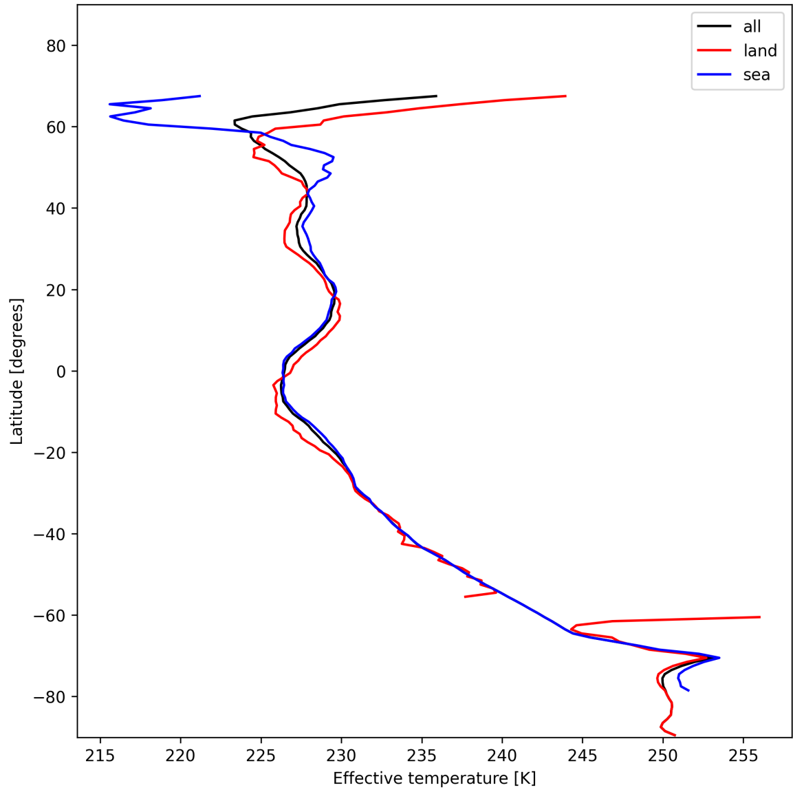
Figure 26: Zonal average of “Effective temperature” for 2025-01-14 to 2025-01-15.
