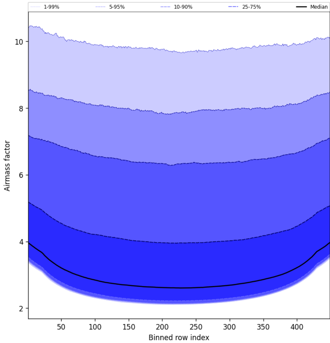
Figure 49: Along track statistics of “Airmass factor” for 2025-01-14 to 2025-01-15
