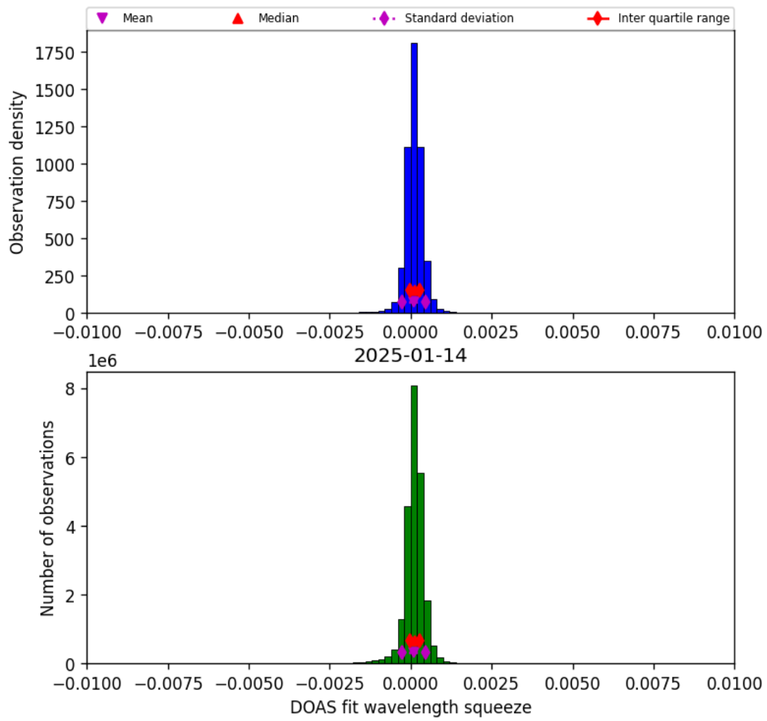
Figure 36: Histogram of “DOAS fit wavelength squeeze” for 2025-01-14 to 2025-01-15
