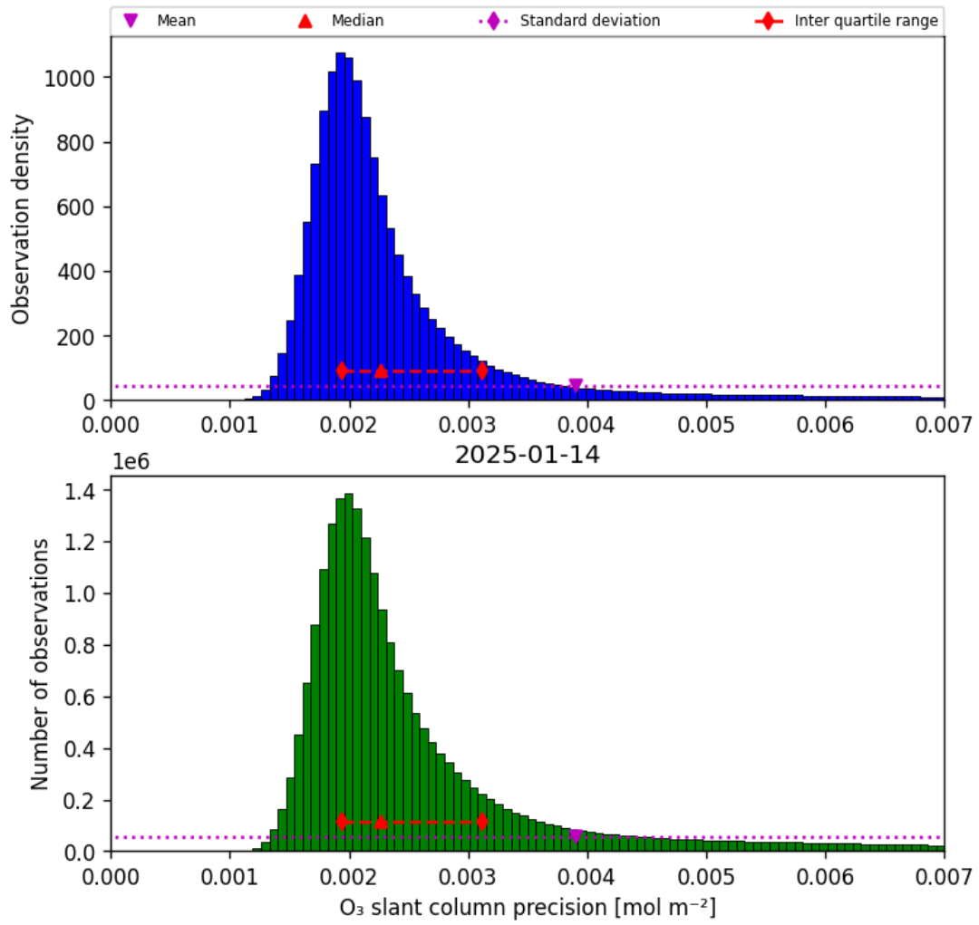
Figure 32: Histogram of “O 3 slant column precision” for 2025-01-14 to 2025-01-15
