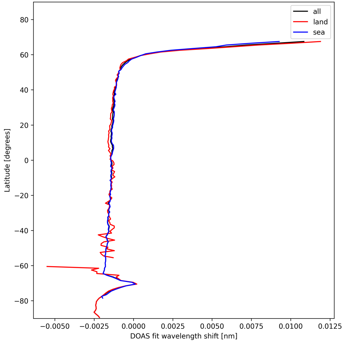
Figure 23: Zonal average of “DOAS fit wavelength shift” for 2025-01-14 to 2025-01-15.
