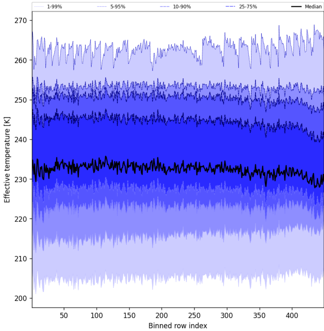
Figure 50: Along track statistics of “Effective temperature” for 2025-01-14 to 2025-01-15
