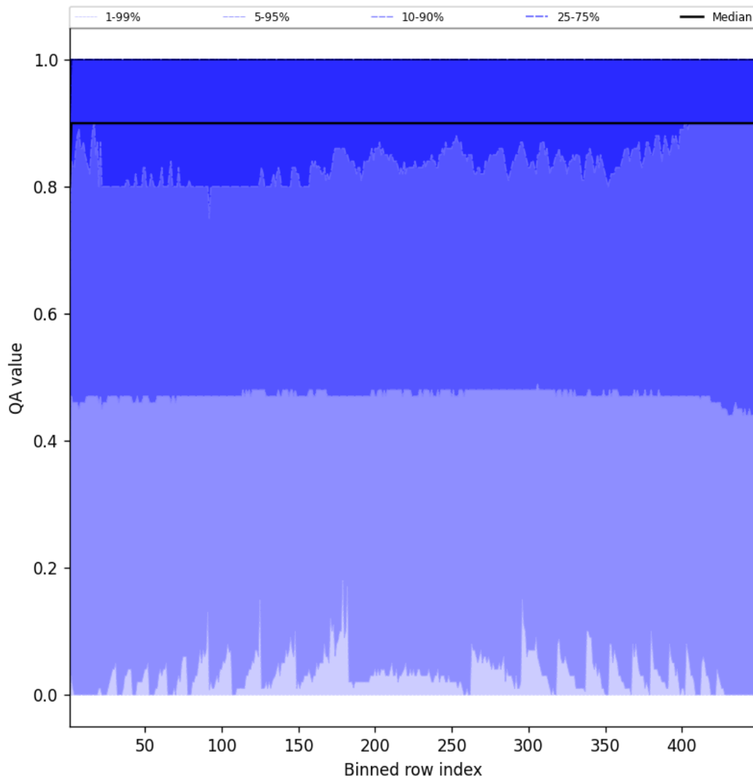
Figure 40: Along track statistics of “QA value” for 2025-01-14 to 2025-01-15
