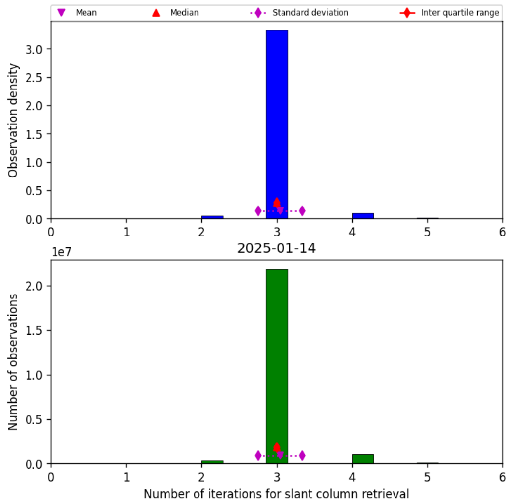
Figure 33: Histogram of “Number of iterations for slant column retrieval” for 2025-01-14 to 2025-01-15
