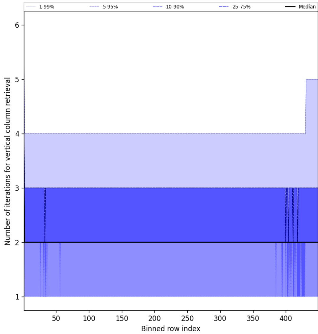
Figure 51: Along track statistics of “Number of iterations for vertical column retrieval” for 2025-01-14 to 2025-01-15
