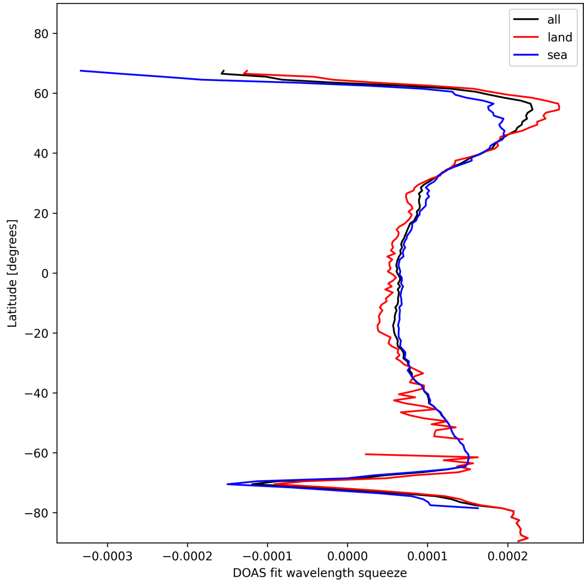
Figure 24: Zonal average of “DOAS fit wavelength squeeze” for 2025-01-14 to 2025-01-15.
