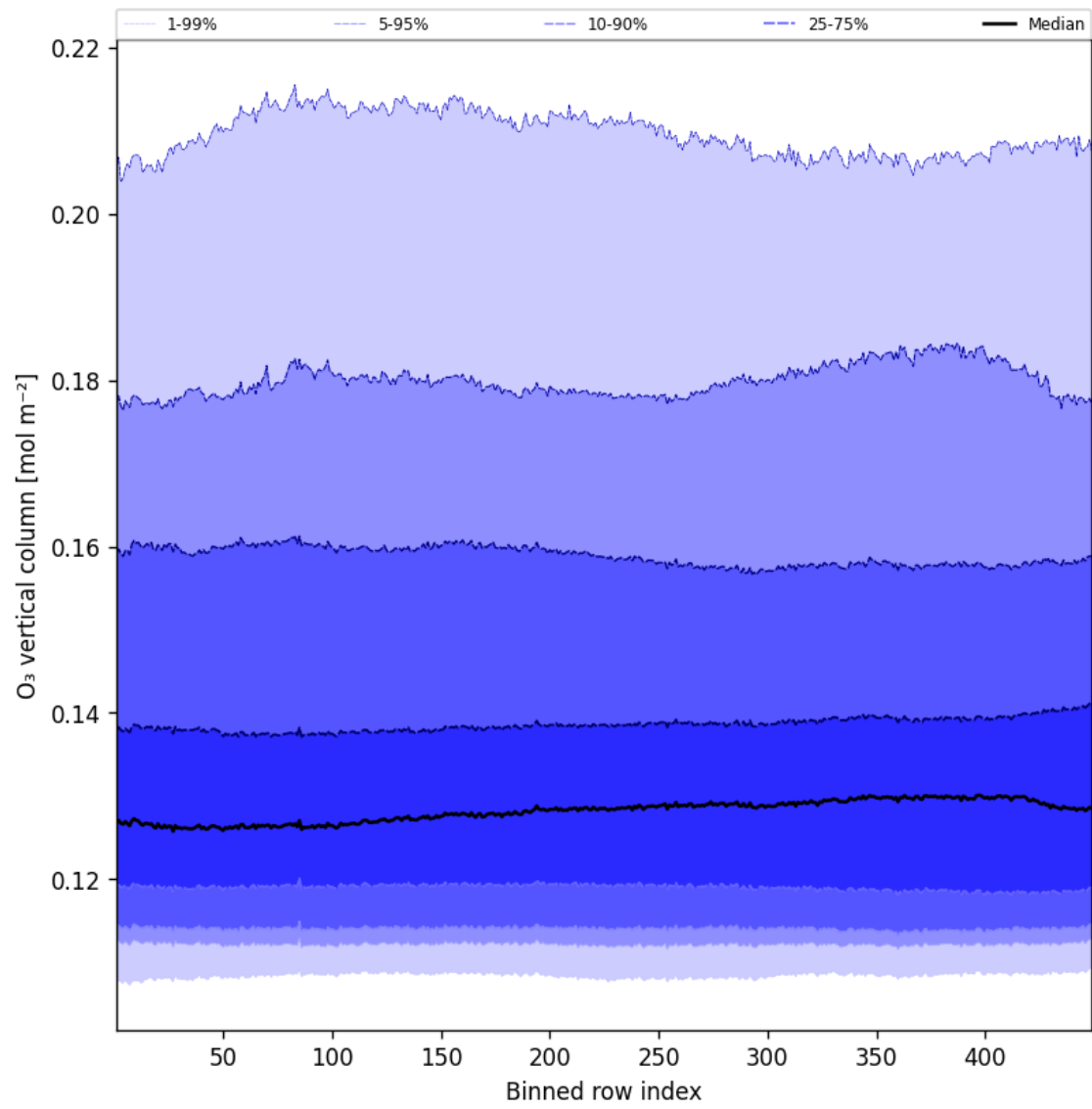
Figure 41: Along track statistics of “O 3 vertical column” for 2025-01-14 to 2025-01-15
