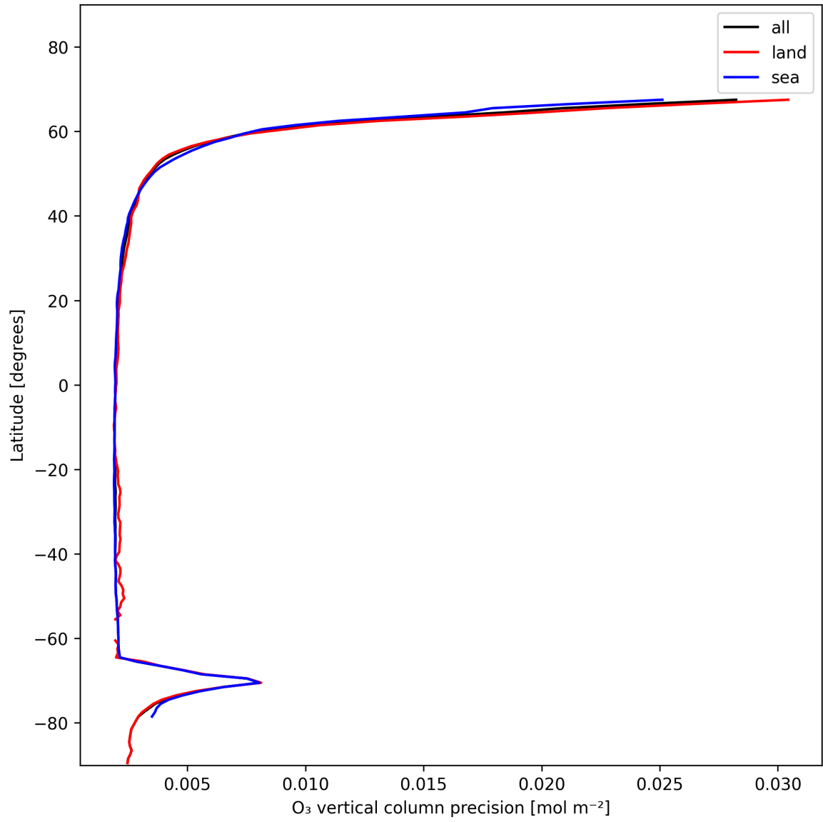
Figure 18: Zonal average of "O 3 vertical column precision" for 2025-01-14 to 2025-01-15.
