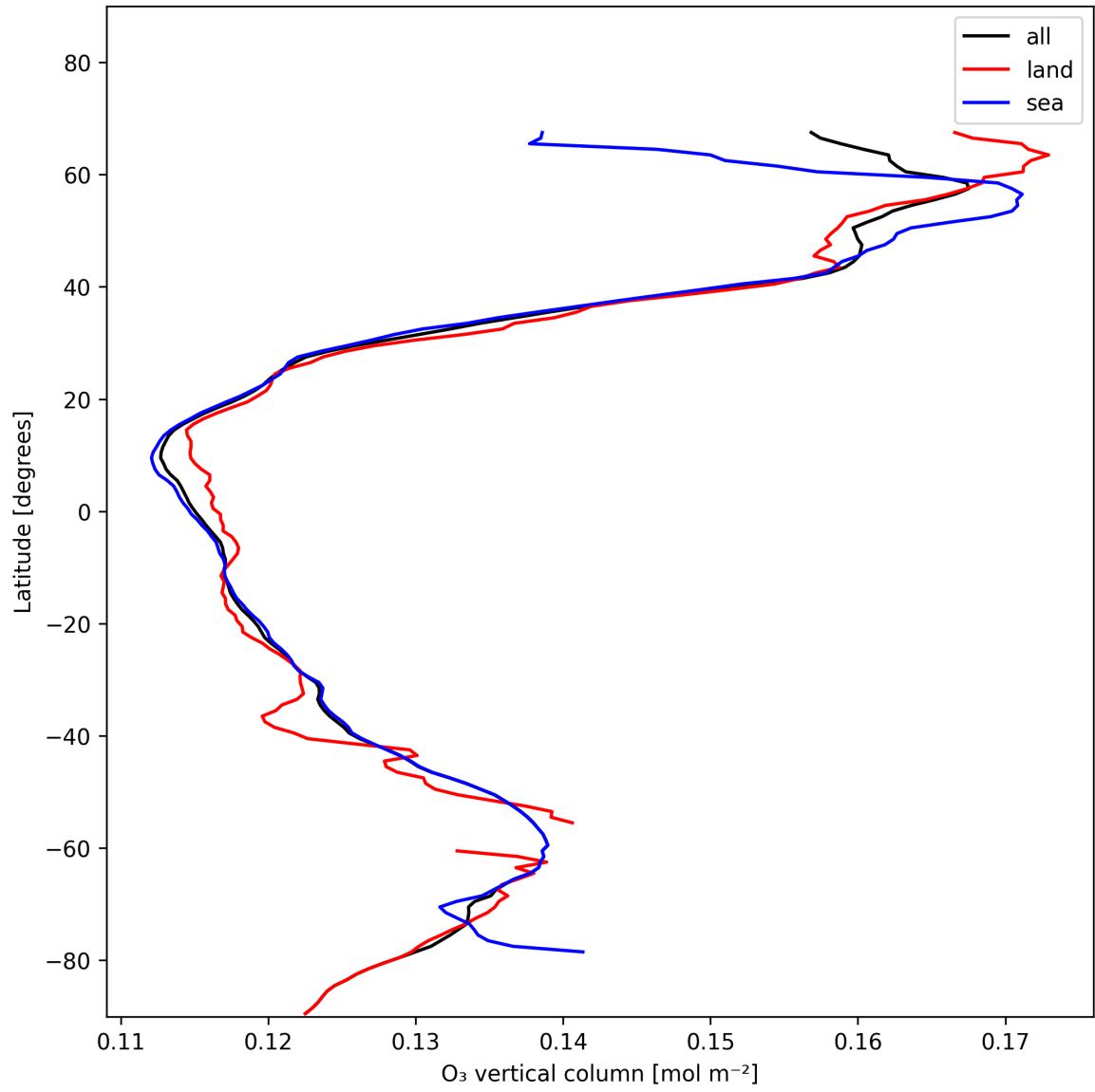
Figure 17: Zonal average of “O 3 vertical column” for 2025-01-14 to 2025-01-15.
