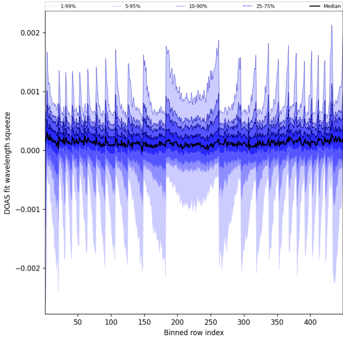
Figure 48: Along track statistics of “DOAS fit wavelength squeeze” for 2025-01-14 to 2025-01-15
