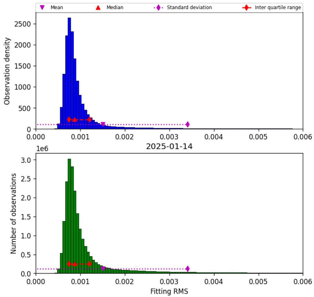
Figure 34: Histogram of “Fitting RMS” for 2025-01-14 to 2025-01-15
