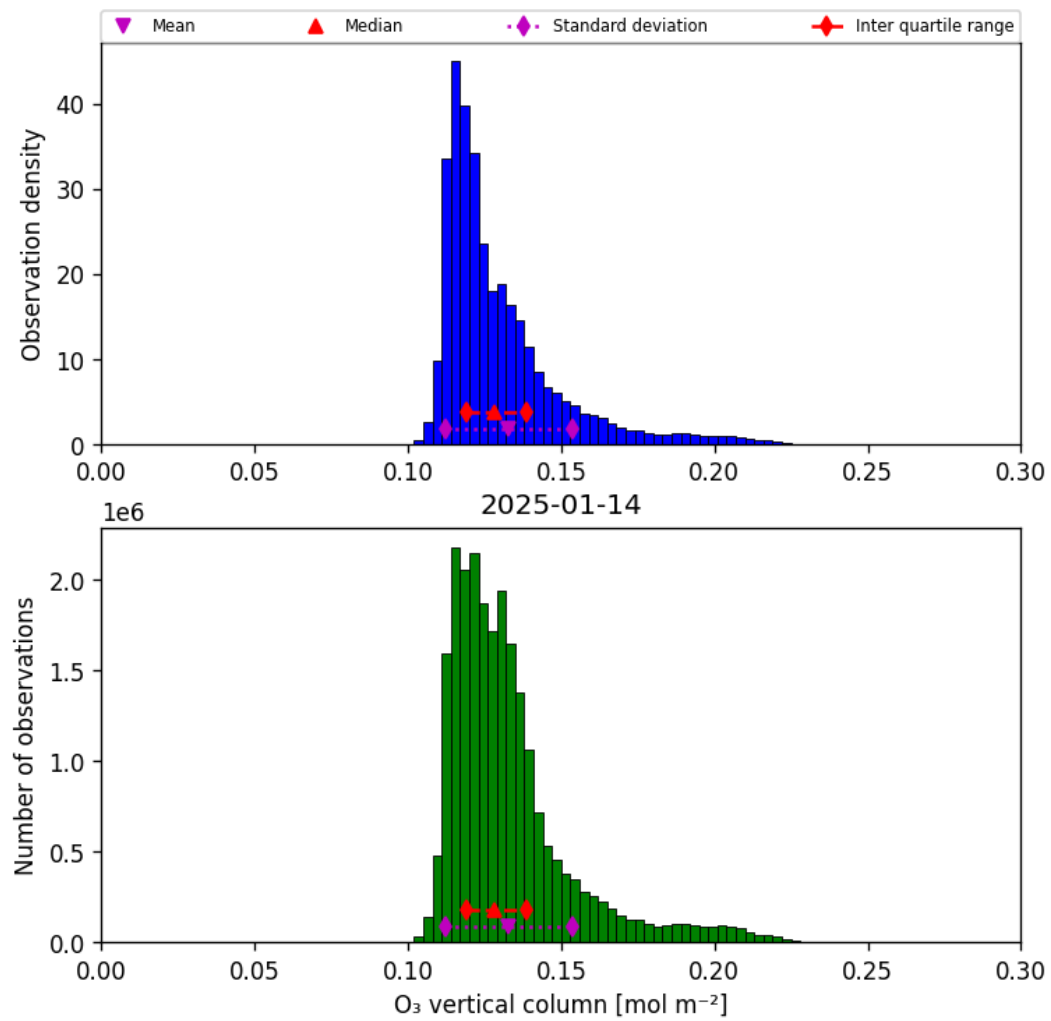
Figure 29: Histogram of “O 3 vertical column” for 2025-01-14 to 2025-01-15
