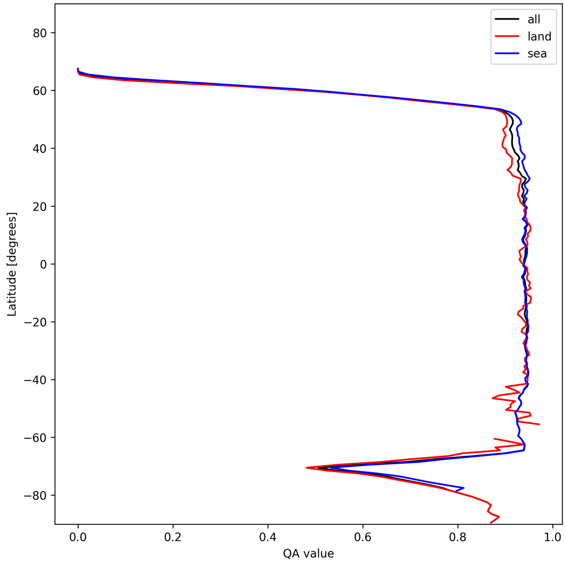
Figure 16: Zonal average of “QA value” for 2025-01-14 to 2025-01-15.
