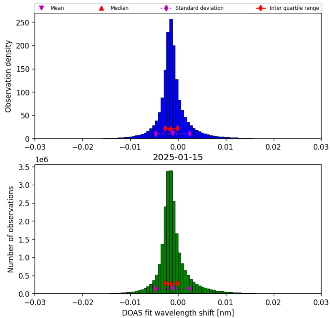
Figure 35: Histogram of “DOAS fit wavelength shift” for 2025-01-15 to 2025-01-15
