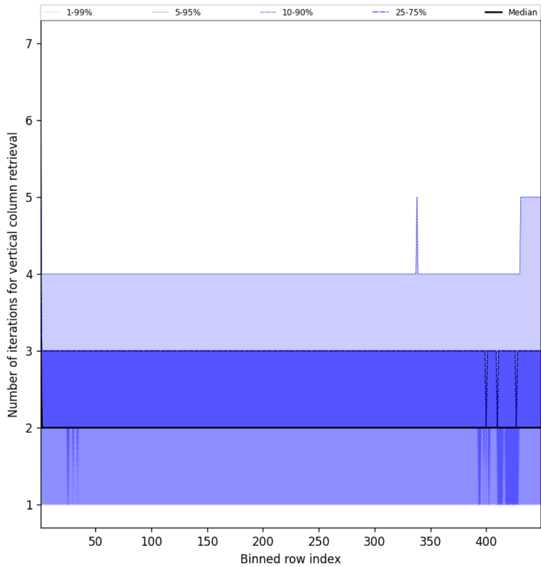
Figure 51: Along track statistics of “Number of iterations for vertical column retrieval” for 2025-01-15 to 2025-01-15
