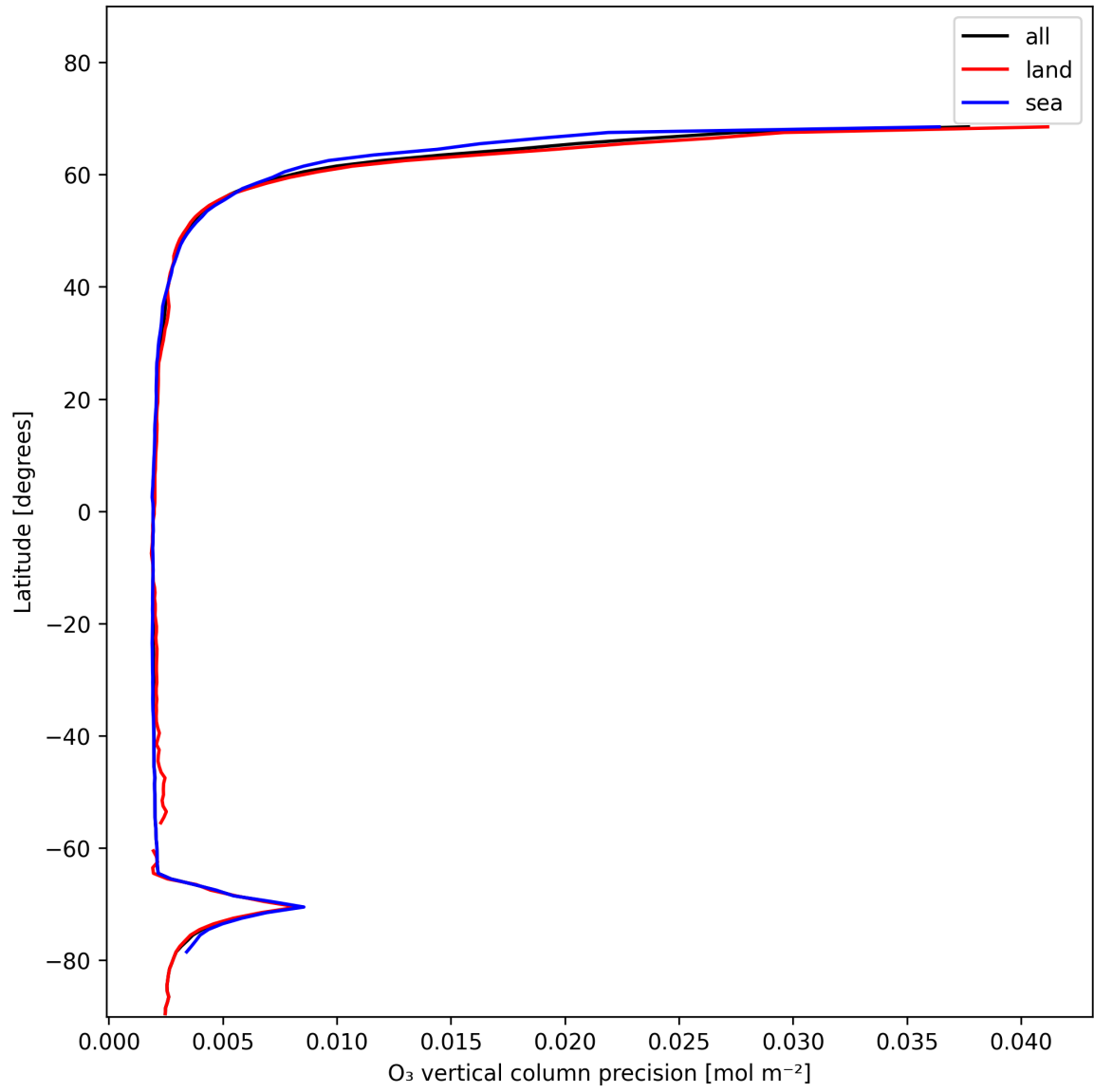
Figure 18: Zonal average of “O 3 vertical column precision” for 2025-01-15 to 2025-01-15.
