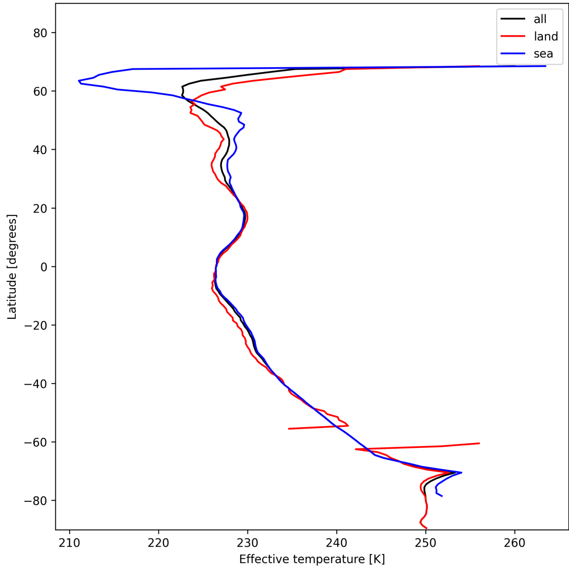
Figure 26: Zonal average of “Effective temperature” for 2025-01-15 to 2025-01-15.
