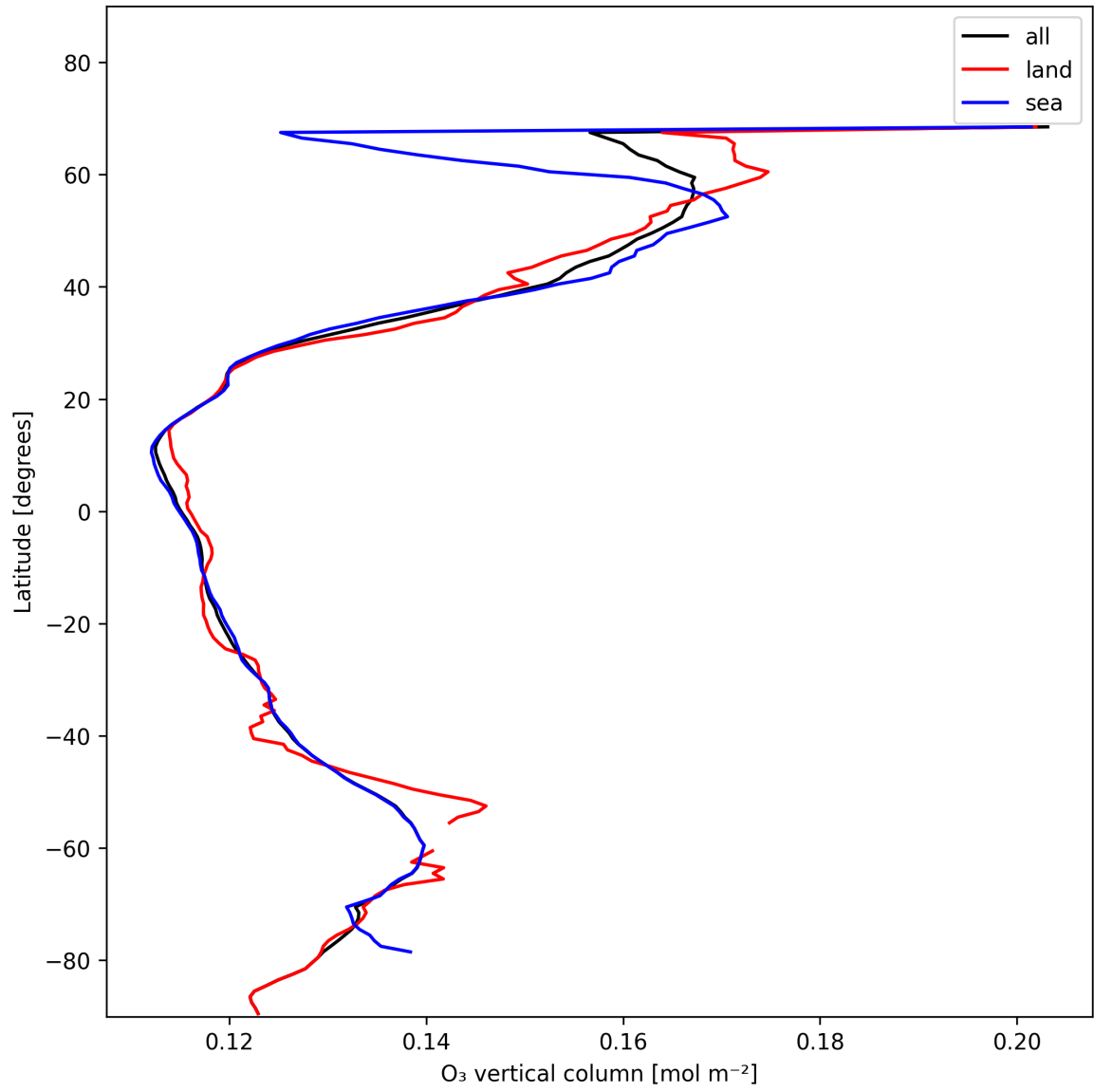
Figure 17: Zonal average of “O 3 vertical column” for 2025-01-15 to 2025-01-15.
