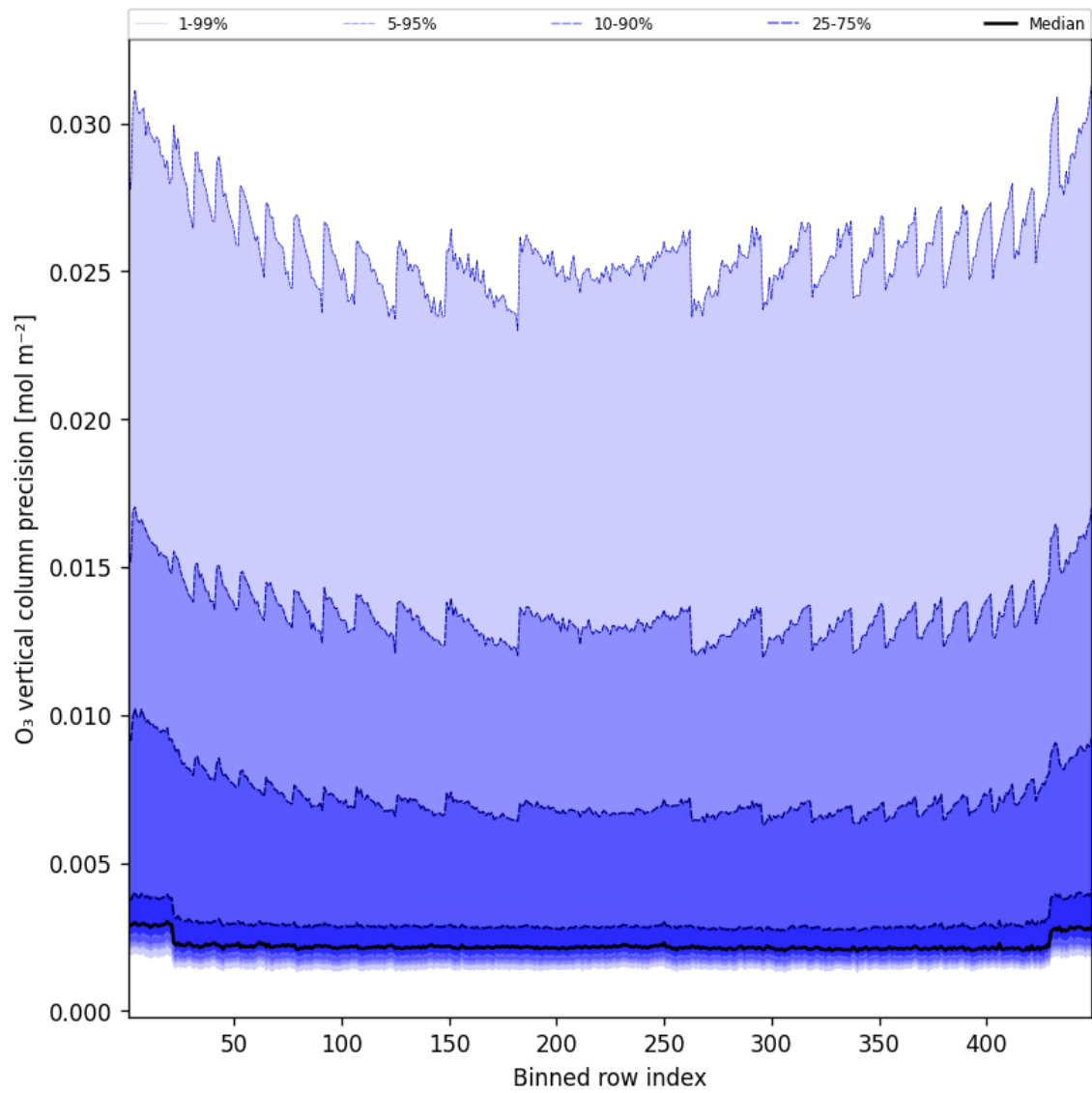
Figure 42: Along track statistics of “O 3 vertical column precision” for 2025-01-15 to 2025-01-15
