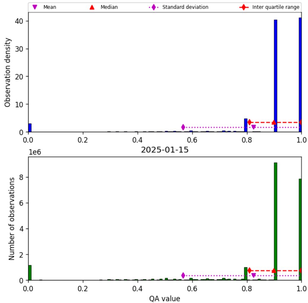
Figure 28: Histogram of “QA value” for 2025-01-15 to 2025-01-15
