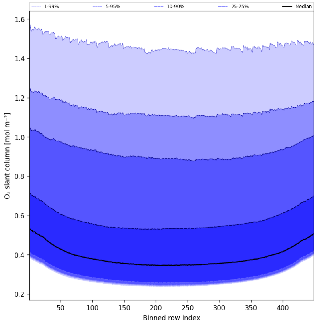
Figure 43: Along track statistics of “O 3 slant column” for 2025-01-15 to 2025-01-15
