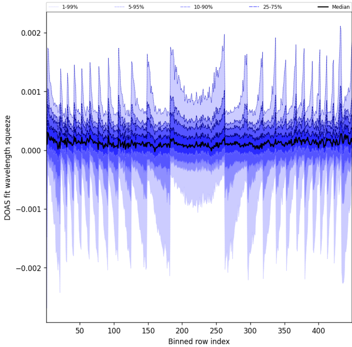
Figure 48: Along track statistics of “DOAS fit wavelength squeeze” for 2025-01-15 to 2025-01-15
