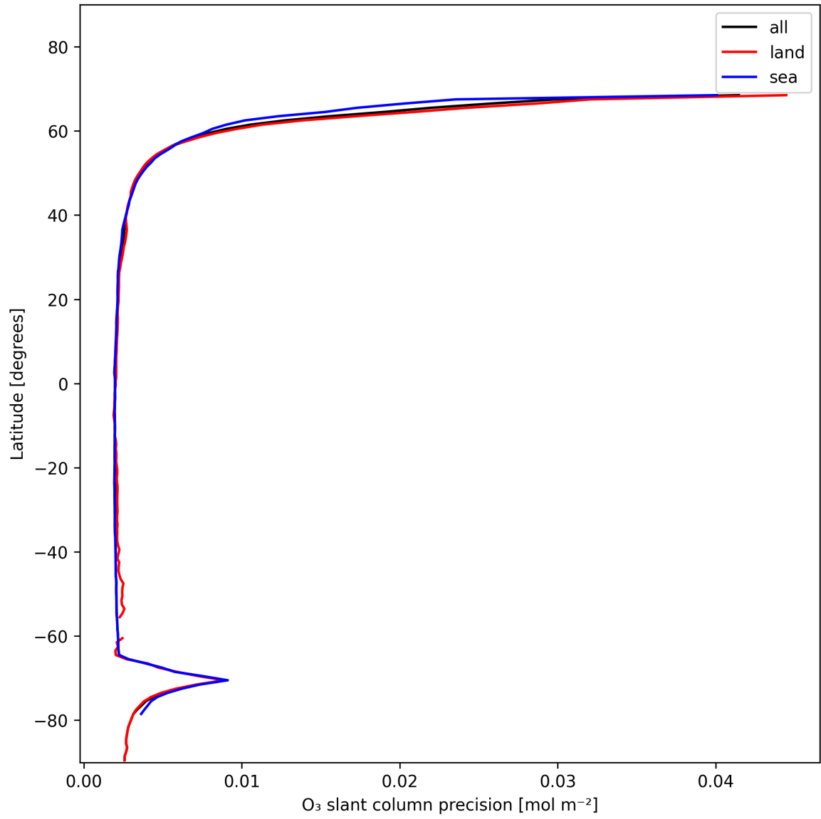
Figure 20: Zonal average of “O 3 slant column precision” for 2025-01-15 to 2025-01-15.
