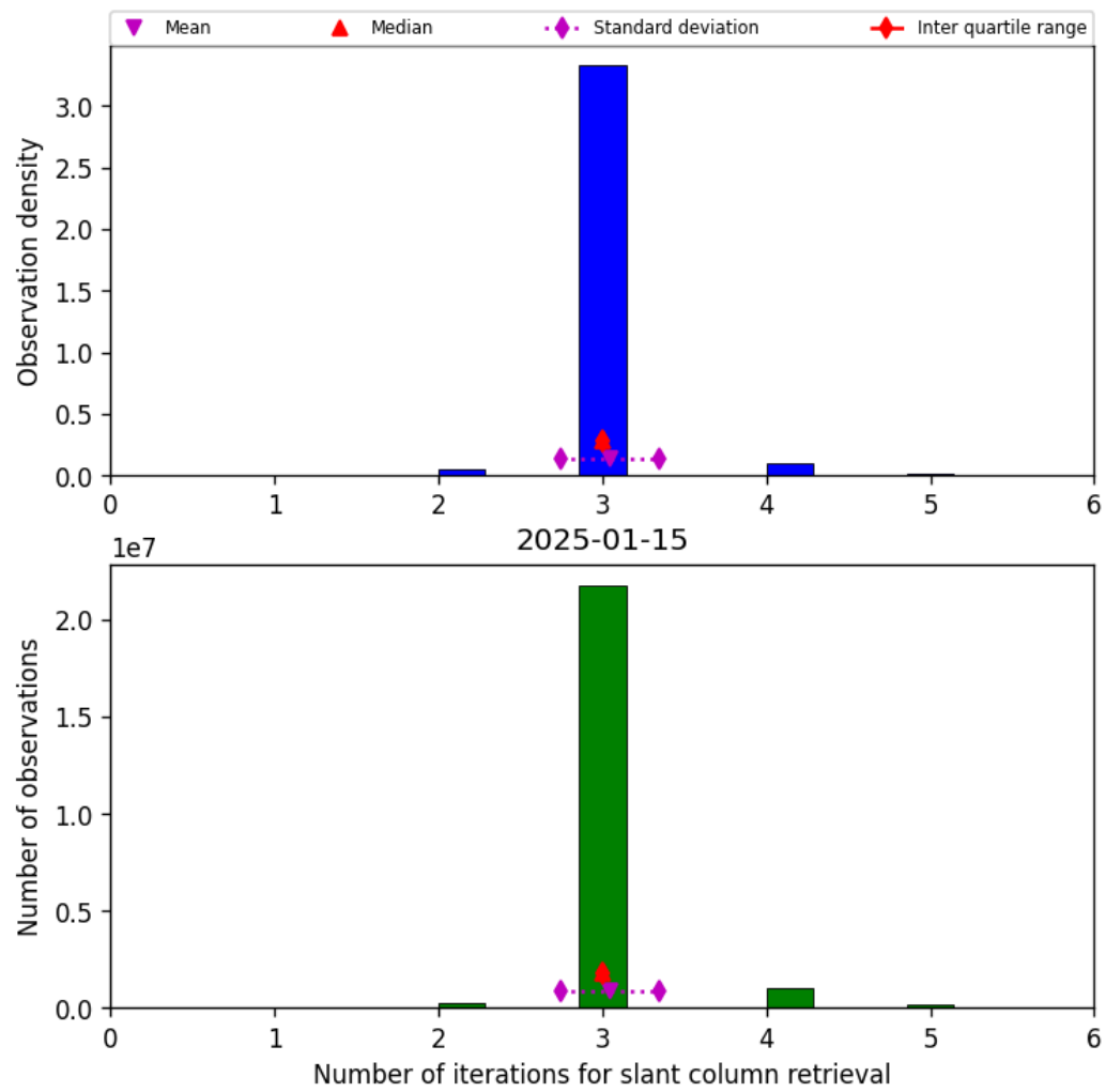
Figure 33: Histogram of "Number of iterations for slant column retrieval" for 2025-01-15 to 2025-01-15
