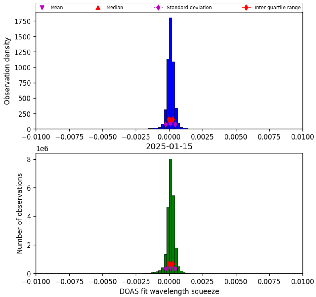
Figure 36: Histogram of “DOAS fit wavelength squeeze” for 2025-01-15 to 2025-01-15
