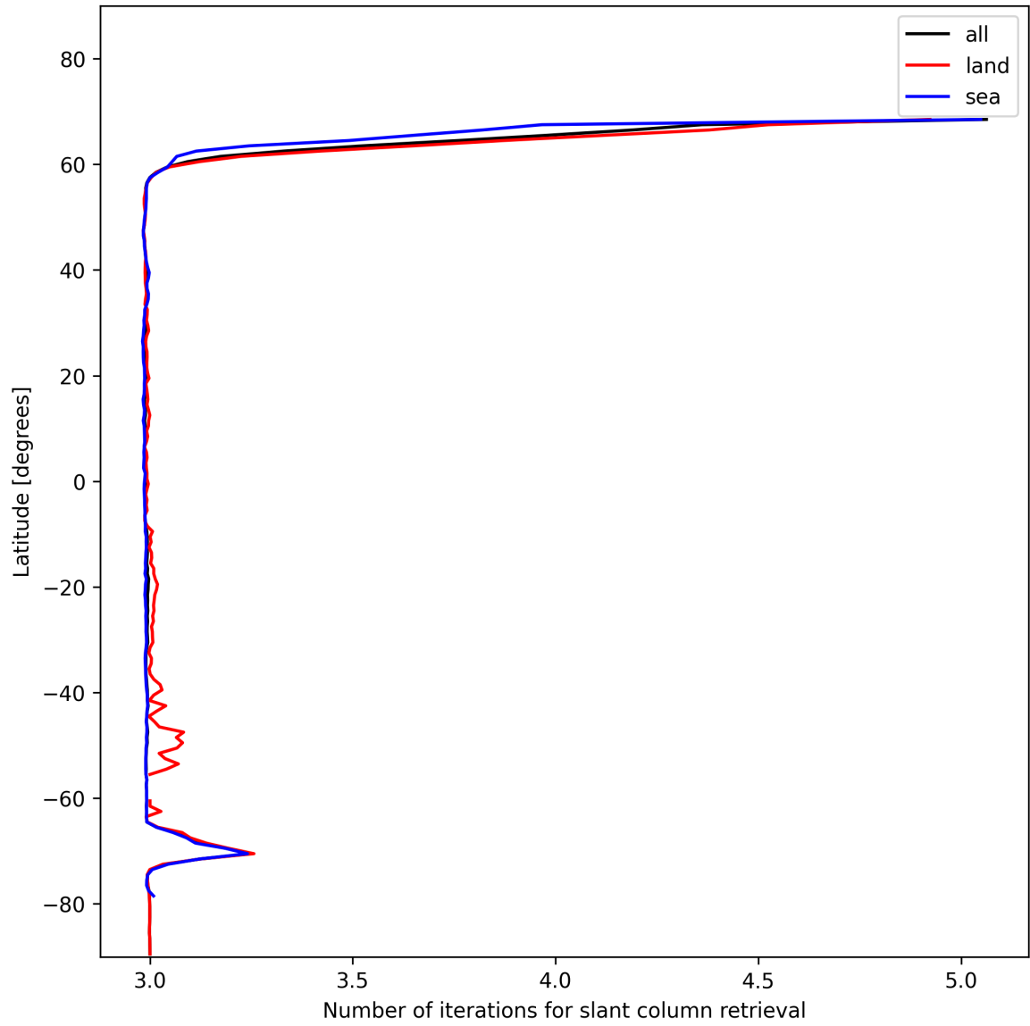
Figure 21: Zonal average of “Number of iterations for slant column retrieval” for 2025-01-15 to 2025-01-15.
