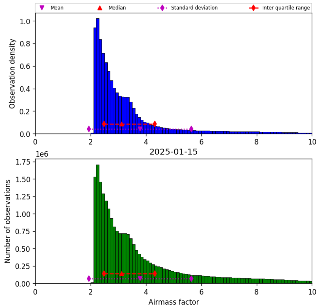
Figure 37: Histogram of “Airmass factor” for 2025-01-15 to 2025-01-15
