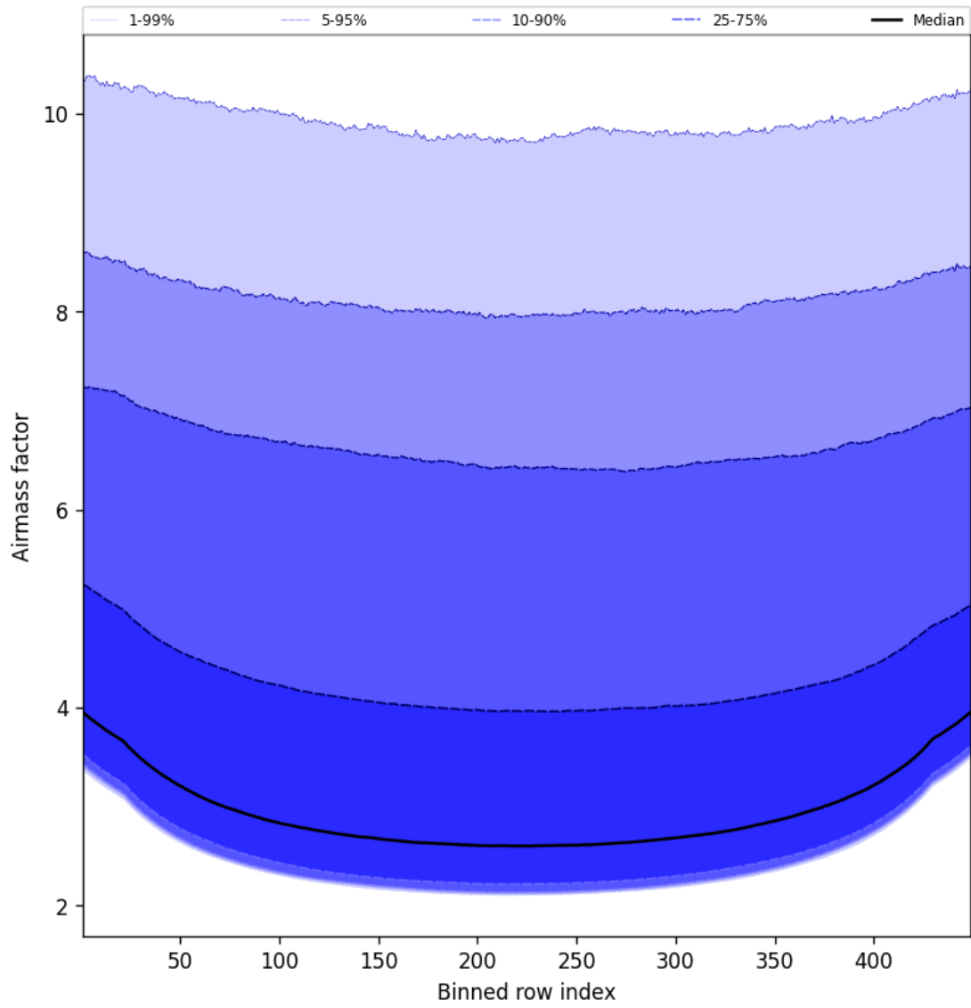
Figure 49: Along track statistics of “Airmass factor” for 2025-01-15 to 2025-01-15
