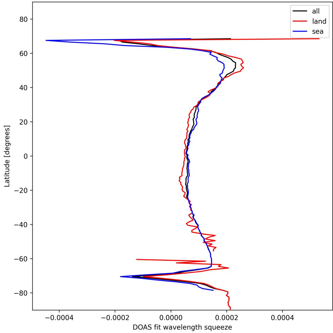
Figure 24: Zonal average of “DOAS fit wavelength squeeze” for 2025-01-15 to 2025-01-15.
