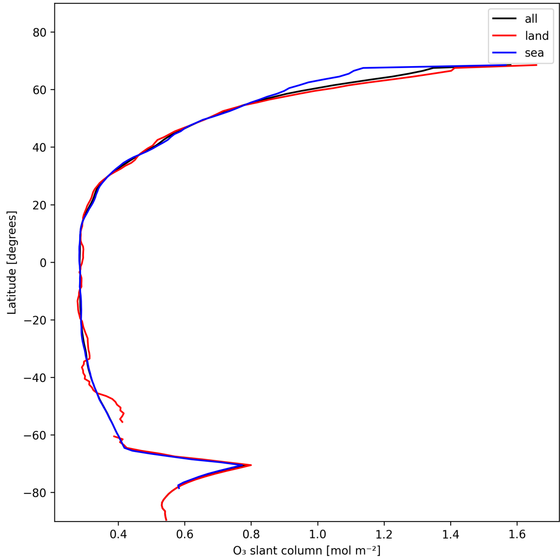
Figure 19: Zonal average of “O 3 slant column” for 2025-01-15 to 2025-01-15.
