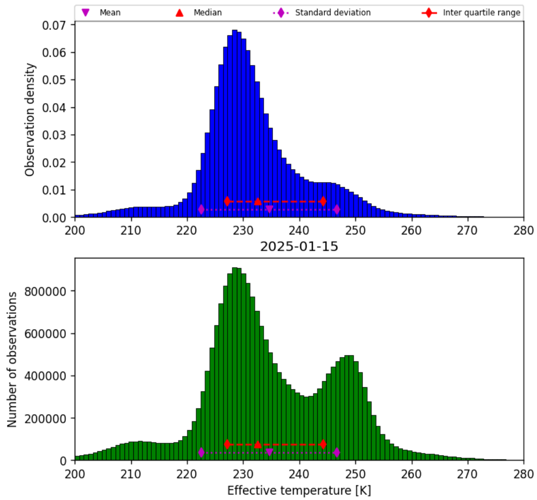
Figure 38: Histogram of “Effective temperature” for 2025-01-15 to 2025-01-15
