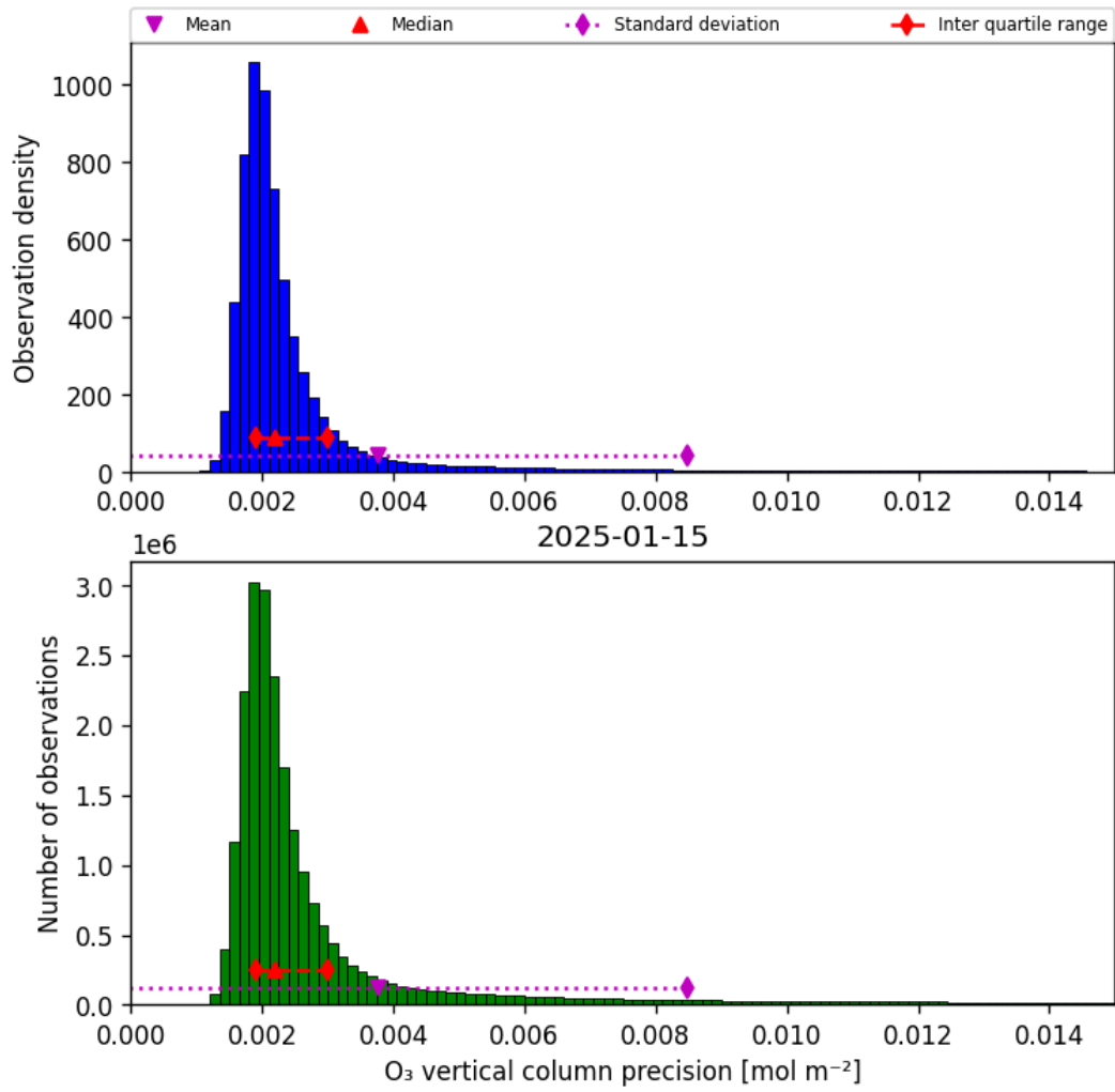
Figure 30: Histogram of “O 3 vertical column precision” for 2025-01-15 to 2025-01-15
