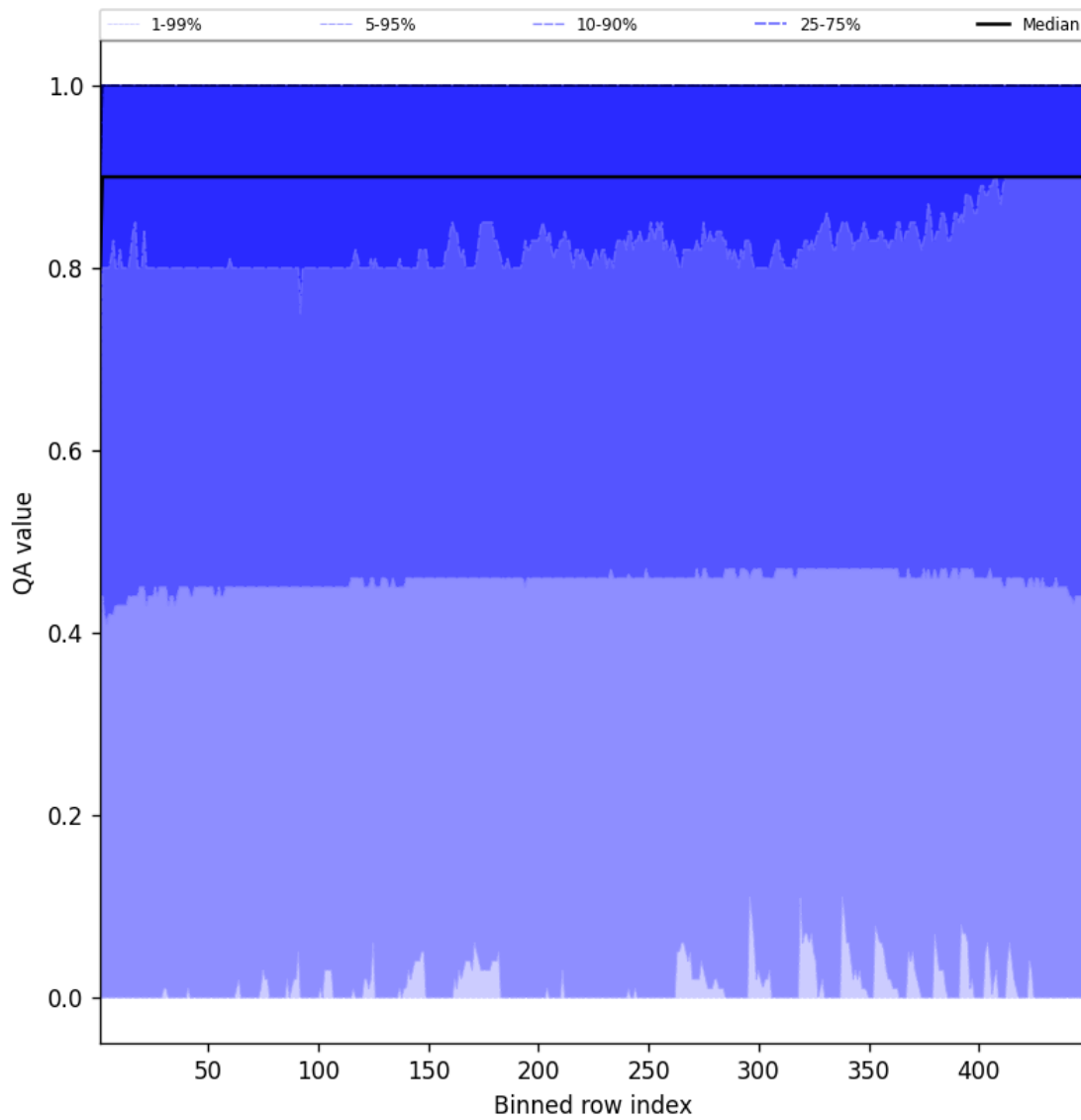
Figure 40: Along track statistics of “QA value” for 2025-01-15 to 2025-01-15
