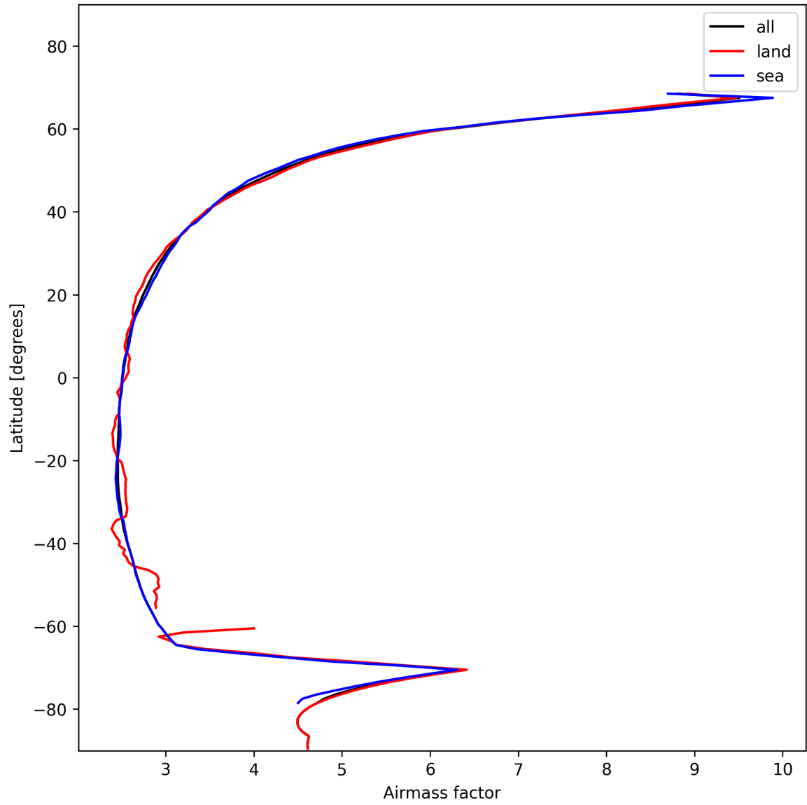
Figure 25: Zonal average of “Airmass factor” for 2025-01-15 to 2025-01-15.
