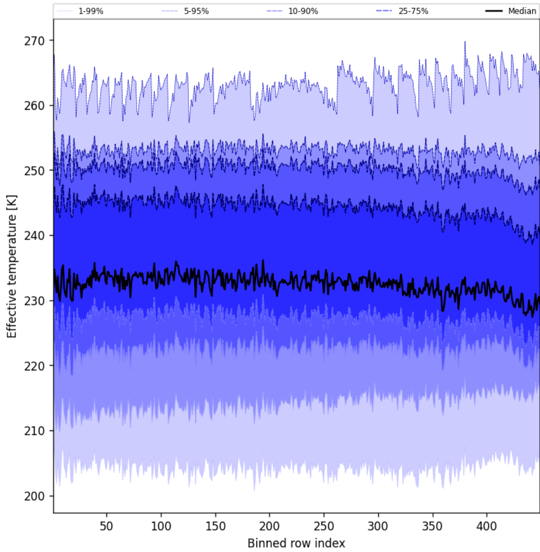
Figure 50: Along track statistics of “Effective temperature” for 2025-01-15 to 2025-01-15
