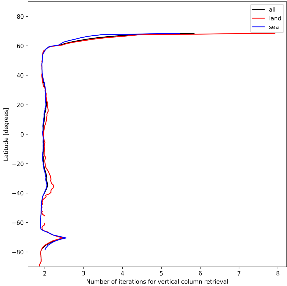
Figure 27: Zonal average of “Number of iterations for vertical column retrieval” for 2025-01-15 to 2025-01-15.
