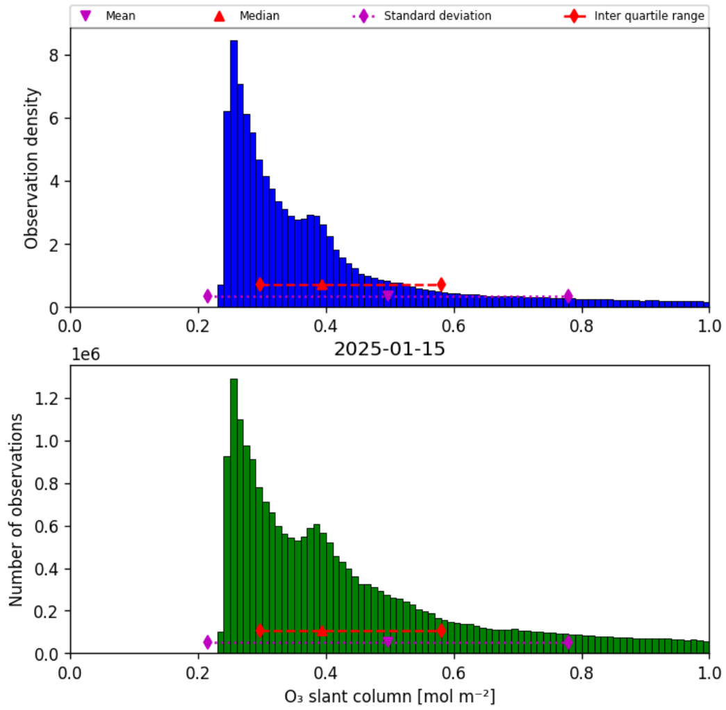
Figure 31: Histogram of “O 3 slant column” for 2025-01-15 to 2025-01-15
