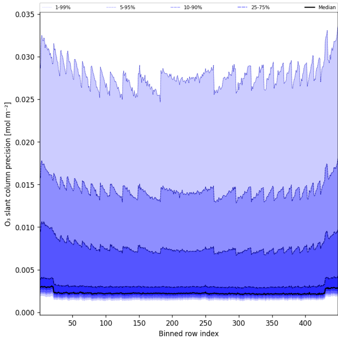
Figure 44: Along track statistics of “O 3 slant column precision” for 2025-01-15 to 2025-01-15
