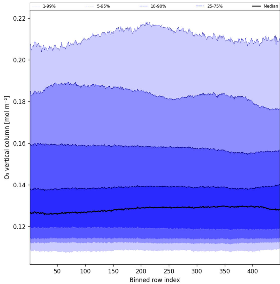
Figure 41: Along track statistics of “O 3 vertical column” for 2025-01-15 to 2025-01-15
