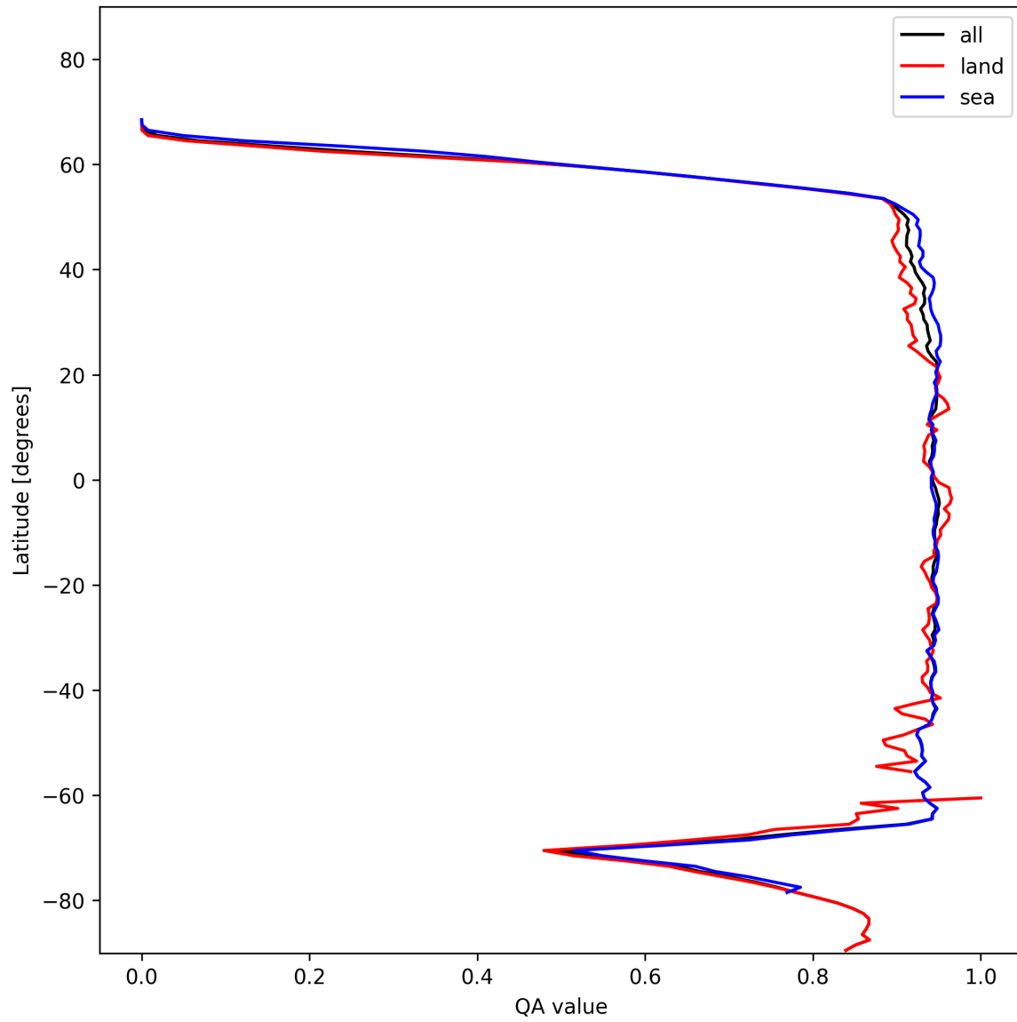
Figure 16: Zonal average of “QA value” for 2025-01-15 to 2025-01-15.
