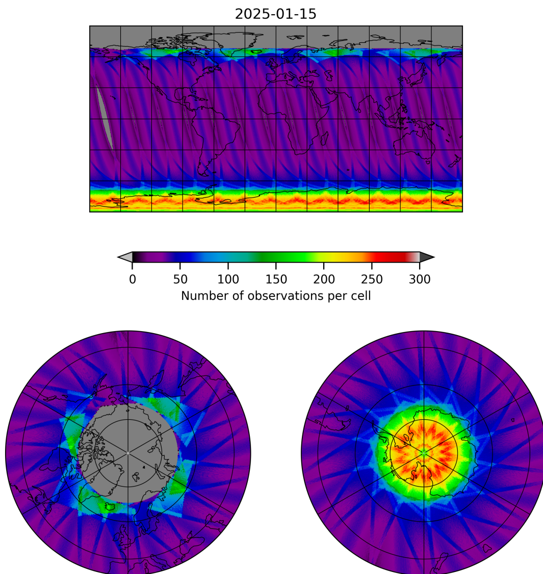
Figure 15: Map of the number of observations for 2025-01-15 to 2025-01-15
