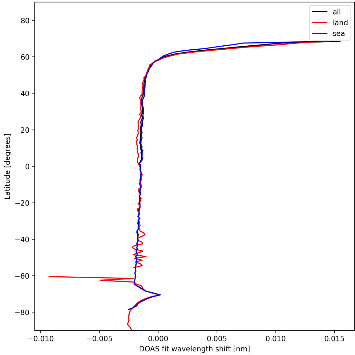
Figure 23: Zonal average of “DOAS fit wavelength shift” for 2025-01-15 to 2025-01-15.
