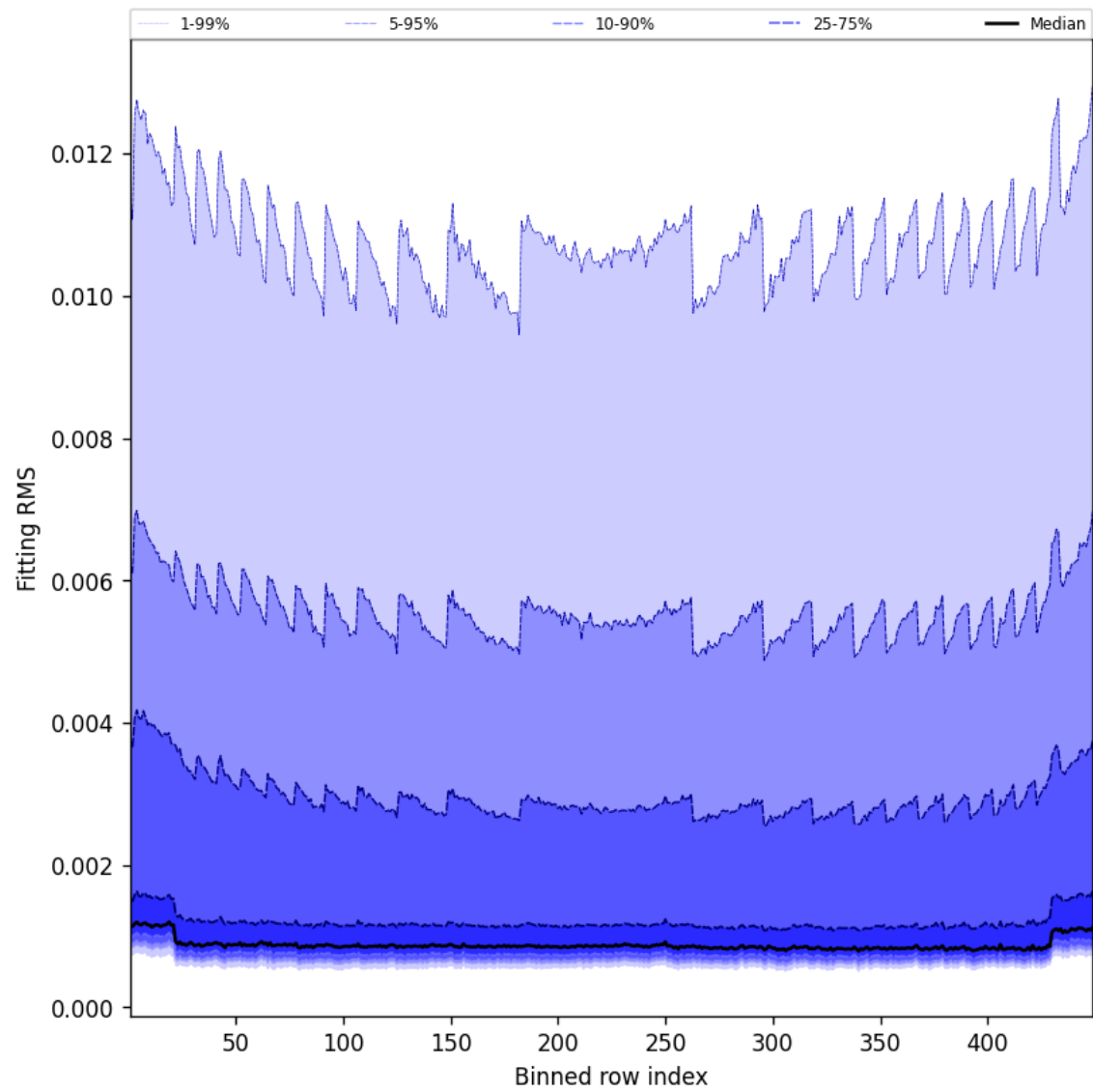
Figure 46: Along track statistics of “Fitting RMS” for 2025-01-15 to 2025-01-15
