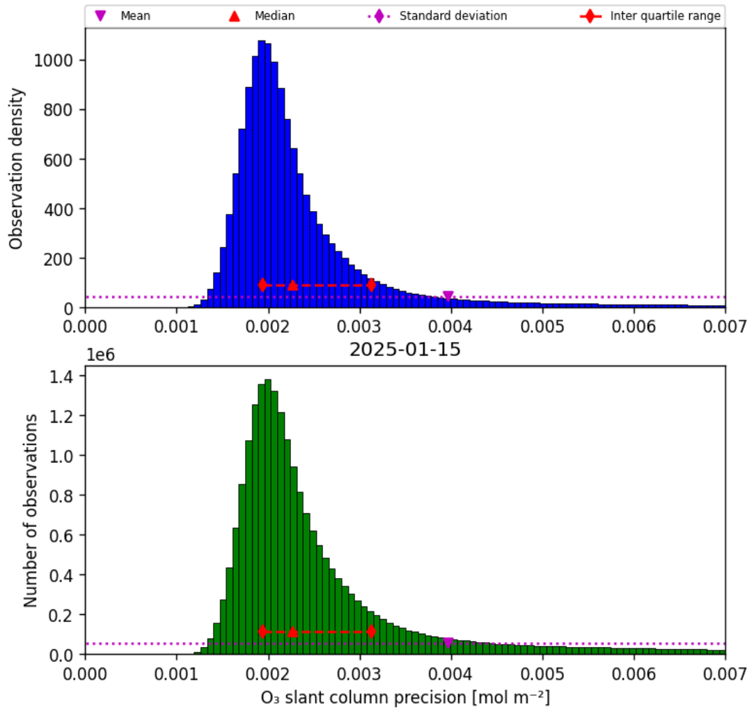
Figure 32: Histogram of "O 3 slant column precision" for 2025-01-15 to 2025-01-15
