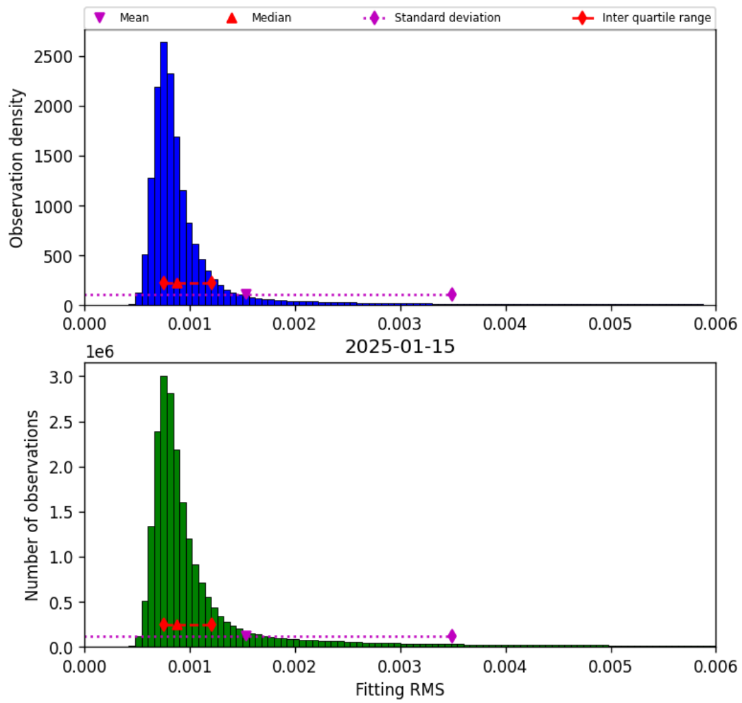
Figure 34: Histogram of “Fitting RMS” for 2025-01-15 to 2025-01-15
