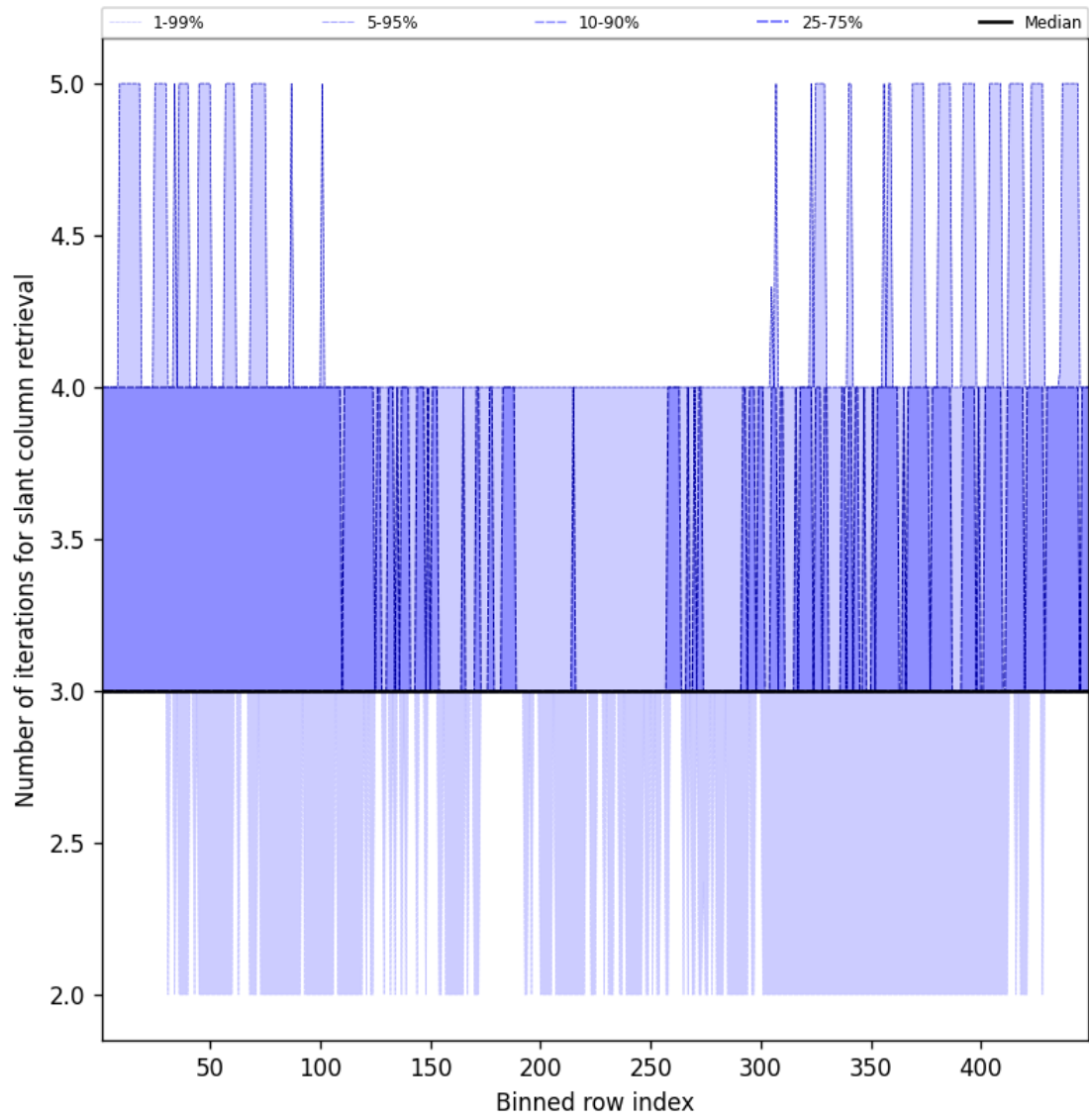
Figure 45: Along track statistics of “Number of iterations for slant column retrieval” for 2025-01-15 to 2025-01-15
