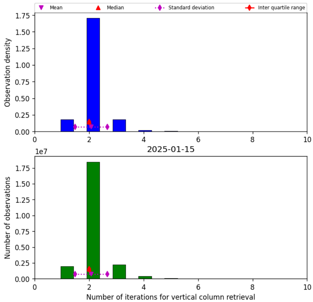
Figure 39: Histogram of “Number of iterations for vertical column retrieval” for 2025-01-15 to 2025-01-15
