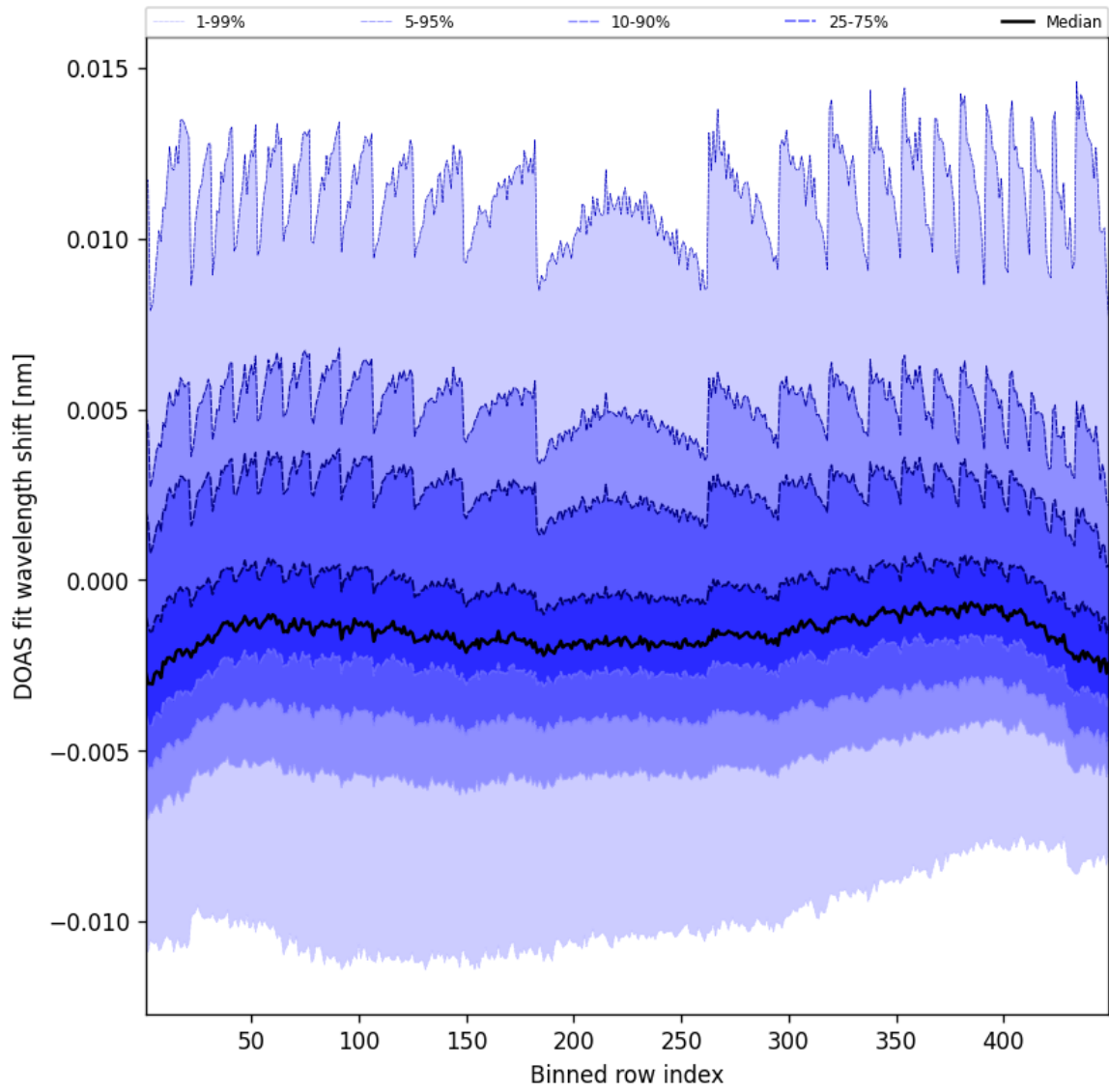
Figure 47: Along track statistics of “DOAS fit wavelength shift” for 2025-01-15 to 2025-01-15
