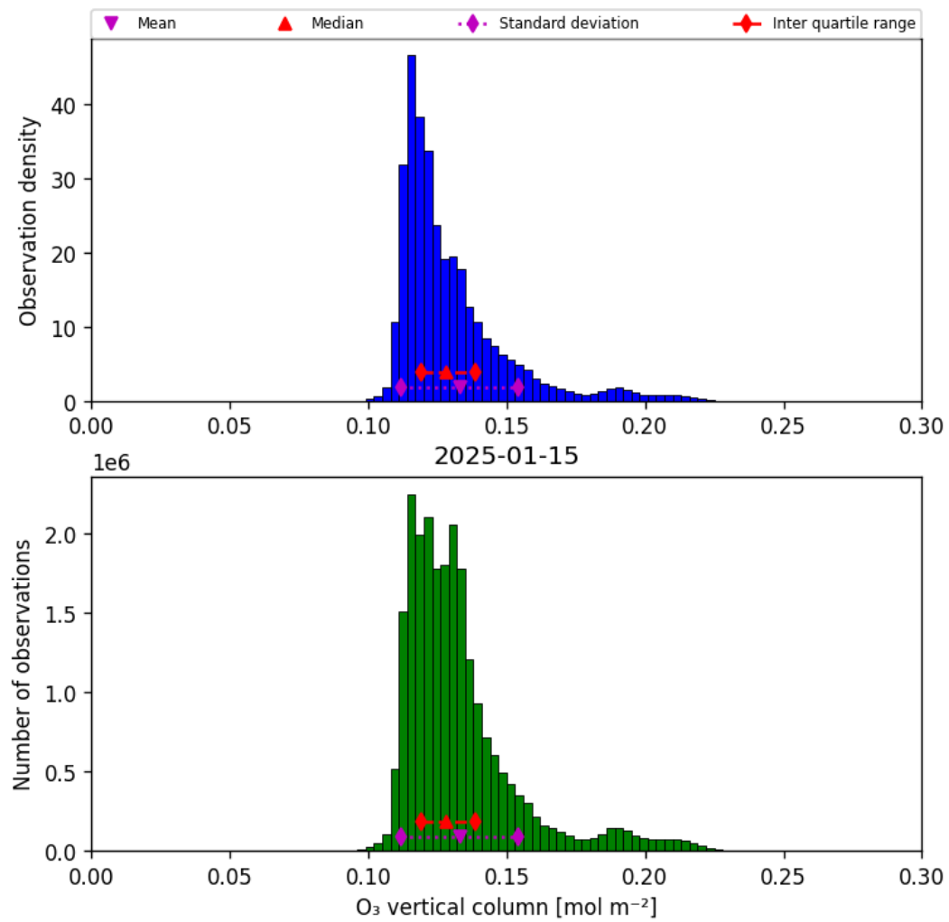
Figure 29: Histogram of “O 3 vertical column” for 2025-01-15 to 2025-01-15
