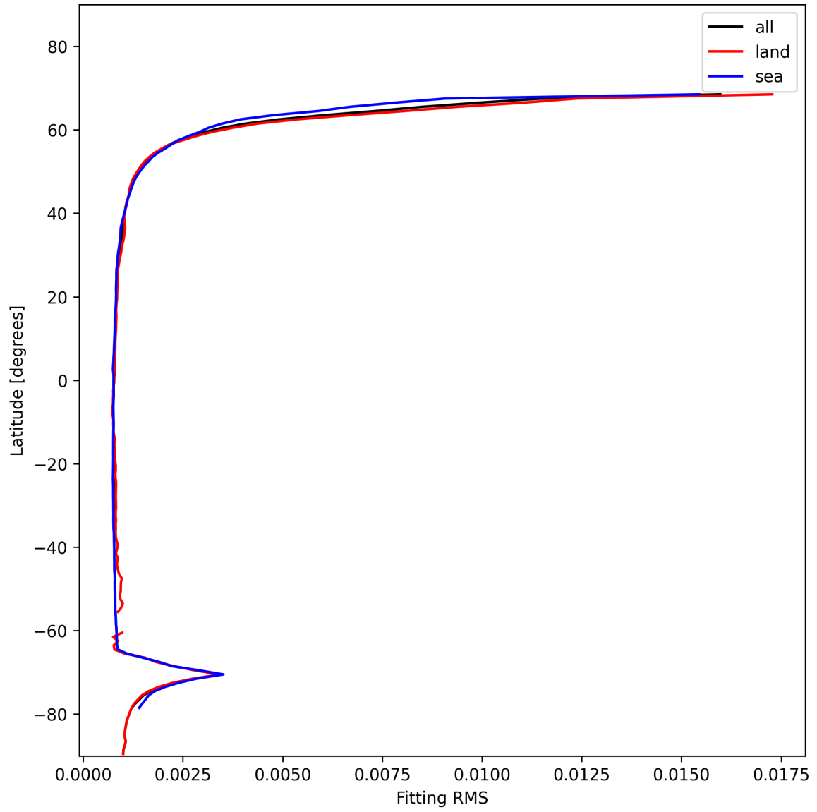
Figure 22: Zonal average of “Fitting RMS” for 2025-01-15 to 2025-01-15.
