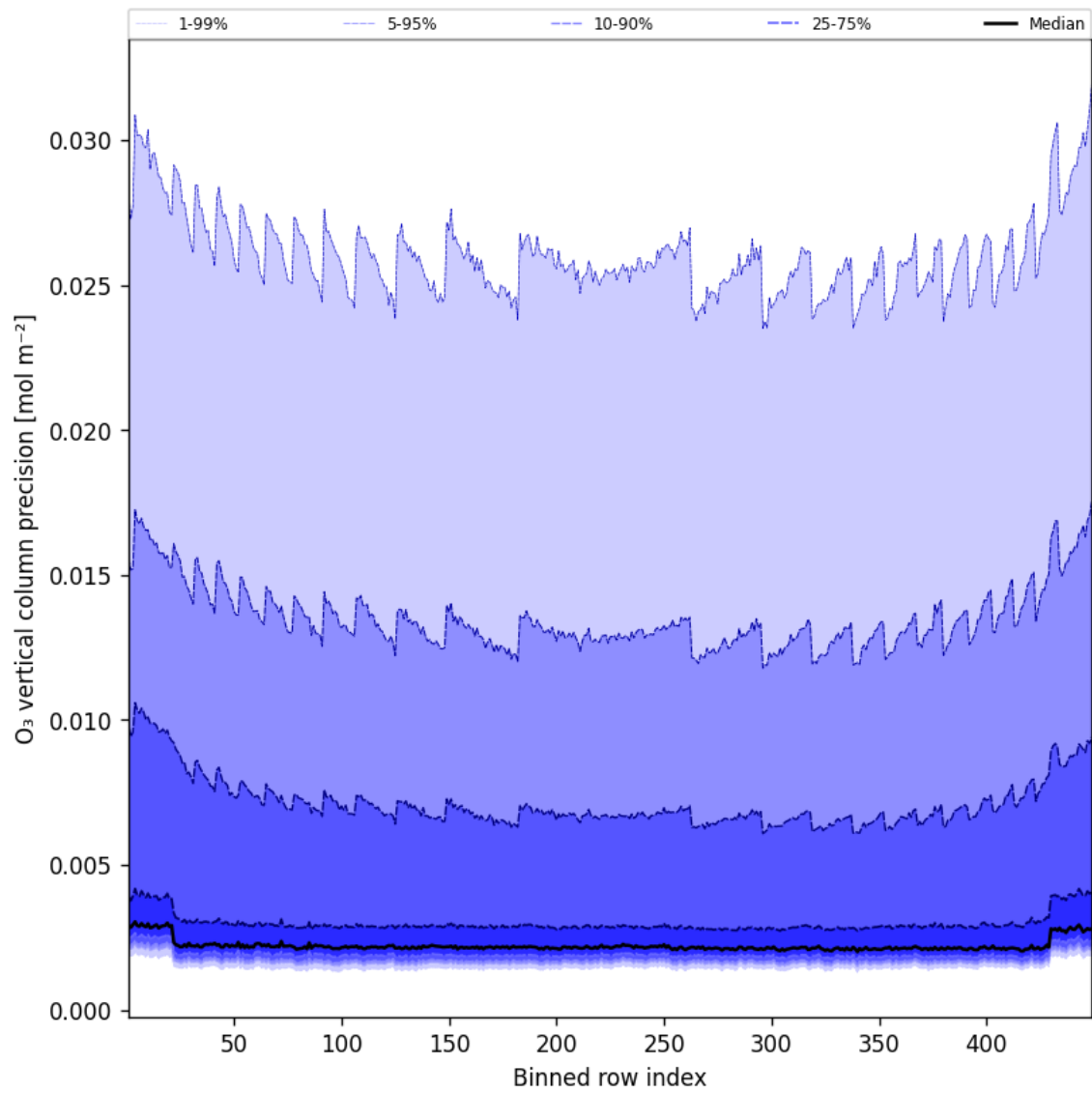
Figure 42: Along track statistics of “O 3 vertical column precision” for 2025-01-16 to 2025-01-17
