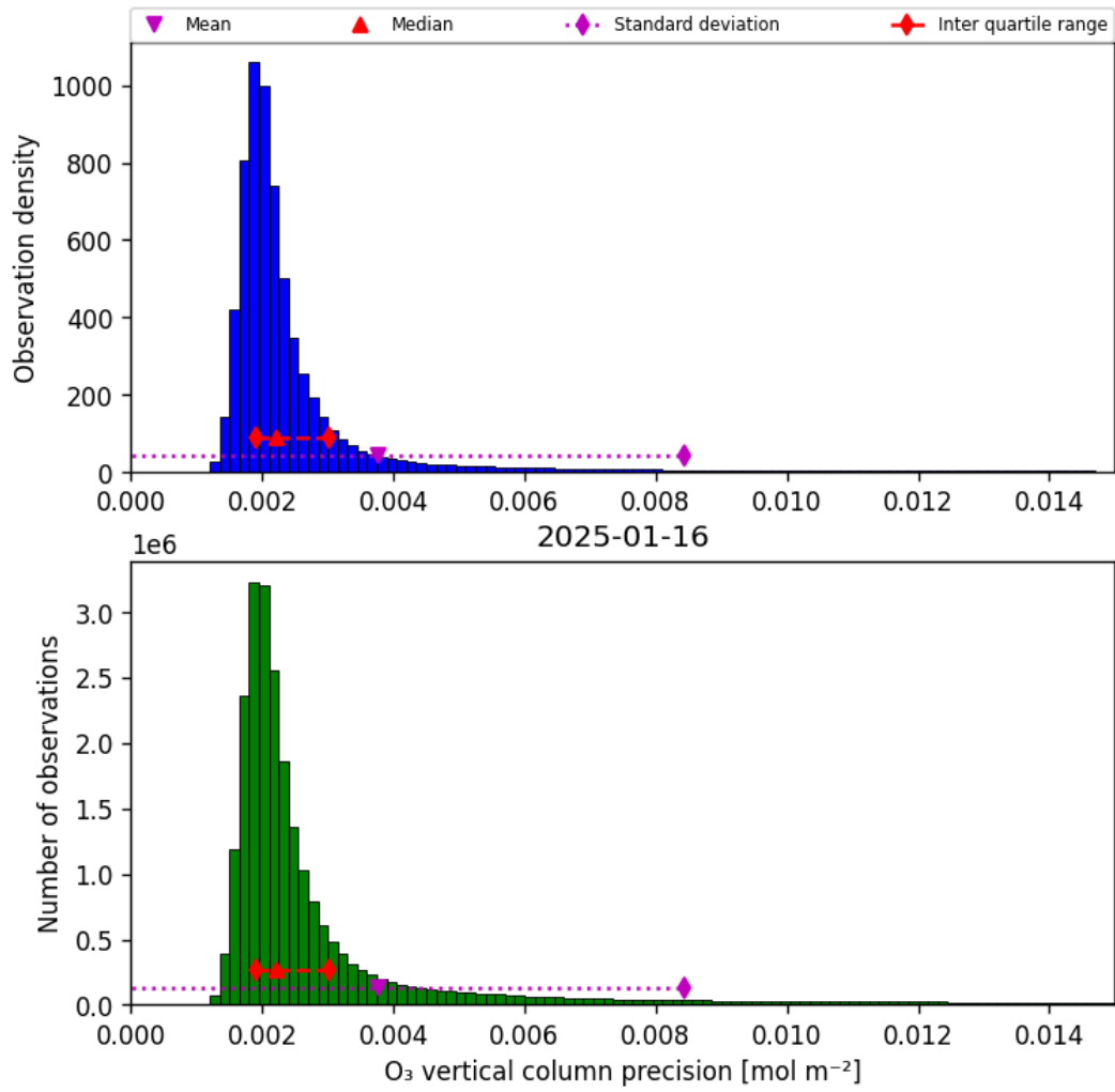
Figure 30: Histogram of “O 3 vertical column precision” for 2025-01-16 to 2025-01-17
