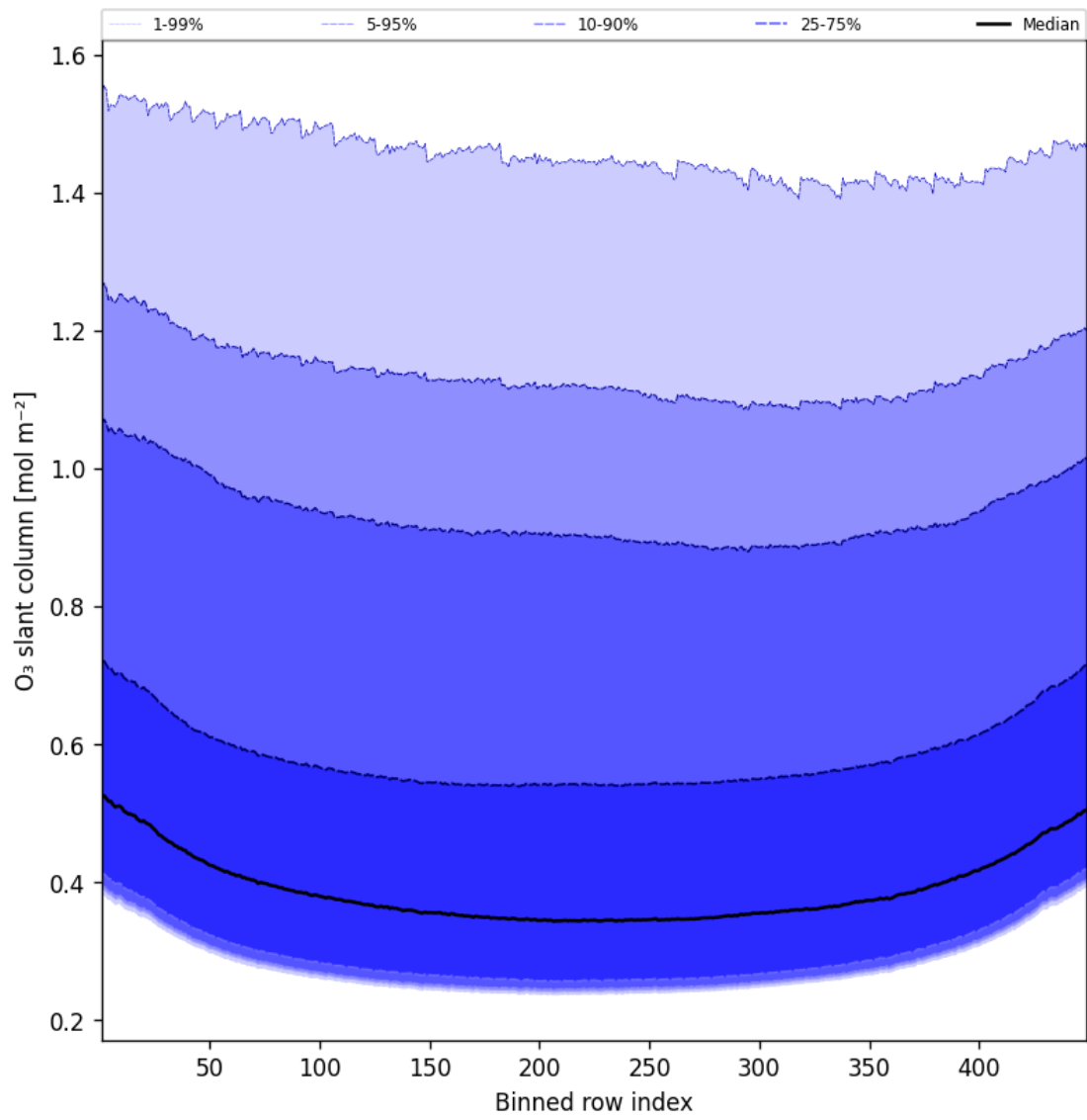
Figure 43: Along track statistics of “O 3 slant column” for 2025-01-16 to 2025-01-17
