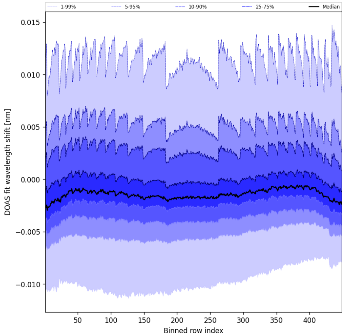
Figure 47: Along track statistics of “DOAS fit wavelength shift” for 2025-01-16 to 2025-01-17
