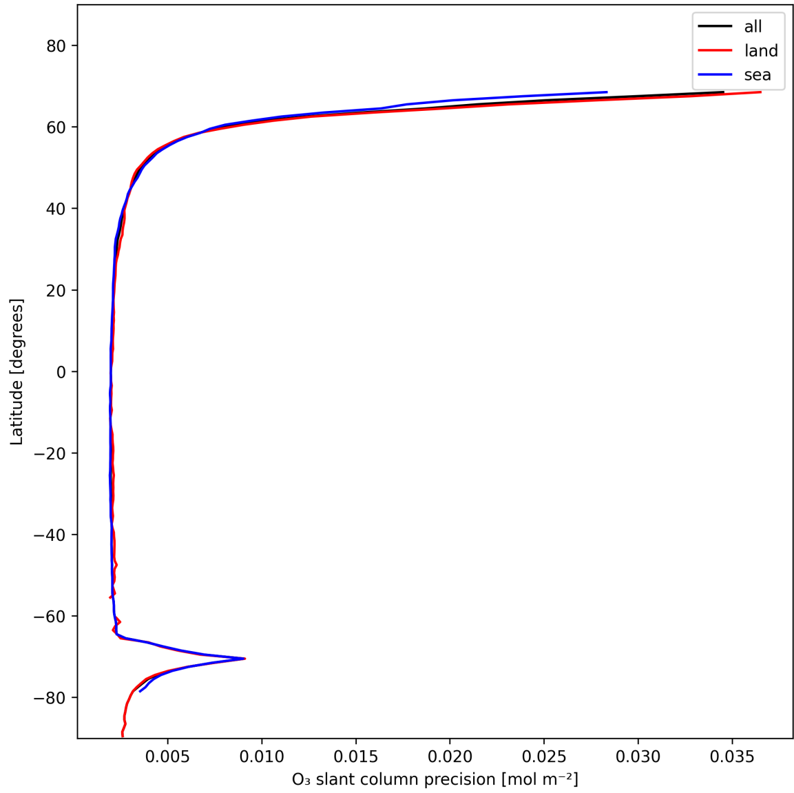
Figure 20: Zonal average of “O 3 slant column precision” for 2025-01-16 to 2025-01-17.
