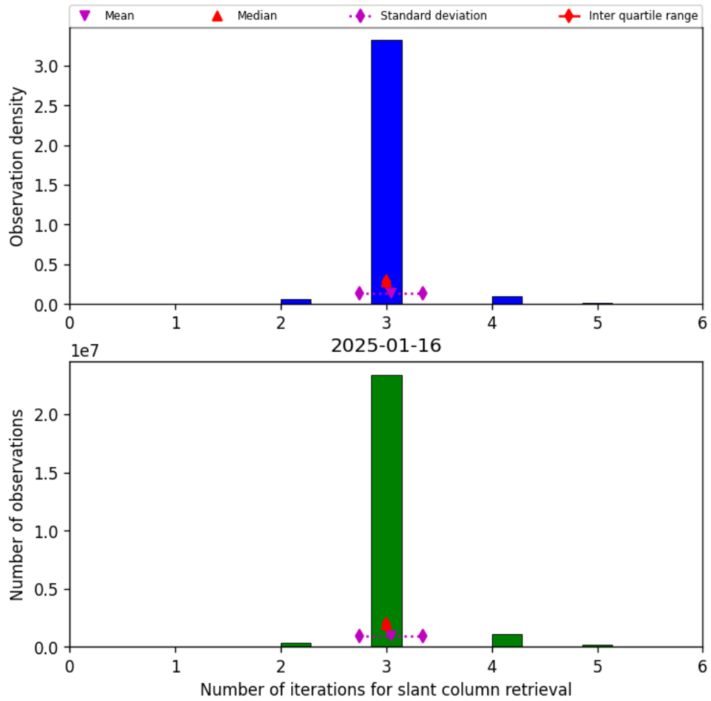
Figure 33: Histogram of “Number of iterations for slant column retrieval” for 2025-01-16 to 2025-01-17
