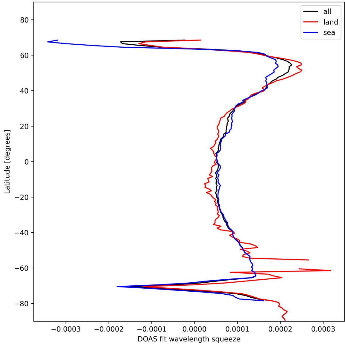
Figure 24: Zonal average of “DOAS fit wavelength squeeze” for 2025-01-16 to 2025-01-17.
