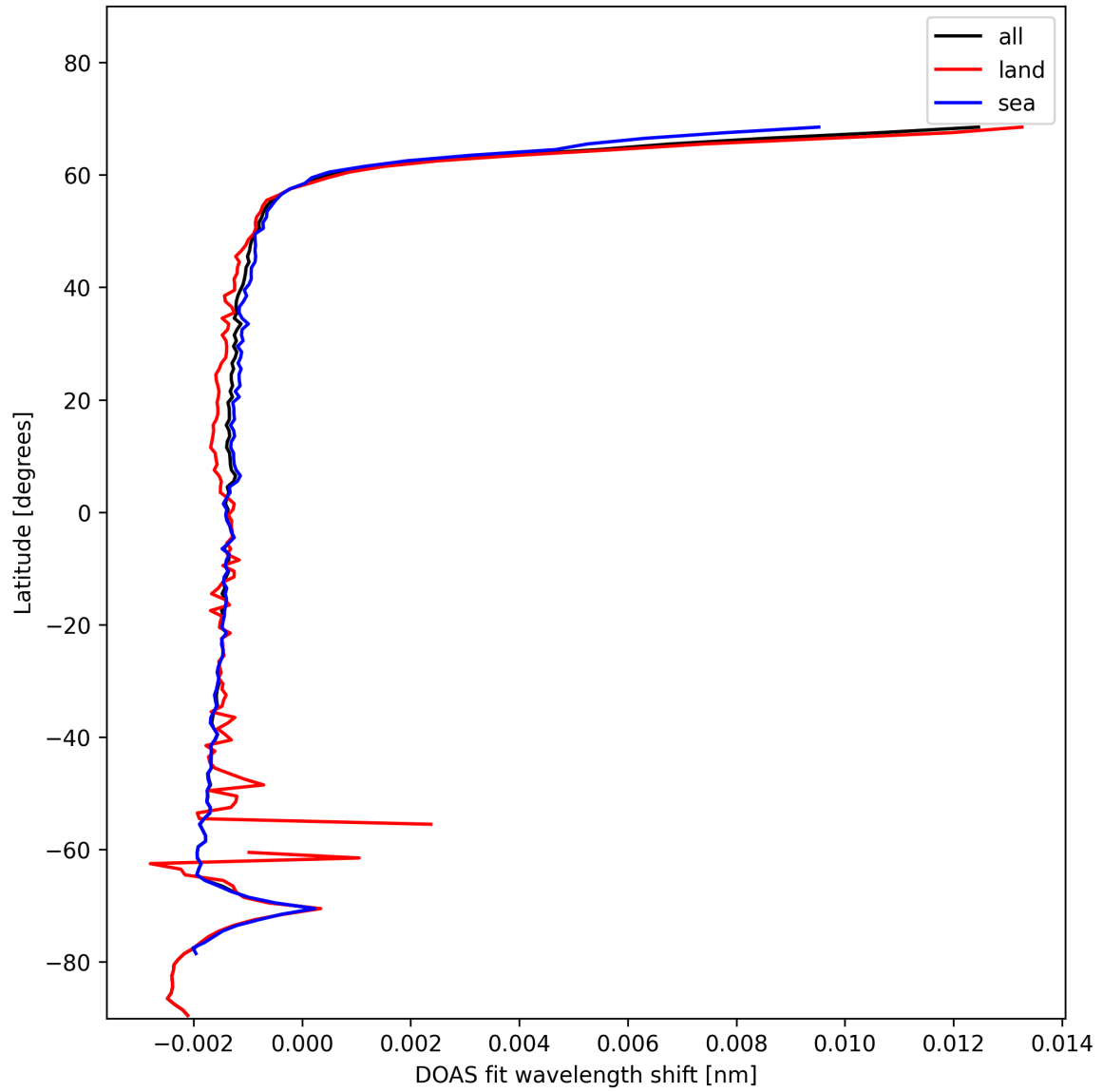
Figure 23: Zonal average of “DOAS fit wavelength shift” for 2025-01-16 to 2025-01-17.
