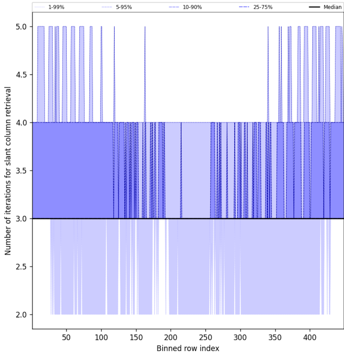
Figure 45: Along track statistics of “Number of iterations for slant column retrieval” for 2025-01-16 to 2025-01-17
