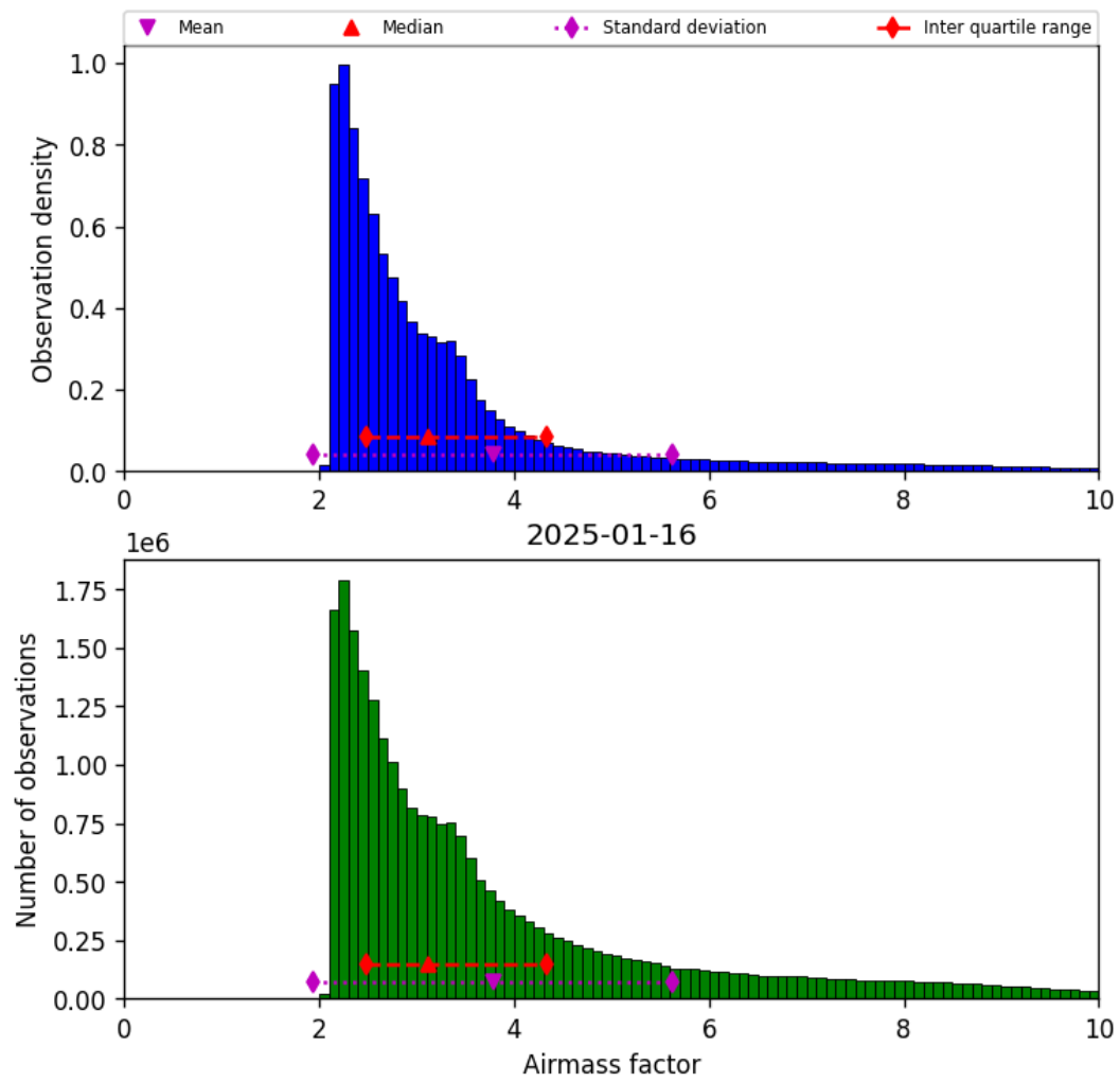
Figure 37: Histogram of “Airmass factor” for 2025-01-16 to 2025-01-17
