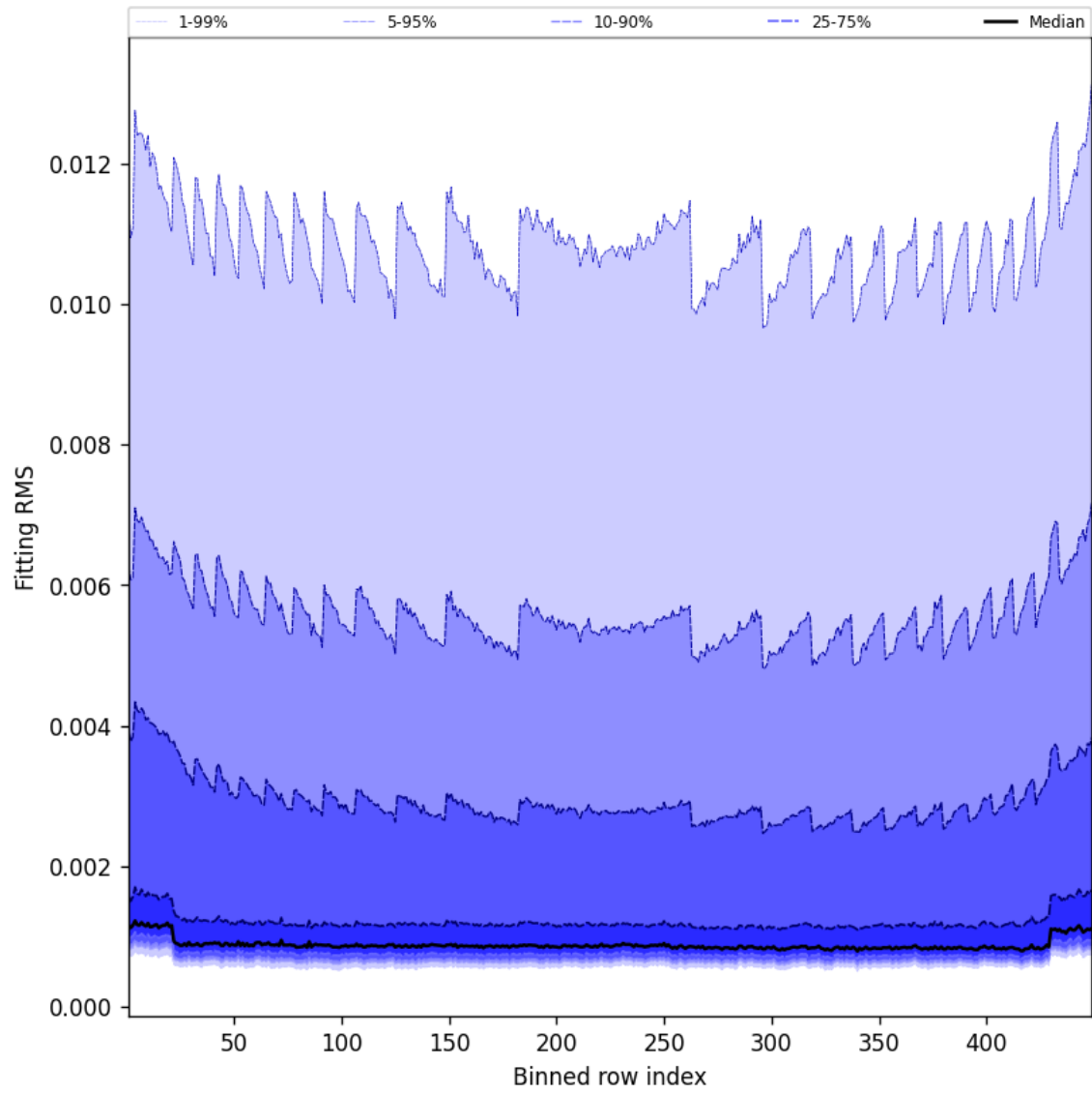
Figure 46: Along track statistics of “Fitting RMS” for 2025-01-16 to 2025-01-17
