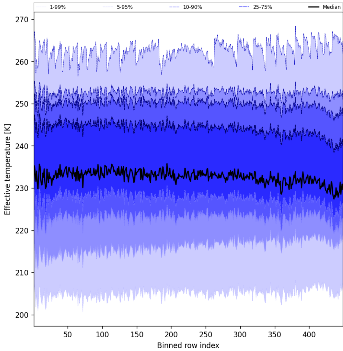
Figure 50: Along track statistics of “Effective temperature” for 2025-01-16 to 2025-01-17
