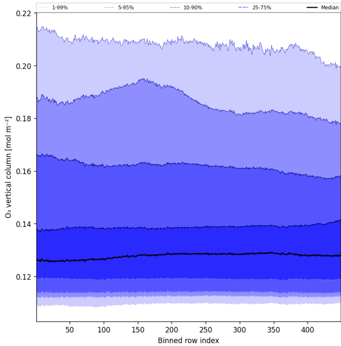
Figure 41: Along track statistics of “O 3 vertical column” for 2025-01-16 to 2025-01-17
