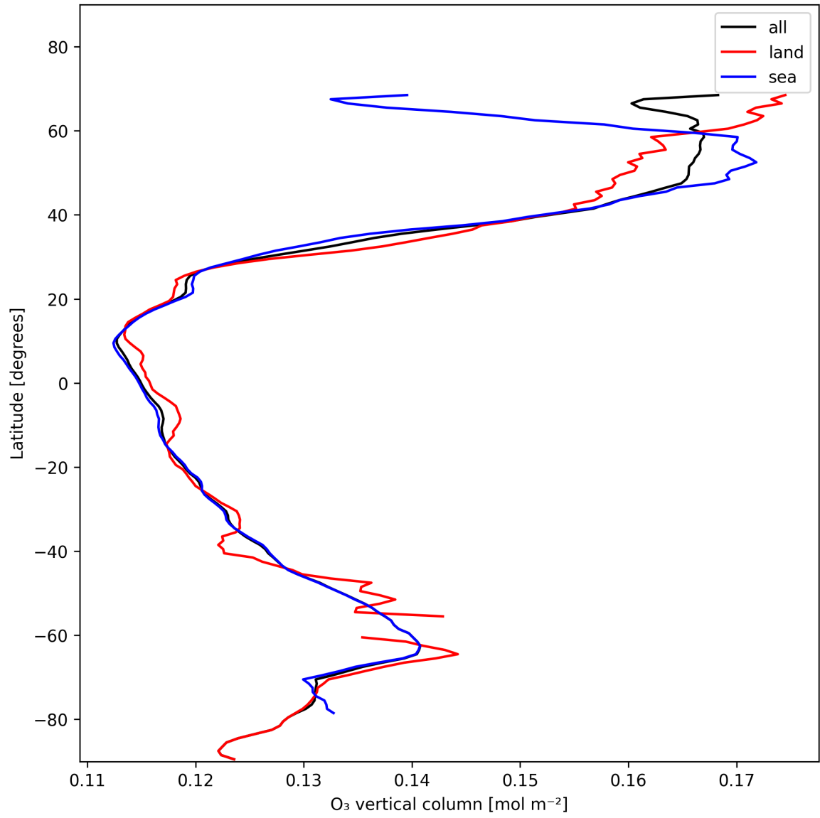
Figure 17: Zonal average of “O 3 vertical column” for 2025-01-16 to 2025-01-17.
