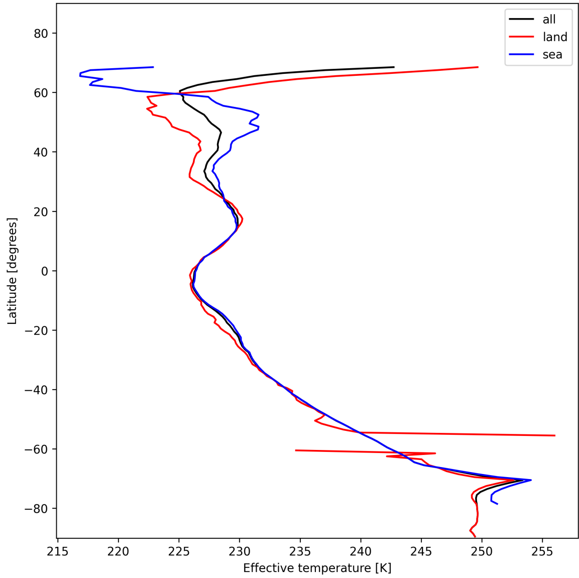
Figure 26: Zonal average of “Effective temperature” for 2025-01-16 to 2025-01-17.
