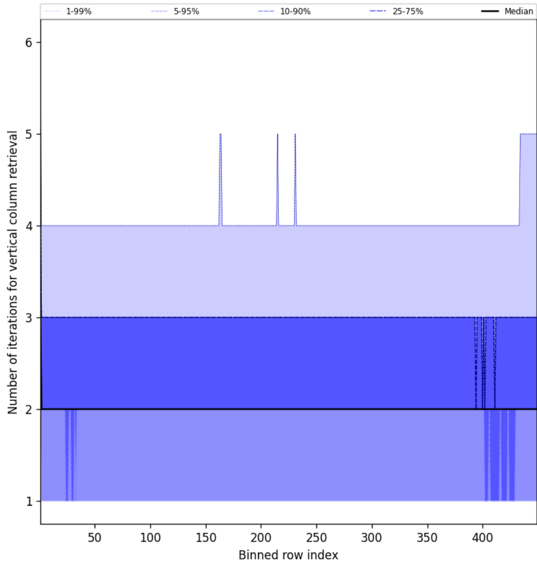
Figure 51: Along track statistics of “Number of iterations for vertical column retrieval” for 2025-01-16 to 2025-01-17
