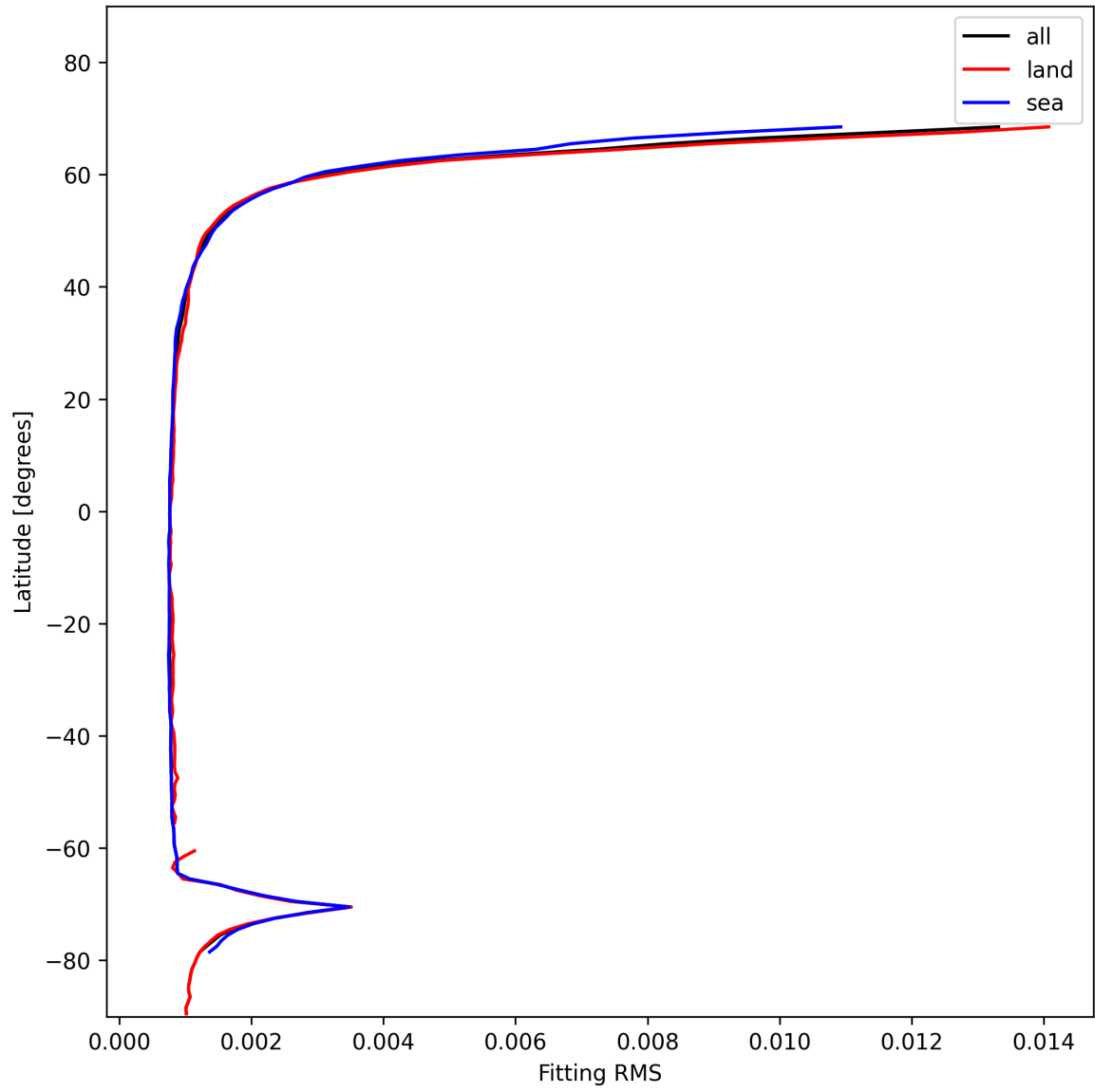
Figure 22: Zonal average of “Fitting RMS” for 2025-01-16 to 2025-01-17.
