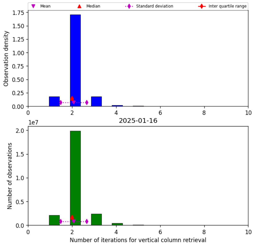
Figure 39: Histogram of “Number of iterations for vertical column retrieval” for 2025-01-16 to 2025-01-17
