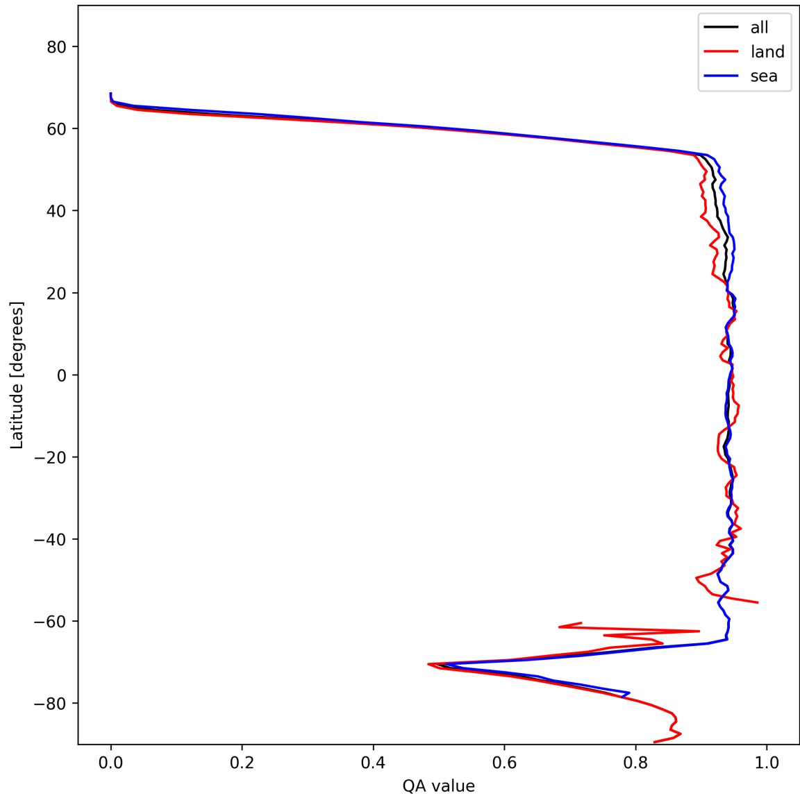
Figure 16: Zonal average of “QA value” for 2025-01-16 to 2025-01-17.
