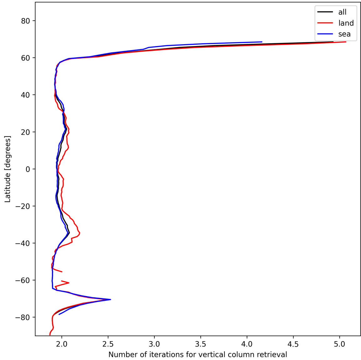
Figure 27: Zonal average of “Number of iterations for vertical column retrieval” for 2025-01-16 to 2025-01-17.
