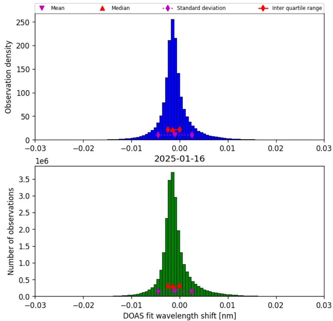
Figure 35: Histogram of “DOAS fit wavelength shift” for 2025-01-16 to 2025-01-17
