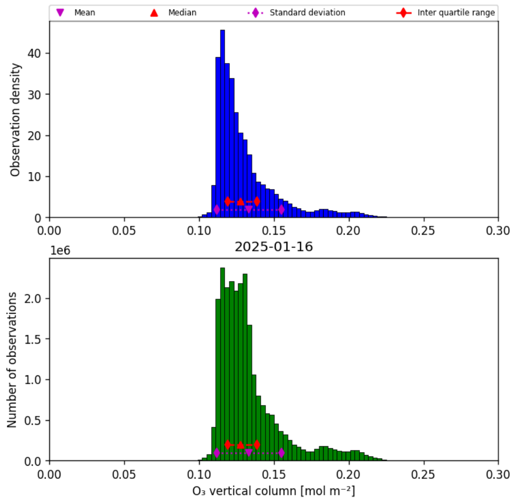
Figure 29: Histogram of “O 3 vertical column” for 2025-01-16 to 2025-01-17
