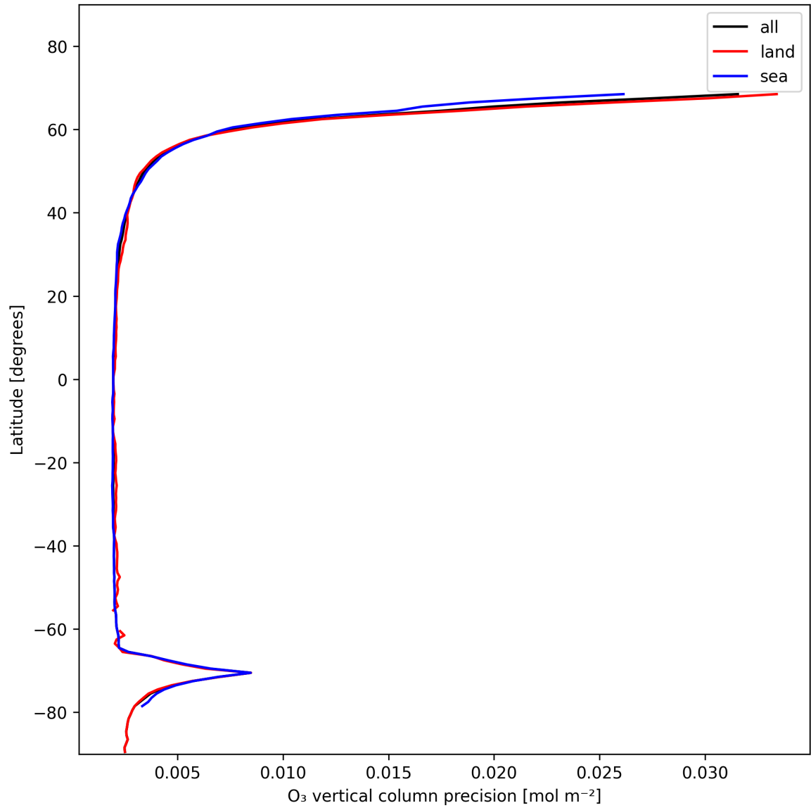
Figure 18: Zonal average of “O 3 vertical column precision” for 2025-01-16 to 2025-01-17.
