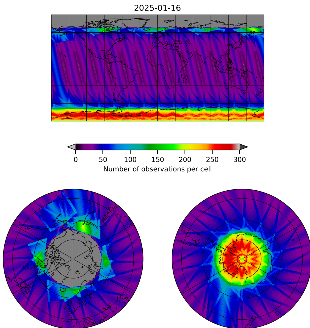
Figure 15: Map of the number of observations for 2025-01-16 to 2025-01-17
