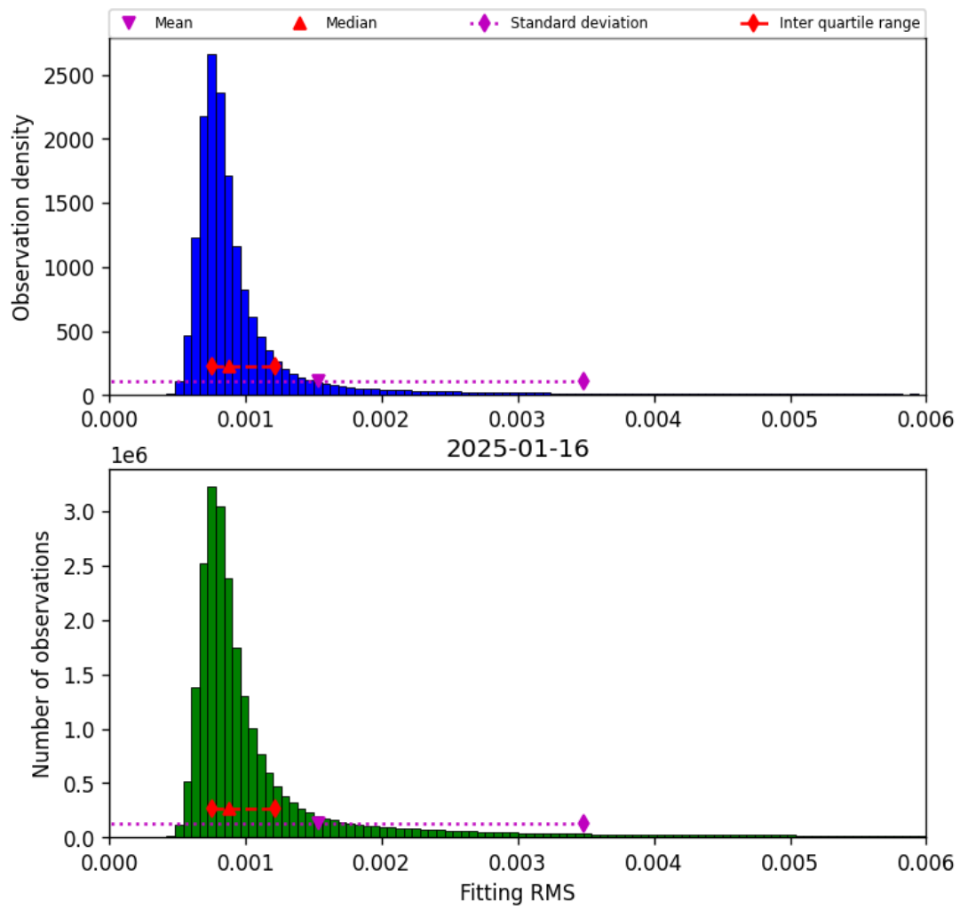
Figure 34: Histogram of “Fitting RMS” for 2025-01-16 to 2025-01-17
