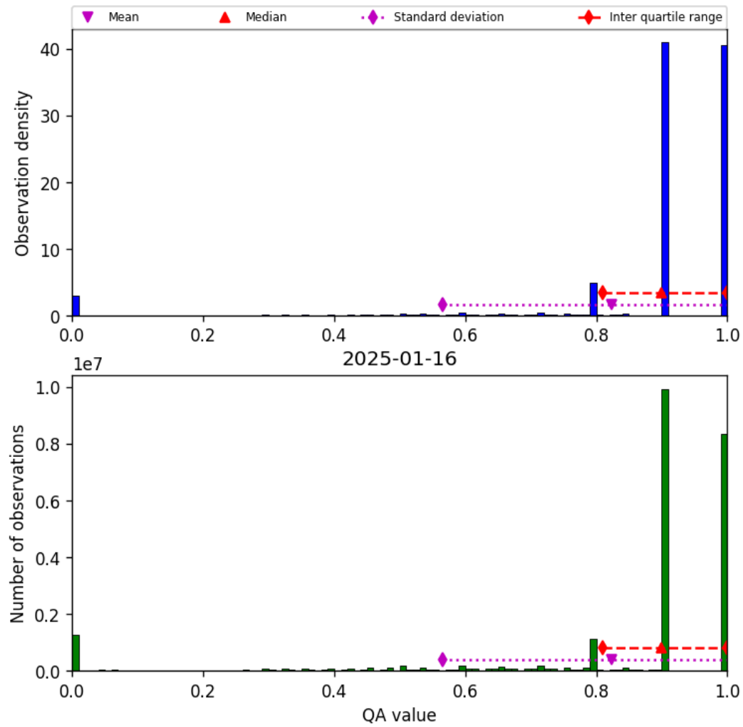
Figure 28: Histogram of “QA value” for 2025-01-16 to 2025-01-17
