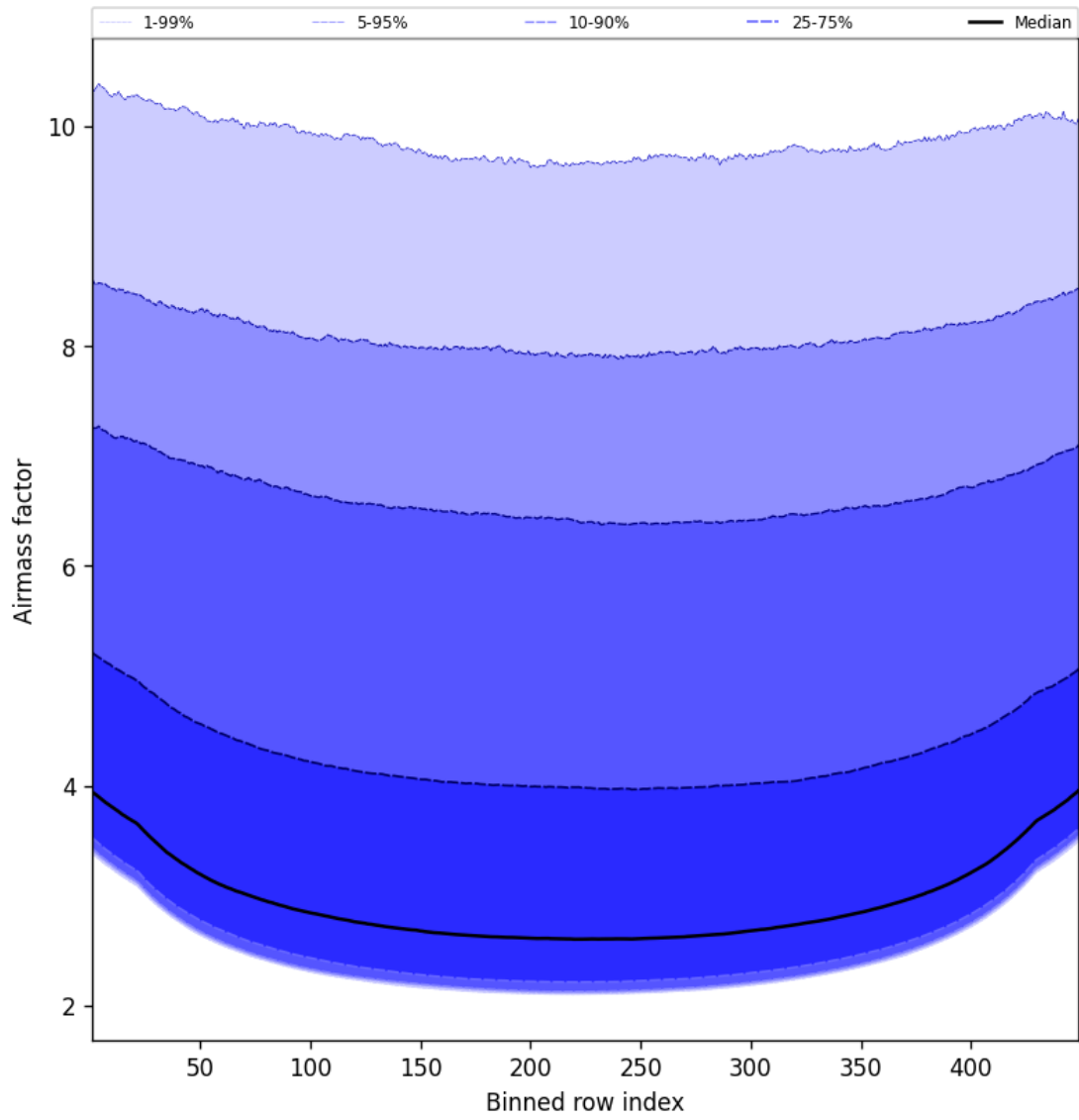
Figure 49: Along track statistics of “Airmass factor” for 2025-01-16 to 2025-01-17
