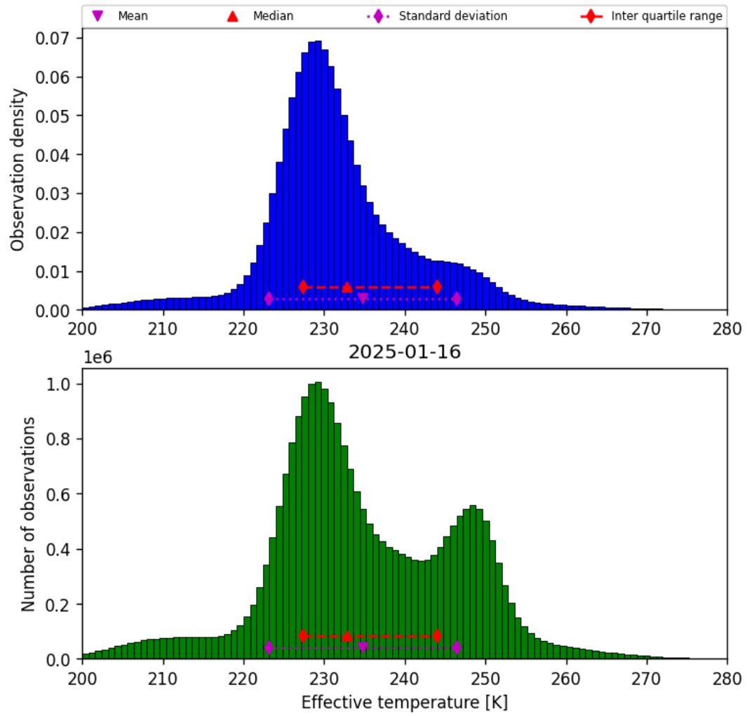
Figure 38: Histogram of “Effective temperature” for 2025-01-16 to 2025-01-17
