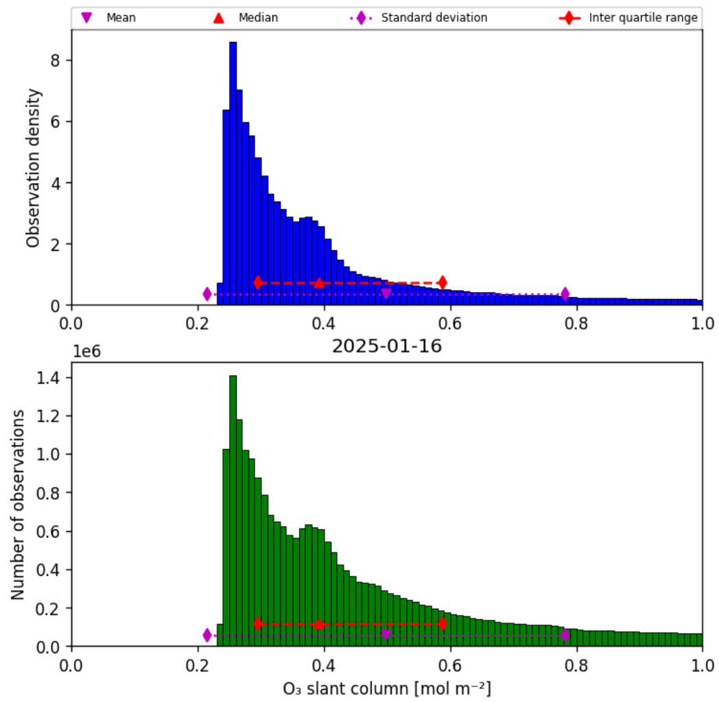
Figure 31: Histogram of “O 3 slant column” for 2025-01-16 to 2025-01-17
