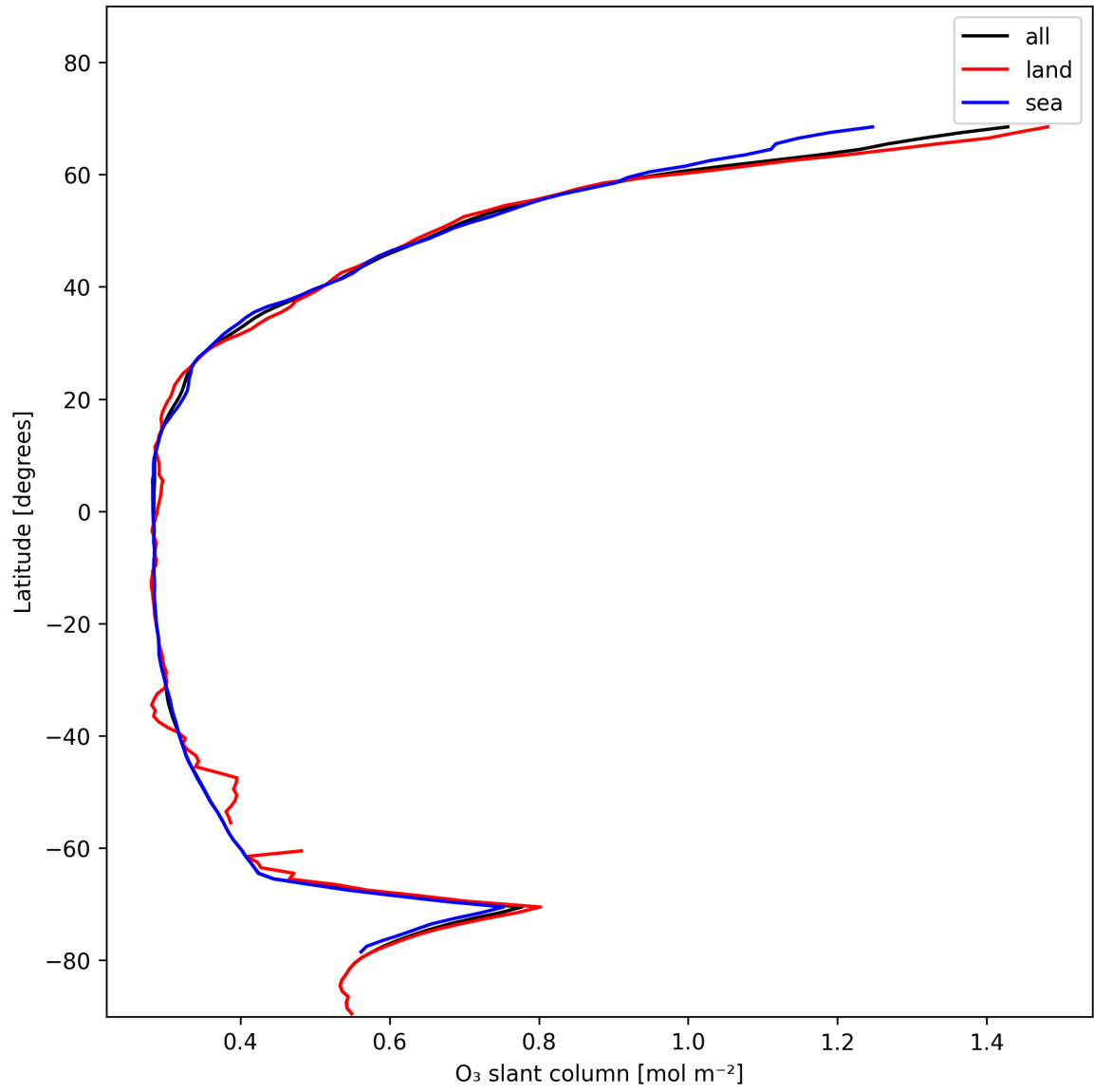
Figure 19: Zonal average of “O 3 slant column” for 2025-01-16 to 2025-01-17.
