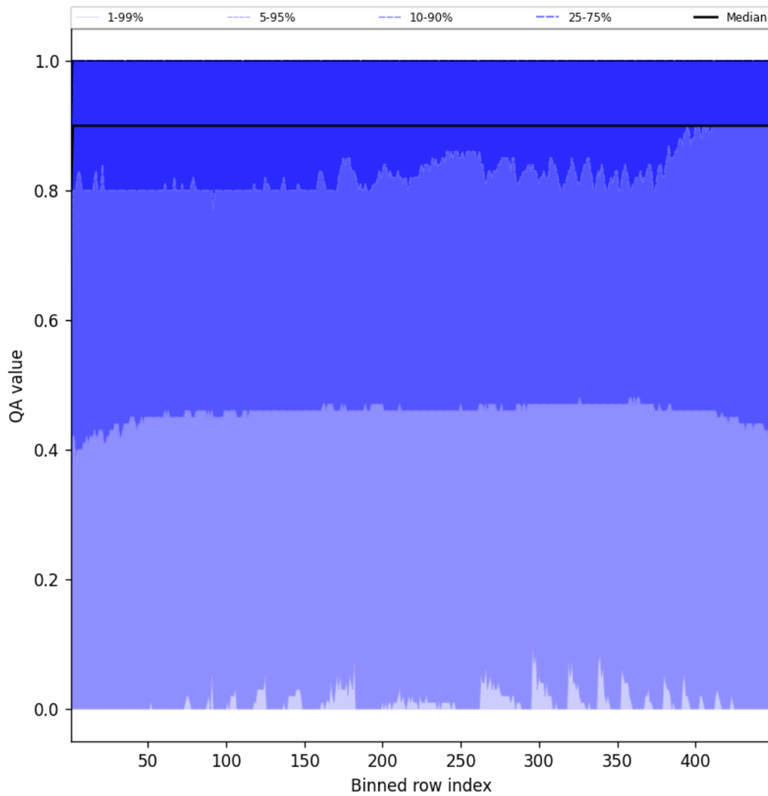
Figure 40: Along track statistics of “QA value” for 2025-01-16 to 2025-01-17
