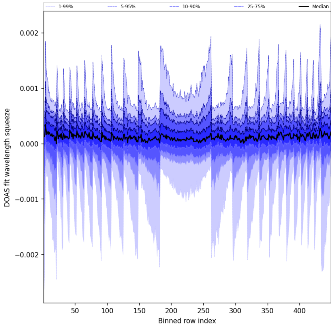
Figure 48: Along track statistics of “DOAS fit wavelength squeeze” for 2025-01-16 to 2025-01-17
