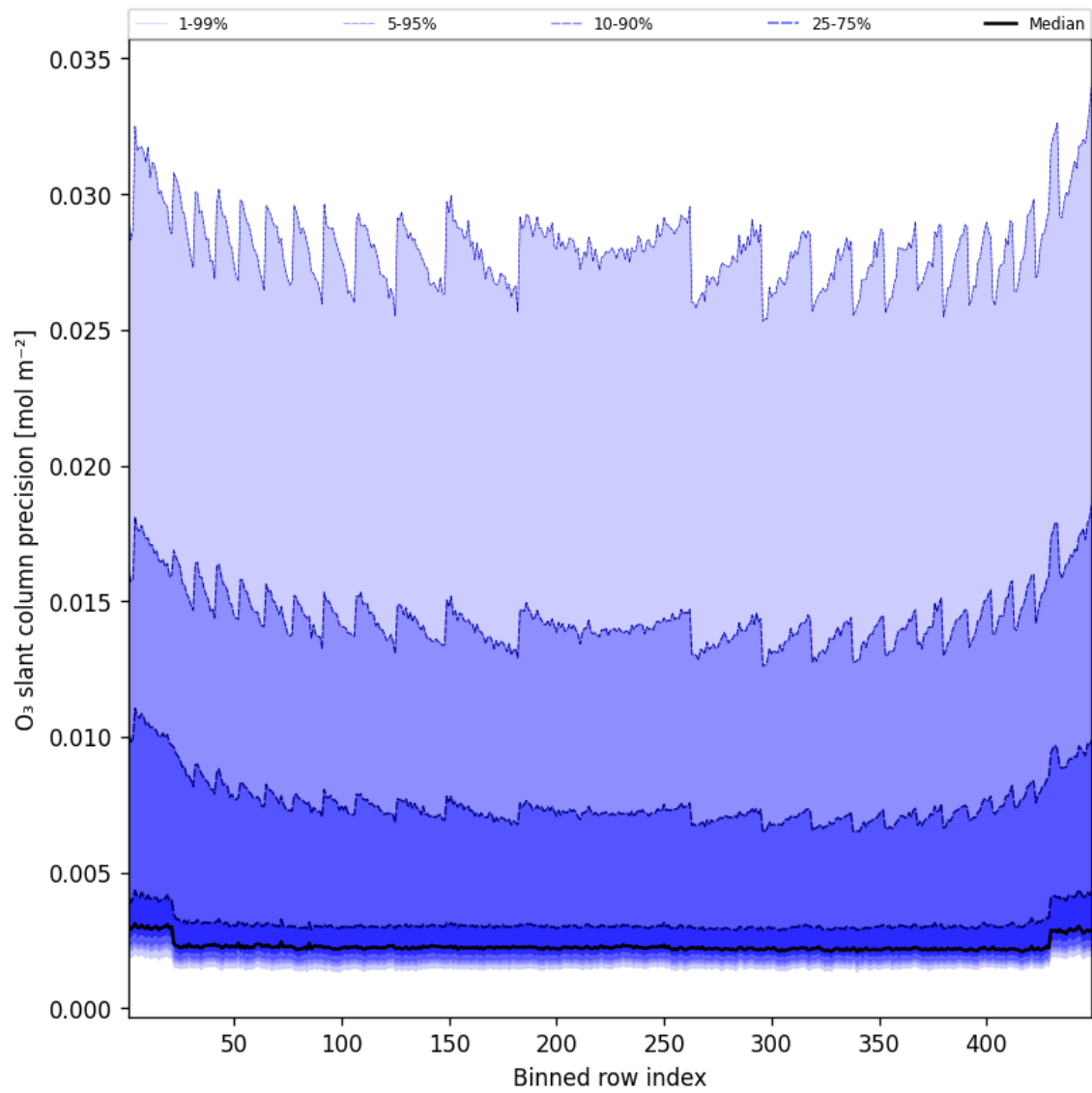
Figure 44: Along track statistics of “O 3 slant column precision” for 2025-01-16 to 2025-01-17
