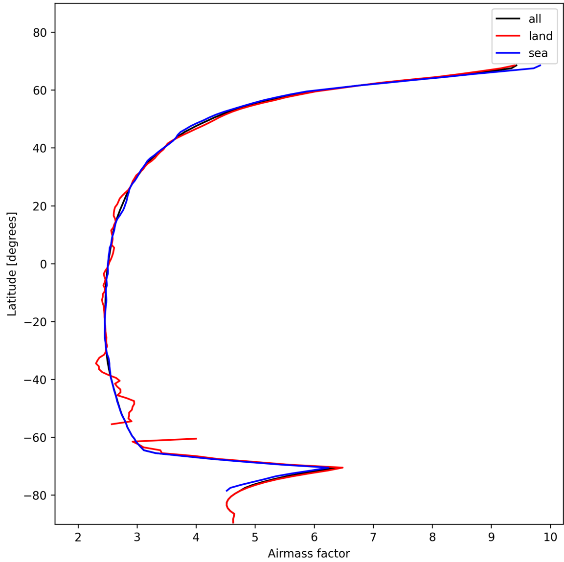
Figure 25: Zonal average of “Airmass factor” for 2025-01-16 to 2025-01-17.
