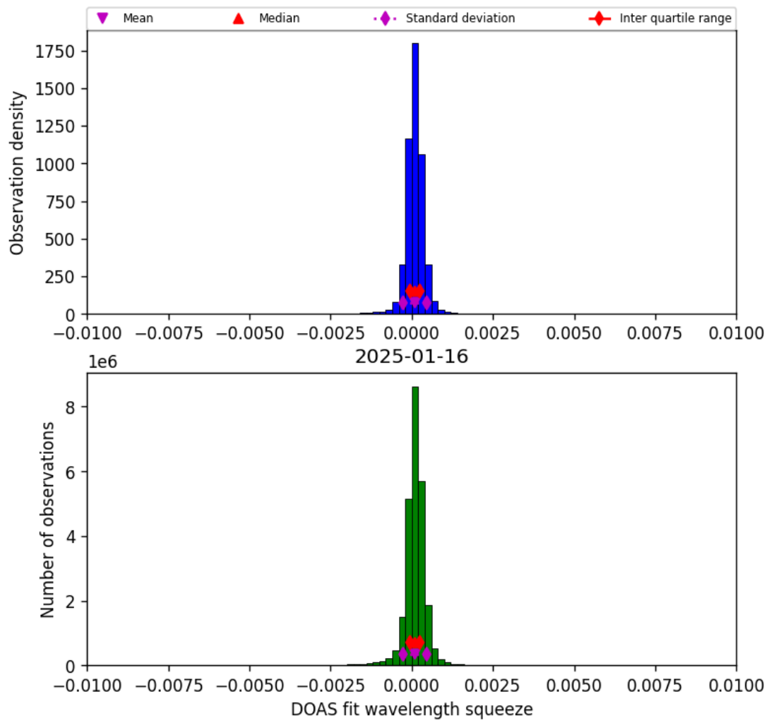
Figure 36: Histogram of “DOAS fit wavelength squeeze” for 2025-01-16 to 2025-01-17
