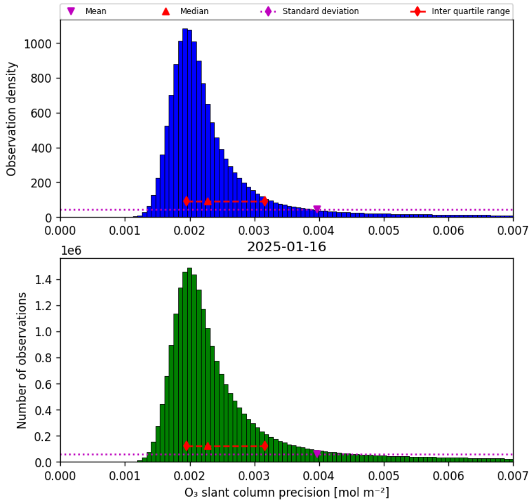
Figure 32: Histogram of “O 3 slant column precision” for 2025-01-16 to 2025-01-17
