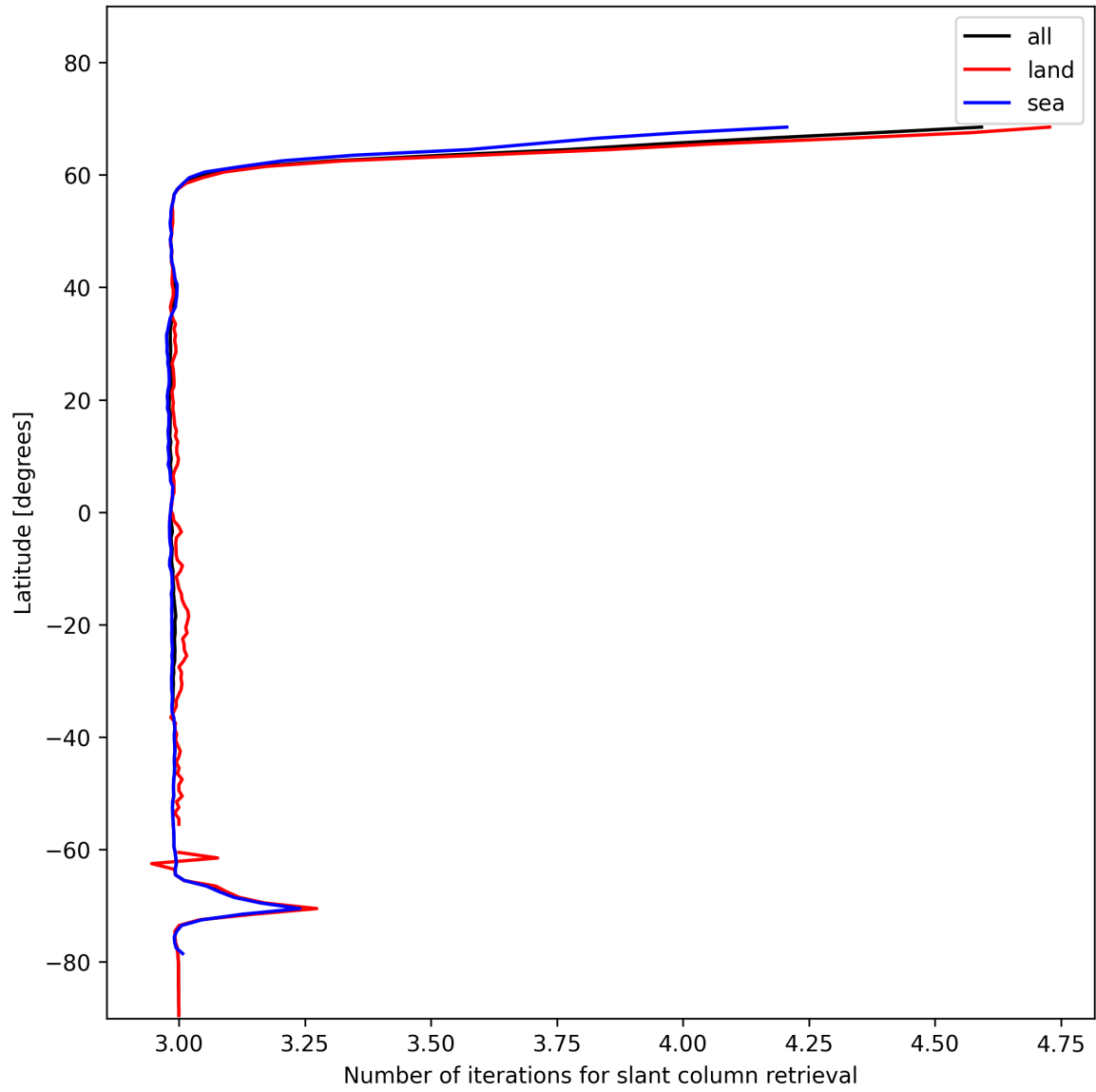
Figure 21: Zonal average of “Number of iterations for slant column retrieval” for 2025-01-16 to 2025-01-17.
