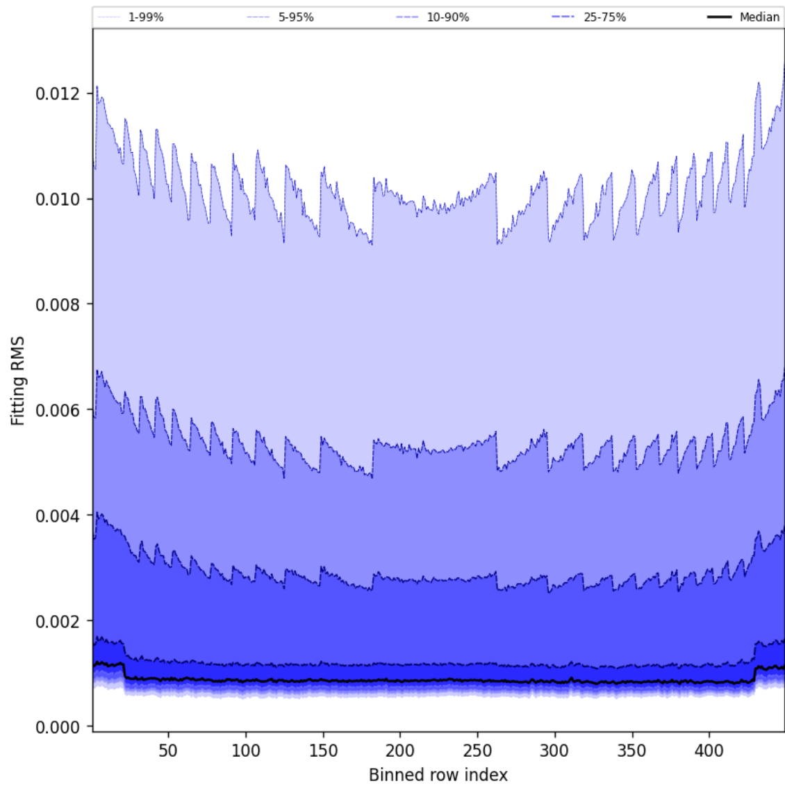
Figure 46: Along track statistics of “Fitting RMS” for 2025-01-17 to 2025-01-18
