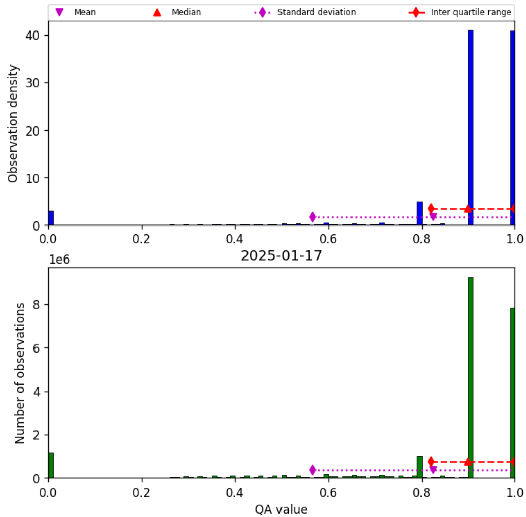
Figure 28: Histogram of “QA value” for 2025-01-17 to 2025-01-18
