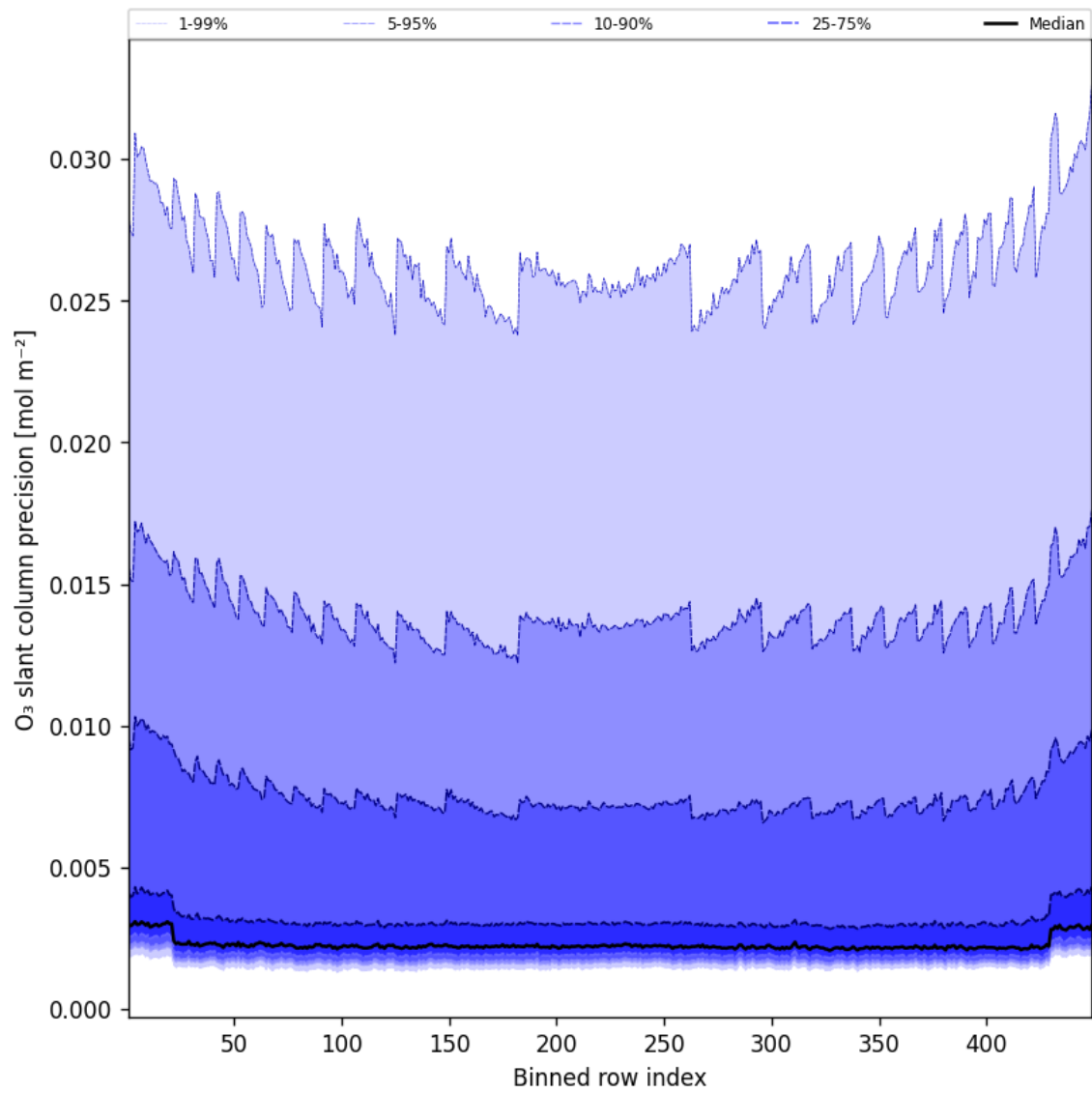
Figure 44: Along track statistics of “O 3 slant column precision” for 2025-01-17 to 2025-01-18
