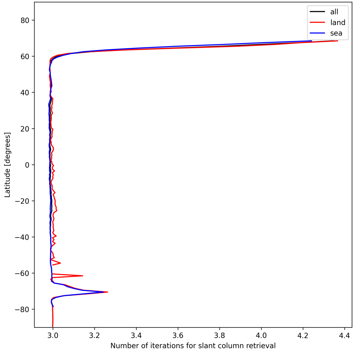
Figure 21: Zonal average of “Number of iterations for slant column retrieval” for 2025-01-17 to 2025-01-18.
