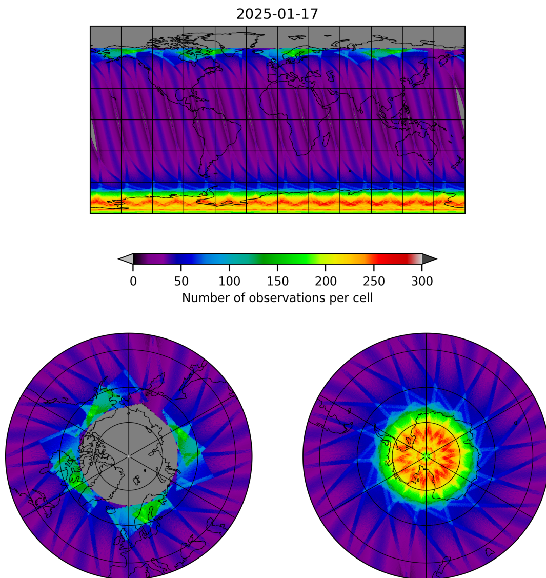
Figure 15: Map of the number of observations for 2025-01-17 to 2025-01-18
