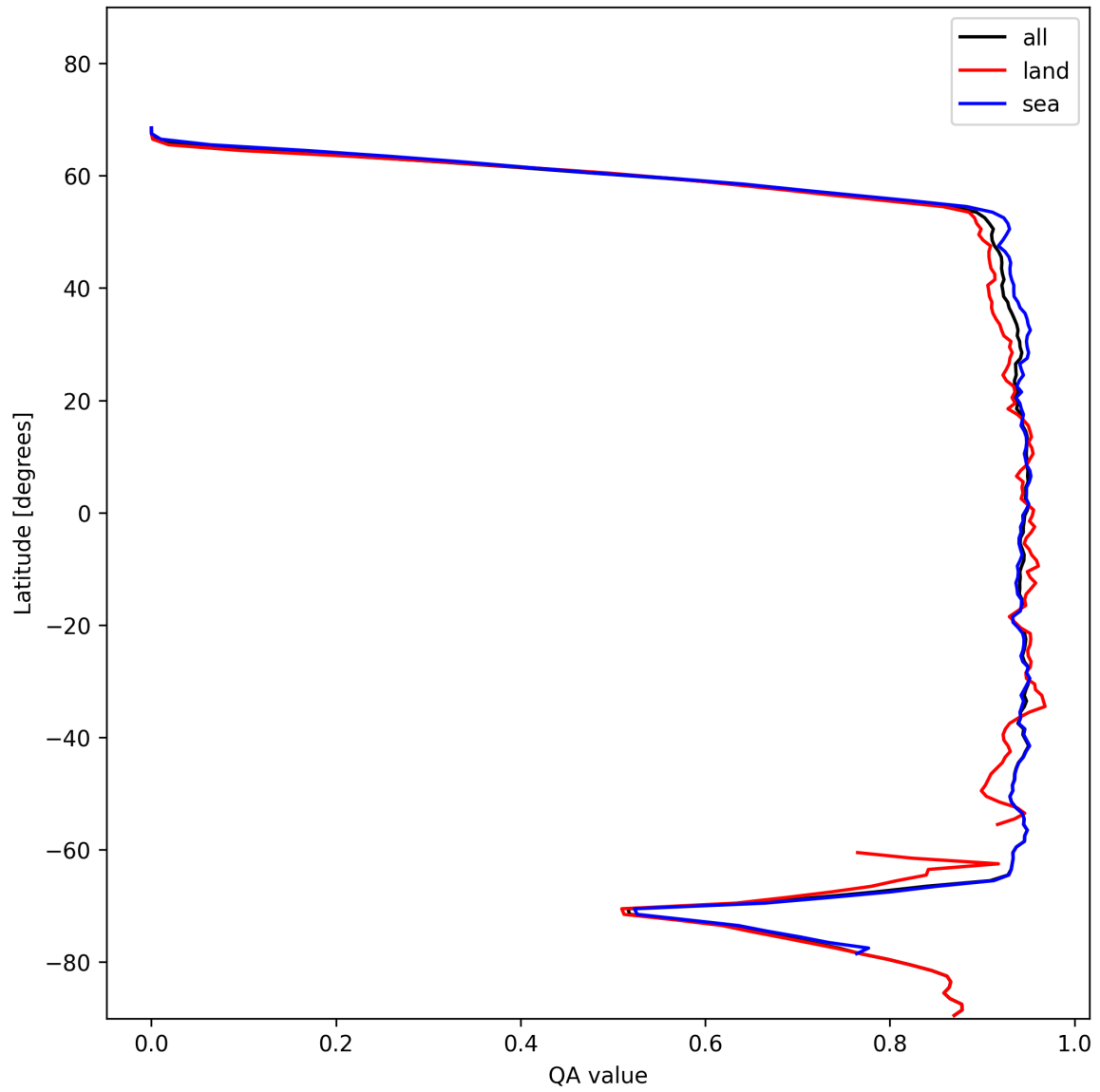
Figure 16: Zonal average of “QA value” for 2025-01-17 to 2025-01-18.
