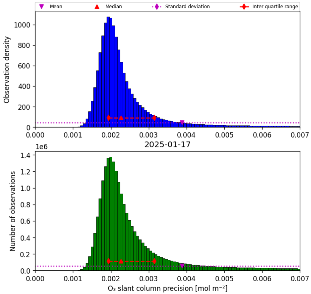
Figure 32: Histogram of “O 3 slant column precision” for 2025-01-17 to 2025-01-18
