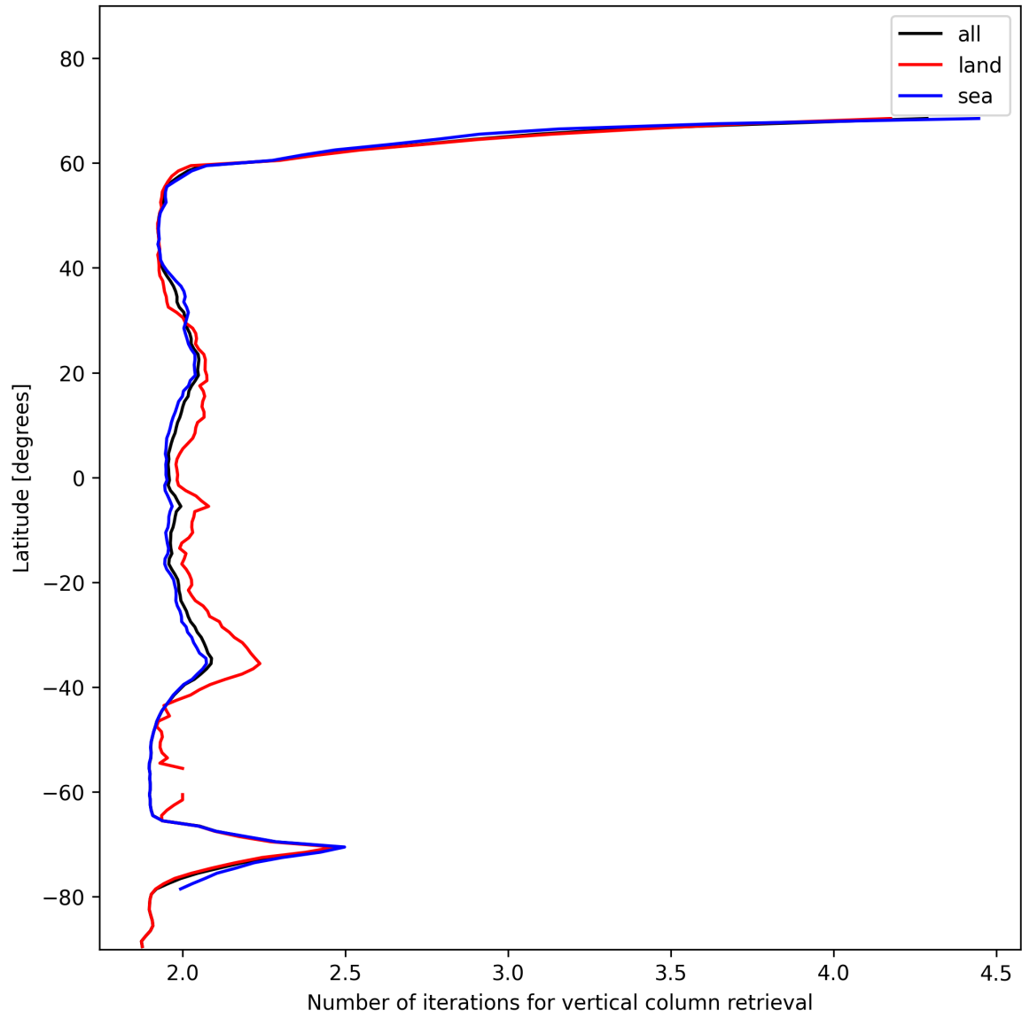
Figure 27: Zonal average of “Number of iterations for vertical column retrieval” for 2025-01-17 to 2025-01-18.
