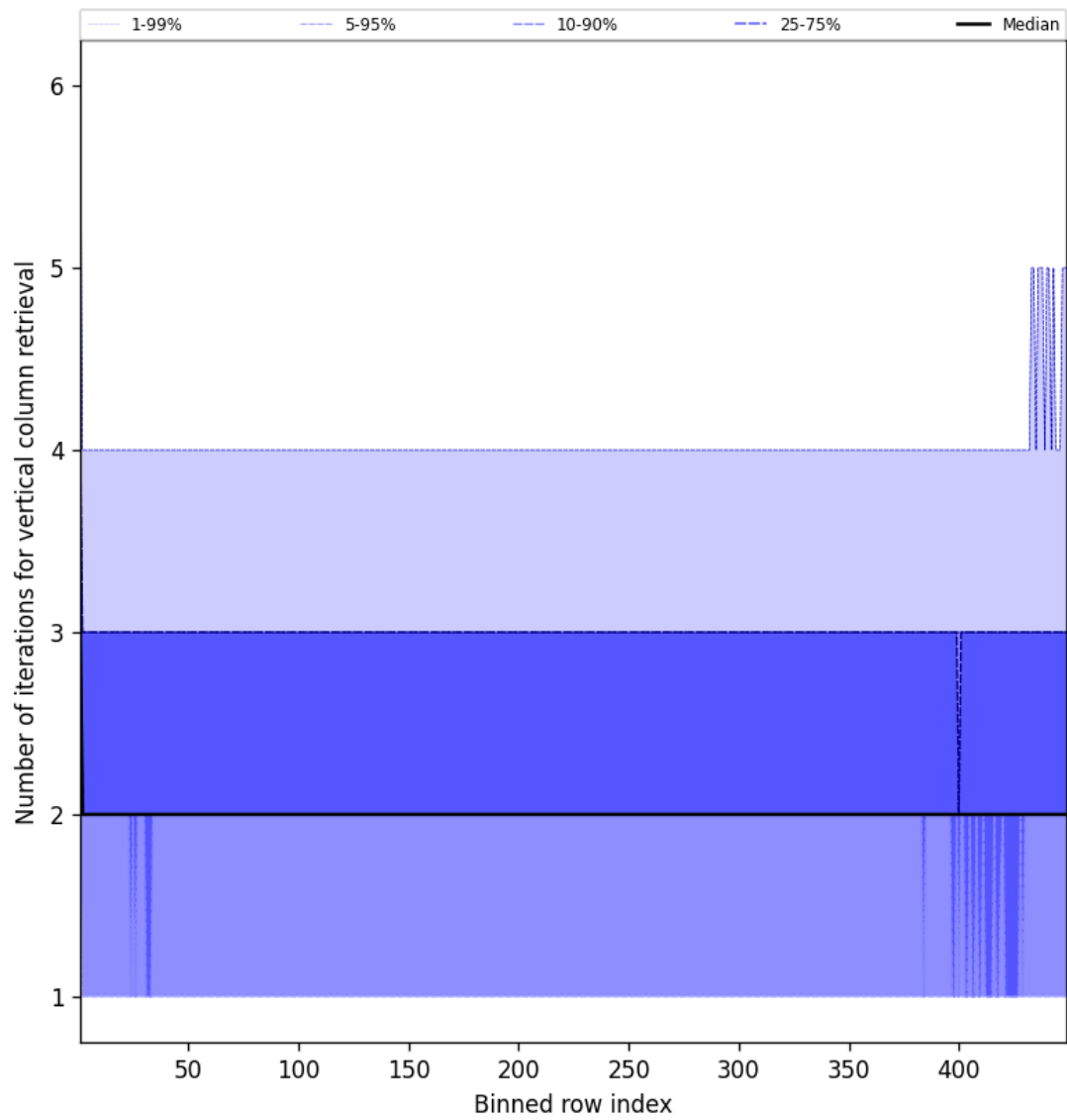
Figure 51: Along track statistics of “Number of iterations for vertical column retrieval” for 2025-01-17 to 2025-01-18
