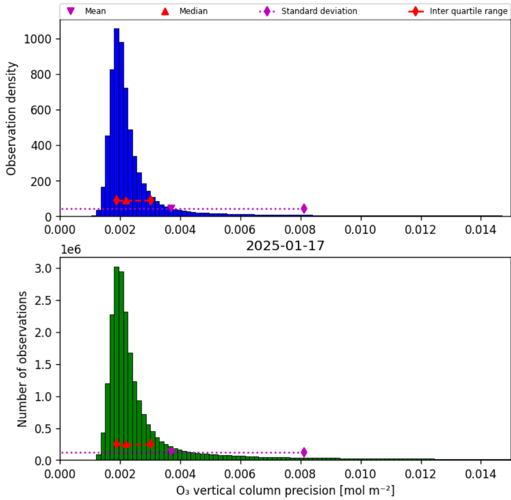
Figure 30: Histogram of “O 3 vertical column precision” for 2025-01-17 to 2025-01-18
