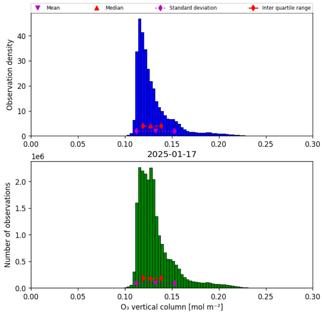
Figure 29: Histogram of “O 3 vertical column” for 2025-01-17 to 2025-01-18
