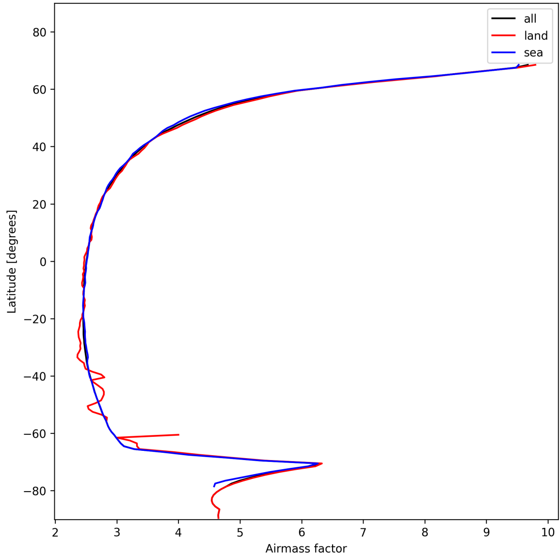
Figure 25: Zonal average of “Airmass factor” for 2025-01-17 to 2025-01-18.
