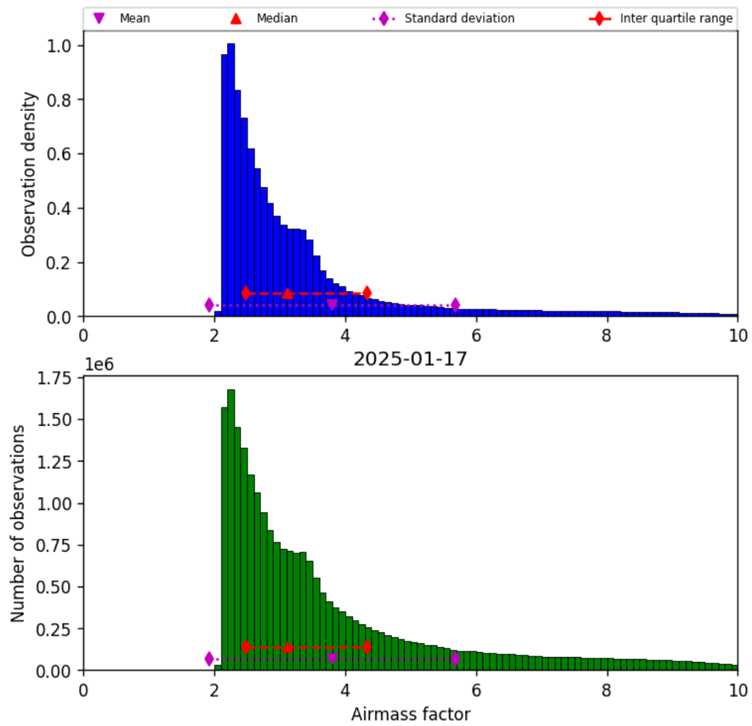
Figure 37: Histogram of “Airmass factor” for 2025-01-17 to 2025-01-18
