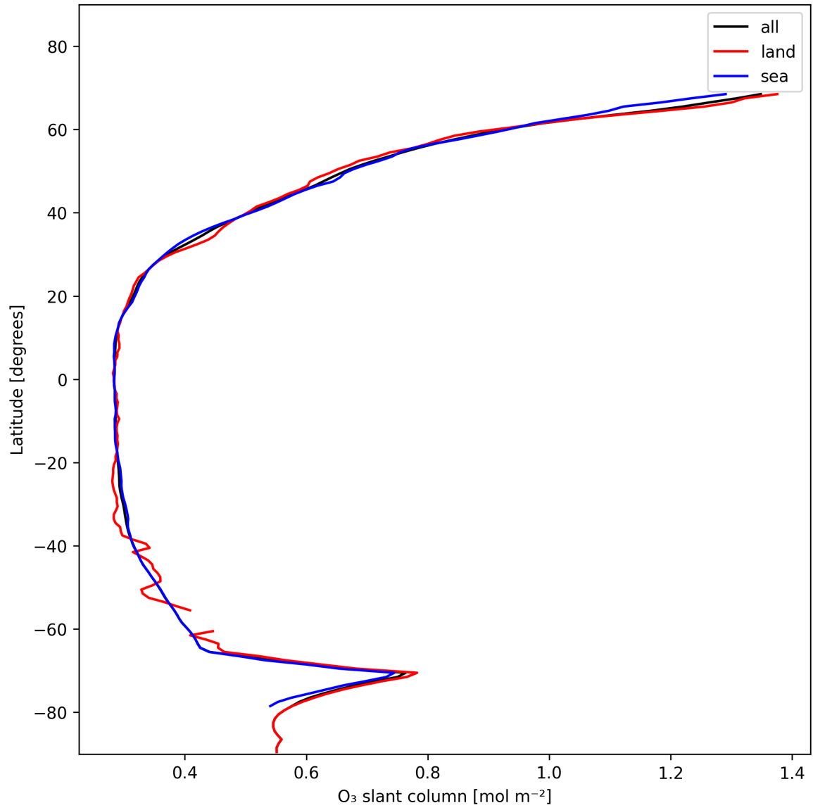
Figure 19: Zonal average of “O 3 slant column” for 2025-01-17 to 2025-01-18.
