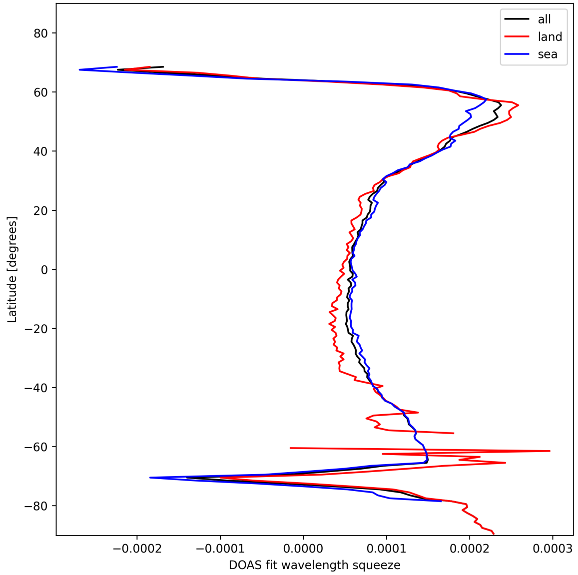
Figure 24: Zonal average of “DOAS fit wavelength squeeze” for 2025-01-17 to 2025-01-18.
