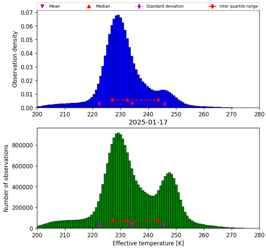
Figure 38: Histogram of “Effective temperature” for 2025-01-17 to 2025-01-18
