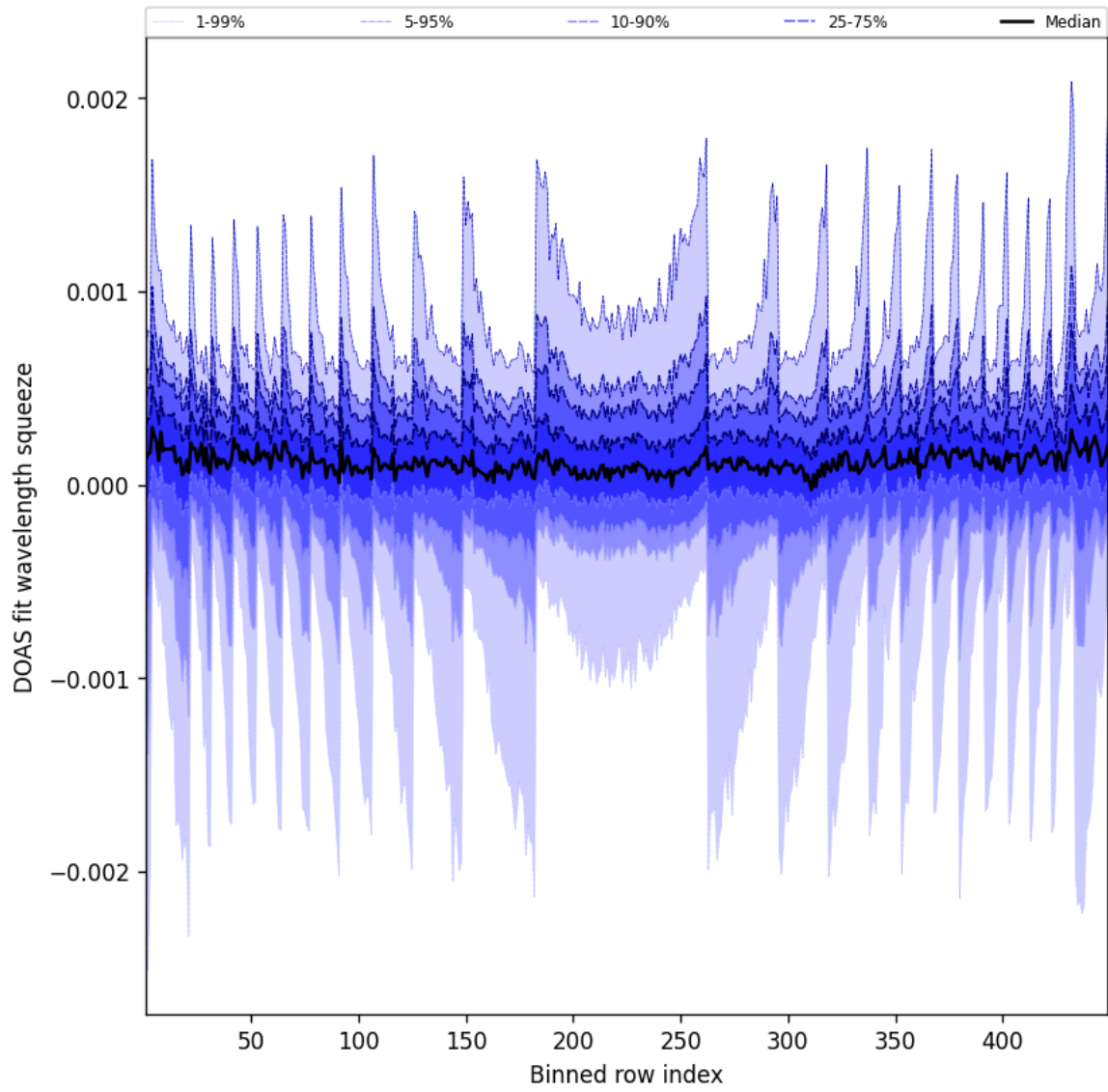
Figure 48: Along track statistics of “DOAS fit wavelength squeeze” for 2025-01-17 to 2025-01-18
