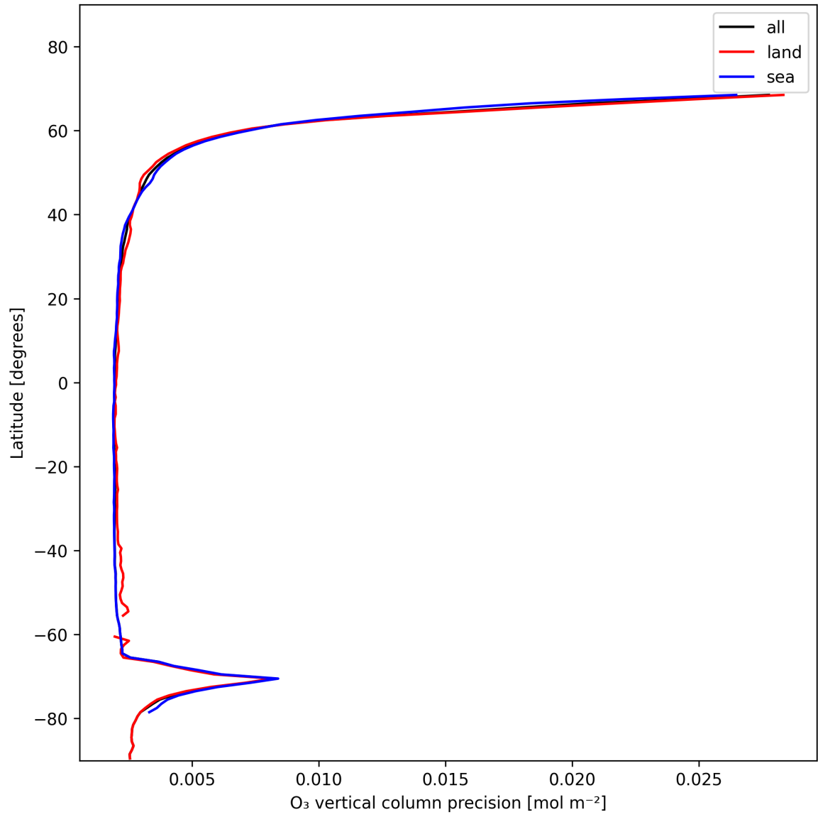
Figure 18: Zonal average of “O 3 vertical column precision” for 2025-01-17 to 2025-01-18.
