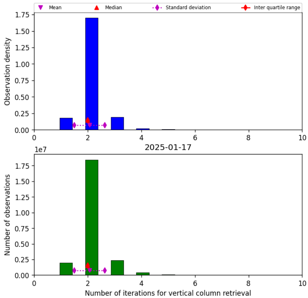
Figure 39: Histogram of “Number of iterations for vertical column retrieval” for 2025-01-17 to 2025-01-18
