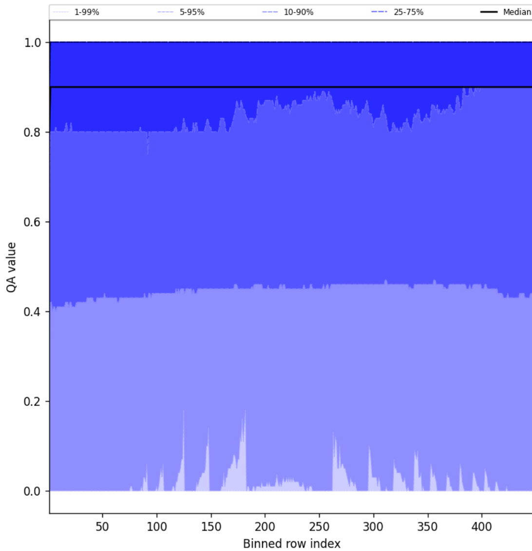
Figure 40: Along track statistics of “QA value” for 2025-01-17 to 2025-01-18
