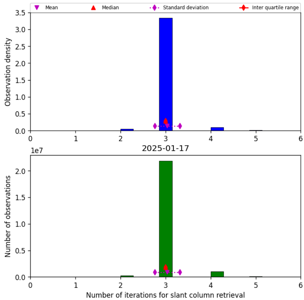
Figure 33: Histogram of “Number of iterations for slant column retrieval” for 2025-01-17 to 2025-01-18
