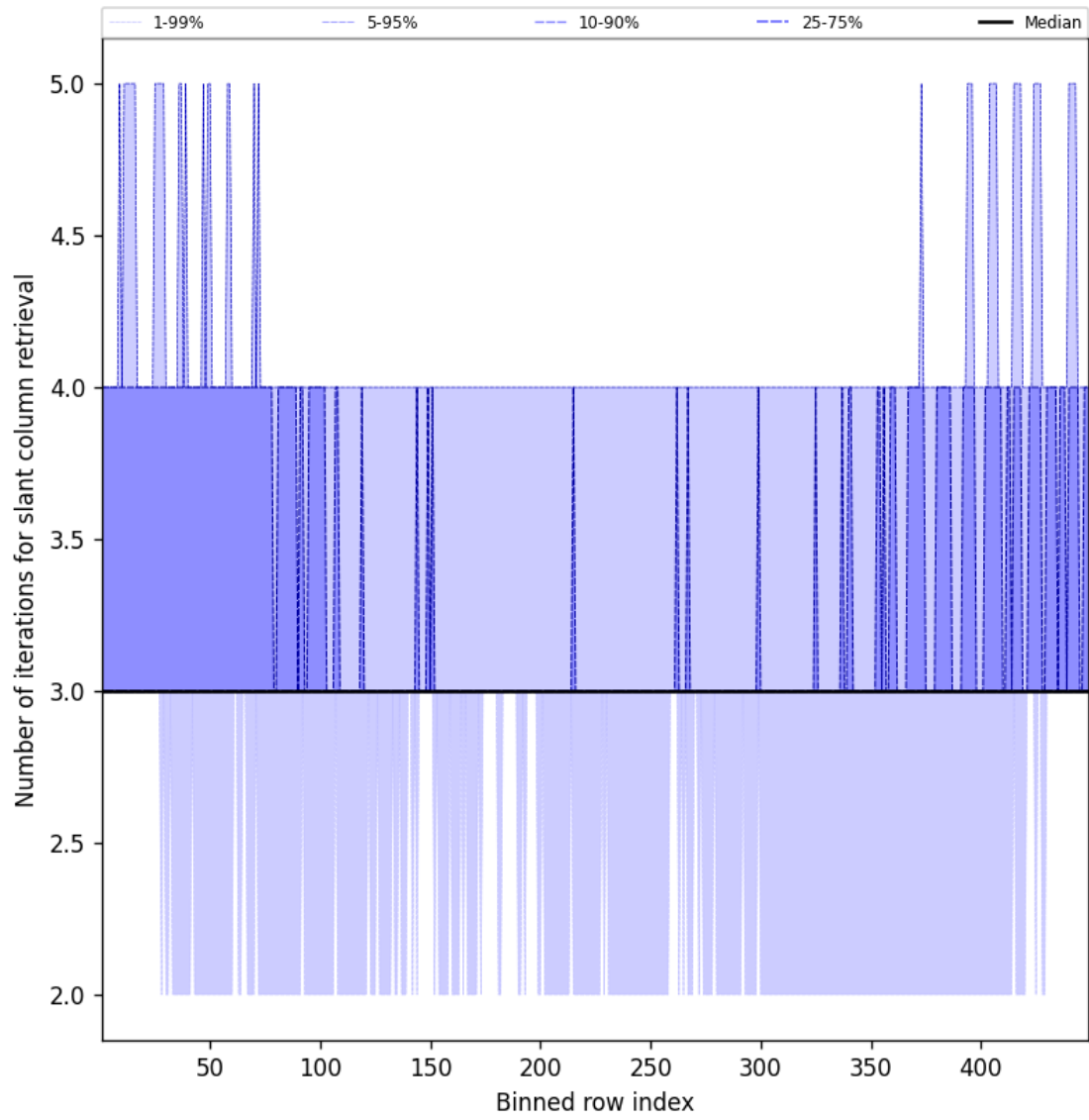
Figure 45: Along track statistics of “Number of iterations for slant column retrieval” for 2025-01-17 to 2025-01-18
