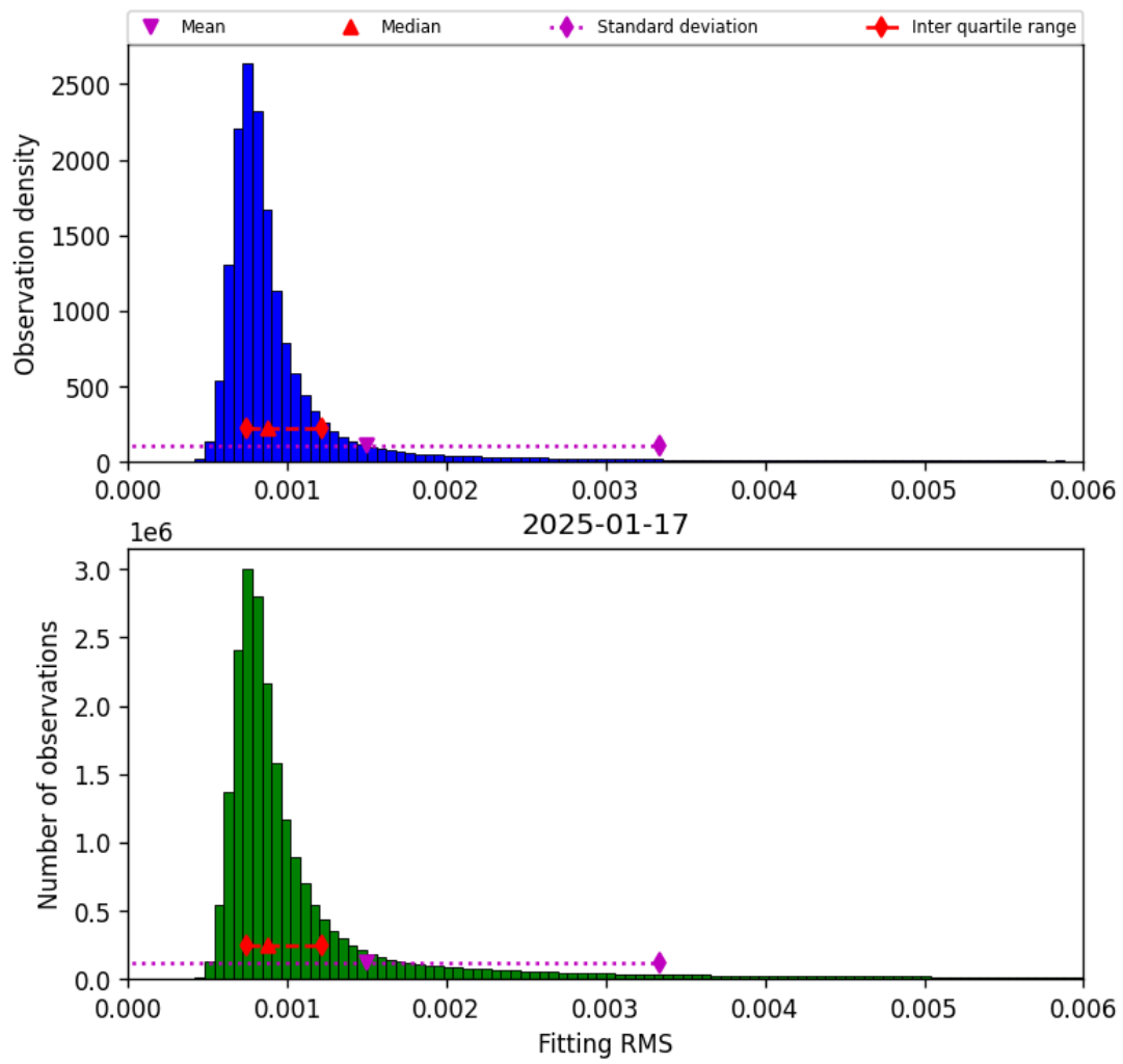
Figure 34: Histogram of “Fitting RMS” for 2025-01-17 to 2025-01-18
