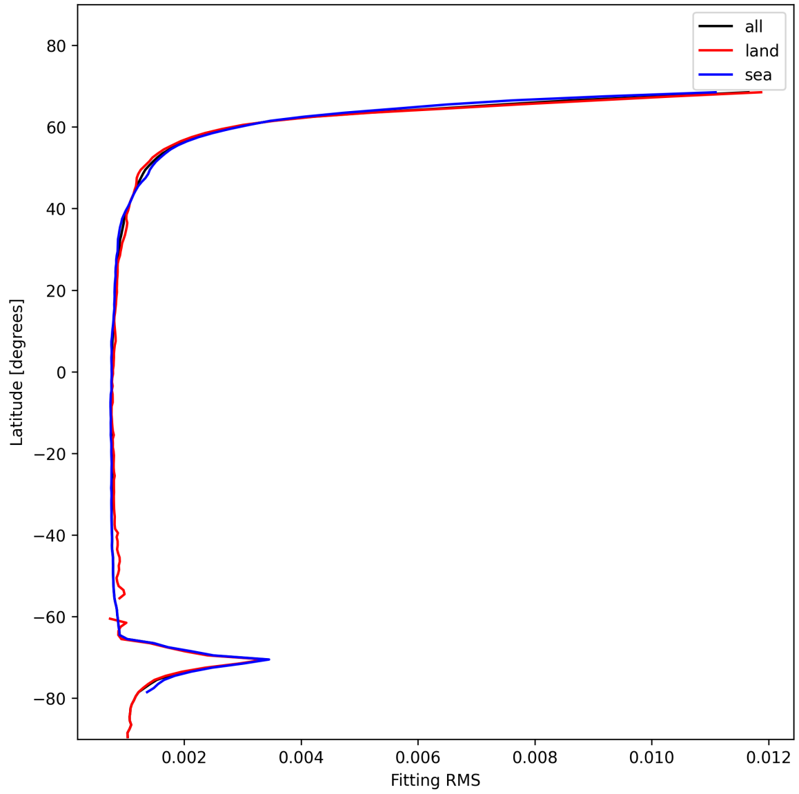
Figure 22: Zonal average of “Fitting RMS” for 2025-01-17 to 2025-01-18.
