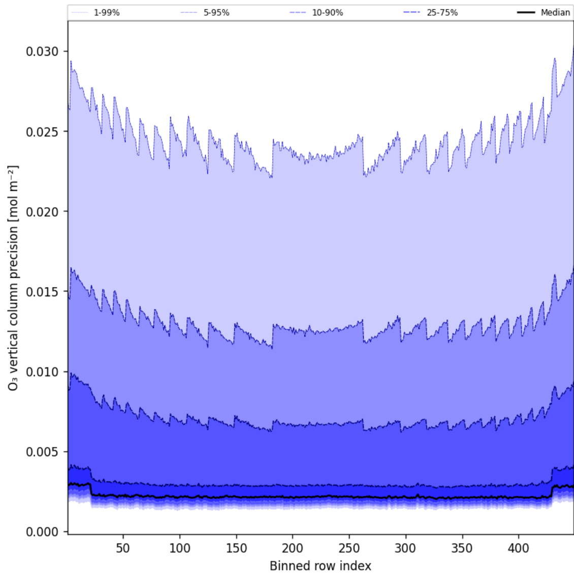
Figure 42: Along track statistics of “O 3 vertical column precision” for 2025-01-17 to 2025-01-18
