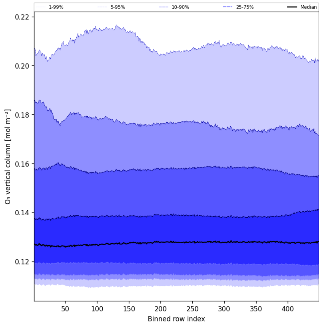
Figure 41: Along track statistics of “O 3 vertical column” for 2025-01-17 to 2025-01-18
