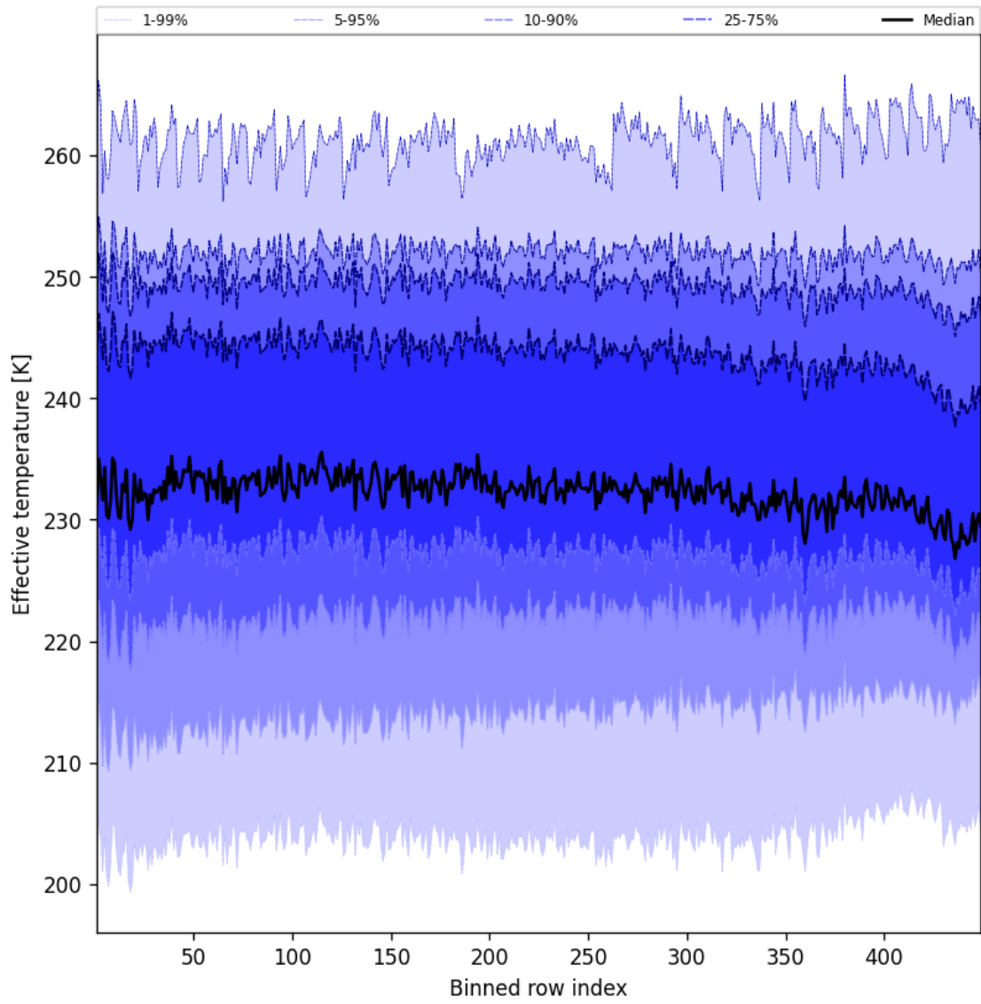
Figure 50: Along track statistics of “Effective temperature” for 2025-01-17 to 2025-01-18
