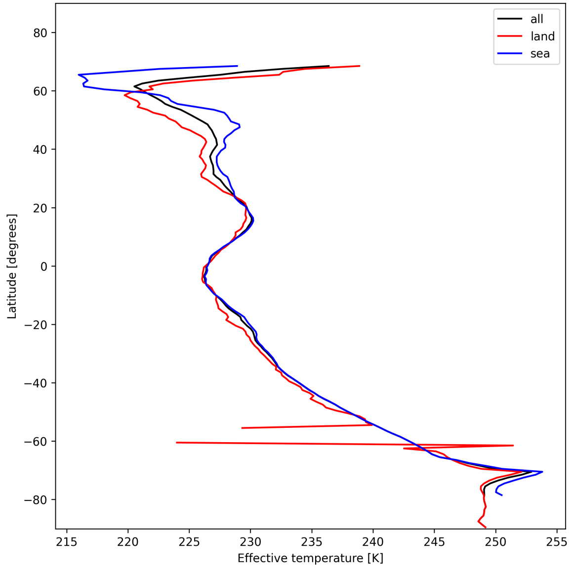
Figure 26: Zonal average of “Effective temperature” for 2025-01-17 to 2025-01-18.
