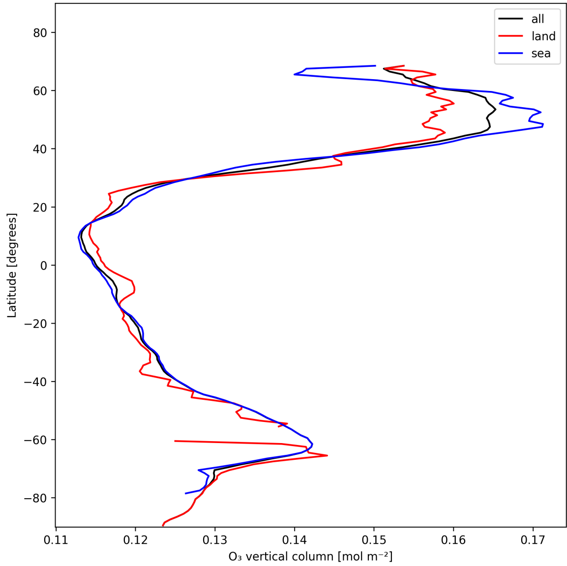
Figure 17: Zonal average of “O 3 vertical column” for 2025-01-17 to 2025-01-18.
