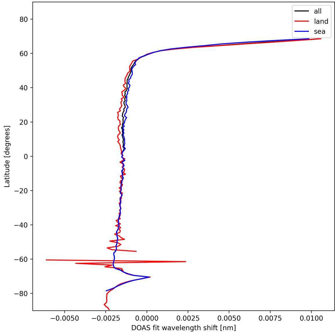
Figure 23: Zonal average of “DOAS fit wavelength shift” for 2025-01-17 to 2025-01-18.
