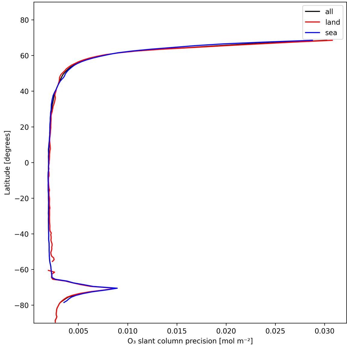
Figure 20: Zonal average of “O 3 slant column precision” for 2025-01-17 to 2025-01-18.
