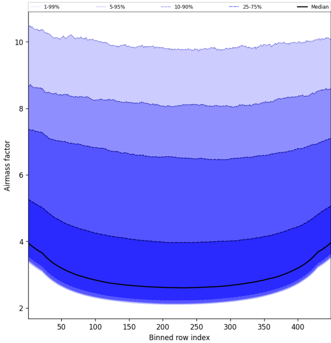
Figure 49: Along track statistics of “Airmass factor” for 2025-01-17 to 2025-01-18
