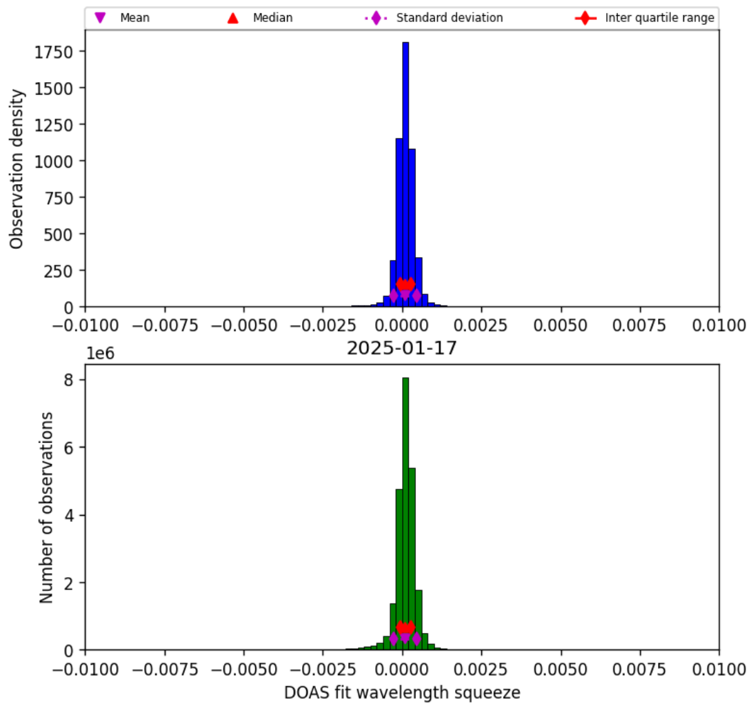
Figure 36: Histogram of “DOAS fit wavelength squeeze” for 2025-01-17 to 2025-01-18
