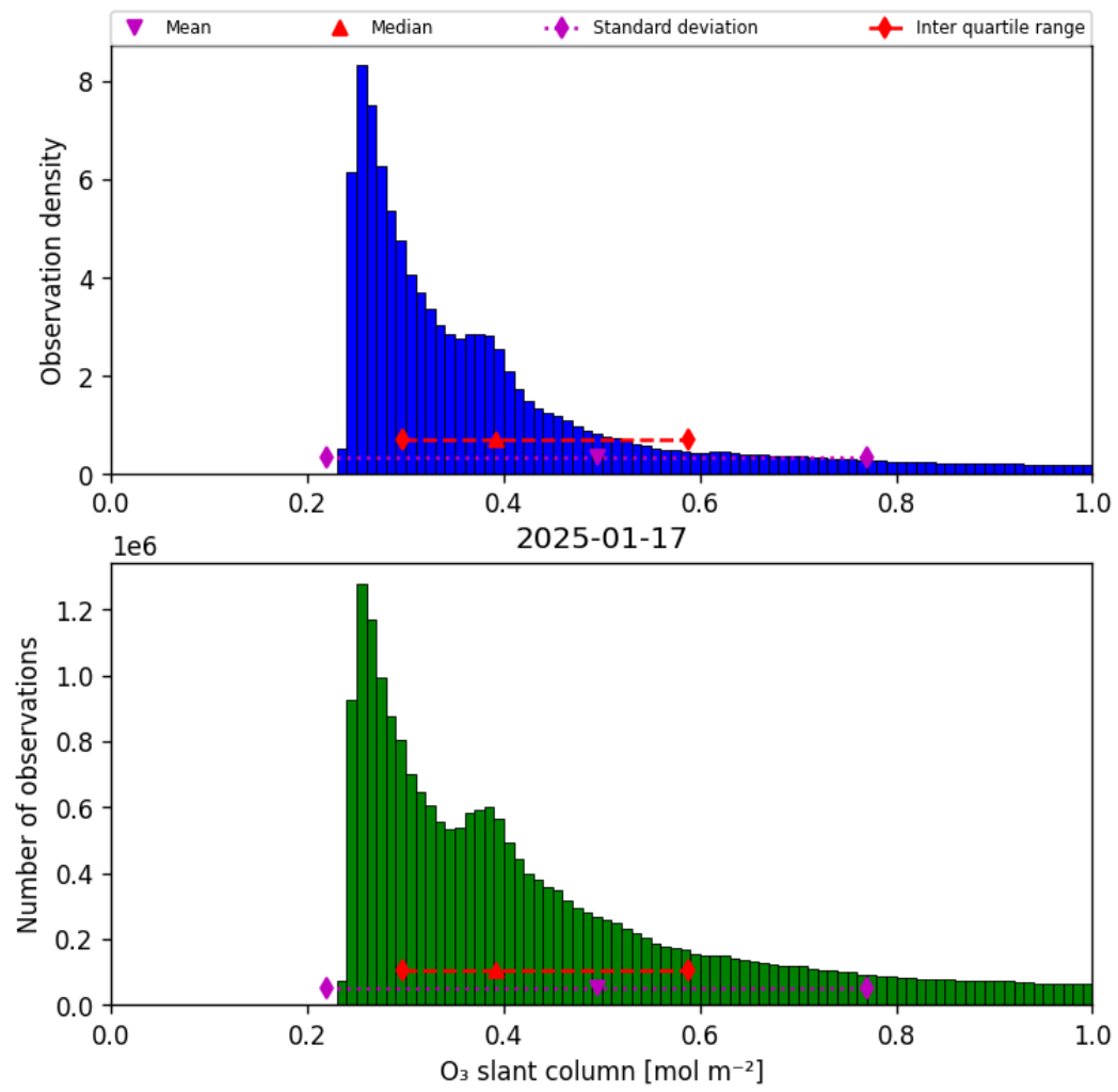
Figure 31: Histogram of “O 3 slant column” for 2025-01-17 to 2025-01-18
