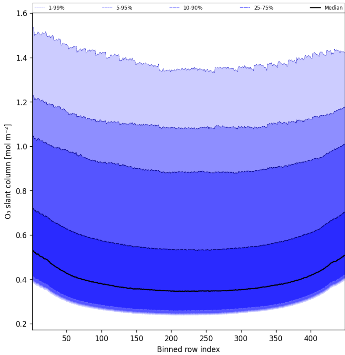
Figure 43: Along track statistics of “O 3 slant column” for 2025-01-17 to 2025-01-18
