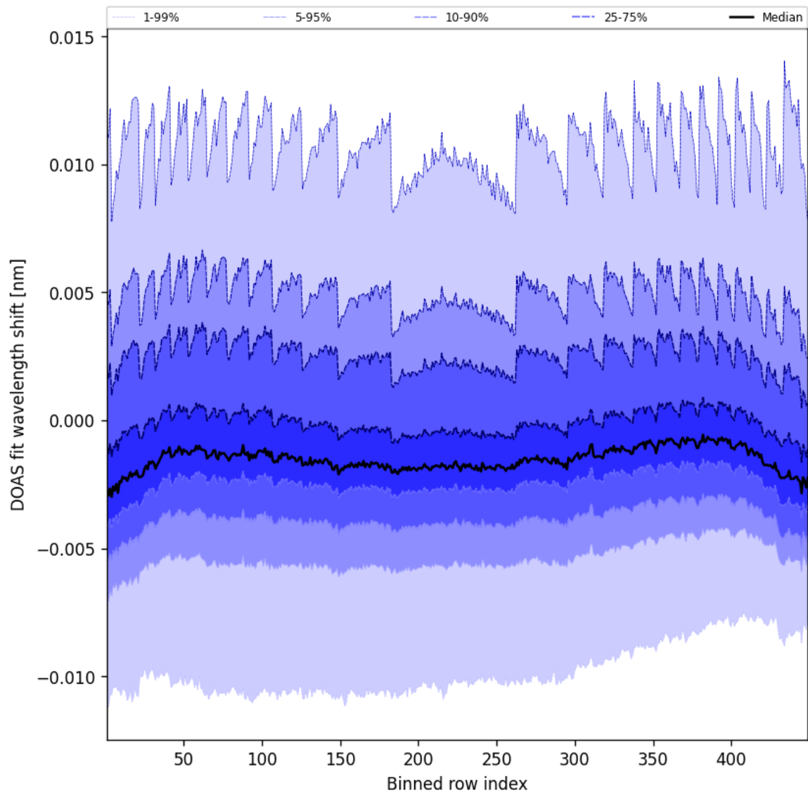
Figure 47: Along track statistics of “DOAS fit wavelength shift” for 2025-01-17 to 2025-01-18
