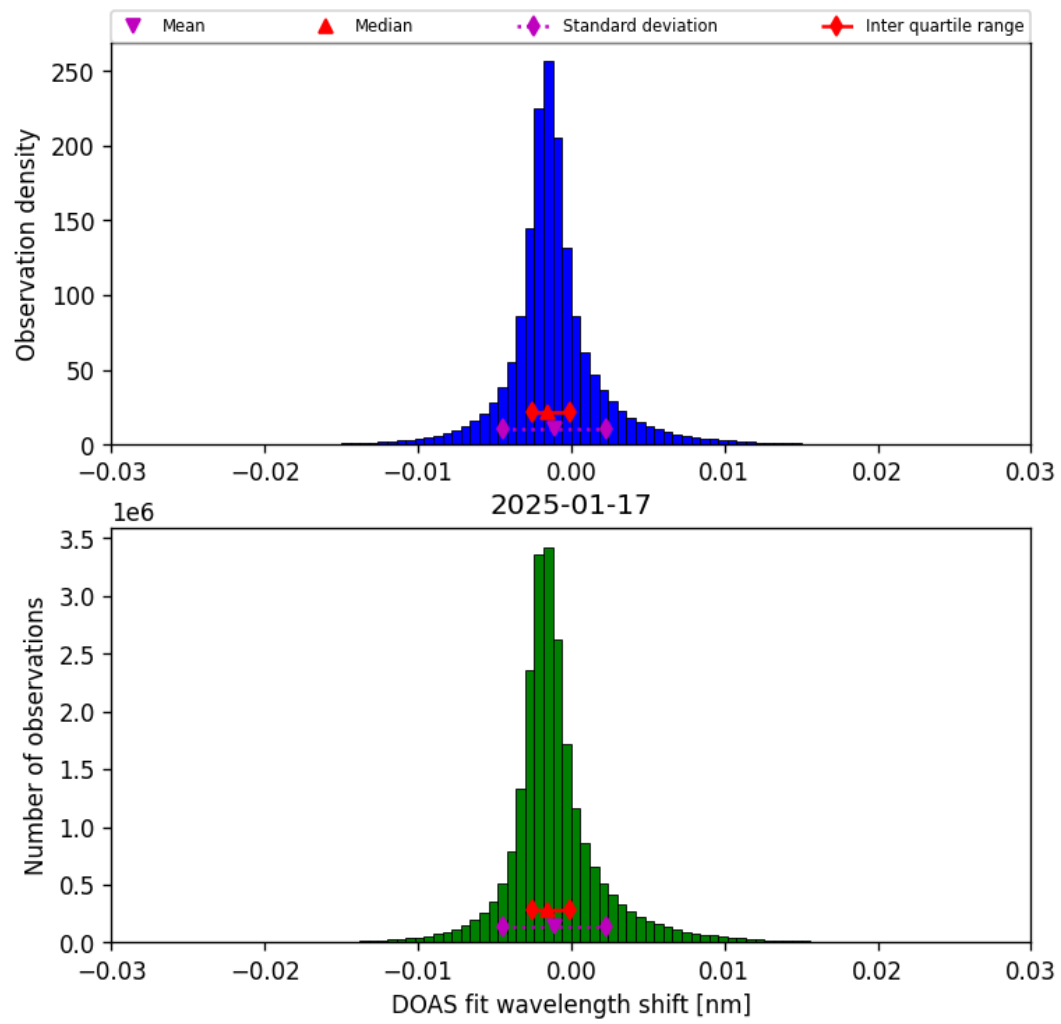
Figure 35: Histogram of “DOAS fit wavelength shift” for 2025-01-17 to 2025-01-18
