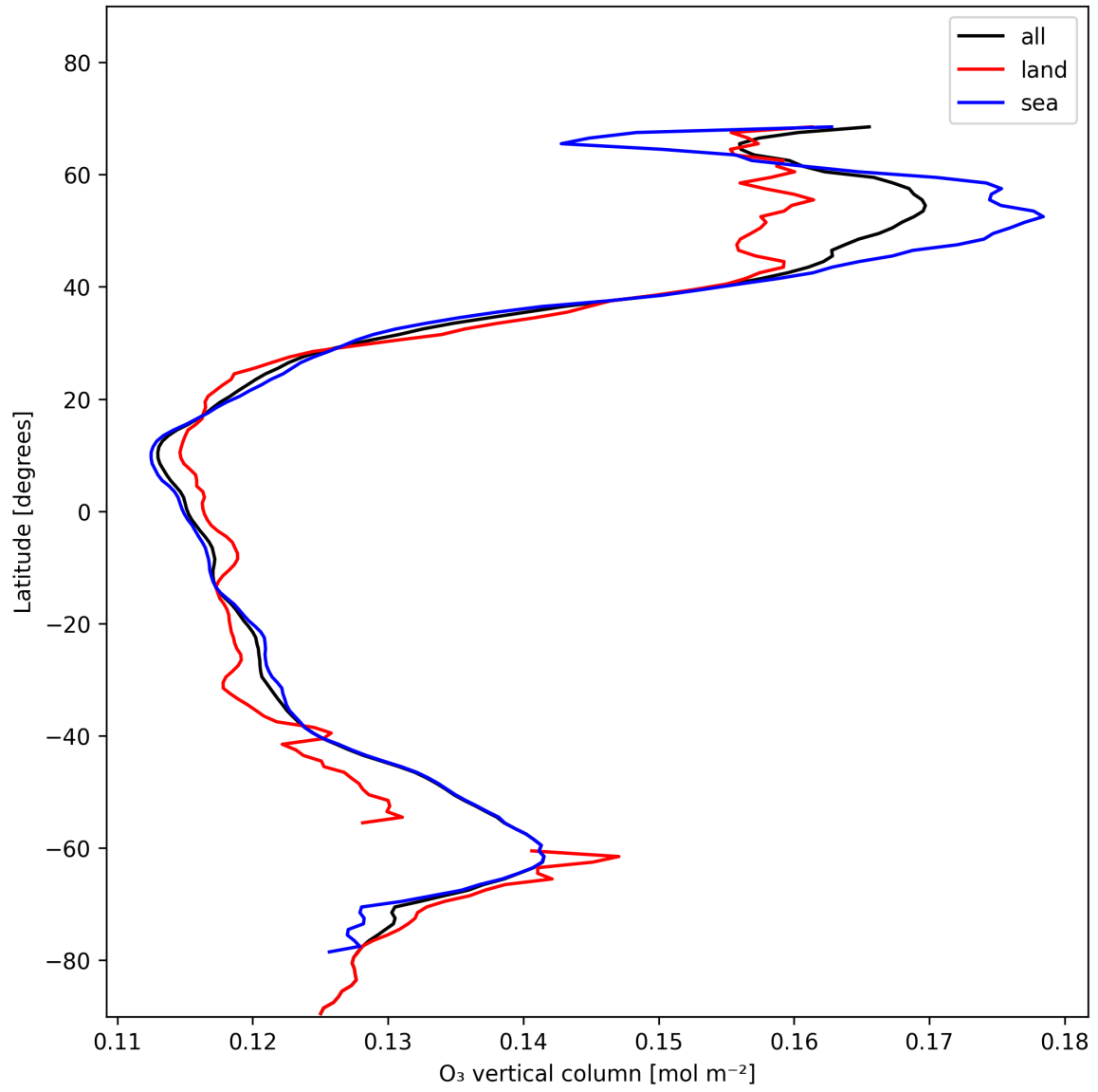
Figure 17: Zonal average of “O 3 vertical column” for 2025-01-18 to 2025-01-19.
