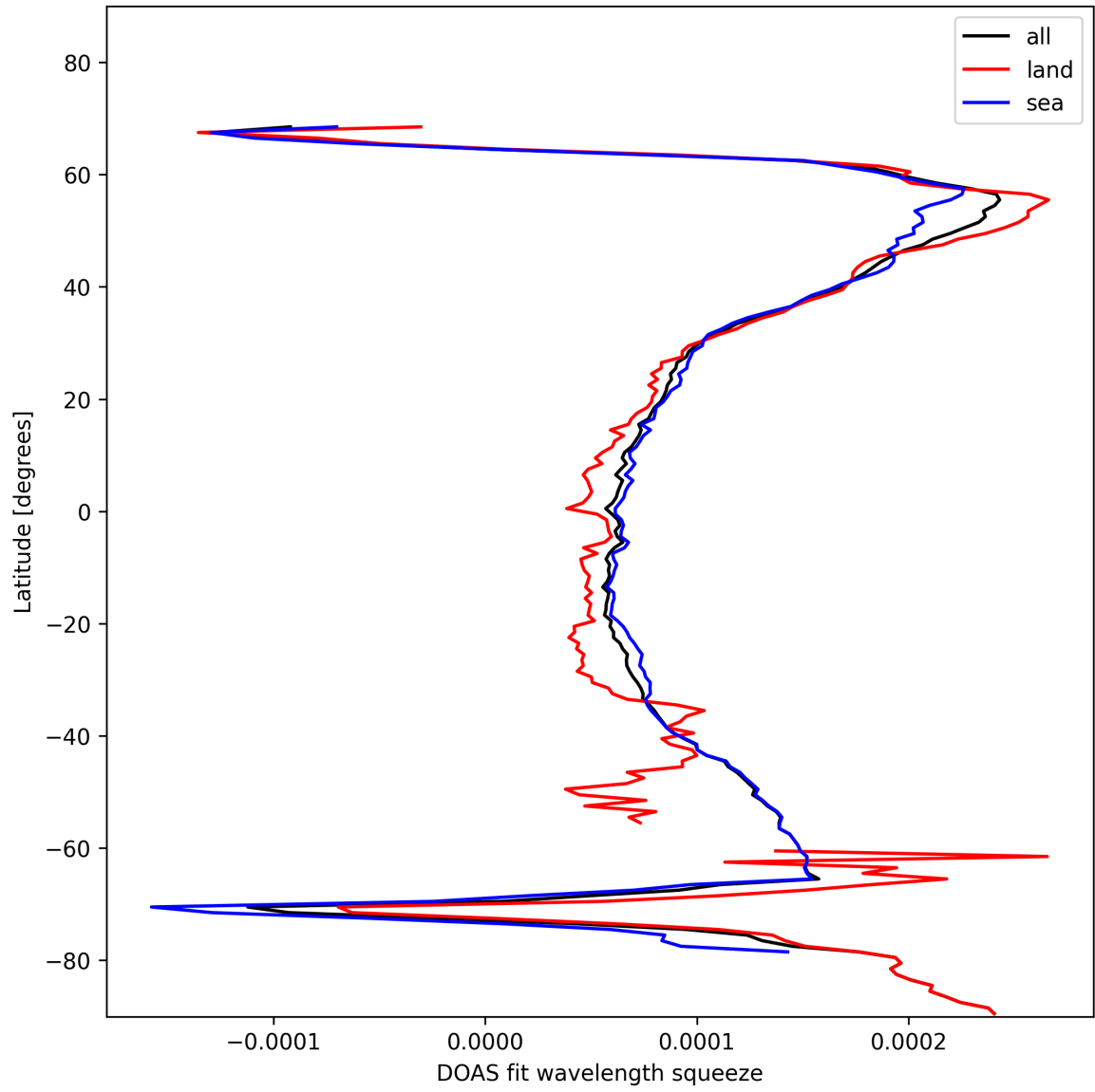
Figure 24: Zonal average of “DOAS fit wavelength squeeze” for 2025-01-18 to 2025-01-19.
