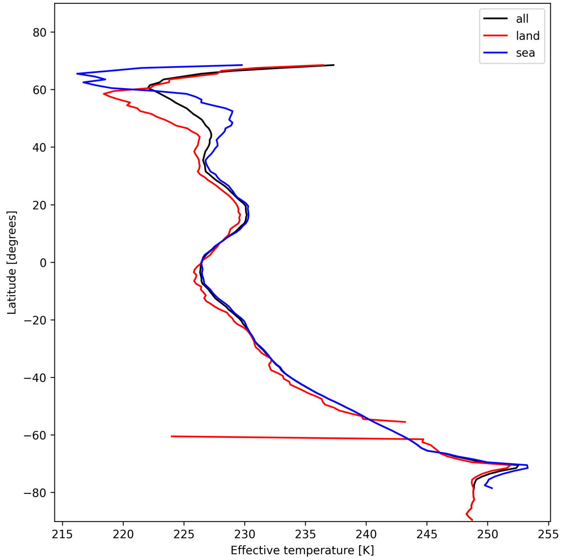
Figure 26: Zonal average of “Effective temperature” for 2025-01-18 to 2025-01-19.
