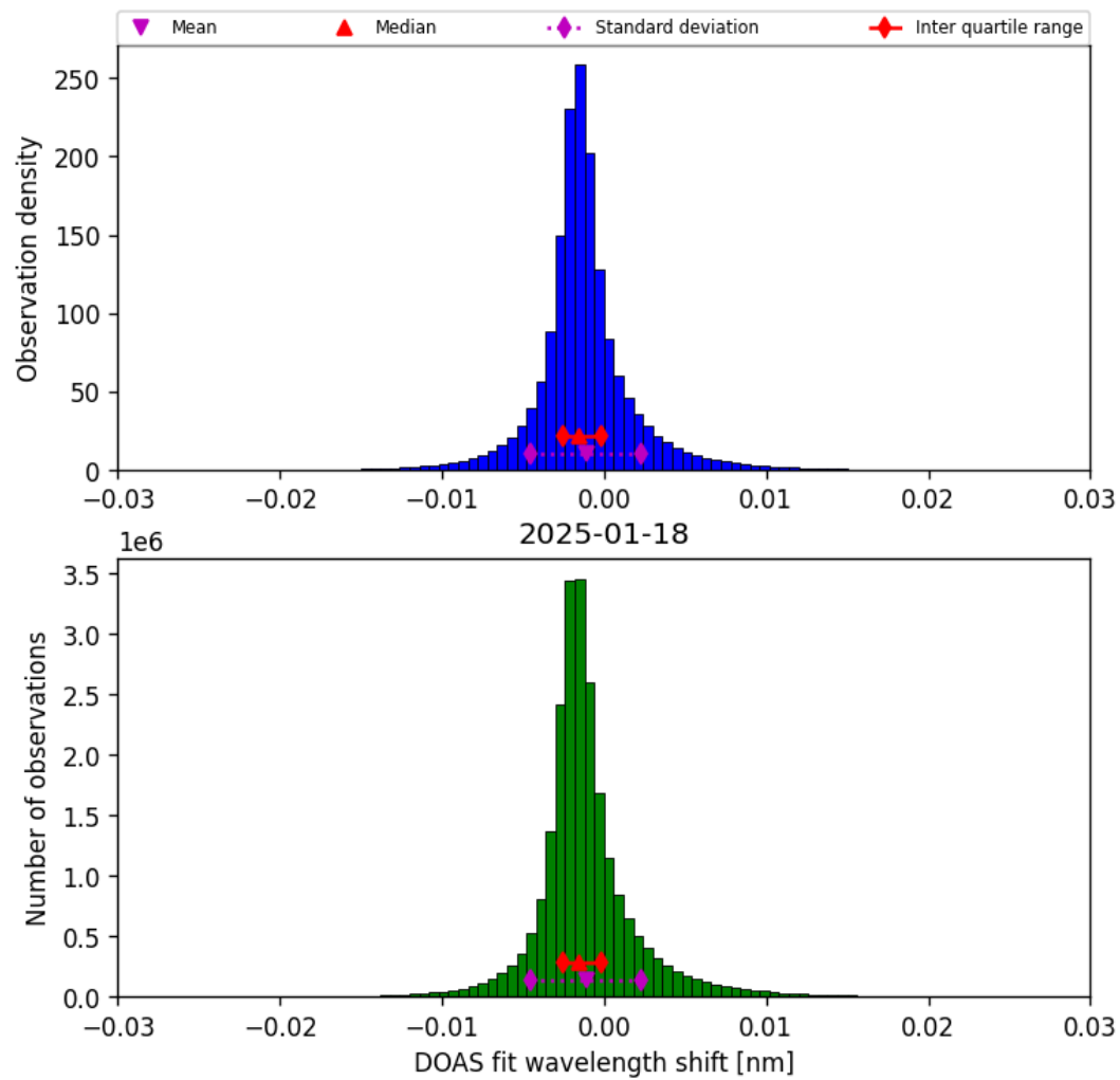
Figure 35: Histogram of “DOAS fit wavelength shift” for 2025-01-18 to 2025-01-19
