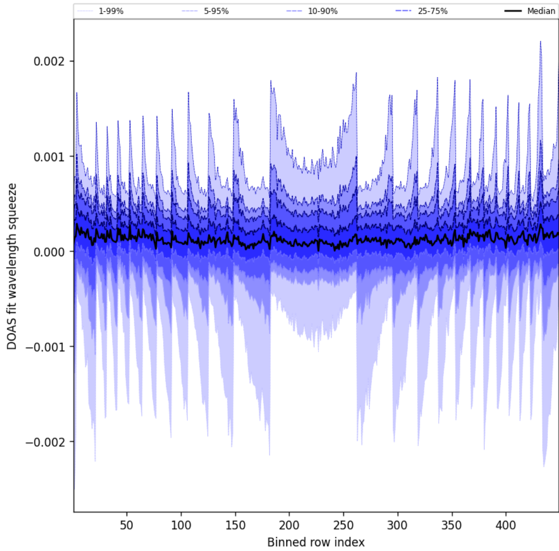
Figure 48: Along track statistics of “DOAS fit wavelength squeeze” for 2025-01-18 to 2025-01-19
