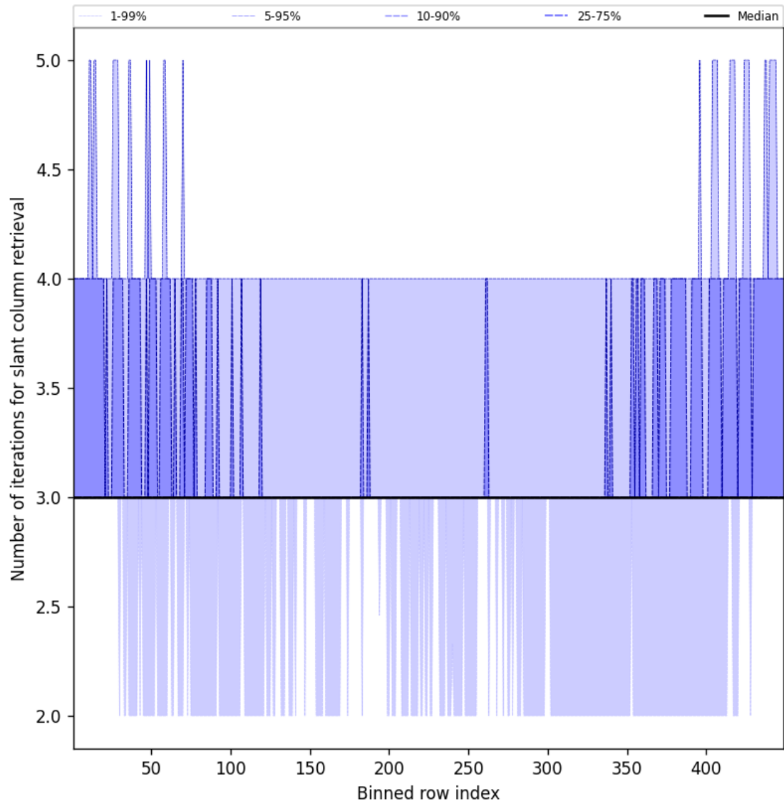
Figure 45: Along track statistics of “Number of iterations for slant column retrieval” for 2025-01-18 to 2025-01-19
