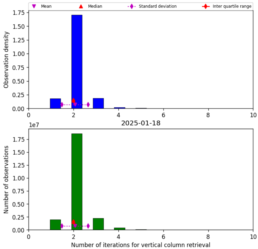
Figure 39: Histogram of “Number of iterations for vertical column retrieval” for 2025-01-18 to 2025-01-19
