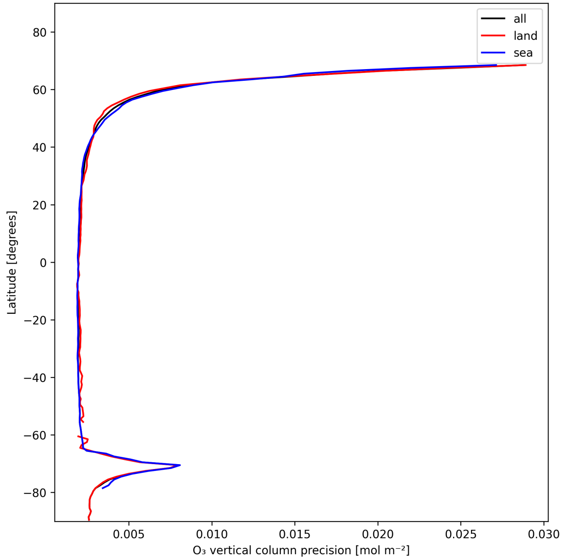
Figure 18: Zonal average of "O 3 vertical column precision" for 2025-01-18 to 2025-01-19.
