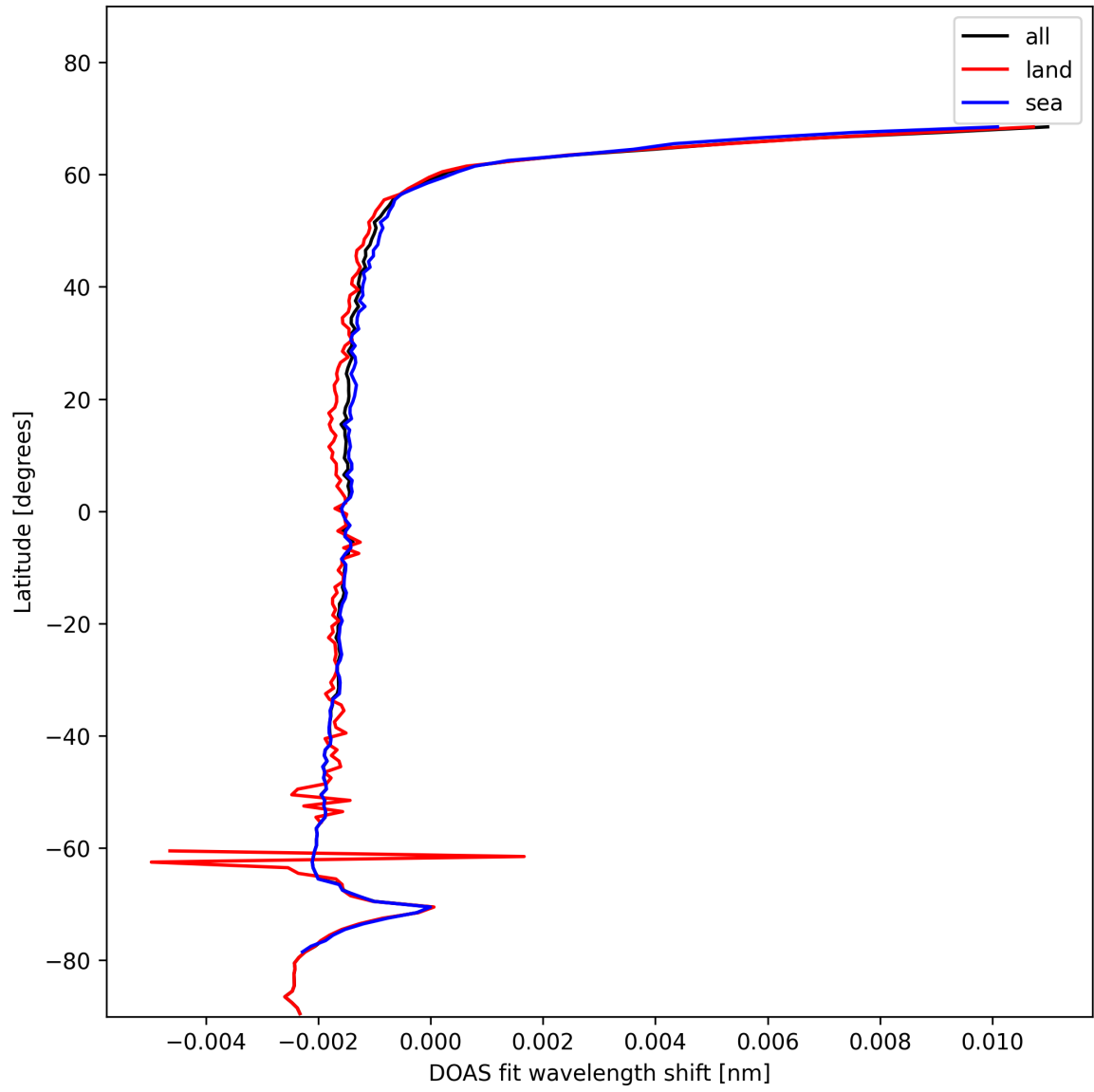
Figure 23: Zonal average of “DOAS fit wavelength shift” for 2025-01-18 to 2025-01-19.
