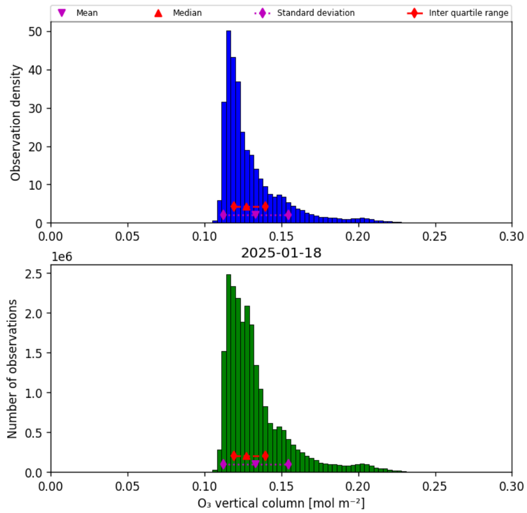
Figure 29: Histogram of “O 3 vertical column” for 2025-01-18 to 2025-01-19
