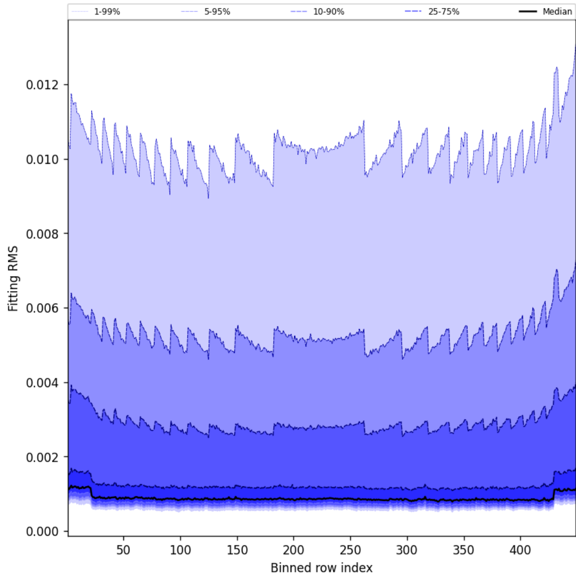
Figure 46: Along track statistics of “Fitting RMS” for 2025-01-18 to 2025-01-19
