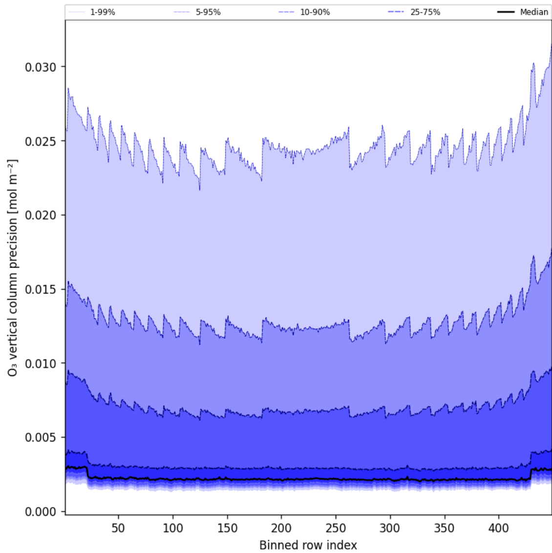
Figure 42: Along track statistics of “O 3 vertical column precision” for 2025-01-18 to 2025-01-19
