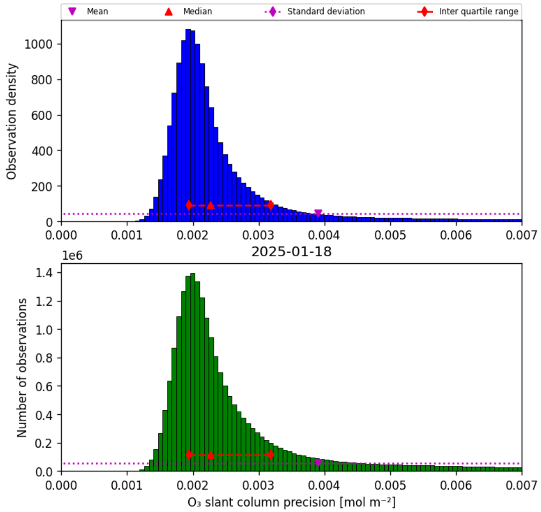
Figure 32: Histogram of “O 3 slant column precision” for 2025-01-18 to 2025-01-19
