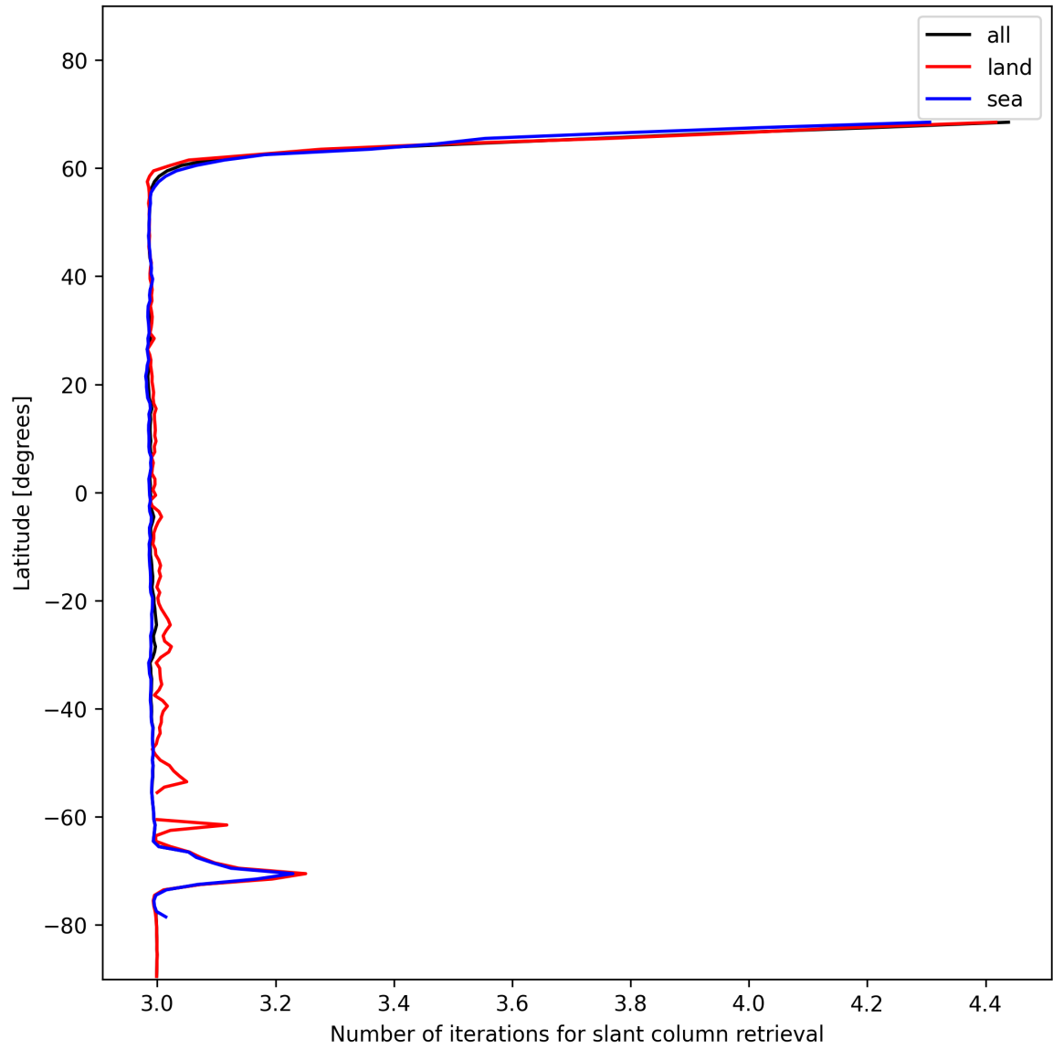
Figure 21: Zonal average of “Number of iterations for slant column retrieval” for 2025-01-18 to 2025-01-19.
