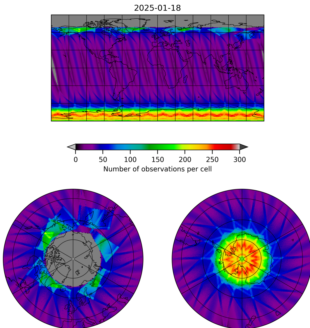
Figure 15: Map of the number of observations for 2025-01-18 to 2025-01-19
