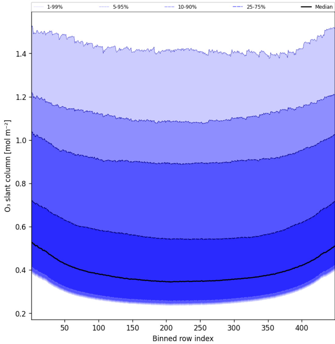
Figure 43: Along track statistics of “O 3 slant column” for 2025-01-18 to 2025-01-19
