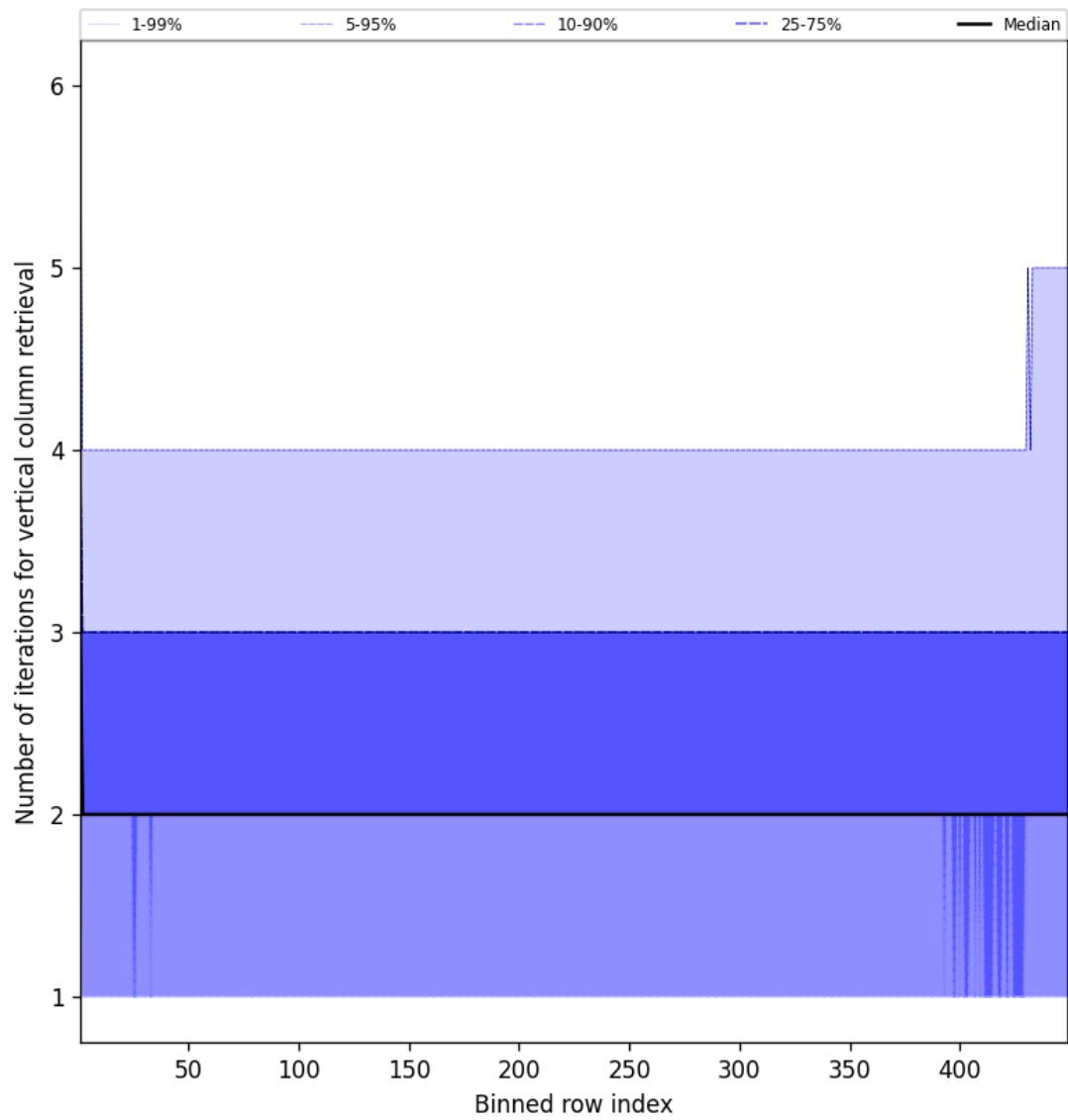
Figure 51: Along track statistics of “Number of iterations for vertical column retrieval” for 2025-01-18 to 2025-01-19
