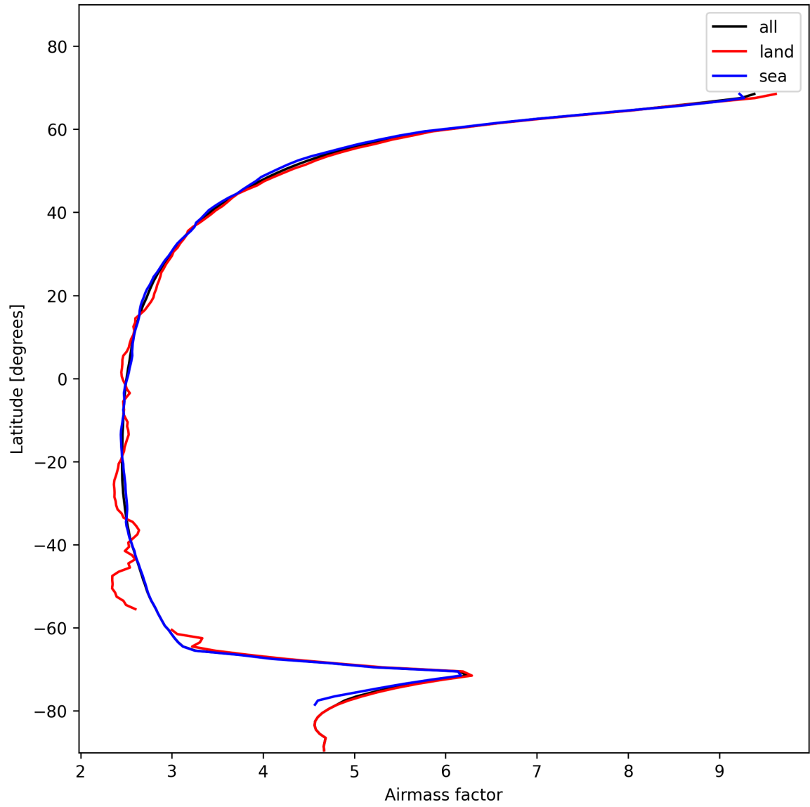
Figure 25: Zonal average of “Airmass factor” for 2025-01-18 to 2025-01-19.
