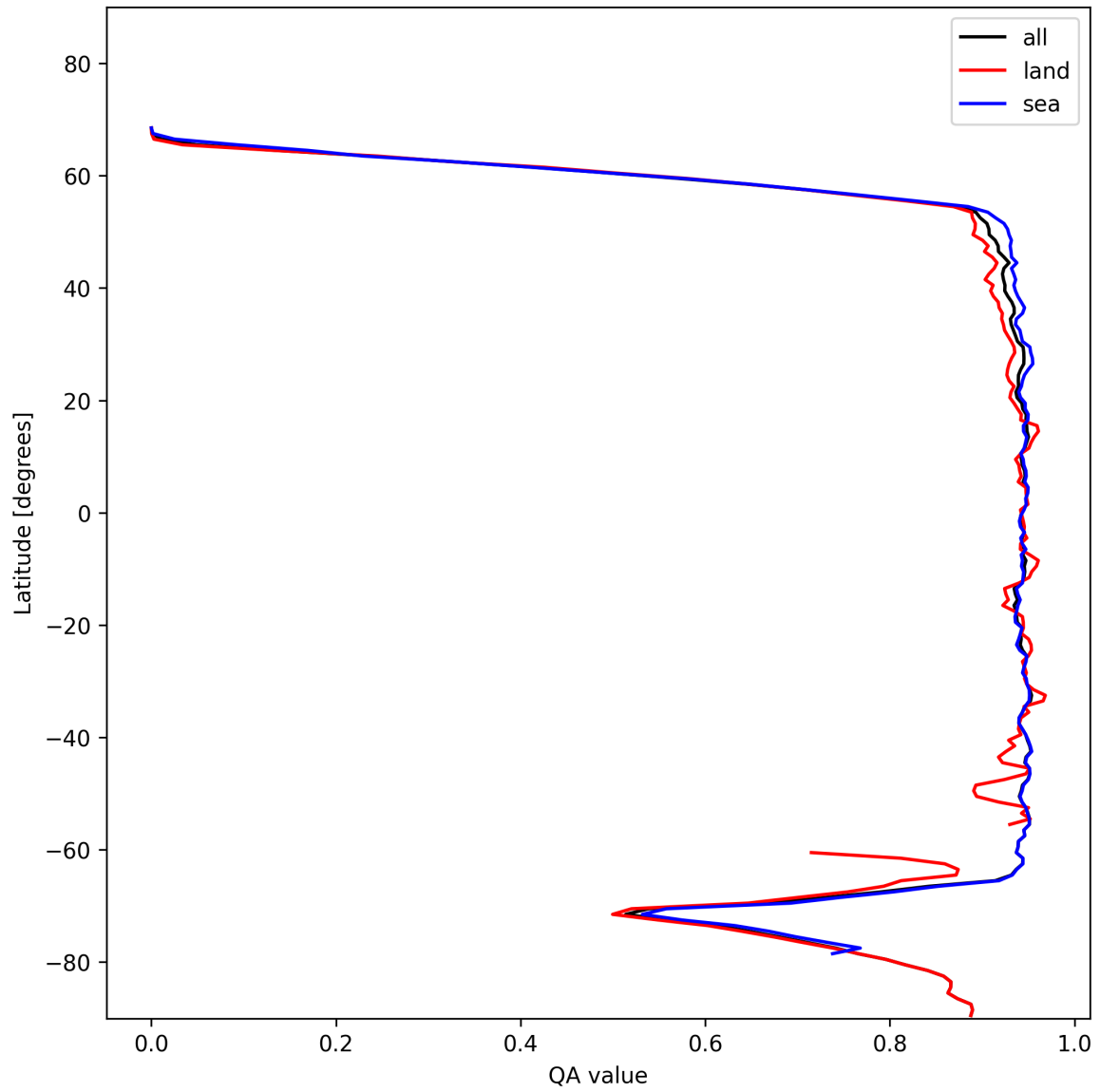
Figure 16: Zonal average of “QA value” for 2025-01-18 to 2025-01-19.
