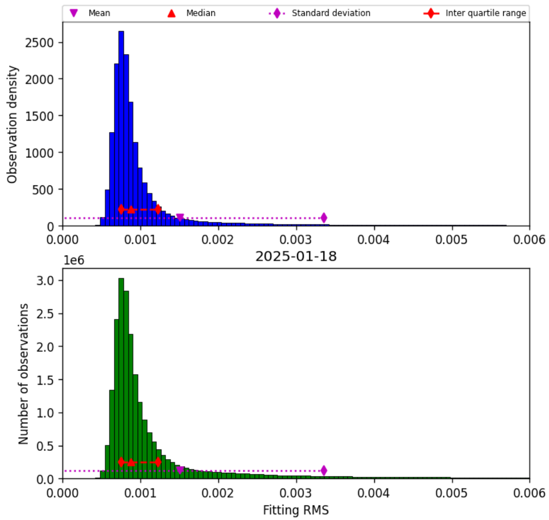
Figure 34: Histogram of “Fitting RMS” for 2025-01-18 to 2025-01-19
