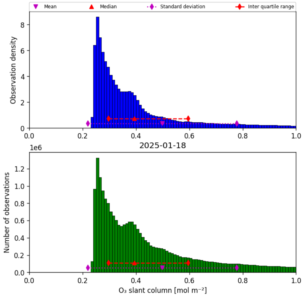
Figure 31: Histogram of “O 3 slant column” for 2025-01-18 to 2025-01-19
