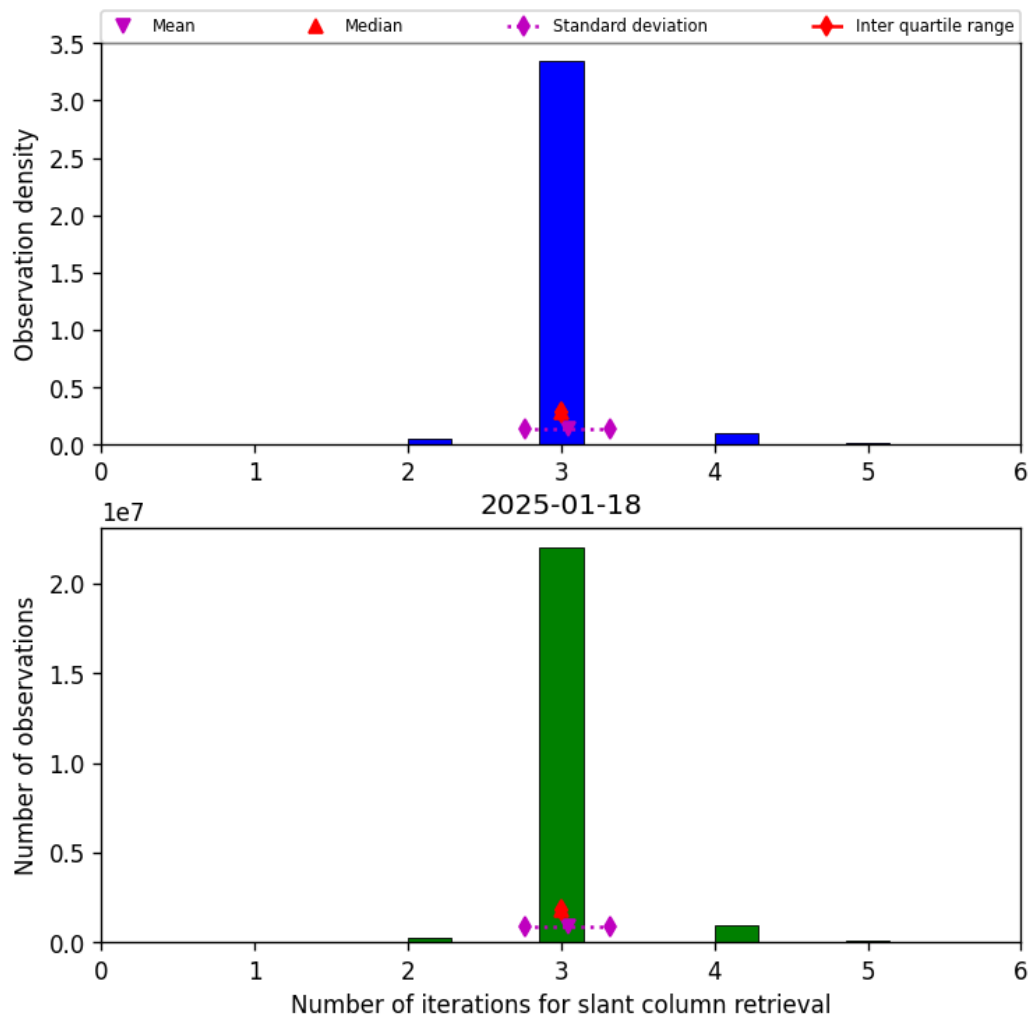
Figure 33: Histogram of “Number of iterations for slant column retrieval” for 2025-01-18 to 2025-01-19
