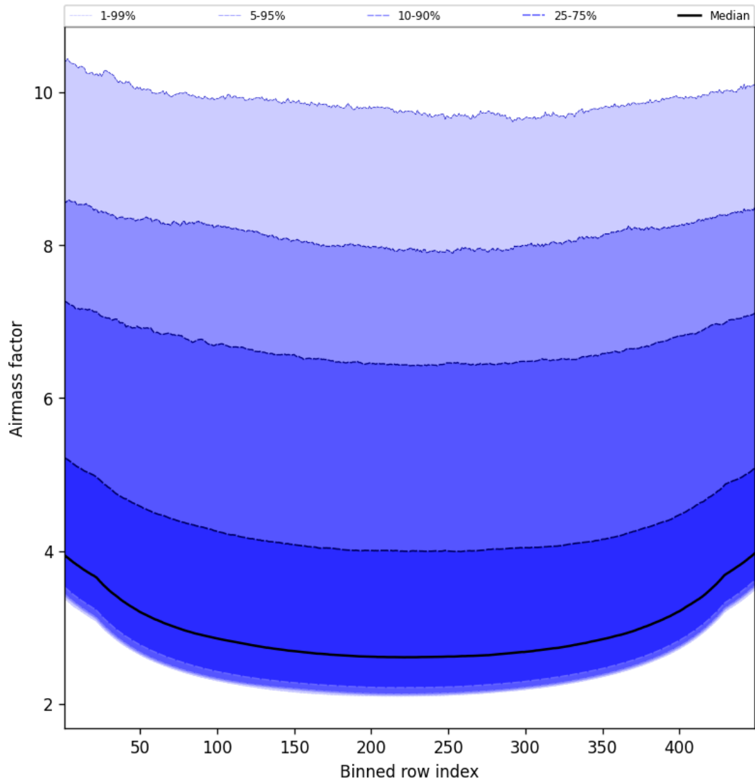
Figure 49: Along track statistics of “Airmass factor” for 2025-01-18 to 2025-01-19
