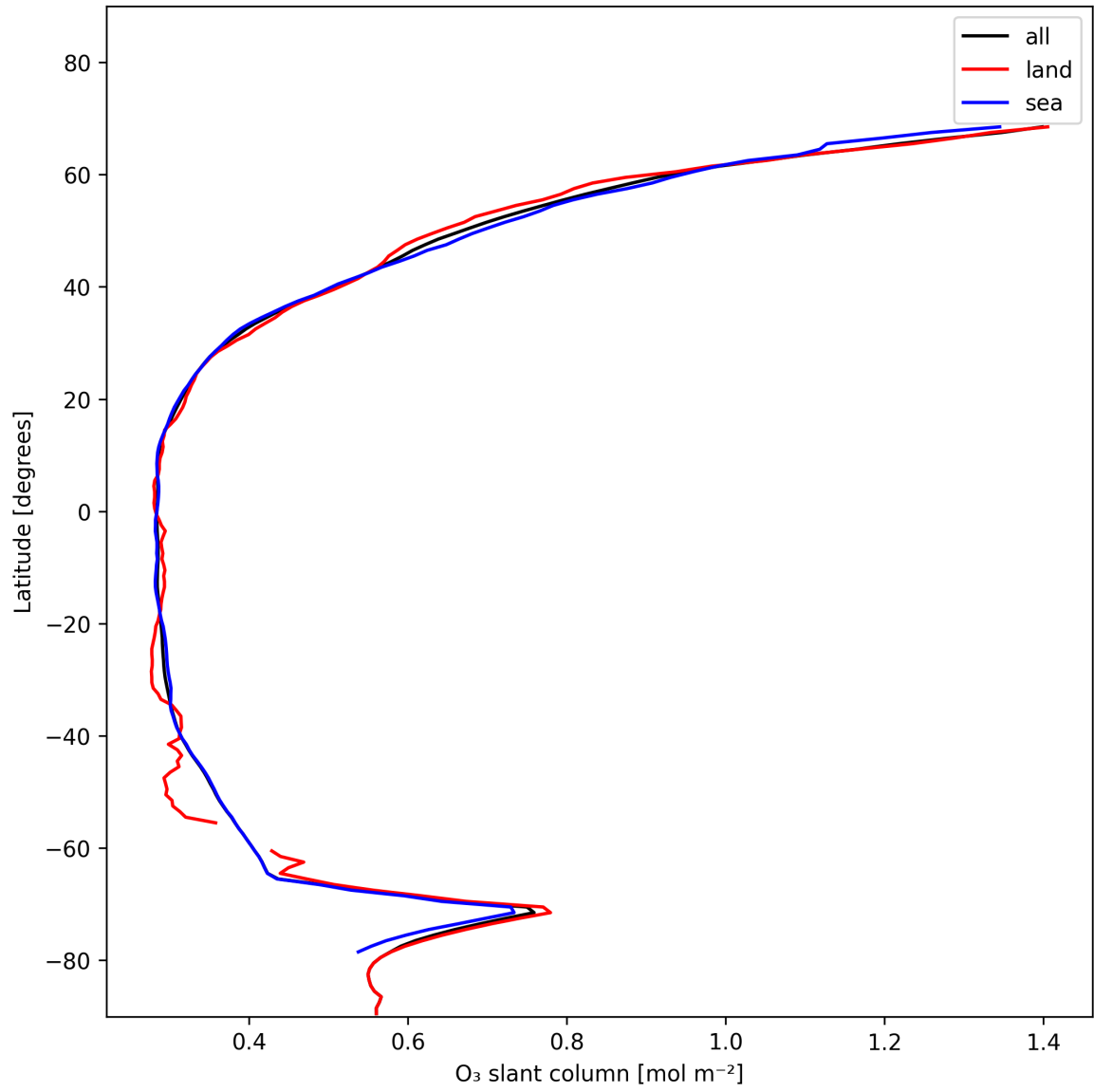
Figure 19: Zonal average of “O 3 slant column” for 2025-01-18 to 2025-01-19.
