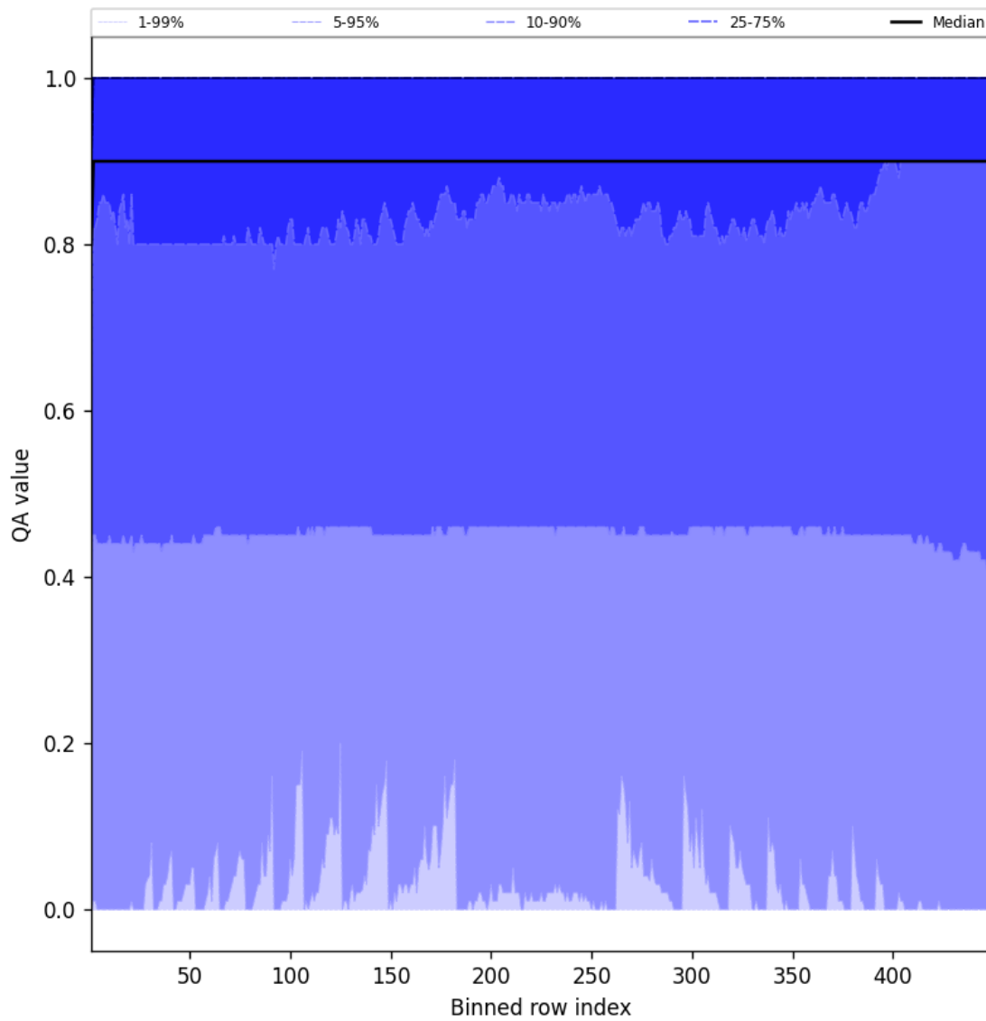
Figure 40: Along track statistics of “QA value” for 2025-01-18 to 2025-01-19
