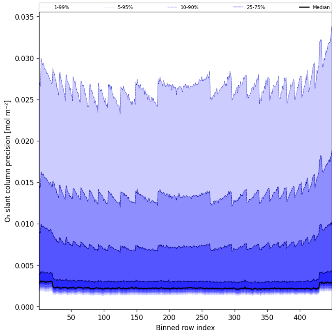
Figure 44: Along track statistics of “O 3 slant column precision” for 2025-01-18 to 2025-01-19
