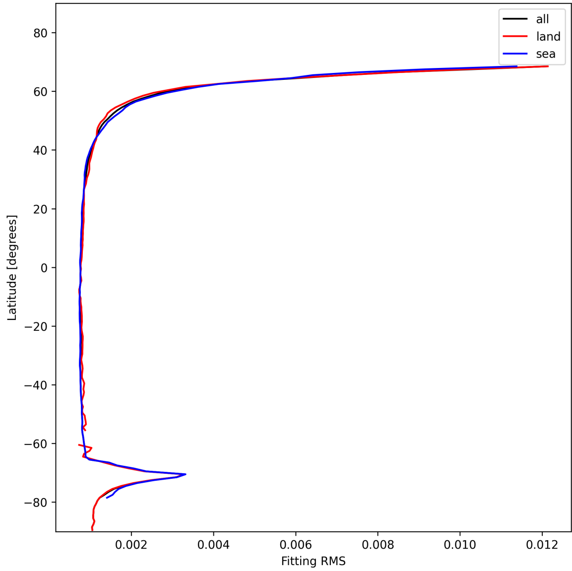
Figure 22: Zonal average of “Fitting RMS” for 2025-01-18 to 2025-01-19.
