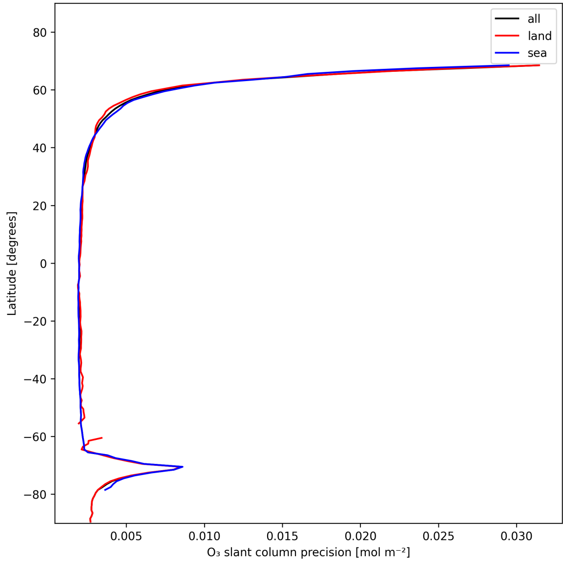
Figure 20: Zonal average of “O 3 slant column precision” for 2025-01-18 to 2025-01-19.
