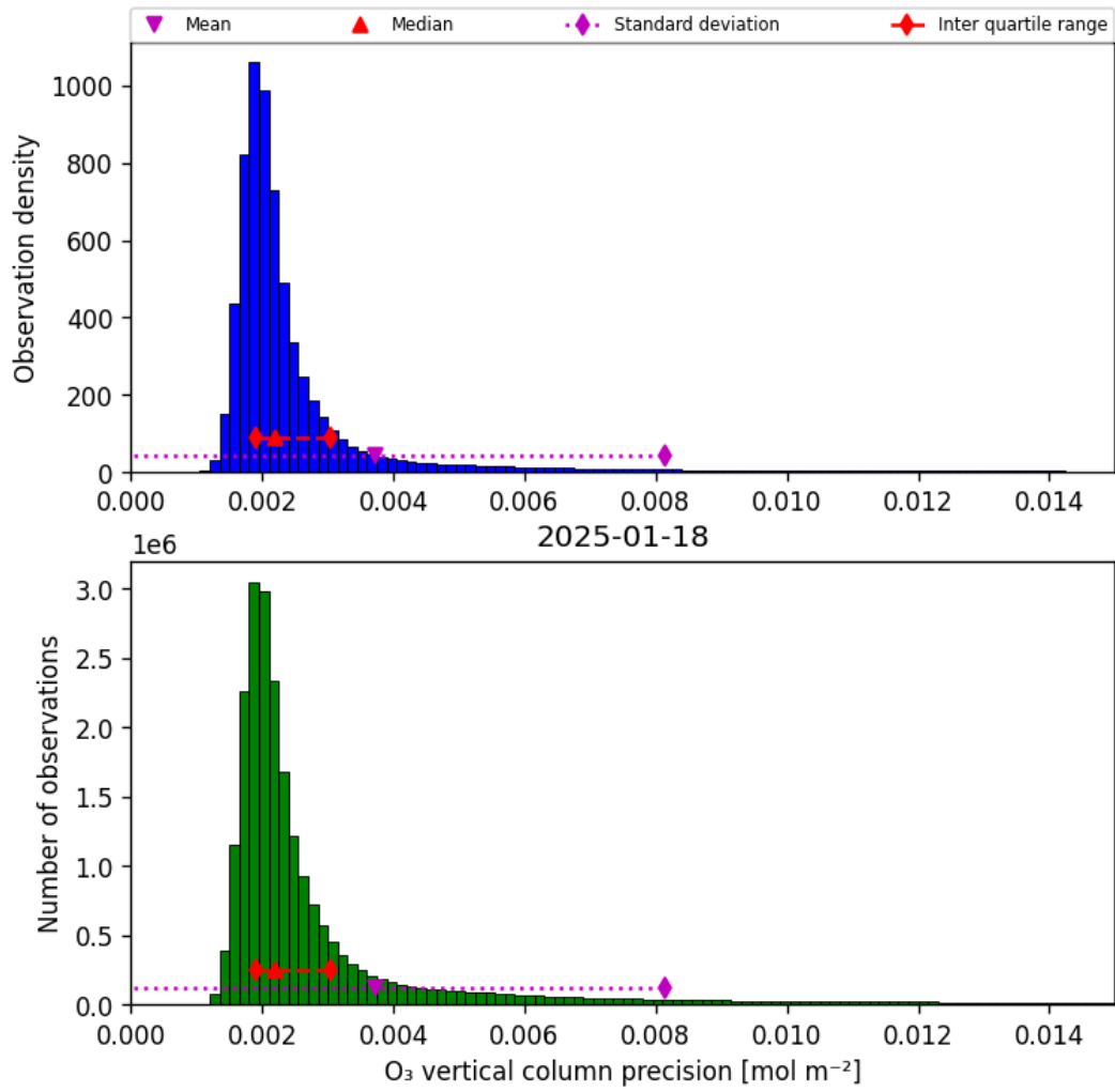
Figure 30: Histogram of “O 3 vertical column precision” for 2025-01-18 to 2025-01-19
