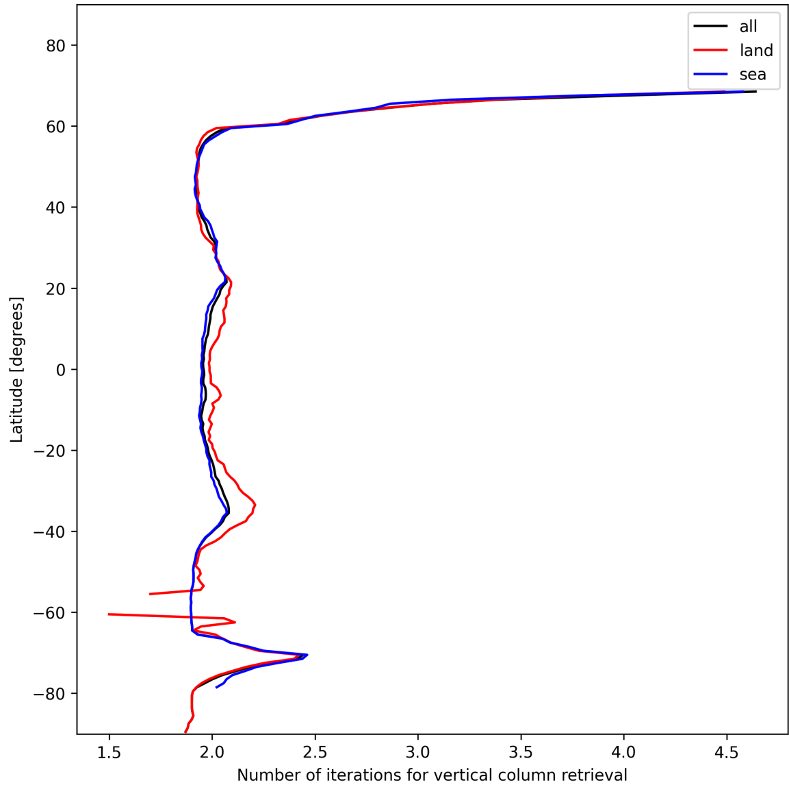
Figure 27: Zonal average of “Number of iterations for vertical column retrieval” for 2025-01-18 to 2025-01-19.
