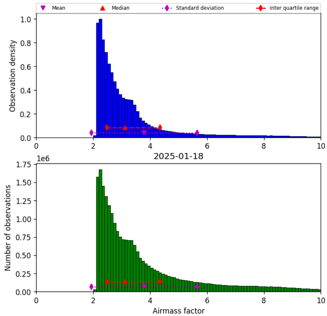
Figure 37: Histogram of “Airmass factor” for 2025-01-18 to 2025-01-19
