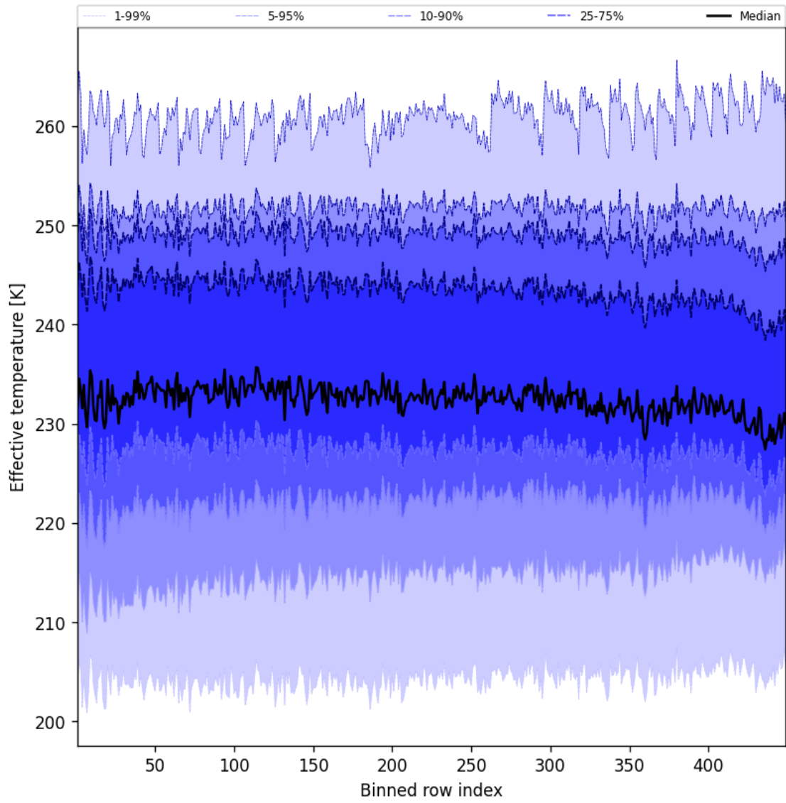
Figure 50: Along track statistics of “Effective temperature” for 2025-01-18 to 2025-01-19
