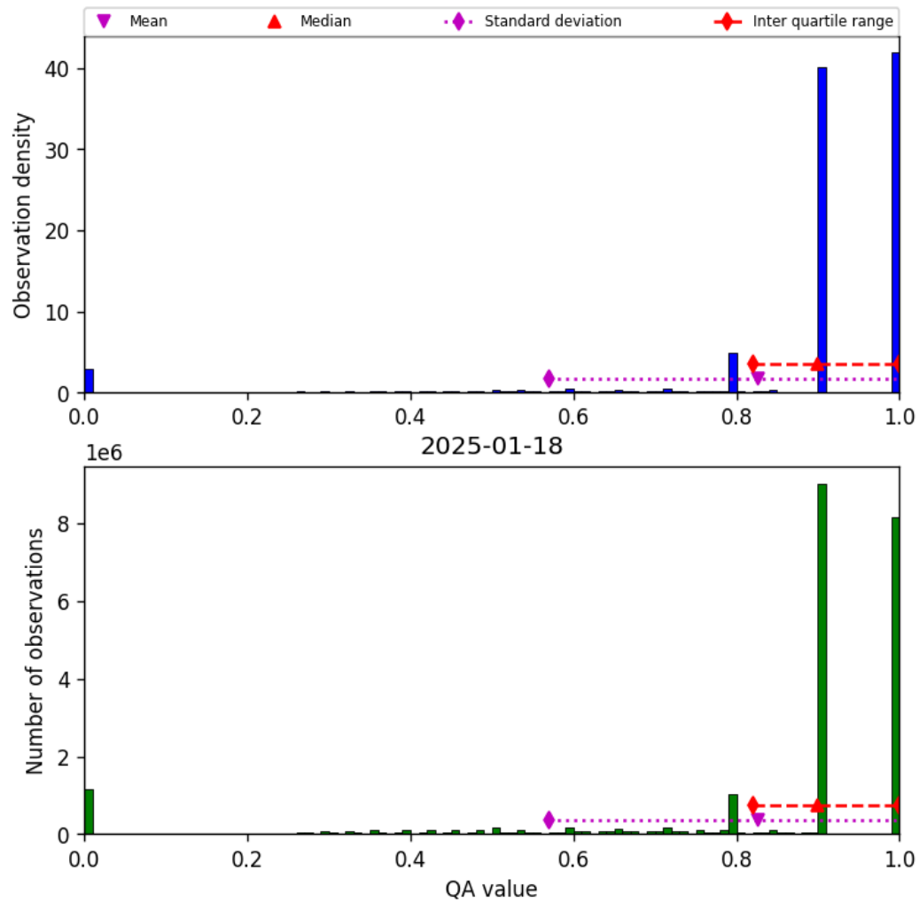
Figure 28: Histogram of “QA value” for 2025-01-18 to 2025-01-19
