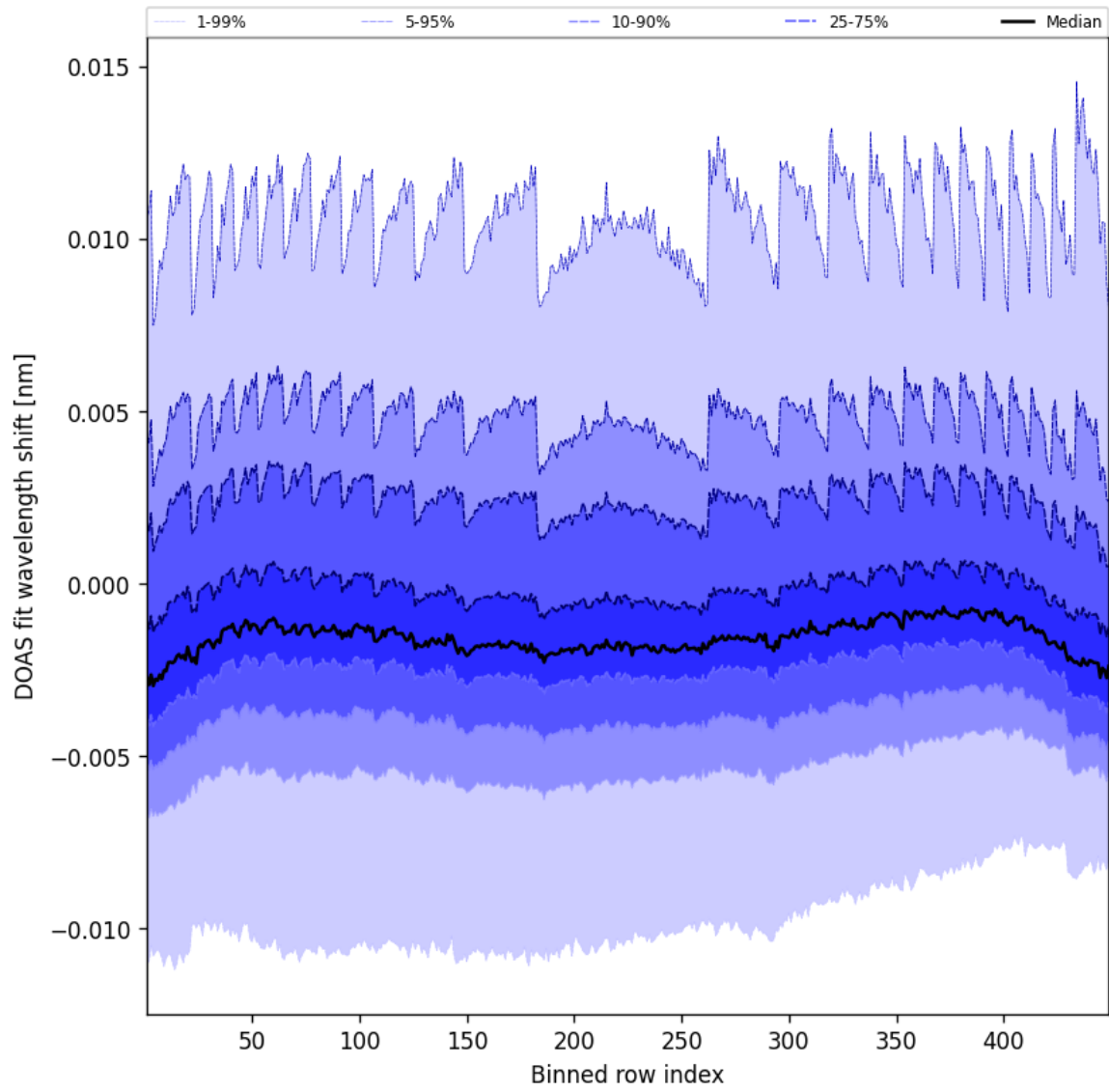
Figure 47: Along track statistics of “DOAS fit wavelength shift” for 2025-01-18 to 2025-01-19
