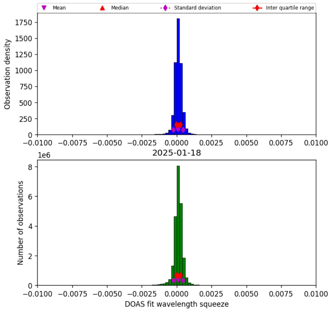
Figure 36: Histogram of “DOAS fit wavelength squeeze” for 2025-01-18 to 2025-01-19
