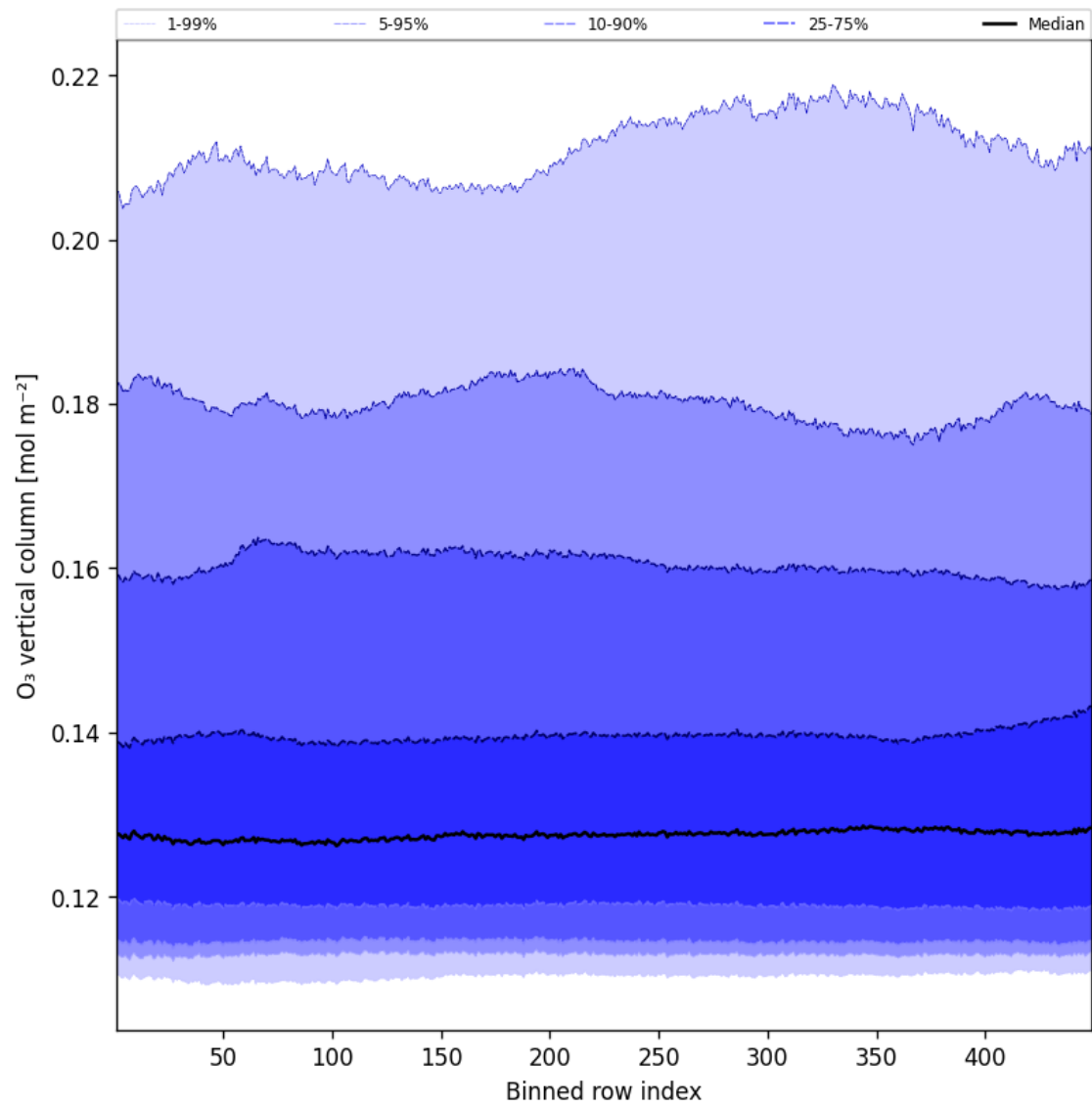
Figure 41: Along track statistics of “O 3 vertical column” for 2025-01-18 to 2025-01-19
