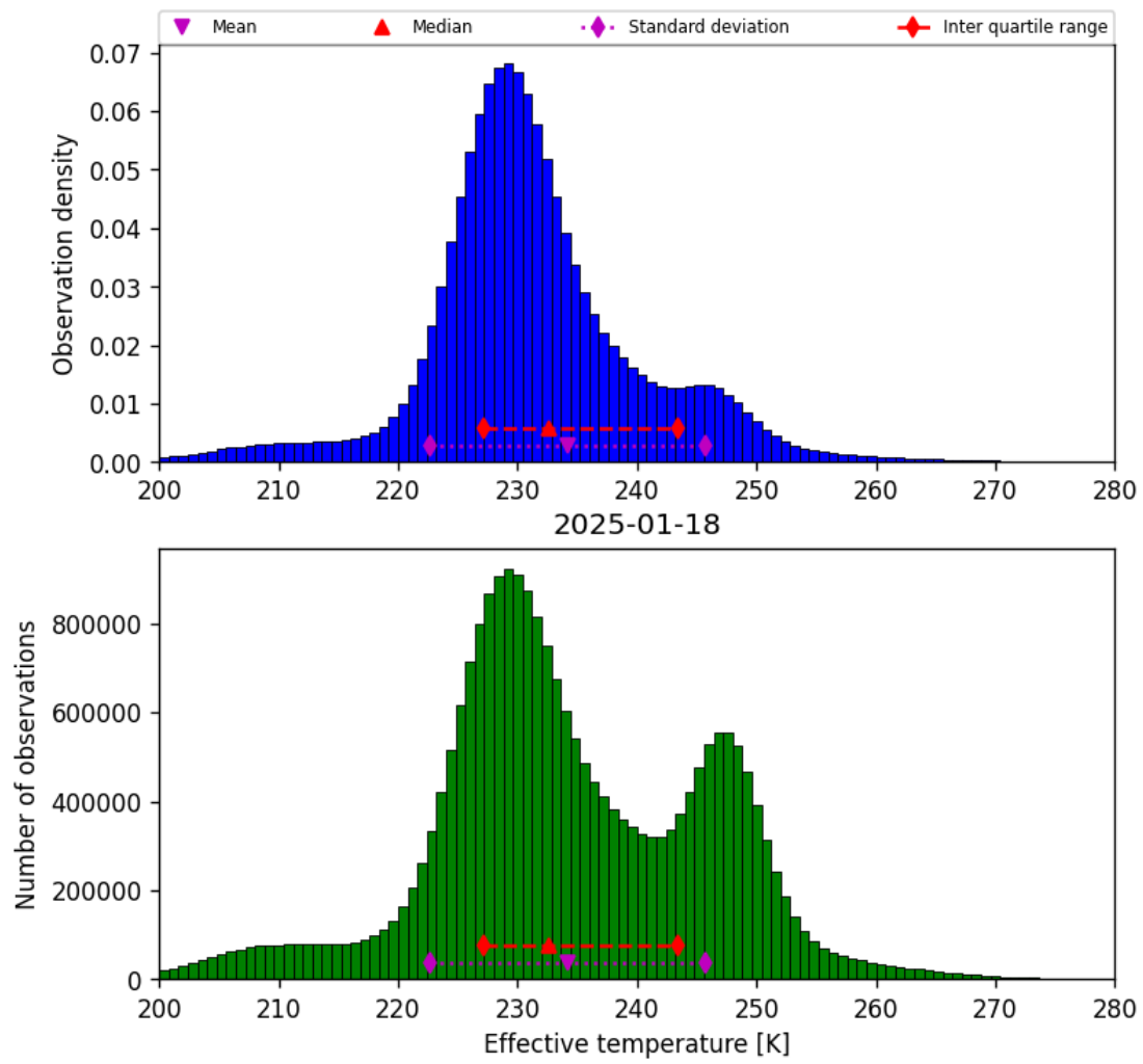
Figure 38: Histogram of “Effective temperature” for 2025-01-18 to 2025-01-19
