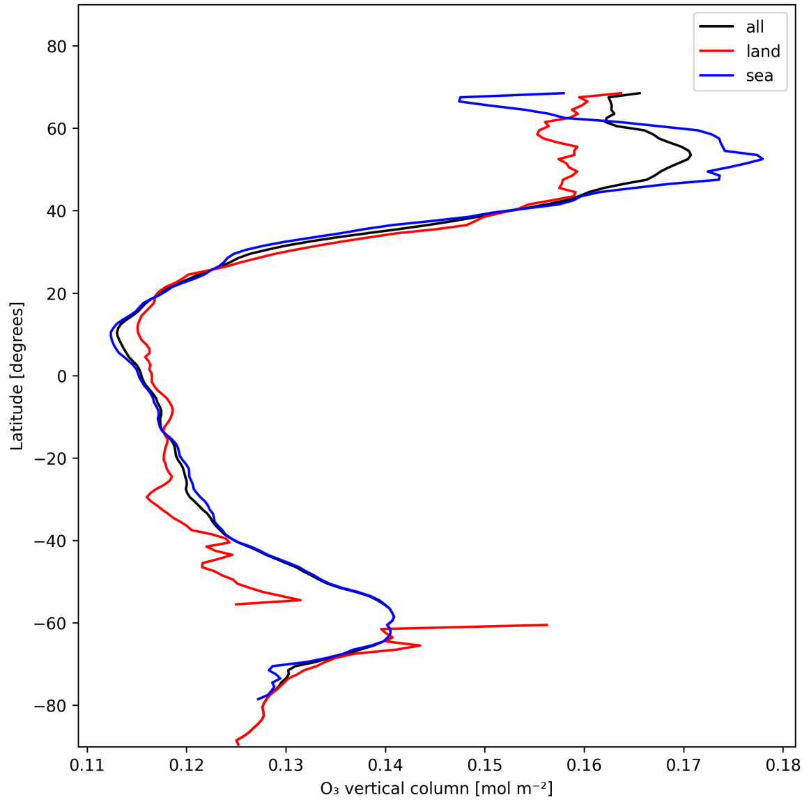
Figure 17: Zonal average of “O 3 vertical column” for 2025-01-19 to 2025-01-20.
