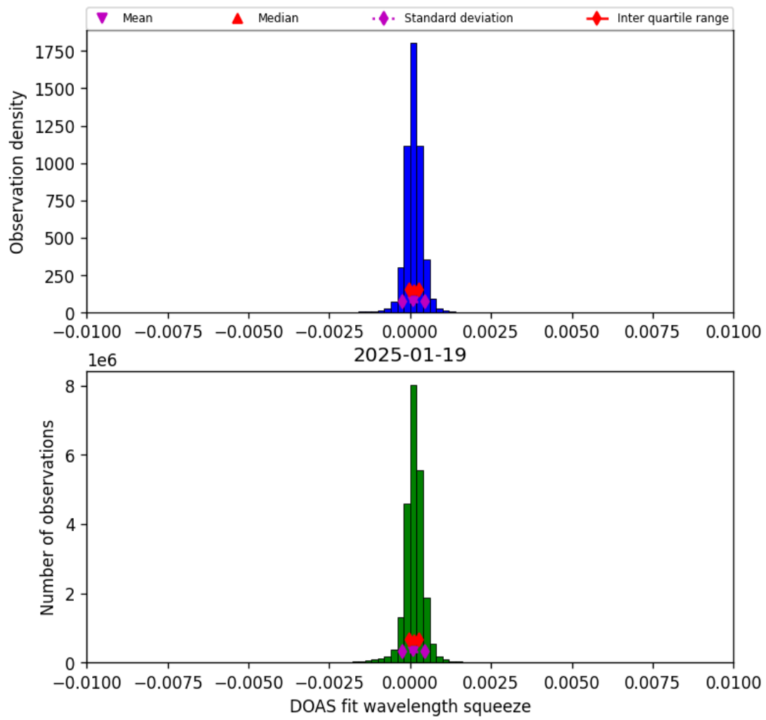
Figure 36: Histogram of “DOAS fit wavelength squeeze” for 2025-01-19 to 2025-01-20
