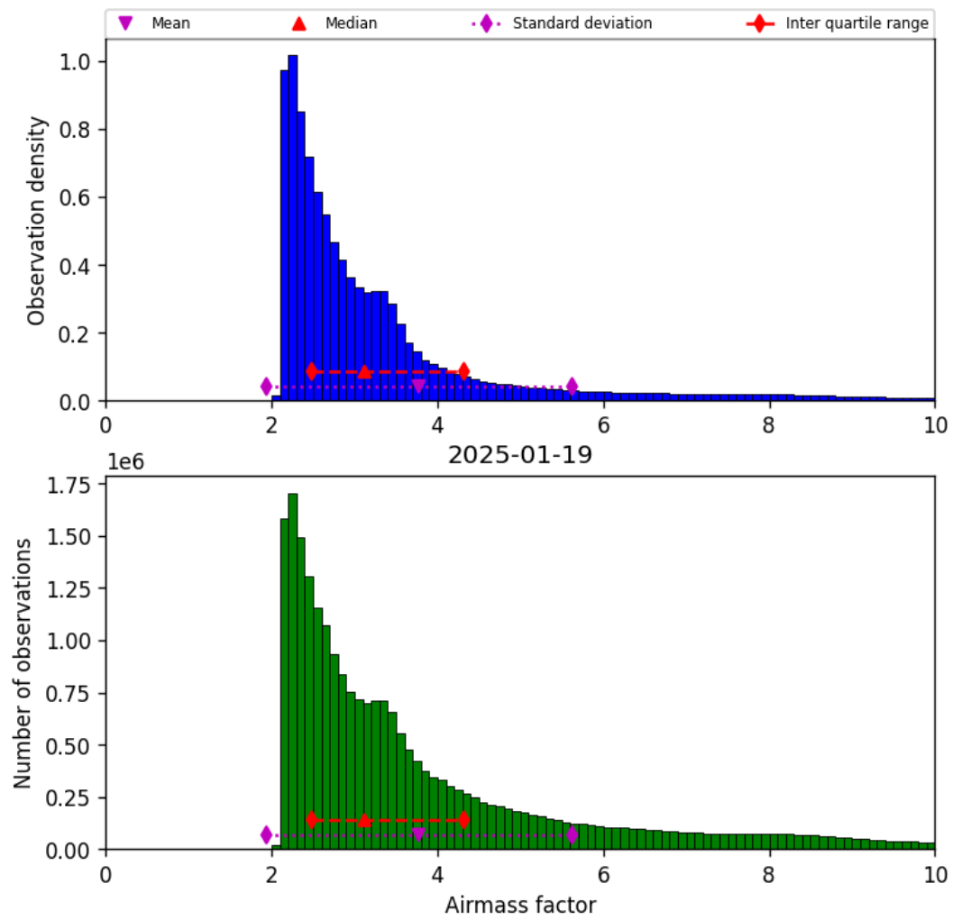
Figure 37: Histogram of “Airmass factor” for 2025-01-19 to 2025-01-20
