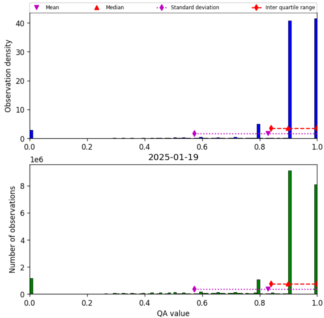
Figure 28: Histogram of “QA value” for 2025-01-19 to 2025-01-20
