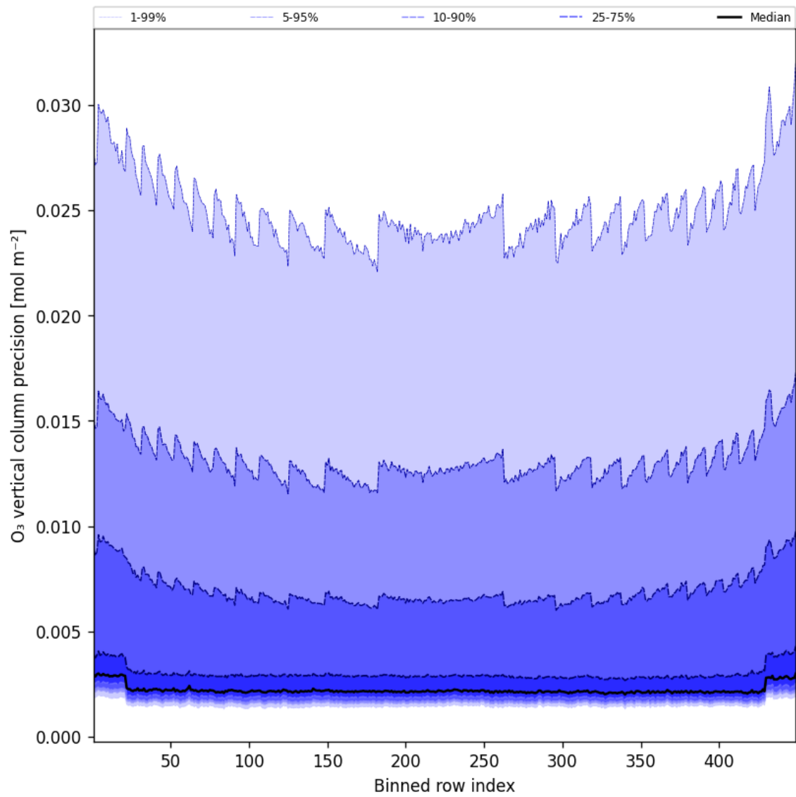
Figure 42: Along track statistics of “O 3 vertical column precision” for 2025-01-19 to 2025-01-20
