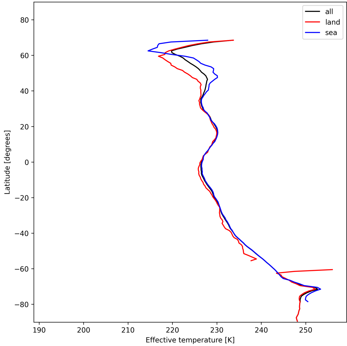
Figure 26: Zonal average of "Effective temperature" for 2025-01-19 to 2025-01-20.
