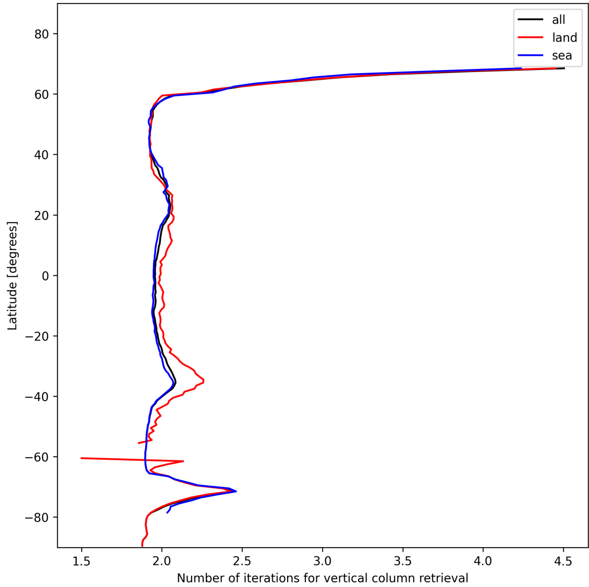
Figure 27: Zonal average of “Number of iterations for vertical column retrieval” for 2025-01-19 to 2025-01-20.
