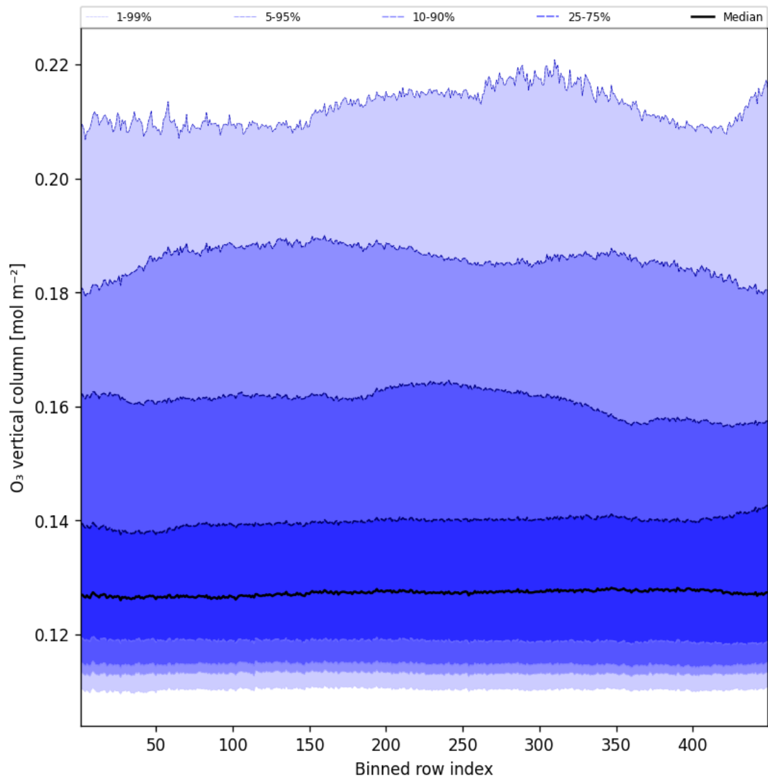
Figure 41: Along track statistics of “O 3 vertical column” for 2025-01-19 to 2025-01-20
