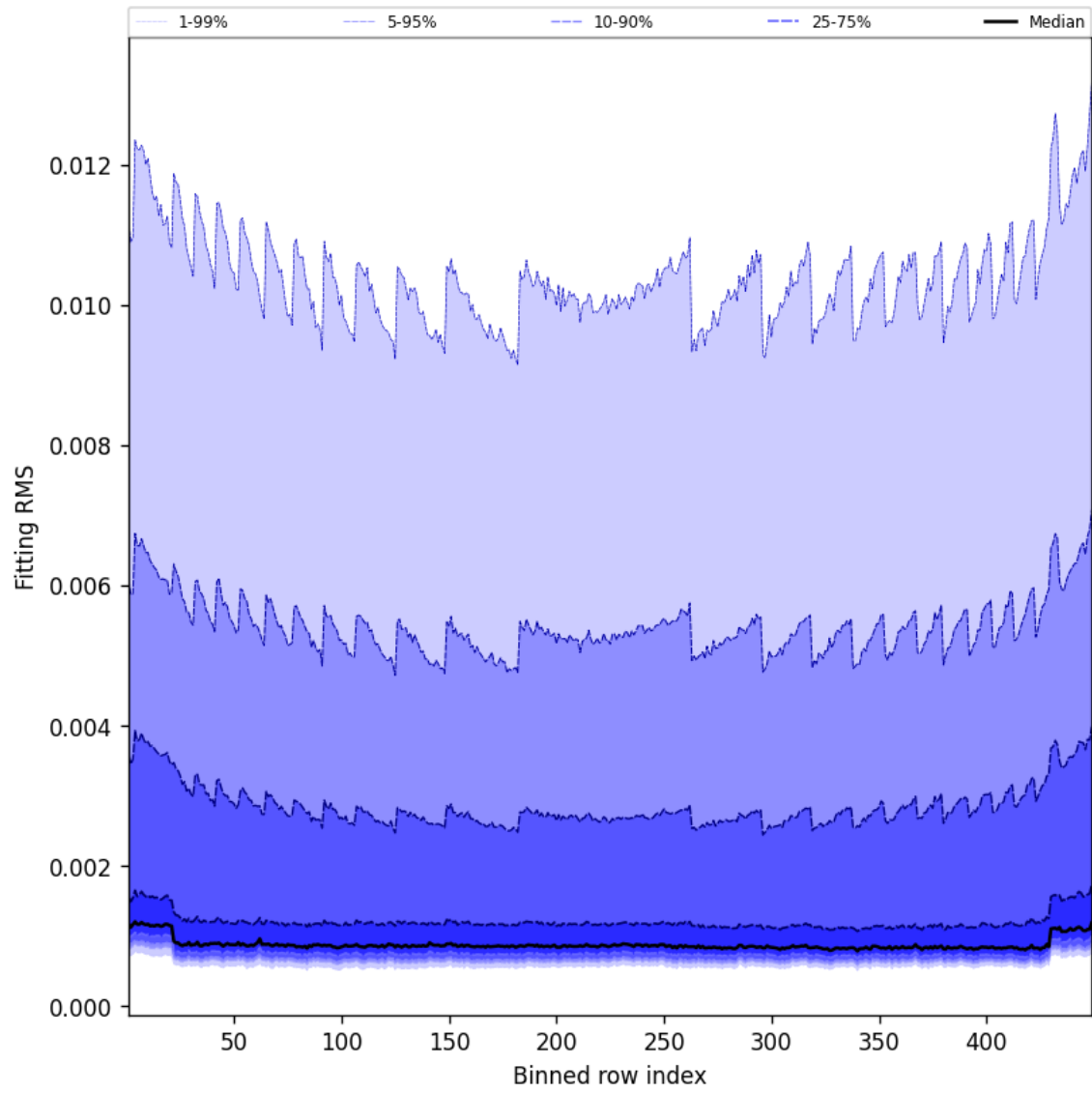
Figure 46: Along track statistics of “Fitting RMS” for 2025-01-19 to 2025-01-20
