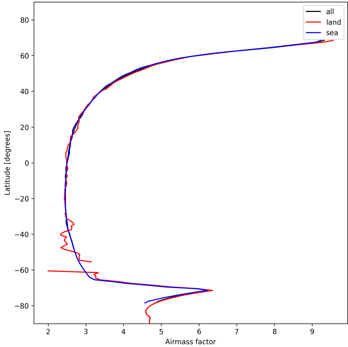
Figure 25: Zonal average of “Airmass factor” for 2025-01-19 to 2025-01-20.
