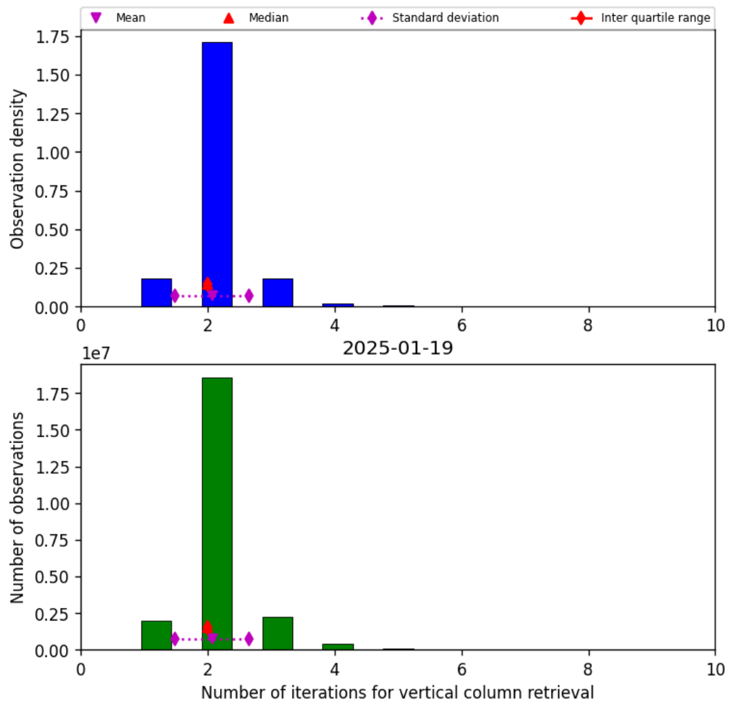
Figure 39: Histogram of “Number of iterations for vertical column retrieval” for 2025-01-19 to 2025-01-20
