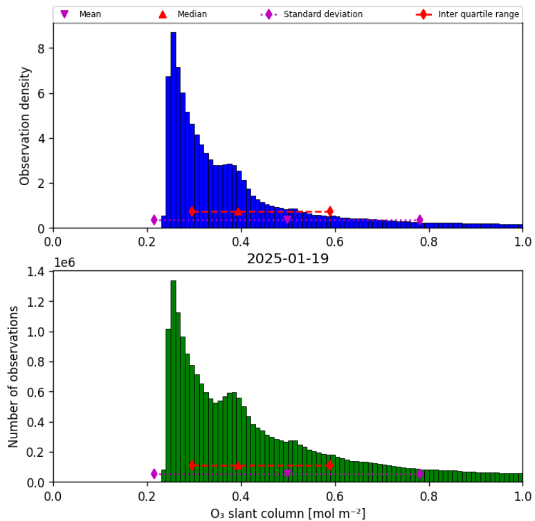
Figure 31: Histogram of “O 3 slant column” for 2025-01-19 to 2025-01-20
