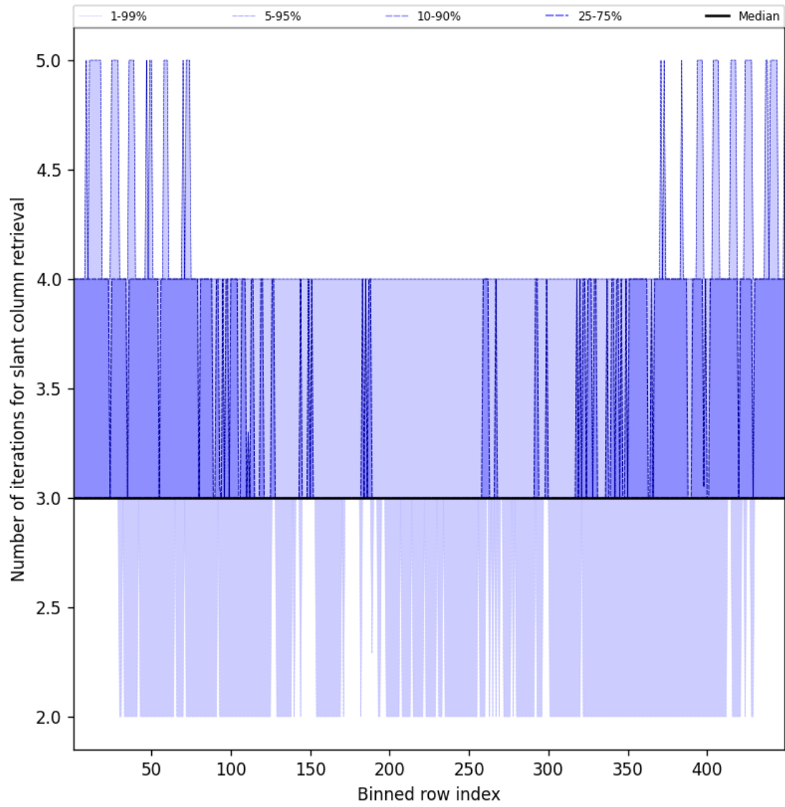
Figure 45: Along track statistics of “Number of iterations for slant column retrieval” for 2025-01-19 to 2025-01-20
