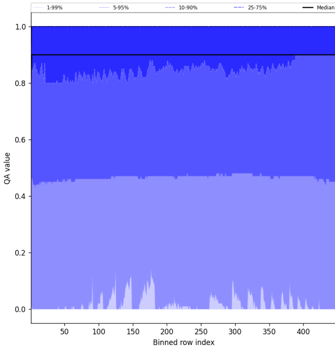
Figure 40: Along track statistics of “QA value” for 2025-01-19 to 2025-01-20
