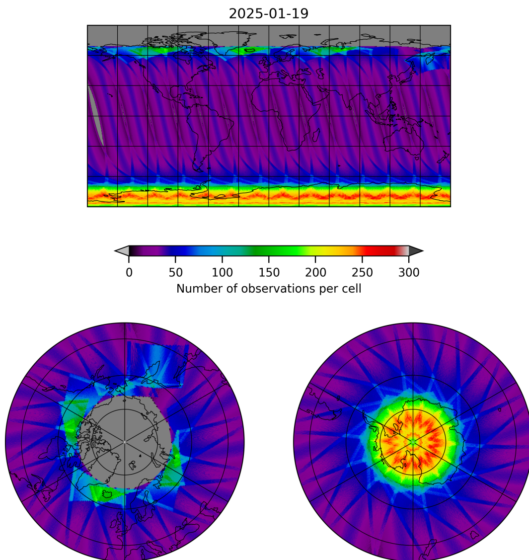
Figure 15: Map of the number of observations for 2025-01-19 to 2025-01-20
