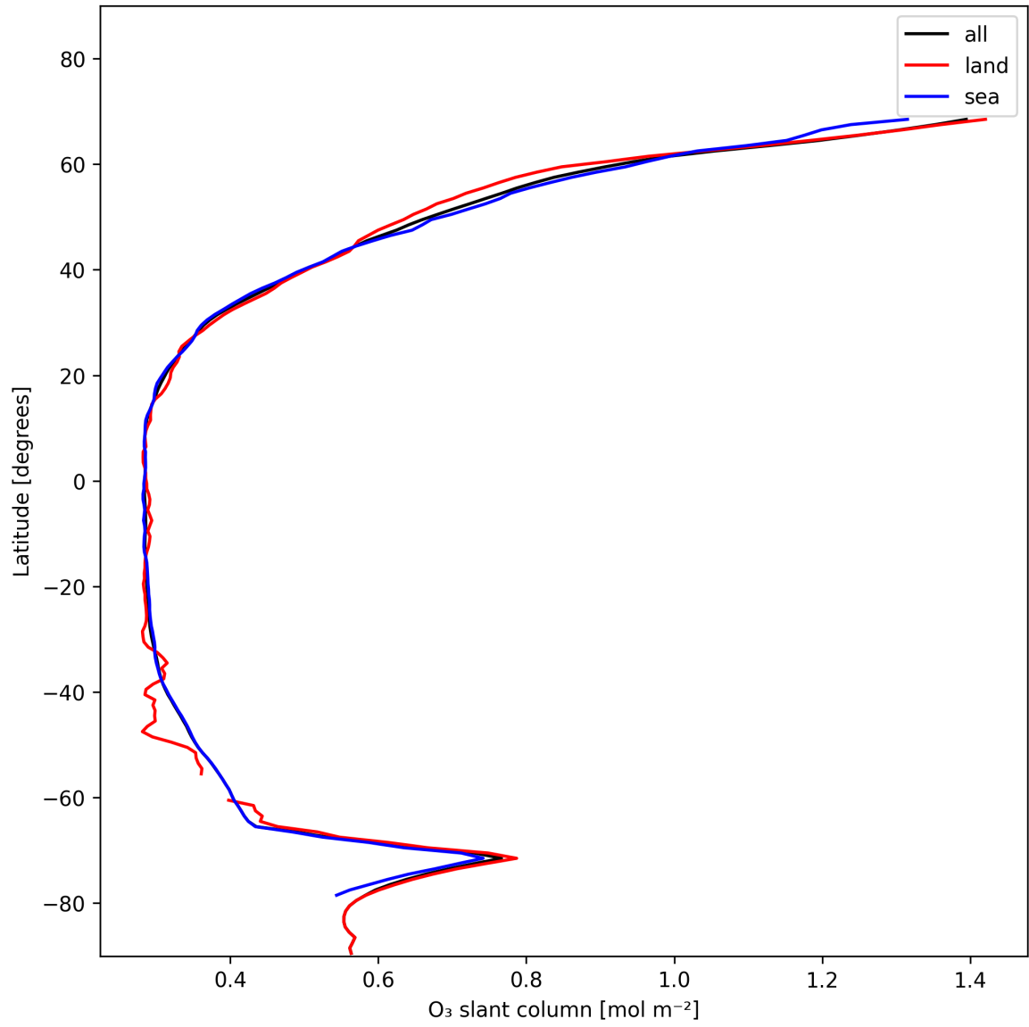
Figure 19: Zonal average of “O 3 slant column” for 2025-01-19 to 2025-01-20.
