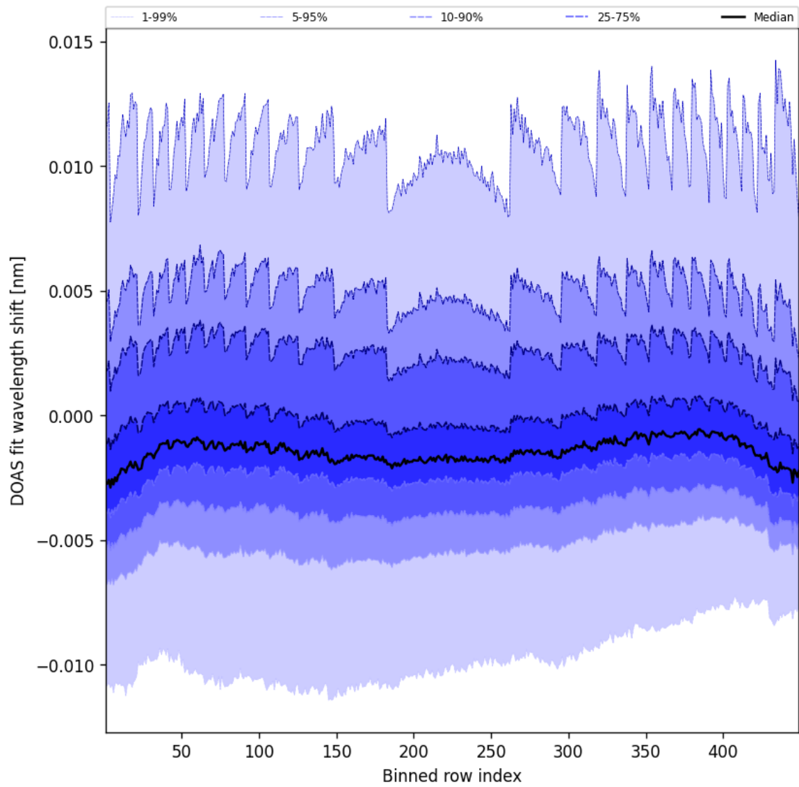
Figure 47: Along track statistics of “DOAS fit wavelength shift” for 2025-01-19 to 2025-01-20
