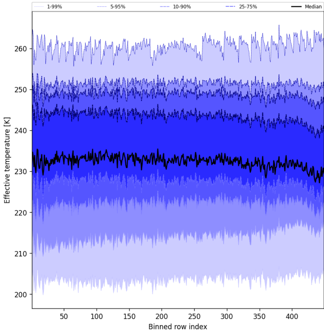
Figure 50: Along track statistics of “Effective temperature” for 2025-01-19 to 2025-01-20
