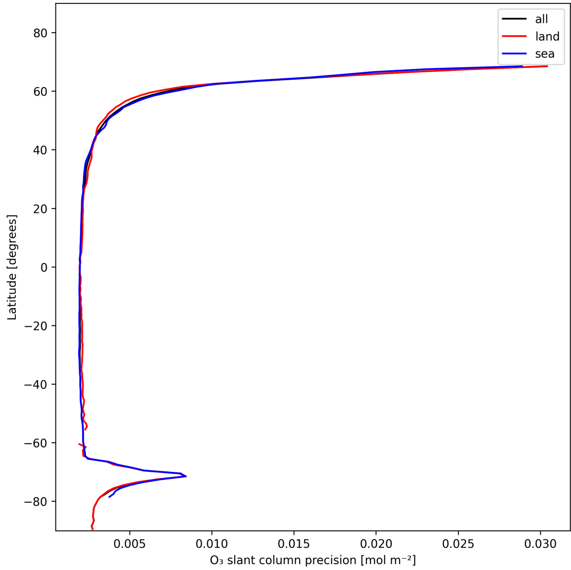
Figure 20: Zonal average of “O 3 slant column precision” for 2025-01-19 to 2025-01-20.
