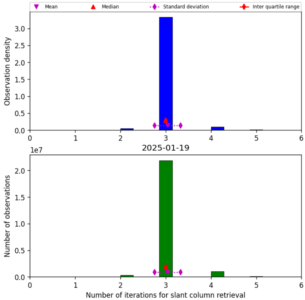
Figure 33: Histogram of “Number of iterations for slant column retrieval” for 2025-01-19 to 2025-01-20
