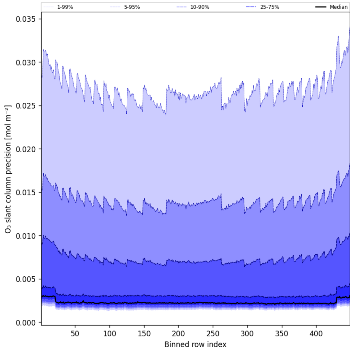
Figure 44: Along track statistics of “O 3 slant column precision” for 2025-01-19 to 2025-01-20
