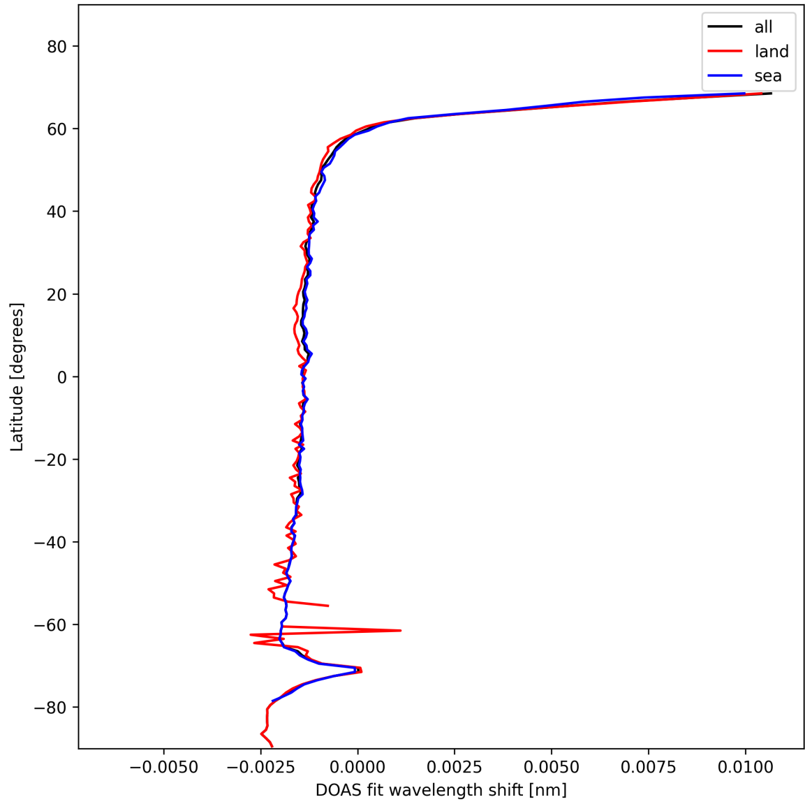
Figure 23: Zonal average of "DOAS fit wavelength shift" for 2025-01-19 to 2025-01-20.
