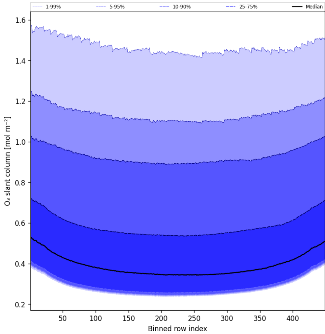
Figure 43: Along track statistics of “O 3 slant column” for 2025-01-19 to 2025-01-20
