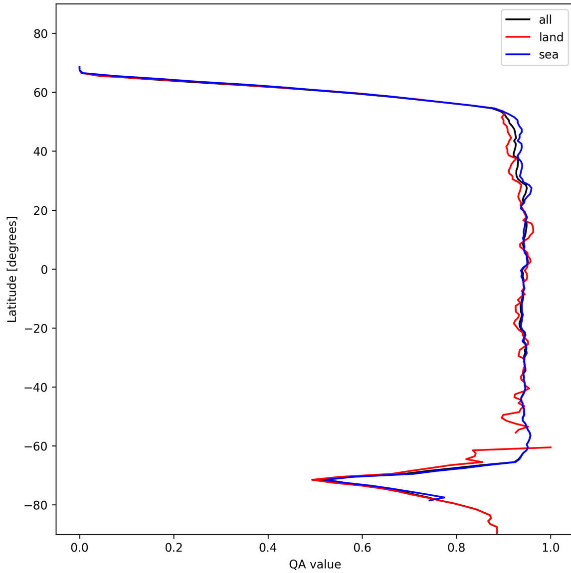
Figure 16: Zonal average of “QA value” for 2025-01-19 to 2025-01-20.
