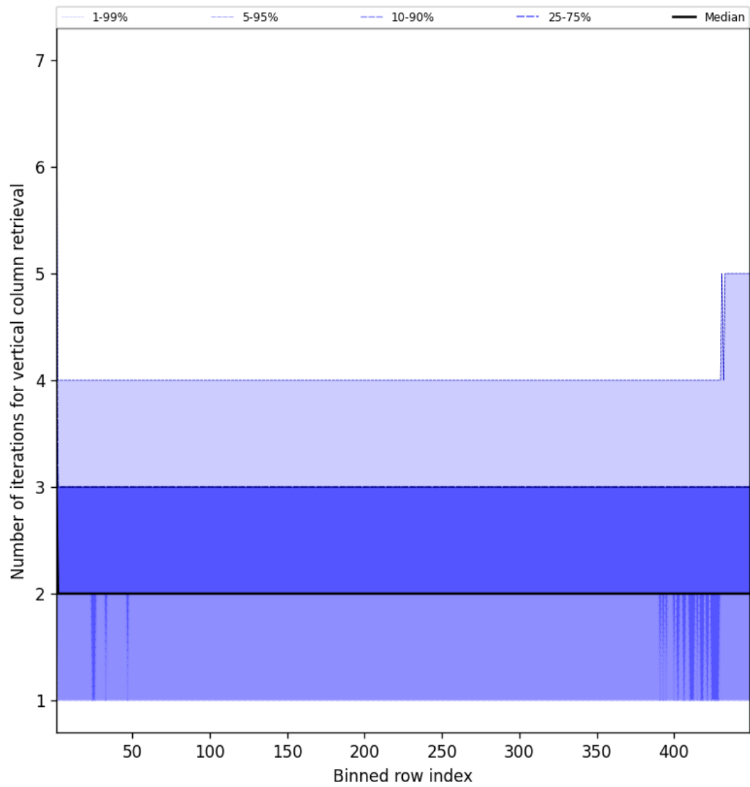
Figure 51: Along track statistics of “Number of iterations for vertical column retrieval” for 2025-01-19 to 2025-01-20
