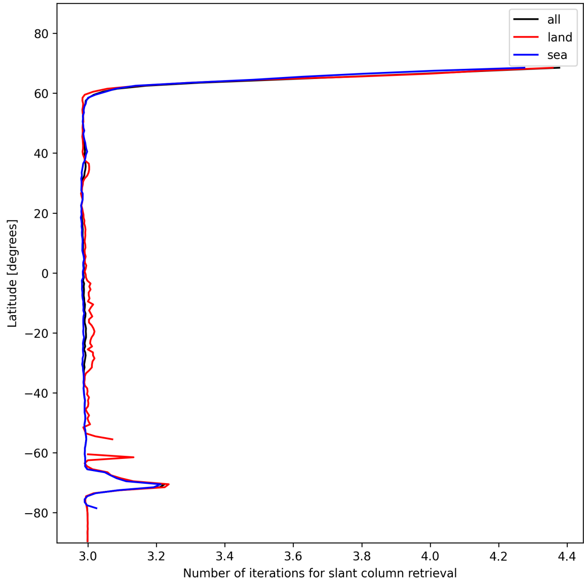
Figure 21: Zonal average of “Number of iterations for slant column retrieval” for 2025-01-19 to 2025-01-20.
