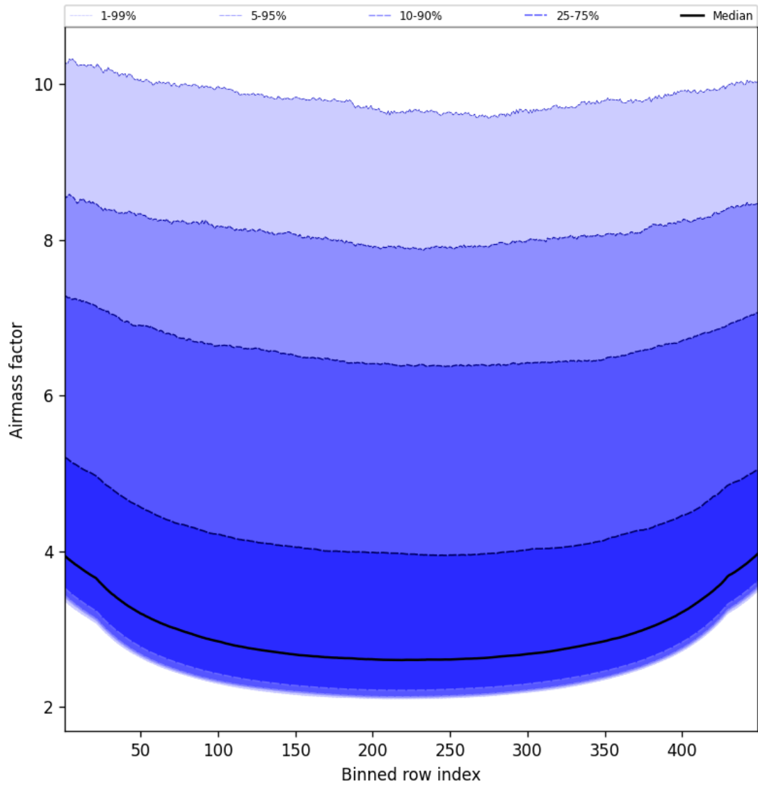
Figure 49: Along track statistics of “Airmass factor” for 2025-01-19 to 2025-01-20
