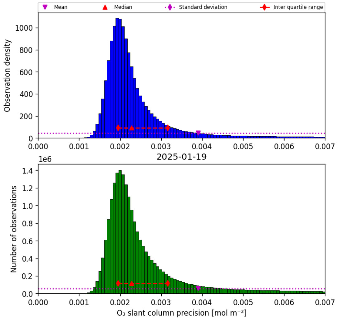
Figure 32: Histogram of “O 3 slant column precision” for 2025-01-19 to 2025-01-20
