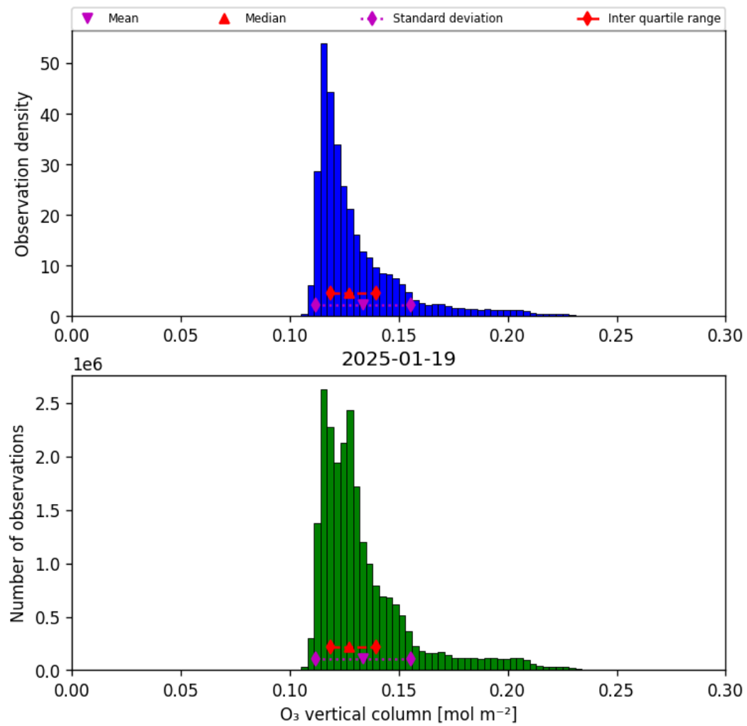
Figure 29: Histogram of “O 3 vertical column” for 2025-01-19 to 2025-01-20
