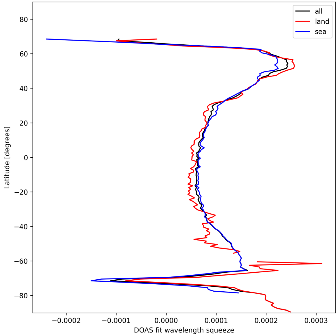
Figure 24: Zonal average of “DOAS fit wavelength squeeze” for 2025-01-19 to 2025-01-20.
