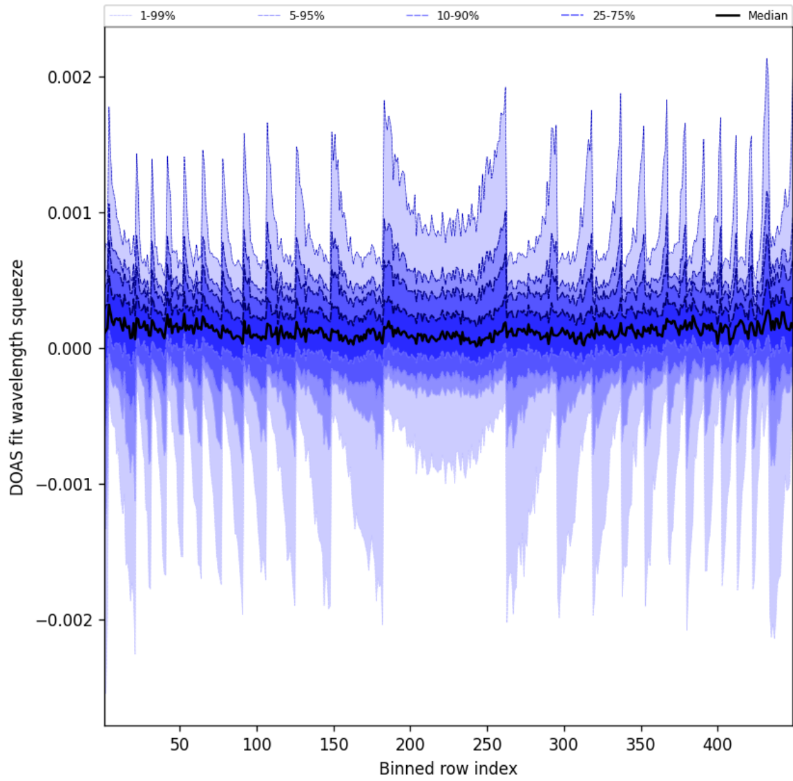
Figure 48: Along track statistics of “DOAS fit wavelength squeeze” for 2025-01-19 to 2025-01-20
