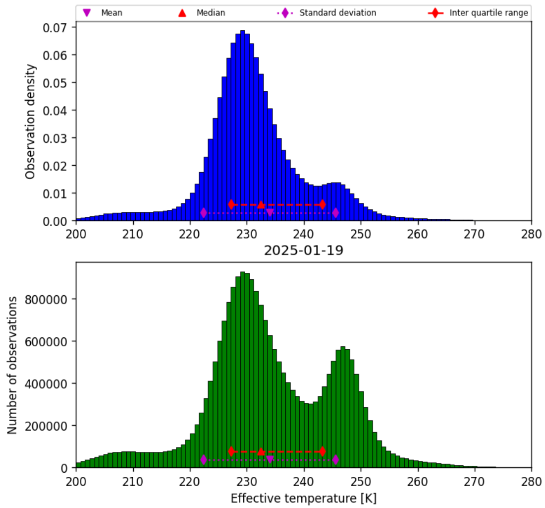
Figure 38: Histogram of “Effective temperature” for 2025-01-19 to 2025-01-20
