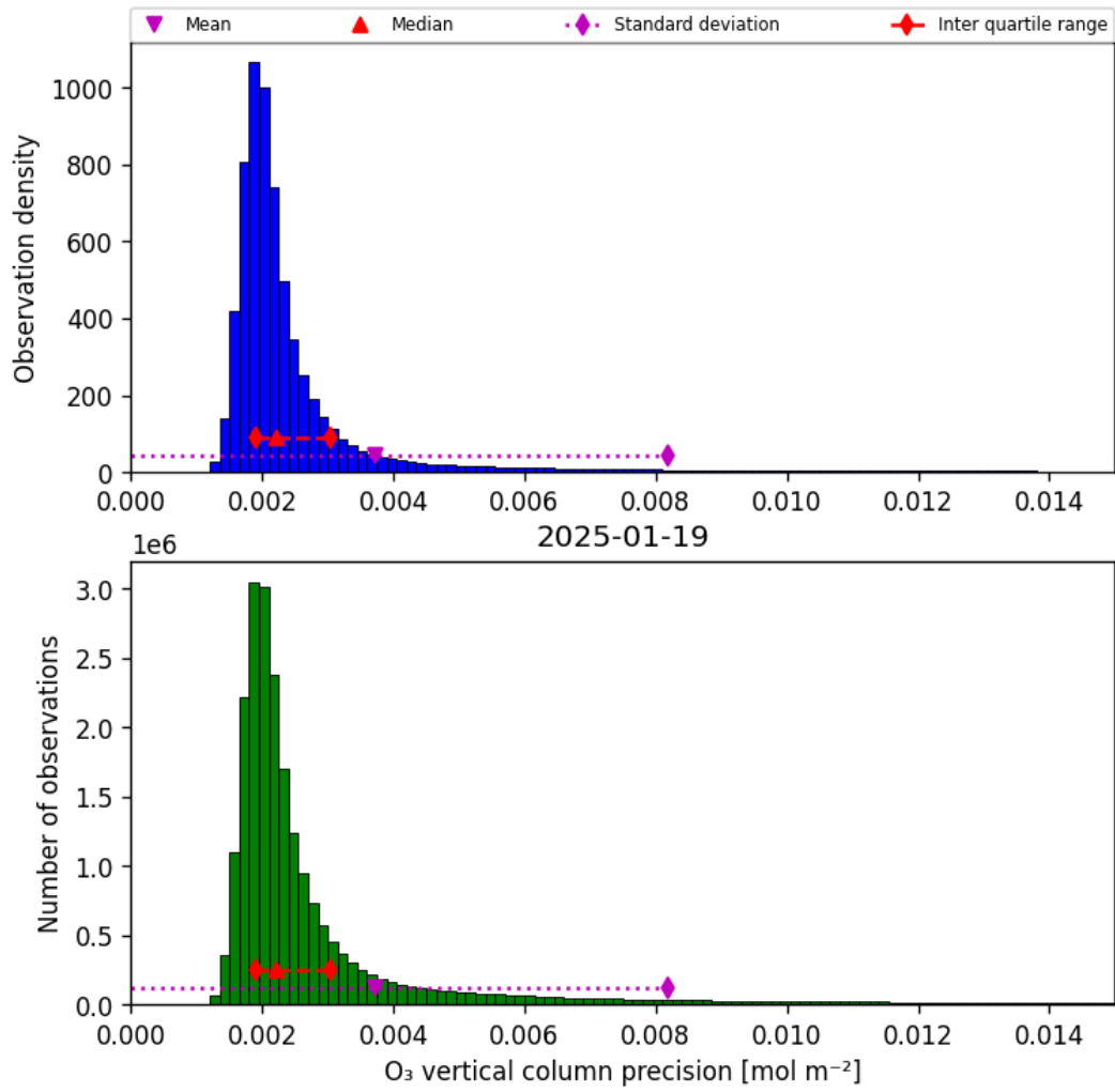
Figure 30: Histogram of “O 3 vertical column precision” for 2025-01-19 to 2025-01-20
