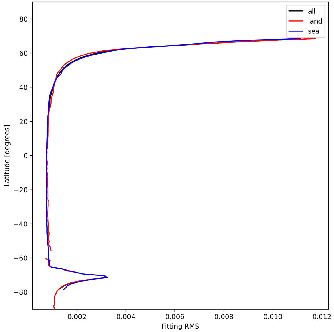
Figure 22: Zonal average of “Fitting RMS” for 2025-01-19 to 2025-01-20.
