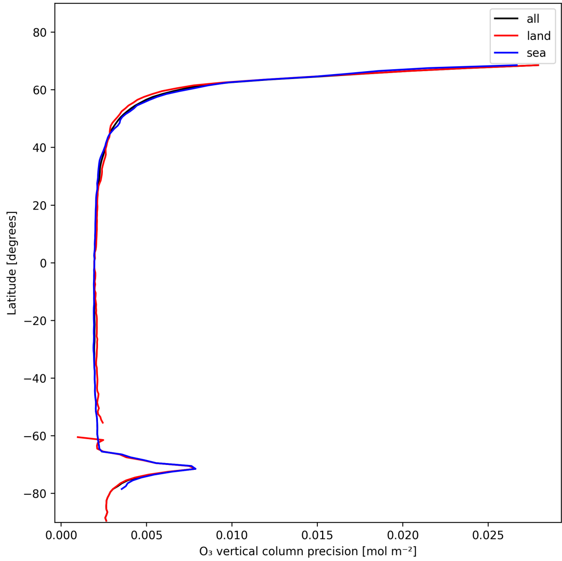
Figure 18: Zonal average of “O 3 vertical column precision” for 2025-01-19 to 2025-01-20.
