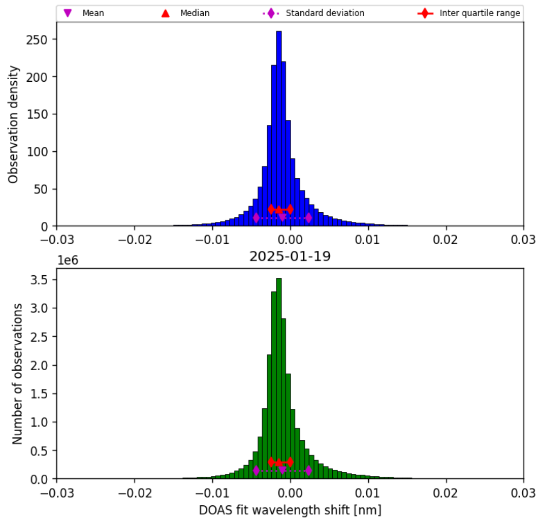
Figure 35: Histogram of “DOAS fit wavelength shift” for 2025-01-19 to 2025-01-20
