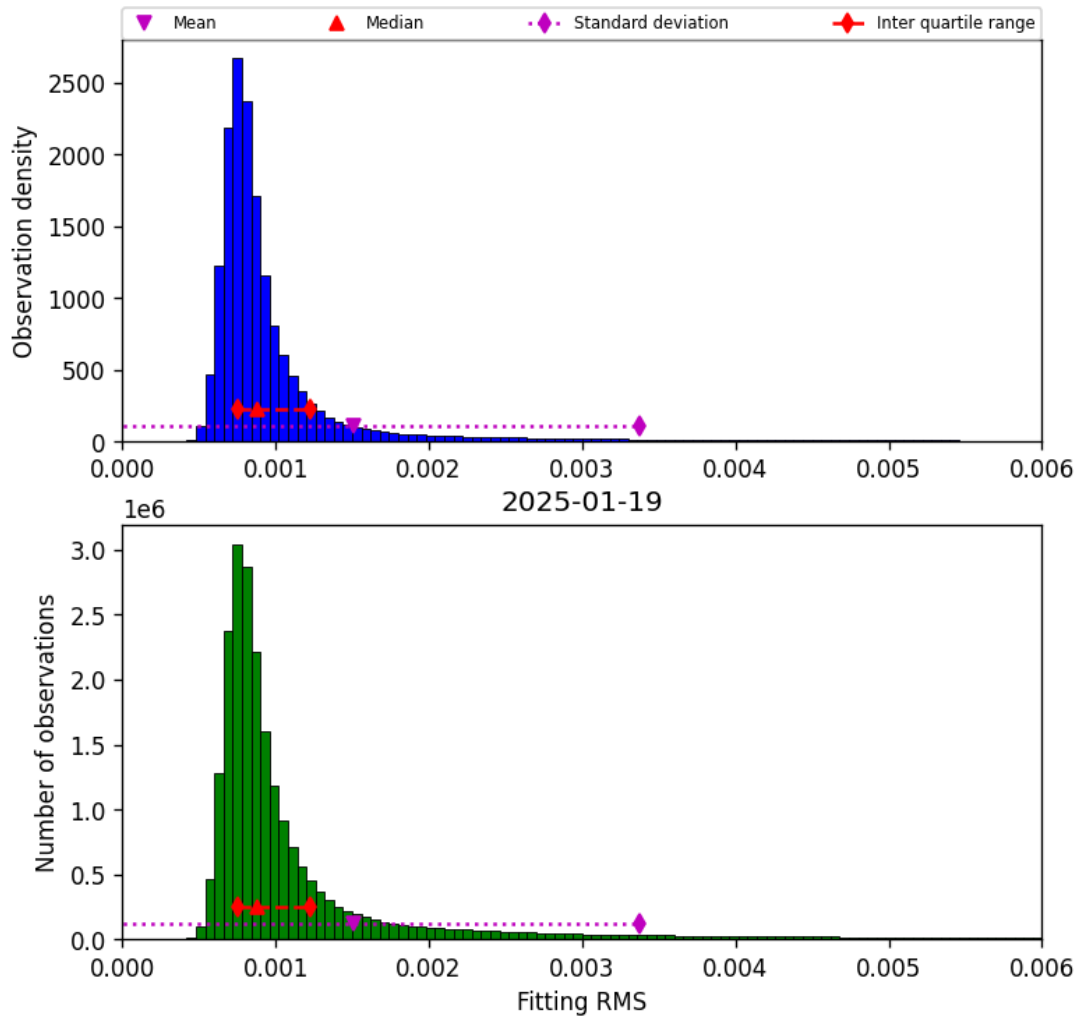
Figure 34: Histogram of “Fitting RMS” for 2025-01-19 to 2025-01-20
