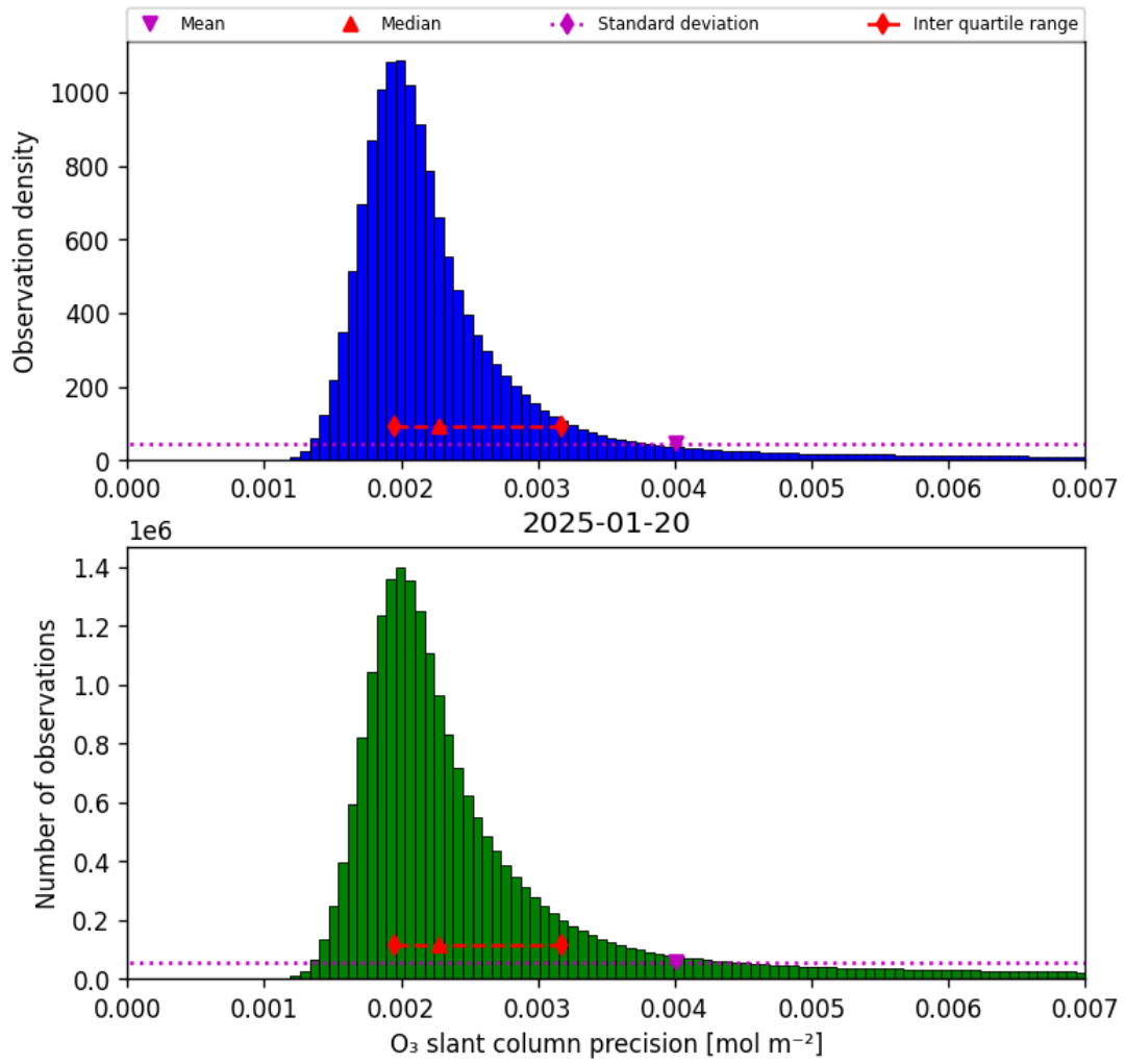
Figure 32: Histogram of “O 3 slant column precision” for 2025-01-20 to 2025-01-21
