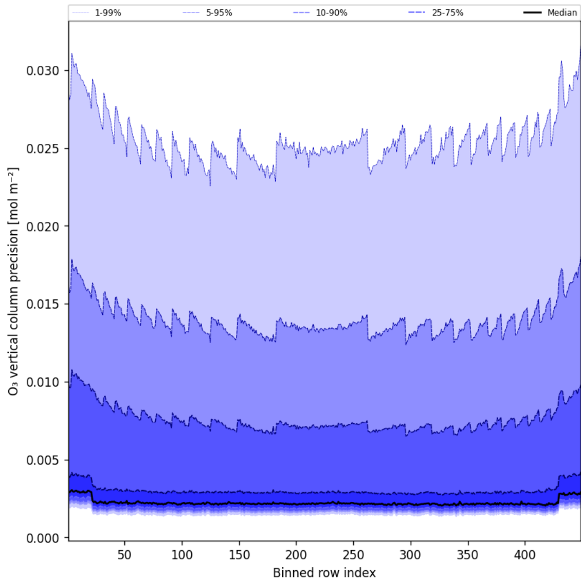
Figure 42: Along track statistics of “O 3 vertical column precision” for 2025-01-20 to 2025-01-21
