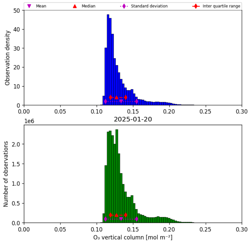
Figure 29: Histogram of “O 3 vertical column” for 2025-01-20 to 2025-01-21
