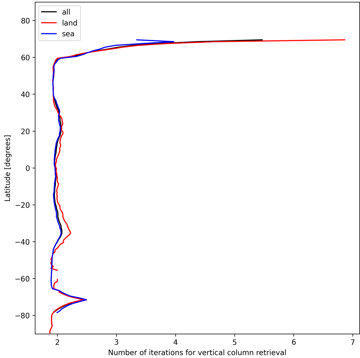
Figure 27: Zonal average of “Number of iterations for vertical column retrieval” for 2025-01-20 to 2025-01-21.
