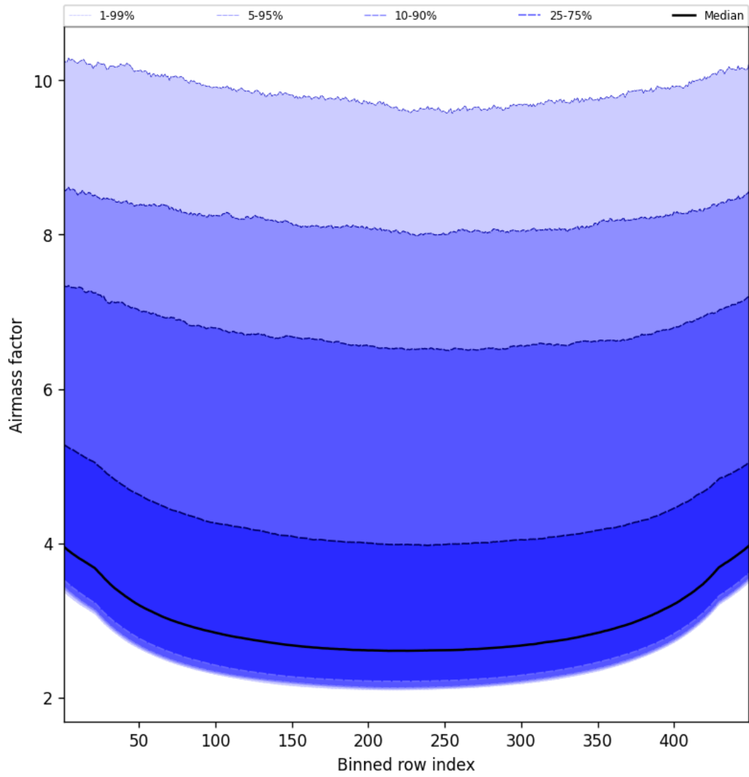
Figure 49: Along track statistics of “Airmass factor” for 2025-01-20 to 2025-01-21
