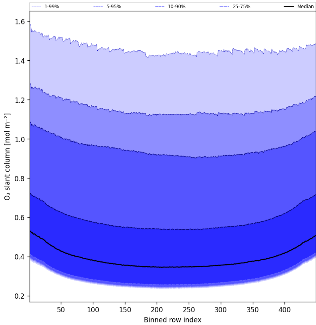
Figure 43: Along track statistics of “O 3 slant column” for 2025-01-20 to 2025-01-21
