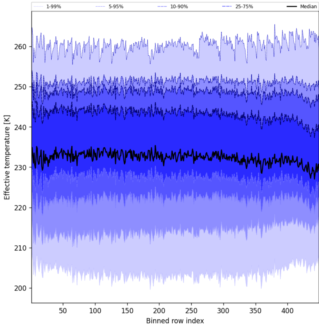
Figure 50: Along track statistics of “Effective temperature” for 2025-01-20 to 2025-01-21
