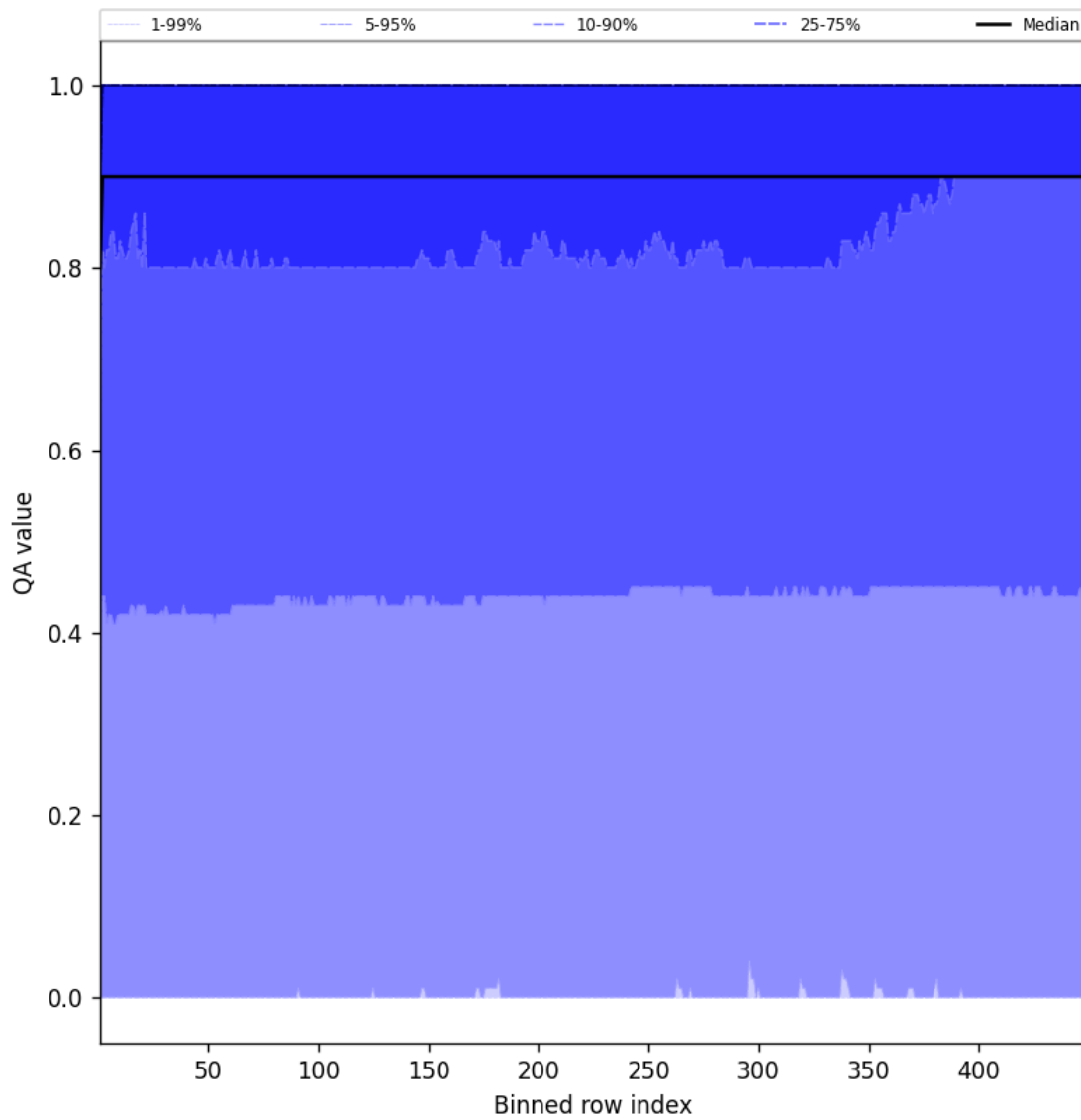
Figure 40: Along track statistics of “QA value” for 2025-01-20 to 2025-01-21
