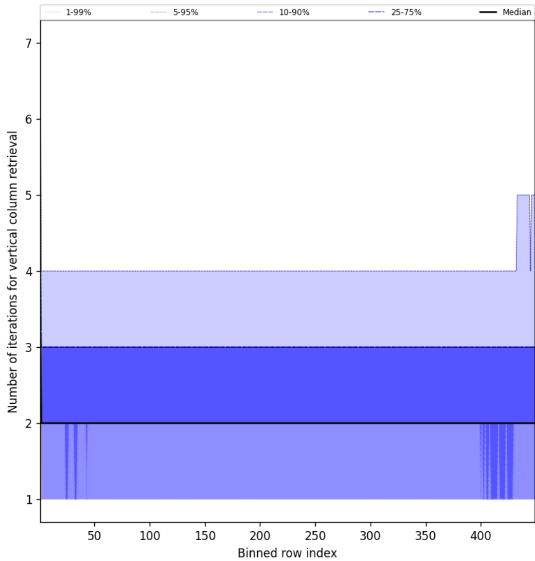
Figure 51: Along track statistics of “Number of iterations for vertical column retrieval” for 2025-01-20 to 2025-01-21
