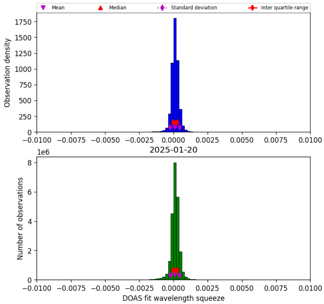
Figure 36: Histogram of “DOAS fit wavelength squeeze” for 2025-01-20 to 2025-01-21
