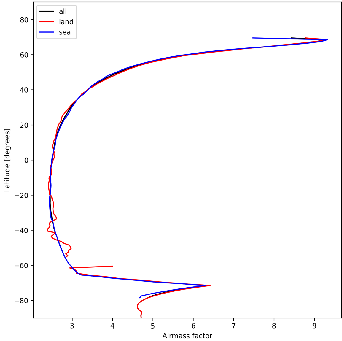
Figure 25: Zonal average of “Airmass factor” for 2025-01-20 to 2025-01-21.
