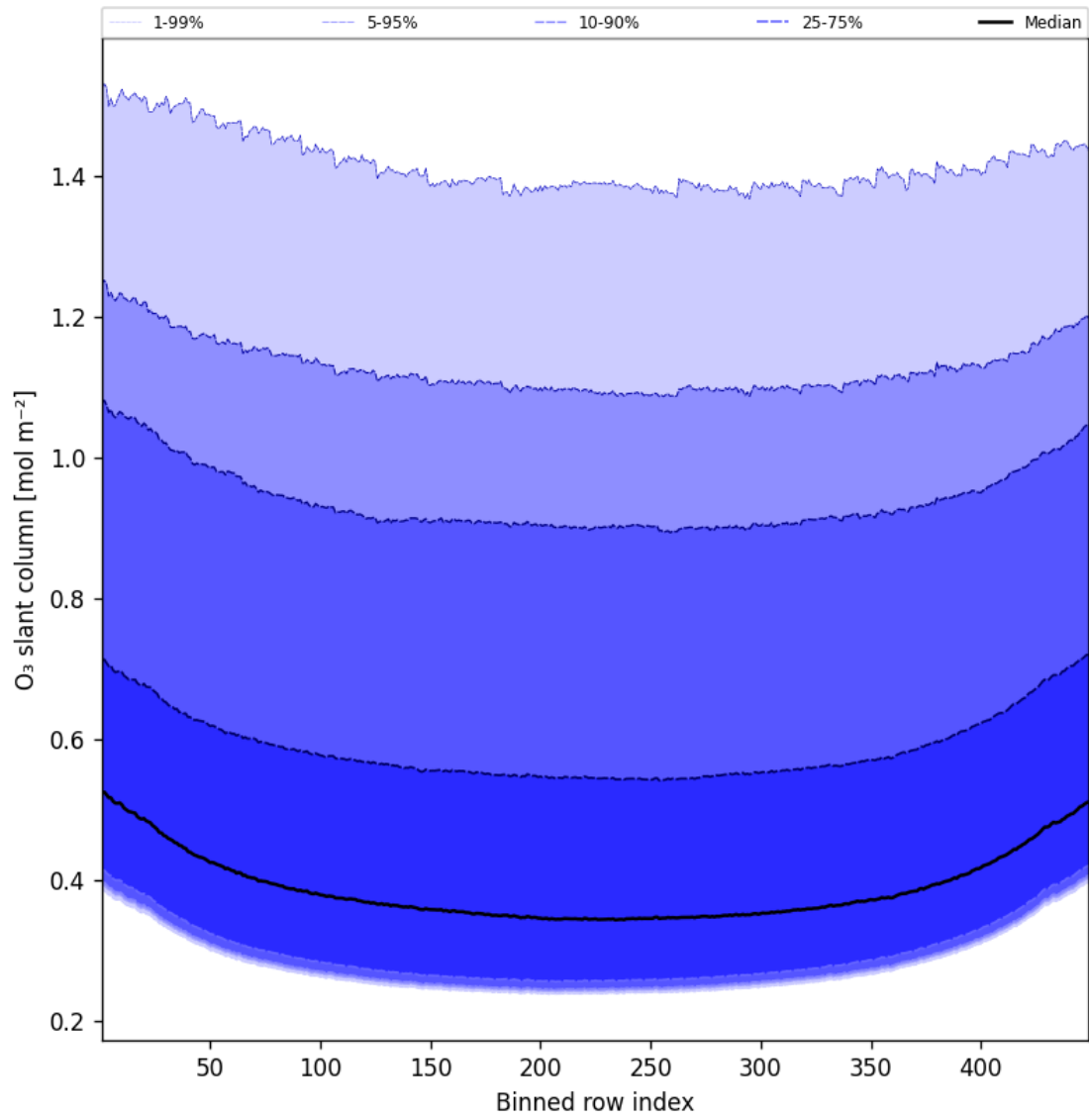
Figure 43: Along track statistics of “O 3 slant column” for 2025-01-21 to 2025-01-21
