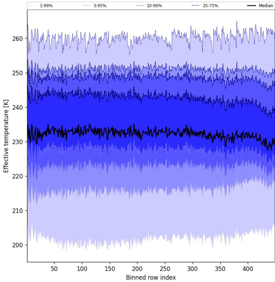
Figure 50: Along track statistics of “Effective temperature” for 2025-01-21 to 2025-01-21
