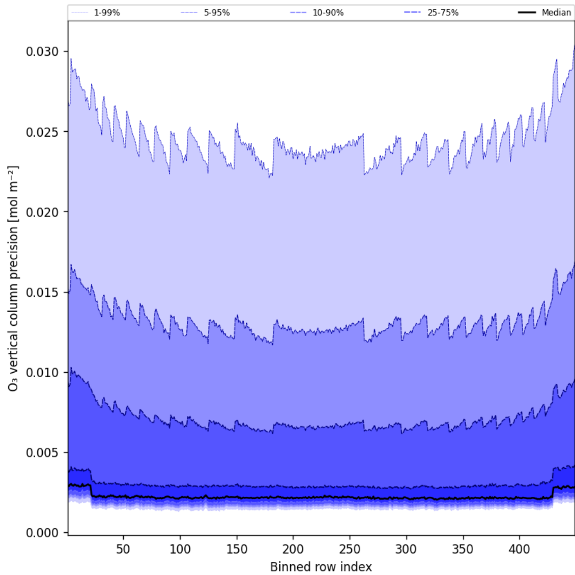
Figure 42: Along track statistics of “O 3 vertical column precision” for 2025-01-21 to 2025-01-21
