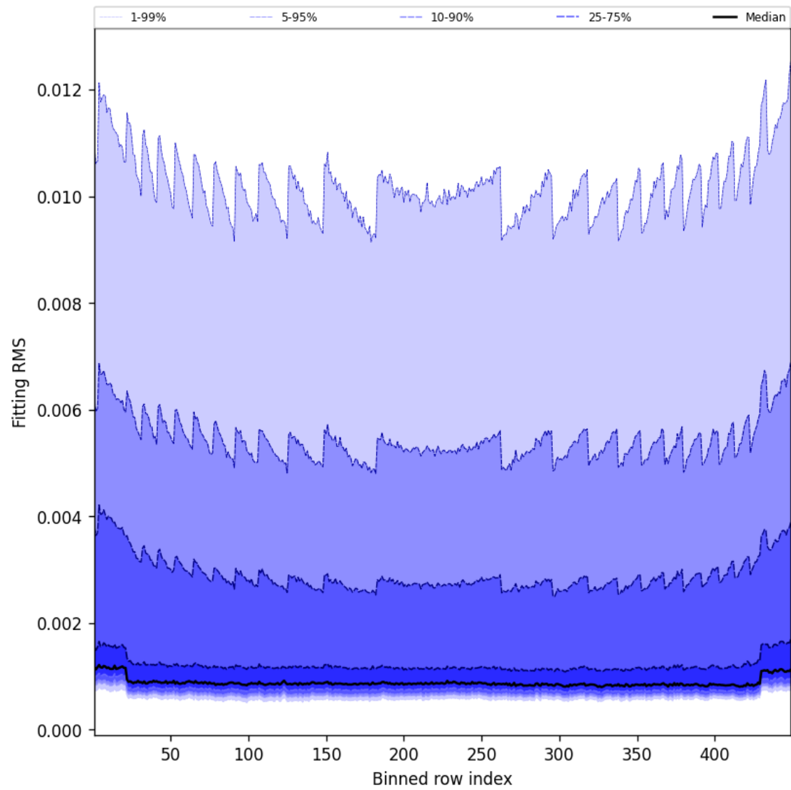
Figure 46: Along track statistics of “Fitting RMS” for 2025-01-21 to 2025-01-21
