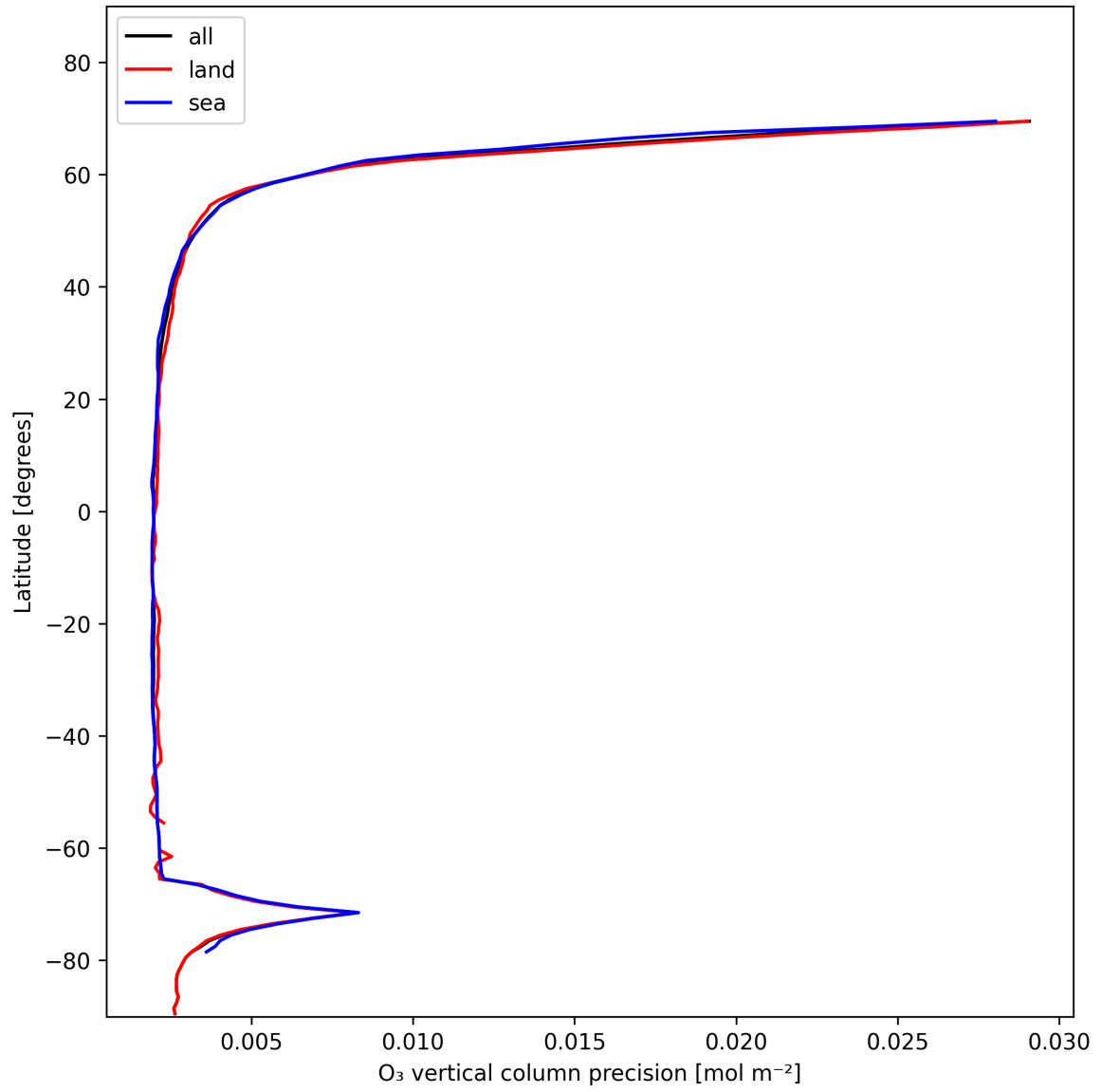
Figure 18: Zonal average of “O 3 vertical column precision” for 2025-01-21 to 2025-01-21.
