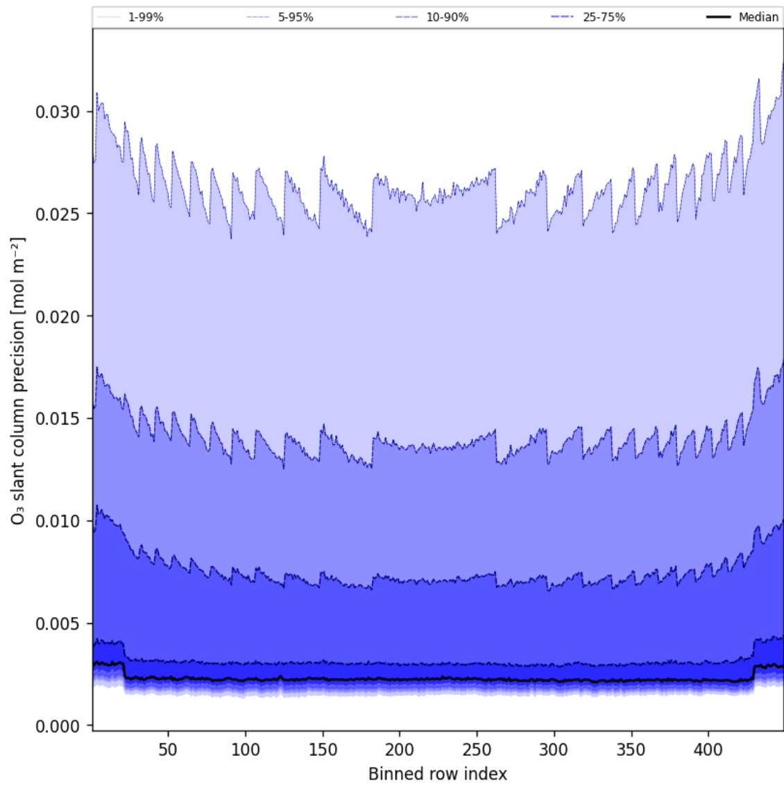
Figure 44: Along track statistics of “O 3 slant column precision” for 2025-01-21 to 2025-01-21
