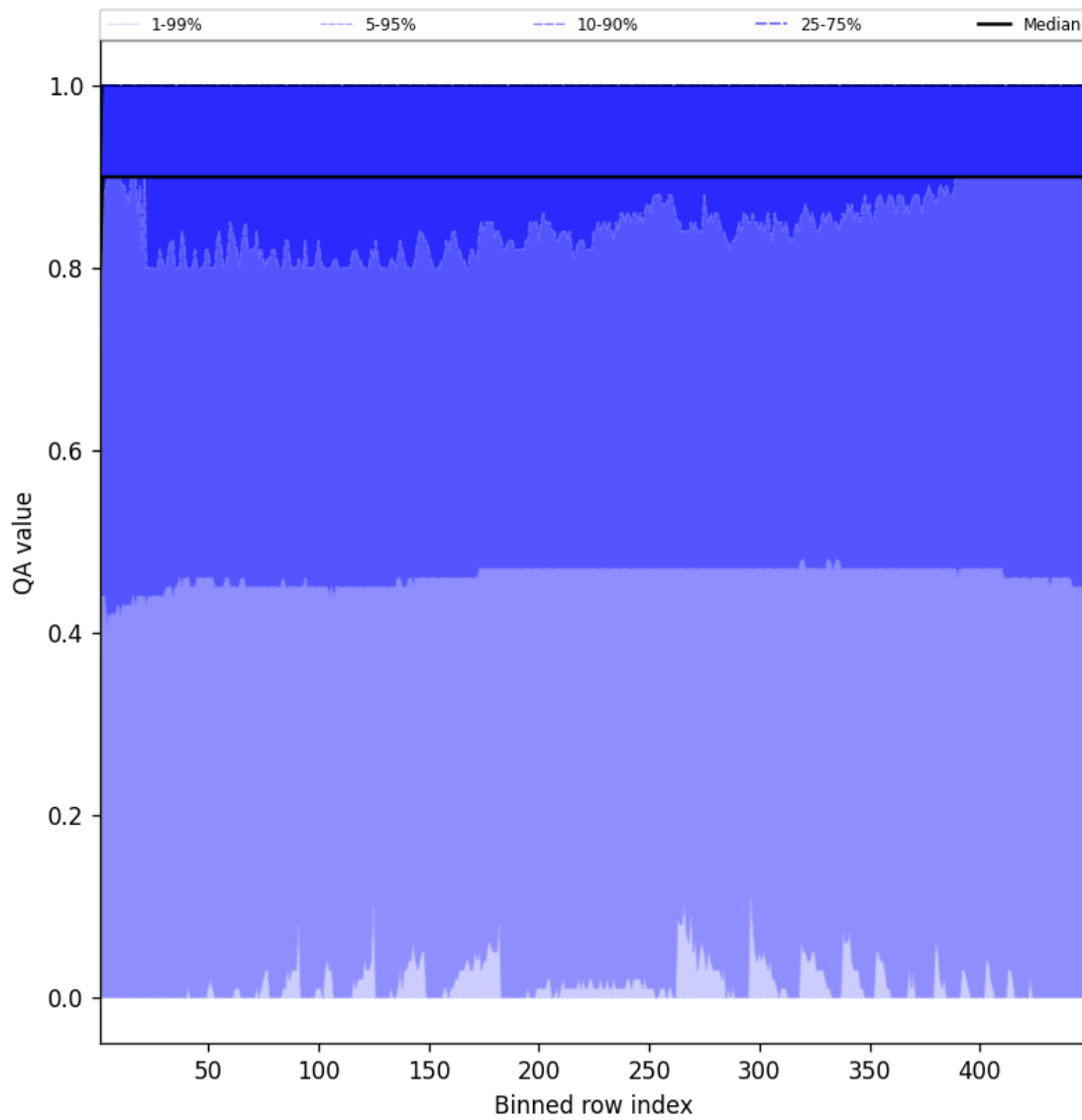
Figure 40: Along track statistics of “QA value” for 2025-01-21 to 2025-01-21
