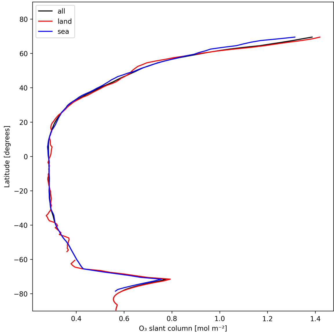
Figure 19: Zonal average of “O 3 slant column” for 2025-01-21 to 2025-01-21.
