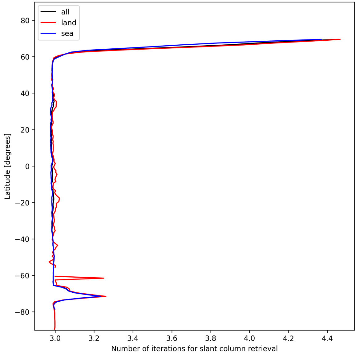
Figure 21: Zonal average of “Number of iterations for slant column retrieval” for 2025-01-21 to 2025-01-21.
