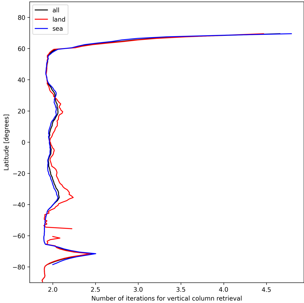
Figure 27: Zonal average of “Number of iterations for vertical column retrieval” for 2025-01-21 to 2025-01-21.
