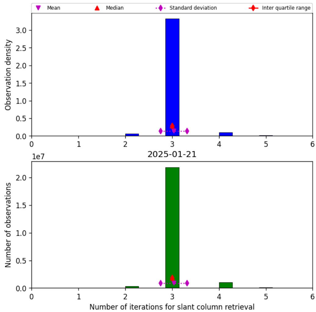
Figure 33: Histogram of “Number of iterations for slant column retrieval” for 2025-01-21 to 2025-01-21
