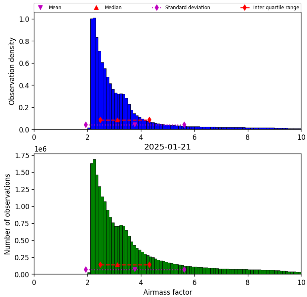
Figure 37: Histogram of “Airmass factor” for 2025-01-21 to 2025-01-21
