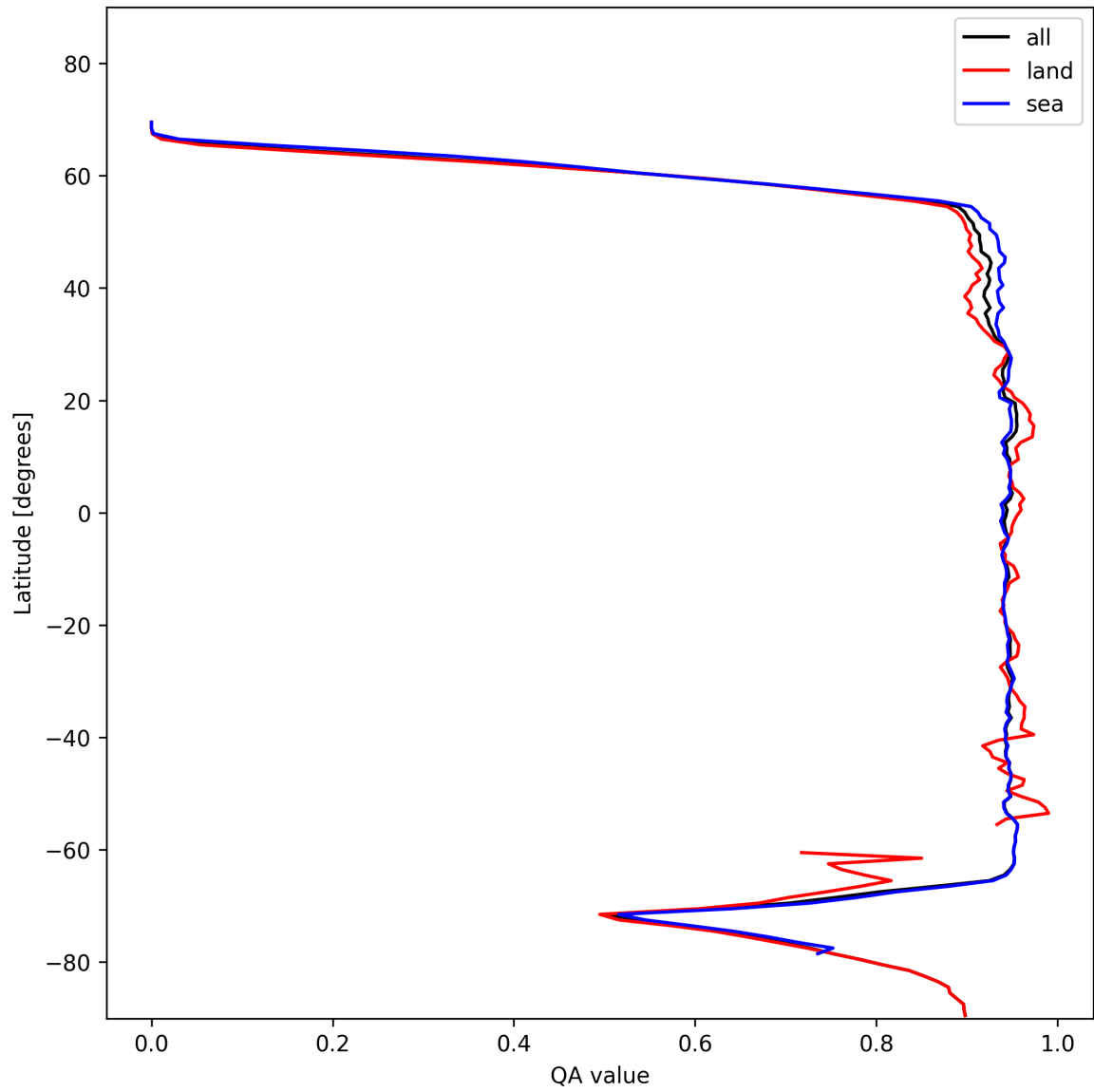
Figure 16: Zonal average of “QA value” for 2025-01-21 to 2025-01-21.
