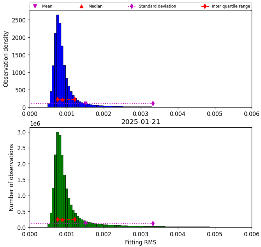
Figure 34: Histogram of “Fitting RMS” for 2025-01-21 to 2025-01-21
