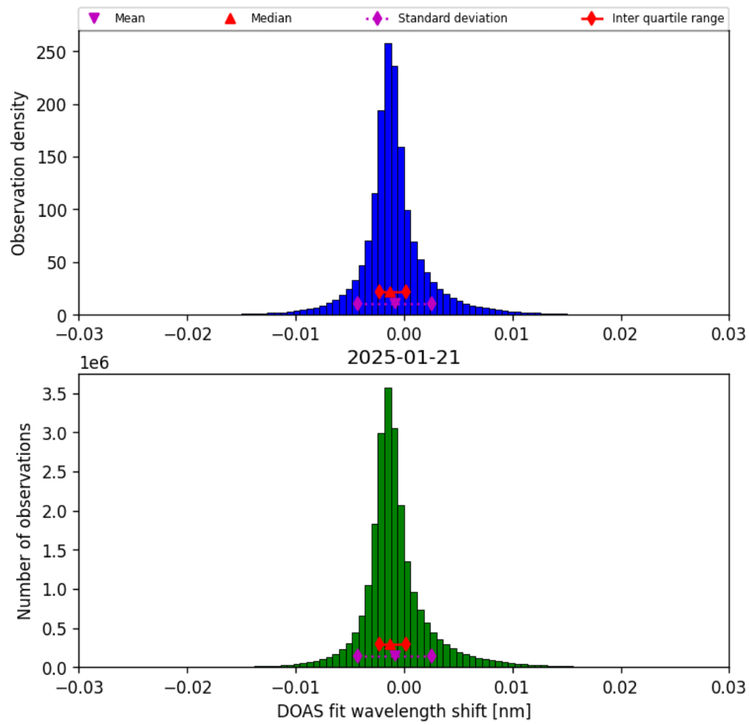
Figure 35: Histogram of “DOAS fit wavelength shift” for 2025-01-21 to 2025-01-21
