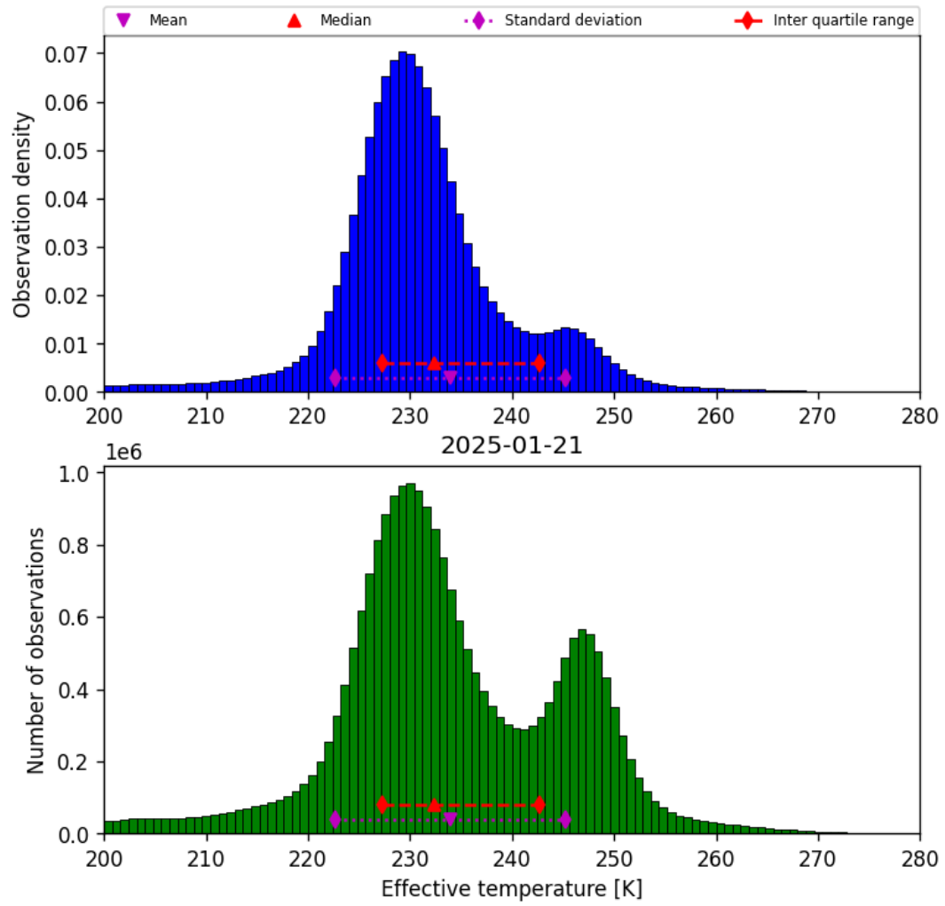
Figure 38: Histogram of “Effective temperature” for 2025-01-21 to 2025-01-21
