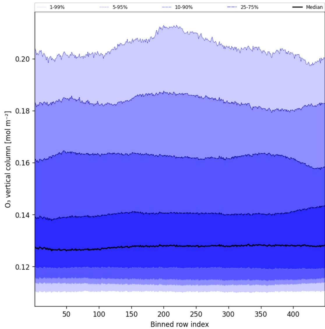
Figure 41: Along track statistics of “O 3 vertical column” for 2025-01-21 to 2025-01-21
