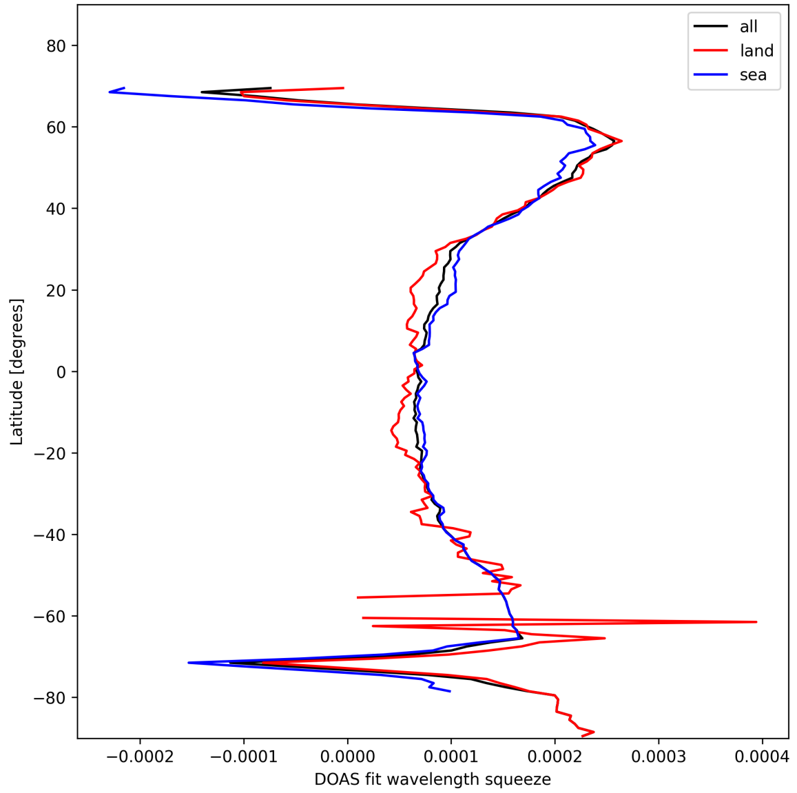
Figure 24: Zonal average of “DOAS fit wavelength squeeze” for 2025-01-21 to 2025-01-21.
