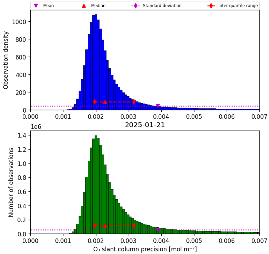
Figure 32: Histogram of “O 3 slant column precision” for 2025-01-21 to 2025-01-21
