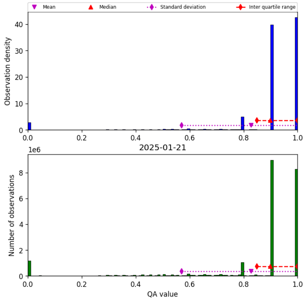
Figure 28: Histogram of “QA value” for 2025-01-21 to 2025-01-21
