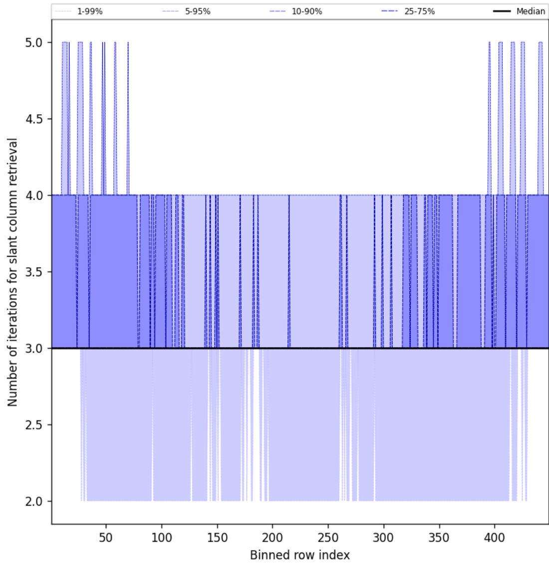
Figure 45: Along track statistics of “Number of iterations for slant column retrieval” for 2025-01-21 to 2025-01-21
