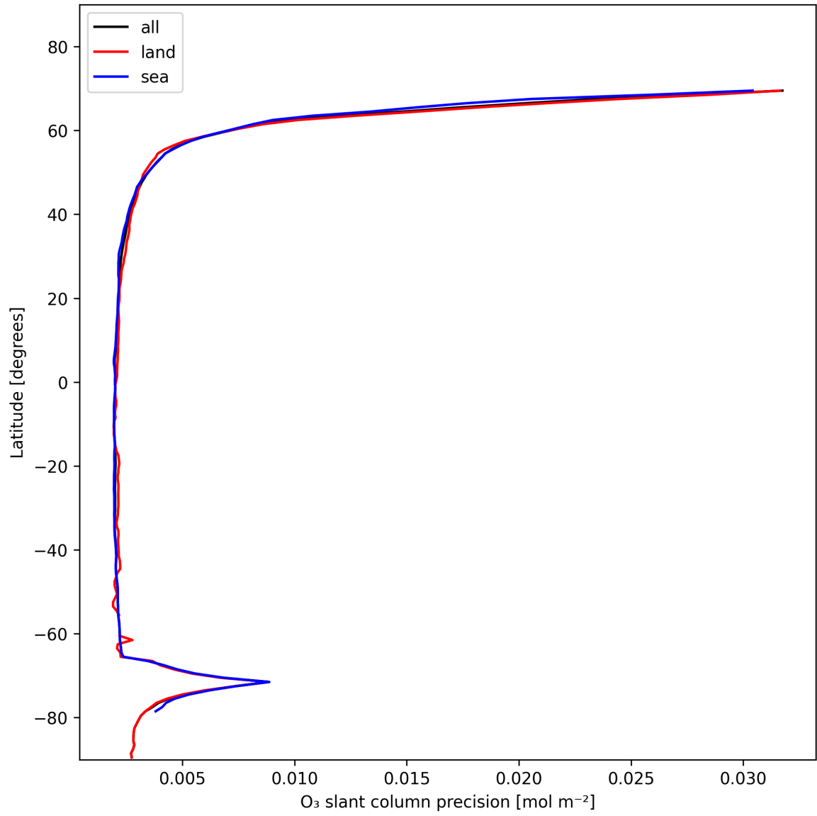
Figure 20: Zonal average of “O 3 slant column precision” for 2025-01-21 to 2025-01-21.
