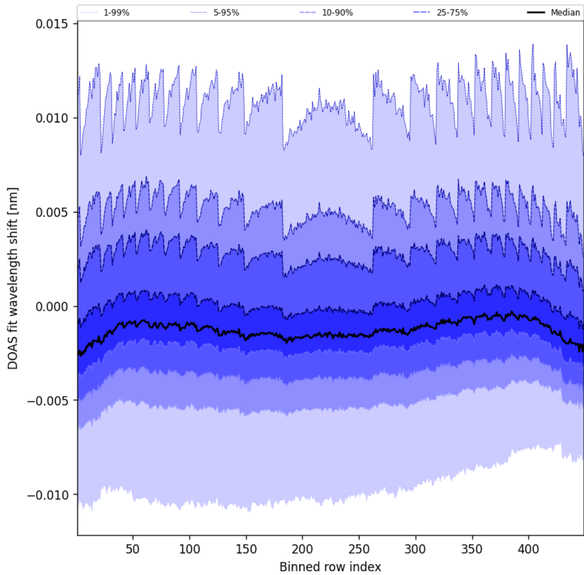
Figure 47: Along track statistics of "DOAS fit wavelength shift" for 2025-01-21 to 2025-01-21
