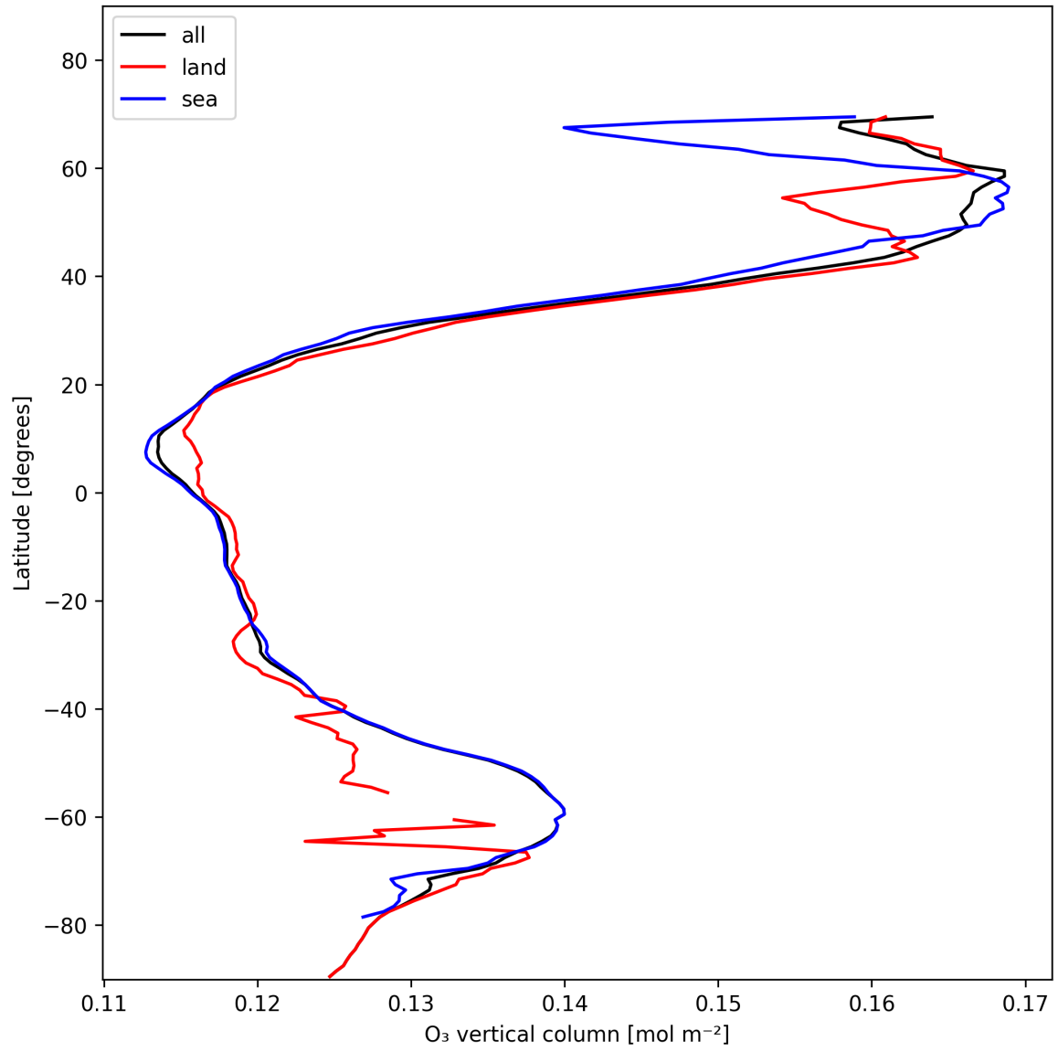
Figure 17: Zonal average of “O 3 vertical column” for 2025-01-21 to 2025-01-21.
