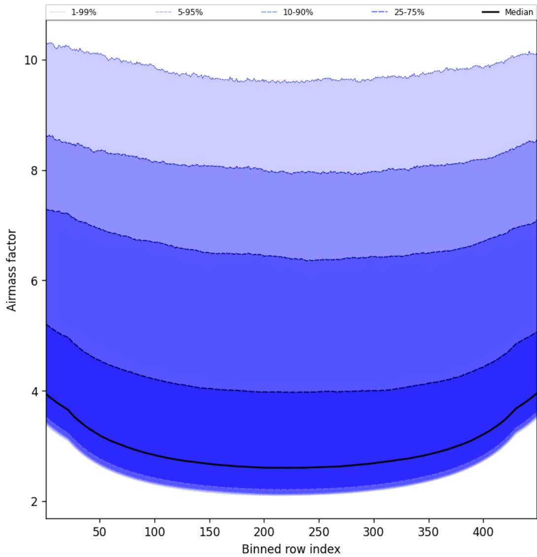
Figure 49: Along track statistics of “Airmass factor” for 2025-01-21 to 2025-01-21
