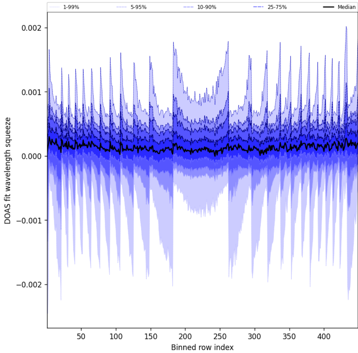
Figure 48: Along track statistics of “DOAS fit wavelength squeeze” for 2025-01-21 to 2025-01-21
