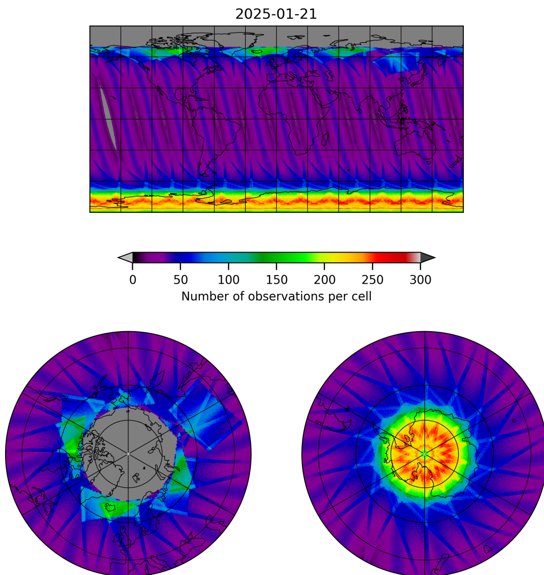
Figure 15: Map of the number of observations for 2025-01-21 to 2025-01-21
