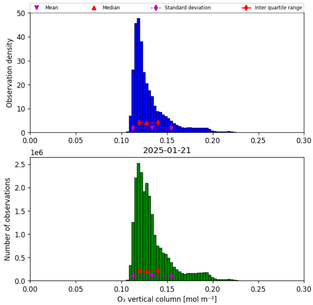
Figure 29: Histogram of “O 3 vertical column” for 2025-01-21 to 2025-01-21
