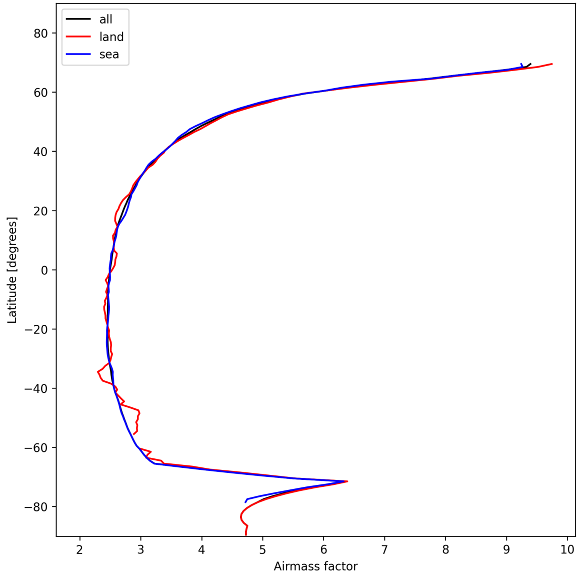
Figure 25: Zonal average of “Airmass factor” for 2025-01-21 to 2025-01-21.
