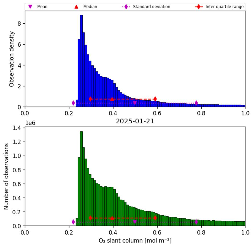
Figure 31: Histogram of “O 3 slant column” for 2025-01-21 to 2025-01-21
