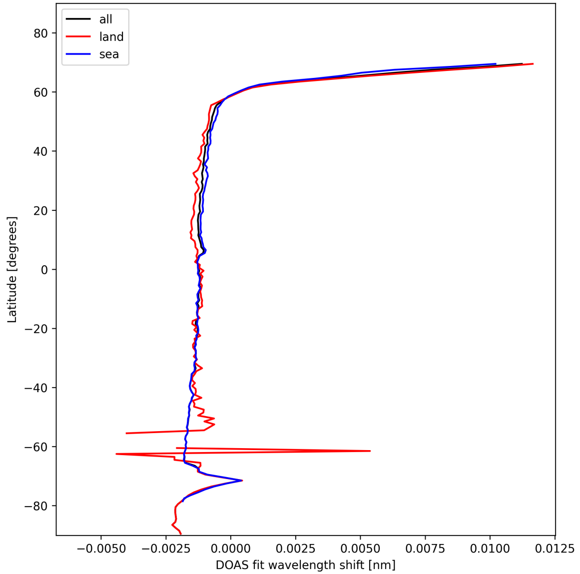
Figure 23: Zonal average of “DOAS fit wavelength shift” for 2025-01-21 to 2025-01-21.
