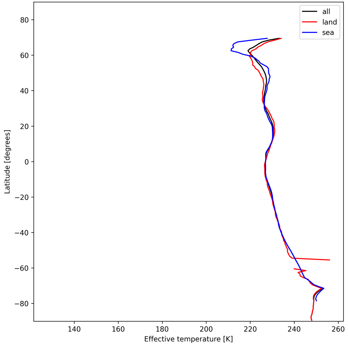
Figure 26: Zonal average of “Effective temperature” for 2025-01-21 to 2025-01-21.
