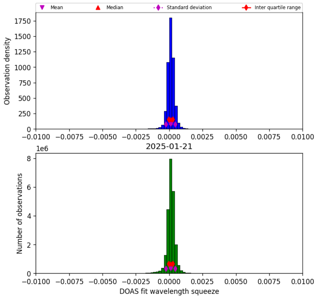
Figure 36: Histogram of “DOAS fit wavelength squeeze” for 2025-01-21 to 2025-01-21
