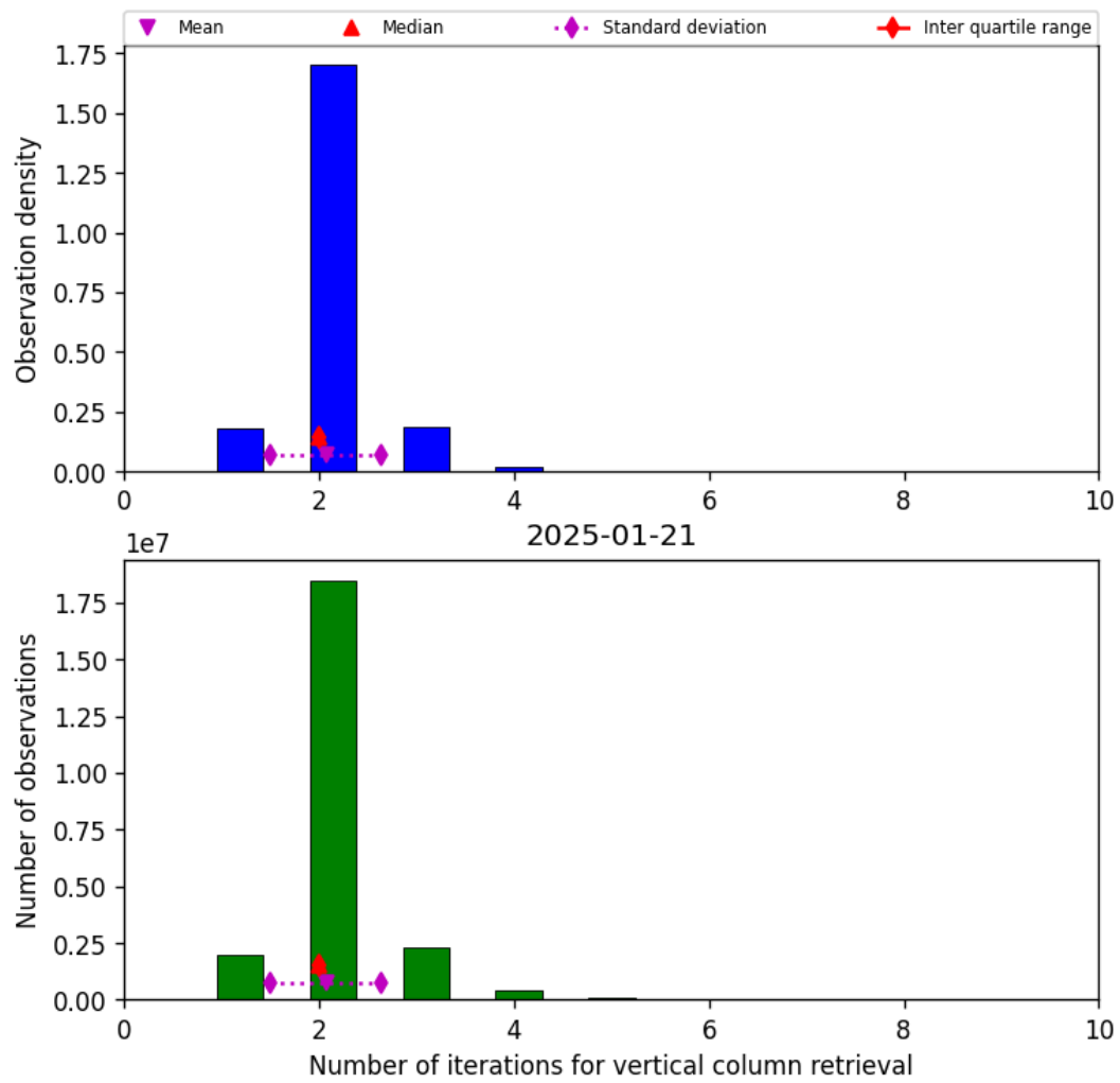
Figure 39: Histogram of “Number of iterations for vertical column retrieval” for 2025-01-21 to 2025-01-21
