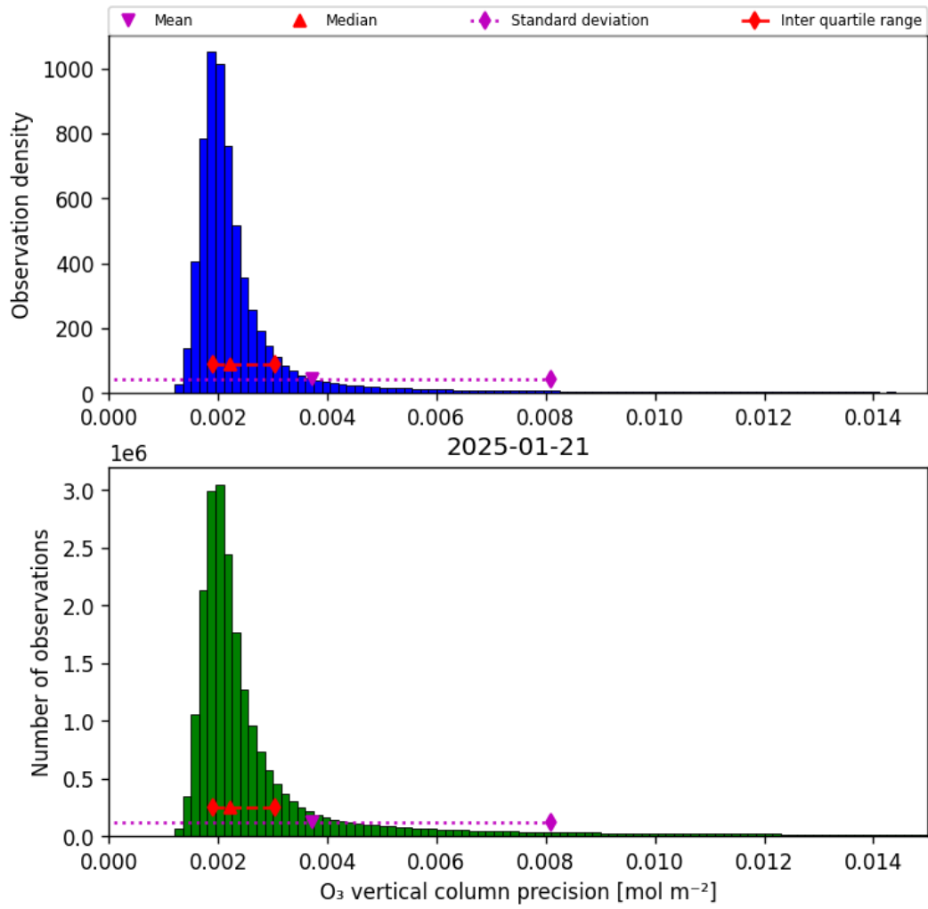
Figure 30: Histogram of “O 3 vertical column precision” for 2025-01-21 to 2025-01-21
