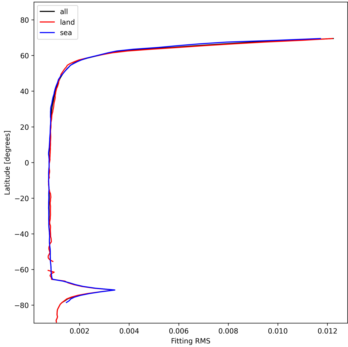
Figure 22: Zonal average of “Fitting RMS” for 2025-01-21 to 2025-01-21.
