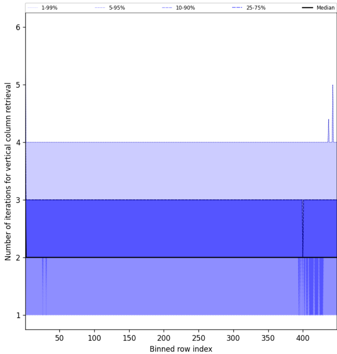
Figure 51: Along track statistics of “Number of iterations for vertical column retrieval” for 2025-01-21 to 2025-01-21
