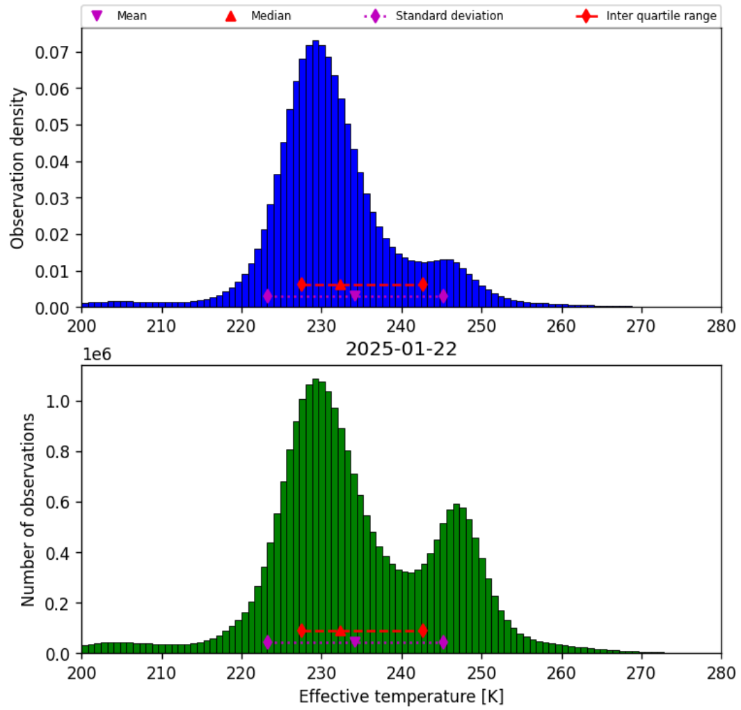
Figure 38: Histogram of “Effective temperature” for 2025-01-22 to 2025-01-23
