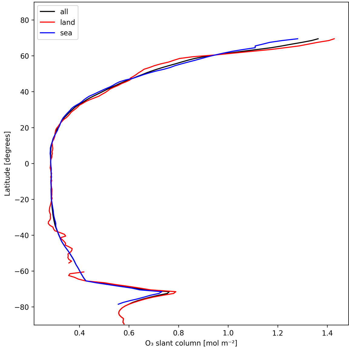
Figure 19: Zonal average of “O 3 slant column” for 2025-01-22 to 2025-01-23.
