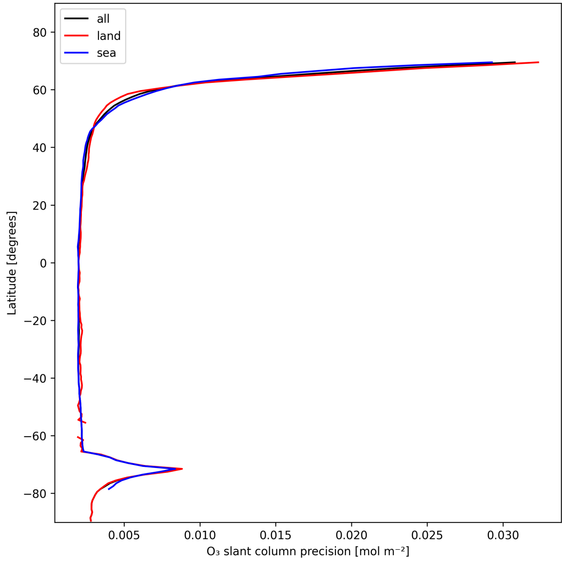
Figure 20: Zonal average of “O 3 slant column precision” for 2025-01-22 to 2025-01-23.
