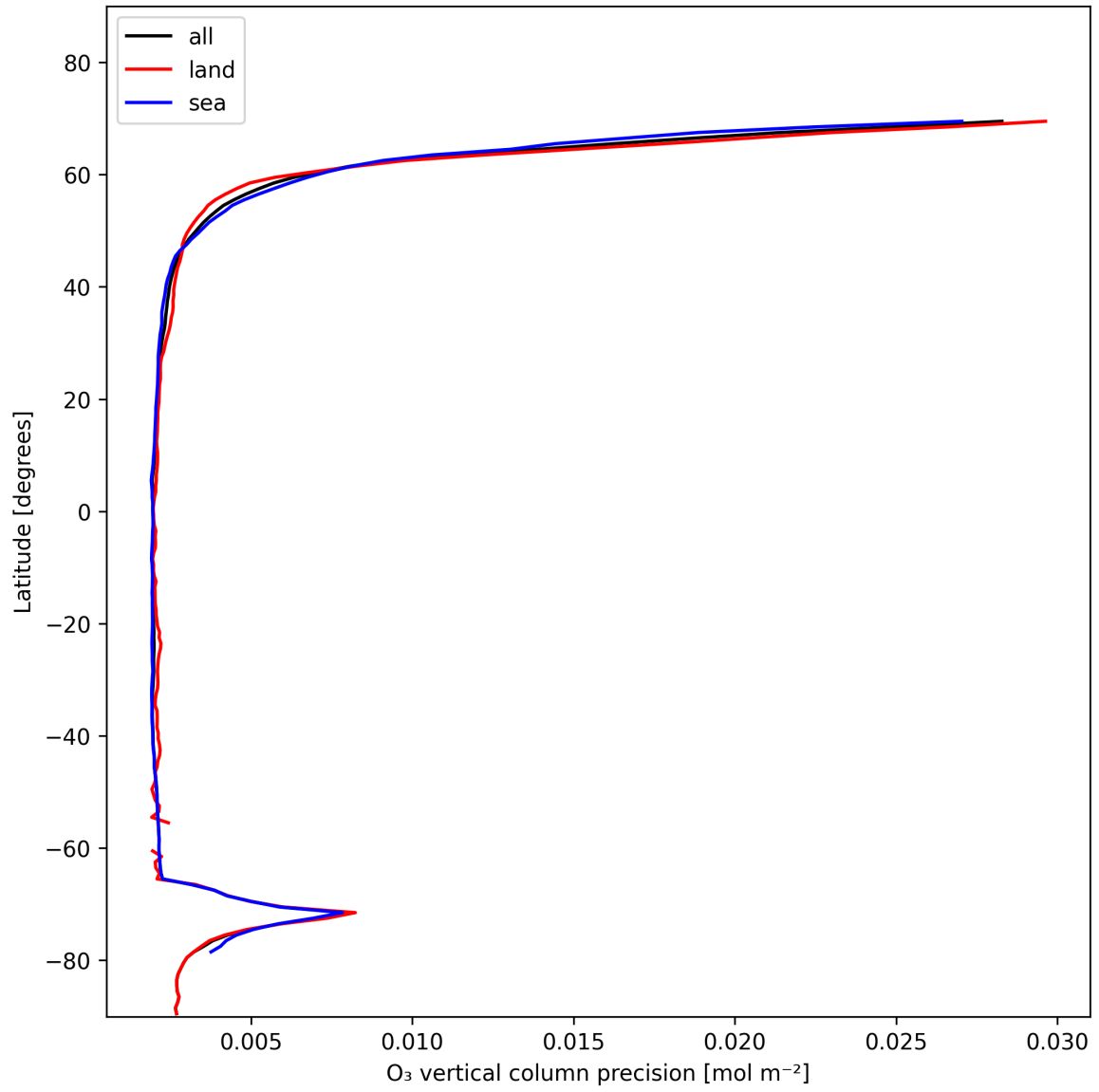
Figure 18: Zonal average of “O 3 vertical column precision” for 2025-01-22 to 2025-01-23.
