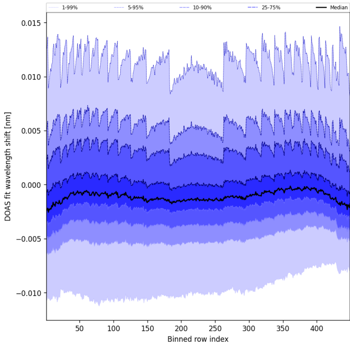
Figure 47: Along track statistics of "DOAS fit wavelength shift" for 2025-01-22 to 2025-01-23
