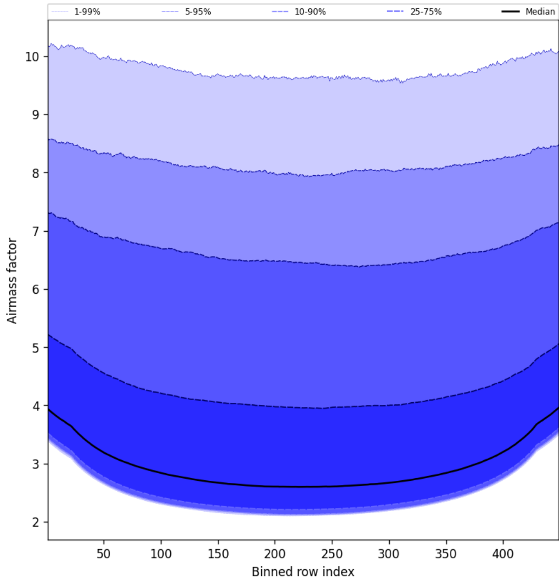
Figure 49: Along track statistics of “Airmass factor” for 2025-01-22 to 2025-01-23
