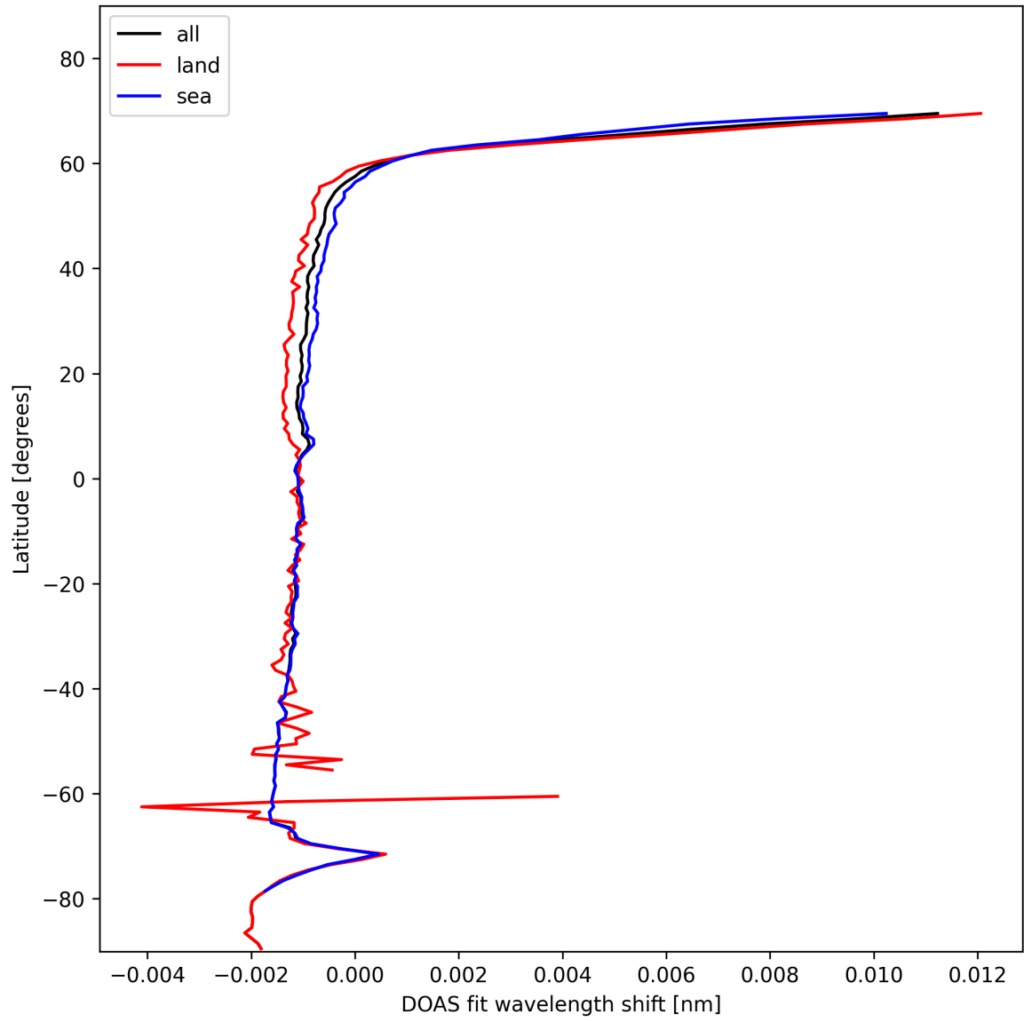
Figure 23: Zonal average of “DOAS fit wavelength shift” for 2025-01-22 to 2025-01-23.
