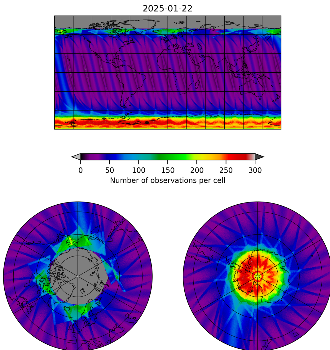
Figure 15: Map of the number of observations for 2025-01-22 to 2025-01-23
