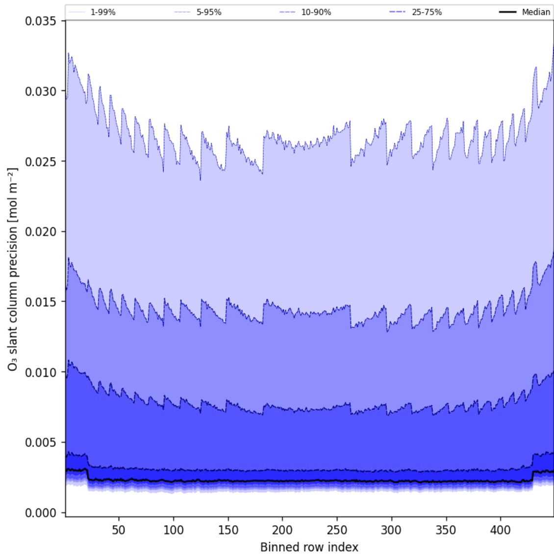
Figure 44: Along track statistics of “O 3 slant column precision” for 2025-01-22 to 2025-01-23
