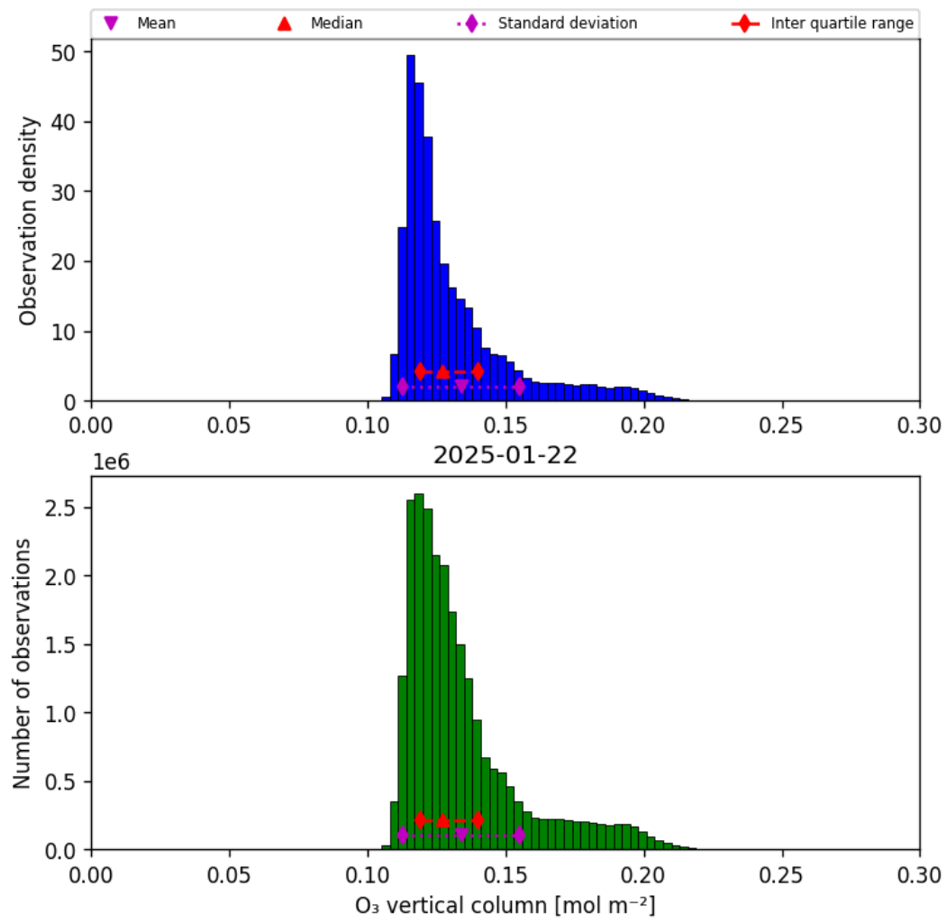
Figure 29: Histogram of “O 3 vertical column” for 2025-01-22 to 2025-01-23
