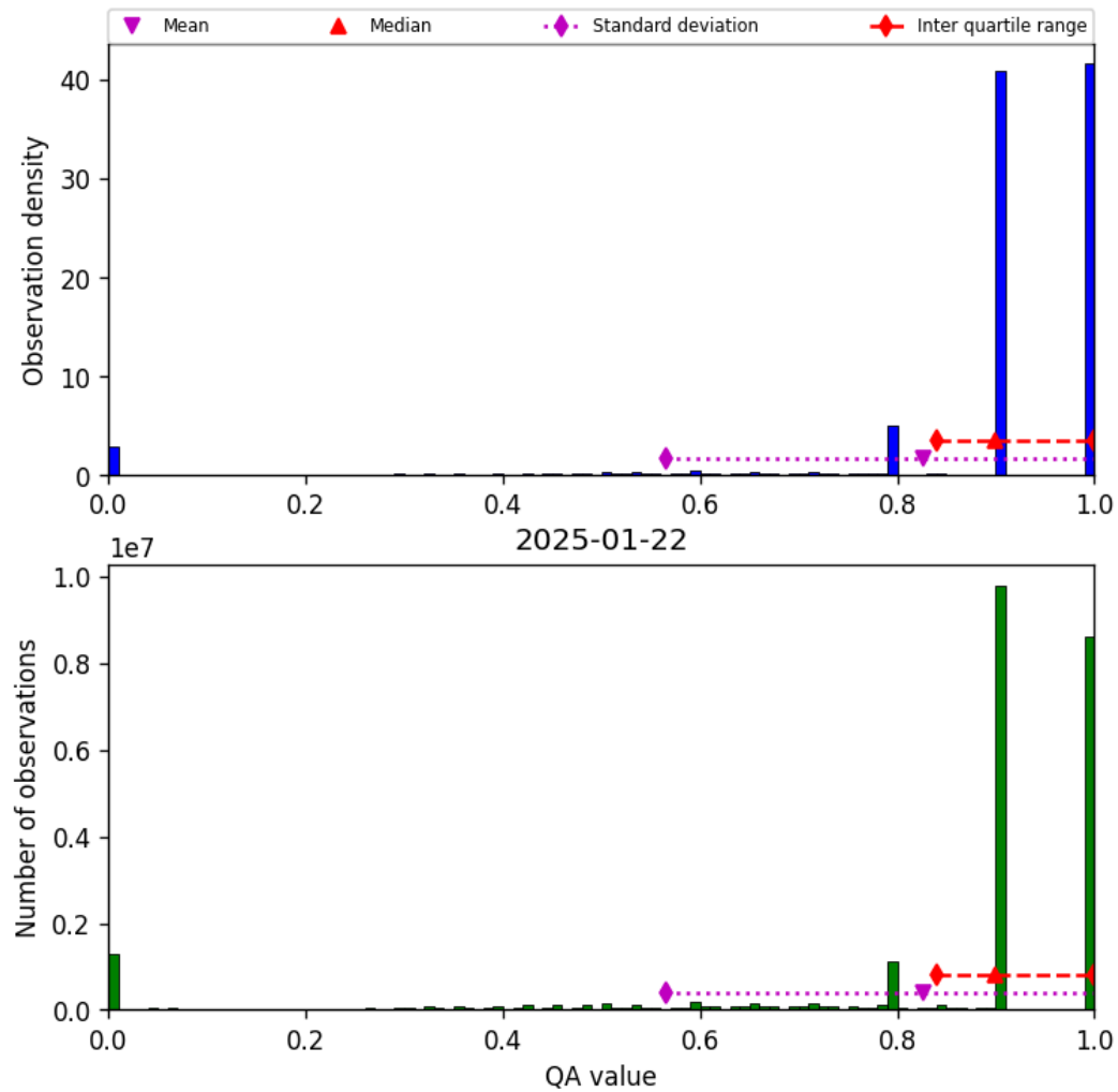
Figure 28: Histogram of “QA value” for 2025-01-22 to 2025-01-23
