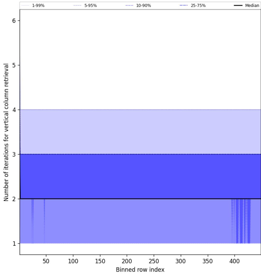
Figure 51: Along track statistics of “Number of iterations for vertical column retrieval” for 2025-01-22 to 2025-01-23
