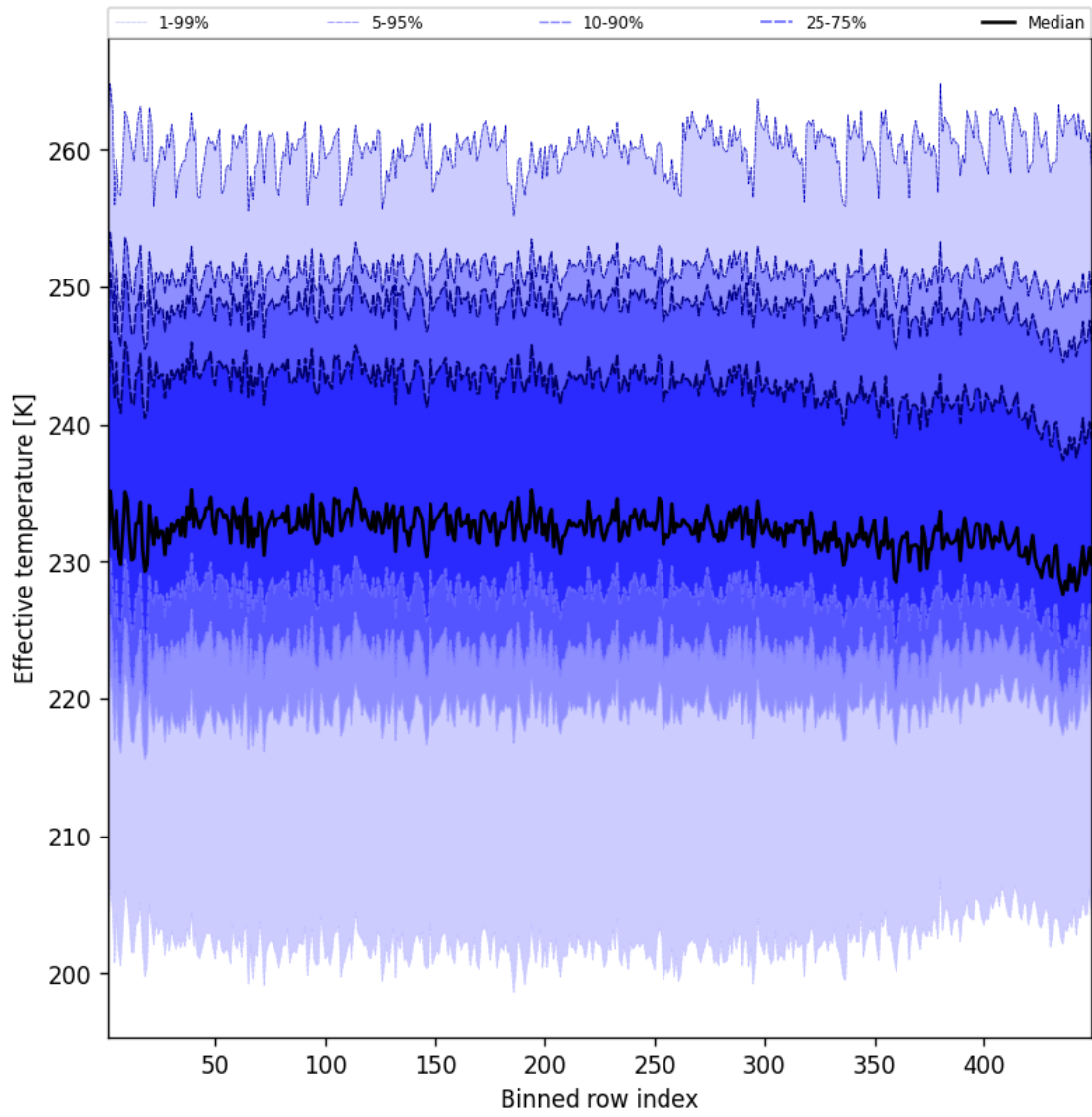
Figure 50: Along track statistics of “Effective temperature” for 2025-01-22 to 2025-01-23
