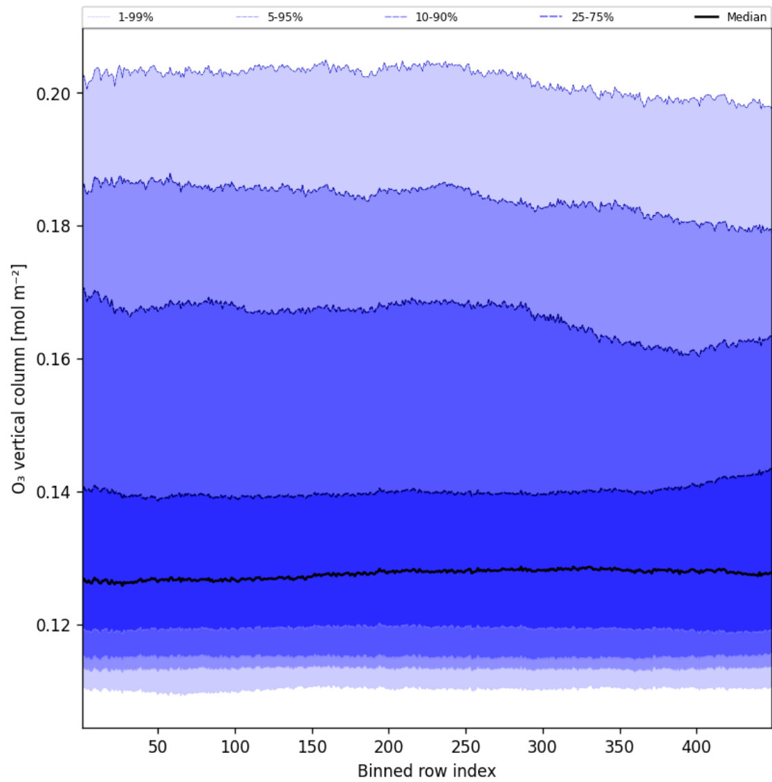
Figure 41: Along track statistics of “ O_3 vertical column” for 2025-01-22 to 2025-01-23
