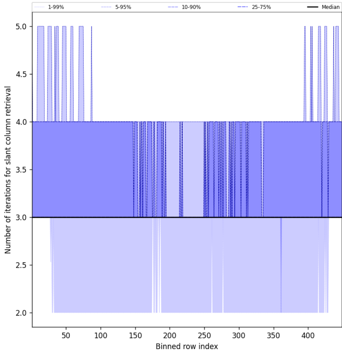
Figure 45: Along track statistics of “Number of iterations for slant column retrieval” for 2025-01-22 to 2025-01-23
