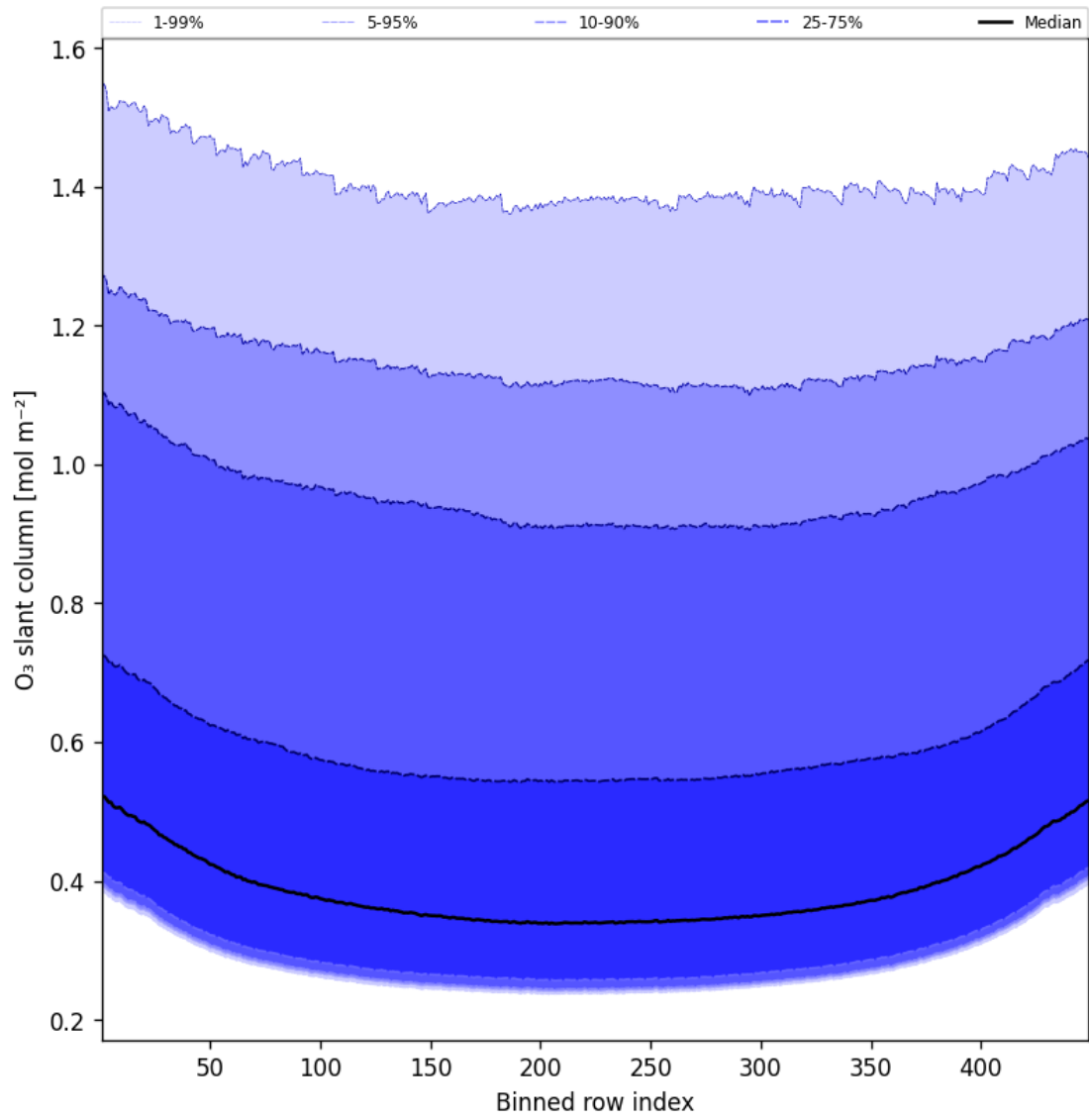
Figure 43: Along track statistics of “O 3 slant column” for 2025-01-22 to 2025-01-23
