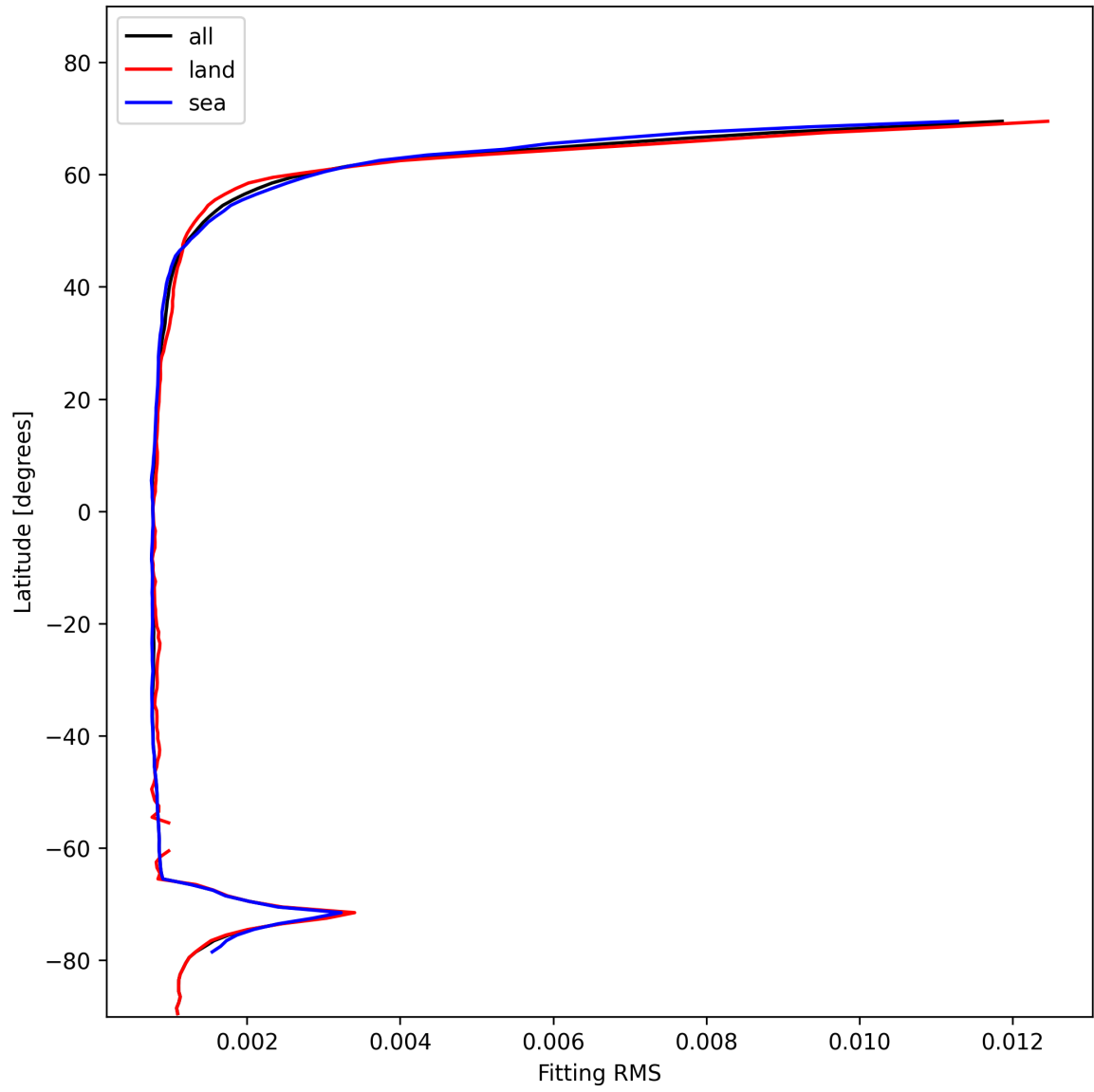
Figure 22: Zonal average of “Fitting RMS” for 2025-01-22 to 2025-01-23.
