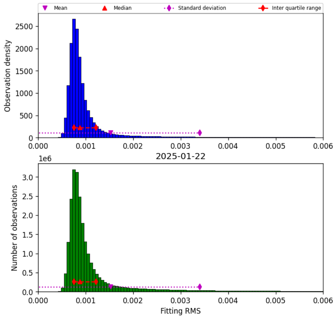
Figure 34: Histogram of “Fitting RMS” for 2025-01-22 to 2025-01-23
