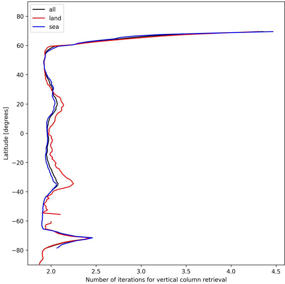
Figure 27: Zonal average of “Number of iterations for vertical column retrieval” for 2025-01-22 to 2025-01-23.
