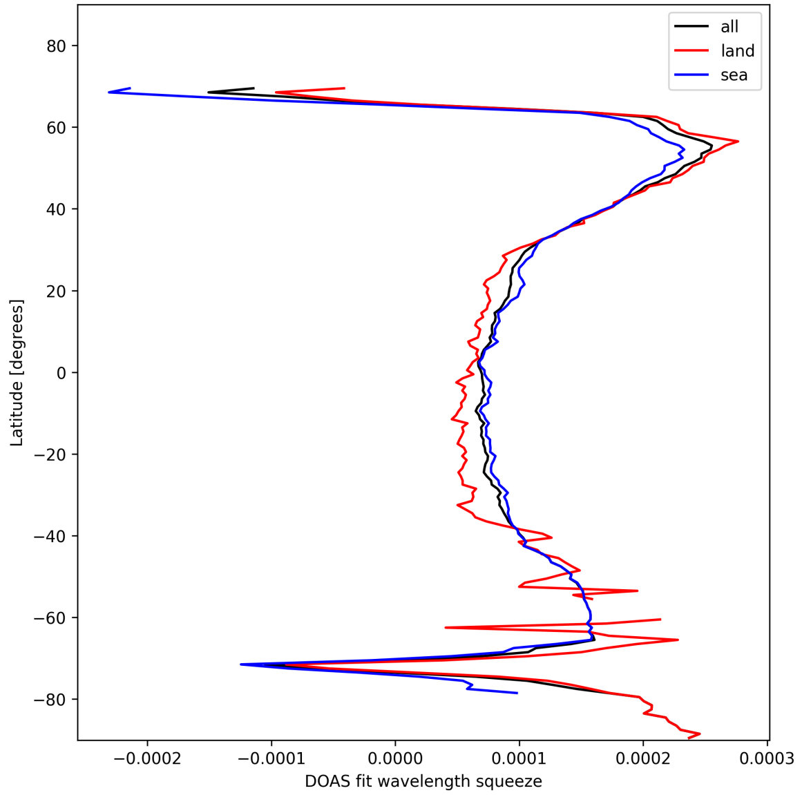
Figure 24: Zonal average of “DOAS fit wavelength squeeze” for 2025-01-22 to 2025-01-23.
