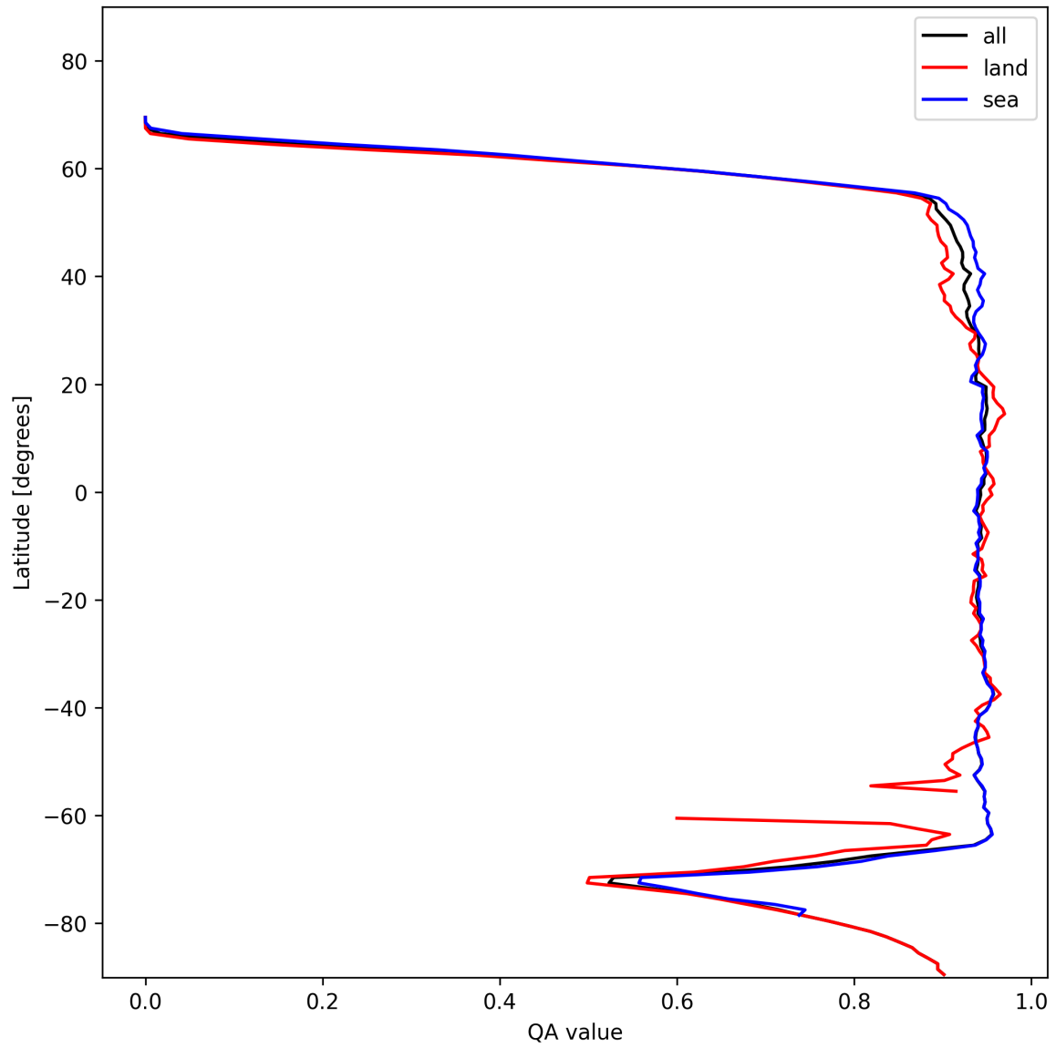
Figure 16: Zonal average of “QA value” for 2025-01-22 to 2025-01-23.
