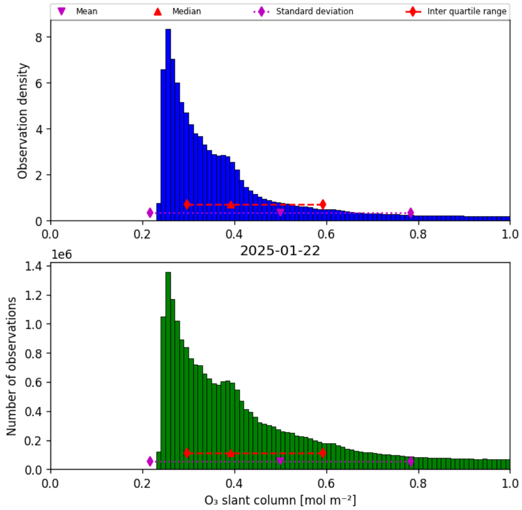
Figure 31: Histogram of “O 3 slant column” for 2025-01-22 to 2025-01-23
