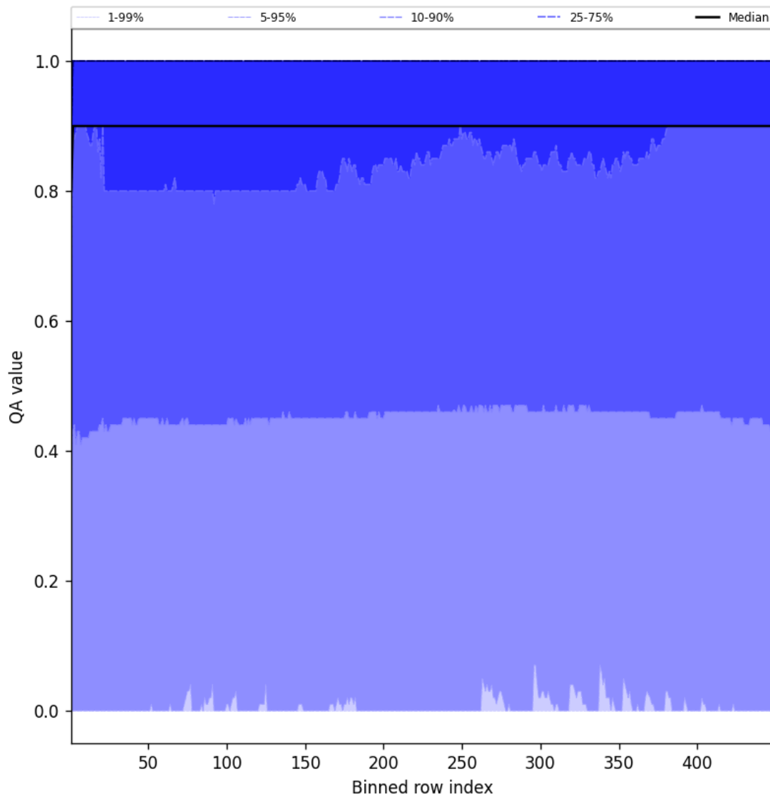
Figure 40: Along track statistics of “QA value” for 2025-01-22 to 2025-01-23
