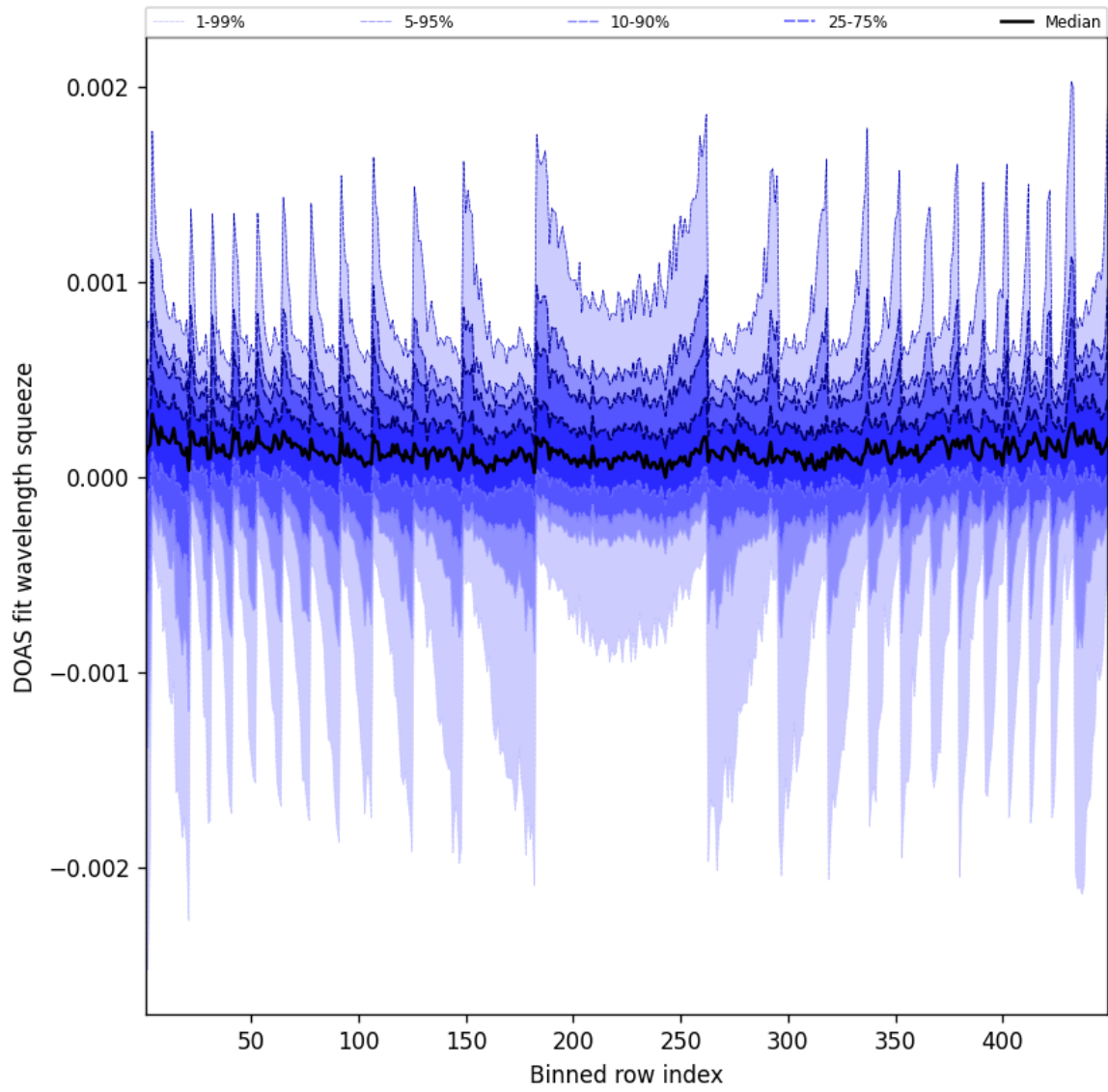
Figure 48: Along track statistics of “DOAS fit wavelength squeeze” for 2025-01-22 to 2025-01-23
