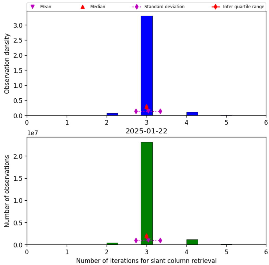
Figure 33: Histogram of “Number of iterations for slant column retrieval” for 2025-01-22 to 2025-01-23
