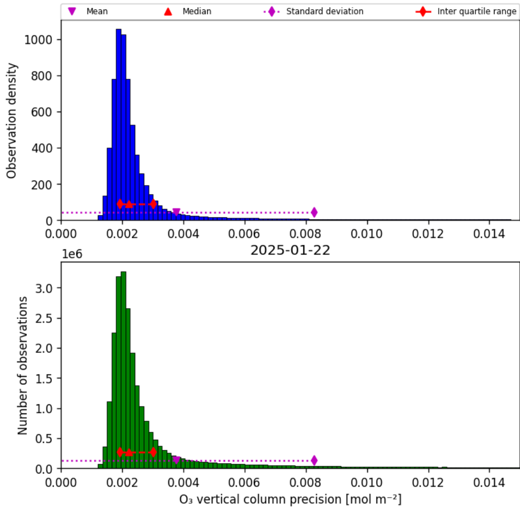
Figure 30: Histogram of “O 3 vertical column precision” for 2025-01-22 to 2025-01-23
