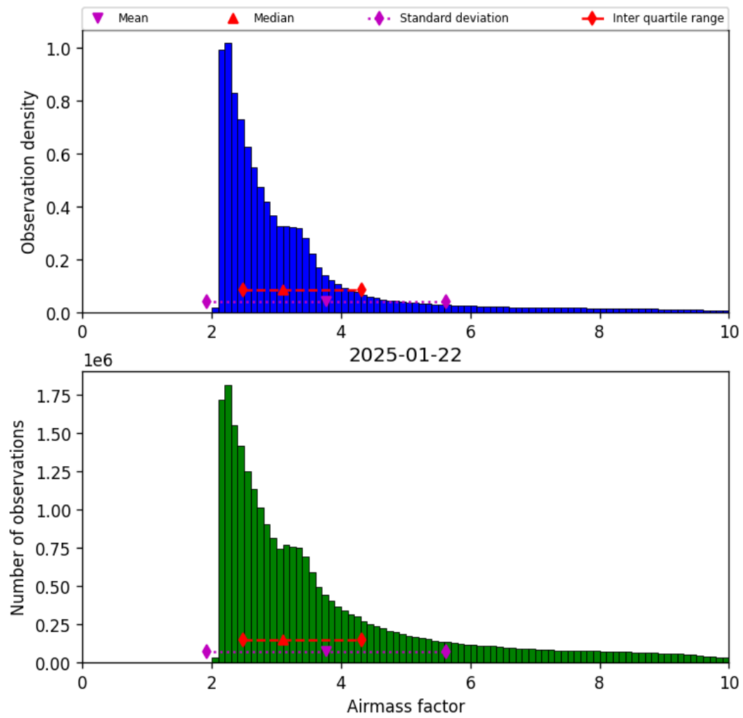
Figure 37: Histogram of “Airmass factor” for 2025-01-22 to 2025-01-23
