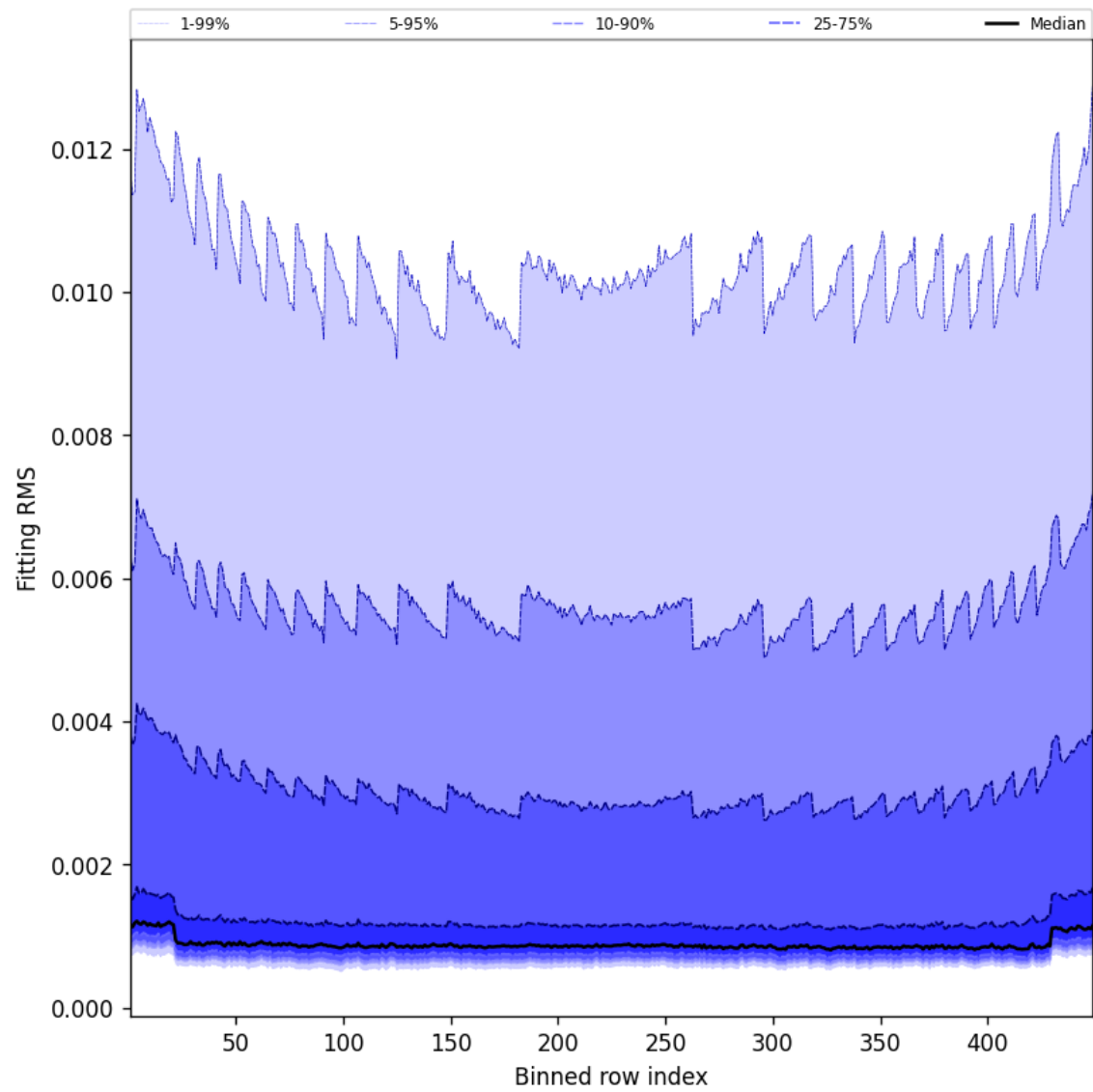
Figure 46: Along track statistics of “Fitting RMS” for 2025-01-22 to 2025-01-23
