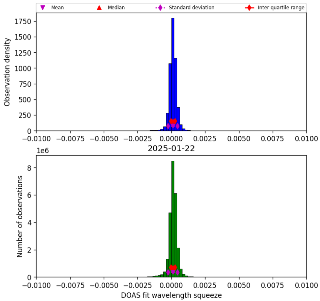
Figure 36: Histogram of “DOAS fit wavelength squeeze” for 2025-01-22 to 2025-01-23
