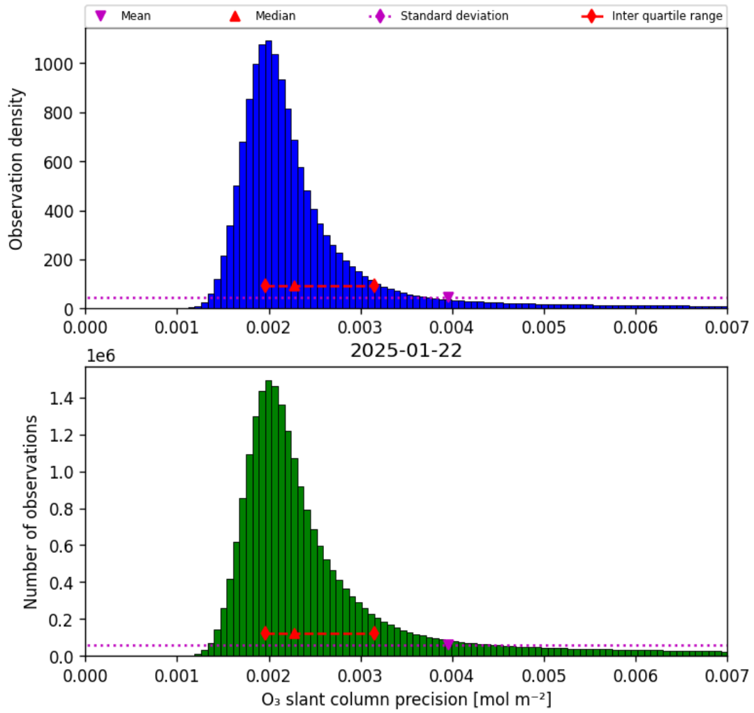
Figure 32: Histogram of “O 3 slant column precision” for 2025-01-22 to 2025-01-23
