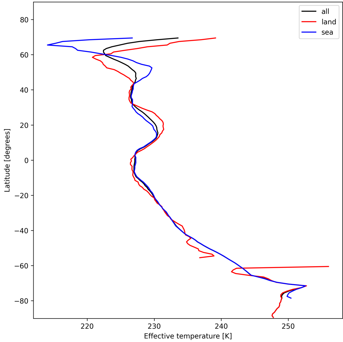
Figure 26: Zonal average of “Effective temperature” for 2025-01-22 to 2025-01-23.
