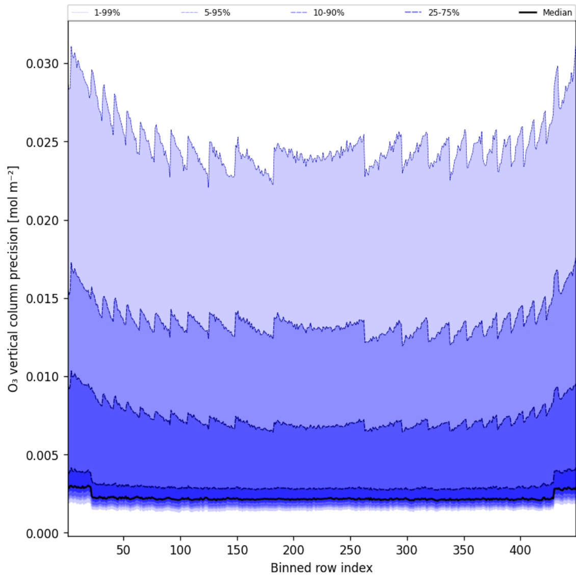
Figure 42: Along track statistics of “O 3 vertical column precision” for 2025-01-22 to 2025-01-23
