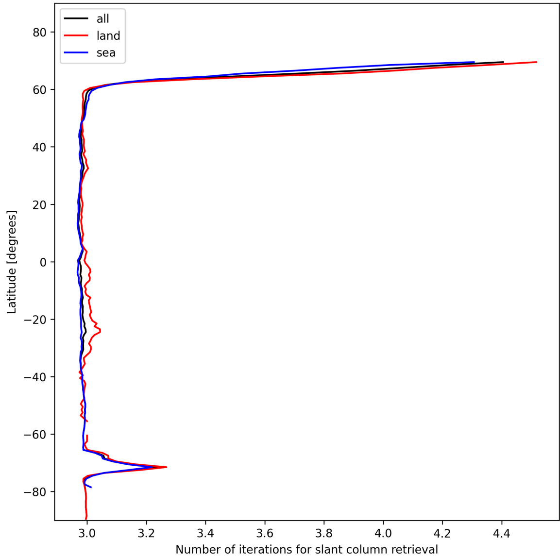
Figure 21: Zonal average of “Number of iterations for slant column retrieval” for 2025-01-22 to 2025-01-23.
