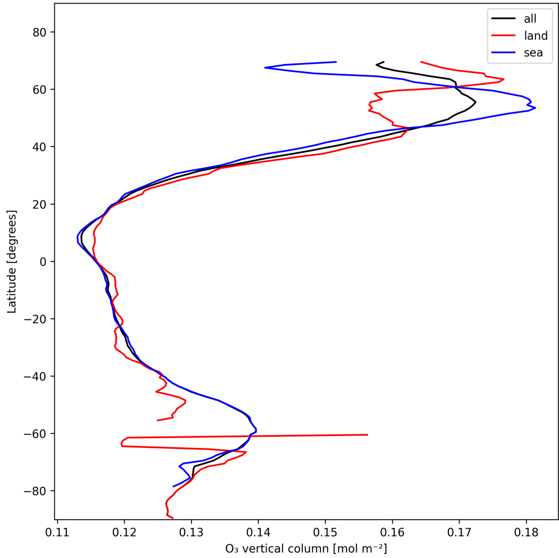
Figure 17: Zonal average of “O 3 vertical column” for 2025-01-22 to 2025-01-23.
