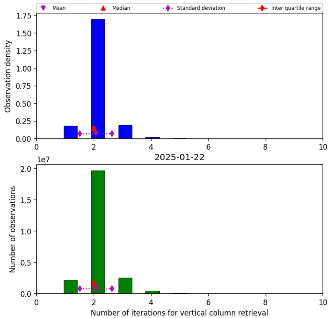
Figure 39: Histogram of “Number of iterations for vertical column retrieval” for 2025-01-22 to 2025-01-23
