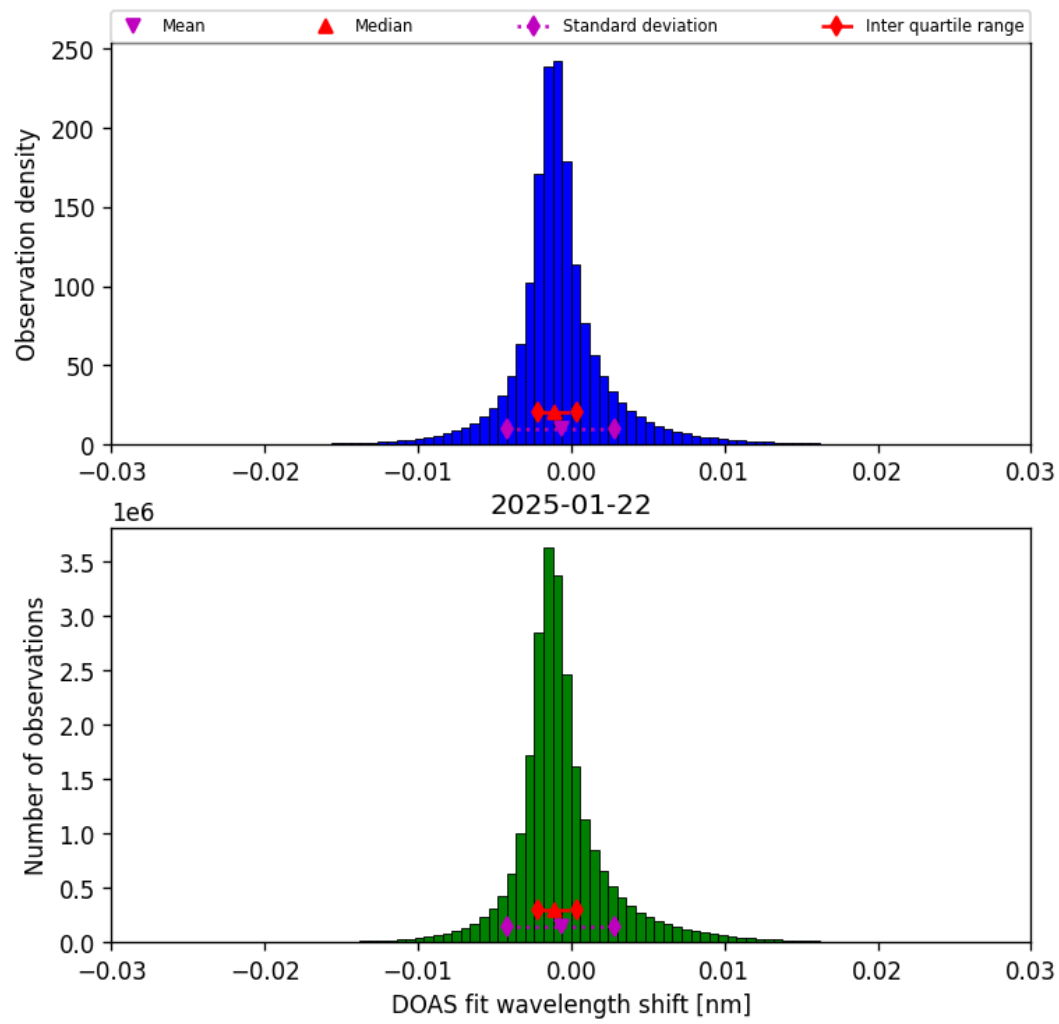
Figure 35: Histogram of “DOAS fit wavelength shift” for 2025-01-22 to 2025-01-23
