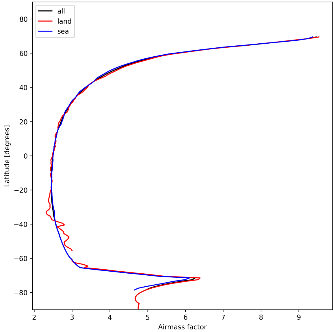
Figure 25: Zonal average of “Airmass factor” for 2025-01-22 to 2025-01-23.
