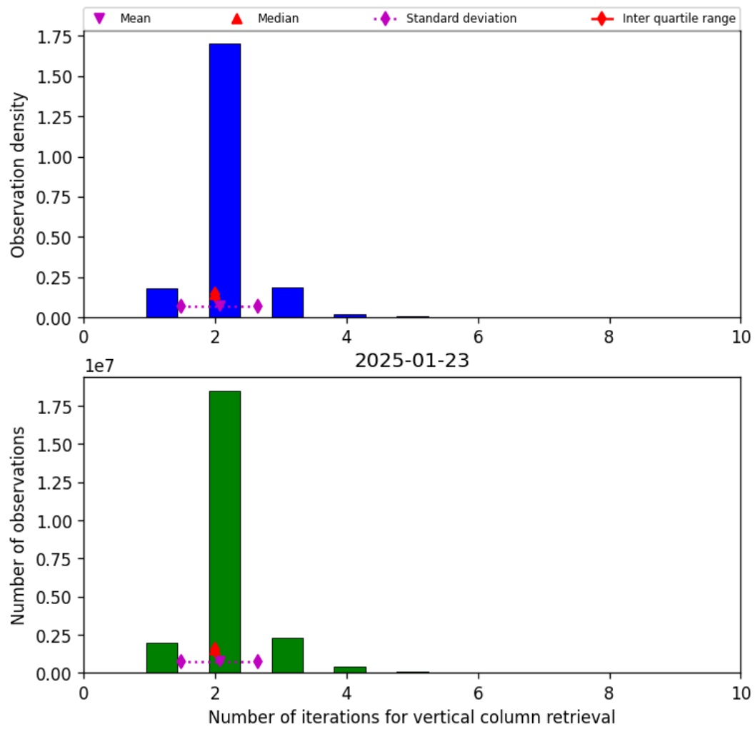
Figure 39: Histogram of “Number of iterations for vertical column retrieval” for 2025-01-23 to 2025-01-24
