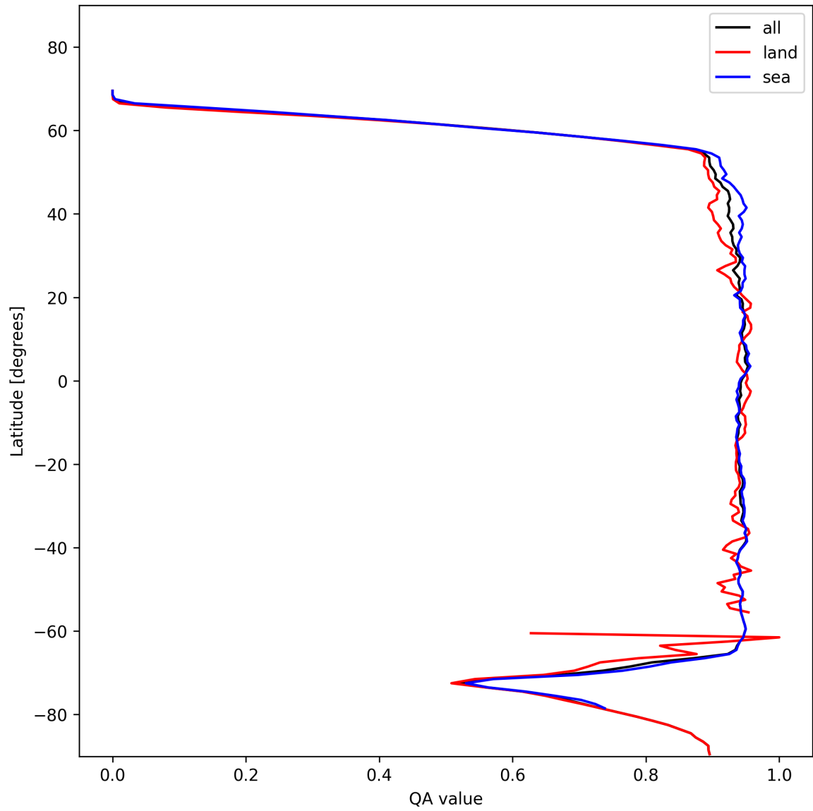
Figure 16: Zonal average of “QA value” for 2025-01-23 to 2025-01-24.
