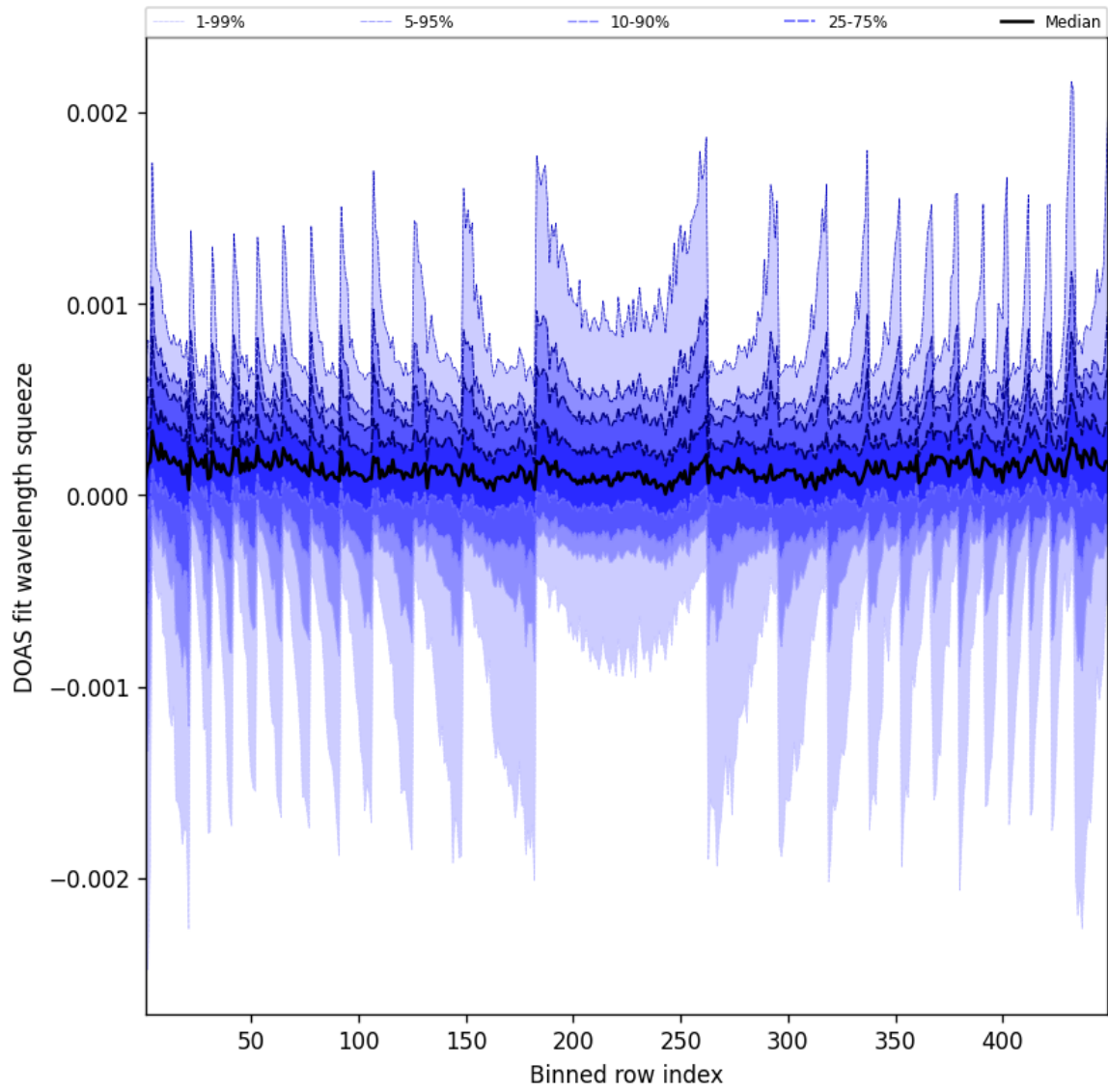
Figure 48: Along track statistics of “DOAS fit wavelength squeeze” for 2025-01-23 to 2025-01-24
