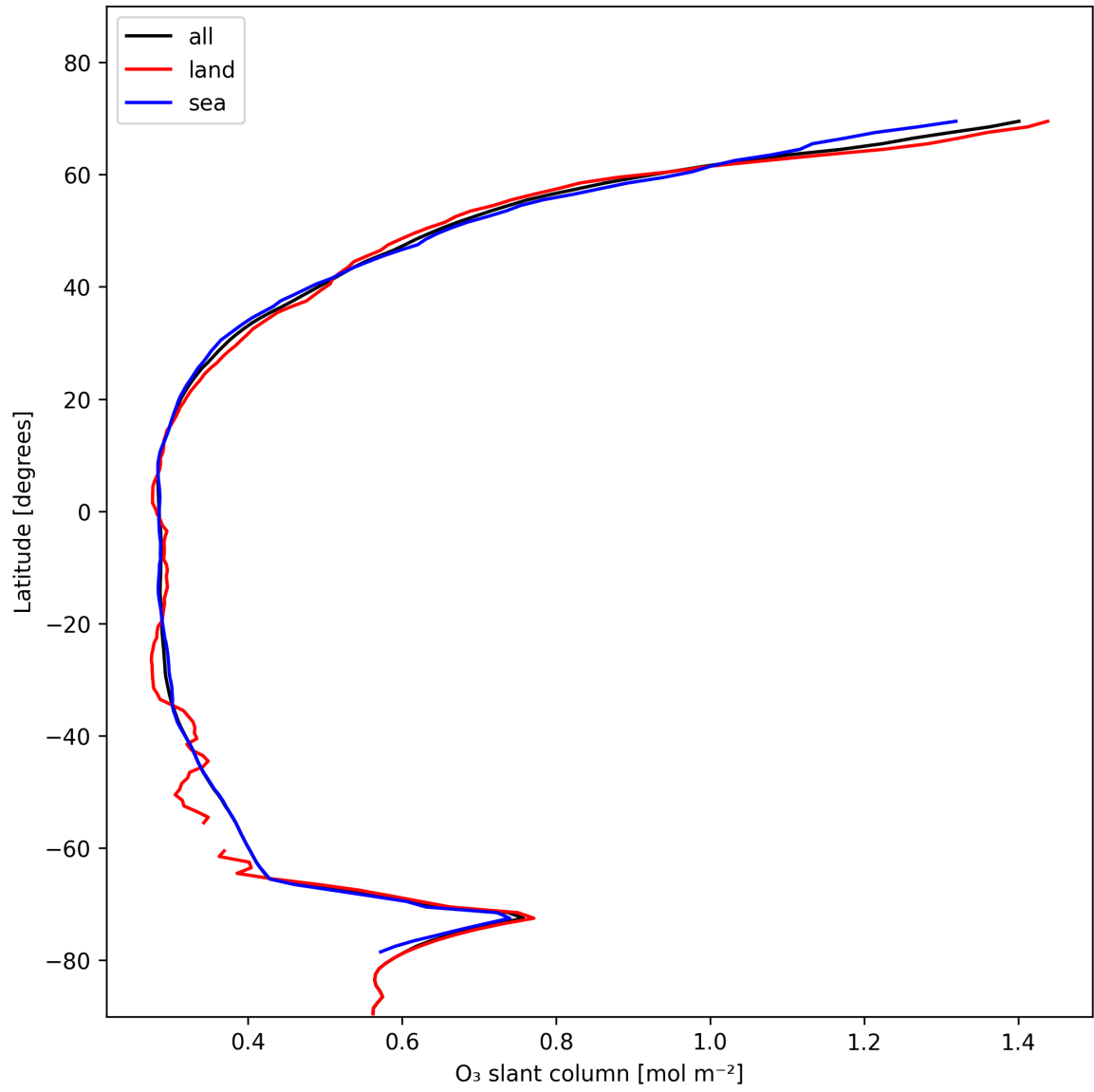
Figure 19: Zonal average of “O 3 slant column” for 2025-01-23 to 2025-01-24.
