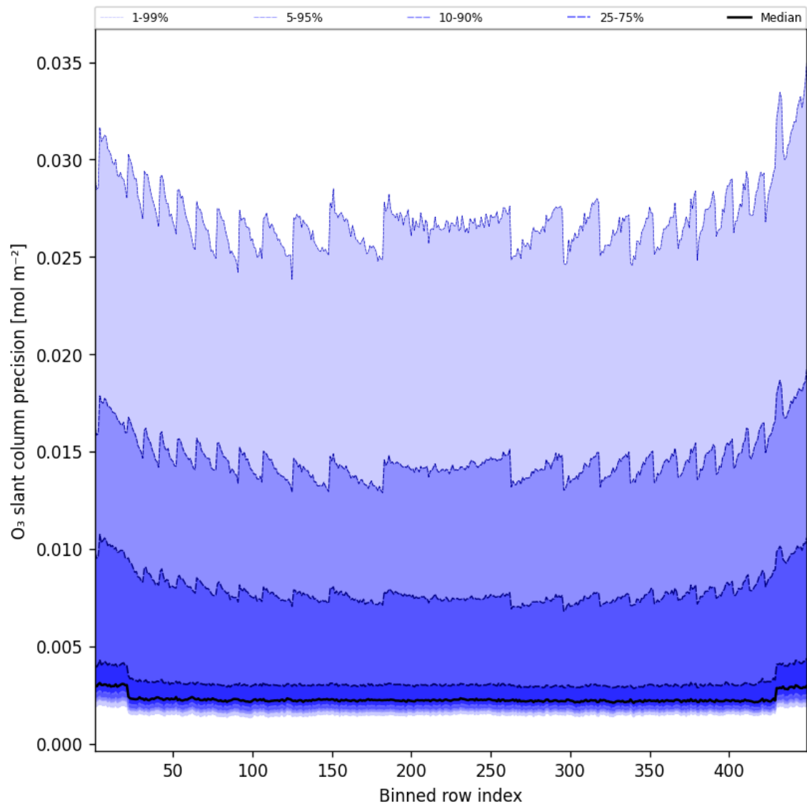
Figure 44: Along track statistics of “O 3 slant column precision” for 2025-01-23 to 2025-01-24
