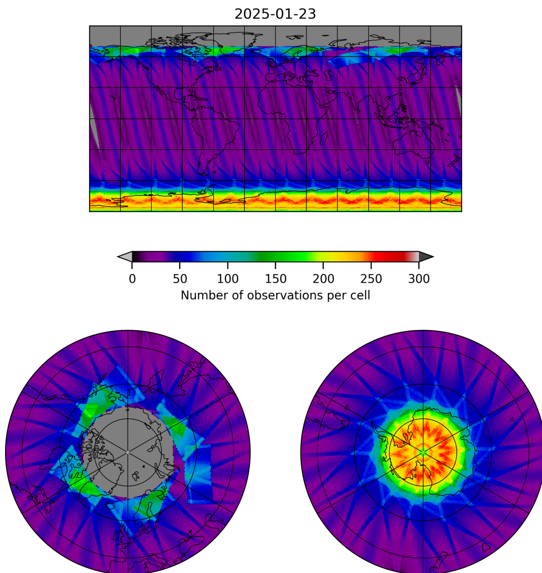
Figure 15: Map of the number of observations for 2025-01-23 to 2025-01-24
