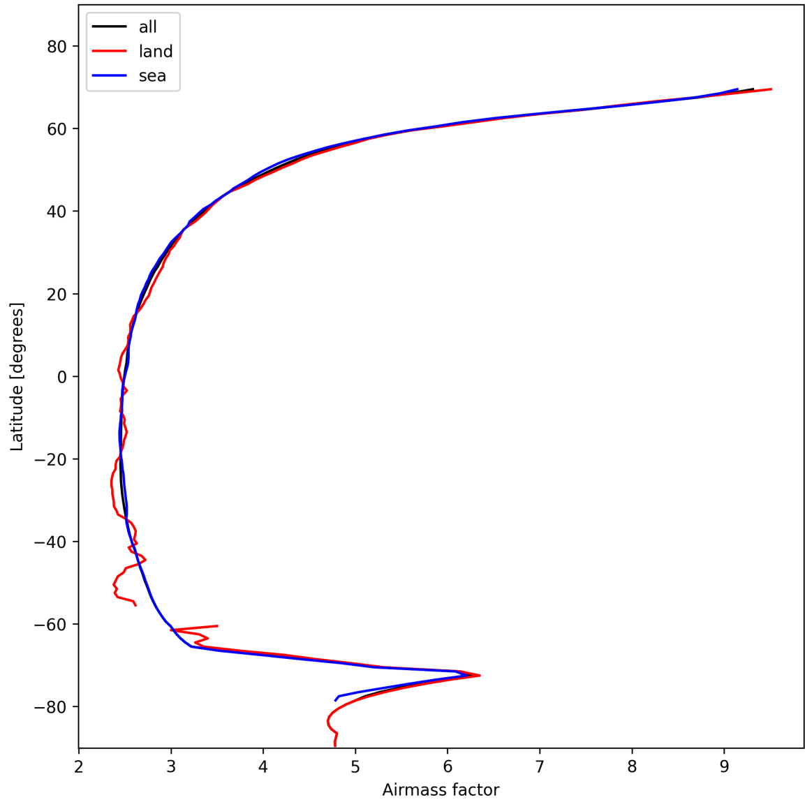
Figure 25: Zonal average of “Airmass factor” for 2025-01-23 to 2025-01-24.
