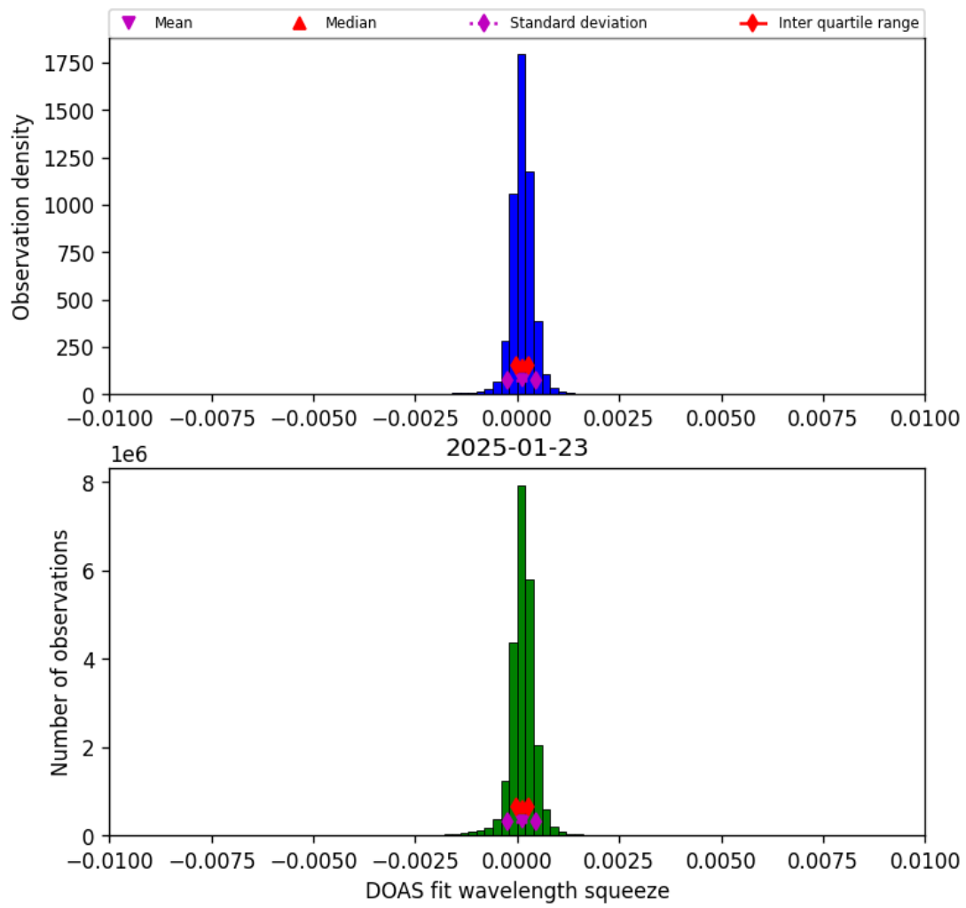
Figure 36: Histogram of “DOAS fit wavelength squeeze” for 2025-01-23 to 2025-01-24
