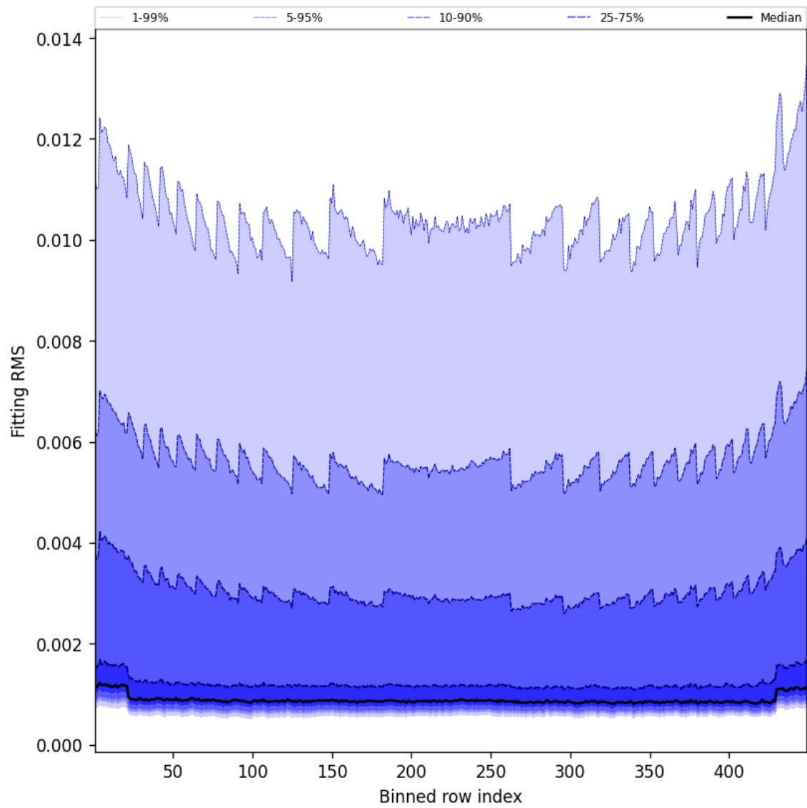
Figure 46: Along track statistics of “Fitting RMS” for 2025-01-23 to 2025-01-24
