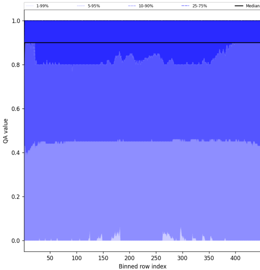
Figure 40: Along track statistics of “QA value” for 2025-01-23 to 2025-01-24
