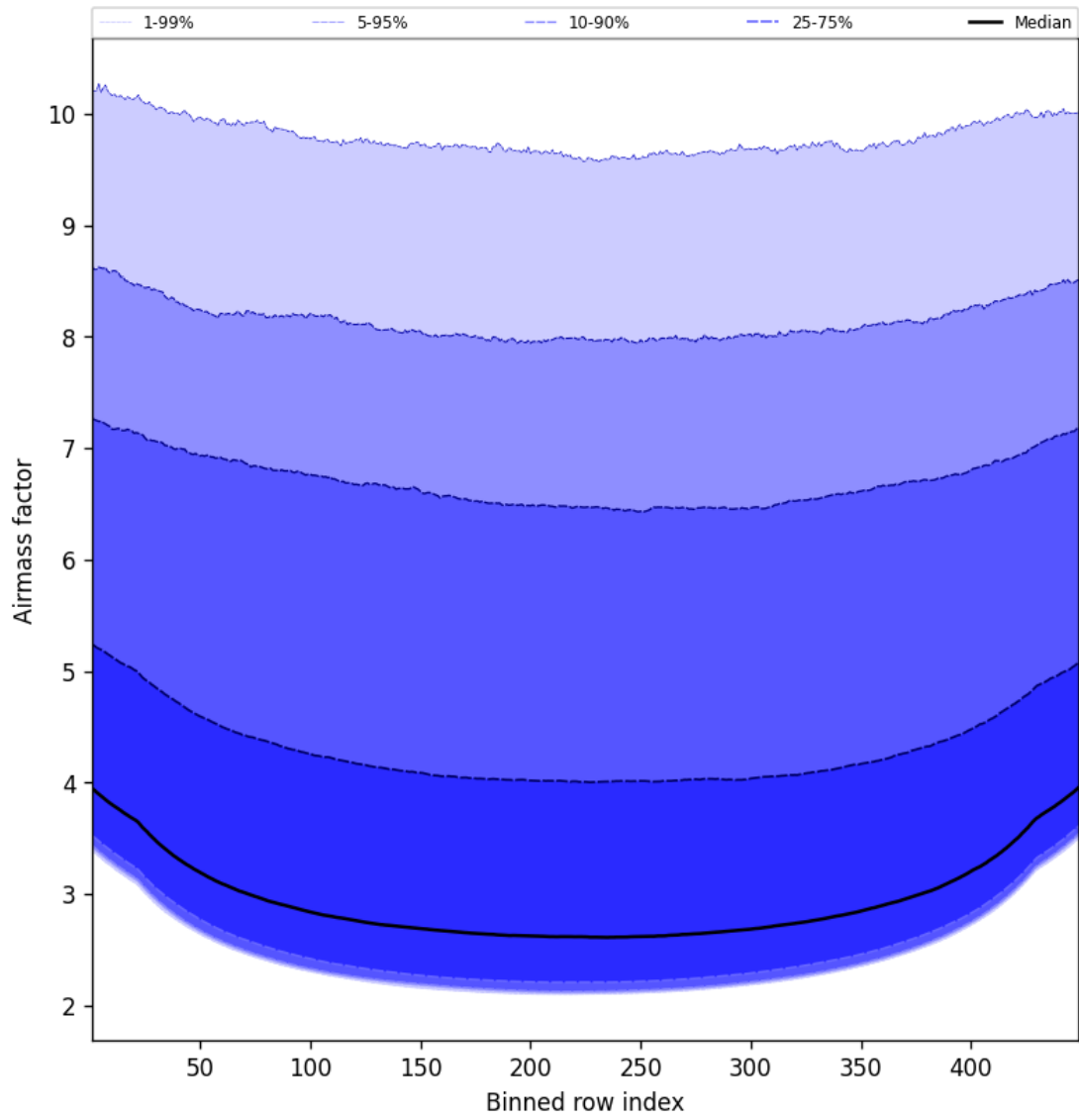
Figure 49: Along track statistics of “Airmass factor” for 2025-01-23 to 2025-01-24
