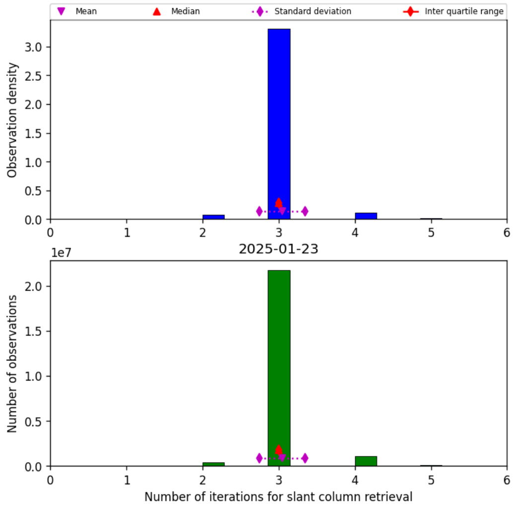
Figure 33: Histogram of “Number of iterations for slant column retrieval” for 2025-01-23 to 2025-01-24
