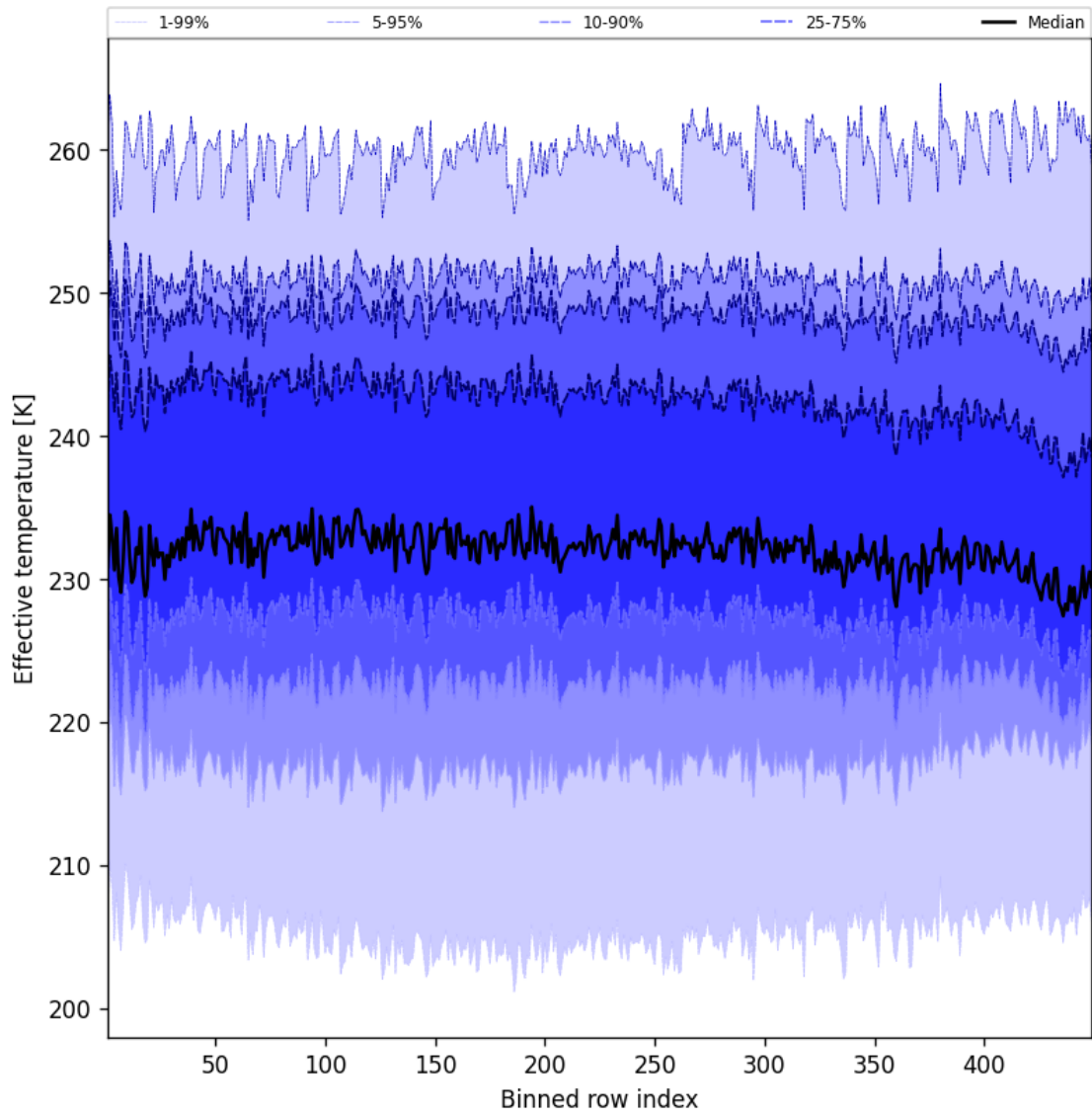
Figure 50: Along track statistics of “Effective temperature” for 2025-01-23 to 2025-01-24
