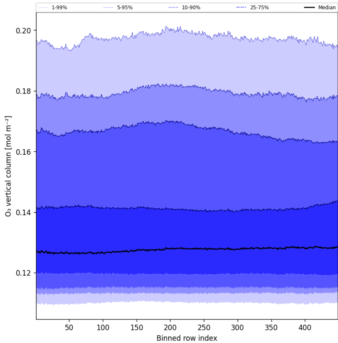
Figure 41: Along track statistics of “O 3 vertical column” for 2025-01-23 to 2025-01-24
