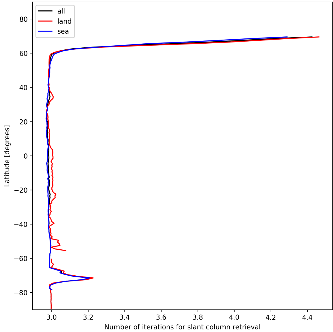
Figure 21: Zonal average of “Number of iterations for slant column retrieval” for 2025-01-23 to 2025-01-24.
