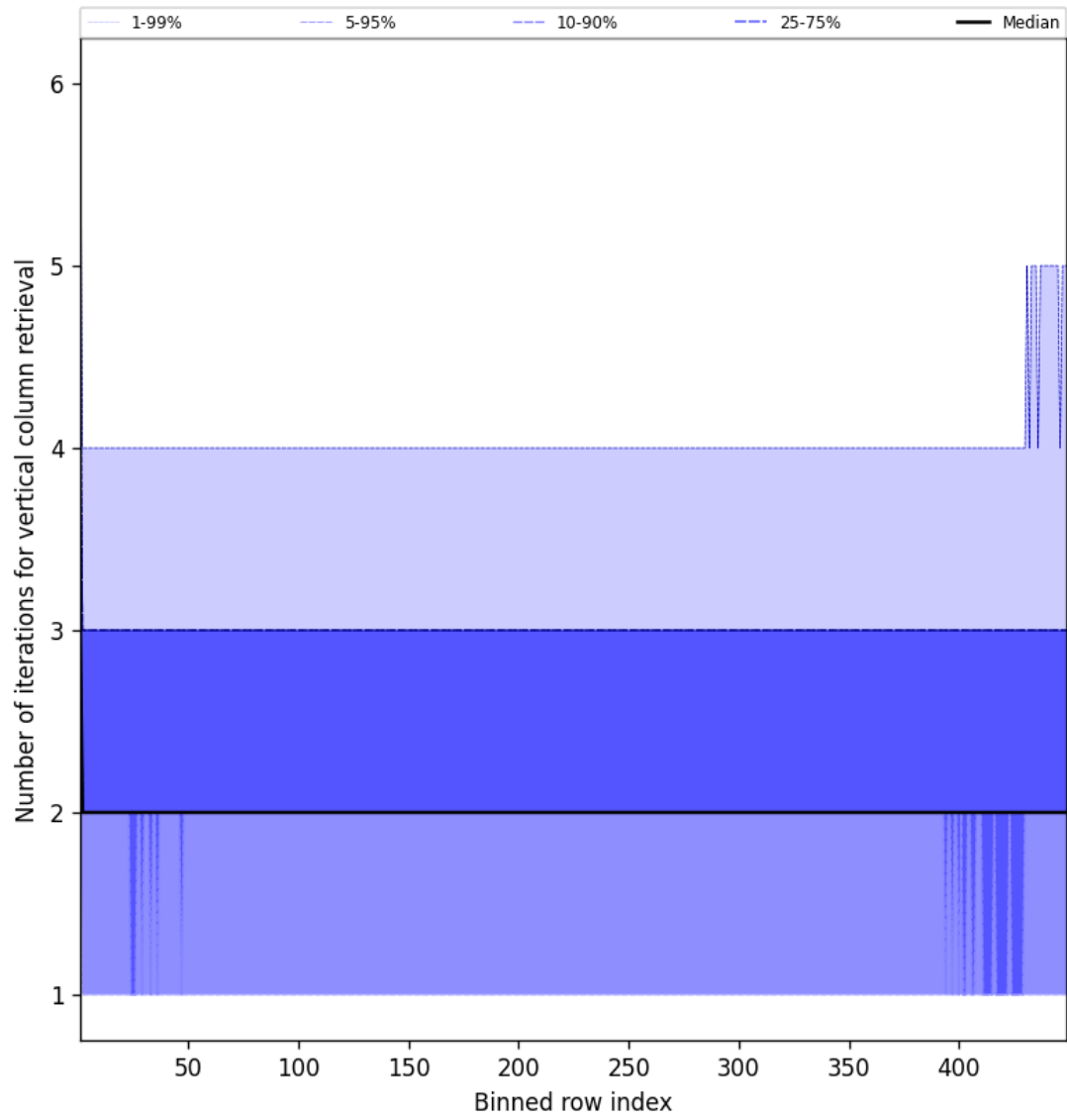
Figure 51: Along track statistics of “Number of iterations for vertical column retrieval” for 2025-01-23 to 2025-01-24
