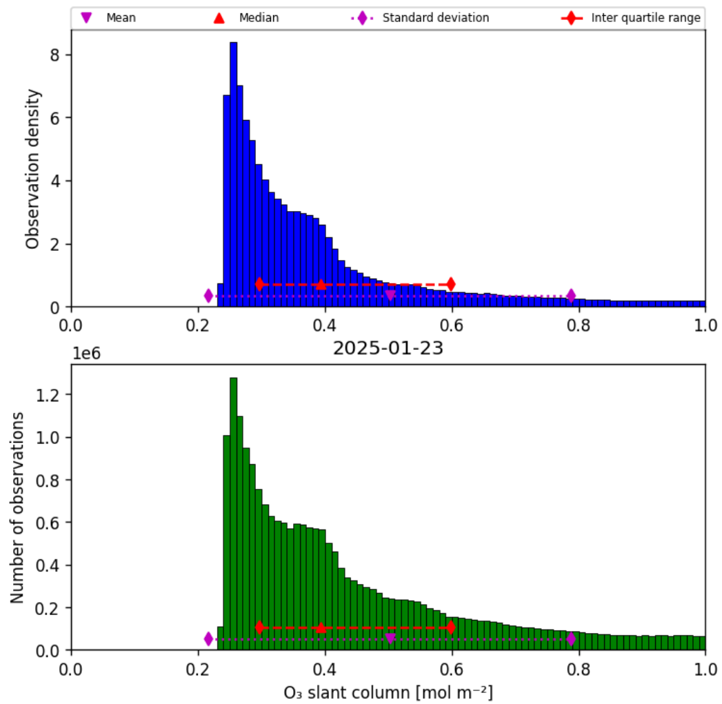
Figure 31: Histogram of “O 3 slant column” for 2025-01-23 to 2025-01-24
