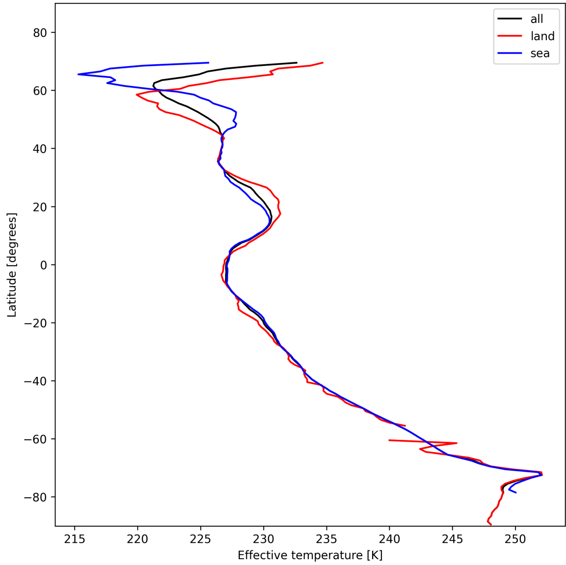
Figure 26: Zonal average of “Effective temperature” for 2025-01-23 to 2025-01-24.
