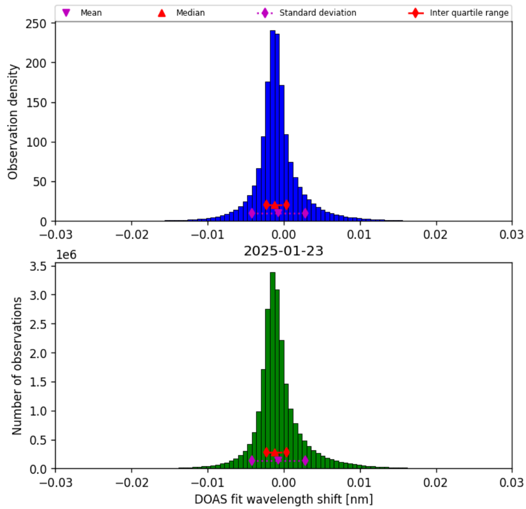
Figure 35: Histogram of “DOAS fit wavelength shift” for 2025-01-23 to 2025-01-24
