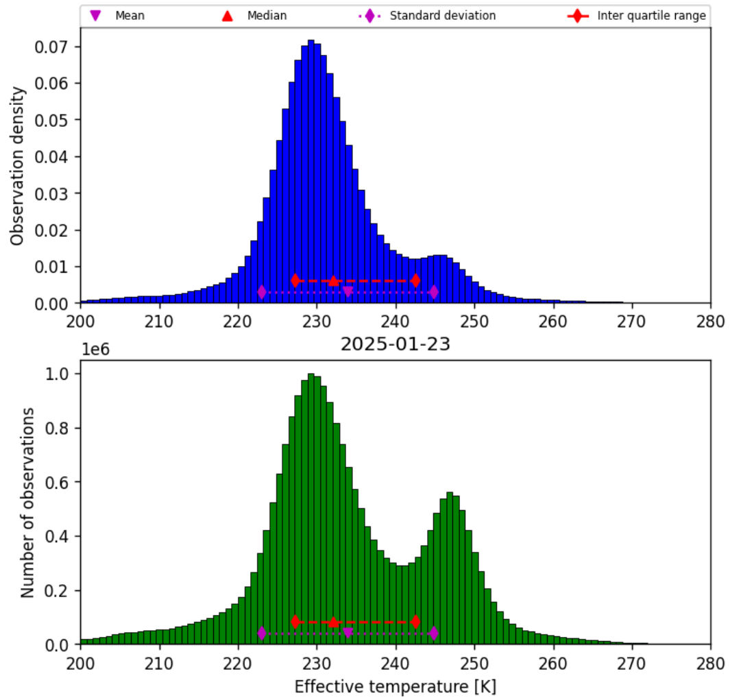
Figure 38: Histogram of “Effective temperature” for 2025-01-23 to 2025-01-24
