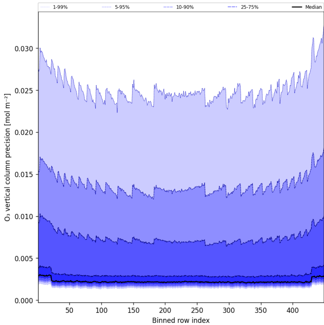
Figure 42: Along track statistics of “O 3 vertical column precision” for 2025-01-23 to 2025-01-24
