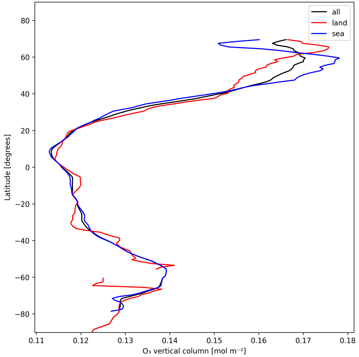
Figure 17: Zonal average of “O 3 vertical column” for 2025-01-23 to 2025-01-24.
