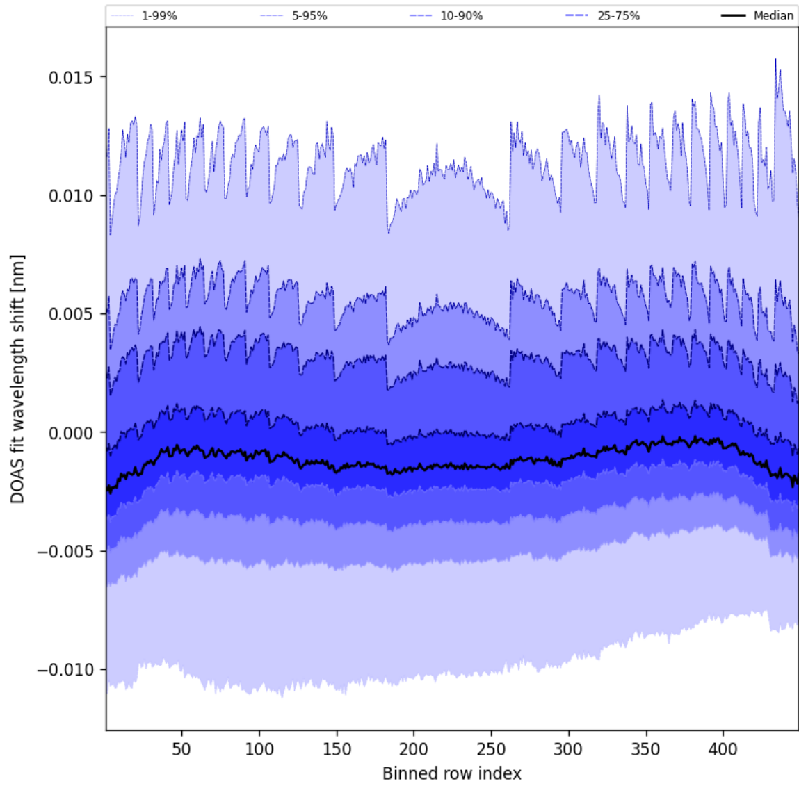
Figure 47: Along track statistics of “DOAS fit wavelength shift” for 2025-01-23 to 2025-01-24
