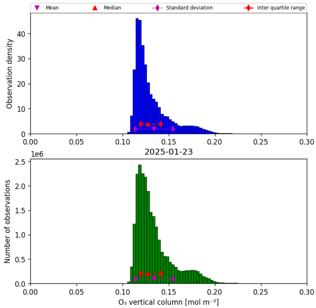
Figure 29: Histogram of “O 3 vertical column” for 2025-01-23 to 2025-01-24
