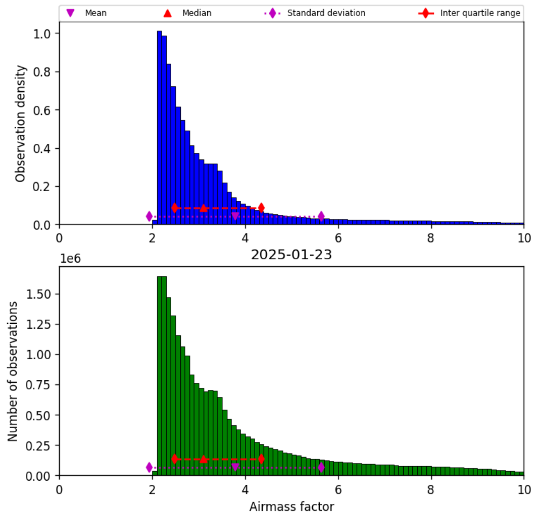
Figure 37: Histogram of “Airmass factor” for 2025-01-23 to 2025-01-24
