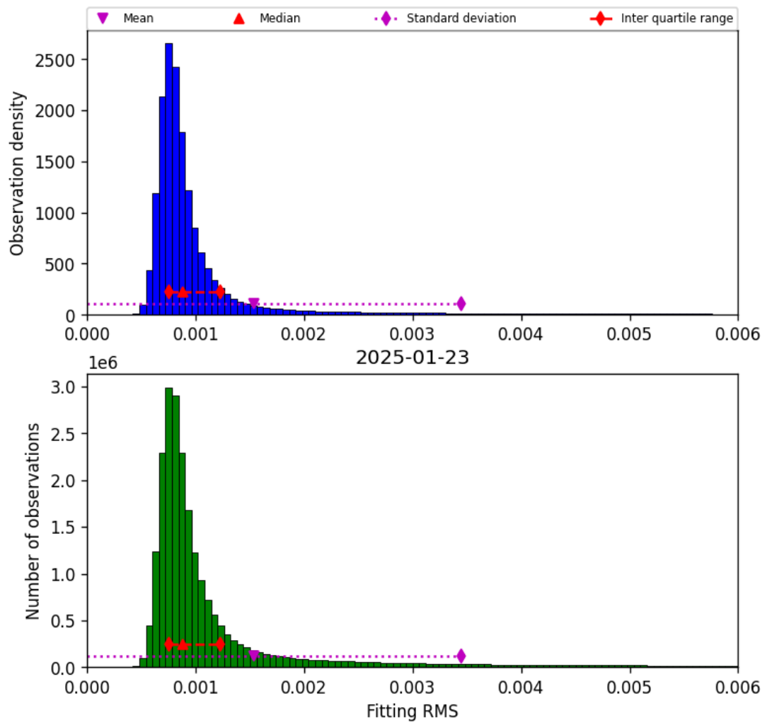
Figure 34: Histogram of “Fitting RMS” for 2025-01-23 to 2025-01-24
