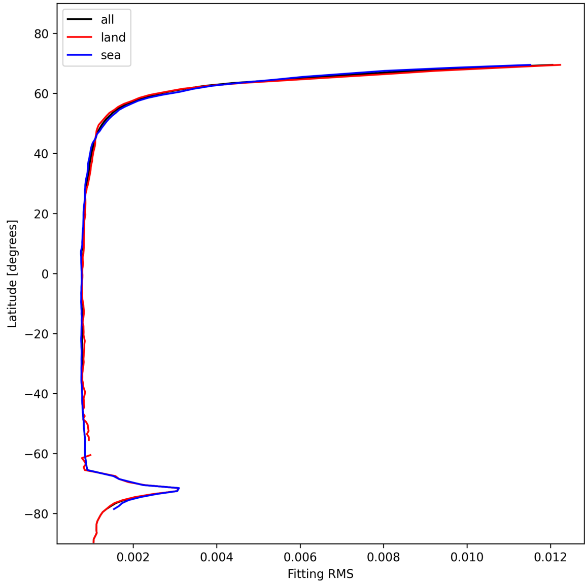
Figure 22: Zonal average of “Fitting RMS” for 2025-01-23 to 2025-01-24.
