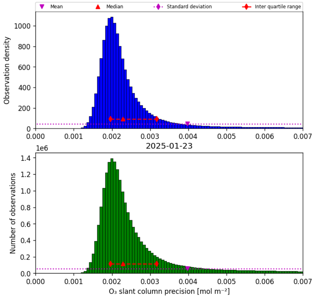
Figure 32: Histogram of “O 3 slant column precision” for 2025-01-23 to 2025-01-24
