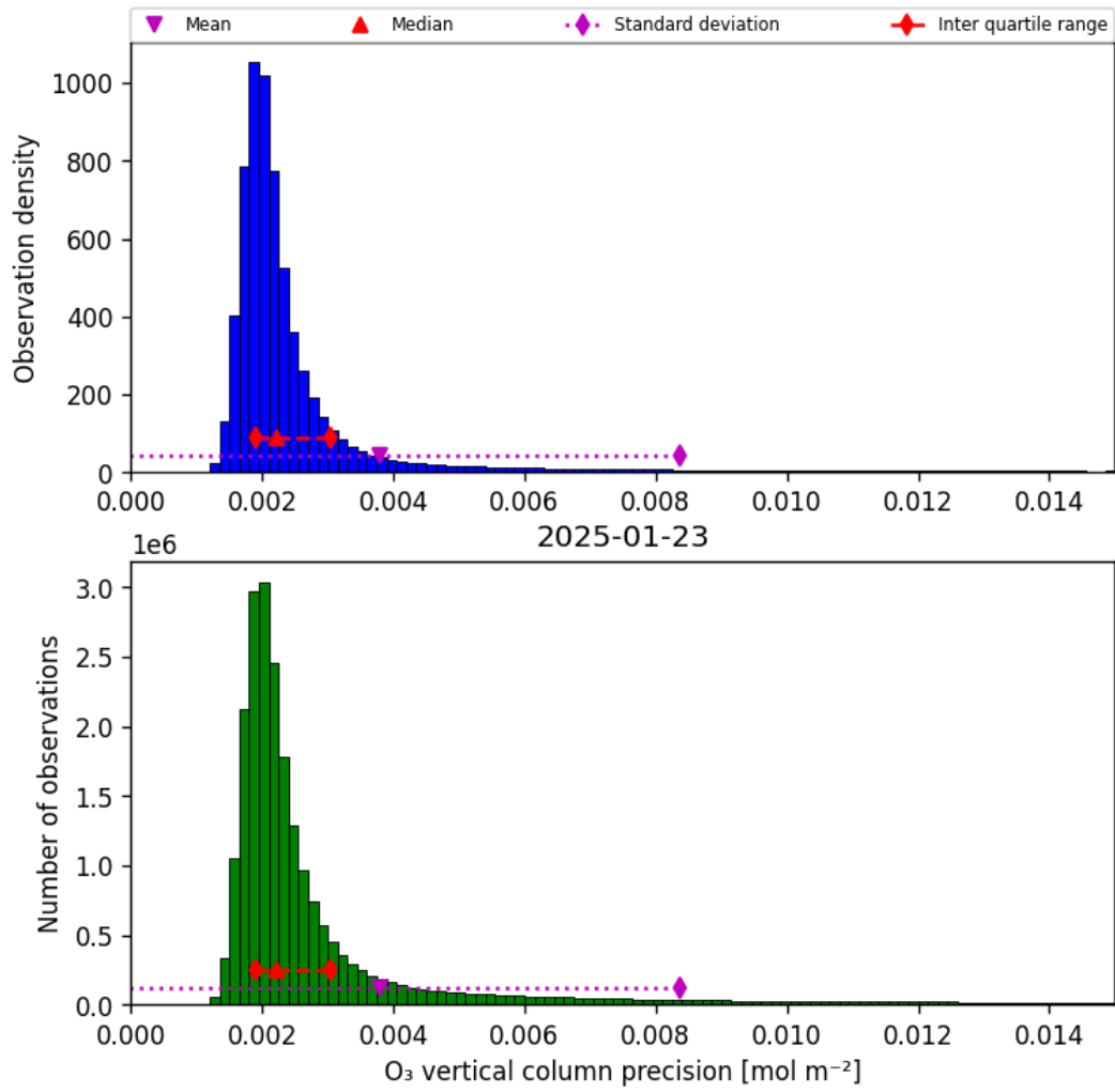
Figure 30: Histogram of “O 3 vertical column precision” for 2025-01-23 to 2025-01-24
