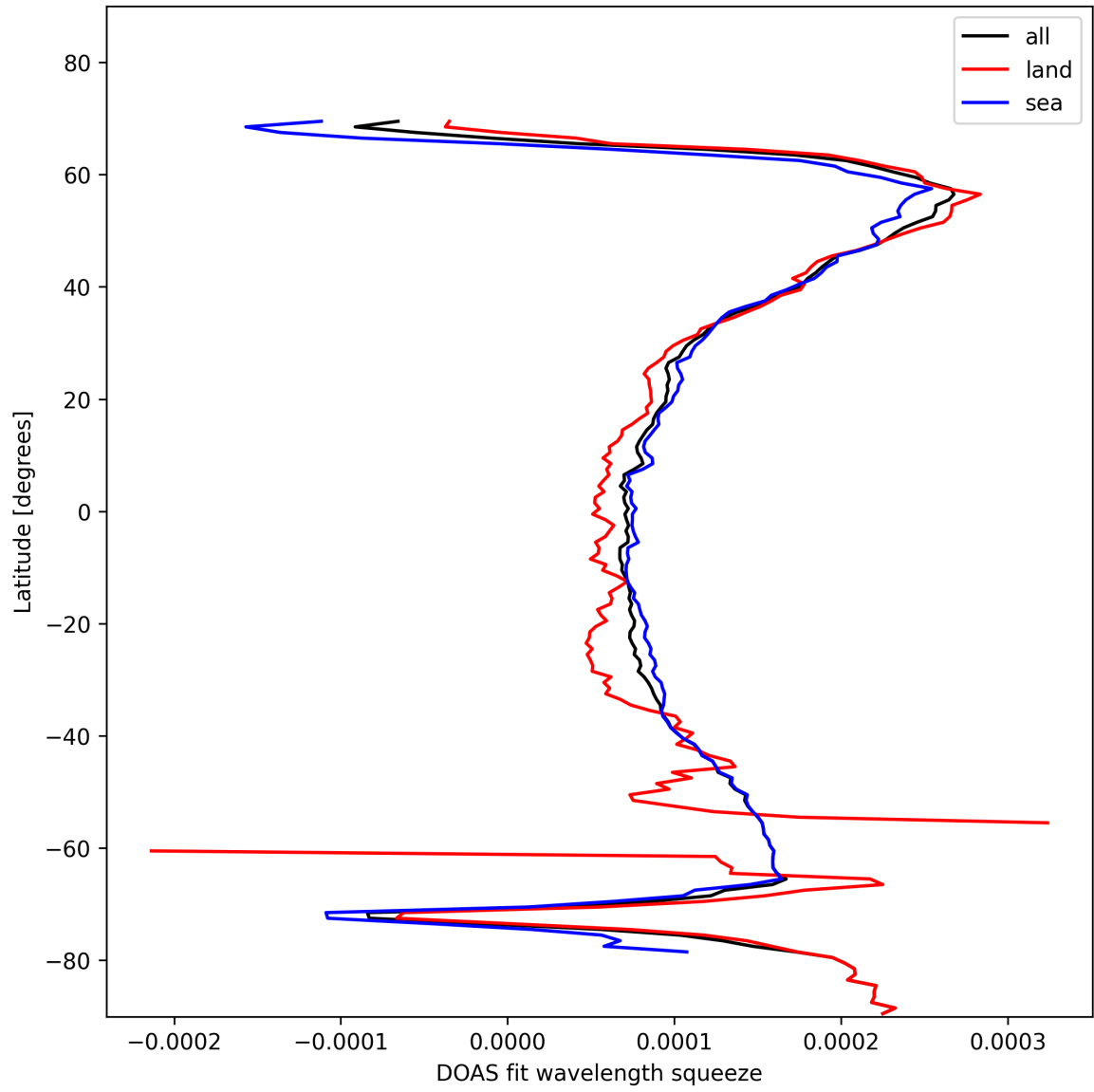
Figure 24: Zonal average of “DOAS fit wavelength squeeze” for 2025-01-23 to 2025-01-24.
