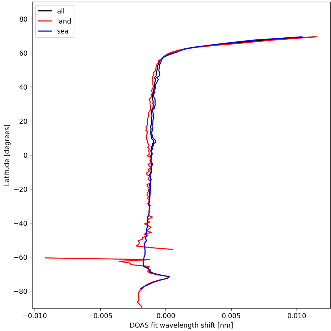
Figure 23: Zonal average of “DOAS fit wavelength shift” for 2025-01-23 to 2025-01-24.
