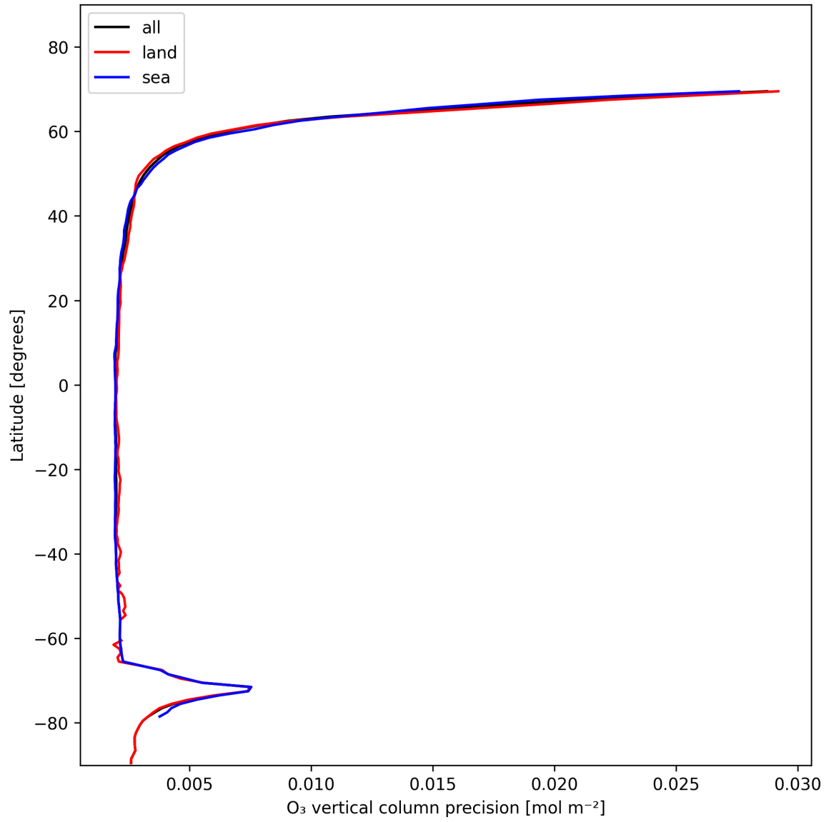
Figure 18: Zonal average of "O 3 vertical column precision" for 2025-01-23 to 2025-01-24.
