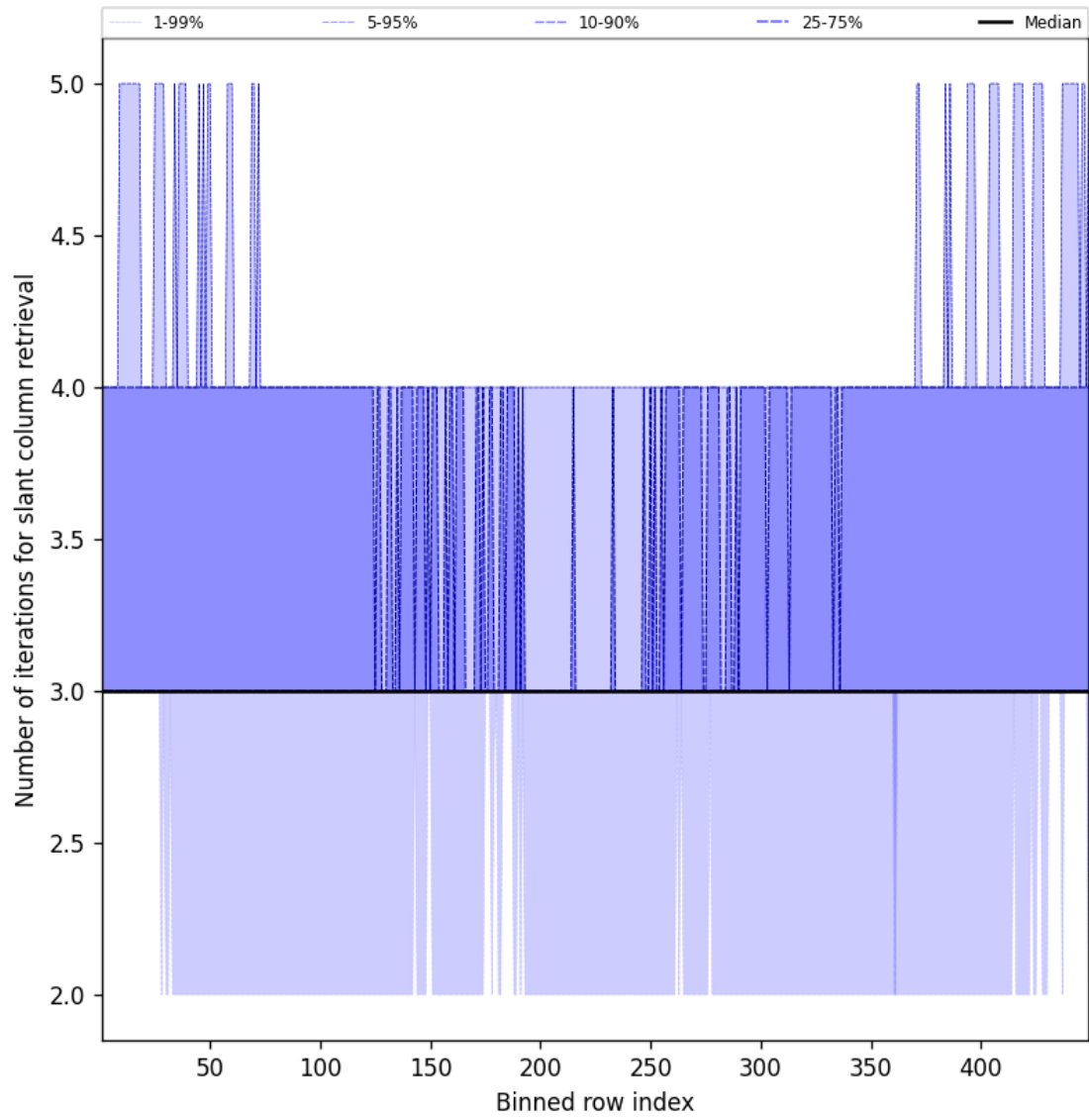
Figure 45: Along track statistics of “Number of iterations for slant column retrieval” for 2025-01-23 to 2025-01-24
