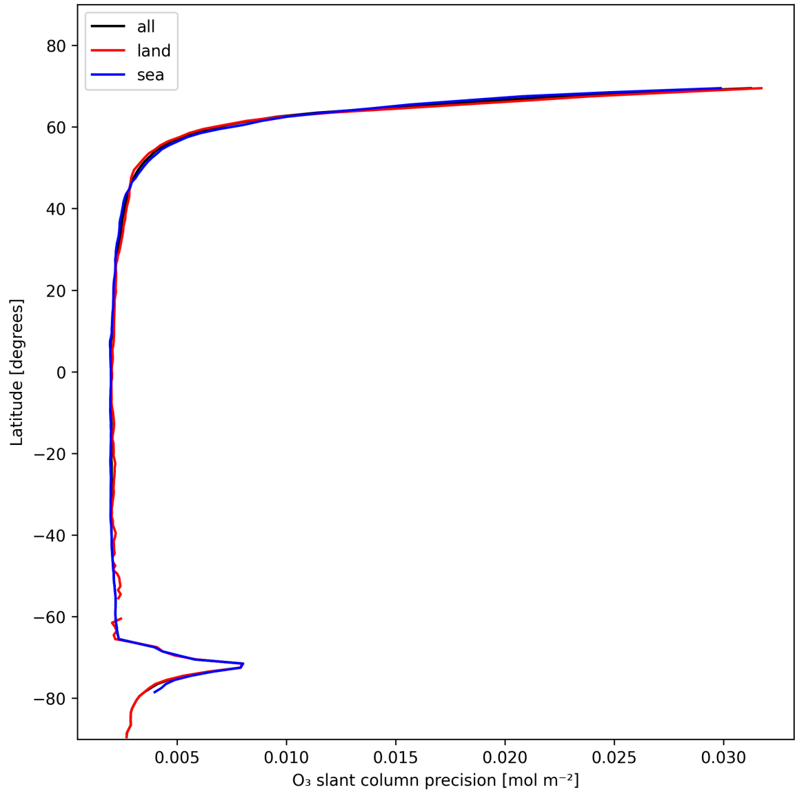
Figure 20: Zonal average of “O 3 slant column precision” for 2025-01-23 to 2025-01-24.
