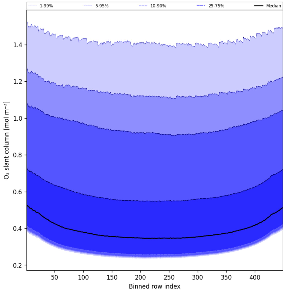
Figure 43: Along track statistics of “O 3 slant column” for 2025-01-23 to 2025-01-24
