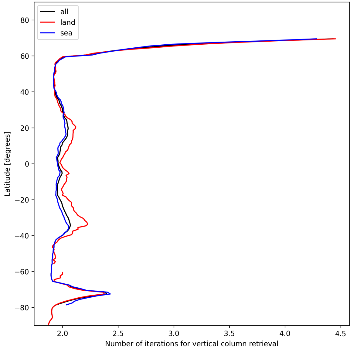
Figure 27: Zonal average of “Number of iterations for vertical column retrieval” for 2025-01-23 to 2025-01-24.
