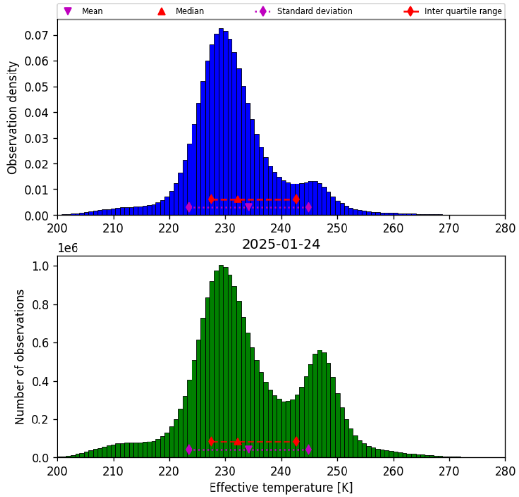
Figure 38: Histogram of “Effective temperature” for 2025-01-24 to 2025-01-25
