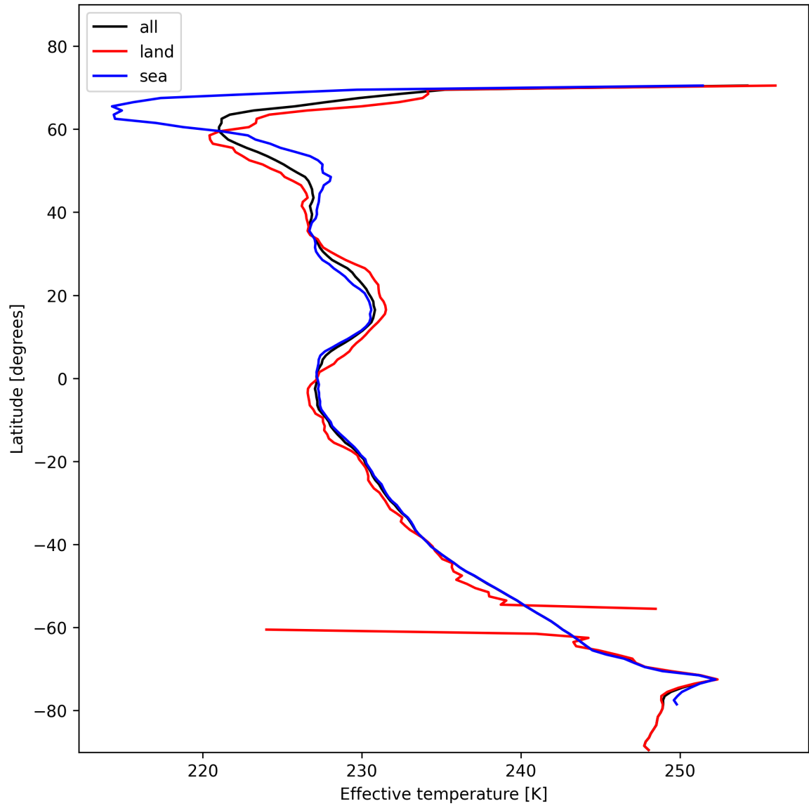
Figure 26: Zonal average of “Effective temperature” for 2025-01-24 to 2025-01-25.
