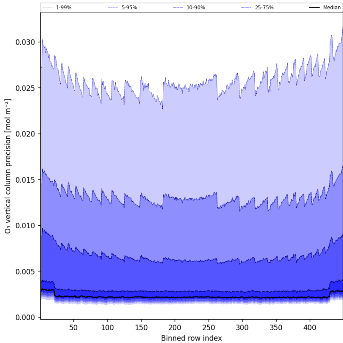
Figure 42: Along track statistics of “O 3 vertical column precision” for 2025-01-24 to 2025-01-25
