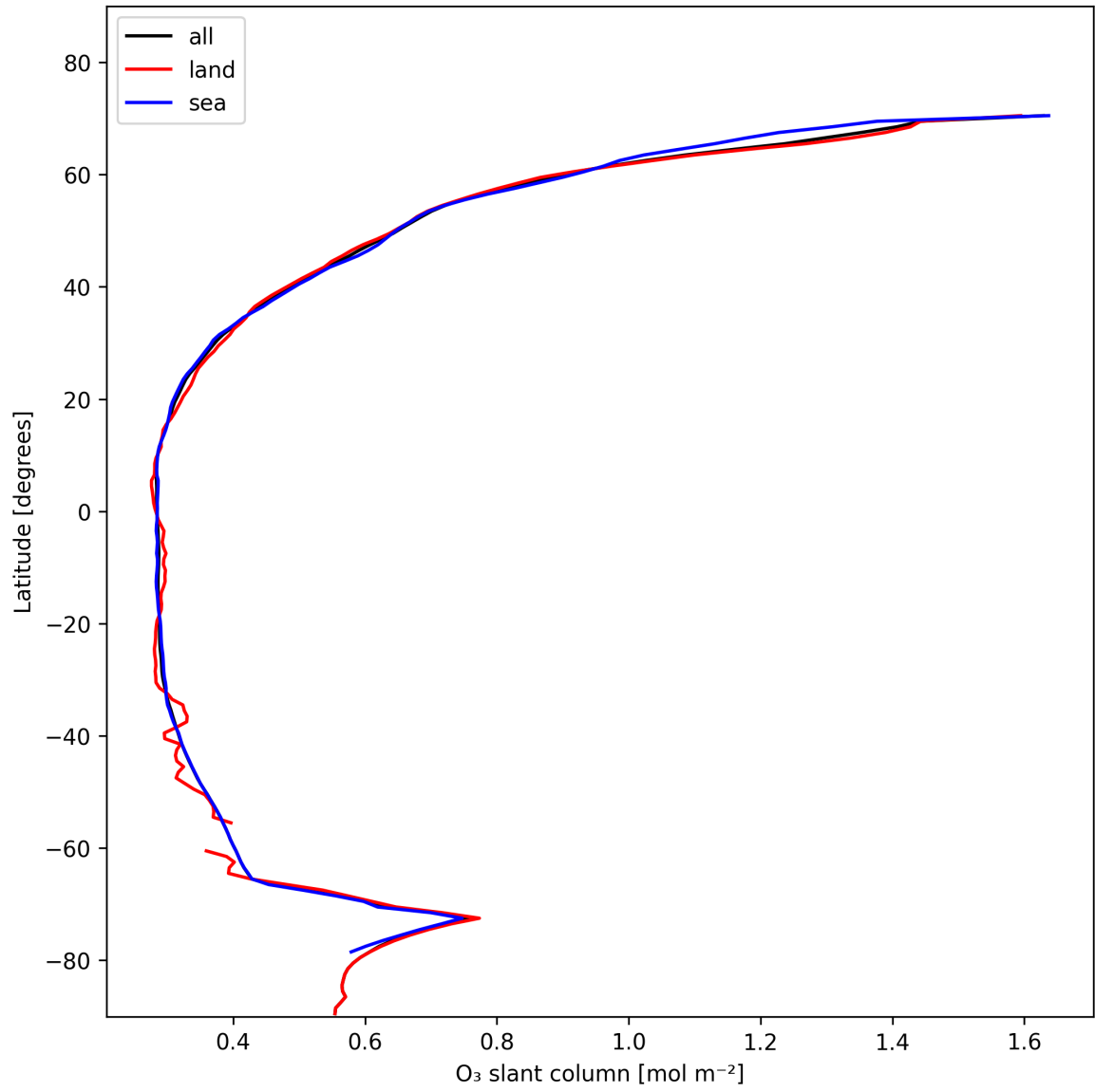
Figure 19: Zonal average of “O 3 slant column” for 2025-01-24 to 2025-01-25.
