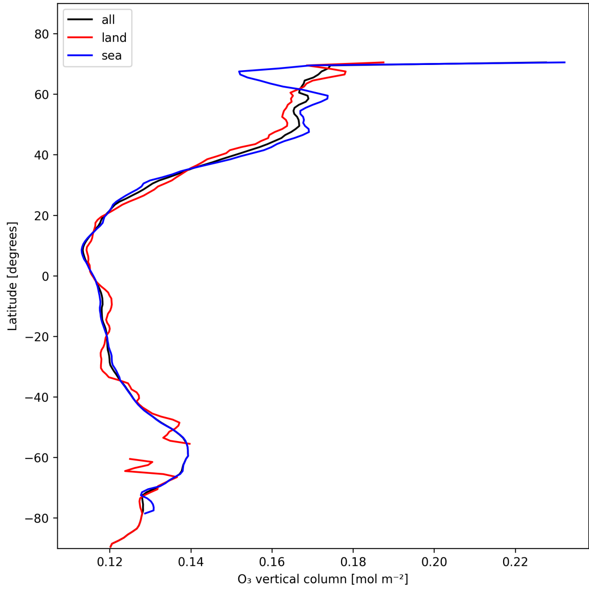
Figure 17: Zonal average of “O 3 vertical column” for 2025-01-24 to 2025-01-25.
