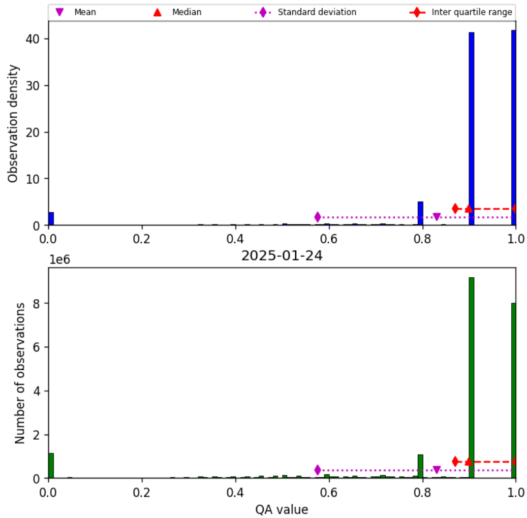
Figure 28: Histogram of “QA value” for 2025-01-24 to 2025-01-25
