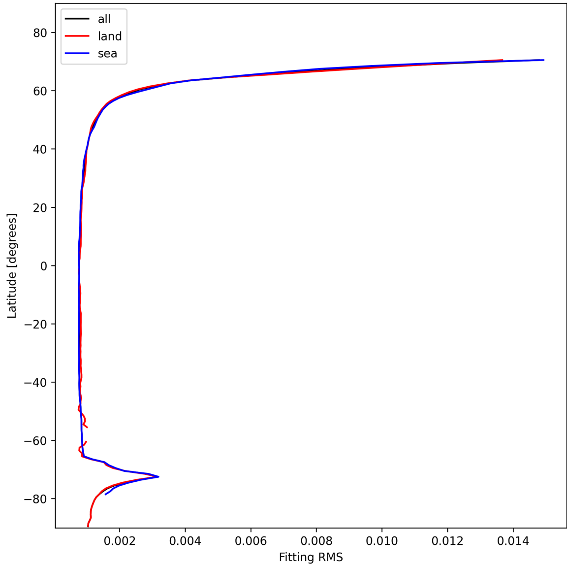
Figure 22: Zonal average of “Fitting RMS” for 2025-01-24 to 2025-01-25.
