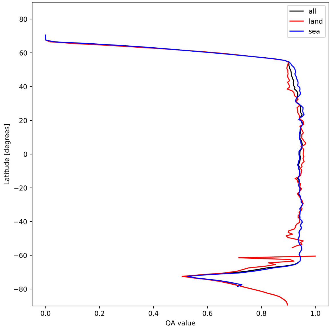
Figure 16: Zonal average of “QA value” for 2025-01-24 to 2025-01-25.
