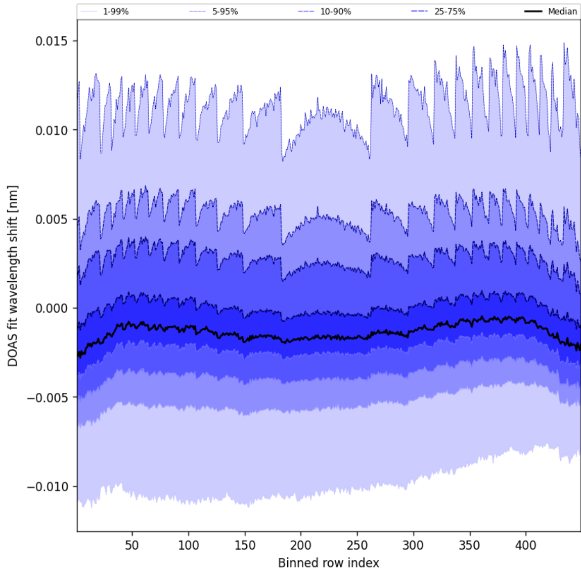
Figure 47: Along track statistics of “DOAS fit wavelength shift” for 2025-01-24 to 2025-01-25
