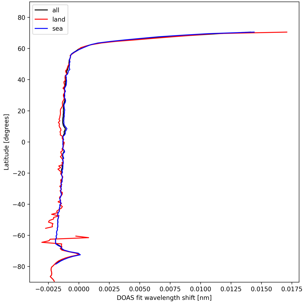
Figure 23: Zonal average of “DOAS fit wavelength shift” for 2025-01-24 to 2025-01-25.
