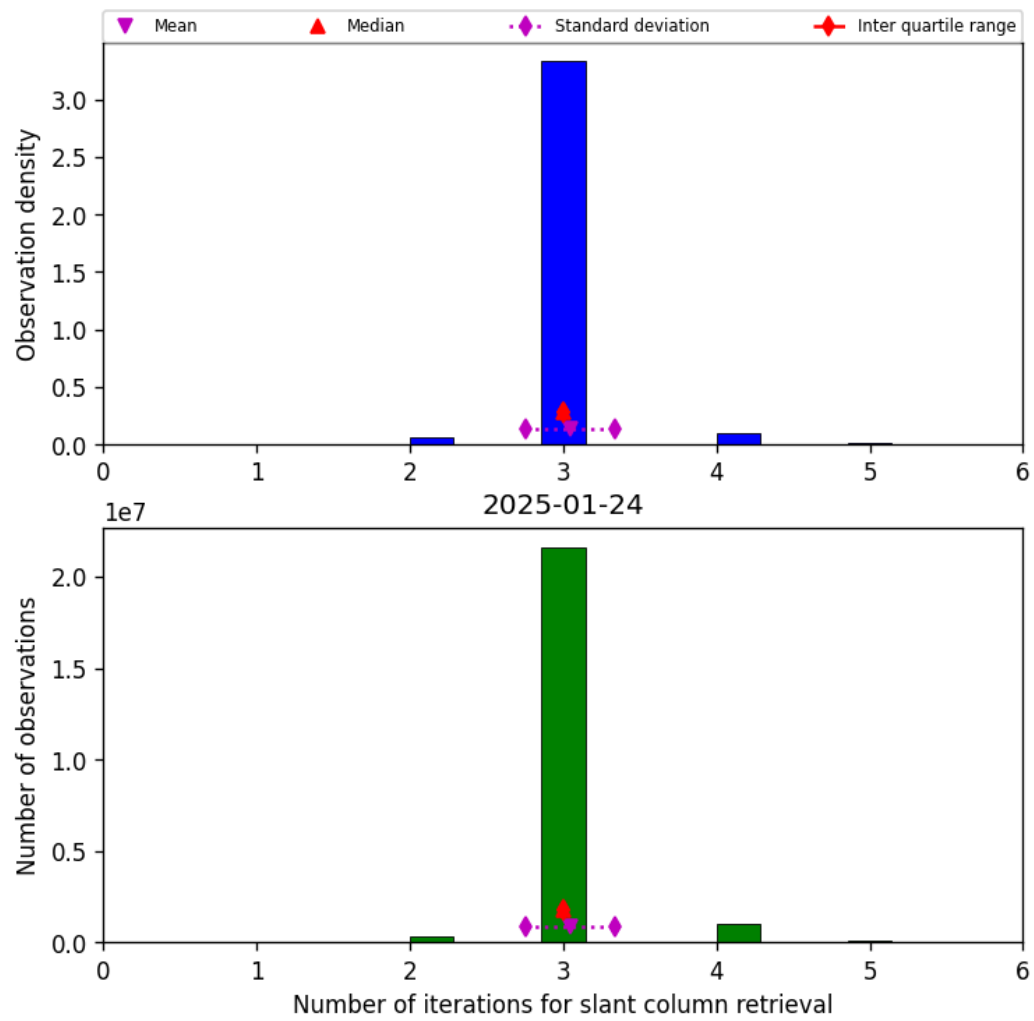
Figure 33: Histogram of “Number of iterations for slant column retrieval” for 2025-01-24 to 2025-01-25
