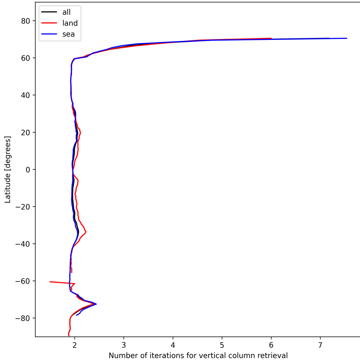
Figure 27: Zonal average of “Number of iterations for vertical column retrieval” for 2025-01-24 to 2025-01-25.
