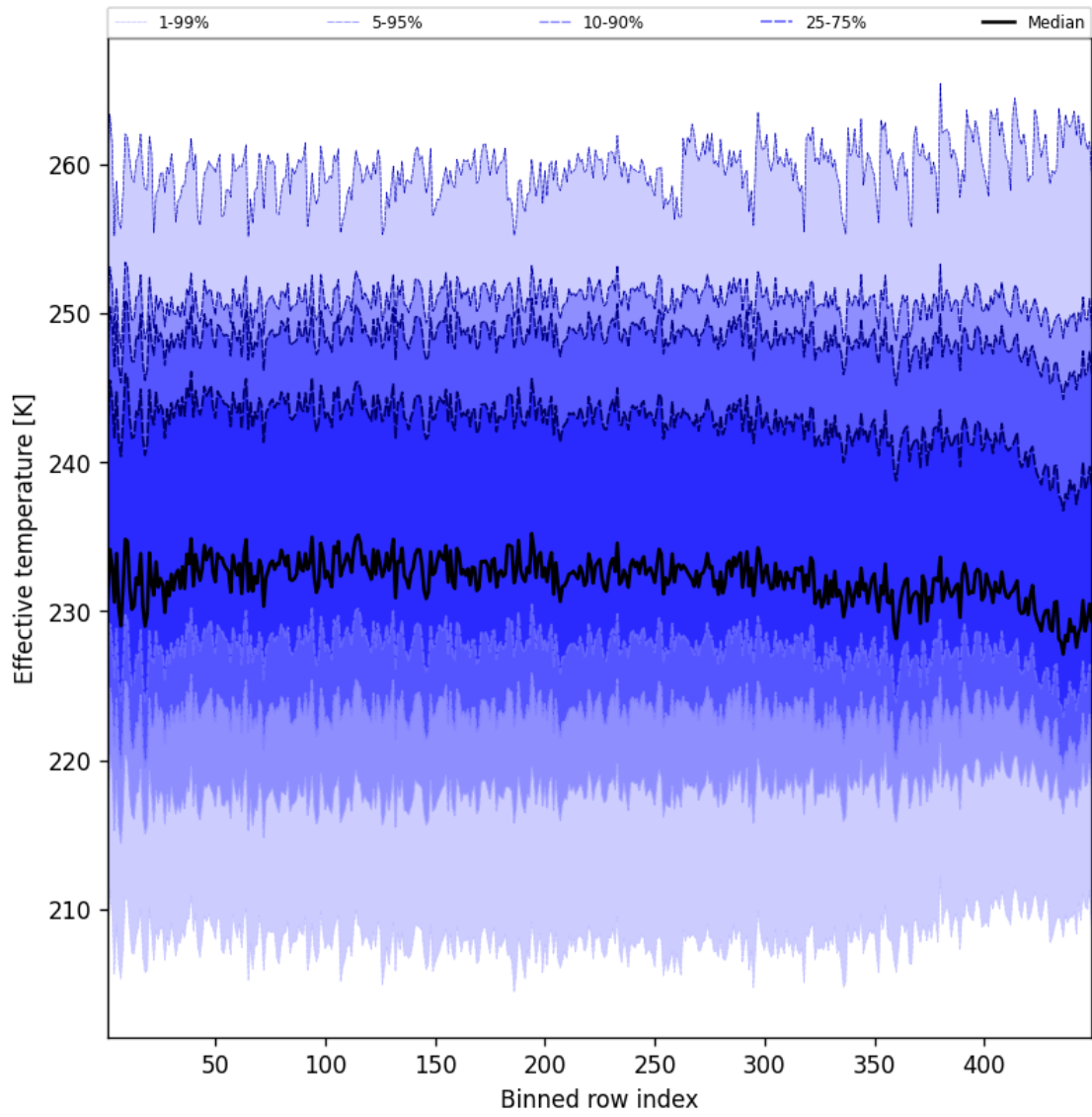
Figure 50: Along track statistics of “Effective temperature” for 2025-01-24 to 2025-01-25
