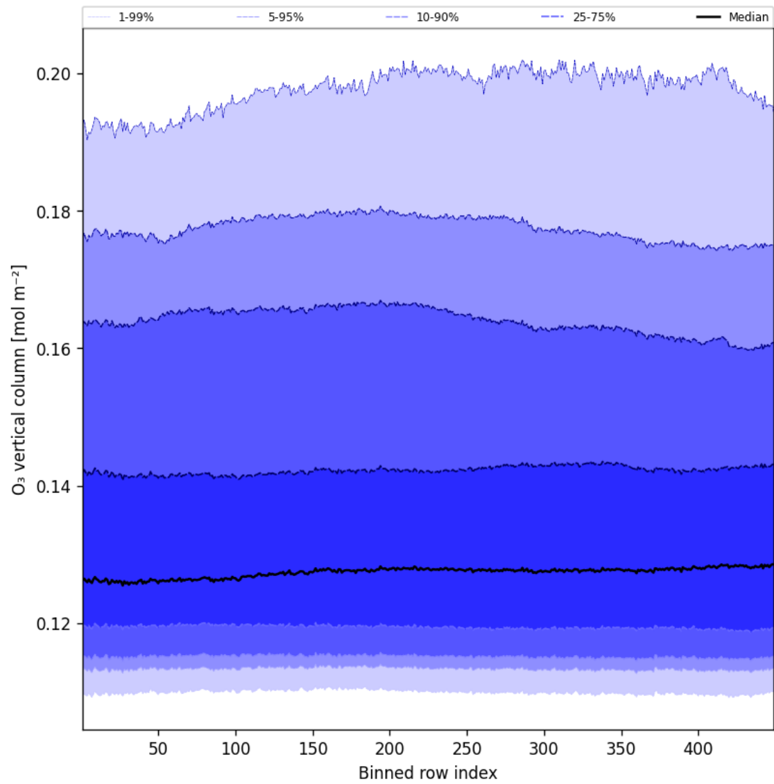
Figure 41: Along track statistics of “ \text{O}_3 vertical column” for 2025-01-24 to 2025-01-25
