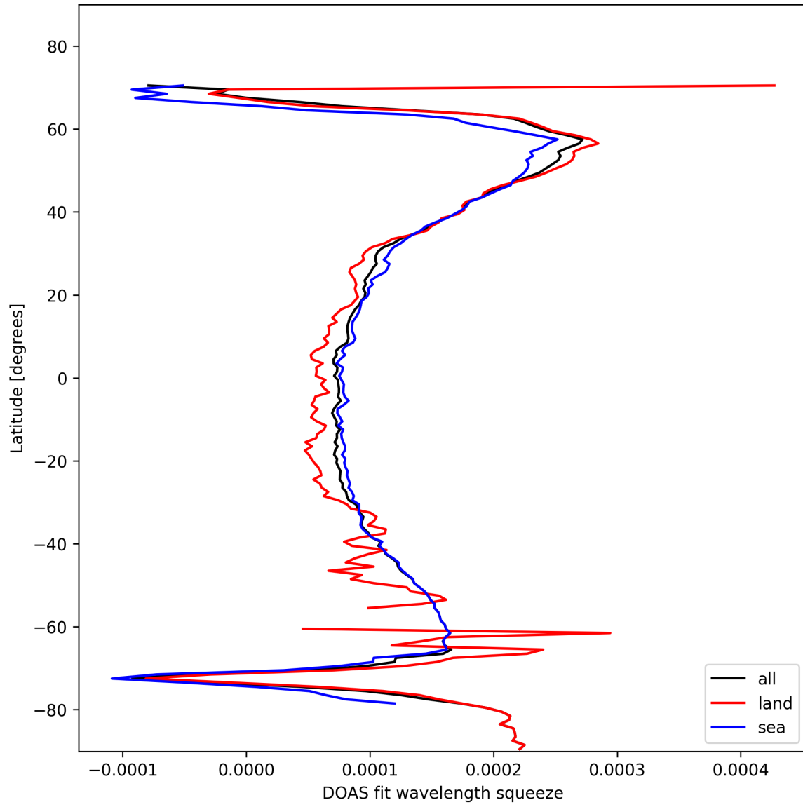
Figure 24: Zonal average of “DOAS fit wavelength squeeze” for 2025-01-24 to 2025-01-25.
