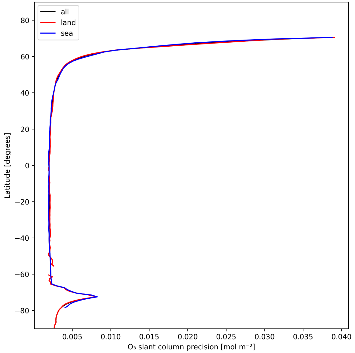
Figure 20: Zonal average of “O 3 slant column precision” for 2025-01-24 to 2025-01-25.
