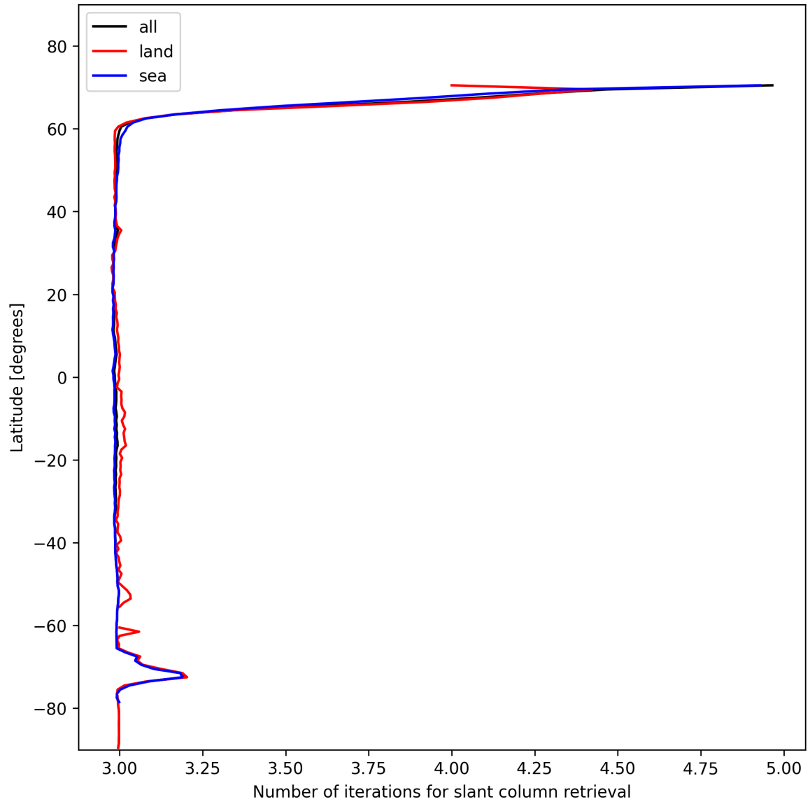
Figure 21: Zonal average of “Number of iterations for slant column retrieval” for 2025-01-24 to 2025-01-25.
