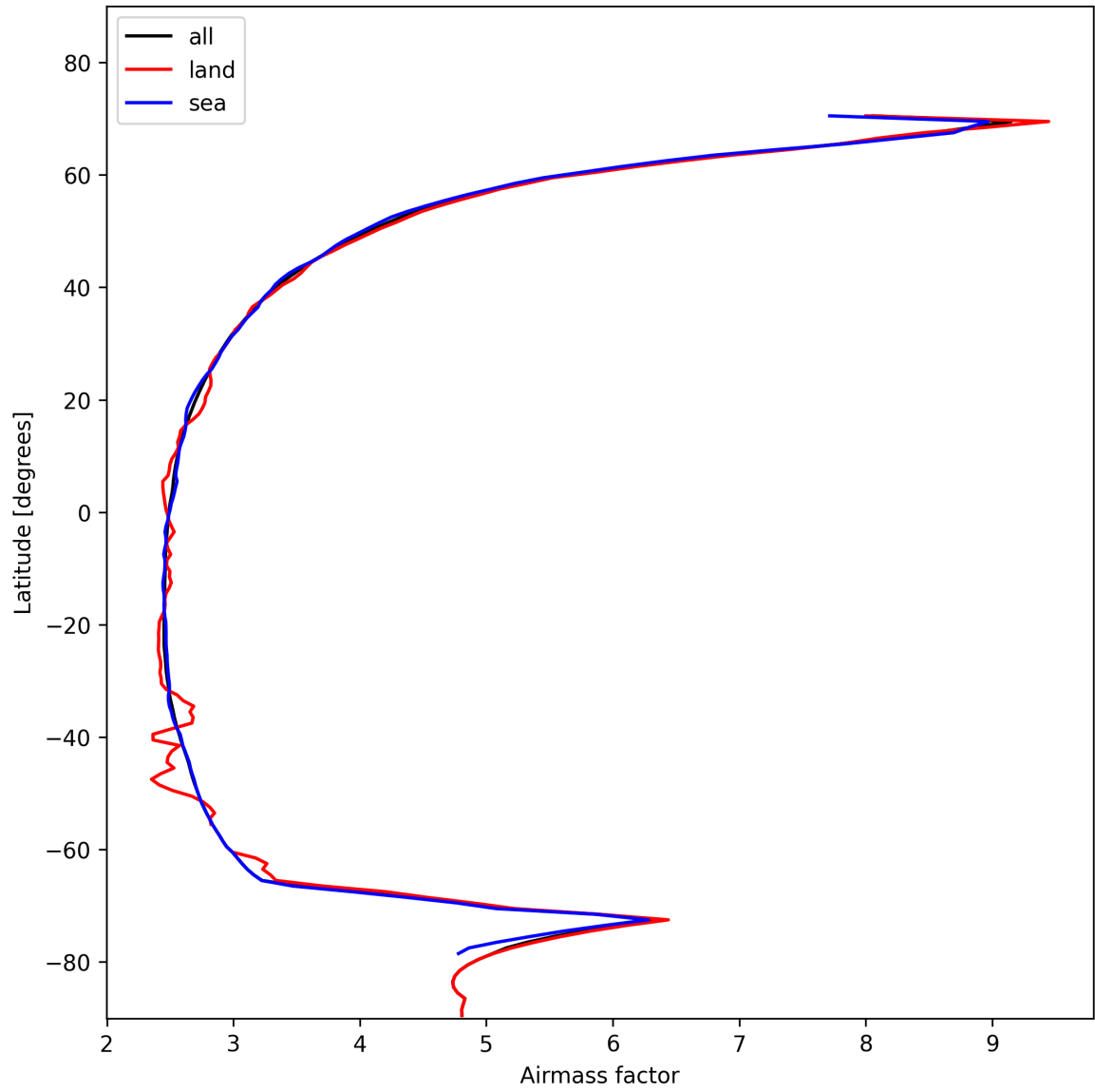
Figure 25: Zonal average of “Airmass factor” for 2025-01-24 to 2025-01-25.
