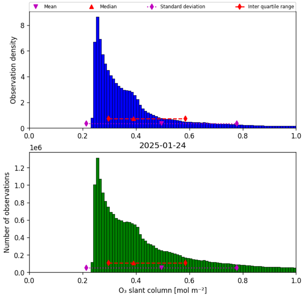
Figure 31: Histogram of “O 3 slant column” for 2025-01-24 to 2025-01-25
