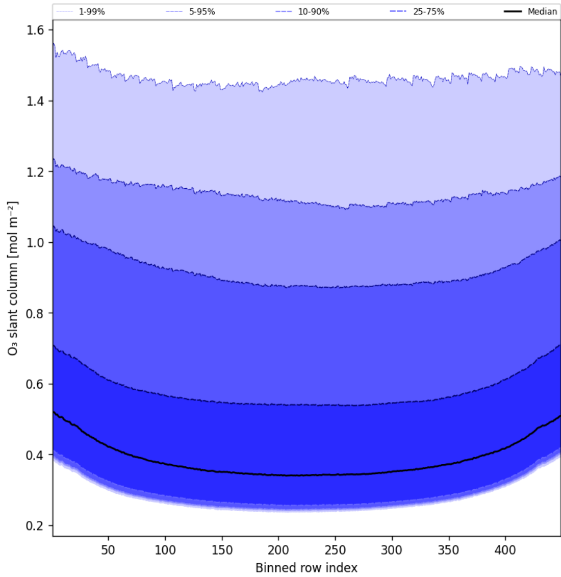
Figure 43: Along track statistics of “O 3 slant column” for 2025-01-24 to 2025-01-25
