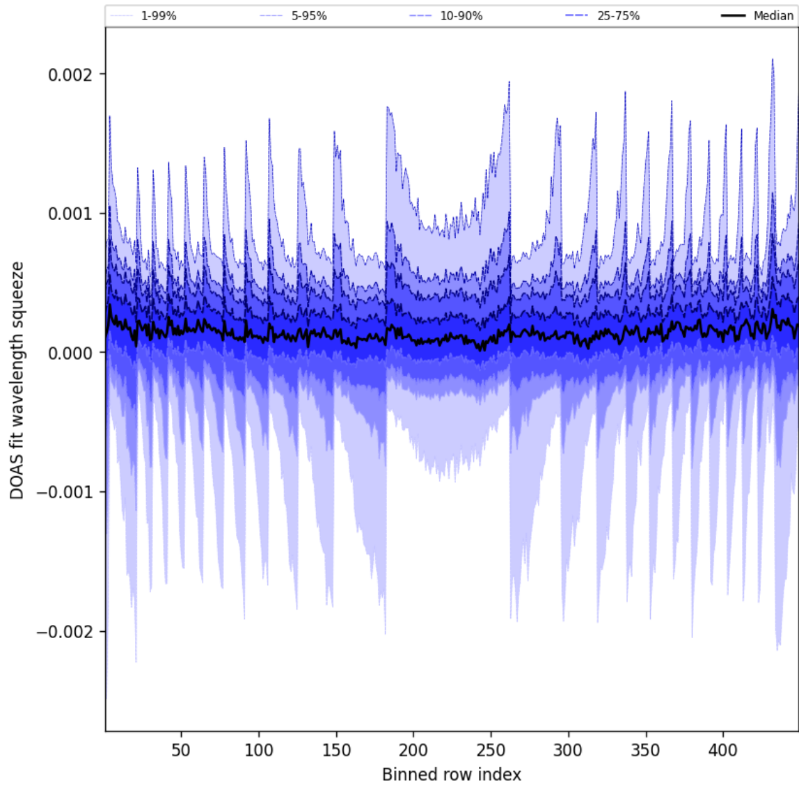
Figure 48: Along track statistics of “DOAS fit wavelength squeeze” for 2025-01-24 to 2025-01-25
