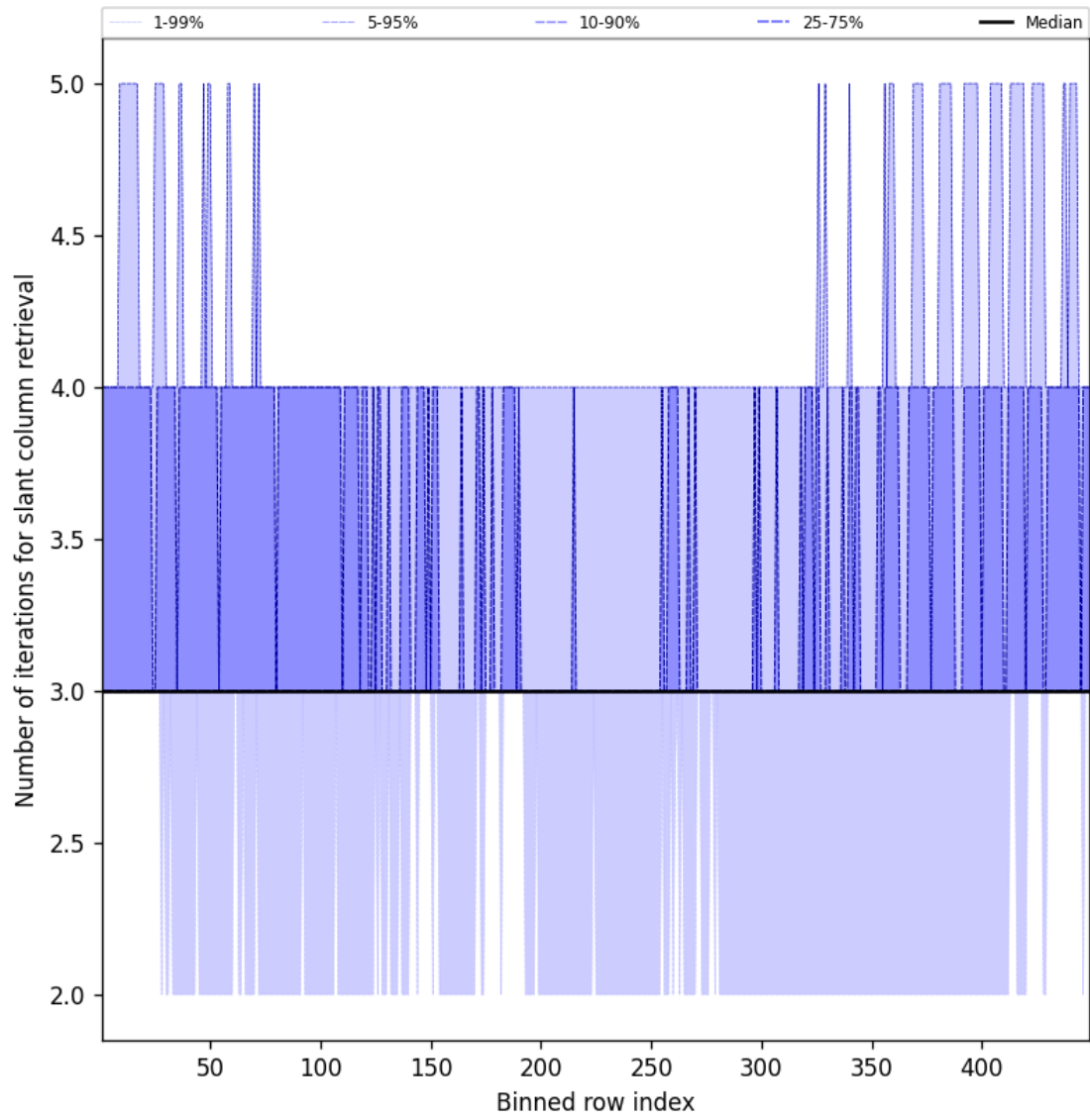
Figure 45: Along track statistics of “Number of iterations for slant column retrieval” for 2025-01-24 to 2025-01-25
