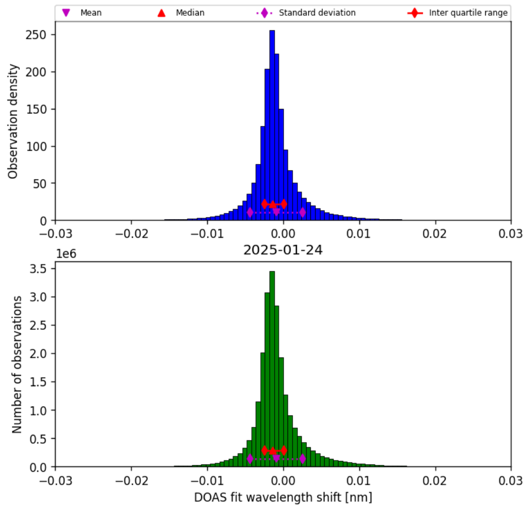
Figure 35: Histogram of “DOAS fit wavelength shift” for 2025-01-24 to 2025-01-25
