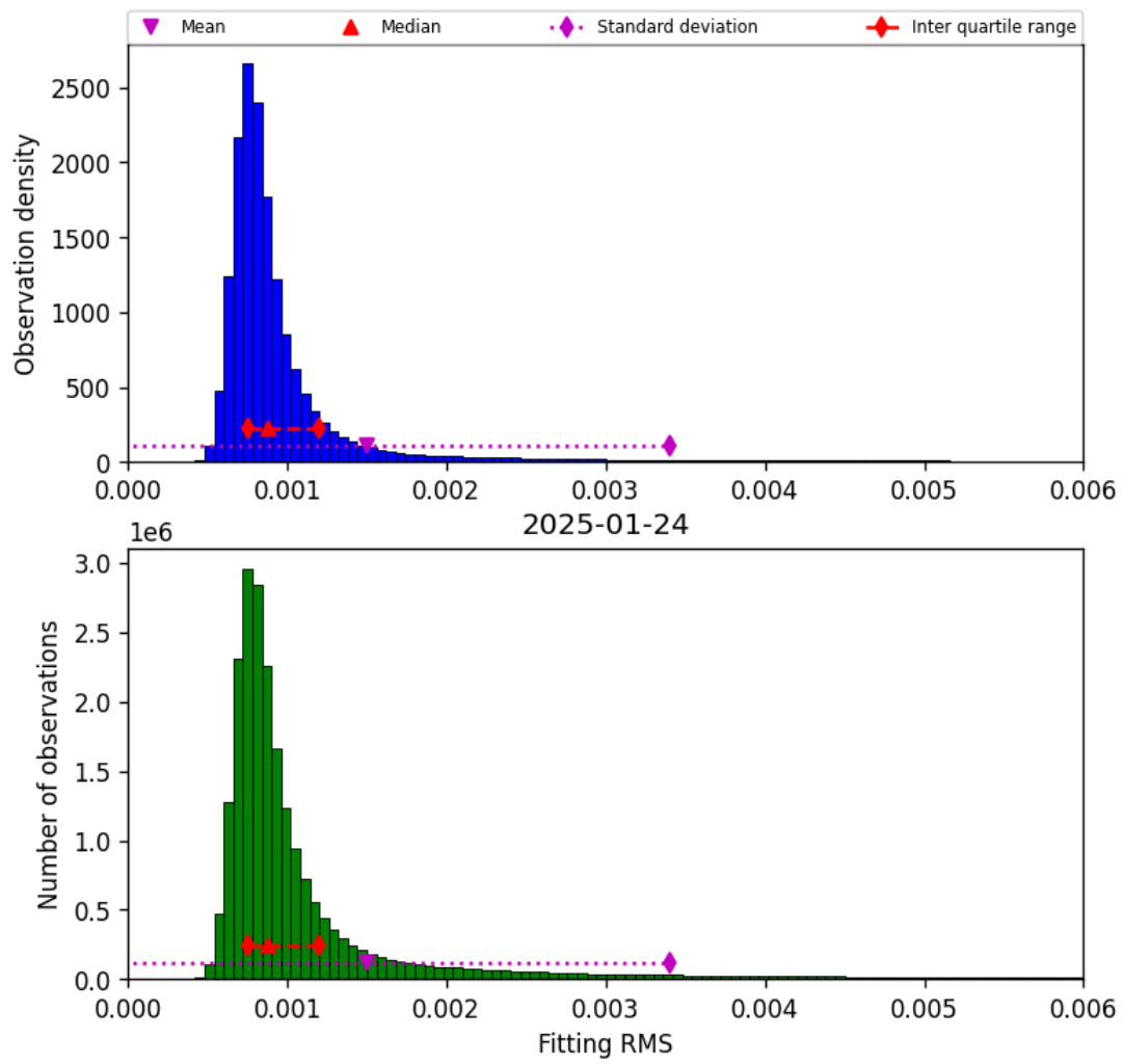
Figure 34: Histogram of “Fitting RMS” for 2025-01-24 to 2025-01-25
