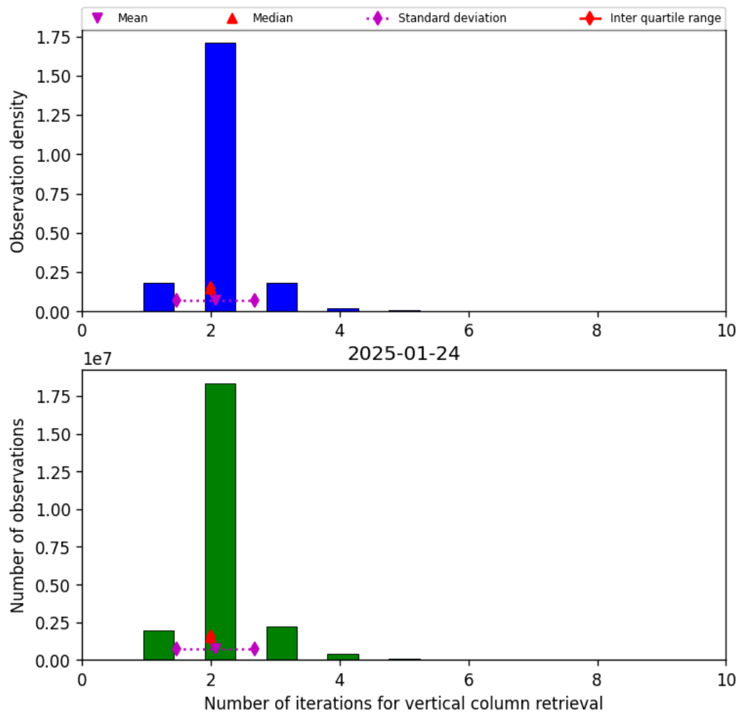
Figure 39: Histogram of “Number of iterations for vertical column retrieval” for 2025-01-24 to 2025-01-25
