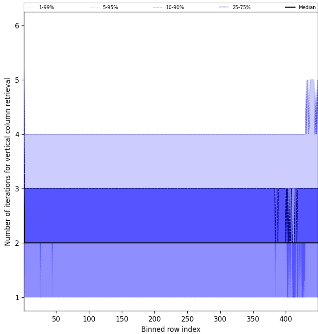
Figure 51: Along track statistics of “Number of iterations for vertical column retrieval” for 2025-01-24 to 2025-01-25
