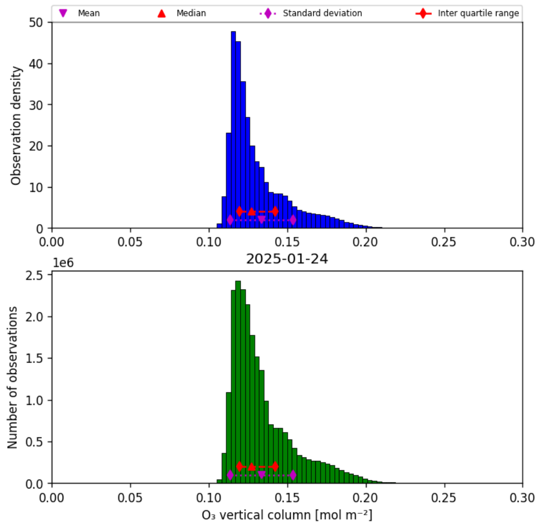
Figure 29: Histogram of “O 3 vertical column” for 2025-01-24 to 2025-01-25
