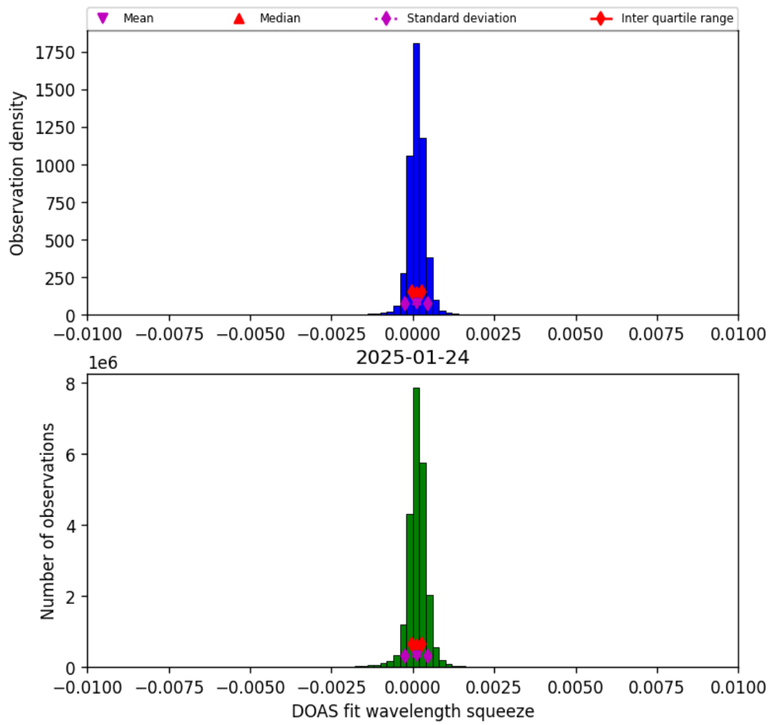
Figure 36: Histogram of “DOAS fit wavelength squeeze” for 2025-01-24 to 2025-01-25
