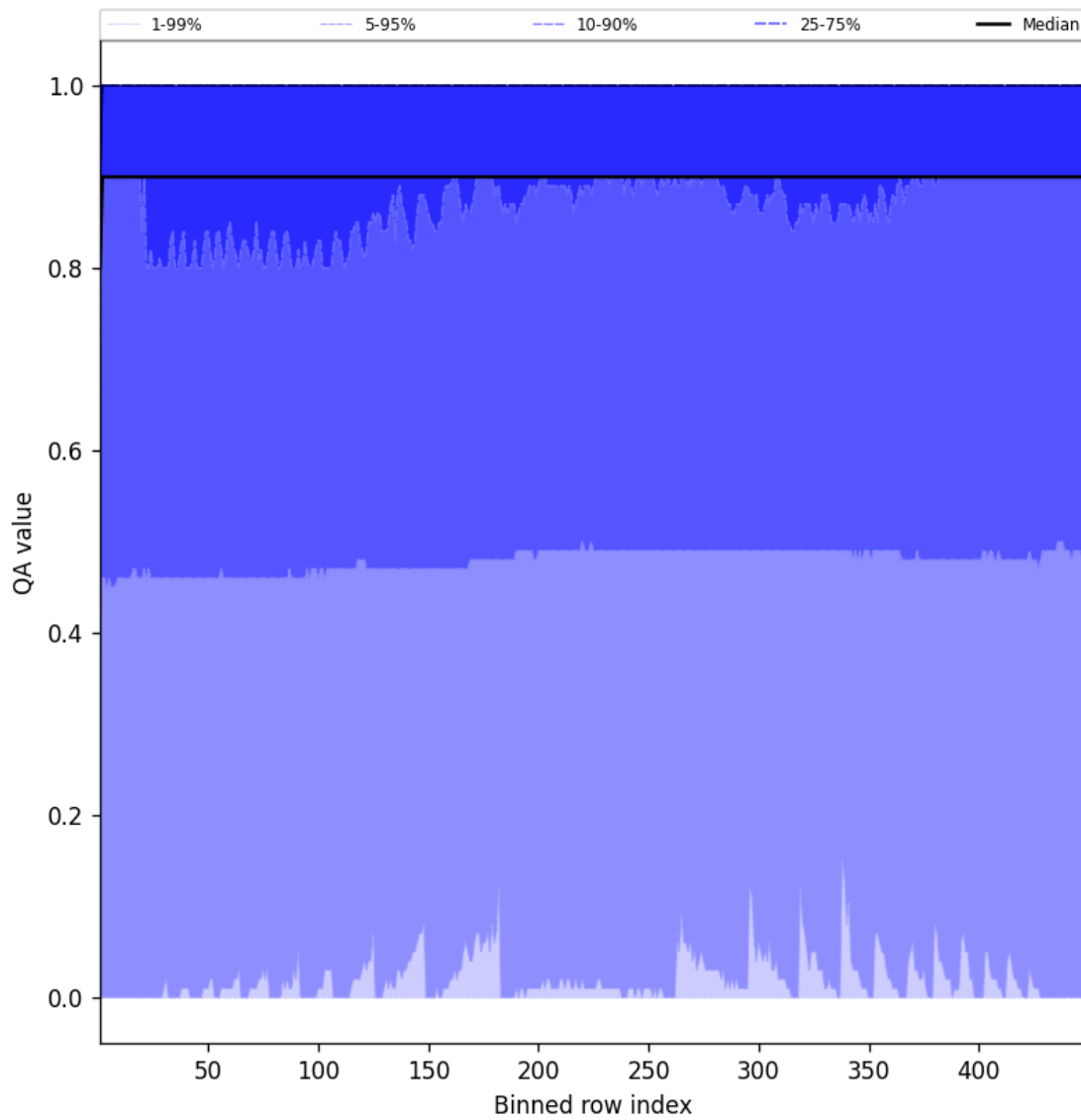
Figure 40: Along track statistics of “QA value” for 2025-01-24 to 2025-01-25
