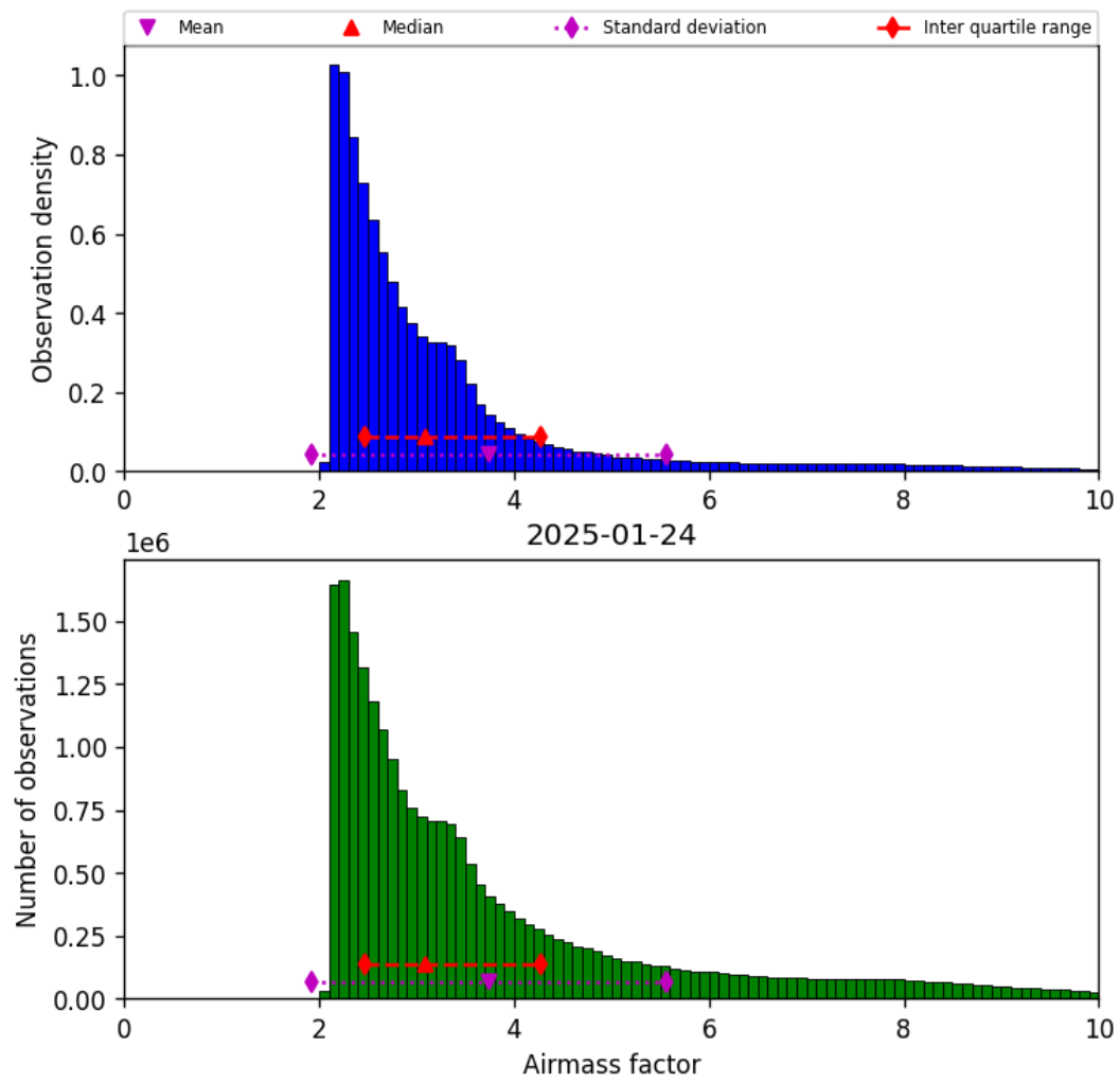
Figure 37: Histogram of “Airmass factor” for 2025-01-24 to 2025-01-25
