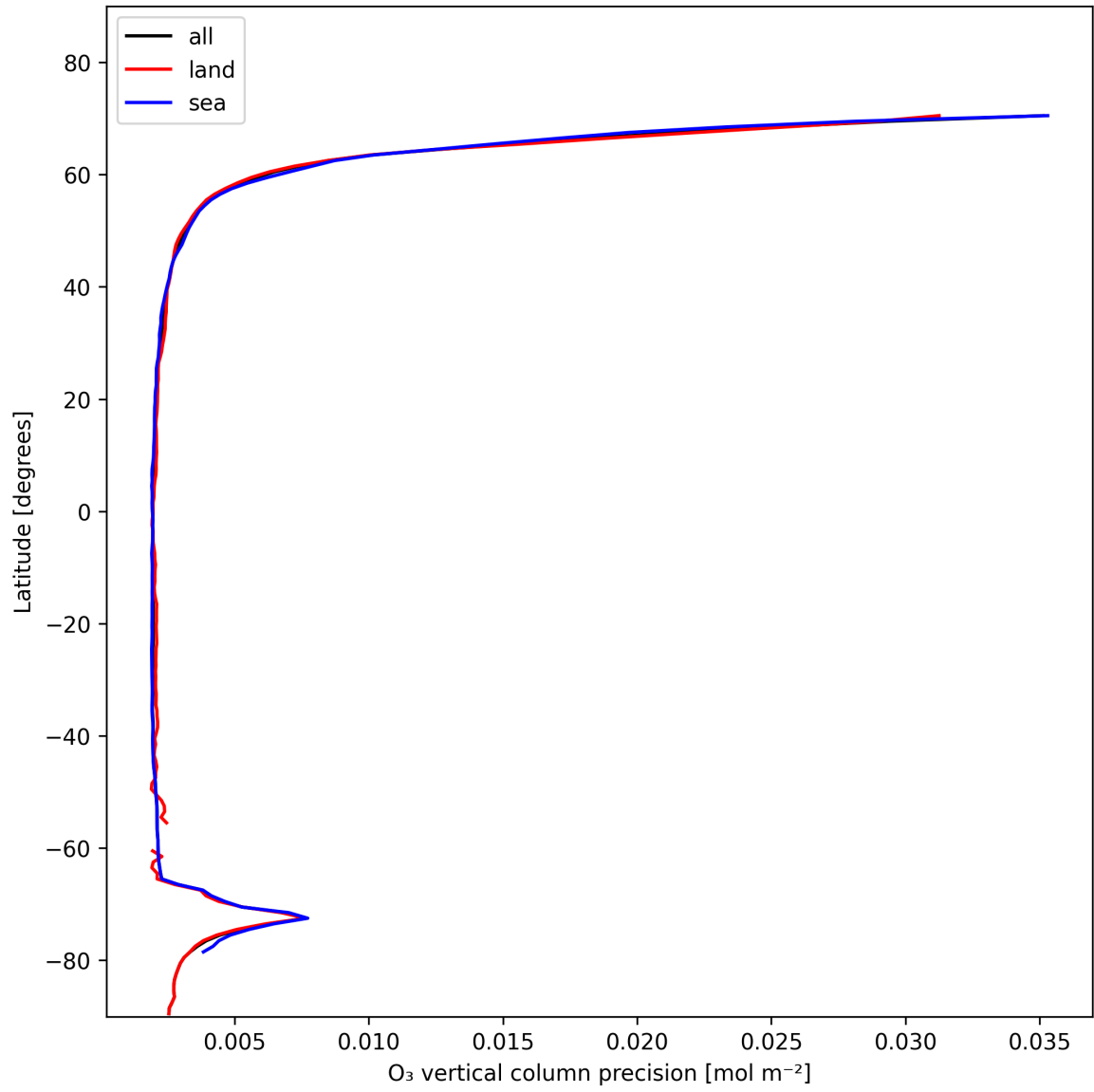
Figure 18: Zonal average of “O 3 vertical column precision” for 2025-01-24 to 2025-01-25.
