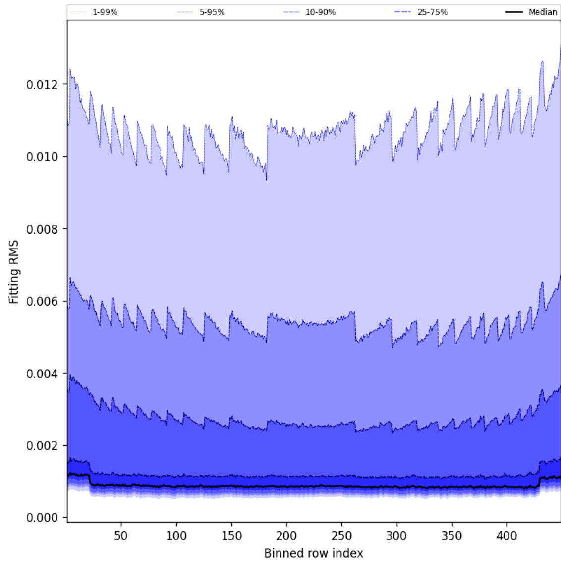
Figure 46: Along track statistics of “Fitting RMS” for 2025-01-24 to 2025-01-25
