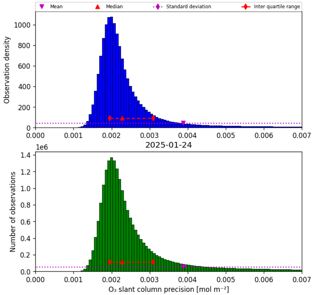
Figure 32: Histogram of “O 3 slant column precision” for 2025-01-24 to 2025-01-25
