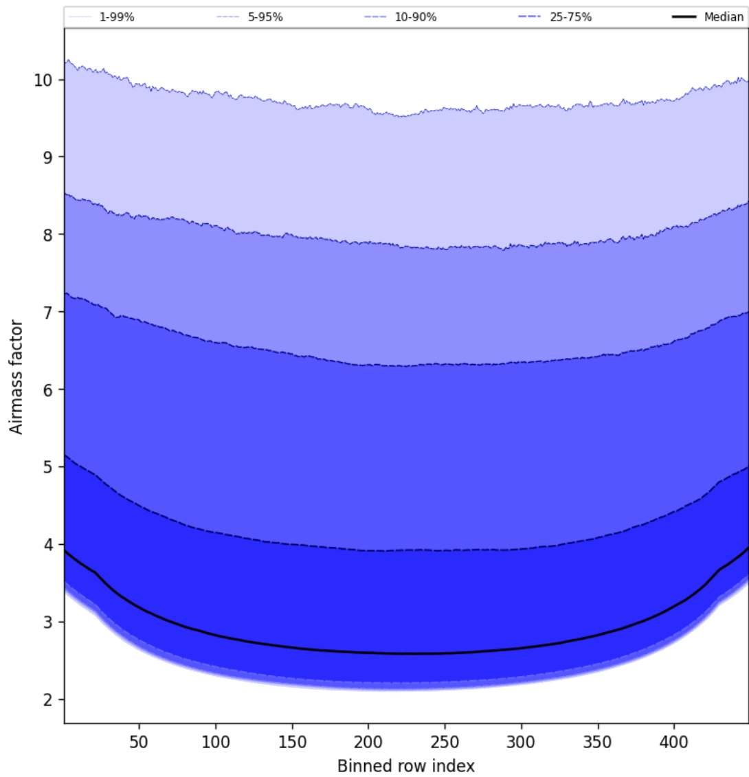
Figure 49: Along track statistics of “Airmass factor” for 2025-01-24 to 2025-01-25
