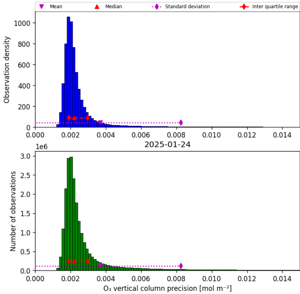
Figure 30: Histogram of “O 3 vertical column precision” for 2025-01-24 to 2025-01-25
