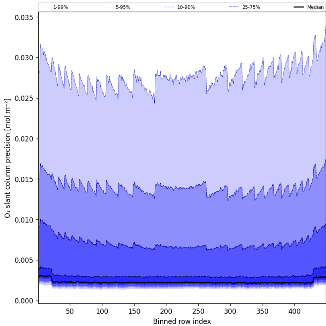
Figure 44: Along track statistics of “O 3 slant column precision” for 2025-01-24 to 2025-01-25
