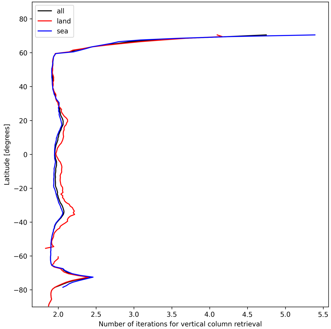
Figure 27: Zonal average of “Number of iterations for vertical column retrieval” for 2025-01-25 to 2025-01-26.
