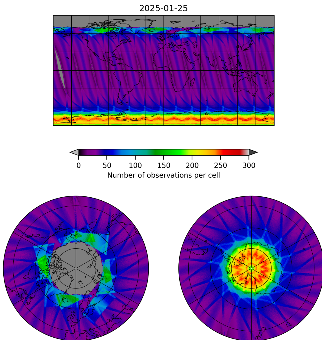
Figure 15: Map of the number of observations for 2025-01-25 to 2025-01-26
