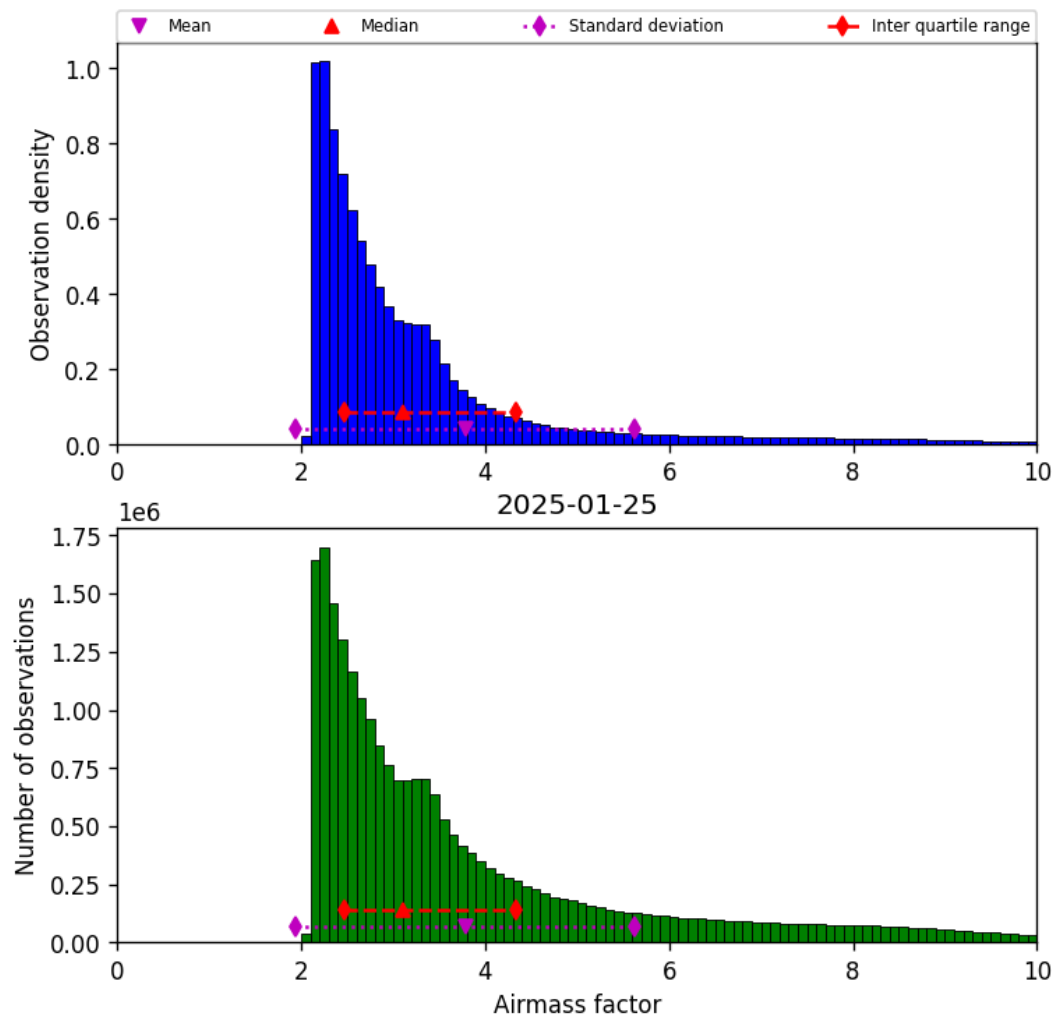
Figure 37: Histogram of “Airmass factor” for 2025-01-25 to 2025-01-26
