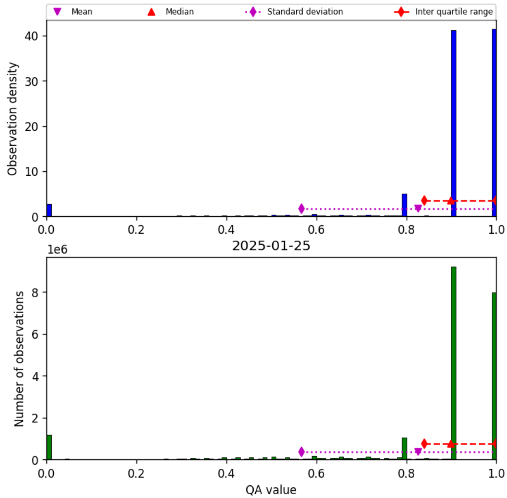
Figure 28: Histogram of “QA value” for 2025-01-25 to 2025-01-26
