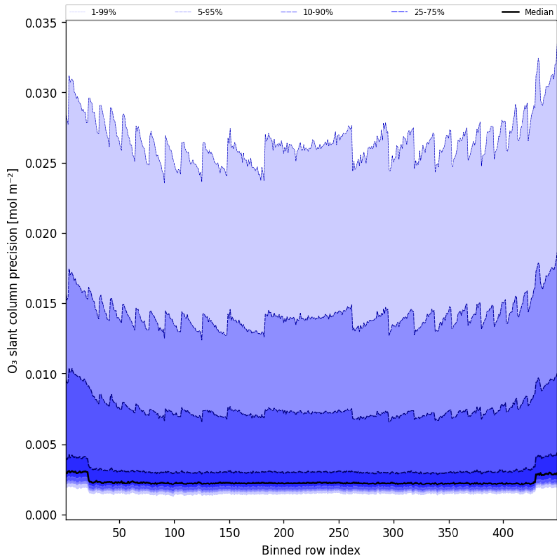
Figure 44: Along track statistics of “O 3 slant column precision” for 2025-01-25 to 2025-01-26
