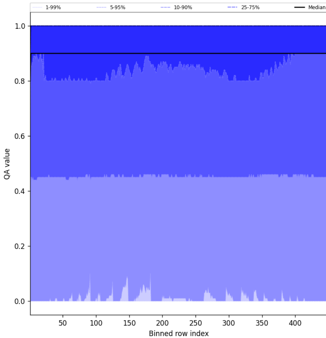
Figure 40: Along track statistics of “QA value” for 2025-01-25 to 2025-01-26
