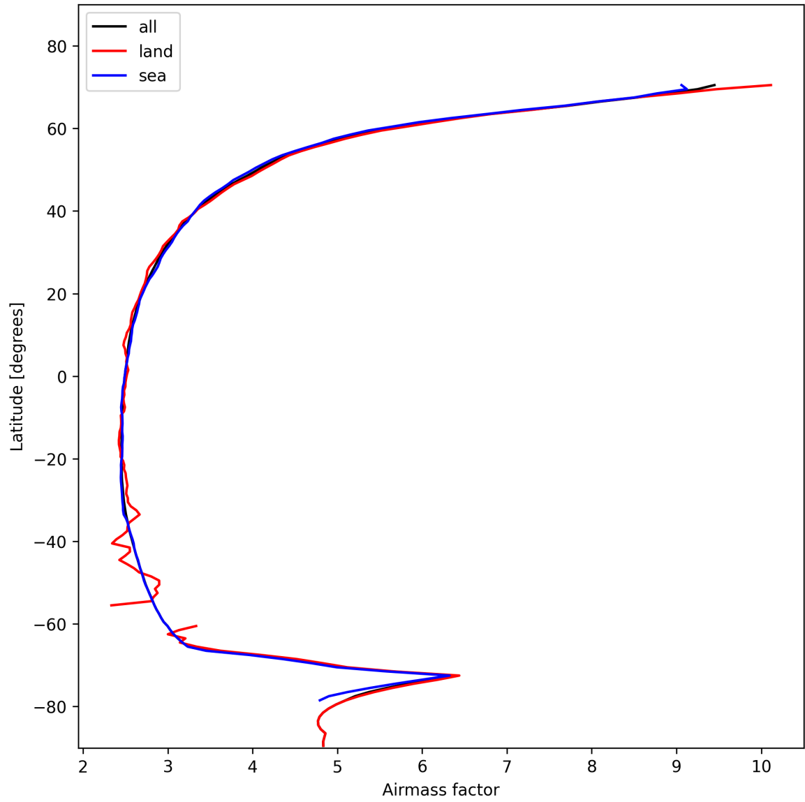
Figure 25: Zonal average of “Airmass factor” for 2025-01-25 to 2025-01-26.
