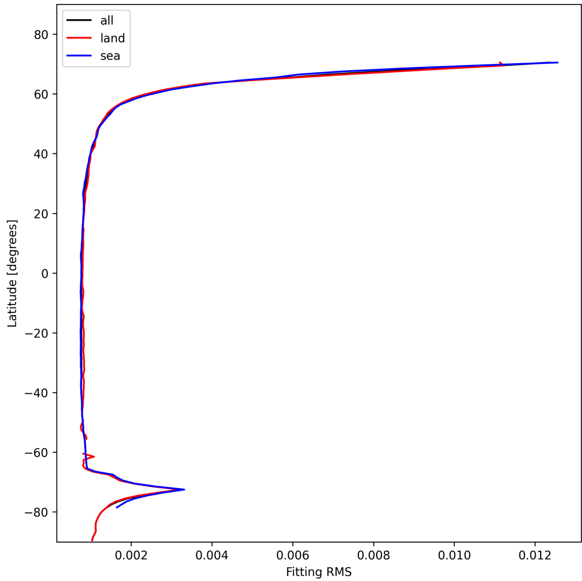
Figure 22: Zonal average of “Fitting RMS” for 2025-01-25 to 2025-01-26.
