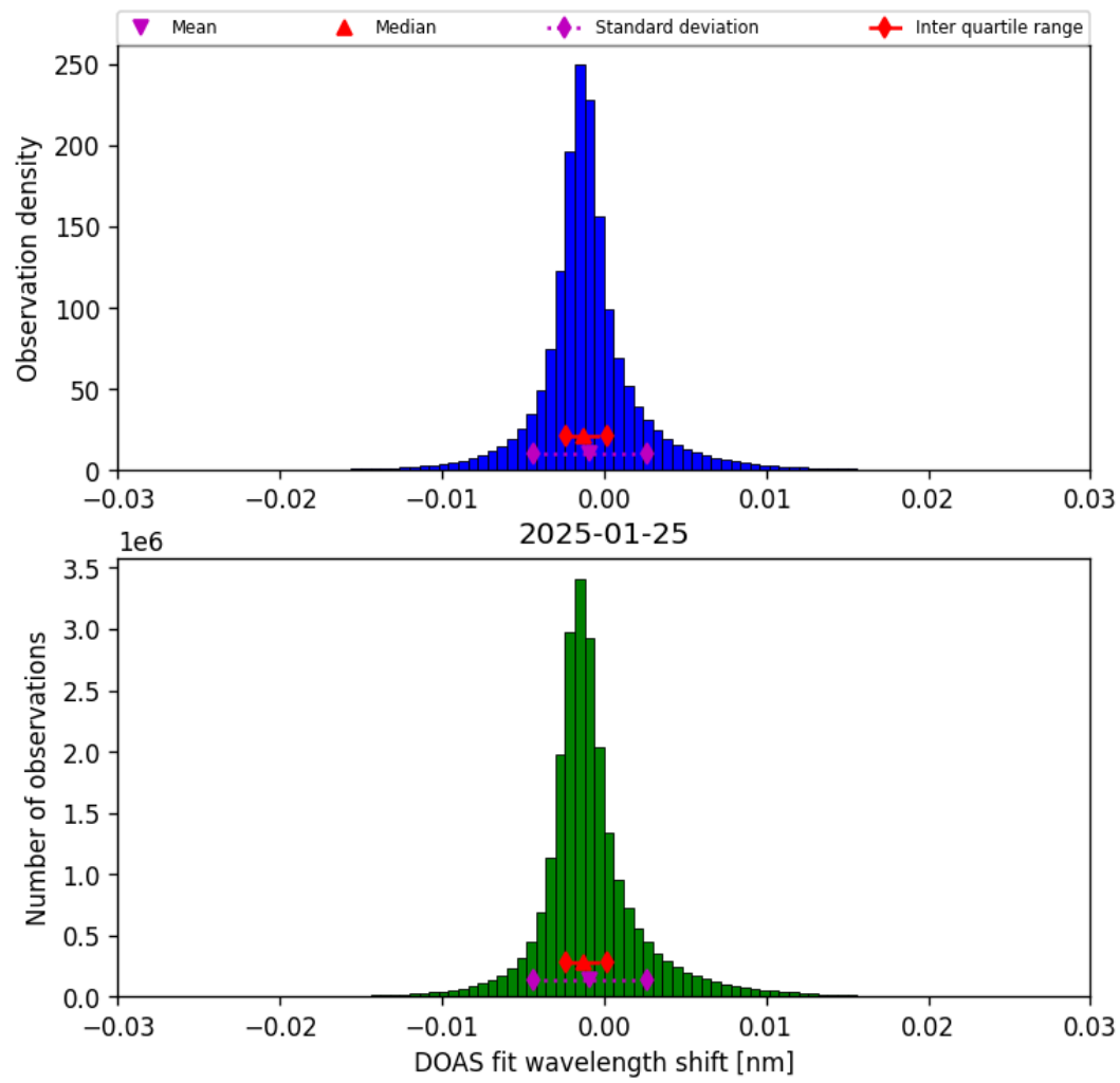
Figure 35: Histogram of “DOAS fit wavelength shift” for 2025-01-25 to 2025-01-26
