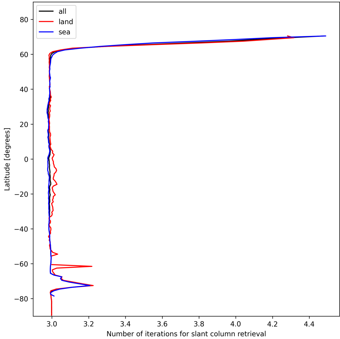
Figure 21: Zonal average of “Number of iterations for slant column retrieval” for 2025-01-25 to 2025-01-26.
