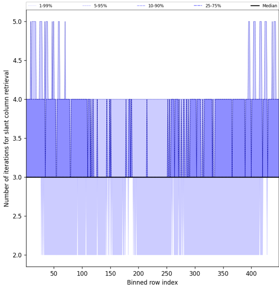
Figure 45: Along track statistics of “Number of iterations for slant column retrieval” for 2025-01-25 to 2025-01-26
