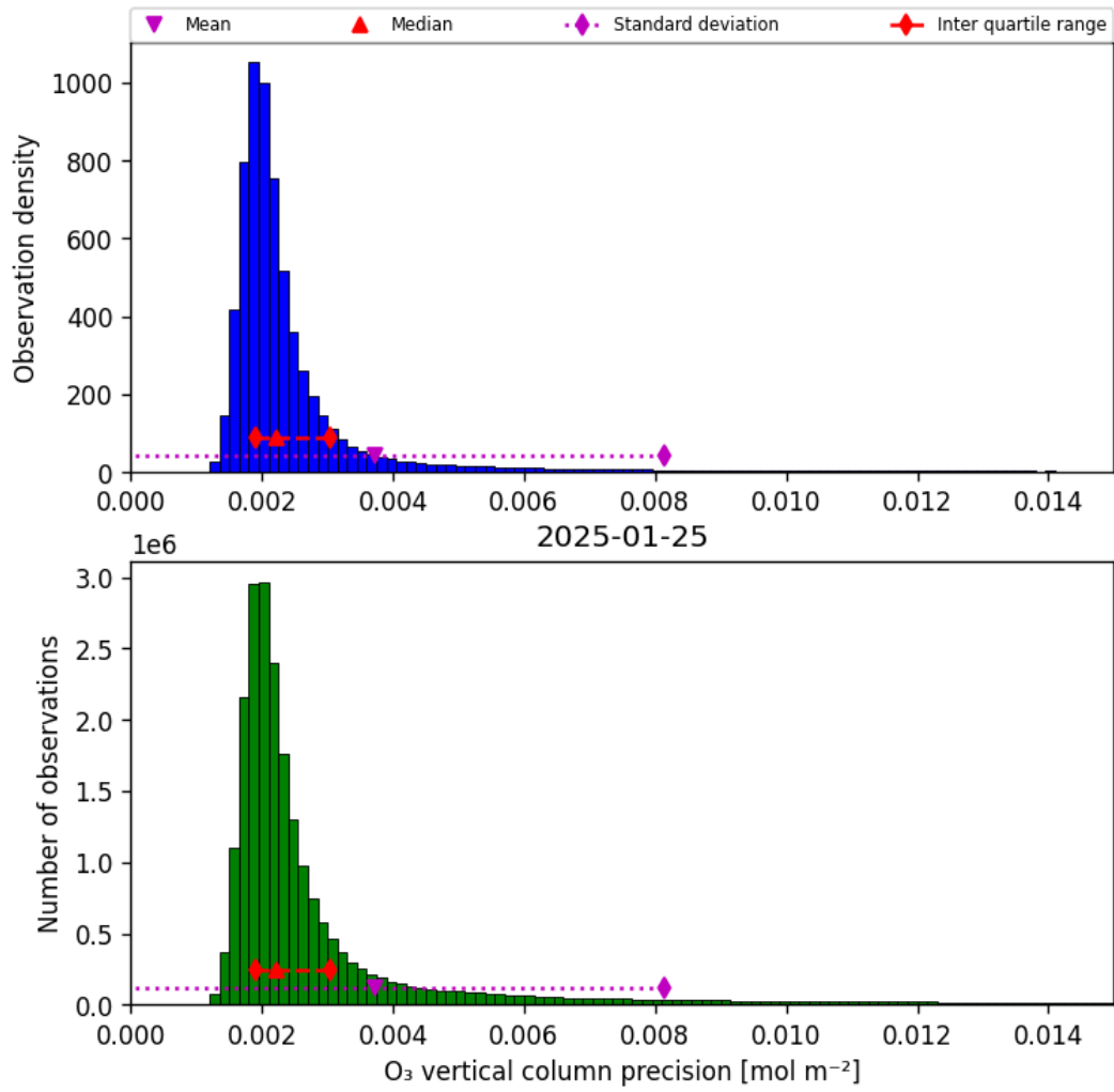
Figure 30: Histogram of “O 3 vertical column precision” for 2025-01-25 to 2025-01-26
