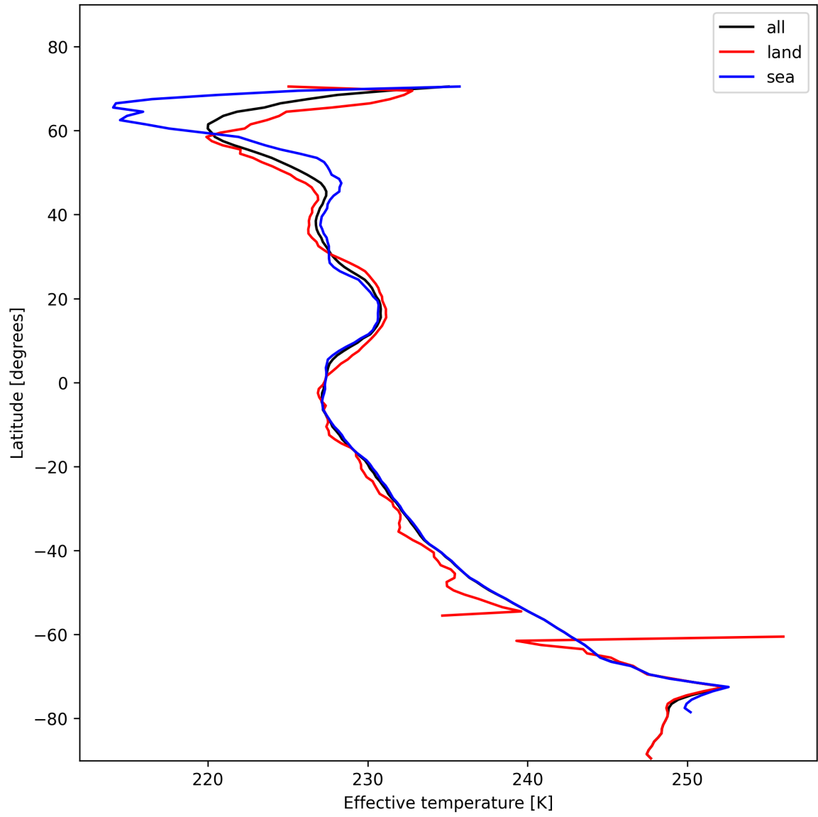
Figure 26: Zonal average of “Effective temperature” for 2025-01-25 to 2025-01-26.
