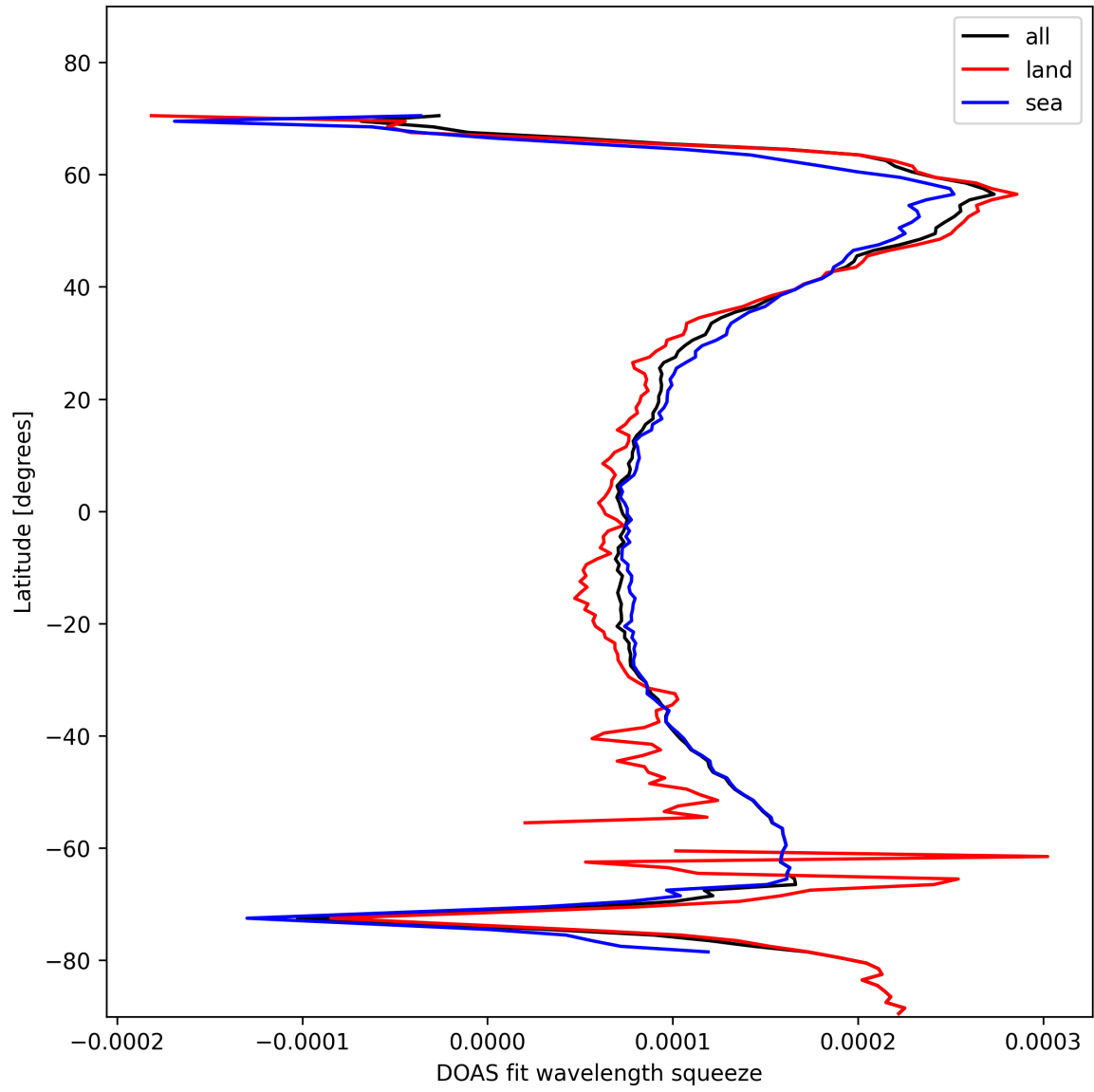
Figure 24: Zonal average of “DOAS fit wavelength squeeze” for 2025-01-25 to 2025-01-26.
