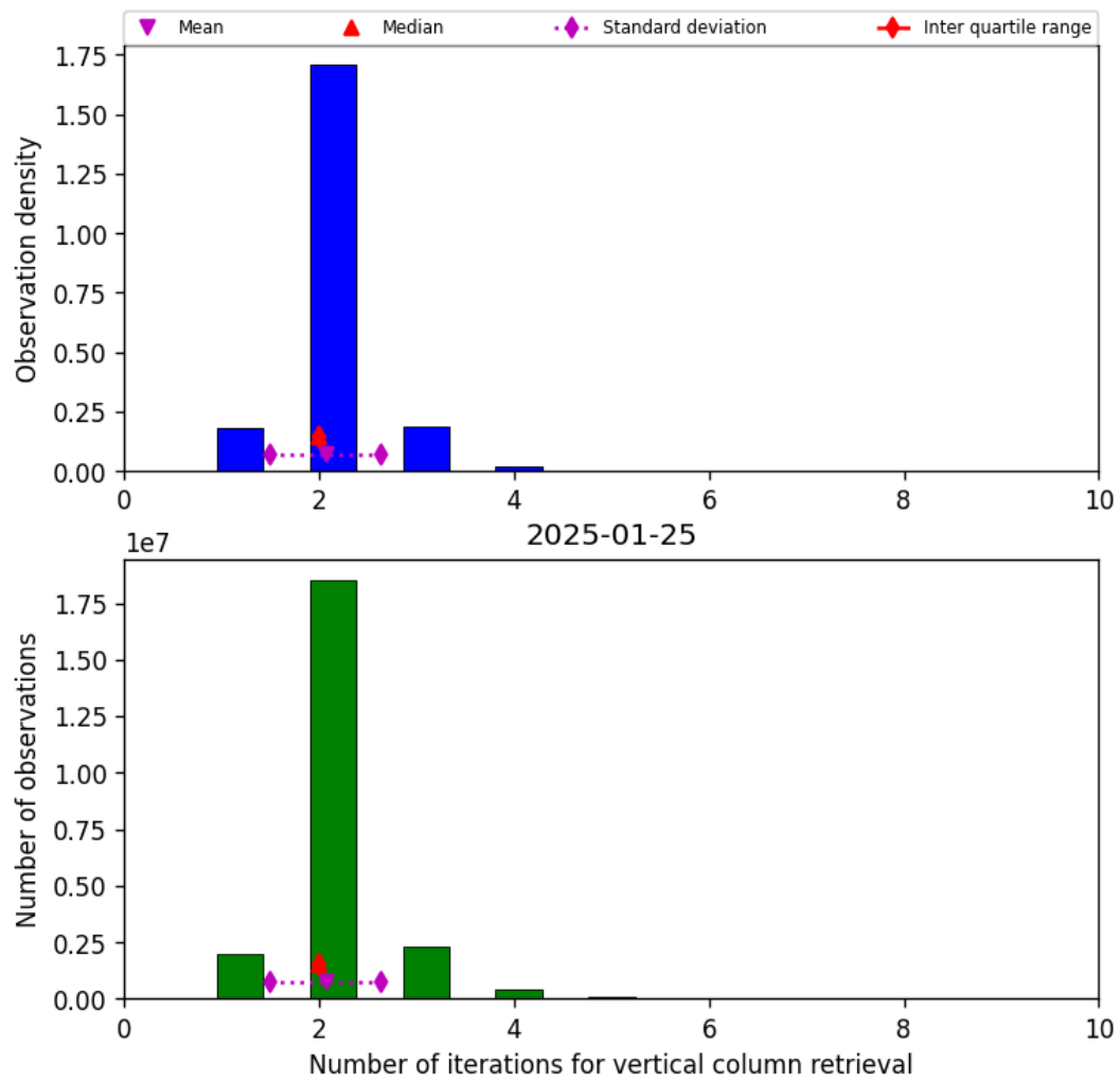
Figure 39: Histogram of “Number of iterations for vertical column retrieval” for 2025-01-25 to 2025-01-26
