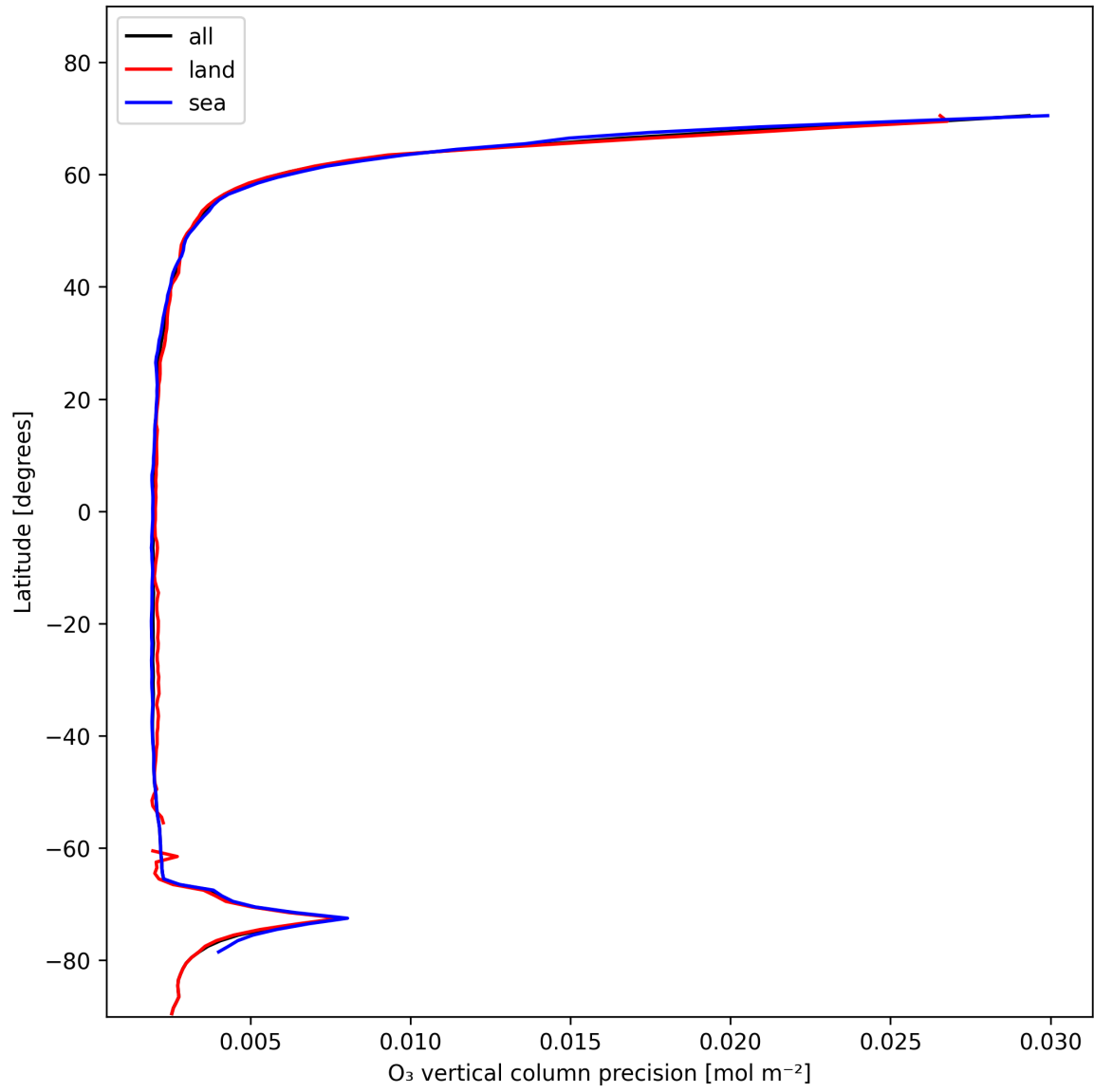
Figure 18: Zonal average of "O 3 vertical column precision" for 2025-01-25 to 2025-01-26.
