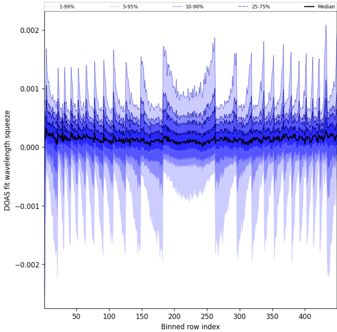
Figure 48: Along track statistics of “DOAS fit wavelength squeeze” for 2025-01-25 to 2025-01-26
