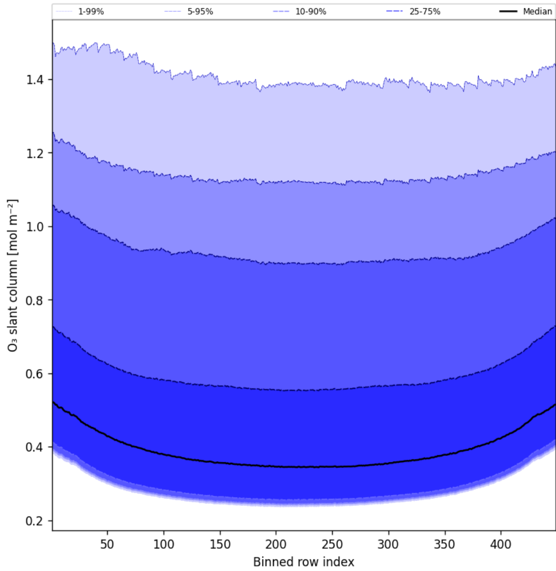
Figure 43: Along track statistics of “O 3 slant column” for 2025-01-25 to 2025-01-26
