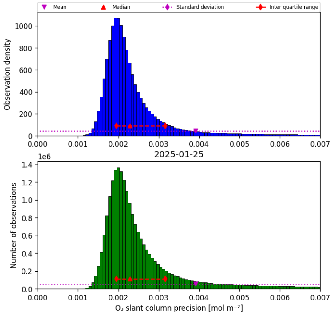
Figure 32: Histogram of “O 3 slant column precision” for 2025-01-25 to 2025-01-26
