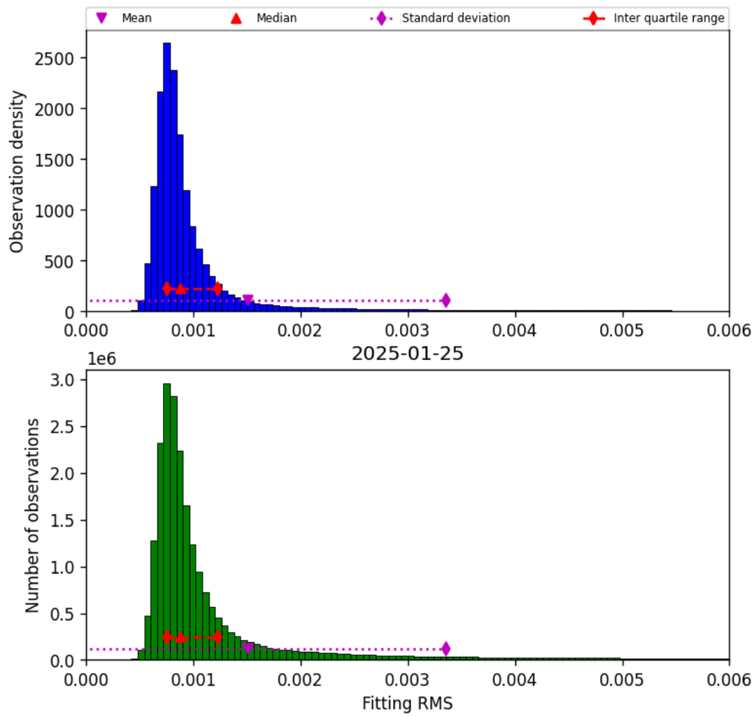
Figure 34: Histogram of “Fitting RMS” for 2025-01-25 to 2025-01-26
