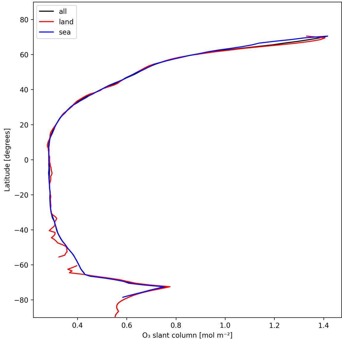
Figure 19: Zonal average of “O 3 slant column” for 2025-01-25 to 2025-01-26.
