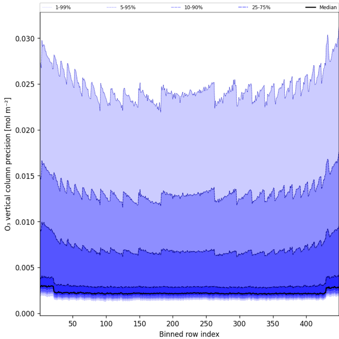
Figure 42: Along track statistics of “O 3 vertical column precision” for 2025-01-25 to 2025-01-26
