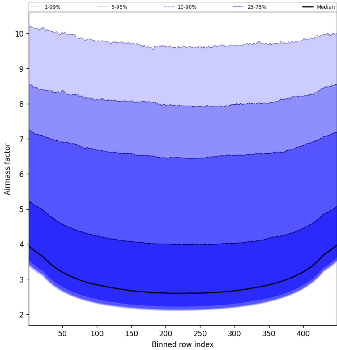
Figure 49: Along track statistics of “Airmass factor” for 2025-01-25 to 2025-01-26
