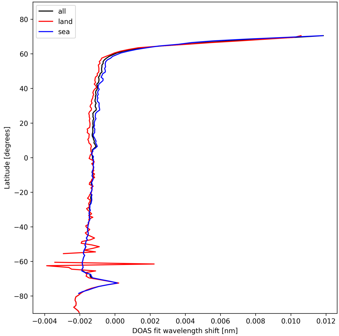
Figure 23: Zonal average of “DOAS fit wavelength shift” for 2025-01-25 to 2025-01-26.
