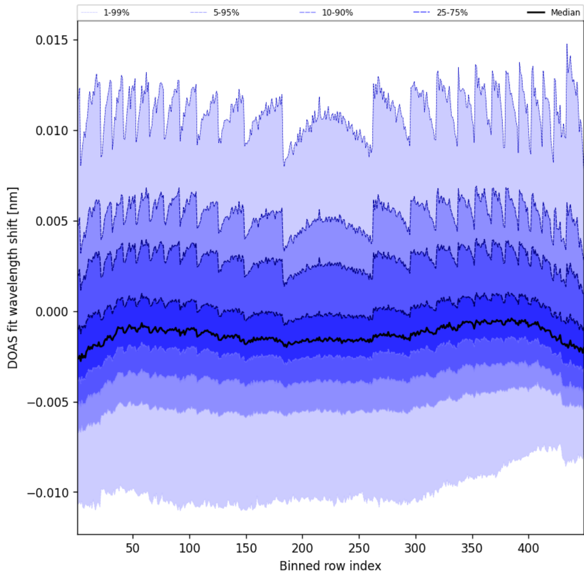
Figure 47: Along track statistics of “DOAS fit wavelength shift” for 2025-01-25 to 2025-01-26
