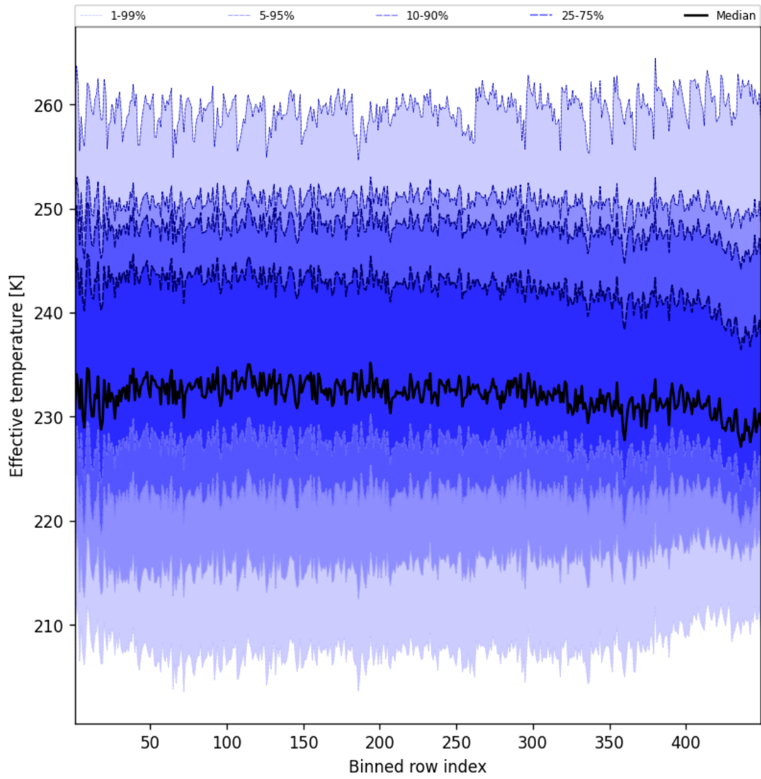
Figure 50: Along track statistics of “Effective temperature” for 2025-01-25 to 2025-01-26
