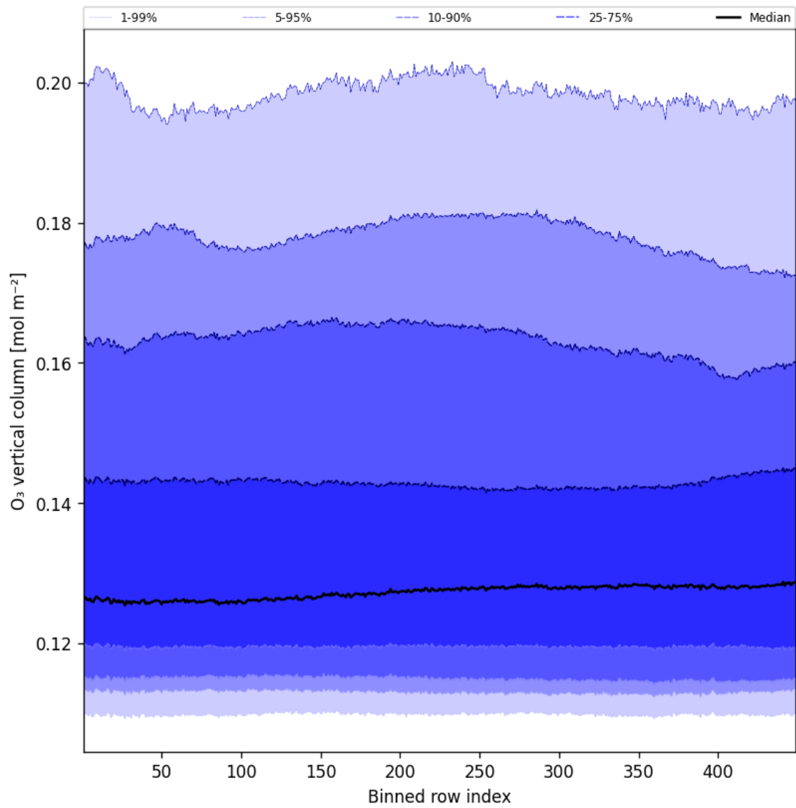
Figure 41: Along track statistics of “O 3 vertical column” for 2025-01-25 to 2025-01-26
