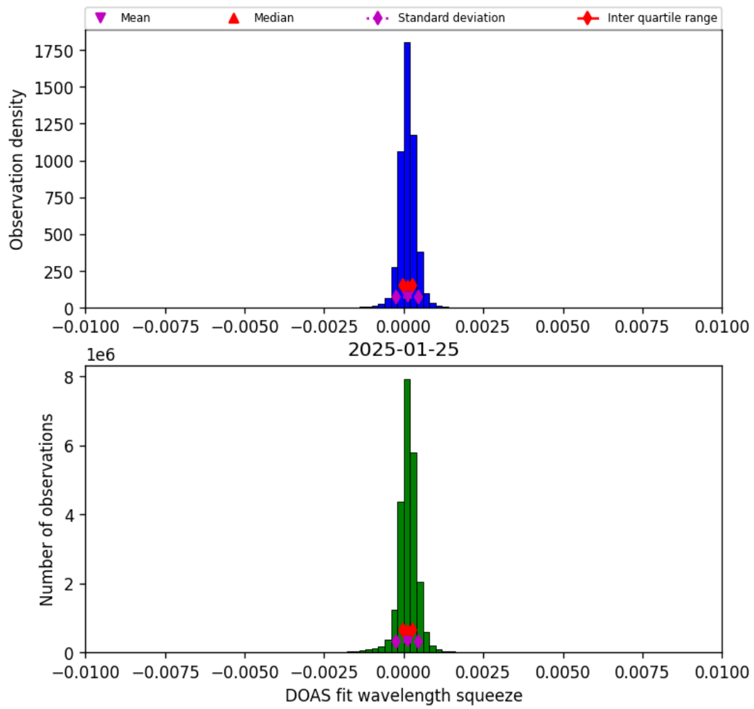
Figure 36: Histogram of “DOAS fit wavelength squeeze” for 2025-01-25 to 2025-01-26
