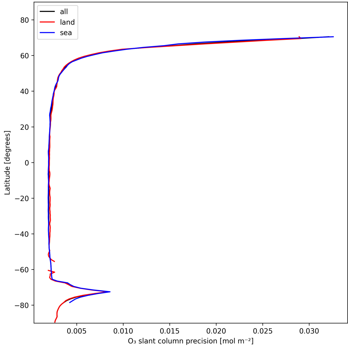
Figure 20: Zonal average of "O 3 slant column precision" for 2025-01-25 to 2025-01-26.
