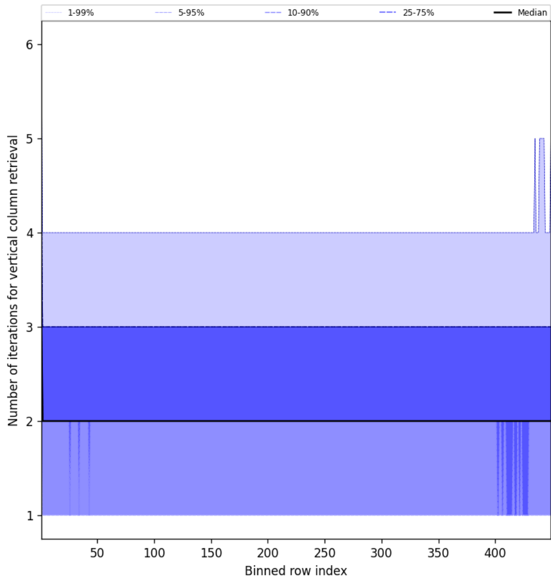
Figure 51: Along track statistics of “Number of iterations for vertical column retrieval” for 2025-01-25 to 2025-01-26
