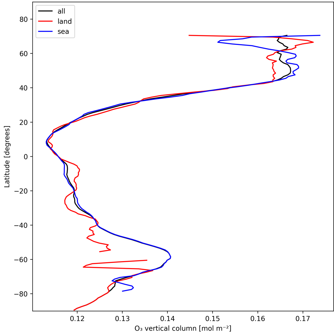
Figure 17: Zonal average of “O 3 vertical column” for 2025-01-25 to 2025-01-26.
