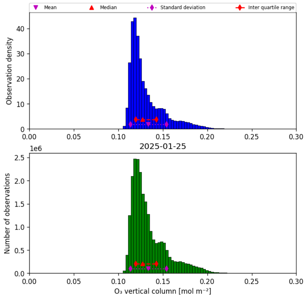
Figure 29: Histogram of “O 3 vertical column” for 2025-01-25 to 2025-01-26
