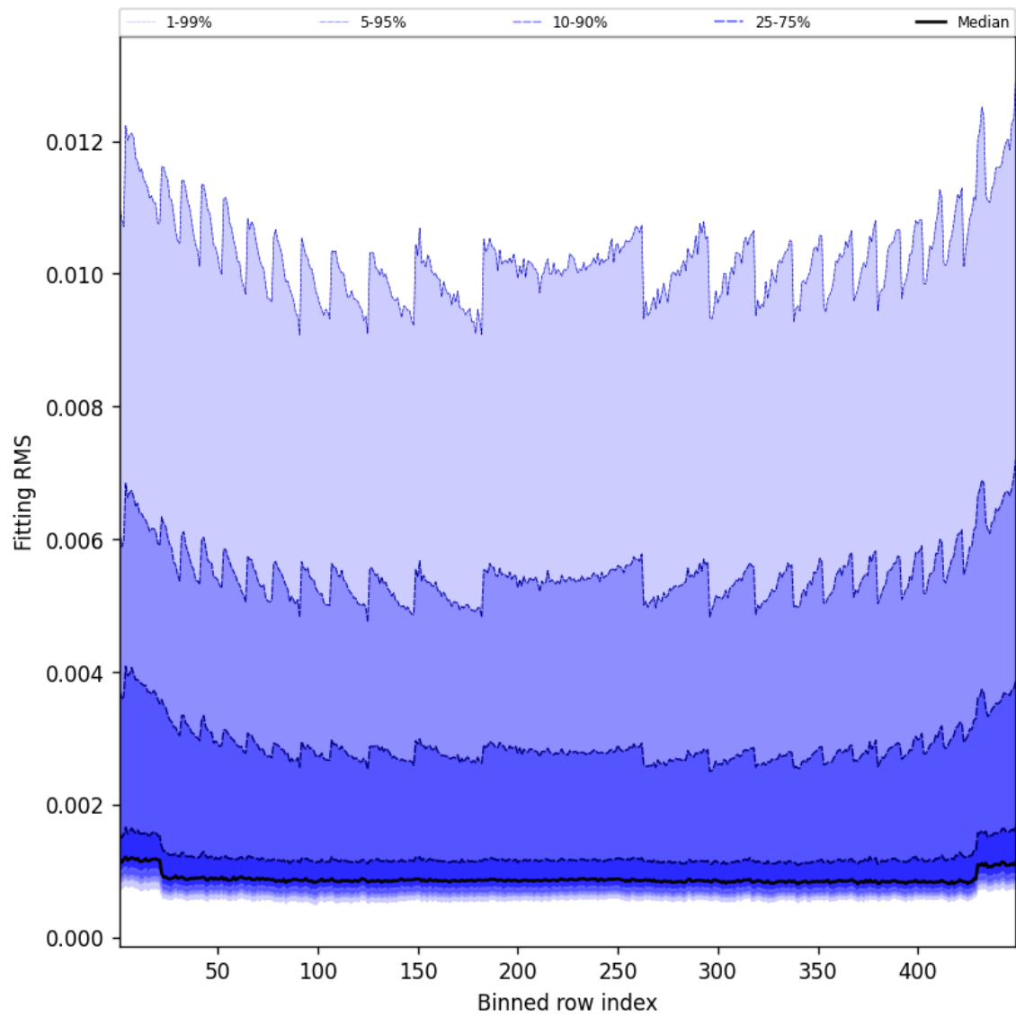
Figure 46: Along track statistics of “Fitting RMS” for 2025-01-25 to 2025-01-26
