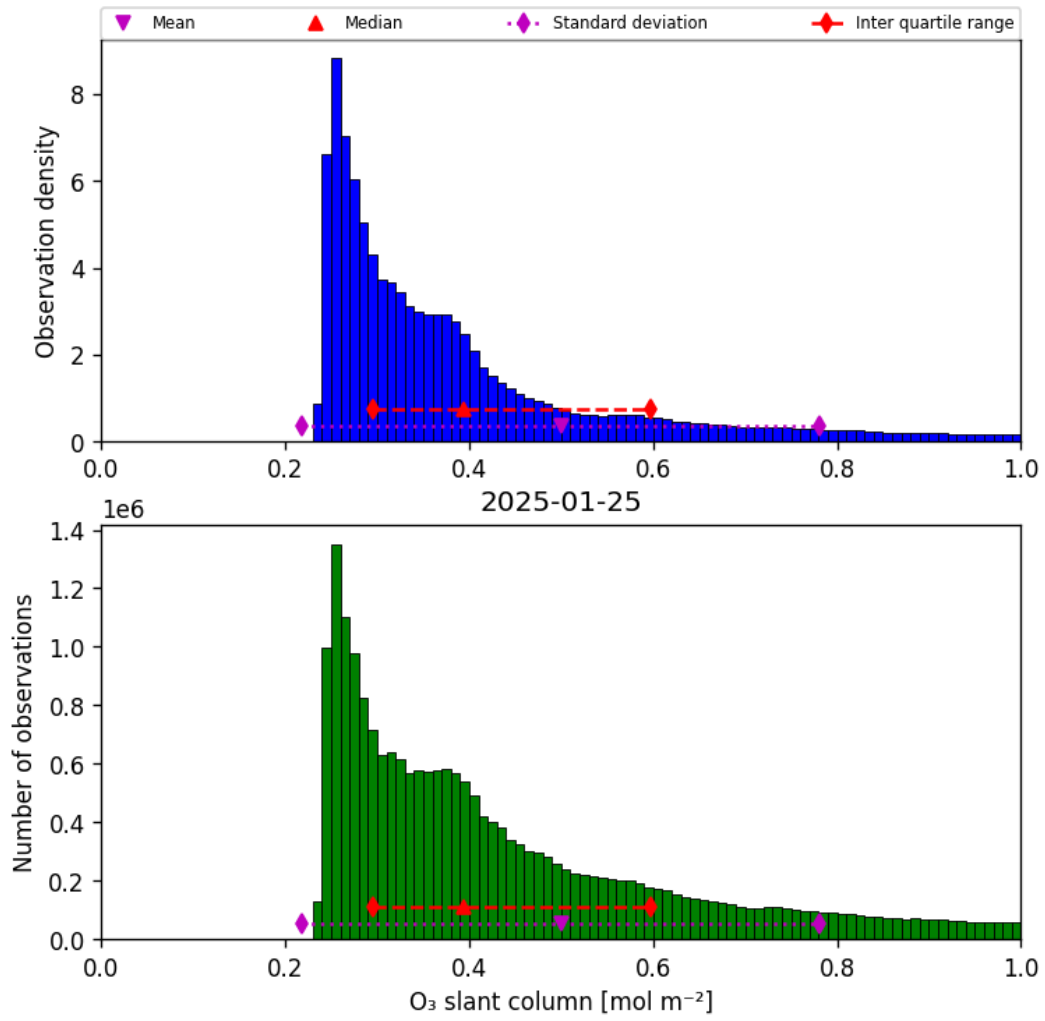
Figure 31: Histogram of “O 3 slant column” for 2025-01-25 to 2025-01-26
