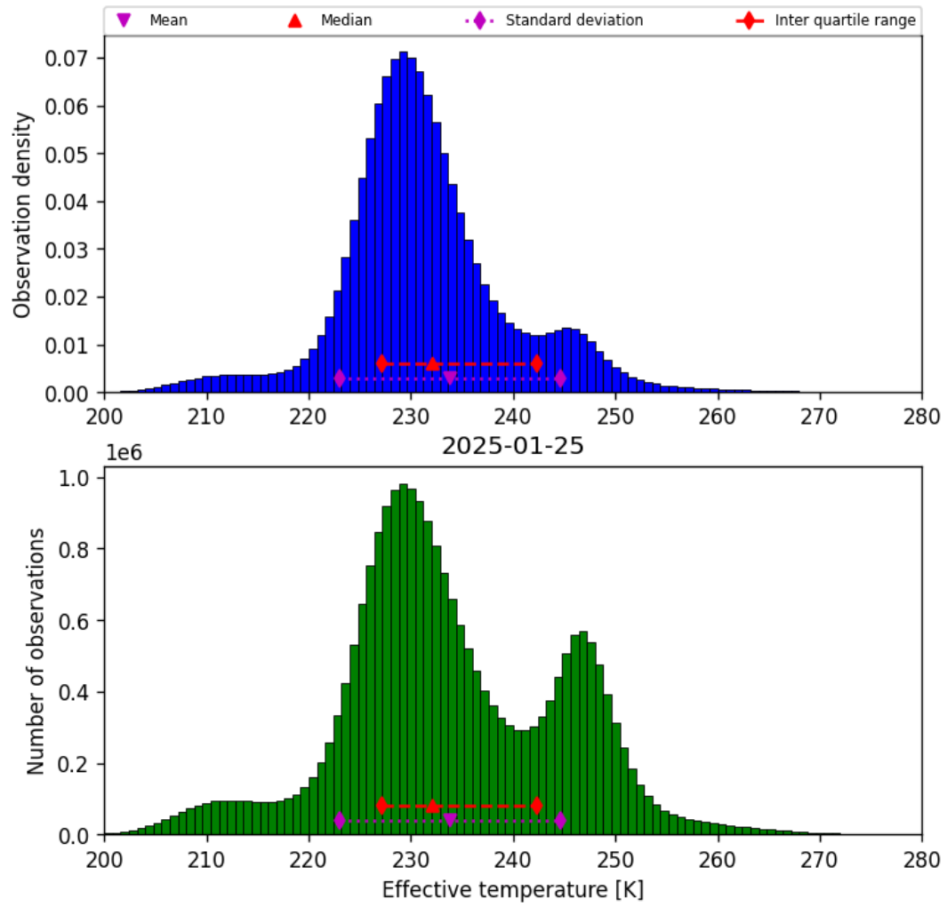
Figure 38: Histogram of “Effective temperature” for 2025-01-25 to 2025-01-26
