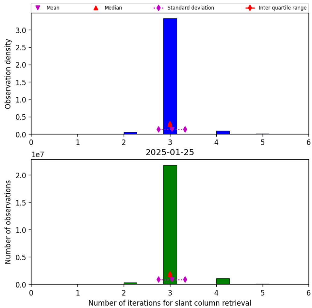
Figure 33: Histogram of “Number of iterations for slant column retrieval” for 2025-01-25 to 2025-01-26
