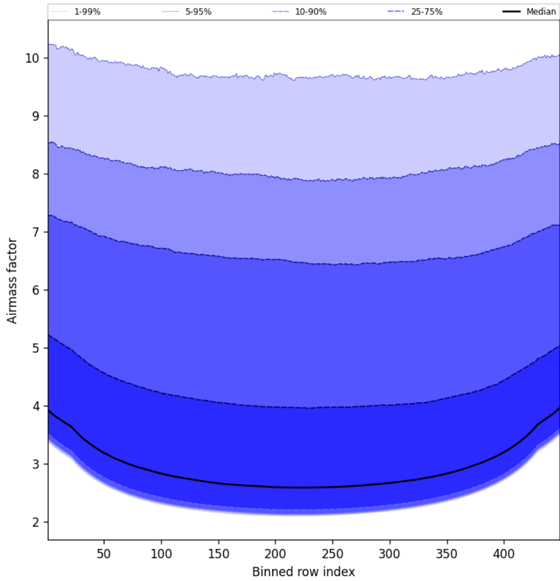
Figure 49: Along track statistics of “Airmass factor” for 2025-01-26 to 2025-01-26
