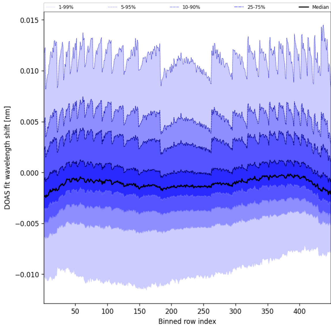
Figure 47: Along track statistics of "DOAS fit wavelength shift" for 2025-01-26 to 2025-01-26
