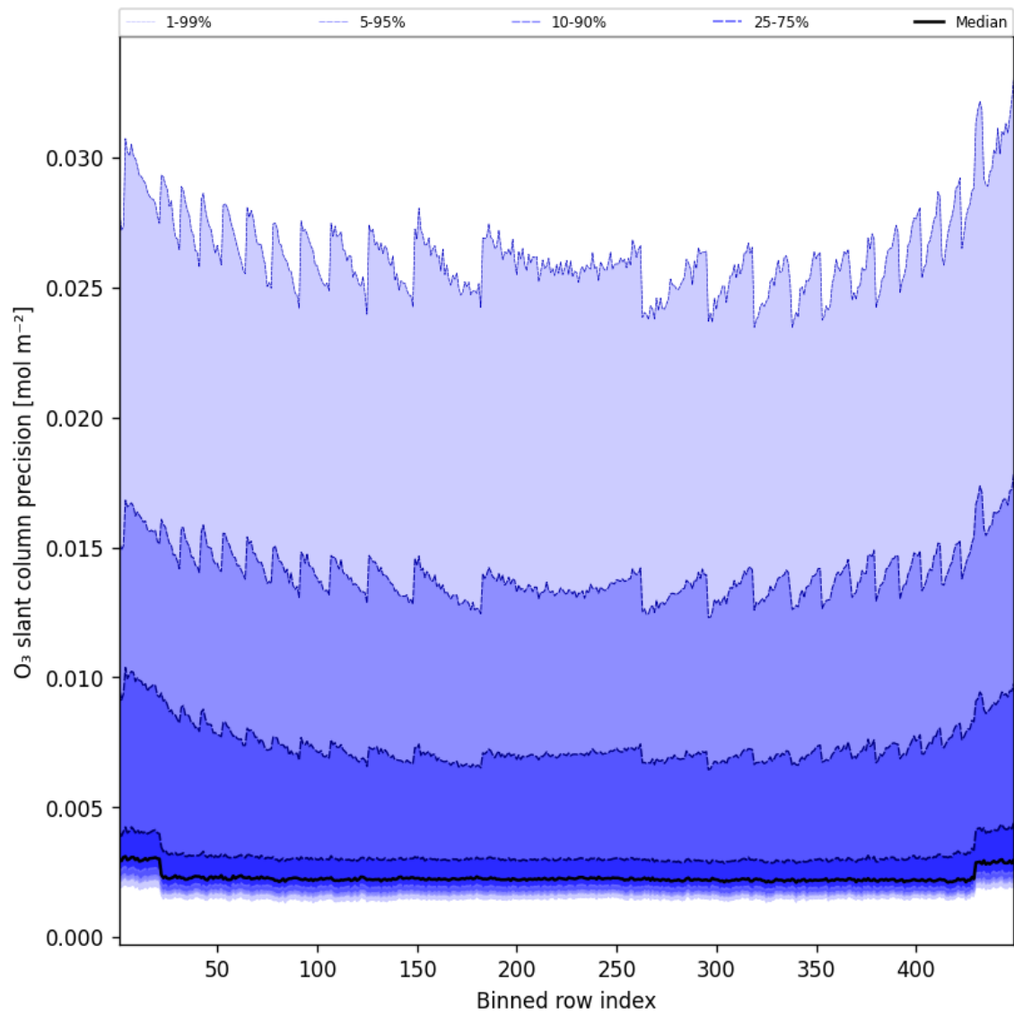
Figure 44: Along track statistics of “O 3 slant column precision” for 2025-01-26 to 2025-01-26
