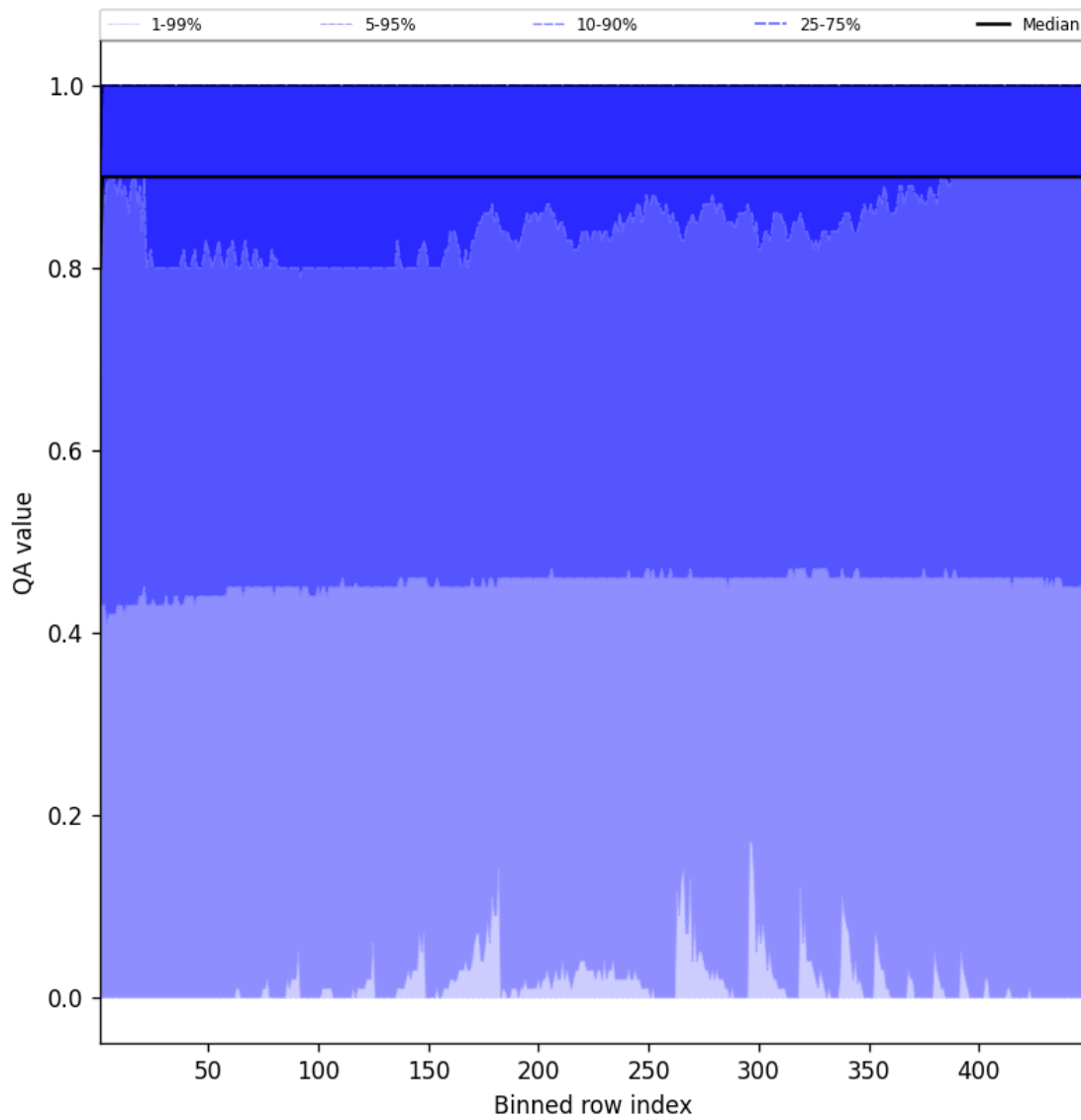
Figure 40: Along track statistics of “QA value” for 2025-01-26 to 2025-01-26
