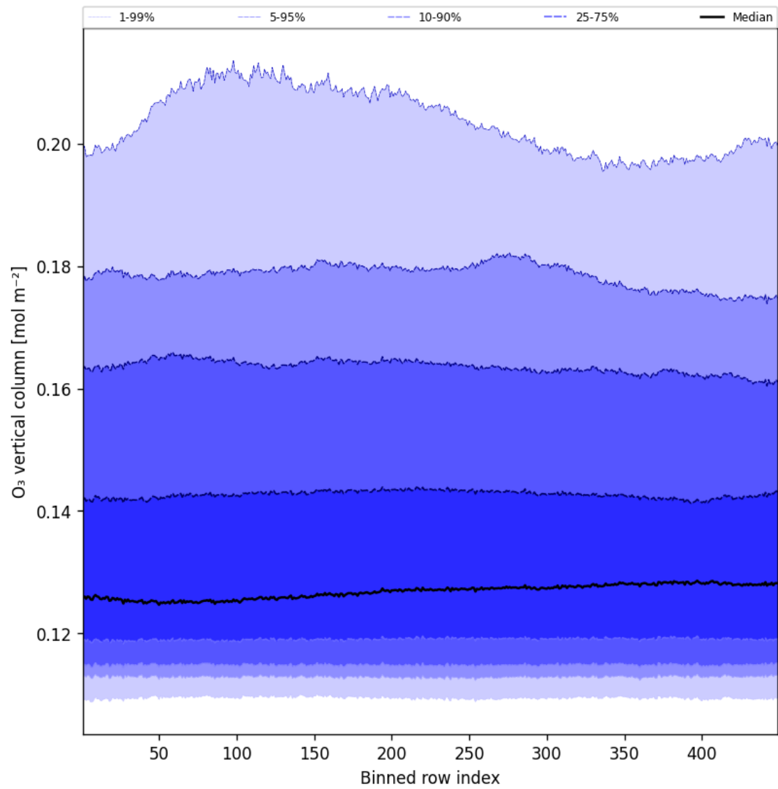
Figure 41: Along track statistics of “O 3 vertical column” for 2025-01-26 to 2025-01-26
