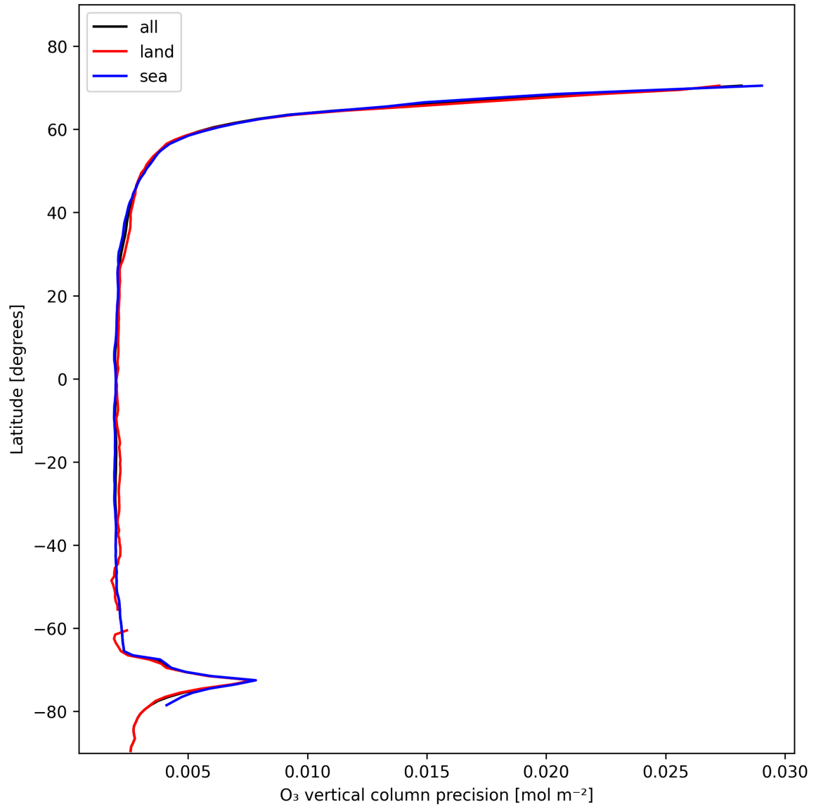
Figure 18: Zonal average of “O 3 vertical column precision” for 2025-01-26 to 2025-01-26.
