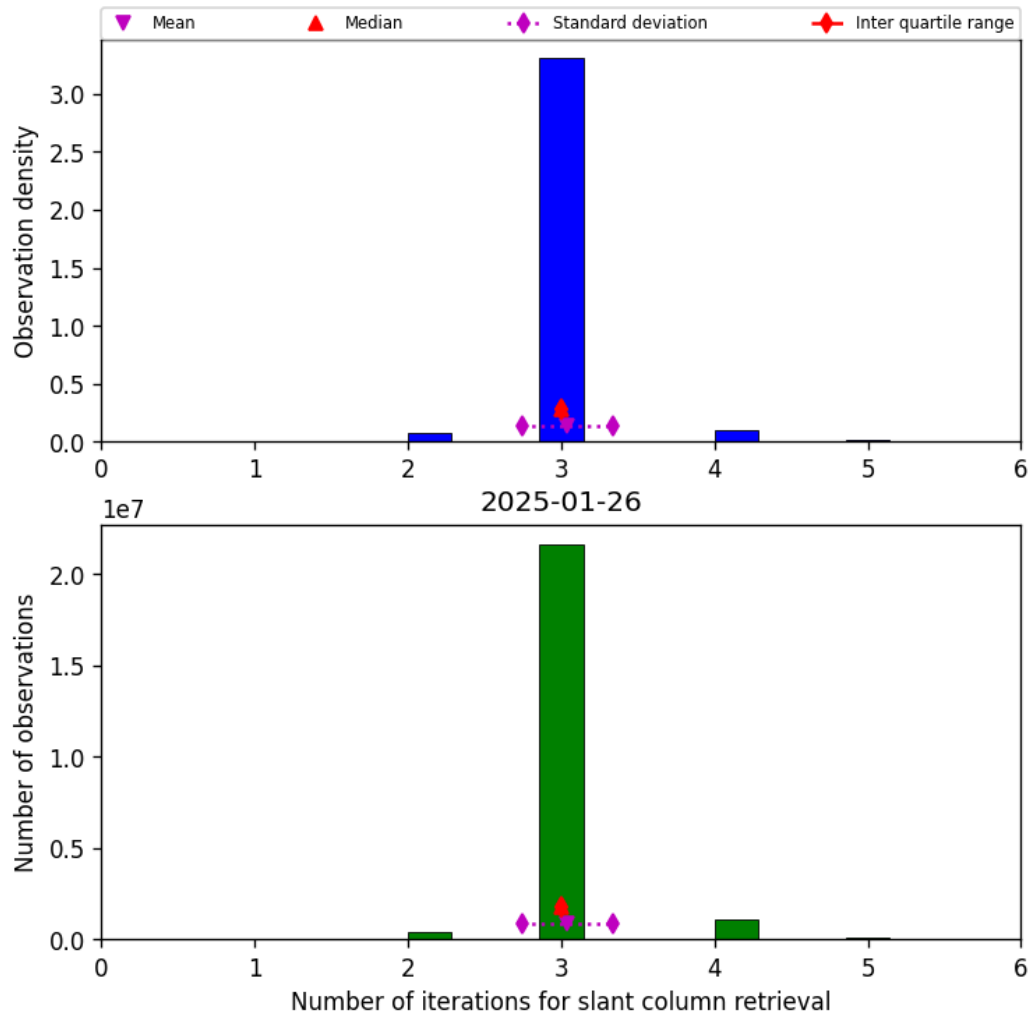
Figure 33: Histogram of “Number of iterations for slant column retrieval” for 2025-01-26 to 2025-01-26
