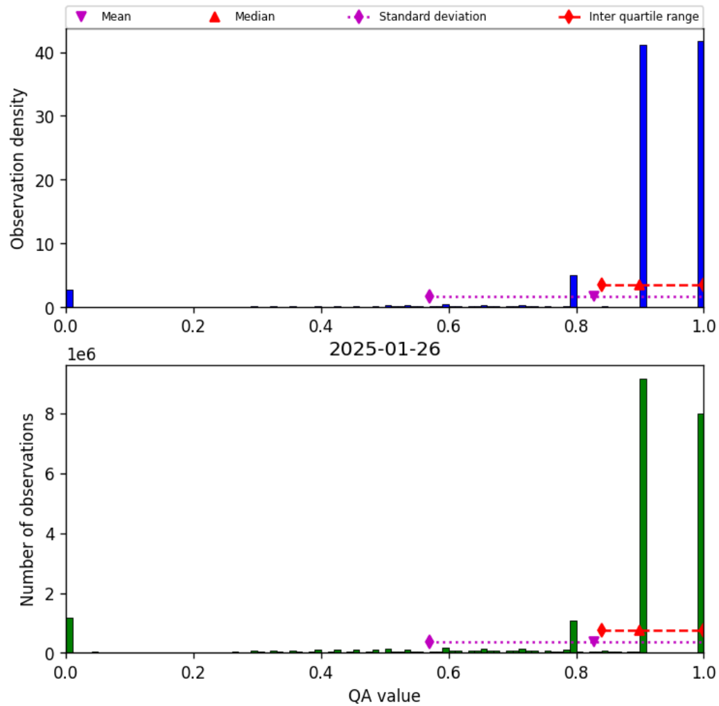
Figure 28: Histogram of “QA value” for 2025-01-26 to 2025-01-26
