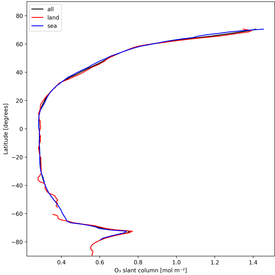
Figure 19: Zonal average of “O 3 slant column” for 2025-01-26 to 2025-01-26.
