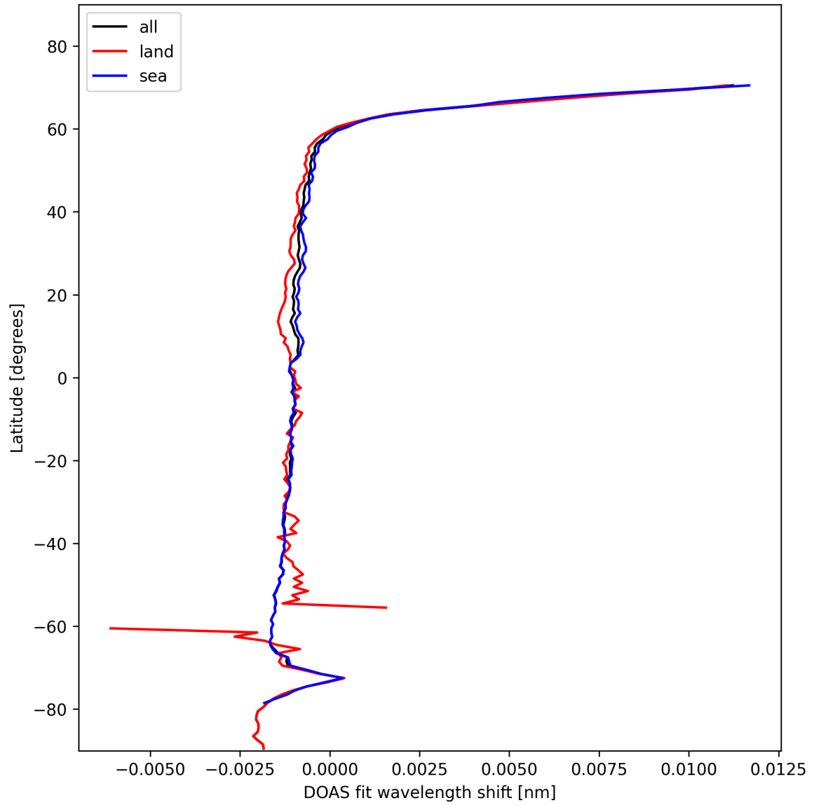
Figure 23: Zonal average of “DOAS fit wavelength shift” for 2025-01-26 to 2025-01-26.
