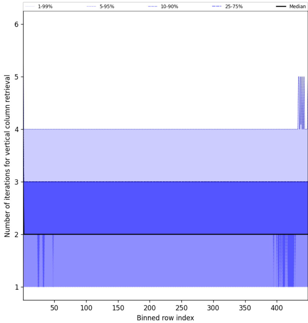
Figure 51: Along track statistics of “Number of iterations for vertical column retrieval” for 2025-01-26 to 2025-01-26
