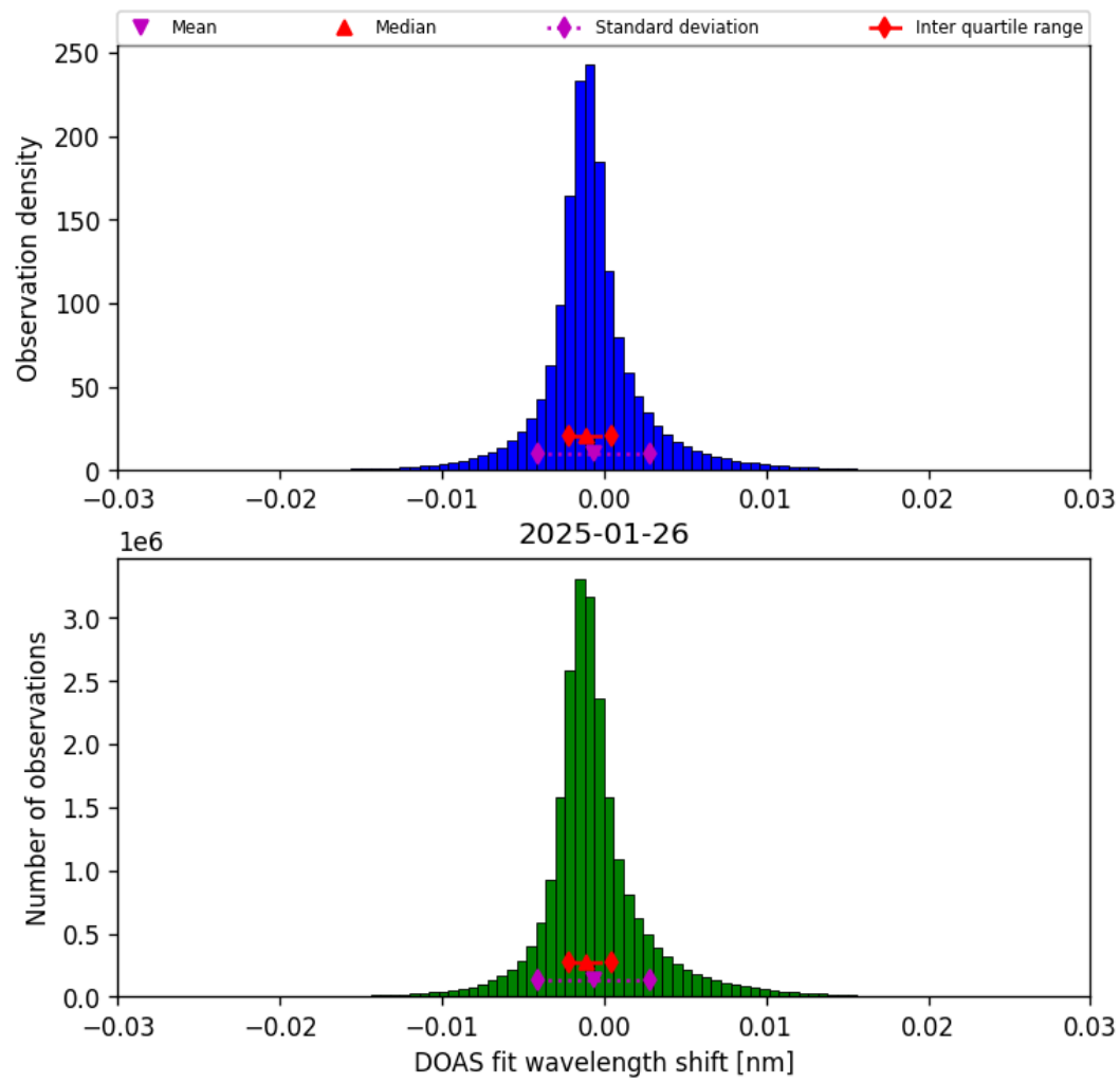
Figure 35: Histogram of “DOAS fit wavelength shift” for 2025-01-26 to 2025-01-26
