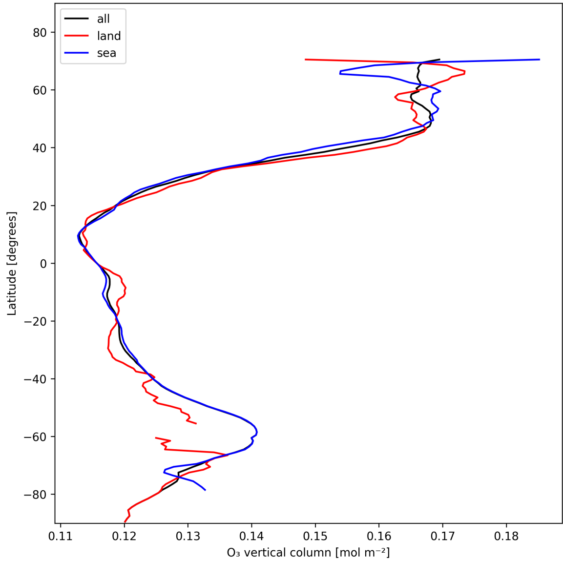
Figure 17: Zonal average of “O 3 vertical column” for 2025-01-26 to 2025-01-26.
