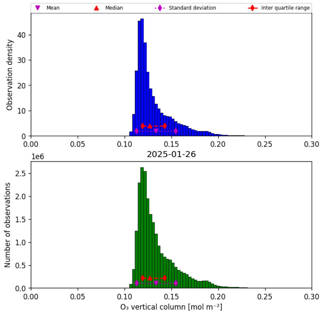
Figure 29: Histogram of “O 3 vertical column” for 2025-01-26 to 2025-01-26
