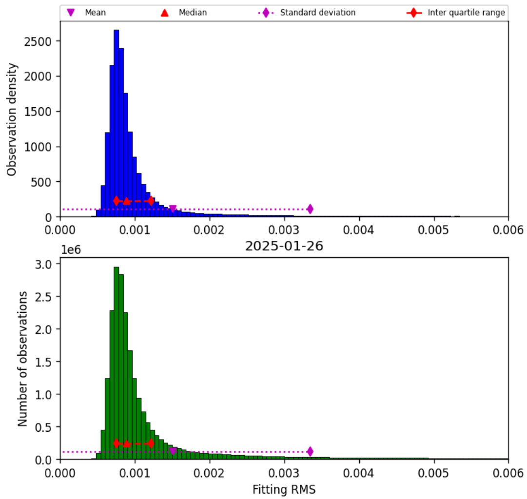
Figure 34: Histogram of “Fitting RMS” for 2025-01-26 to 2025-01-26
