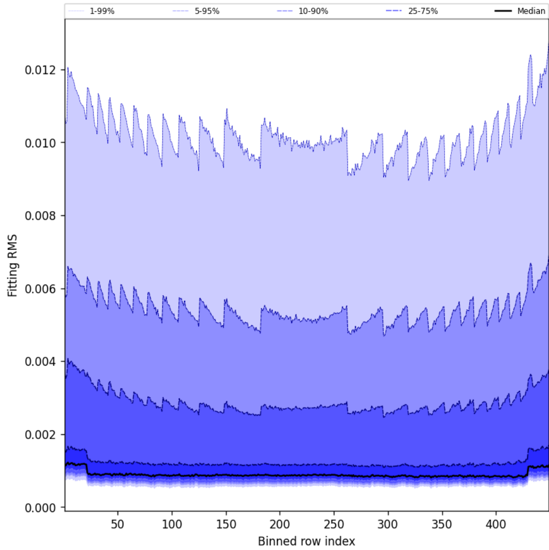
Figure 46: Along track statistics of “Fitting RMS” for 2025-01-26 to 2025-01-26
