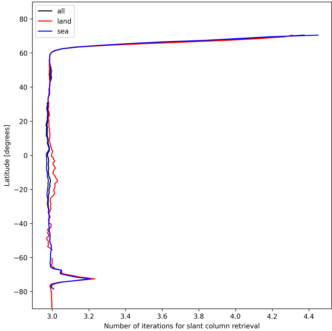
Figure 21: Zonal average of “Number of iterations for slant column retrieval” for 2025-01-26 to 2025-01-26.
