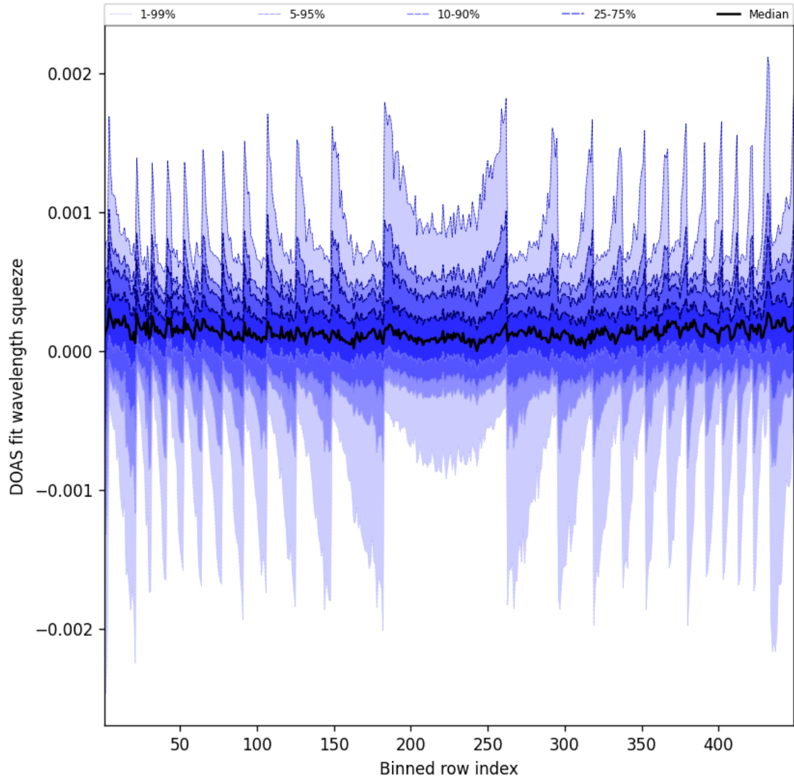
Figure 48: Along track statistics of “DOAS fit wavelength squeeze” for 2025-01-26 to 2025-01-26
