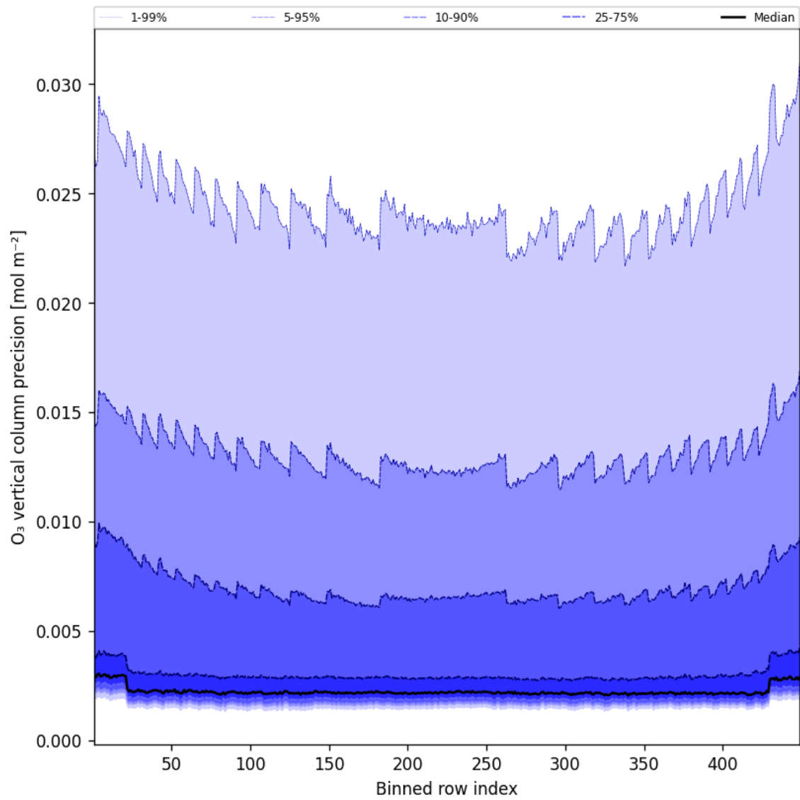
Figure 42: Along track statistics of “O 3 vertical column precision” for 2025-01-26 to 2025-01-26
