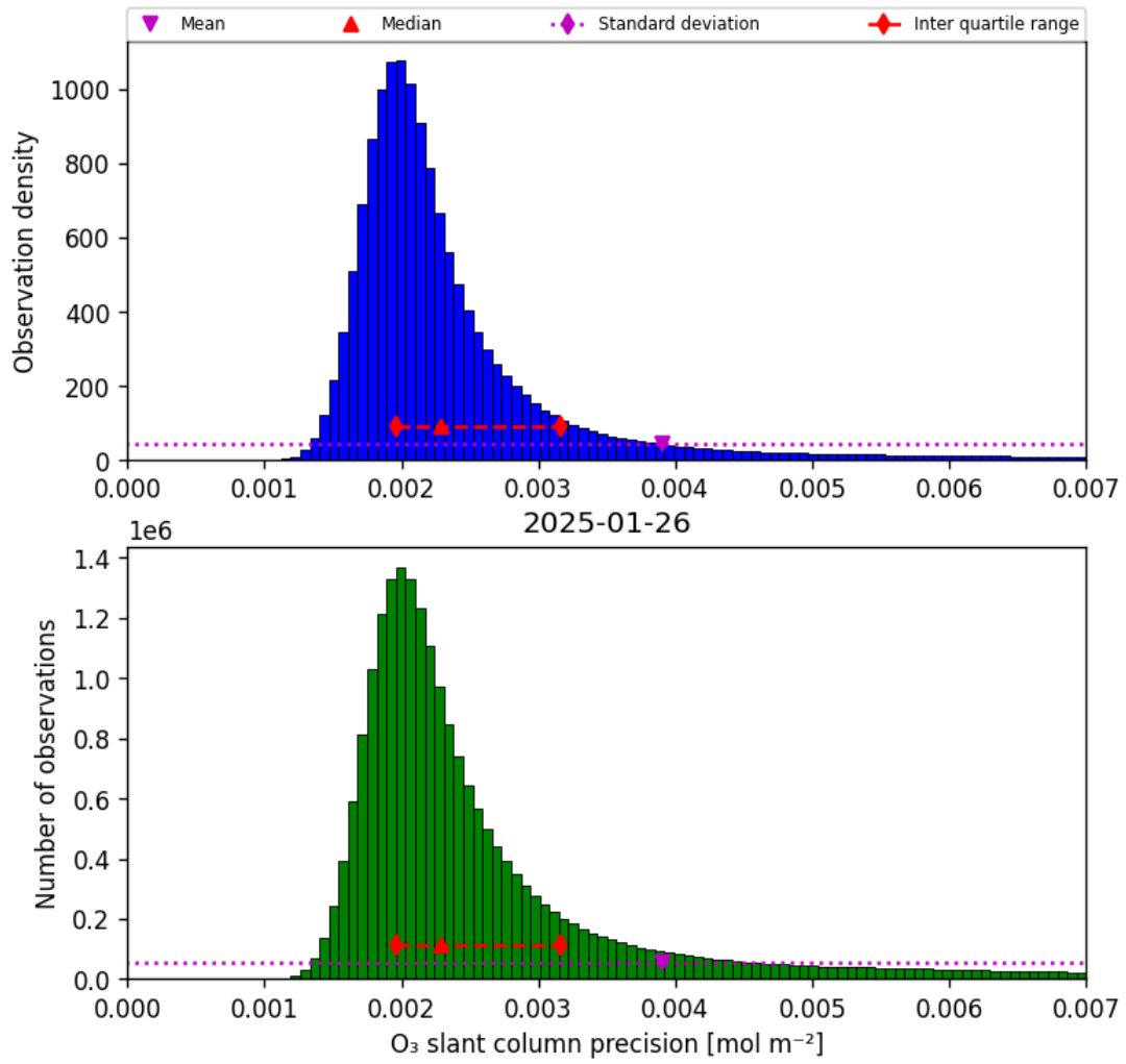
Figure 32: Histogram of “O 3 slant column precision” for 2025-01-26 to 2025-01-26
