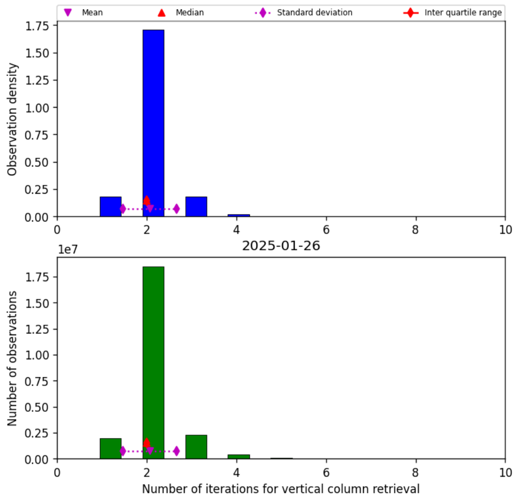
Figure 39: Histogram of “Number of iterations for vertical column retrieval” for 2025-01-26 to 2025-01-26
