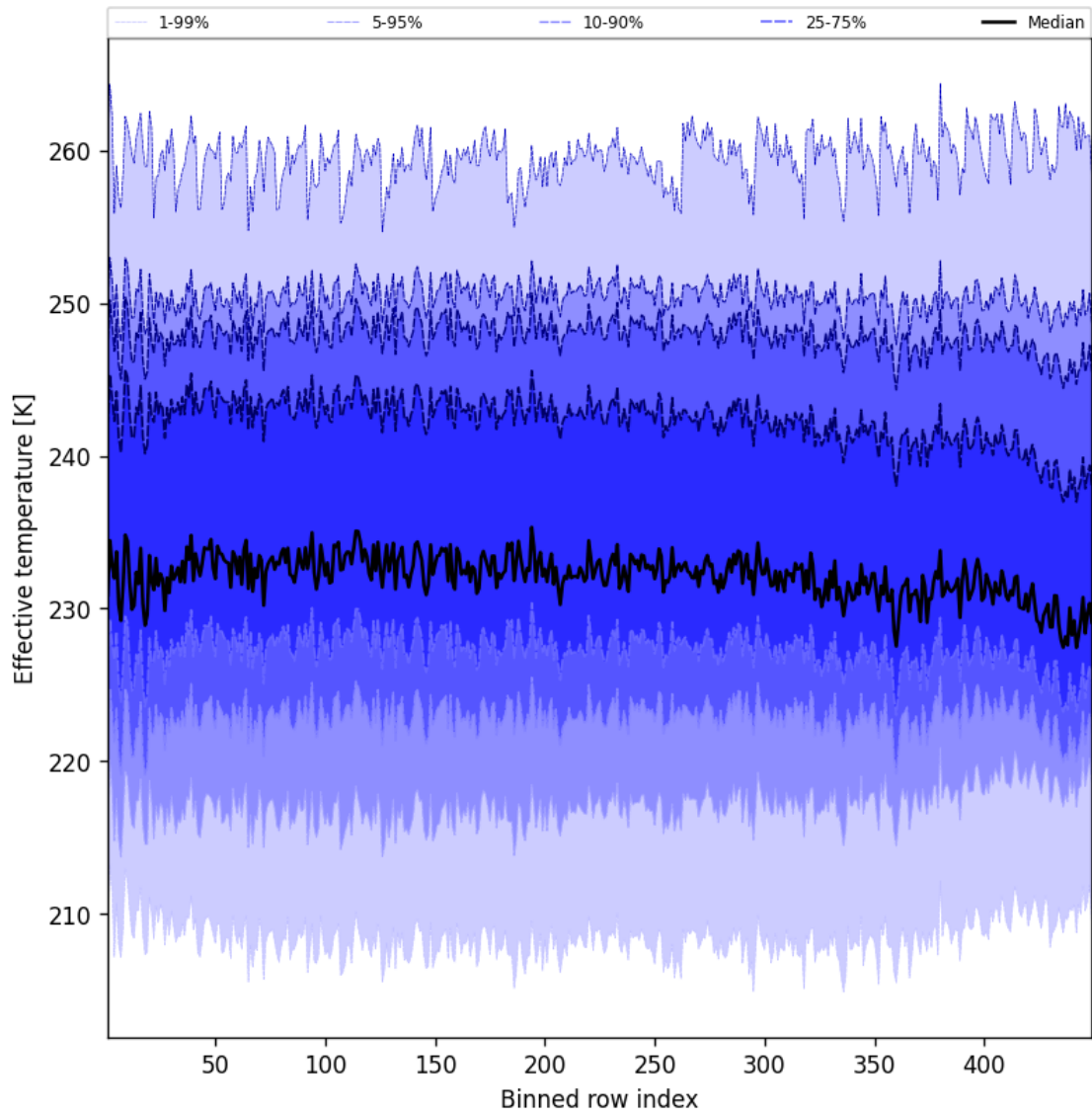
Figure 50: Along track statistics of “Effective temperature” for 2025-01-26 to 2025-01-26
