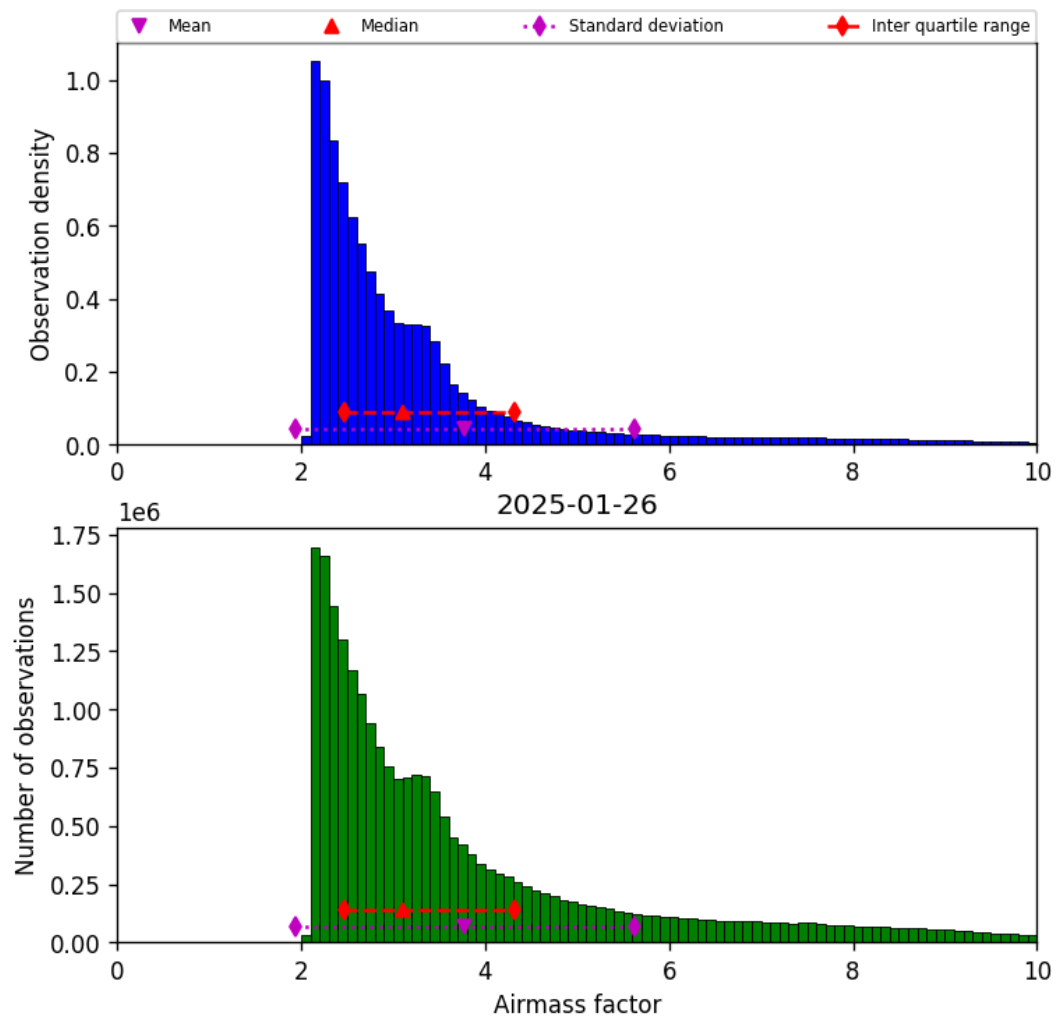
Figure 37: Histogram of “Airmass factor” for 2025-01-26 to 2025-01-26
