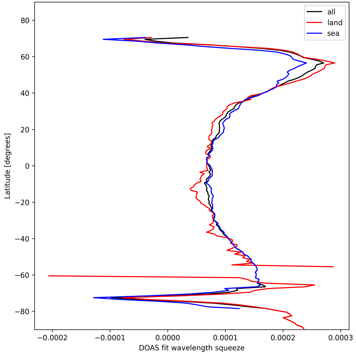
Figure 24: Zonal average of “DOAS fit wavelength squeeze” for 2025-01-26 to 2025-01-26.
