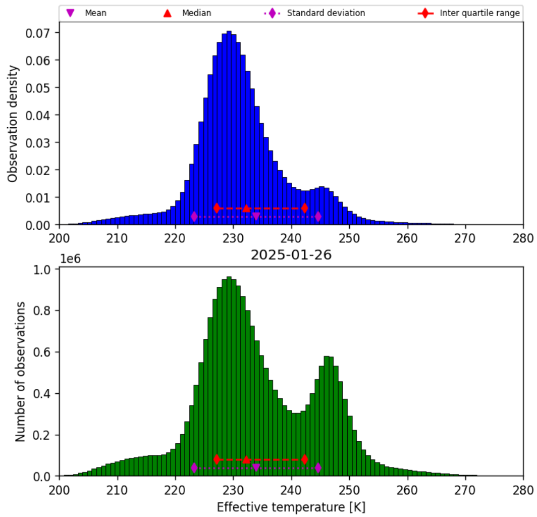
Figure 38: Histogram of “Effective temperature” for 2025-01-26 to 2025-01-26
