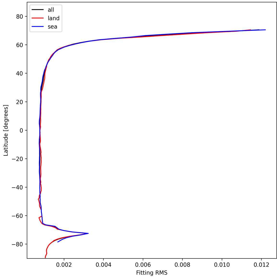
Figure 22: Zonal average of “Fitting RMS” for 2025-01-26 to 2025-01-26.
