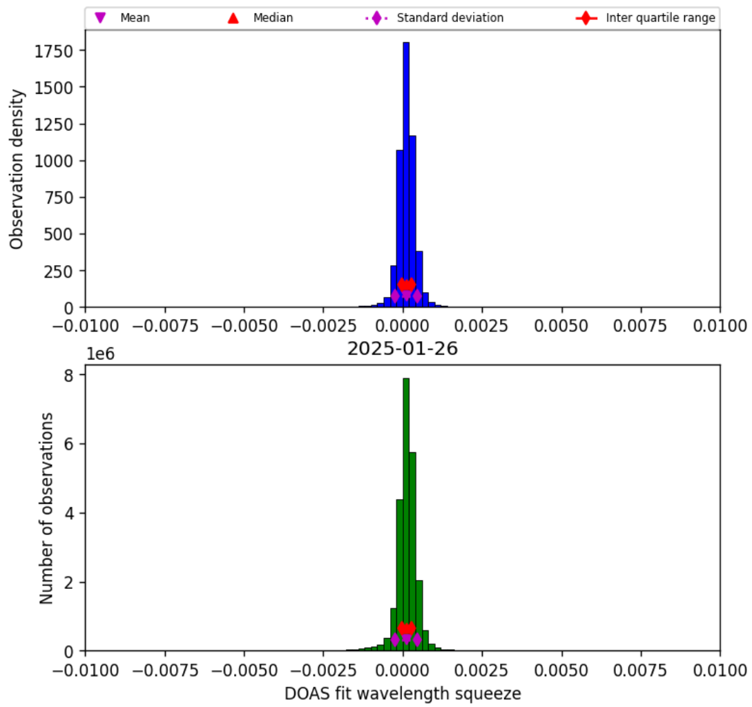
Figure 36: Histogram of “DOAS fit wavelength squeeze” for 2025-01-26 to 2025-01-26
