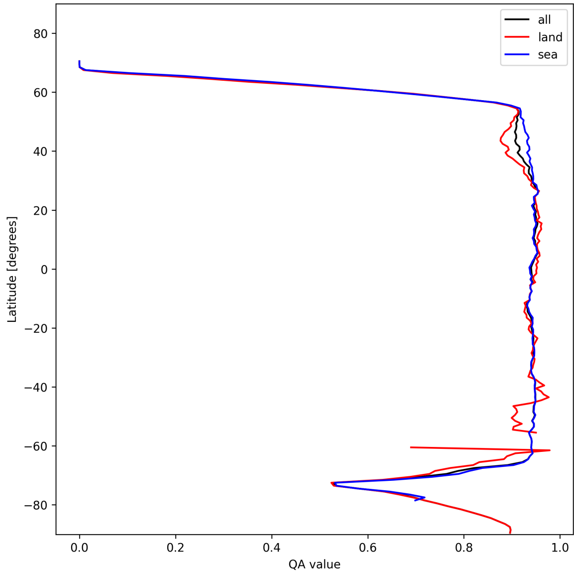
Figure 16: Zonal average of “QA value” for 2025-01-26 to 2025-01-26.
