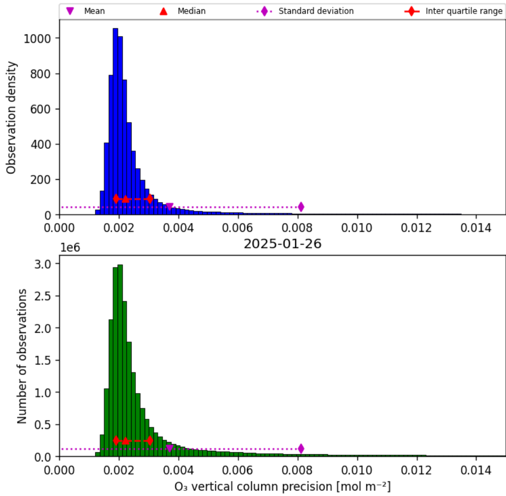
Figure 30: Histogram of “O 3 vertical column precision” for 2025-01-26 to 2025-01-26
