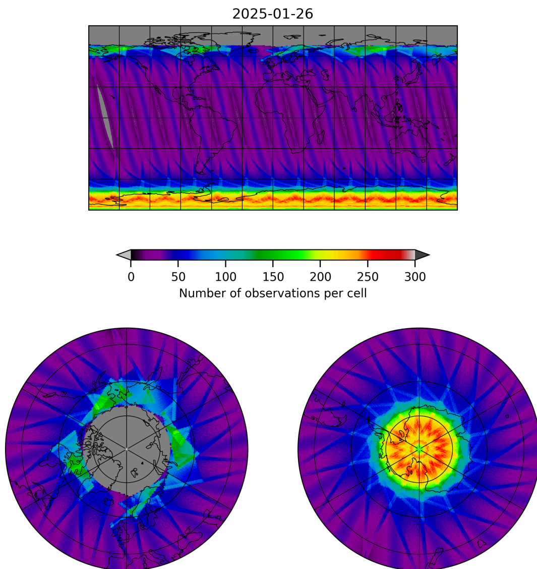
Figure 15: Map of the number of observations for 2025-01-26 to 2025-01-26
