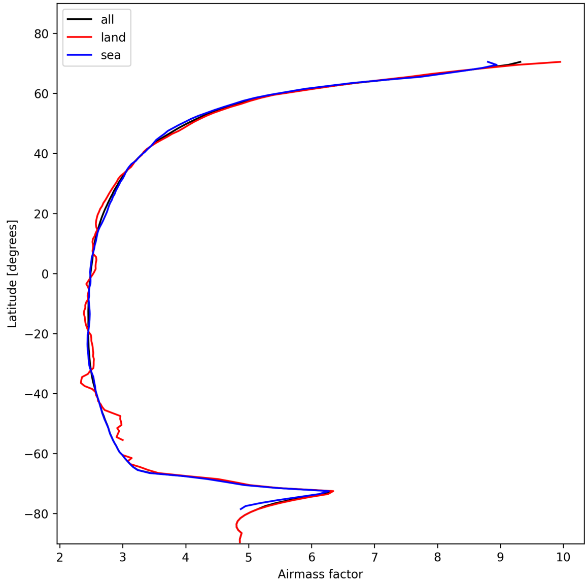
Figure 25: Zonal average of “Airmass factor” for 2025-01-26 to 2025-01-26.
