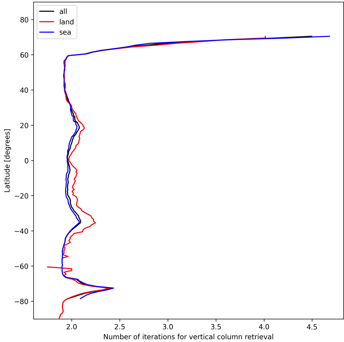
Figure 27: Zonal average of “Number of iterations for vertical column retrieval” for 2025-01-26 to 2025-01-26.
