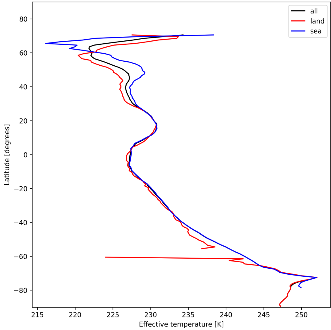
Figure 26: Zonal average of “Effective temperature” for 2025-01-26 to 2025-01-26.
