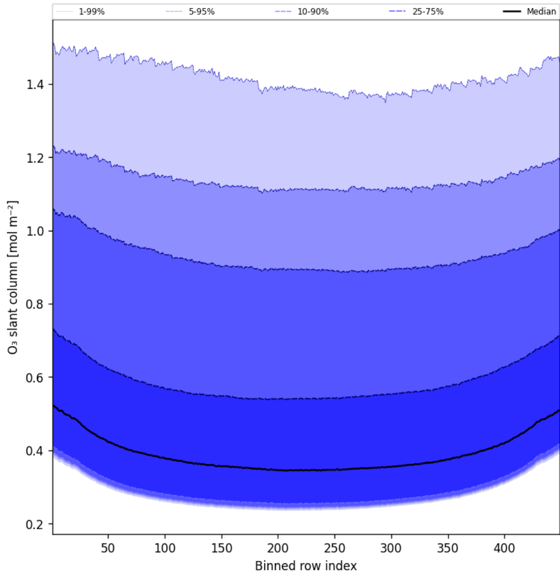
Figure 43: Along track statistics of “O 3 slant column” for 2025-01-26 to 2025-01-26
