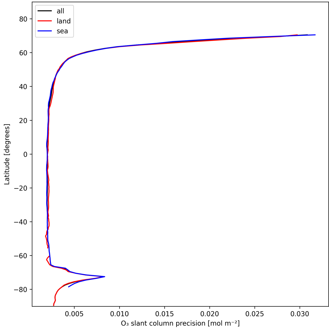
Figure 20: Zonal average of “O 3 slant column precision” for 2025-01-26 to 2025-01-26.
