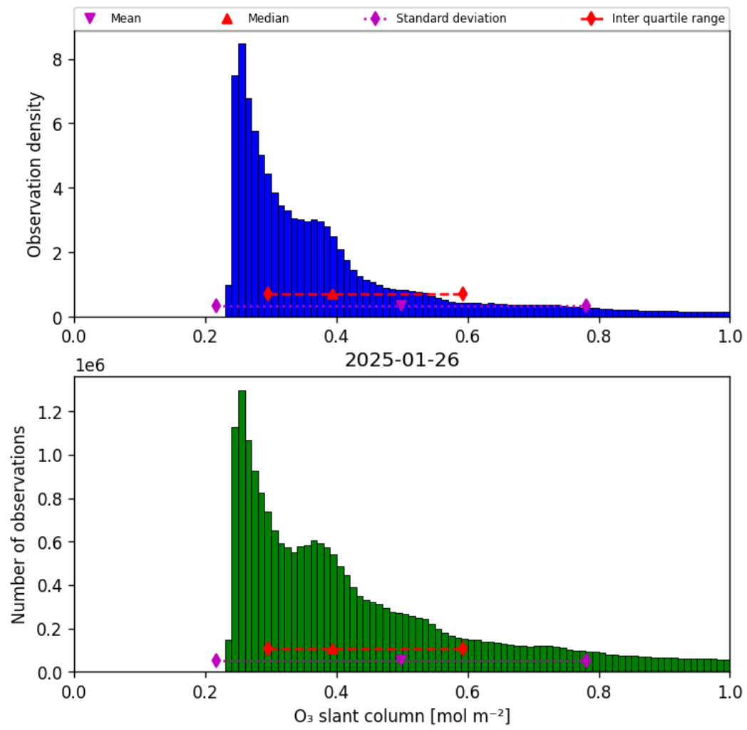
Figure 31: Histogram of “O 3 slant column” for 2025-01-26 to 2025-01-26
