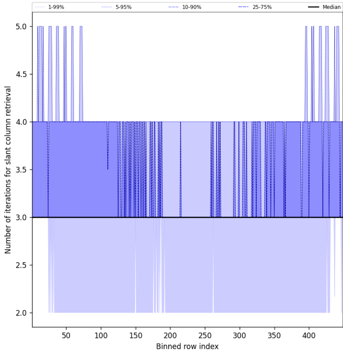
Figure 45: Along track statistics of “Number of iterations for slant column retrieval” for 2025-01-26 to 2025-01-26
