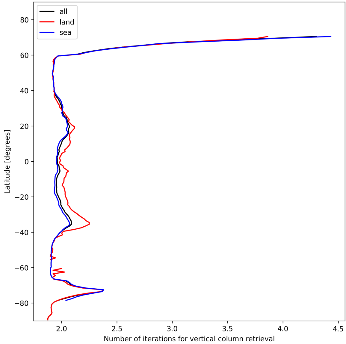
Figure 27: Zonal average of “Number of iterations for vertical column retrieval” for 2025-01-27 to 2025-01-28.
