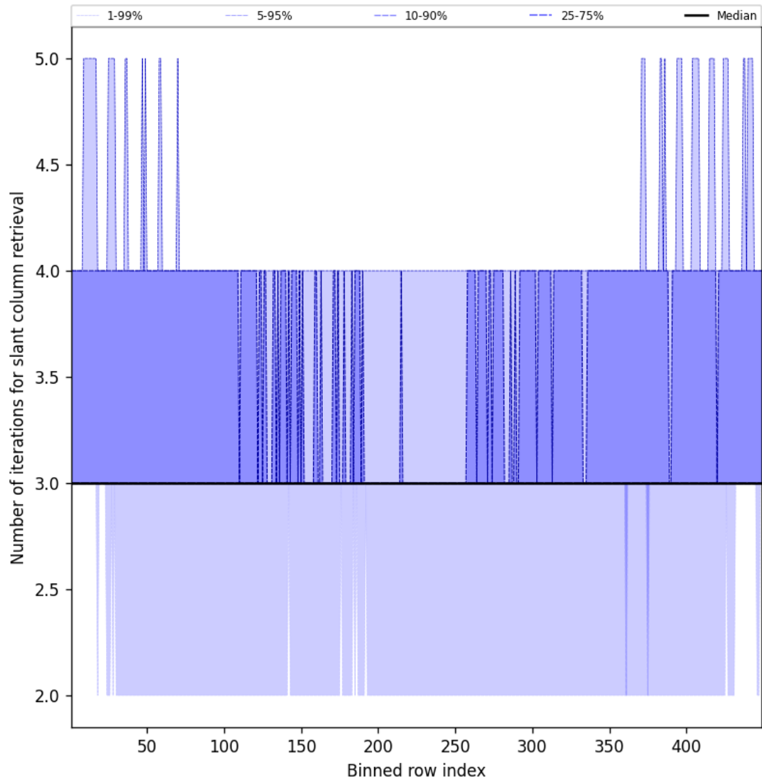
Figure 45: Along track statistics of “Number of iterations for slant column retrieval” for 2025-01-27 to 2025-01-28
