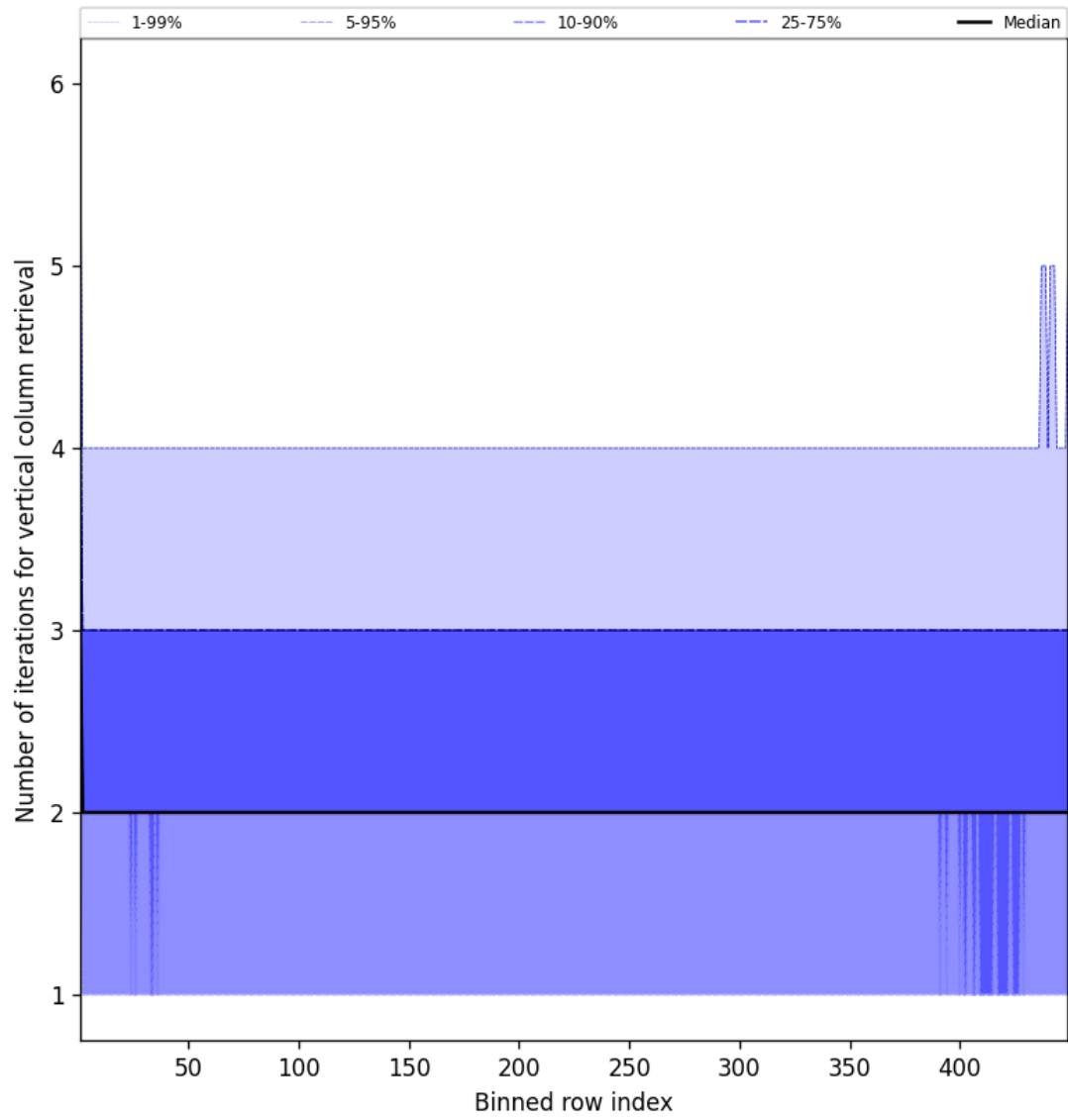
Figure 51: Along track statistics of “Number of iterations for vertical column retrieval” for 2025-01-27 to 2025-01-28
