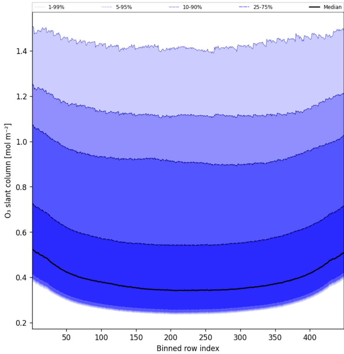
Figure 43: Along track statistics of “O 3 slant column” for 2025-01-27 to 2025-01-28
