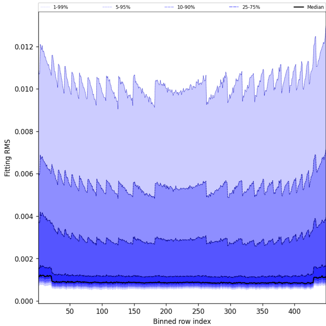
Figure 46: Along track statistics of “Fitting RMS” for 2025-01-27 to 2025-01-28
