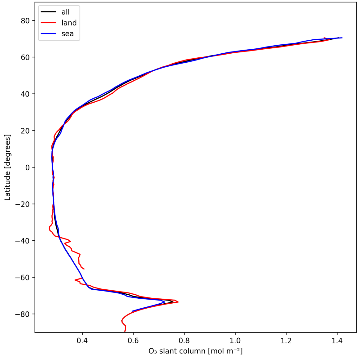
Figure 19: Zonal average of “O 3 slant column” for 2025-01-27 to 2025-01-28.
