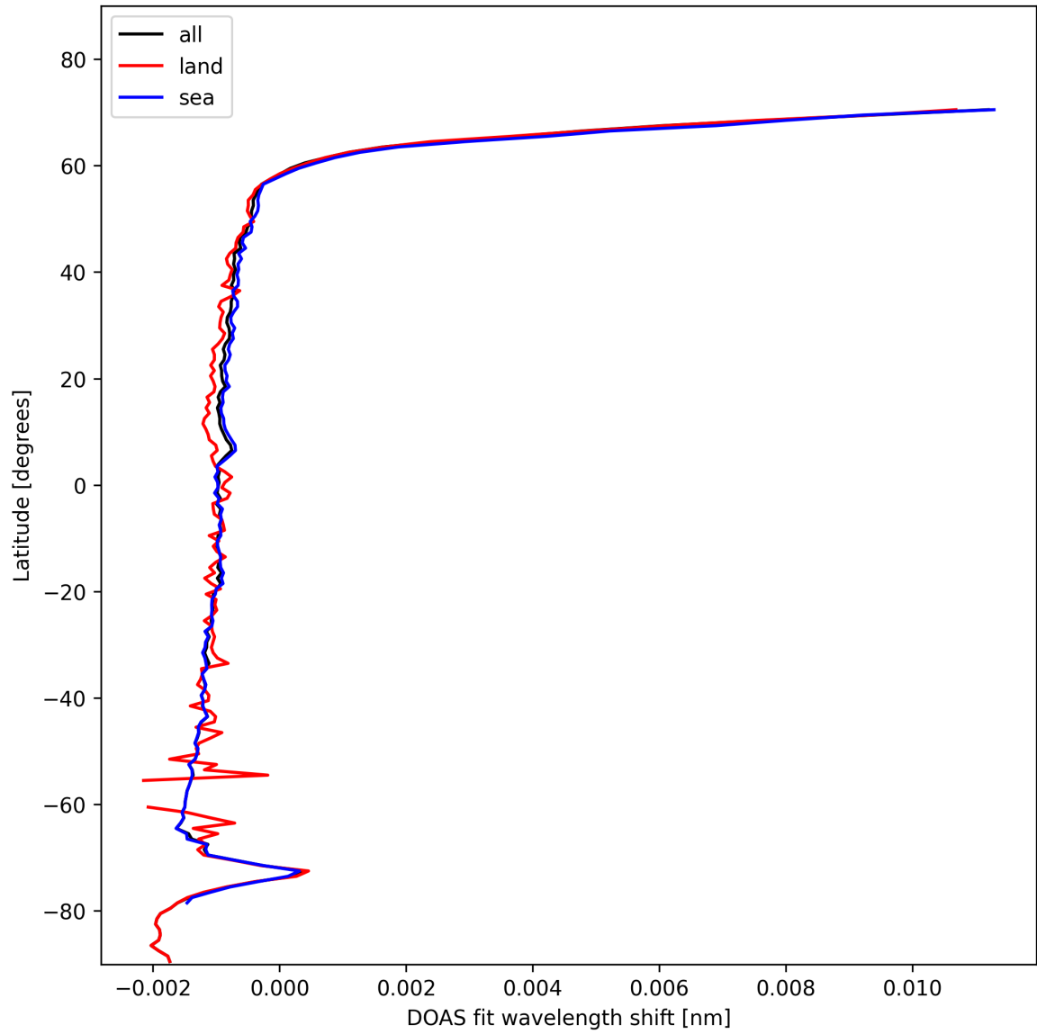
Figure 23: Zonal average of “DOAS fit wavelength shift” for 2025-01-27 to 2025-01-28.
