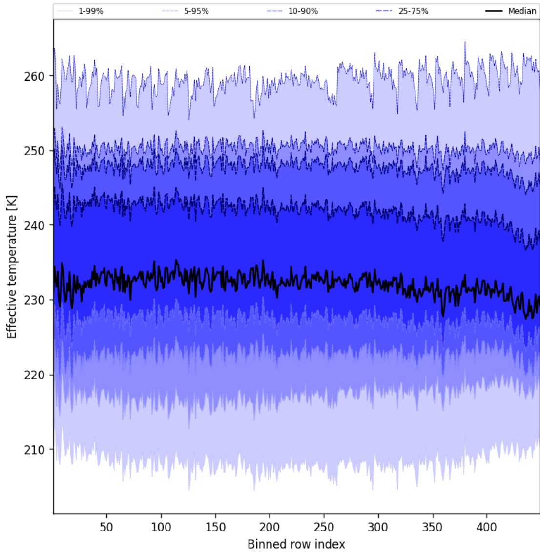
Figure 50: Along track statistics of “Effective temperature” for 2025-01-27 to 2025-01-28
