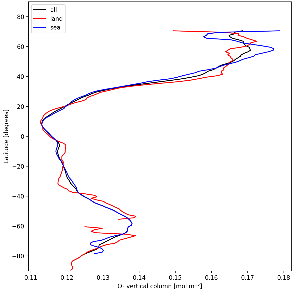
Figure 17: Zonal average of “O 3 vertical column” for 2025-01-27 to 2025-01-28.
