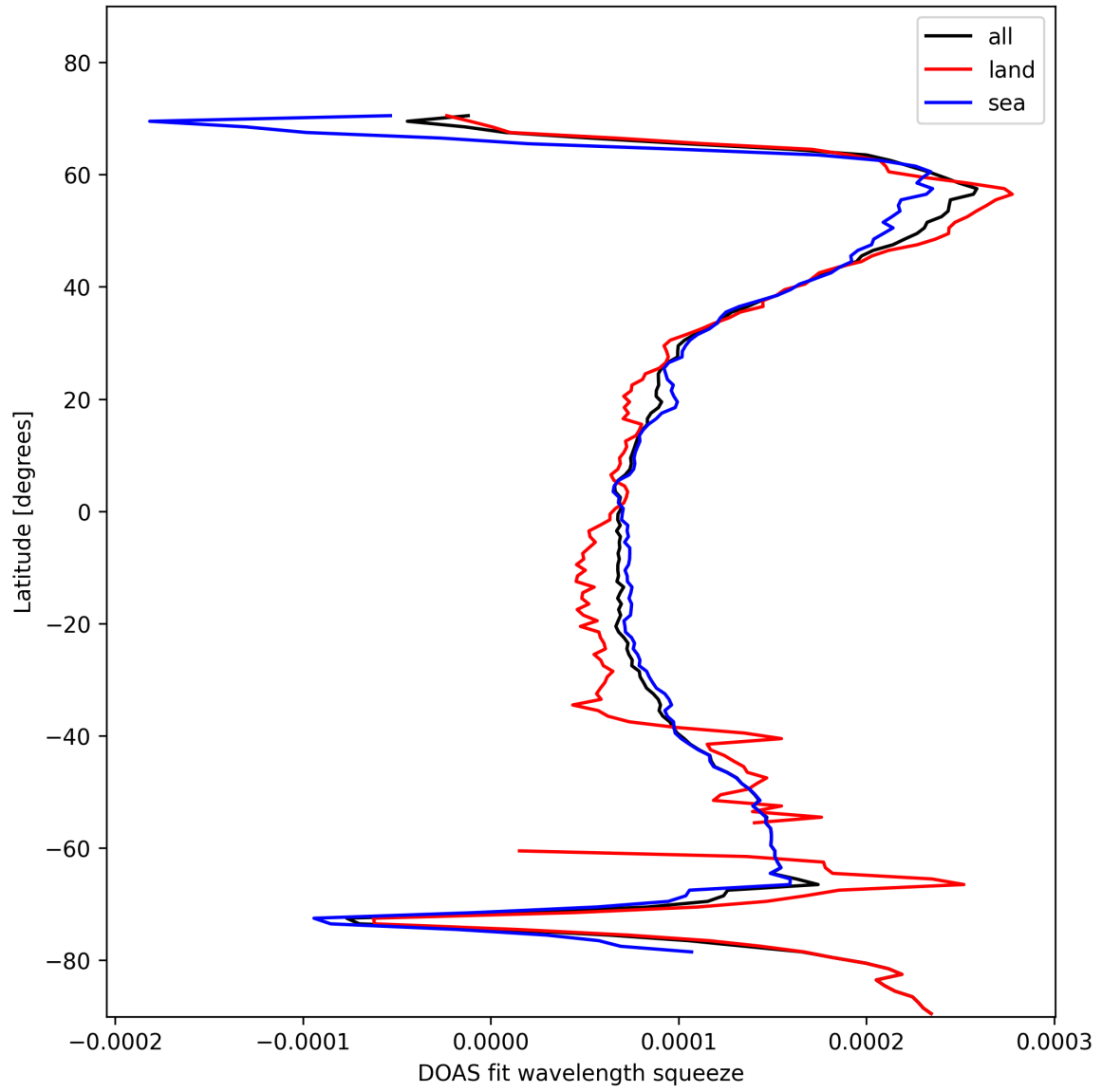
Figure 24: Zonal average of “DOAS fit wavelength squeeze” for 2025-01-27 to 2025-01-28.
