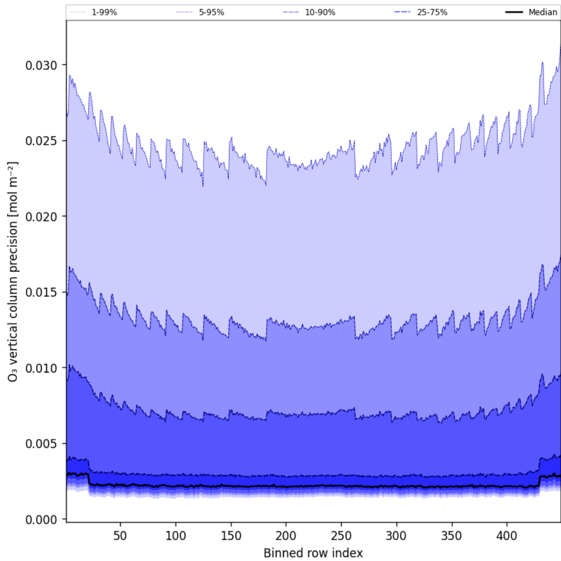
Figure 42: Along track statistics of “O 3 vertical column precision” for 2025-01-27 to 2025-01-28
