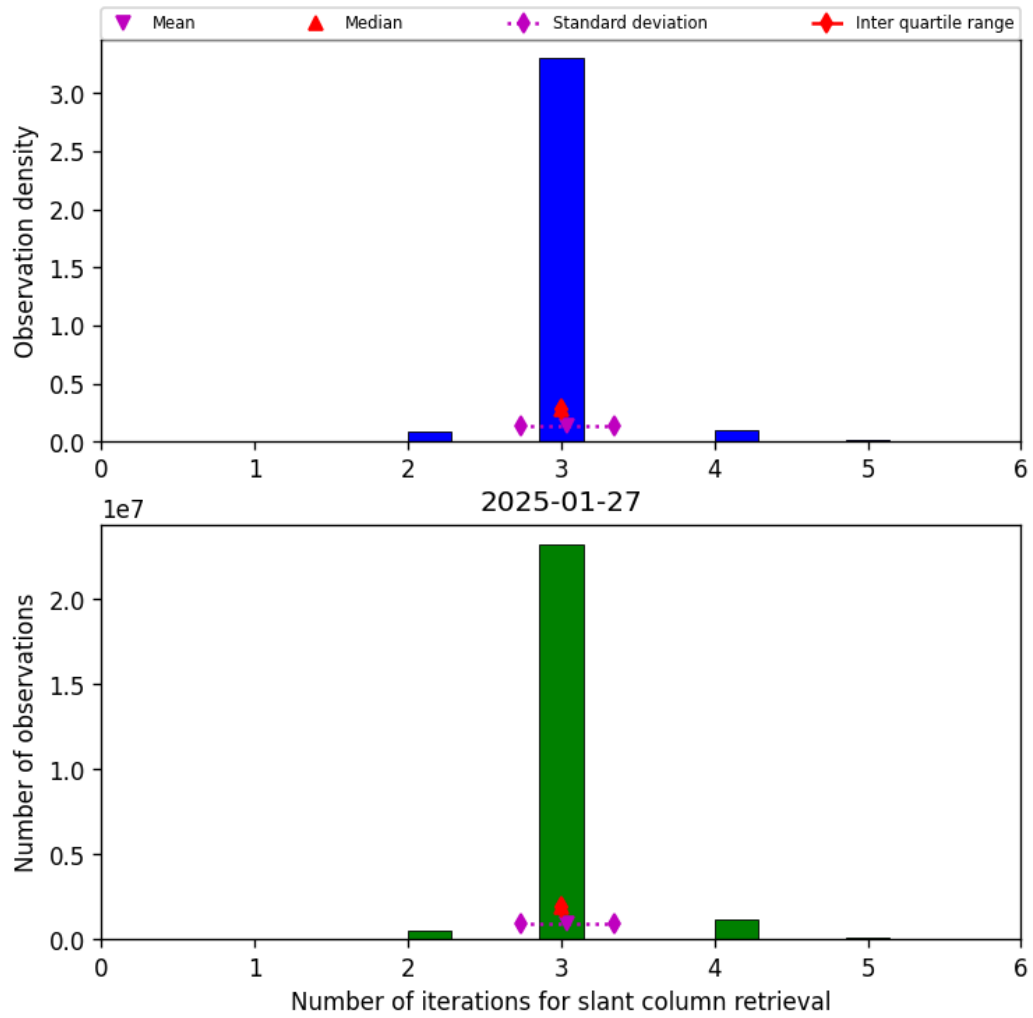
Figure 33: Histogram of “Number of iterations for slant column retrieval” for 2025-01-27 to 2025-01-28
