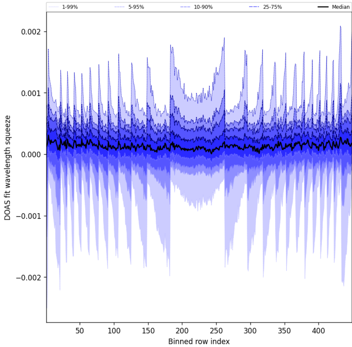
Figure 48: Along track statistics of “DOAS fit wavelength squeeze” for 2025-01-27 to 2025-01-28
