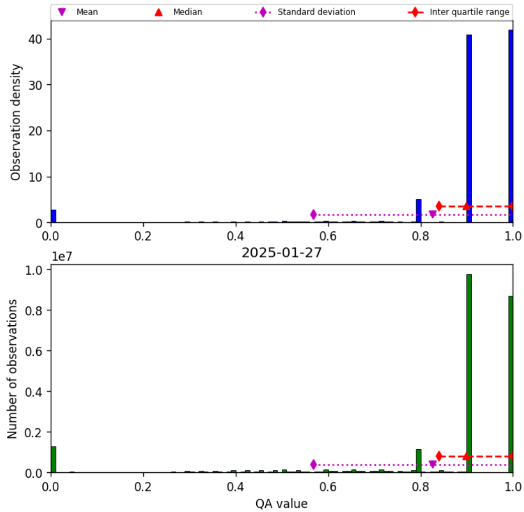
Figure 28: Histogram of “QA value” for 2025-01-27 to 2025-01-28
