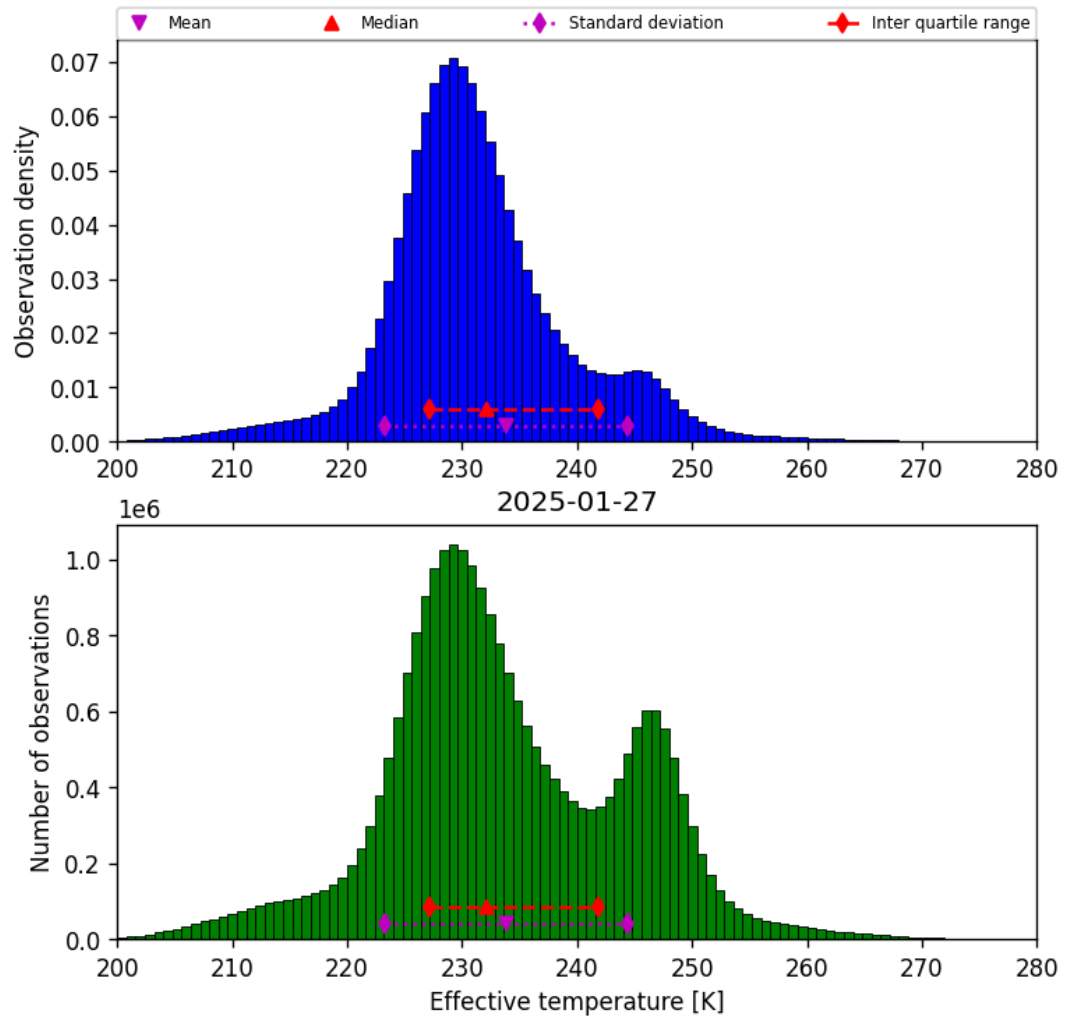
Figure 38: Histogram of “Effective temperature” for 2025-01-27 to 2025-01-28
