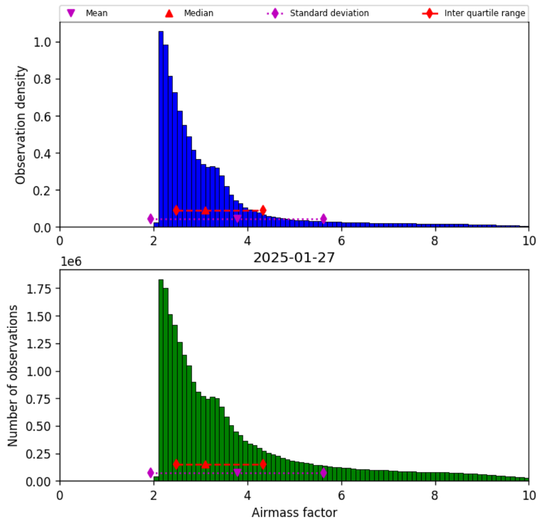
Figure 37: Histogram of “Airmass factor” for 2025-01-27 to 2025-01-28
