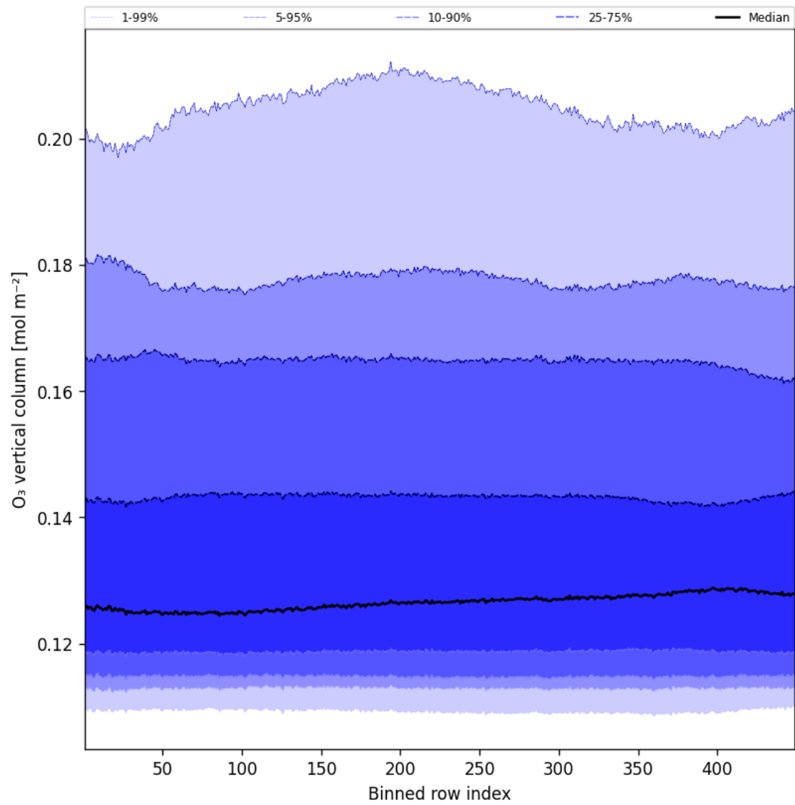
Figure 41: Along track statistics of “ O_3 vertical column” for 2025-01-27 to 2025-01-28
