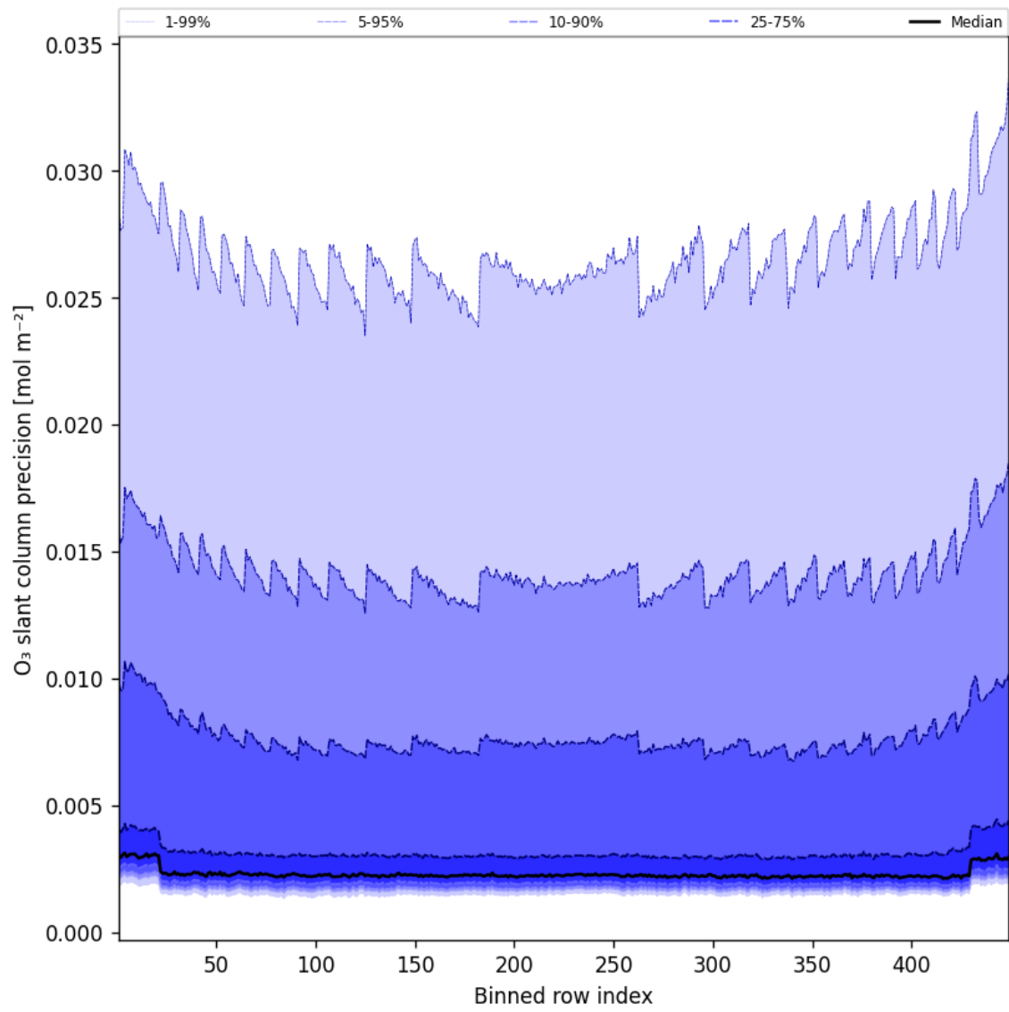
Figure 44: Along track statistics of “O 3 slant column precision” for 2025-01-27 to 2025-01-28
