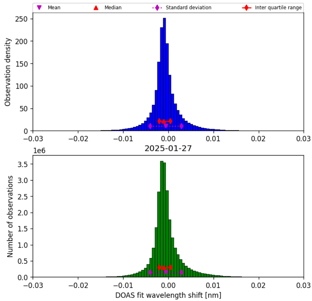
Figure 35: Histogram of “DOAS fit wavelength shift” for 2025-01-27 to 2025-01-28
