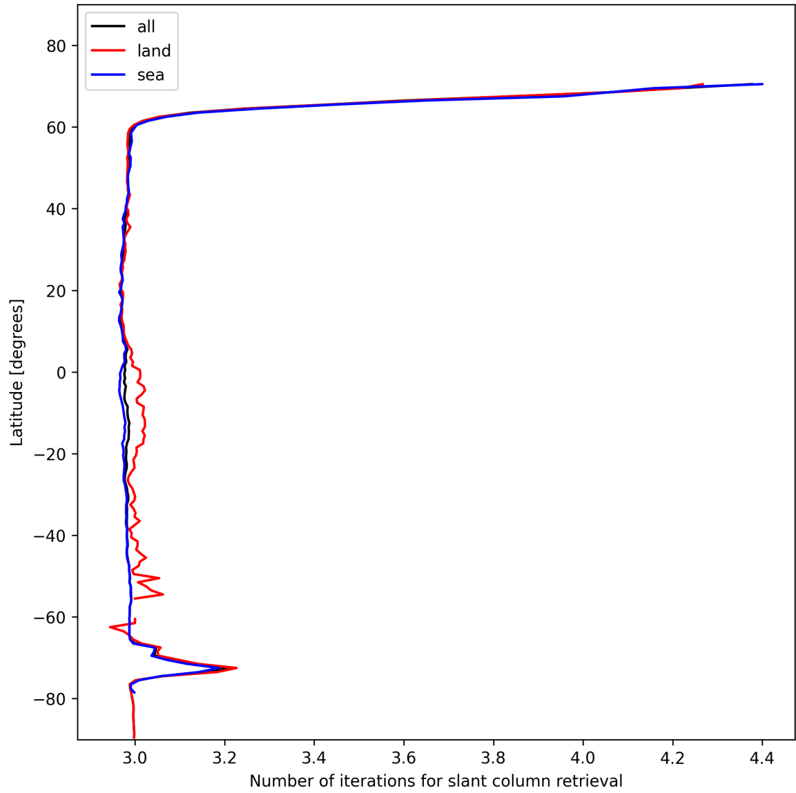
Figure 21: Zonal average of “Number of iterations for slant column retrieval” for 2025-01-27 to 2025-01-28.
