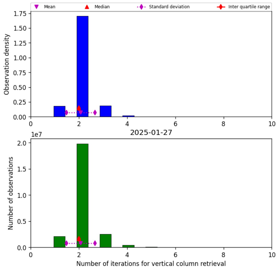
Figure 39: Histogram of “Number of iterations for vertical column retrieval” for 2025-01-27 to 2025-01-28
