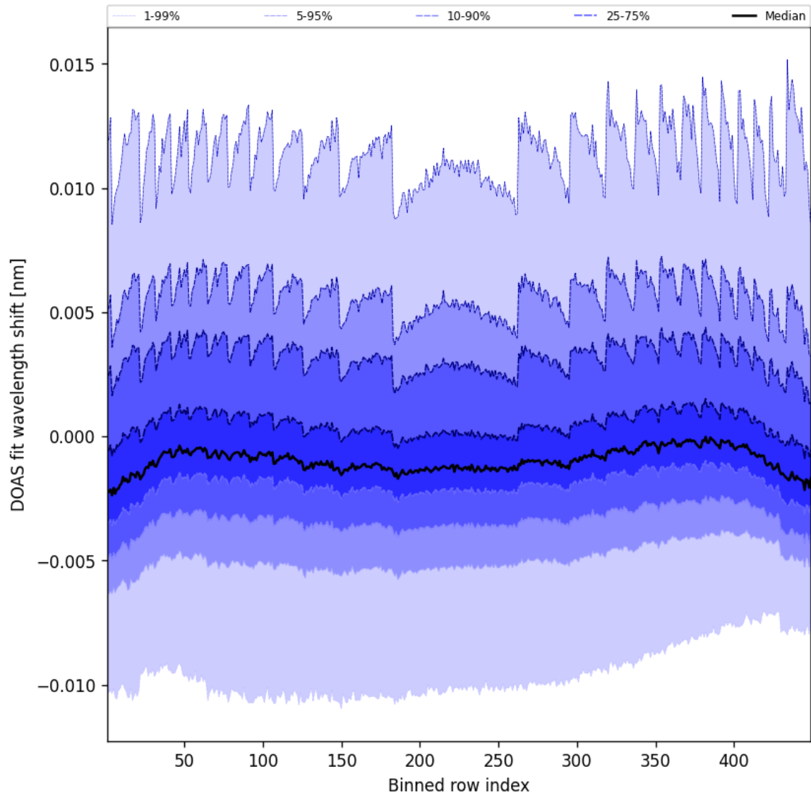
Figure 47: Along track statistics of “DOAS fit wavelength shift” for 2025-01-27 to 2025-01-28
