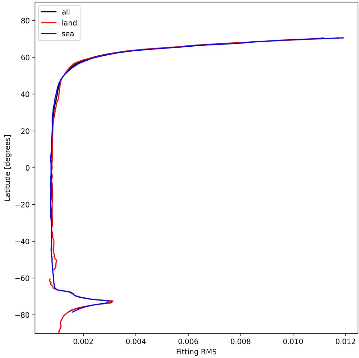
Figure 22: Zonal average of “Fitting RMS” for 2025-01-27 to 2025-01-28.
