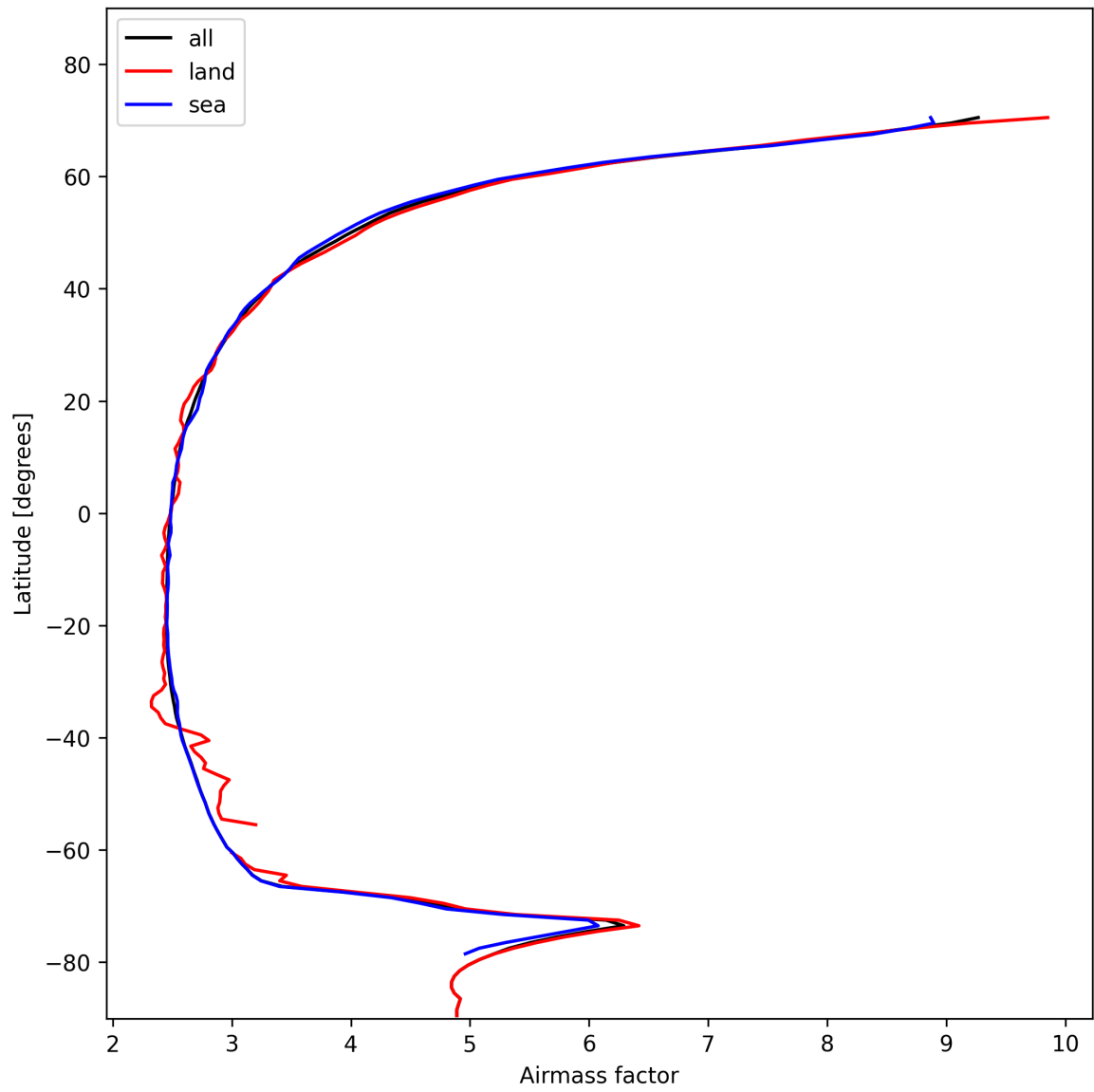
Figure 25: Zonal average of “Airmass factor” for 2025-01-27 to 2025-01-28.
