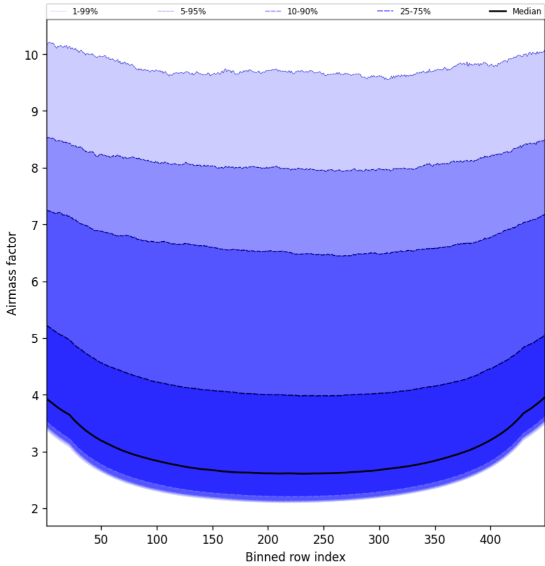
Figure 49: Along track statistics of “Airmass factor” for 2025-01-27 to 2025-01-28
