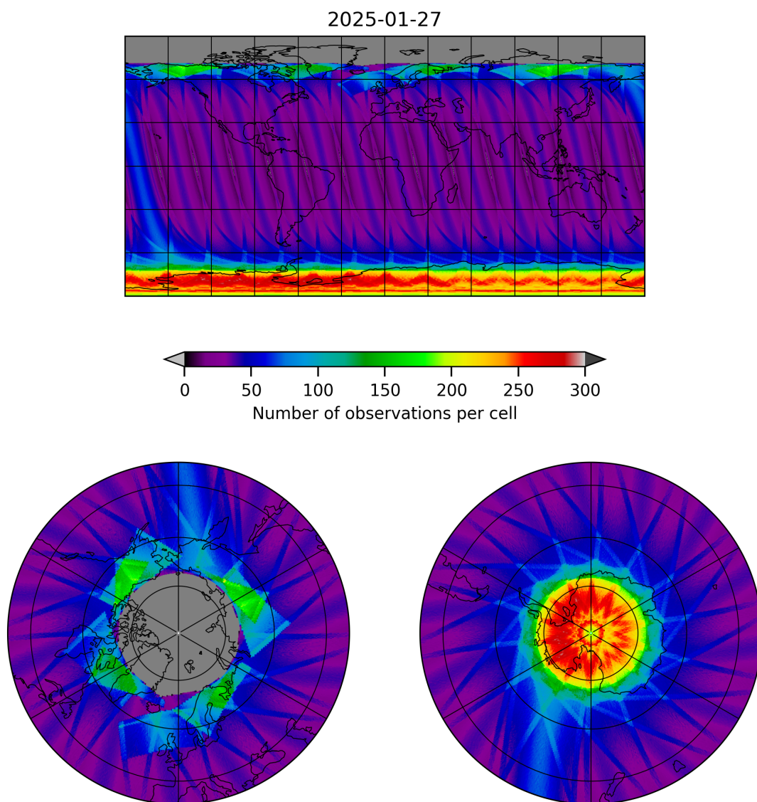
Figure 15: Map of the number of observations for 2025-01-27 to 2025-01-28
