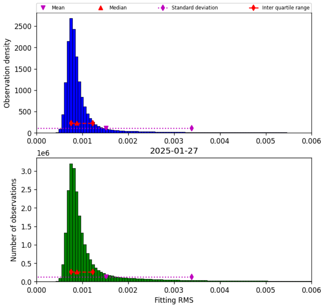
Figure 34: Histogram of “Fitting RMS” for 2025-01-27 to 2025-01-28
