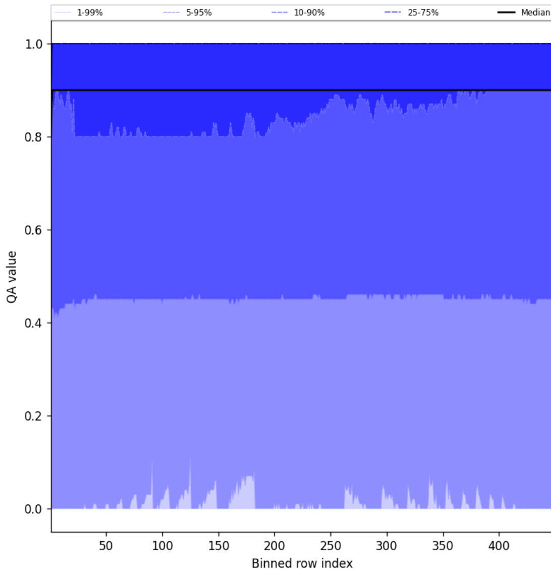
Figure 40: Along track statistics of “QA value” for 2025-01-27 to 2025-01-28
