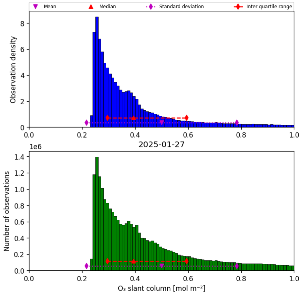
Figure 31: Histogram of “O 3 slant column” for 2025-01-27 to 2025-01-28
