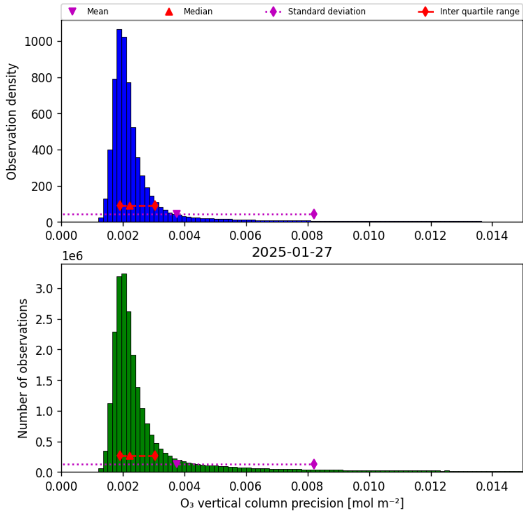
Figure 30: Histogram of “O 3 vertical column precision” for 2025-01-27 to 2025-01-28
