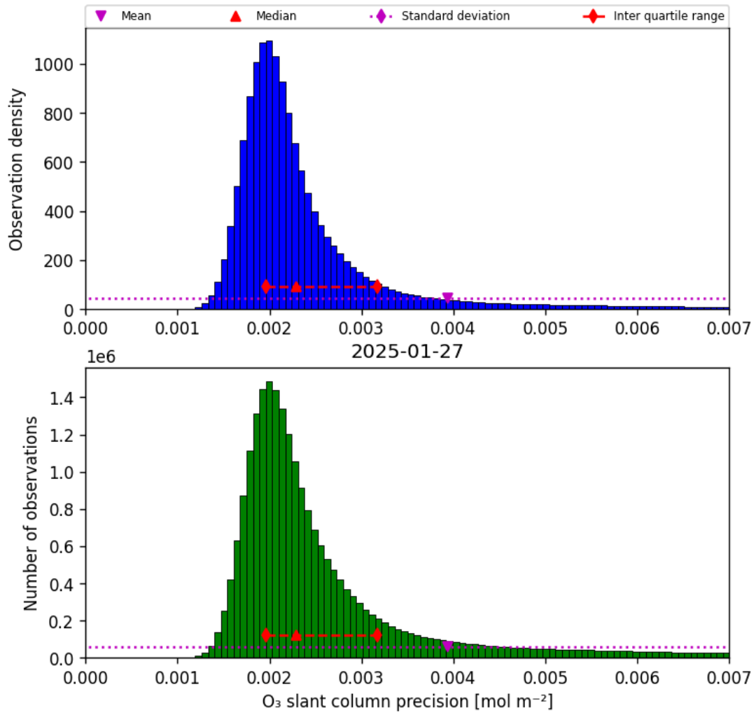
Figure 32: Histogram of “O 3 slant column precision” for 2025-01-27 to 2025-01-28
