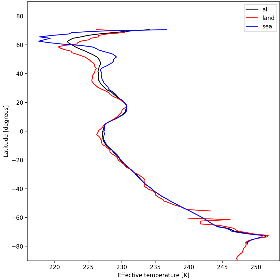
Figure 26: Zonal average of “Effective temperature” for 2025-01-27 to 2025-01-28.
