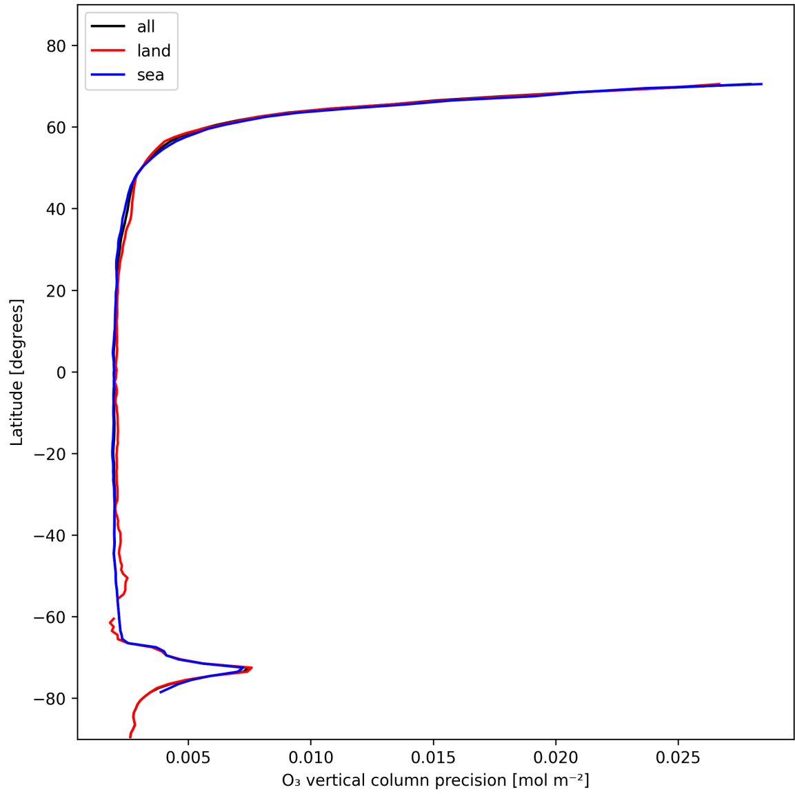
Figure 18: Zonal average of “O 3 vertical column precision” for 2025-01-27 to 2025-01-28.
