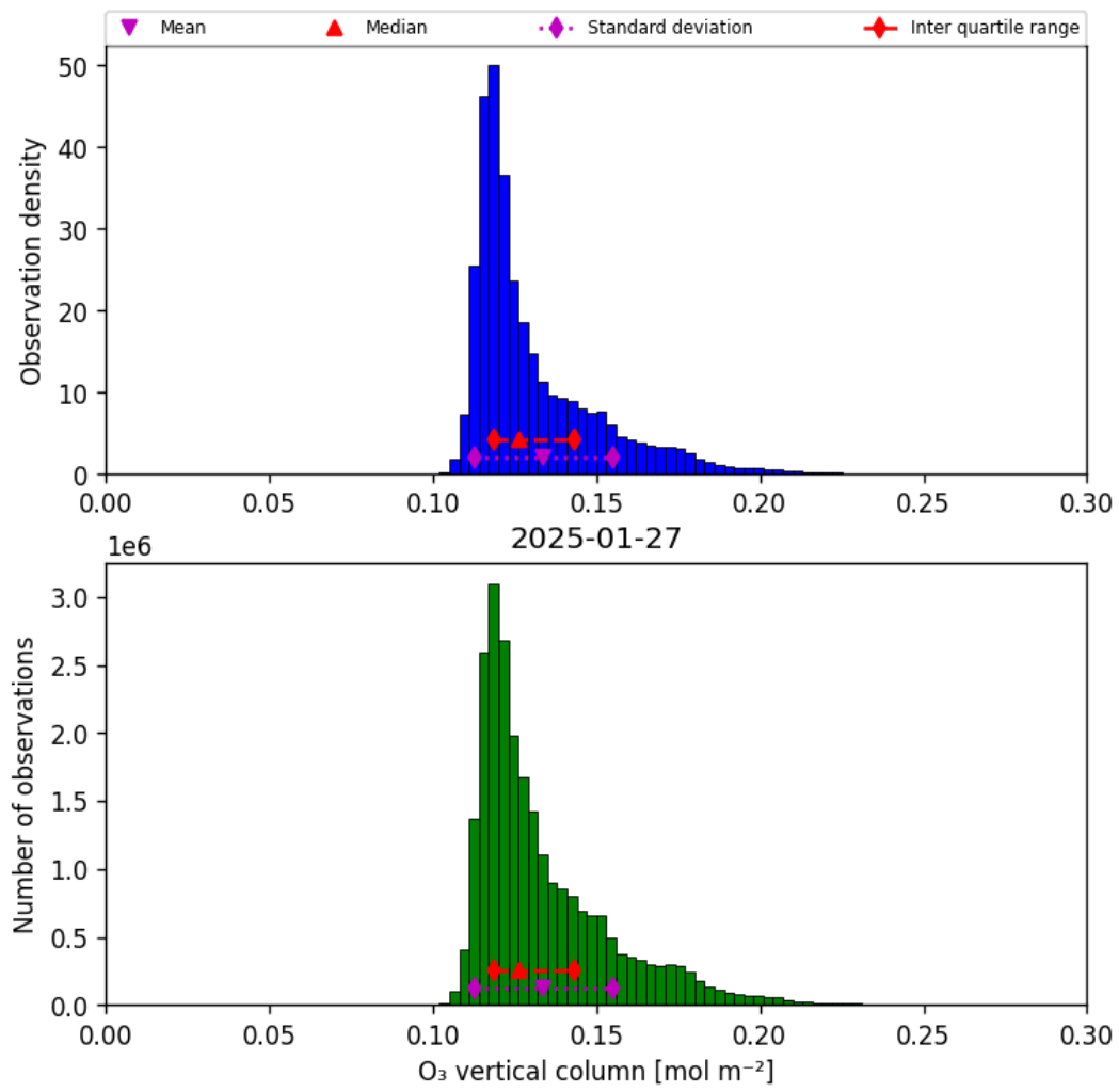
Figure 29: Histogram of “O 3 vertical column” for 2025-01-27 to 2025-01-28
