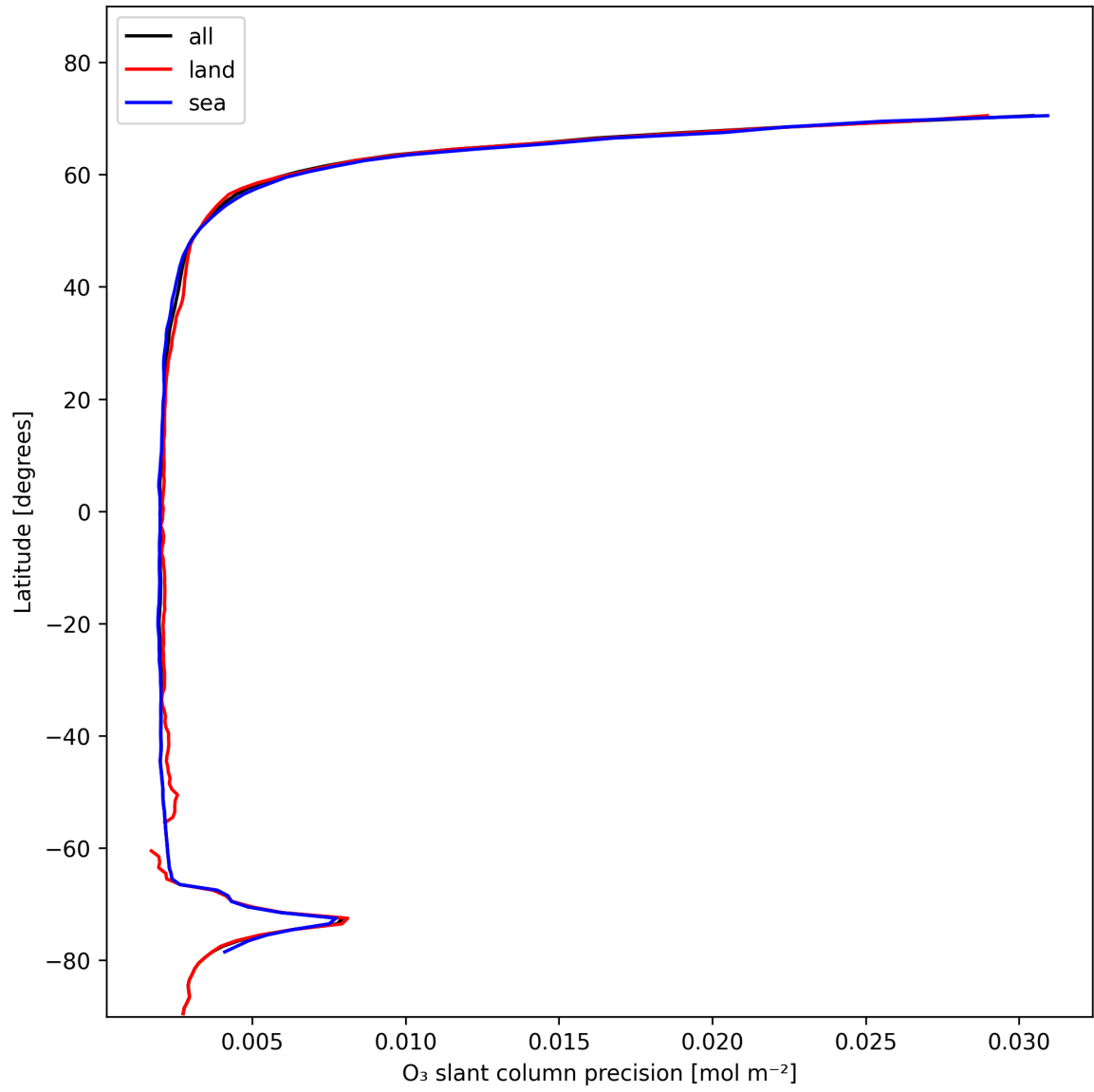
Figure 20: Zonal average of “O 3 slant column precision” for 2025-01-27 to 2025-01-28.
