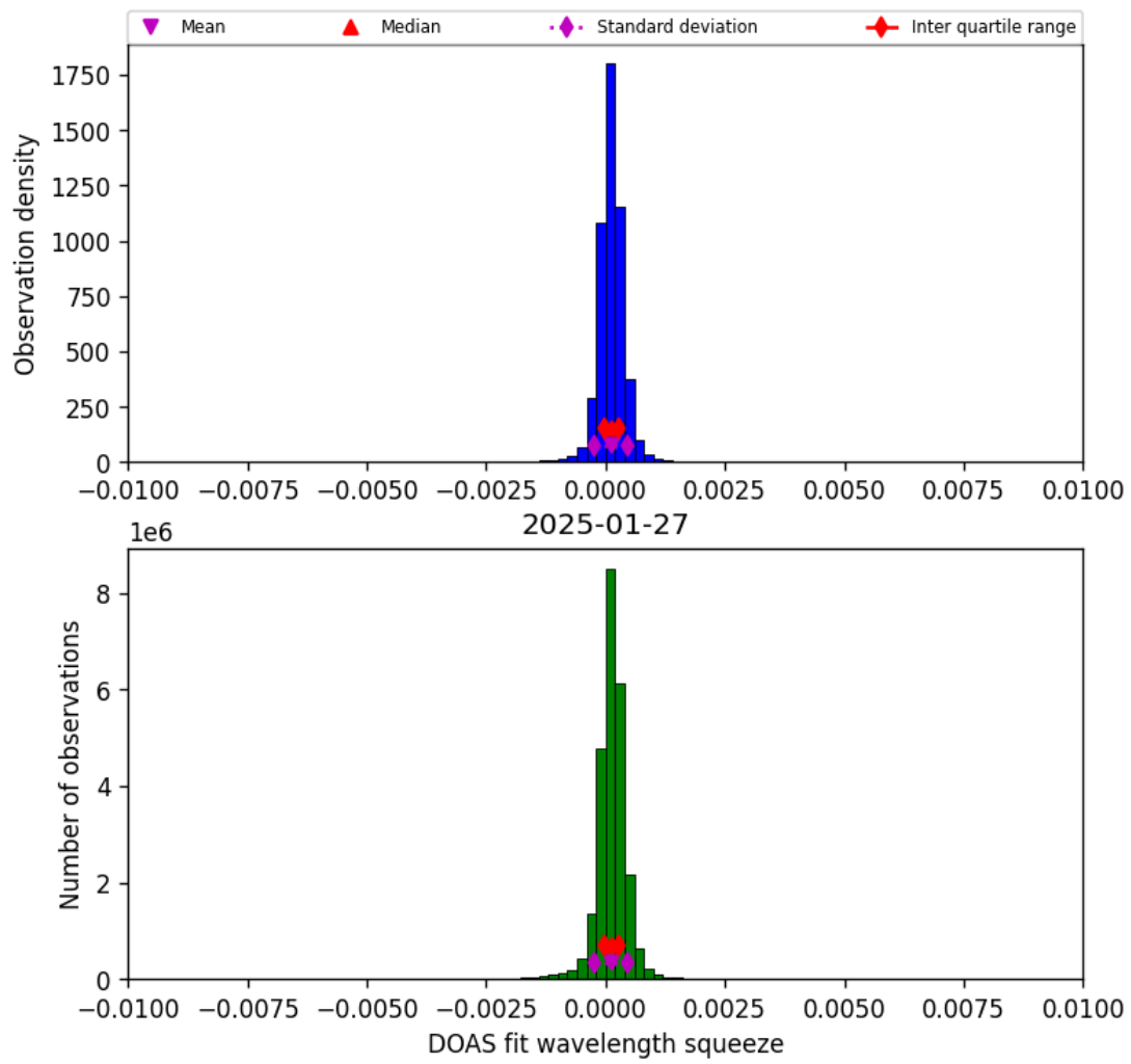
Figure 36: Histogram of “DOAS fit wavelength squeeze” for 2025-01-27 to 2025-01-28
