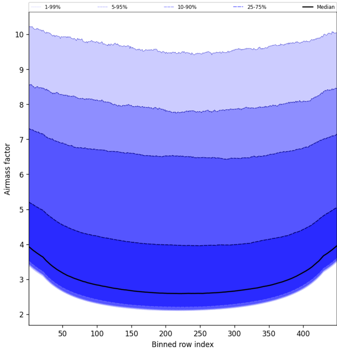
Figure 49: Along track statistics of “Airmass factor” for 2025-01-28 to 2025-01-29
