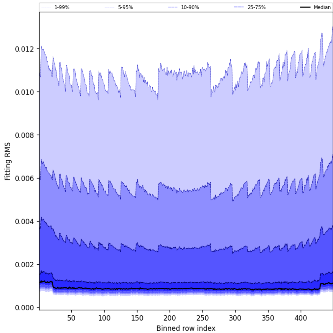
Figure 46: Along track statistics of “Fitting RMS” for 2025-01-28 to 2025-01-29
