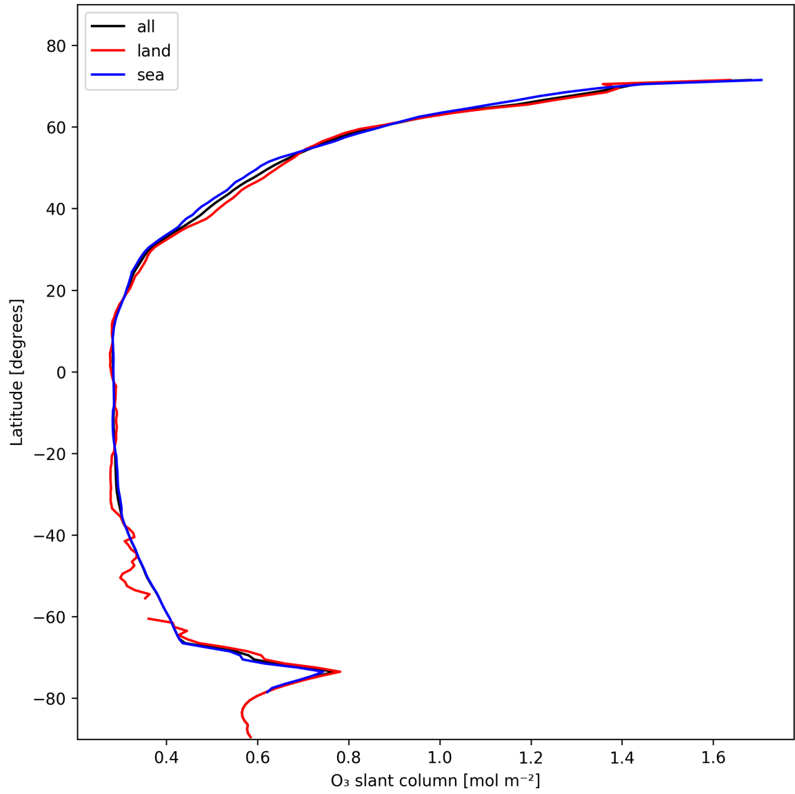
Figure 19: Zonal average of “O 3 slant column” for 2025-01-28 to 2025-01-29.
