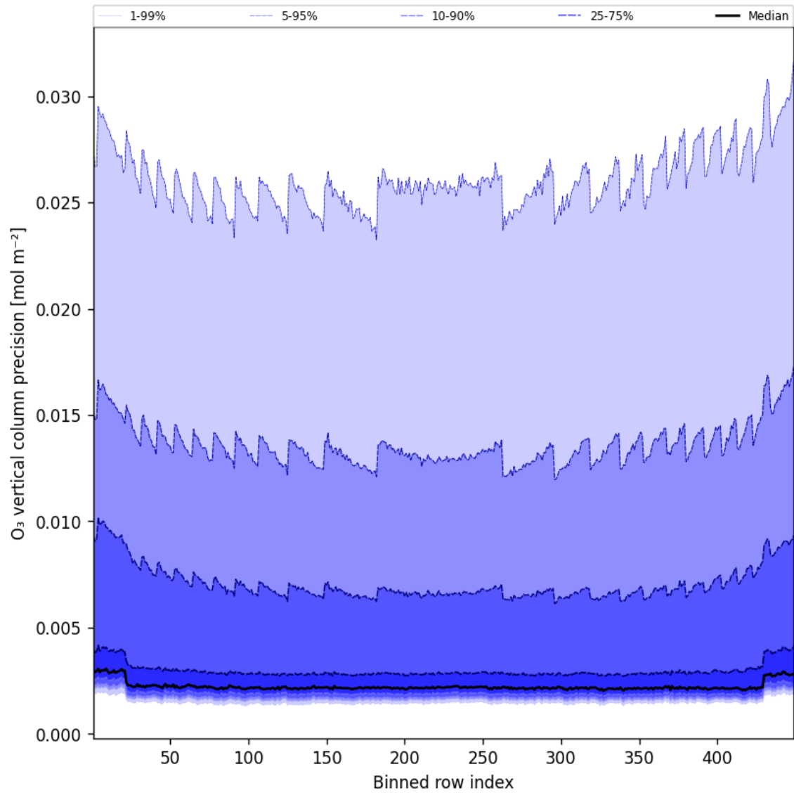
Figure 42: Along track statistics of “O 3 vertical column precision” for 2025-01-28 to 2025-01-29
