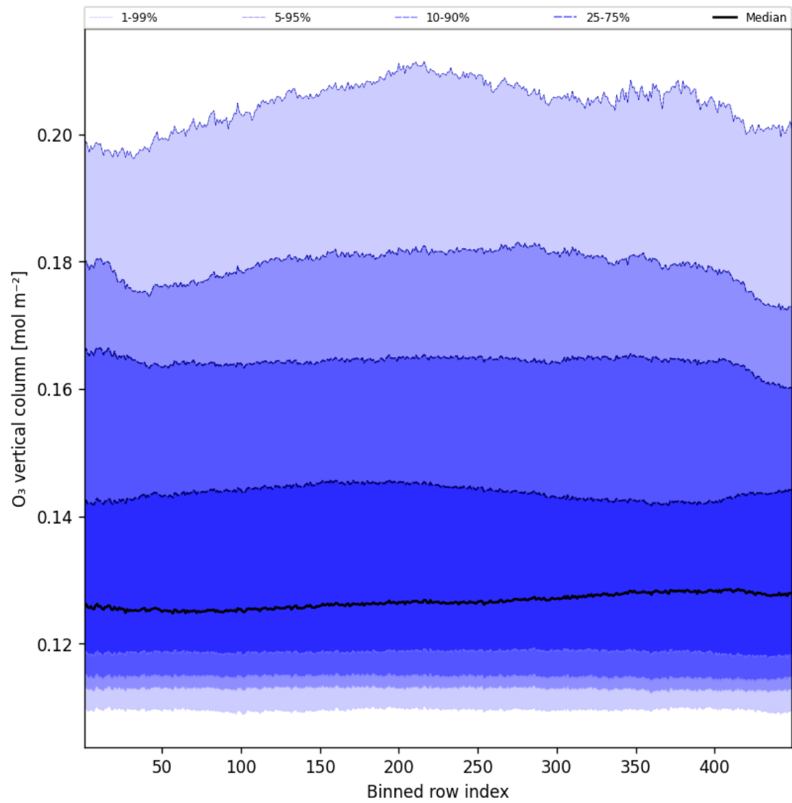
Figure 41: Along track statistics of “O 3 vertical column” for 2025-01-28 to 2025-01-29
