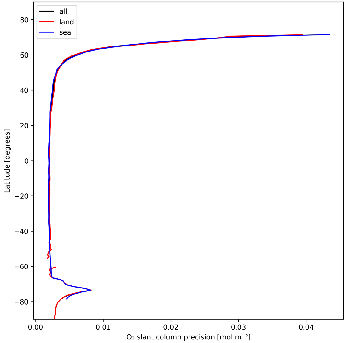
Figure 20: Zonal average of “O 3 slant column precision” for 2025-01-28 to 2025-01-29.
