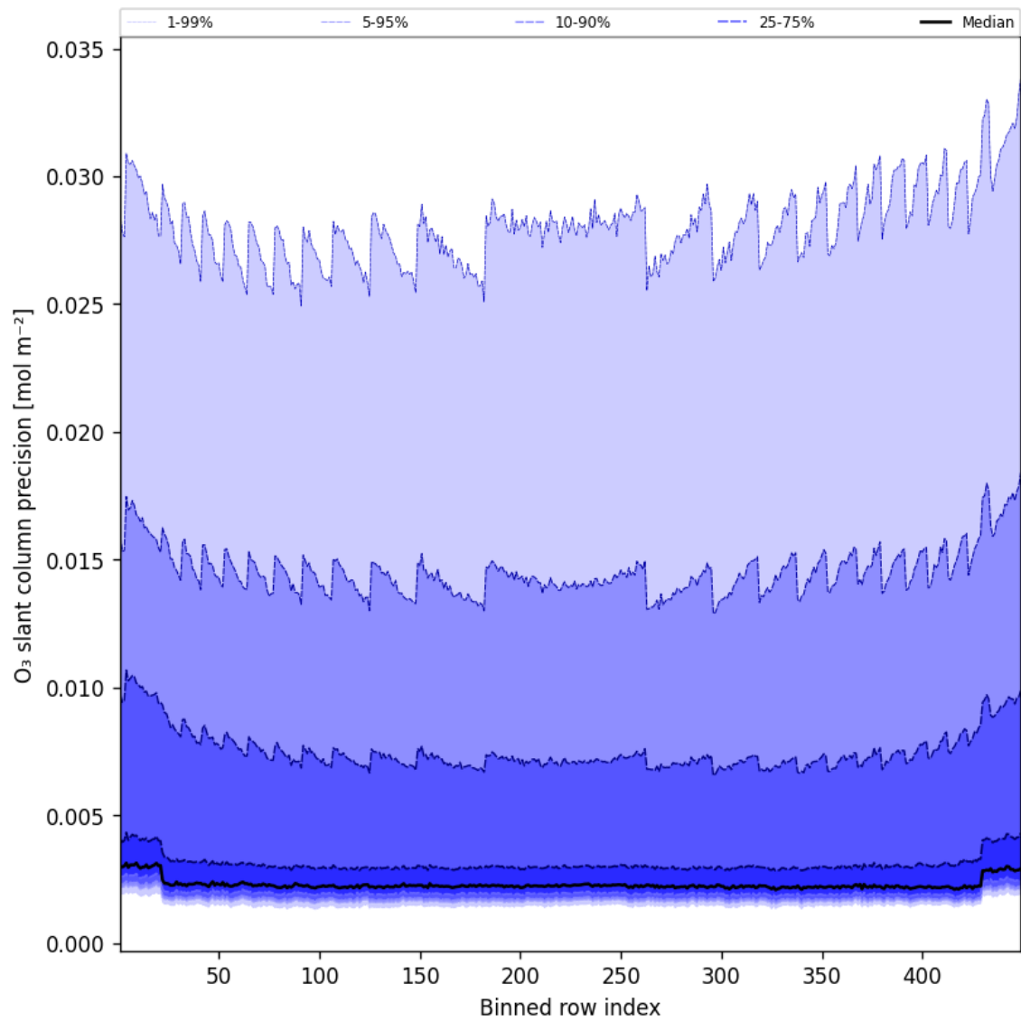
Figure 44: Along track statistics of “O 3 slant column precision” for 2025-01-28 to 2025-01-29
