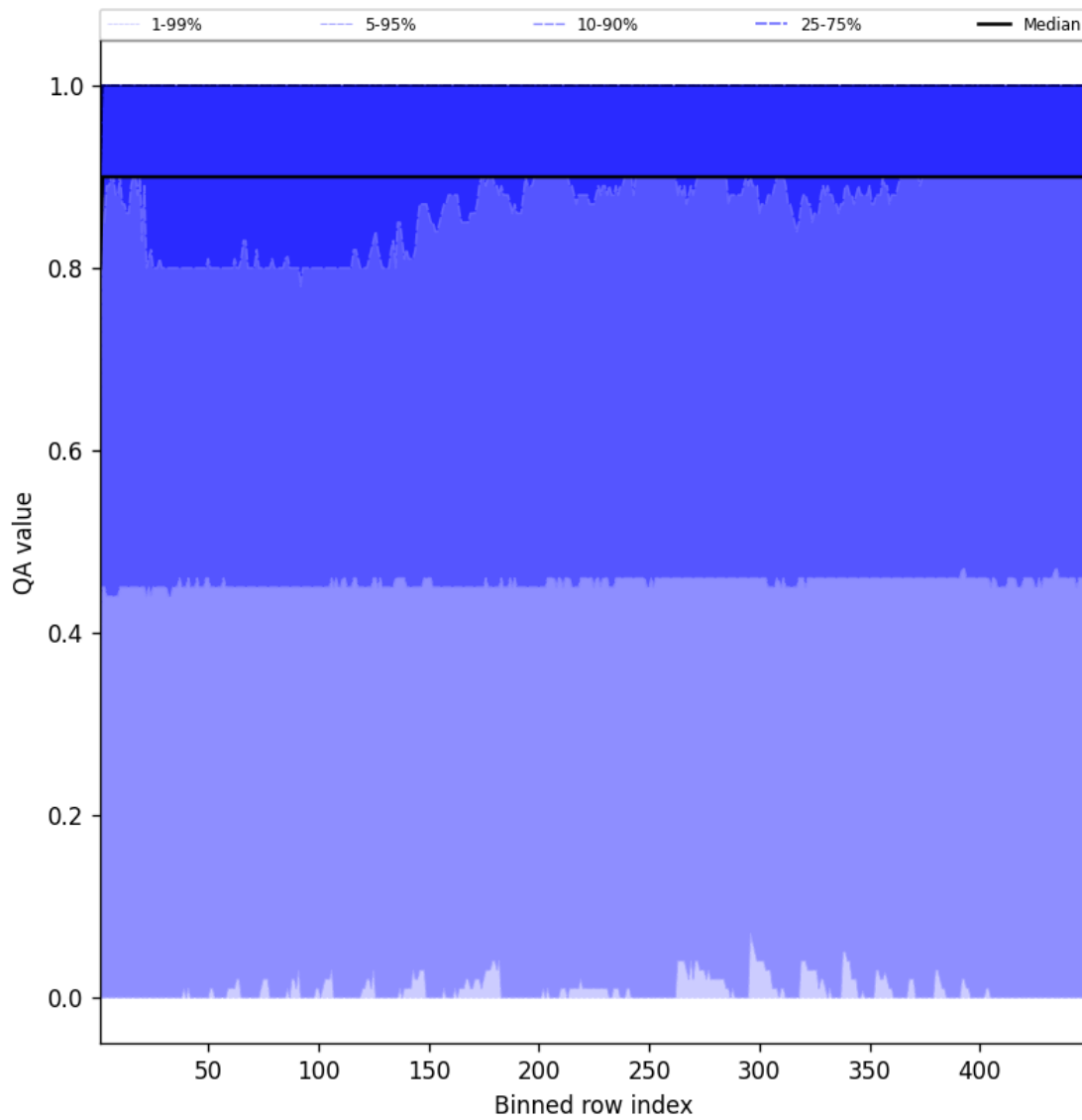
Figure 40: Along track statistics of “QA value” for 2025-01-28 to 2025-01-29
