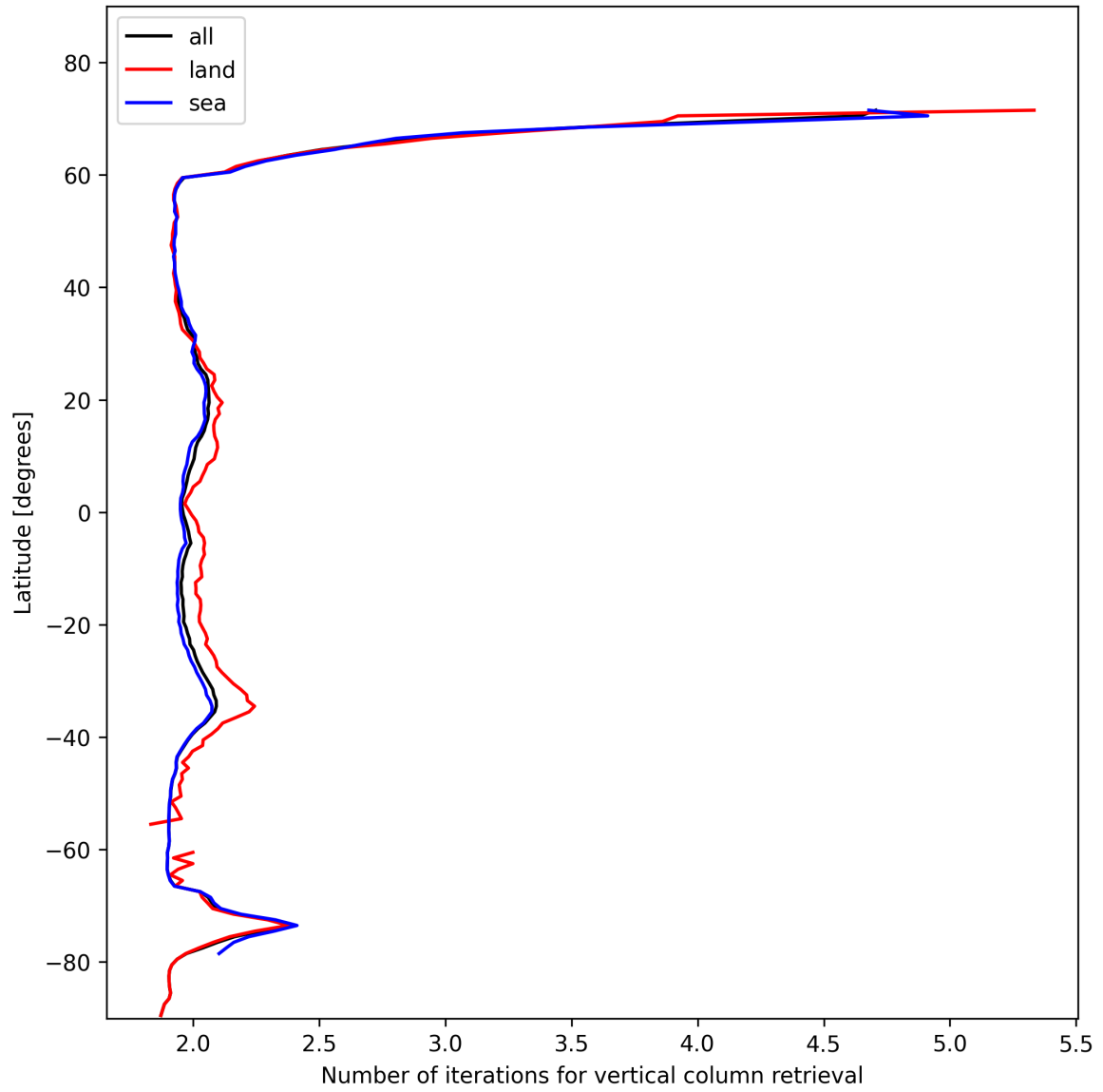
Figure 27: Zonal average of “Number of iterations for vertical column retrieval” for 2025-01-28 to 2025-01-29.
