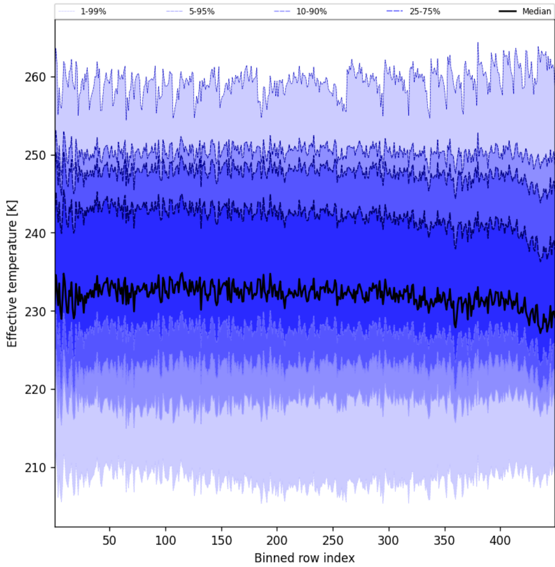
Figure 50: Along track statistics of “Effective temperature” for 2025-01-28 to 2025-01-29
