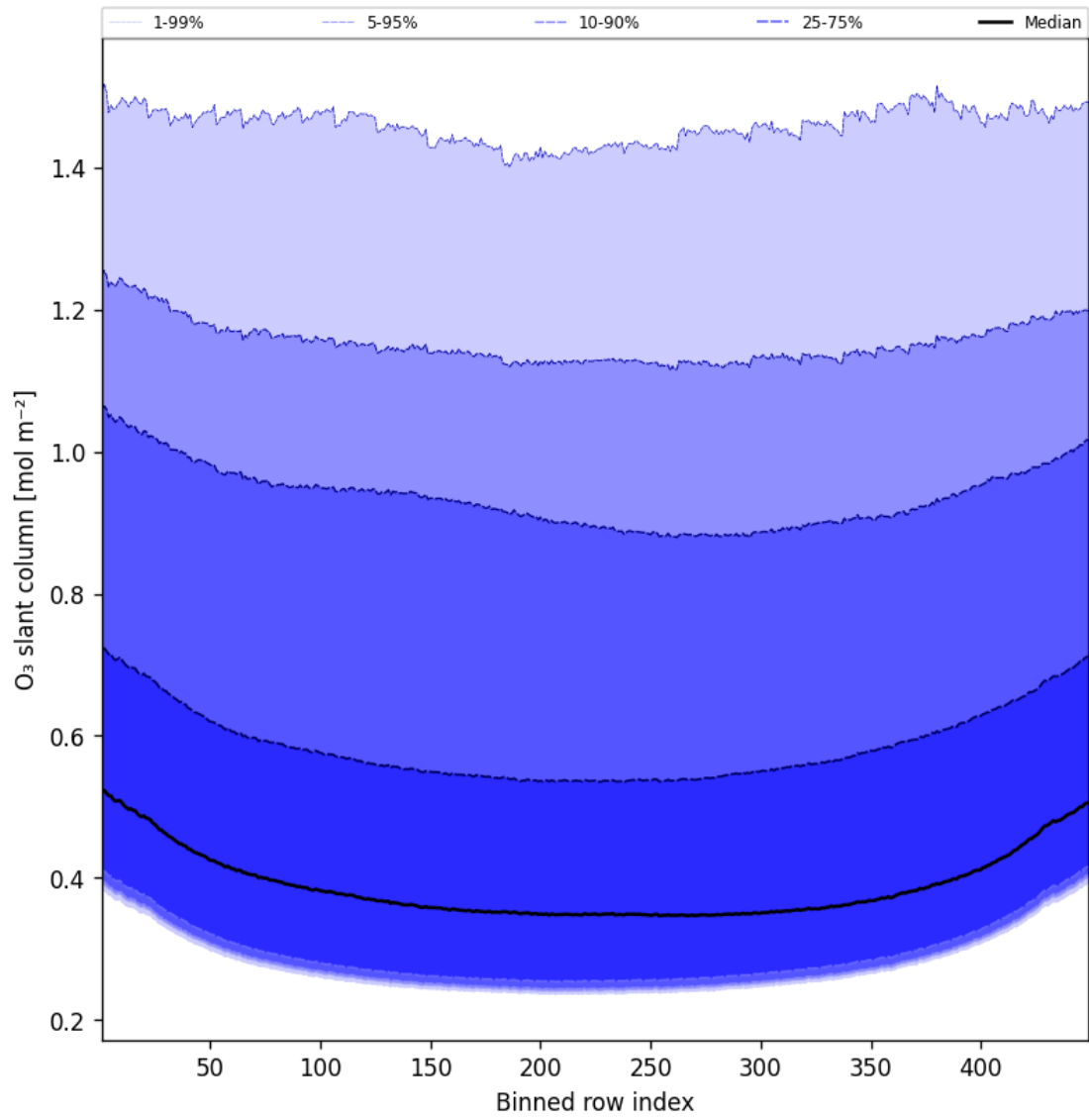
Figure 43: Along track statistics of "O 3 slant column" for 2025-01-28 to 2025-01-29
