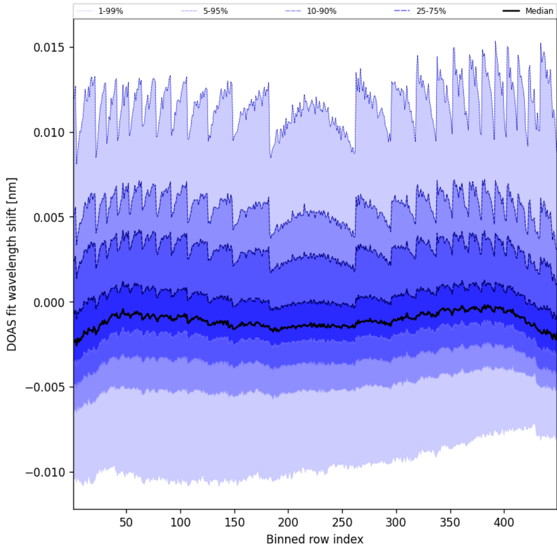
Figure 47: Along track statistics of “DOAS fit wavelength shift” for 2025-01-28 to 2025-01-29
