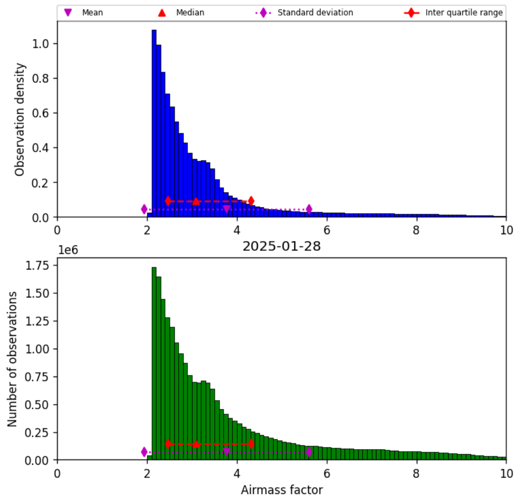
Figure 37: Histogram of “Airmass factor” for 2025-01-28 to 2025-01-29
