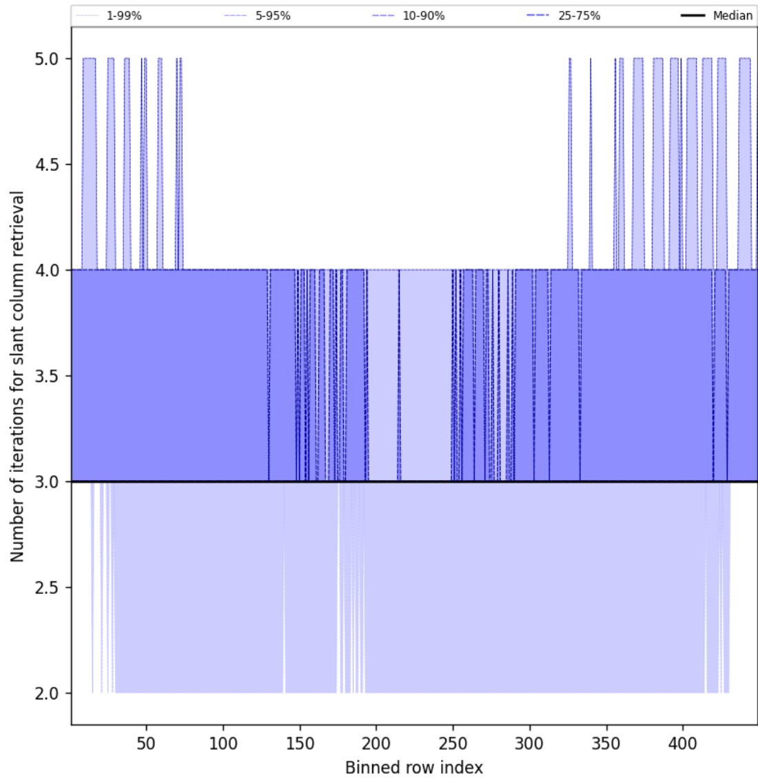
Figure 45: Along track statistics of “Number of iterations for slant column retrieval” for 2025-01-28 to 2025-01-29
