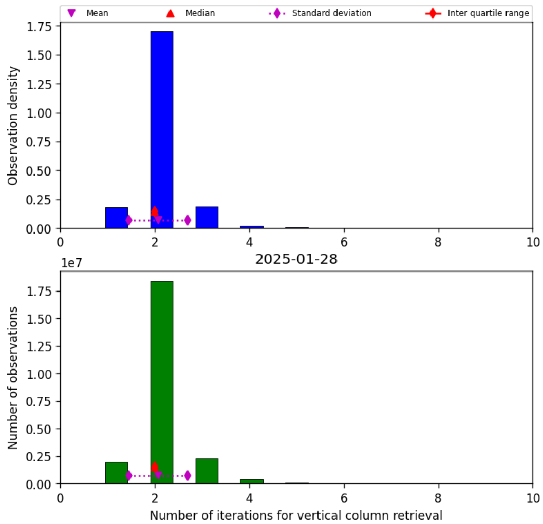
Figure 39: Histogram of “Number of iterations for vertical column retrieval” for 2025-01-28 to 2025-01-29
