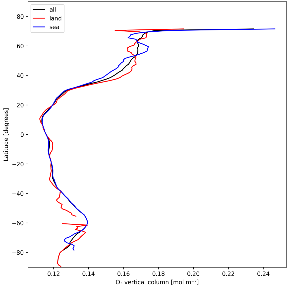
Figure 17: Zonal average of “O 3 vertical column” for 2025-01-28 to 2025-01-29.
