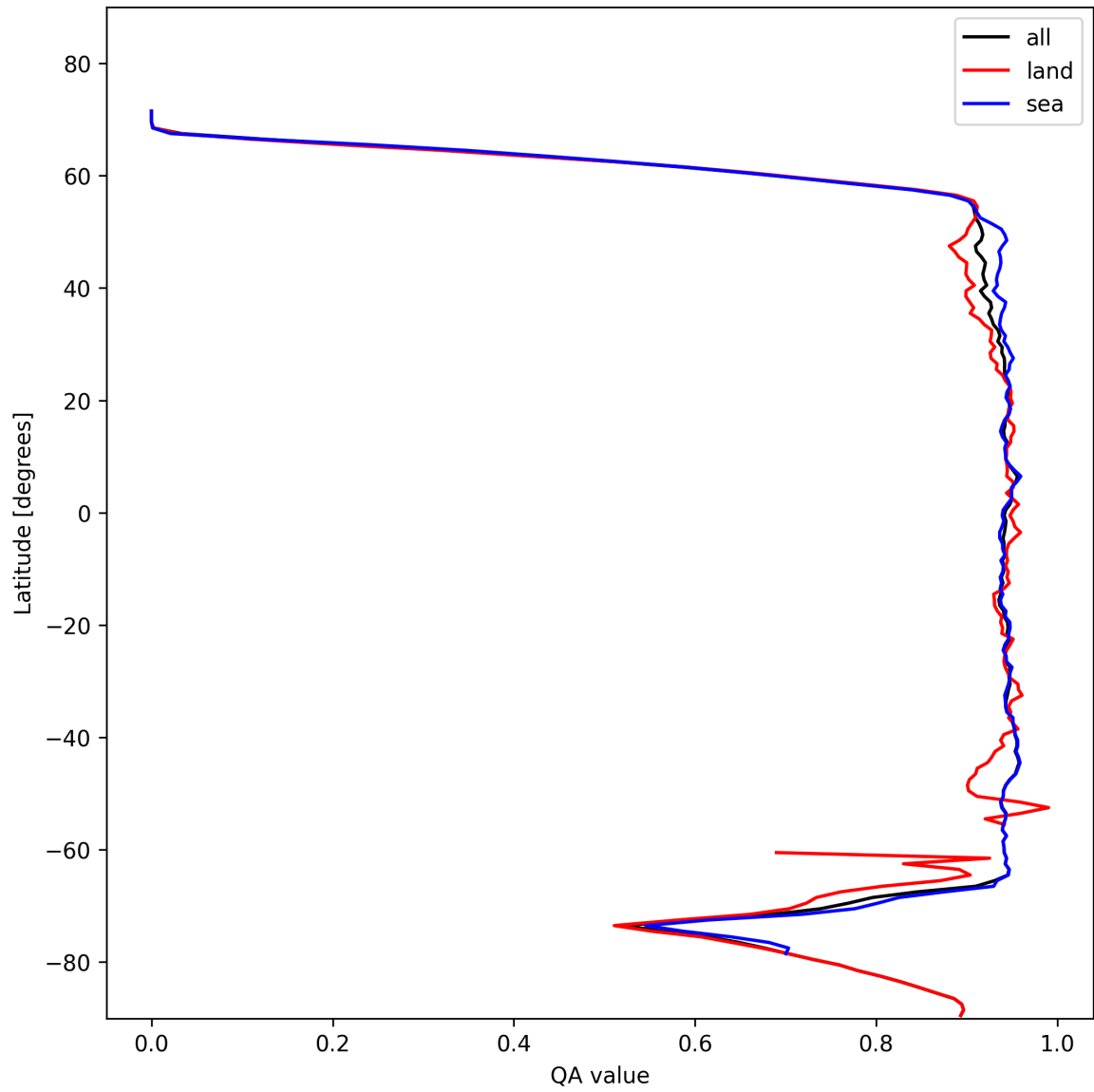
Figure 16: Zonal average of “QA value” for 2025-01-28 to 2025-01-29.
