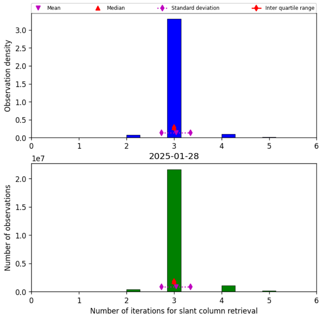
Figure 33: Histogram of “Number of iterations for slant column retrieval” for 2025-01-28 to 2025-01-29
