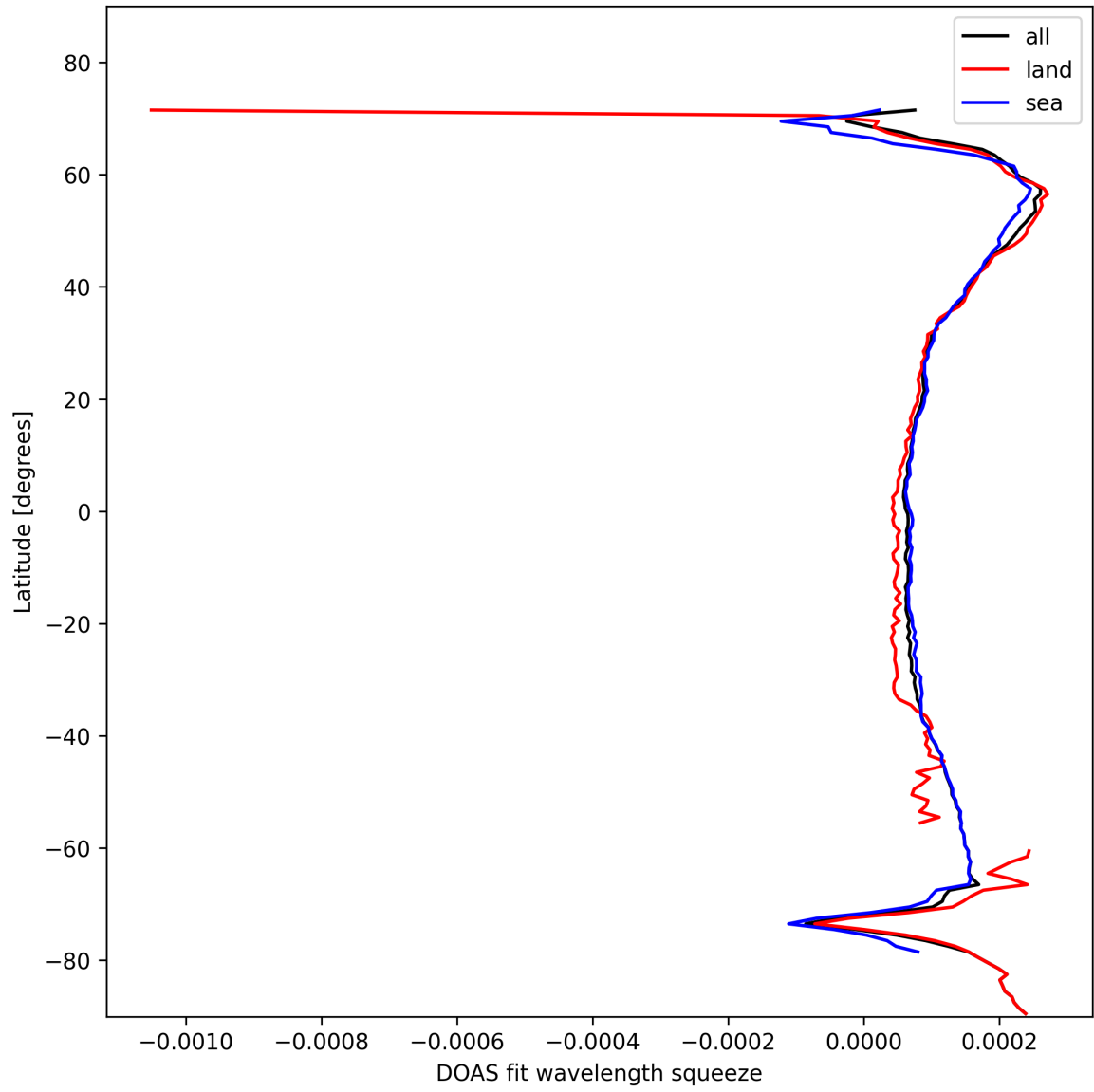
Figure 24: Zonal average of “DOAS fit wavelength squeeze” for 2025-01-28 to 2025-01-29.
