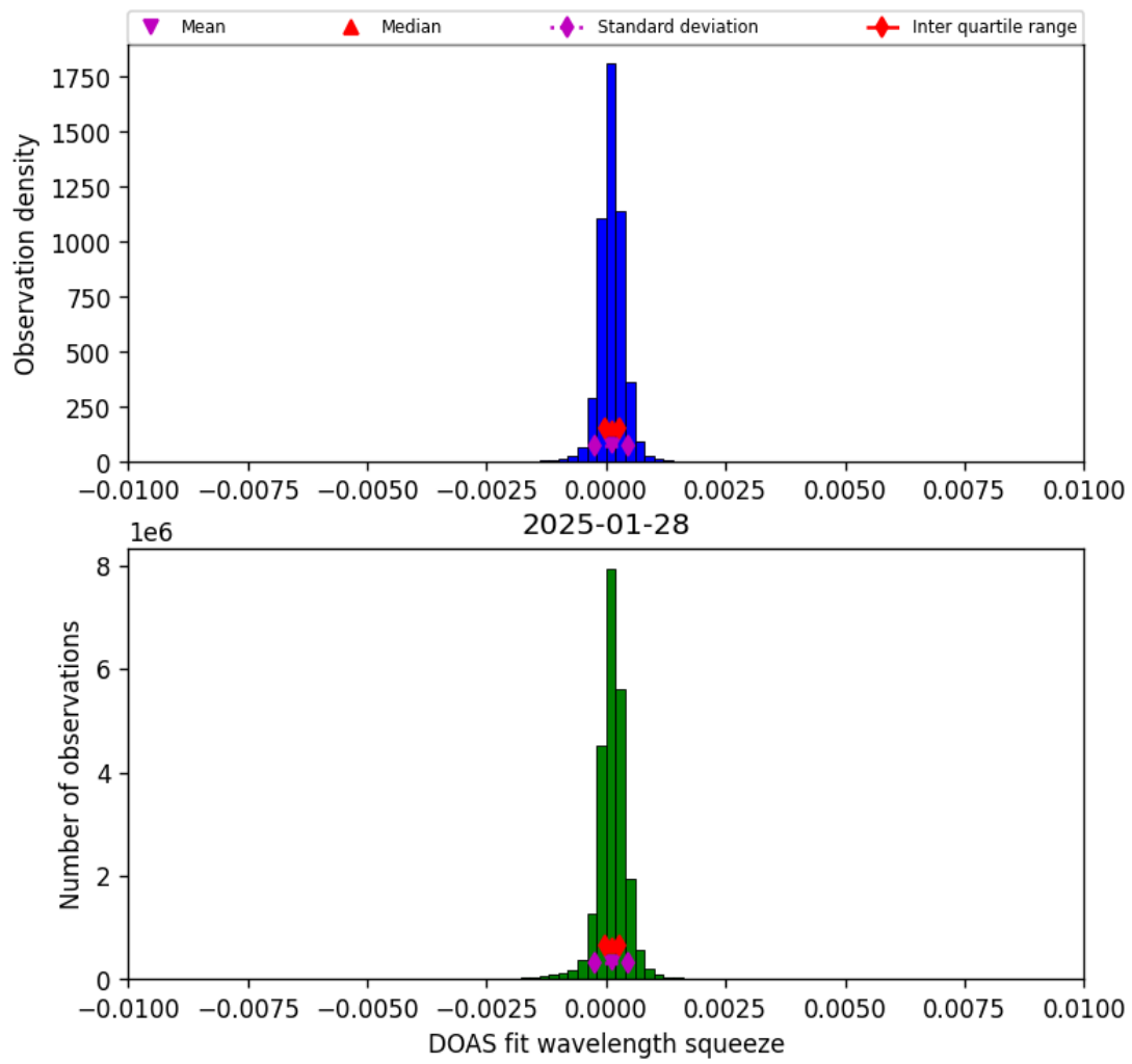
Figure 36: Histogram of “DOAS fit wavelength squeeze” for 2025-01-28 to 2025-01-29
