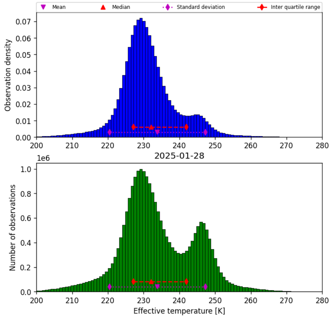
Figure 38: Histogram of “Effective temperature” for 2025-01-28 to 2025-01-29
