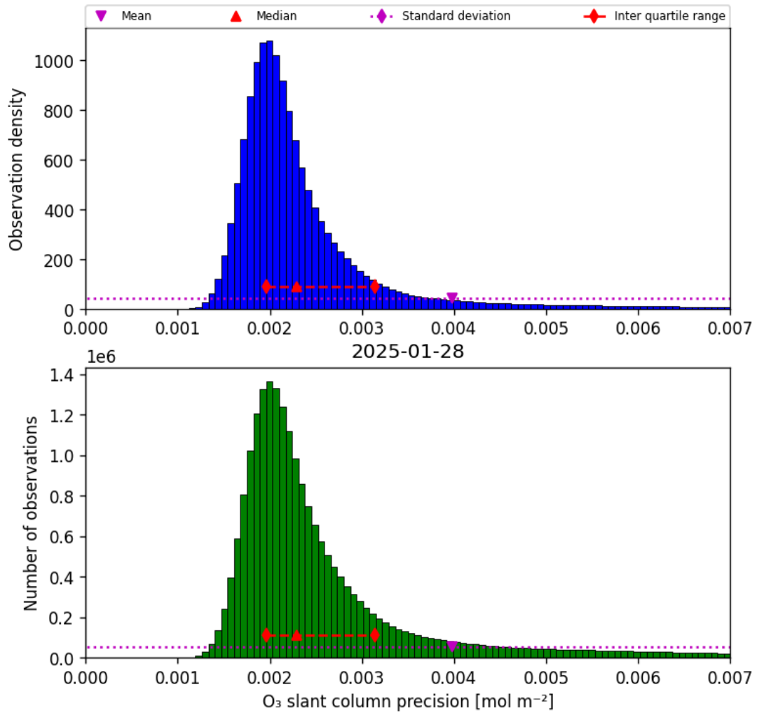
Figure 32: Histogram of “O 3 slant column precision” for 2025-01-28 to 2025-01-29
