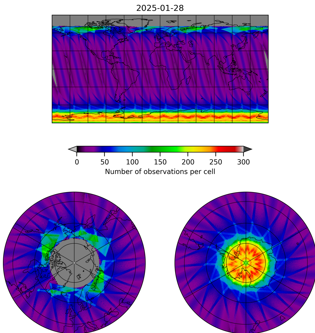
Figure 15: Map of the number of observations for 2025-01-28 to 2025-01-29
