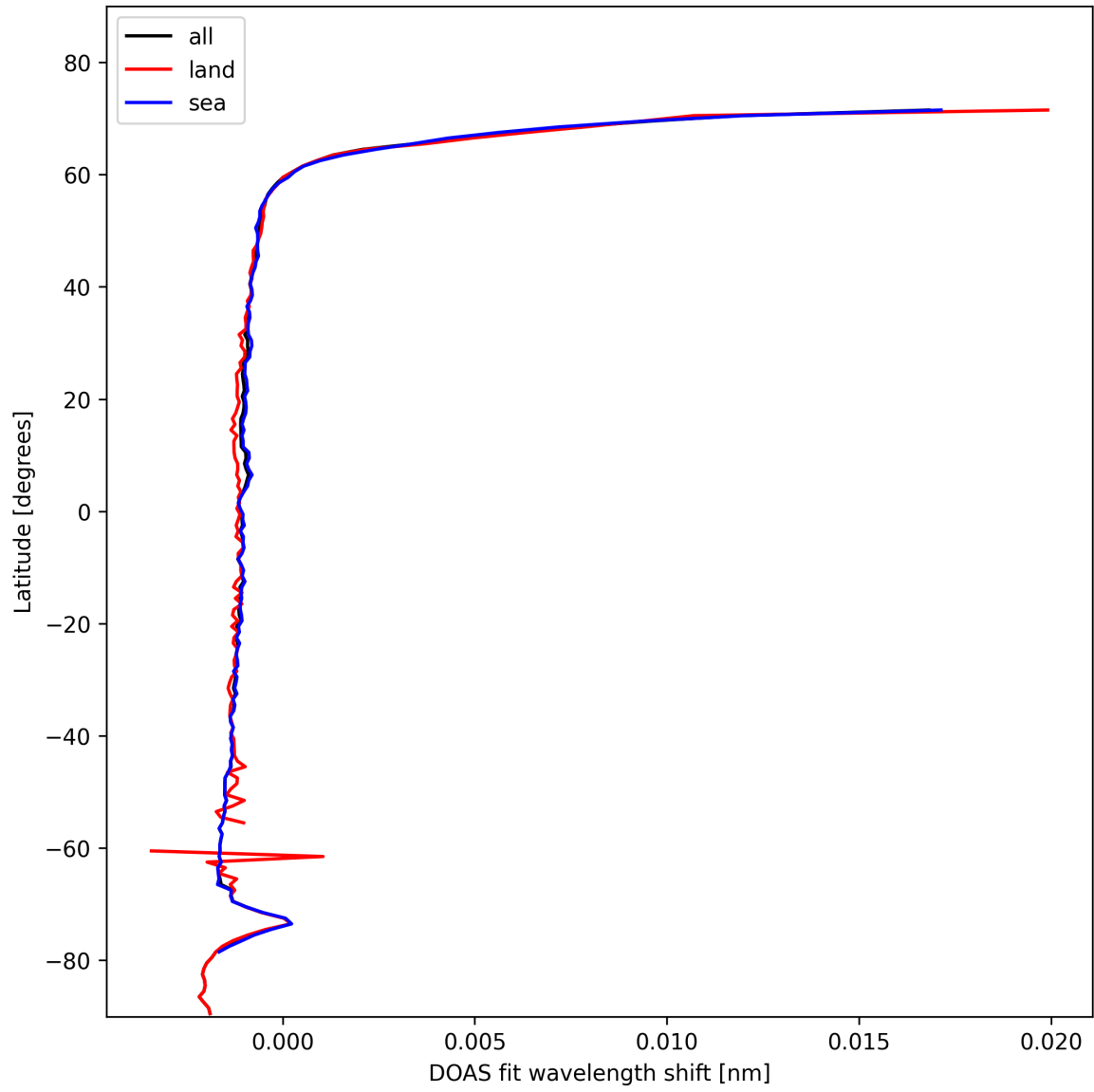
Figure 23: Zonal average of “DOAS fit wavelength shift” for 2025-01-28 to 2025-01-29.
