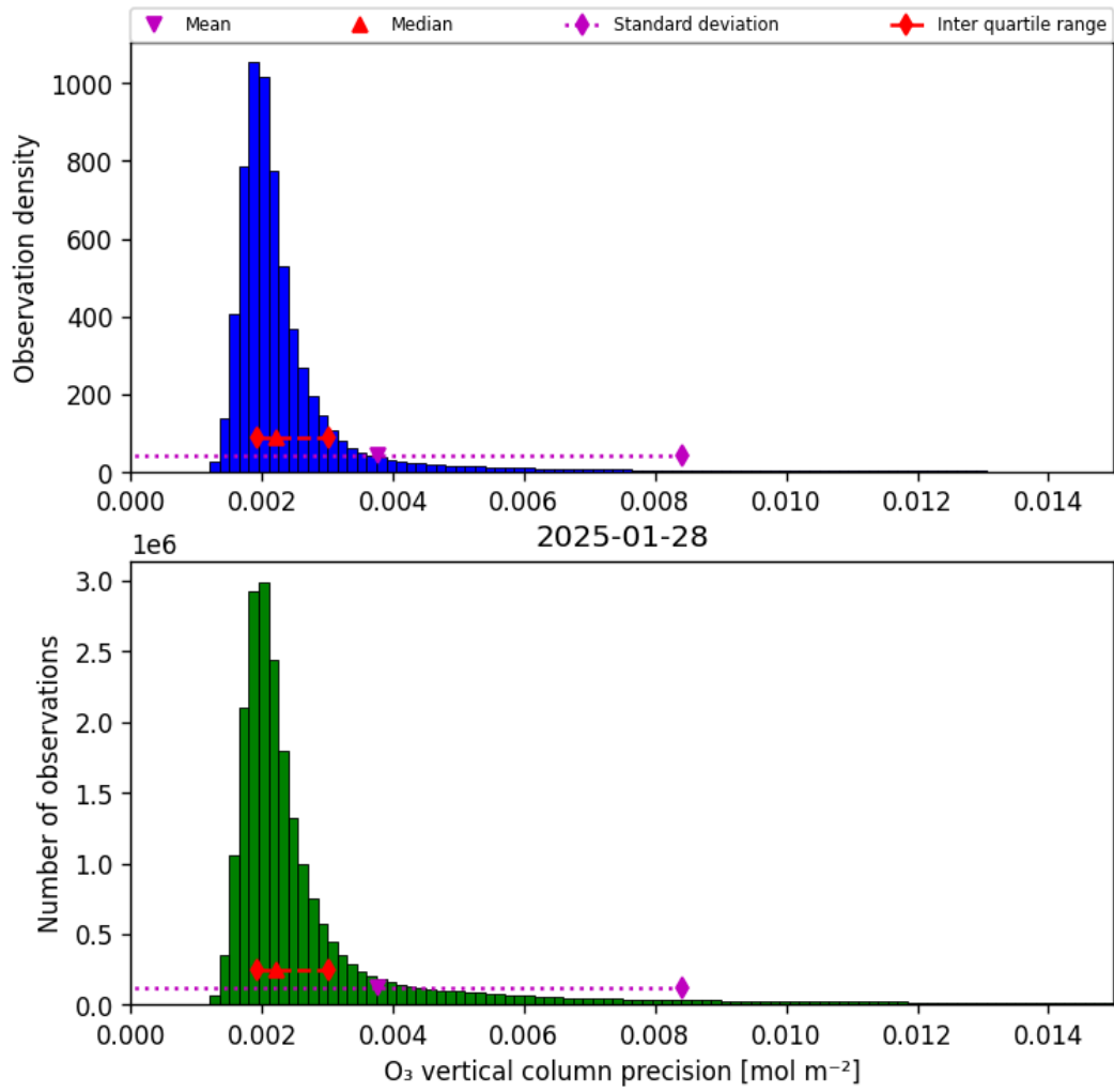
Figure 30: Histogram of “O 3 vertical column precision” for 2025-01-28 to 2025-01-29
