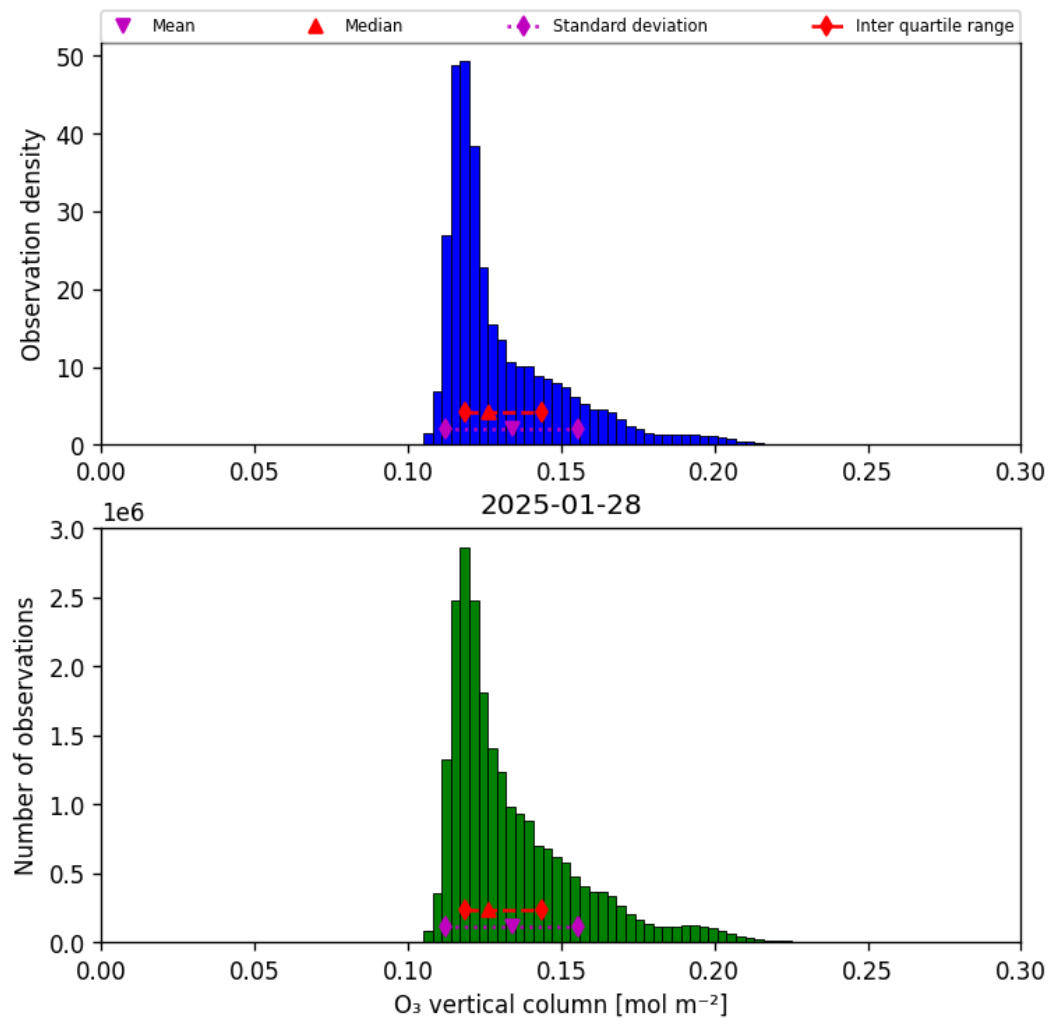
Figure 29: Histogram of “O 3 vertical column” for 2025-01-28 to 2025-01-29
