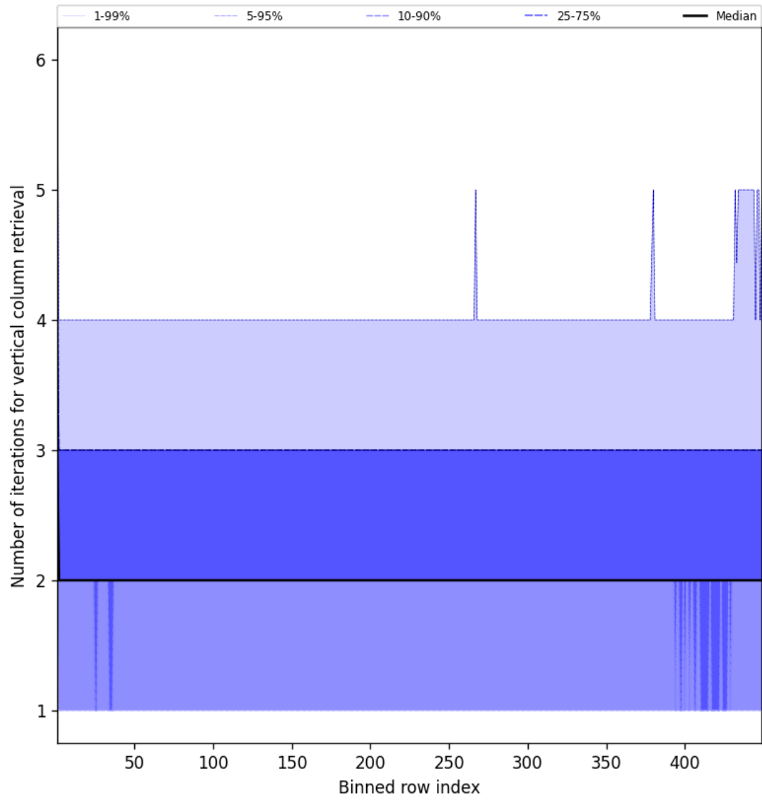
Figure 51: Along track statistics of “Number of iterations for vertical column retrieval” for 2025-01-28 to 2025-01-29
