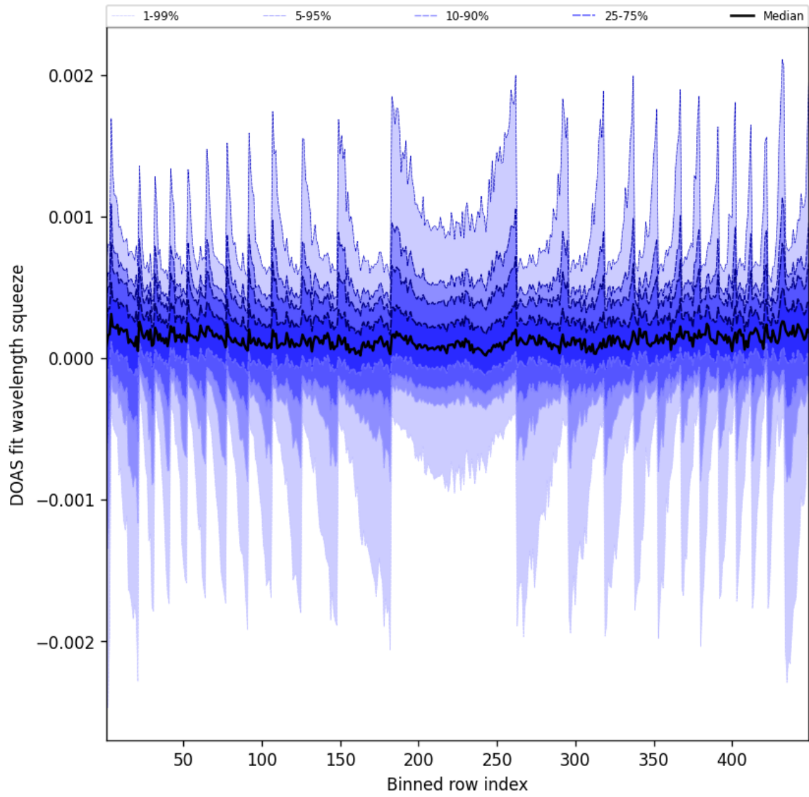
Figure 48: Along track statistics of “DOAS fit wavelength squeeze” for 2025-01-28 to 2025-01-29
