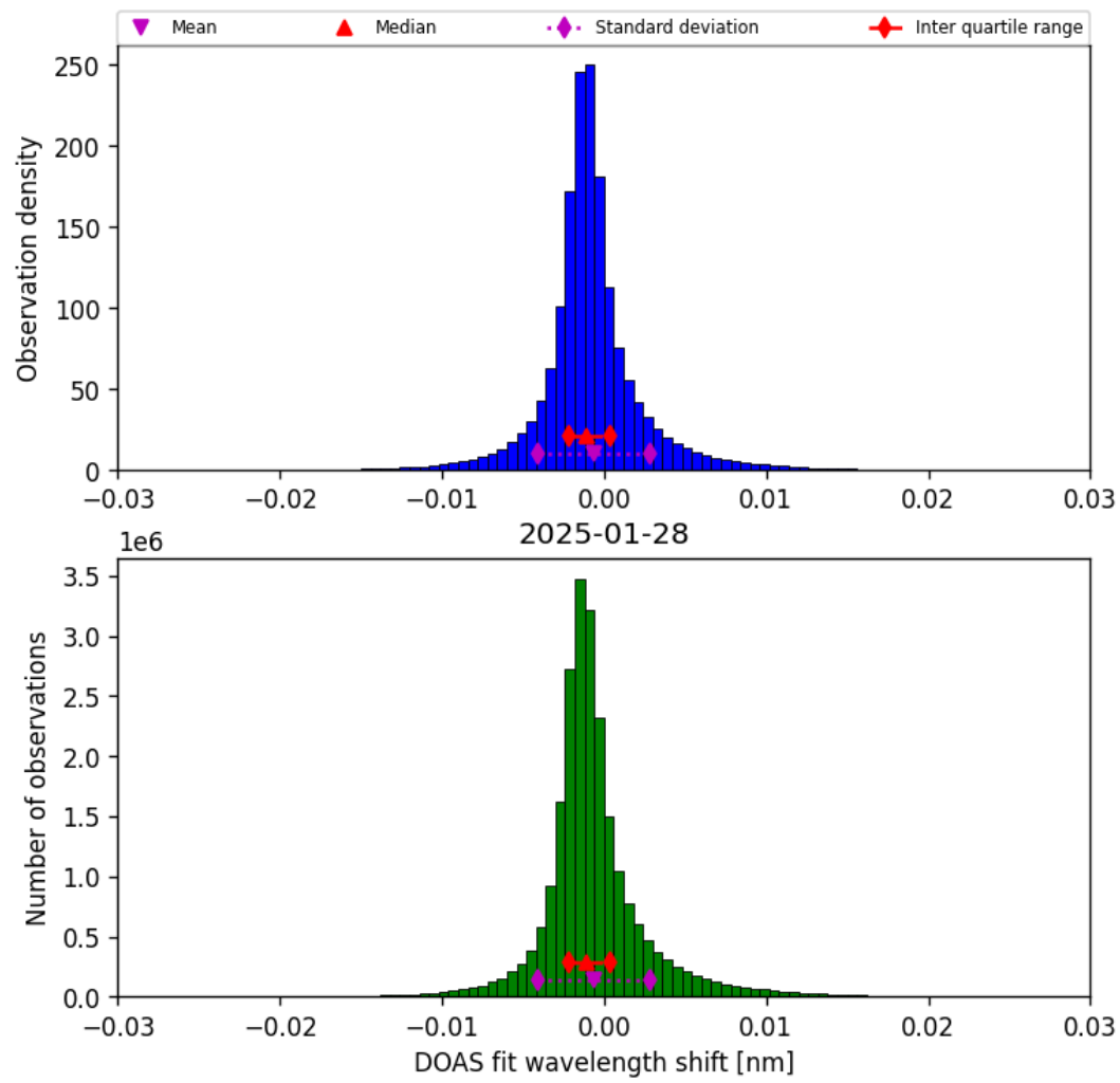
Figure 35: Histogram of “DOAS fit wavelength shift” for 2025-01-28 to 2025-01-29
