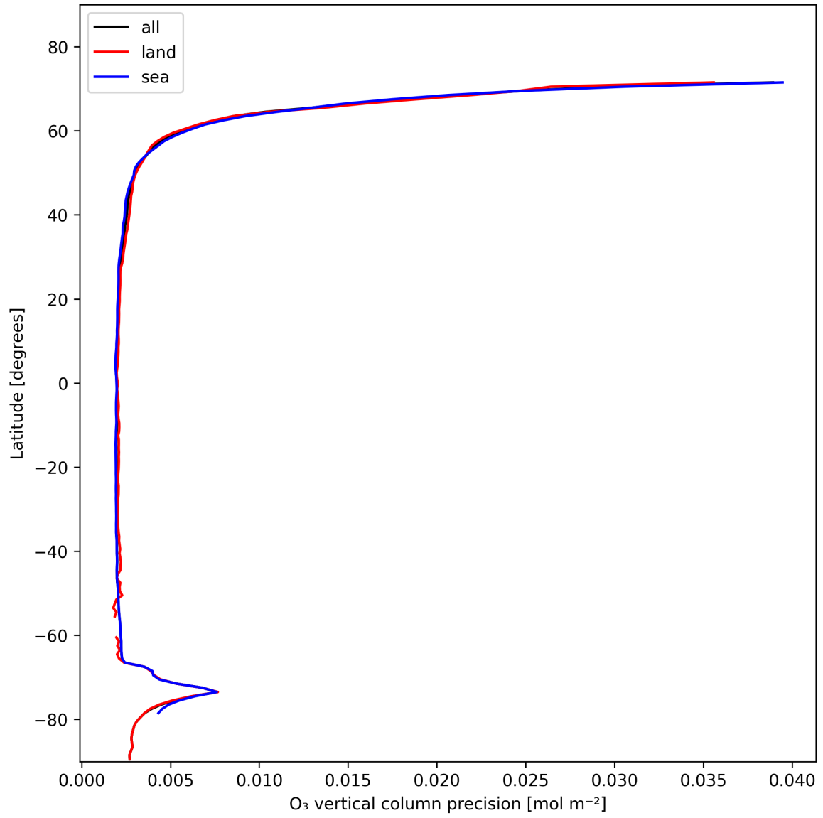
Figure 18: Zonal average of "O 3 vertical column precision" for 2025-01-28 to 2025-01-29.
