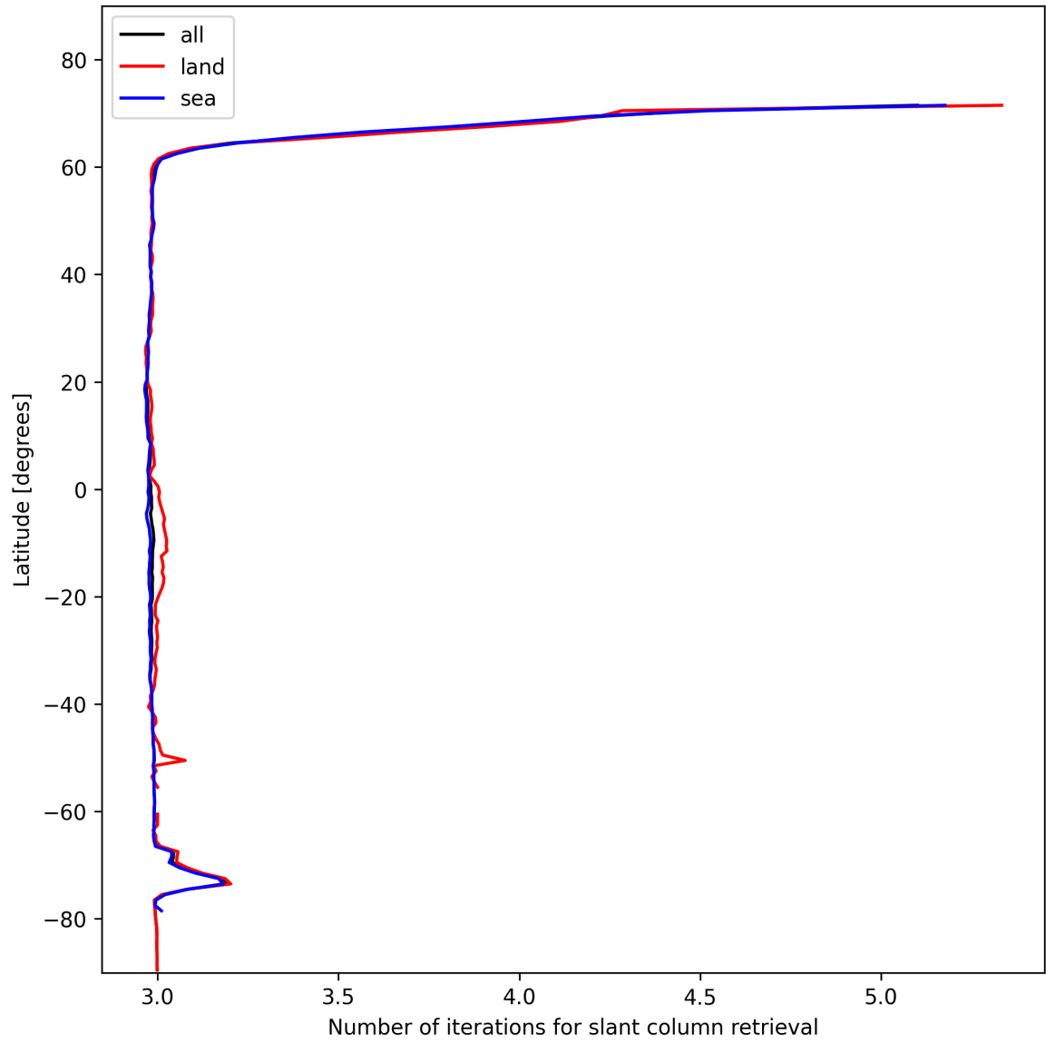
Figure 21: Zonal average of “Number of iterations for slant column retrieval” for 2025-01-28 to 2025-01-29.
