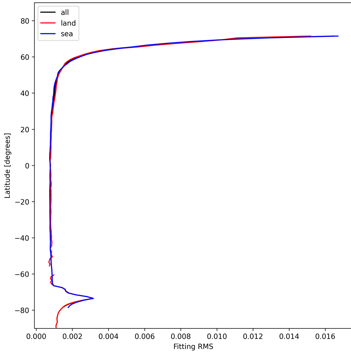
Figure 22: Zonal average of “Fitting RMS” for 2025-01-28 to 2025-01-29.
