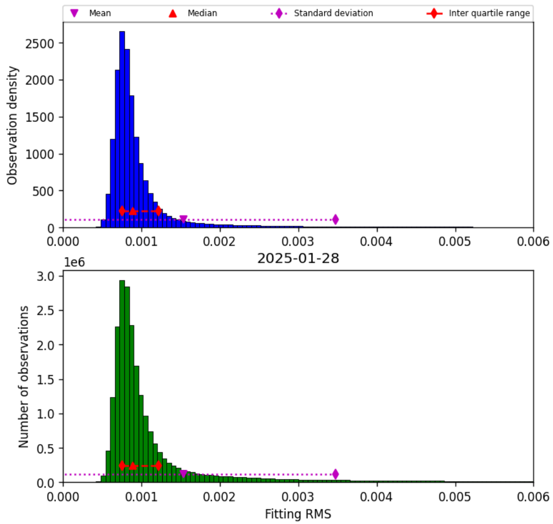
Figure 34: Histogram of “Fitting RMS” for 2025-01-28 to 2025-01-29
