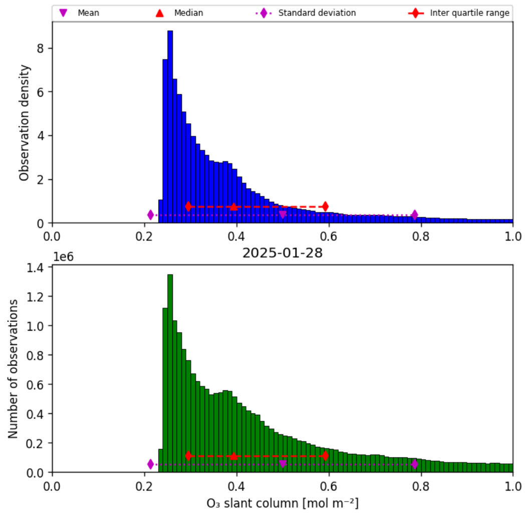
Figure 31: Histogram of “O 3 slant column” for 2025-01-28 to 2025-01-29
