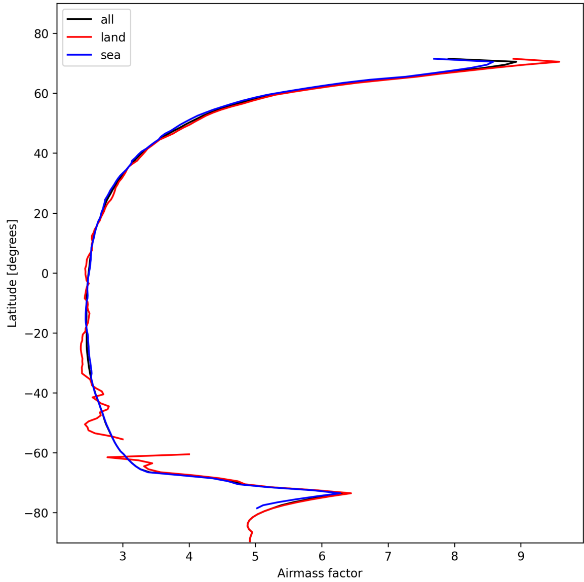
Figure 25: Zonal average of “Airmass factor” for 2025-01-28 to 2025-01-29.
