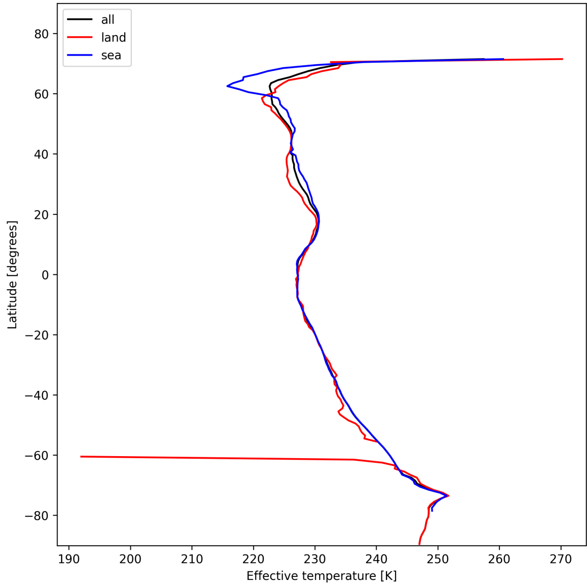
Figure 26: Zonal average of “Effective temperature” for 2025-01-28 to 2025-01-29.
