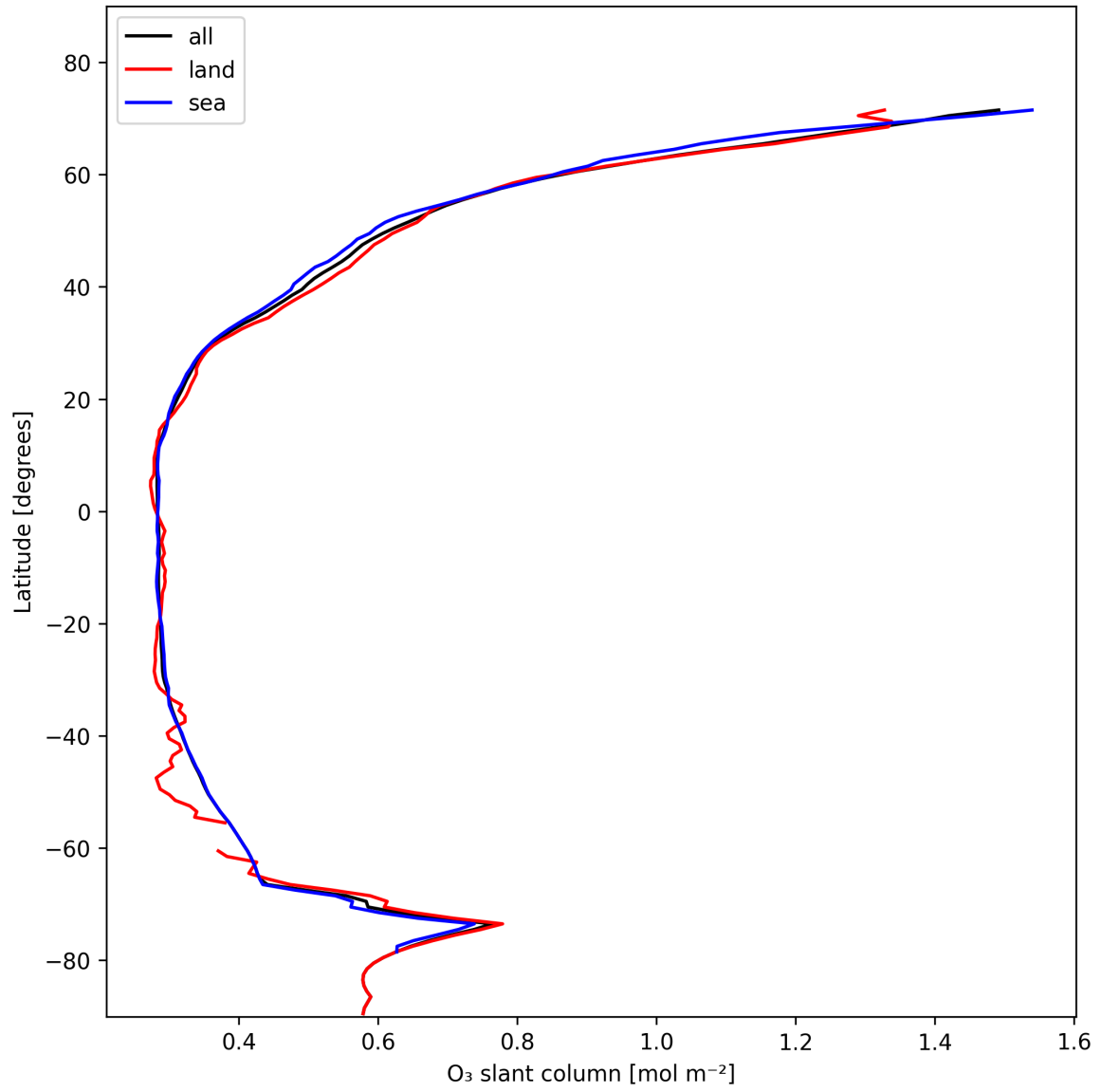
Figure 19: Zonal average of “O 3 slant column” for 2025-01-29 to 2025-01-30.
