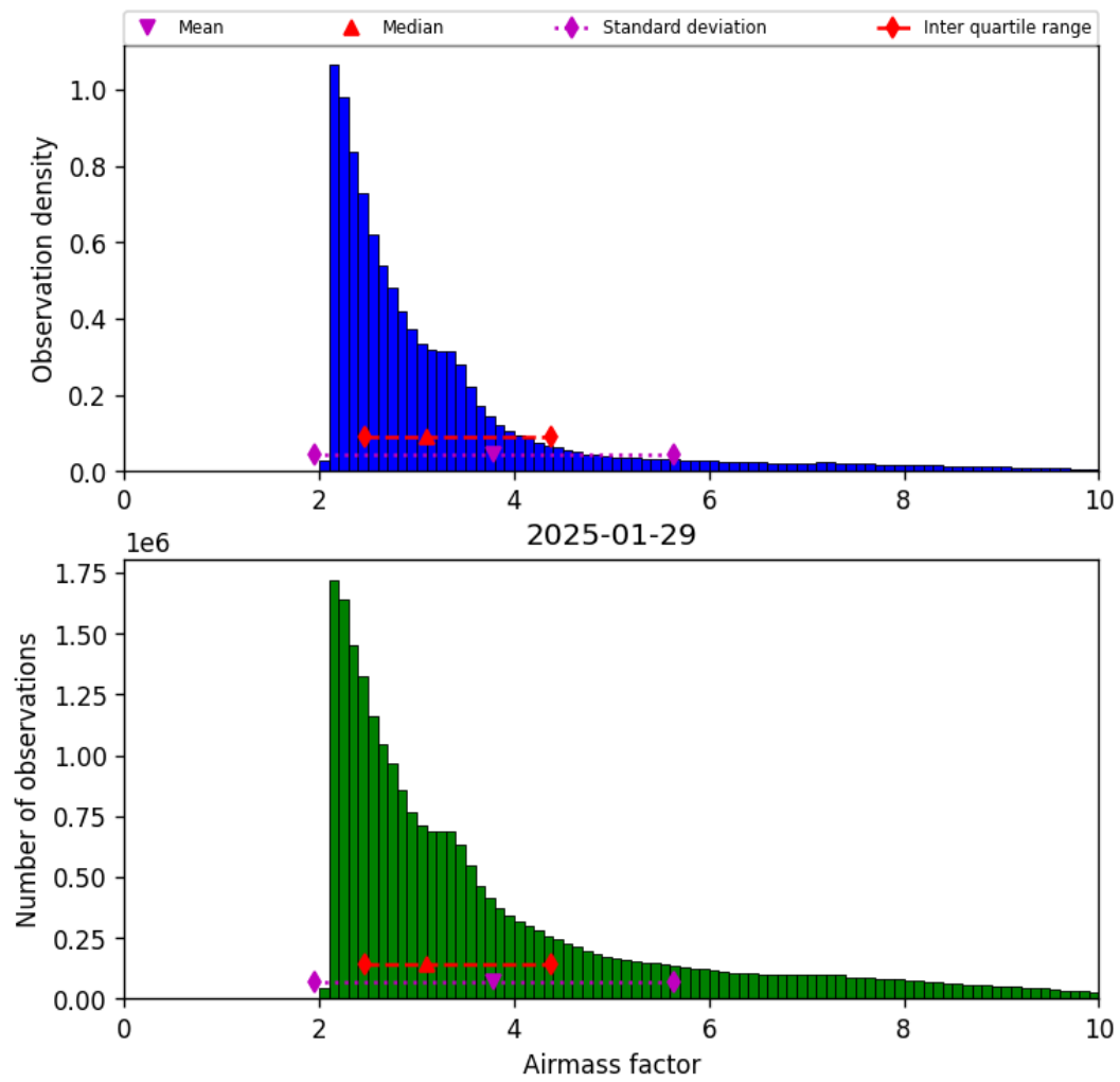
Figure 37: Histogram of “Airmass factor” for 2025-01-29 to 2025-01-30
