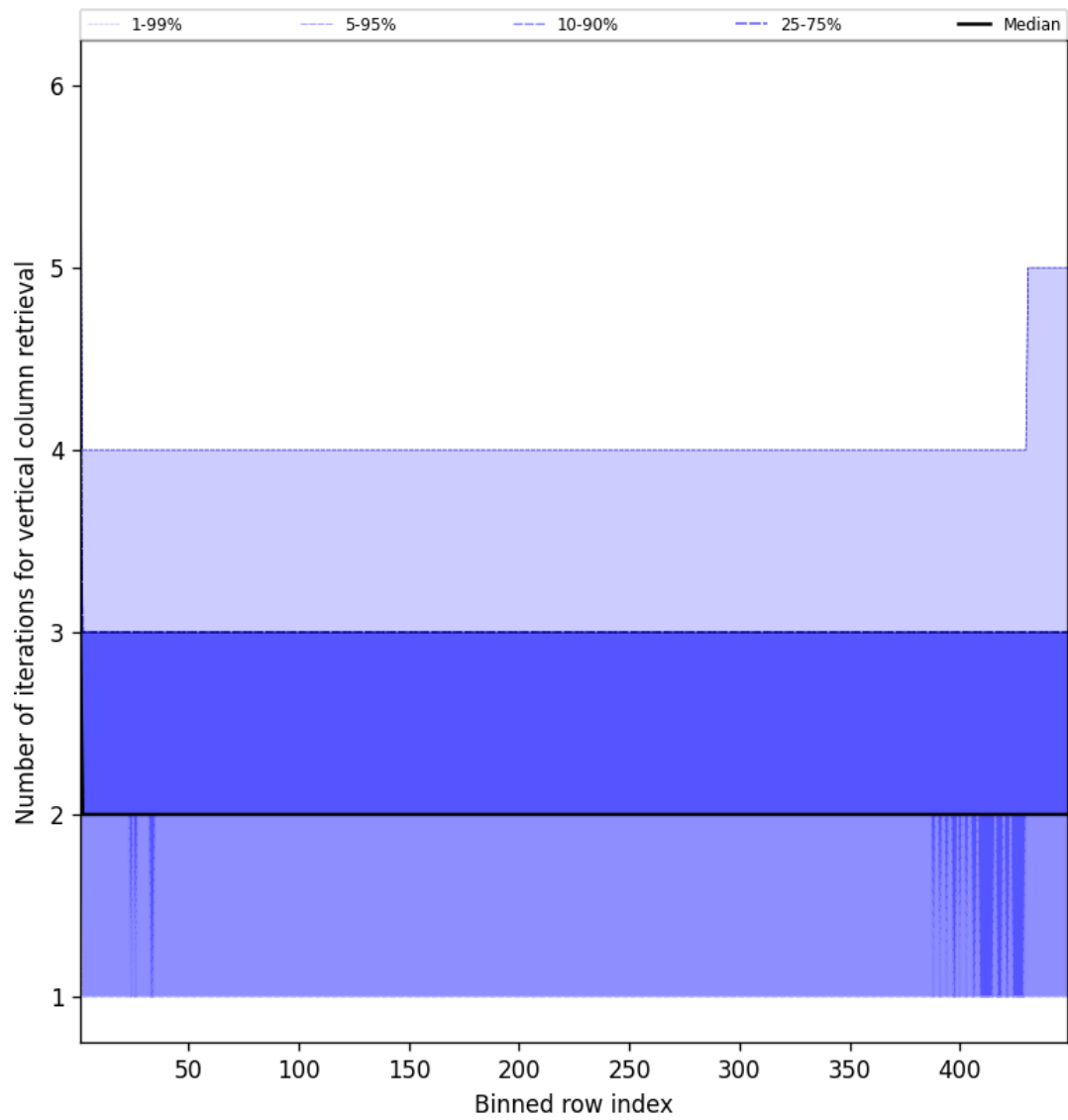
Figure 51: Along track statistics of “Number of iterations for vertical column retrieval” for 2025-01-29 to 2025-01-30
