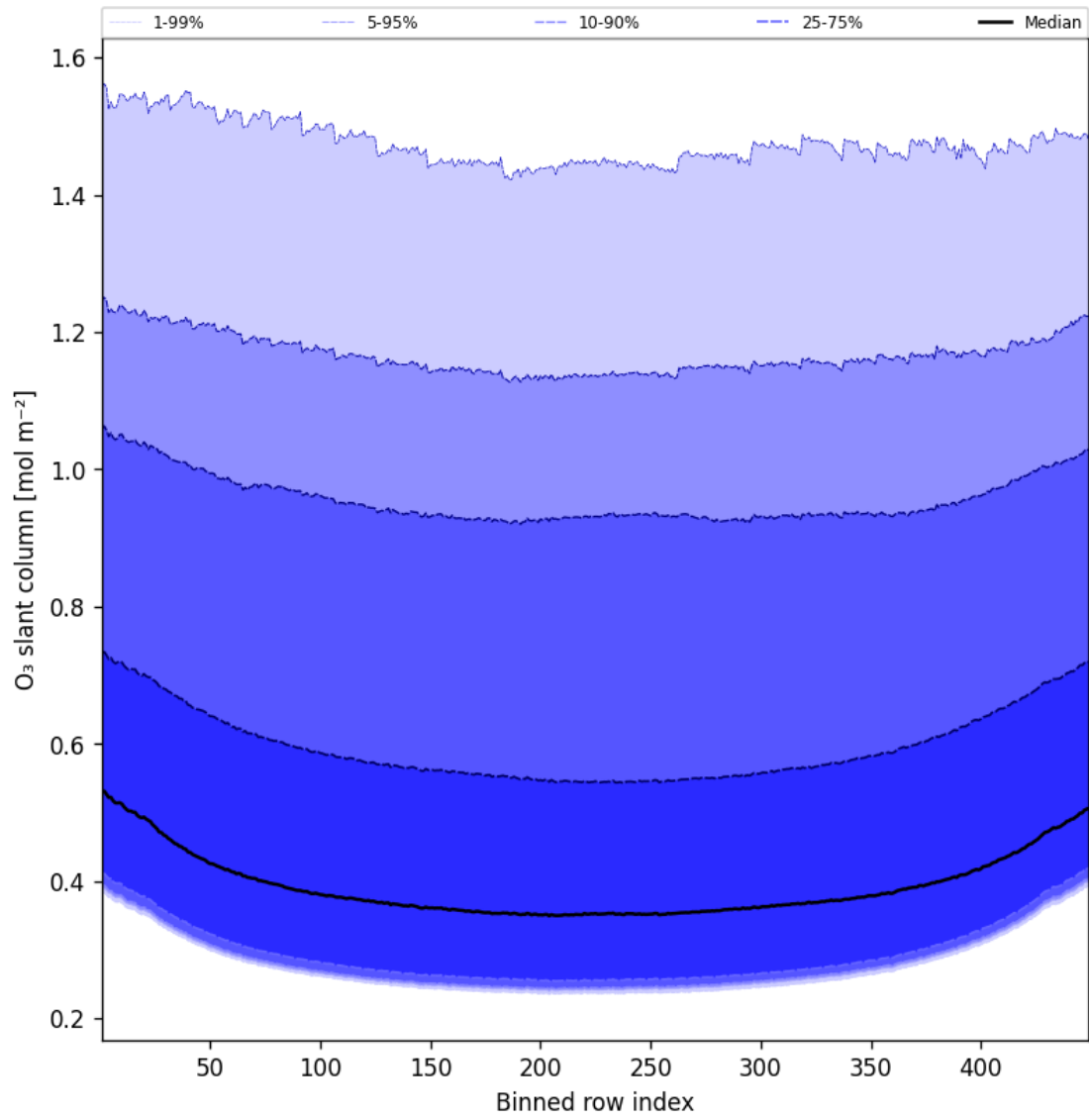
Figure 43: Along track statistics of “O 3 slant column” for 2025-01-29 to 2025-01-30
