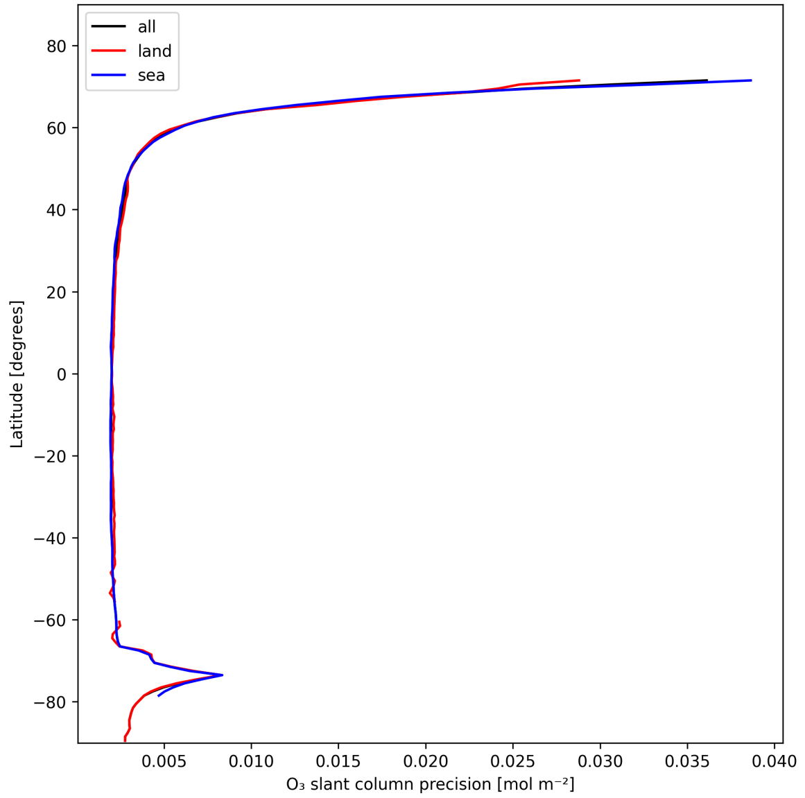
Figure 20: Zonal average of “O 3 slant column precision” for 2025-01-29 to 2025-01-30.
