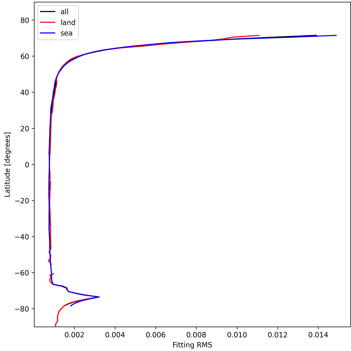
Figure 22: Zonal average of “Fitting RMS” for 2025-01-29 to 2025-01-30.
