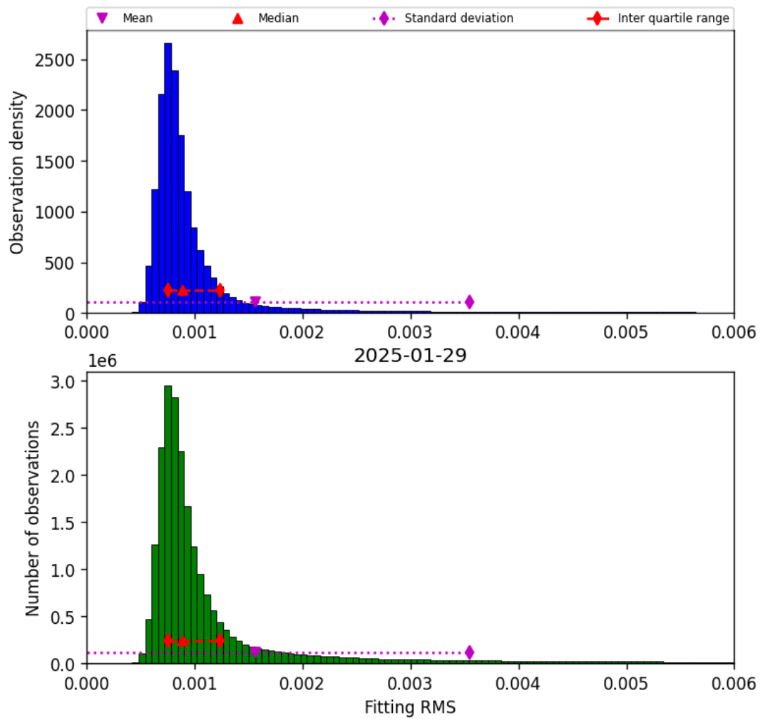
Figure 34: Histogram of “Fitting RMS” for 2025-01-29 to 2025-01-30
