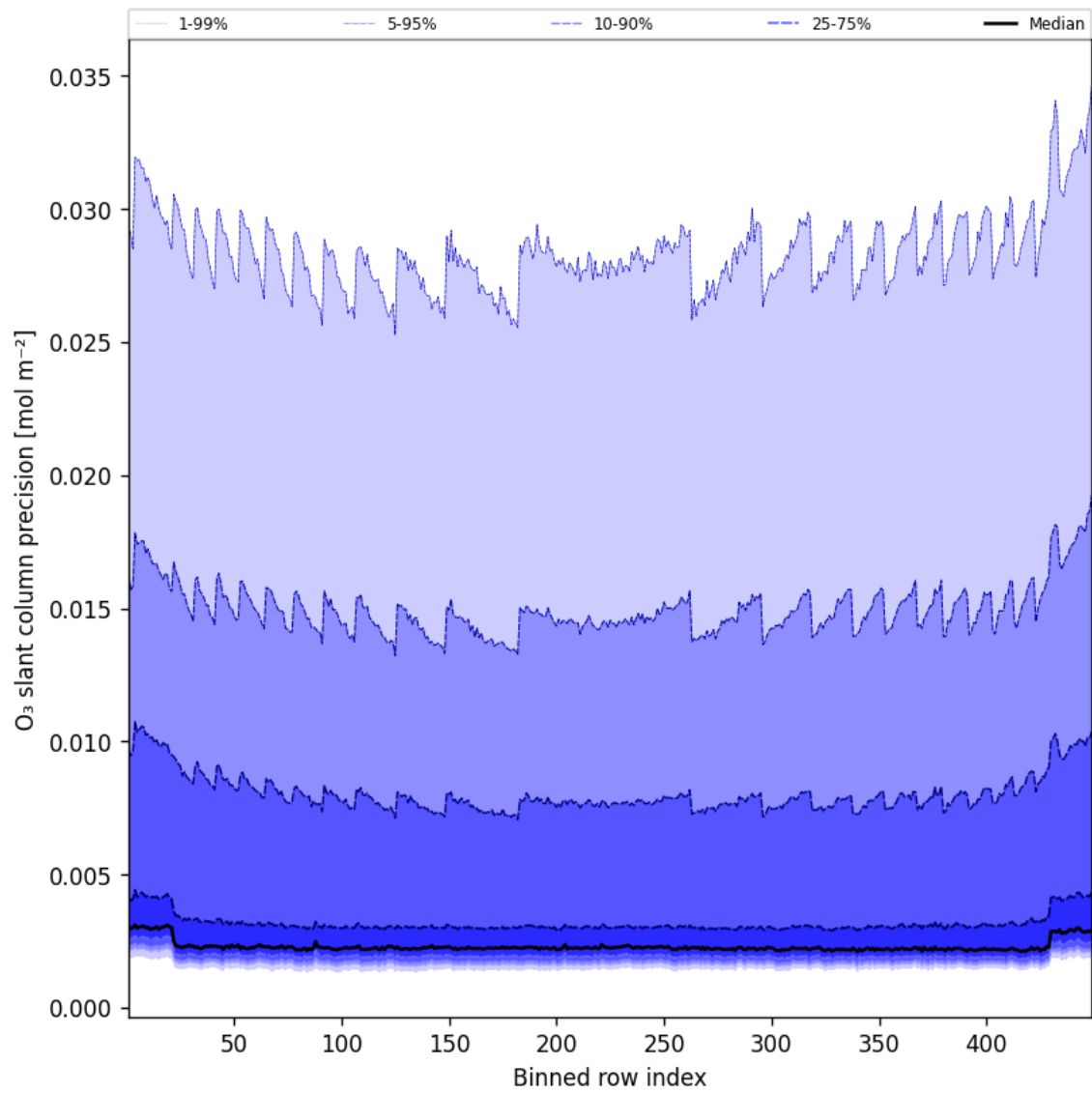
Figure 44: Along track statistics of “O 3 slant column precision” for 2025-01-29 to 2025-01-30
