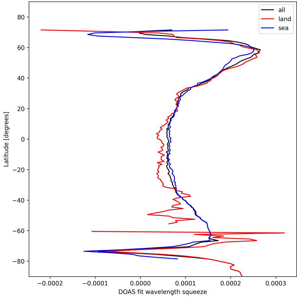
Figure 24: Zonal average of “DOAS fit wavelength squeeze” for 2025-01-29 to 2025-01-30.
