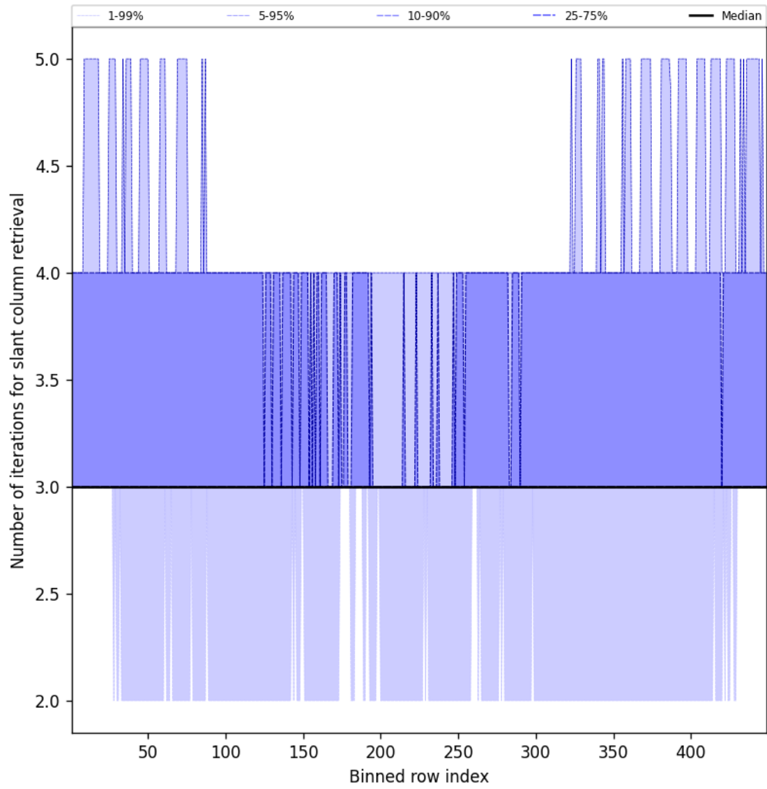
Figure 45: Along track statistics of “Number of iterations for slant column retrieval” for 2025-01-29 to 2025-01-30
