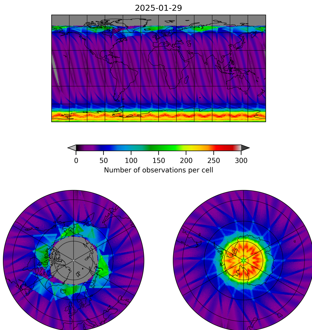
Figure 15: Map of the number of observations for 2025-01-29 to 2025-01-30
