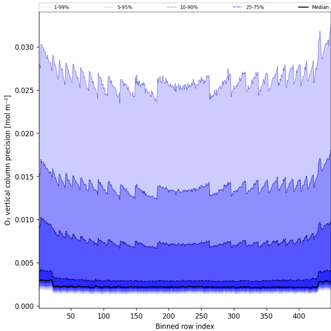
Figure 42: Along track statistics of “O 3 vertical column precision” for 2025-01-29 to 2025-01-30
