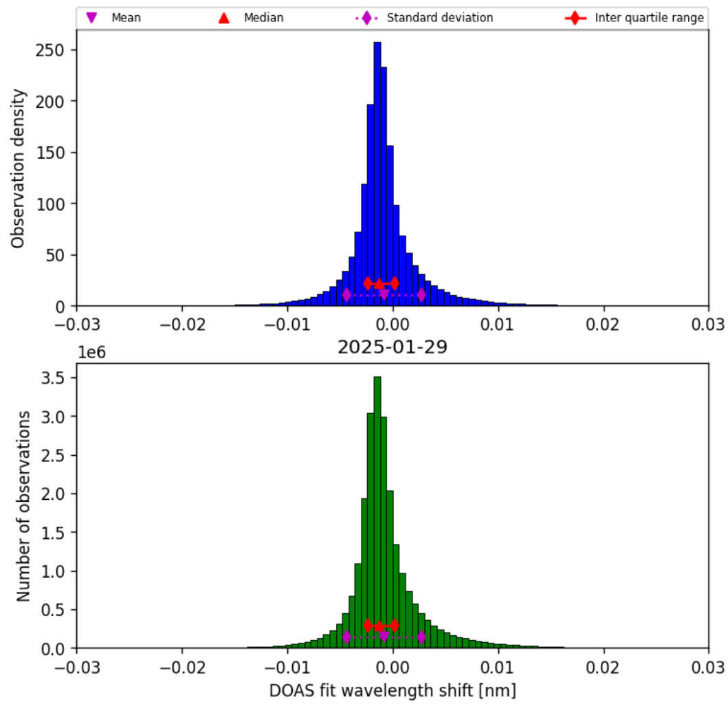
Figure 35: Histogram of “DOAS fit wavelength shift” for 2025-01-29 to 2025-01-30
