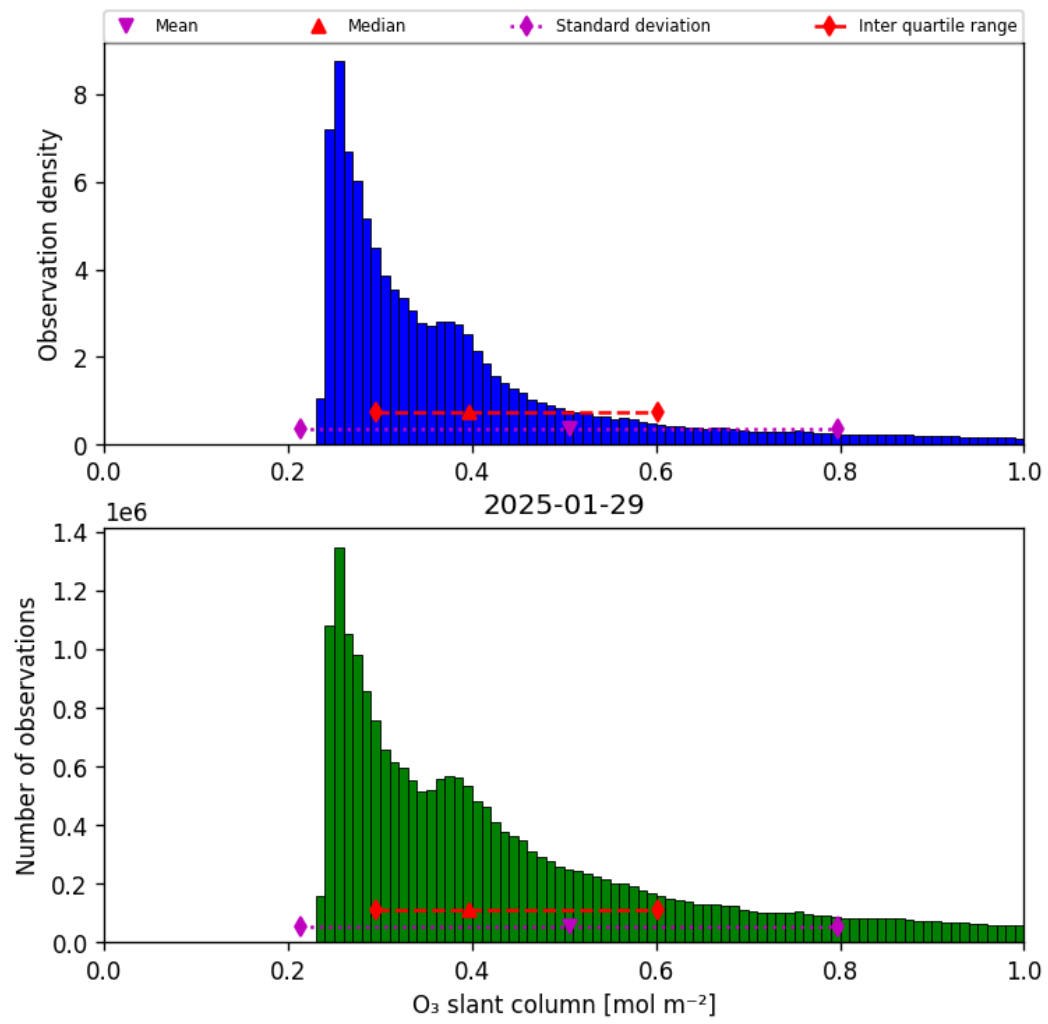
Figure 31: Histogram of “O 3 slant column” for 2025-01-29 to 2025-01-30
