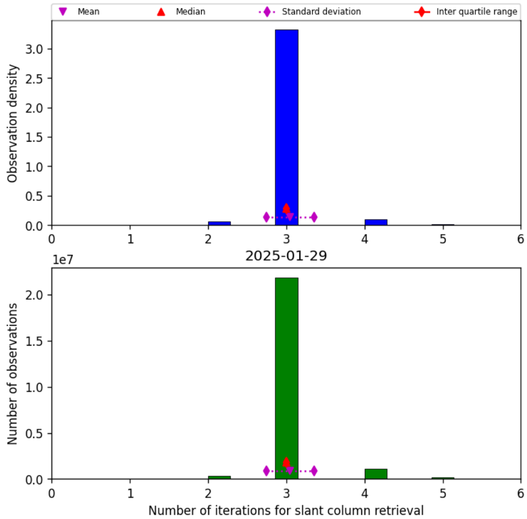
Figure 33: Histogram of "Number of iterations for slant column retrieval" for 2025-01-29 to 2025-01-30
