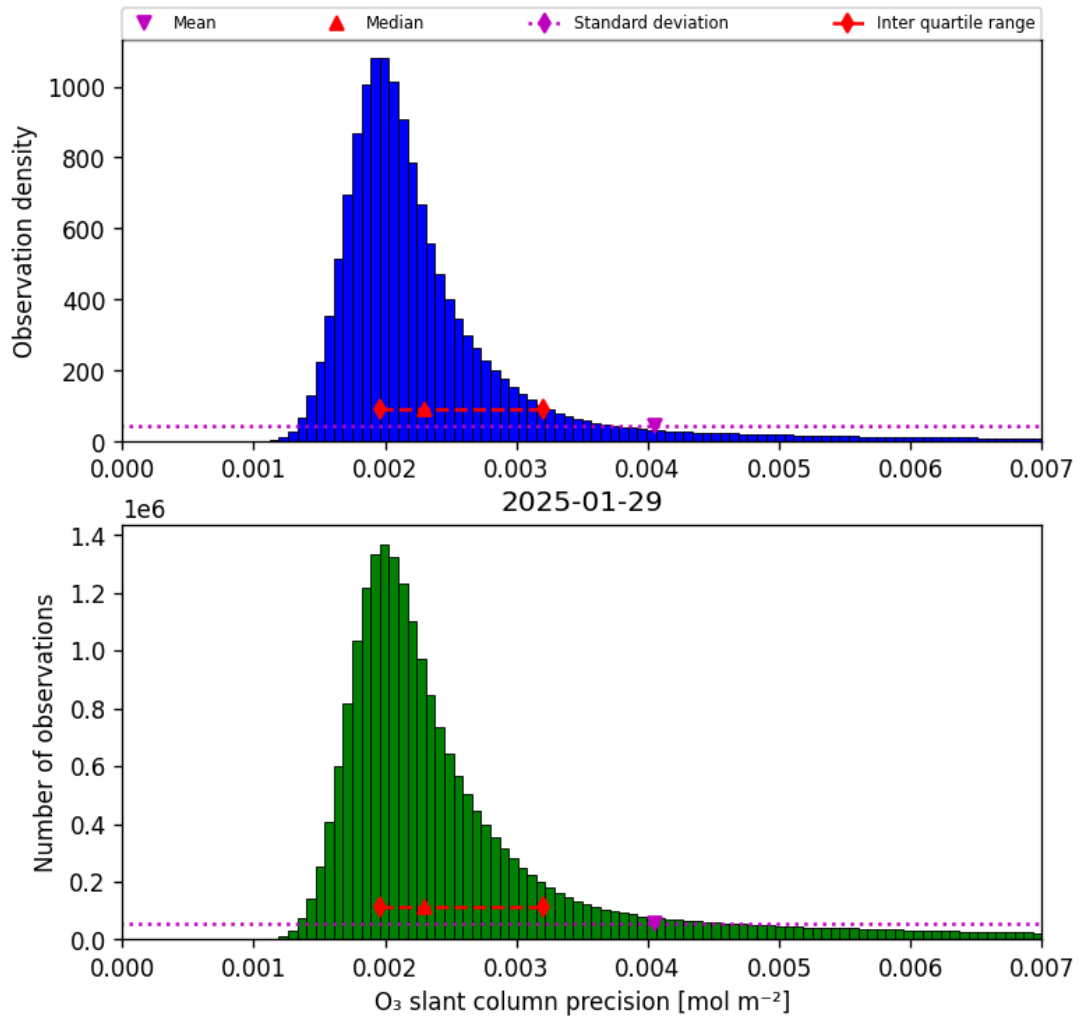
Figure 32: Histogram of “O 3 slant column precision” for 2025-01-29 to 2025-01-30
