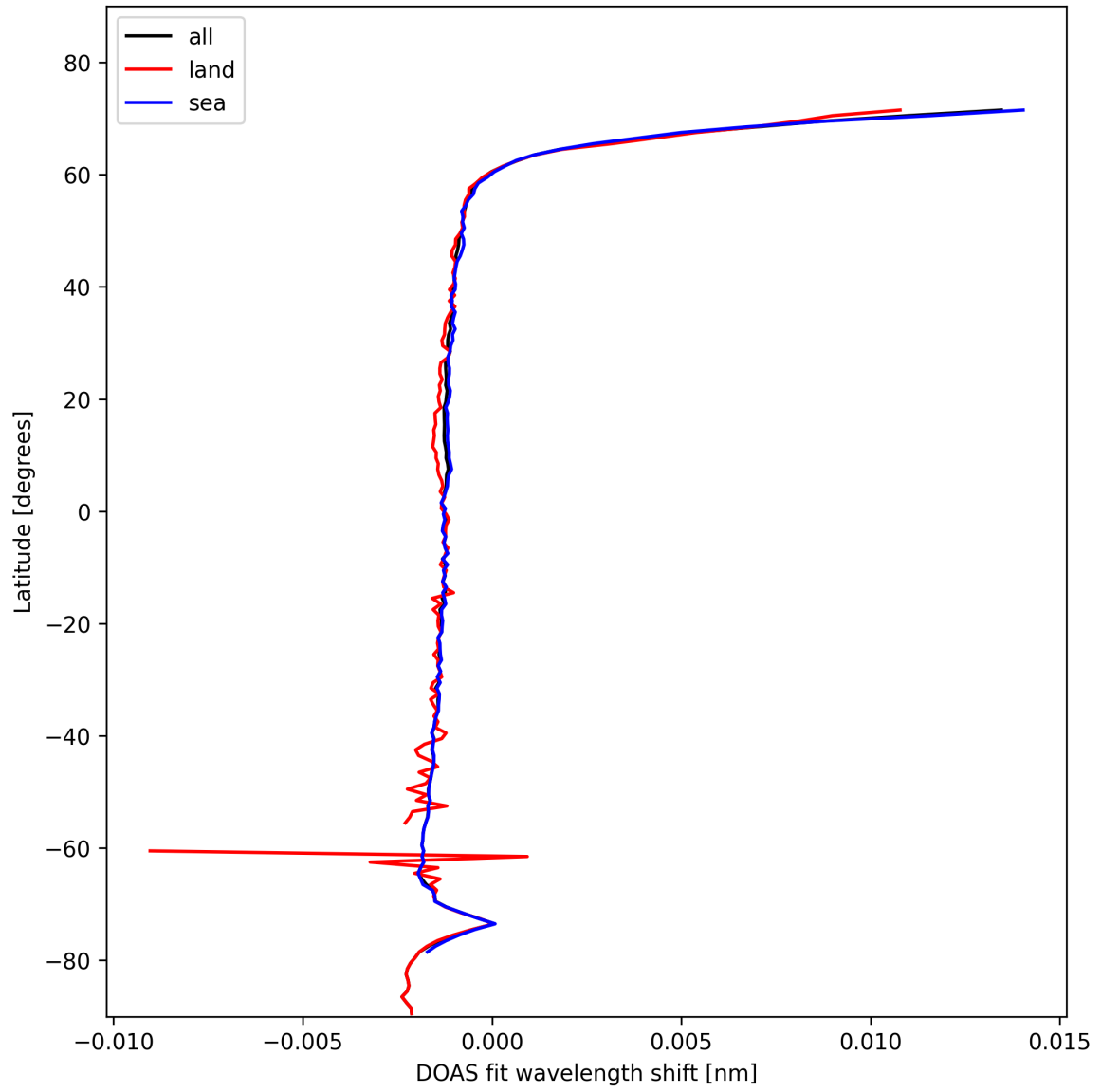
Figure 23: Zonal average of "DOAS fit wavelength shift" for 2025-01-29 to 2025-01-30.
