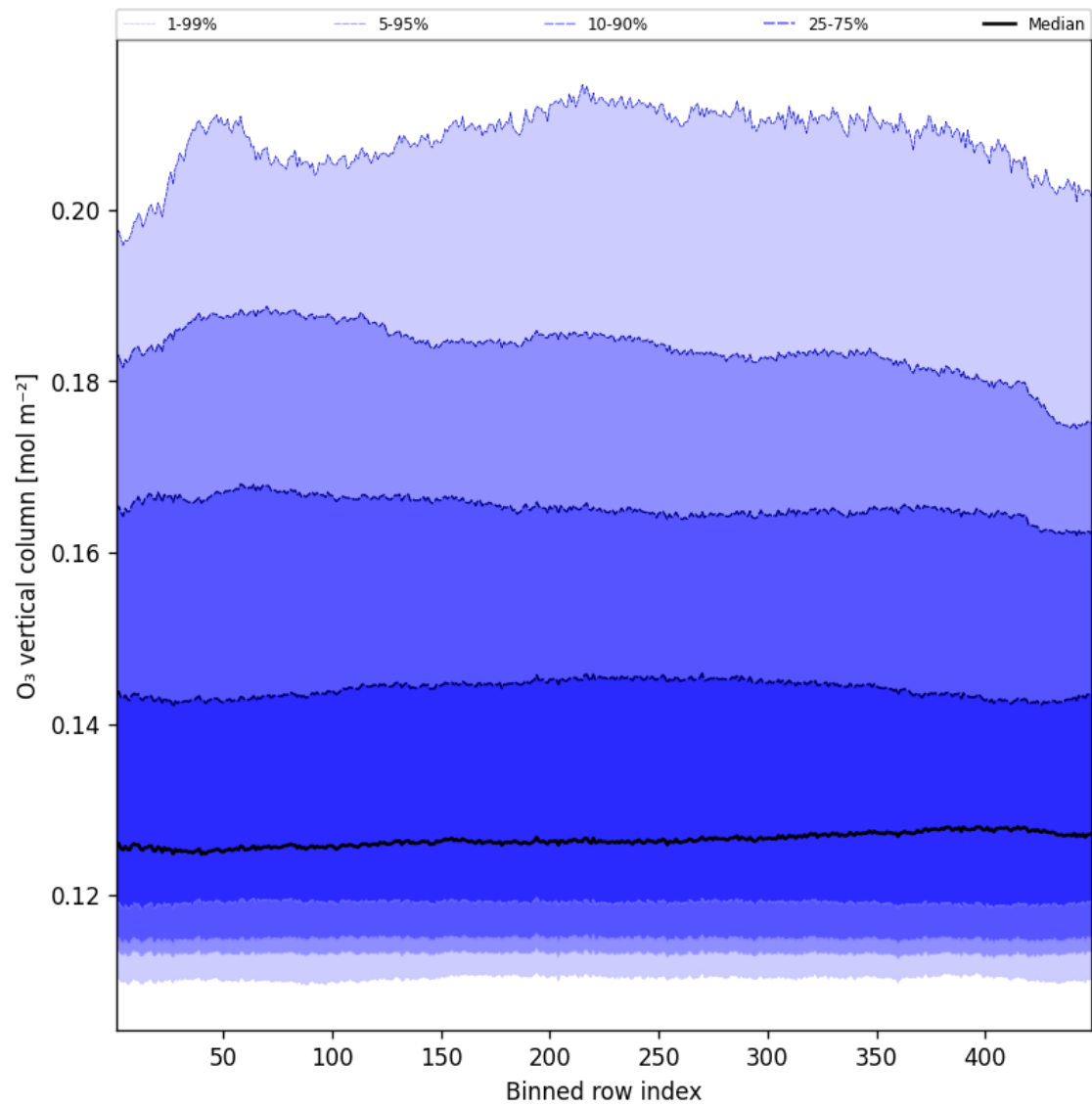
Figure 41: Along track statistics of “O 3 vertical column” for 2025-01-29 to 2025-01-30
