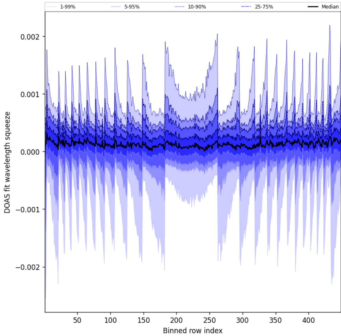
Figure 48: Along track statistics of “DOAS fit wavelength squeeze” for 2025-01-29 to 2025-01-30
