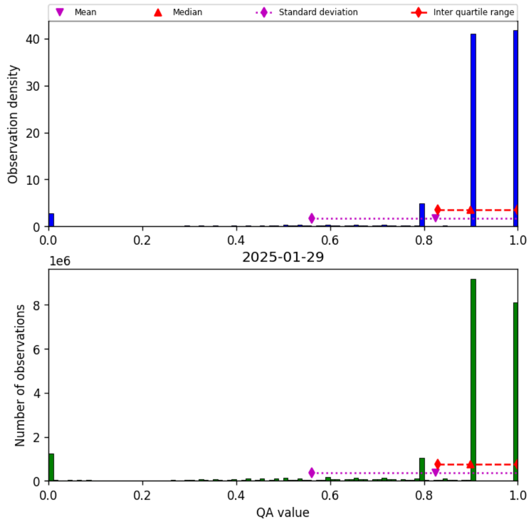
Figure 28: Histogram of “QA value” for 2025-01-29 to 2025-01-30
