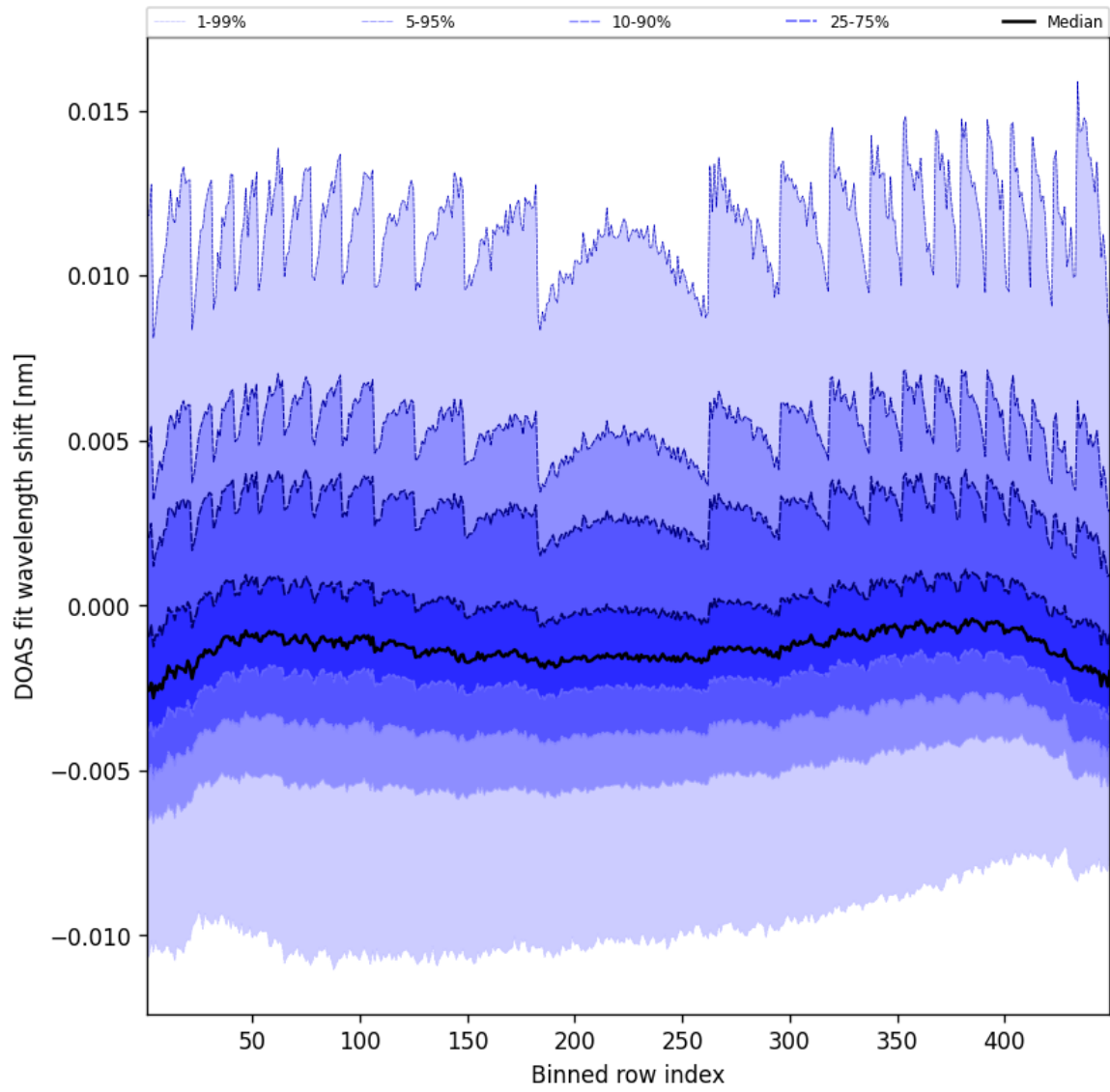
Figure 47: Along track statistics of “DOAS fit wavelength shift” for 2025-01-29 to 2025-01-30
