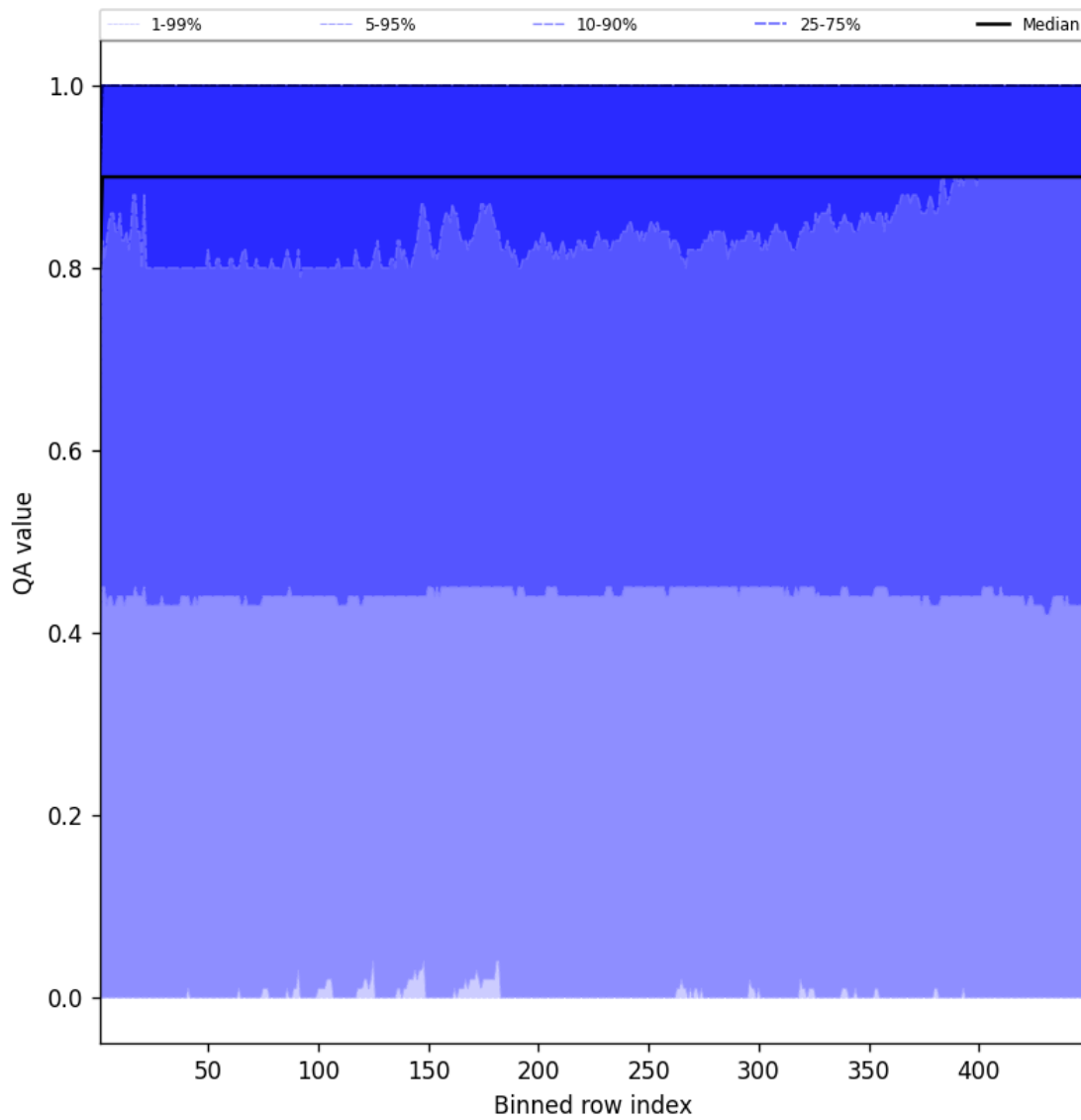
Figure 40: Along track statistics of “QA value” for 2025-01-29 to 2025-01-30
