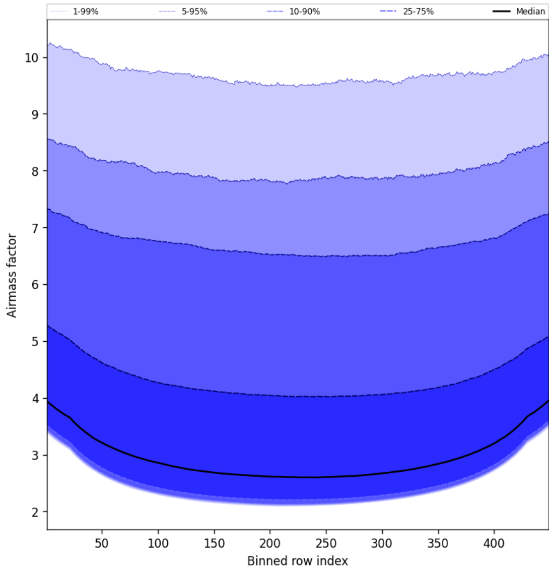
Figure 49: Along track statistics of “Airmass factor” for 2025-01-29 to 2025-01-30
