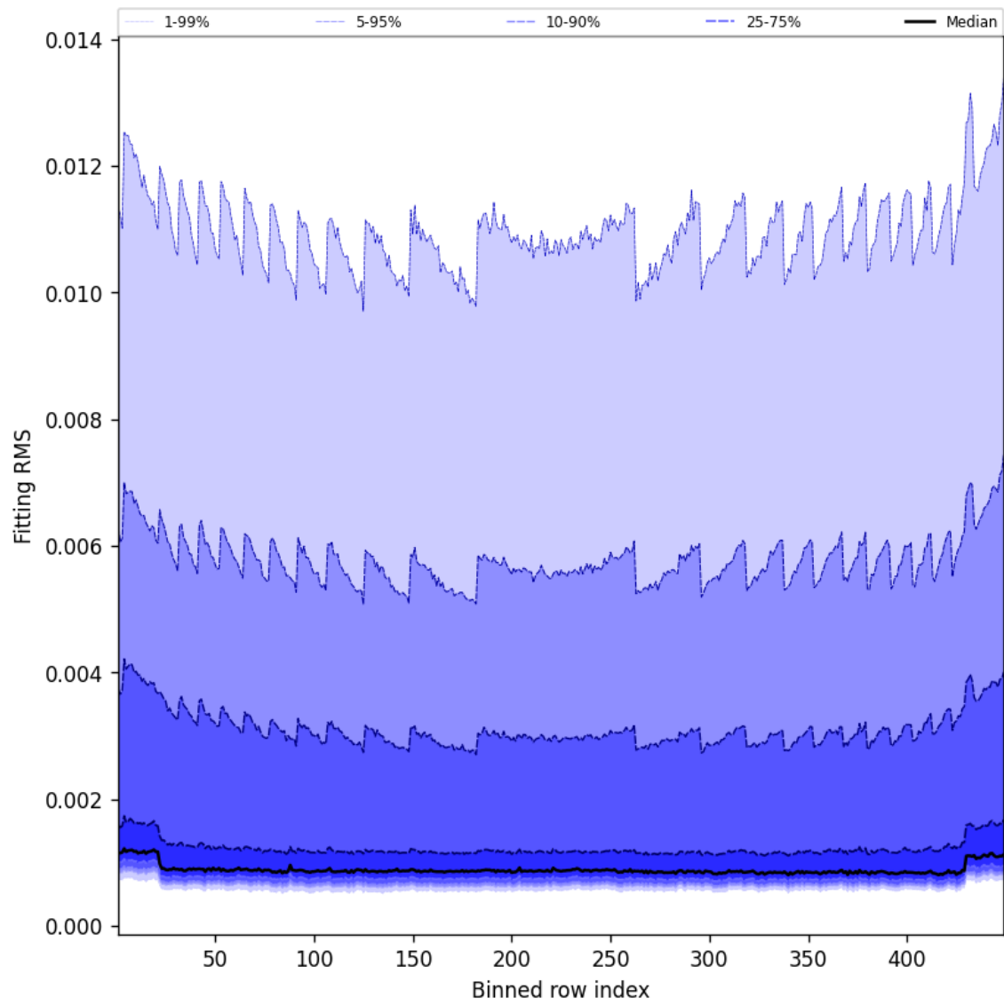
Figure 46: Along track statistics of “Fitting RMS” for 2025-01-29 to 2025-01-30
