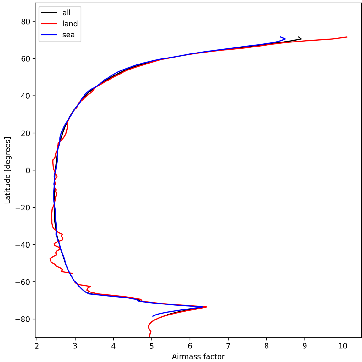
Figure 25: Zonal average of “Airmass factor” for 2025-01-29 to 2025-01-30.
