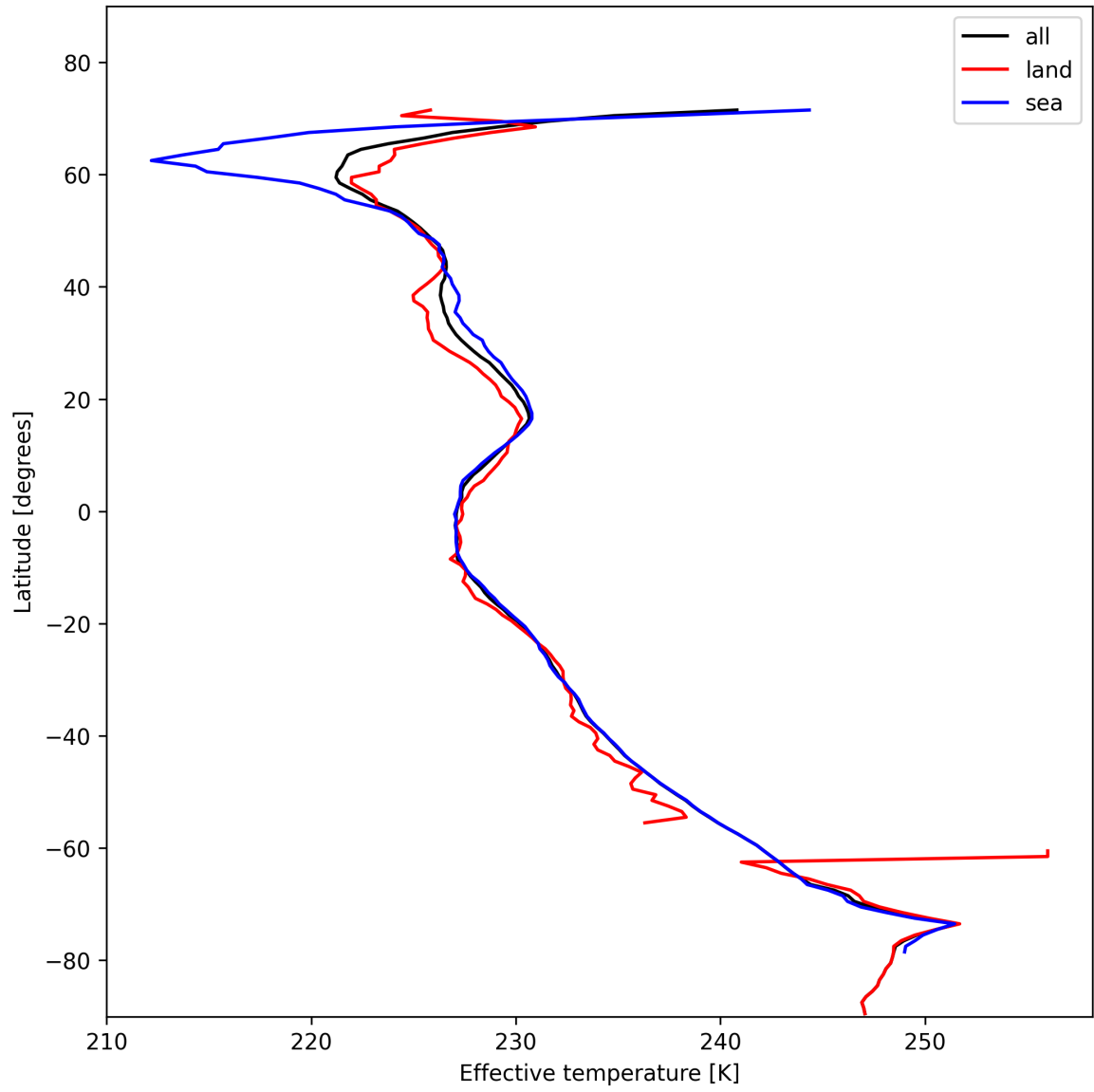
Figure 26: Zonal average of “Effective temperature” for 2025-01-29 to 2025-01-30.
