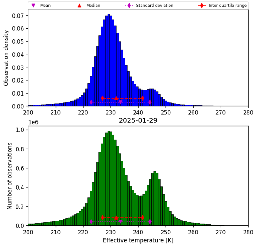
Figure 38: Histogram of “Effective temperature” for 2025-01-29 to 2025-01-30
