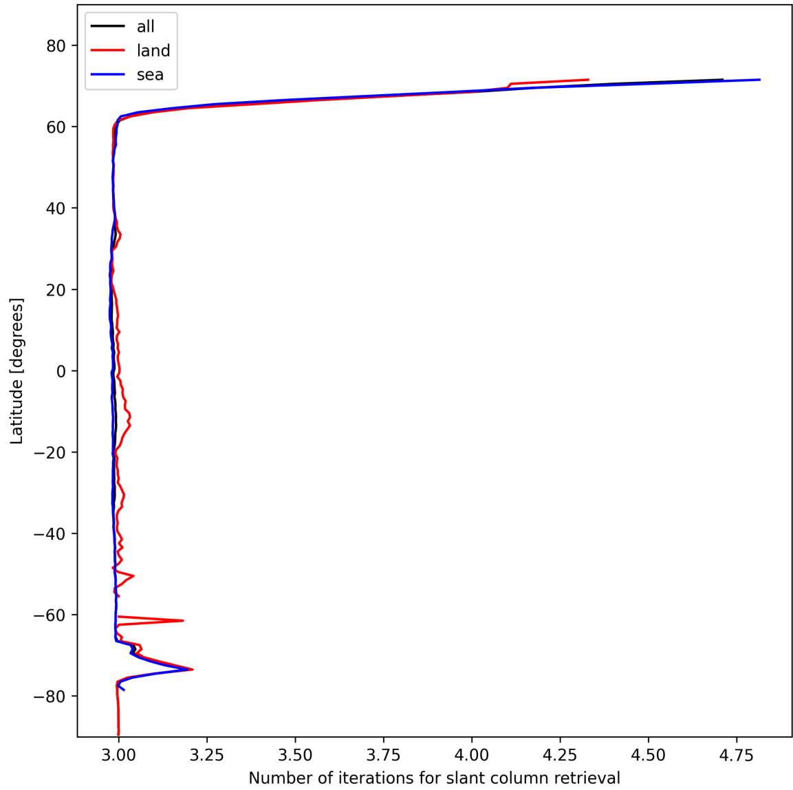
Figure 21: Zonal average of “Number of iterations for slant column retrieval” for 2025-01-29 to 2025-01-30.
