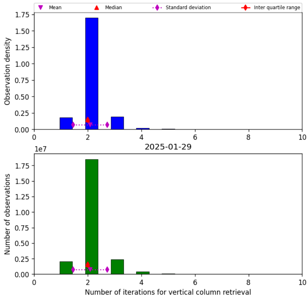
Figure 39: Histogram of “Number of iterations for vertical column retrieval” for 2025-01-29 to 2025-01-30
