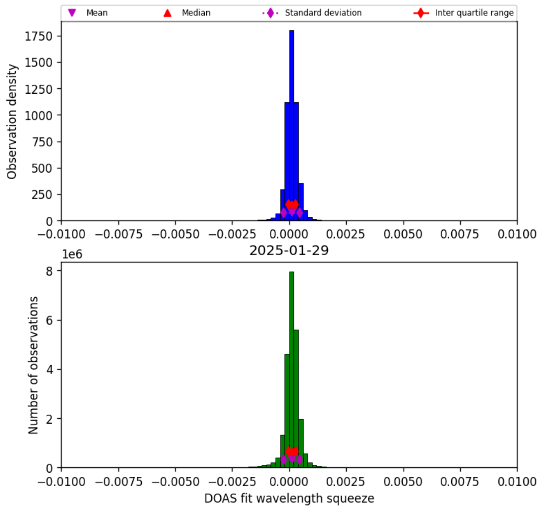
Figure 36: Histogram of “DOAS fit wavelength squeeze” for 2025-01-29 to 2025-01-30
