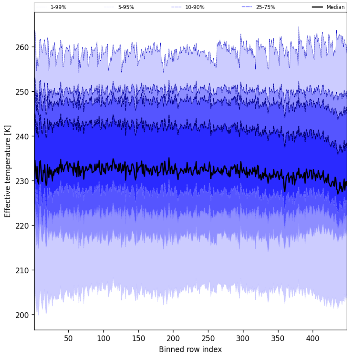
Figure 50: Along track statistics of “Effective temperature” for 2025-01-29 to 2025-01-30
