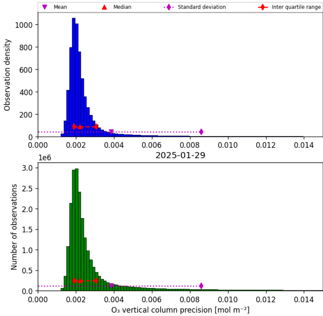
Figure 30: Histogram of "O 3 vertical column precision" for 2025-01-29 to 2025-01-30
