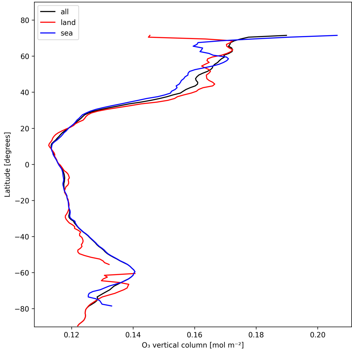
Figure 17: Zonal average of “O 3 vertical column” for 2025-01-29 to 2025-01-30.
