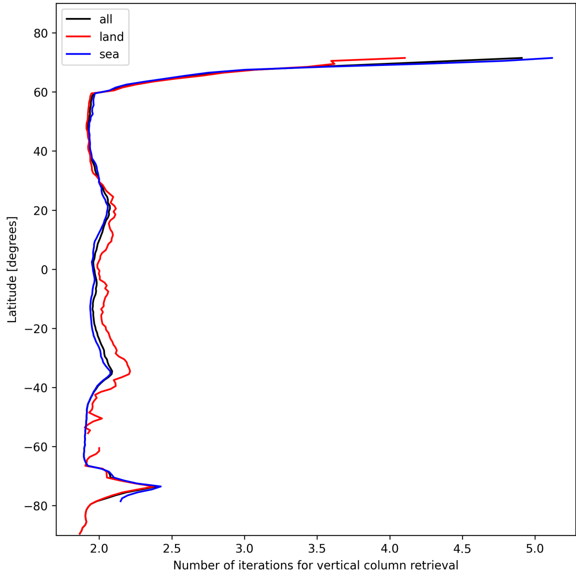
Figure 27: Zonal average of “Number of iterations for vertical column retrieval” for 2025-01-29 to 2025-01-30.
