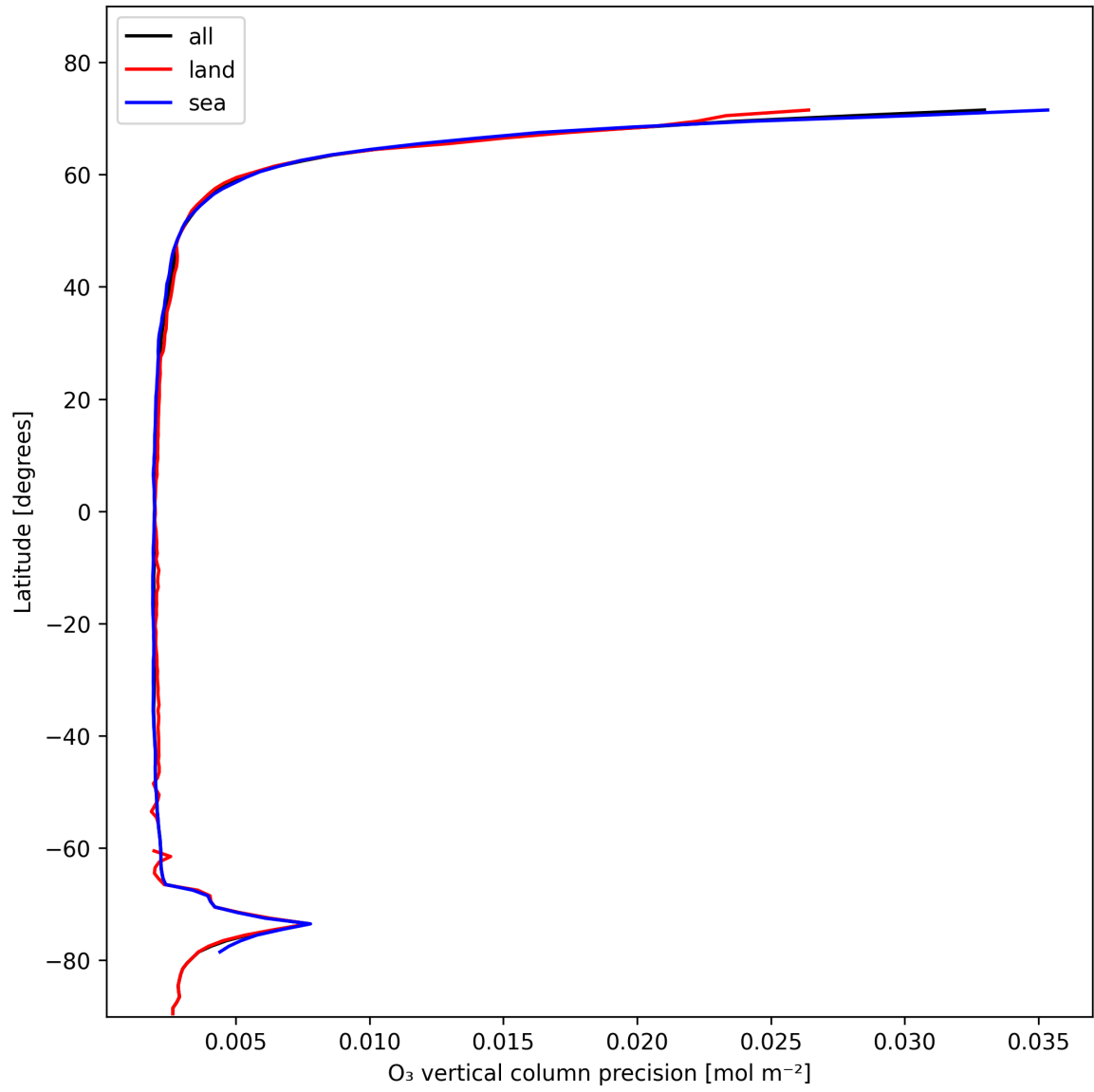
Figure 18: Zonal average of “O 3 vertical column precision” for 2025-01-29 to 2025-01-30.
