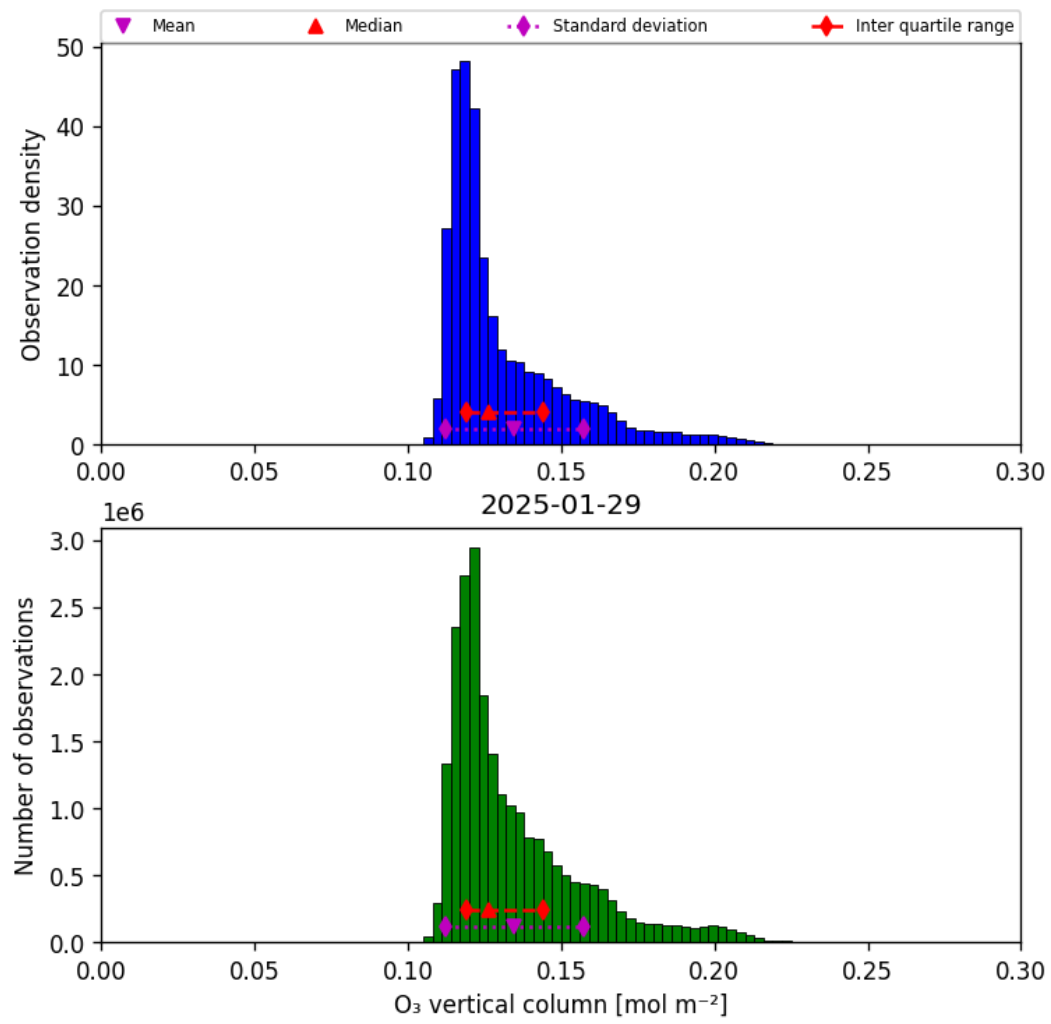
Figure 29: Histogram of “O 3 vertical column” for 2025-01-29 to 2025-01-30
