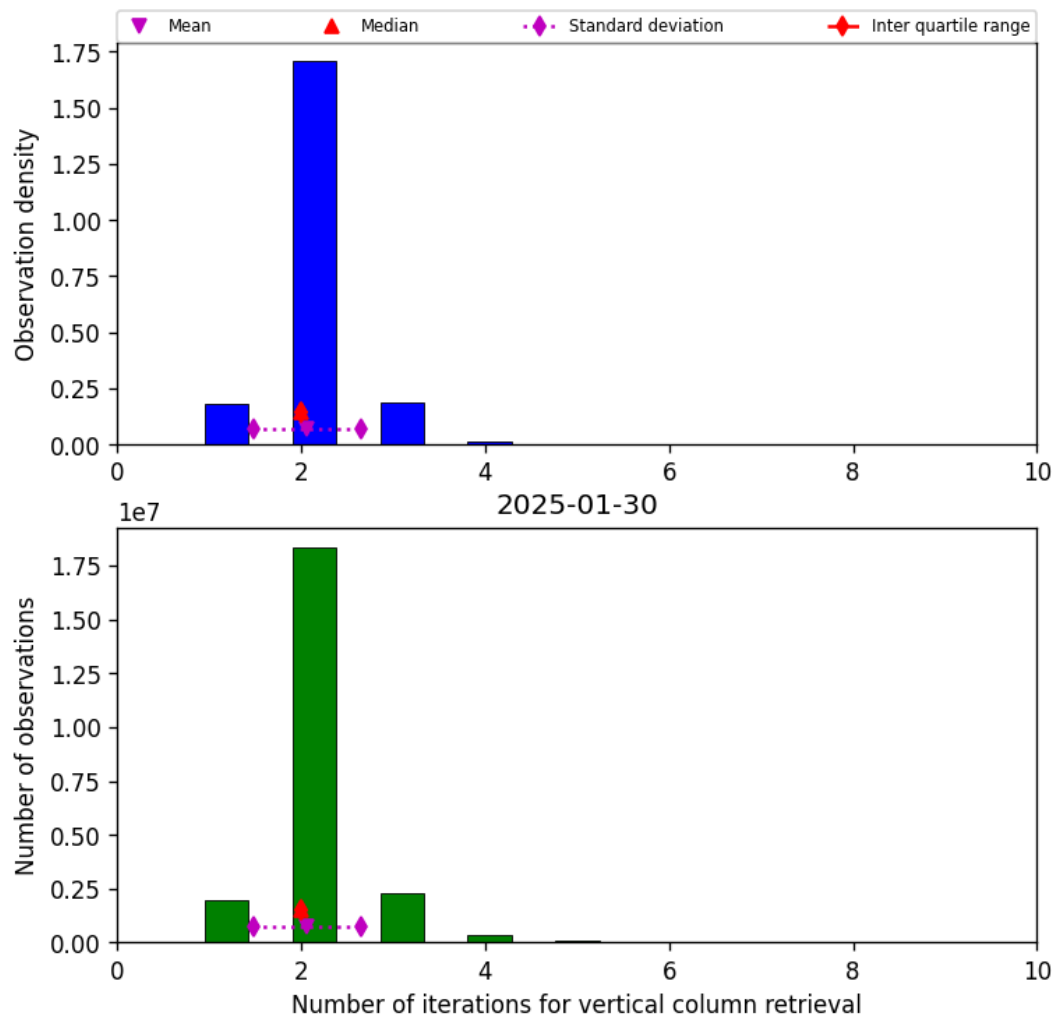
Figure 39: Histogram of “Number of iterations for vertical column retrieval” for 2025-01-30 to 2025-01-31
