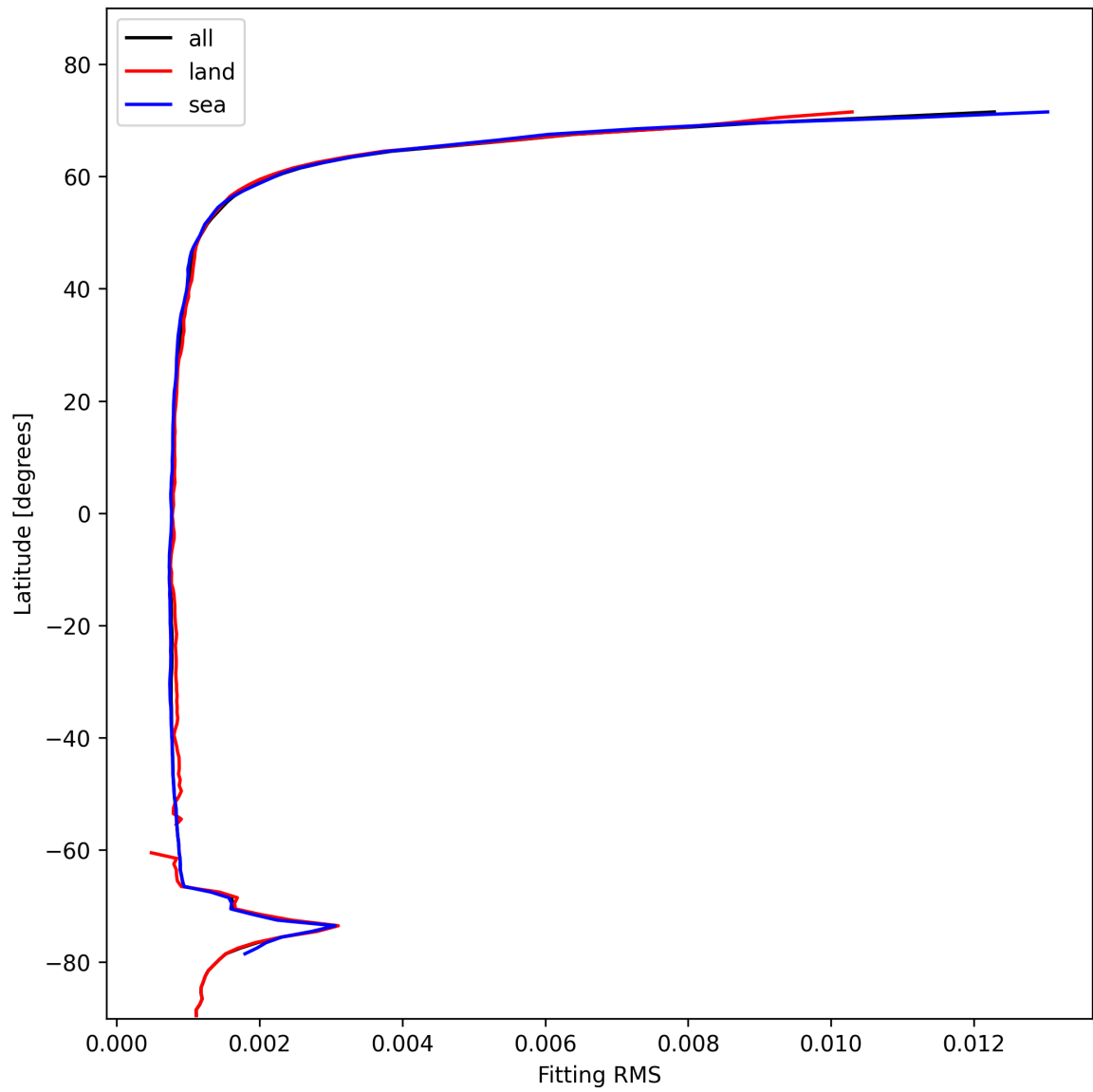
Figure 22: Zonal average of “Fitting RMS” for 2025-01-30 to 2025-01-31.
