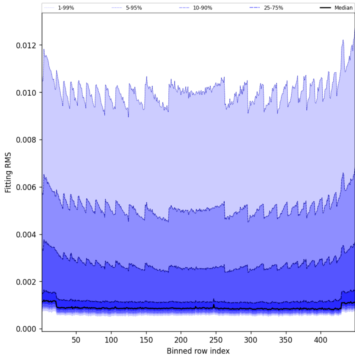
Figure 46: Along track statistics of “Fitting RMS” for 2025-01-30 to 2025-01-31
