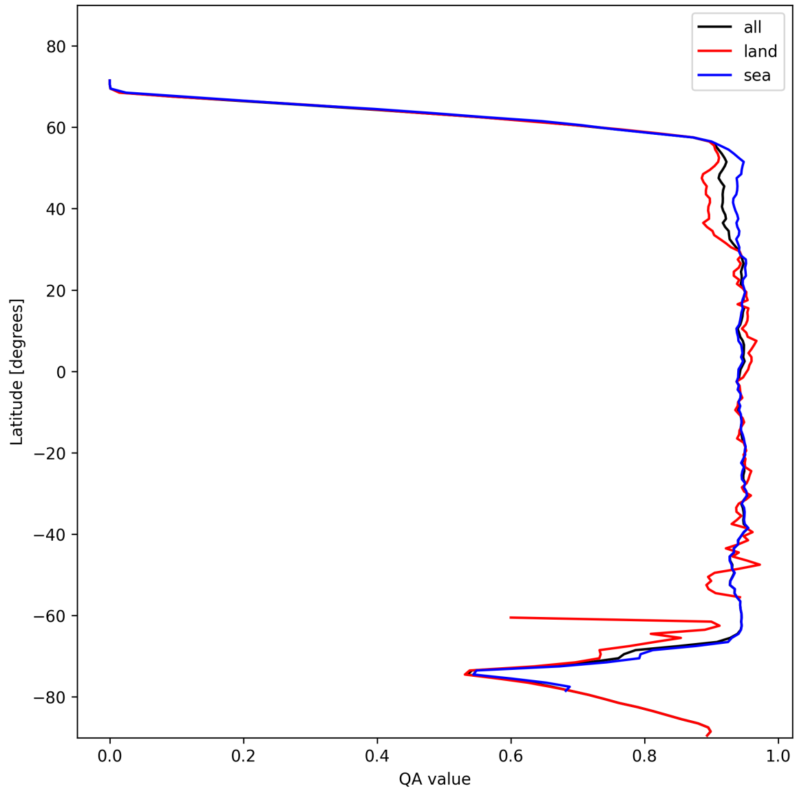
Figure 16: Zonal average of “QA value” for 2025-01-30 to 2025-01-31.
