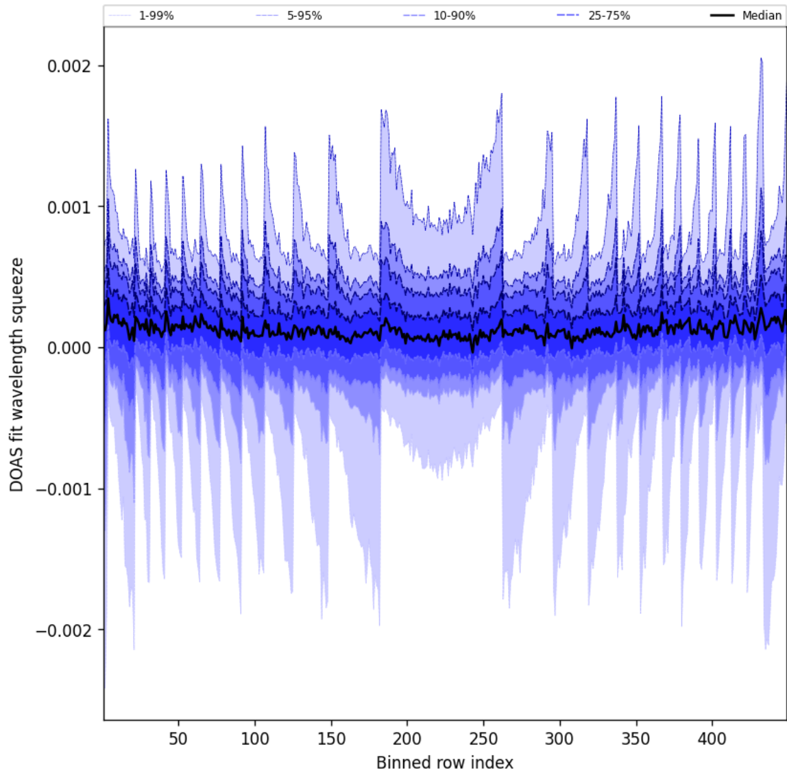
Figure 48: Along track statistics of “DOAS fit wavelength squeeze” for 2025-01-30 to 2025-01-31
