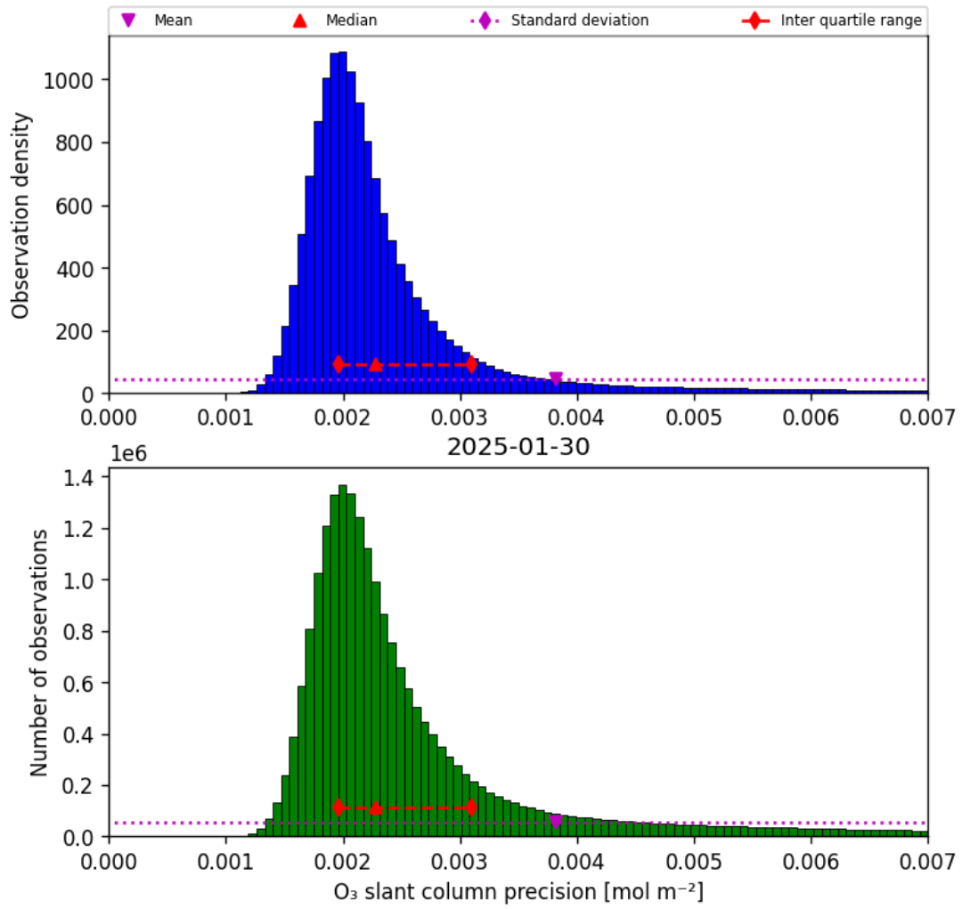
Figure 32: Histogram of “O 3 slant column precision” for 2025-01-30 to 2025-01-31
