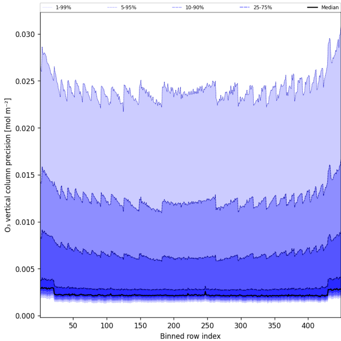
Figure 42: Along track statistics of “O 3 vertical column precision” for 2025-01-30 to 2025-01-31
