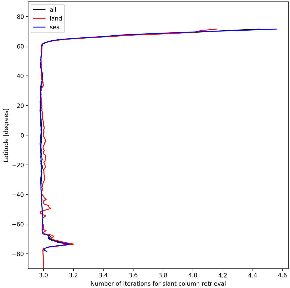
Figure 21: Zonal average of “Number of iterations for slant column retrieval” for 2025-01-30 to 2025-01-31.
