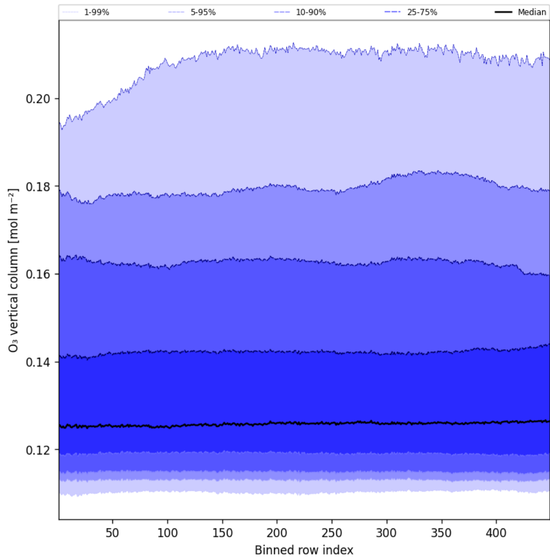
Figure 41: Along track statistics of “O 3 vertical column” for 2025-01-30 to 2025-01-31
