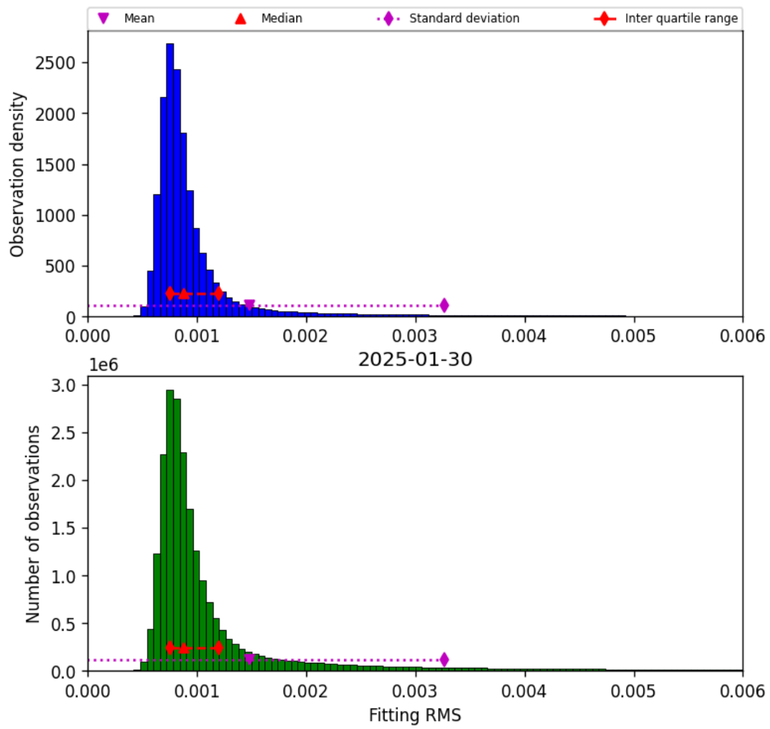
Figure 34: Histogram of “Fitting RMS” for 2025-01-30 to 2025-01-31
