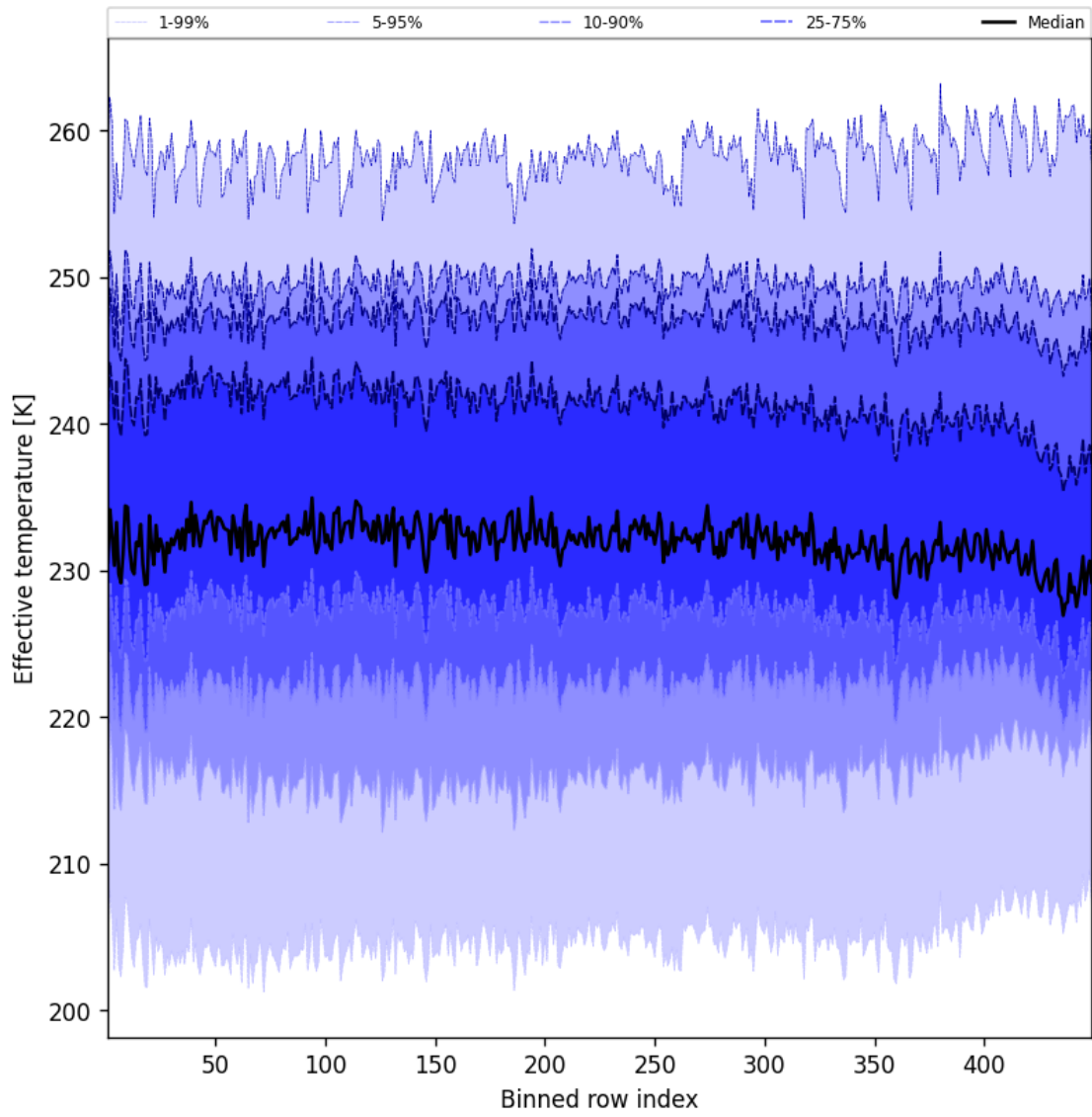
Figure 50: Along track statistics of “Effective temperature” for 2025-01-30 to 2025-01-31
