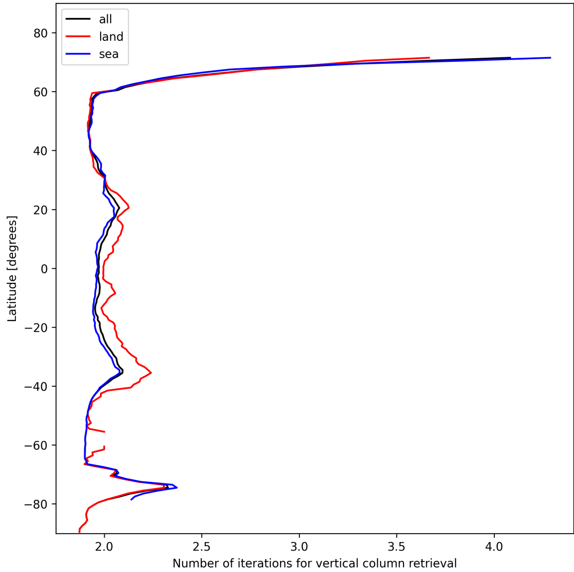
Figure 27: Zonal average of “Number of iterations for vertical column retrieval” for 2025-01-31 to 2025-01-31.
