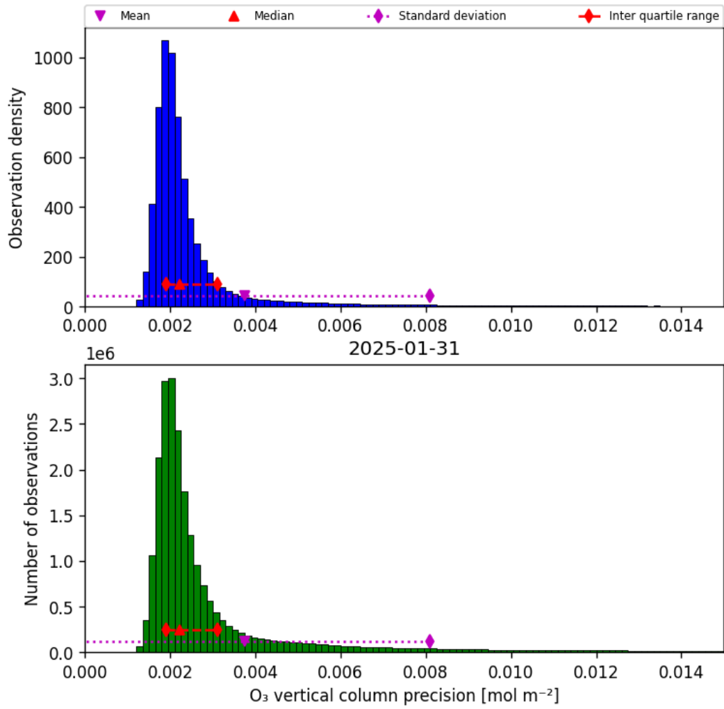
Figure 30: Histogram of “O 3 vertical column precision” for 2025-01-31 to 2025-01-31
