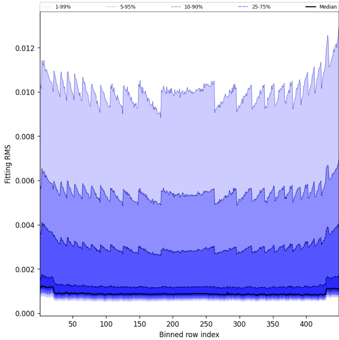
Figure 46: Along track statistics of “Fitting RMS” for 2025-01-31 to 2025-01-31
