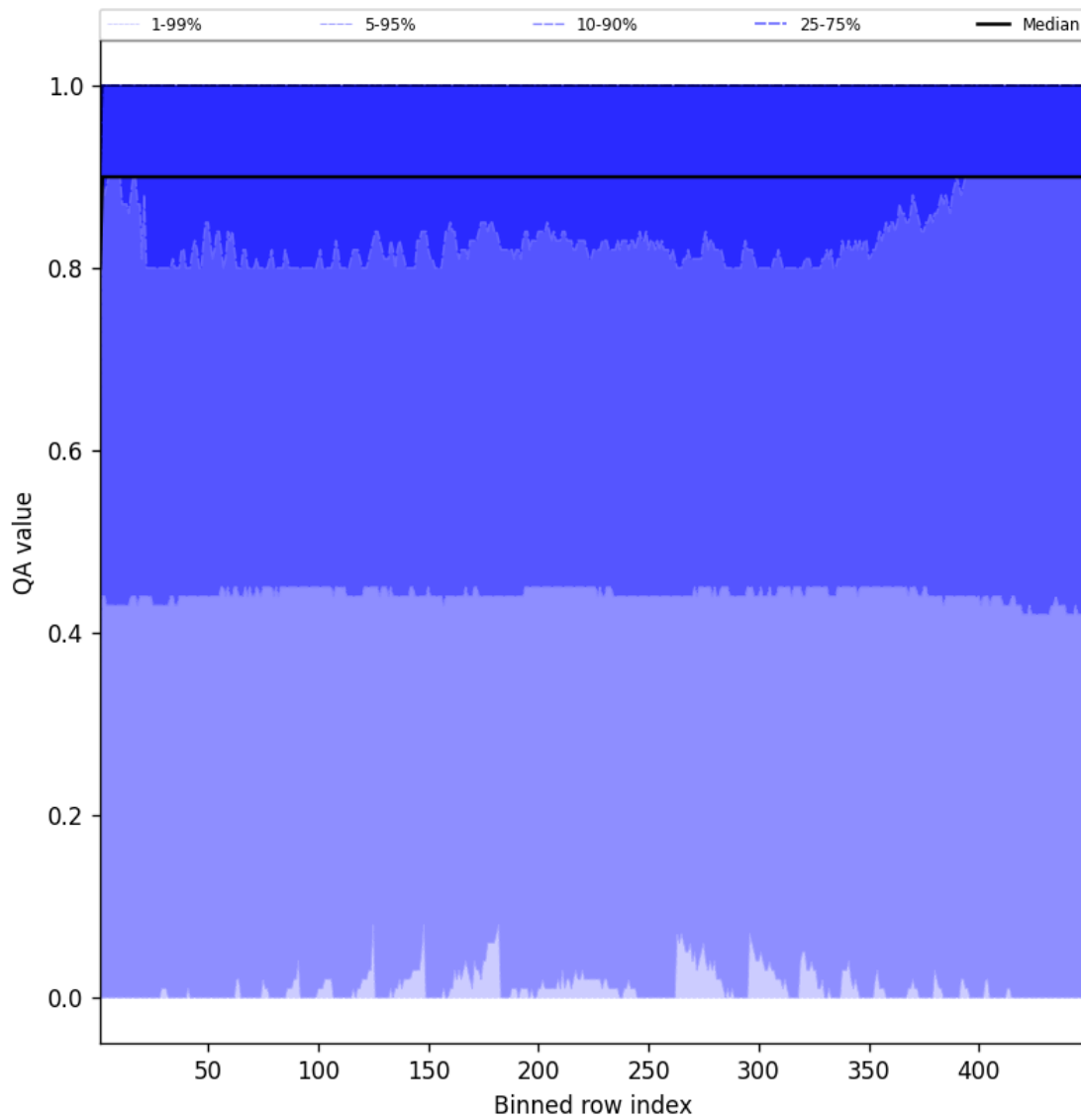
Figure 40: Along track statistics of “QA value” for 2025-01-31 to 2025-01-31
