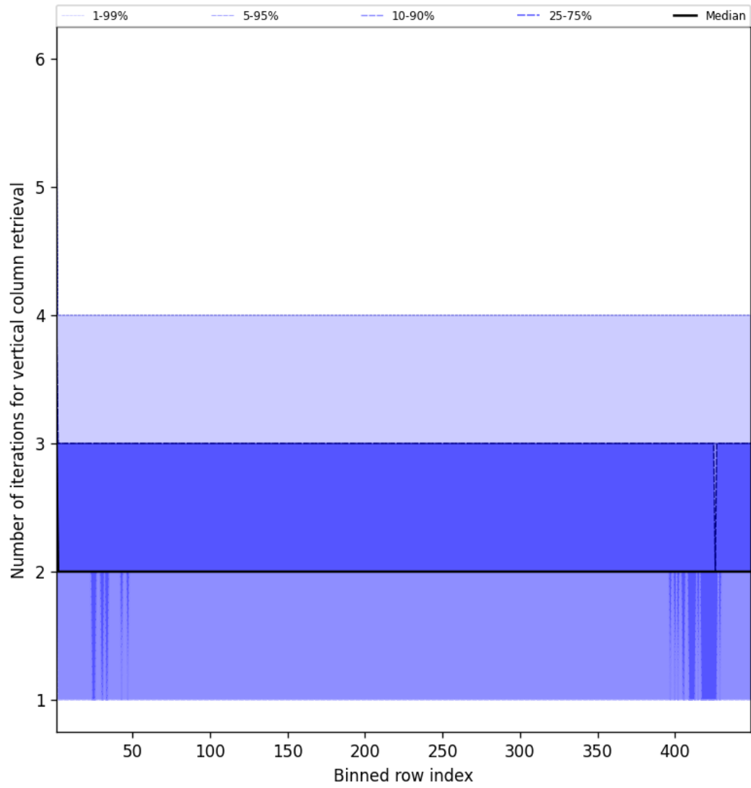
Figure 51: Along track statistics of “Number of iterations for vertical column retrieval” for 2025-01-31 to 2025-01-31
