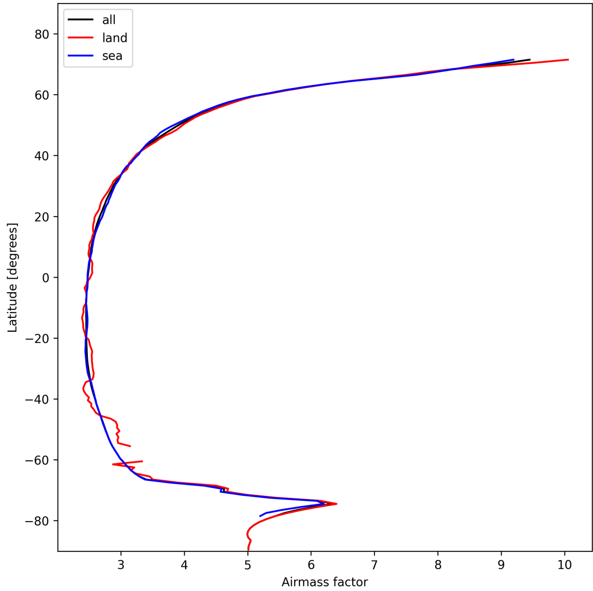
Figure 25: Zonal average of “Airmass factor” for 2025-01-31 to 2025-01-31.
