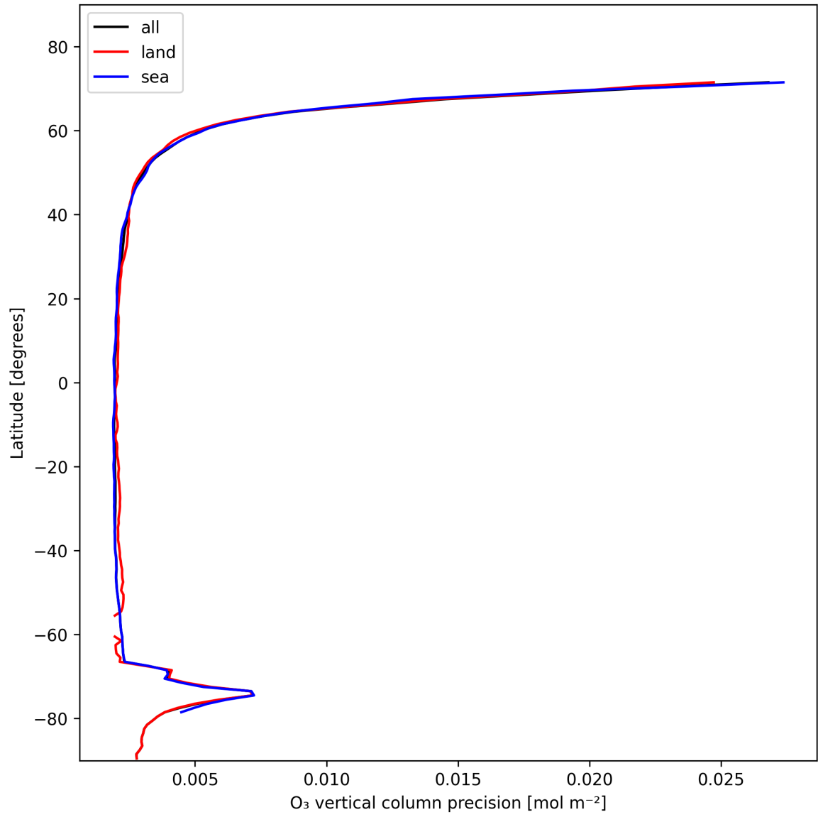
Figure 18: Zonal average of “O 3 vertical column precision” for 2025-01-31 to 2025-01-31.
