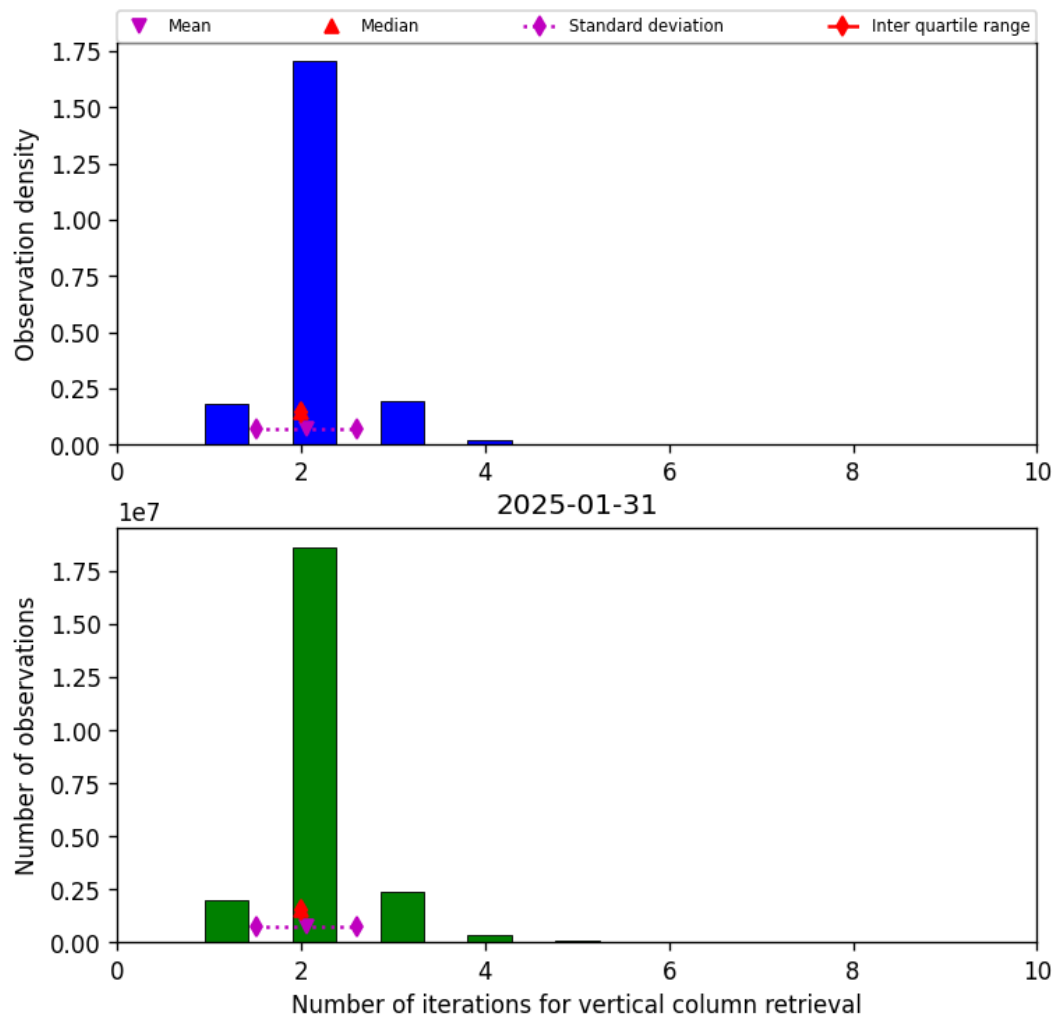
Figure 39: Histogram of “Number of iterations for vertical column retrieval” for 2025-01-31 to 2025-01-31
