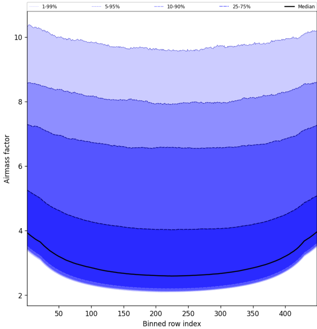
Figure 49: Along track statistics of “Airmass factor” for 2025-01-31 to 2025-01-31
