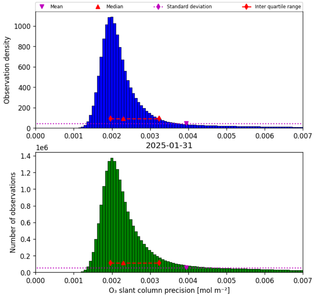
Figure 32: Histogram of “O 3 slant column precision” for 2025-01-31 to 2025-01-31
