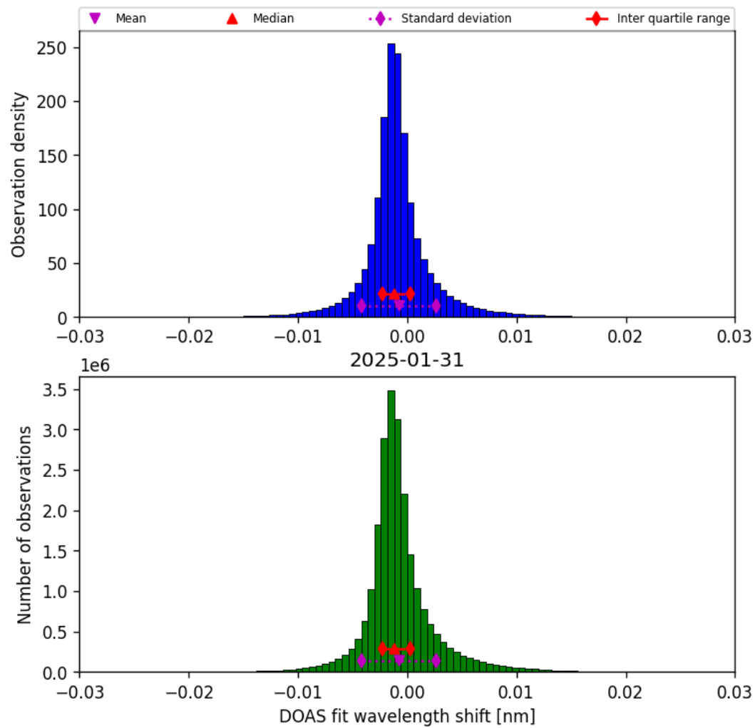
Figure 35: Histogram of “DOAS fit wavelength shift” for 2025-01-31 to 2025-01-31
