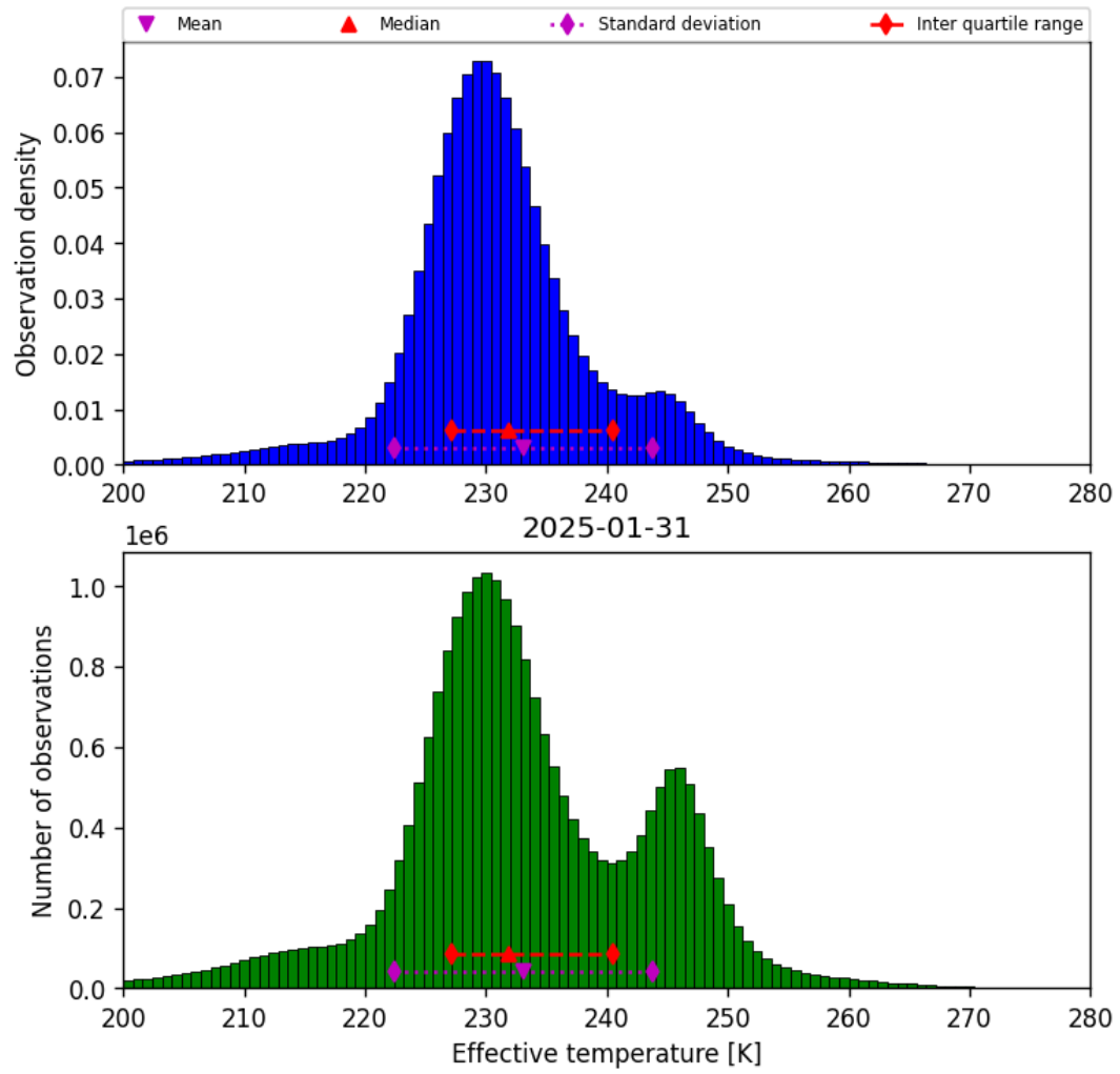
Figure 38: Histogram of “Effective temperature” for 2025-01-31 to 2025-01-31
