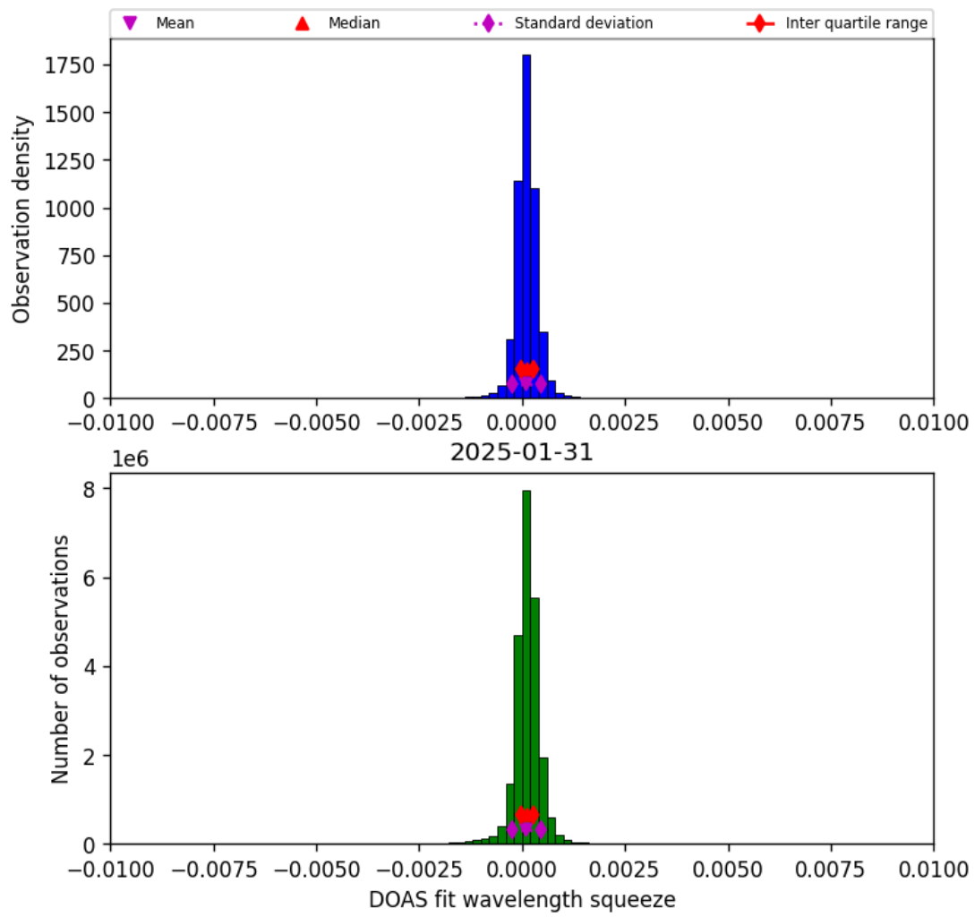
Figure 36: Histogram of “DOAS fit wavelength squeeze” for 2025-01-31 to 2025-01-31
