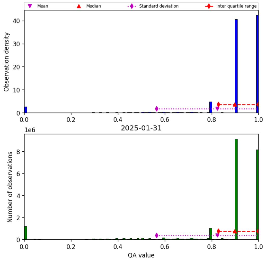
Figure 28: Histogram of “QA value” for 2025-01-31 to 2025-01-31
