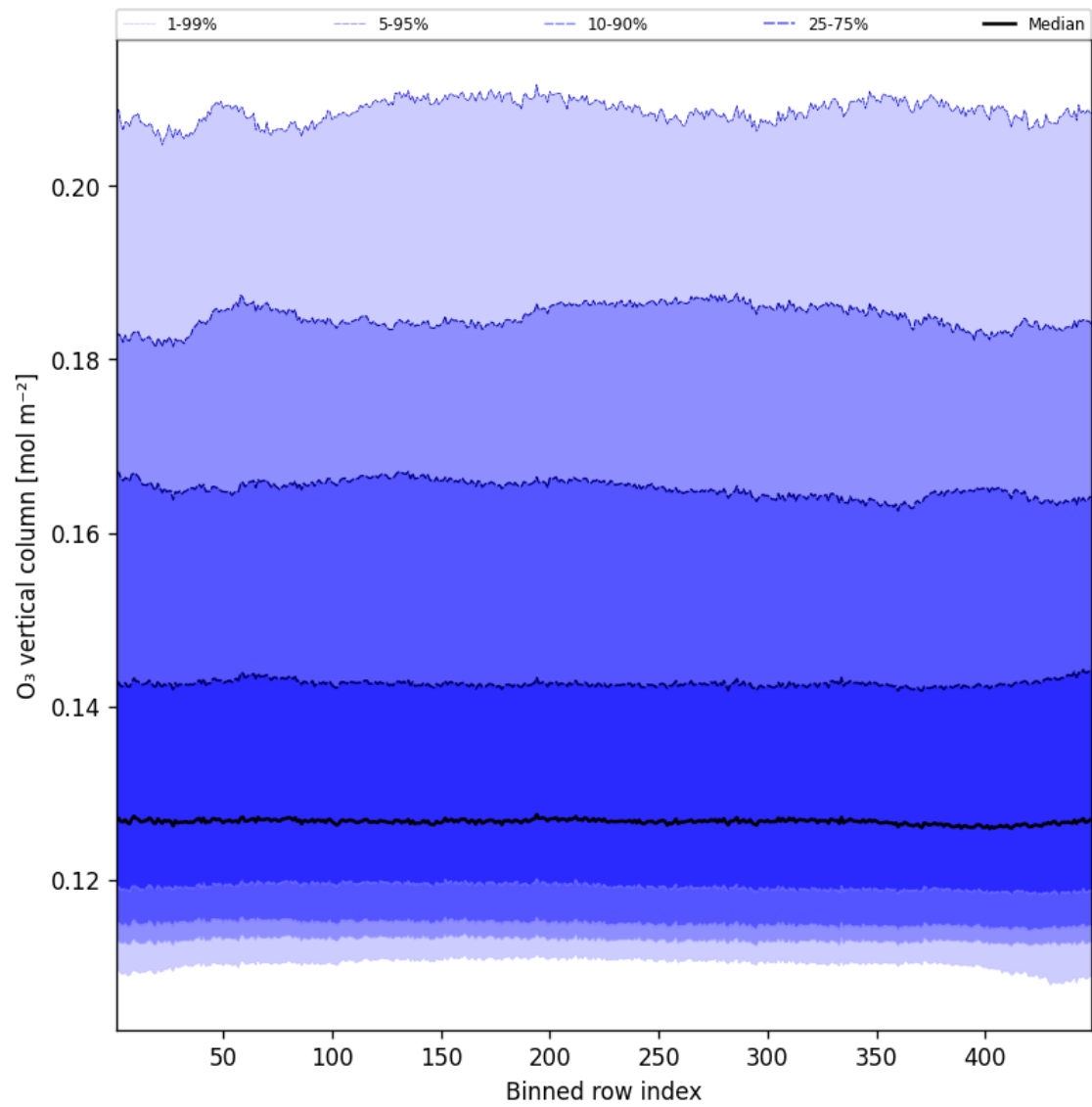
Figure 41: Along track statistics of “O 3 vertical column” for 2025-01-31 to 2025-01-31
