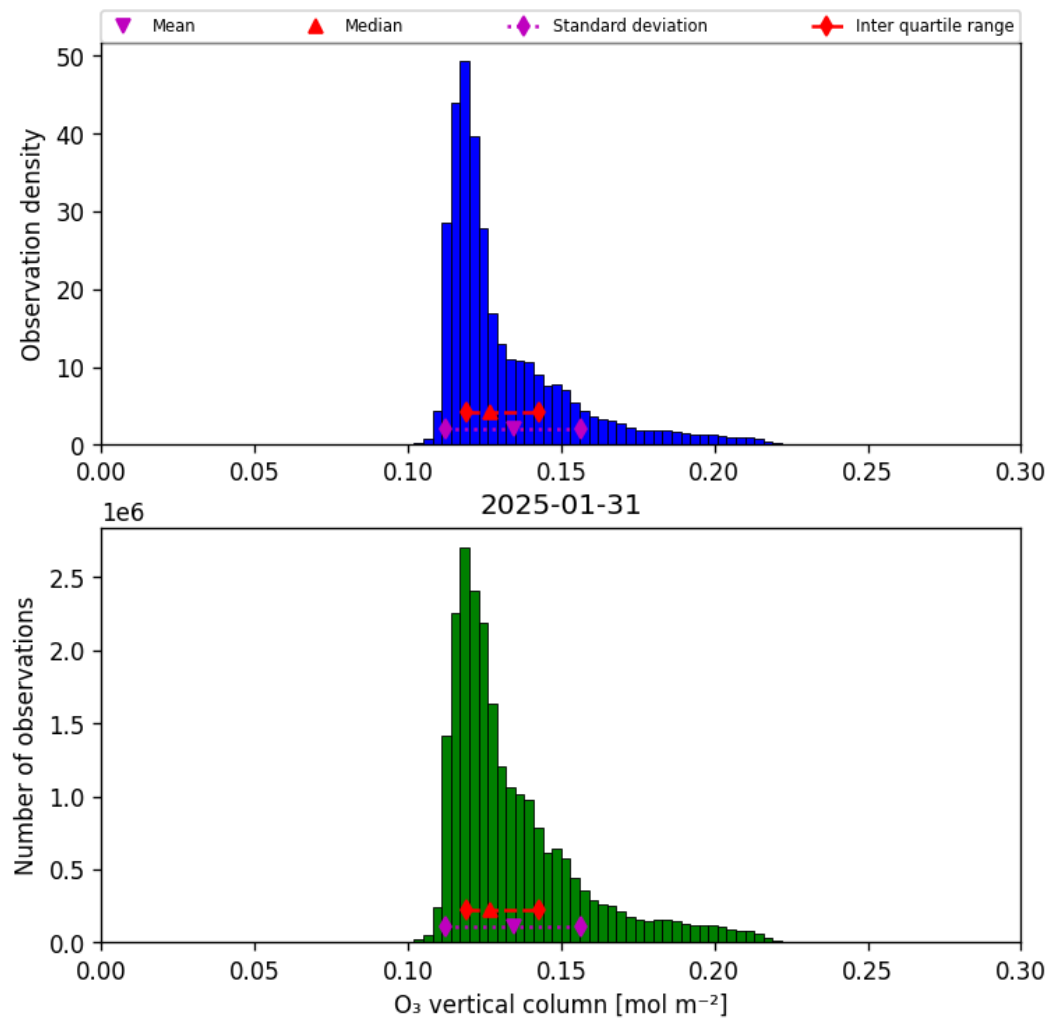
Figure 29: Histogram of “O 3 vertical column” for 2025-01-31 to 2025-01-31
