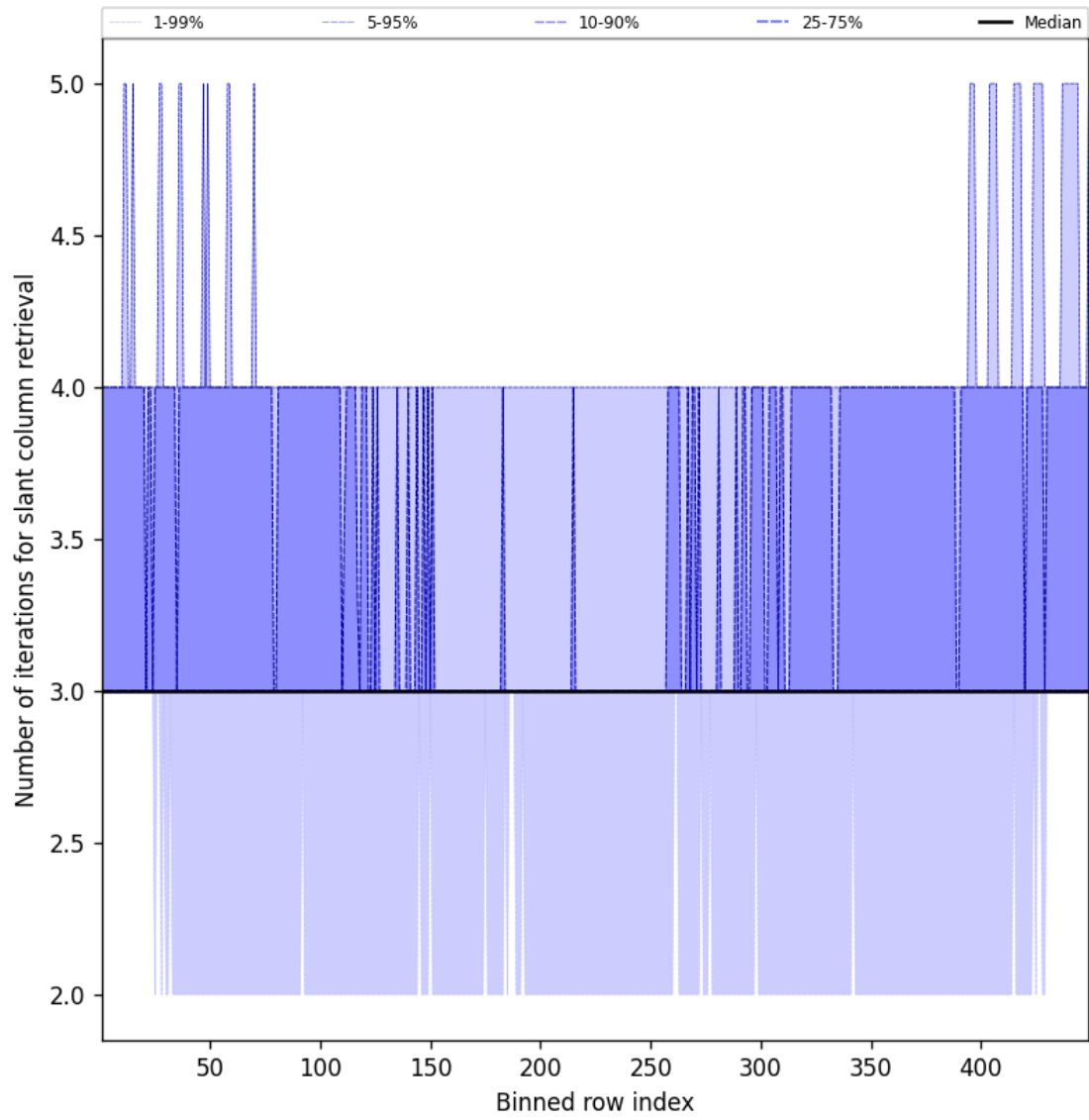
Figure 45: Along track statistics of “Number of iterations for slant column retrieval” for 2025-01-31 to 2025-01-31
