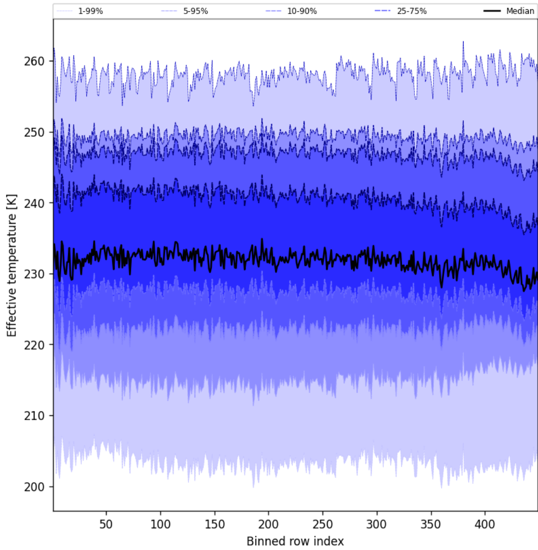
Figure 50: Along track statistics of “Effective temperature” for 2025-01-31 to 2025-01-31
