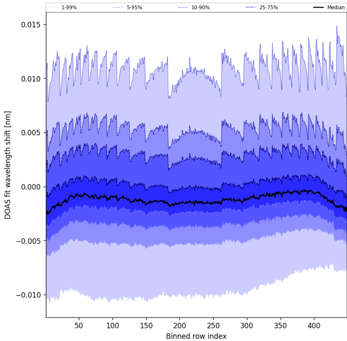
Figure 47: Along track statistics of “DOAS fit wavelength shift” for 2025-01-31 to 2025-01-31
