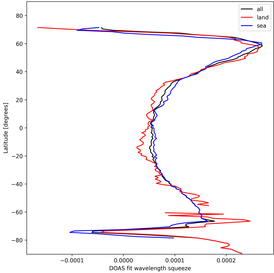
Figure 24: Zonal average of “DOAS fit wavelength squeeze” for 2025-01-31 to 2025-01-31.
