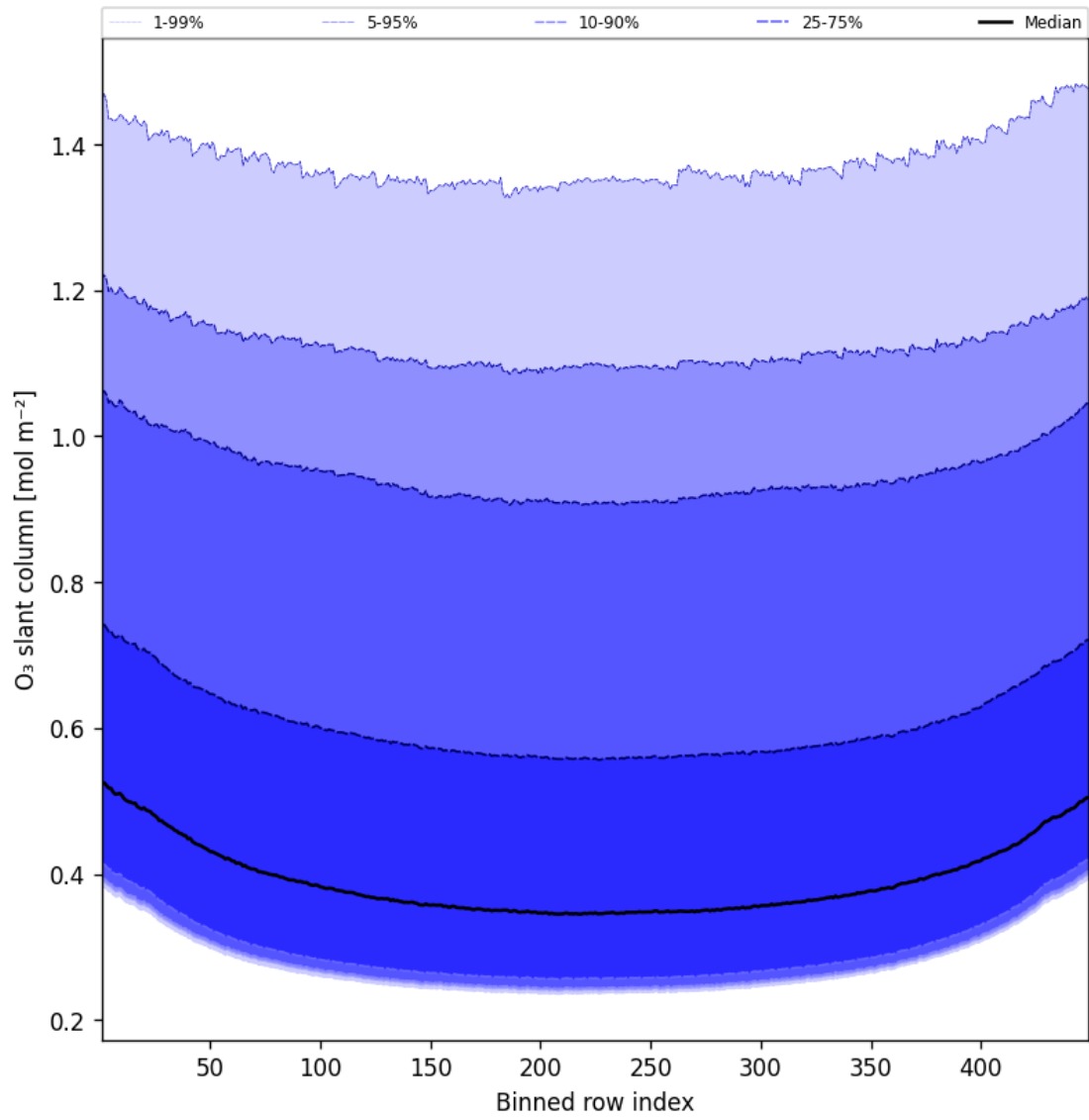
Figure 43: Along track statistics of “O 3 slant column” for 2025-01-31 to 2025-01-31
