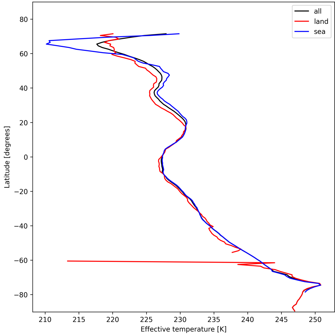
Figure 26: Zonal average of “Effective temperature” for 2025-01-31 to 2025-01-31.
