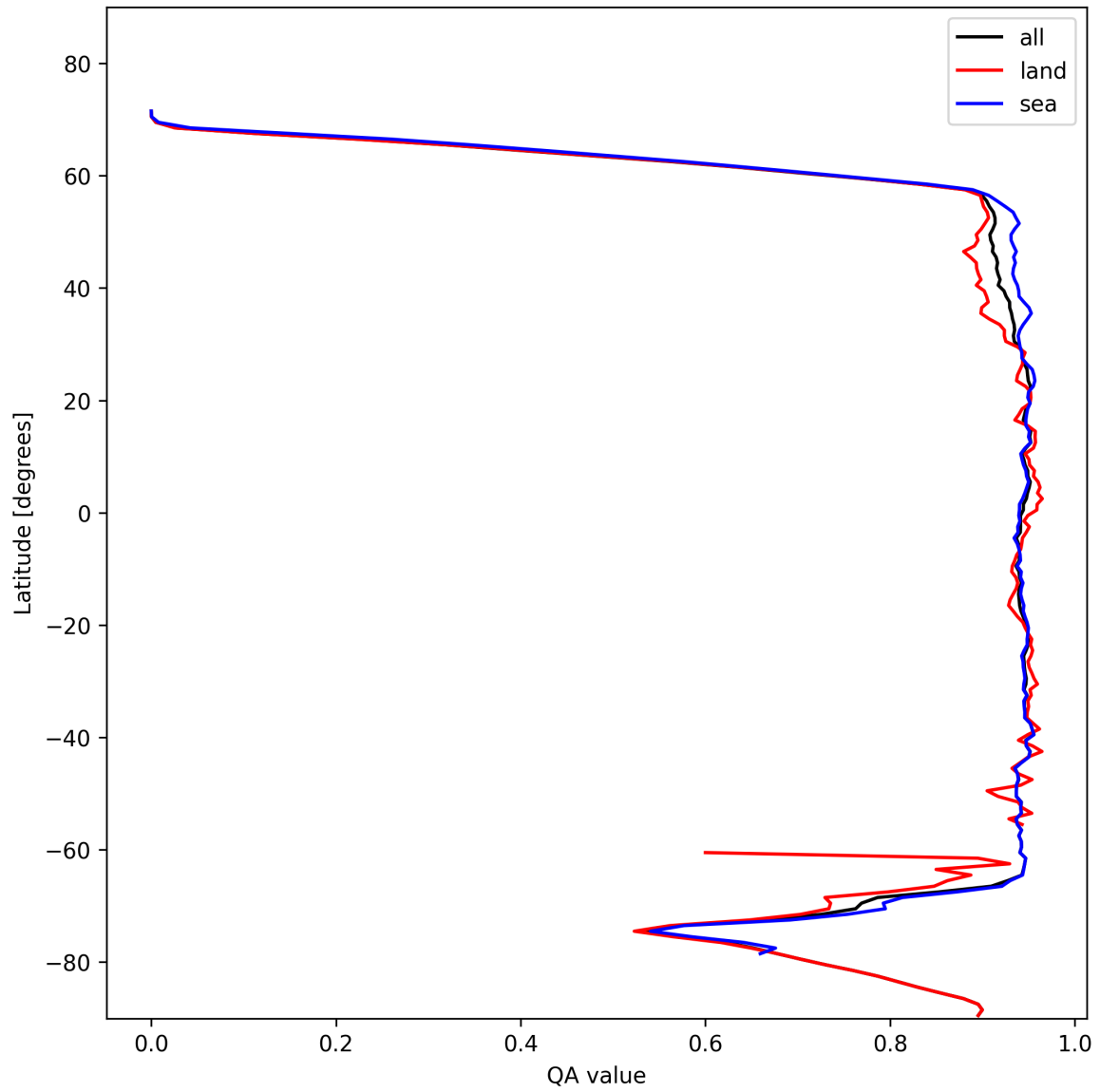
Figure 16: Zonal average of “QA value” for 2025-01-31 to 2025-01-31.
