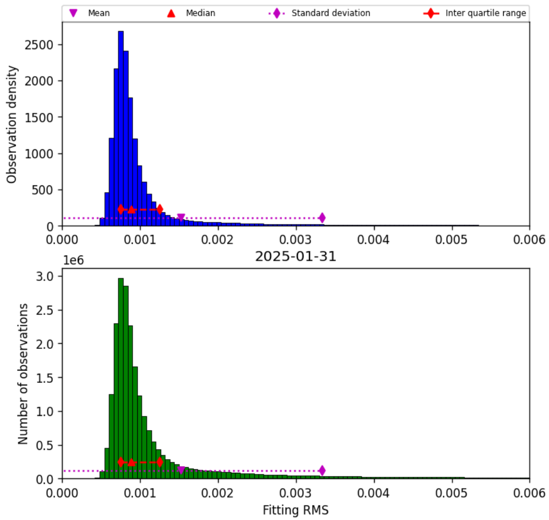
Figure 34: Histogram of “Fitting RMS” for 2025-01-31 to 2025-01-31
