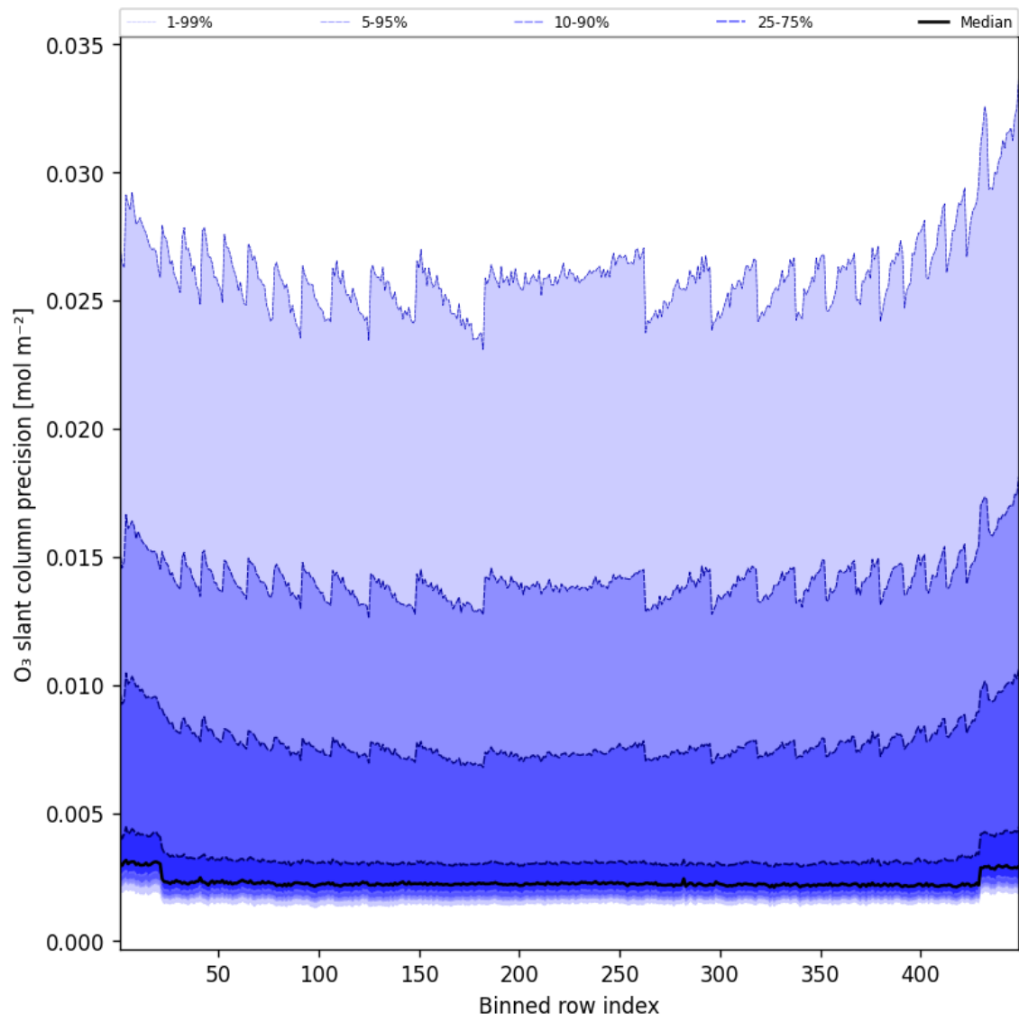
Figure 44: Along track statistics of “O 3 slant column precision” for 2025-01-31 to 2025-01-31
