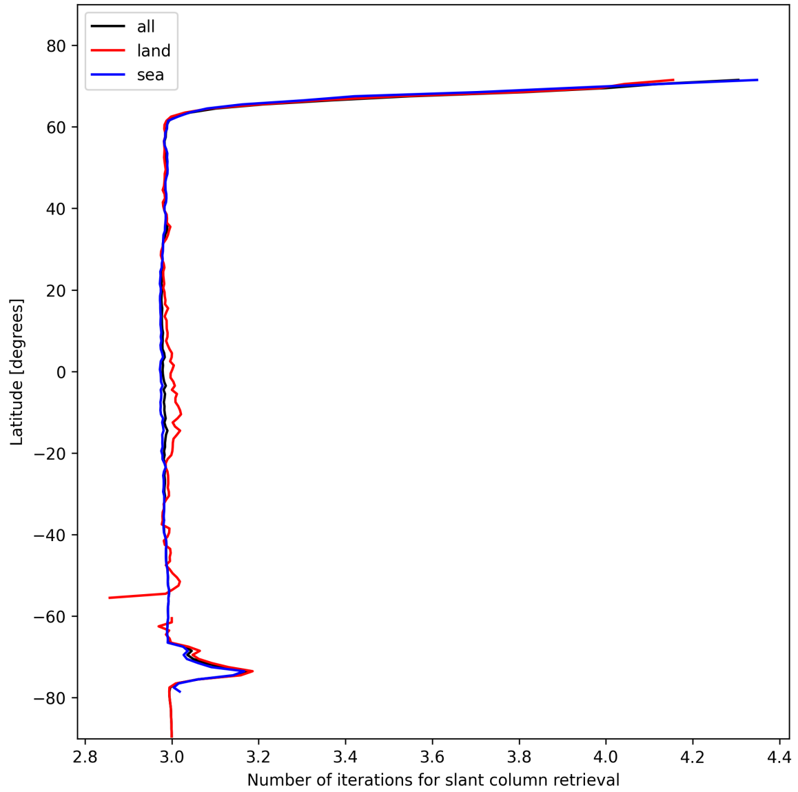
Figure 21: Zonal average of “Number of iterations for slant column retrieval” for 2025-01-31 to 2025-01-31.
