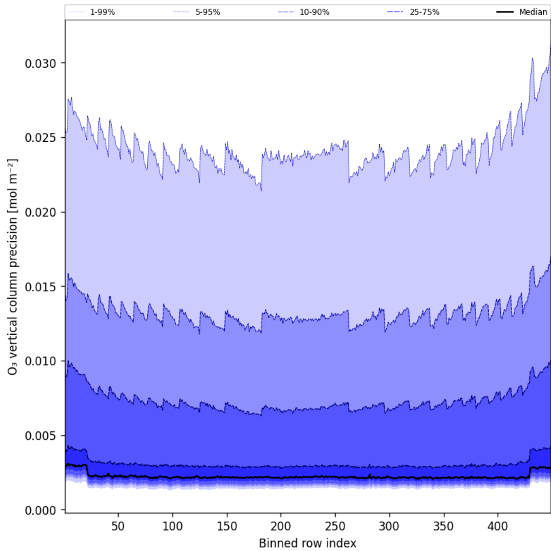
Figure 42: Along track statistics of “O 3 vertical column precision” for 2025-01-31 to 2025-01-31
