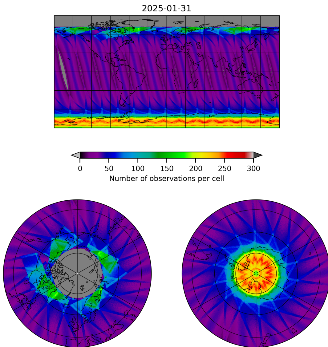
Figure 15: Map of the number of observations for 2025-01-31 to 2025-01-31
