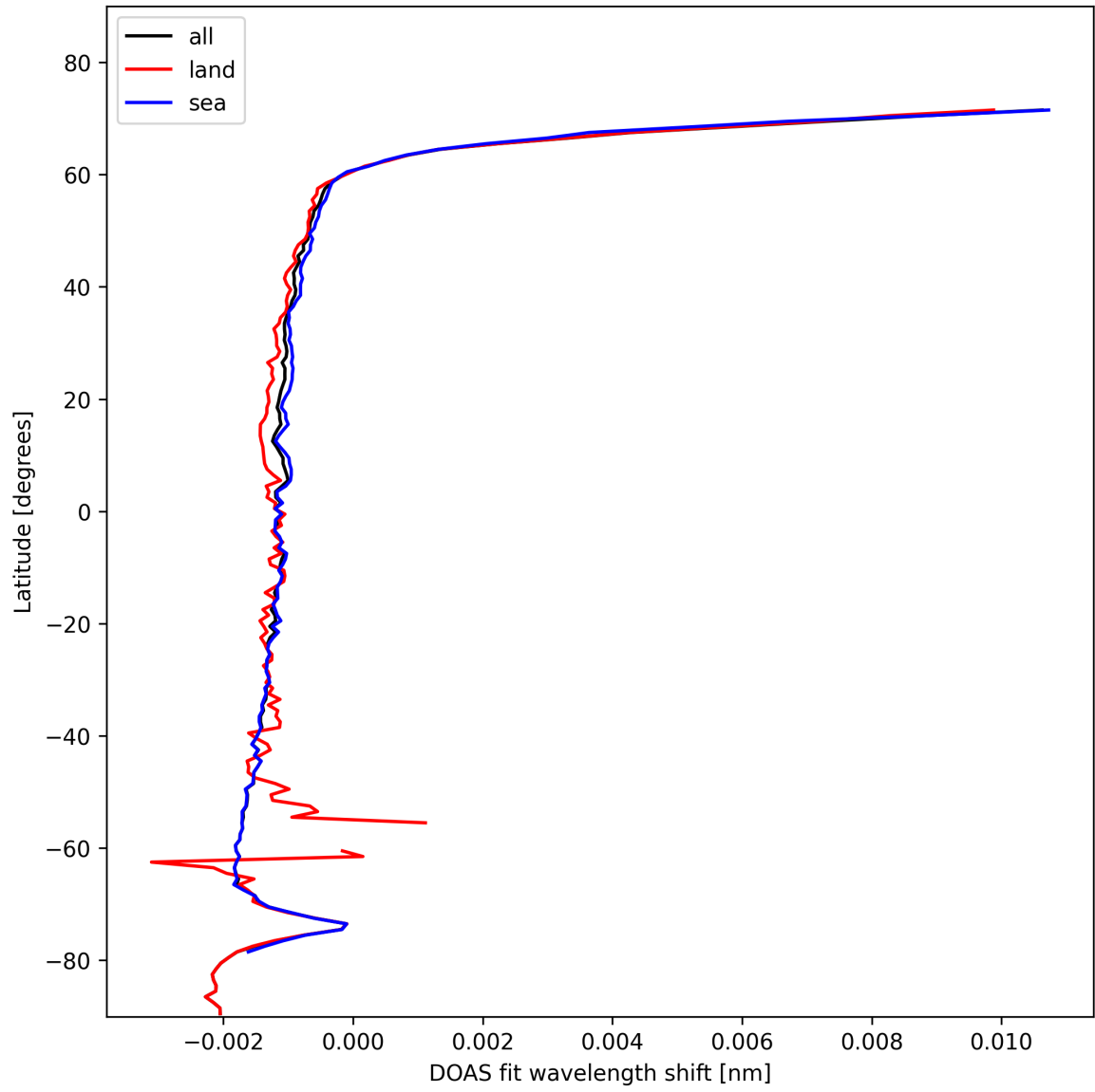
Figure 23: Zonal average of “DOAS fit wavelength shift” for 2025-01-31 to 2025-01-31.
