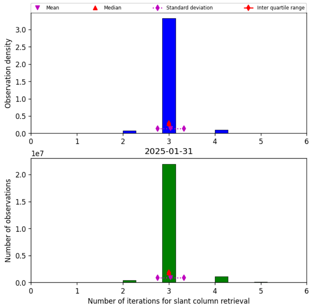
Figure 33: Histogram of “Number of iterations for slant column retrieval” for 2025-01-31 to 2025-01-31
