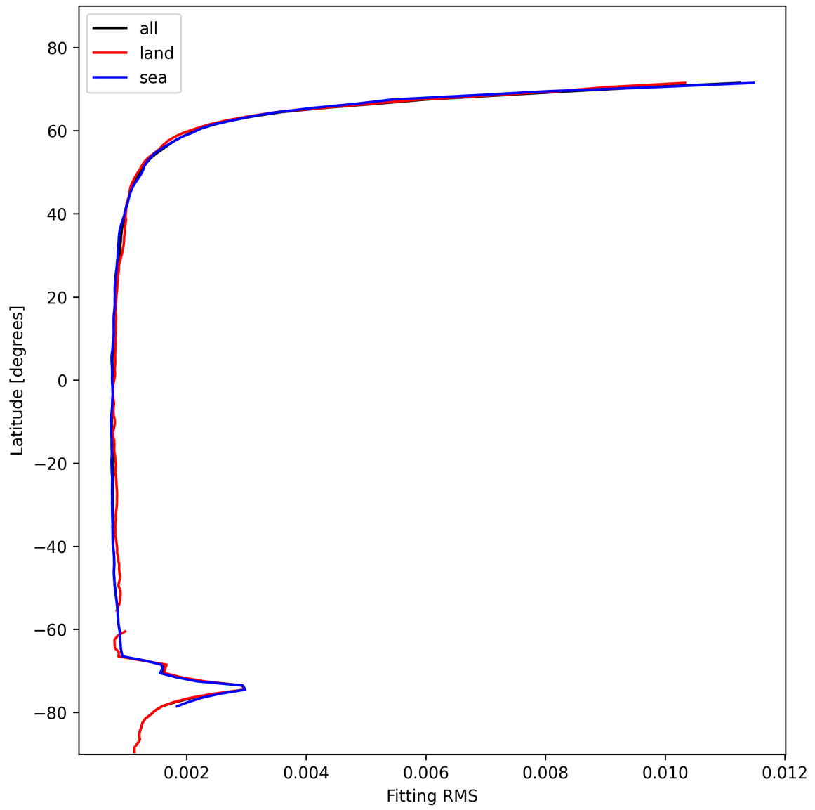
Figure 22: Zonal average of “Fitting RMS” for 2025-01-31 to 2025-01-31.
