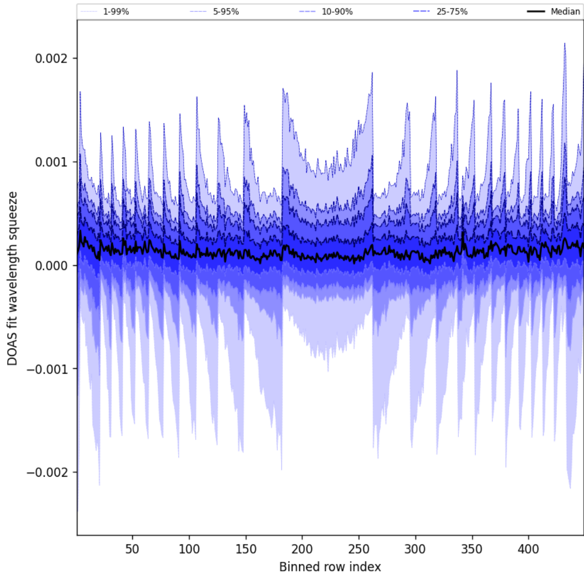
Figure 48: Along track statistics of “DOAS fit wavelength squeeze” for 2025-01-31 to 2025-01-31
