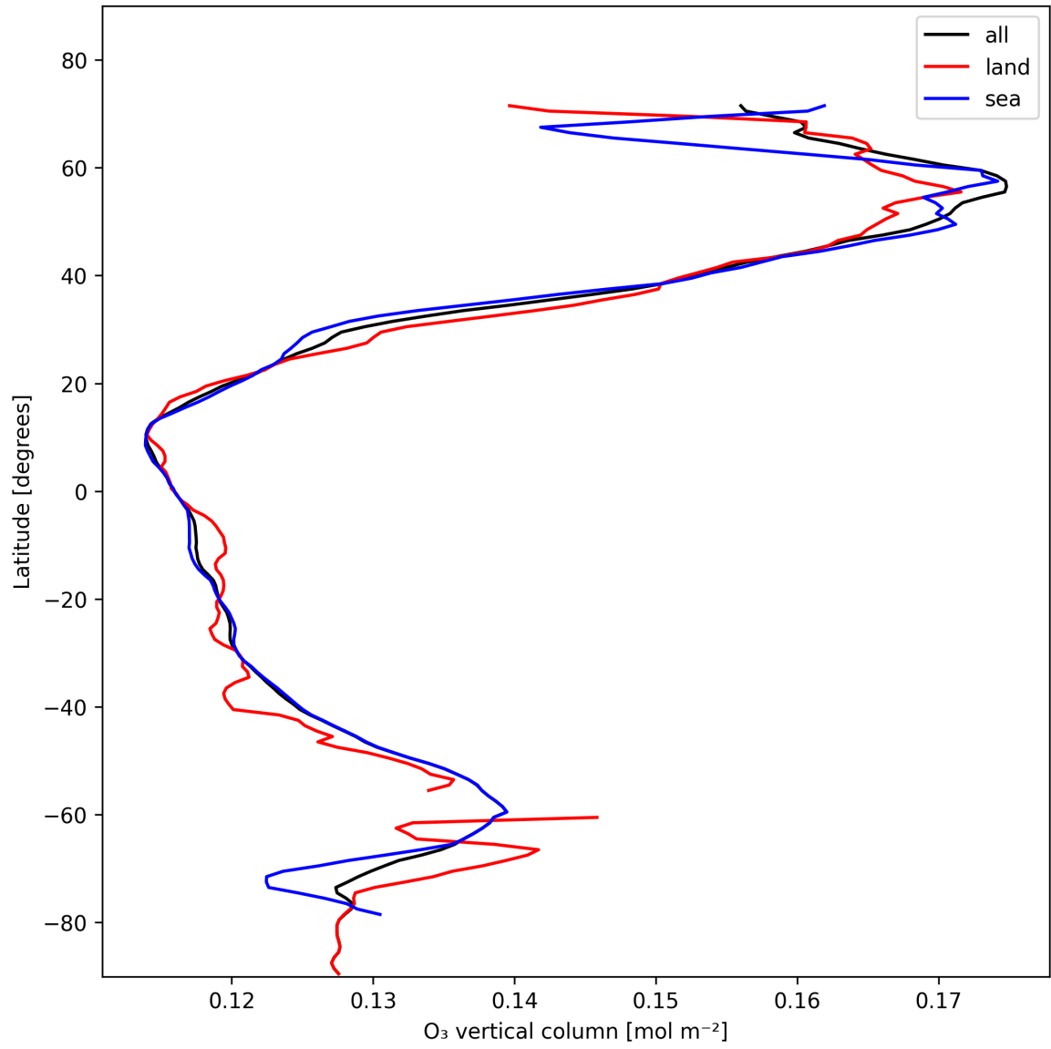
Figure 17: Zonal average of “O 3 vertical column” for 2025-01-31 to 2025-01-31.
