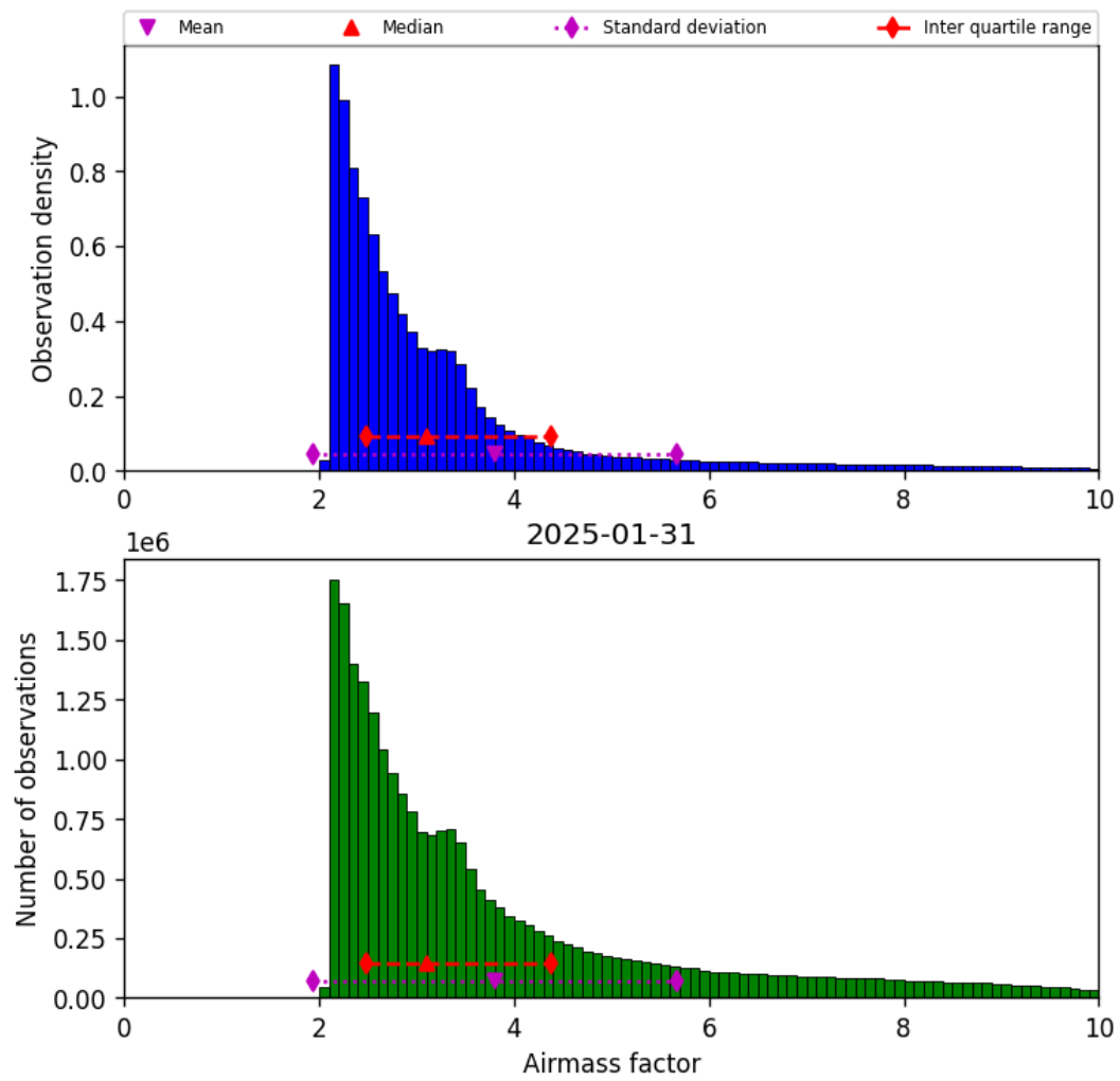
Figure 37: Histogram of “Airmass factor” for 2025-01-31 to 2025-01-31
