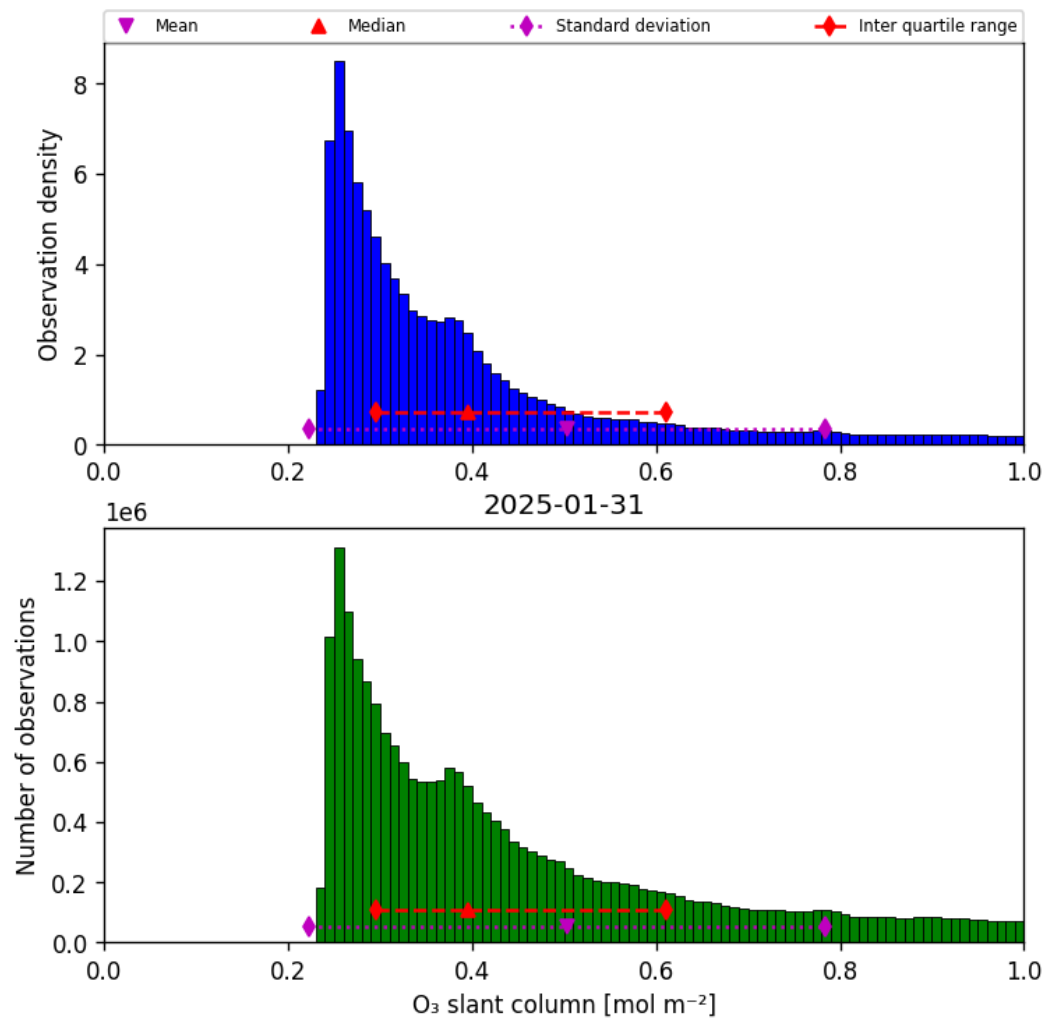
Figure 31: Histogram of “O 3 slant column” for 2025-01-31 to 2025-01-31
