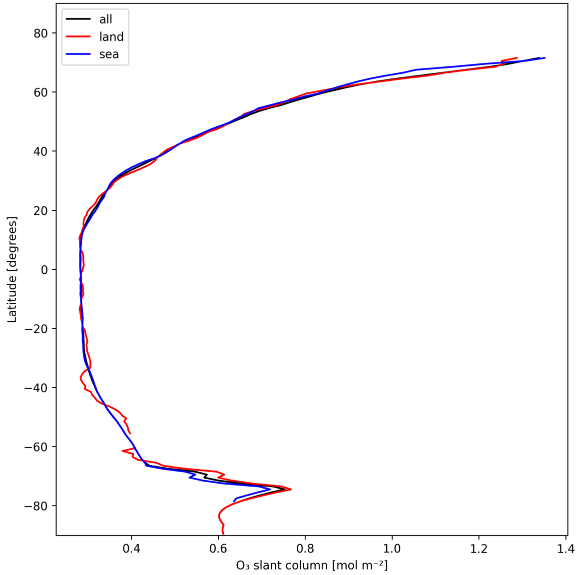
Figure 19: Zonal average of “O 3 slant column” for 2025-01-31 to 2025-01-31.
