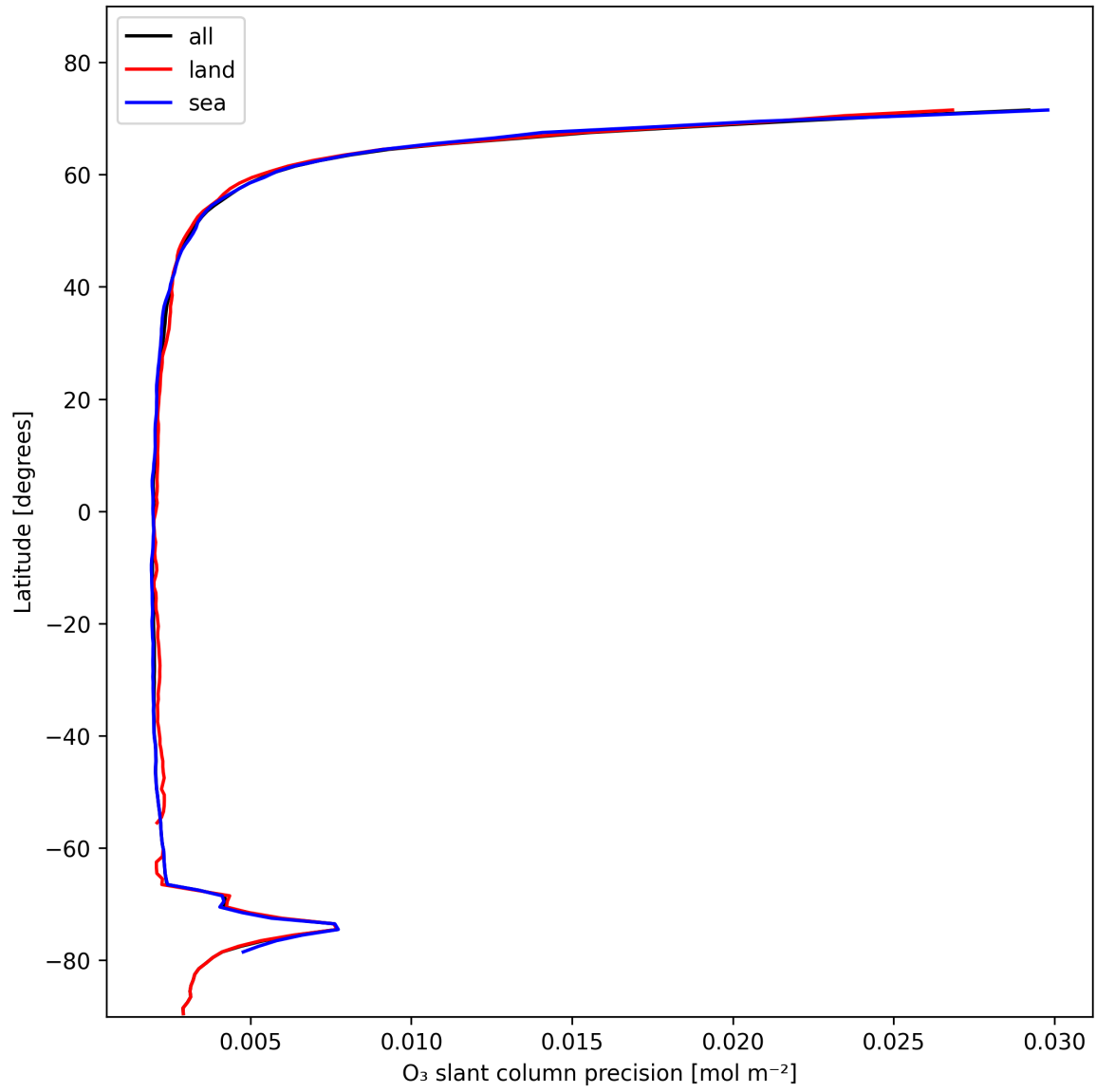
Figure 20: Zonal average of "O 3 slant column precision" for 2025-01-31 to 2025-01-31.
