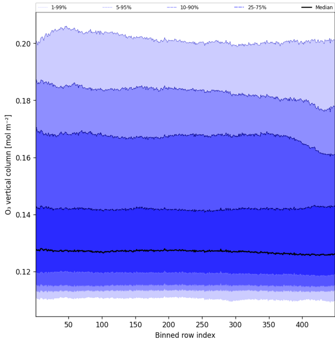
Figure 41: Along track statistics of “ \text{O}_3 vertical column” for 2025-02-01 to 2025-02-02
