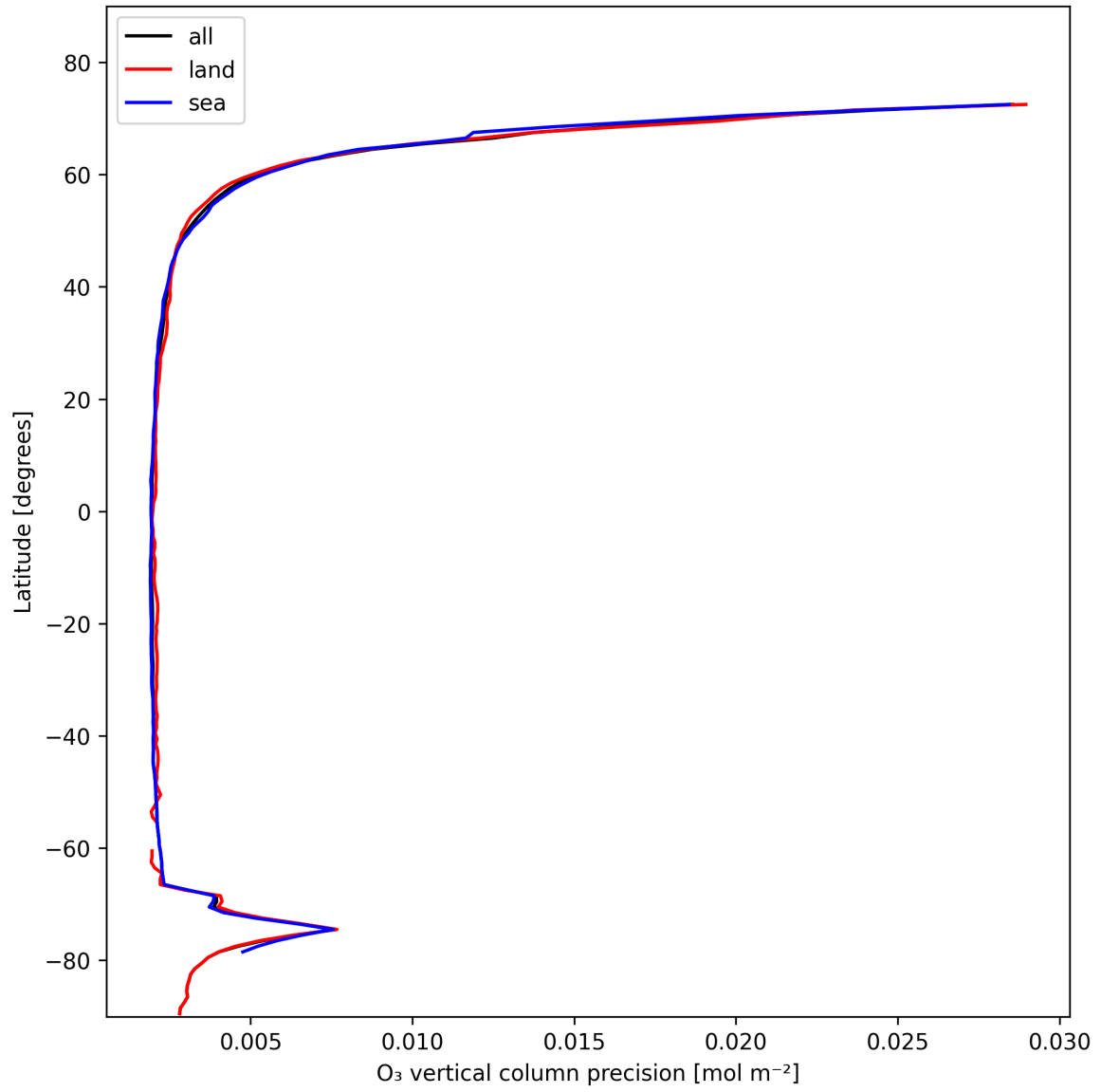
Figure 18: Zonal average of “O 3 vertical column precision” for 2025-02-01 to 2025-02-02.
