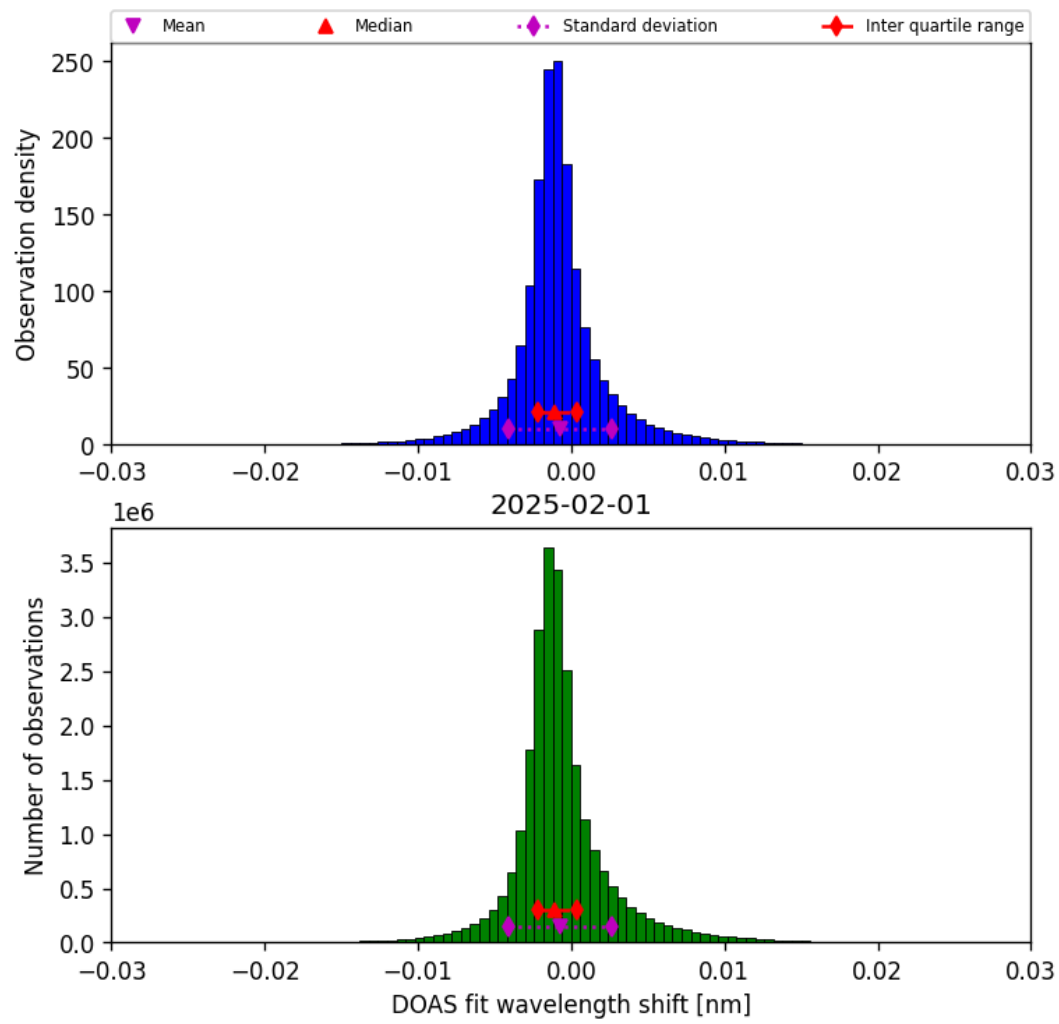
Figure 35: Histogram of “DOAS fit wavelength shift” for 2025-02-01 to 2025-02-02
