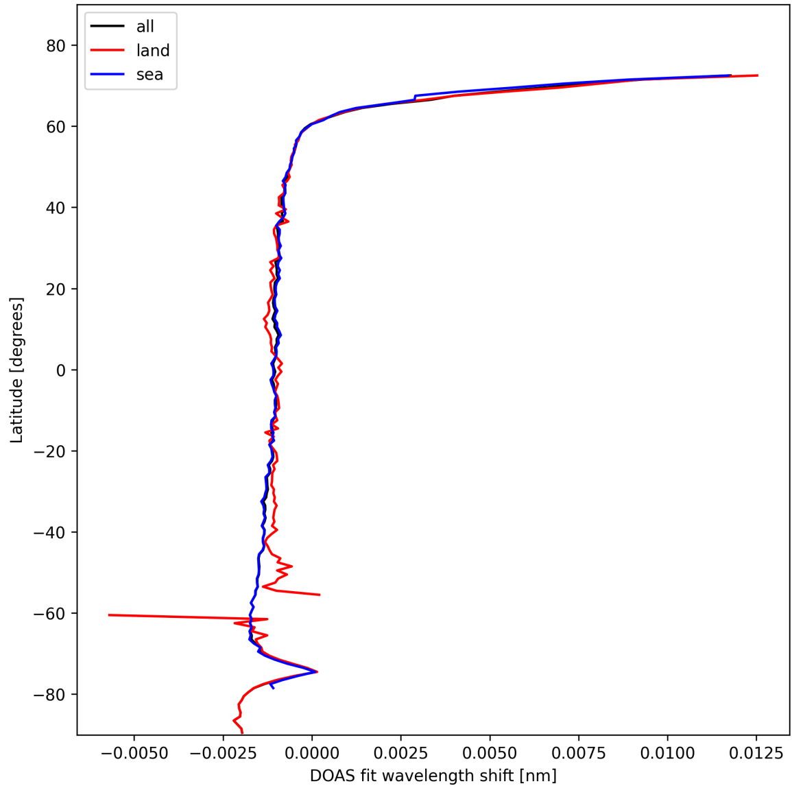
Figure 23: Zonal average of “DOAS fit wavelength shift” for 2025-02-01 to 2025-02-02.
