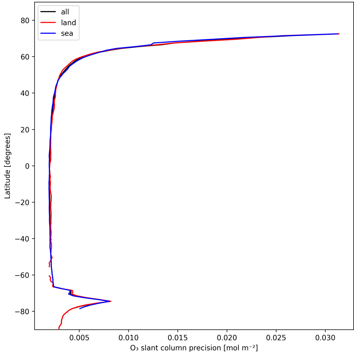
Figure 20: Zonal average of "O 3 slant column precision" for 2025-02-01 to 2025-02-02.
