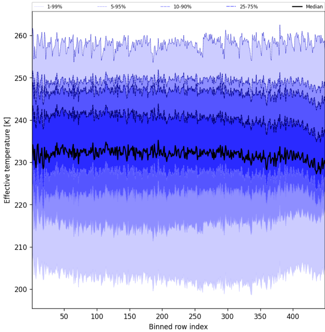
Figure 50: Along track statistics of “Effective temperature” for 2025-02-01 to 2025-02-02
