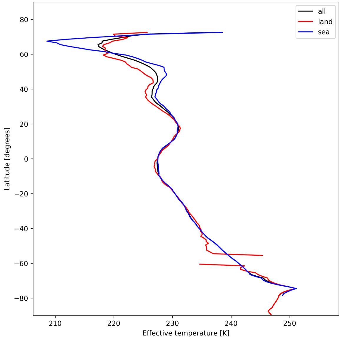
Figure 26: Zonal average of “Effective temperature” for 2025-02-01 to 2025-02-02.
