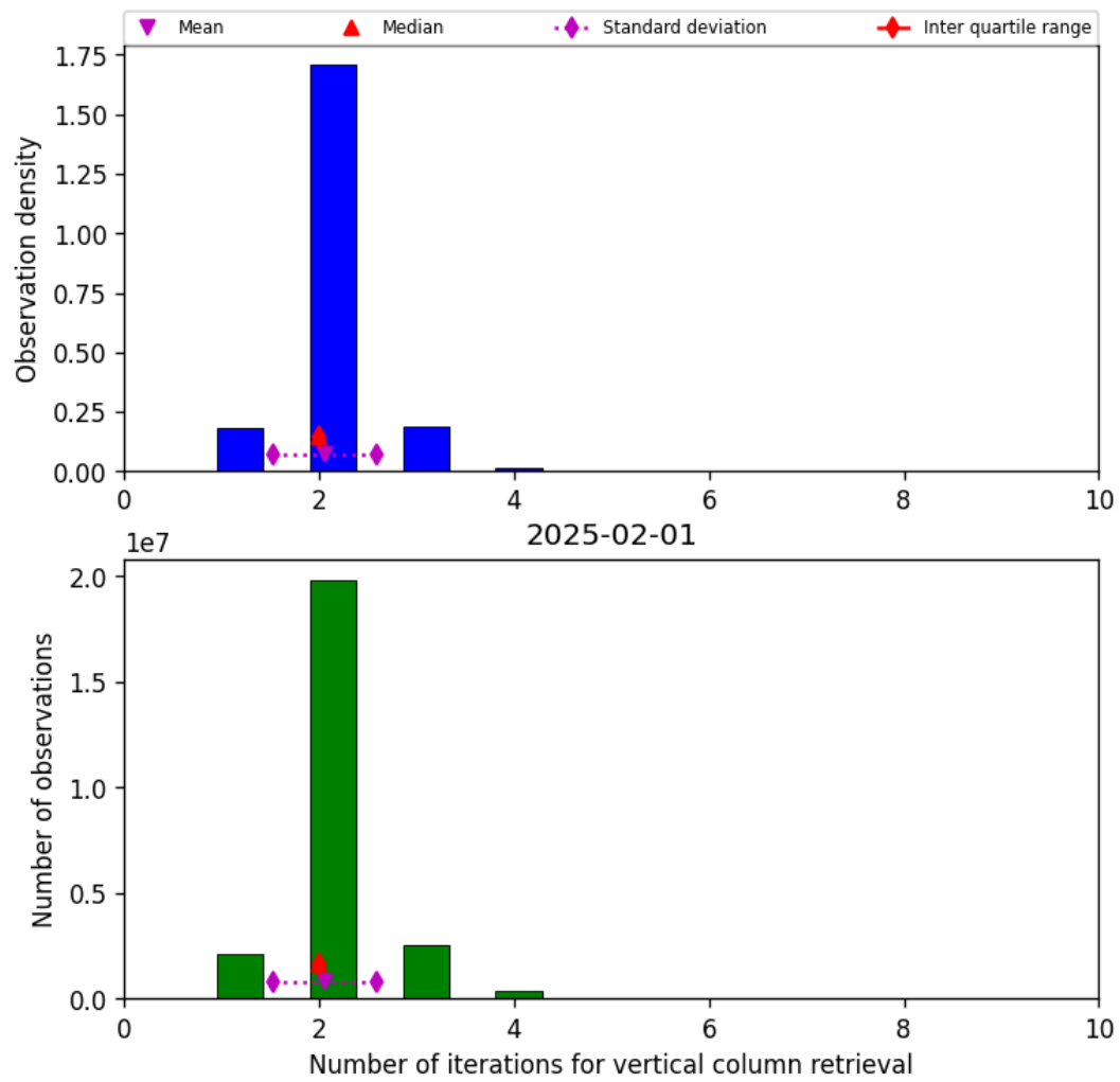
Figure 39: Histogram of “Number of iterations for vertical column retrieval” for 2025-02-01 to 2025-02-02
