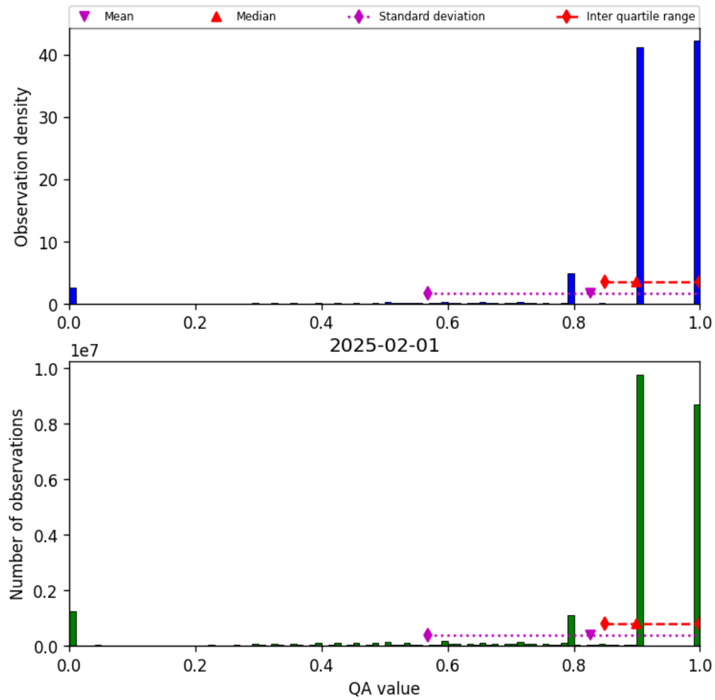
Figure 28: Histogram of “QA value” for 2025-02-01 to 2025-02-02
