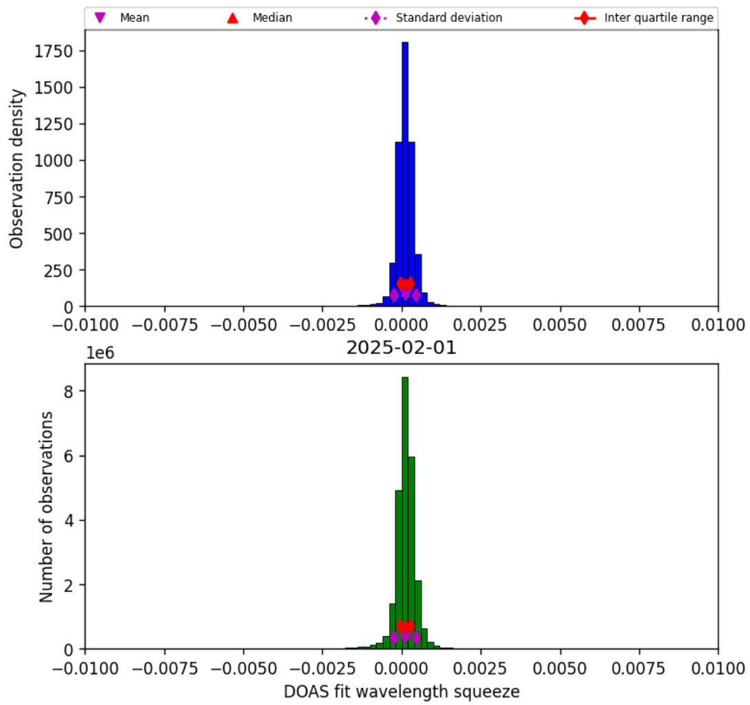
Figure 36: Histogram of “DOAS fit wavelength squeeze” for 2025-02-01 to 2025-02-02
