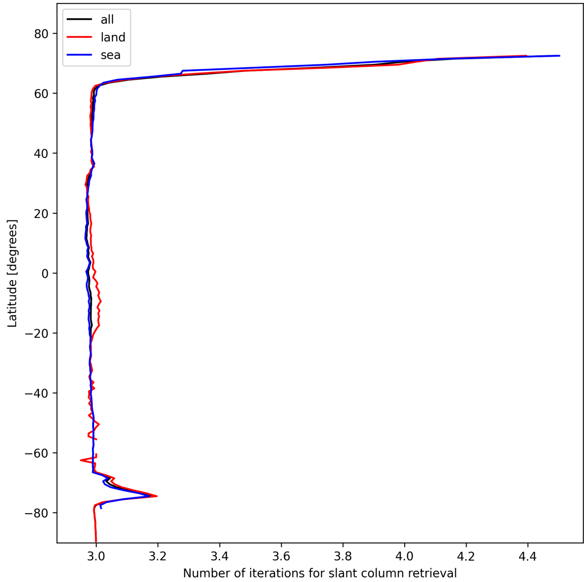
Figure 21: Zonal average of “Number of iterations for slant column retrieval” for 2025-02-01 to 2025-02-02.
