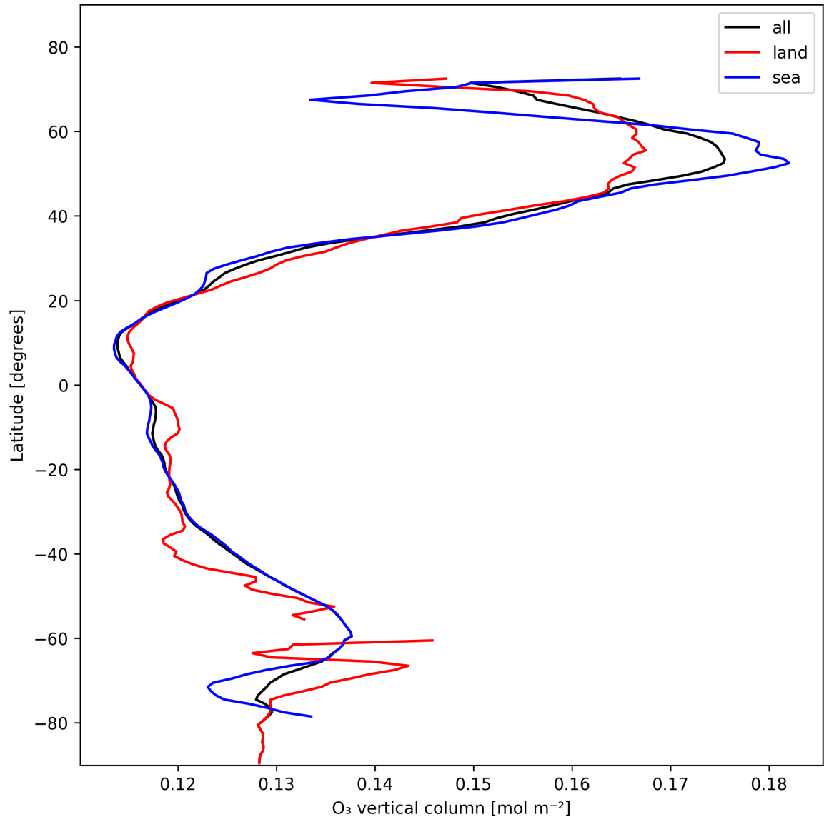
Figure 17: Zonal average of “O 3 vertical column” for 2025-02-01 to 2025-02-02.
