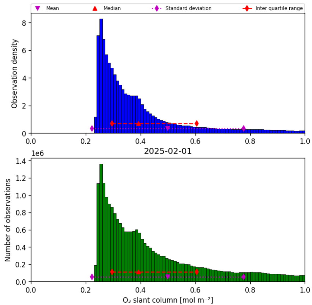
Figure 31: Histogram of “O 3 slant column” for 2025-02-01 to 2025-02-02
