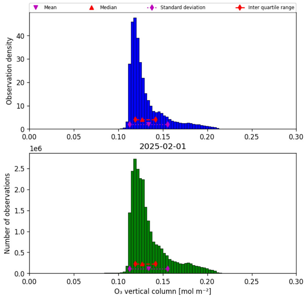
Figure 29: Histogram of “O 3 vertical column” for 2025-02-01 to 2025-02-02
