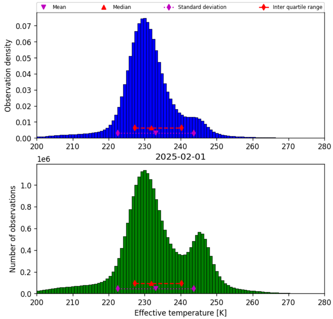
Figure 38: Histogram of “Effective temperature” for 2025-02-01 to 2025-02-02
