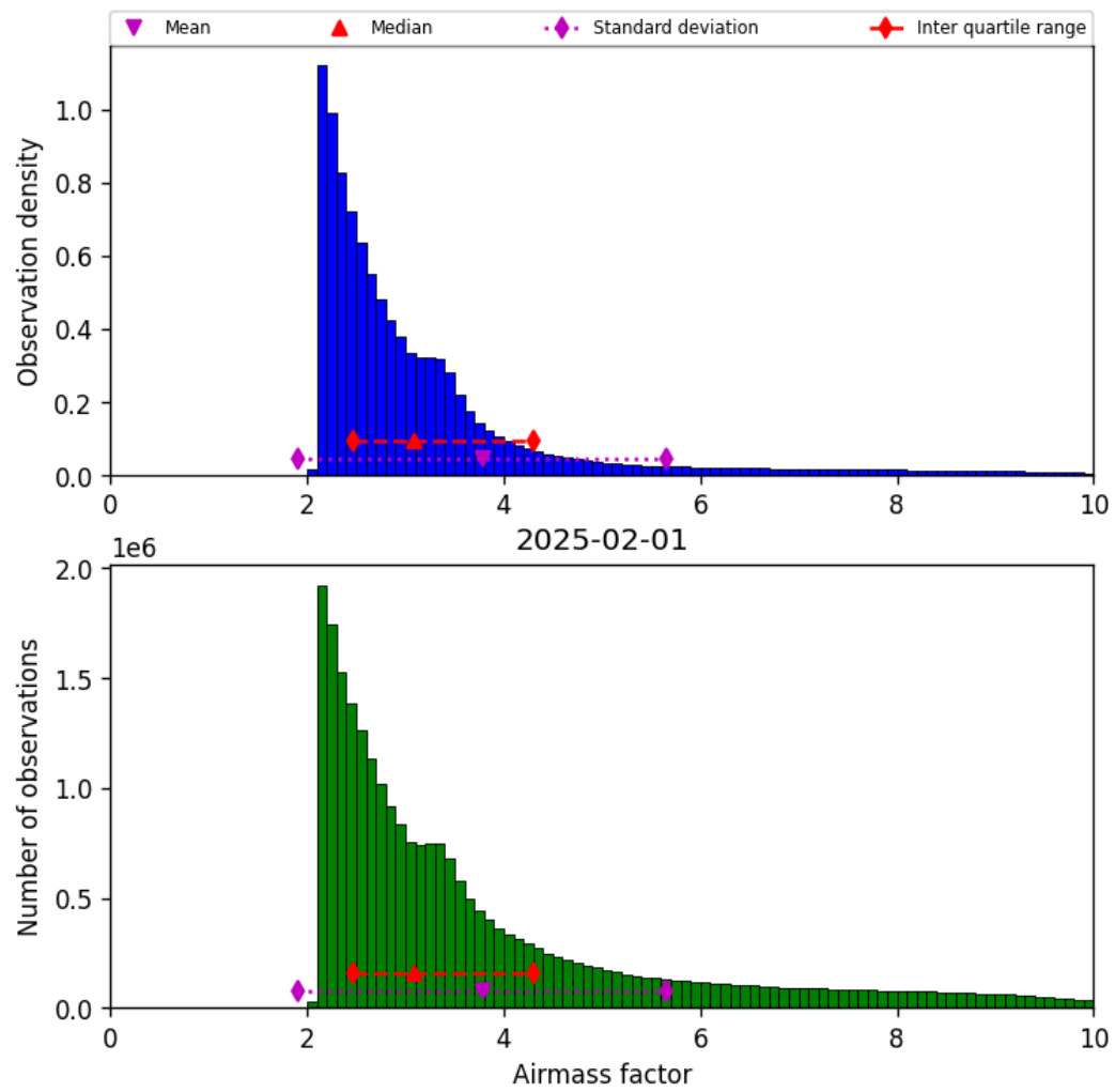
Figure 37: Histogram of “Airmass factor” for 2025-02-01 to 2025-02-02
