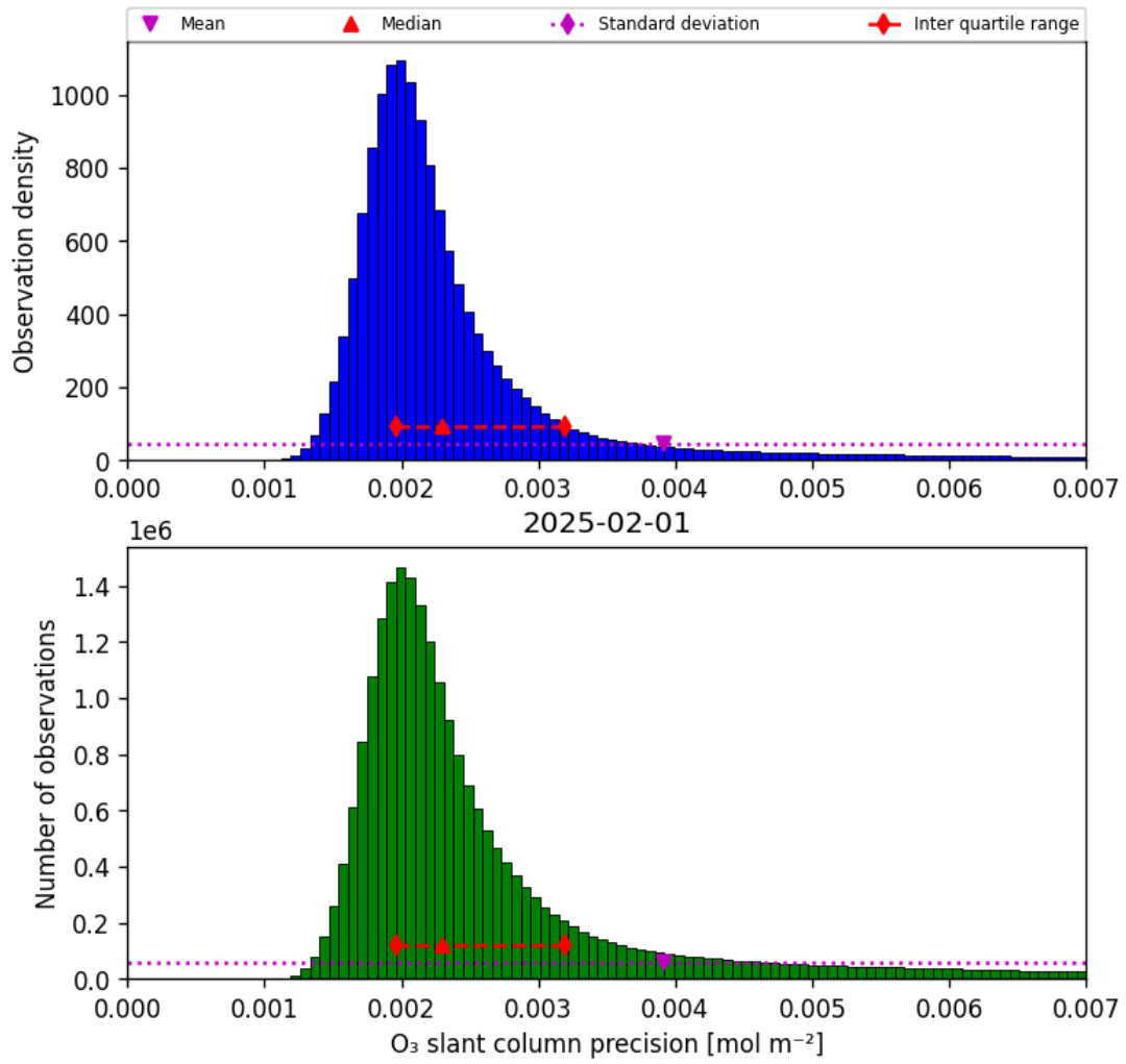
Figure 32: Histogram of “O 3 slant column precision” for 2025-02-01 to 2025-02-02
