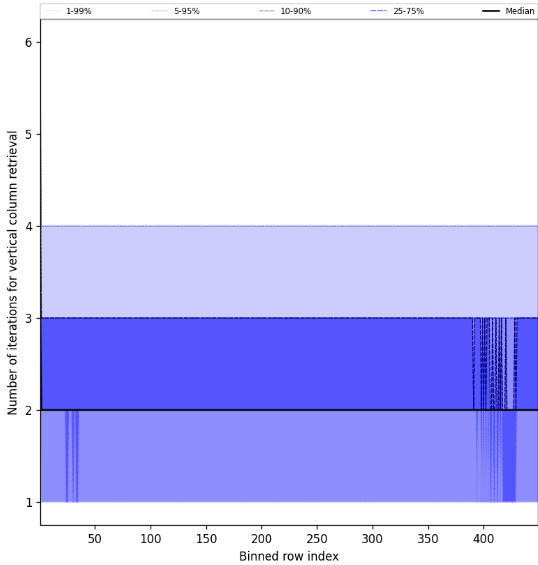
Figure 51: Along track statistics of “Number of iterations for vertical column retrieval” for 2025-02-01 to 2025-02-02
