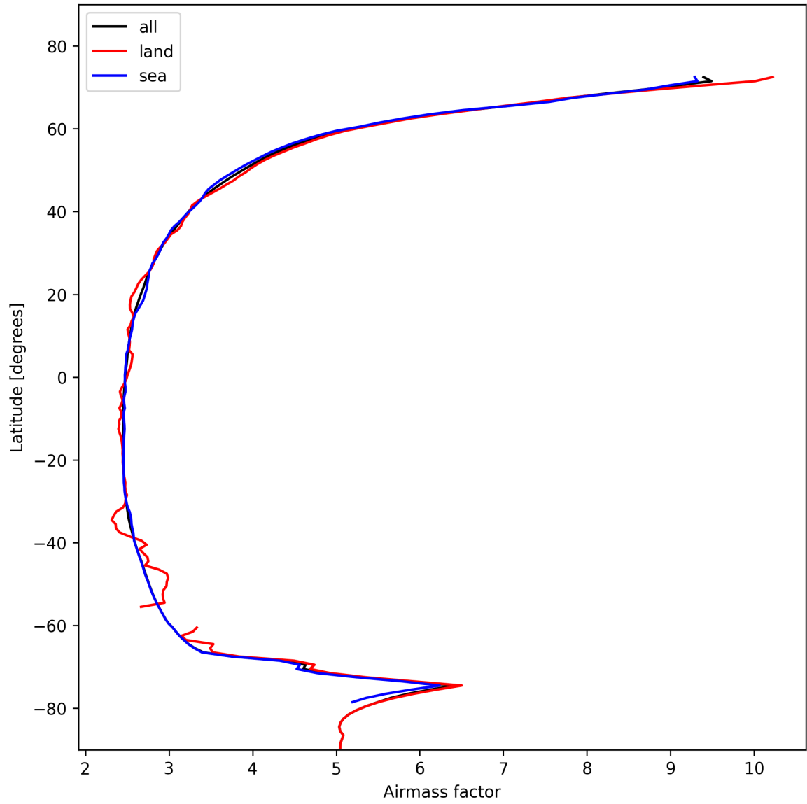
Figure 25: Zonal average of “Airmass factor” for 2025-02-01 to 2025-02-02.
