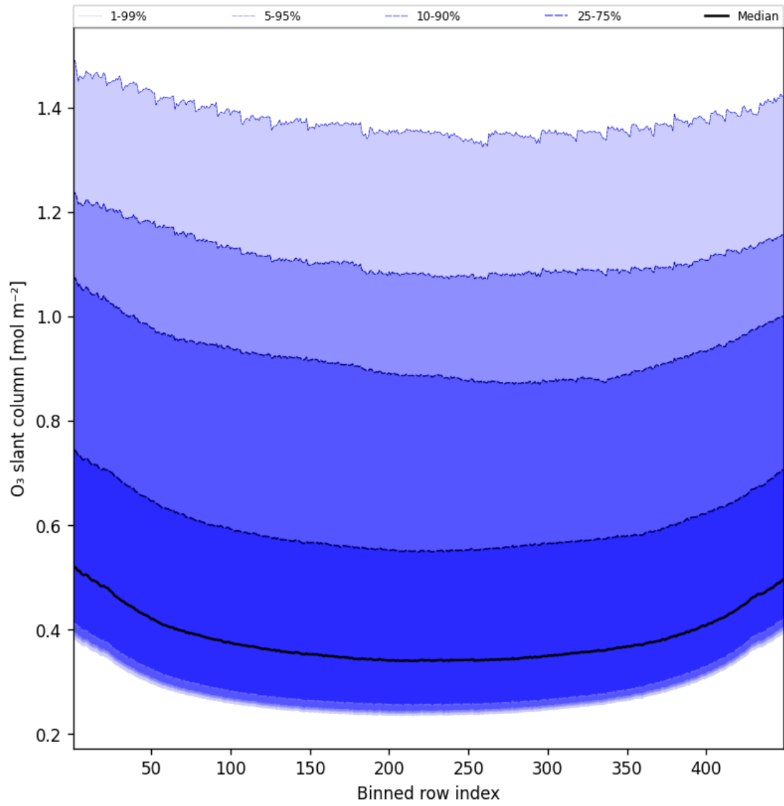
Figure 43: Along track statistics of “O 3 slant column” for 2025-02-01 to 2025-02-02
