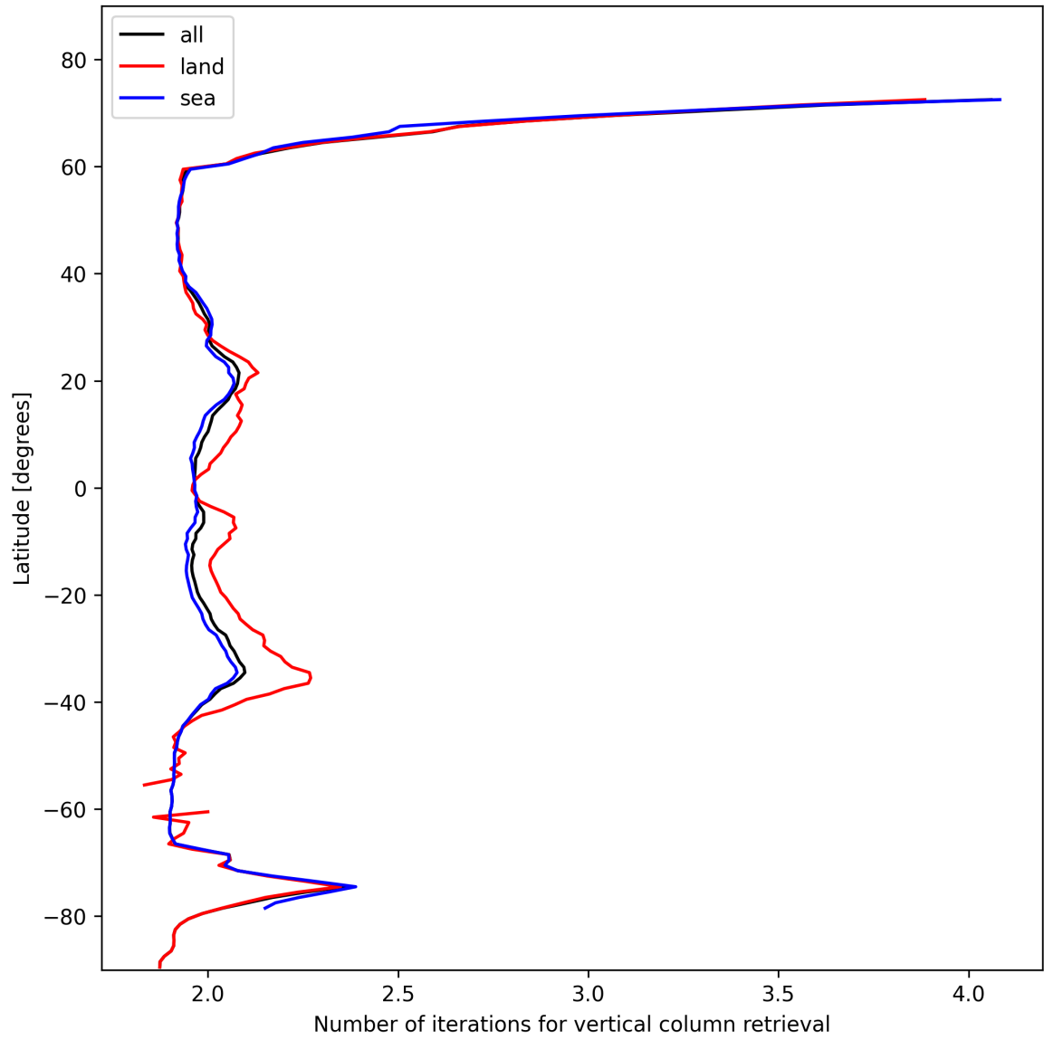
Figure 27: Zonal average of “Number of iterations for vertical column retrieval” for 2025-02-01 to 2025-02-02.
