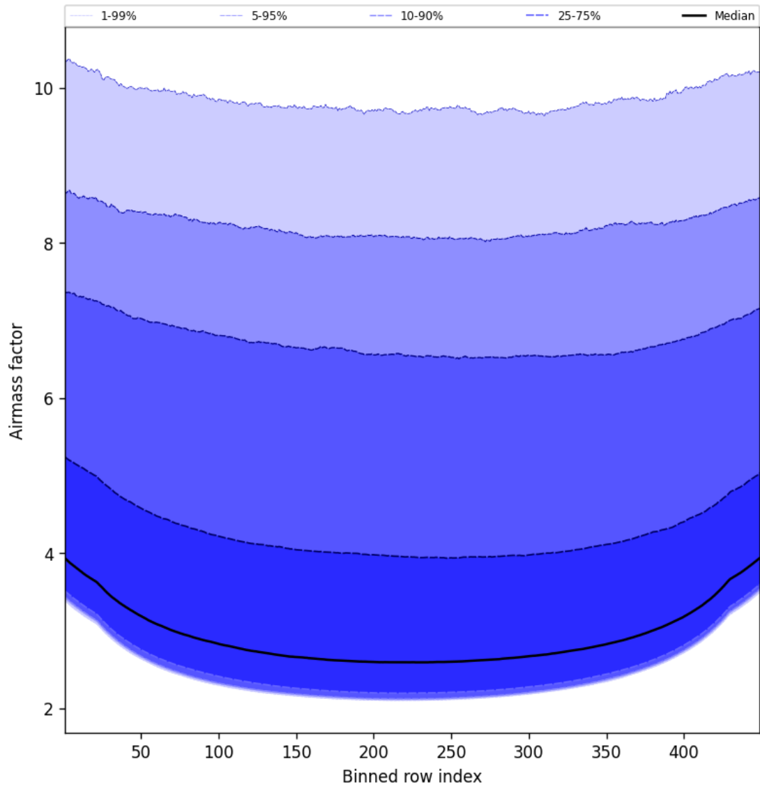
Figure 49: Along track statistics of “Airmass factor” for 2025-02-01 to 2025-02-02
