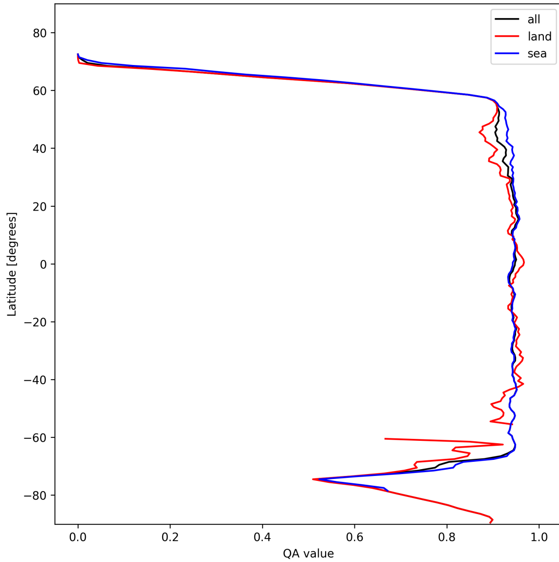
Figure 16: Zonal average of “QA value” for 2025-02-01 to 2025-02-02.
