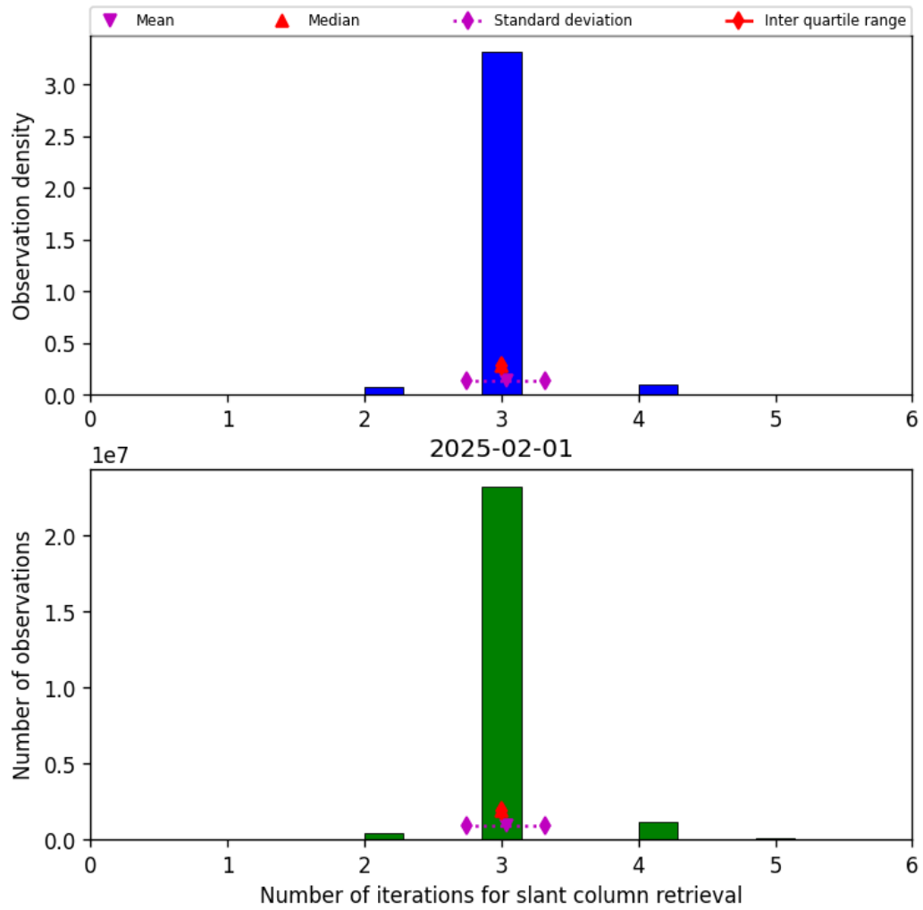
Figure 33: Histogram of “Number of iterations for slant column retrieval” for 2025-02-01 to 2025-02-02
