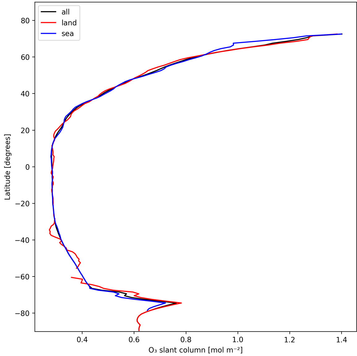
Figure 19: Zonal average of “O 3 slant column” for 2025-02-01 to 2025-02-02.
