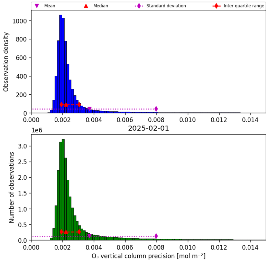
Figure 30: Histogram of “O 3 vertical column precision” for 2025-02-01 to 2025-02-02
