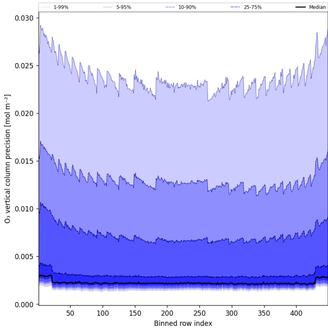
Figure 42: Along track statistics of “O 3 vertical column precision” for 2025-02-01 to 2025-02-02
