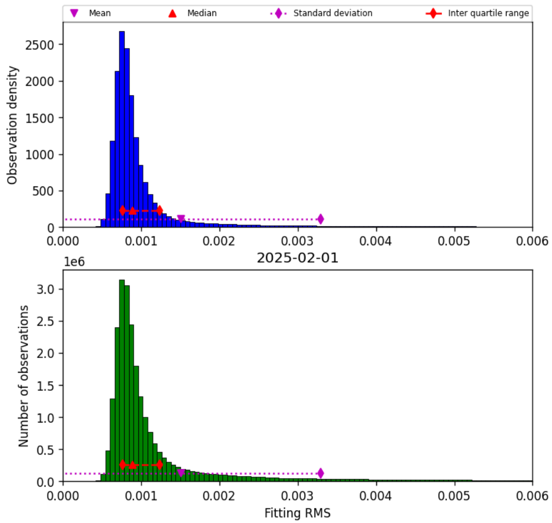
Figure 34: Histogram of “Fitting RMS” for 2025-02-01 to 2025-02-02
