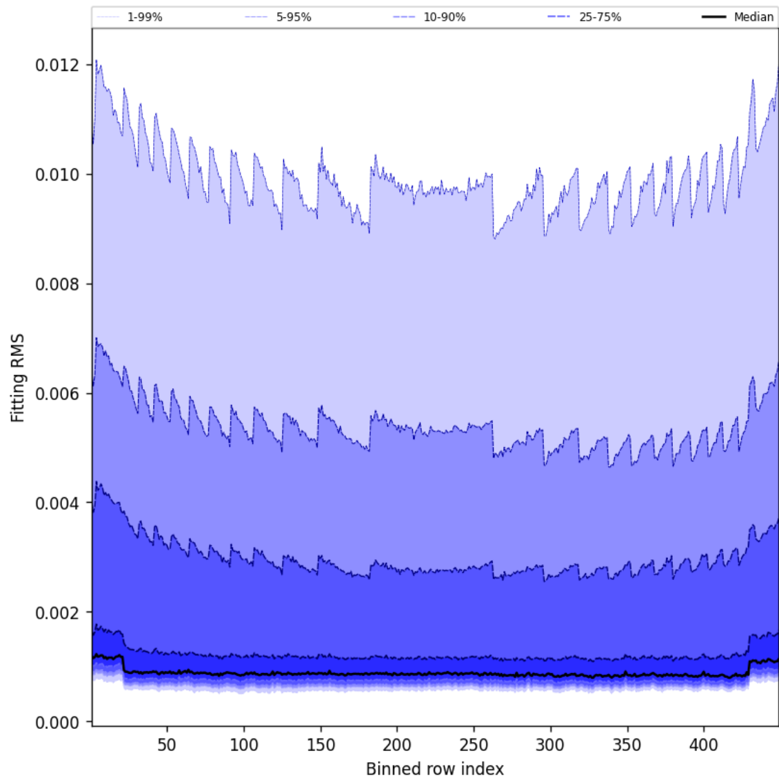
Figure 46: Along track statistics of “Fitting RMS” for 2025-02-01 to 2025-02-02
