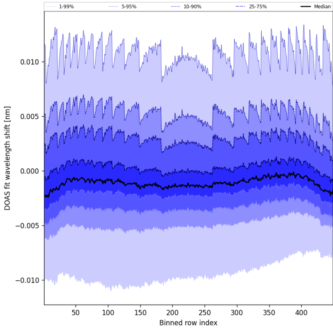
Figure 47: Along track statistics of “DOAS fit wavelength shift” for 2025-02-01 to 2025-02-02
