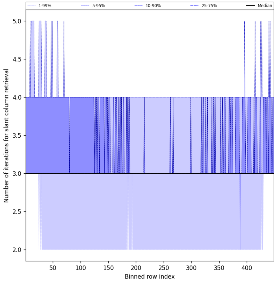
Figure 45: Along track statistics of “Number of iterations for slant column retrieval” for 2025-02-01 to 2025-02-02
