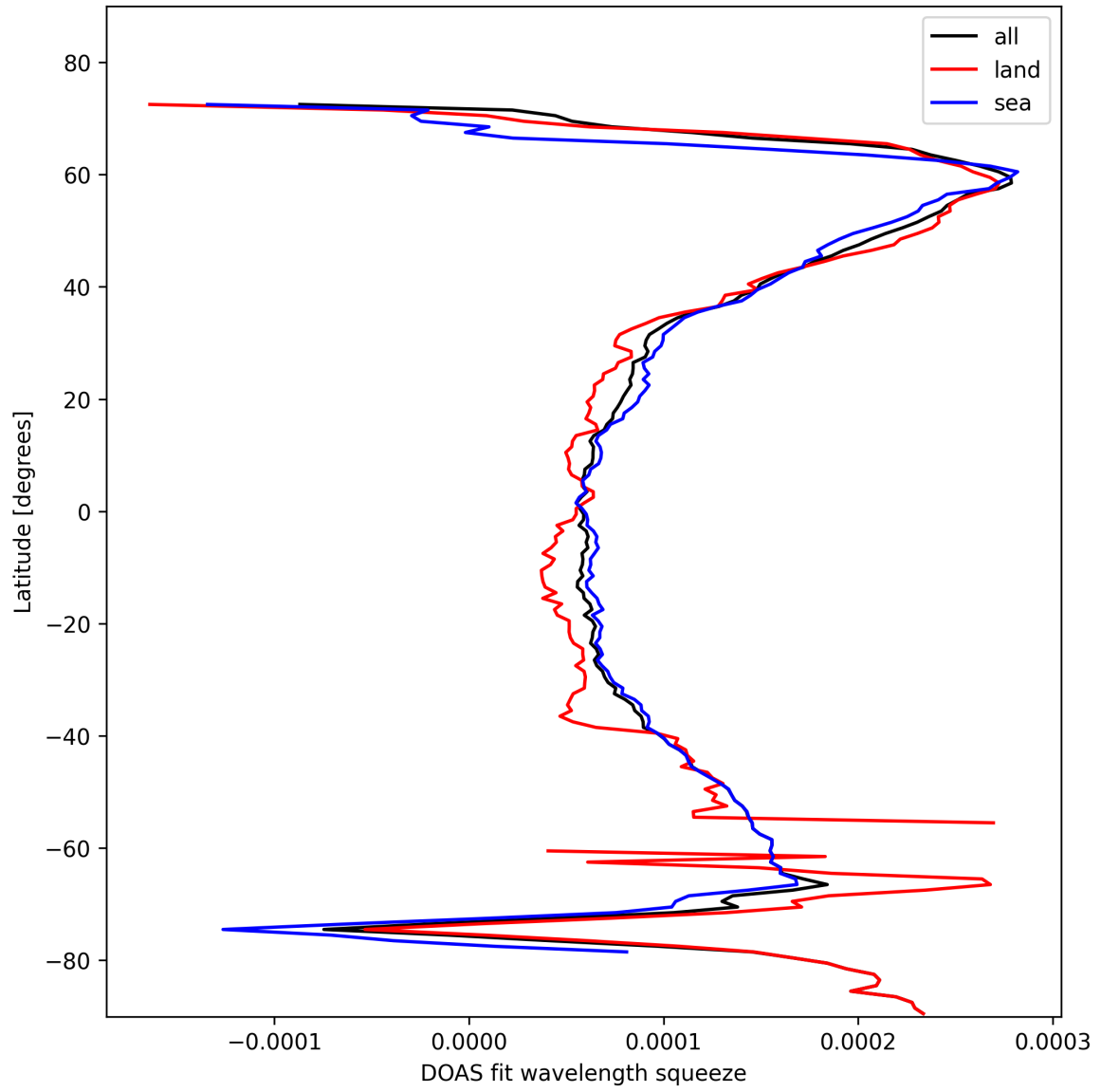
Figure 24: Zonal average of “DOAS fit wavelength squeeze” for 2025-02-01 to 2025-02-02.
