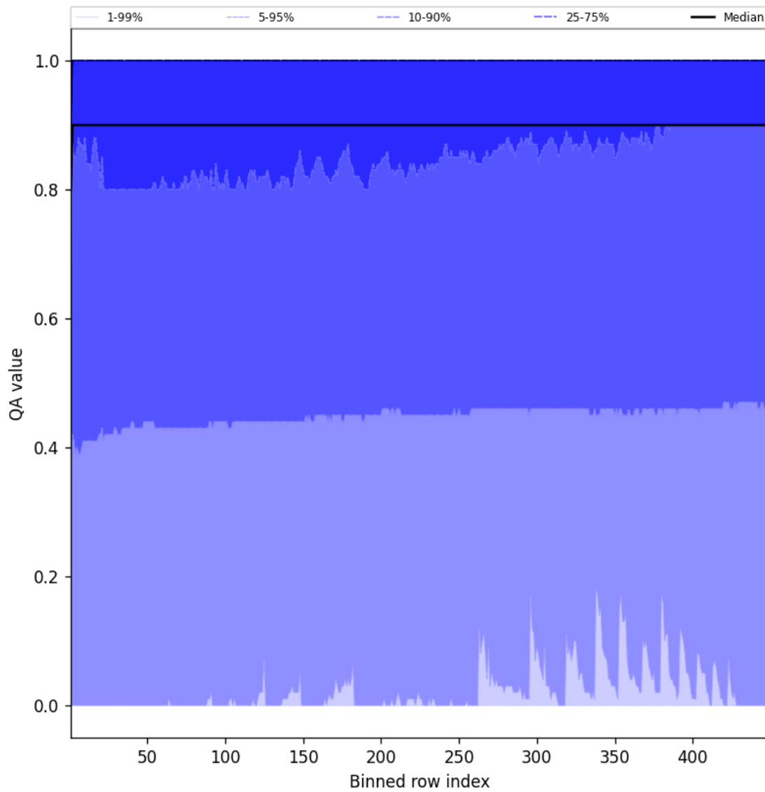
Figure 40: Along track statistics of “QA value” for 2025-02-01 to 2025-02-02
