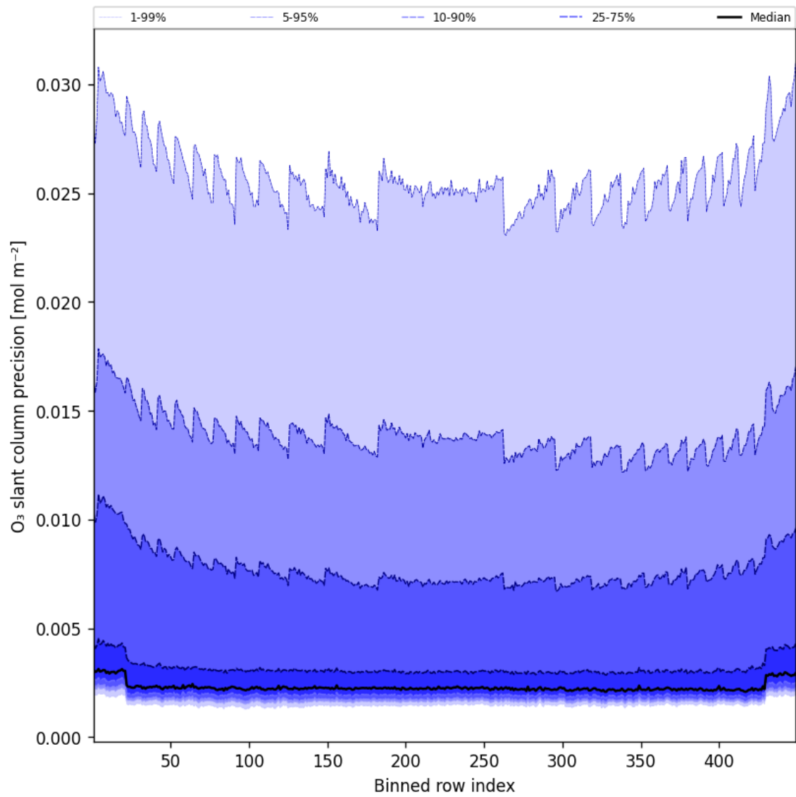
Figure 44: Along track statistics of “O 3 slant column precision” for 2025-02-01 to 2025-02-02
