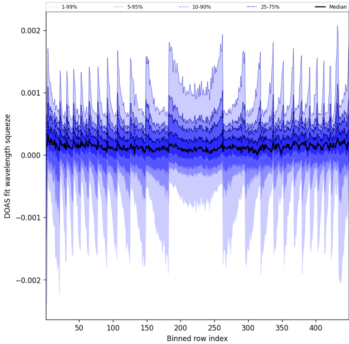
Figure 48: Along track statistics of “DOAS fit wavelength squeeze” for 2025-02-01 to 2025-02-02
