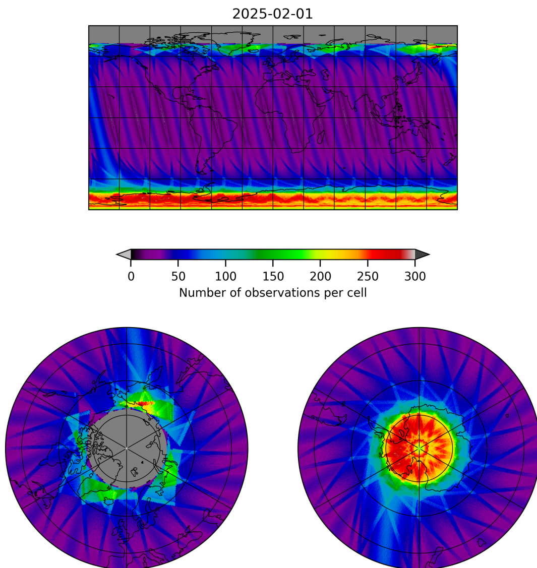
Figure 15: Map of the number of observations for 2025-02-01 to 2025-02-02
