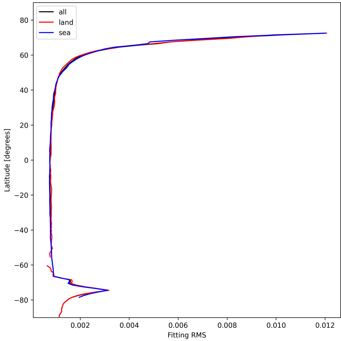
Figure 22: Zonal average of “Fitting RMS” for 2025-02-01 to 2025-02-02.
