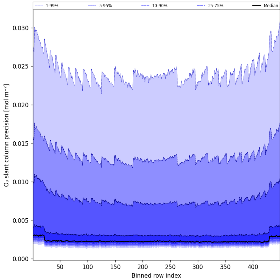
Figure 44: Along track statistics of “O 3 slant column precision” for 2025-02-03 to 2025-02-04
