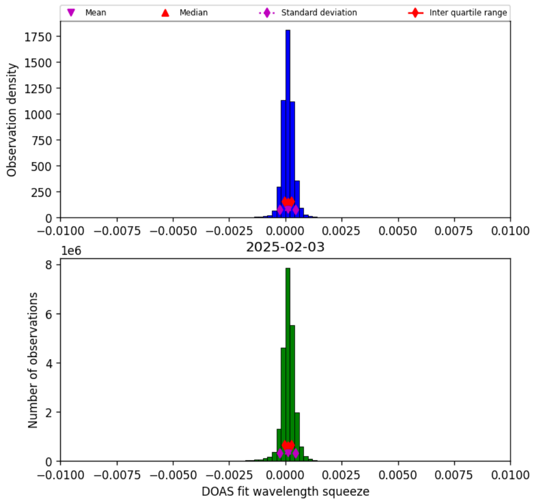
Figure 36: Histogram of “DOAS fit wavelength squeeze” for 2025-02-03 to 2025-02-04
