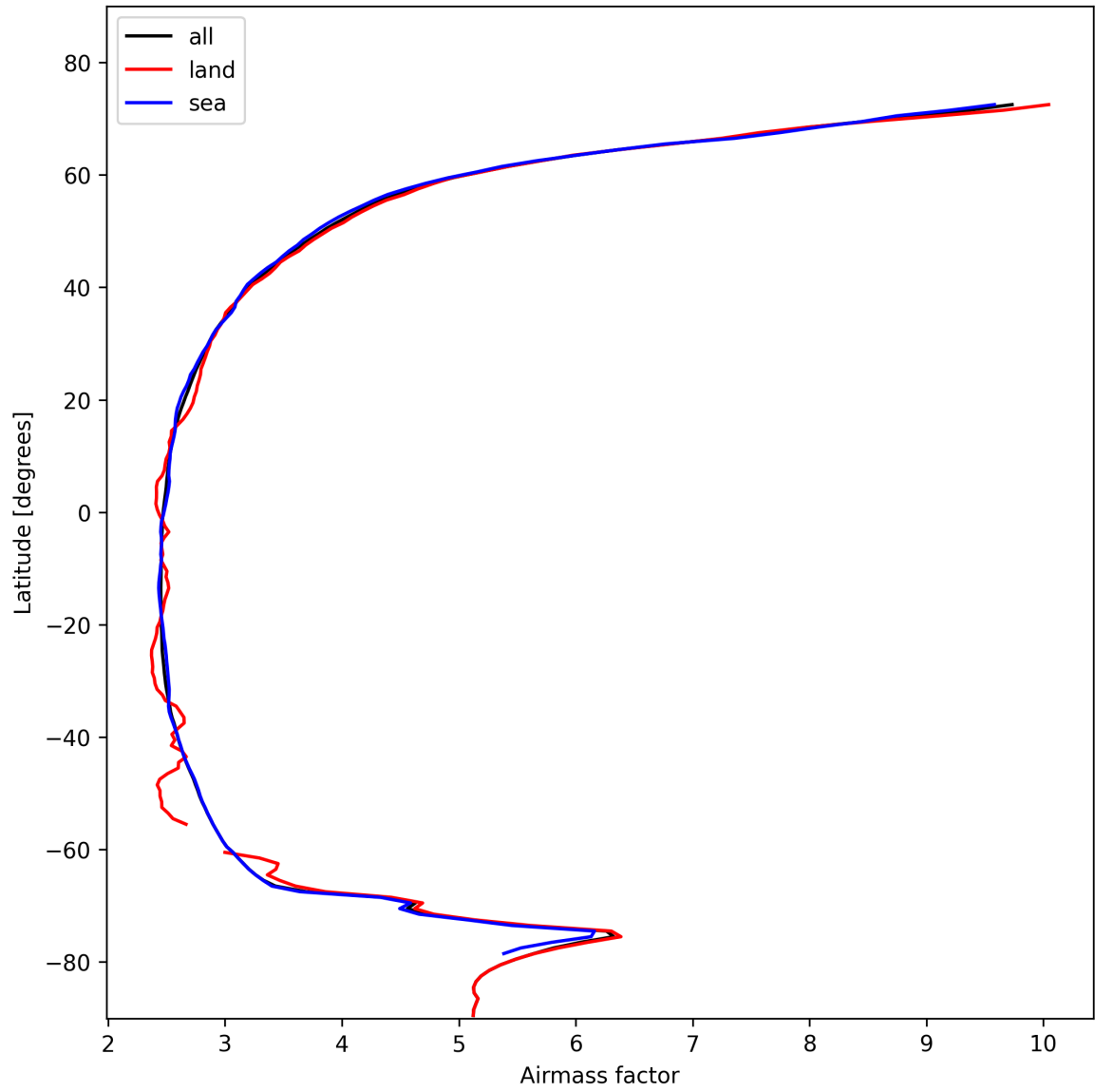
Figure 25: Zonal average of “Airmass factor” for 2025-02-03 to 2025-02-04.
