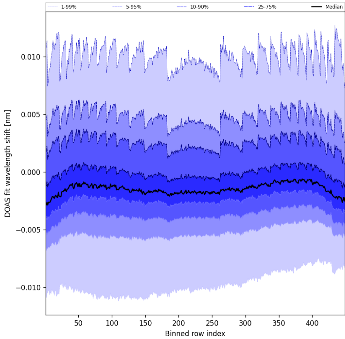
Figure 47: Along track statistics of “DOAS fit wavelength shift” for 2025-02-03 to 2025-02-04
