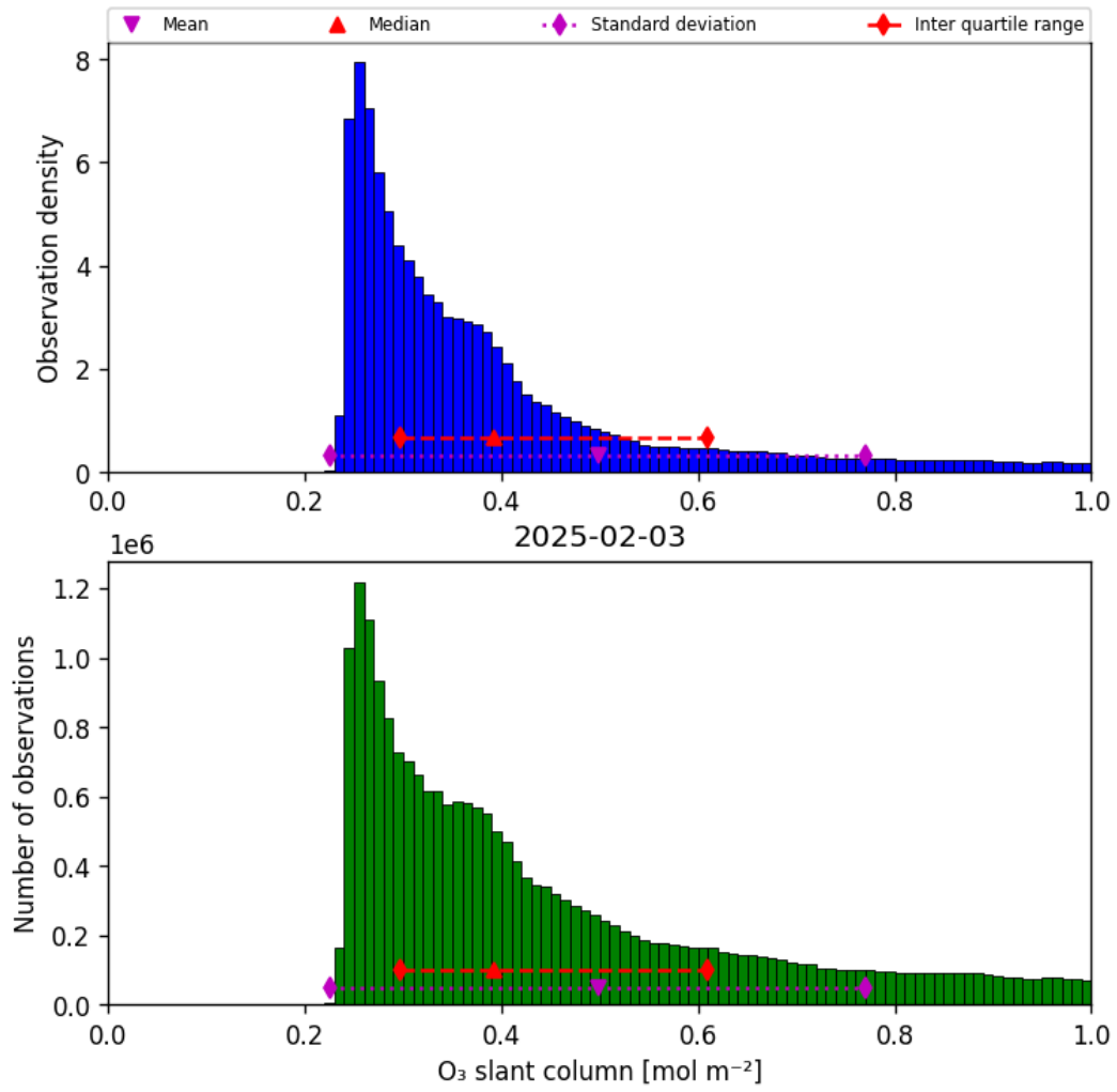
Figure 31: Histogram of “O 3 slant column” for 2025-02-03 to 2025-02-04
