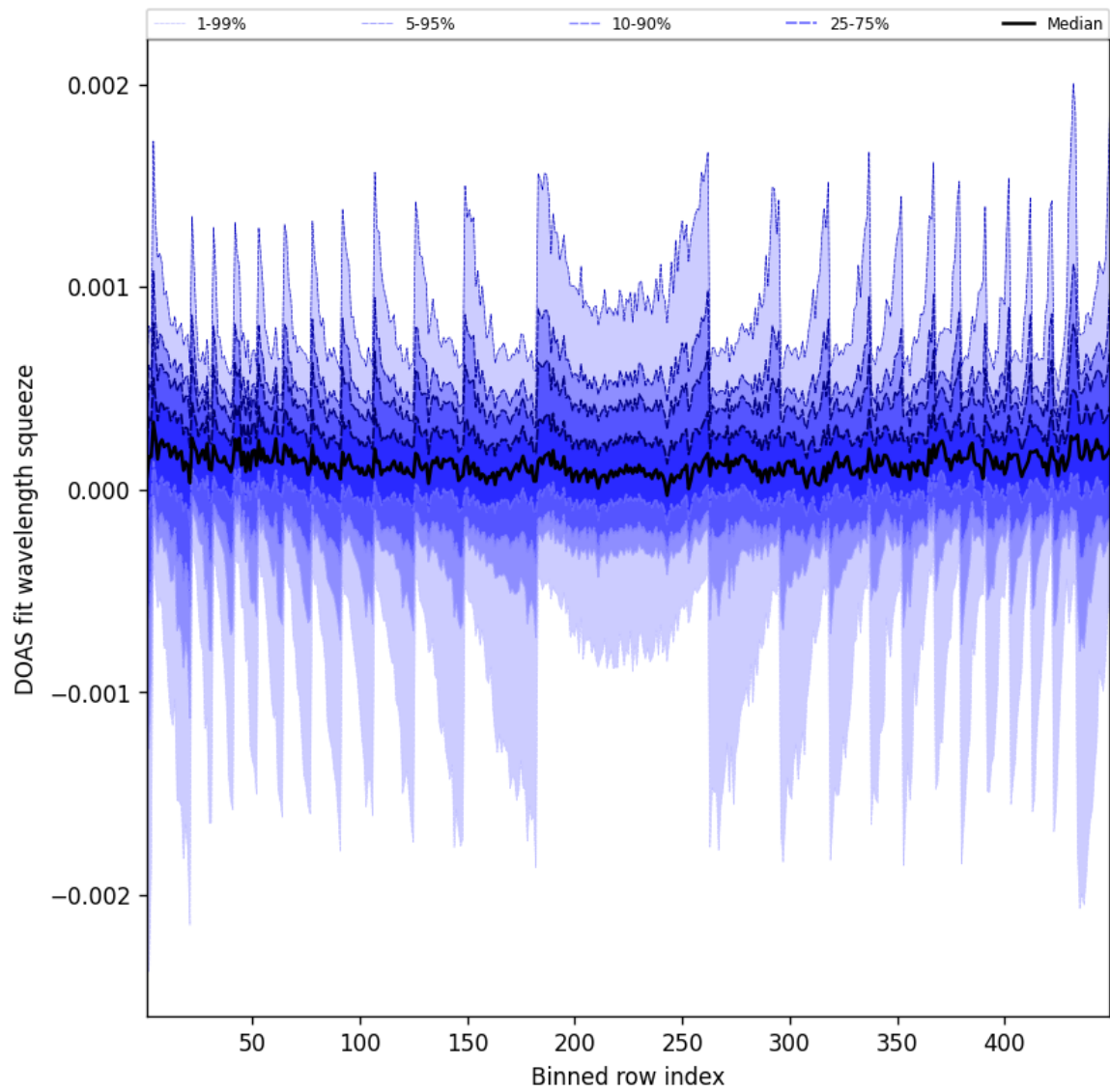
Figure 48: Along track statistics of “DOAS fit wavelength squeeze” for 2025-02-03 to 2025-02-04
