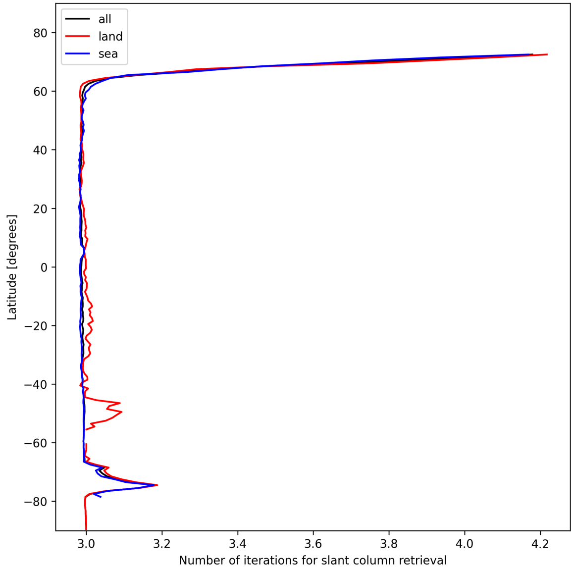
Figure 21: Zonal average of “Number of iterations for slant column retrieval” for 2025-02-03 to 2025-02-04.
