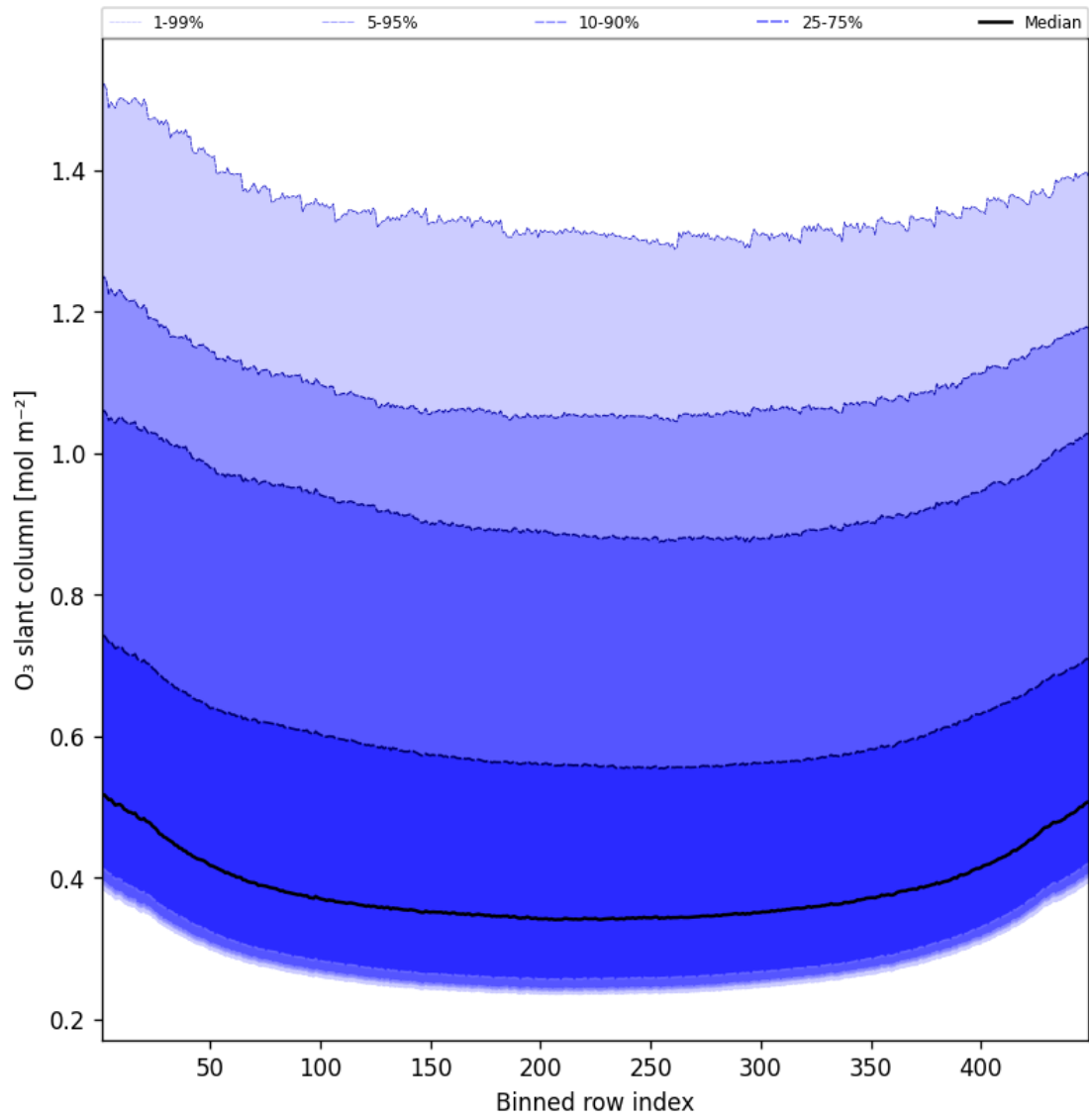
Figure 43: Along track statistics of “O 3 slant column” for 2025-02-03 to 2025-02-04
