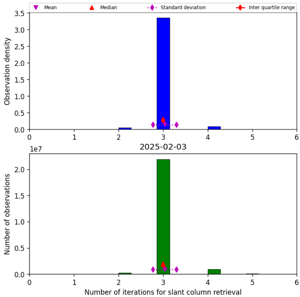
Figure 33: Histogram of “Number of iterations for slant column retrieval” for 2025-02-03 to 2025-02-04
