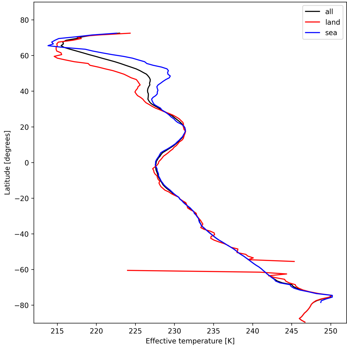
Figure 26: Zonal average of “Effective temperature” for 2025-02-03 to 2025-02-04.
