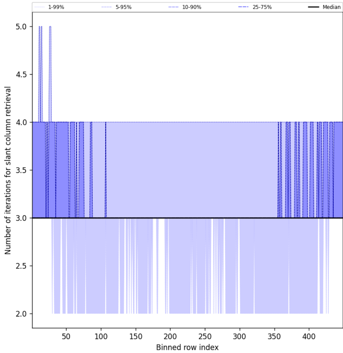
Figure 45: Along track statistics of “Number of iterations for slant column retrieval” for 2025-02-03 to 2025-02-04
