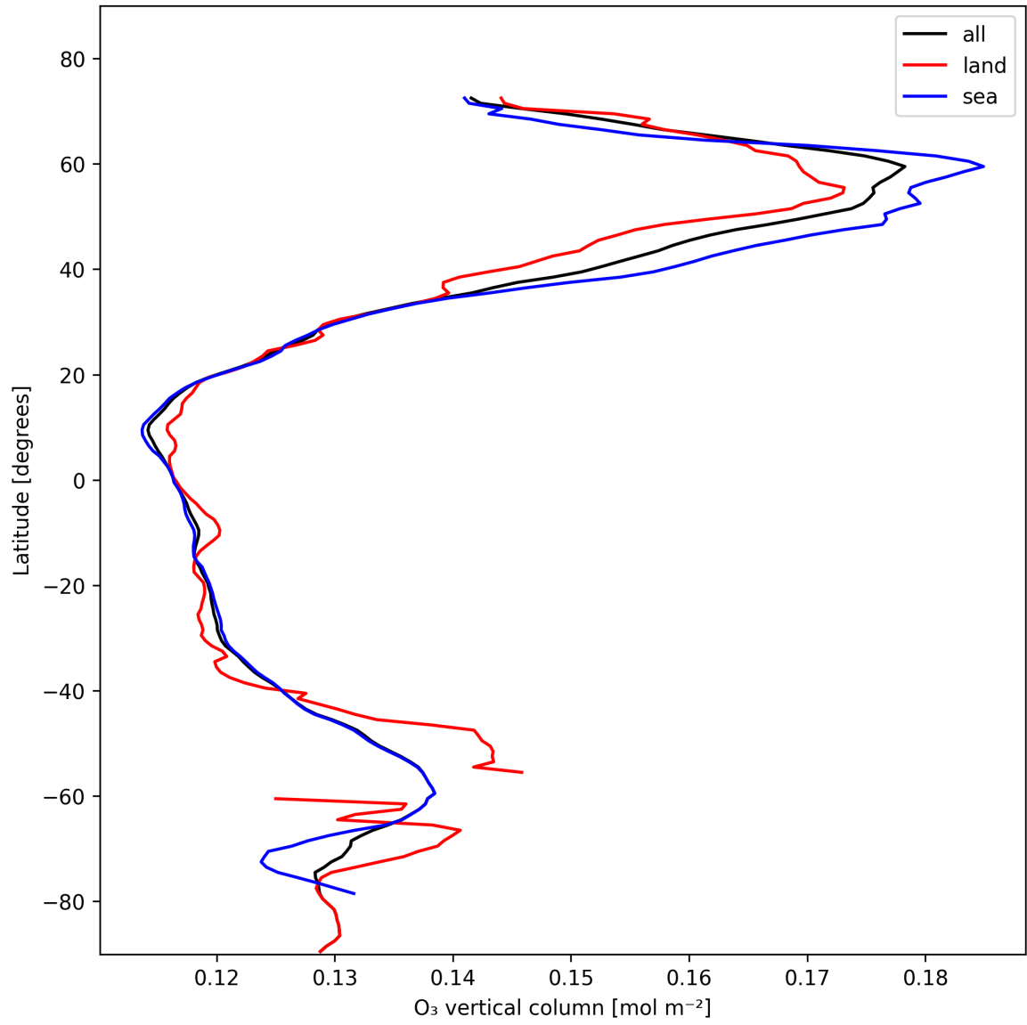
Figure 17: Zonal average of “O 3 vertical column” for 2025-02-03 to 2025-02-04.
