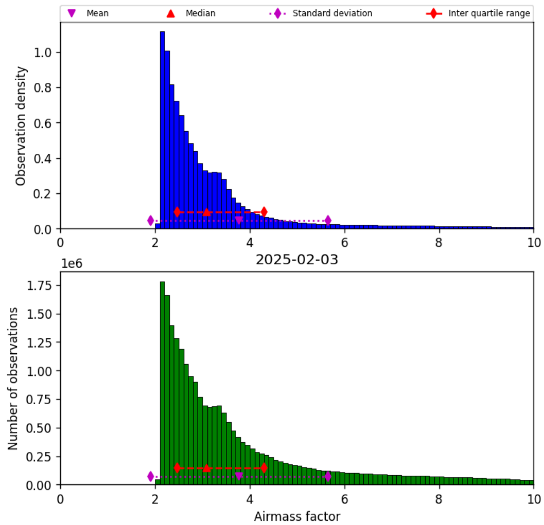
Figure 37: Histogram of “Airmass factor” for 2025-02-03 to 2025-02-04
