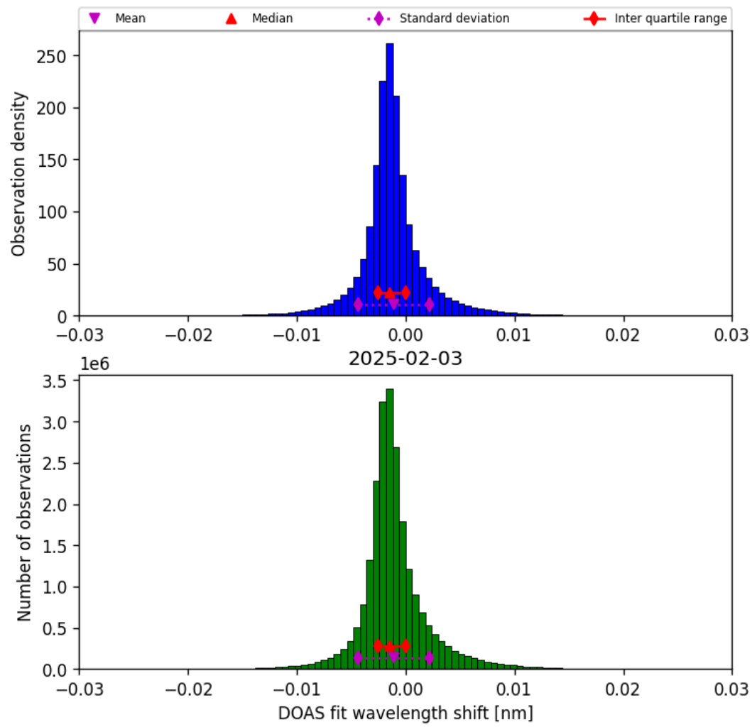
Figure 35: Histogram of “DOAS fit wavelength shift” for 2025-02-03 to 2025-02-04
