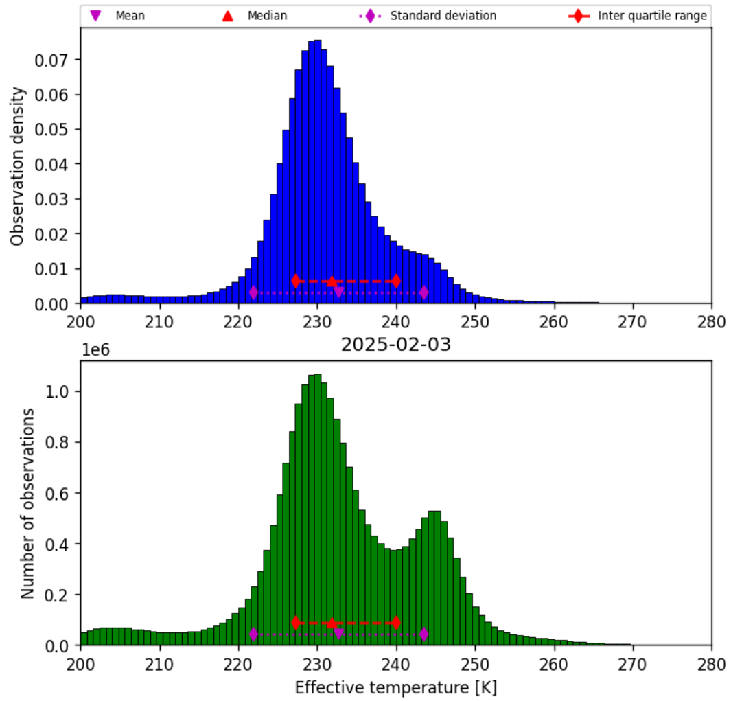
Figure 38: Histogram of “Effective temperature” for 2025-02-03 to 2025-02-04
