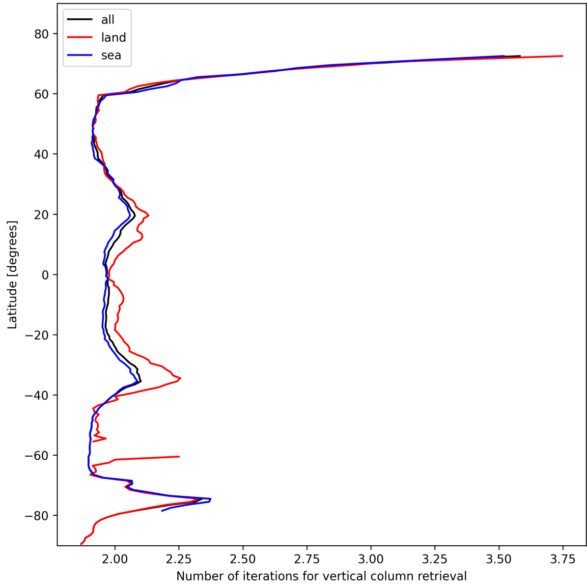
Figure 27: Zonal average of “Number of iterations for vertical column retrieval” for 2025-02-03 to 2025-02-04.
