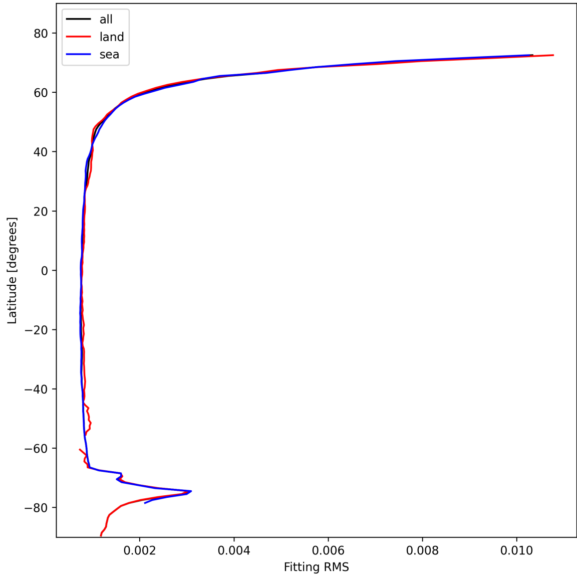
Figure 22: Zonal average of “Fitting RMS” for 2025-02-03 to 2025-02-04.
