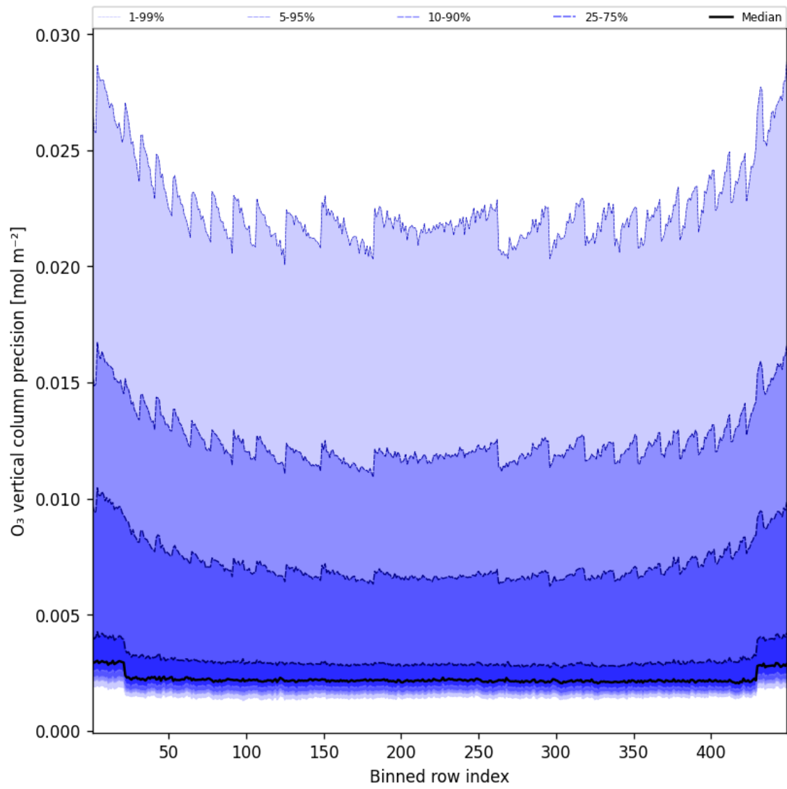
Figure 42: Along track statistics of “O 3 vertical column precision” for 2025-02-03 to 2025-02-04
