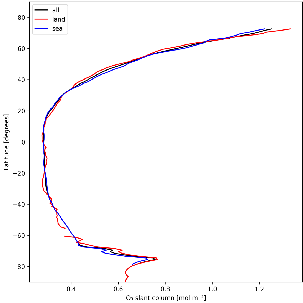
Figure 19: Zonal average of “O 3 slant column” for 2025-02-03 to 2025-02-04.
