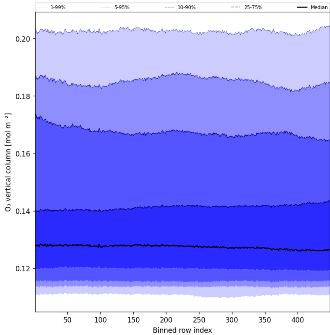
Figure 41: Along track statistics of “ O_3 vertical column” for 2025-02-03 to 2025-02-04
