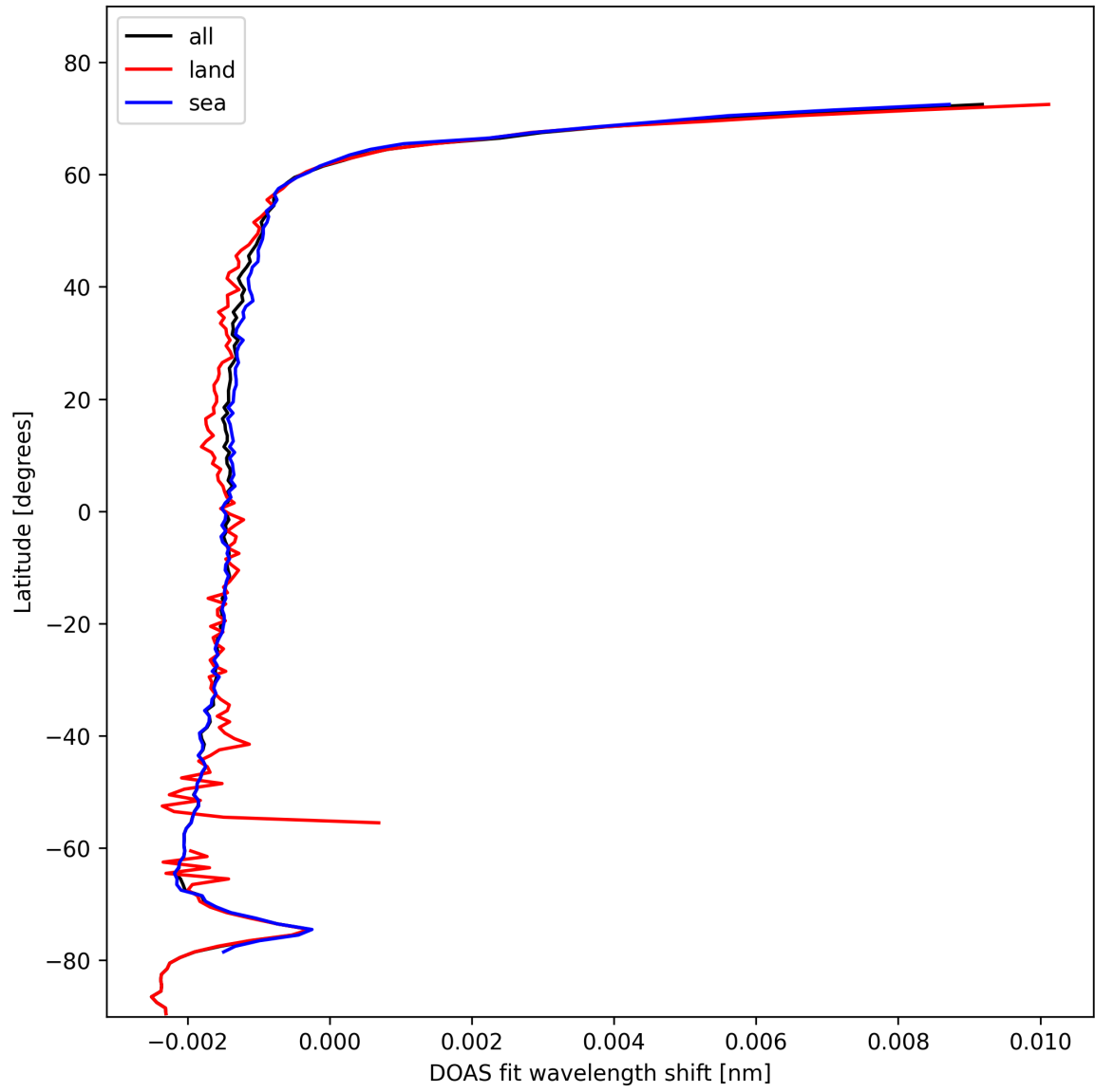
Figure 23: Zonal average of “DOAS fit wavelength shift” for 2025-02-03 to 2025-02-04.
