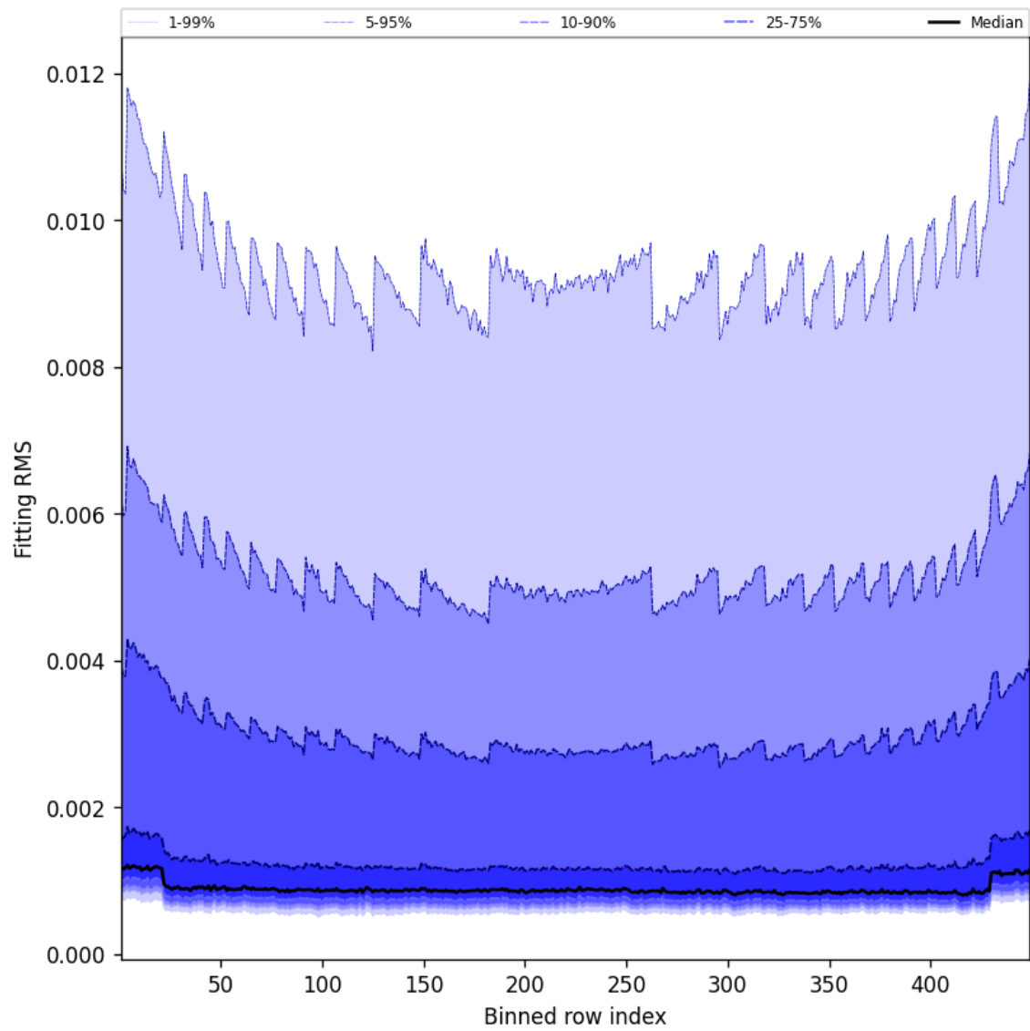
Figure 46: Along track statistics of “Fitting RMS” for 2025-02-03 to 2025-02-04
