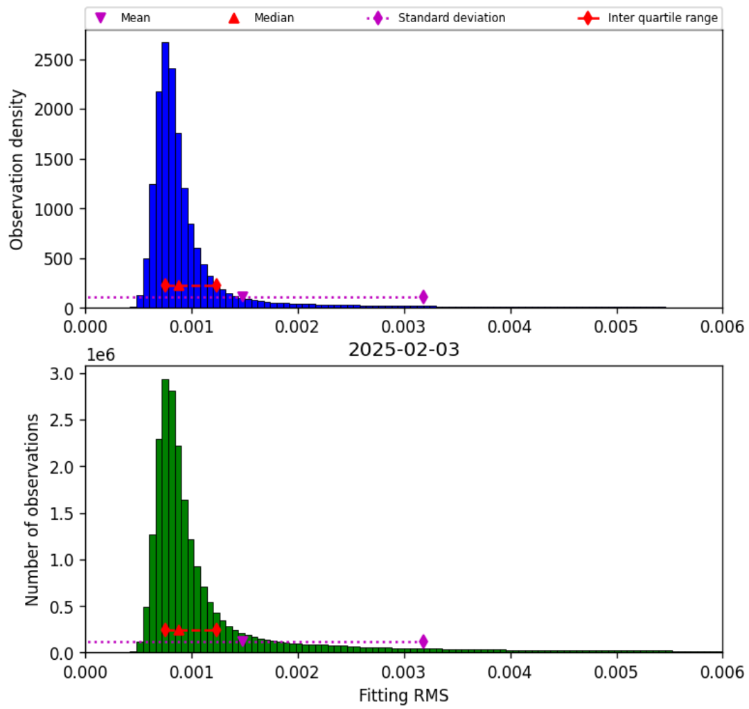
Figure 34: Histogram of “Fitting RMS” for 2025-02-03 to 2025-02-04
