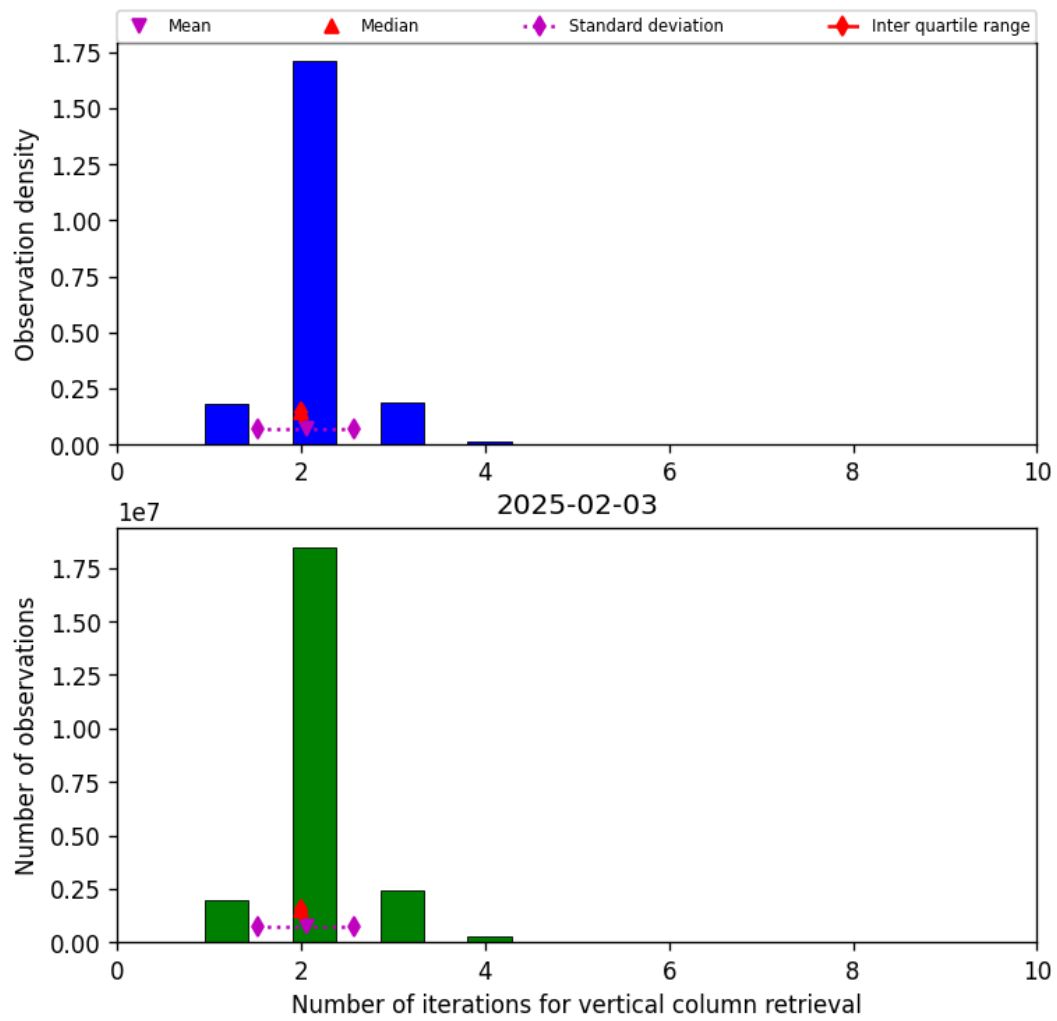
Figure 39: Histogram of “Number of iterations for vertical column retrieval” for 2025-02-03 to 2025-02-04
