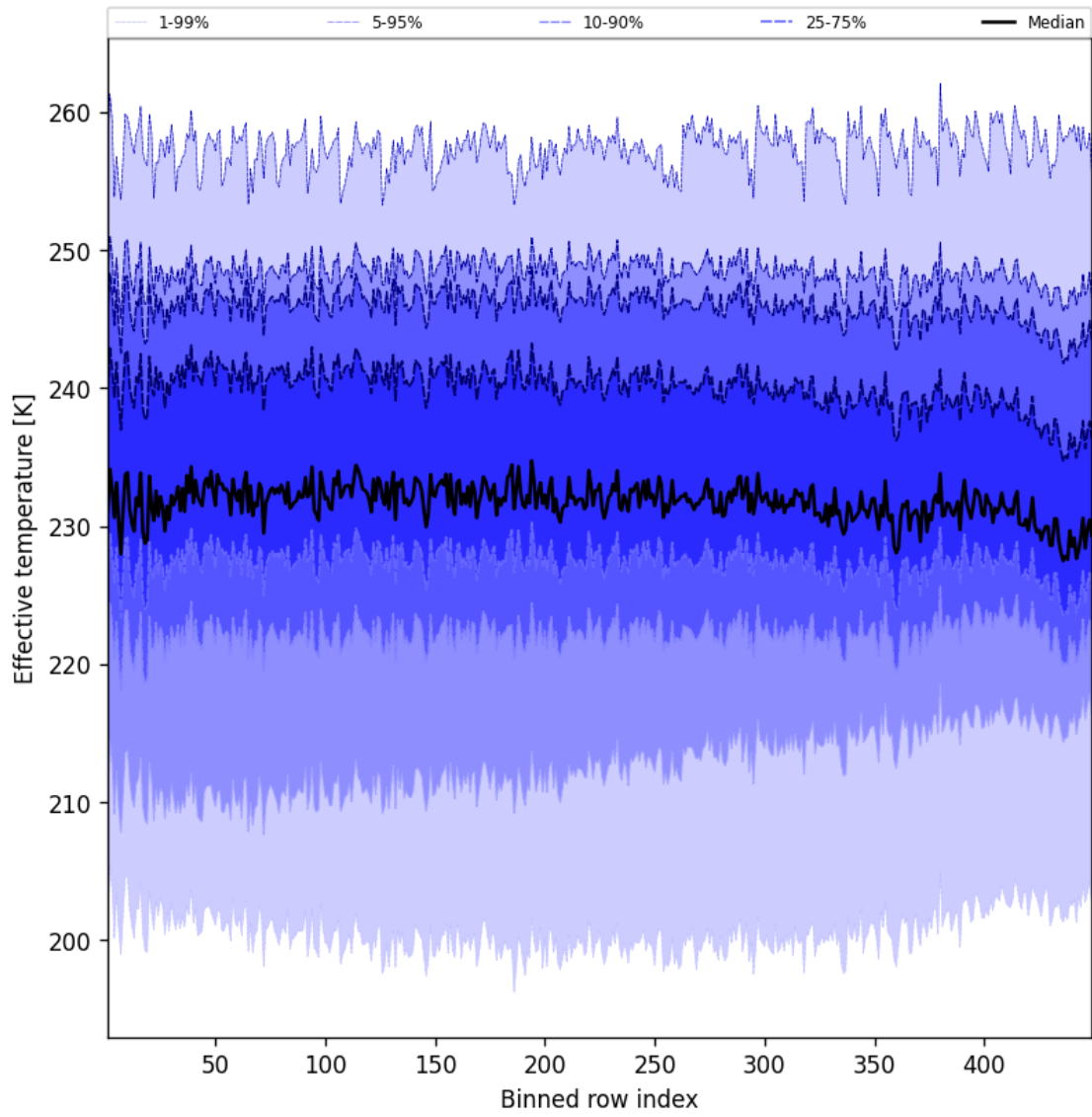
Figure 50: Along track statistics of “Effective temperature” for 2025-02-03 to 2025-02-04
