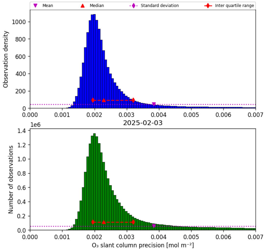
Figure 32: Histogram of “O 3 slant column precision” for 2025-02-03 to 2025-02-04
