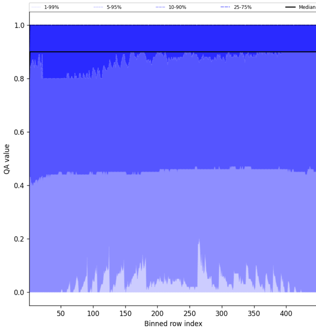
Figure 40: Along track statistics of “QA value” for 2025-02-03 to 2025-02-04
