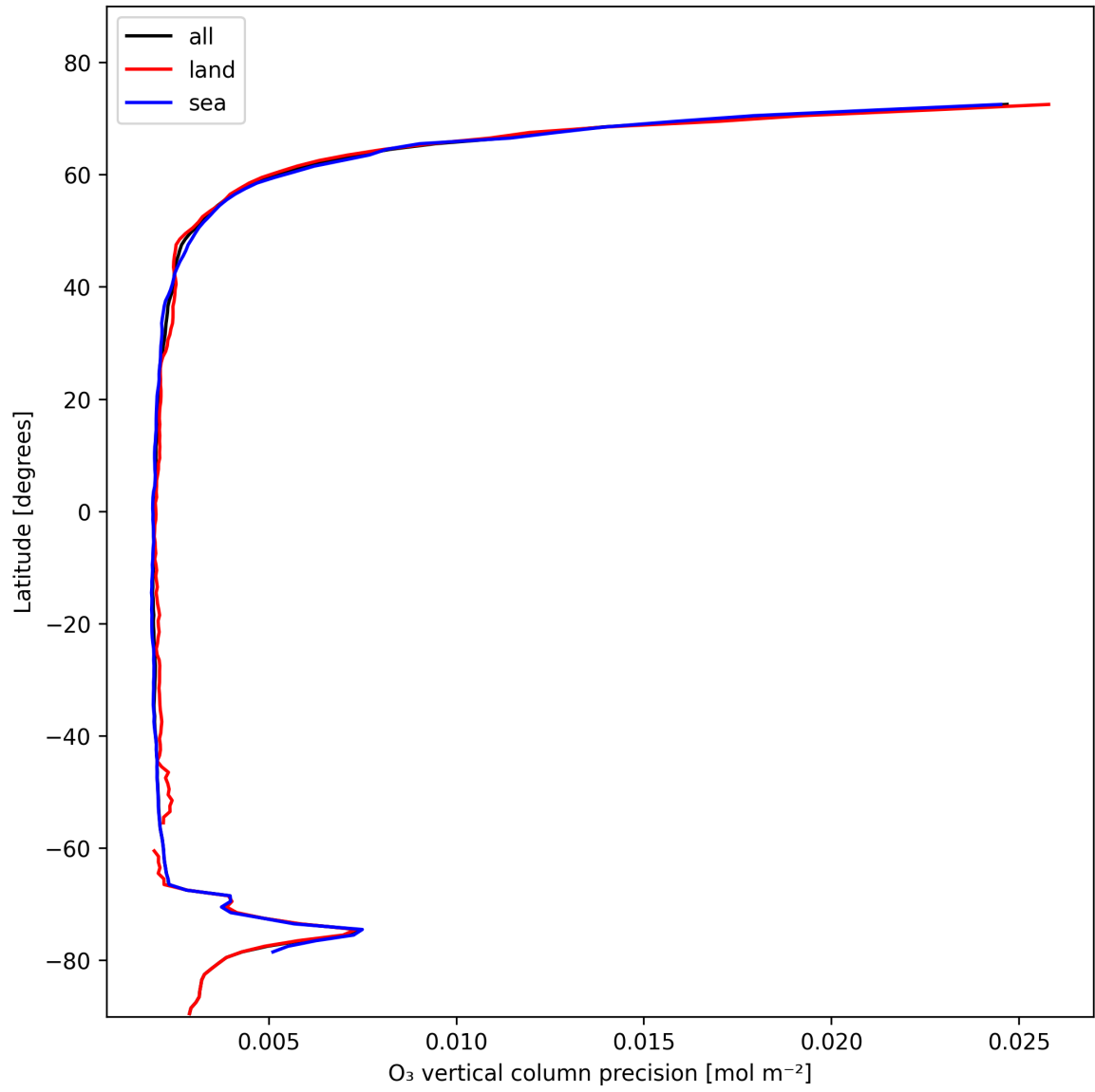
Figure 18: Zonal average of “O 3 vertical column precision” for 2025-02-03 to 2025-02-04.
