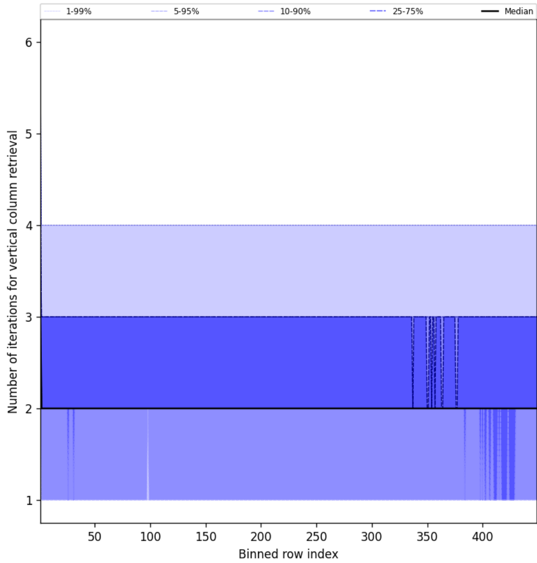
Figure 51: Along track statistics of “Number of iterations for vertical column retrieval” for 2025-02-03 to 2025-02-04
