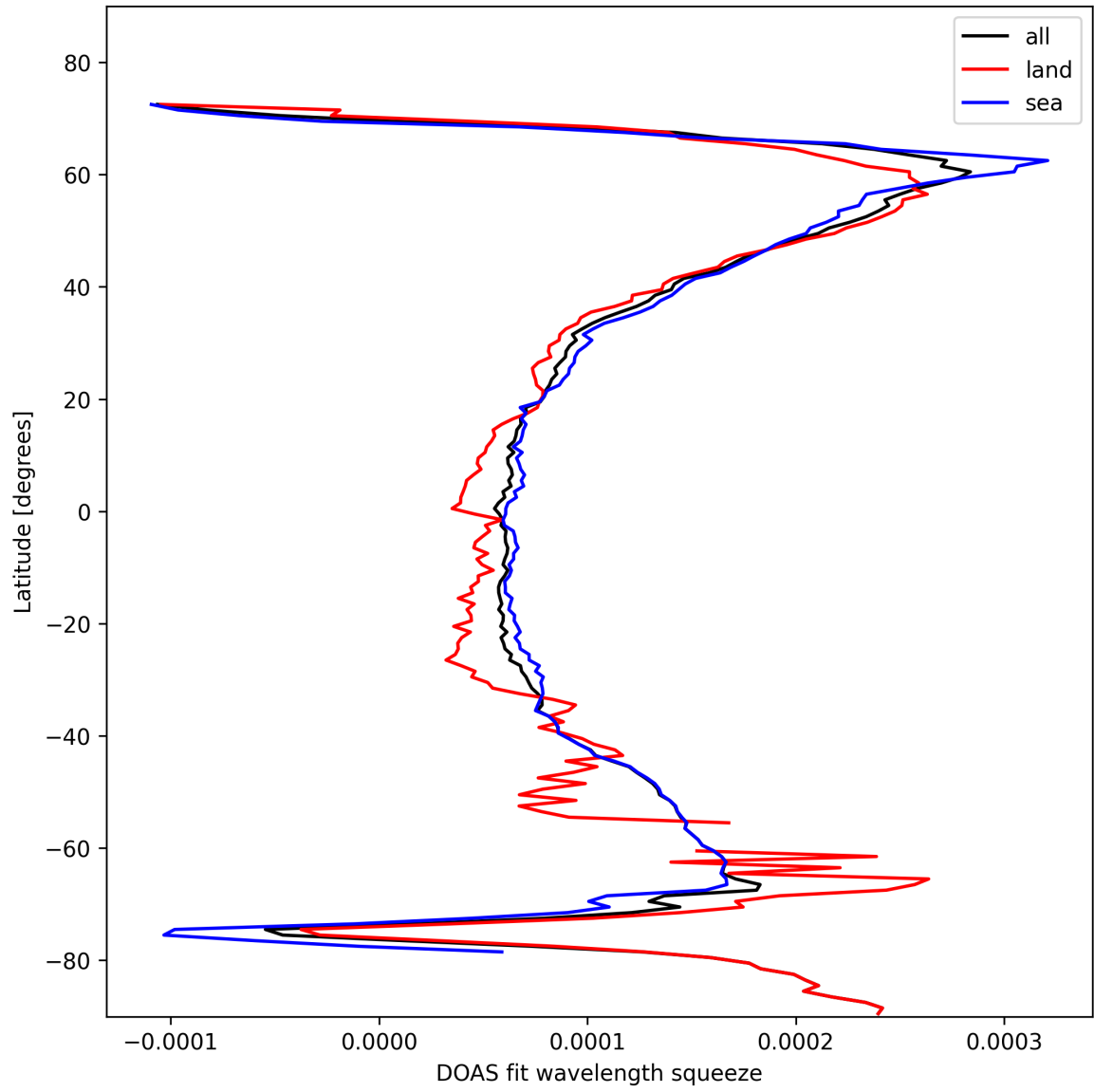
Figure 24: Zonal average of “DOAS fit wavelength squeeze” for 2025-02-03 to 2025-02-04.
