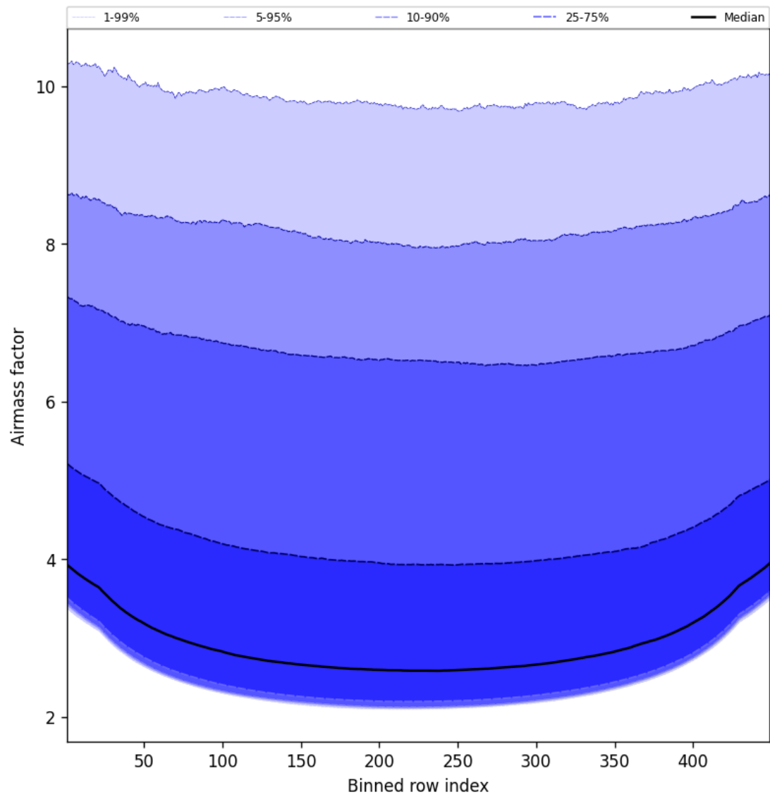
Figure 49: Along track statistics of “Airmass factor” for 2025-02-03 to 2025-02-04
