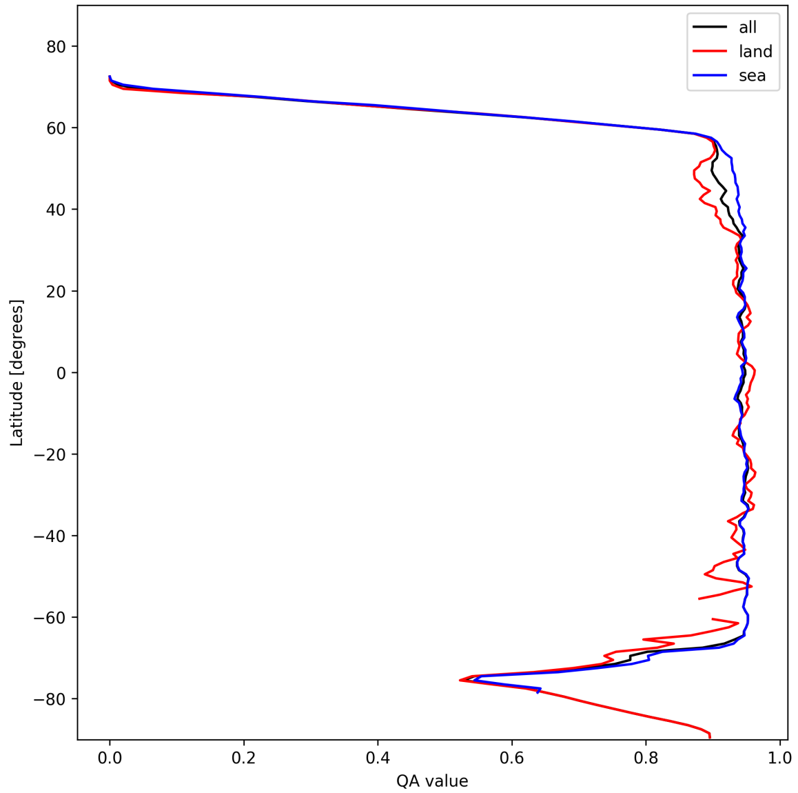
Figure 16: Zonal average of “QA value” for 2025-02-03 to 2025-02-04.
