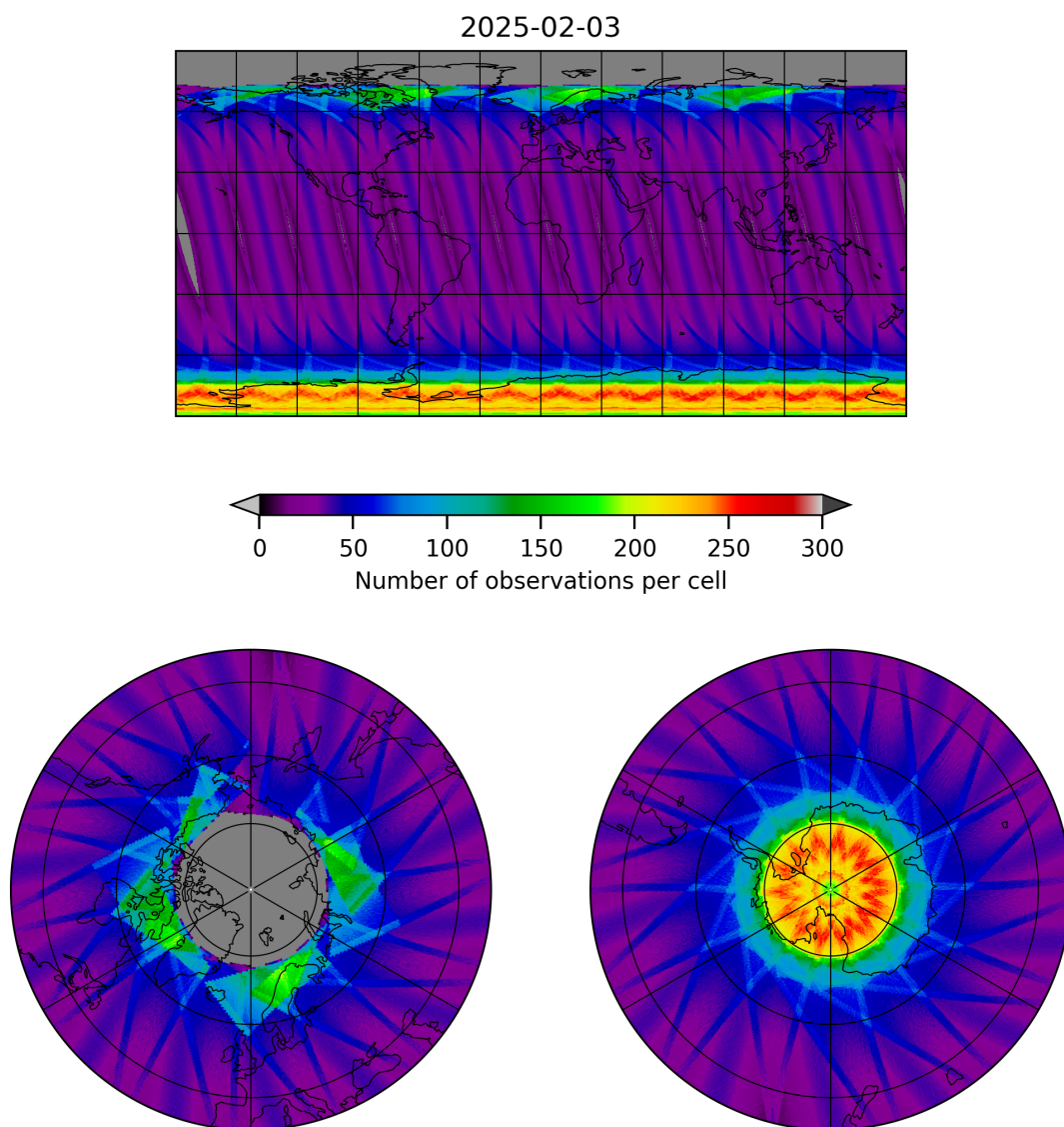
Figure 15: Map of the number of observations for 2025-02-03 to 2025-02-04
