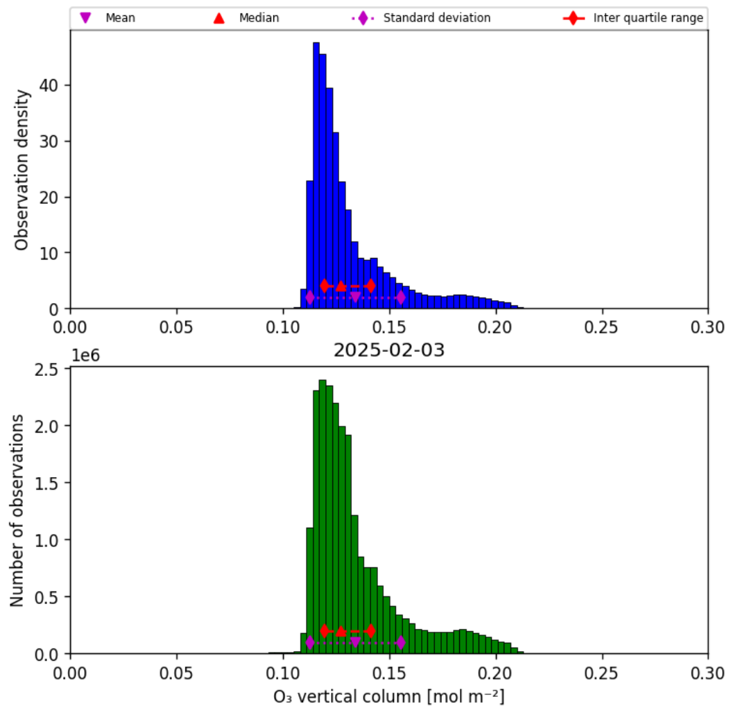
Figure 29: Histogram of “O 3 vertical column” for 2025-02-03 to 2025-02-04
