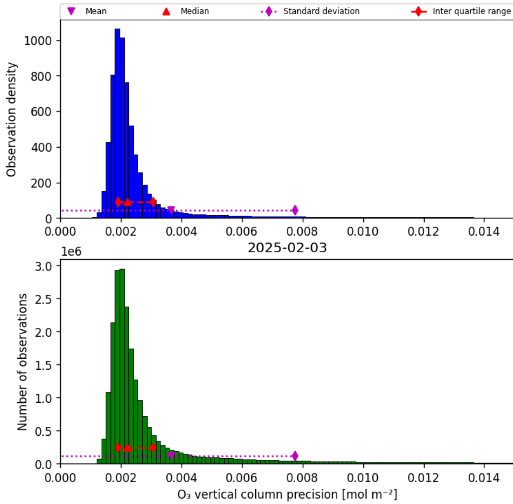
Figure 30: Histogram of “O 3 vertical column precision” for 2025-02-03 to 2025-02-04
