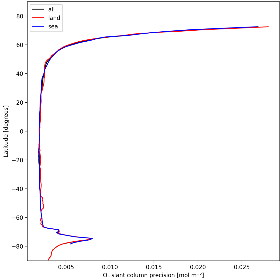
Figure 20: Zonal average of "O 3 slant column precision" for 2025-02-03 to 2025-02-04.
