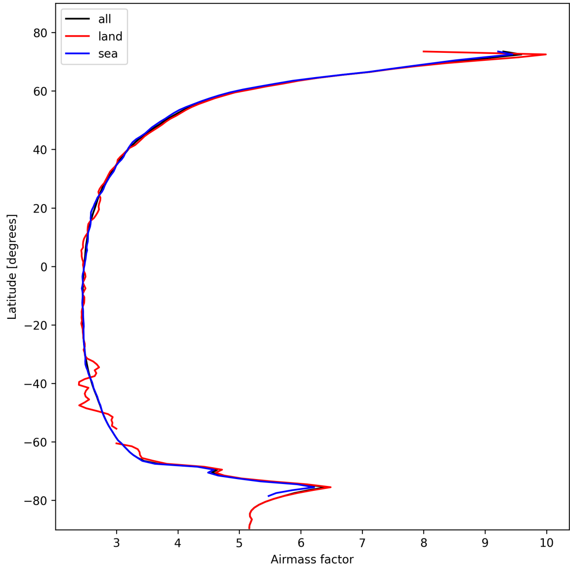
Figure 25: Zonal average of “Airmass factor” for 2025-02-04 to 2025-02-05.
