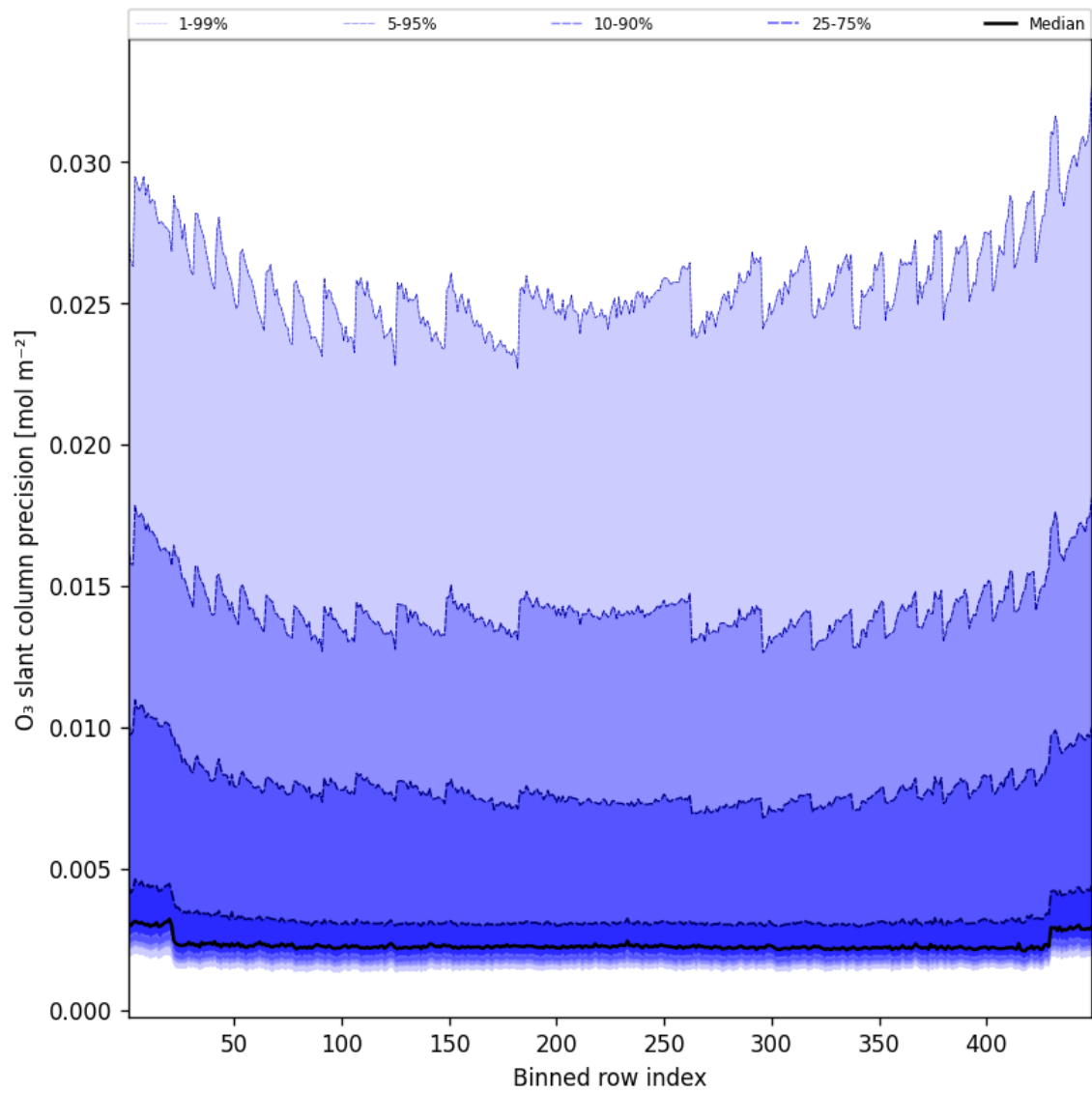
Figure 44: Along track statistics of “O 3 slant column precision” for 2025-02-04 to 2025-02-05
