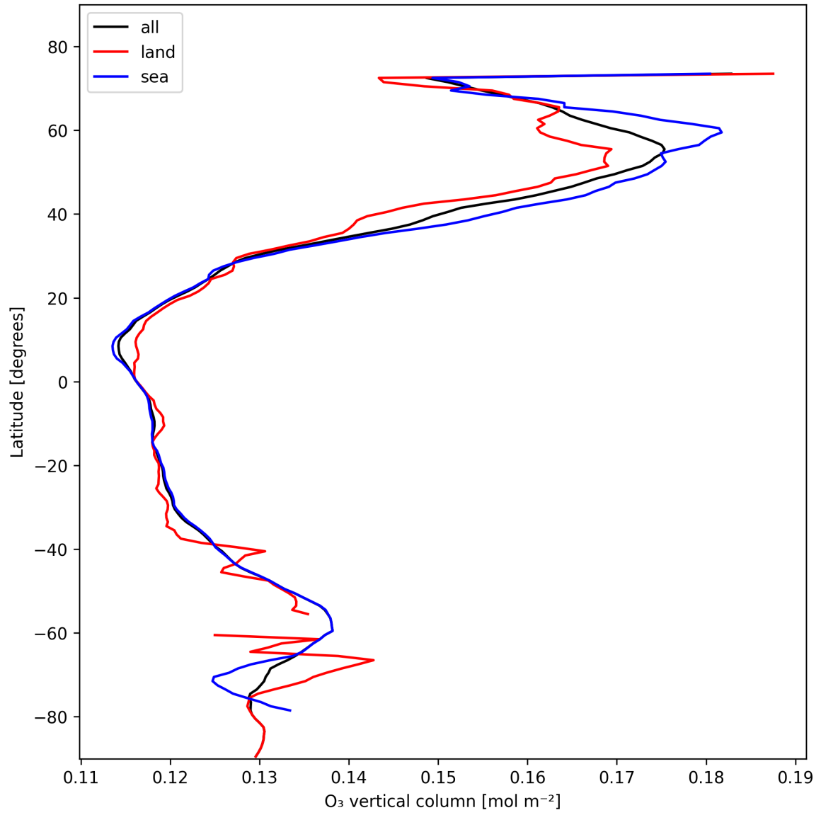
Figure 17: Zonal average of “O 3 vertical column” for 2025-02-04 to 2025-02-05.
