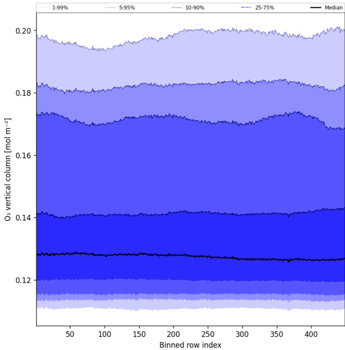
Figure 41: Along track statistics of “O 3 vertical column” for 2025-02-04 to 2025-02-05
