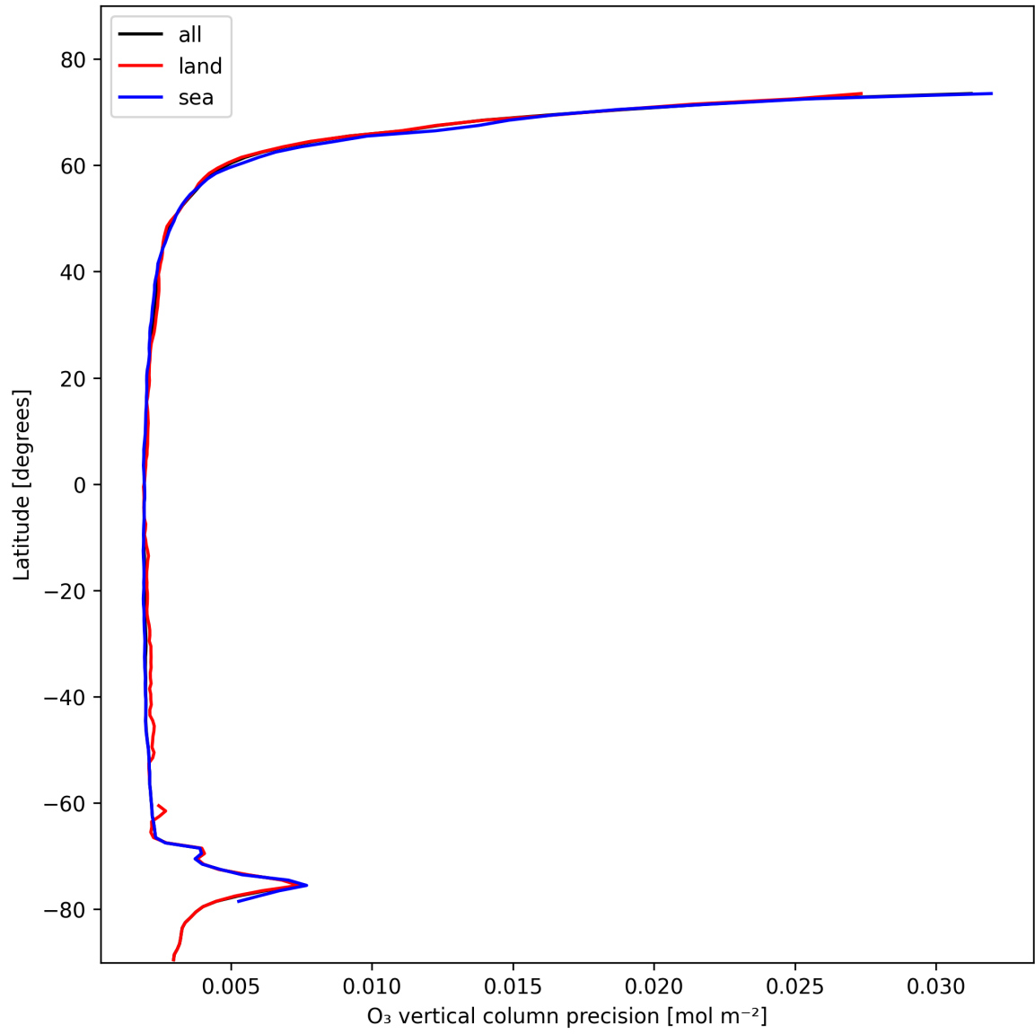
Figure 18: Zonal average of “O 3 vertical column precision” for 2025-02-04 to 2025-02-05.
