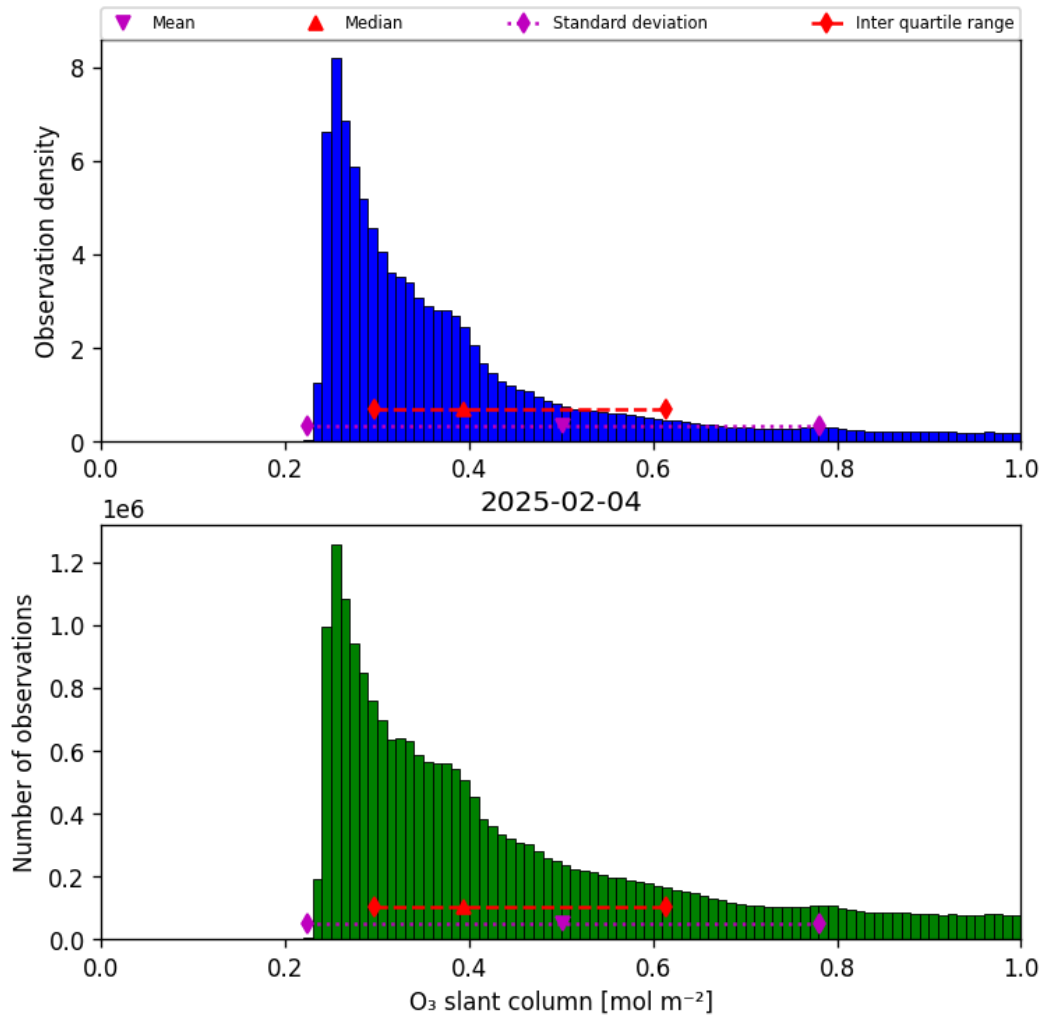
Figure 31: Histogram of “O 3 slant column” for 2025-02-04 to 2025-02-05
