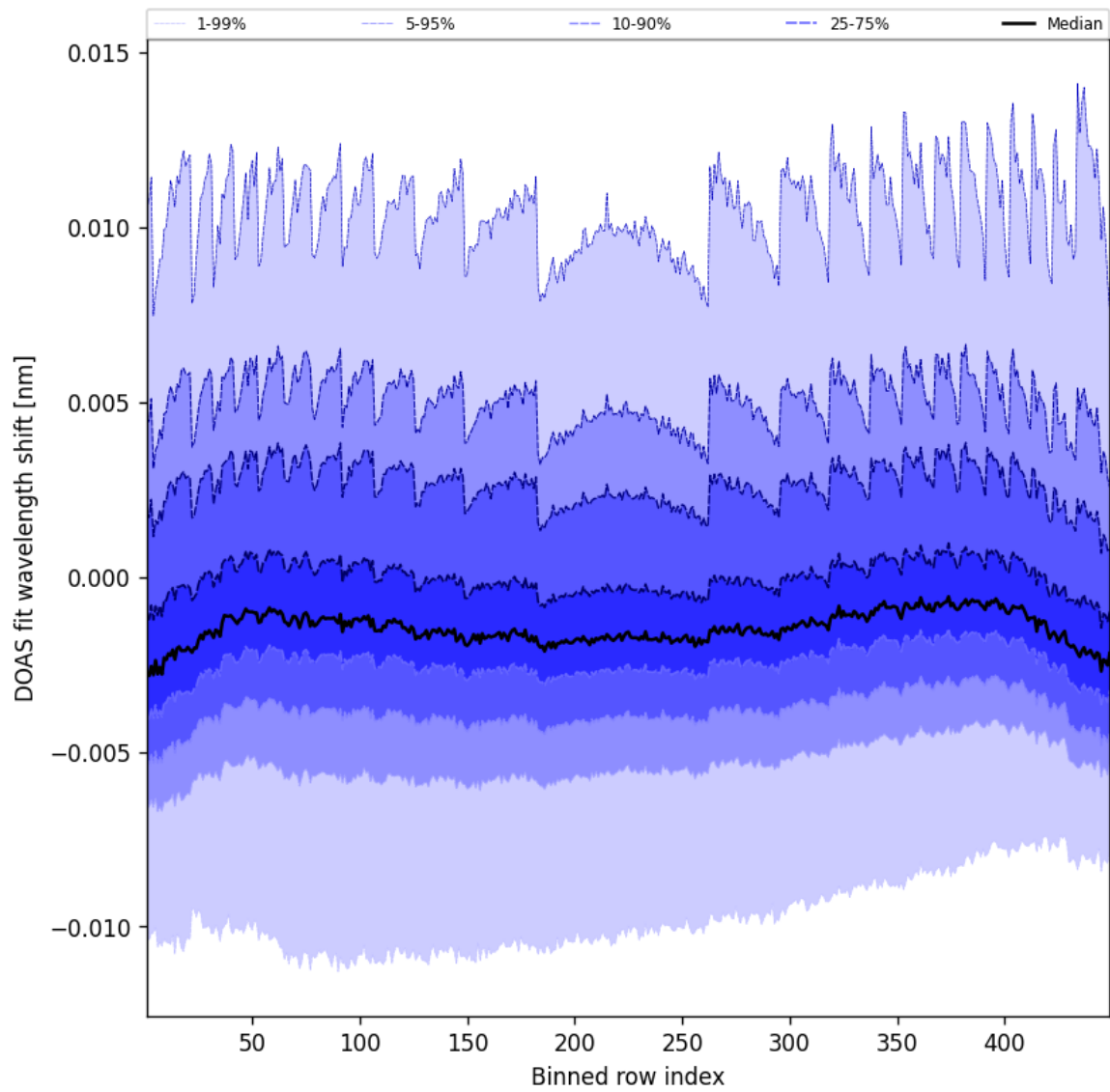
Figure 47: Along track statistics of “DOAS fit wavelength shift” for 2025-02-04 to 2025-02-05
