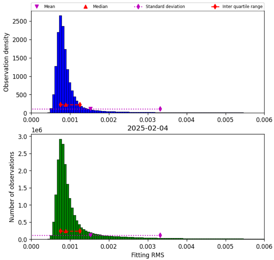
Figure 34: Histogram of “Fitting RMS” for 2025-02-04 to 2025-02-05
