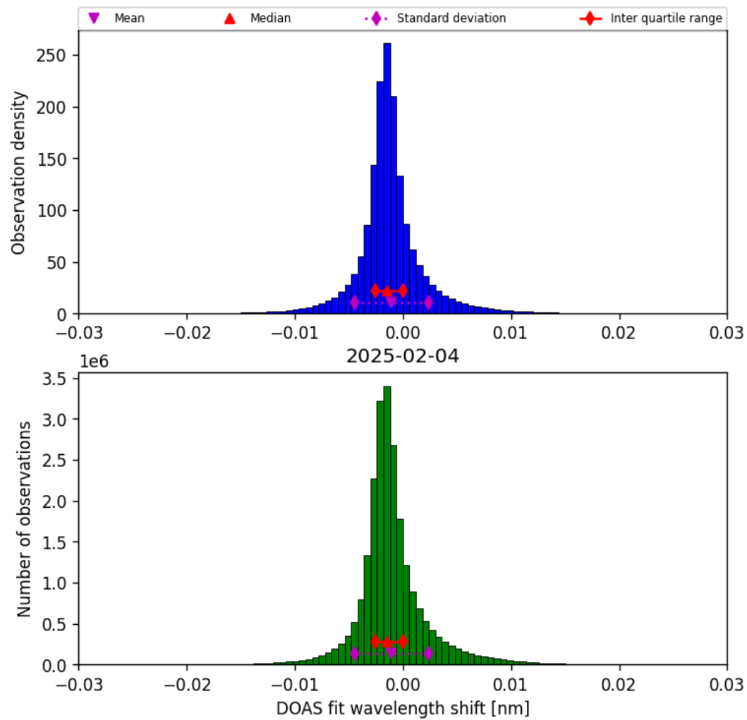
Figure 35: Histogram of “DOAS fit wavelength shift” for 2025-02-04 to 2025-02-05
