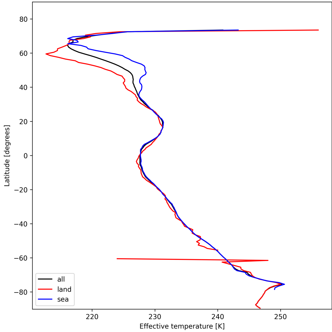
Figure 26: Zonal average of “Effective temperature” for 2025-02-04 to 2025-02-05.
