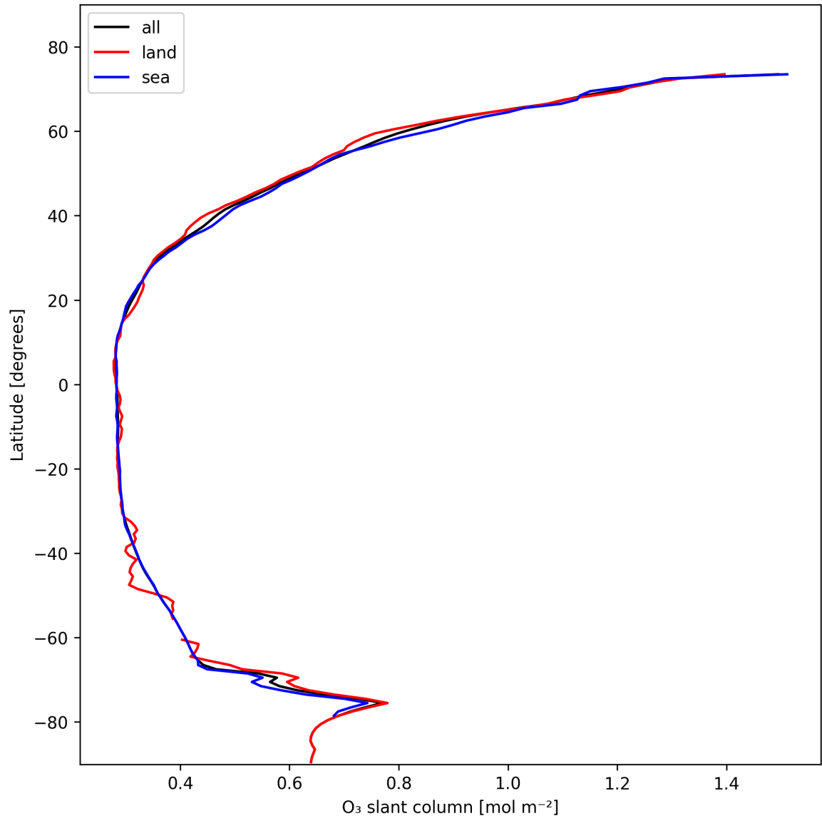
Figure 19: Zonal average of “O 3 slant column” for 2025-02-04 to 2025-02-05.
