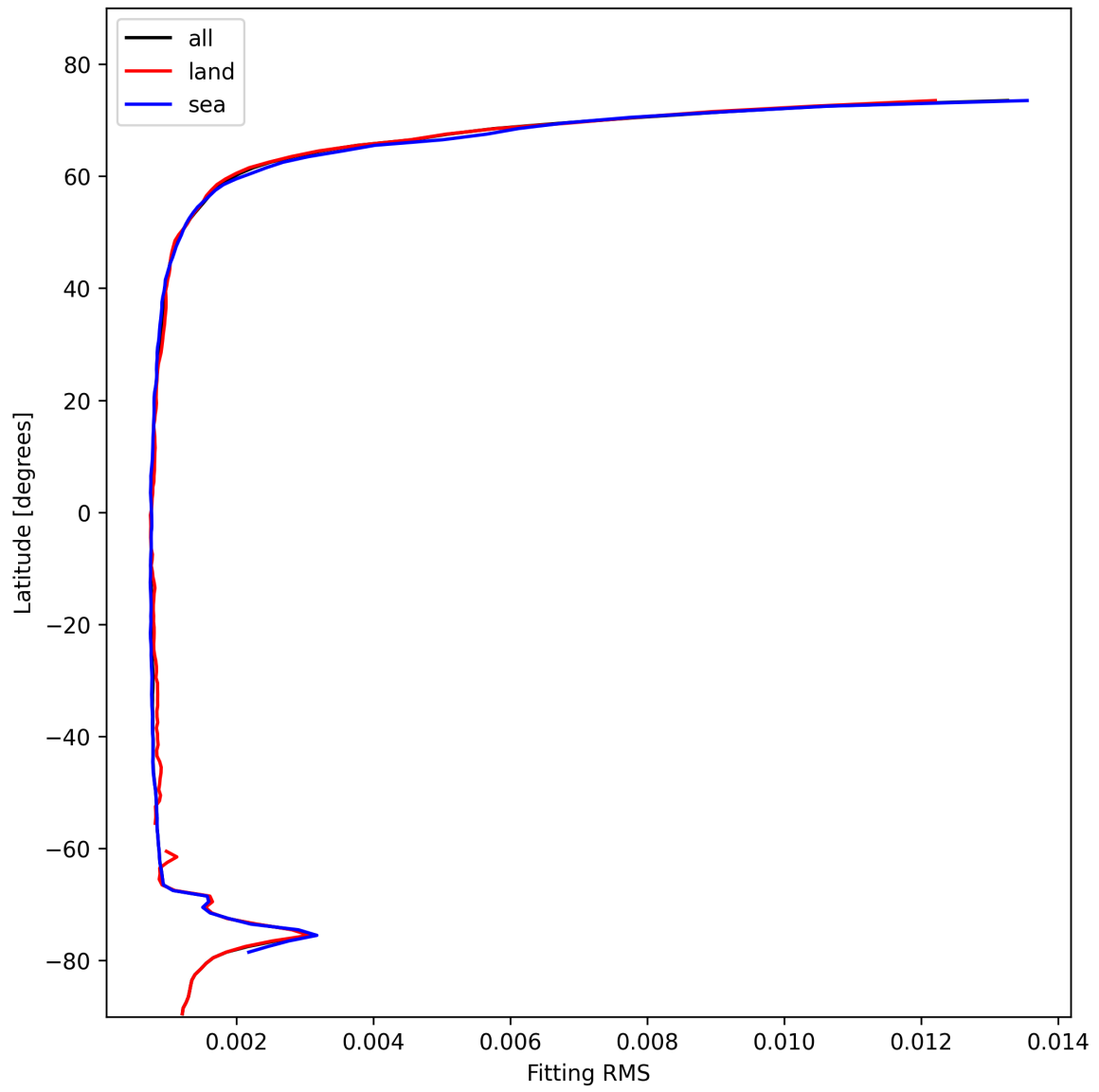
Figure 22: Zonal average of “Fitting RMS” for 2025-02-04 to 2025-02-05.
