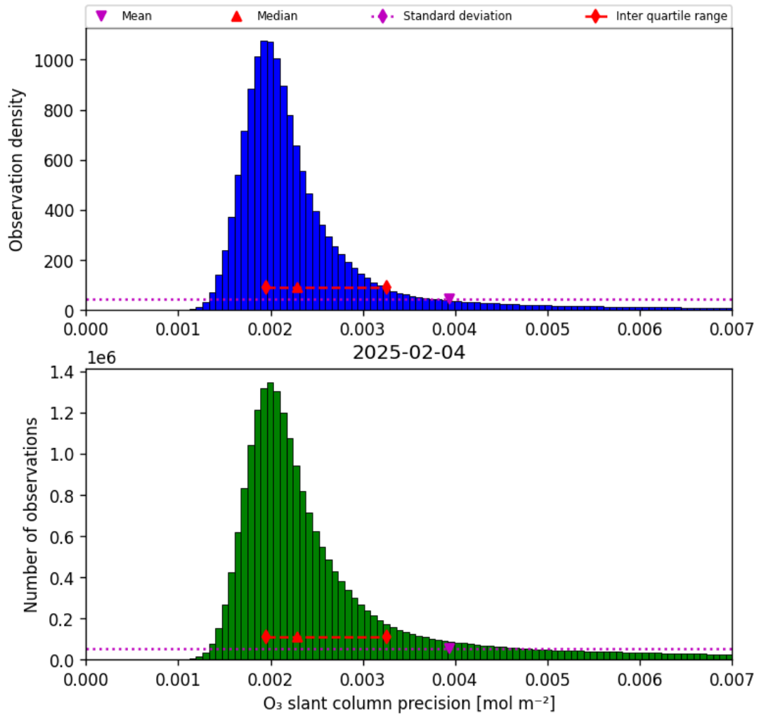
Figure 32: Histogram of “O 3 slant column precision” for 2025-02-04 to 2025-02-05
