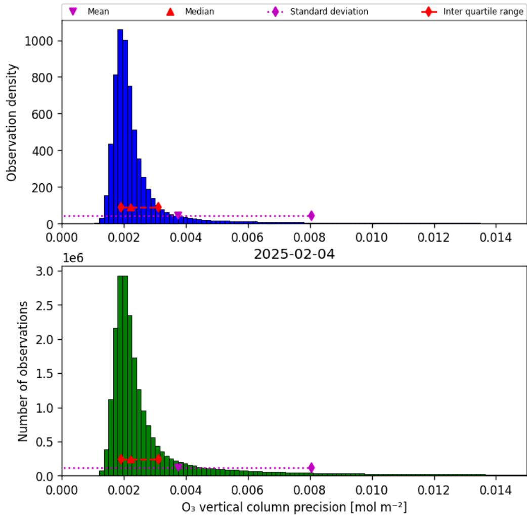
Figure 30: Histogram of “O 3 vertical column precision” for 2025-02-04 to 2025-02-05
