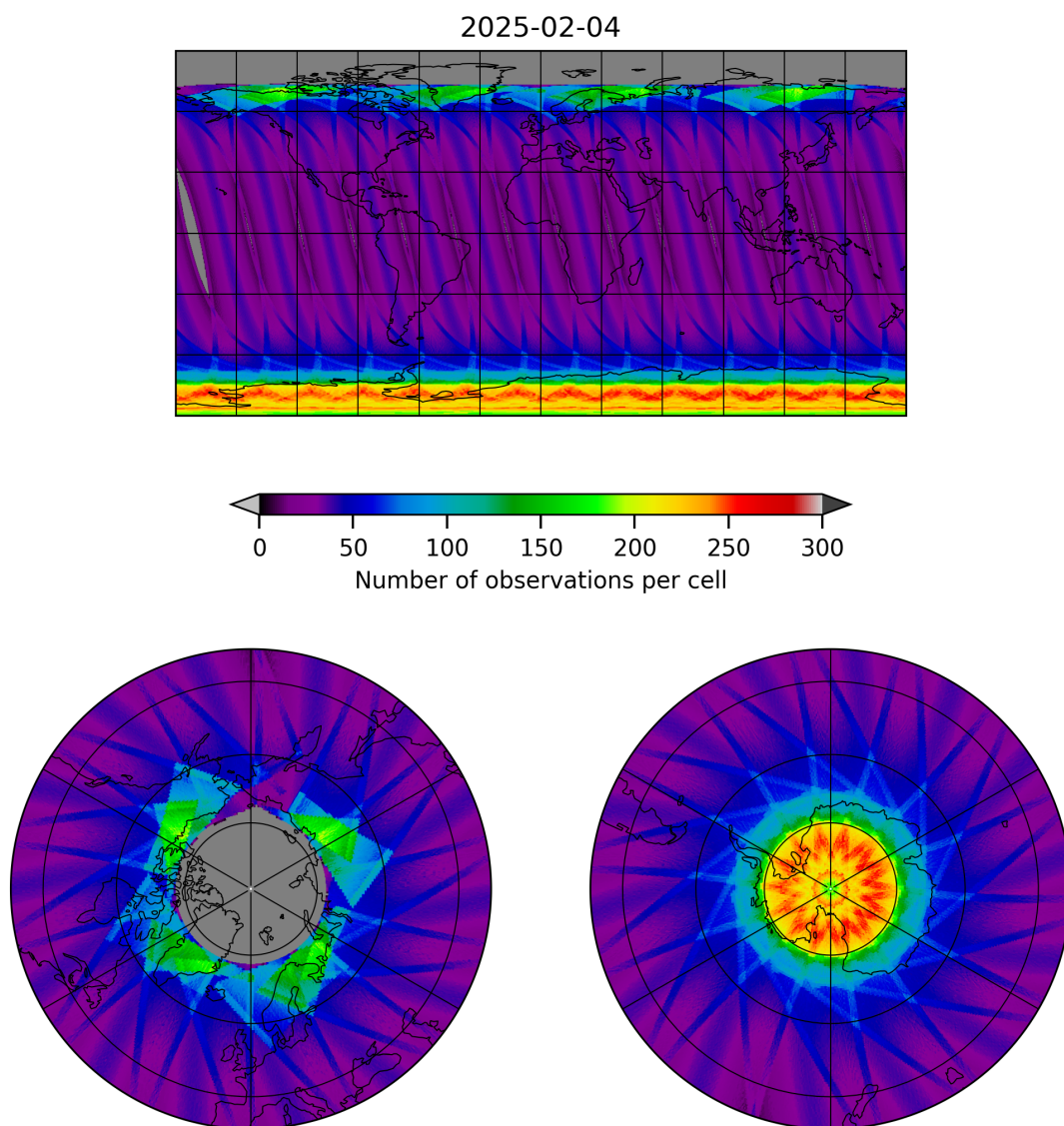
Figure 15: Map of the number of observations for 2025-02-04 to 2025-02-05
