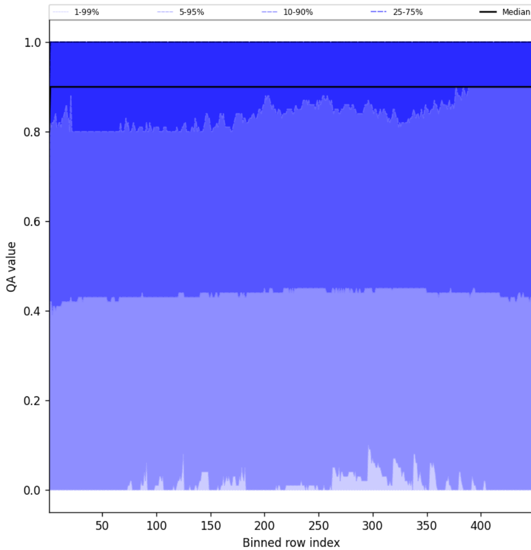
Figure 40: Along track statistics of “QA value” for 2025-02-04 to 2025-02-05
