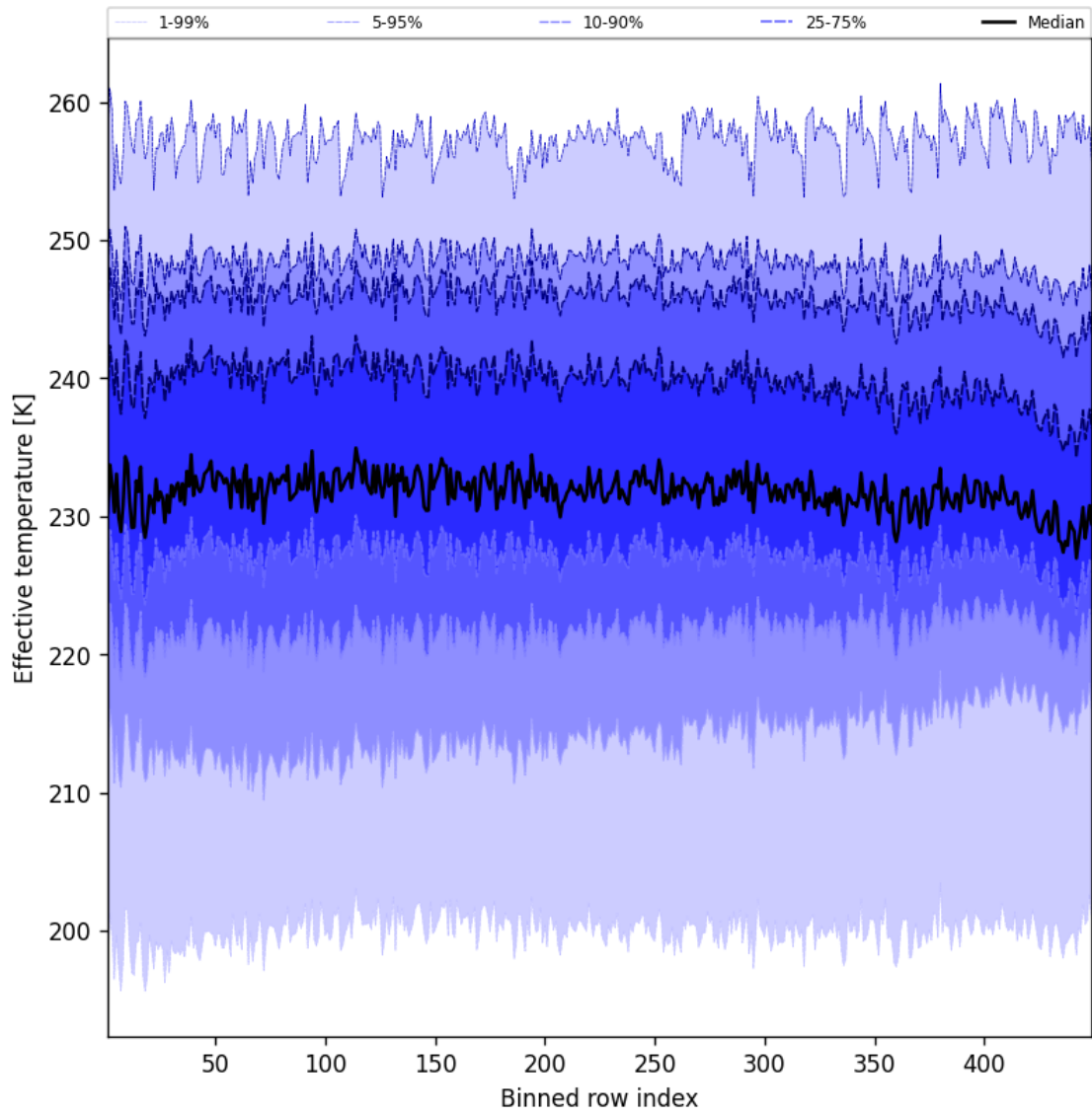
Figure 50: Along track statistics of “Effective temperature” for 2025-02-04 to 2025-02-05
