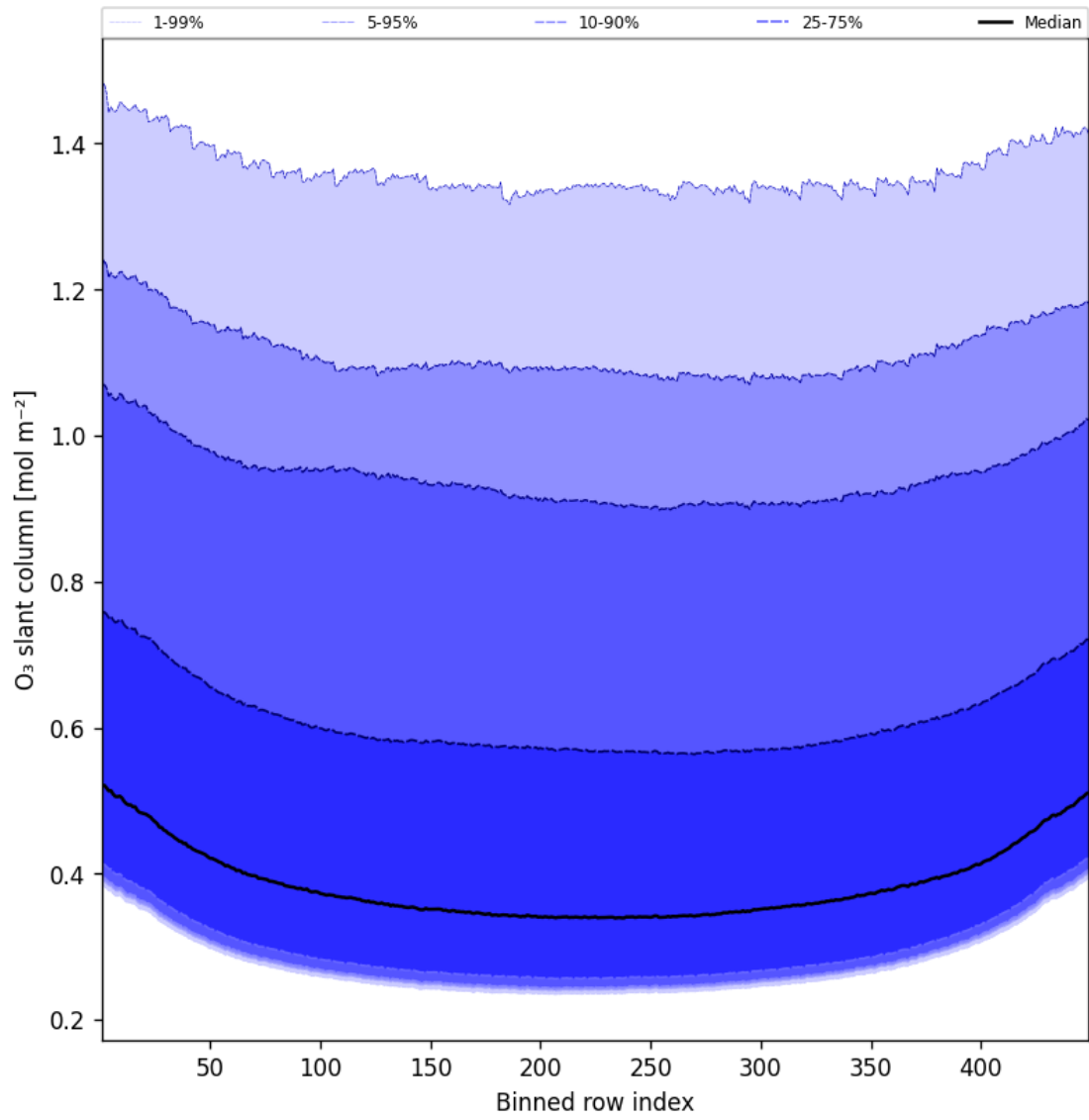
Figure 43: Along track statistics of "O 3 slant column" for 2025-02-04 to 2025-02-05
