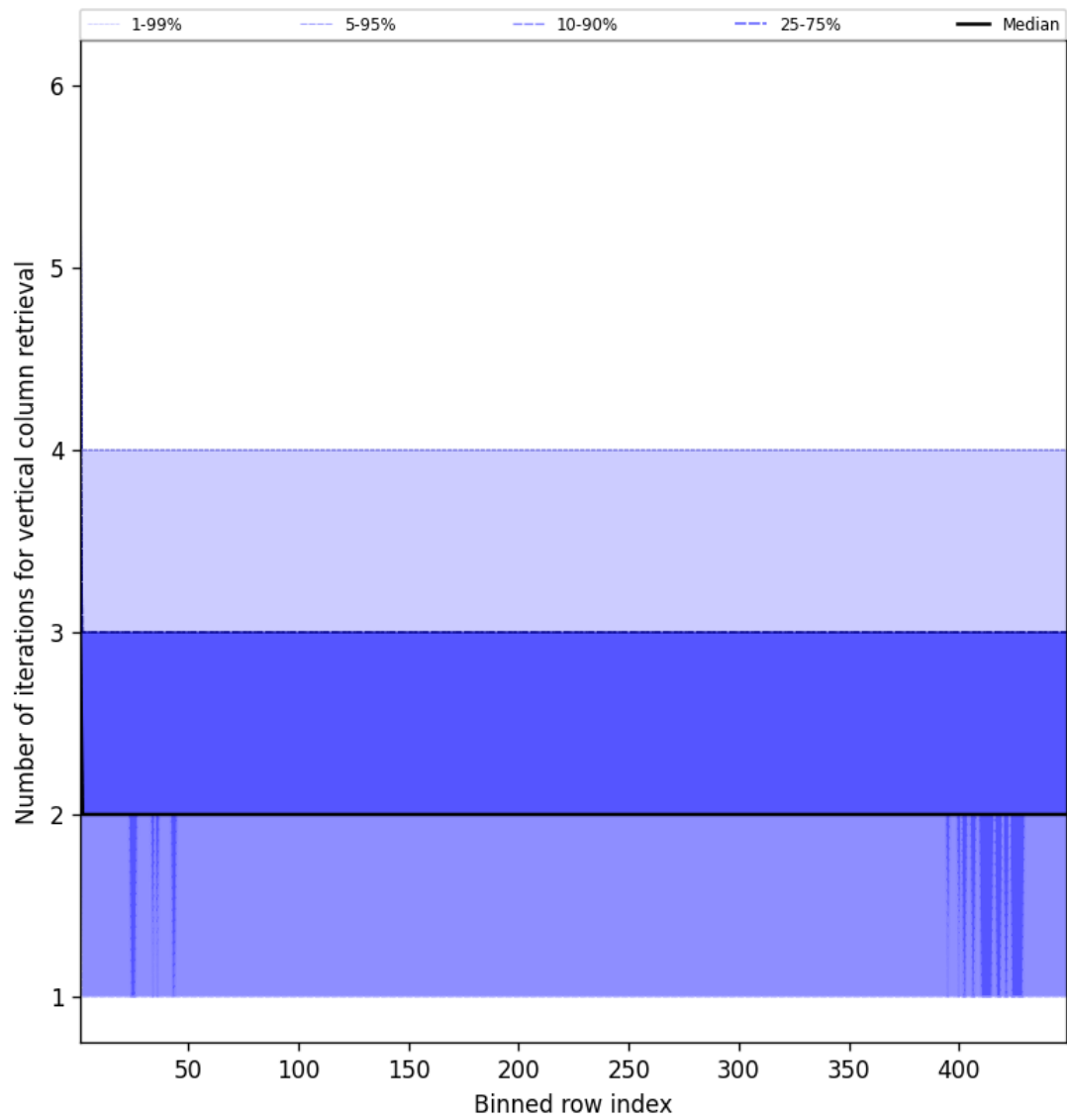
Figure 51: Along track statistics of “Number of iterations for vertical column retrieval” for 2025-02-04 to 2025-02-05
