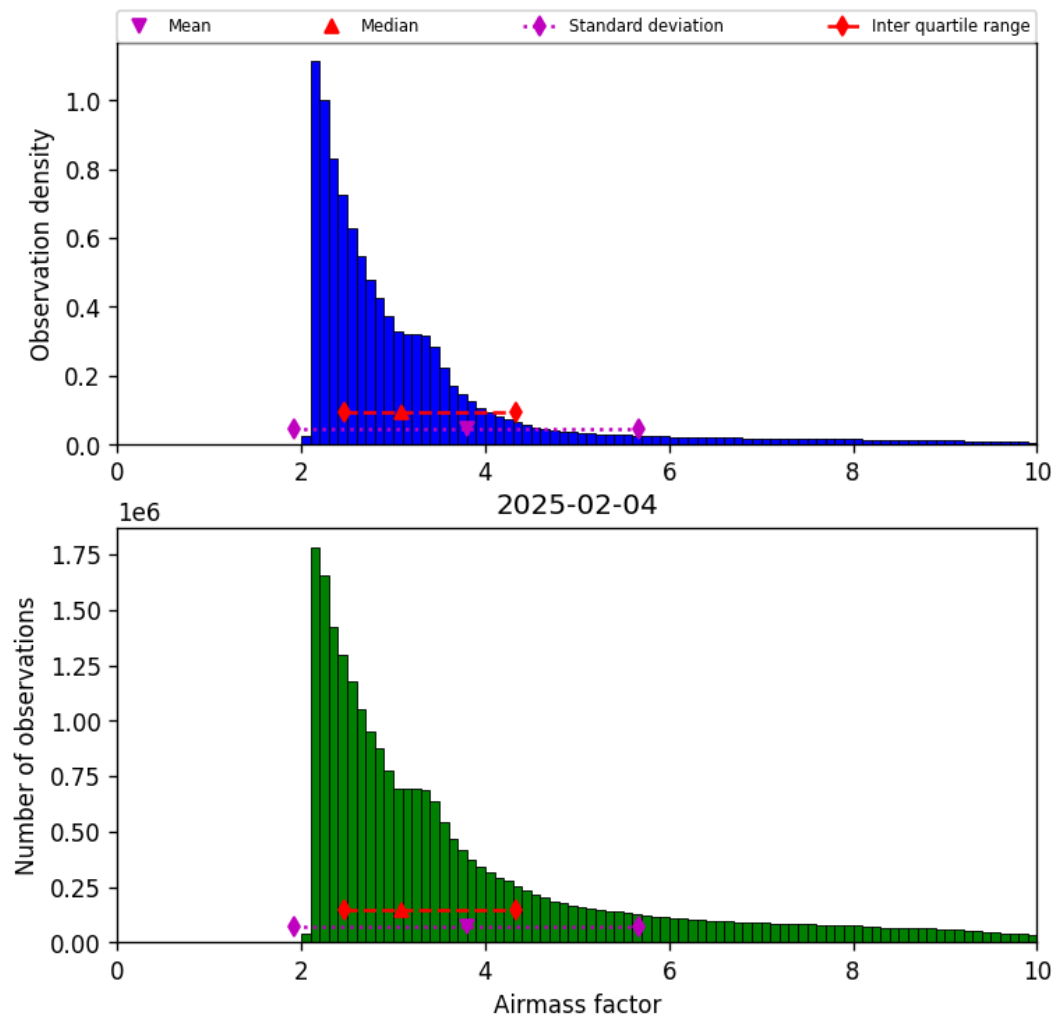
Figure 37: Histogram of “Airmass factor” for 2025-02-04 to 2025-02-05
