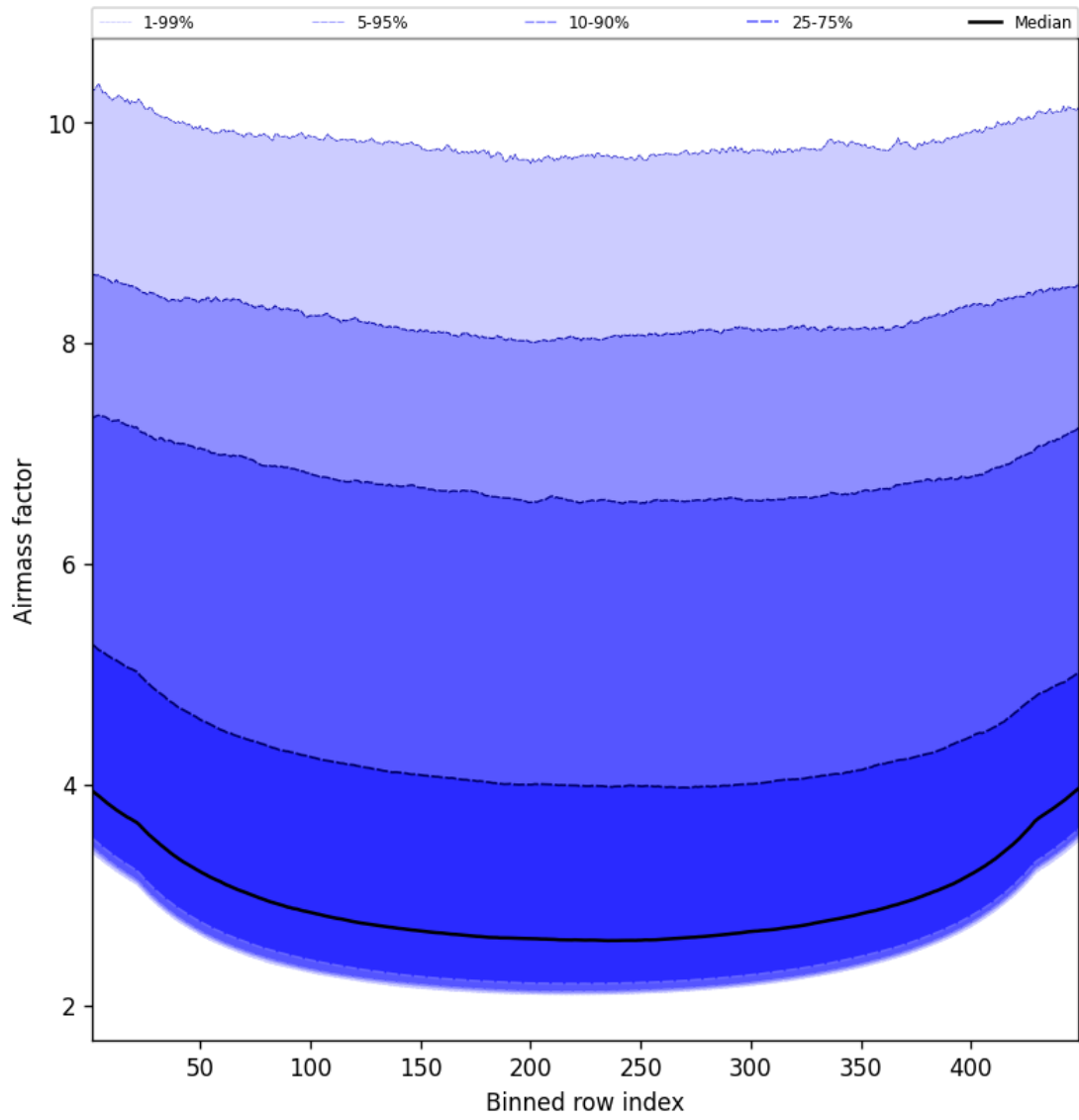
Figure 49: Along track statistics of “Airmass factor” for 2025-02-04 to 2025-02-05
