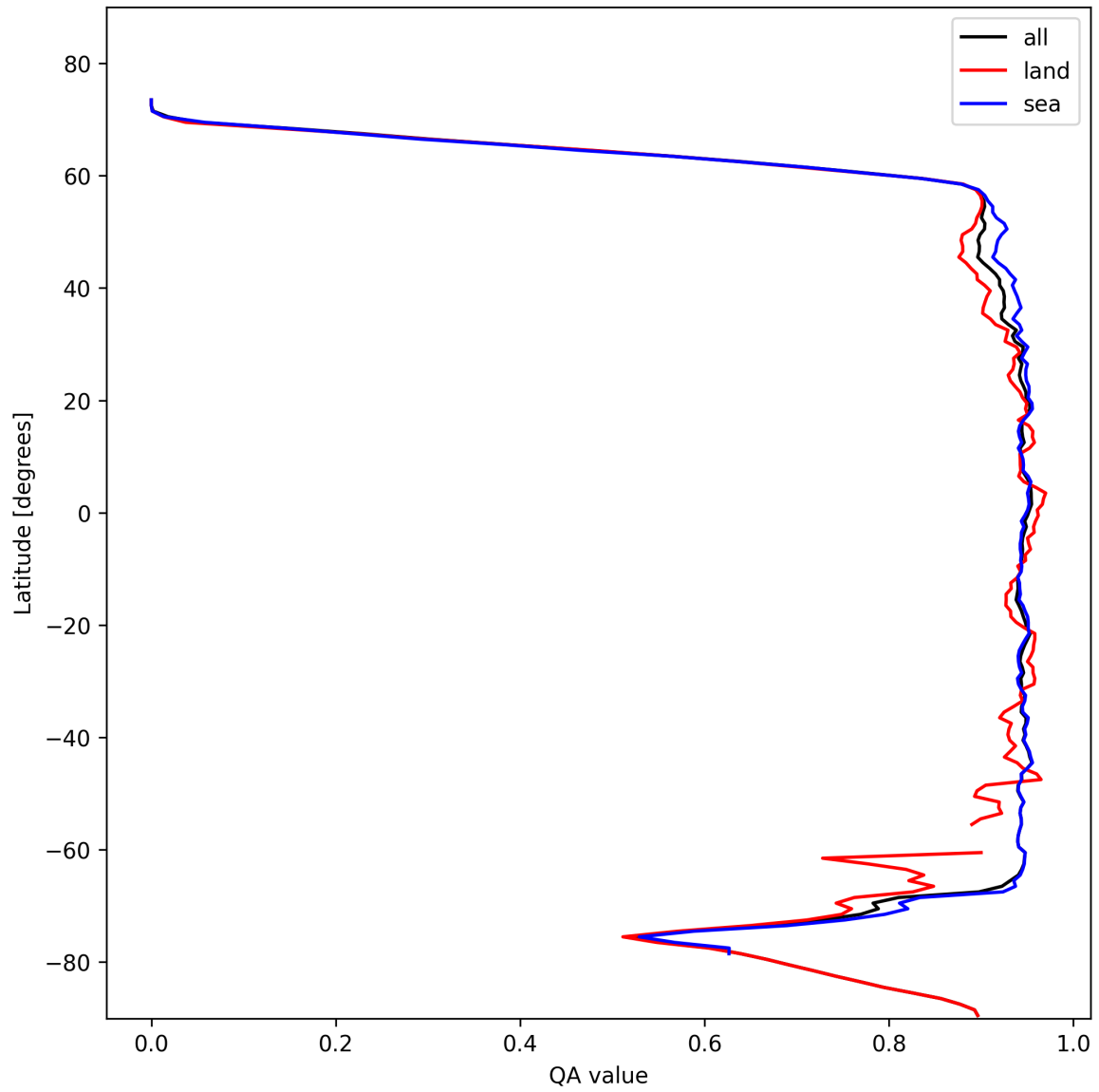
Figure 16: Zonal average of “QA value” for 2025-02-04 to 2025-02-05.
