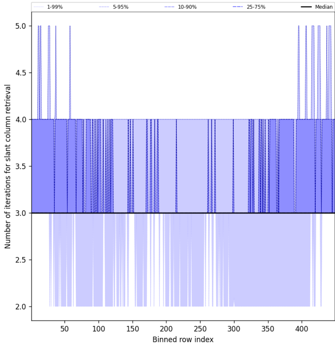
Figure 45: Along track statistics of “Number of iterations for slant column retrieval” for 2025-02-04 to 2025-02-05
