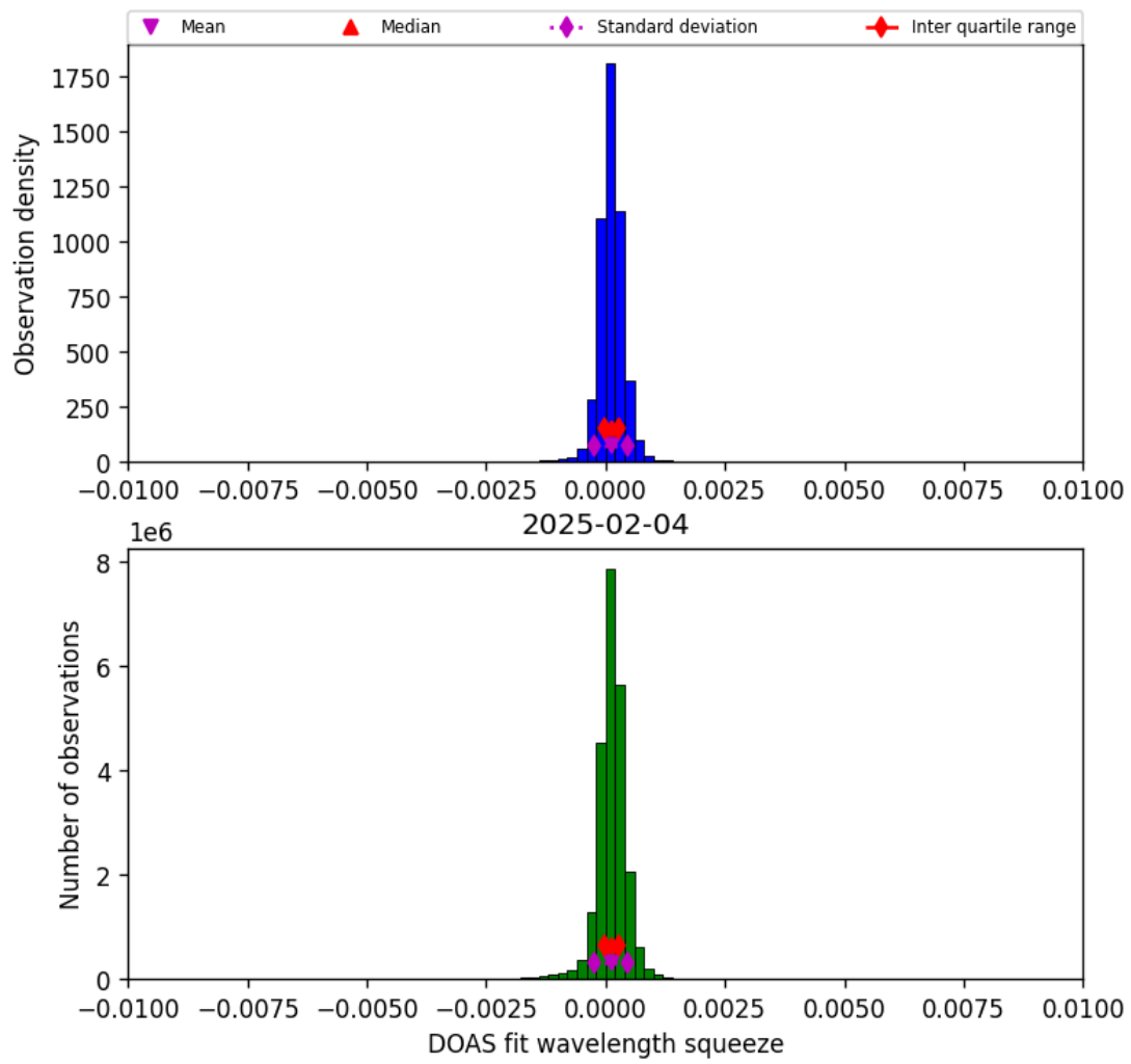
Figure 36: Histogram of “DOAS fit wavelength squeeze” for 2025-02-04 to 2025-02-05
