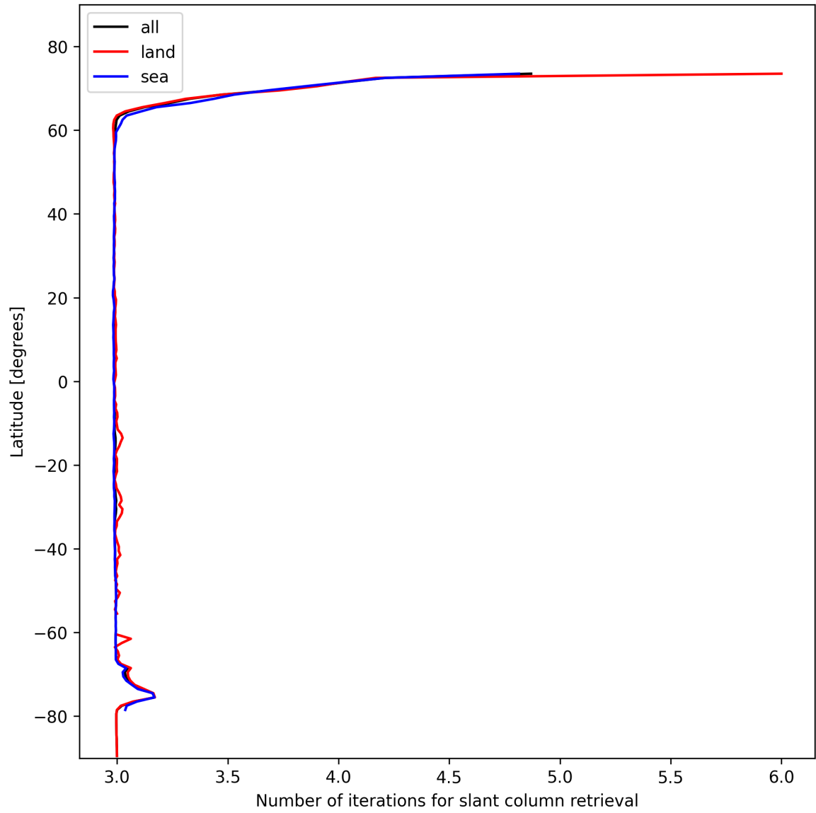
Figure 21: Zonal average of “Number of iterations for slant column retrieval” for 2025-02-04 to 2025-02-05.
