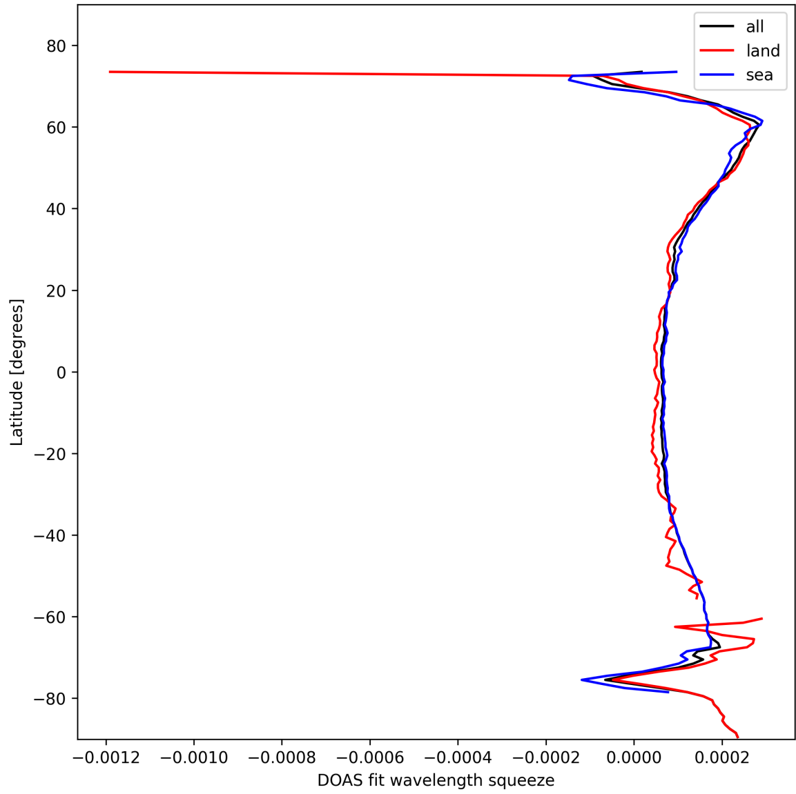
Figure 24: Zonal average of “DOAS fit wavelength squeeze” for 2025-02-04 to 2025-02-05.
