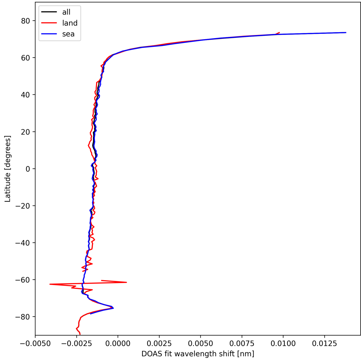
Figure 23: Zonal average of “DOAS fit wavelength shift” for 2025-02-04 to 2025-02-05.
