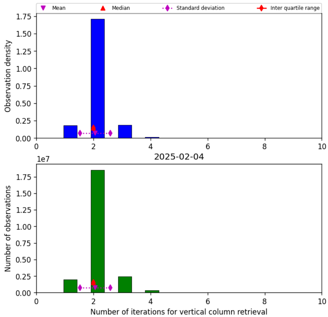
Figure 39: Histogram of “Number of iterations for vertical column retrieval” for 2025-02-04 to 2025-02-05
