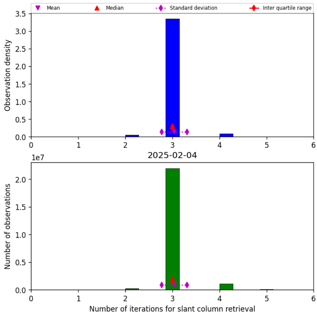
Figure 33: Histogram of “Number of iterations for slant column retrieval” for 2025-02-04 to 2025-02-05
