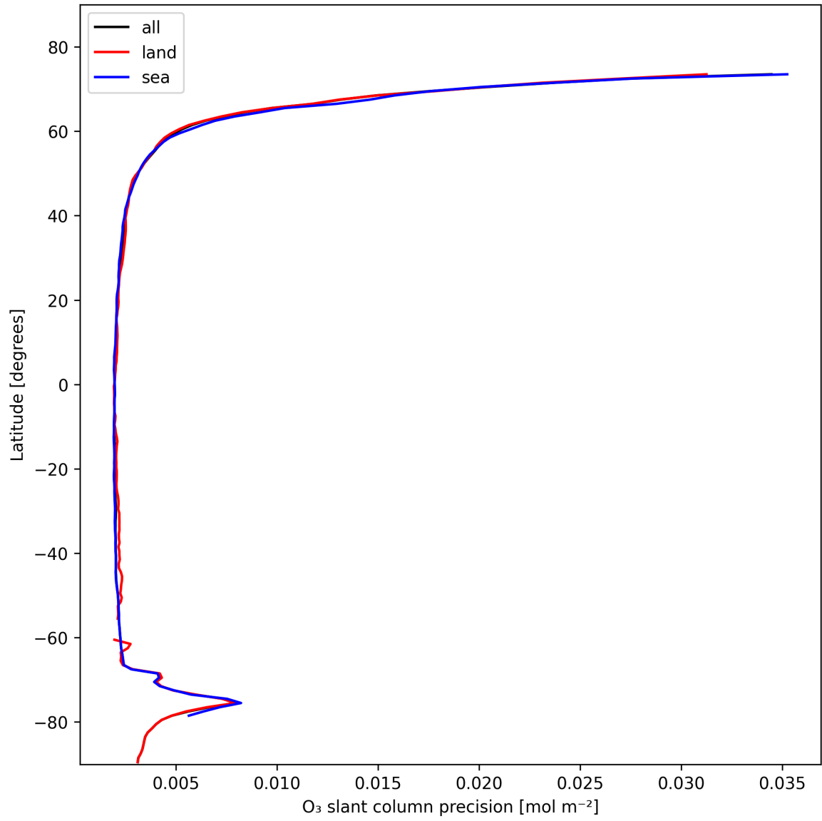
Figure 20: Zonal average of "O 3 slant column precision" for 2025-02-04 to 2025-02-05.
