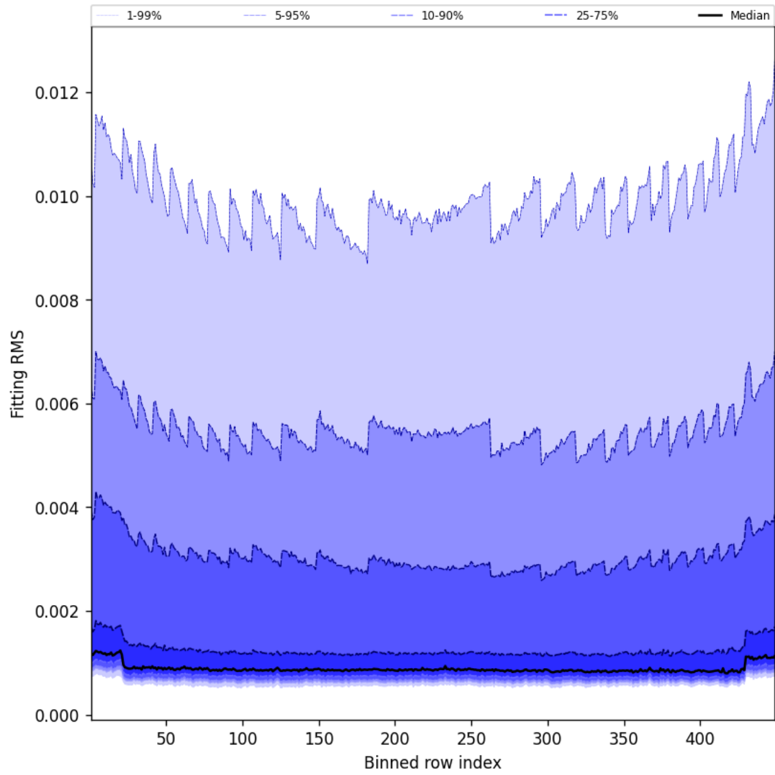
Figure 46: Along track statistics of “Fitting RMS” for 2025-02-04 to 2025-02-05
