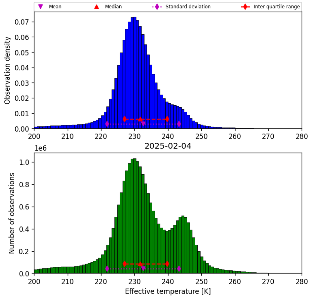
Figure 38: Histogram of “Effective temperature” for 2025-02-04 to 2025-02-05
