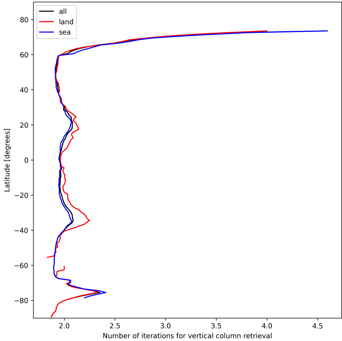
Figure 27: Zonal average of “Number of iterations for vertical column retrieval” for 2025-02-04 to 2025-02-05.
