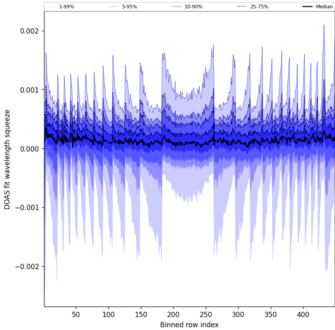
Figure 48: Along track statistics of “DOAS fit wavelength squeeze” for 2025-02-04 to 2025-02-05
