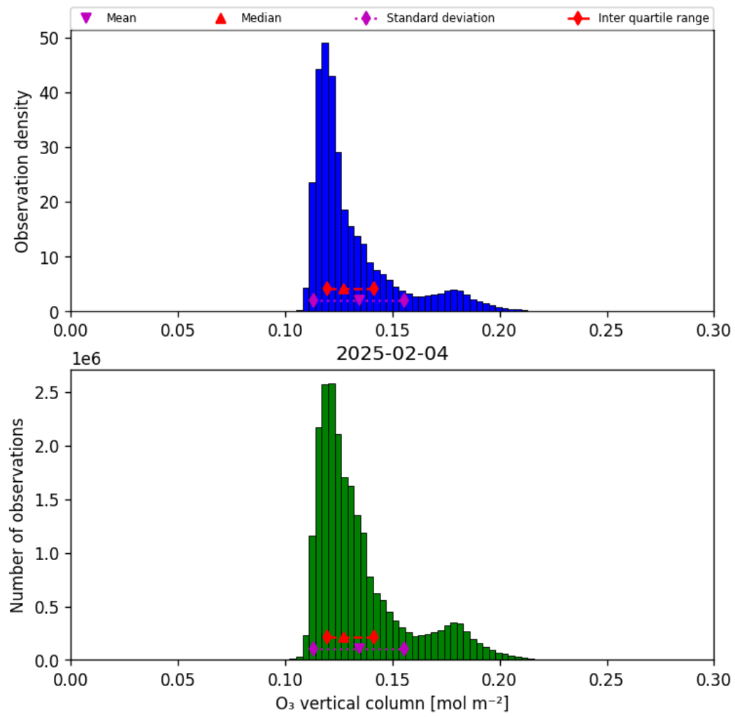
Figure 29: Histogram of “O 3 vertical column” for 2025-02-04 to 2025-02-05
