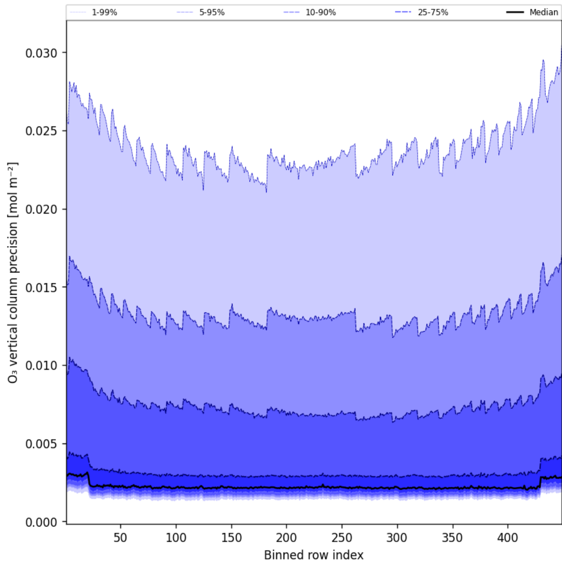
Figure 42: Along track statistics of “O 3 vertical column precision” for 2025-02-04 to 2025-02-05
