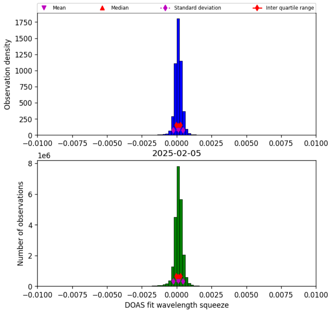
Figure 36: Histogram of “DOAS fit wavelength squeeze” for 2025-02-05 to 2025-02-06
