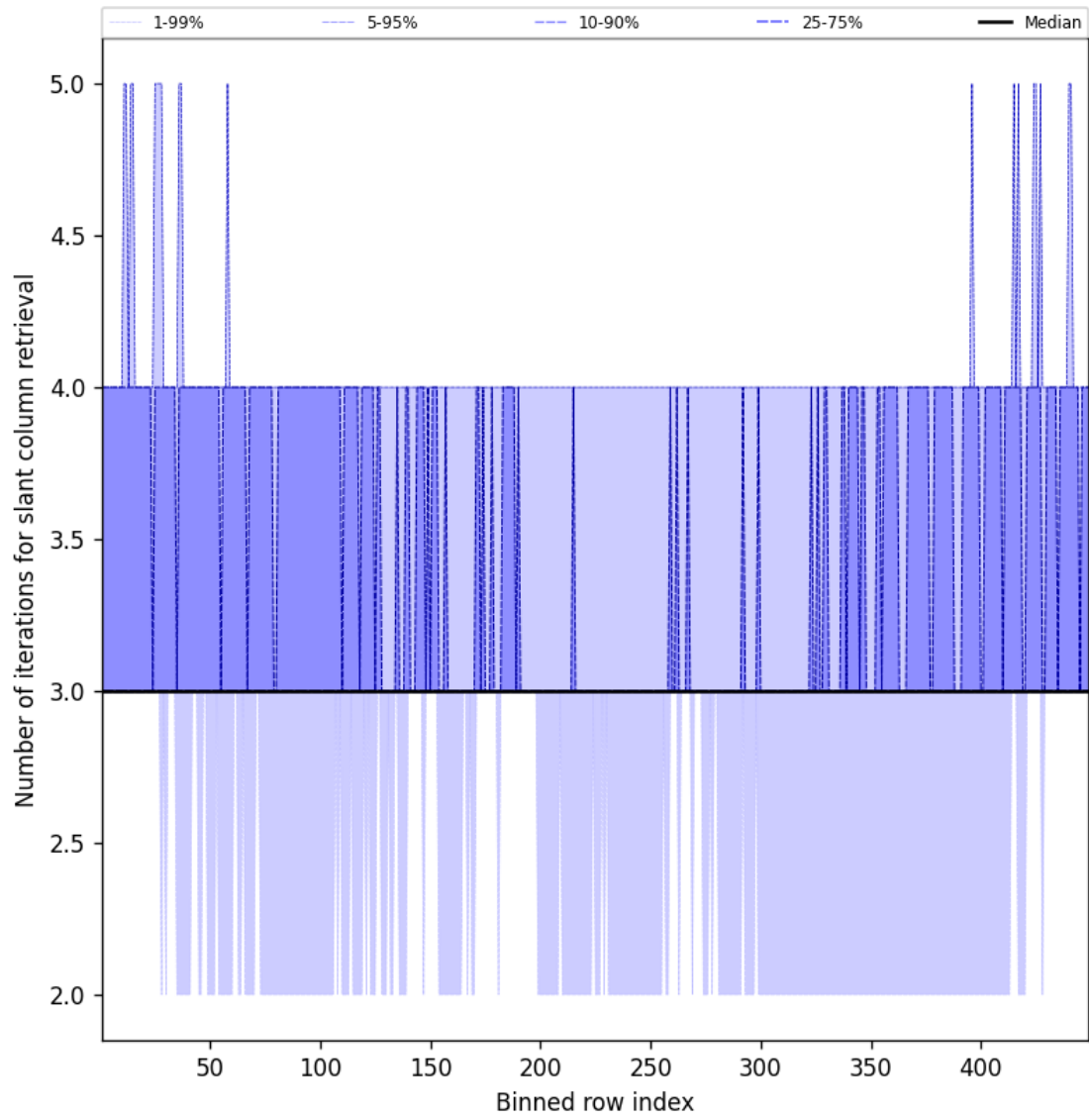
Figure 45: Along track statistics of “Number of iterations for slant column retrieval” for 2025-02-05 to 2025-02-06
