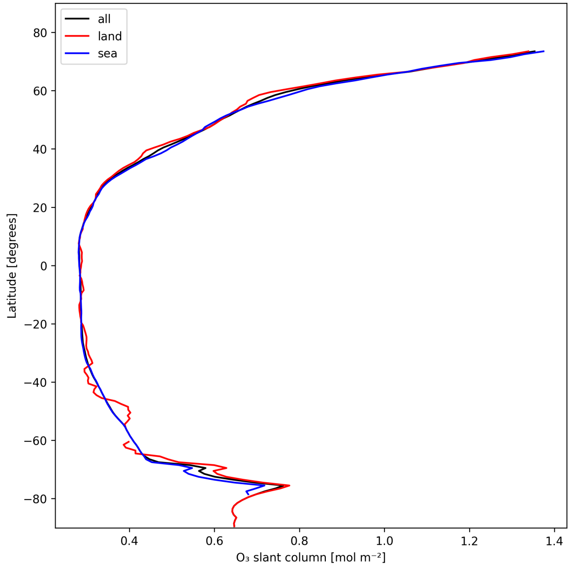
Figure 19: Zonal average of “O 3 slant column” for 2025-02-05 to 2025-02-06.
