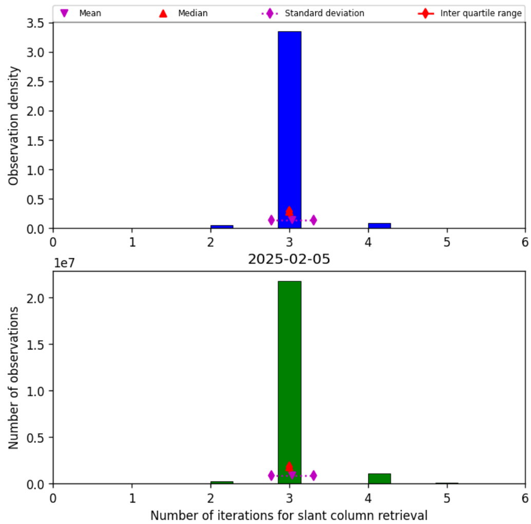
Figure 33: Histogram of “Number of iterations for slant column retrieval” for 2025-02-05 to 2025-02-06
