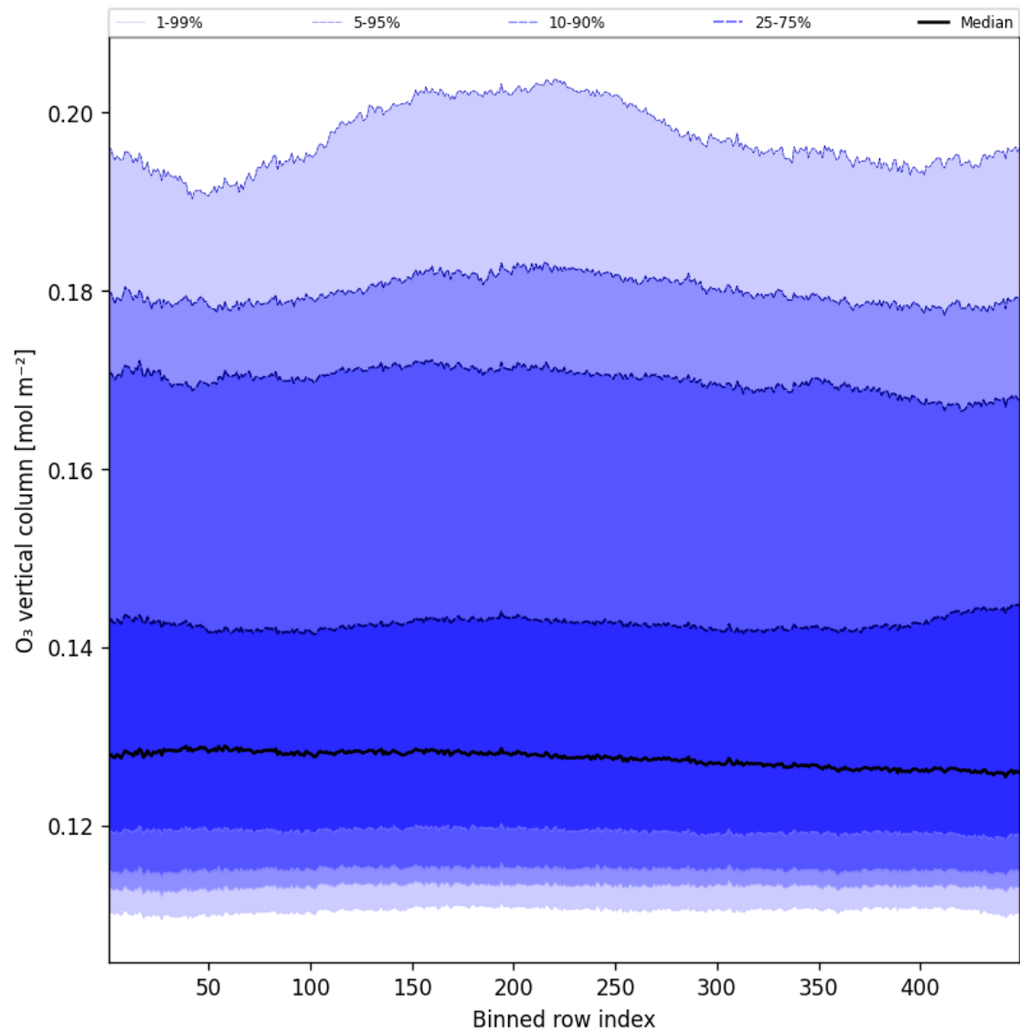
Figure 41: Along track statistics of “O 3 vertical column” for 2025-02-05 to 2025-02-06
