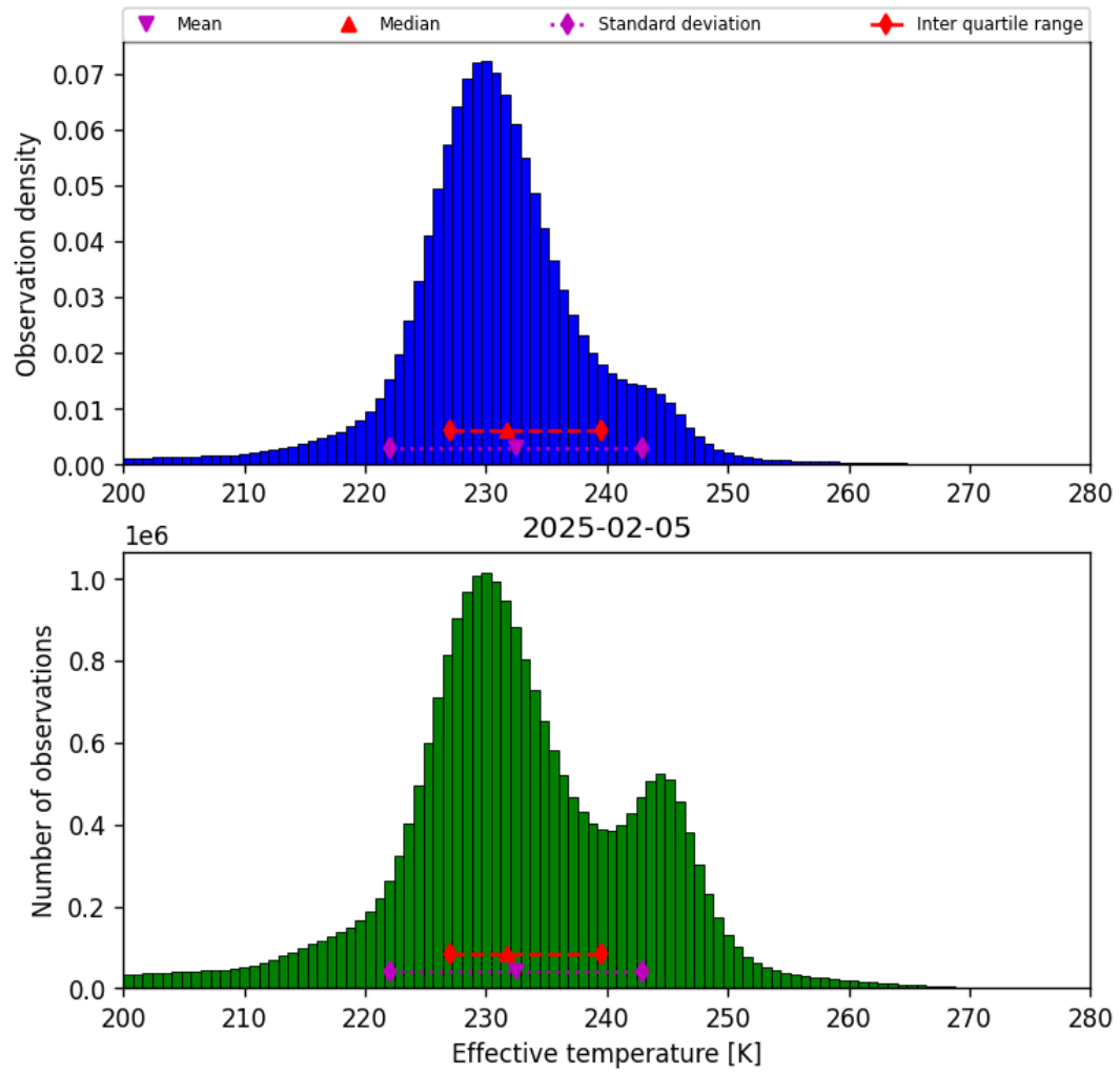
Figure 38: Histogram of “Effective temperature” for 2025-02-05 to 2025-02-06
