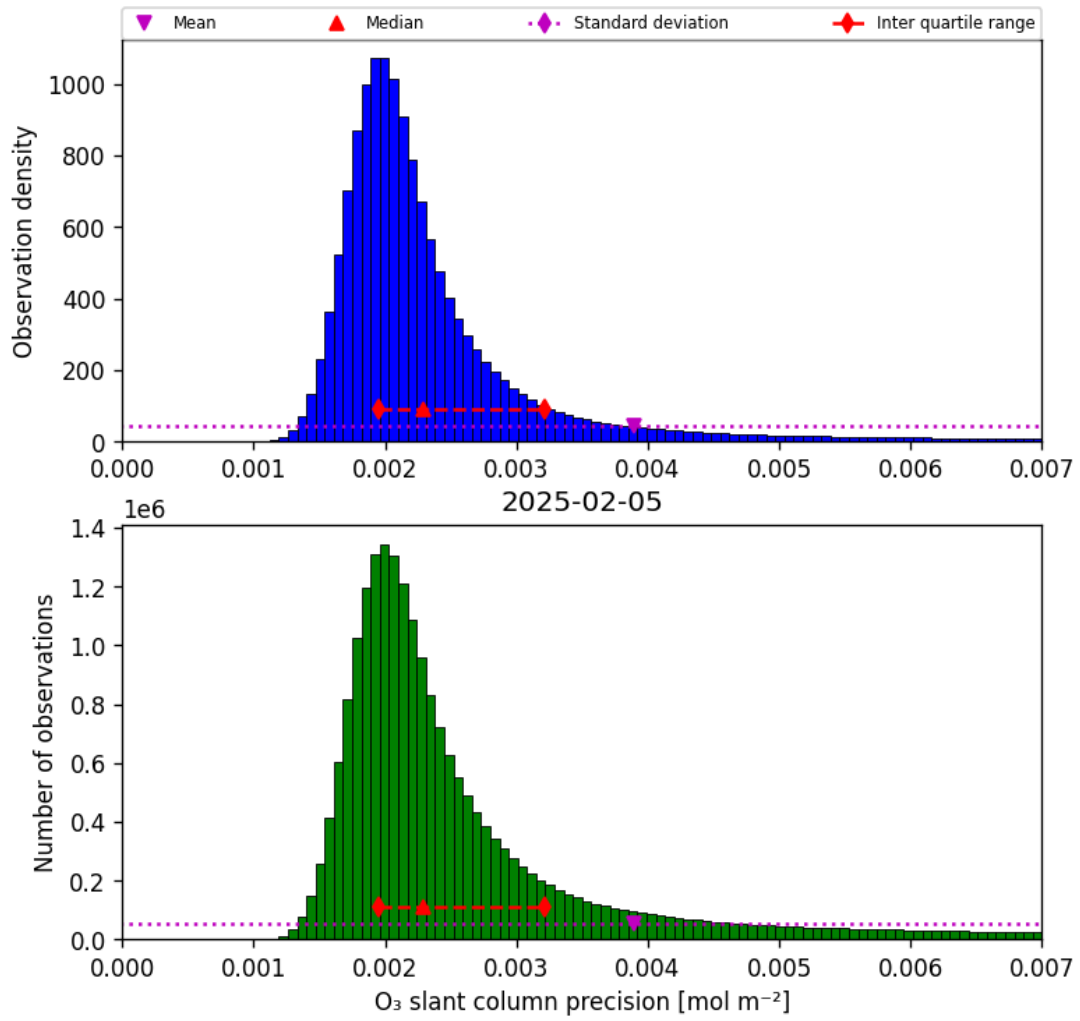
Figure 32: Histogram of “O 3 slant column precision” for 2025-02-05 to 2025-02-06
