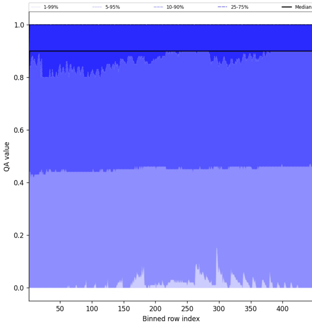
Figure 40: Along track statistics of “QA value” for 2025-02-05 to 2025-02-06
