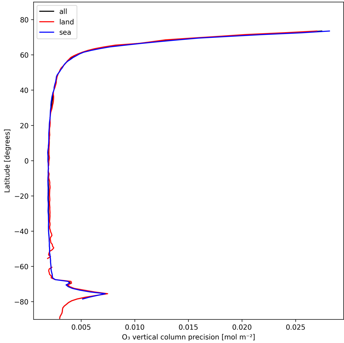
Figure 18: Zonal average of “O 3 vertical column precision” for 2025-02-05 to 2025-02-06.
