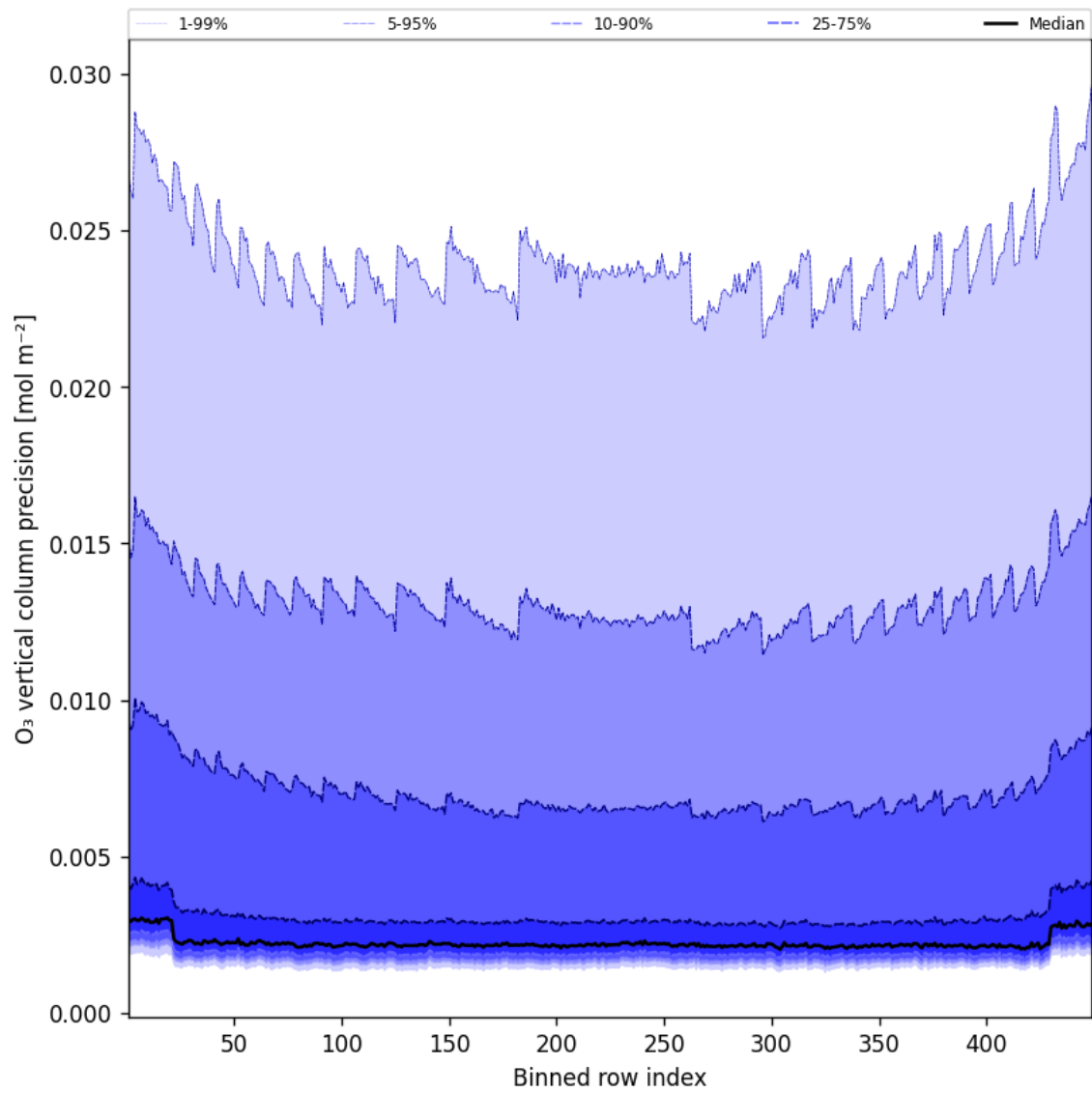
Figure 42: Along track statistics of “O 3 vertical column precision” for 2025-02-05 to 2025-02-06
