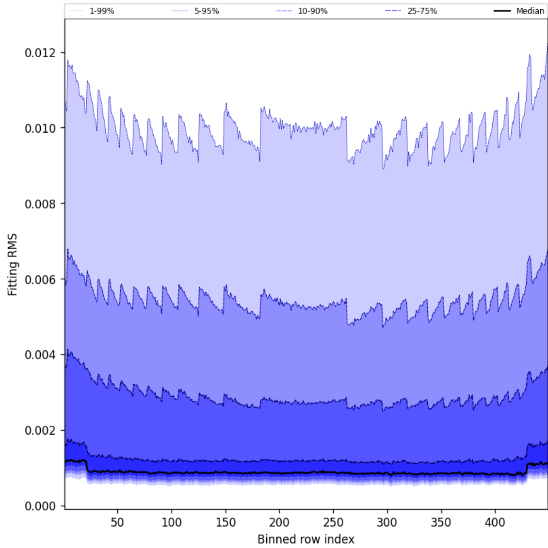
Figure 46: Along track statistics of “Fitting RMS” for 2025-02-05 to 2025-02-06
