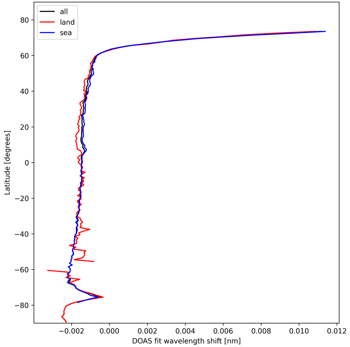
Figure 23: Zonal average of “DOAS fit wavelength shift” for 2025-02-05 to 2025-02-06.
