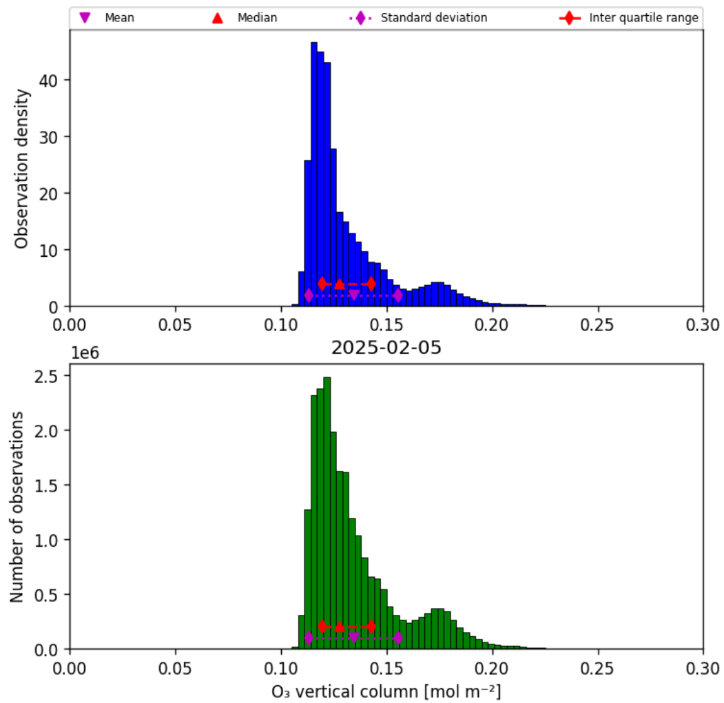
Figure 29: Histogram of “O 3 vertical column” for 2025-02-05 to 2025-02-06
