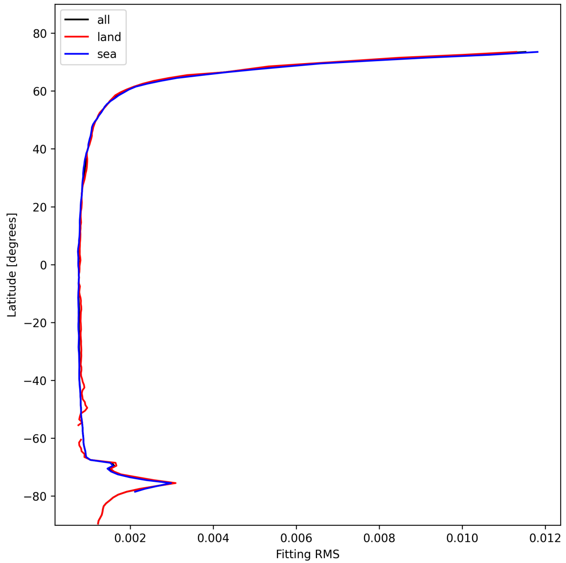
Figure 22: Zonal average of “Fitting RMS” for 2025-02-05 to 2025-02-06.
