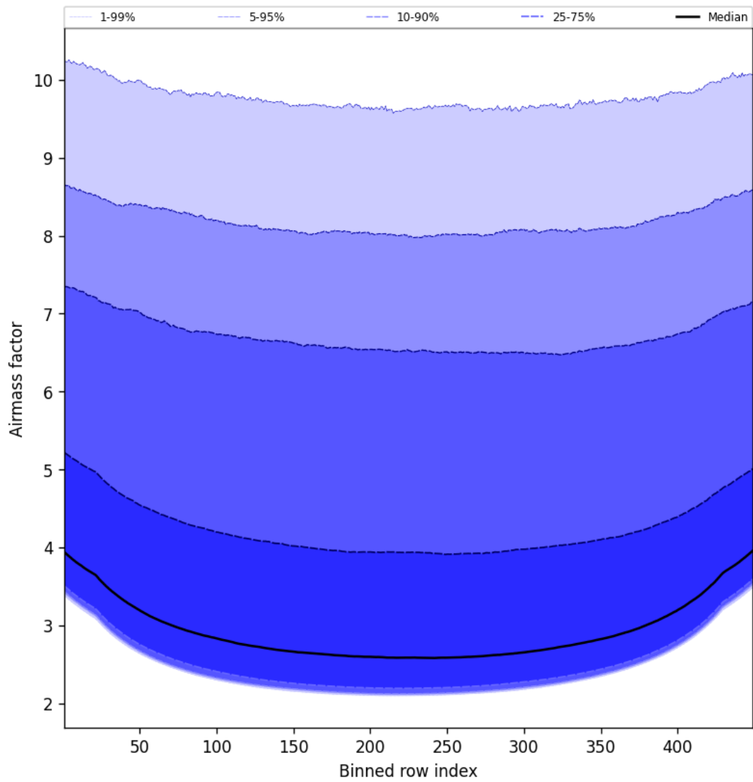
Figure 49: Along track statistics of “Airmass factor” for 2025-02-05 to 2025-02-06
