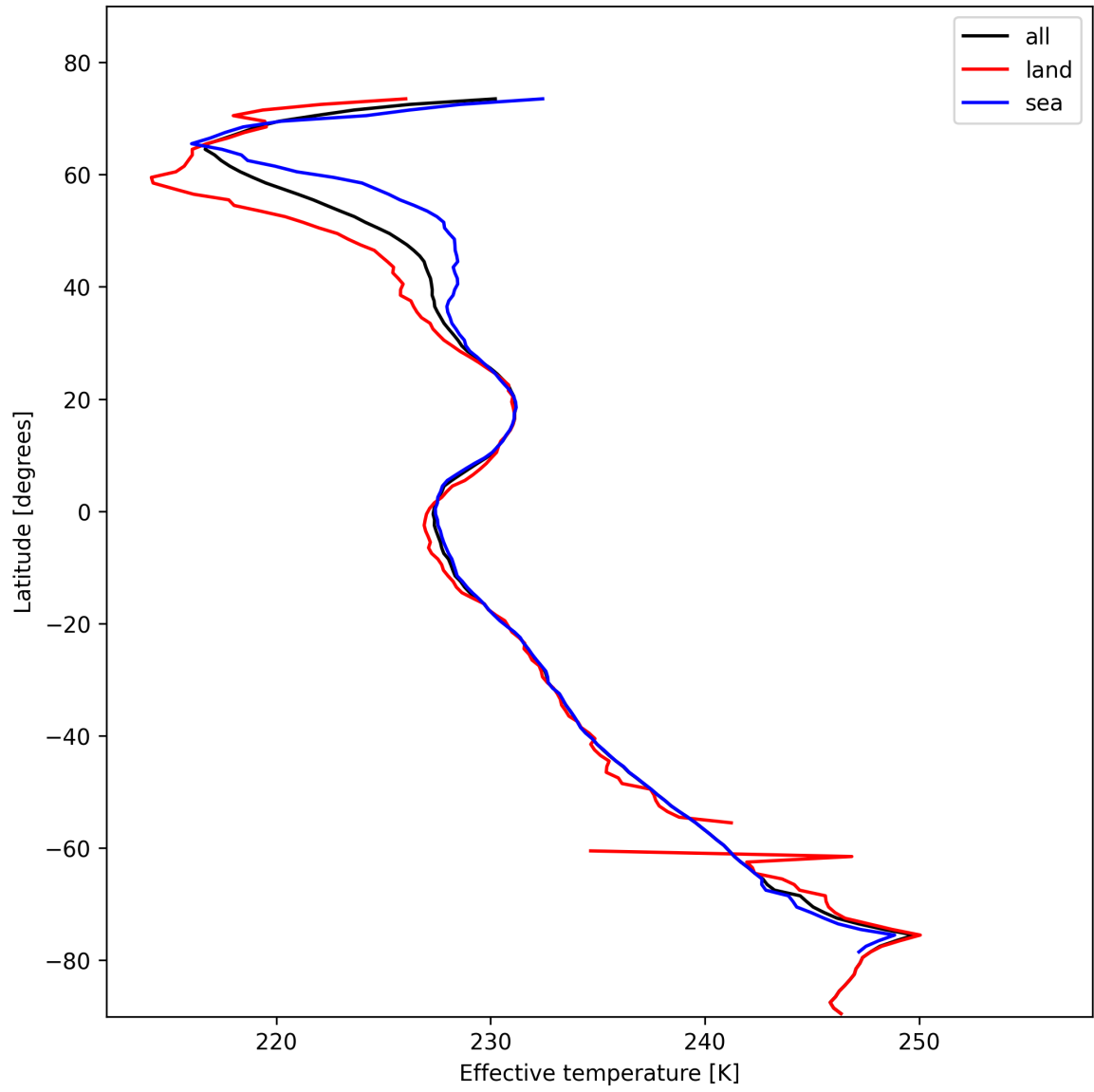
Figure 26: Zonal average of "Effective temperature" for 2025-02-05 to 2025-02-06.
