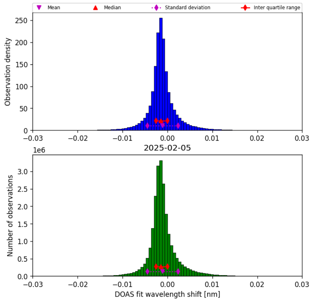
Figure 35: Histogram of “DOAS fit wavelength shift” for 2025-02-05 to 2025-02-06
