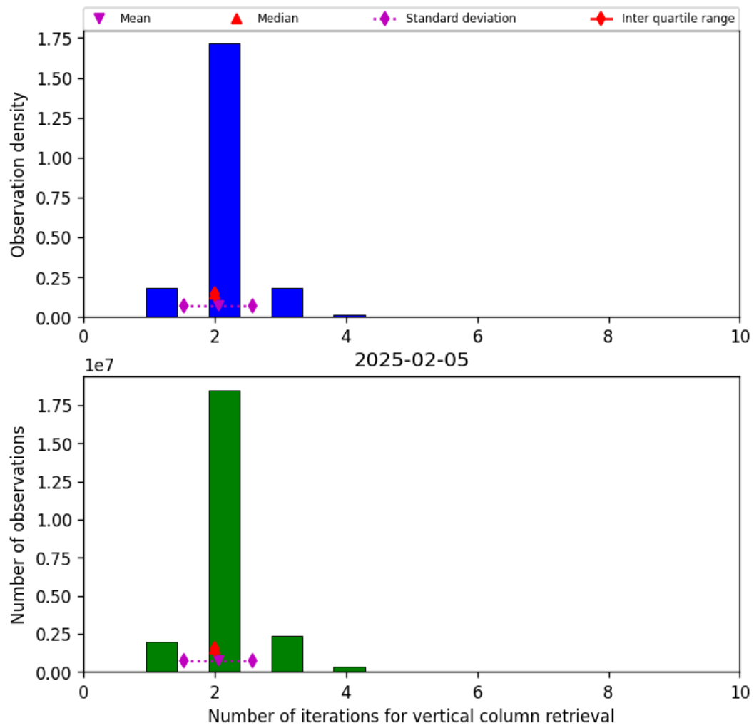
Figure 39: Histogram of “Number of iterations for vertical column retrieval” for 2025-02-05 to 2025-02-06
