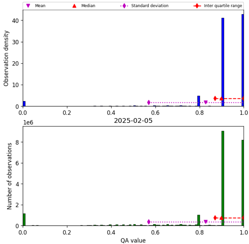
Figure 28: Histogram of “QA value” for 2025-02-05 to 2025-02-06
