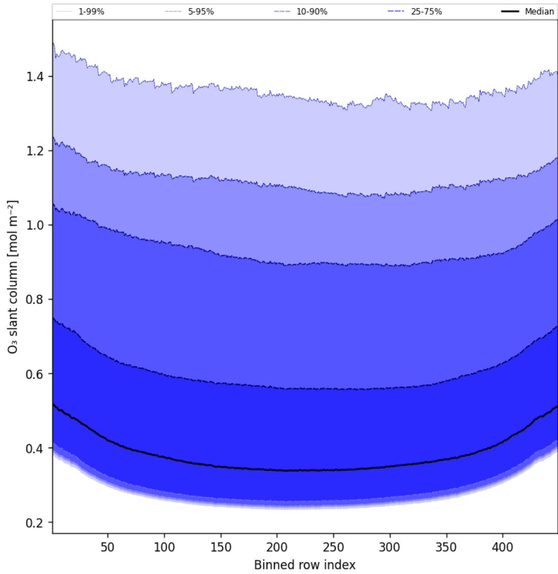
Figure 43: Along track statistics of “O 3 slant column” for 2025-02-05 to 2025-02-06
