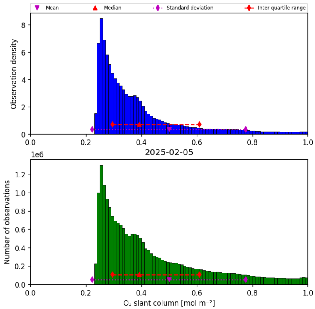
Figure 31: Histogram of “O 3 slant column” for 2025-02-05 to 2025-02-06
