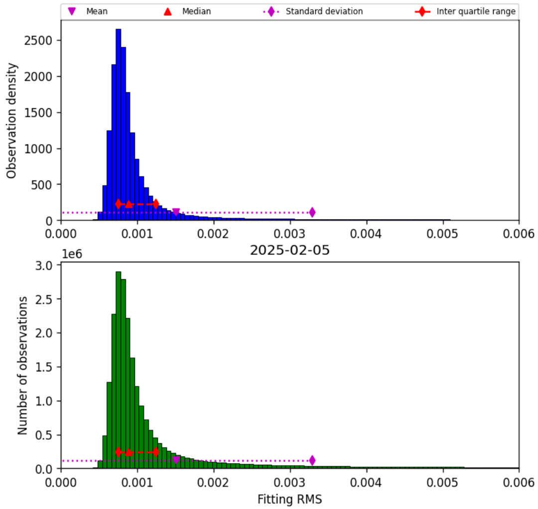
Figure 34: Histogram of “Fitting RMS” for 2025-02-05 to 2025-02-06
