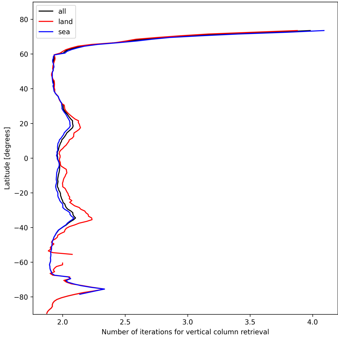
Figure 27: Zonal average of “Number of iterations for vertical column retrieval” for 2025-02-05 to 2025-02-06.
