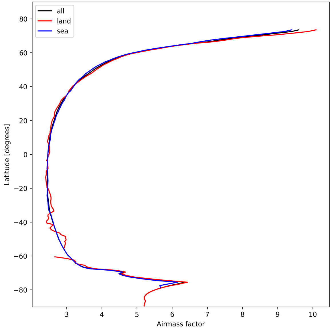
Figure 25: Zonal average of “Airmass factor” for 2025-02-05 to 2025-02-06.
