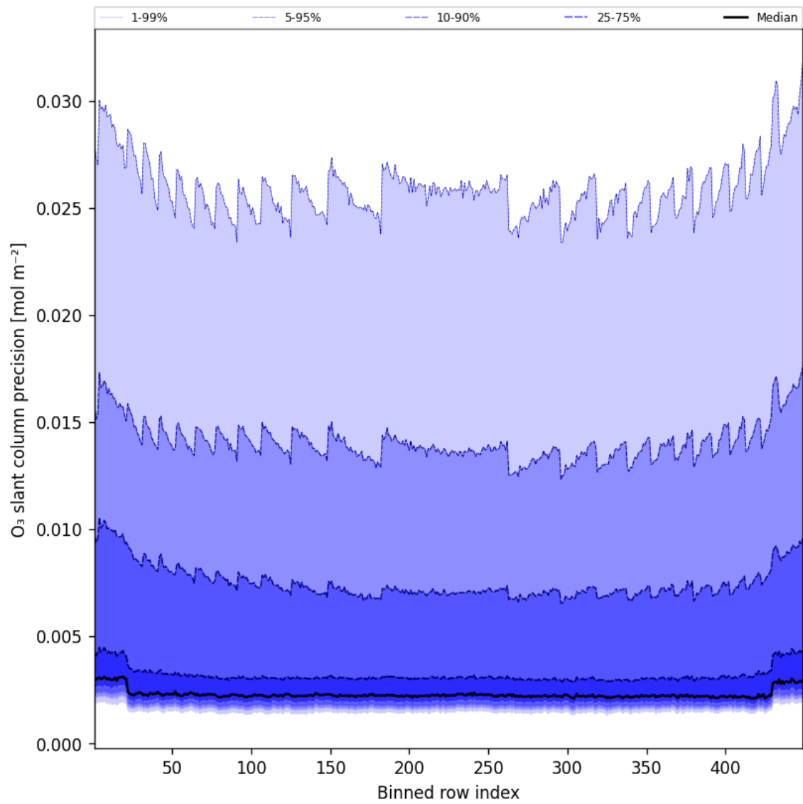
Figure 44: Along track statistics of “O 3 slant column precision” for 2025-02-05 to 2025-02-06
