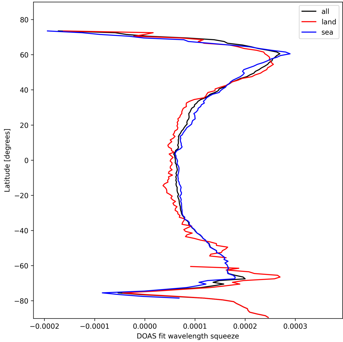
Figure 24: Zonal average of “DOAS fit wavelength squeeze” for 2025-02-05 to 2025-02-06.
