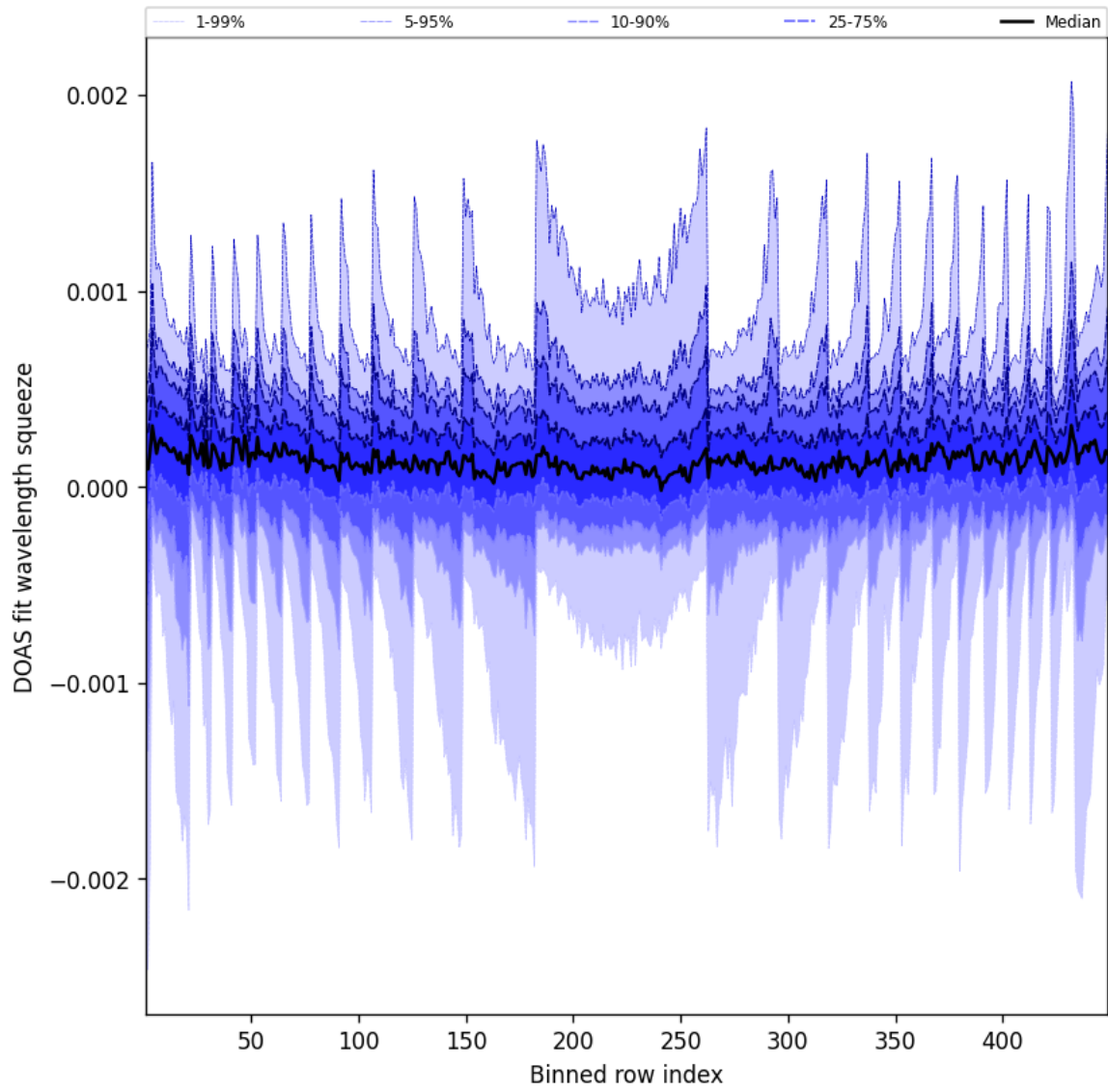
Figure 48: Along track statistics of “DOAS fit wavelength squeeze” for 2025-02-05 to 2025-02-06
