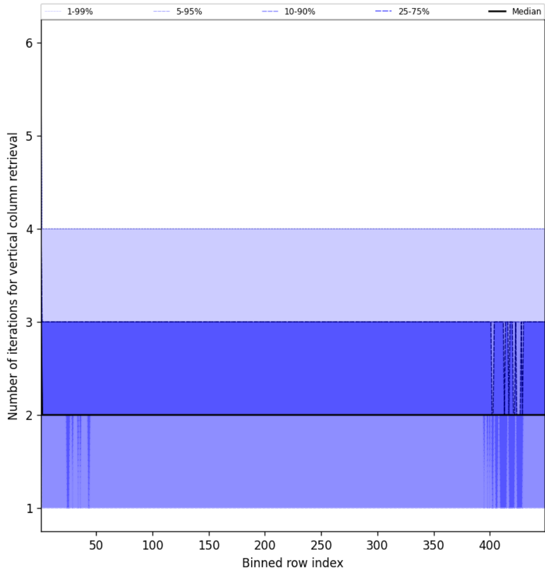
Figure 51: Along track statistics of “Number of iterations for vertical column retrieval” for 2025-02-05 to 2025-02-06
