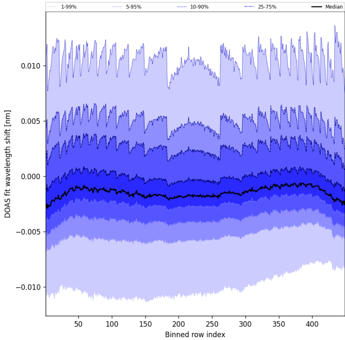
Figure 47: Along track statistics of “DOAS fit wavelength shift” for 2025-02-05 to 2025-02-06
