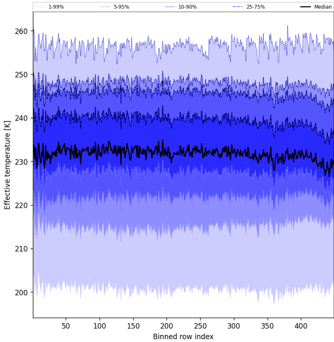
Figure 50: Along track statistics of “Effective temperature” for 2025-02-05 to 2025-02-06
