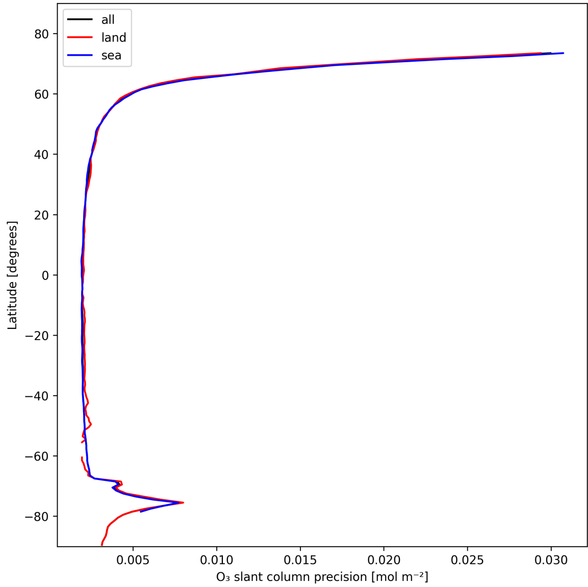
Figure 20: Zonal average of “O 3 slant column precision” for 2025-02-05 to 2025-02-06.
