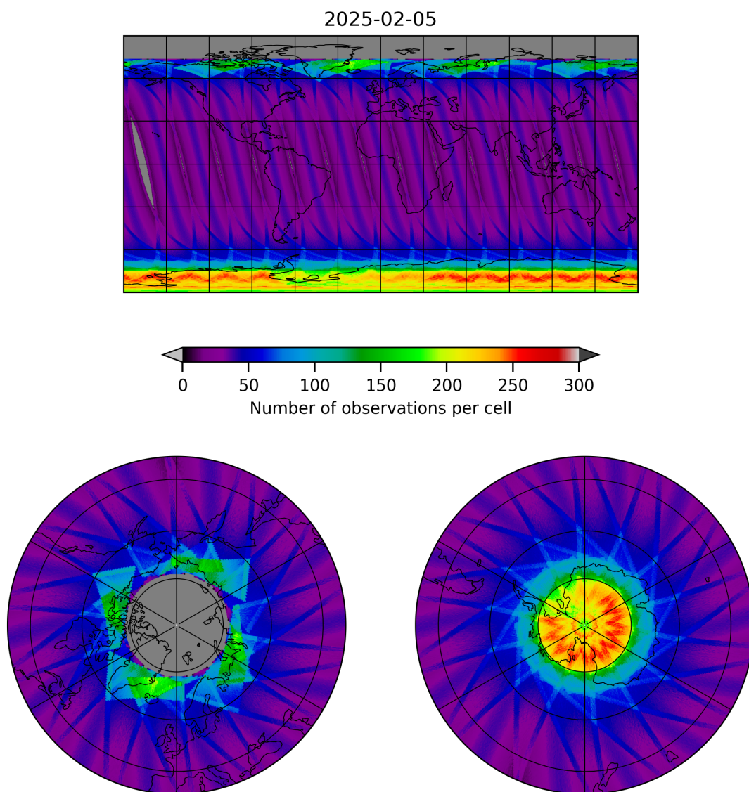
Figure 15: Map of the number of observations for 2025-02-05 to 2025-02-06
