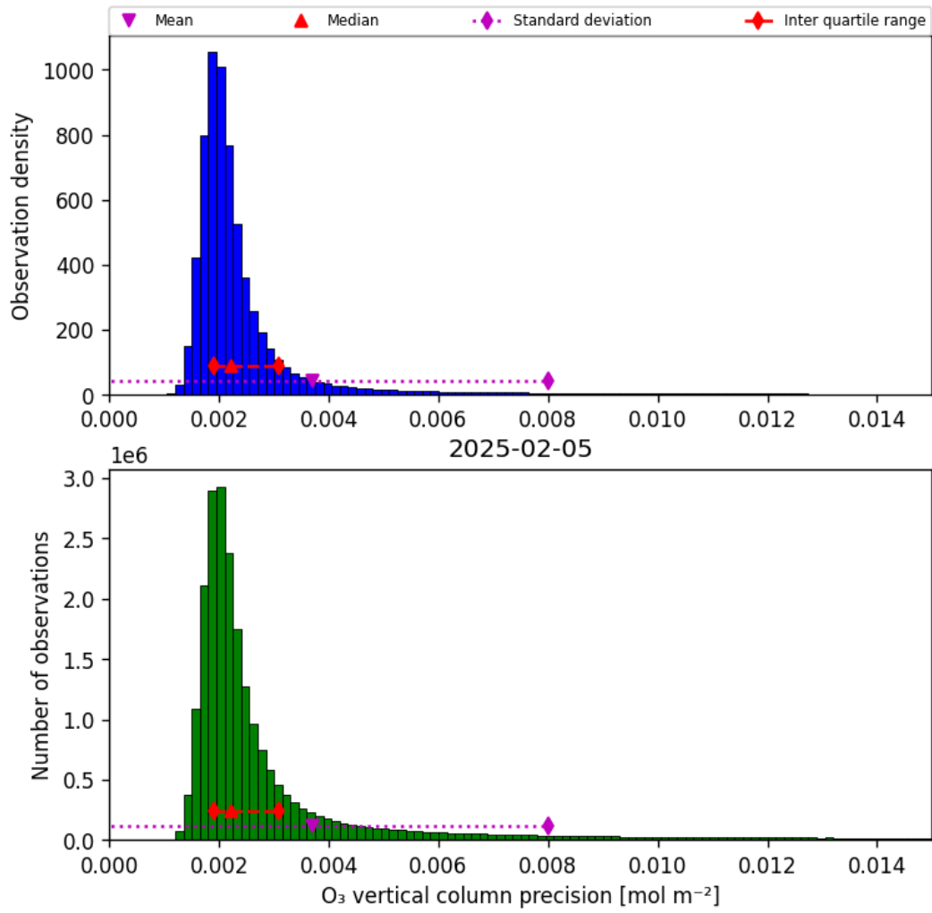
Figure 30: Histogram of “O 3 vertical column precision” for 2025-02-05 to 2025-02-06
