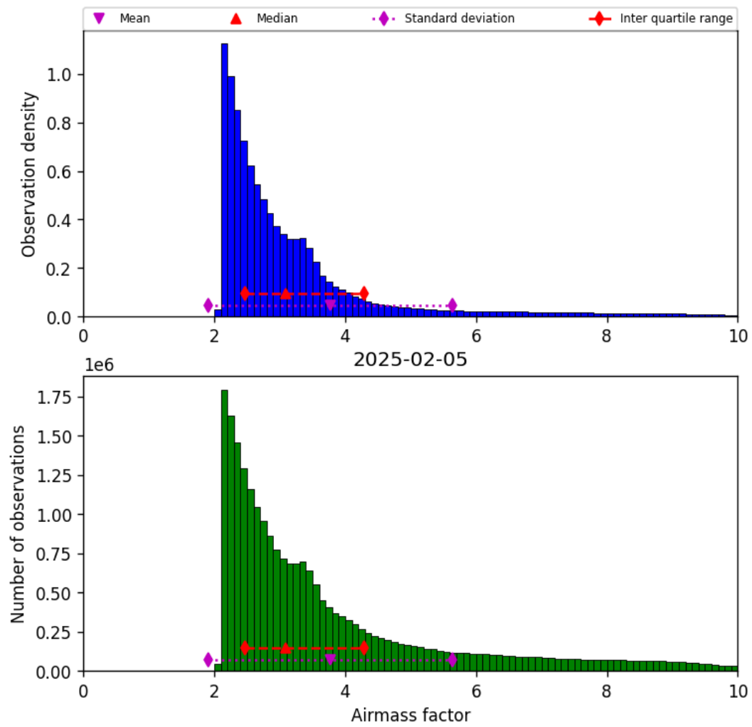
Figure 37: Histogram of “Airmass factor” for 2025-02-05 to 2025-02-06
