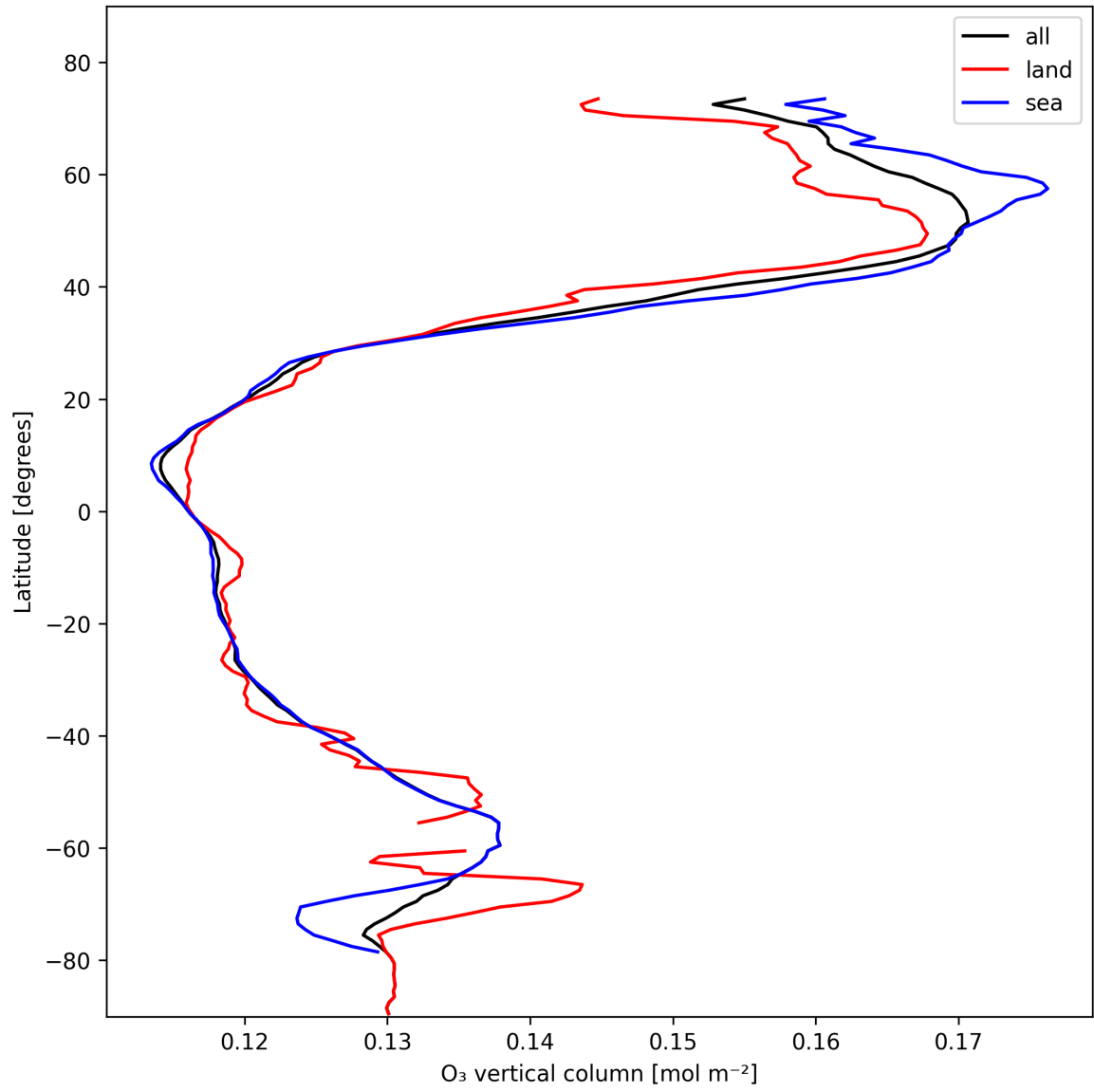
Figure 17: Zonal average of “O 3 vertical column” for 2025-02-05 to 2025-02-06.
