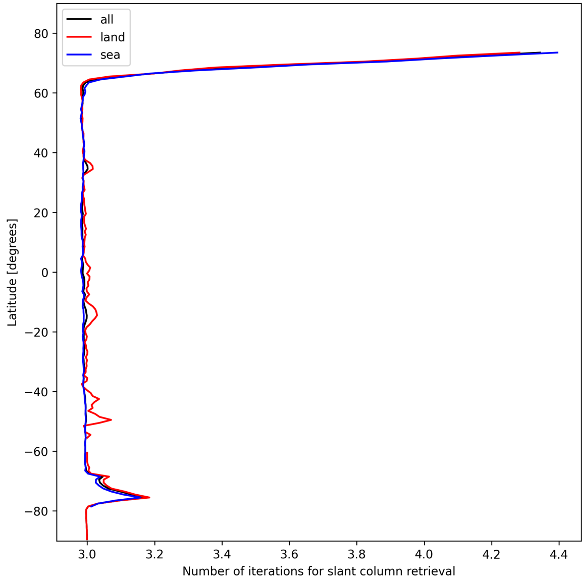
Figure 21: Zonal average of “Number of iterations for slant column retrieval” for 2025-02-05 to 2025-02-06.
