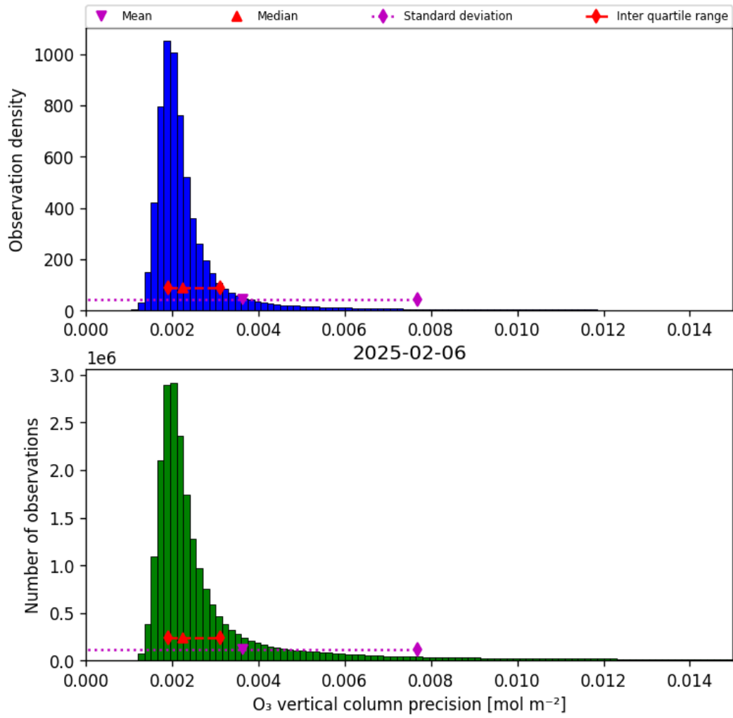
Figure 30: Histogram of “O 3 vertical column precision” for 2025-02-06 to 2025-02-06
