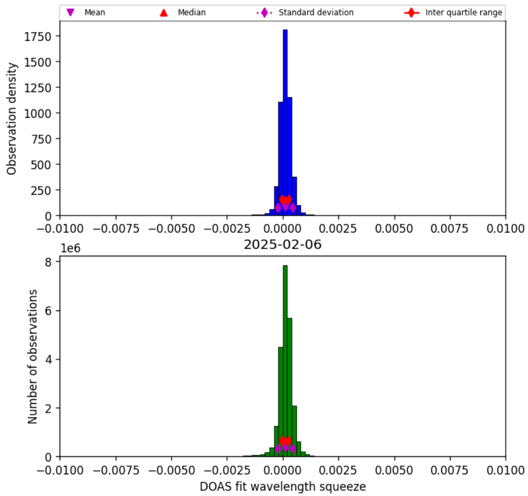
Figure 36: Histogram of “DOAS fit wavelength squeeze” for 2025-02-06 to 2025-02-06
