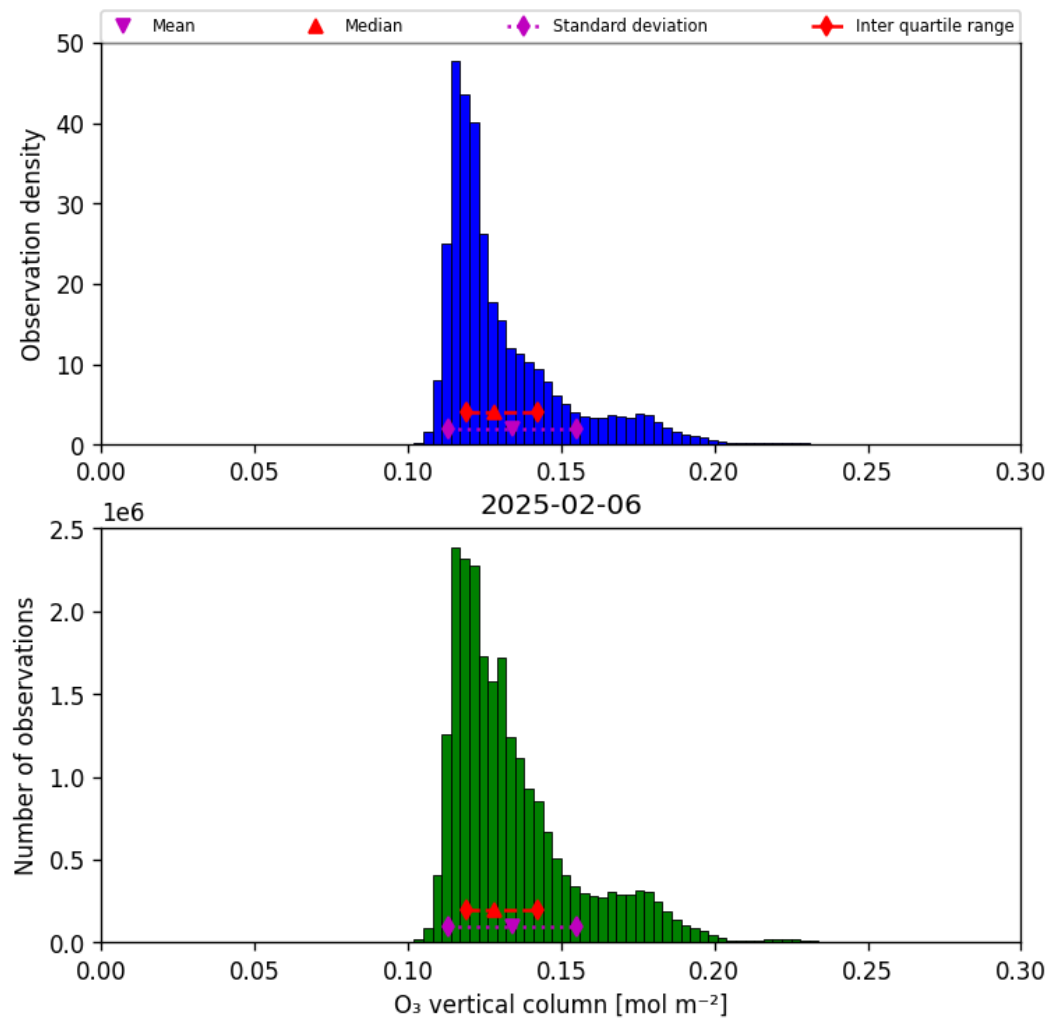
Figure 29: Histogram of “O 3 vertical column” for 2025-02-06 to 2025-02-06
