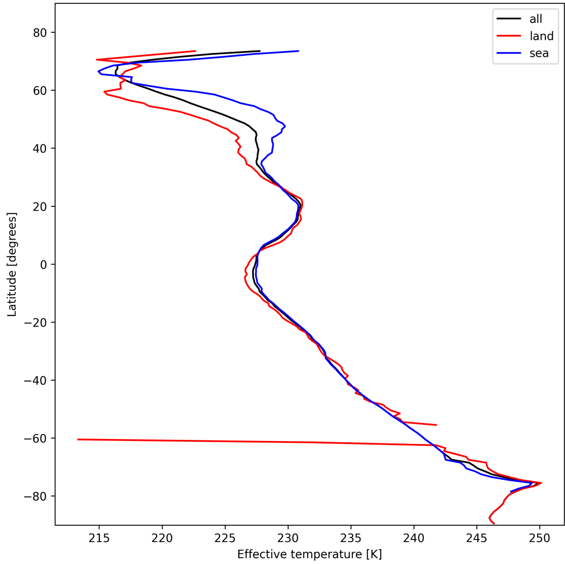
Figure 26: Zonal average of “Effective temperature” for 2025-02-06 to 2025-02-06.
