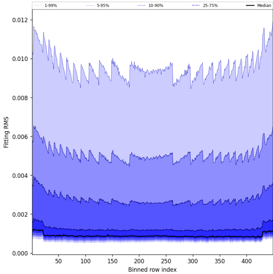
Figure 46: Along track statistics of “Fitting RMS” for 2025-02-06 to 2025-02-06
