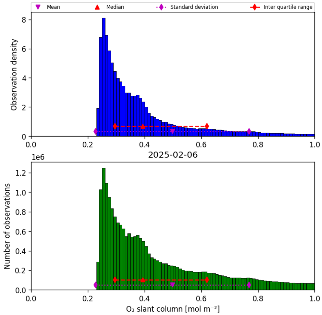
Figure 31: Histogram of “O 3 slant column” for 2025-02-06 to 2025-02-06
