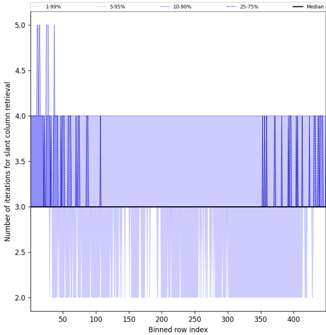
Figure 45: Along track statistics of “Number of iterations for slant column retrieval” for 2025-02-06 to 2025-02-06
