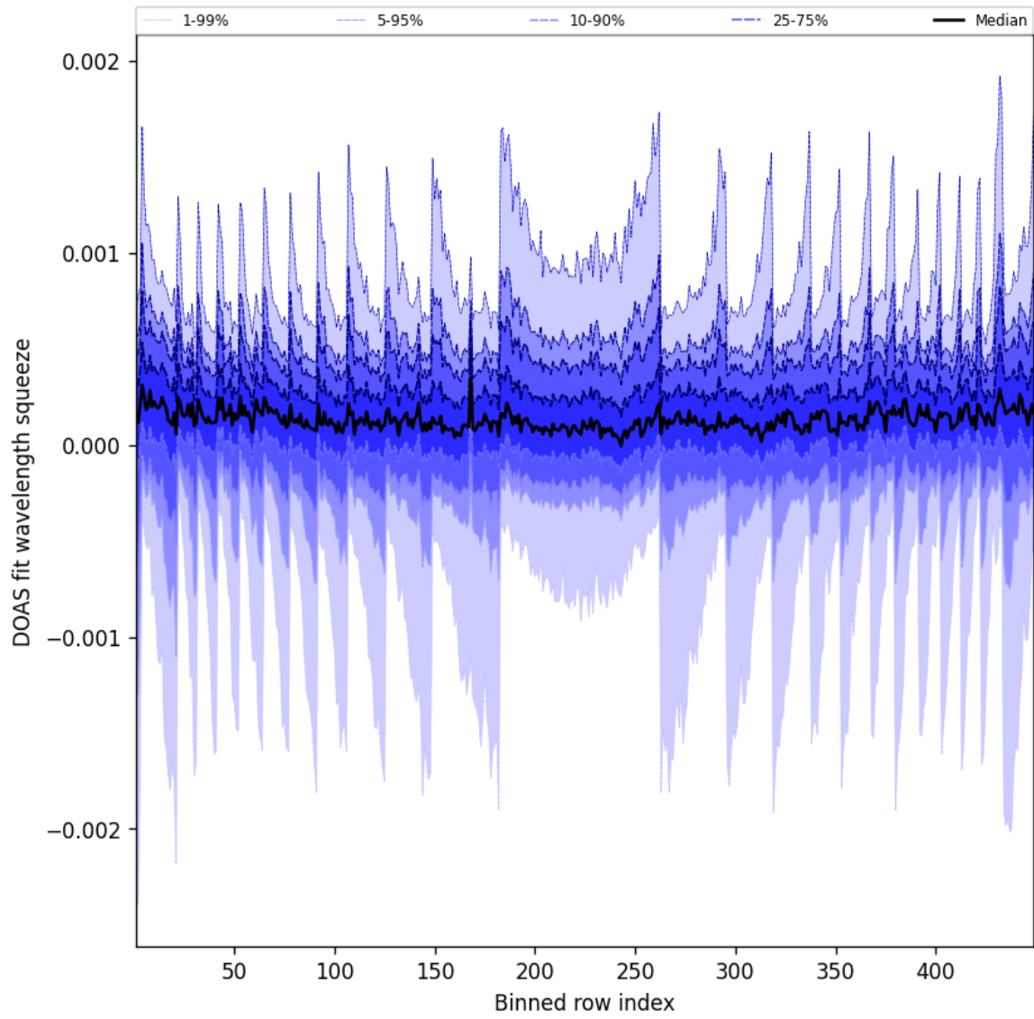
Figure 48: Along track statistics of “DOAS fit wavelength squeeze” for 2025-02-06 to 2025-02-06
