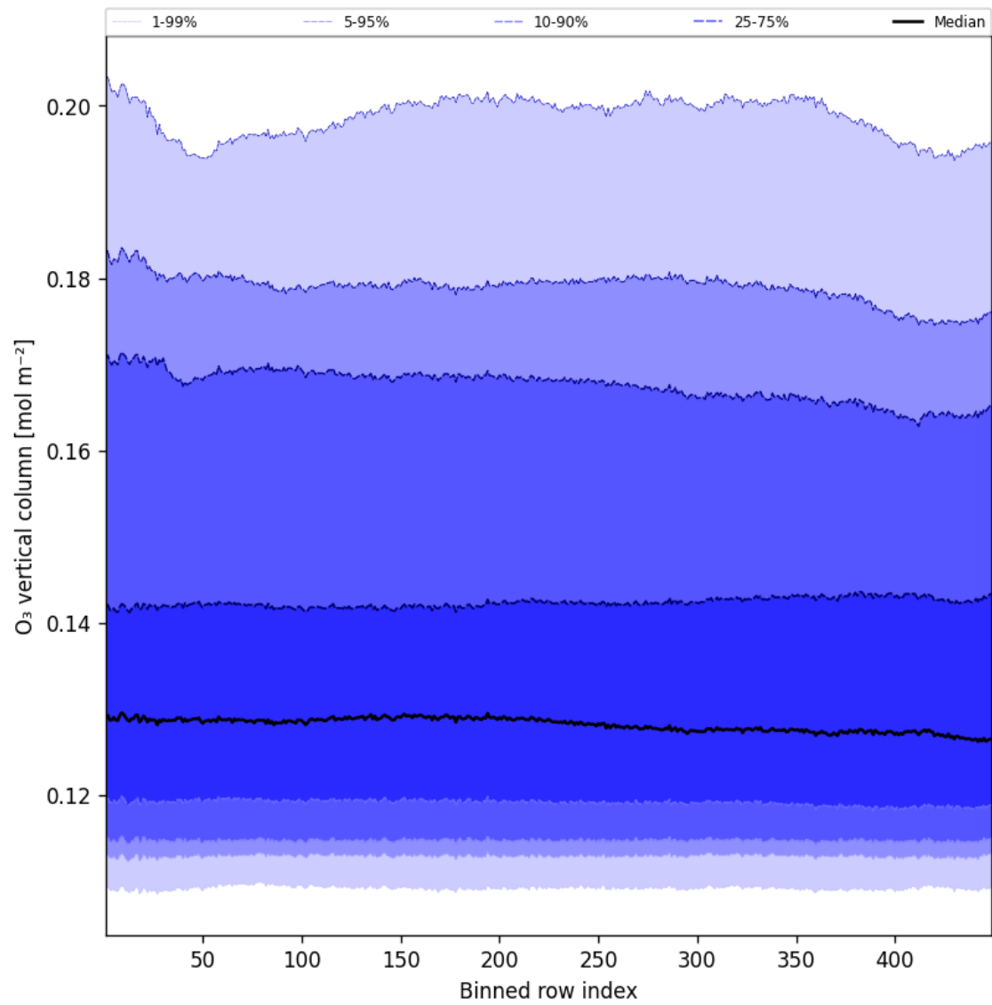
Figure 41: Along track statistics of “O 3 vertical column” for 2025-02-06 to 2025-02-06
