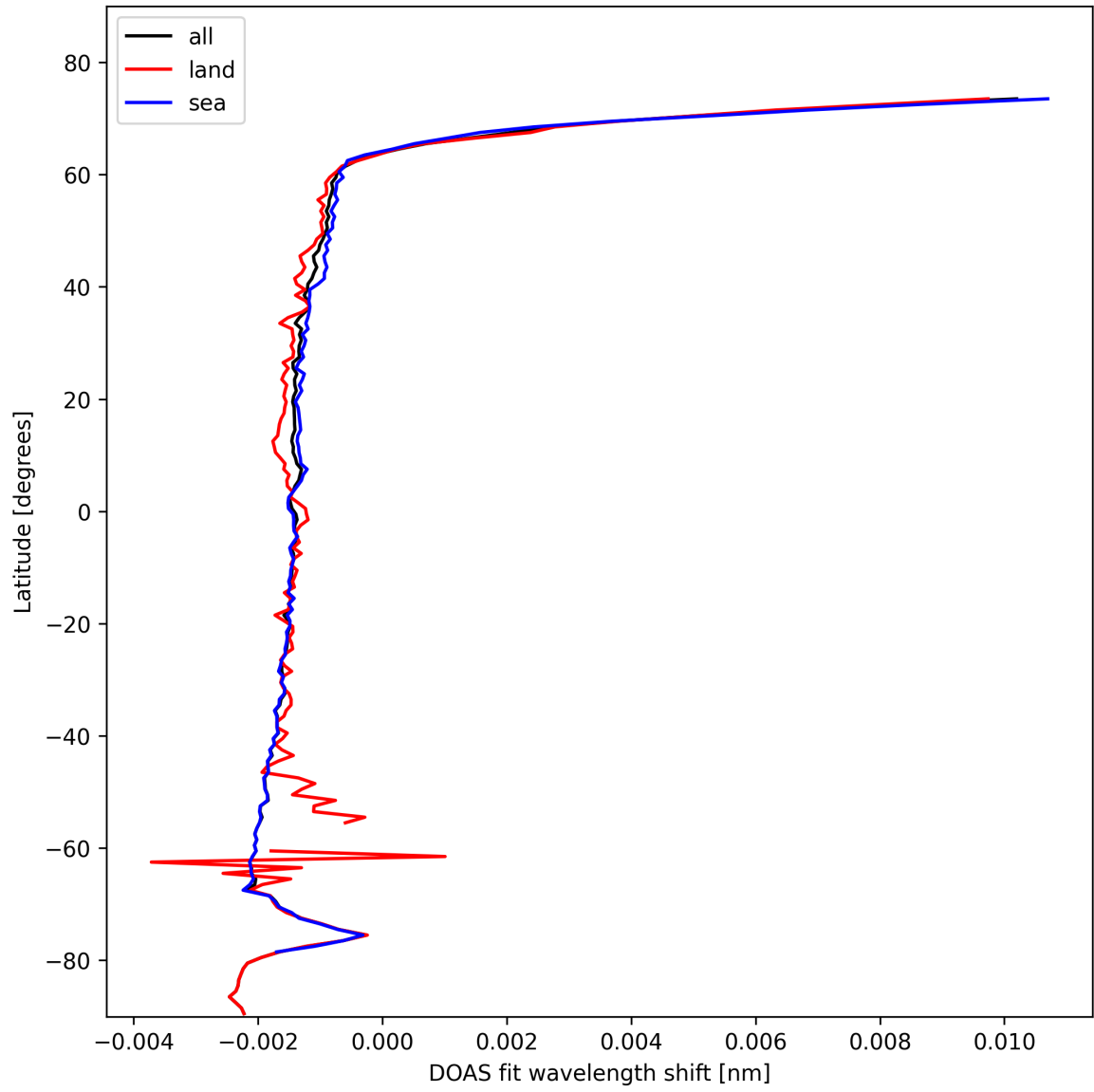
Figure 23: Zonal average of “DOAS fit wavelength shift” for 2025-02-06 to 2025-02-06.
