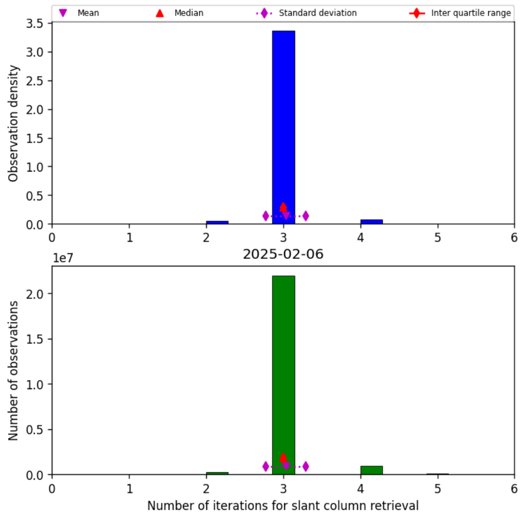
Figure 33: Histogram of "Number of iterations for slant column retrieval" for 2025-02-06 to 2025-02-06
