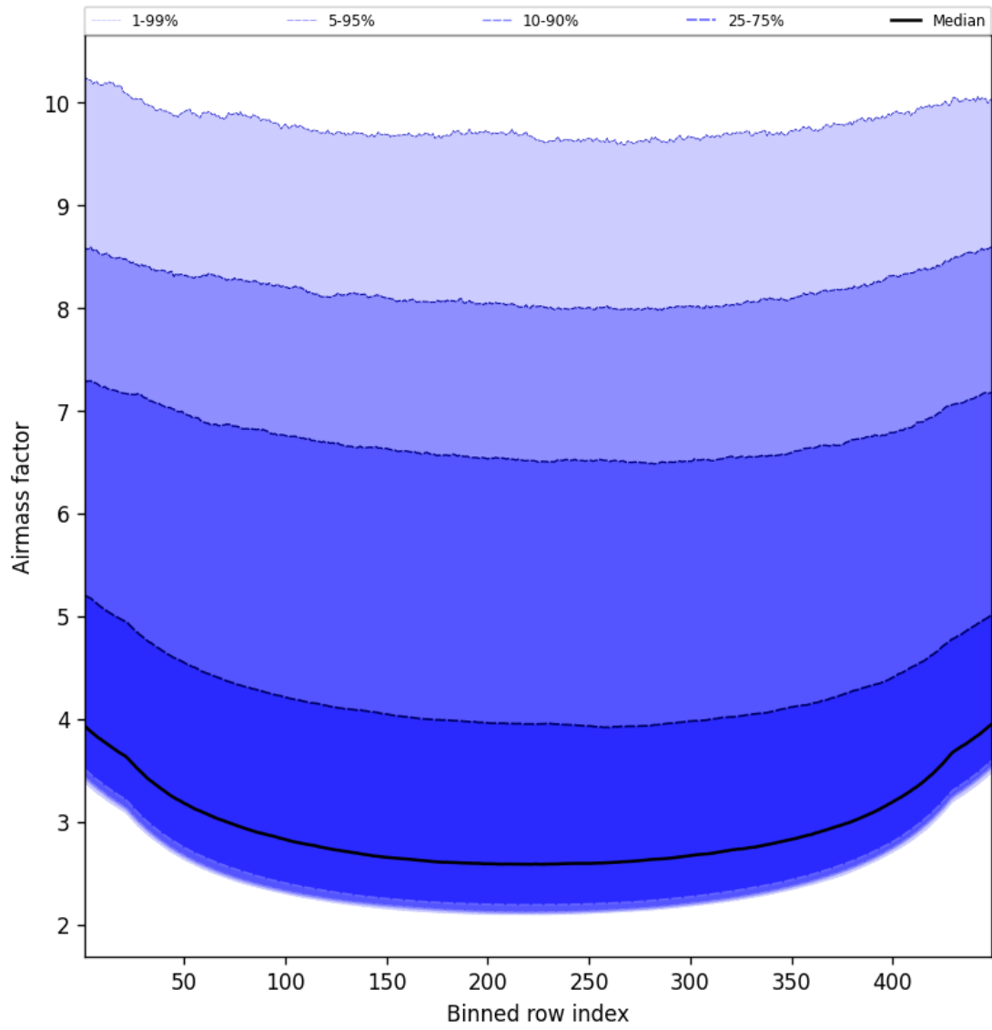
Figure 49: Along track statistics of “Airmass factor” for 2025-02-06 to 2025-02-06
