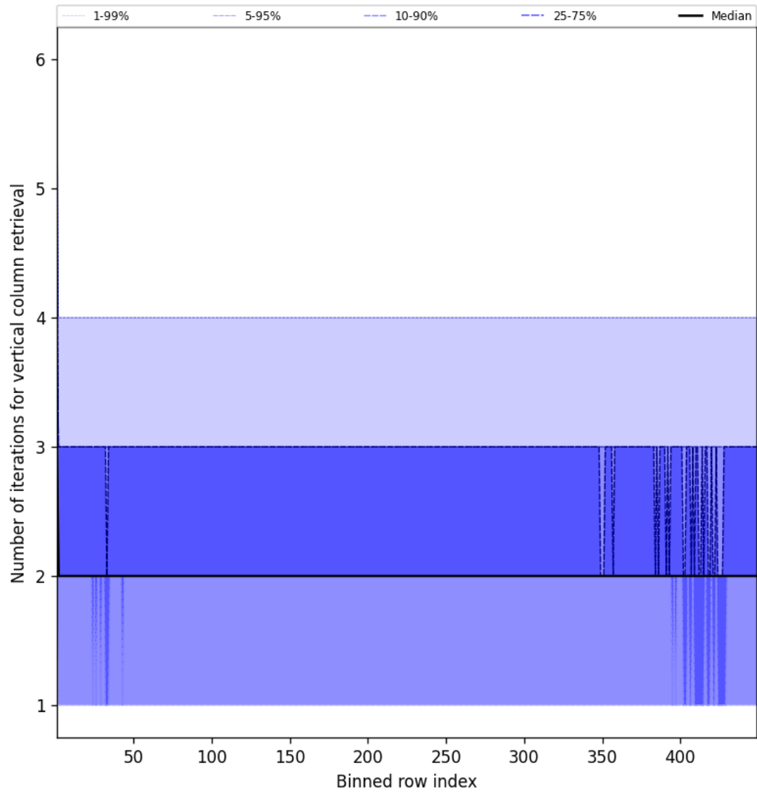
Figure 51: Along track statistics of “Number of iterations for vertical column retrieval” for 2025-02-06 to 2025-02-06
