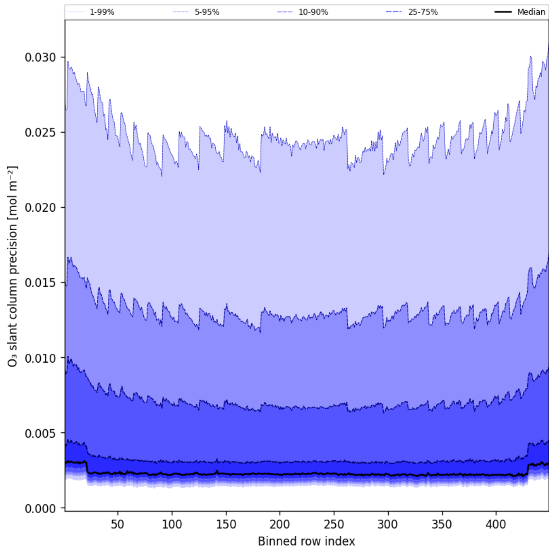
Figure 44: Along track statistics of “O 3 slant column precision” for 2025-02-06 to 2025-02-06
