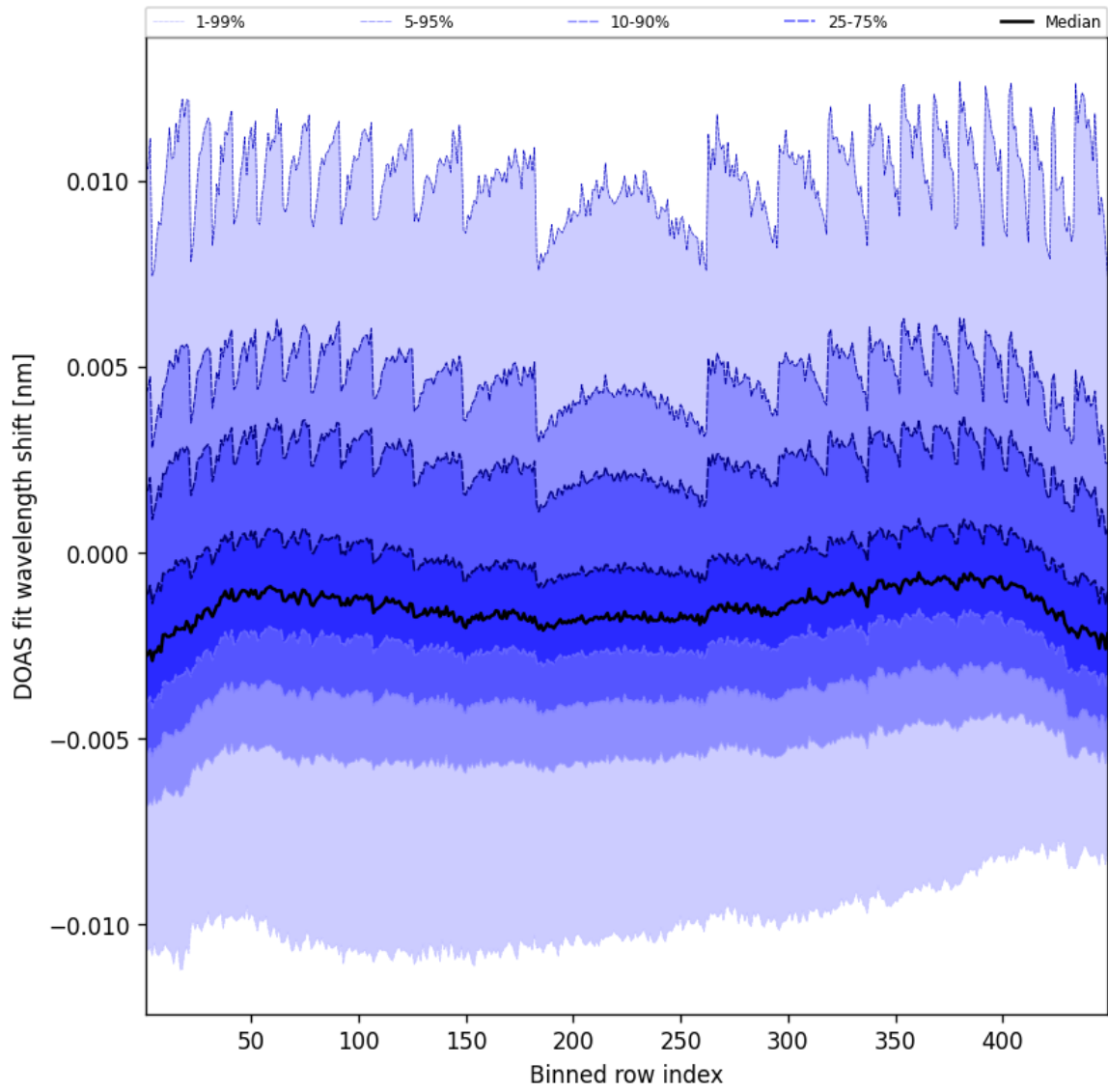
Figure 47: Along track statistics of “DOAS fit wavelength shift” for 2025-02-06 to 2025-02-06
