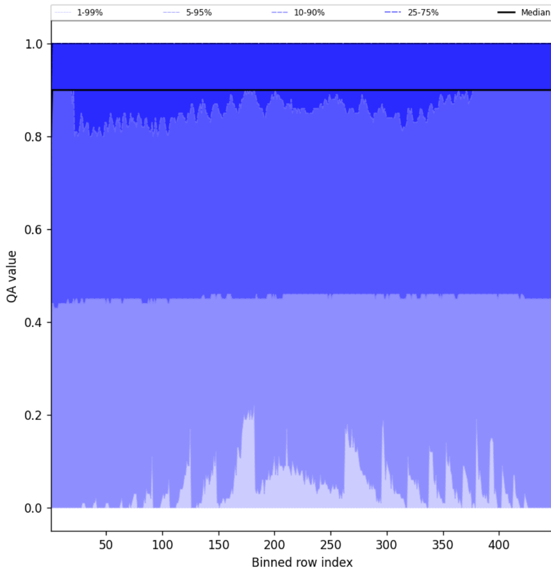
Figure 40: Along track statistics of “QA value” for 2025-02-06 to 2025-02-06
