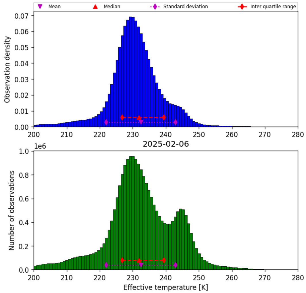
Figure 38: Histogram of “Effective temperature” for 2025-02-06 to 2025-02-06
