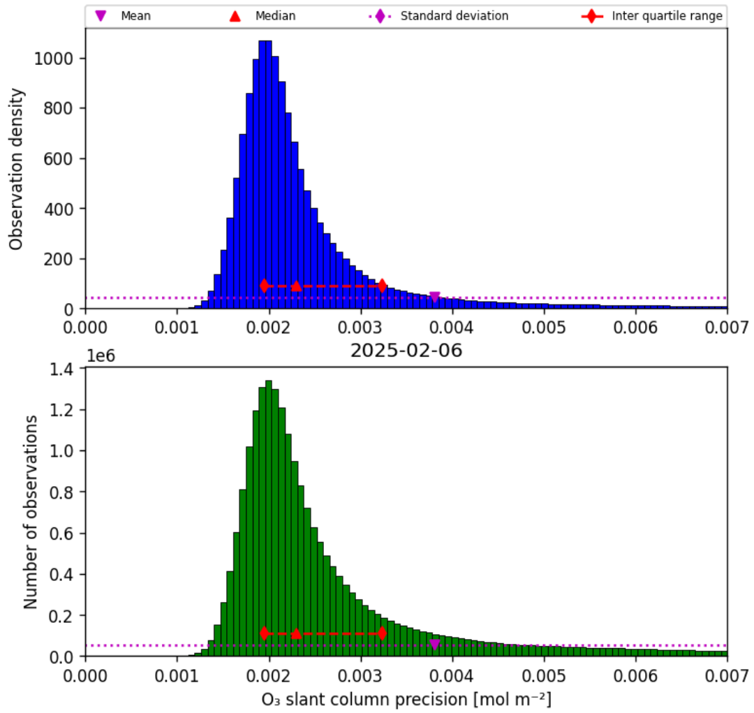
Figure 32: Histogram of “O 3 slant column precision” for 2025-02-06 to 2025-02-06
