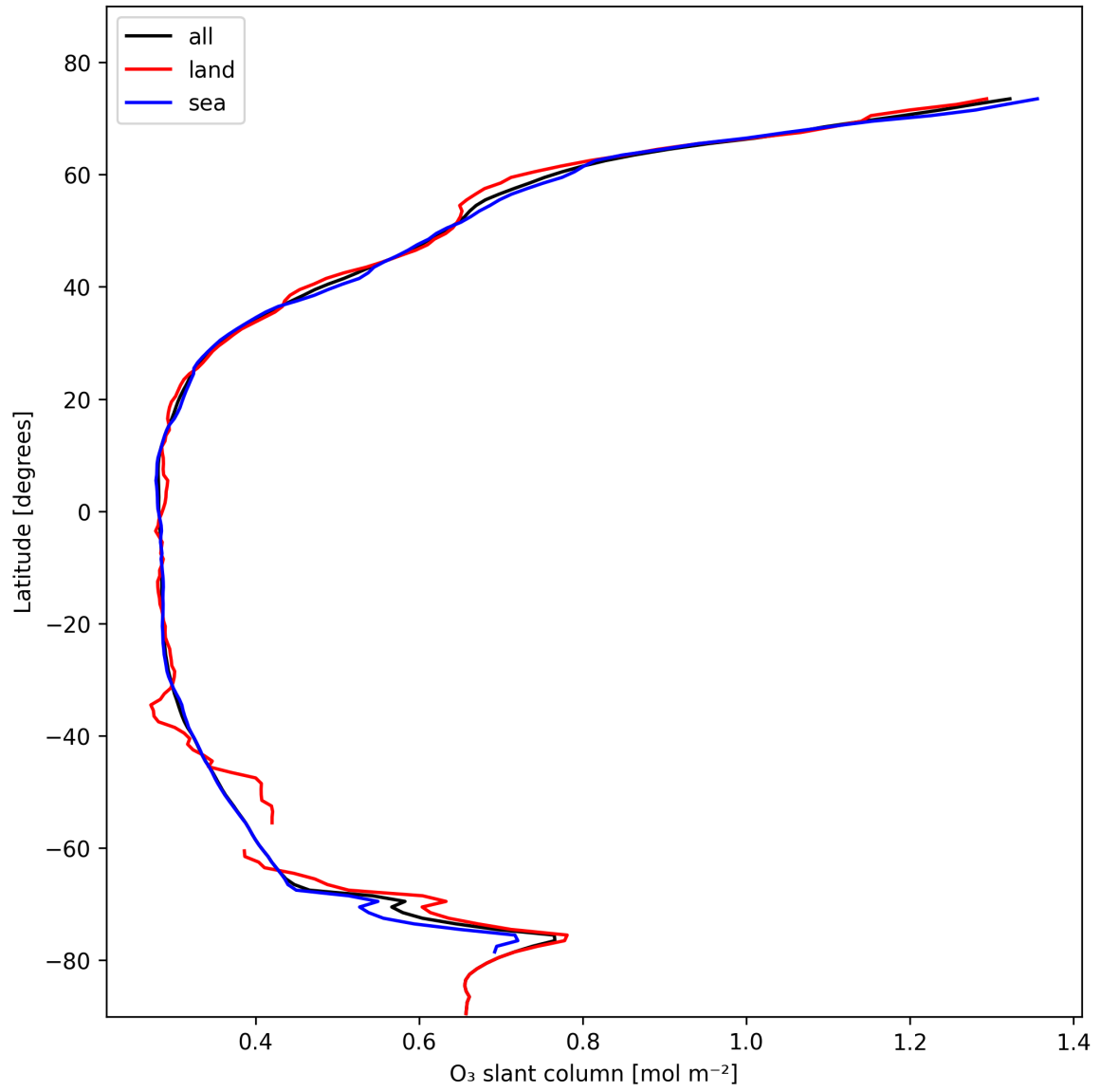
Figure 19: Zonal average of “O 3 slant column” for 2025-02-06 to 2025-02-06.
