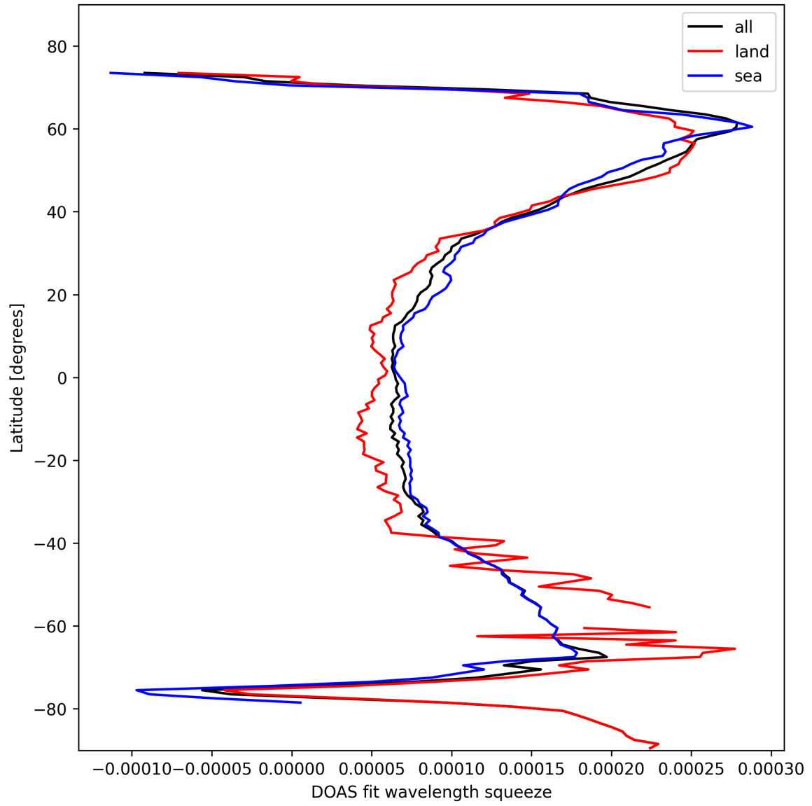
Figure 24: Zonal average of “DOAS fit wavelength squeeze” for 2025-02-06 to 2025-02-06.
