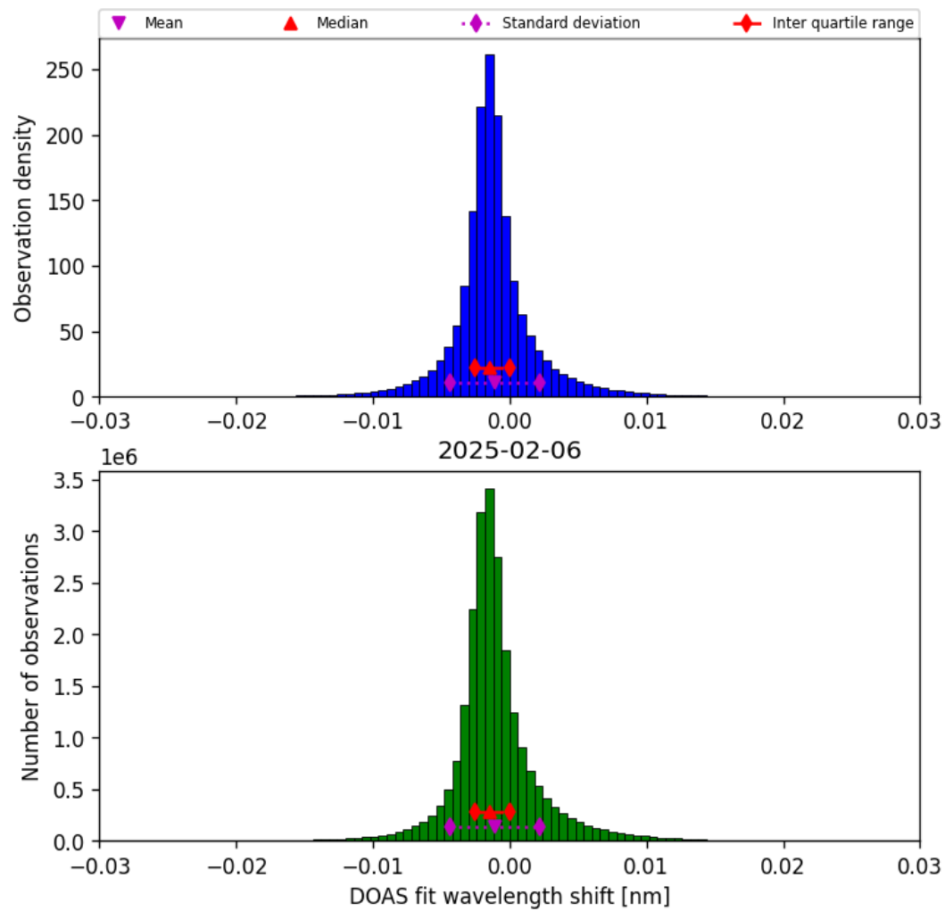
Figure 35: Histogram of “DOAS fit wavelength shift” for 2025-02-06 to 2025-02-06
