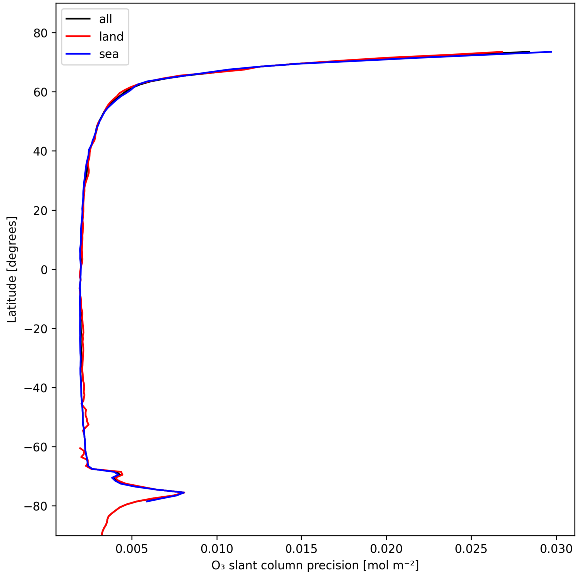
Figure 20: Zonal average of “O 3 slant column precision” for 2025-02-06 to 2025-02-06.
