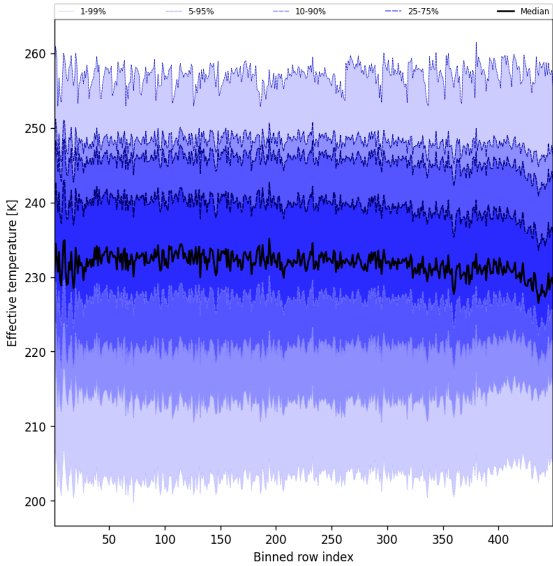
Figure 50: Along track statistics of “Effective temperature” for 2025-02-06 to 2025-02-06
