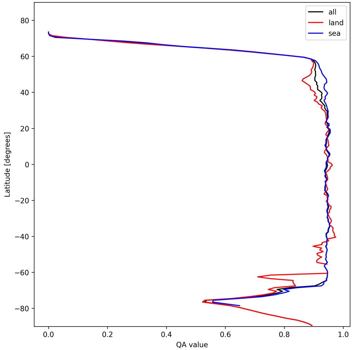
Figure 16: Zonal average of “QA value” for 2025-02-06 to 2025-02-06.
