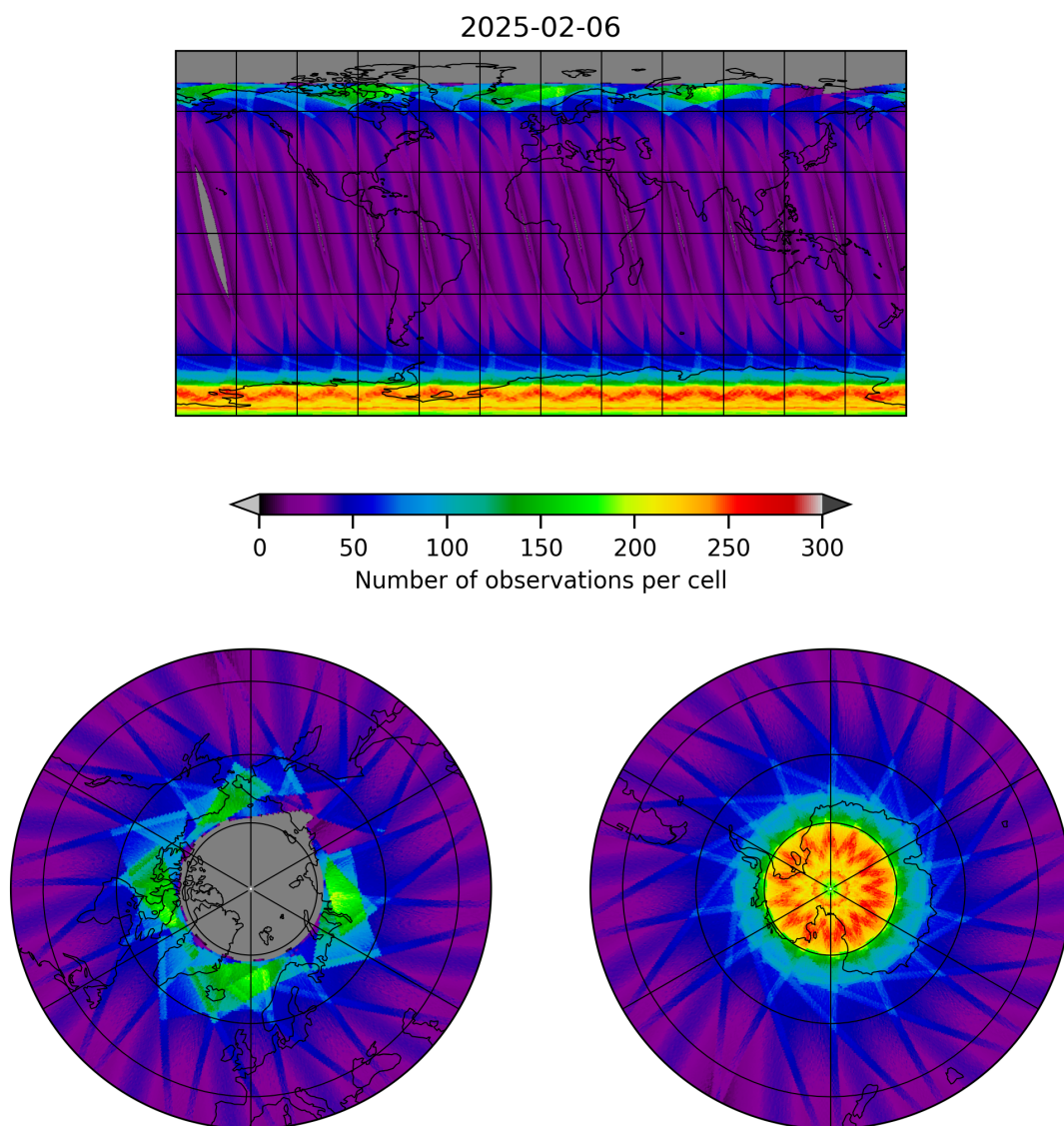
Figure 15: Map of the number of observations for 2025-02-06 to 2025-02-06
