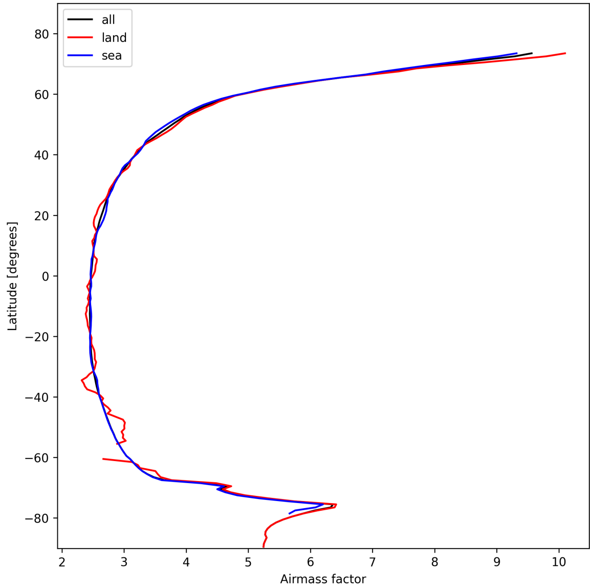
Figure 25: Zonal average of “Airmass factor” for 2025-02-06 to 2025-02-06.
