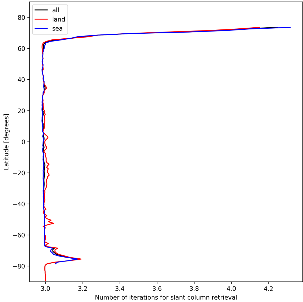
Figure 21: Zonal average of “Number of iterations for slant column retrieval” for 2025-02-06 to 2025-02-06.
