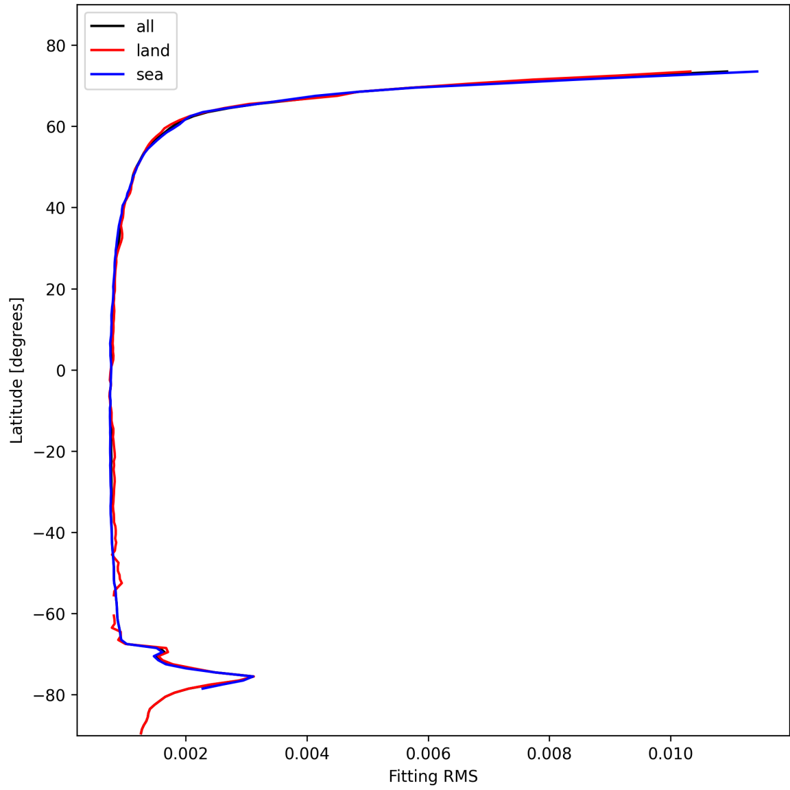
Figure 22: Zonal average of “Fitting RMS” for 2025-02-06 to 2025-02-06.
