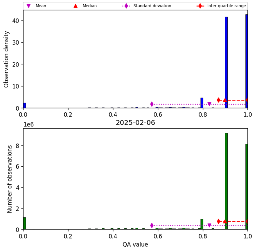
Figure 28: Histogram of “QA value” for 2025-02-06 to 2025-02-06
