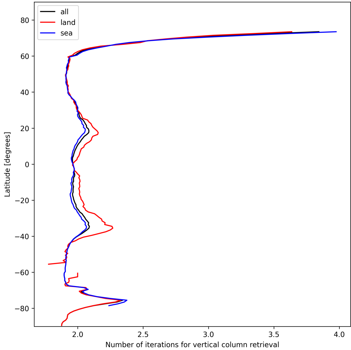
Figure 27: Zonal average of “Number of iterations for vertical column retrieval” for 2025-02-06 to 2025-02-06.
