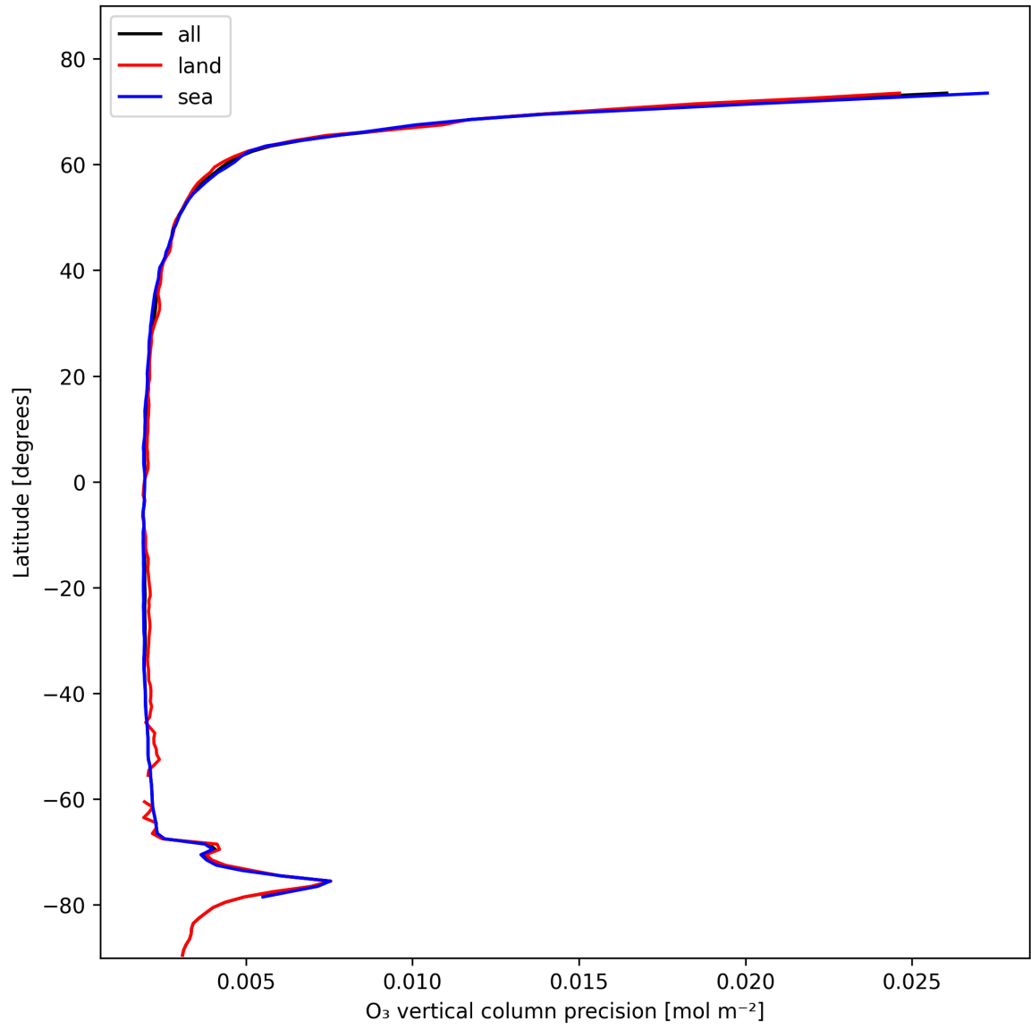
Figure 18: Zonal average of “O 3 vertical column precision” for 2025-02-06 to 2025-02-06.
