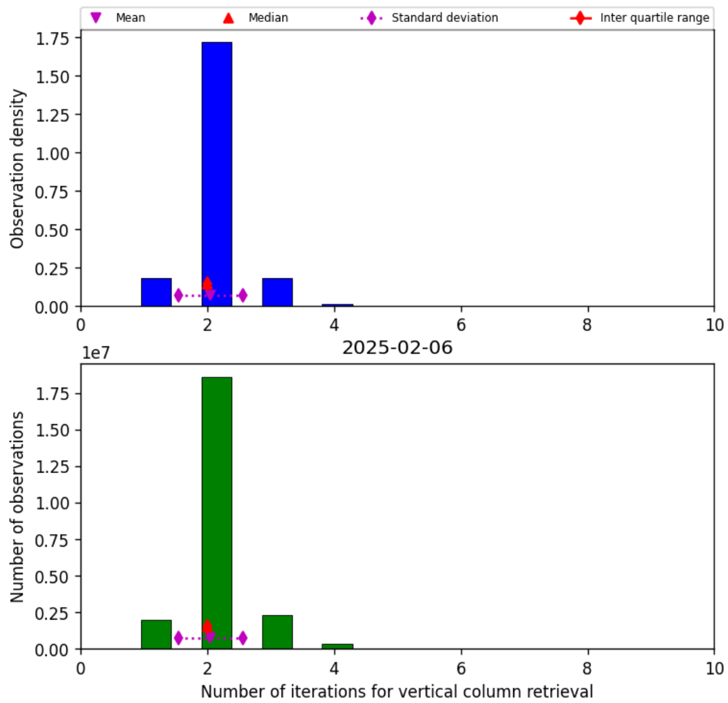
Figure 39: Histogram of “Number of iterations for vertical column retrieval” for 2025-02-06 to 2025-02-06
