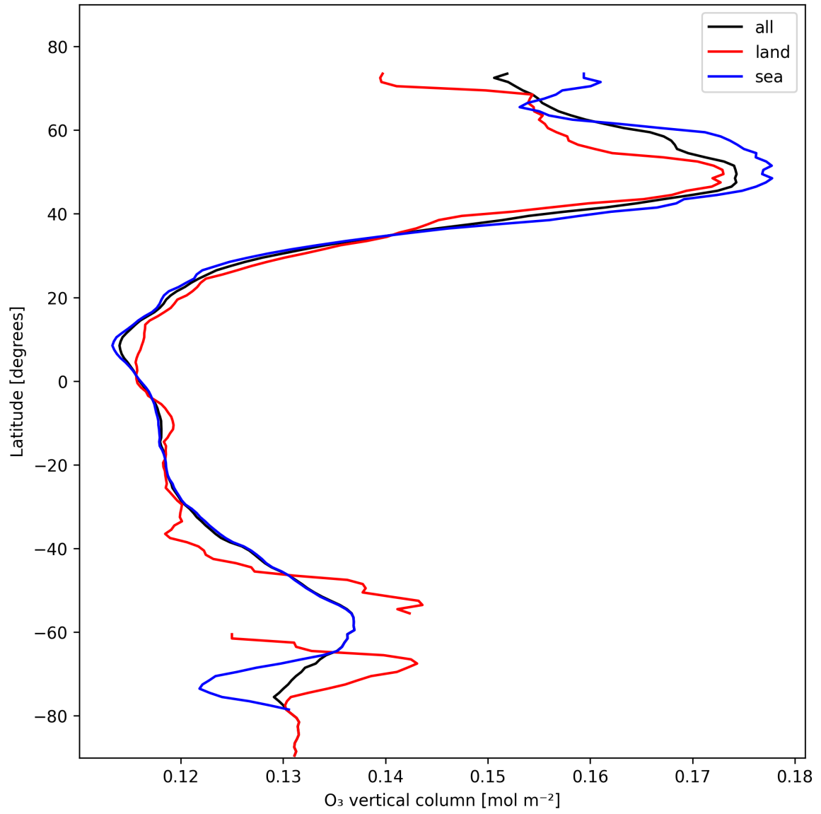
Figure 17: Zonal average of “O 3 vertical column” for 2025-02-06 to 2025-02-06.
