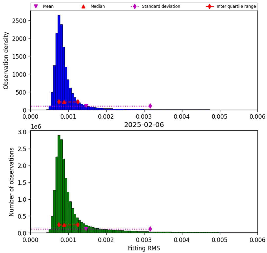
Figure 34: Histogram of “Fitting RMS” for 2025-02-06 to 2025-02-06
