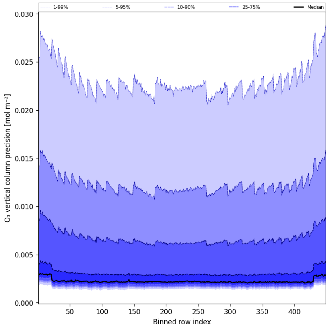
Figure 42: Along track statistics of “O 3 vertical column precision” for 2025-02-06 to 2025-02-06
