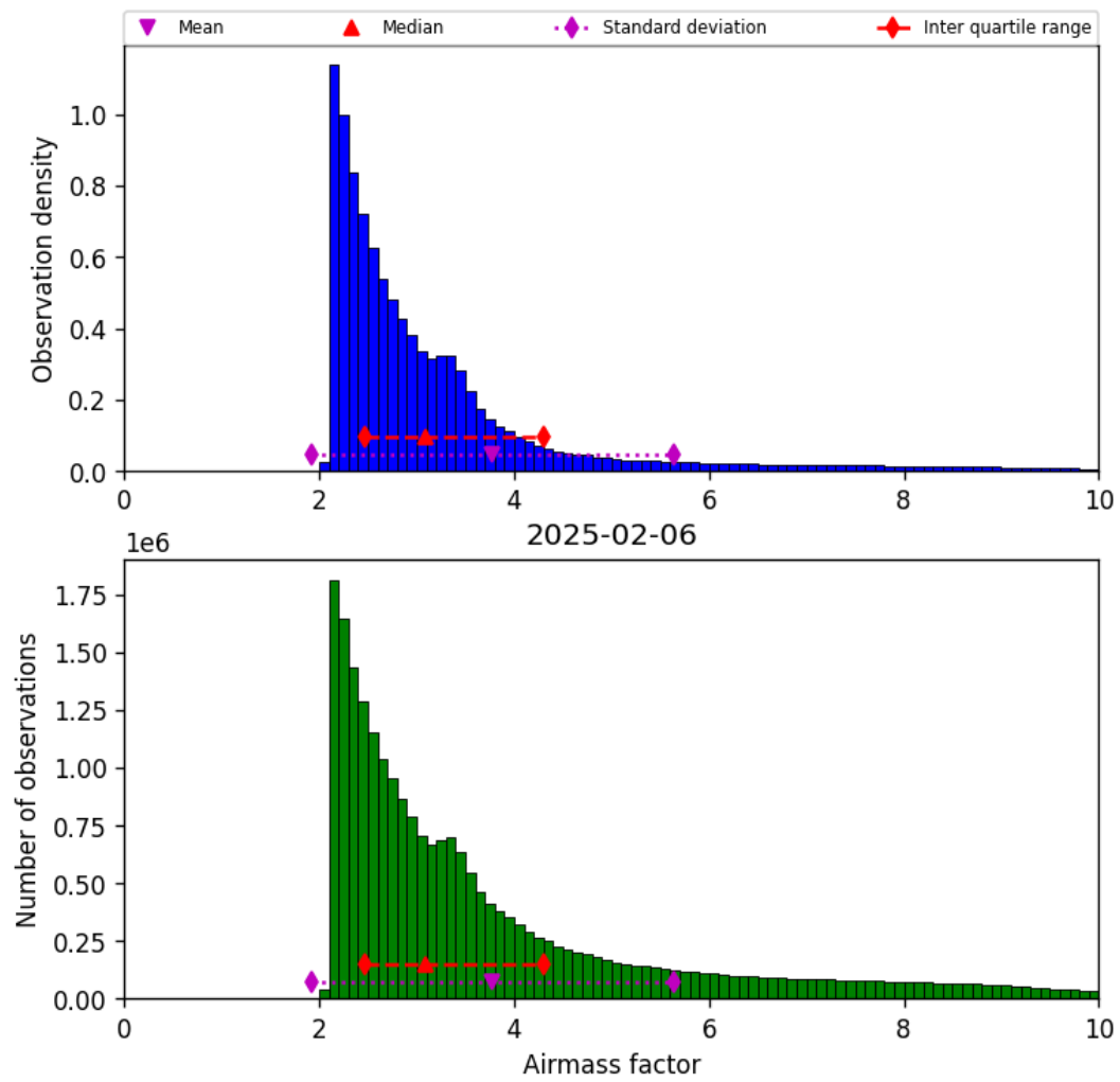
Figure 37: Histogram of “Airmass factor” for 2025-02-06 to 2025-02-06
