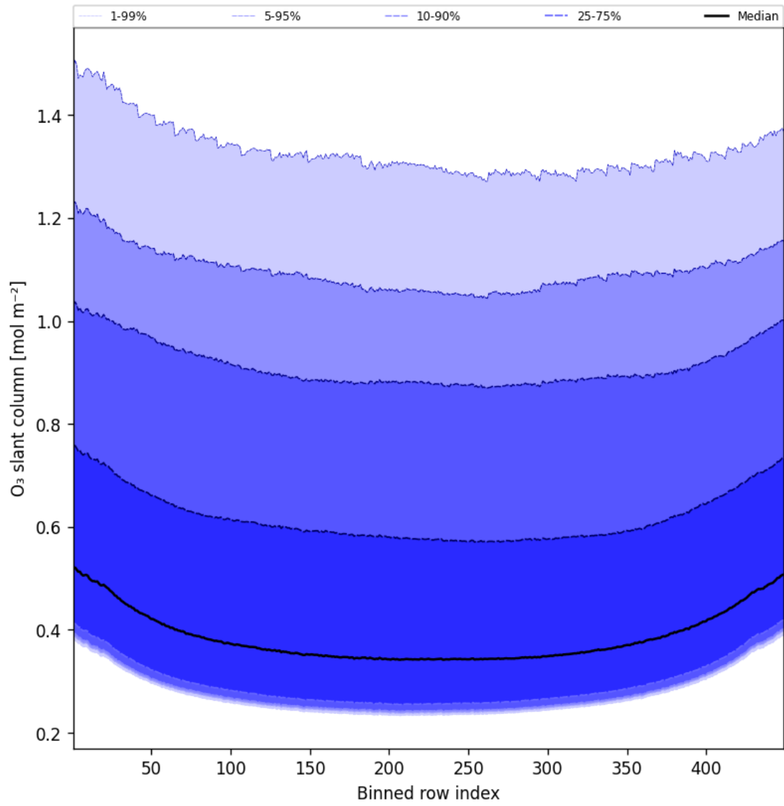
Figure 43: Along track statistics of “O 3 slant column” for 2025-02-06 to 2025-02-06
